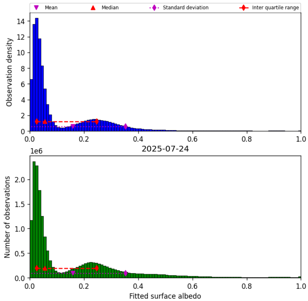
Figure 43: Histogram of “Fitted surface albedo” for 2025-07-24 to 2025-07-25
