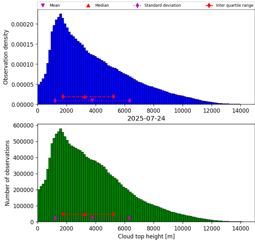
Figure 38: Histogram of “Cloud top height” for 2025-07-24 to 2025-07-25
