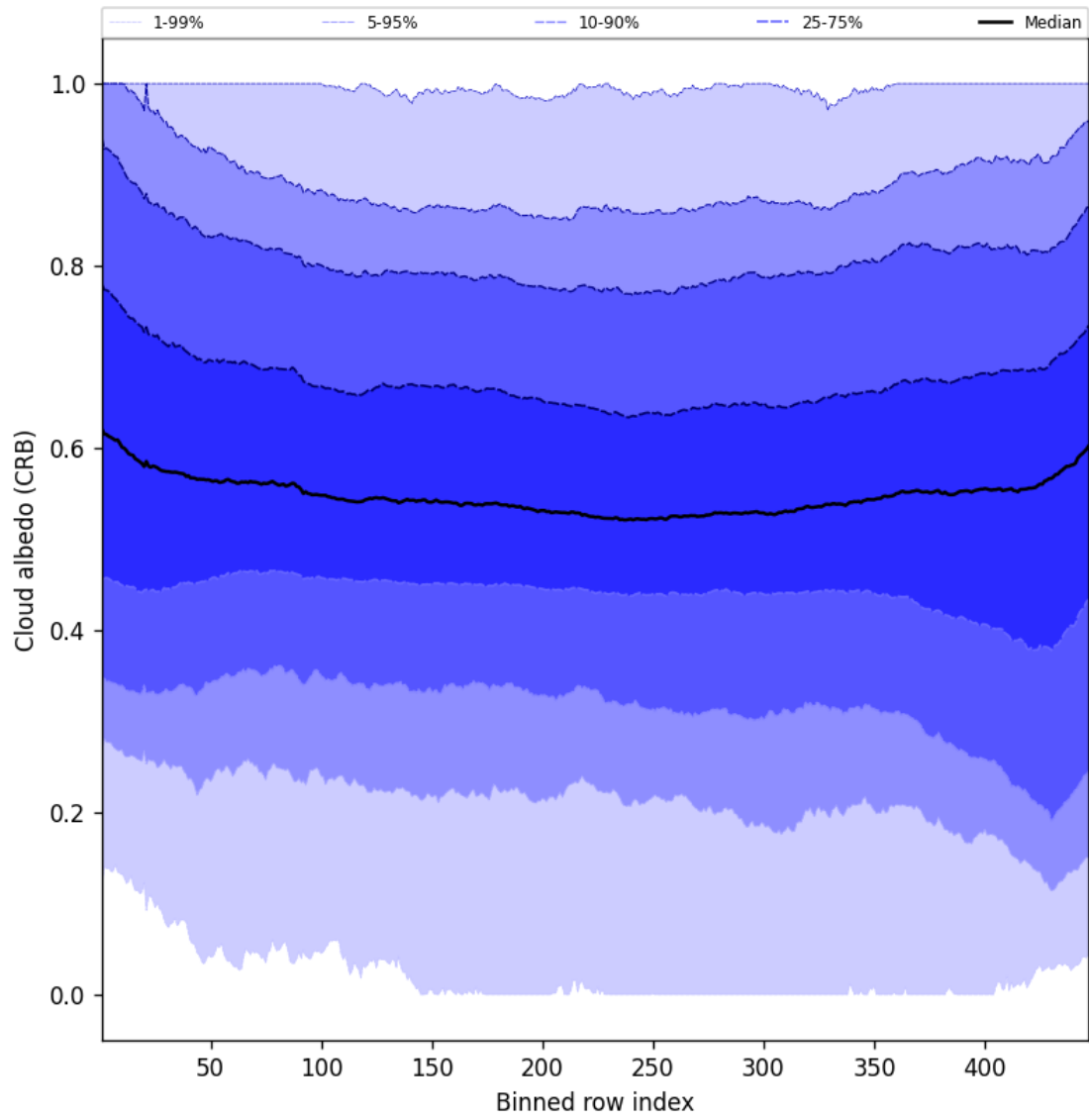
Figure 58: Along track statistics of “Cloud albedo (CRB)” for 2025-07-24 to 2025-07-25
