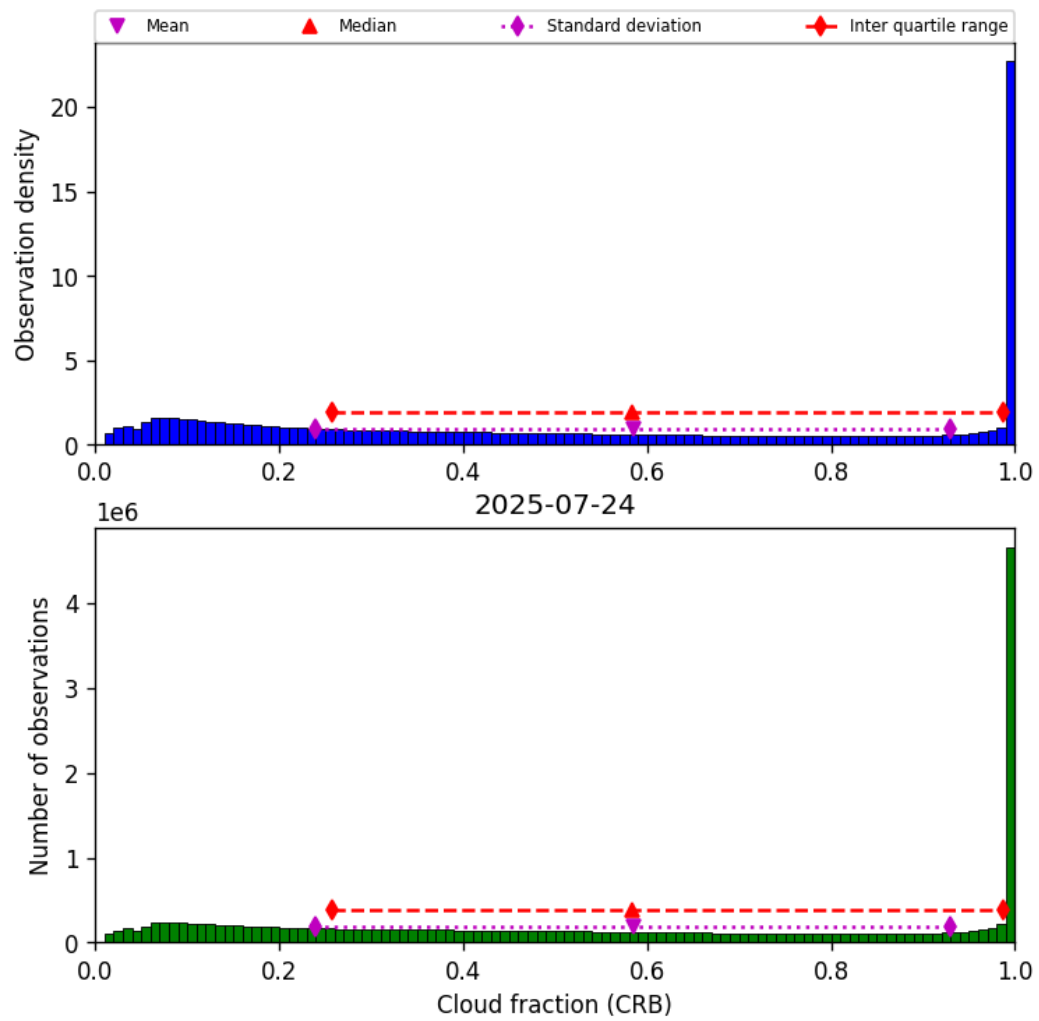
Figure 40: Histogram of “Cloud fraction (CRB)” for 2025-07-24 to 2025-07-25
