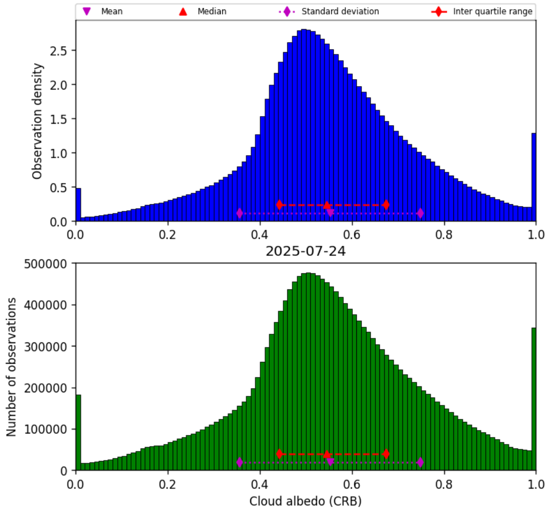
Figure 42: Histogram of “Cloud albedo (CRB)” for 2025-07-24 to 2025-07-25
