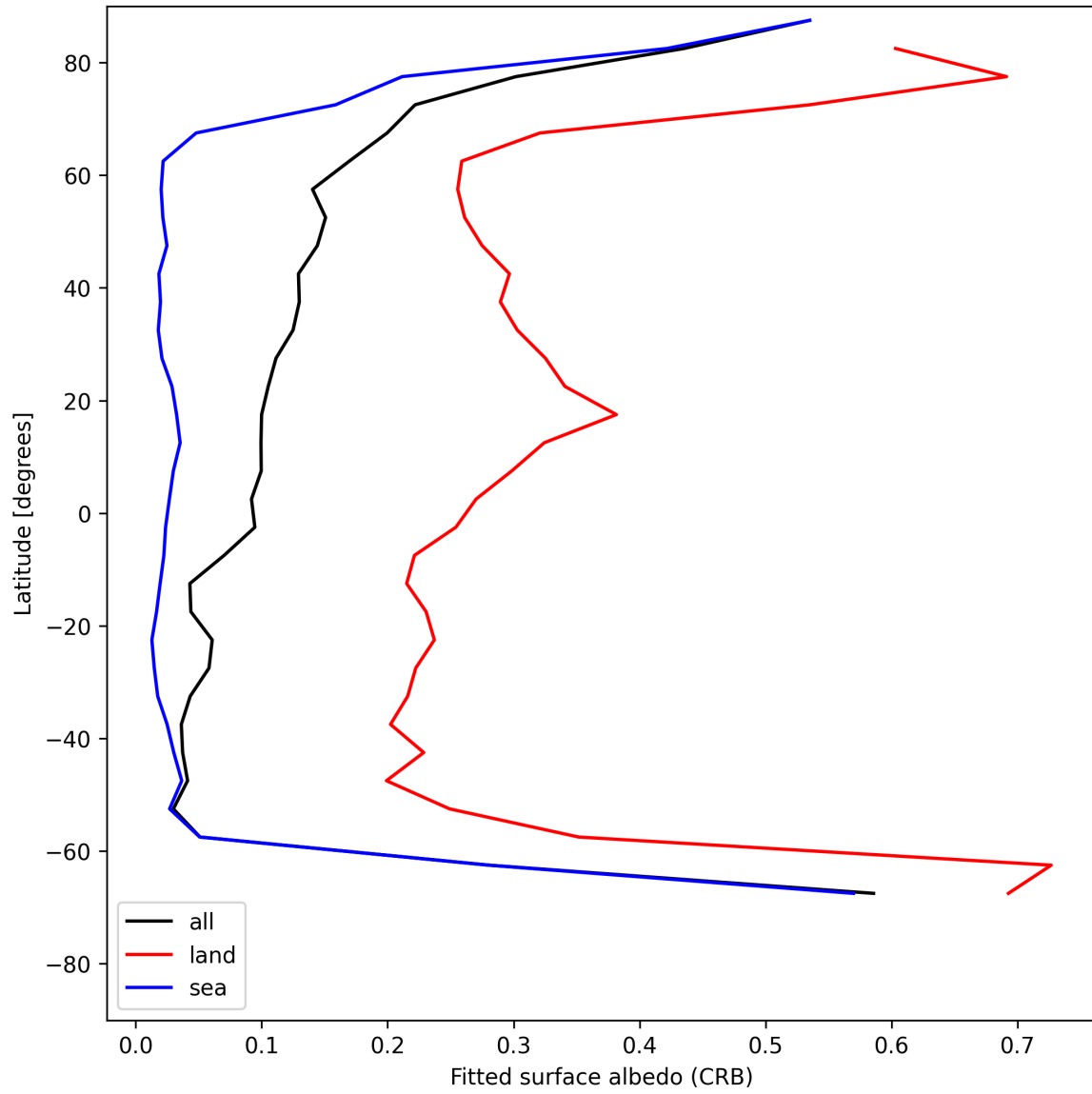
Figure 28: Zonal average of “Fitted surface albedo (CRB)” for 2025-07-24 to 2025-07-25.
