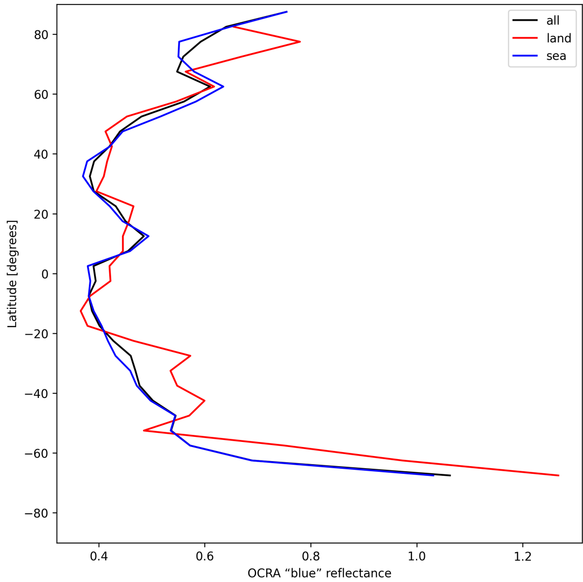
Figure 33: Zonal average of “OCRA “blue” reflectance” for 2025-07-24 to 2025-07-25.
