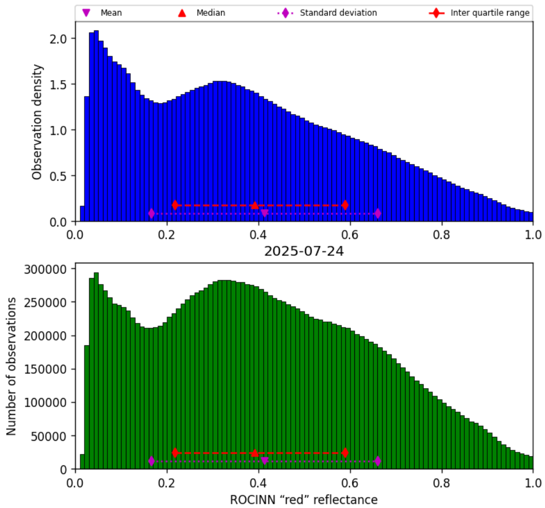
Figure 51: Histogram of “ROCINN “red” reflectance” for 2025-07-24 to 2025-07-25
