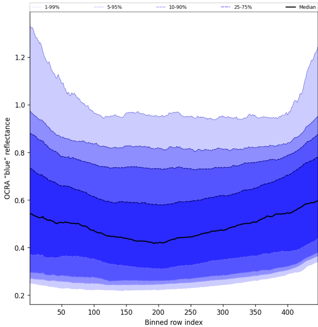
Figure 65: Along track statistics of “OCRA “blue” reflectance” for 2025-07-24 to 2025-07-25
