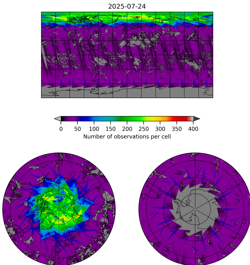
Figure 19: Map of the number of observations for 2025-07-24 to 2025-07-25
