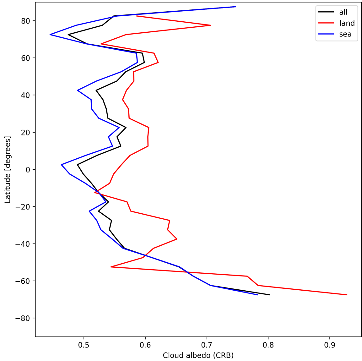
Figure 26: Zonal average of “Cloud albedo (CRB)” for 2025-07-24 to 2025-07-25.
