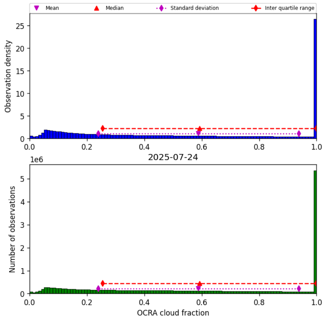
Figure 48: Histogram of “OCRA cloud fraction” for 2025-07-24 to 2025-07-25
