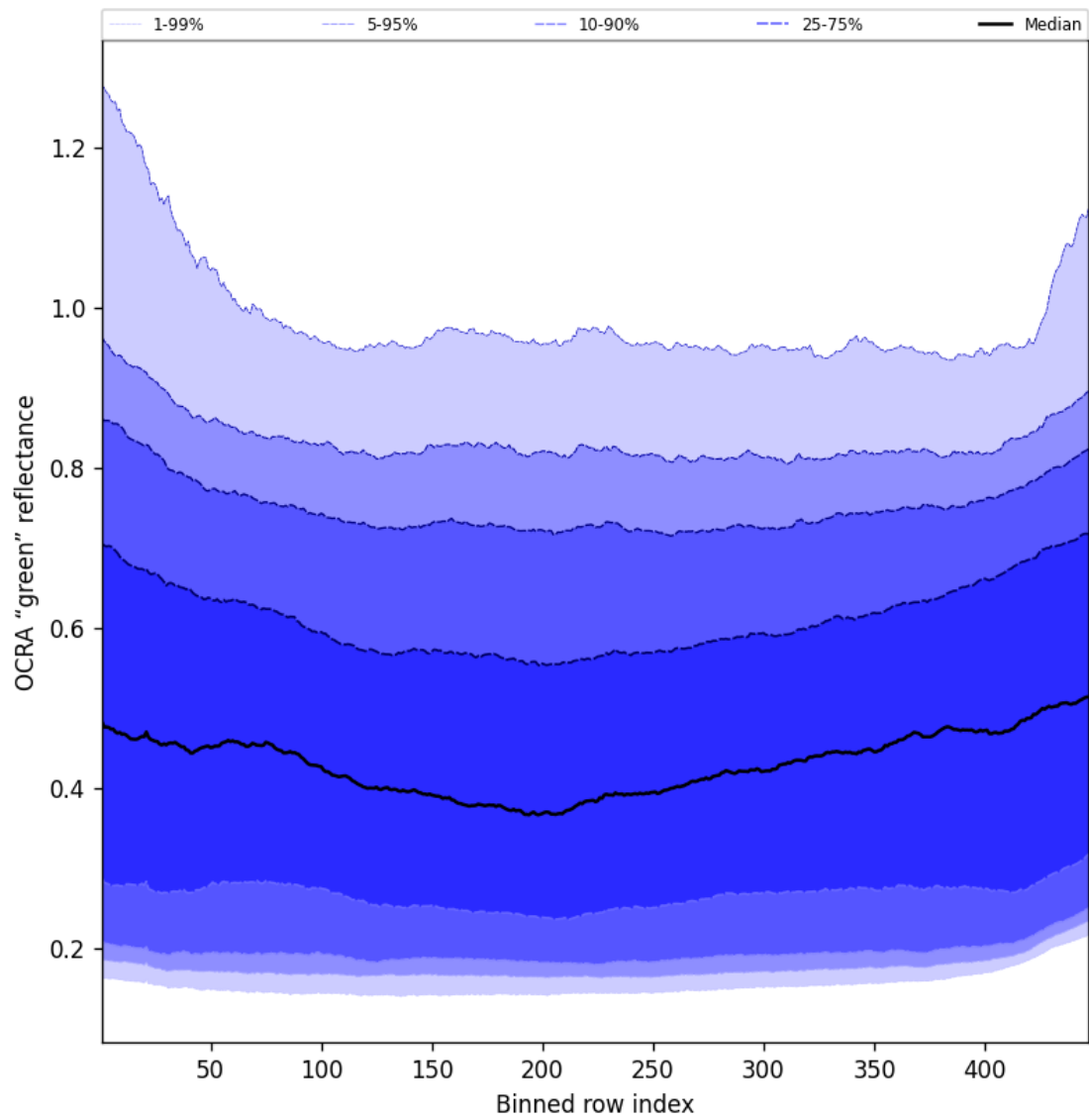
Figure 66: Along track statistics of “OCRA “green” reflectance” for 2025-07-24 to 2025-07-25
