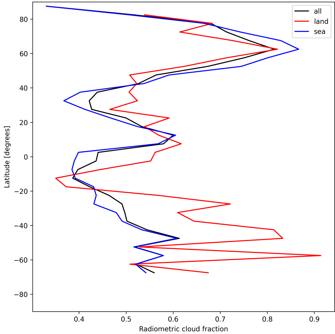
Figure 21: Zonal average of “Radiometric cloud fraction” for 2025-07-24 to 2025-07-25.
