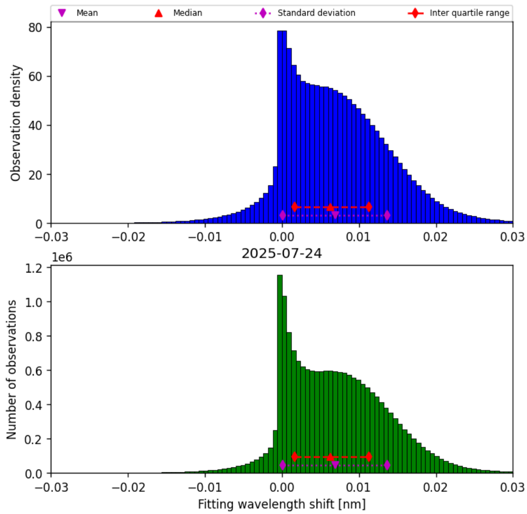
Figure 47: Histogram of “Fitting wavelength shift” for 2025-07-24 to 2025-07-25
