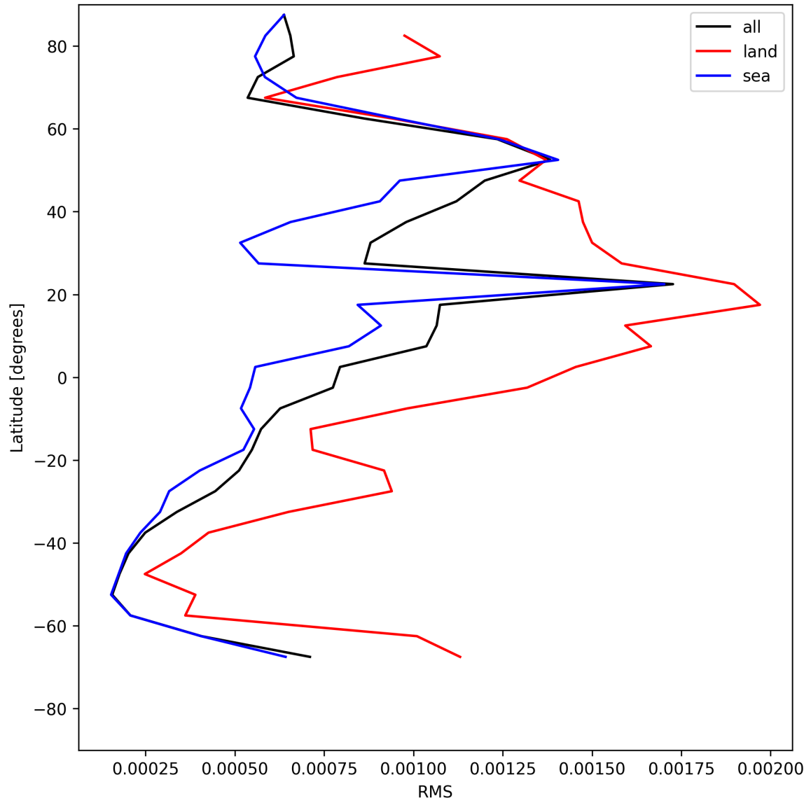
Figure 29: Zonal average of “RMS” for 2025-07-24 to 2025-07-25.
