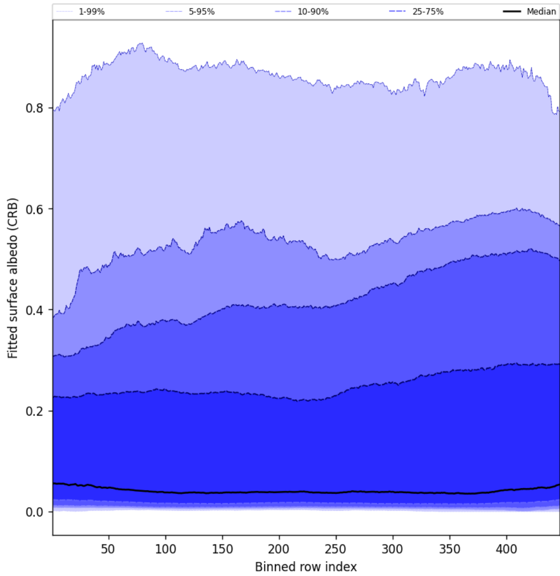
Figure 60: Along track statistics of “Fitted surface albedo (CRB)” for 2025-07-24 to 2025-07-25
