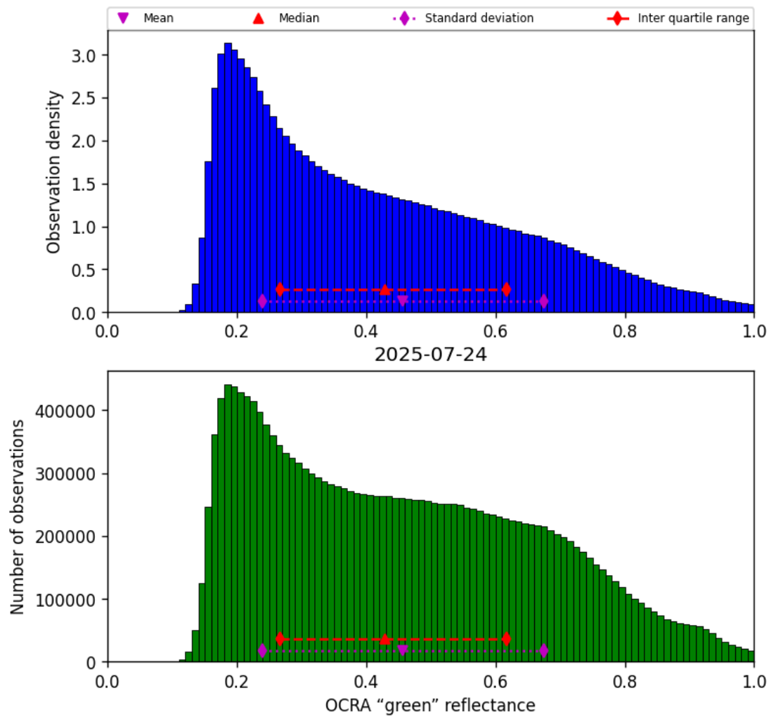
Figure 50: Histogram of “OCRA “green” reflectance” for 2025-07-24 to 2025-07-25
