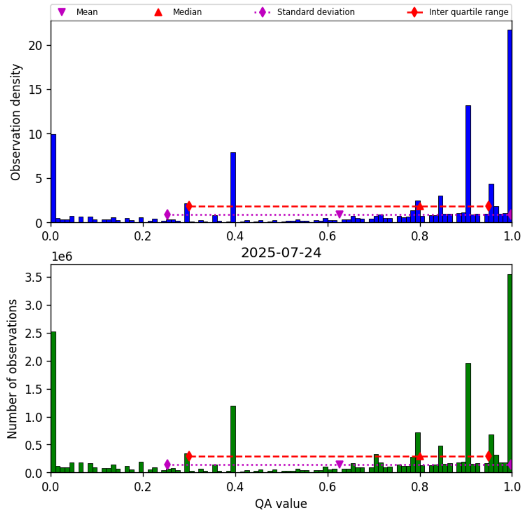
Figure 36: Histogram of “QA value” for 2025-07-24 to 2025-07-25
