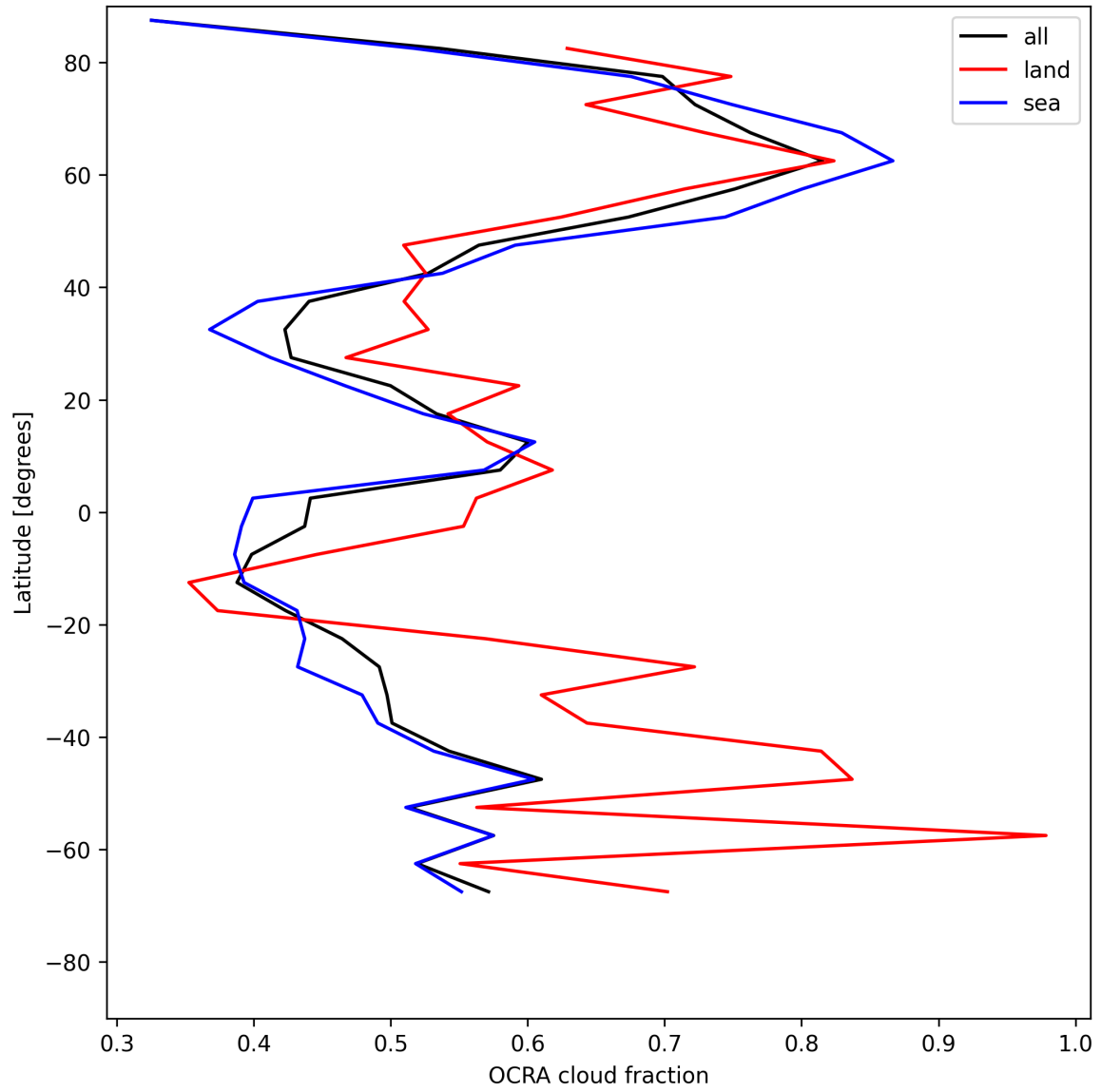
Figure 32: Zonal average of “OCRA cloud fraction” for 2025-07-24 to 2025-07-25.
