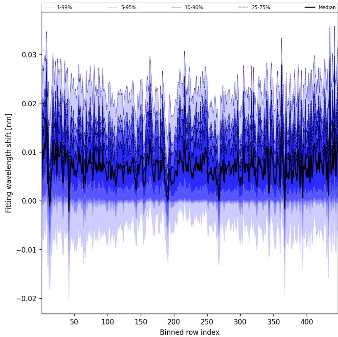
Figure 63: Along track statistics of “Fitting wavelength shift” for 2025-07-24 to 2025-07-25
