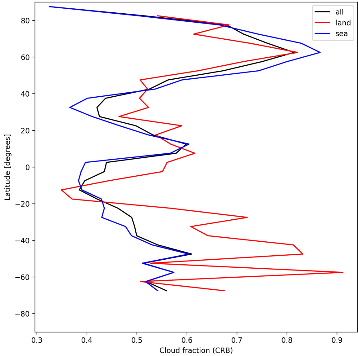
Figure 24: Zonal average of “Cloud fraction (CRB)” for 2025-07-24 to 2025-07-25.
