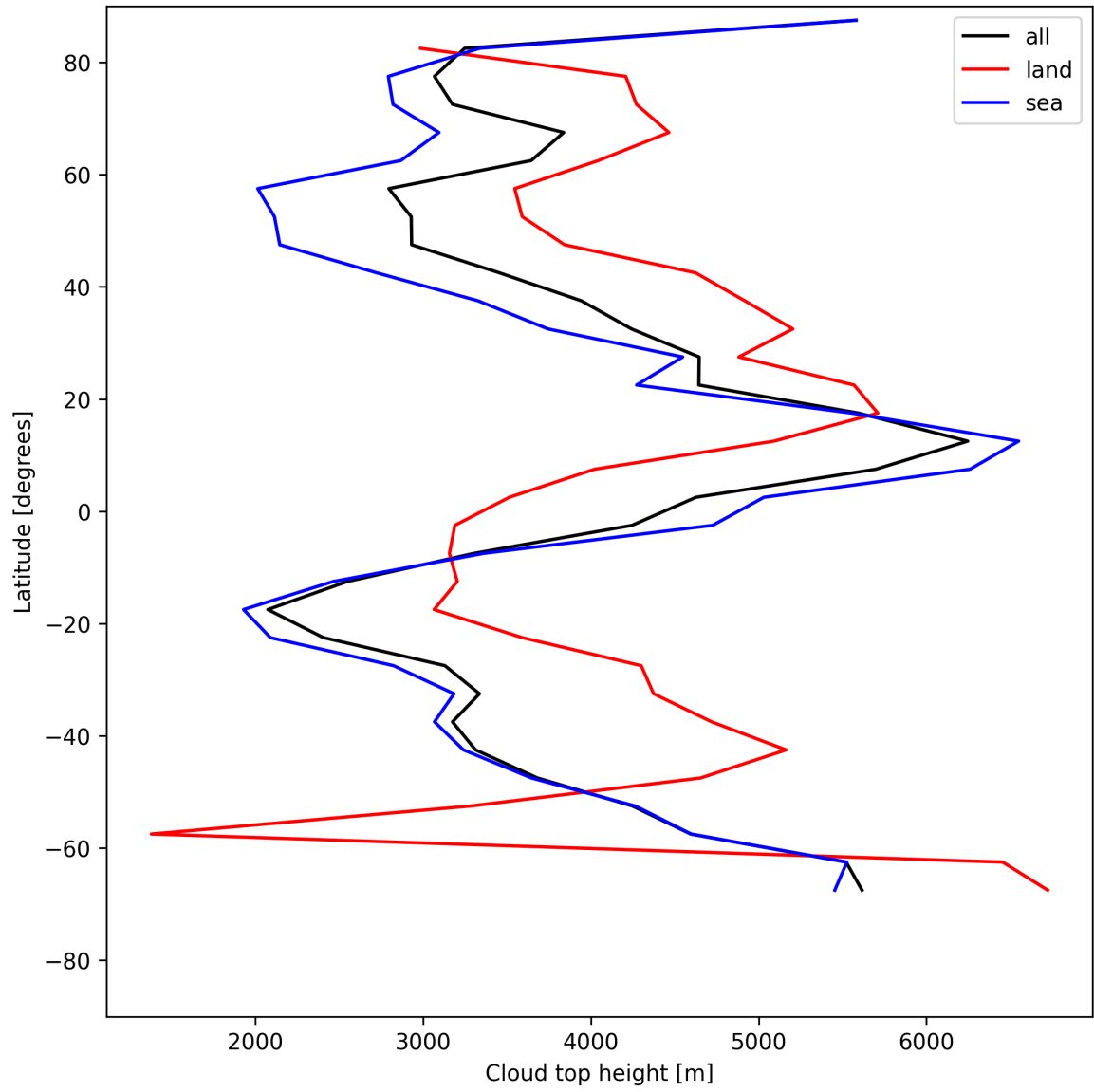
Figure 22: Zonal average of “Cloud top height” for 2025-07-24 to 2025-07-25.
