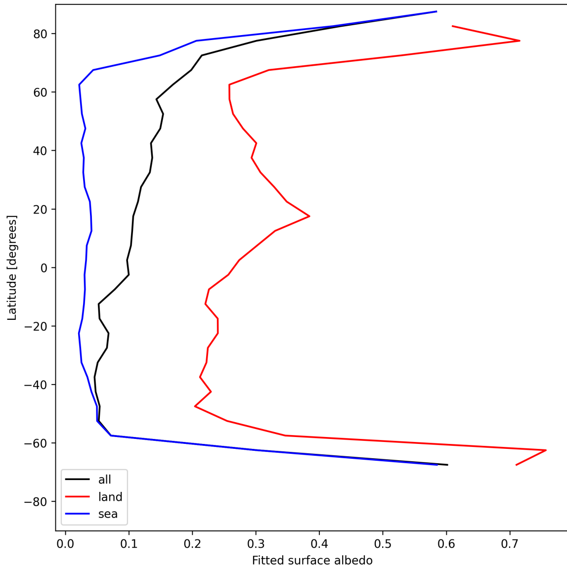
Figure 27: Zonal average of “Fitted surface albedo” for 2025-07-24 to 2025-07-25.
