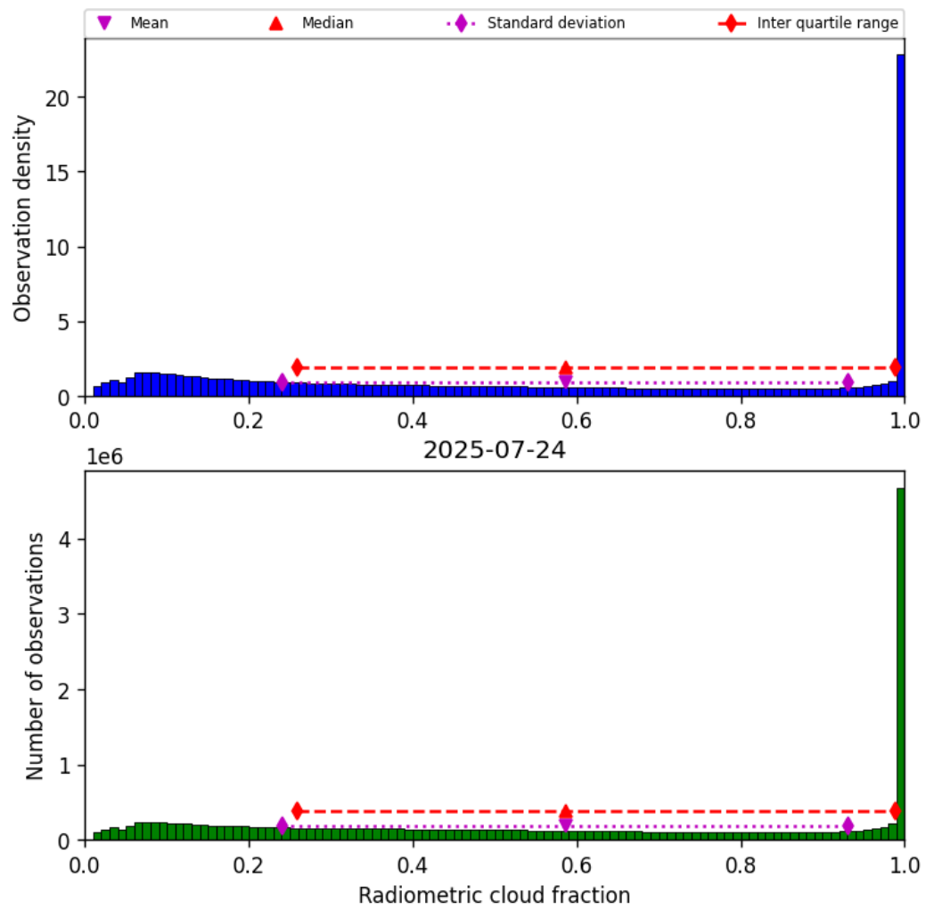
Figure 37: Histogram of “Radiometric cloud fraction” for 2025-07-24 to 2025-07-25
