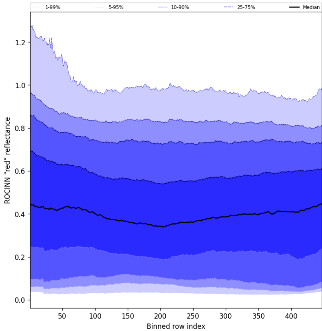
Figure 67: Along track statistics of "ROCINN "red" reflectance" for 2025-07-24 to 2025-07-25
