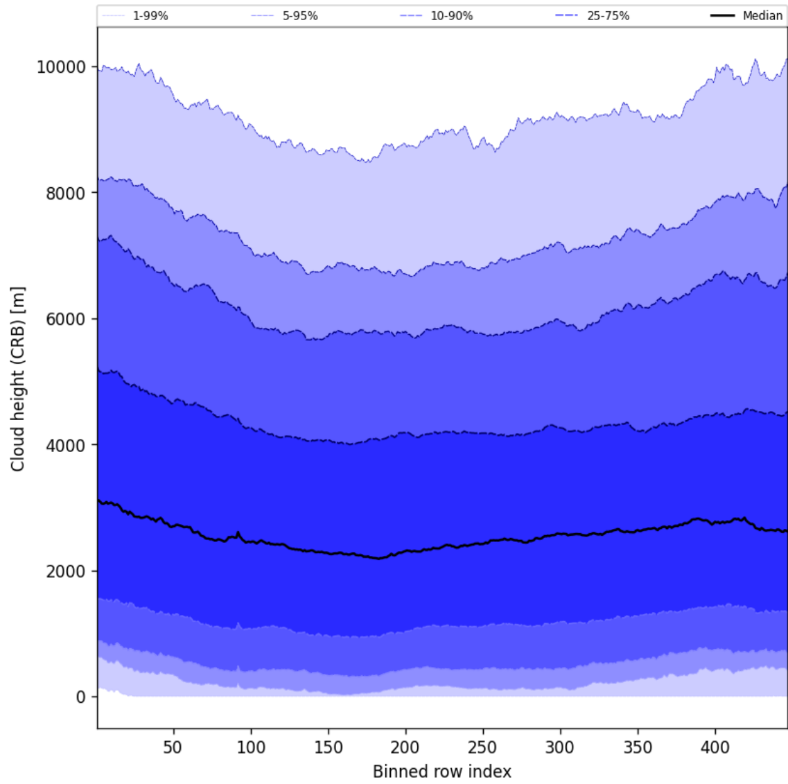
Figure 57: Along track statistics of “Cloud height (CRB)” for 2025-07-24 to 2025-07-25
