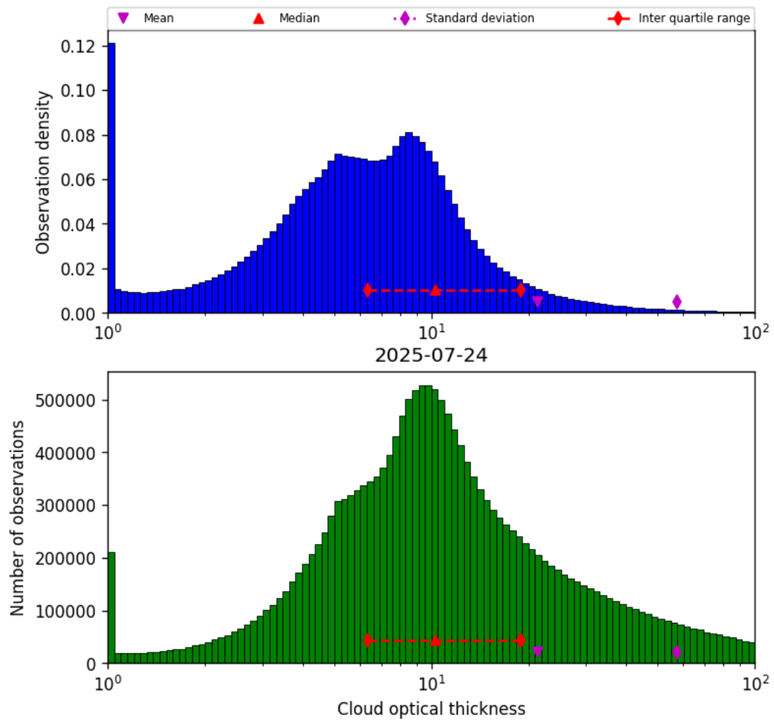
Figure 39: Histogram of “Cloud optical thickness” for 2025-07-24 to 2025-07-25
