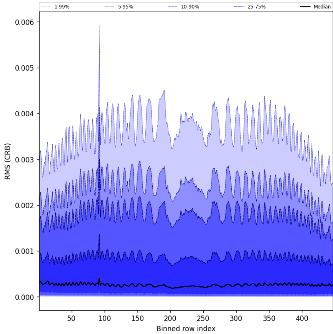
Figure 62: Along track statistics of “RMS (CRB)” for 2025-07-24 to 2025-07-25
