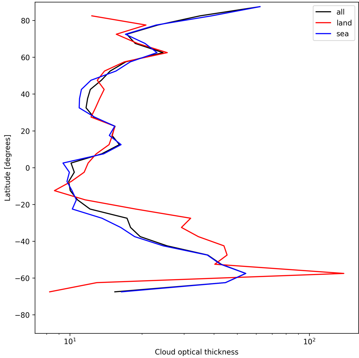
Figure 23: Zonal average of “Cloud optical thickness” for 2025-07-24 to 2025-07-25.
