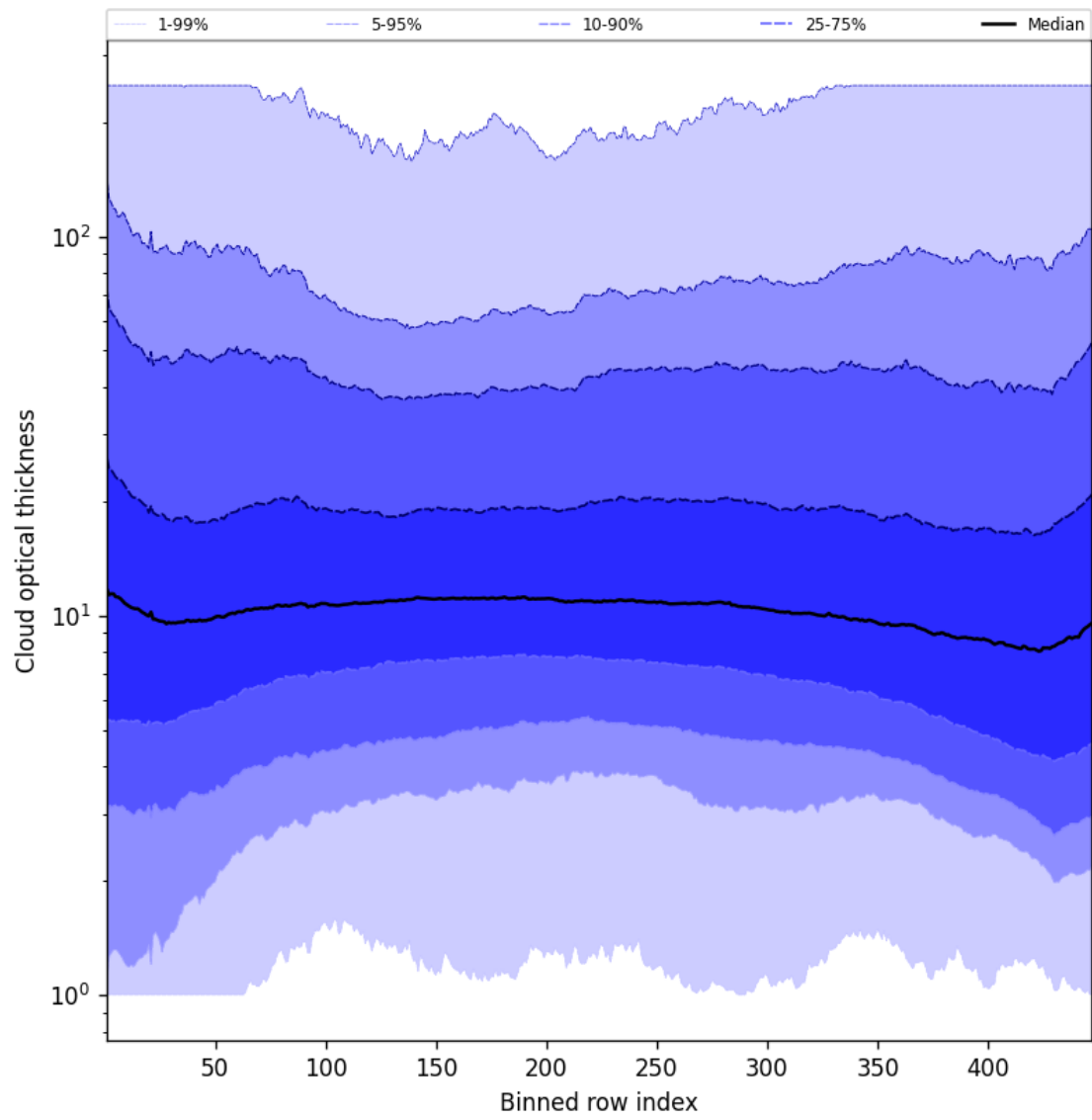
Figure 55: Along track statistics of “Cloud optical thickness” for 2025-07-24 to 2025-07-25
