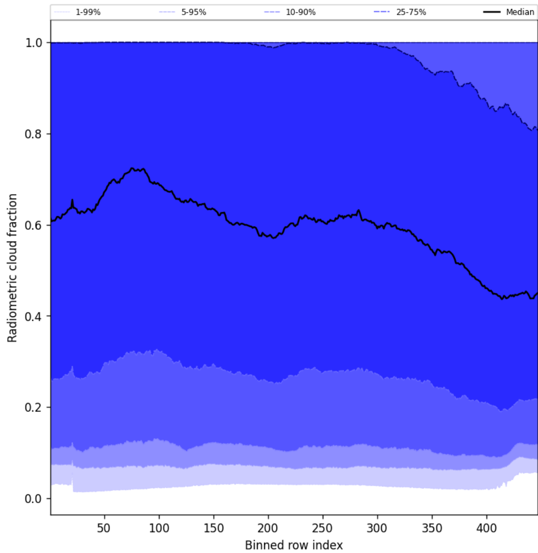
Figure 53: Along track statistics of “Radiometric cloud fraction” for 2025-07-24 to 2025-07-25
