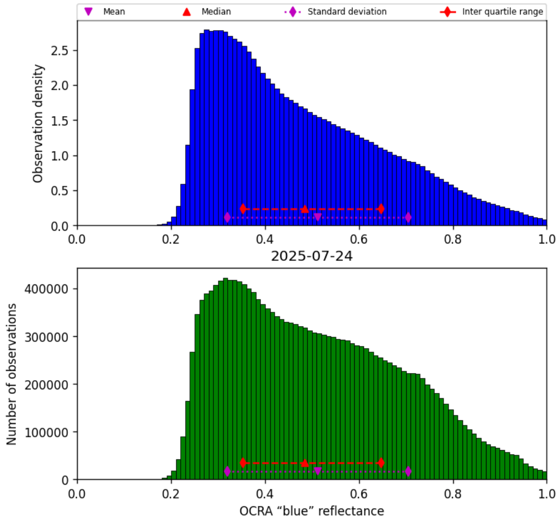
Figure 49: Histogram of “OCRA “blue” reflectance” for 2025-07-24 to 2025-07-25
