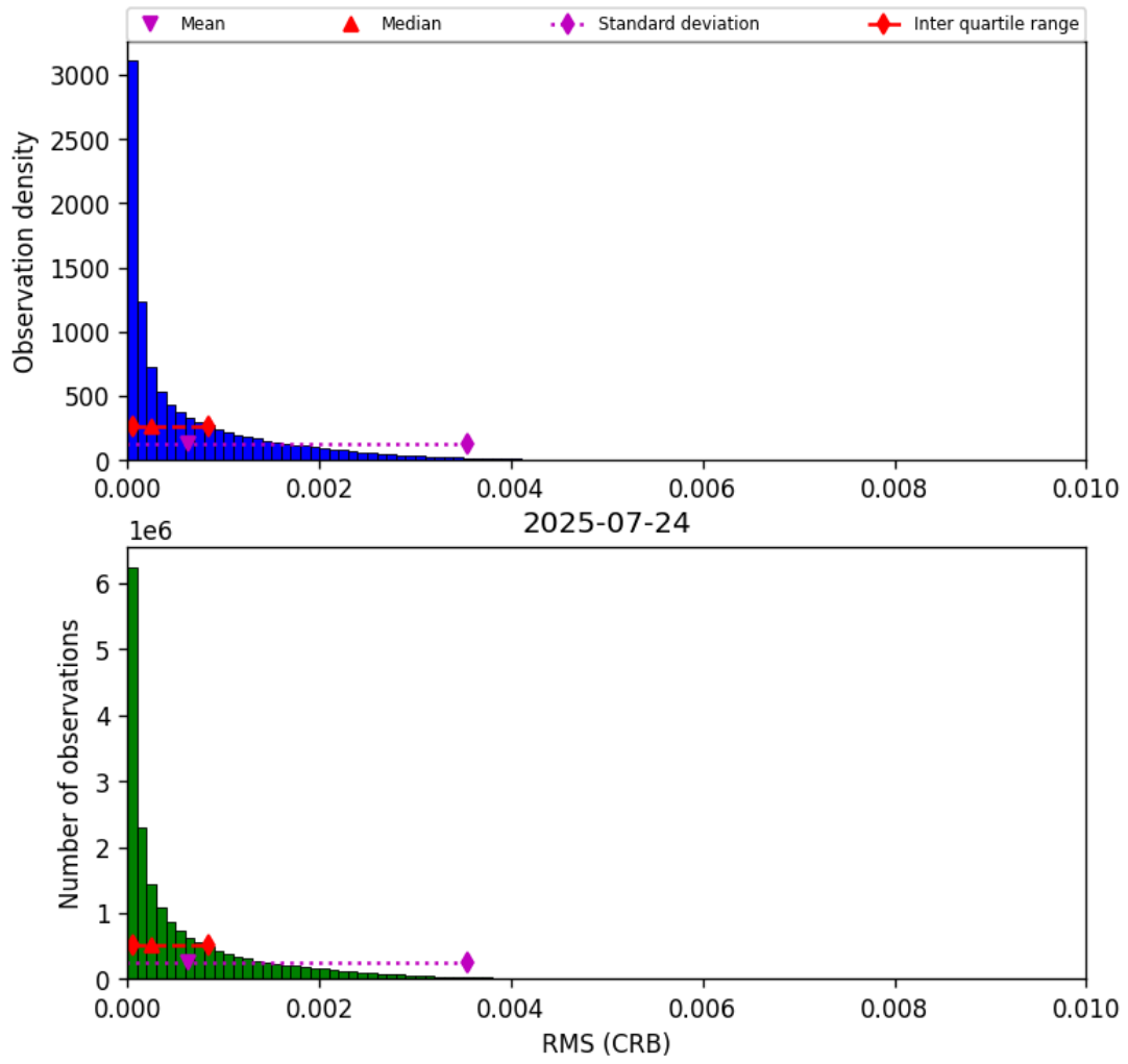
Figure 46: Histogram of “RMS (CRB)” for 2025-07-24 to 2025-07-25
