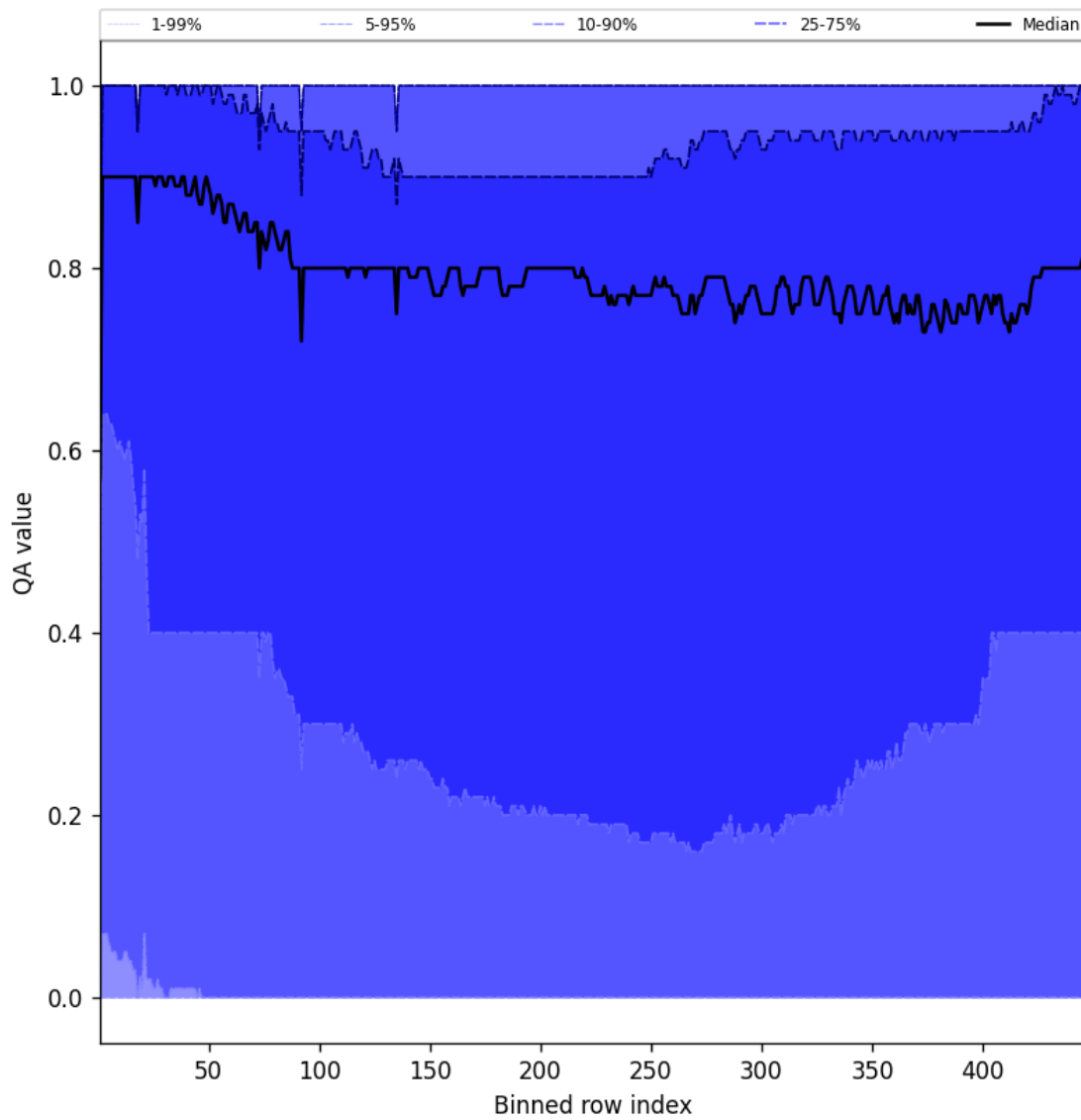
Figure 52: Along track statistics of “QA value” for 2025-07-24 to 2025-07-25
