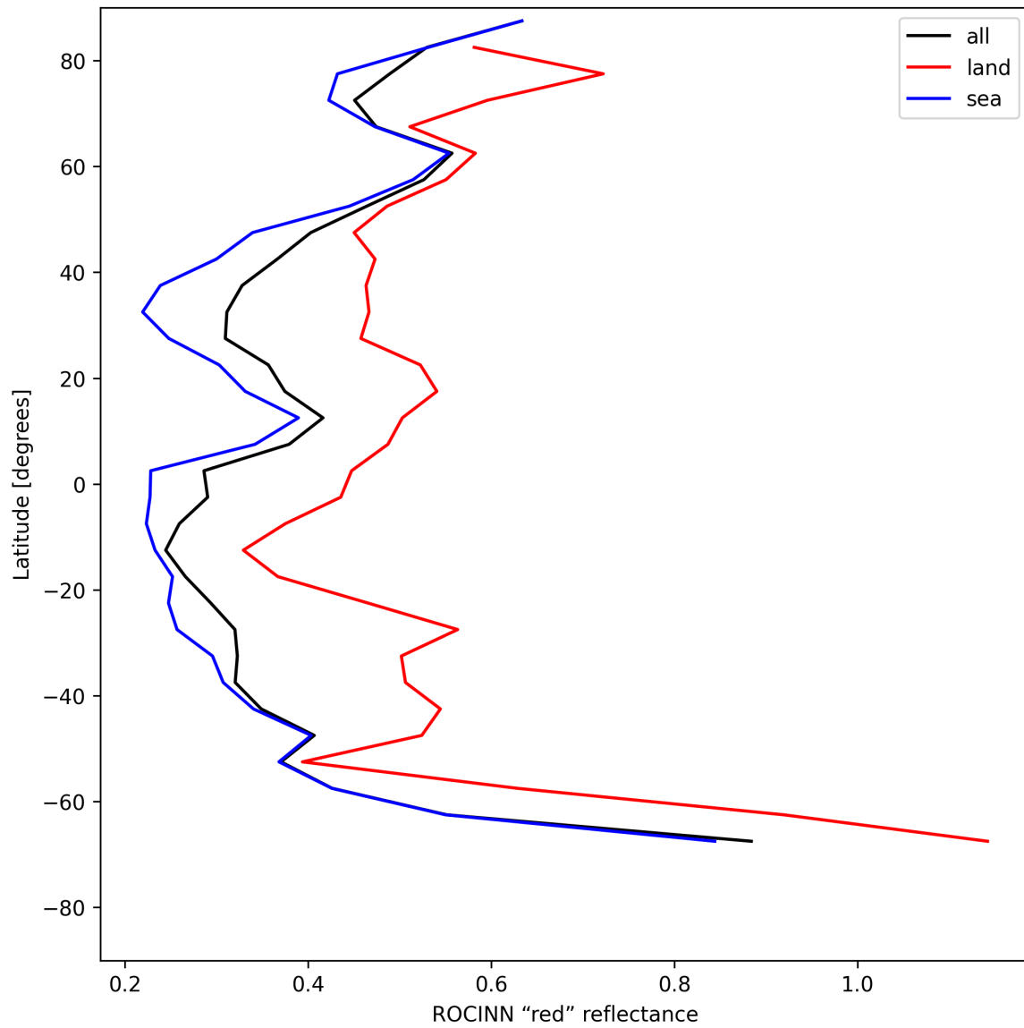
Figure 35: Zonal average of “ROCINN “red” reflectance” for 2025-07-24 to 2025-07-25.
