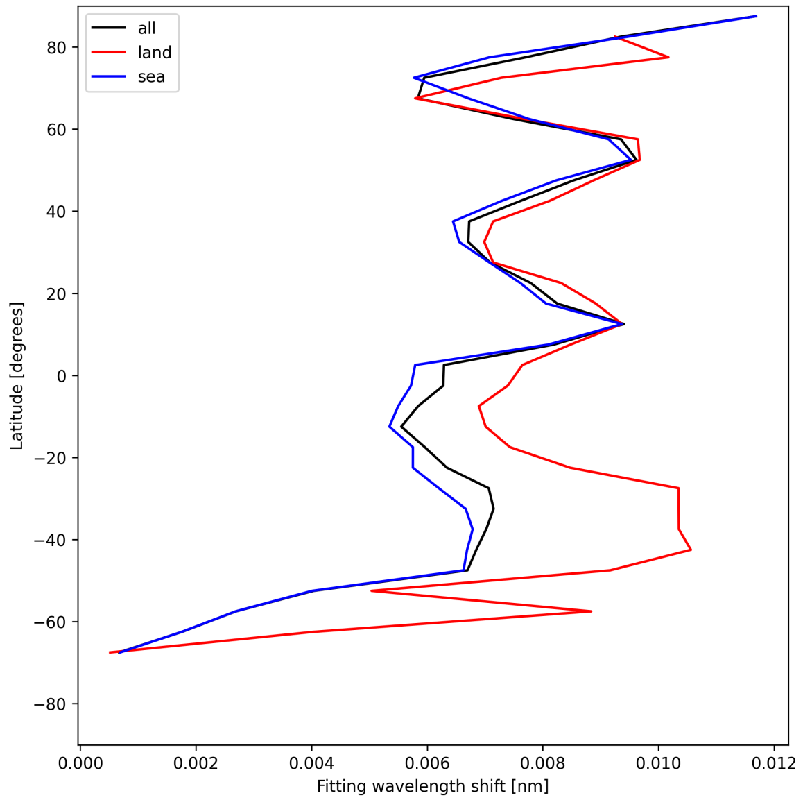
Figure 31: Zonal average of “Fitting wavelength shift” for 2025-07-24 to 2025-07-25.
