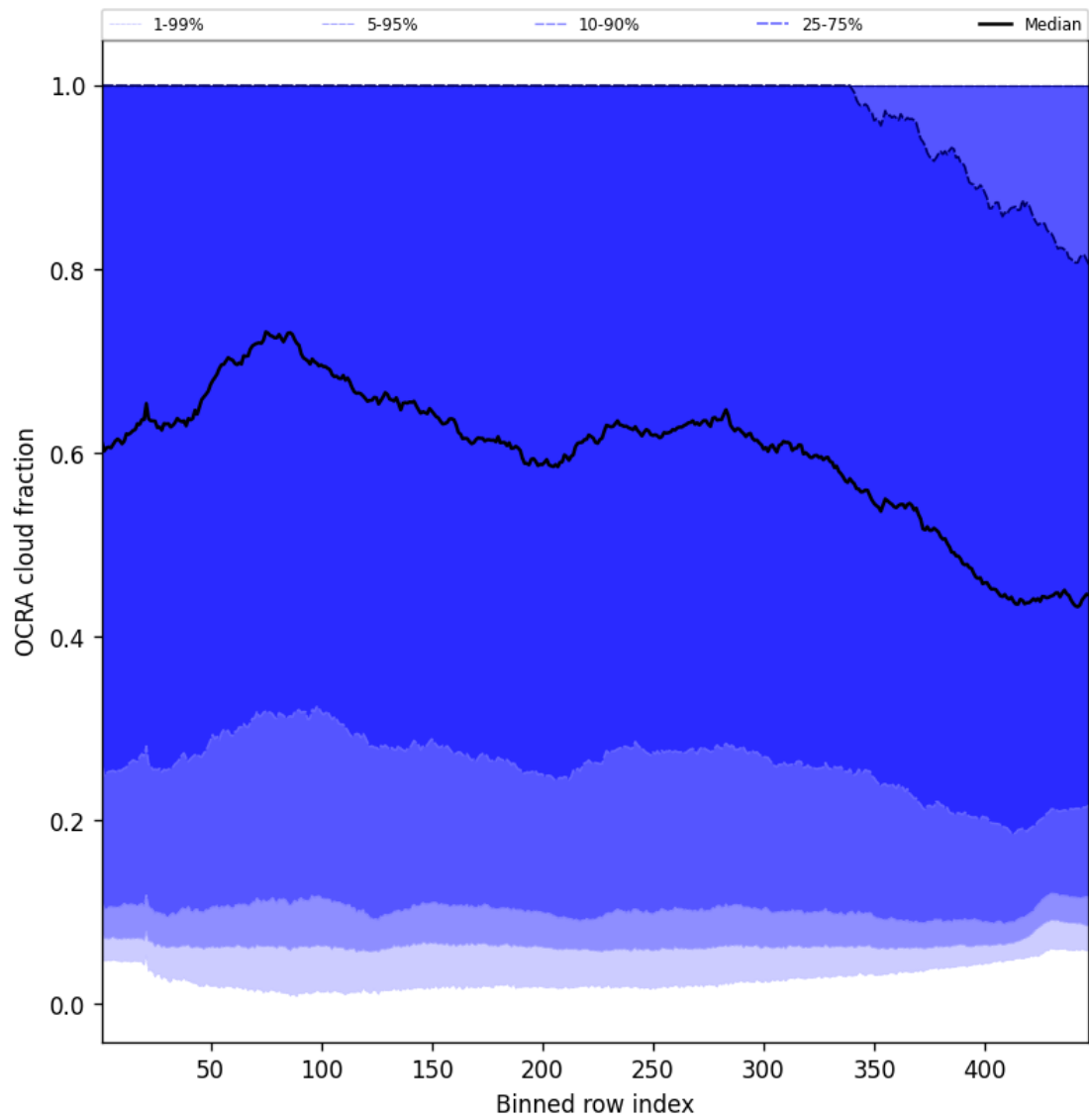
Figure 64: Along track statistics of “OCRA cloud fraction” for 2025-07-24 to 2025-07-25
