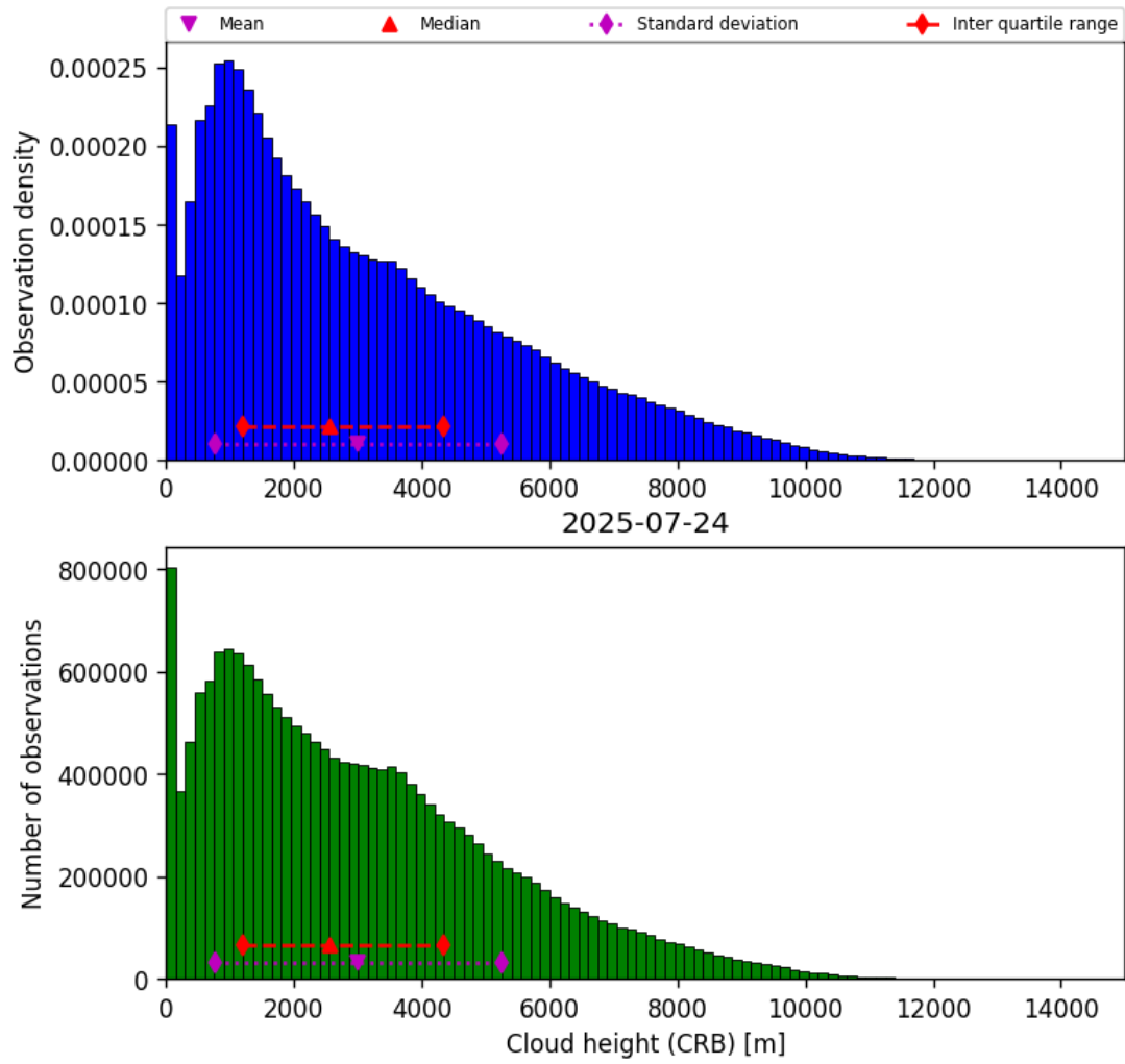
Figure 41: Histogram of “Cloud height (CRB)” for 2025-07-24 to 2025-07-25
