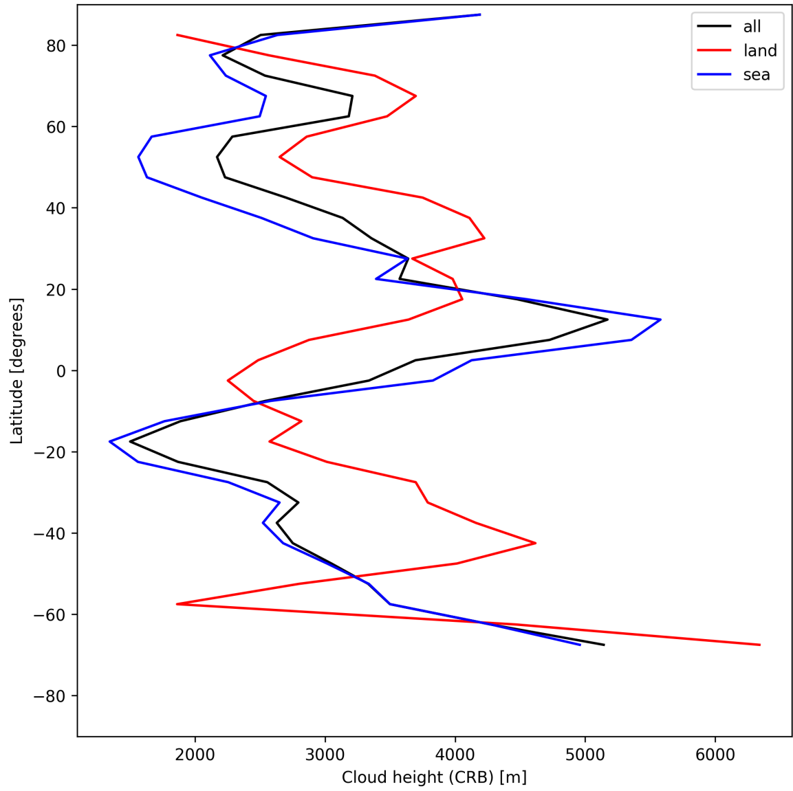
Figure 25: Zonal average of “Cloud height (CRB)” for 2025-07-24 to 2025-07-25.
