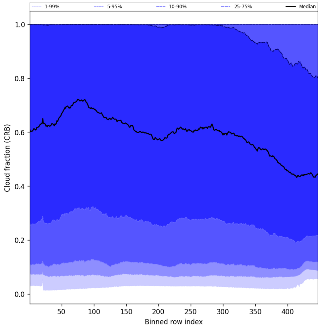
Figure 56: Along track statistics of “Cloud fraction (CRB)” for 2025-07-24 to 2025-07-25
