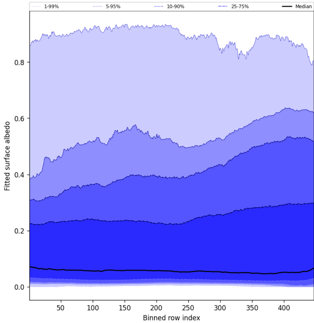
Figure 59: Along track statistics of “Fitted surface albedo” for 2025-07-24 to 2025-07-25
