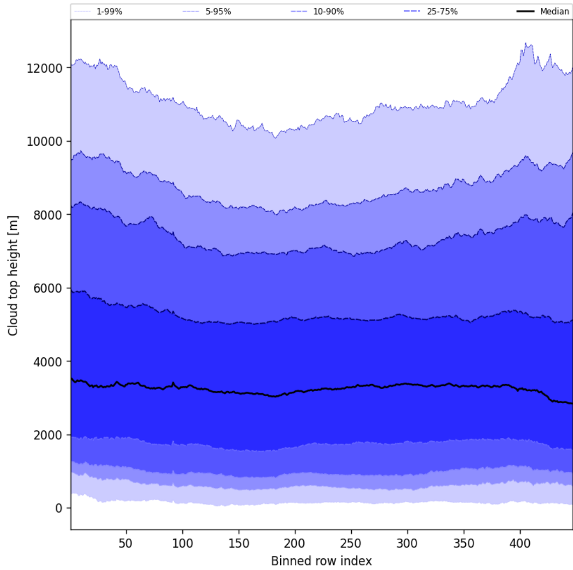
Figure 54: Along track statistics of “Cloud top height” for 2025-07-24 to 2025-07-25
