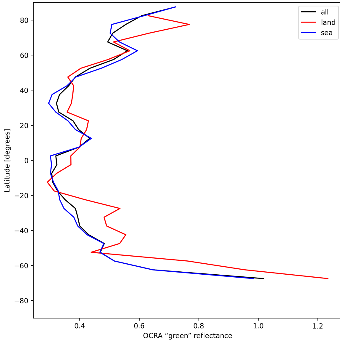
Figure 34: Zonal average of “OCRA “green” reflectance” for 2025-07-24 to 2025-07-25.
