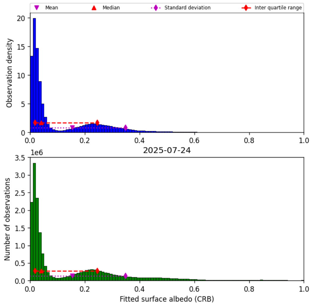
Figure 44: Histogram of “Fitted surface albedo (CRB)” for 2025-07-24 to 2025-07-25
