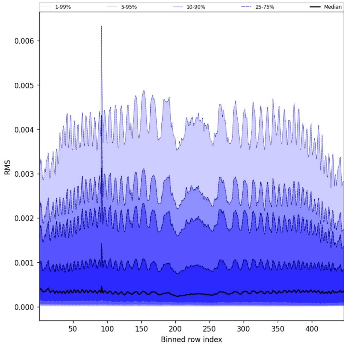
Figure 61: Along track statistics of “RMS” for 2025-07-24 to 2025-07-25
