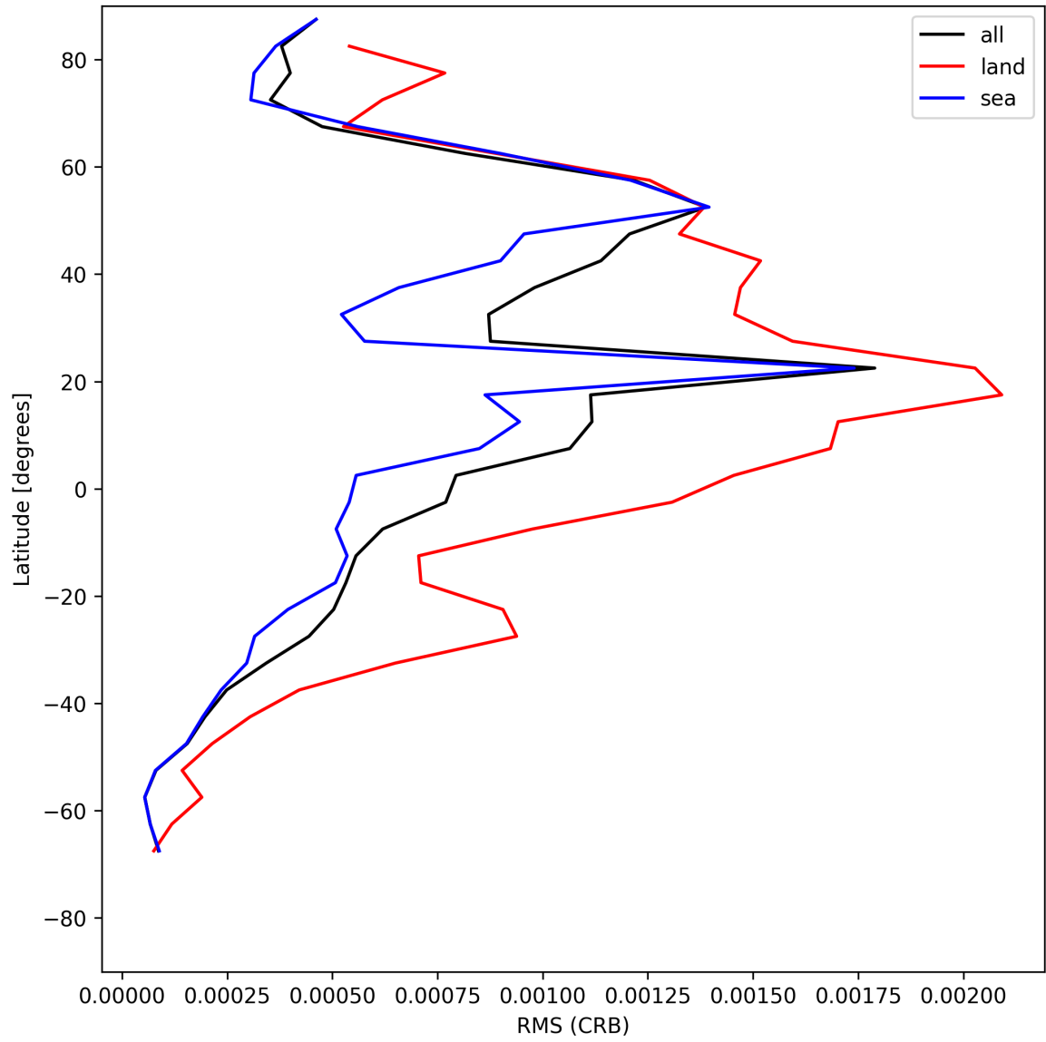
Figure 30: Zonal average of “RMS (CRB)” for 2025-07-24 to 2025-07-25.
