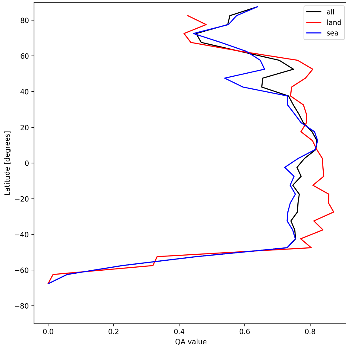
Figure 20: Zonal average of “QA value” for 2025-07-24 to 2025-07-25.
