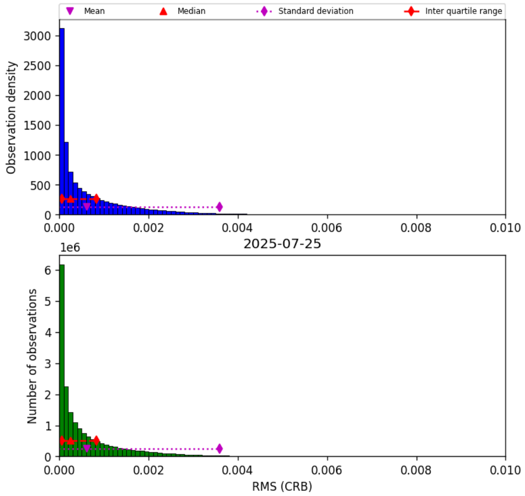
Figure 46: Histogram of “RMS (CRB)” for 2025-07-25 to 2025-07-26
