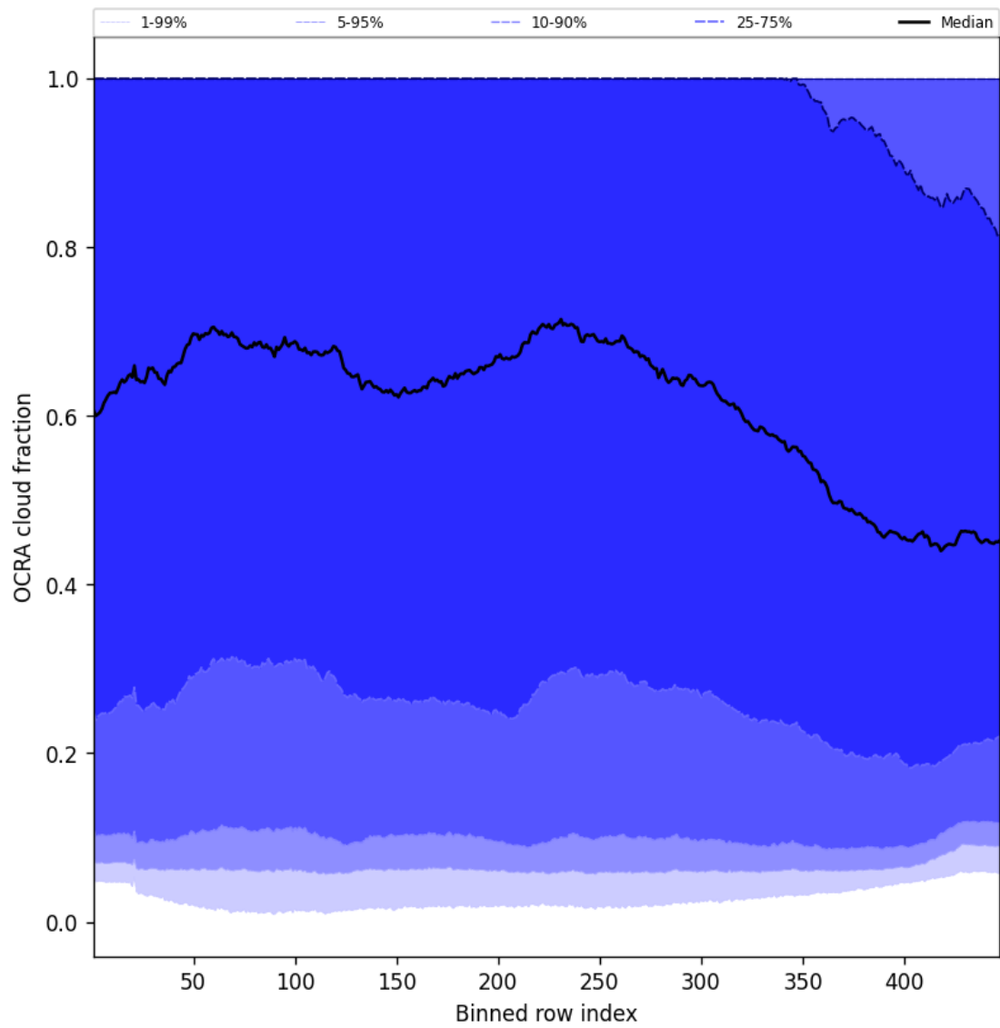
Figure 64: Along track statistics of “OCRA cloud fraction” for 2025-07-25 to 2025-07-26
