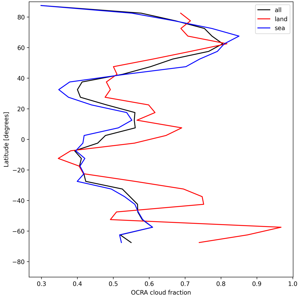
Figure 32: Zonal average of “OCRA cloud fraction” for 2025-07-25 to 2025-07-26.
