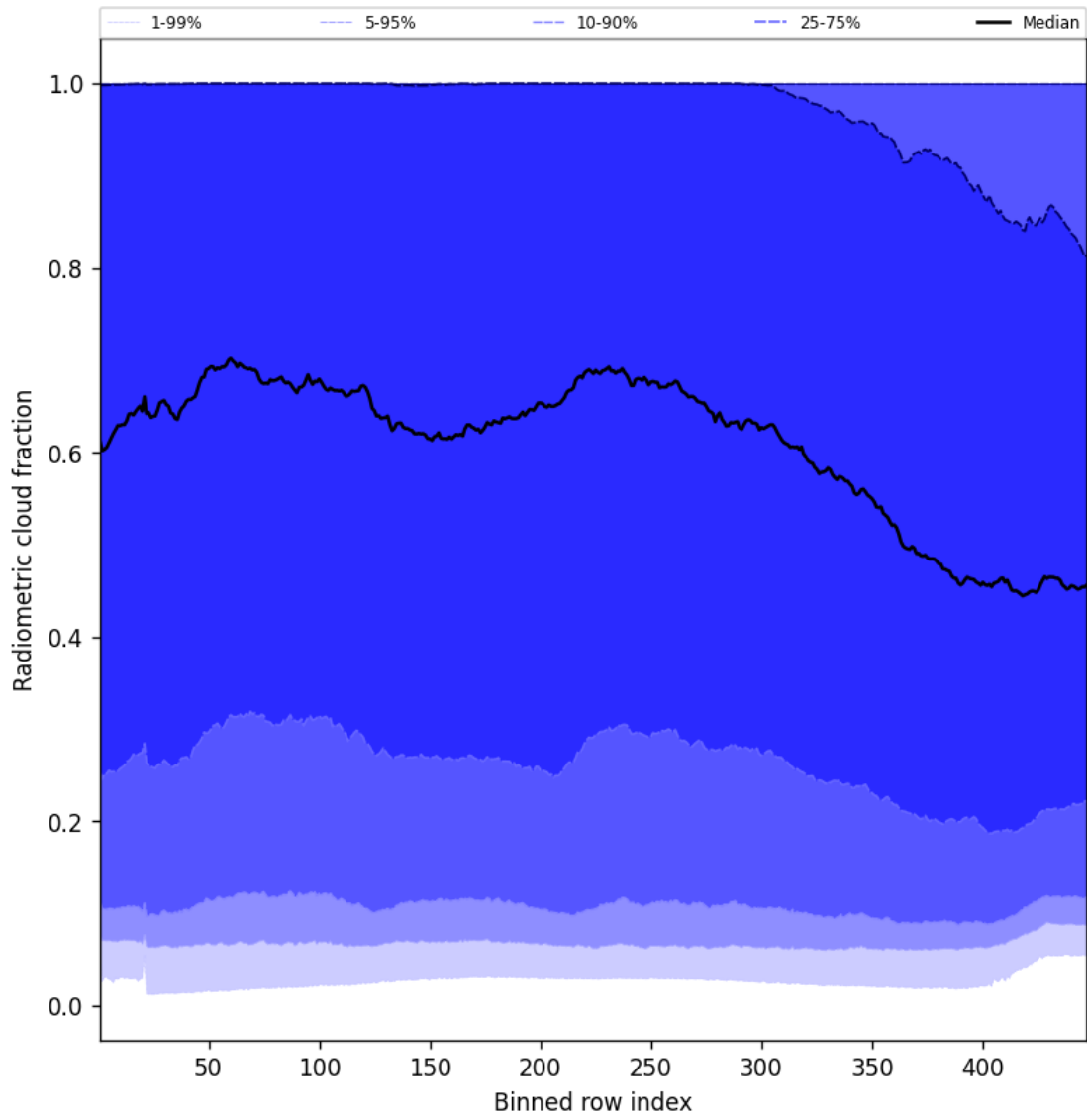
Figure 53: Along track statistics of “Radiometric cloud fraction” for 2025-07-25 to 2025-07-26
