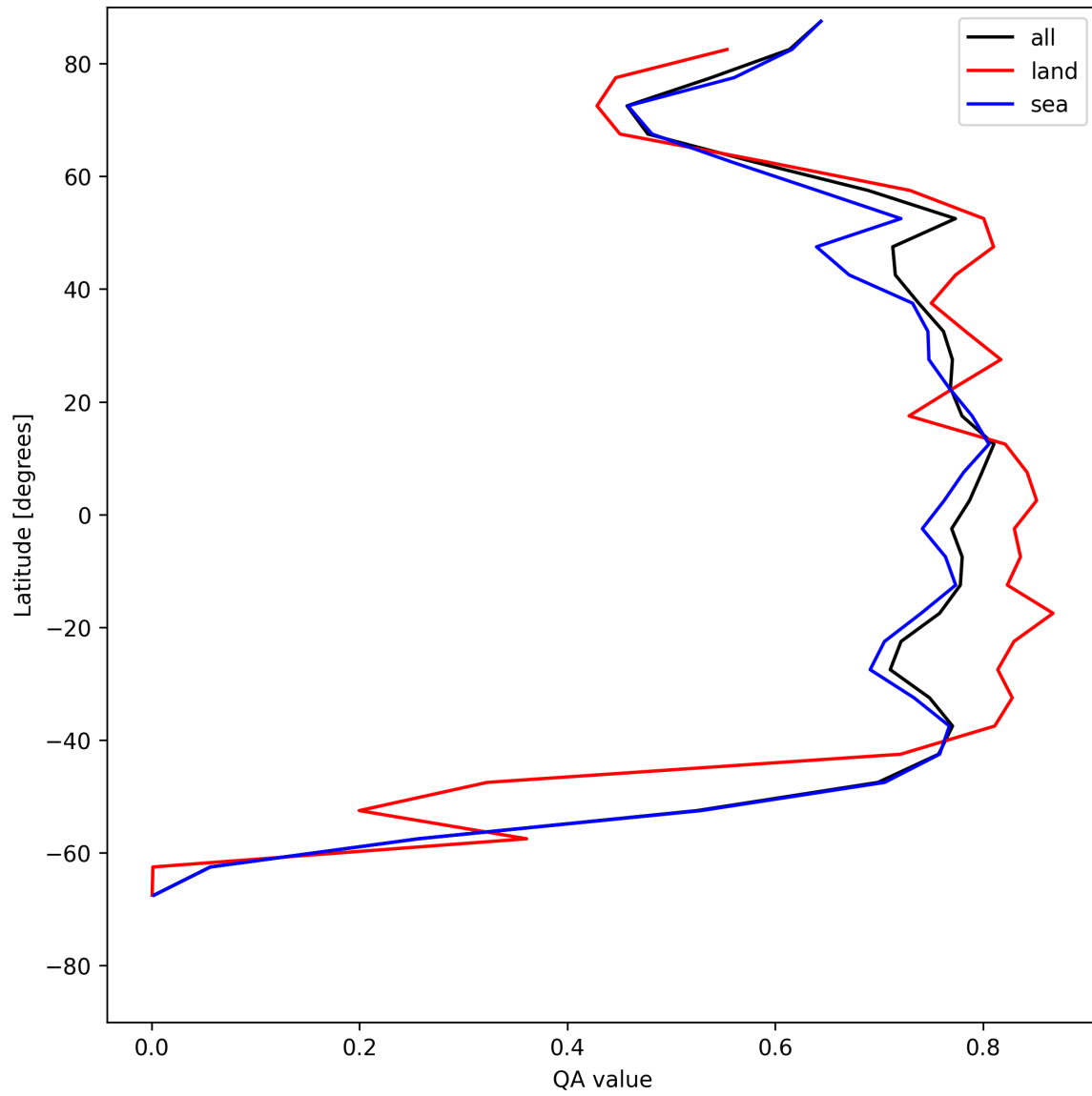
Figure 20: Zonal average of “QA value” for 2025-07-25 to 2025-07-26.
