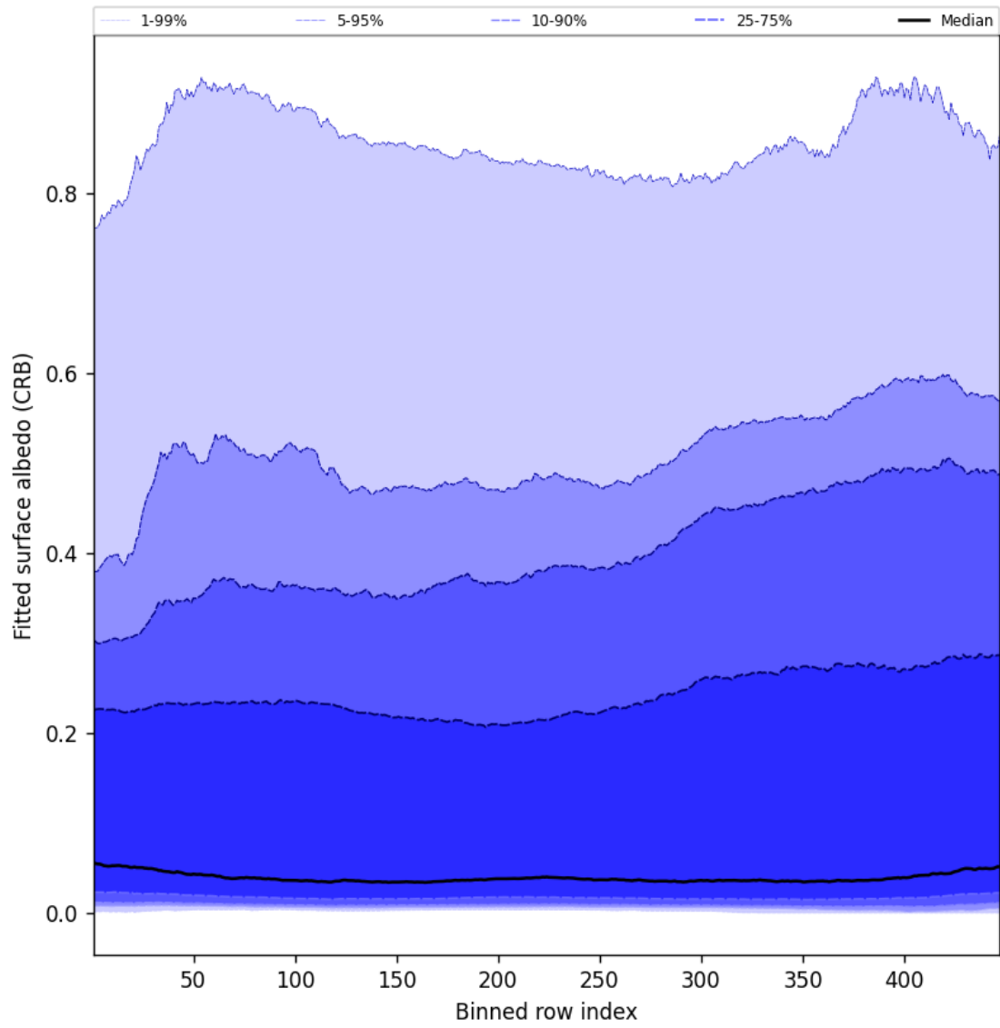
Figure 60: Along track statistics of “Fitted surface albedo (CRB)” for 2025-07-25 to 2025-07-26
