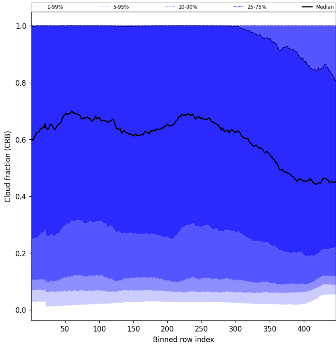
Figure 56: Along track statistics of “Cloud fraction (CRB)” for 2025-07-25 to 2025-07-26
