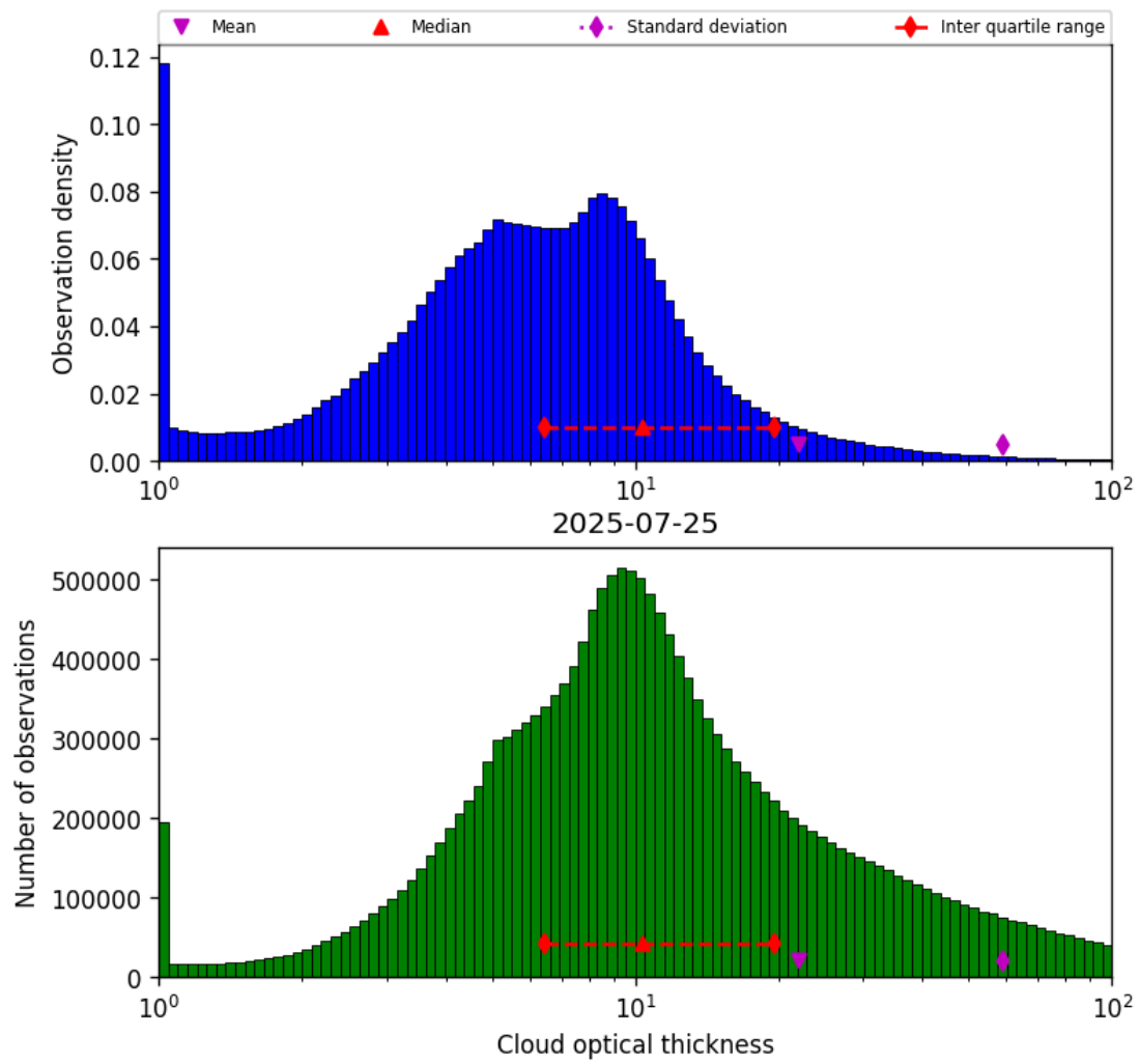
Figure 39: Histogram of “Cloud optical thickness” for 2025-07-25 to 2025-07-26
