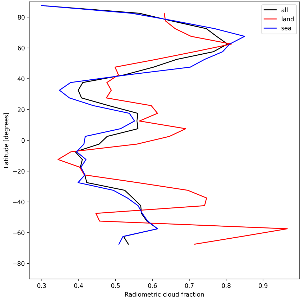
Figure 21: Zonal average of “Radiometric cloud fraction” for 2025-07-25 to 2025-07-26.
