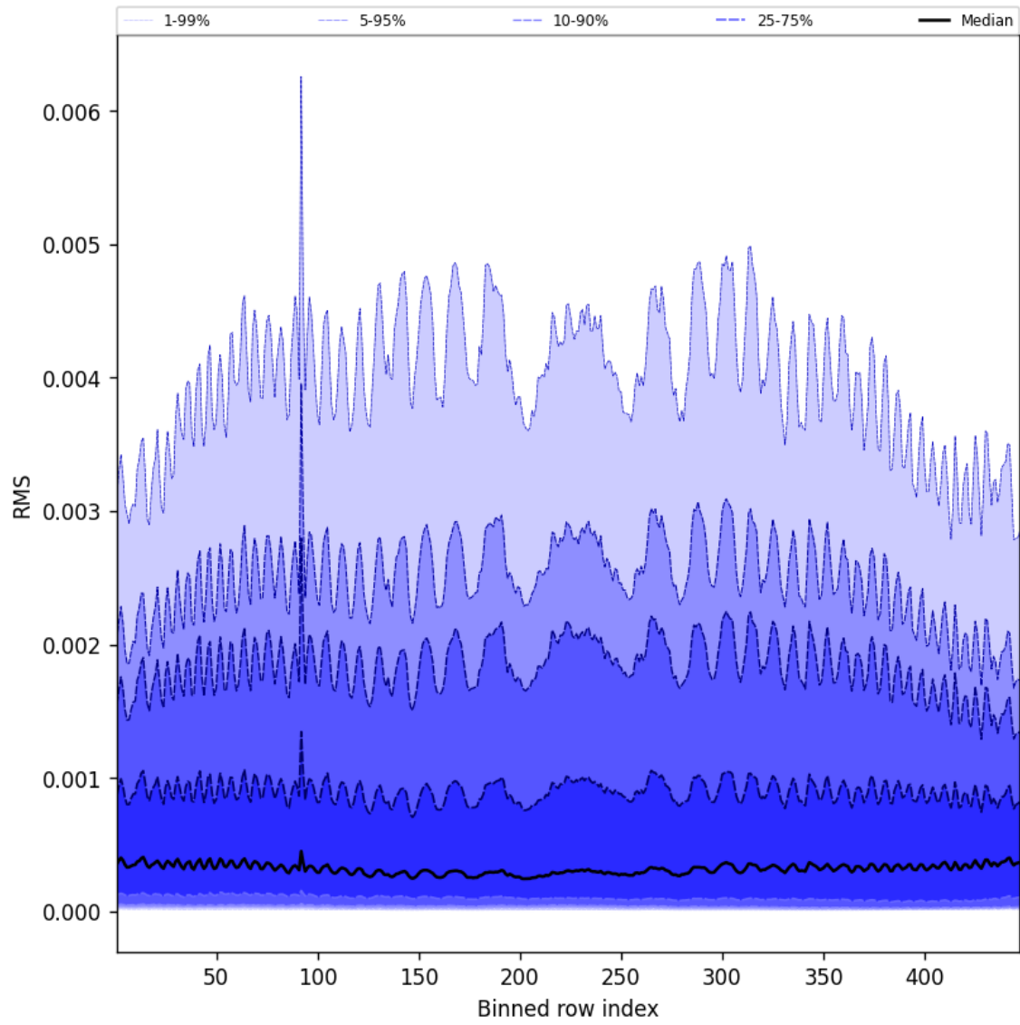
Figure 61: Along track statistics of “RMS” for 2025-07-25 to 2025-07-26
