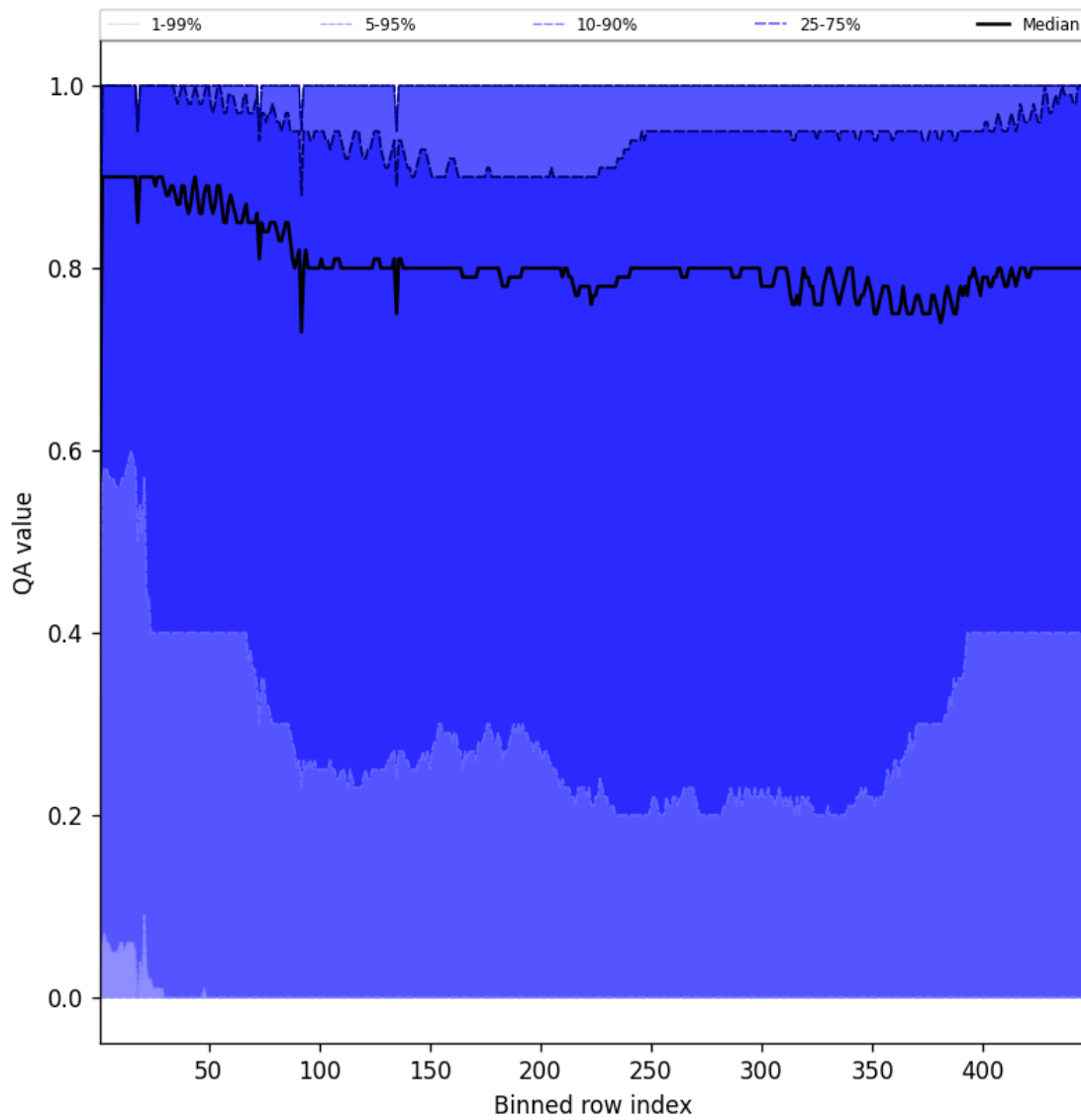
Figure 52: Along track statistics of “QA value” for 2025-07-25 to 2025-07-26
