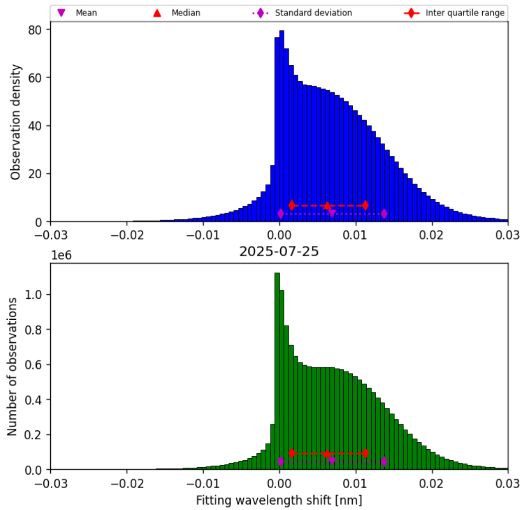
Figure 47: Histogram of “Fitting wavelength shift” for 2025-07-25 to 2025-07-26
