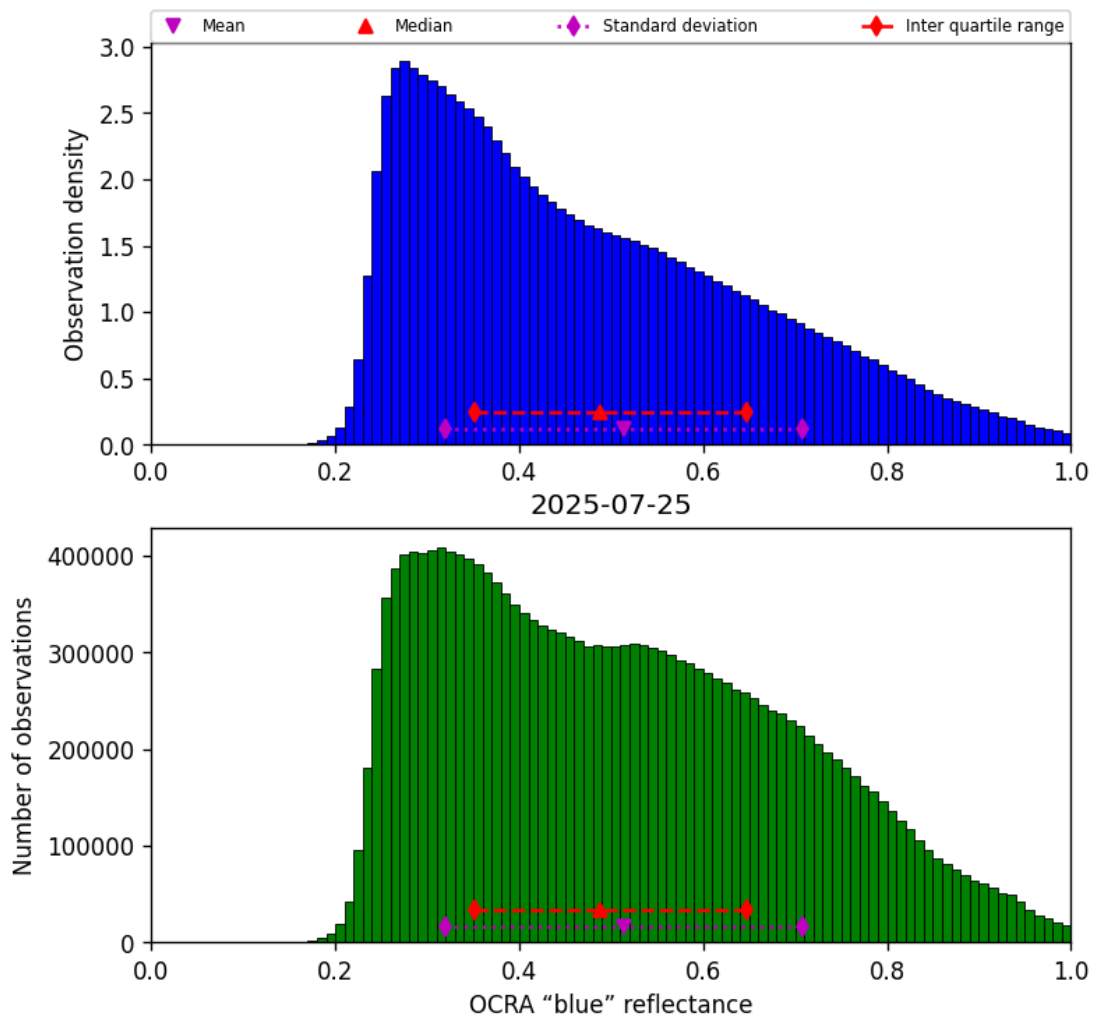
Figure 49: Histogram of “OCRA “blue” reflectance” for 2025-07-25 to 2025-07-26
