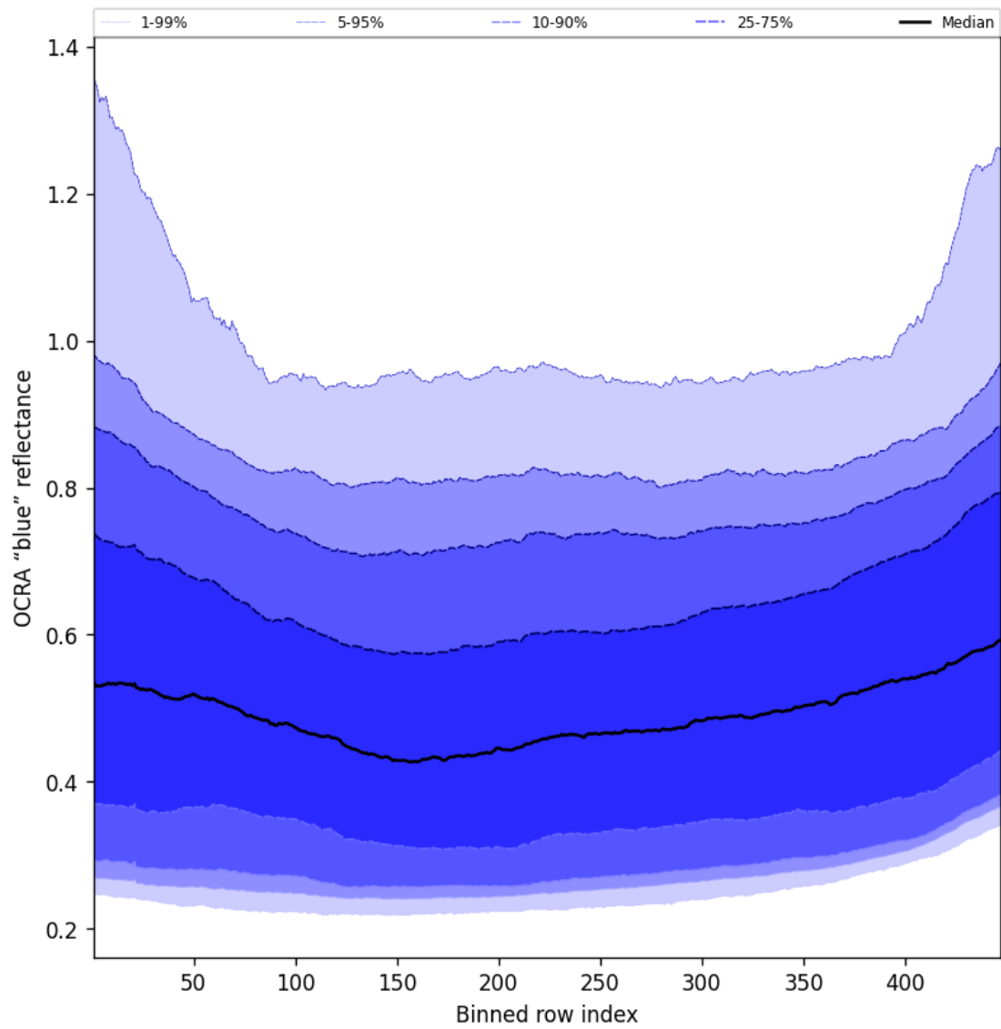
Figure 65: Along track statistics of “OCRA “blue” reflectance” for 2025-07-25 to 2025-07-26
