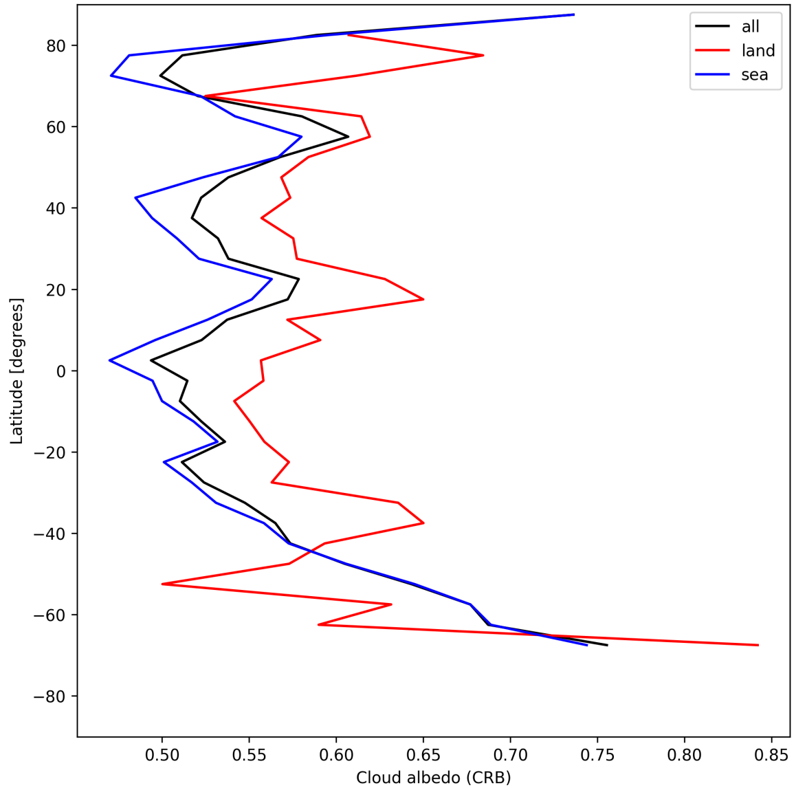
Figure 26: Zonal average of “Cloud albedo (CRB)” for 2025-07-25 to 2025-07-26.
