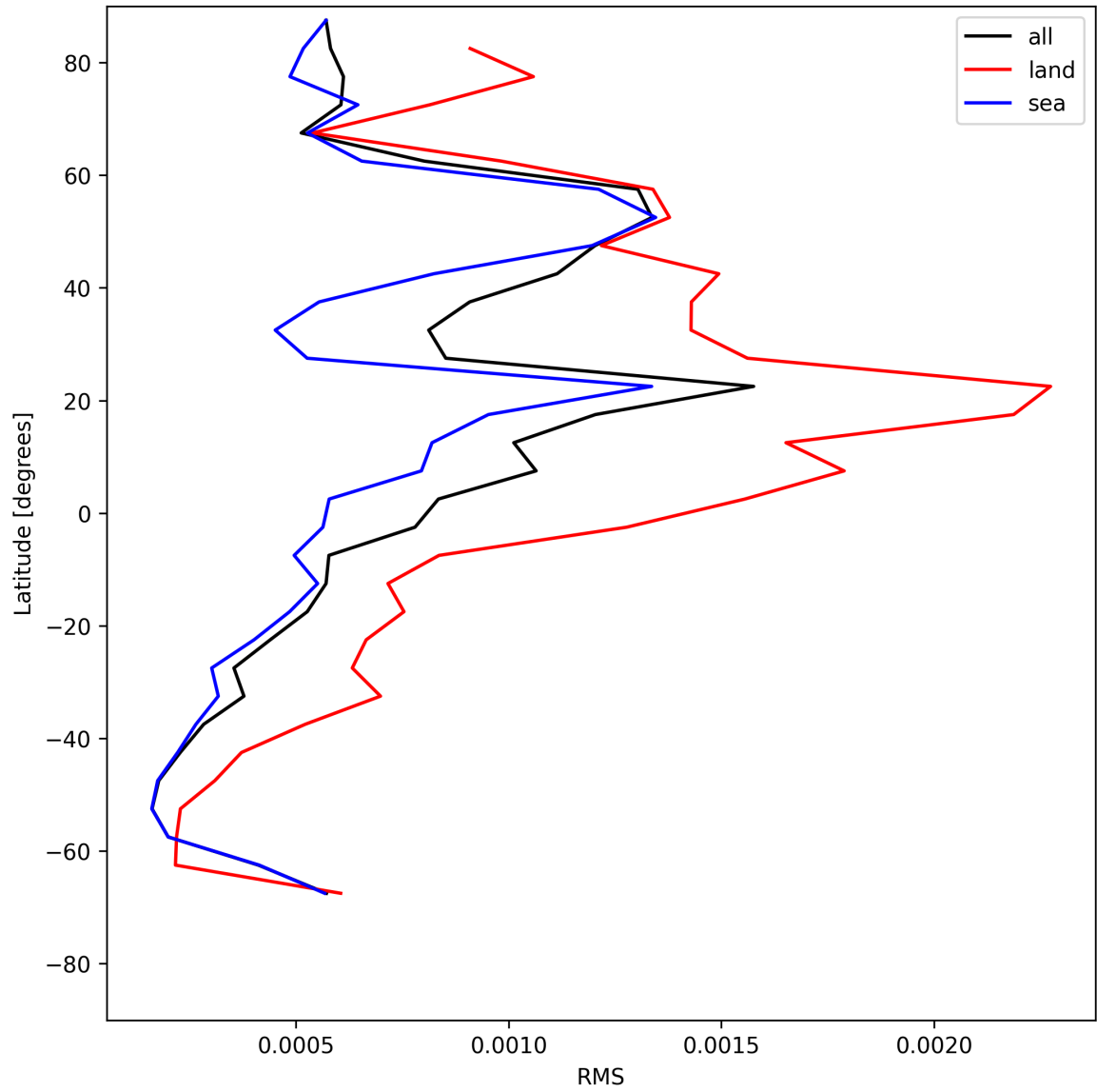
Figure 29: Zonal average of “RMS” for 2025-07-25 to 2025-07-26.
