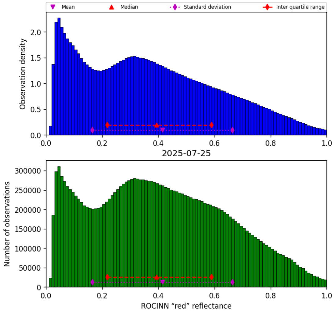
Figure 51: Histogram of “ROCINN “red” reflectance” for 2025-07-25 to 2025-07-26
