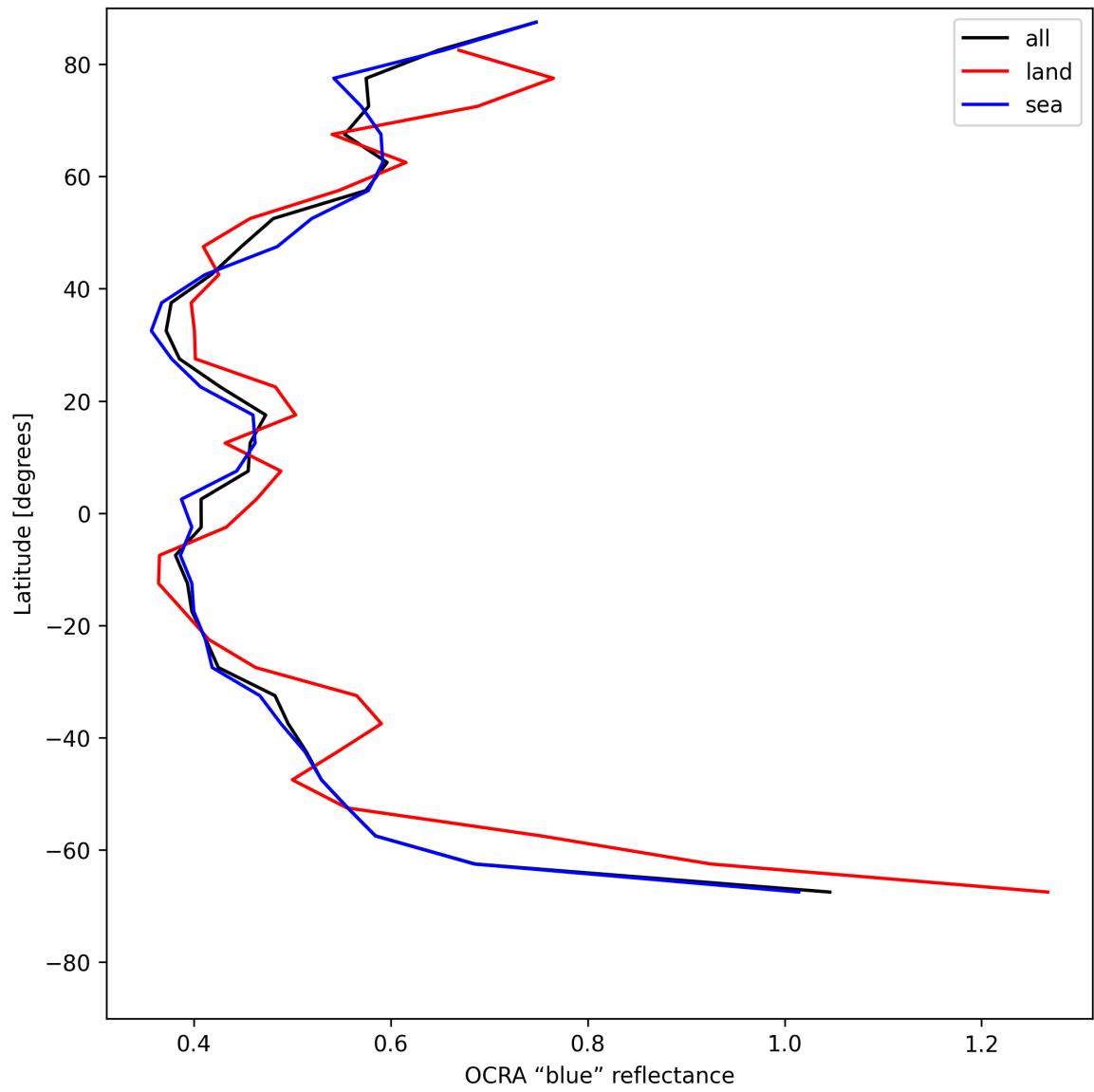
Figure 33: Zonal average of “OCRA “blue” reflectance” for 2025-07-25 to 2025-07-26.
