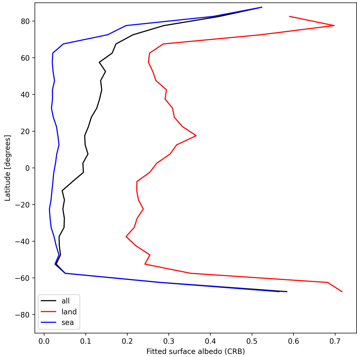
Figure 28: Zonal average of “Fitted surface albedo (CRB)” for 2025-07-25 to 2025-07-26.
