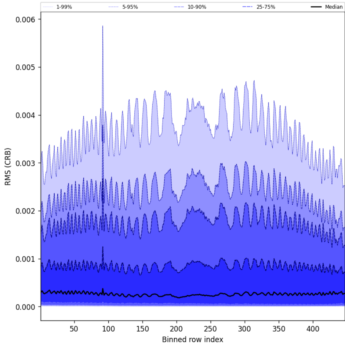
Figure 62: Along track statistics of “RMS (CRB)” for 2025-07-25 to 2025-07-26
