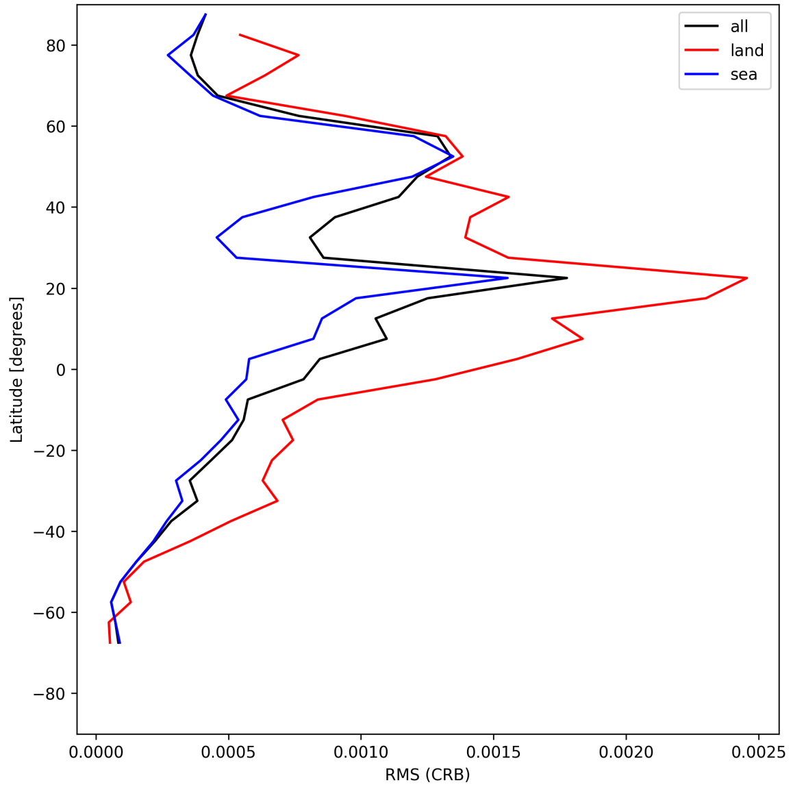
Figure 30: Zonal average of “RMS (CRB)” for 2025-07-25 to 2025-07-26.
