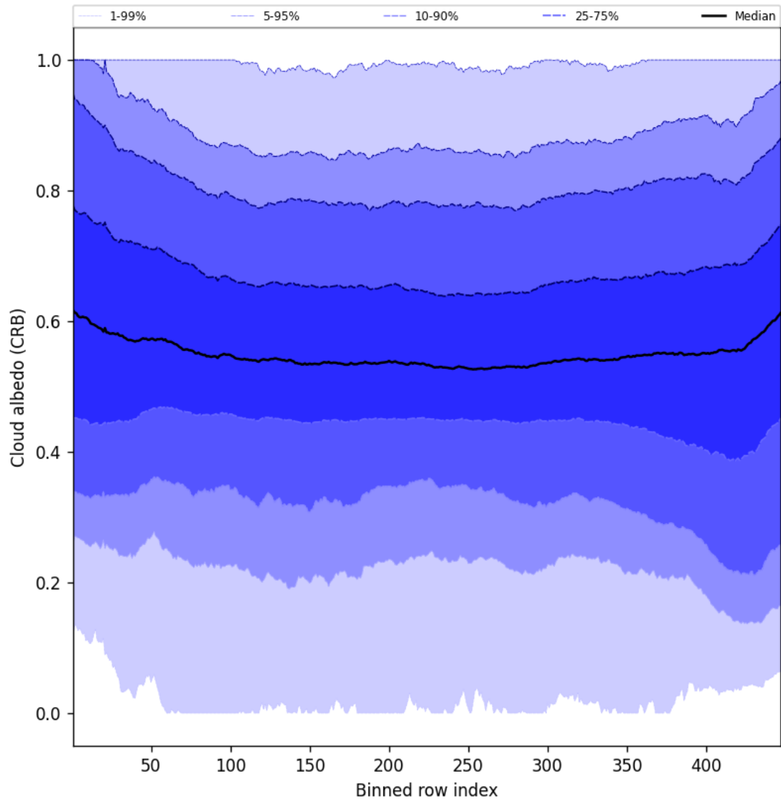
Figure 58: Along track statistics of “Cloud albedo (CRB)” for 2025-07-25 to 2025-07-26
