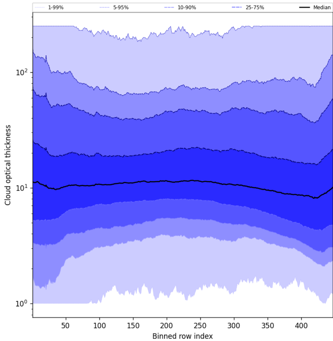
Figure 55: Along track statistics of “Cloud optical thickness” for 2025-07-25 to 2025-07-26
