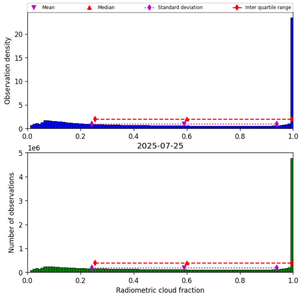
Figure 37: Histogram of “Radiometric cloud fraction” for 2025-07-25 to 2025-07-26
