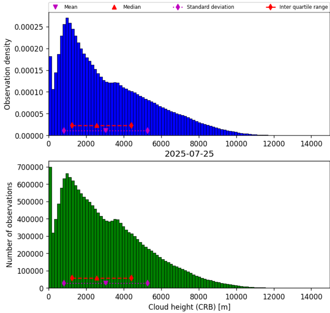
Figure 41: Histogram of “Cloud height (CRB)” for 2025-07-25 to 2025-07-26
