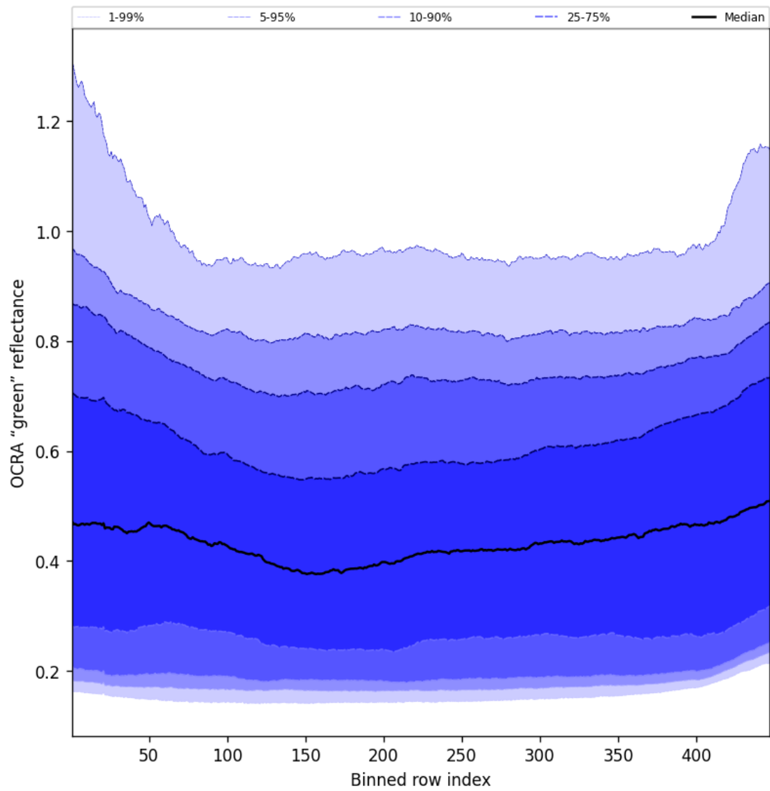
Figure 66: Along track statistics of “OCRA “green” reflectance” for 2025-07-25 to 2025-07-26
