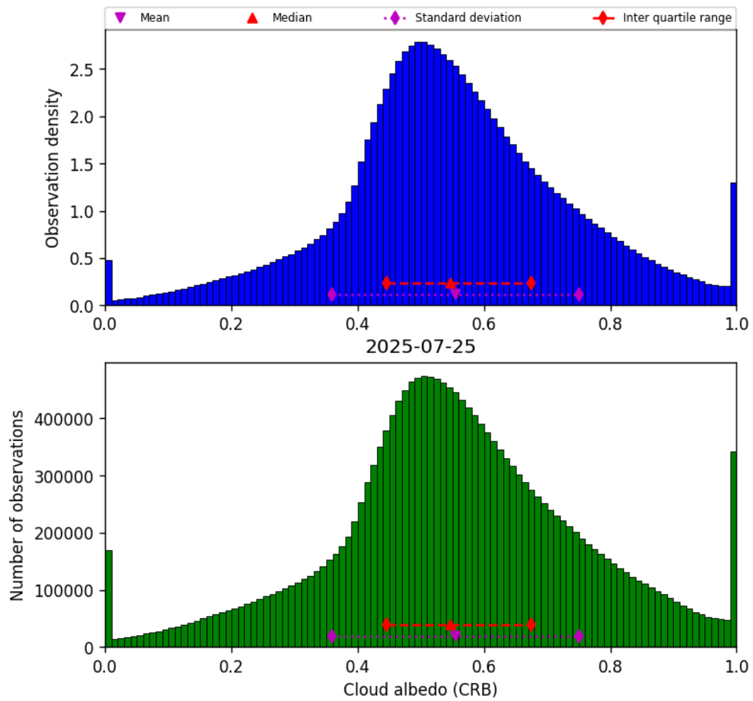
Figure 42: Histogram of “Cloud albedo (CRB)” for 2025-07-25 to 2025-07-26
