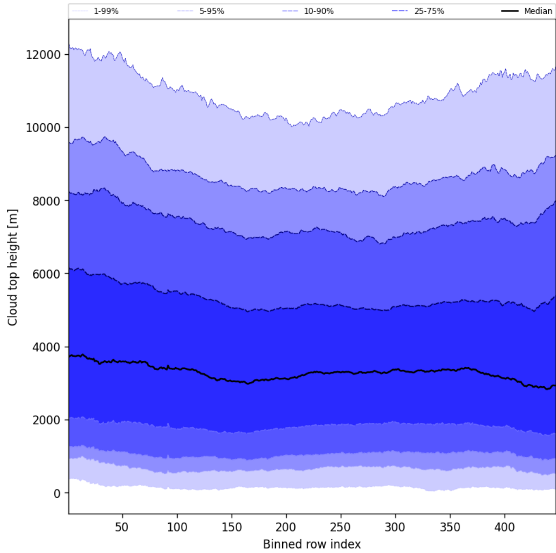
Figure 54: Along track statistics of “Cloud top height” for 2025-07-25 to 2025-07-26
