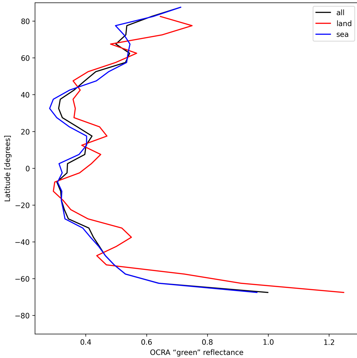
Figure 34: Zonal average of “OCRA “green” reflectance” for 2025-07-25 to 2025-07-26.
