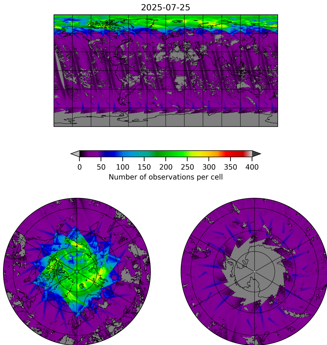
Figure 19: Map of the number of observations for 2025-07-25 to 2025-07-26
