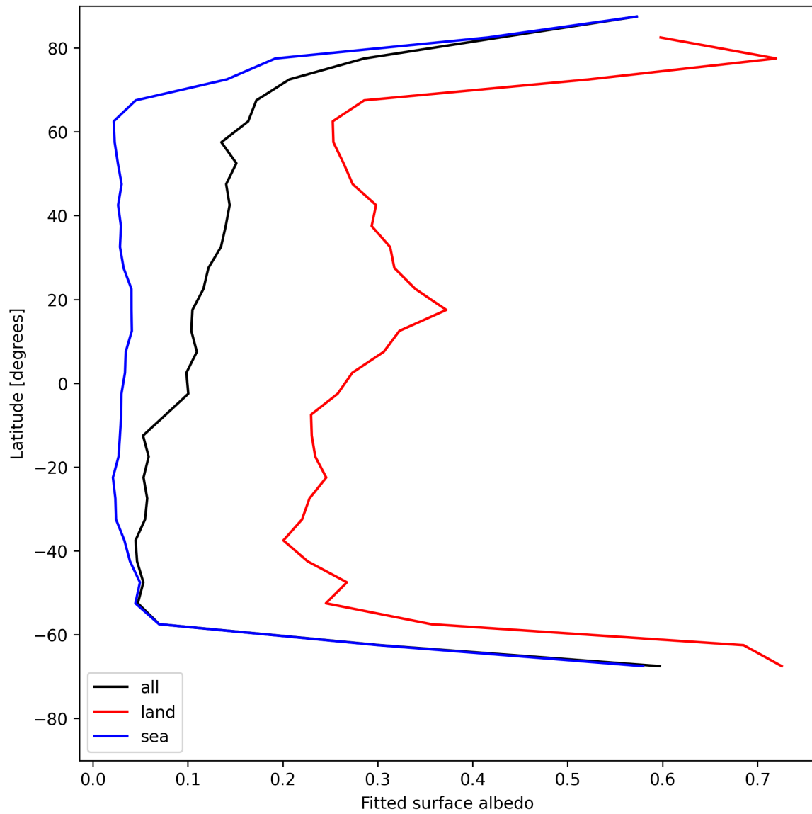
Figure 27: Zonal average of “Fitted surface albedo” for 2025-07-25 to 2025-07-26.
