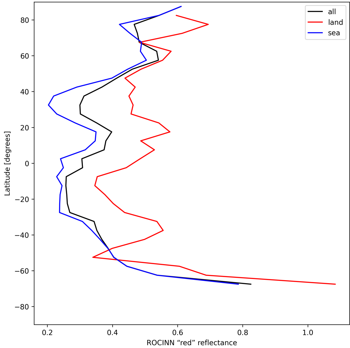
Figure 35: Zonal average of “ROCINN “red” reflectance” for 2025-07-25 to 2025-07-26.
