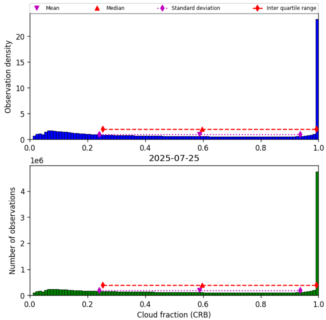
Figure 40: Histogram of “Cloud fraction (CRB)” for 2025-07-25 to 2025-07-26
