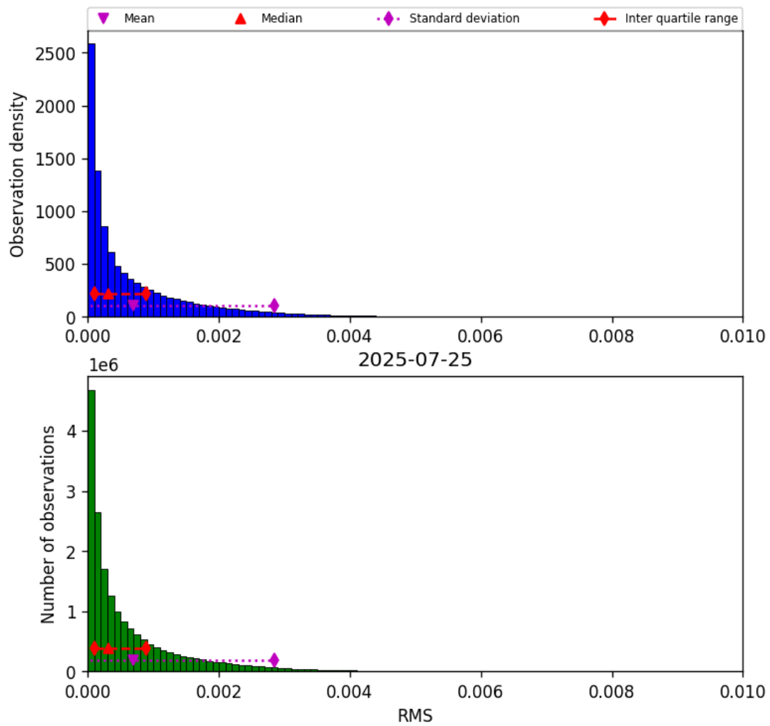
Figure 45: Histogram of “RMS” for 2025-07-25 to 2025-07-26
