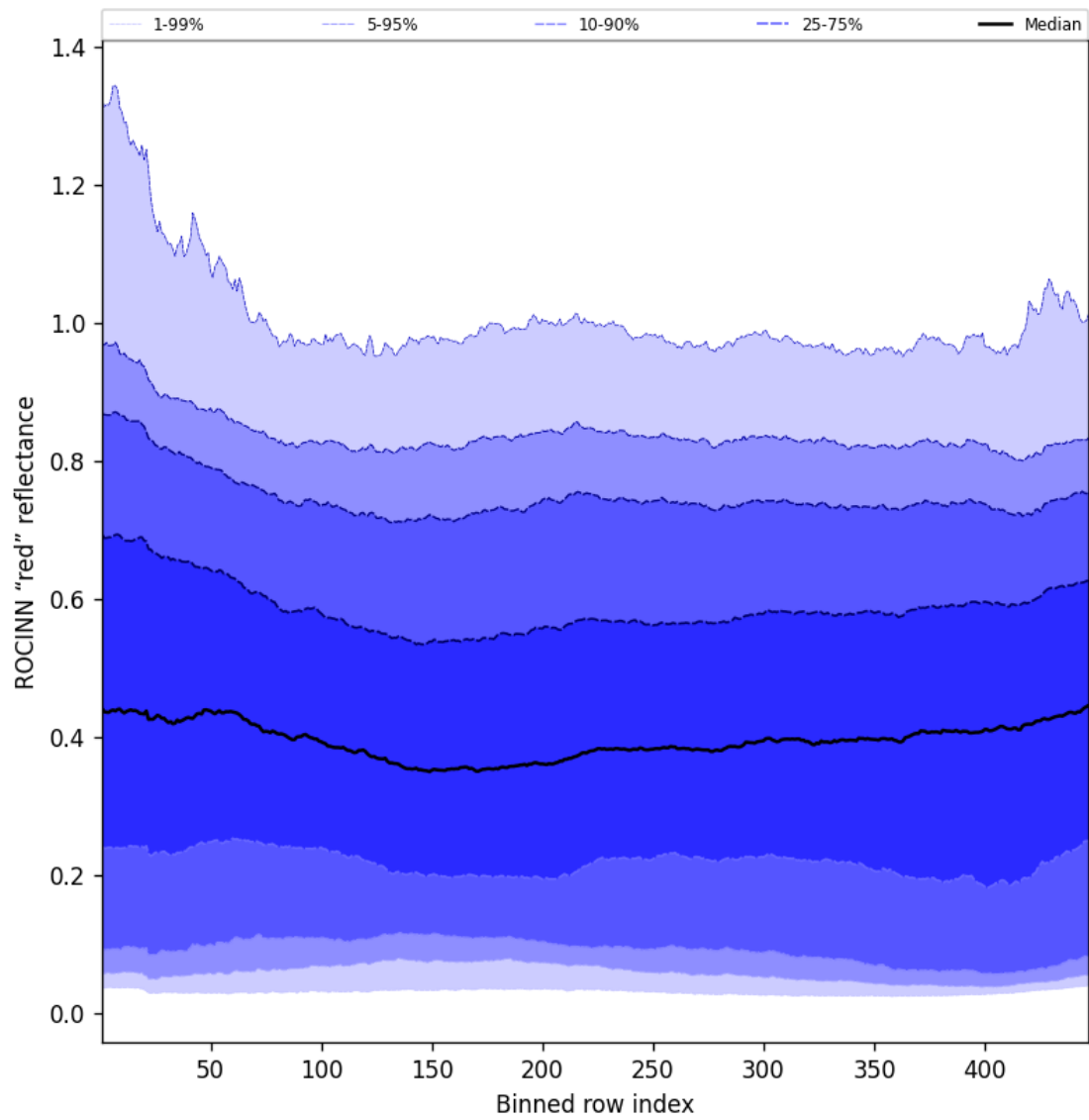
Figure 67: Along track statistics of "ROCINN "red" reflectance" for 2025-07-25 to 2025-07-26
