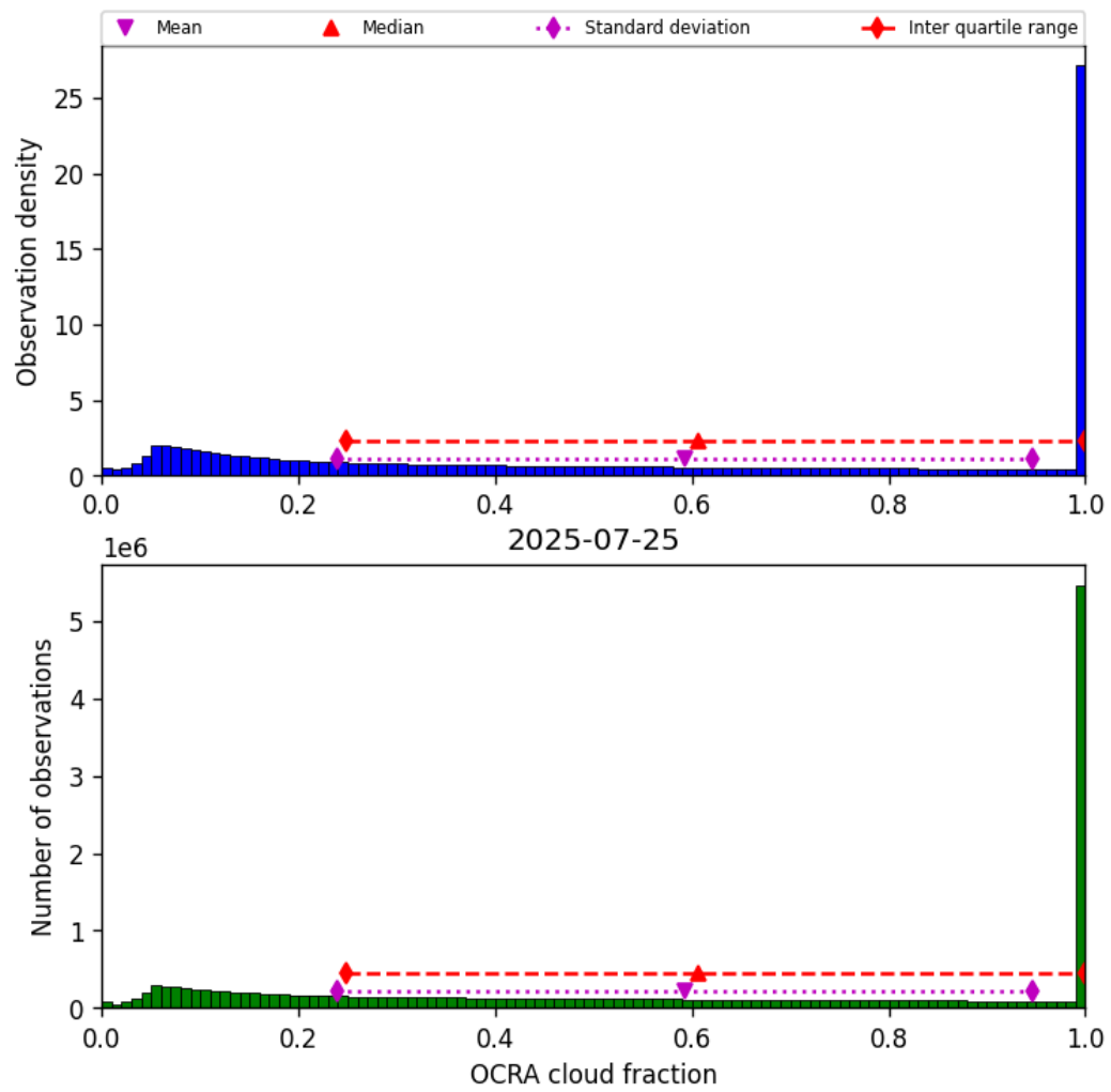
Figure 48: Histogram of “OCRA cloud fraction” for 2025-07-25 to 2025-07-26
