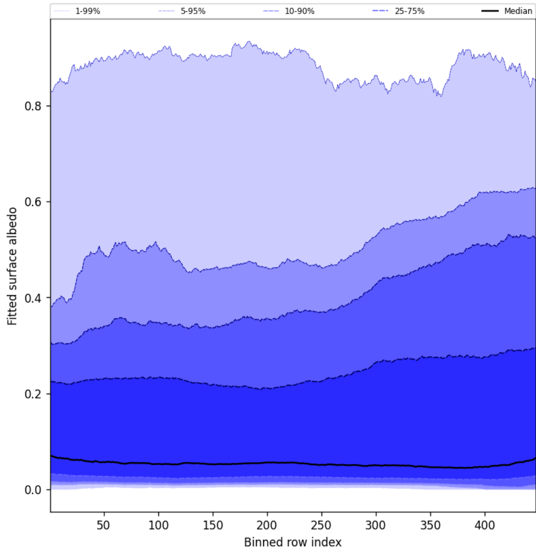
Figure 59: Along track statistics of “Fitted surface albedo” for 2025-07-25 to 2025-07-26
