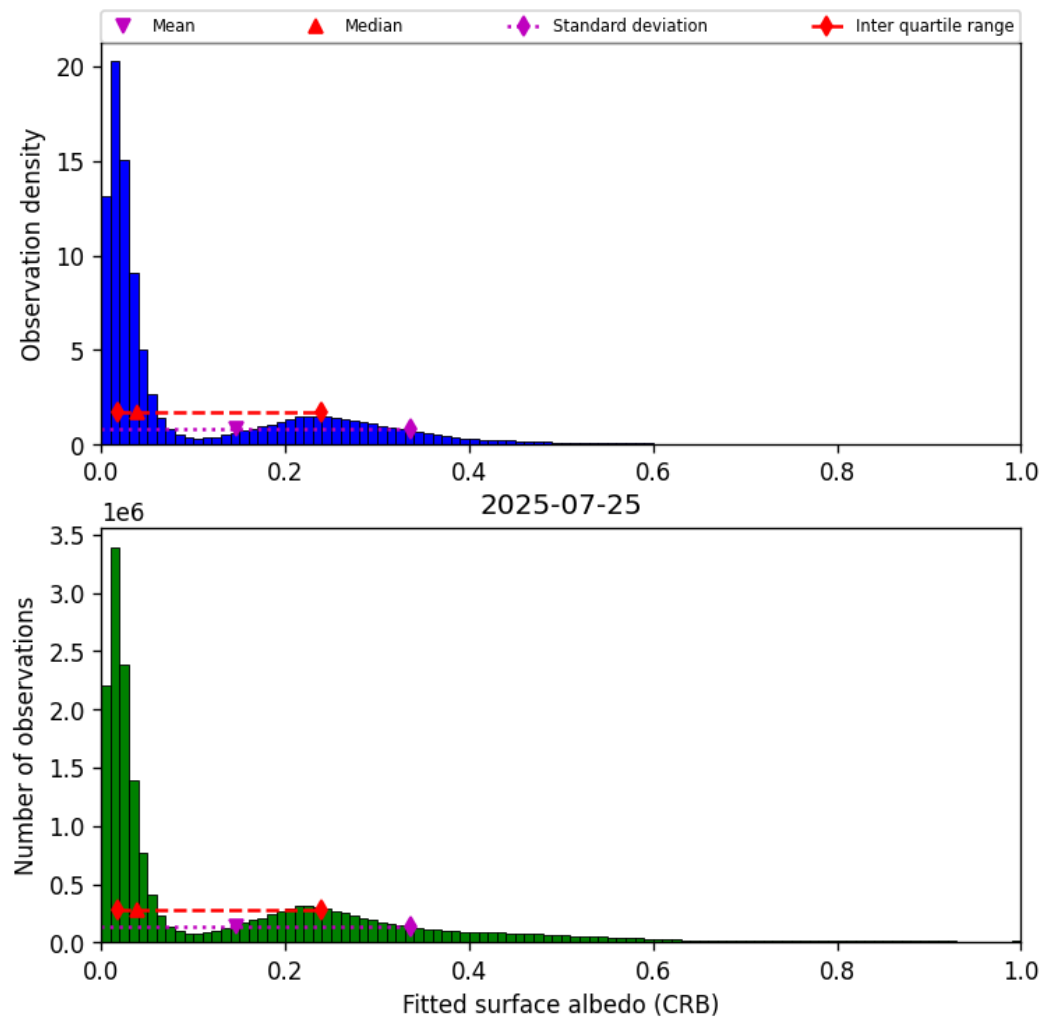
Figure 44: Histogram of “Fitted surface albedo (CRB)” for 2025-07-25 to 2025-07-26
