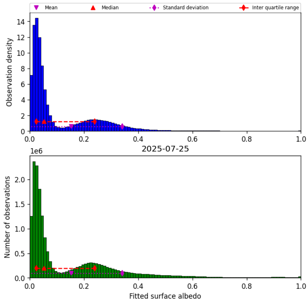
Figure 43: Histogram of “Fitted surface albedo” for 2025-07-25 to 2025-07-26
