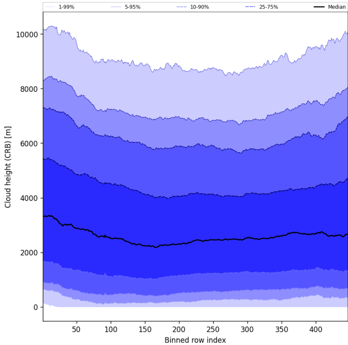
Figure 57: Along track statistics of “Cloud height (CRB)” for 2025-07-25 to 2025-07-26
