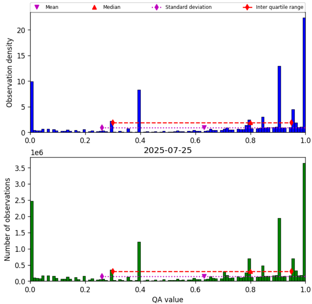
Figure 36: Histogram of “QA value” for 2025-07-25 to 2025-07-26
