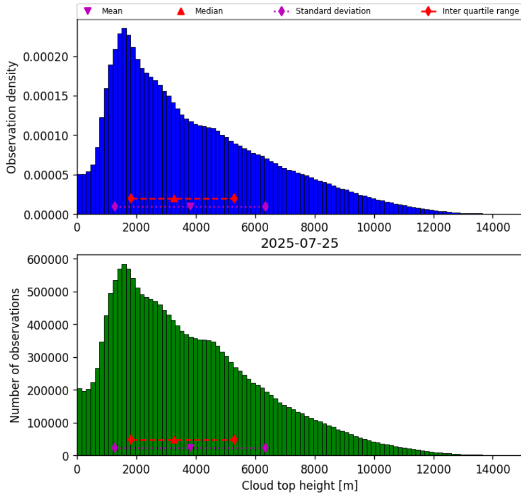
Figure 38: Histogram of “Cloud top height” for 2025-07-25 to 2025-07-26
