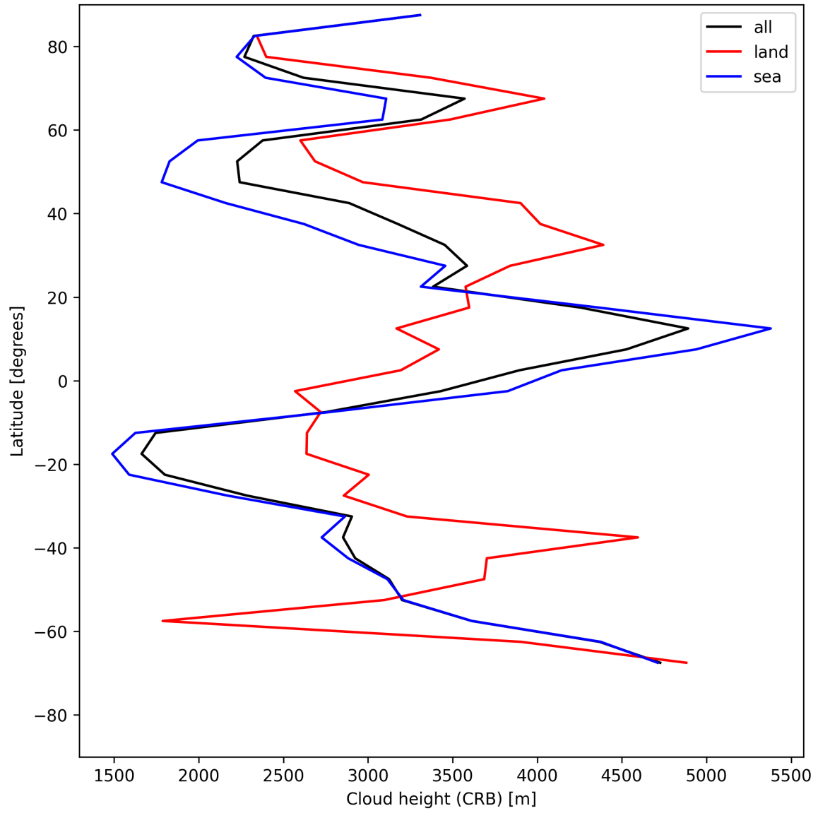
Figure 25: Zonal average of “Cloud height (CRB)” for 2025-07-25 to 2025-07-26.
