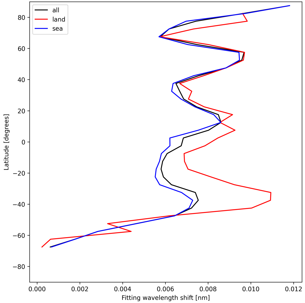
Figure 31: Zonal average of “Fitting wavelength shift” for 2025-07-25 to 2025-07-26.
