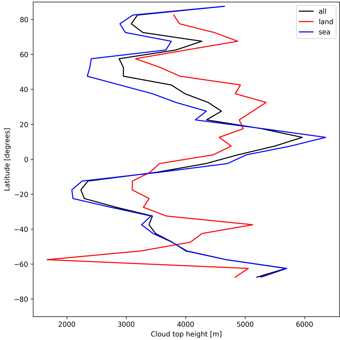
Figure 22: Zonal average of “Cloud top height” for 2025-07-25 to 2025-07-26.
