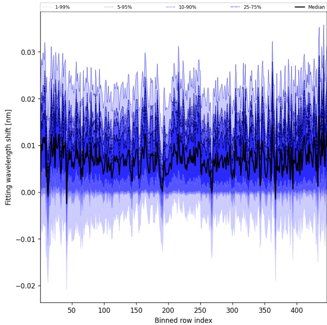
Figure 63: Along track statistics of “Fitting wavelength shift” for 2025-07-25 to 2025-07-26
