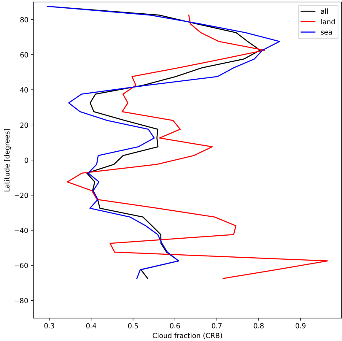
Figure 24: Zonal average of “Cloud fraction (CRB)” for 2025-07-25 to 2025-07-26.
