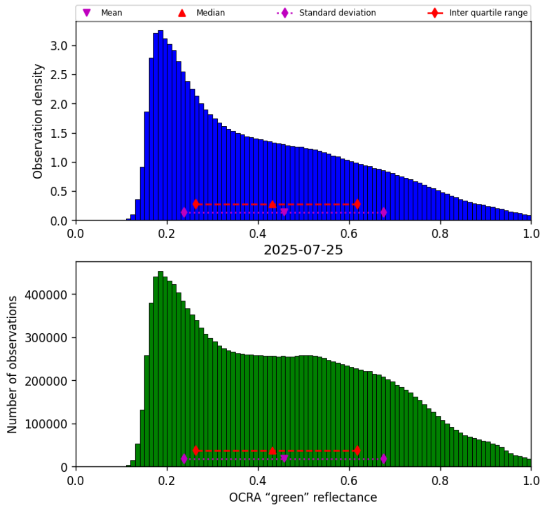
Figure 50: Histogram of “OCRA “green” reflectance” for 2025-07-25 to 2025-07-26
