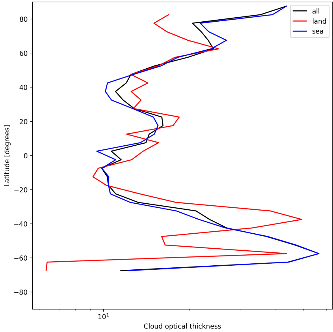
Figure 23: Zonal average of “Cloud optical thickness” for 2025-07-25 to 2025-07-26.
