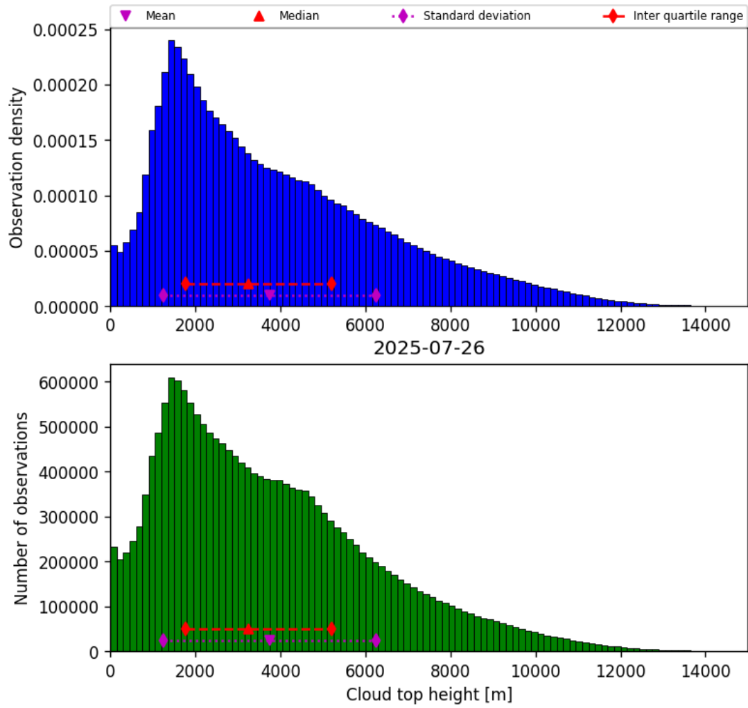
Figure 38: Histogram of “Cloud top height” for 2025-07-26 to 2025-07-27
