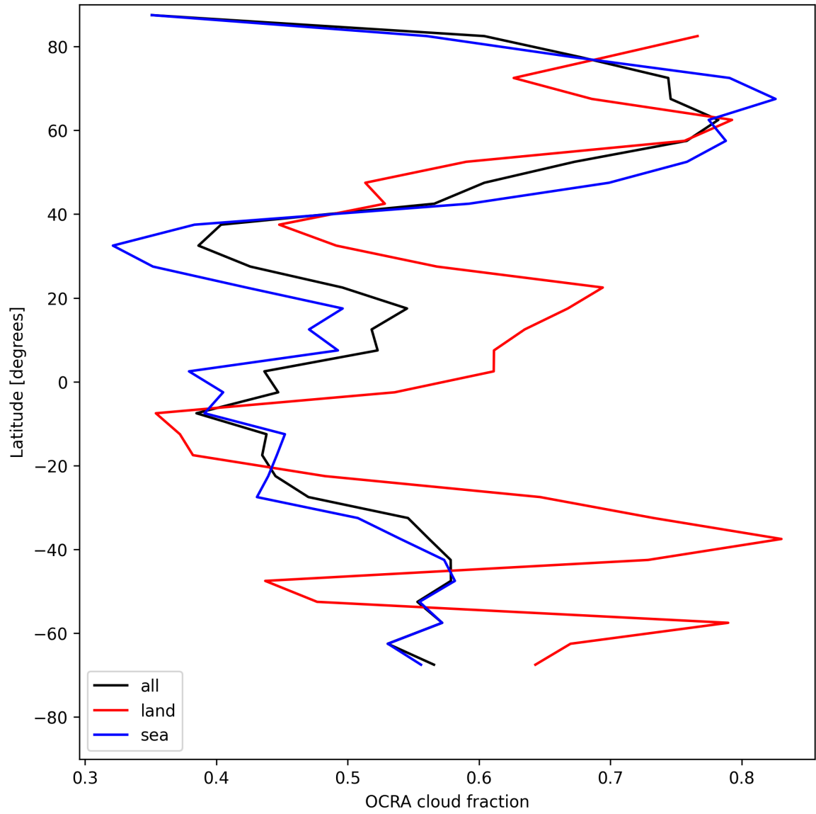
Figure 32: Zonal average of “OCRA cloud fraction” for 2025-07-26 to 2025-07-27.
