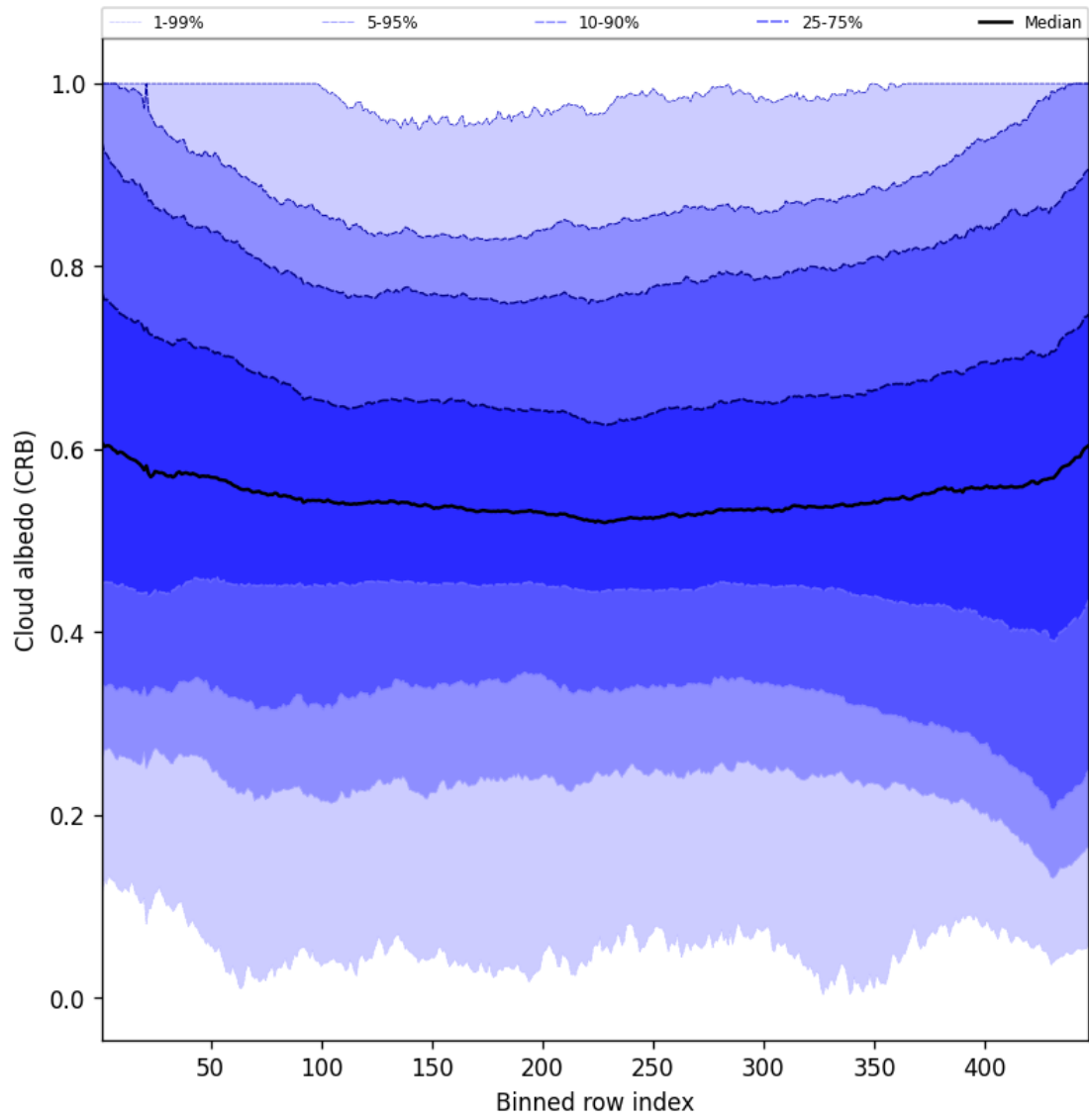
Figure 58: Along track statistics of “Cloud albedo (CRB)” for 2025-07-26 to 2025-07-27
