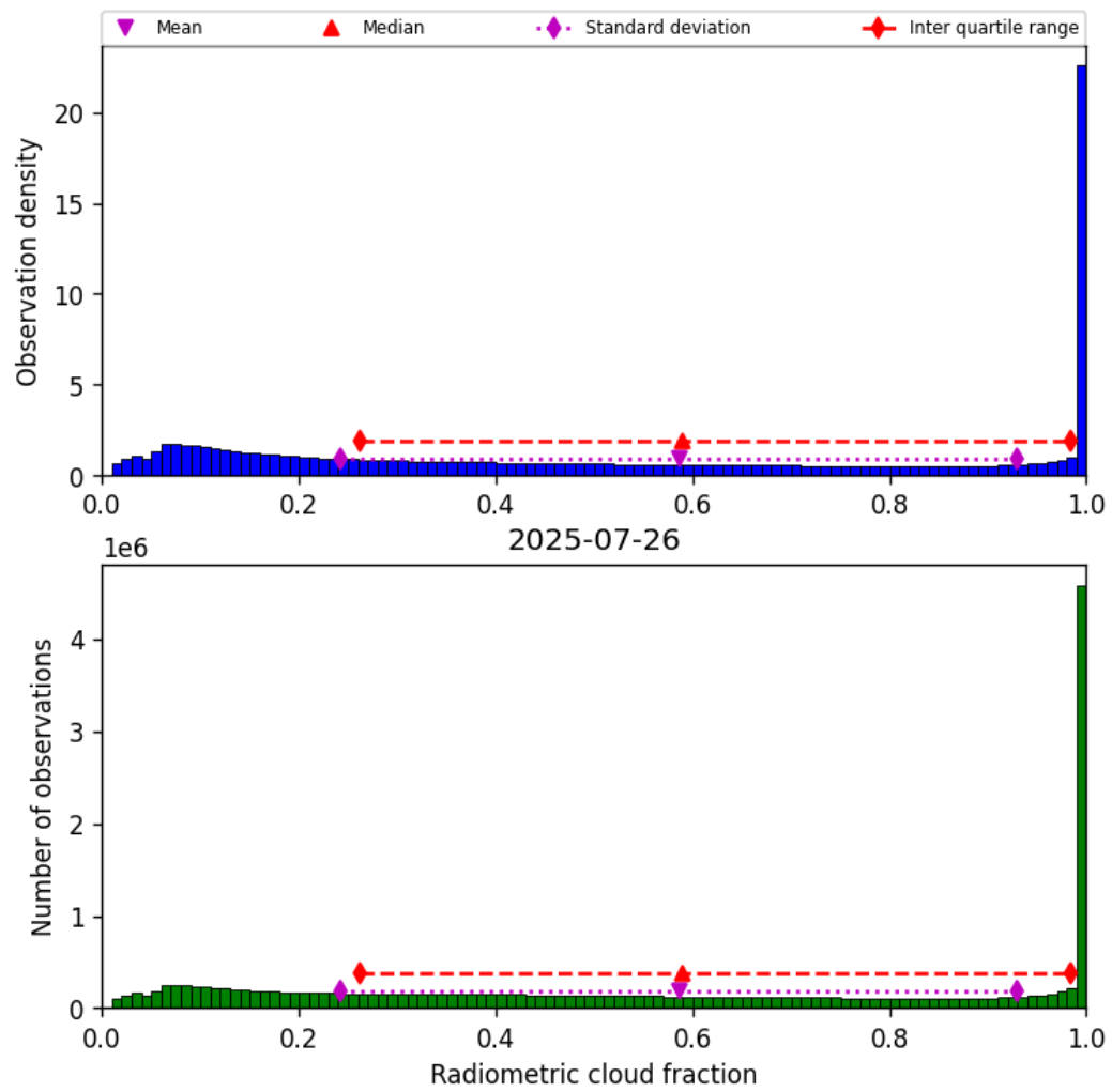
Figure 37: Histogram of “Radiometric cloud fraction” for 2025-07-26 to 2025-07-27
