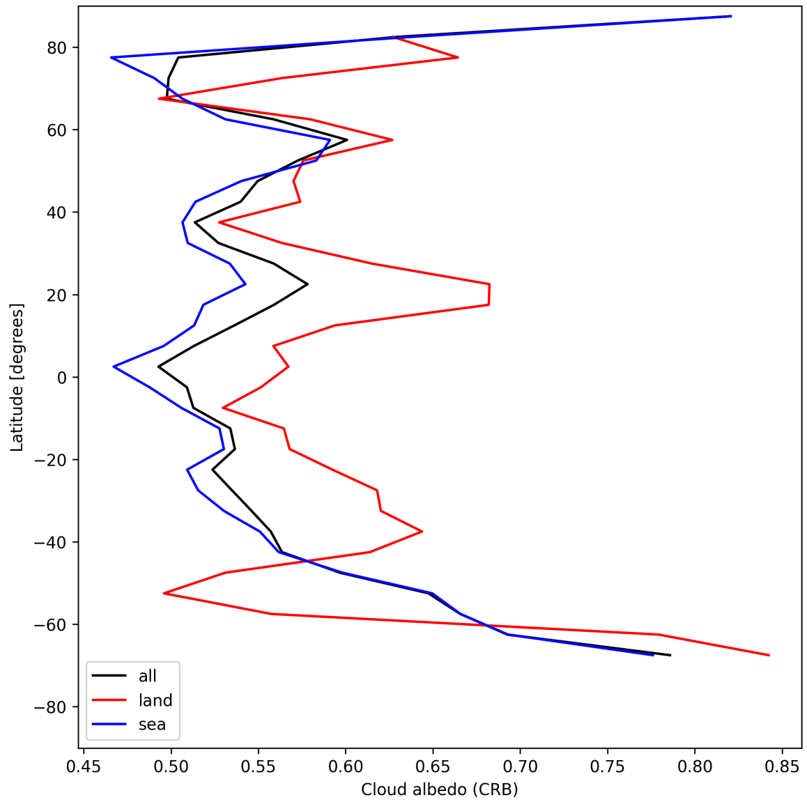
Figure 26: Zonal average of “Cloud albedo (CRB)” for 2025-07-26 to 2025-07-27.
