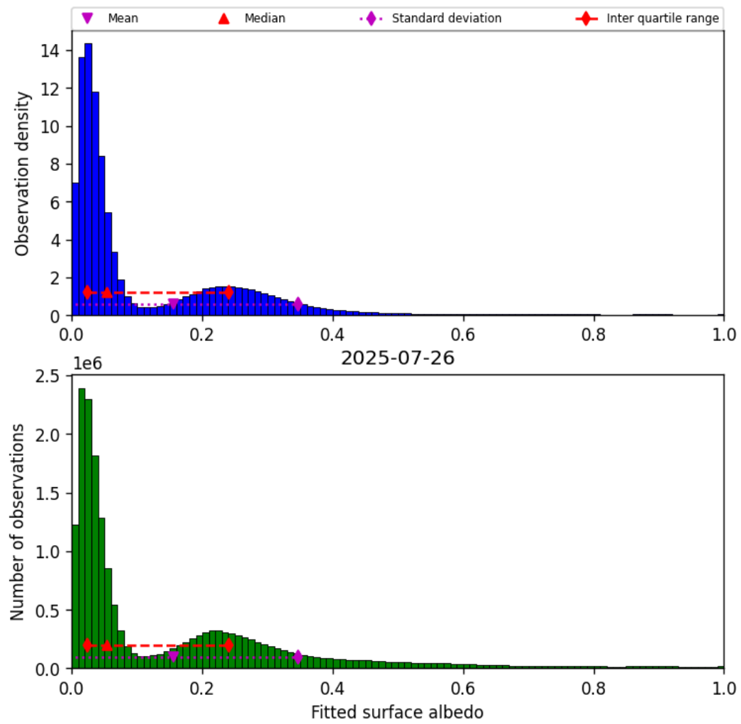
Figure 43: Histogram of “Fitted surface albedo” for 2025-07-26 to 2025-07-27
