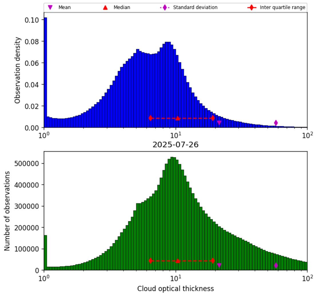
Figure 39: Histogram of “Cloud optical thickness” for 2025-07-26 to 2025-07-27
