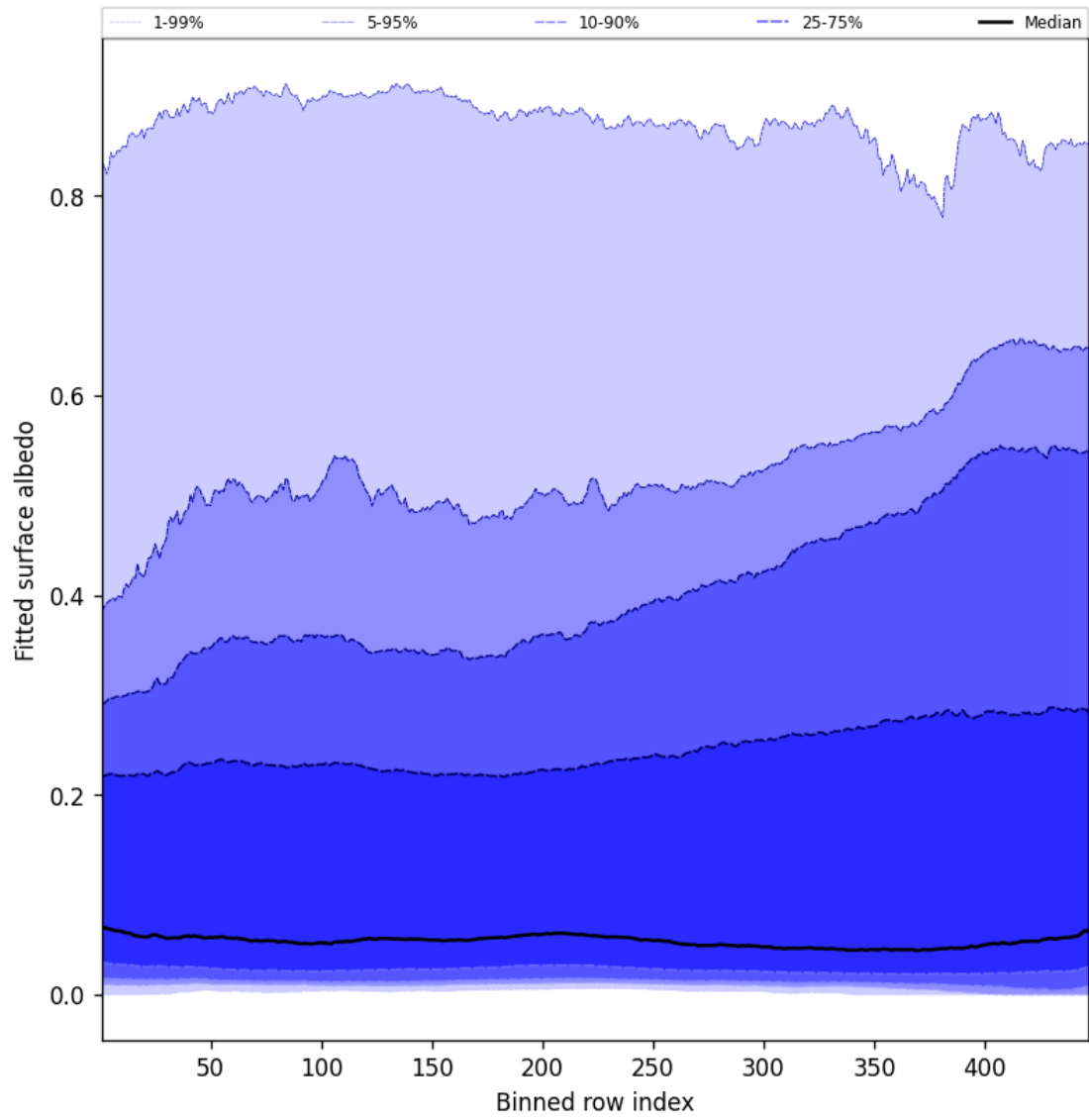
Figure 59: Along track statistics of “Fitted surface albedo” for 2025-07-26 to 2025-07-27
