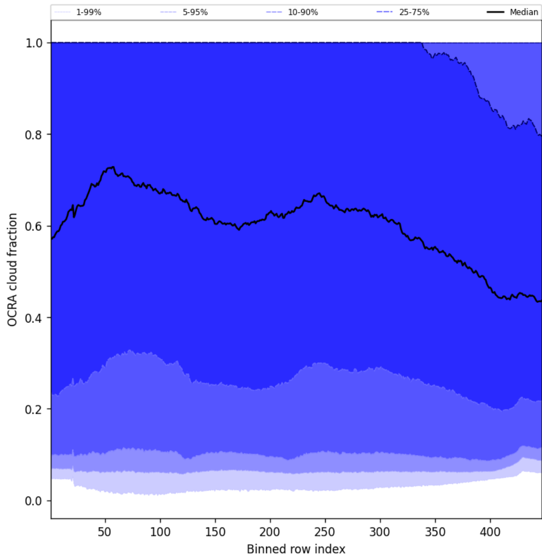
Figure 64: Along track statistics of “OCRA cloud fraction” for 2025-07-26 to 2025-07-27
