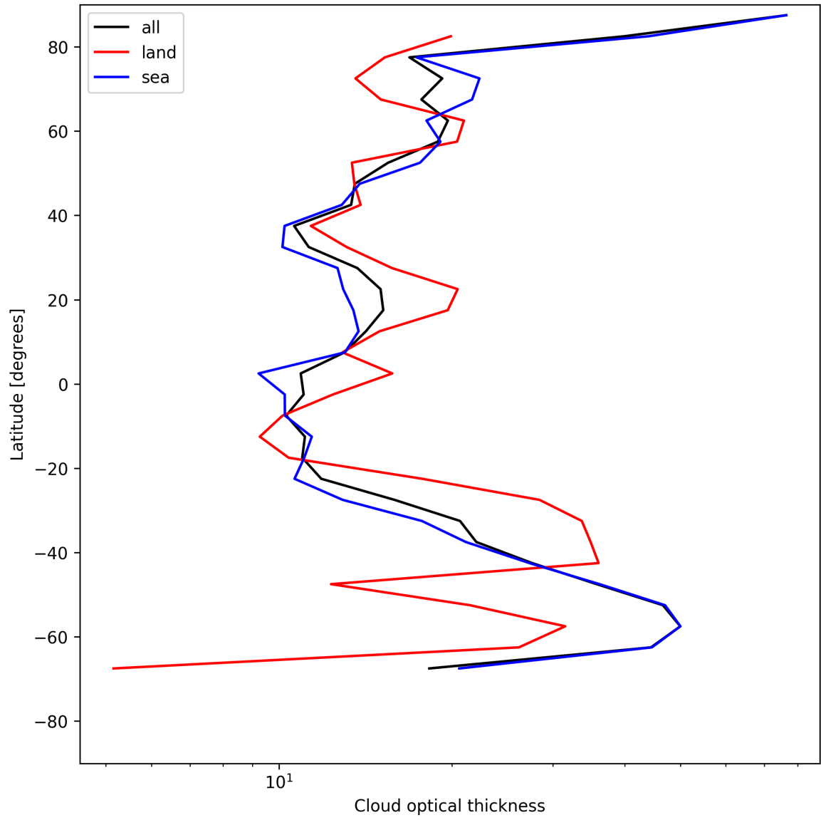
Figure 23: Zonal average of “Cloud optical thickness” for 2025-07-26 to 2025-07-27.
