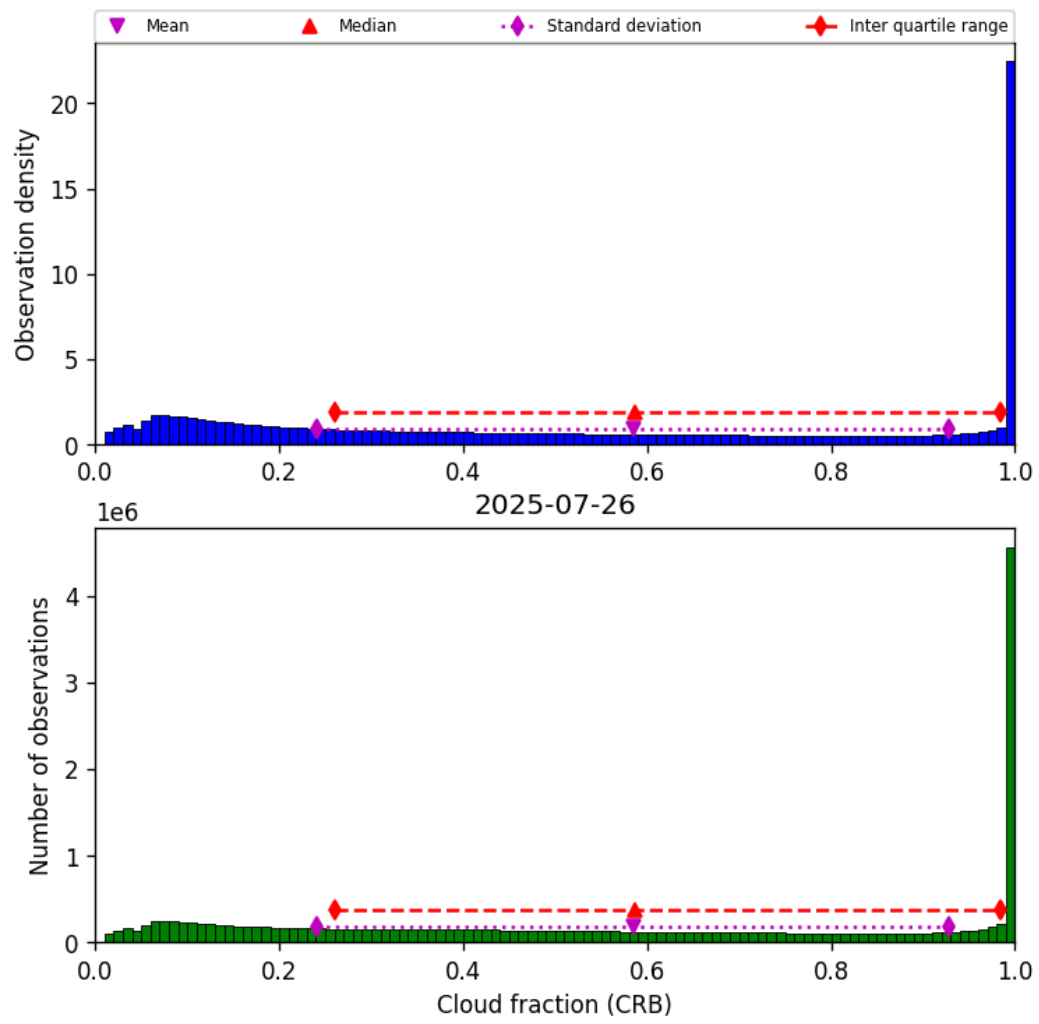
Figure 40: Histogram of “Cloud fraction (CRB)” for 2025-07-26 to 2025-07-27
