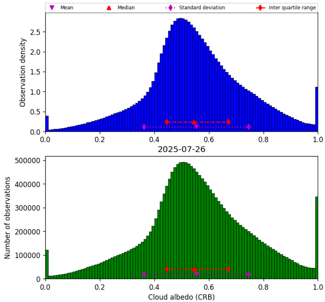
Figure 42: Histogram of “Cloud albedo (CRB)” for 2025-07-26 to 2025-07-27
