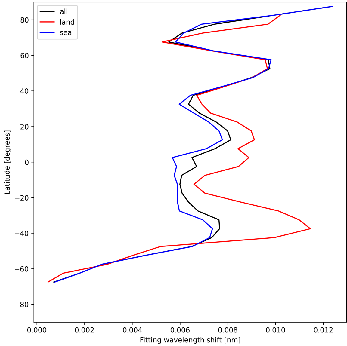
Figure 31: Zonal average of “Fitting wavelength shift” for 2025-07-26 to 2025-07-27.
