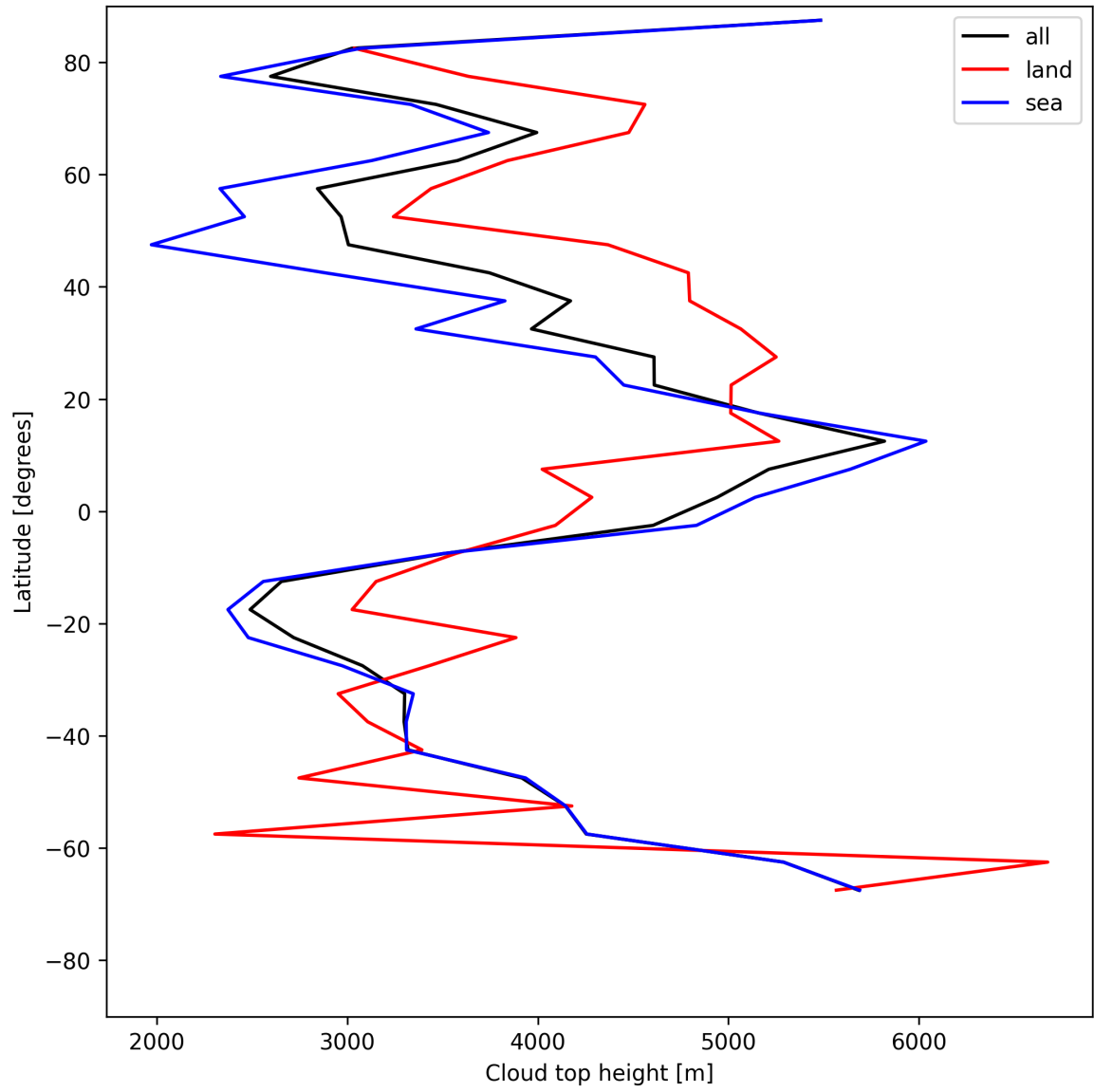
Figure 22: Zonal average of “Cloud top height” for 2025-07-26 to 2025-07-27.
