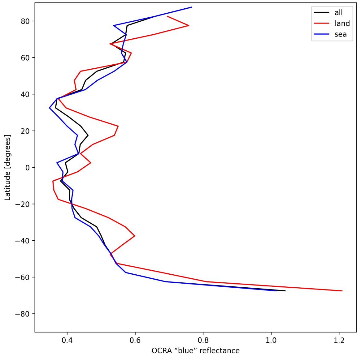
Figure 33: Zonal average of "OCRA "blue" reflectance" for 2025-07-26 to 2025-07-27.
