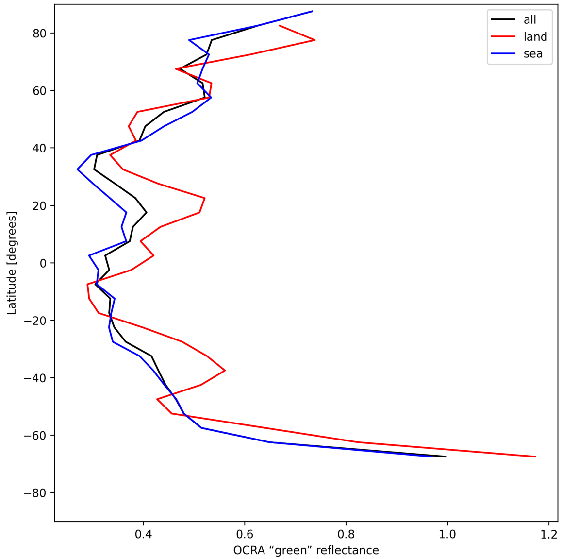
Figure 34: Zonal average of “OCRA “green” reflectance” for 2025-07-26 to 2025-07-27.
