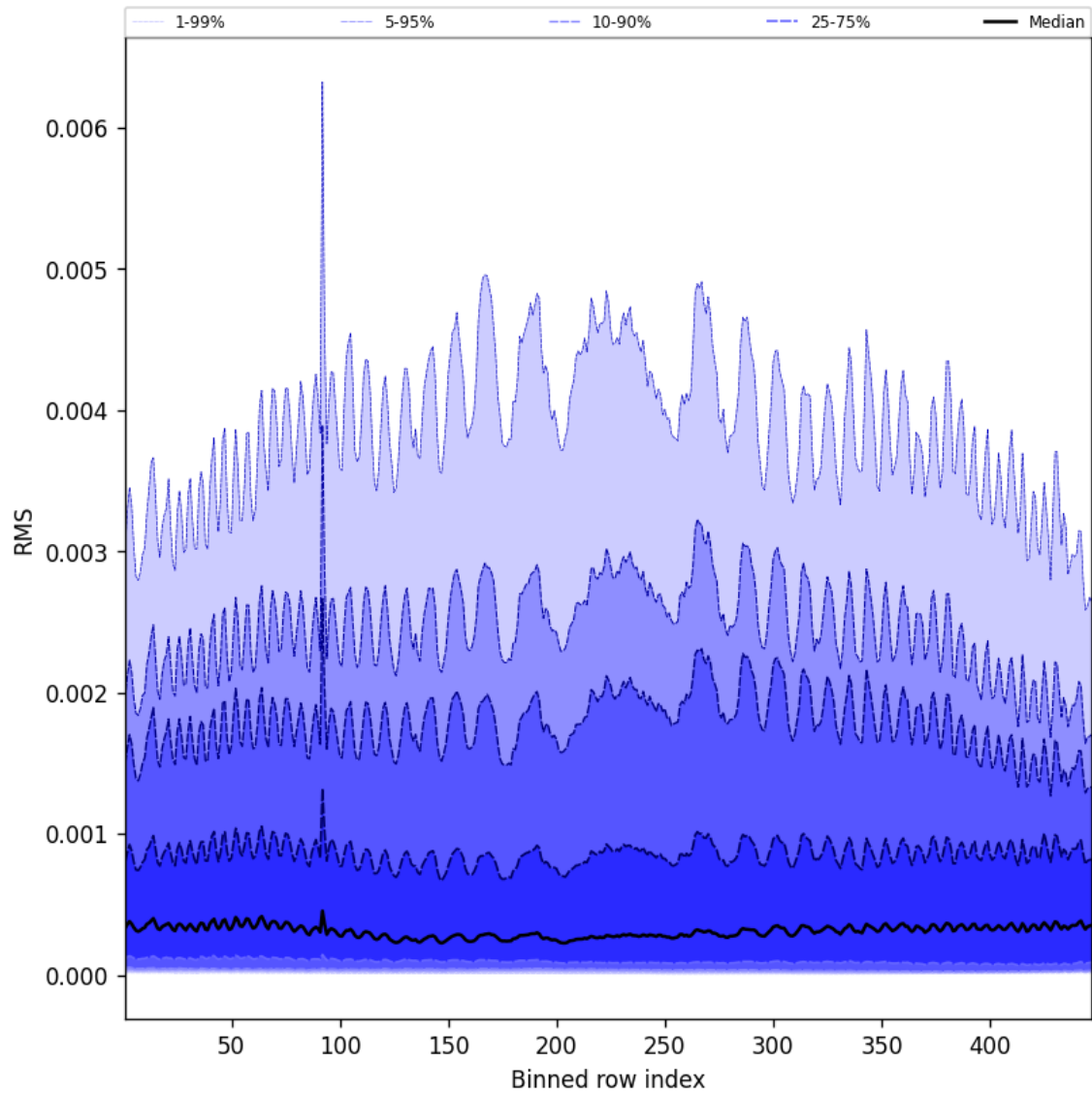
Figure 61: Along track statistics of “RMS” for 2025-07-26 to 2025-07-27
