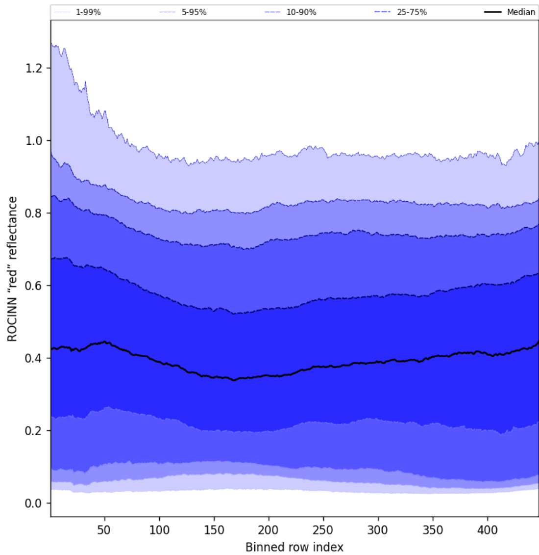
Figure 67: Along track statistics of “ROCINN “red” reflectance” for 2025-07-26 to 2025-07-27
