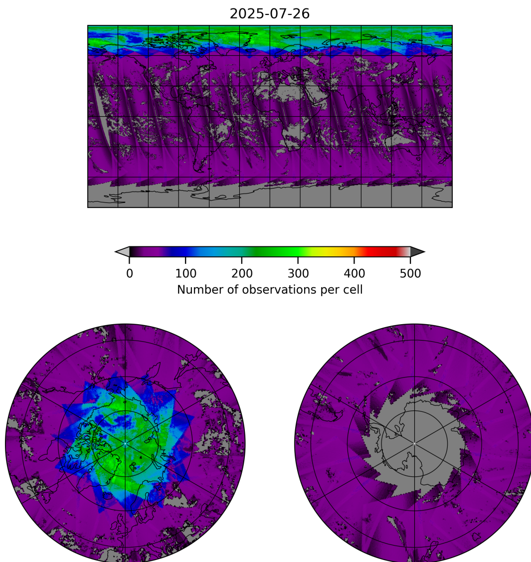
Figure 19: Map of the number of observations for 2025-07-26 to 2025-07-27
