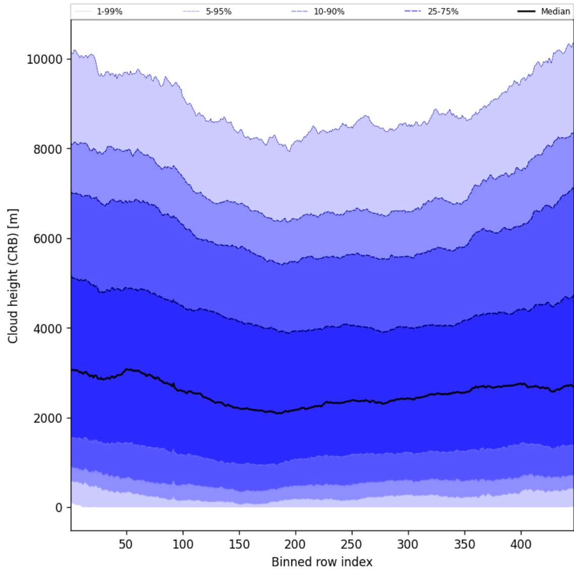
Figure 57: Along track statistics of “Cloud height (CRB)” for 2025-07-26 to 2025-07-27
