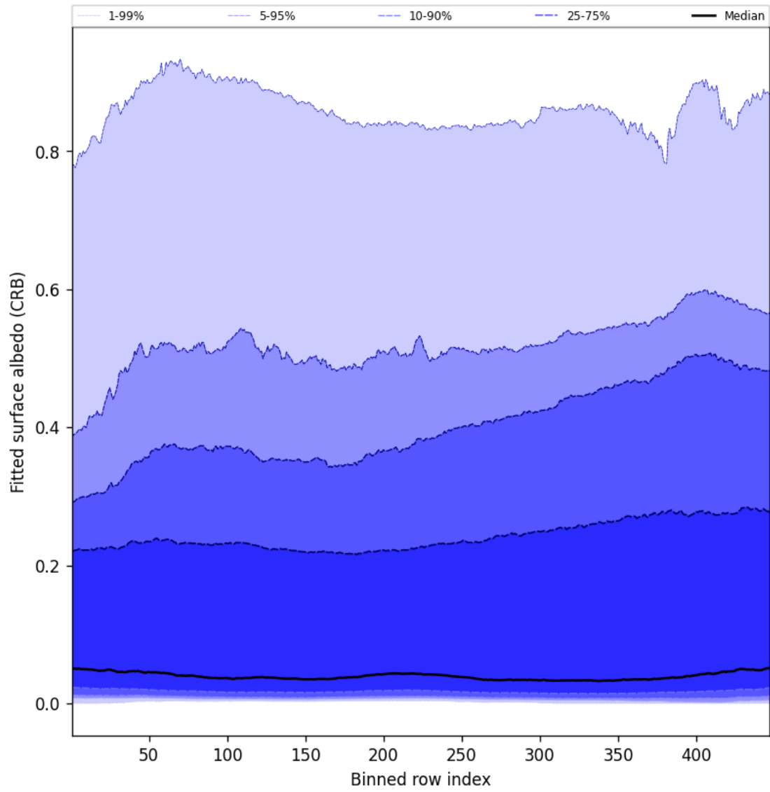
Figure 60: Along track statistics of “Fitted surface albedo (CRB)” for 2025-07-26 to 2025-07-27
