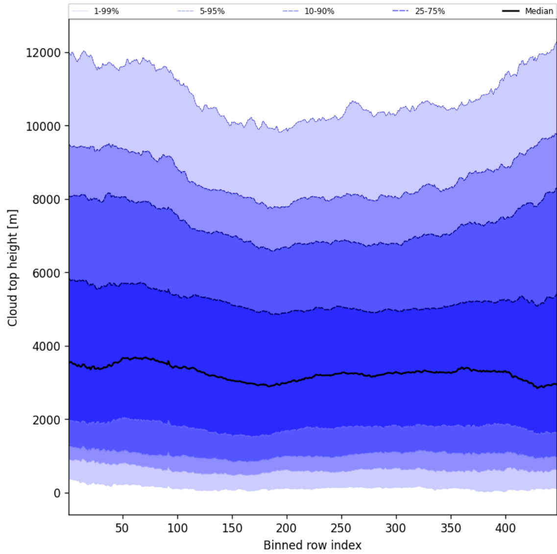
Figure 54: Along track statistics of “Cloud top height” for 2025-07-26 to 2025-07-27
