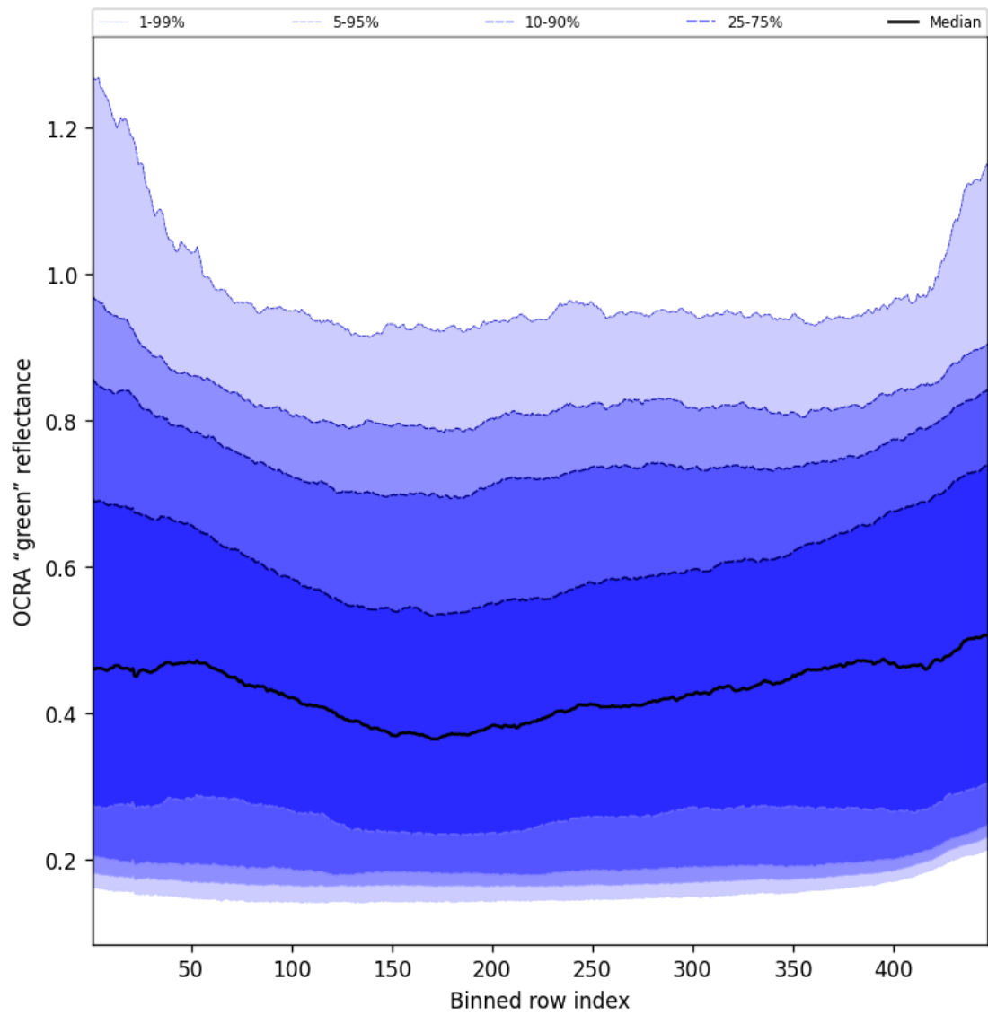
Figure 66: Along track statistics of “OCRA “green” reflectance” for 2025-07-26 to 2025-07-27
