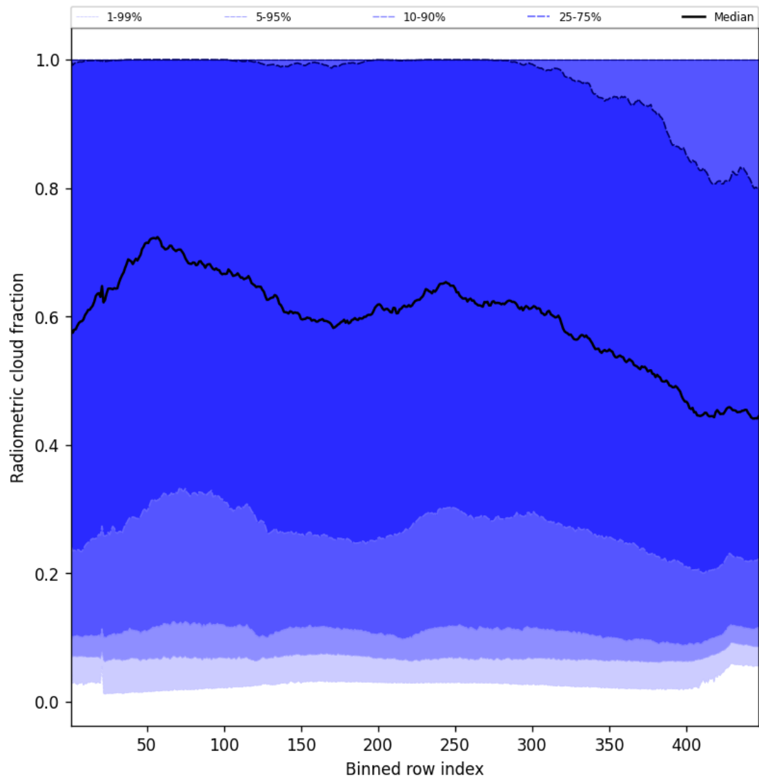
Figure 53: Along track statistics of “Radiometric cloud fraction” for 2025-07-26 to 2025-07-27
