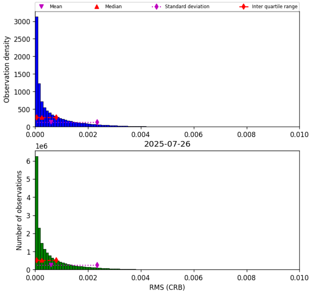
Figure 46: Histogram of “RMS (CRB)” for 2025-07-26 to 2025-07-27
