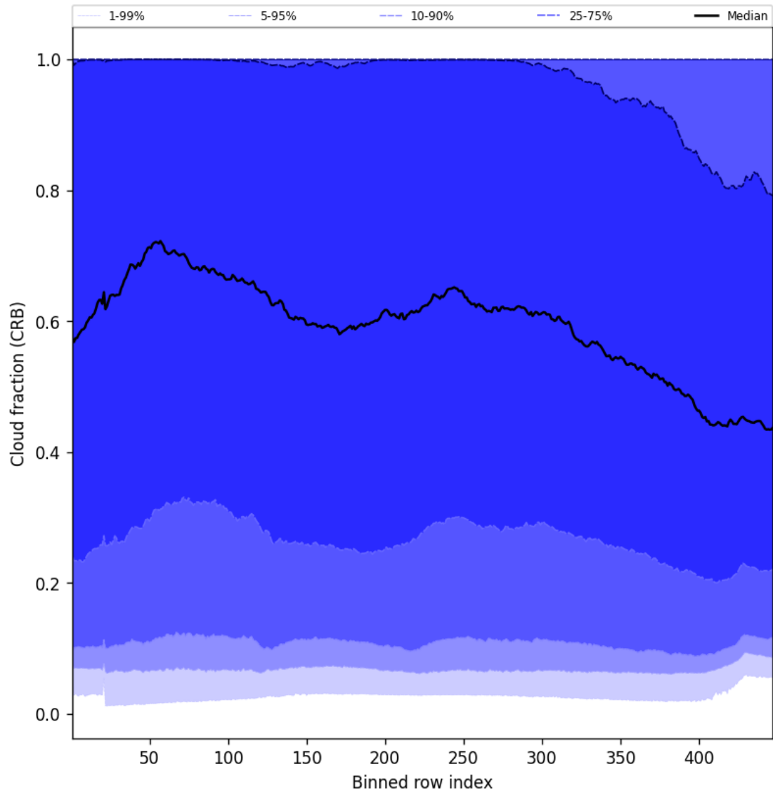
Figure 56: Along track statistics of “Cloud fraction (CRB)” for 2025-07-26 to 2025-07-27
