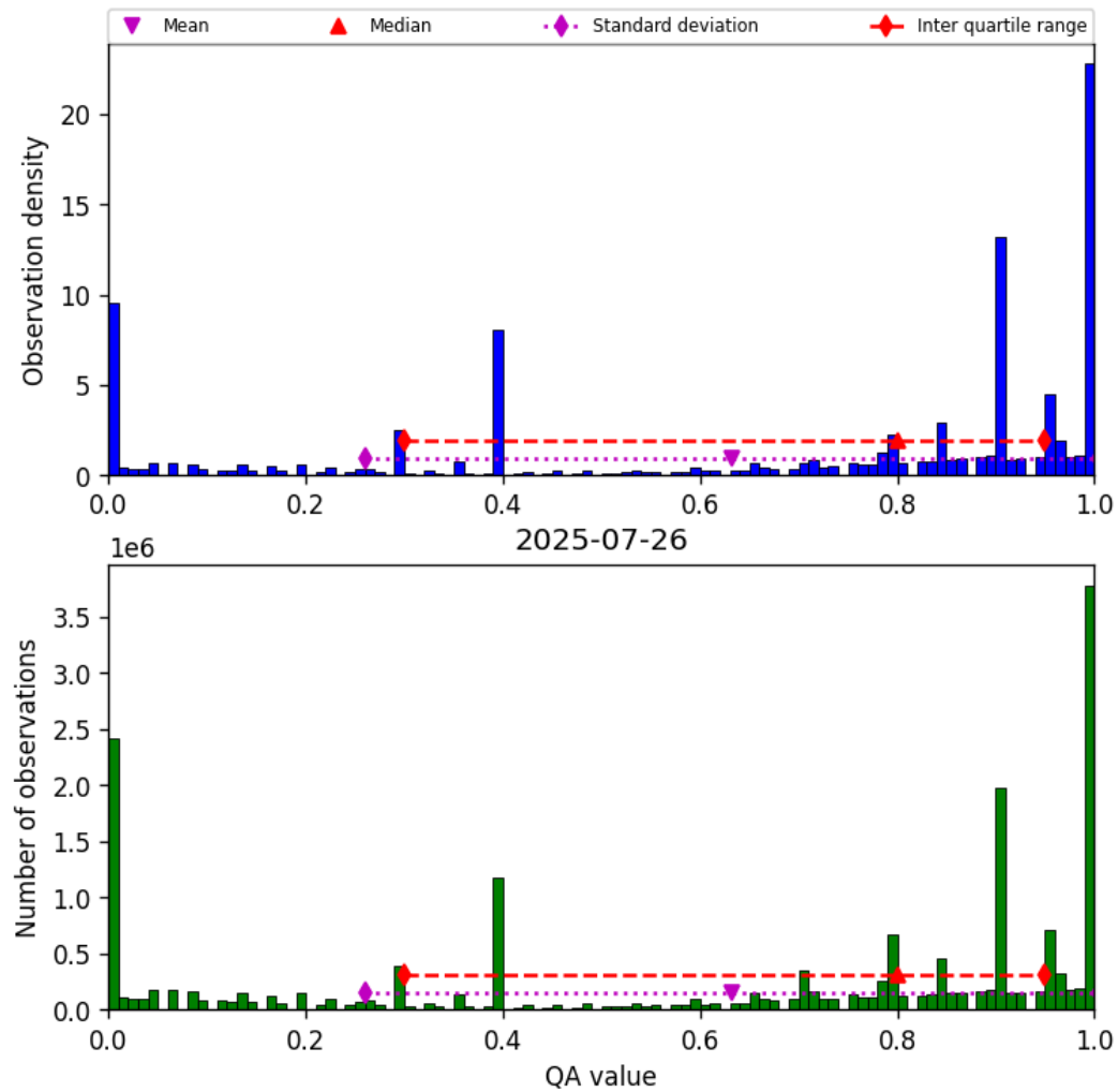
Figure 36: Histogram of “QA value” for 2025-07-26 to 2025-07-27
