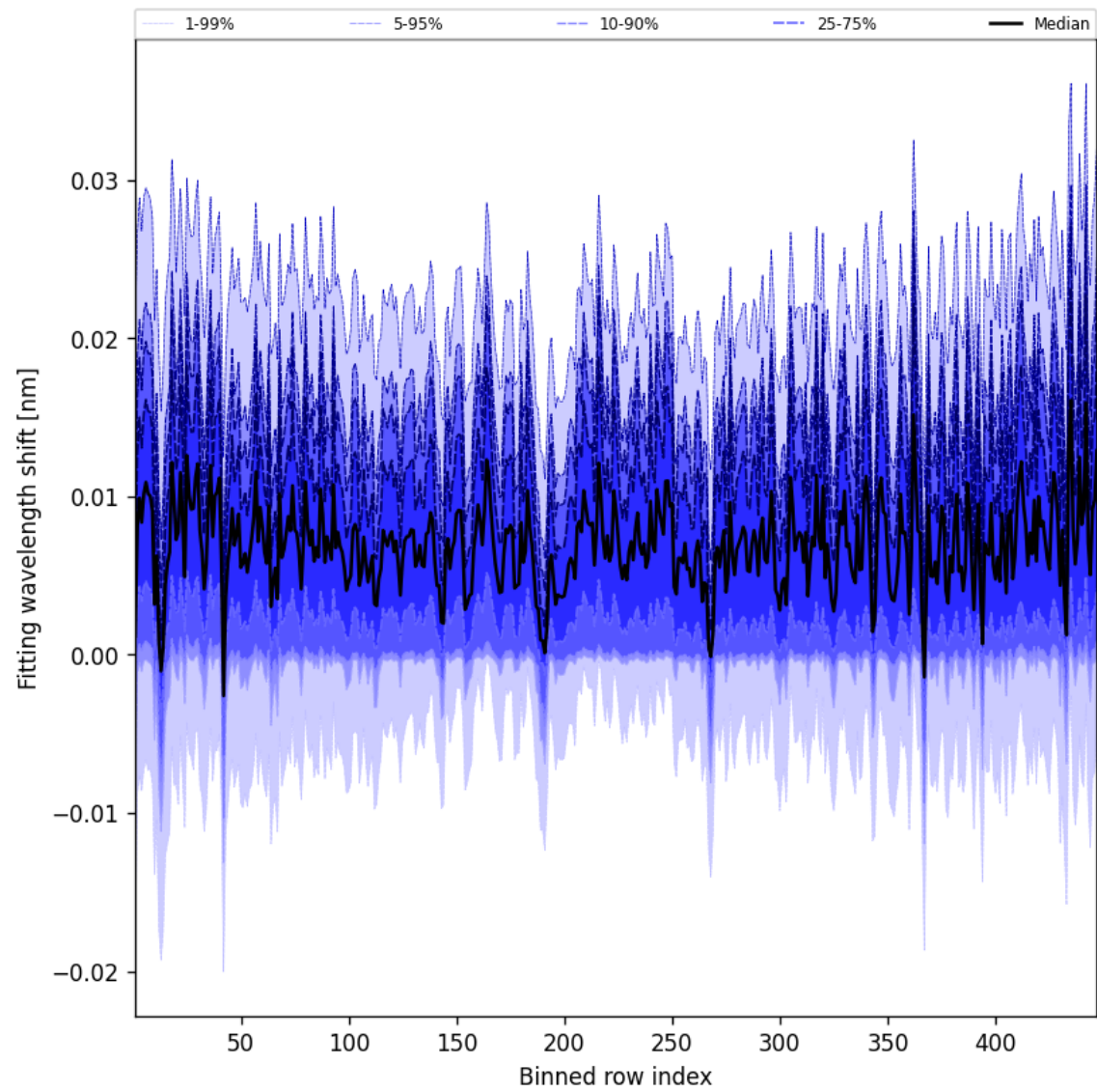
Figure 63: Along track statistics of “Fitting wavelength shift” for 2025-07-26 to 2025-07-27
