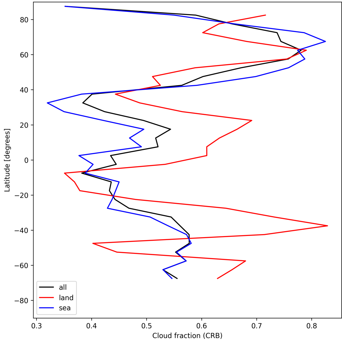
Figure 24: Zonal average of “Cloud fraction (CRB)” for 2025-07-26 to 2025-07-27.
