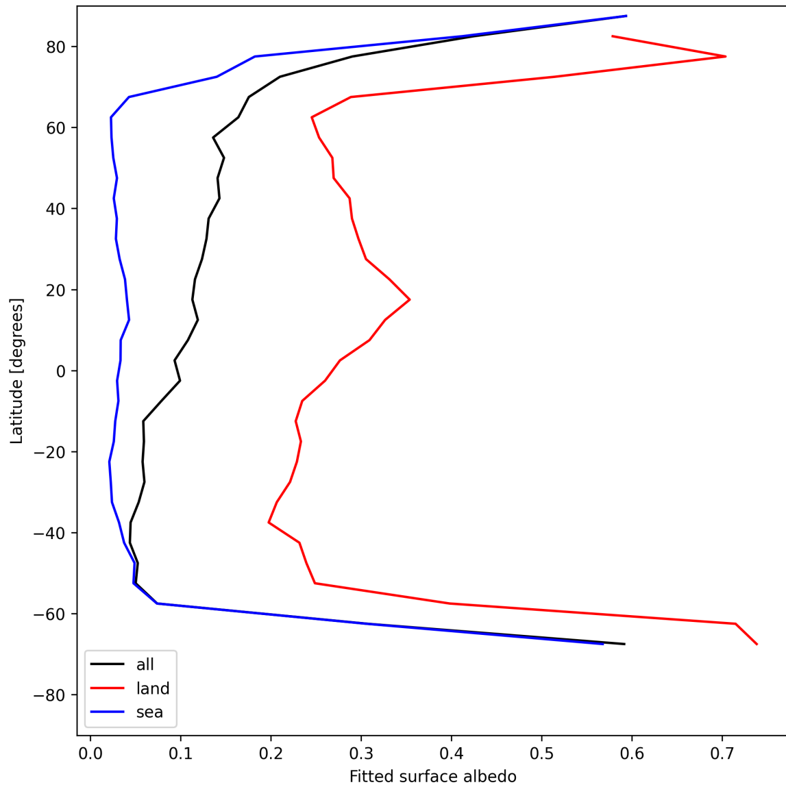
Figure 27: Zonal average of “Fitted surface albedo” for 2025-07-26 to 2025-07-27.
