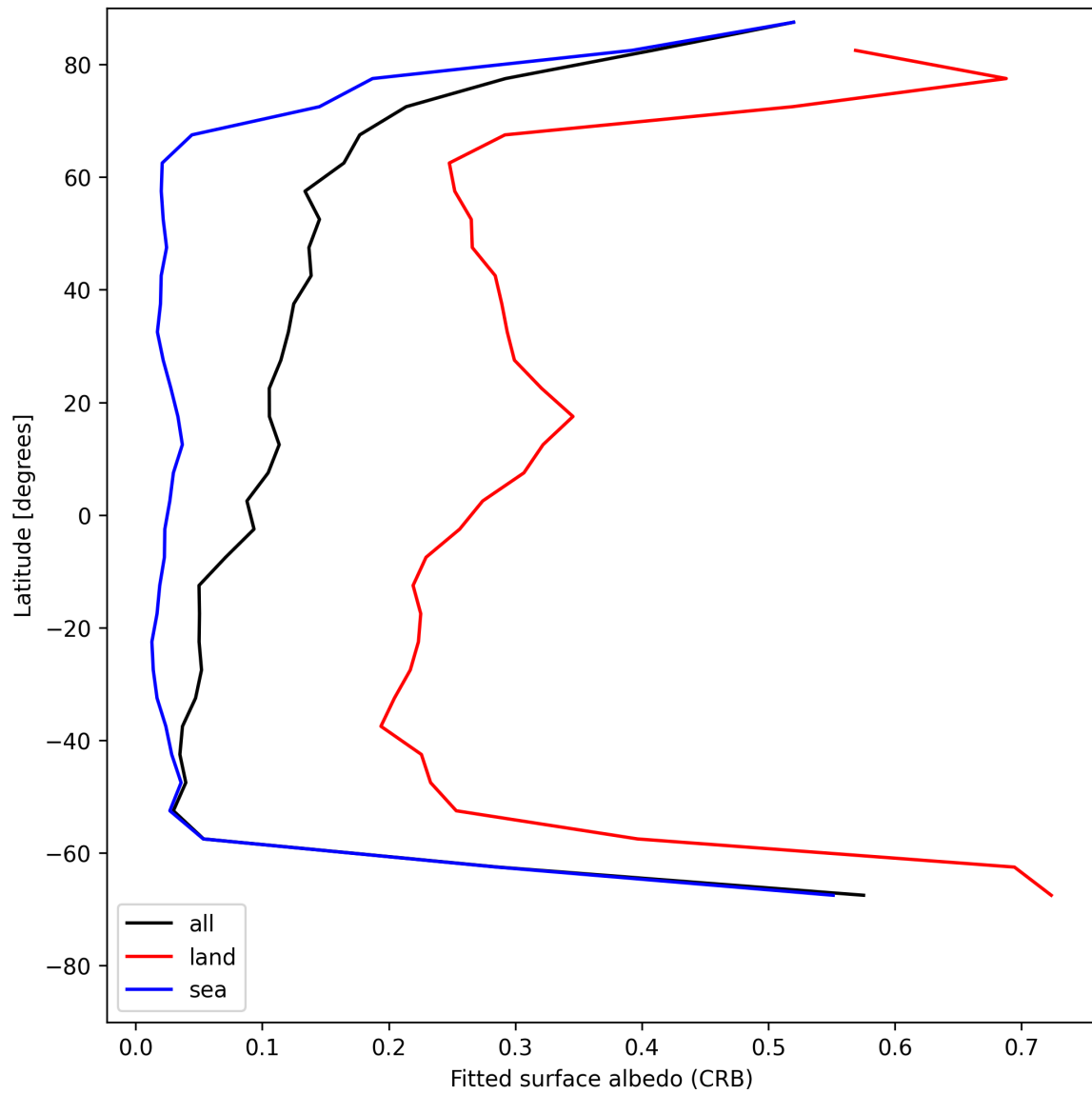
Figure 28: Zonal average of “Fitted surface albedo (CRB)” for 2025-07-26 to 2025-07-27.
