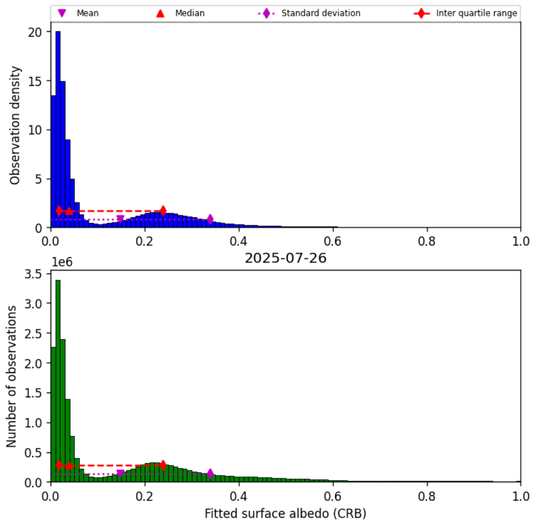
Figure 44: Histogram of “Fitted surface albedo (CRB)” for 2025-07-26 to 2025-07-27
