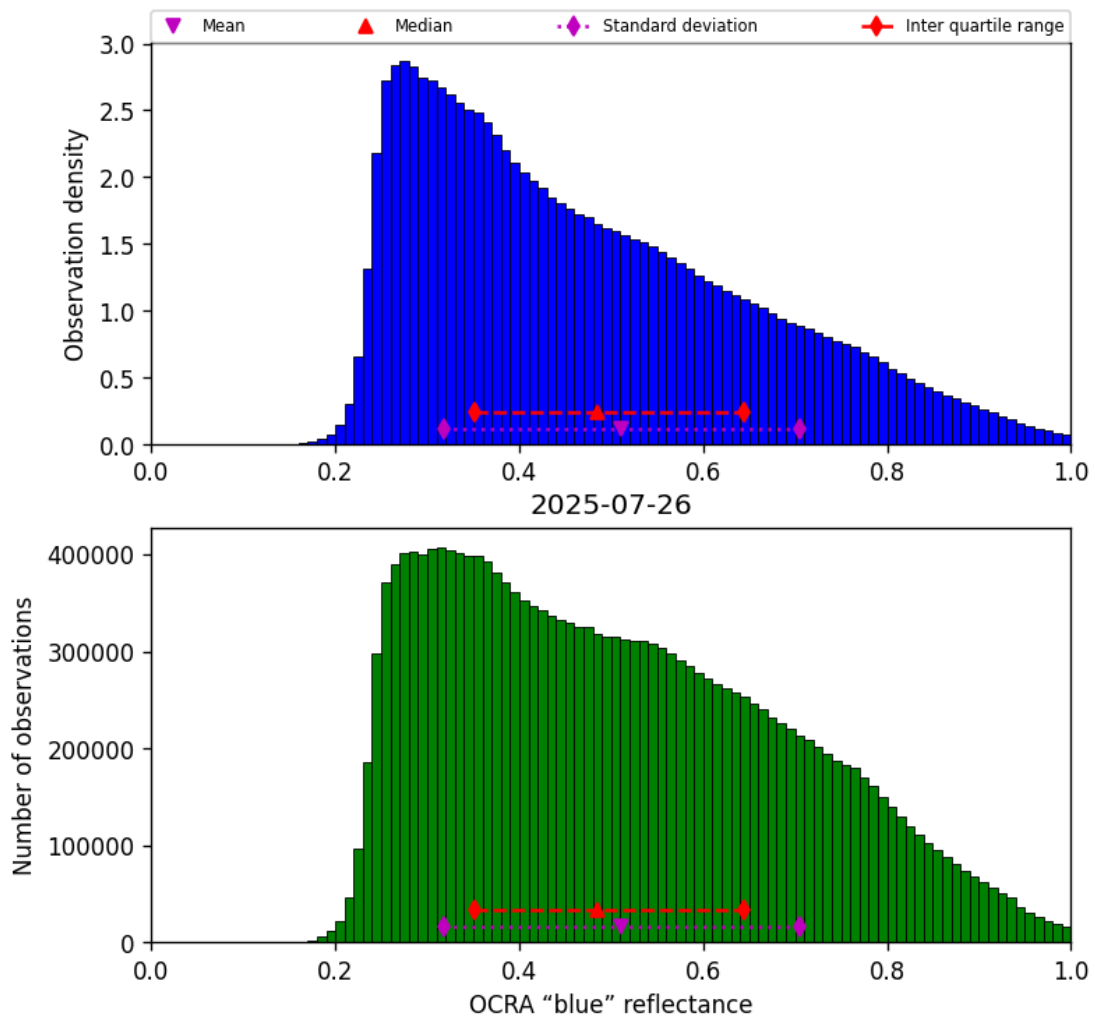
Figure 49: Histogram of “OCRA “blue” reflectance” for 2025-07-26 to 2025-07-27
