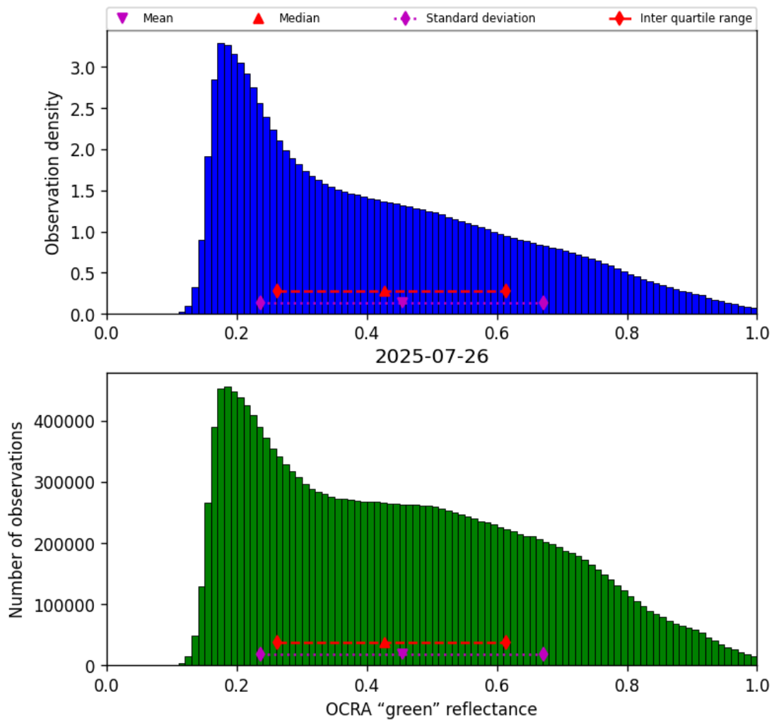
Figure 50: Histogram of “OCRA “green” reflectance” for 2025-07-26 to 2025-07-27
