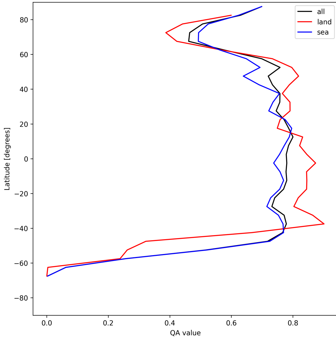
Figure 20: Zonal average of “QA value” for 2025-07-26 to 2025-07-27.
