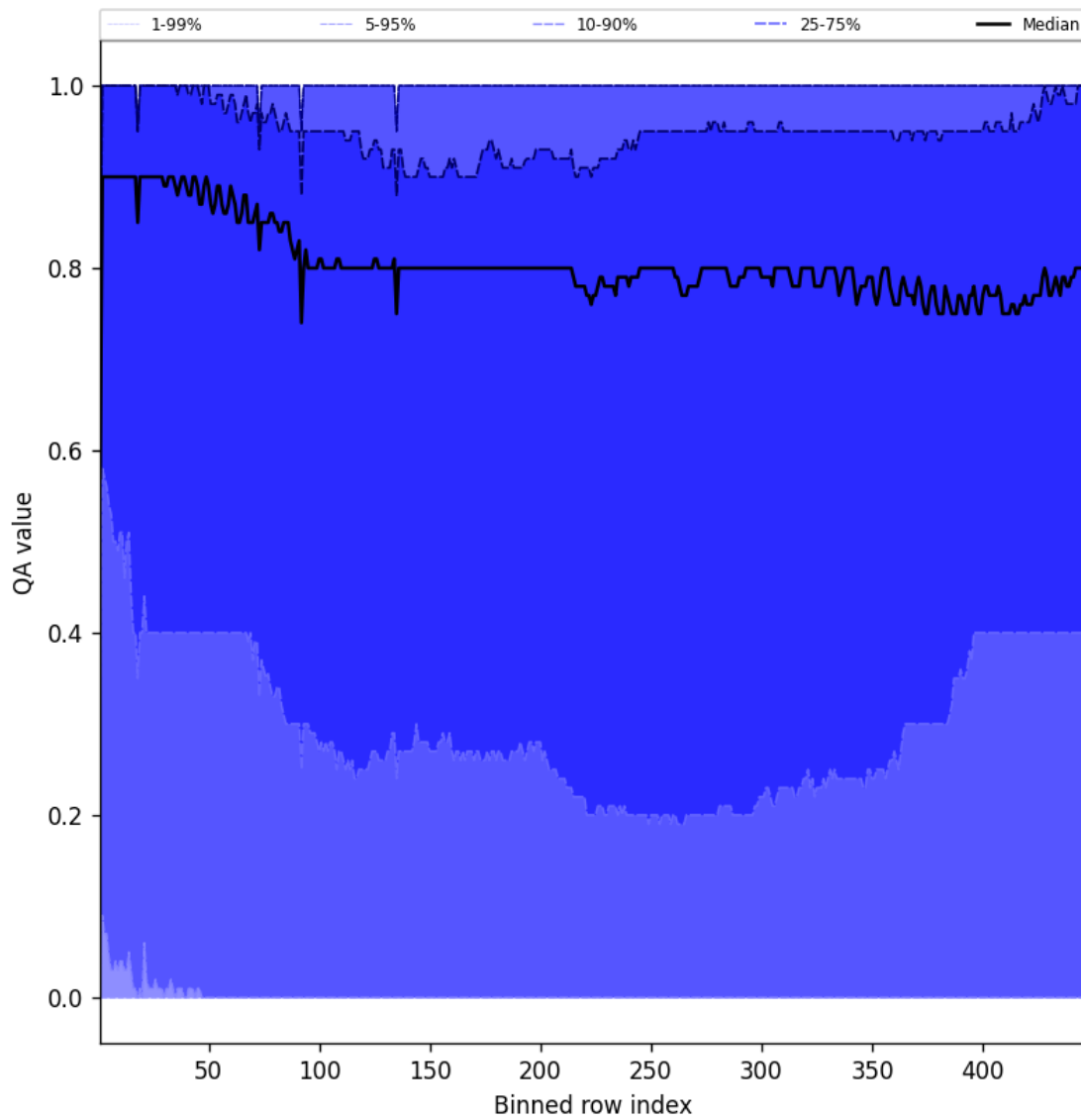
Figure 52: Along track statistics of “QA value” for 2025-07-26 to 2025-07-27
