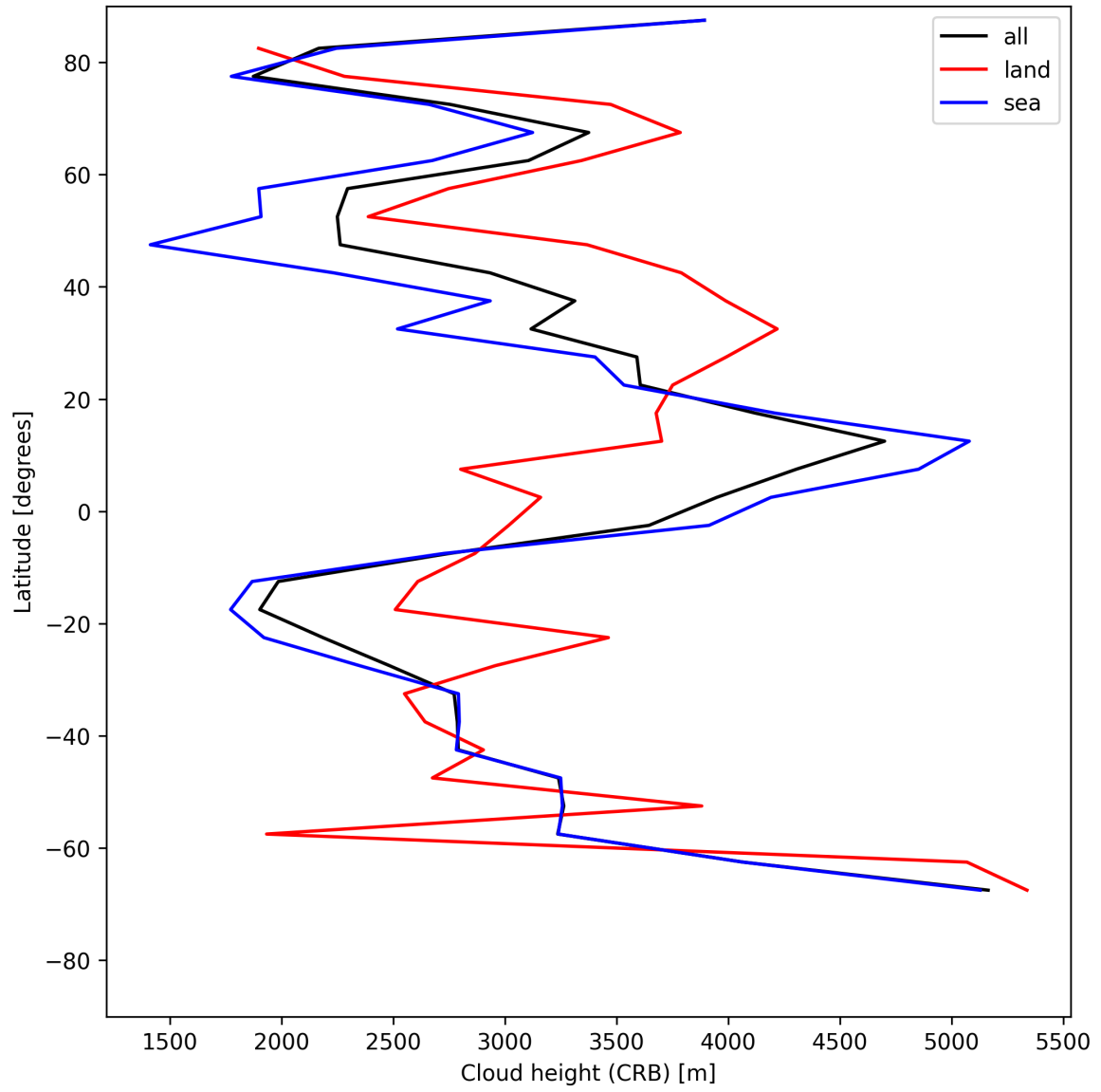
Figure 25: Zonal average of “Cloud height (CRB)” for 2025-07-26 to 2025-07-27.
