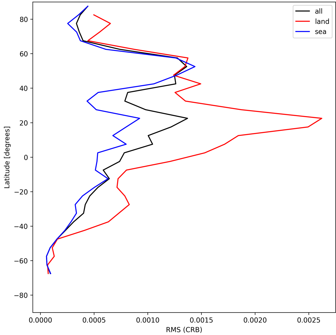
Figure 30: Zonal average of “RMS (CRB)” for 2025-07-26 to 2025-07-27.
