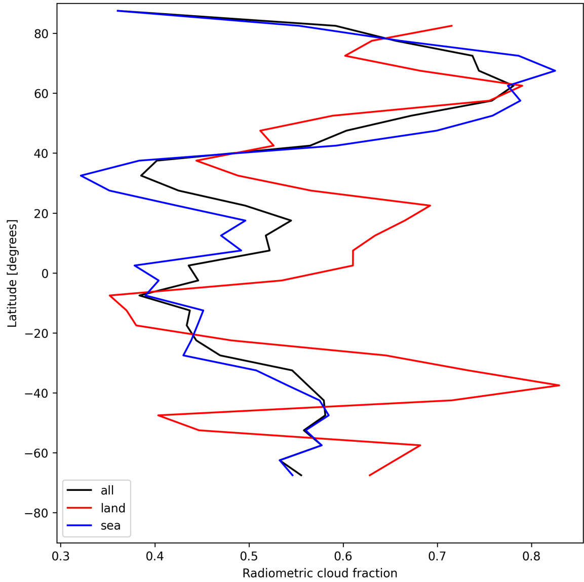
Figure 21: Zonal average of “Radiometric cloud fraction” for 2025-07-26 to 2025-07-27.
