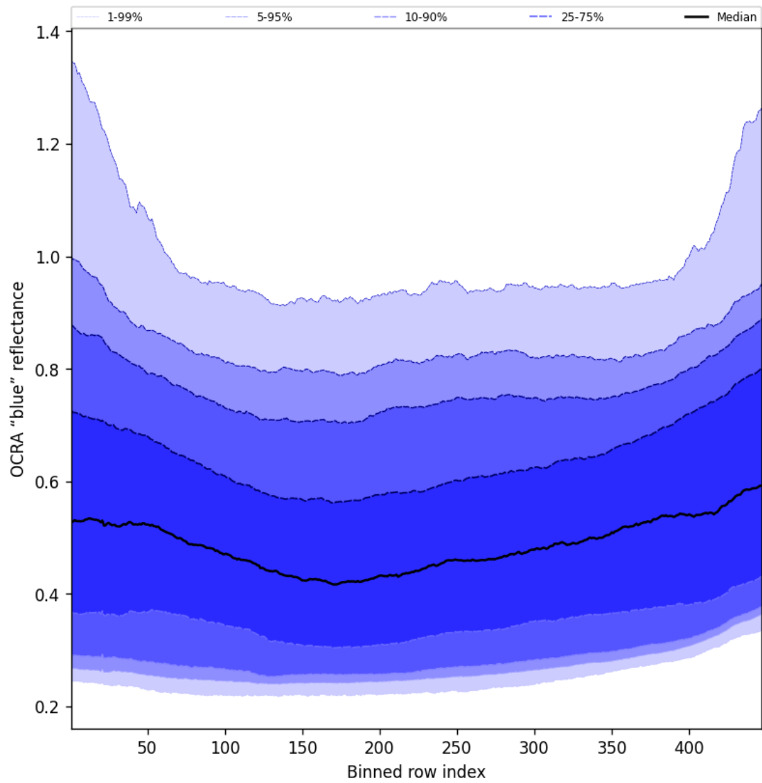
Figure 65: Along track statistics of “OCRA “blue” reflectance” for 2025-07-26 to 2025-07-27
