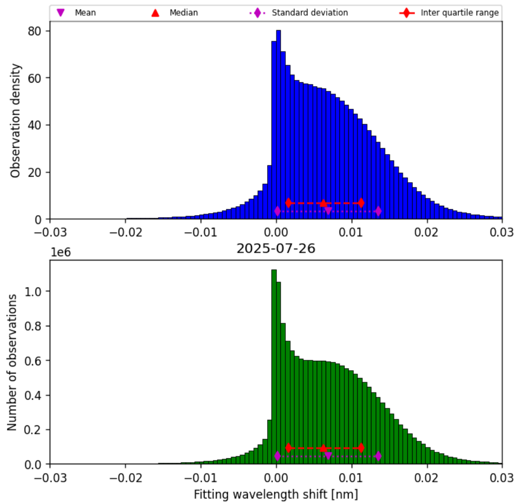
Figure 47: Histogram of “Fitting wavelength shift” for 2025-07-26 to 2025-07-27
