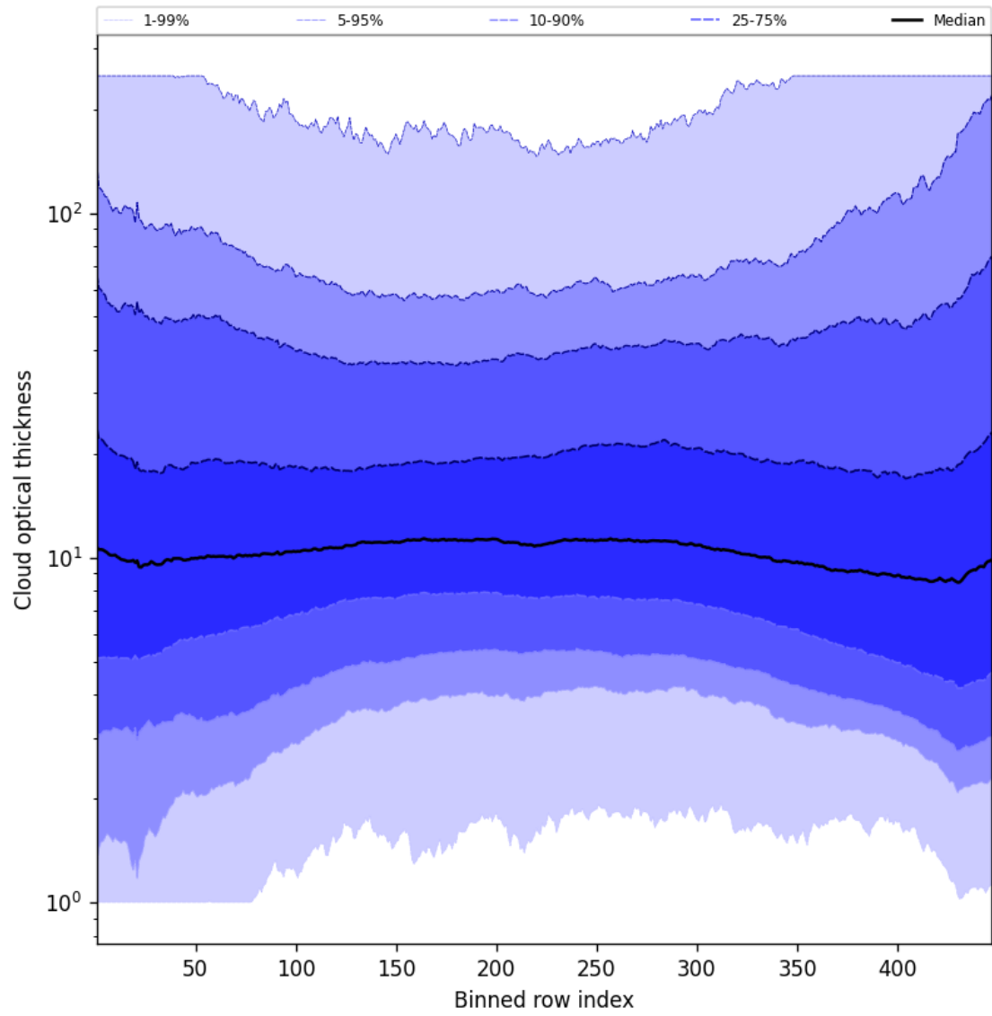
Figure 55: Along track statistics of “Cloud optical thickness” for 2025-07-26 to 2025-07-27
