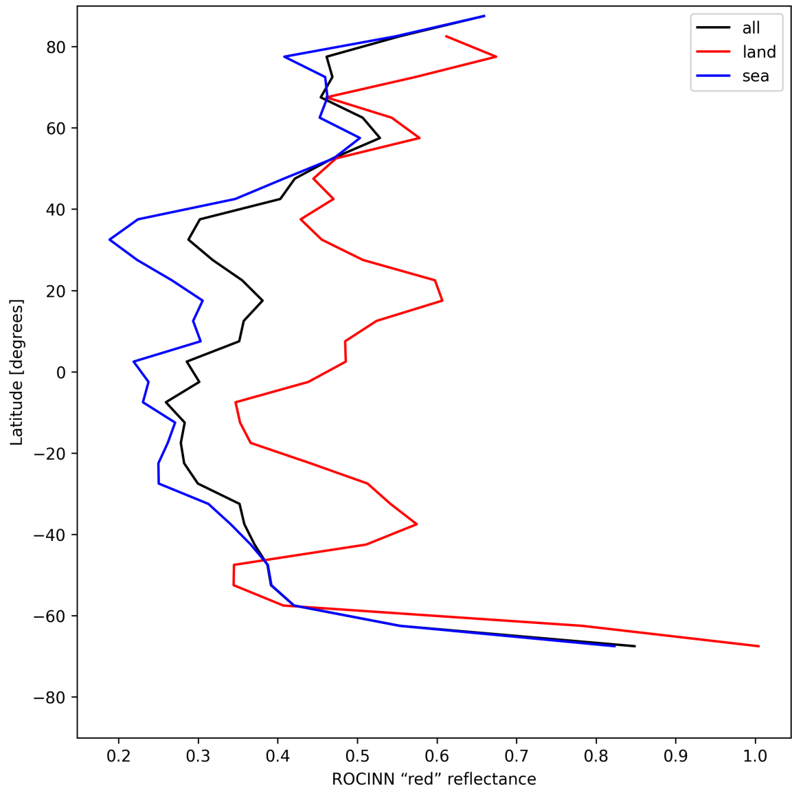
Figure 35: Zonal average of “ROCINN “red” reflectance” for 2025-07-26 to 2025-07-27.
