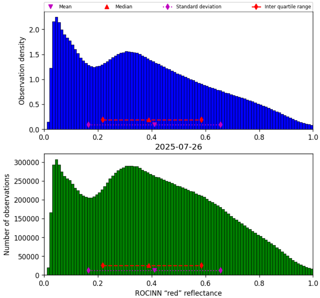
Figure 51: Histogram of "ROCINN "red" reflectance" for 2025-07-26 to 2025-07-27
