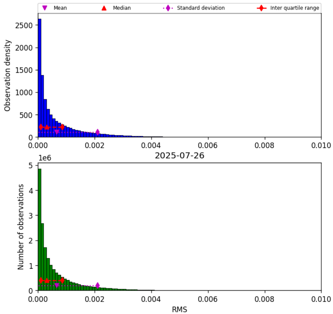
Figure 45: Histogram of “RMS” for 2025-07-26 to 2025-07-27
