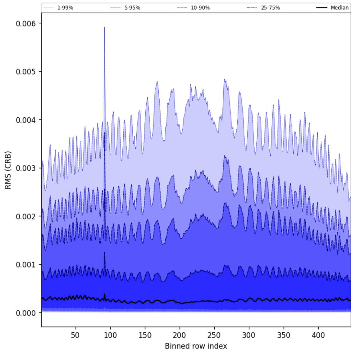
Figure 62: Along track statistics of “RMS (CRB)” for 2025-07-26 to 2025-07-27
