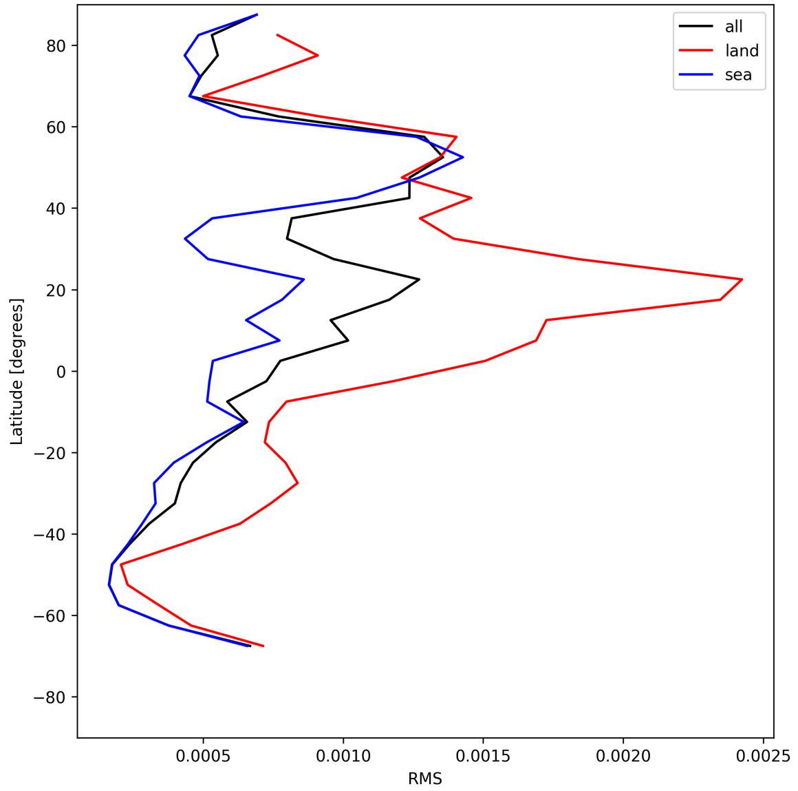
Figure 29: Zonal average of “RMS” for 2025-07-26 to 2025-07-27.
