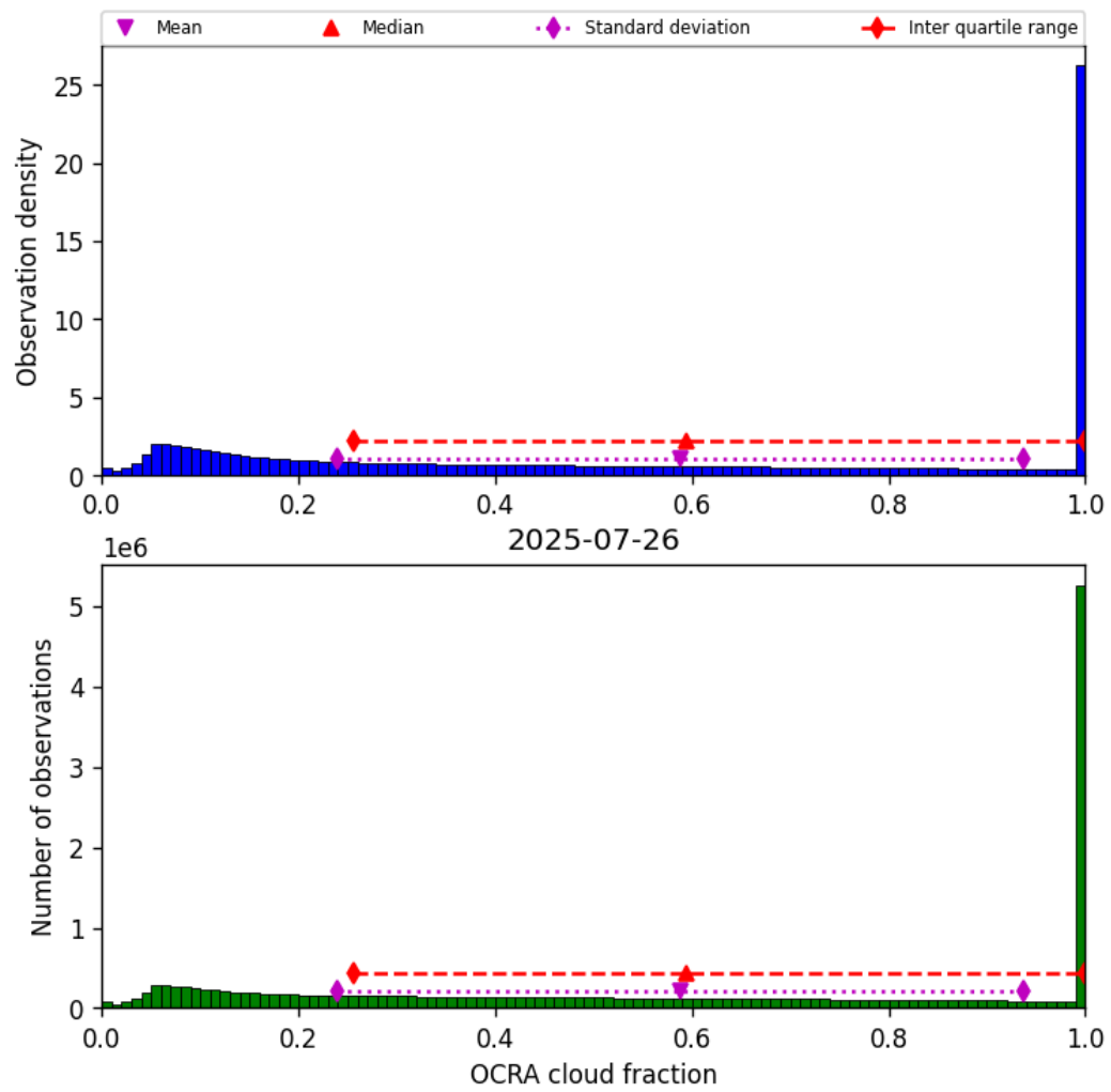
Figure 48: Histogram of “OCRA cloud fraction” for 2025-07-26 to 2025-07-27
