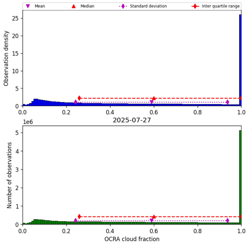
Figure 48: Histogram of “OCRA cloud fraction” for 2025-07-27 to 2025-07-27
