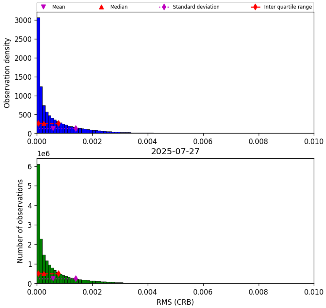
Figure 46: Histogram of “RMS (CRB)” for 2025-07-27 to 2025-07-27
