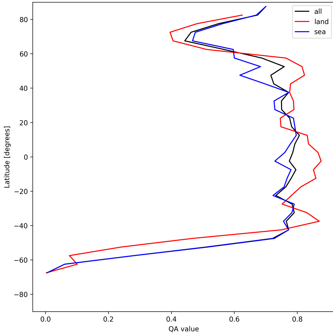
Figure 20: Zonal average of “QA value” for 2025-07-27 to 2025-07-27.
