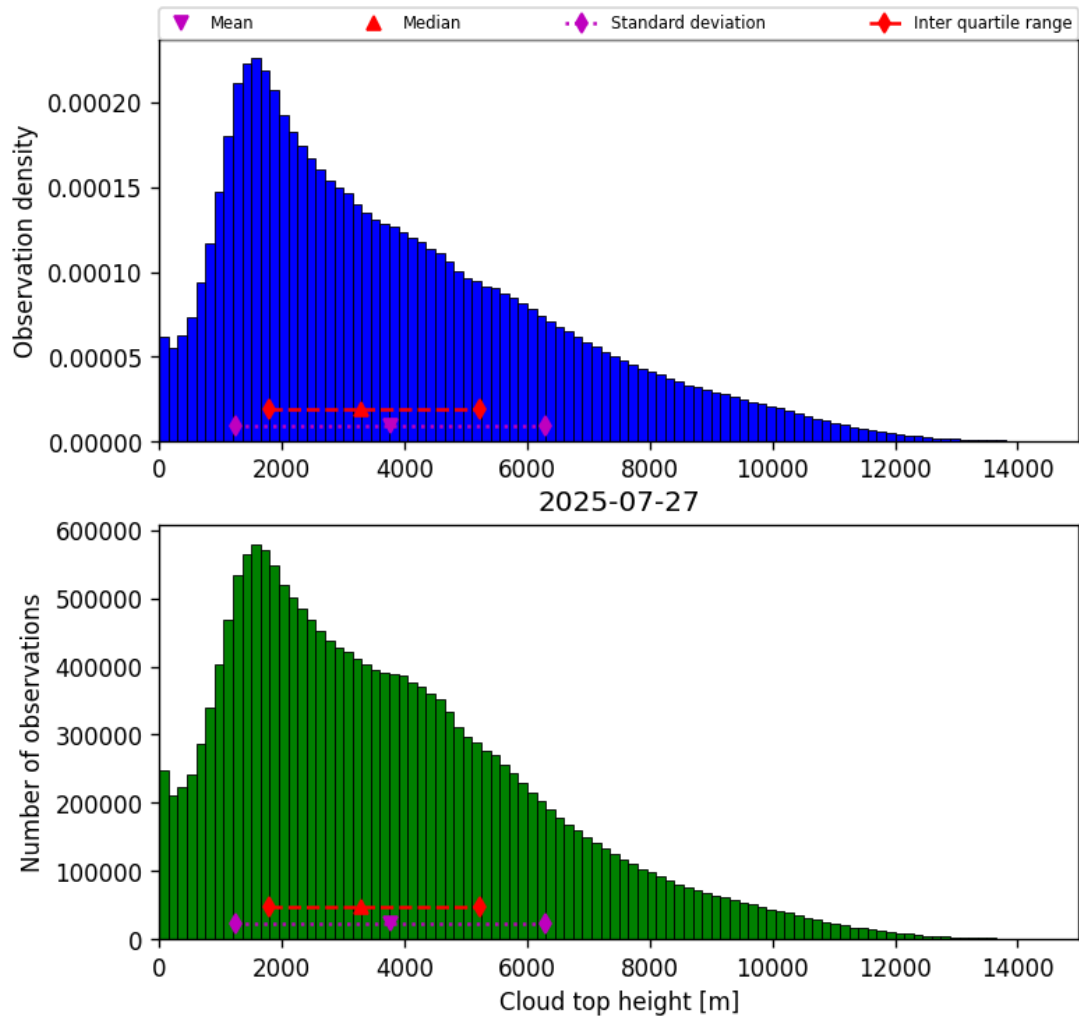
Figure 38: Histogram of “Cloud top height” for 2025-07-27 to 2025-07-27
