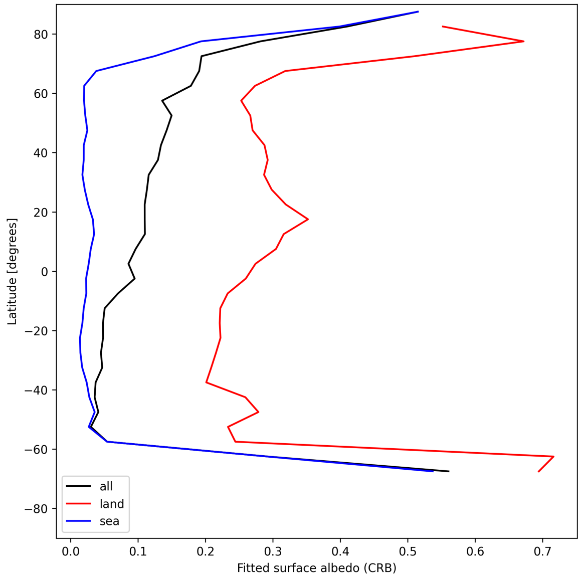
Figure 28: Zonal average of “Fitted surface albedo (CRB)” for 2025-07-27 to 2025-07-27.
