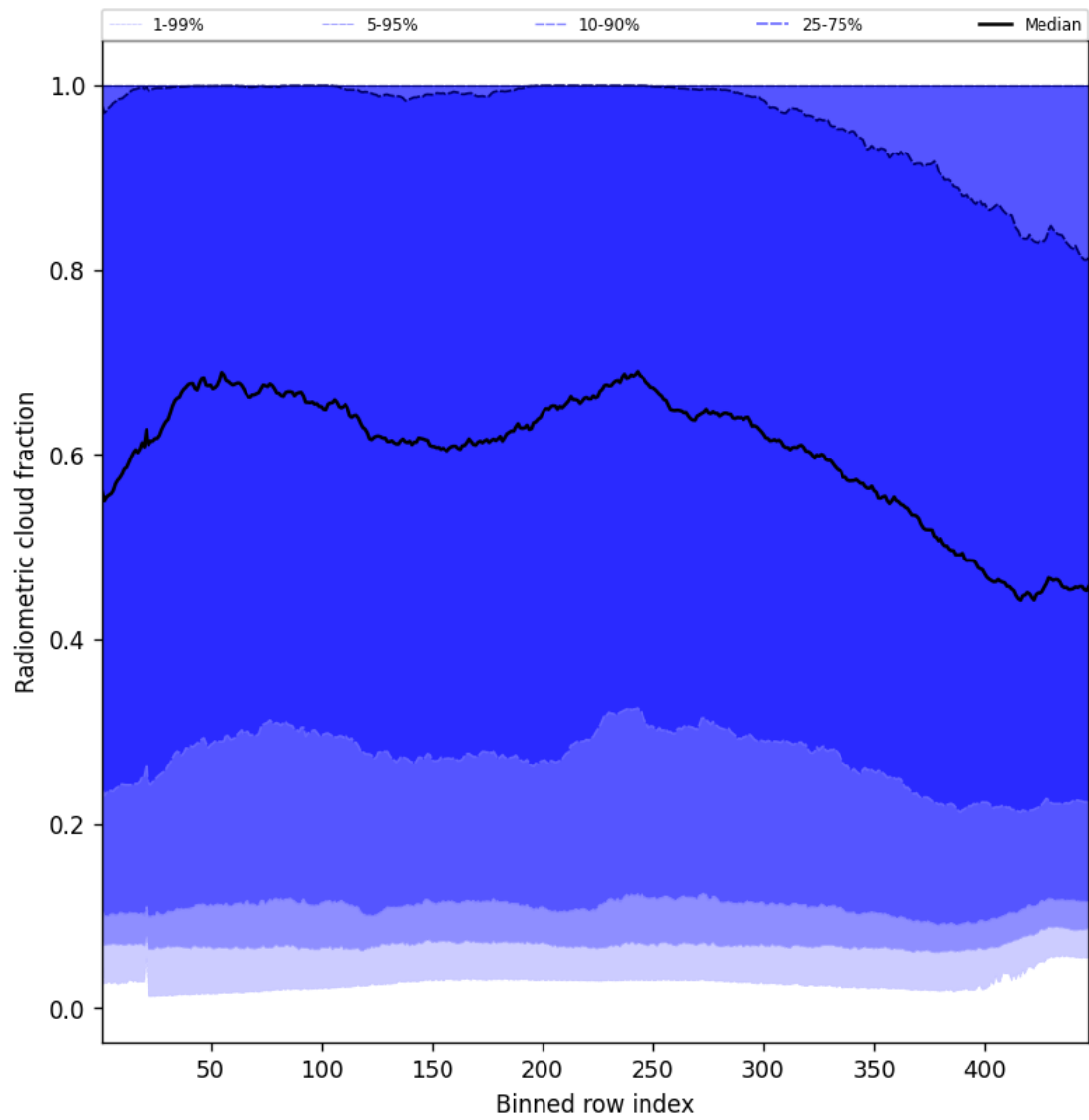
Figure 53: Along track statistics of “Radiometric cloud fraction” for 2025-07-27 to 2025-07-27
