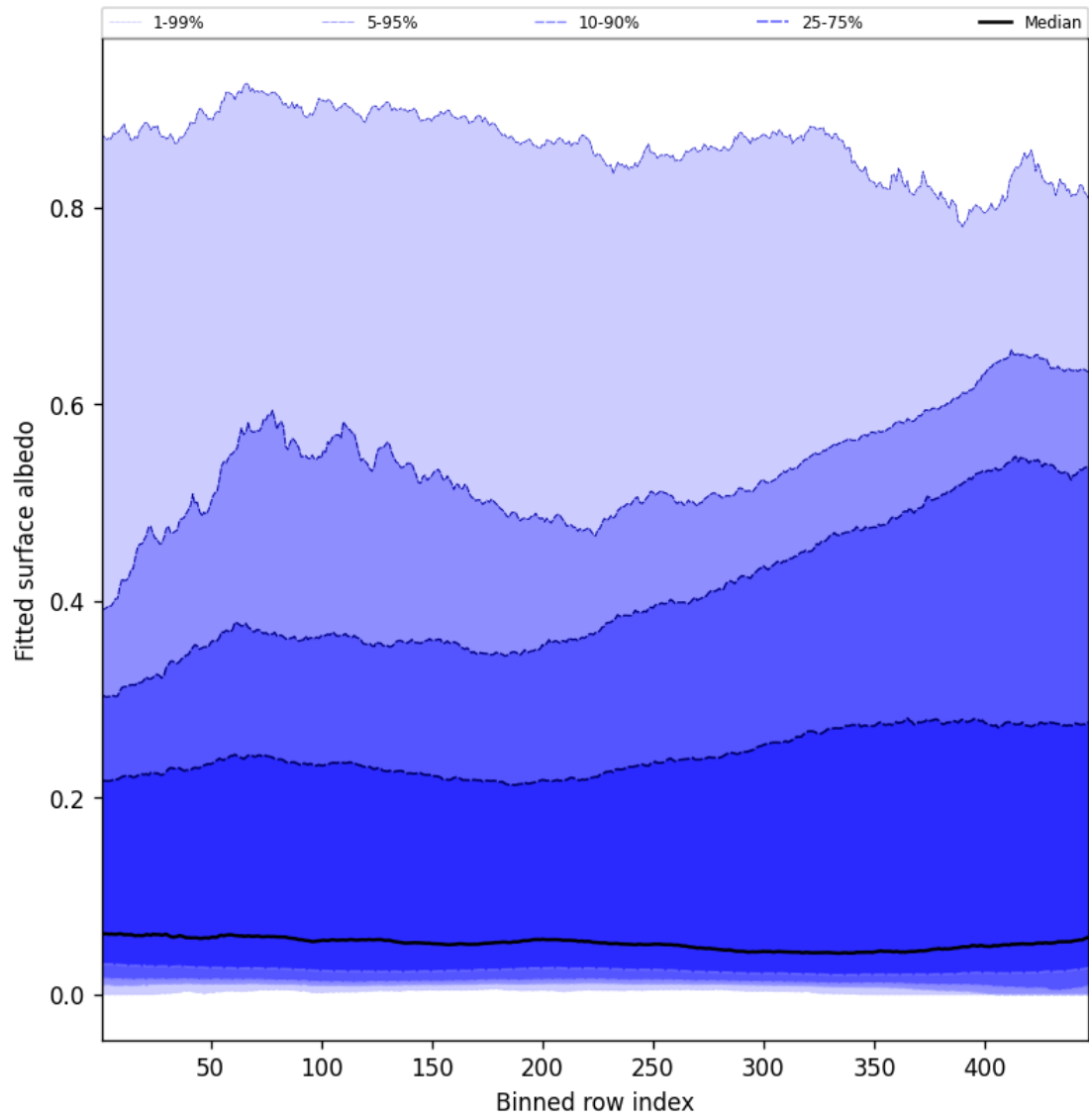
Figure 59: Along track statistics of “Fitted surface albedo” for 2025-07-27 to 2025-07-27
