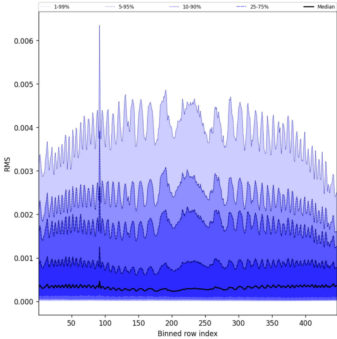
Figure 61: Along track statistics of “RMS” for 2025-07-27 to 2025-07-27
