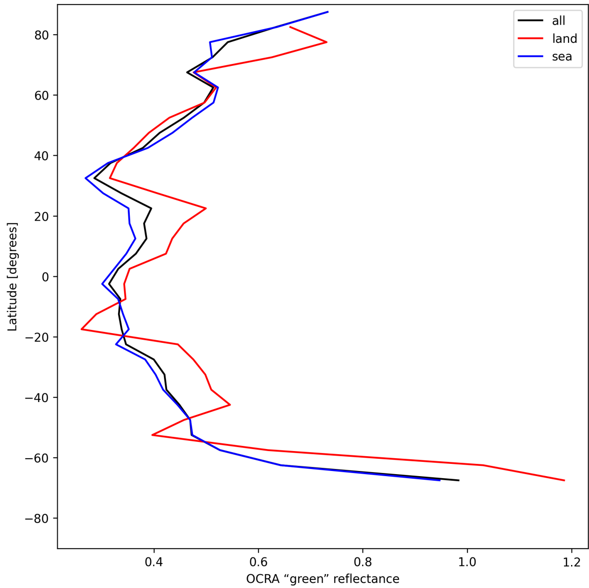
Figure 34: Zonal average of “OCRA “green” reflectance” for 2025-07-27 to 2025-07-27.
