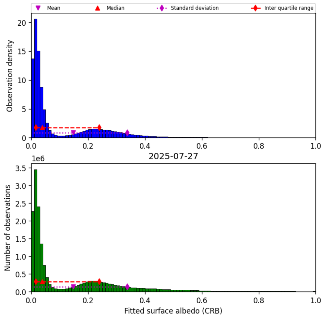
Figure 44: Histogram of “Fitted surface albedo (CRB)” for 2025-07-27 to 2025-07-27
