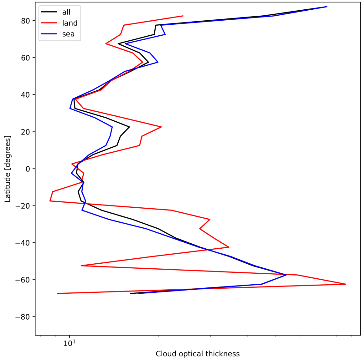
Figure 23: Zonal average of “Cloud optical thickness” for 2025-07-27 to 2025-07-27.
