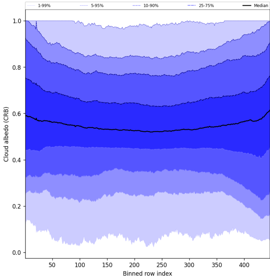
Figure 58: Along track statistics of “Cloud albedo (CRB)” for 2025-07-27 to 2025-07-27
