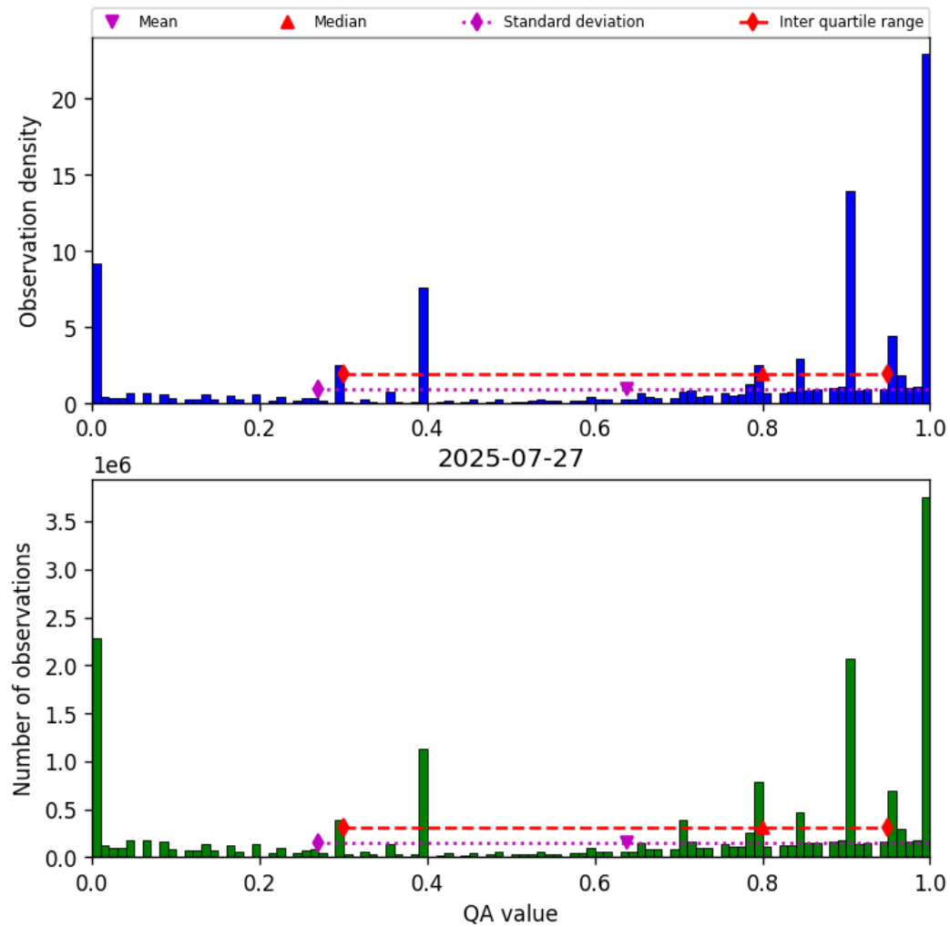
Figure 36: Histogram of “QA value” for 2025-07-27 to 2025-07-27
