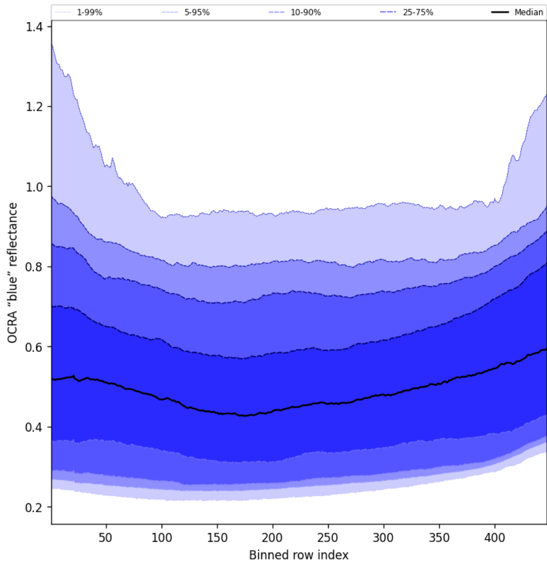
Figure 65: Along track statistics of “OCRA “blue” reflectance” for 2025-07-27 to 2025-07-27
