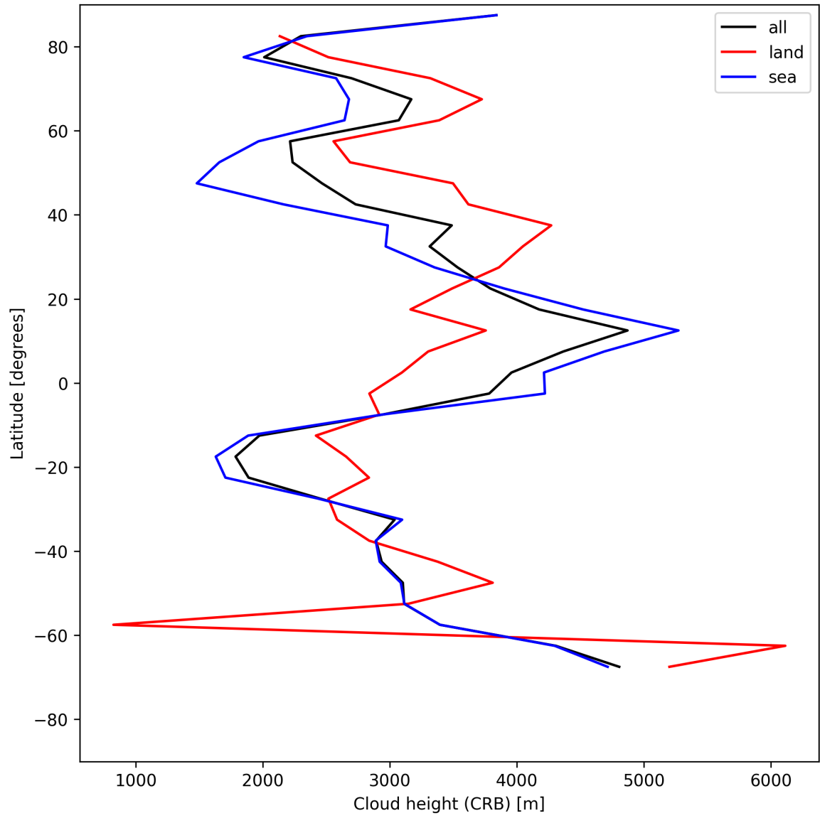
Figure 25: Zonal average of “Cloud height (CRB)” for 2025-07-27 to 2025-07-27.
