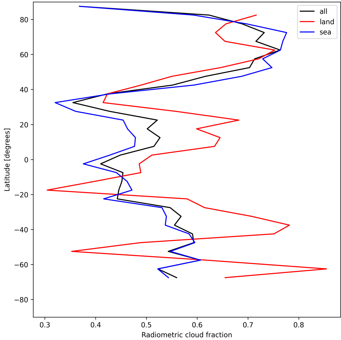
Figure 21: Zonal average of “Radiometric cloud fraction” for 2025-07-27 to 2025-07-27.
