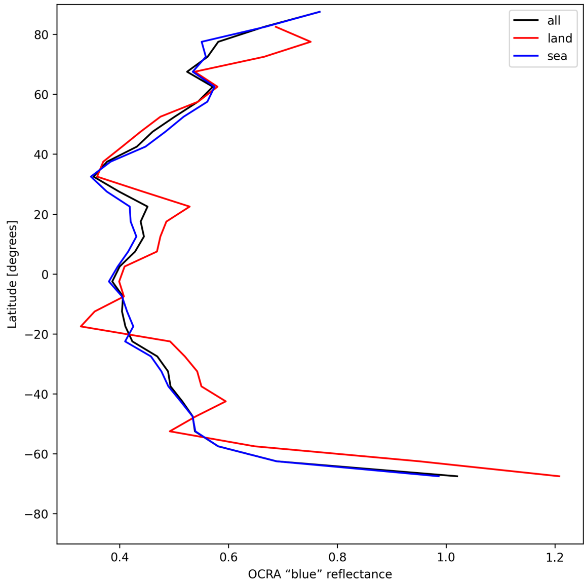
Figure 33: Zonal average of “OCRA “blue” reflectance” for 2025-07-27 to 2025-07-27.
