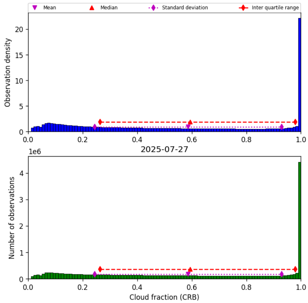
Figure 40: Histogram of “Cloud fraction (CRB)” for 2025-07-27 to 2025-07-27
