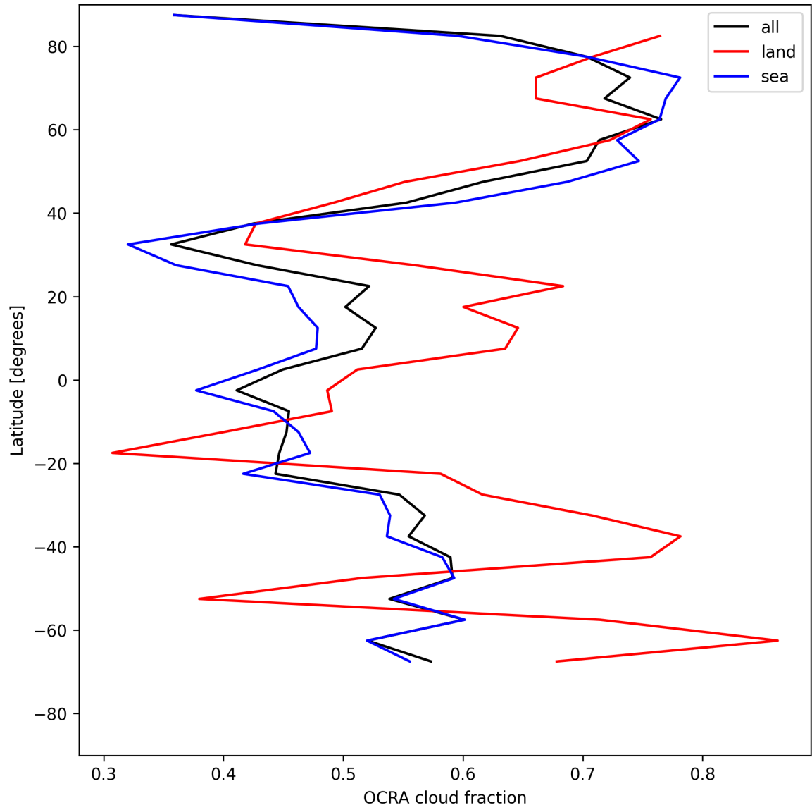
Figure 32: Zonal average of “OCRA cloud fraction” for 2025-07-27 to 2025-07-27.
