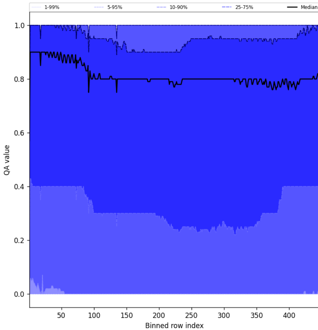
Figure 52: Along track statistics of “QA value” for 2025-07-27 to 2025-07-27
