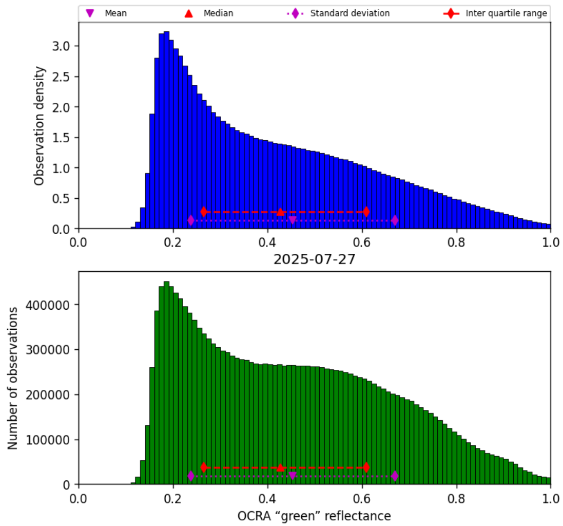
Figure 50: Histogram of “OCRA “green” reflectance” for 2025-07-27 to 2025-07-27
