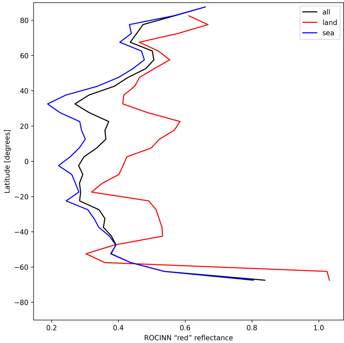
Figure 35: Zonal average of “ROCINN “red” reflectance” for 2025-07-27 to 2025-07-27.
