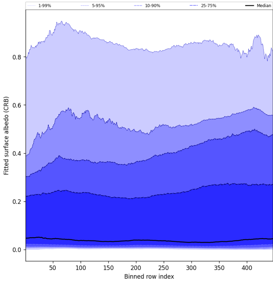
Figure 60: Along track statistics of “Fitted surface albedo (CRB)” for 2025-07-27 to 2025-07-27
