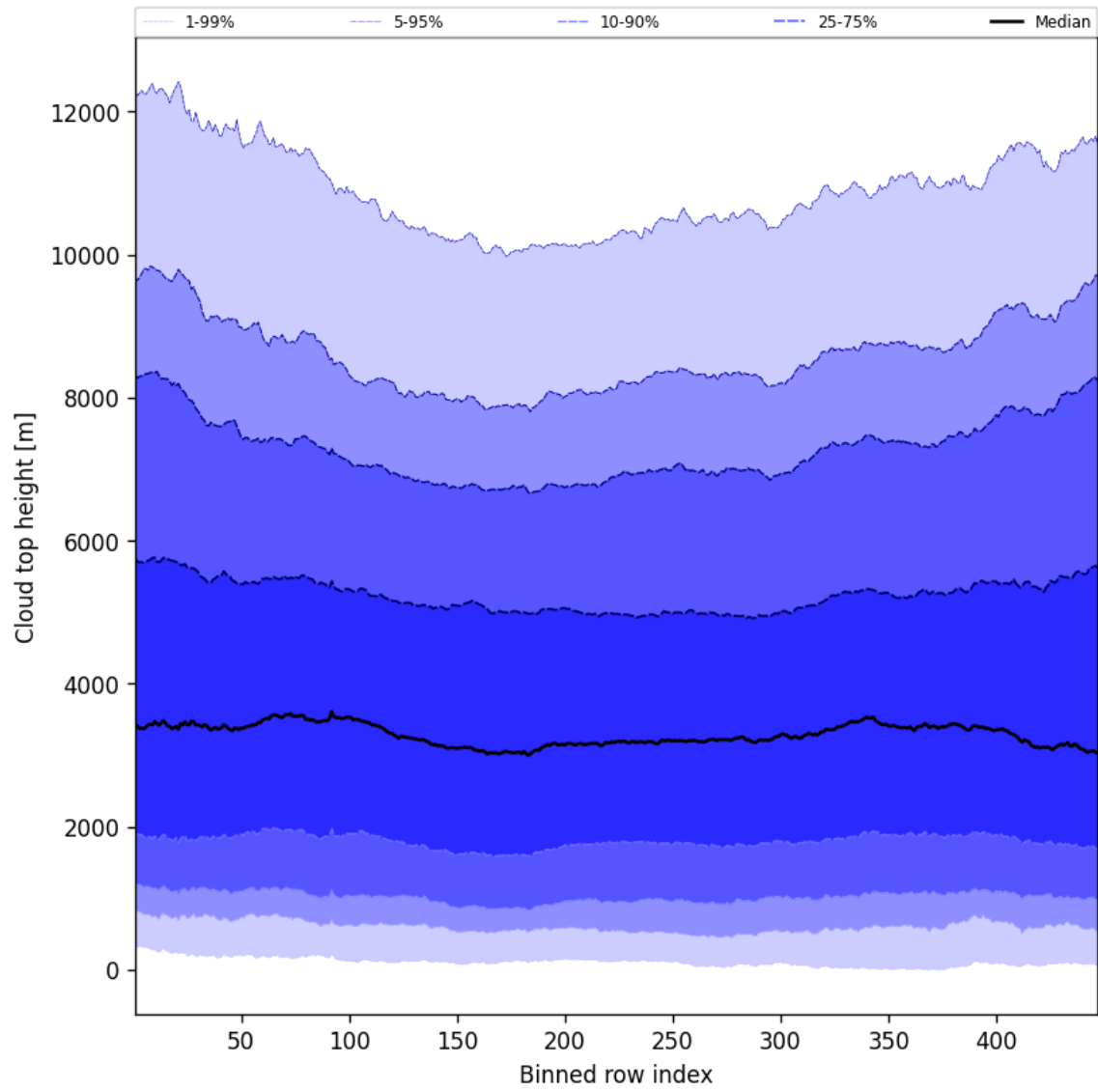
Figure 54: Along track statistics of “Cloud top height” for 2025-07-27 to 2025-07-27
