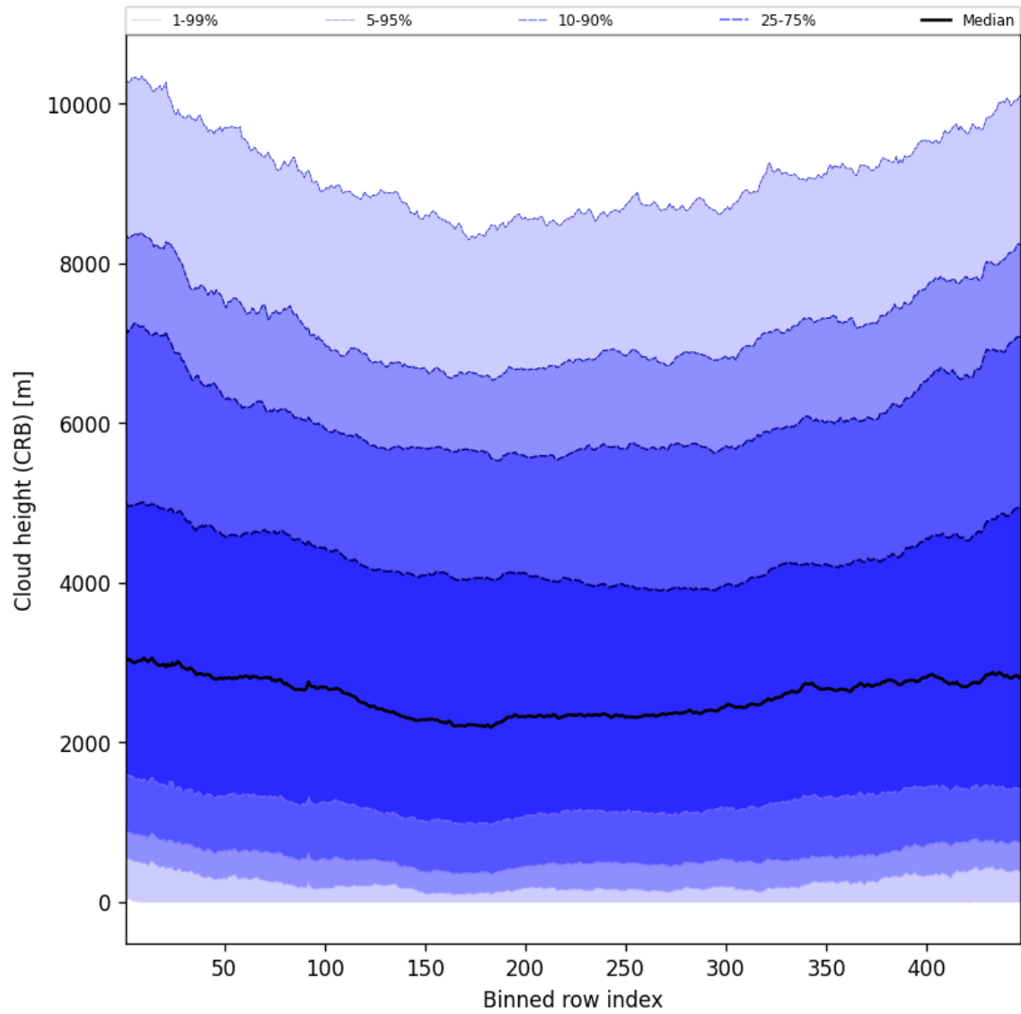
Figure 57: Along track statistics of “Cloud height (CRB)” for 2025-07-27 to 2025-07-27
