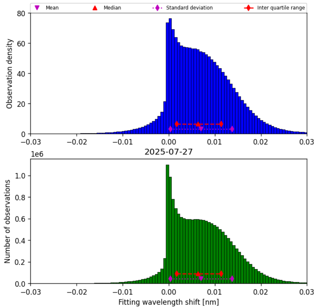
Figure 47: Histogram of “Fitting wavelength shift” for 2025-07-27 to 2025-07-27
