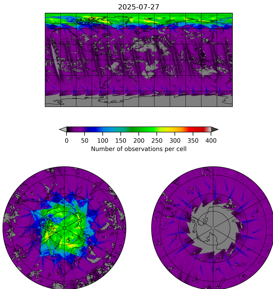
Figure 19: Map of the number of observations for 2025-07-27 to 2025-07-27
