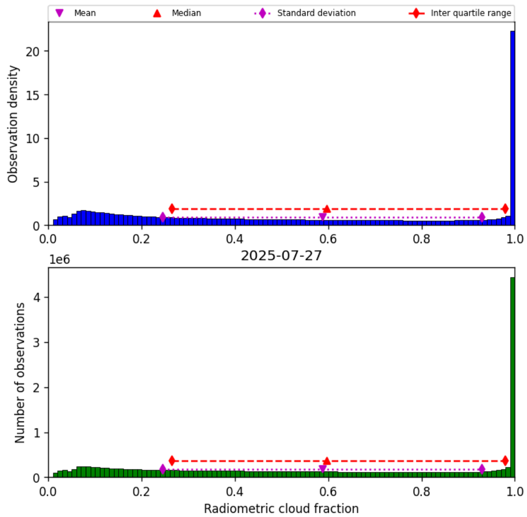
Figure 37: Histogram of “Radiometric cloud fraction” for 2025-07-27 to 2025-07-27
