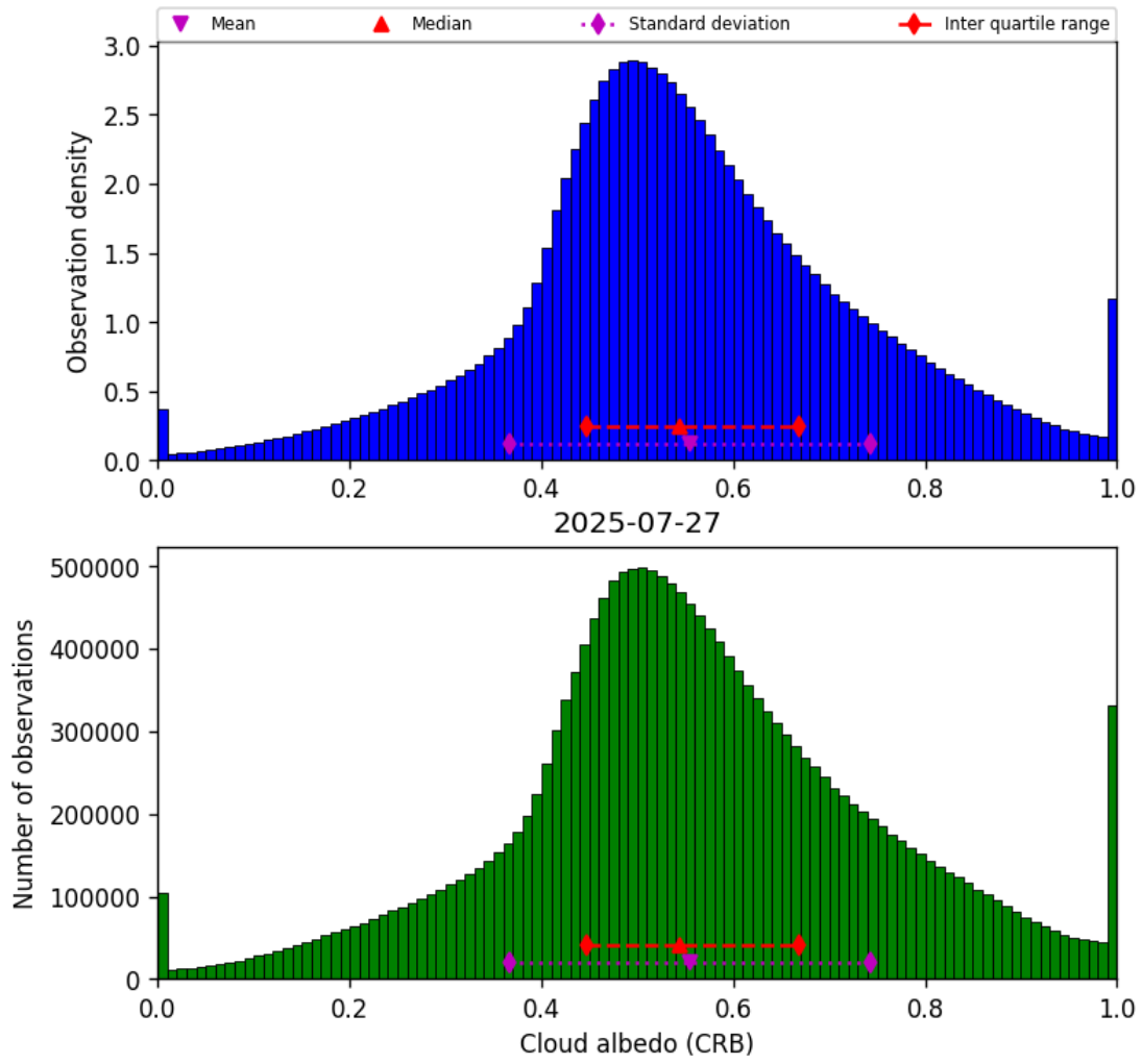
Figure 42: Histogram of “Cloud albedo (CRB)” for 2025-07-27 to 2025-07-27
