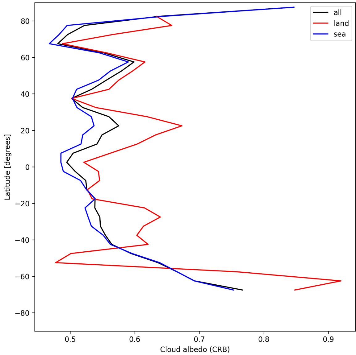
Figure 26: Zonal average of “Cloud albedo (CRB)” for 2025-07-27 to 2025-07-27.
