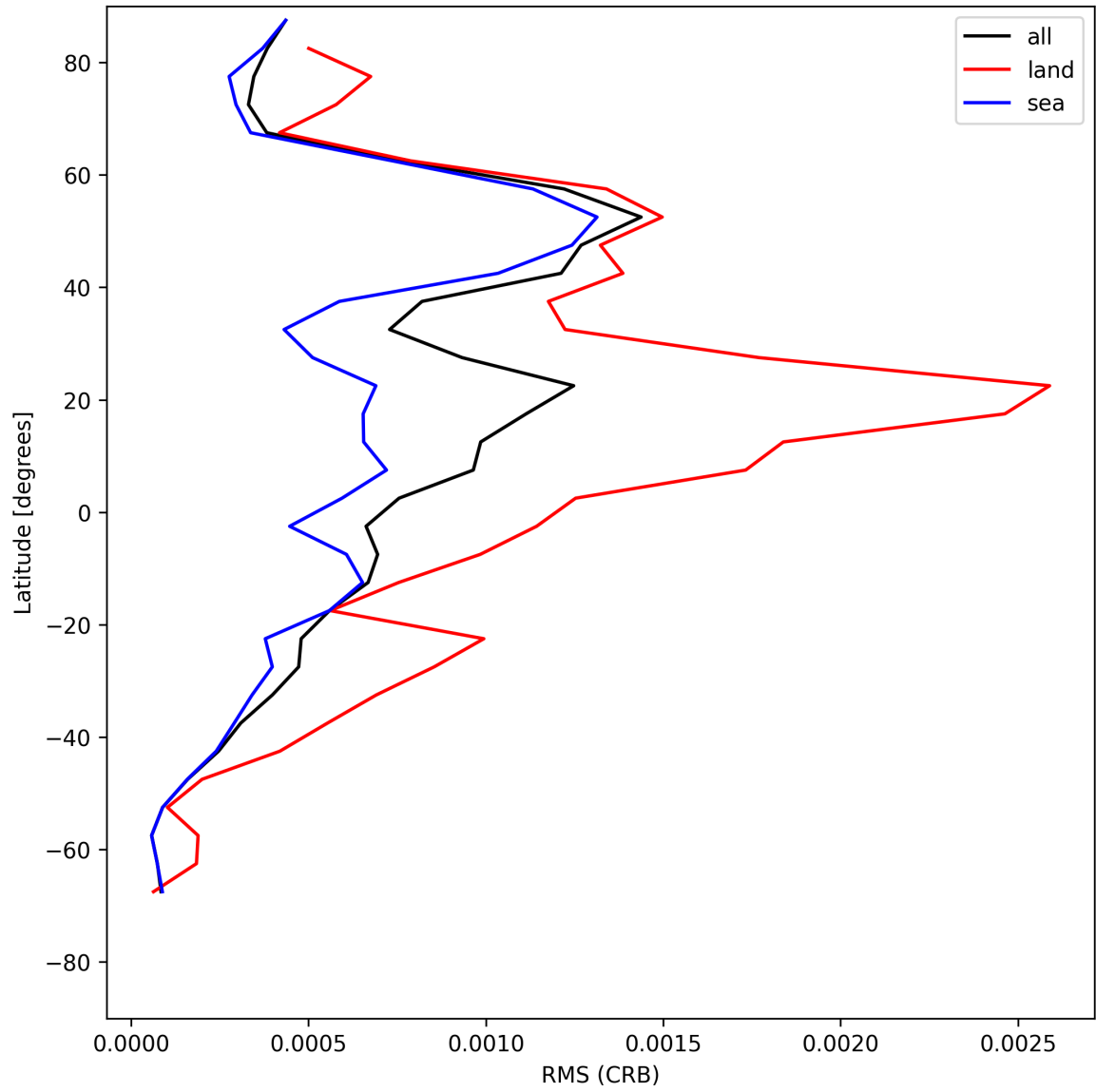
Figure 30: Zonal average of “RMS (CRB)” for 2025-07-27 to 2025-07-27.
