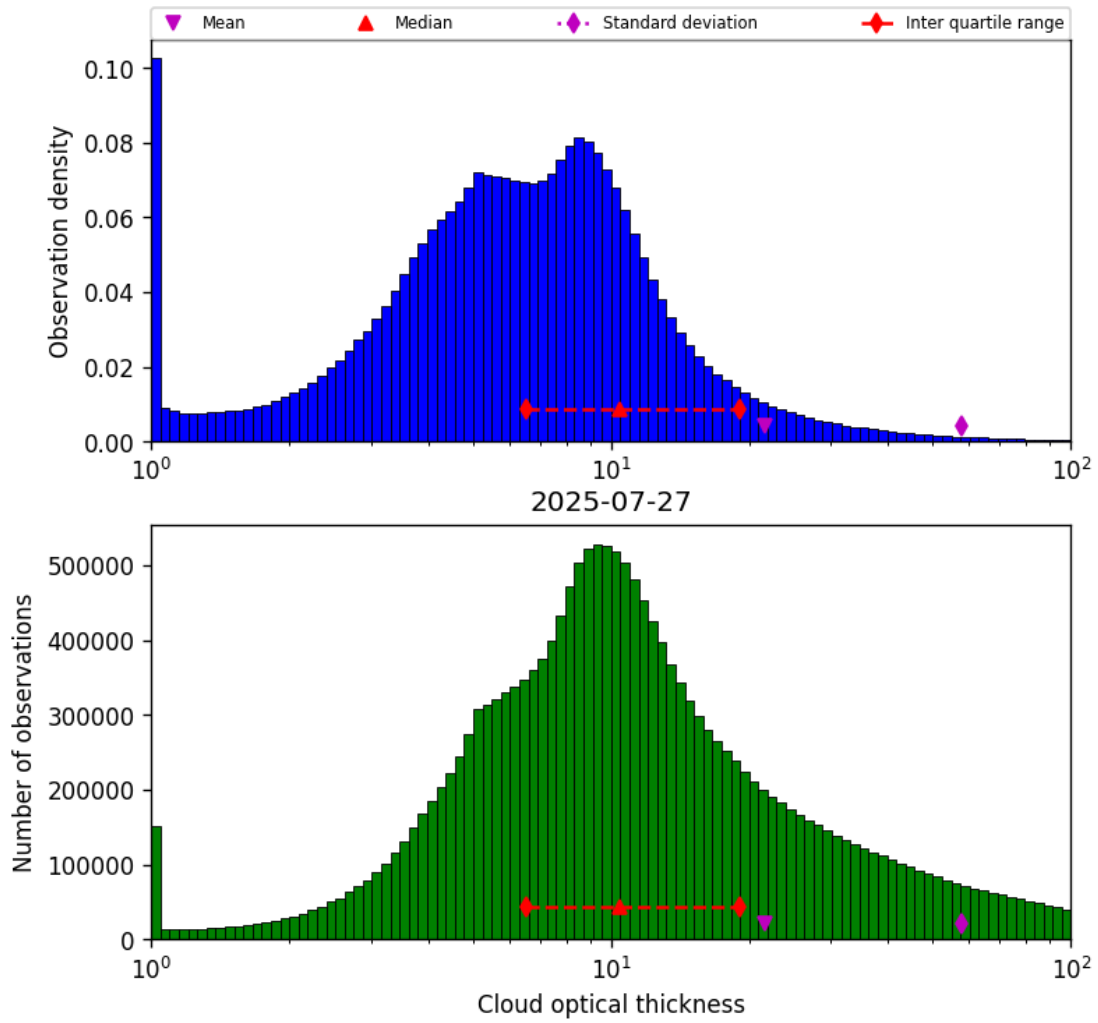
Figure 39: Histogram of “Cloud optical thickness” for 2025-07-27 to 2025-07-27
