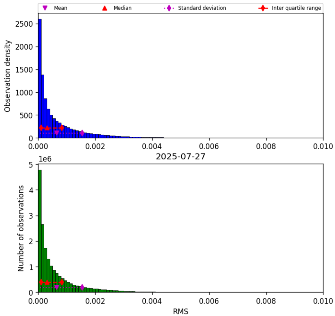
Figure 45: Histogram of “RMS” for 2025-07-27 to 2025-07-27
