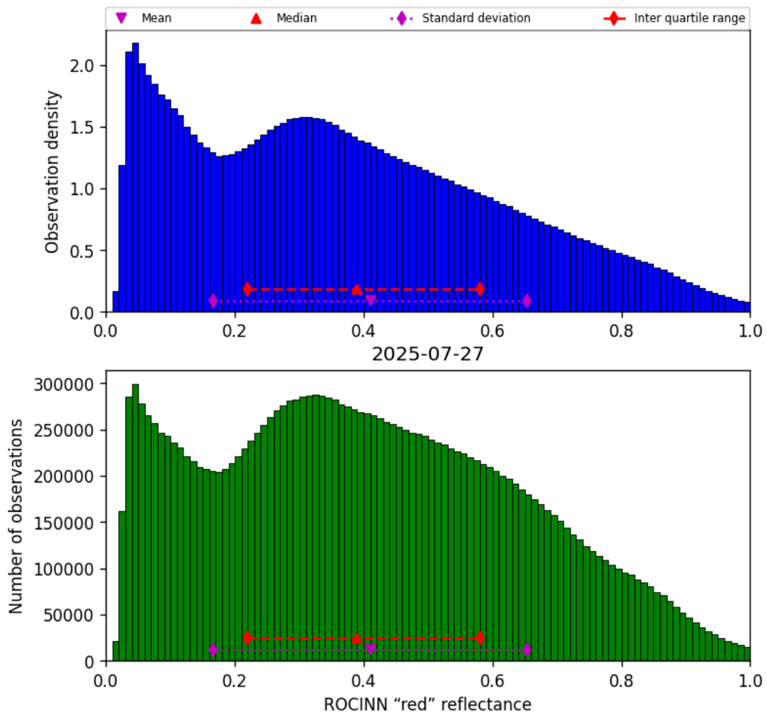
Figure 51: Histogram of “ROCINN “red” reflectance” for 2025-07-27 to 2025-07-27
