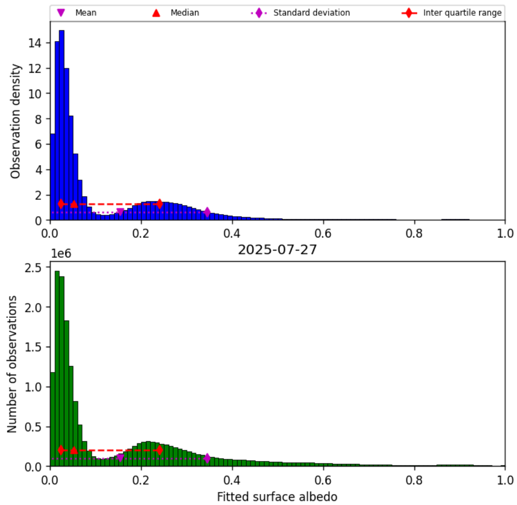
Figure 43: Histogram of “Fitted surface albedo” for 2025-07-27 to 2025-07-27
