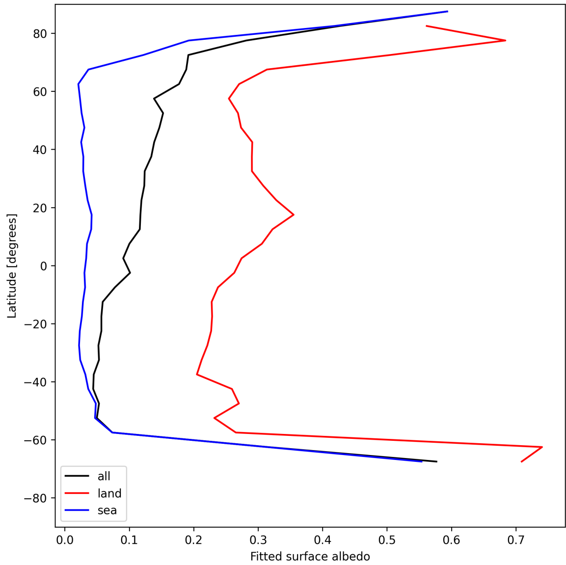
Figure 27: Zonal average of “Fitted surface albedo” for 2025-07-27 to 2025-07-27.
