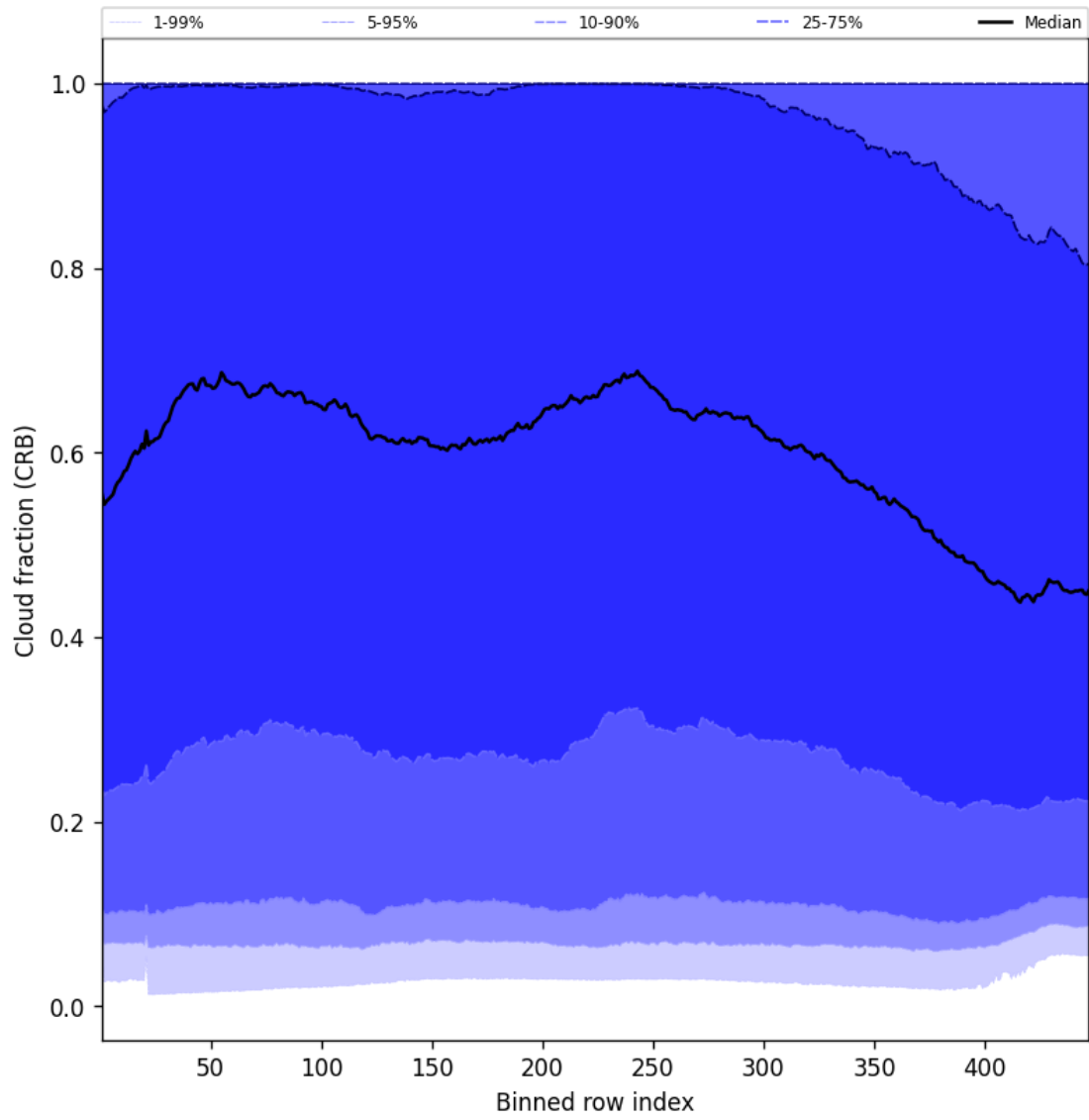
Figure 56: Along track statistics of “Cloud fraction (CRB)” for 2025-07-27 to 2025-07-27
