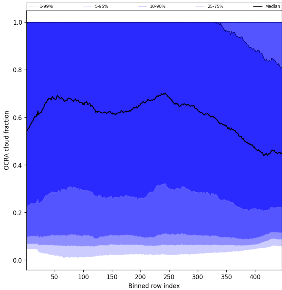
Figure 64: Along track statistics of “OCRA cloud fraction” for 2025-07-27 to 2025-07-27
