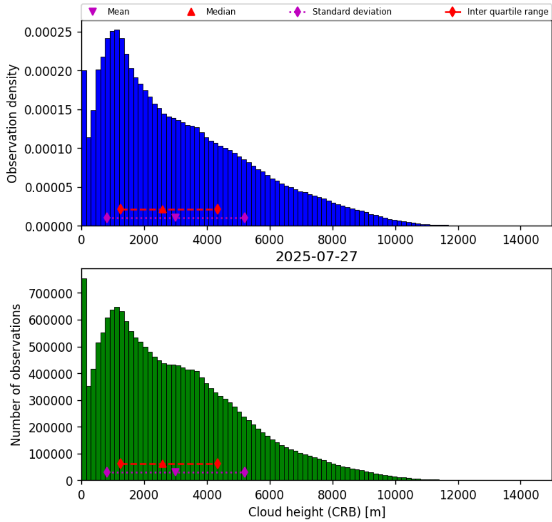
Figure 41: Histogram of “Cloud height (CRB)” for 2025-07-27 to 2025-07-27
