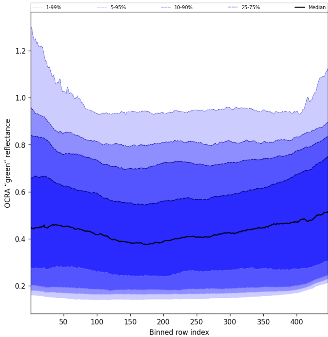
Figure 66: Along track statistics of “OCRA “green” reflectance” for 2025-07-27 to 2025-07-27
