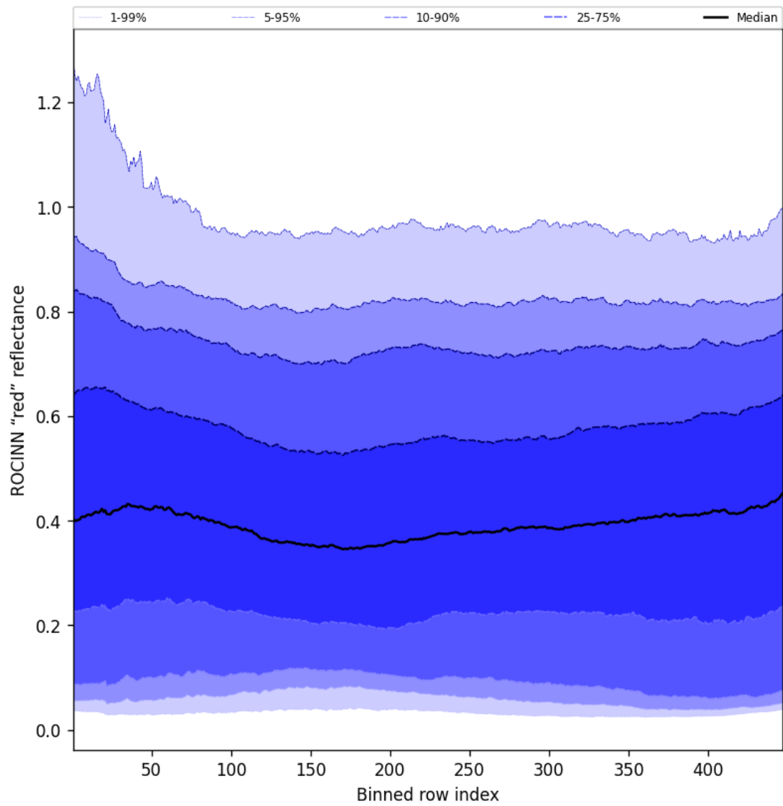
Figure 67: Along track statistics of “ROCINN “red” reflectance” for 2025-07-27 to 2025-07-27
