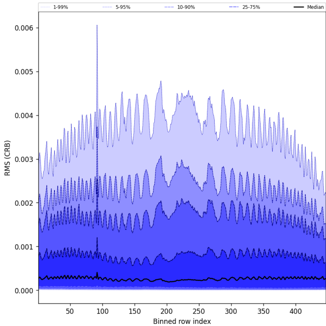
Figure 62: Along track statistics of “RMS (CRB)” for 2025-07-27 to 2025-07-27
