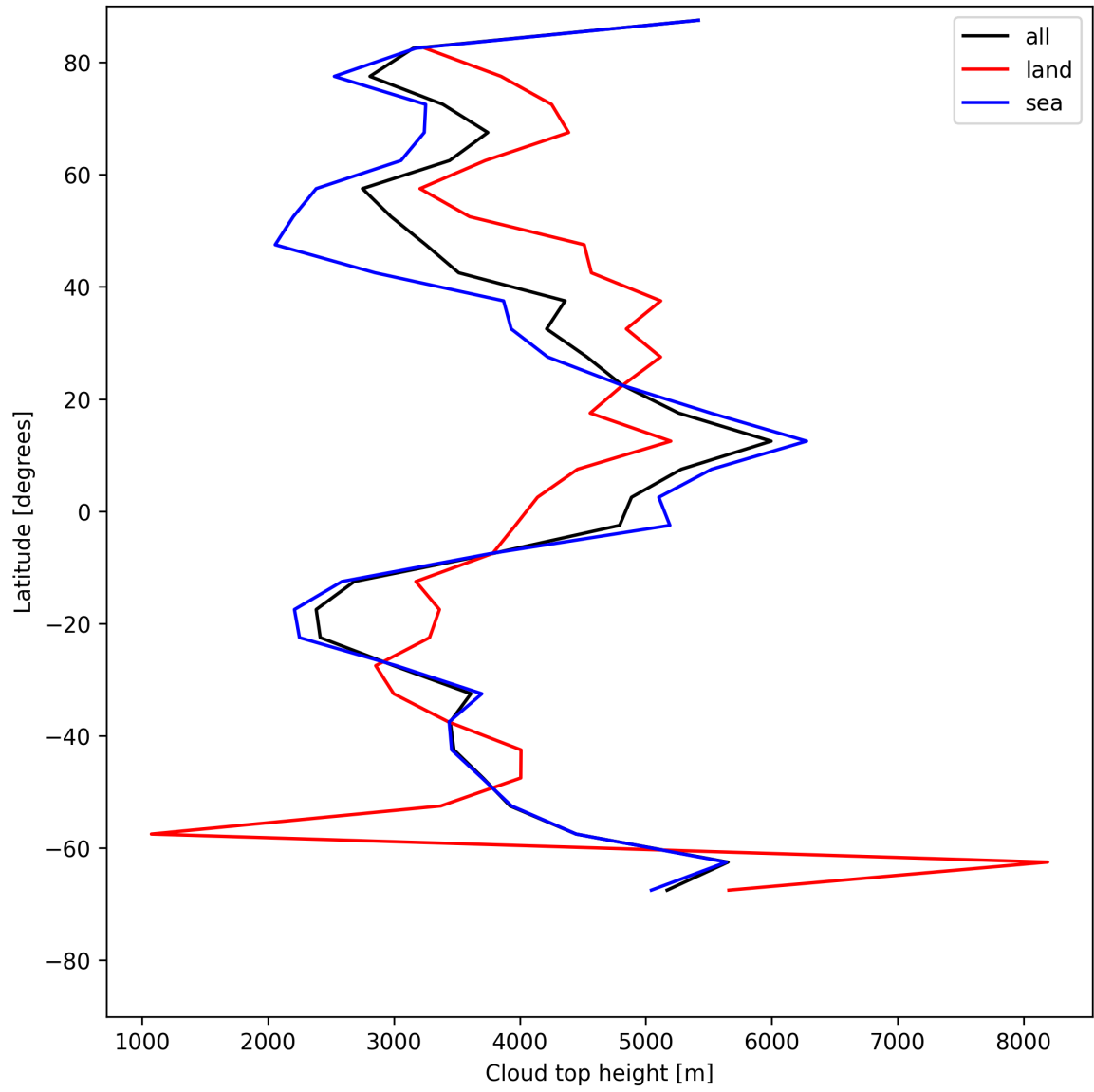
Figure 22: Zonal average of “Cloud top height” for 2025-07-27 to 2025-07-27.
