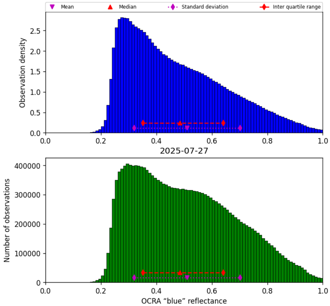
Figure 49: Histogram of “OCRA “blue” reflectance” for 2025-07-27 to 2025-07-27
