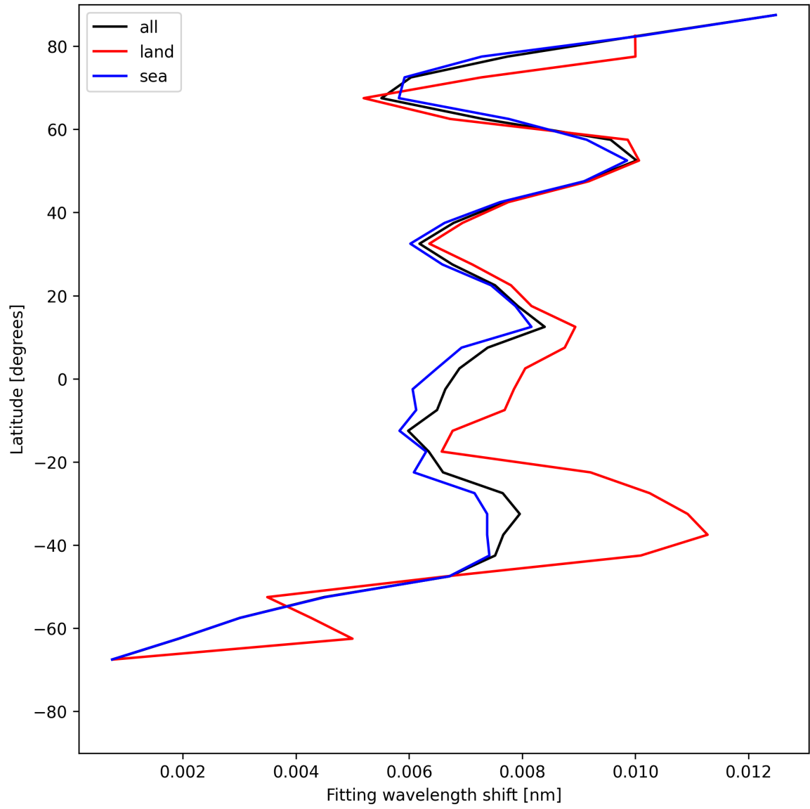
Figure 31: Zonal average of “Fitting wavelength shift” for 2025-07-27 to 2025-07-27.
