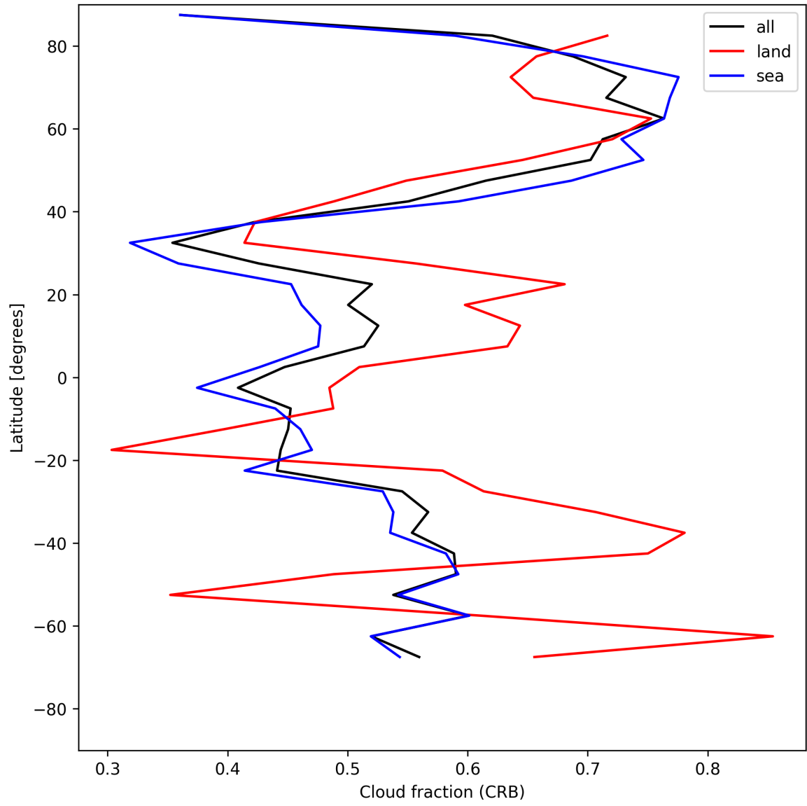
Figure 24: Zonal average of “Cloud fraction (CRB)” for 2025-07-27 to 2025-07-27.
