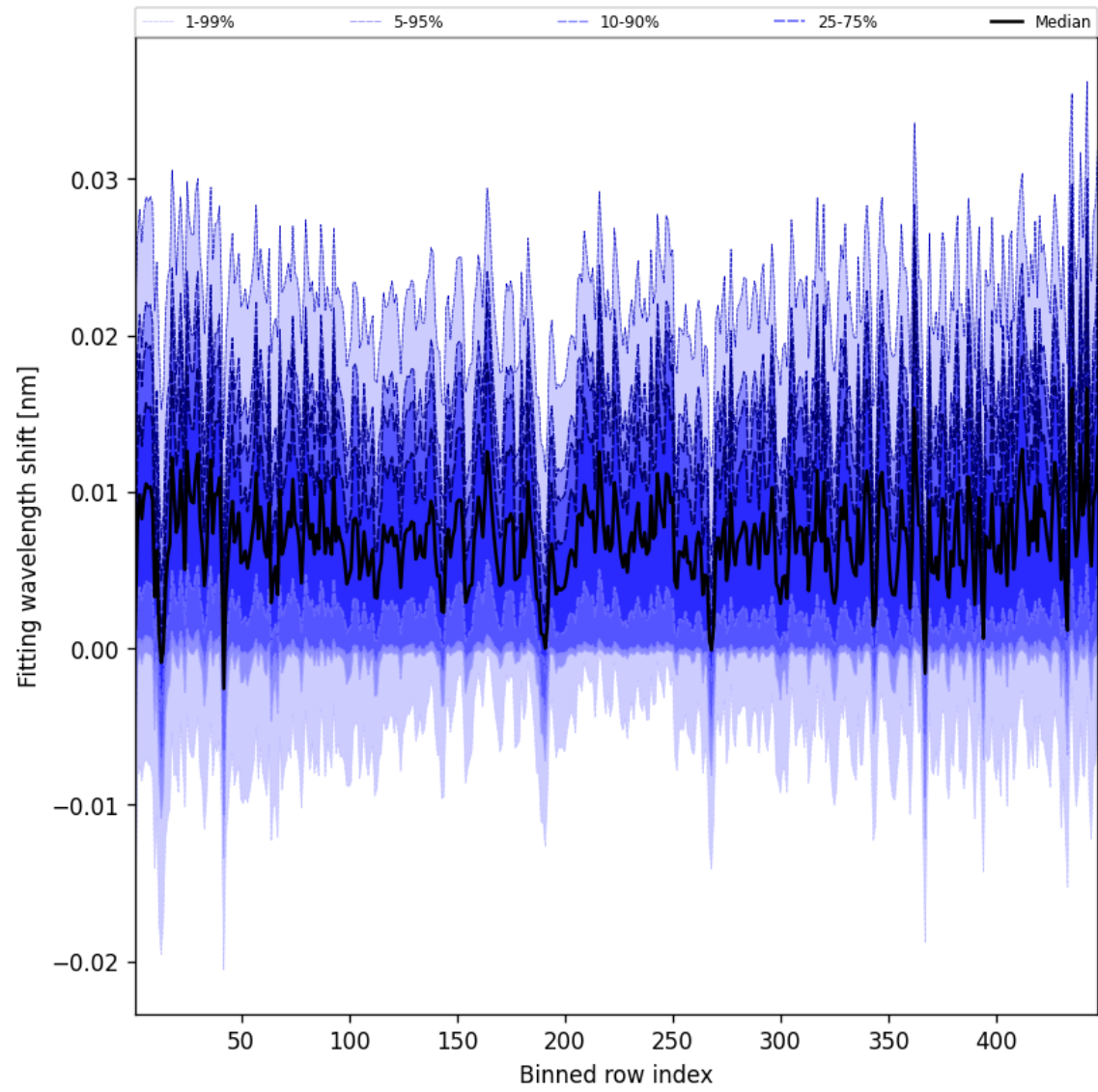
Figure 63: Along track statistics of “Fitting wavelength shift” for 2025-07-27 to 2025-07-27
