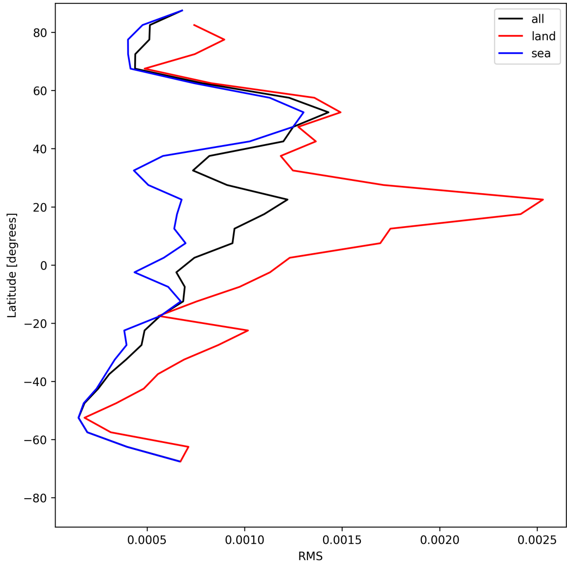
Figure 29: Zonal average of “RMS” for 2025-07-27 to 2025-07-27.
