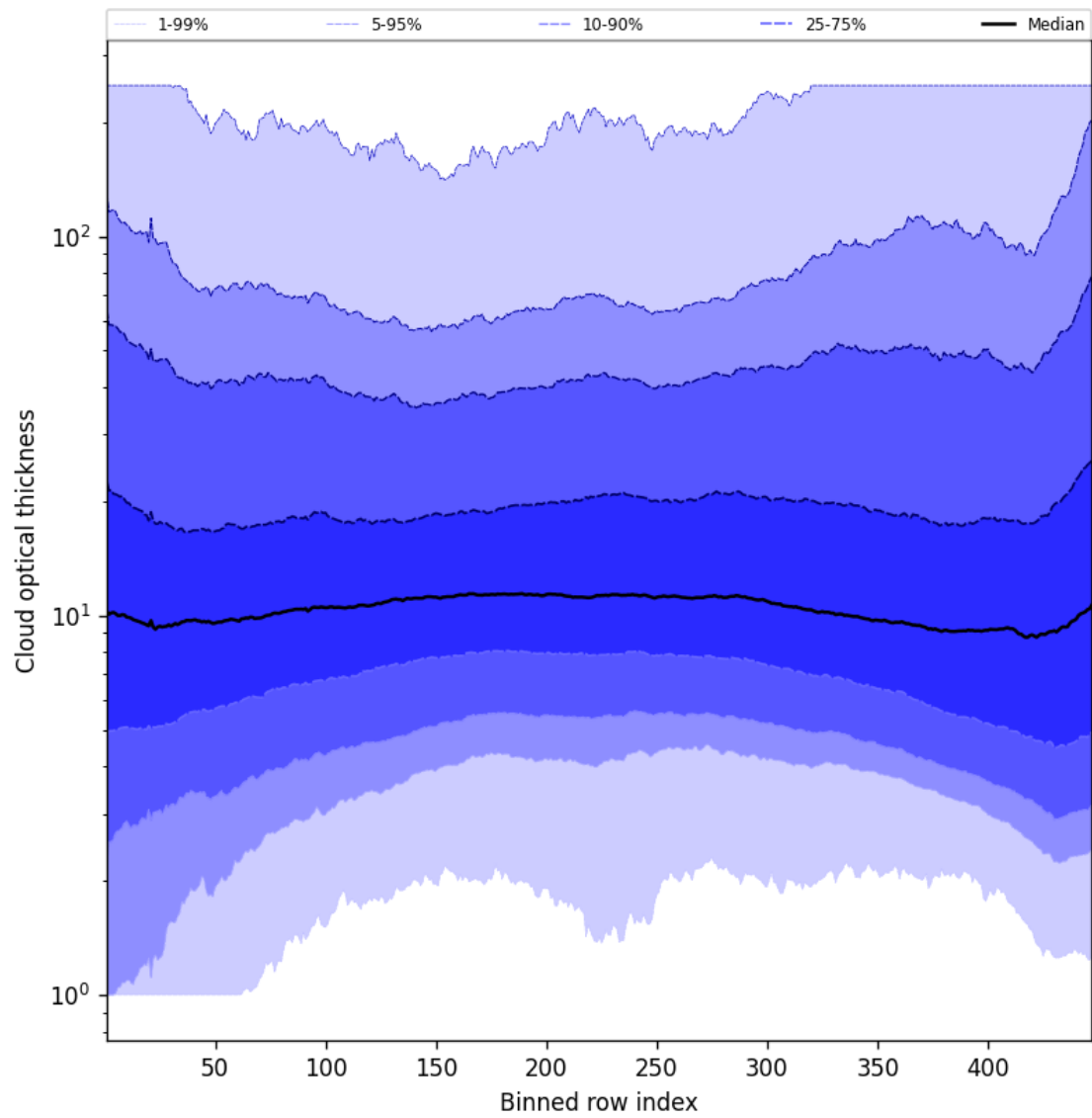
Figure 55: Along track statistics of “Cloud optical thickness” for 2025-07-27 to 2025-07-27
