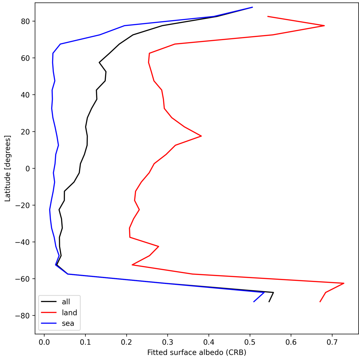
Figure 28: Zonal average of “Fitted surface albedo (CRB)” for 2025-07-29 to 2025-07-30.
