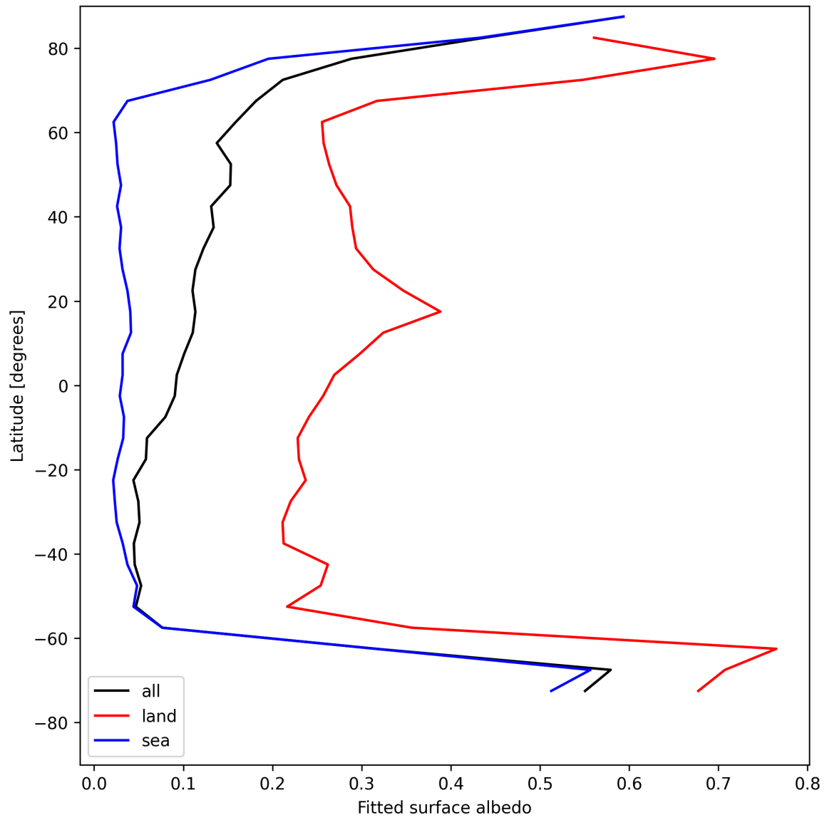
Figure 27: Zonal average of “Fitted surface albedo” for 2025-07-29 to 2025-07-30.
