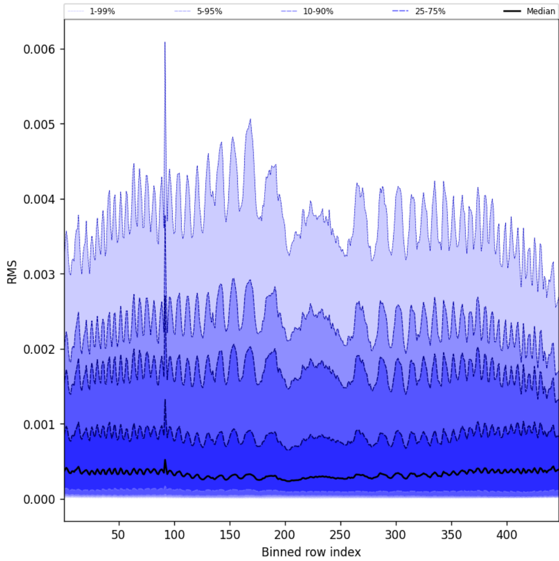
Figure 61: Along track statistics of “RMS” for 2025-07-29 to 2025-07-30
