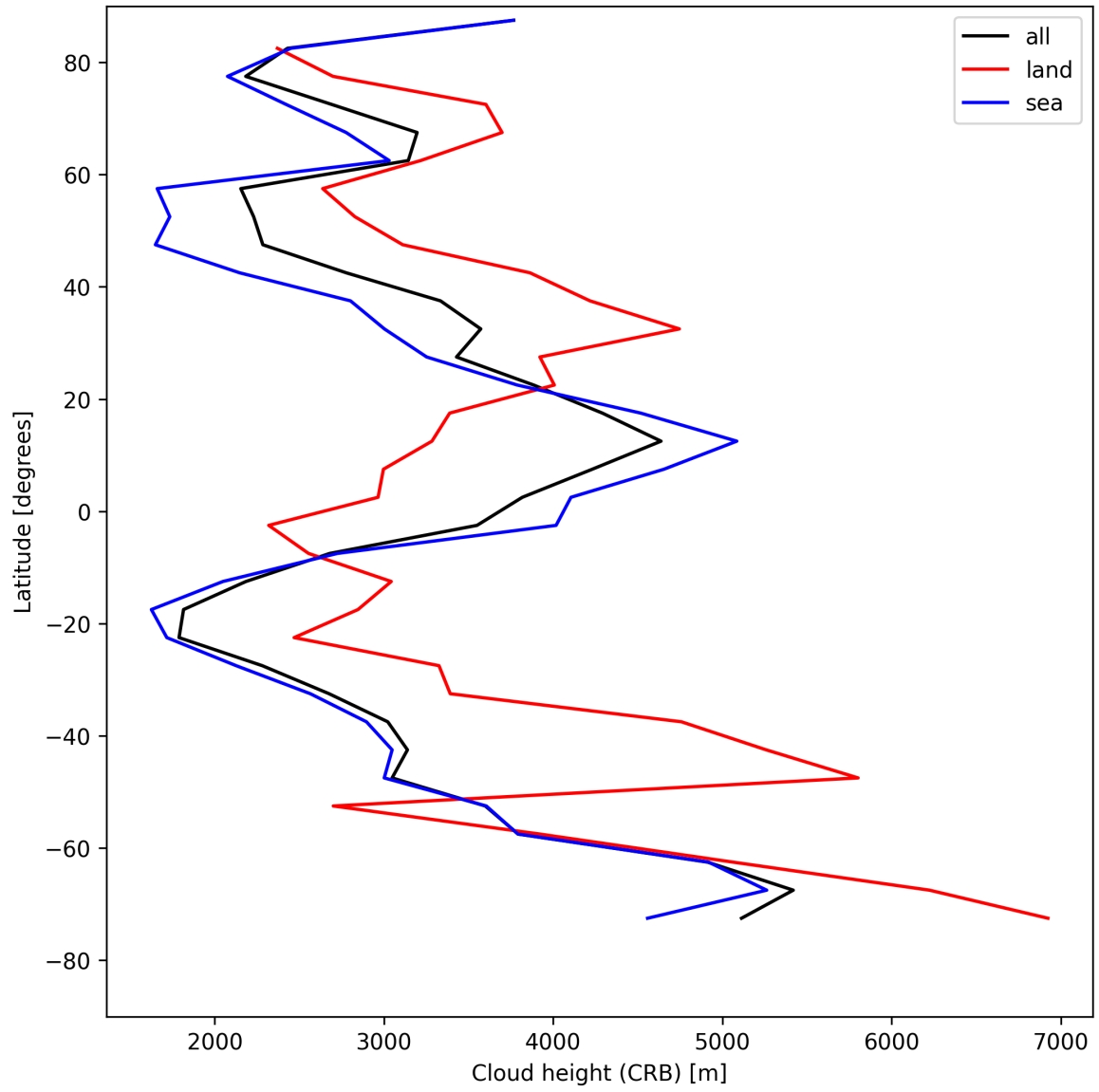
Figure 25: Zonal average of “Cloud height (CRB)” for 2025-07-29 to 2025-07-30.
