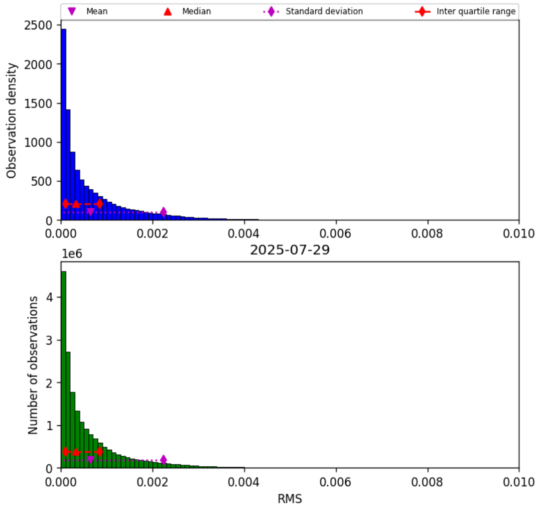
Figure 45: Histogram of “RMS” for 2025-07-29 to 2025-07-30
