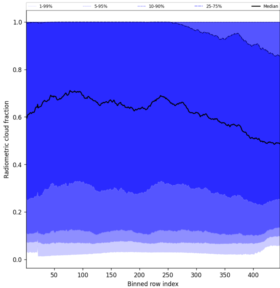
Figure 53: Along track statistics of “Radiometric cloud fraction” for 2025-07-29 to 2025-07-30
