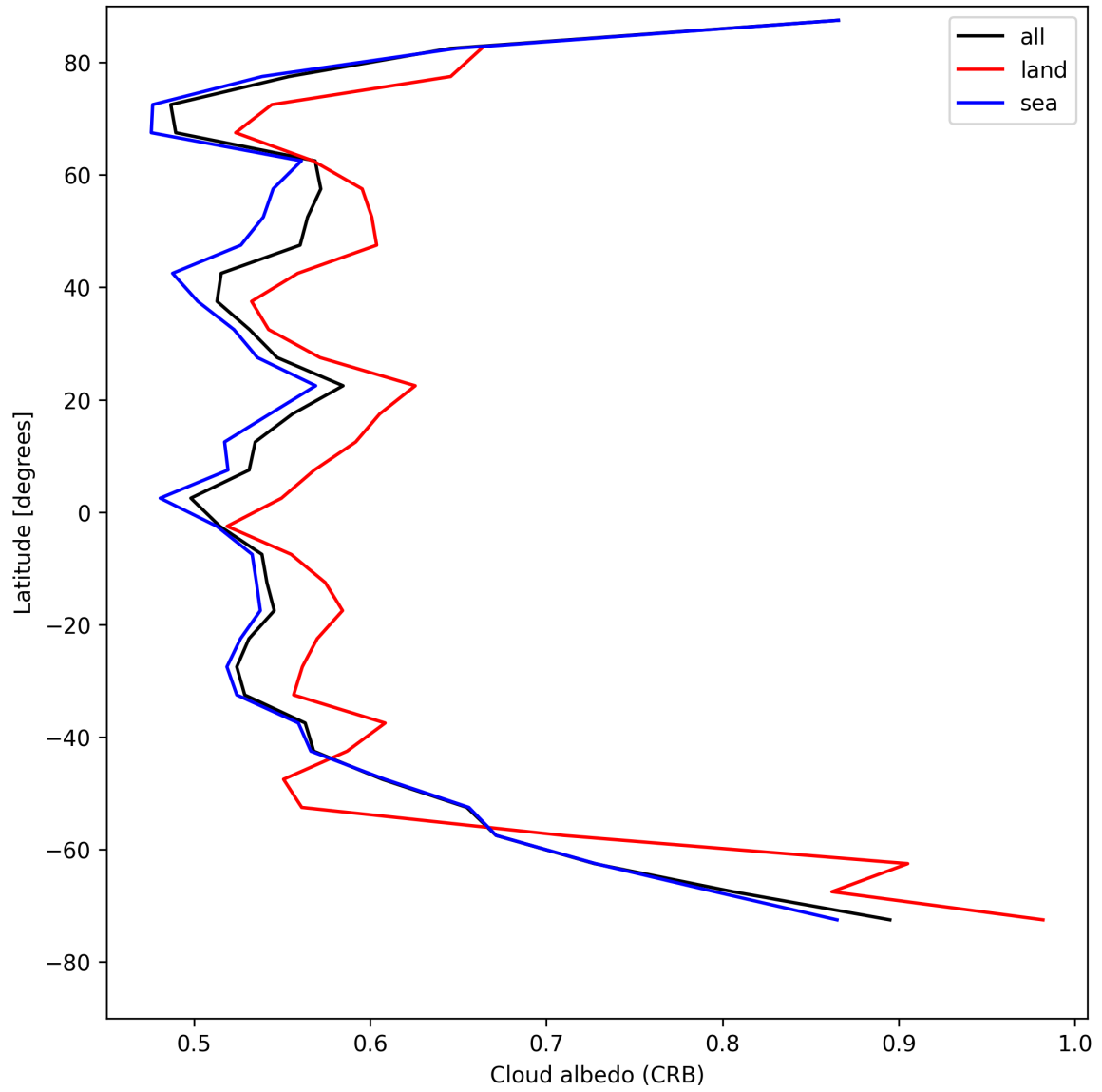
Figure 26: Zonal average of “Cloud albedo (CRB)” for 2025-07-29 to 2025-07-30.
