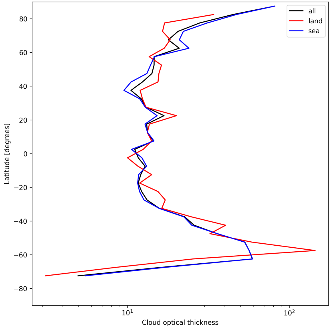
Figure 23: Zonal average of “Cloud optical thickness” for 2025-07-29 to 2025-07-30.
