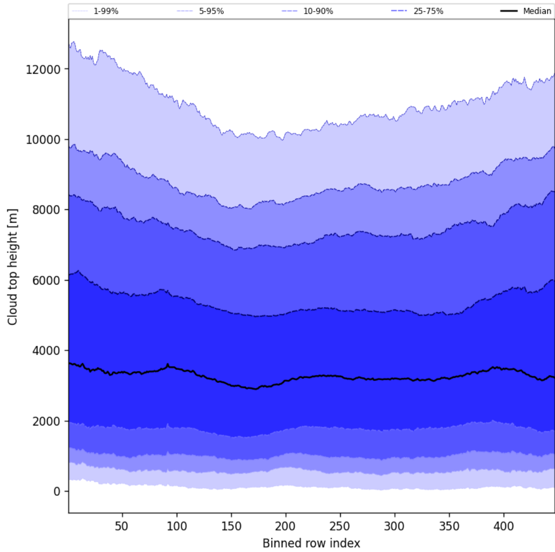
Figure 54: Along track statistics of “Cloud top height” for 2025-07-29 to 2025-07-30
