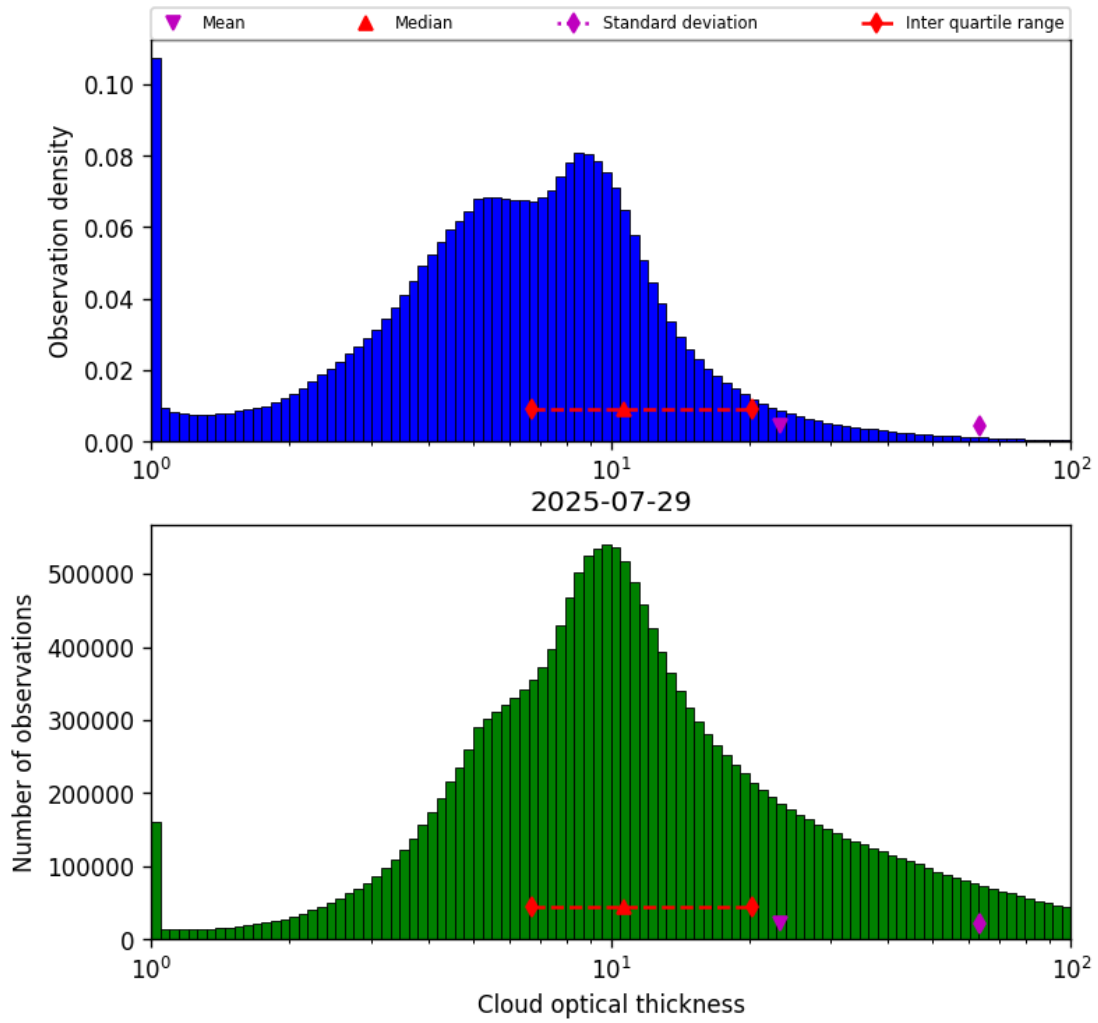
Figure 39: Histogram of “Cloud optical thickness” for 2025-07-29 to 2025-07-30
