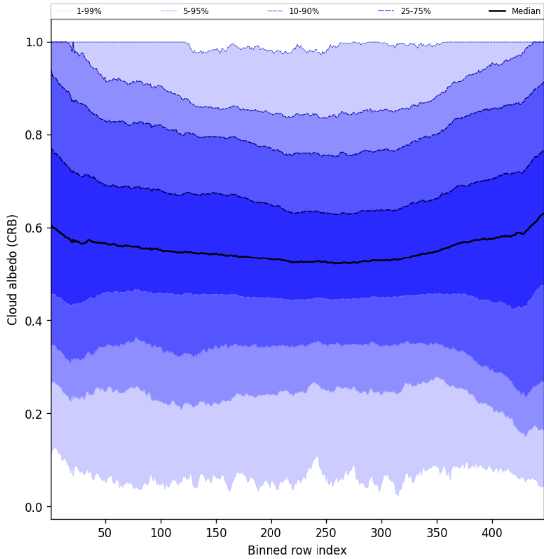
Figure 58: Along track statistics of “Cloud albedo (CRB)” for 2025-07-29 to 2025-07-30
