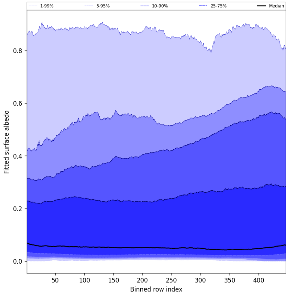
Figure 59: Along track statistics of “Fitted surface albedo” for 2025-07-29 to 2025-07-30
