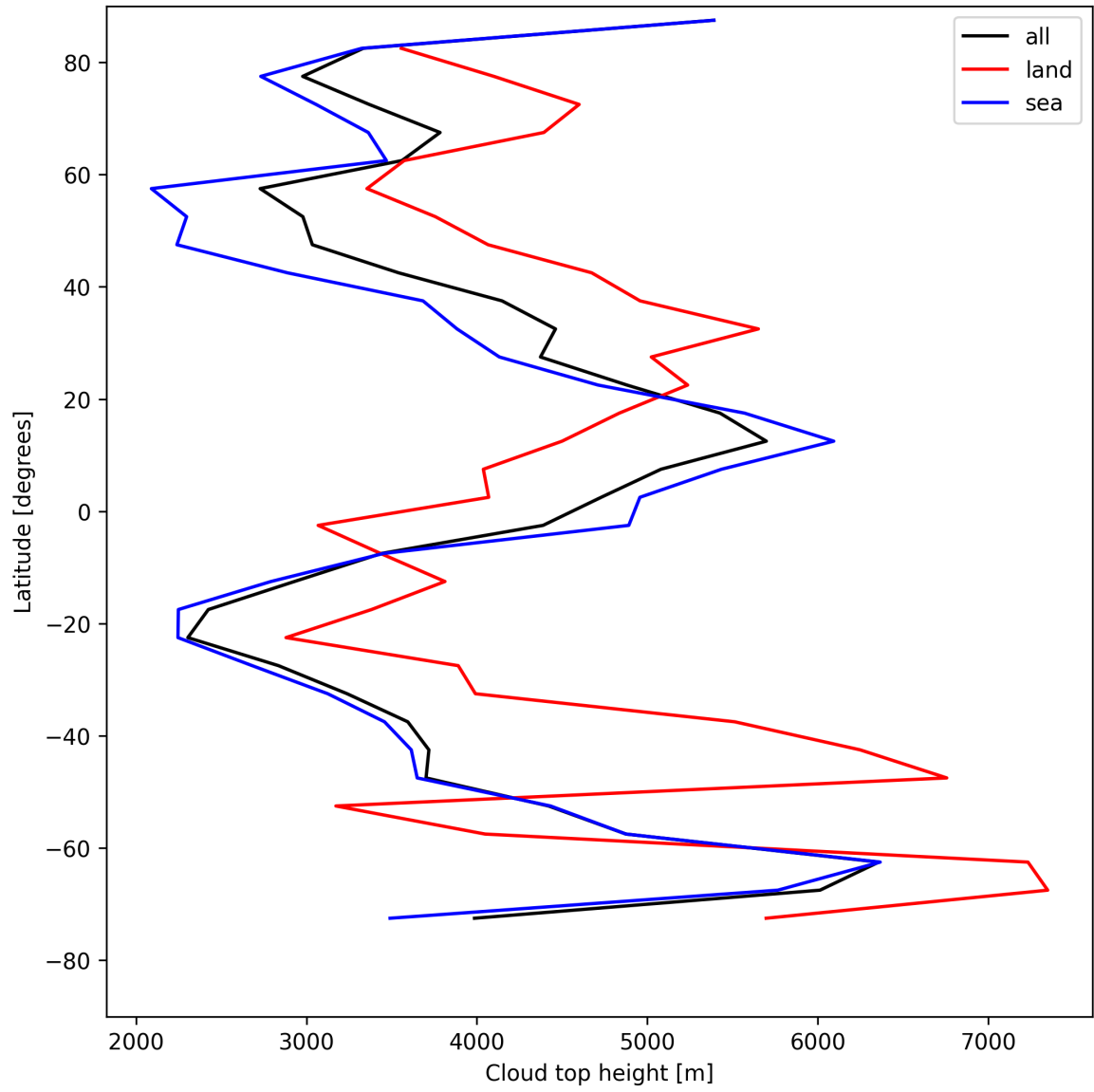
Figure 22: Zonal average of “Cloud top height” for 2025-07-29 to 2025-07-30.
