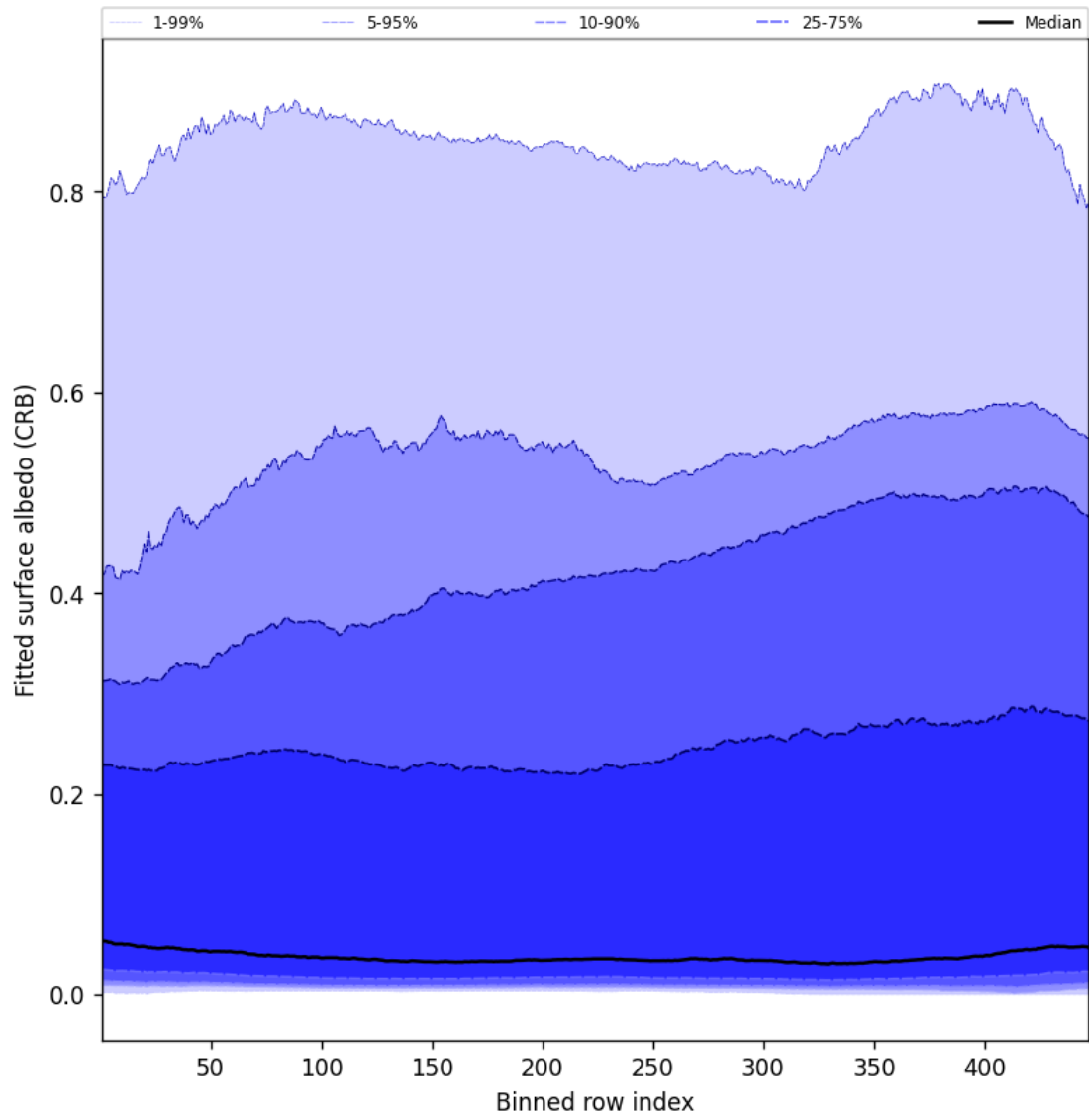
Figure 60: Along track statistics of “Fitted surface albedo (CRB)” for 2025-07-29 to 2025-07-30
