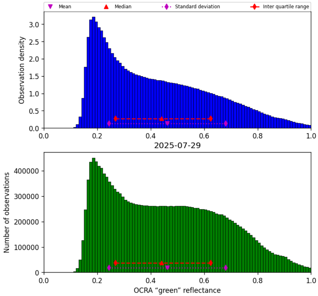
Figure 50: Histogram of “OCRA “green” reflectance” for 2025-07-29 to 2025-07-30
