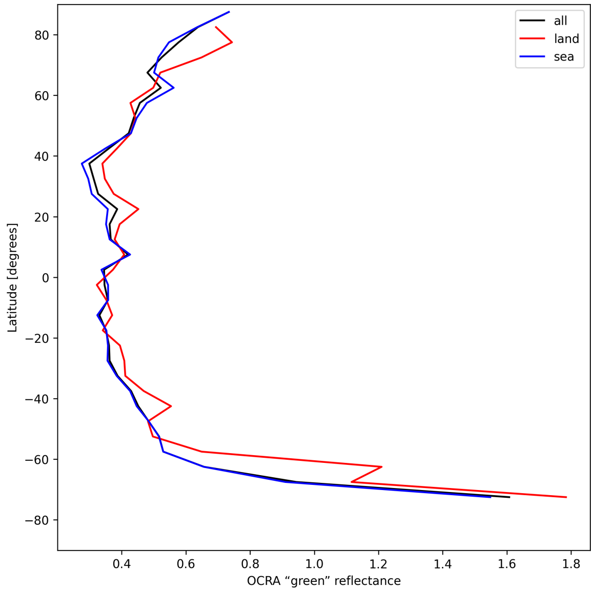
Figure 34: Zonal average of “OCRA “green” reflectance” for 2025-07-29 to 2025-07-30.
