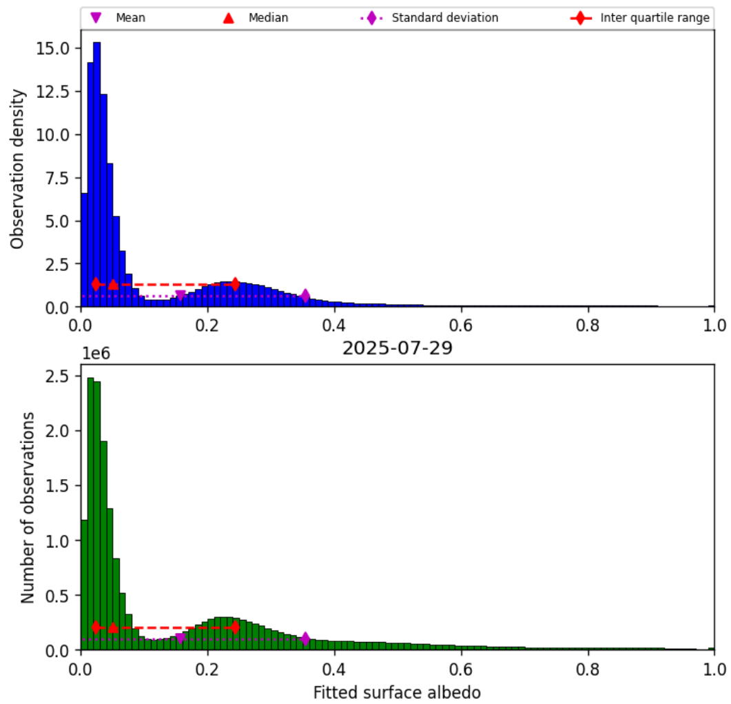
Figure 43: Histogram of “Fitted surface albedo” for 2025-07-29 to 2025-07-30
