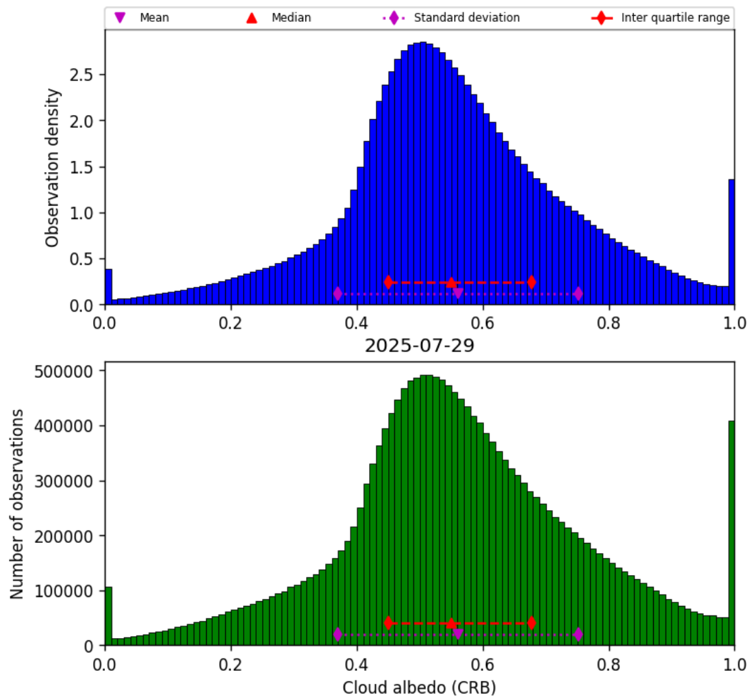
Figure 42: Histogram of “Cloud albedo (CRB)” for 2025-07-29 to 2025-07-30
