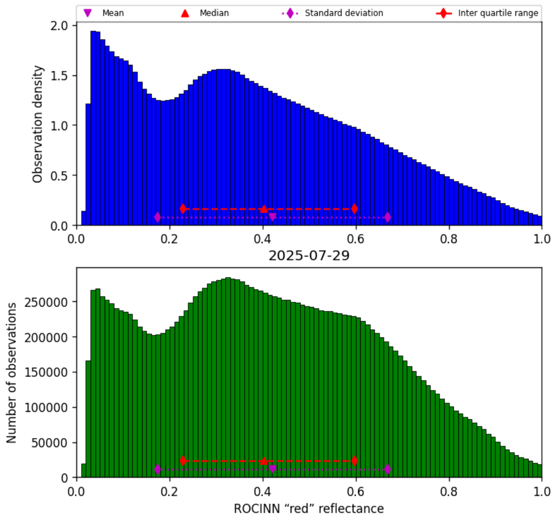
Figure 51: Histogram of “ROCINN “red” reflectance” for 2025-07-29 to 2025-07-30
