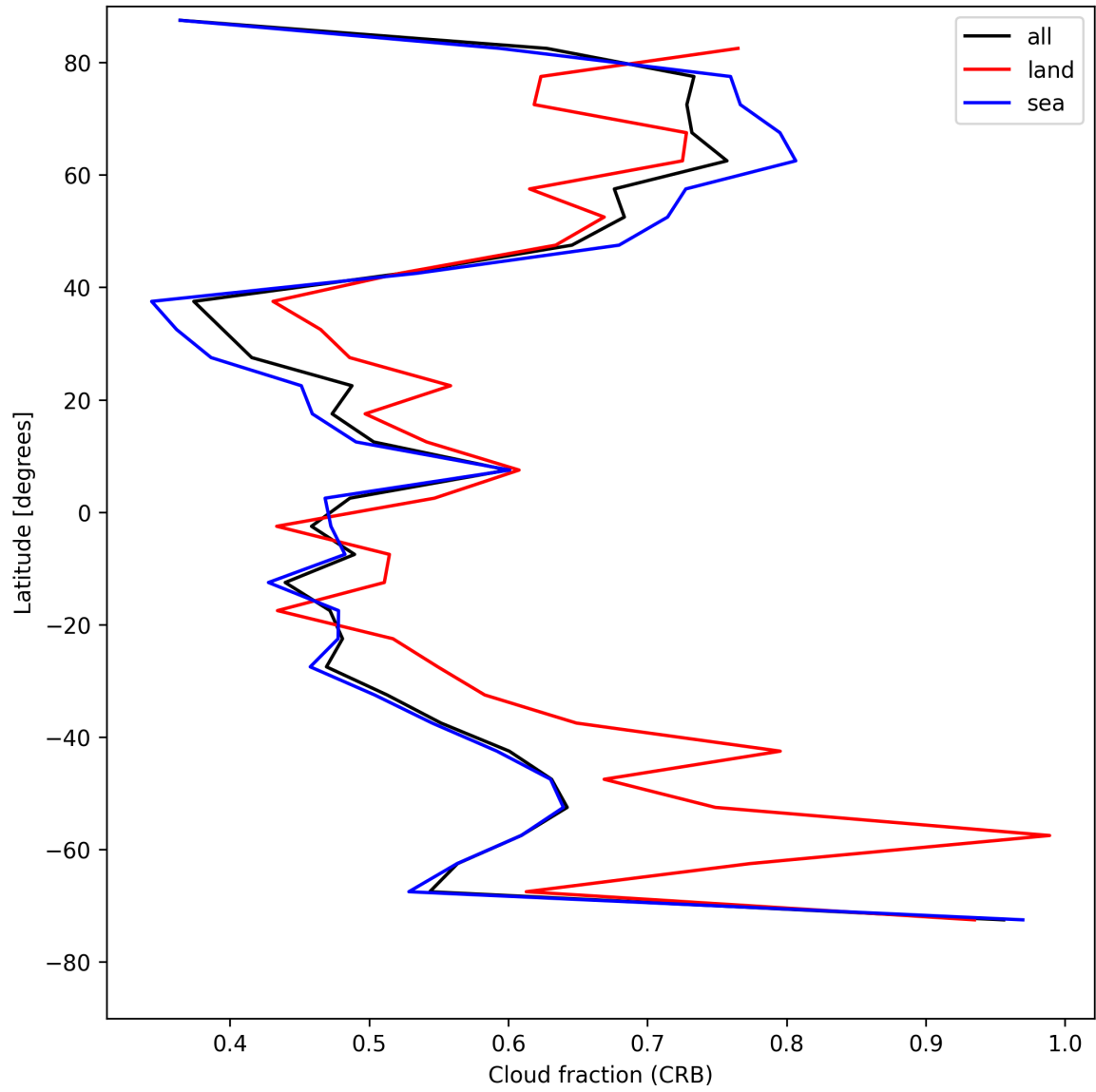
Figure 24: Zonal average of “Cloud fraction (CRB)” for 2025-07-29 to 2025-07-30.
