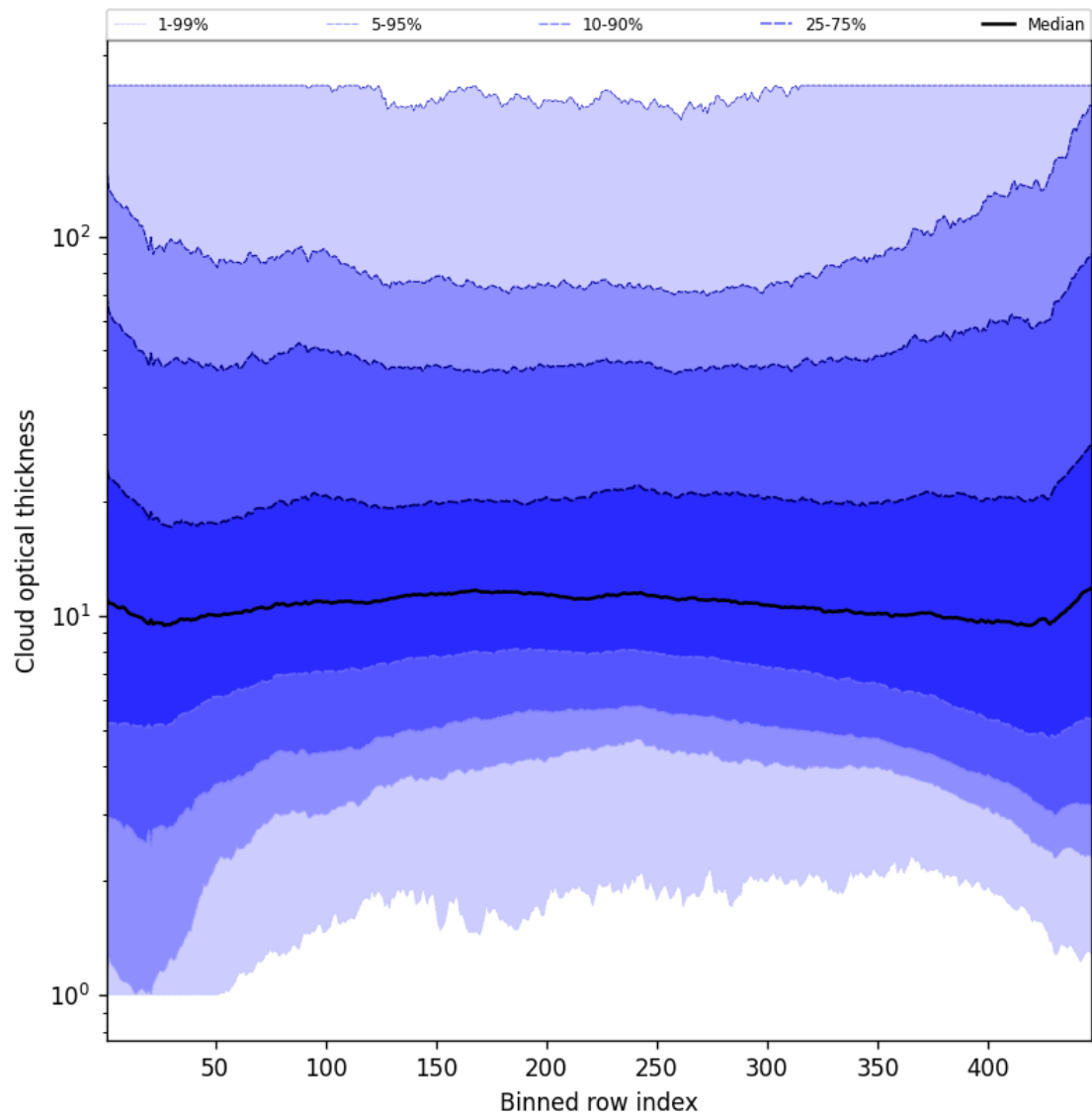
Figure 55: Along track statistics of “Cloud optical thickness” for 2025-07-29 to 2025-07-30
