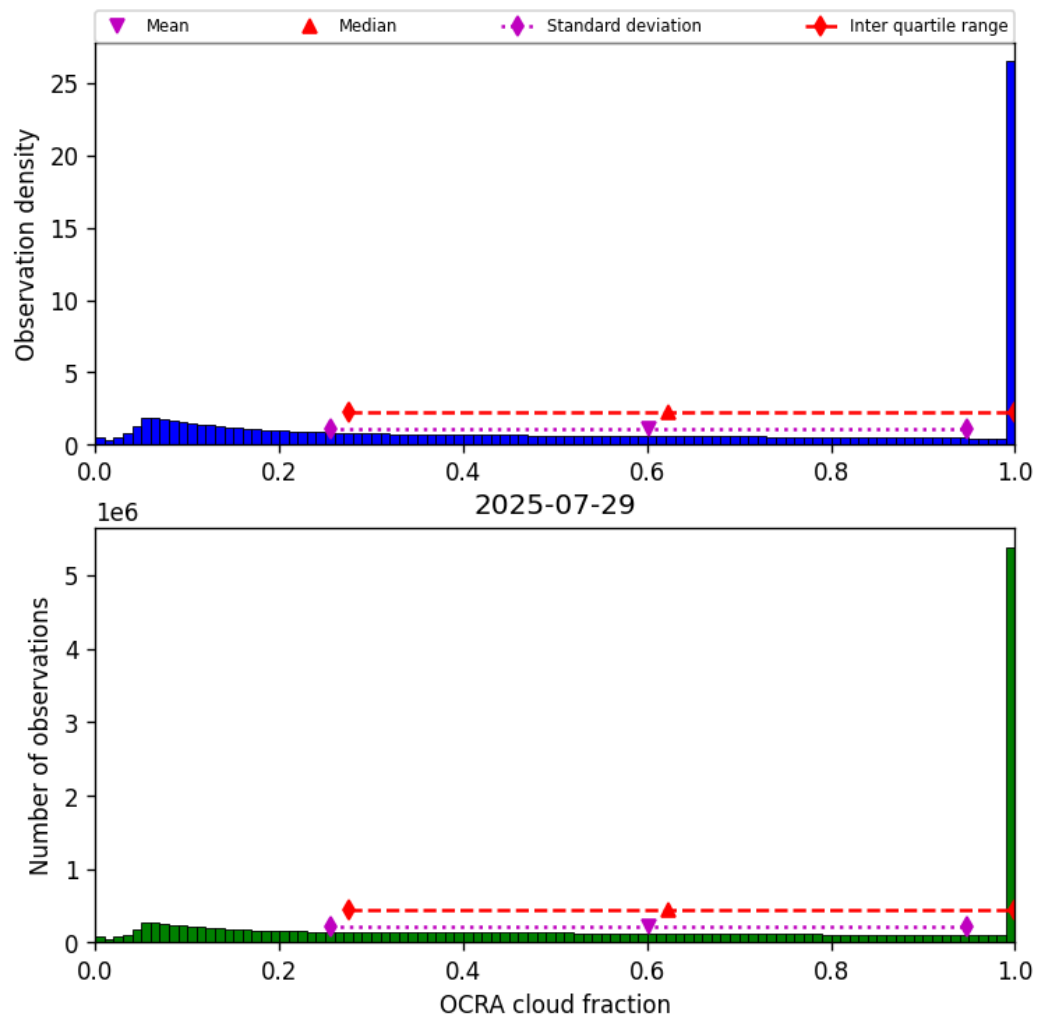
Figure 48: Histogram of “OCRA cloud fraction” for 2025-07-29 to 2025-07-30
