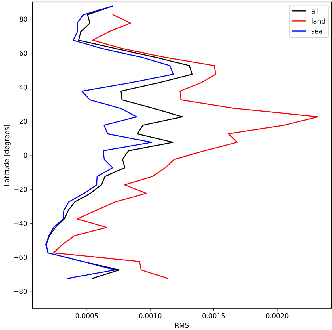
Figure 29: Zonal average of “RMS” for 2025-07-29 to 2025-07-30.
