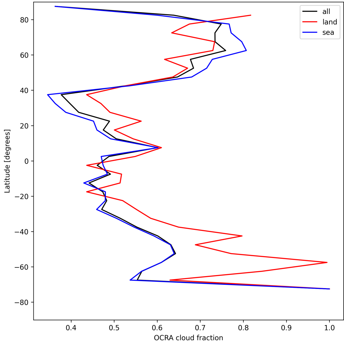
Figure 32: Zonal average of “OCRA cloud fraction” for 2025-07-29 to 2025-07-30.
