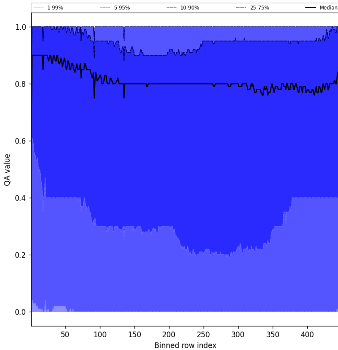
Figure 52: Along track statistics of “QA value” for 2025-07-29 to 2025-07-30
