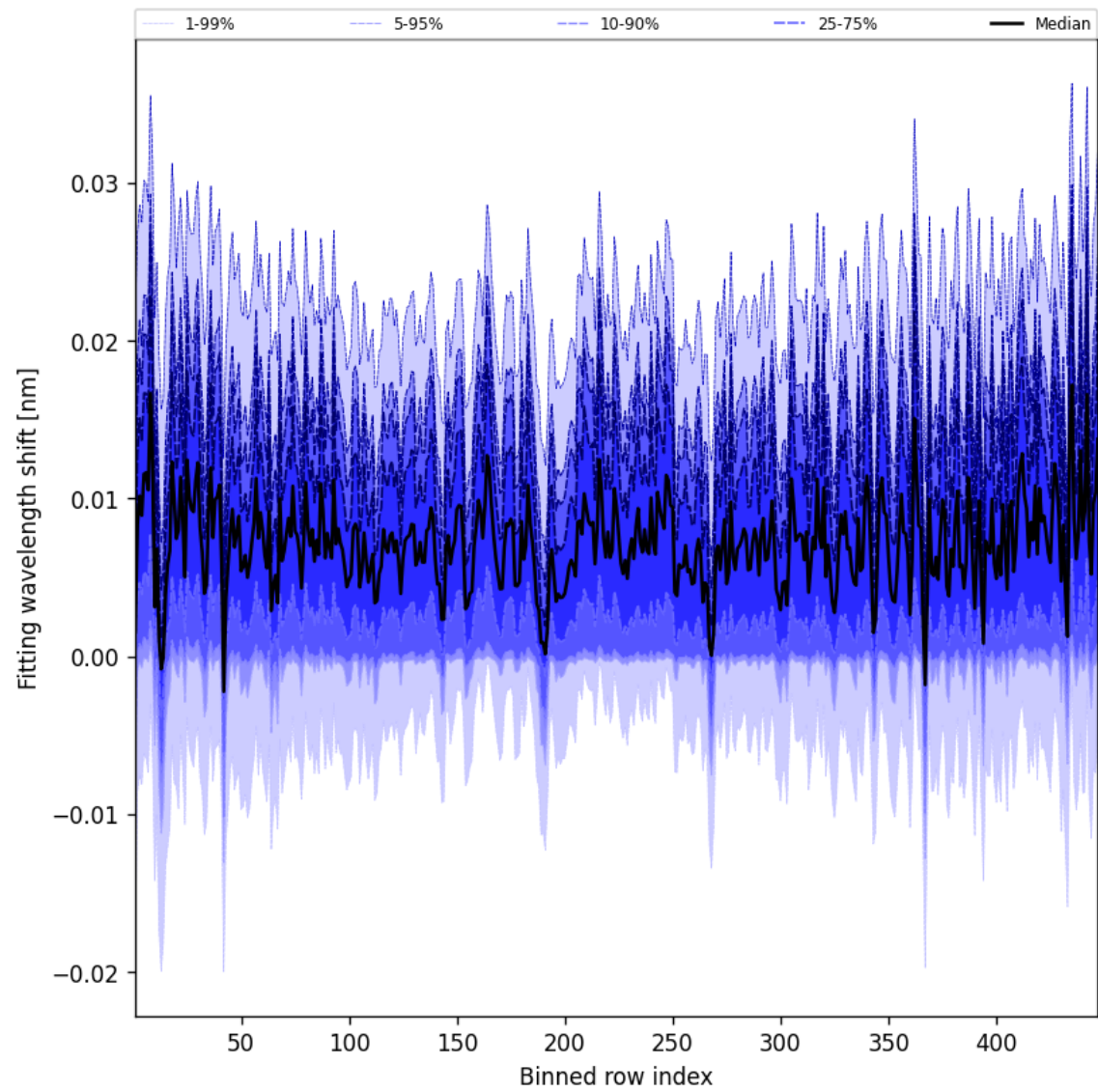
Figure 63: Along track statistics of “Fitting wavelength shift” for 2025-07-29 to 2025-07-30
