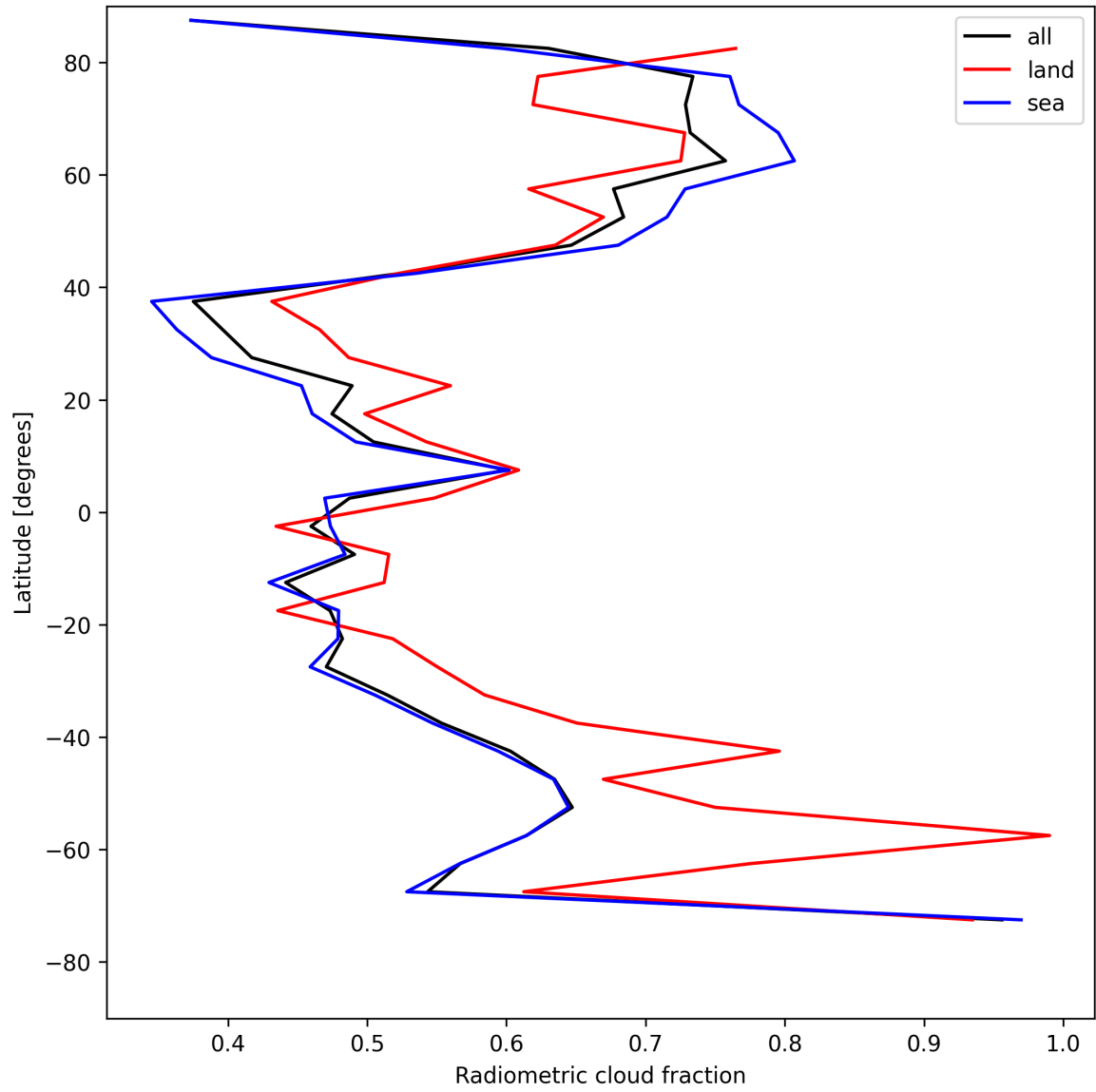
Figure 21: Zonal average of “Radiometric cloud fraction” for 2025-07-29 to 2025-07-30.
