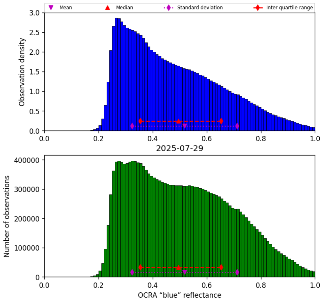
Figure 49: Histogram of “OCRA “blue” reflectance” for 2025-07-29 to 2025-07-30
