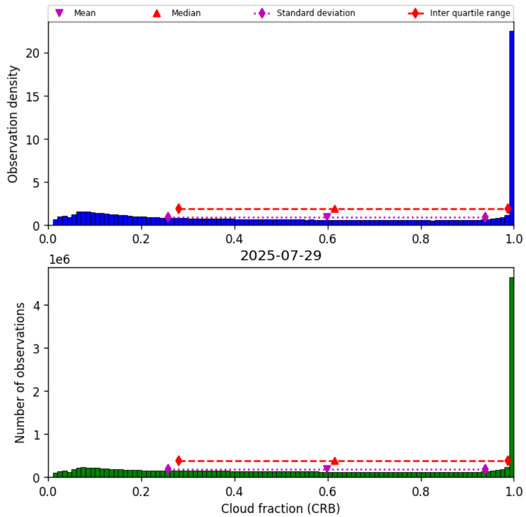
Figure 40: Histogram of “Cloud fraction (CRB)” for 2025-07-29 to 2025-07-30
