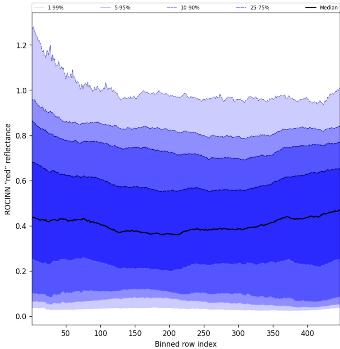
Figure 67: Along track statistics of "ROCINN "red" reflectance" for 2025-07-29 to 2025-07-30
