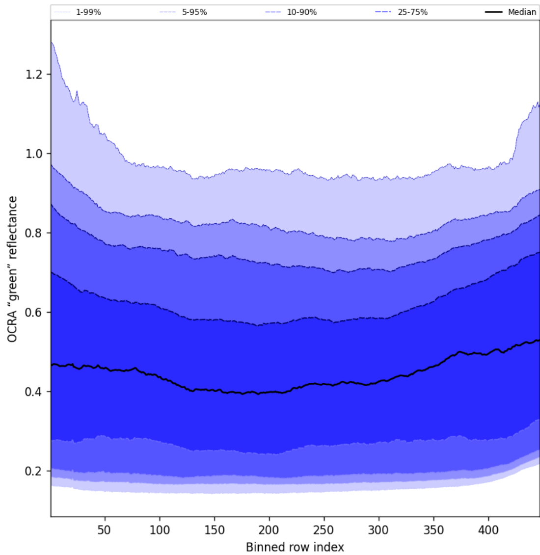
Figure 66: Along track statistics of “OCRA “green” reflectance” for 2025-07-29 to 2025-07-30
