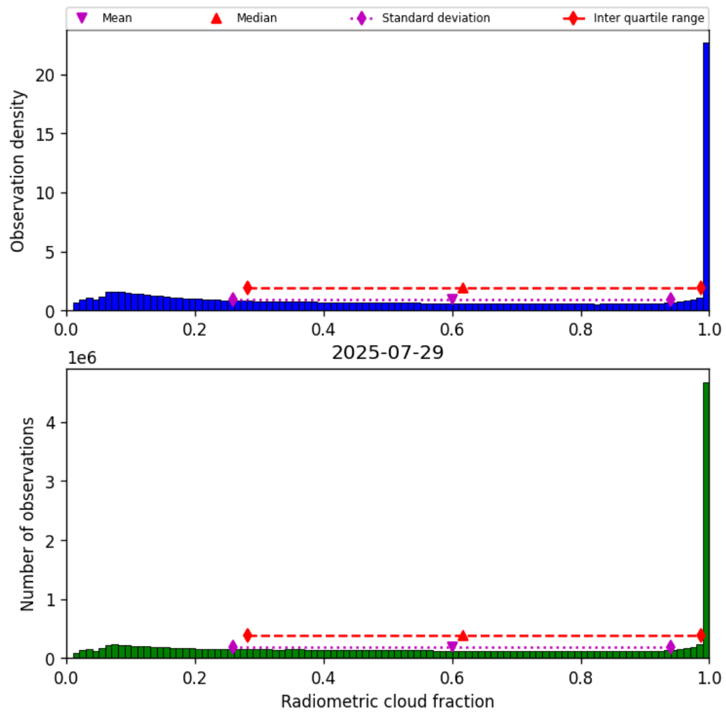
Figure 37: Histogram of “Radiometric cloud fraction” for 2025-07-29 to 2025-07-30
