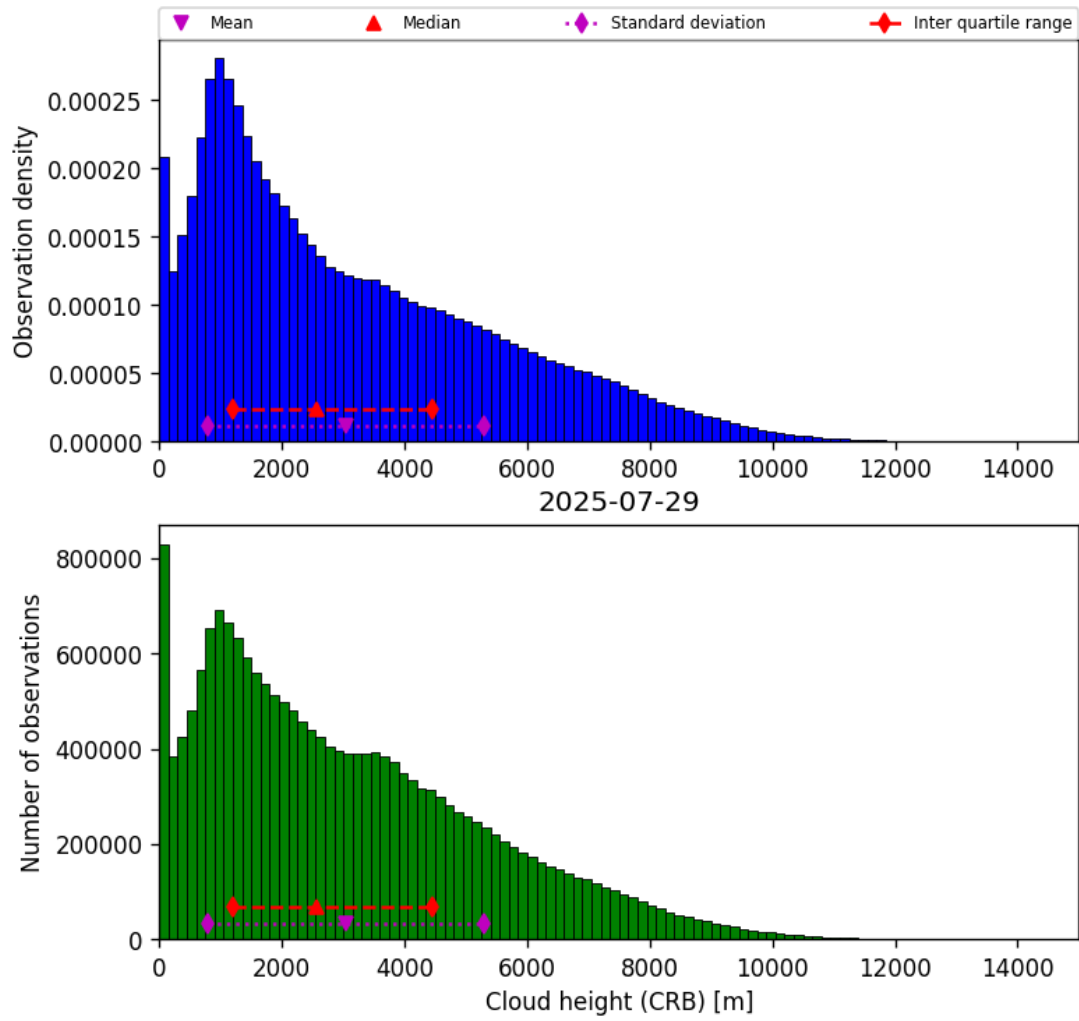
Figure 41: Histogram of “Cloud height (CRB)” for 2025-07-29 to 2025-07-30
