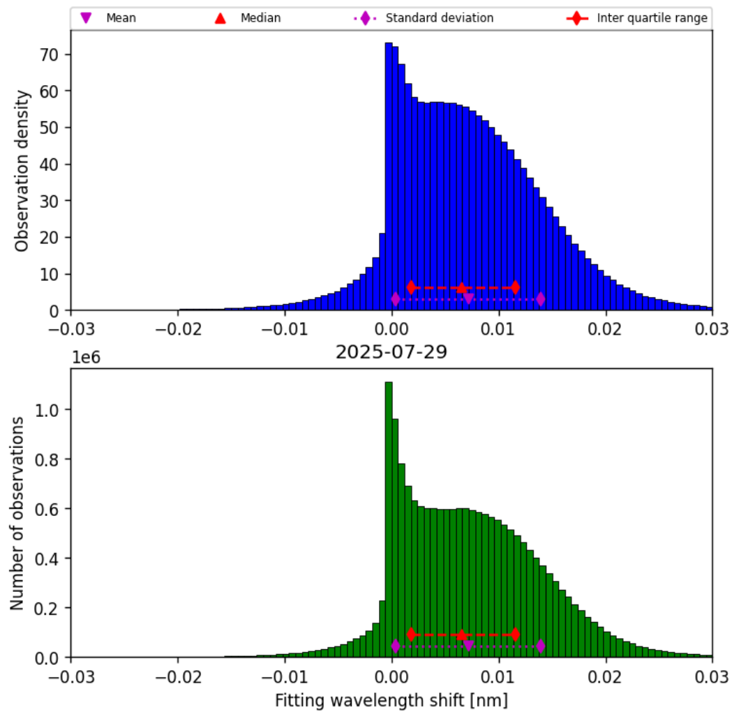
Figure 47: Histogram of “Fitting wavelength shift” for 2025-07-29 to 2025-07-30
