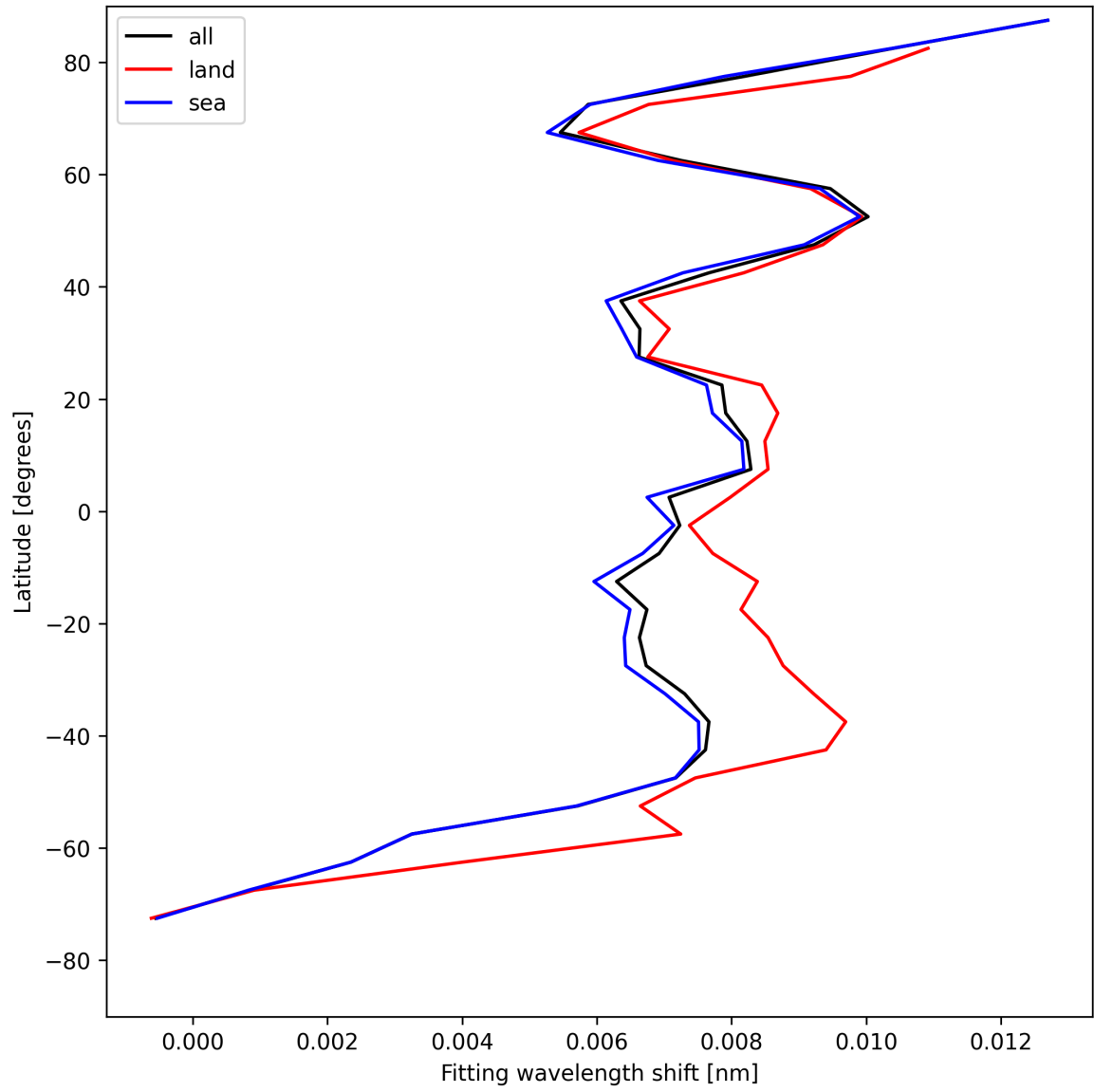
Figure 31: Zonal average of “Fitting wavelength shift” for 2025-07-29 to 2025-07-30.
