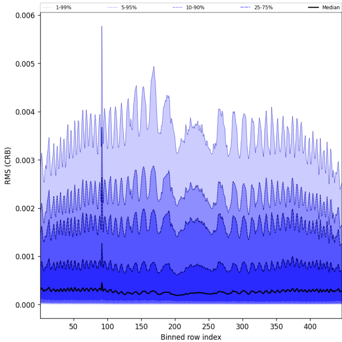
Figure 62: Along track statistics of “RMS (CRB)” for 2025-07-29 to 2025-07-30
