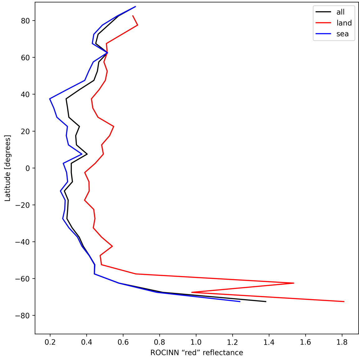
Figure 35: Zonal average of “ROCINN “red” reflectance” for 2025-07-29 to 2025-07-30.
