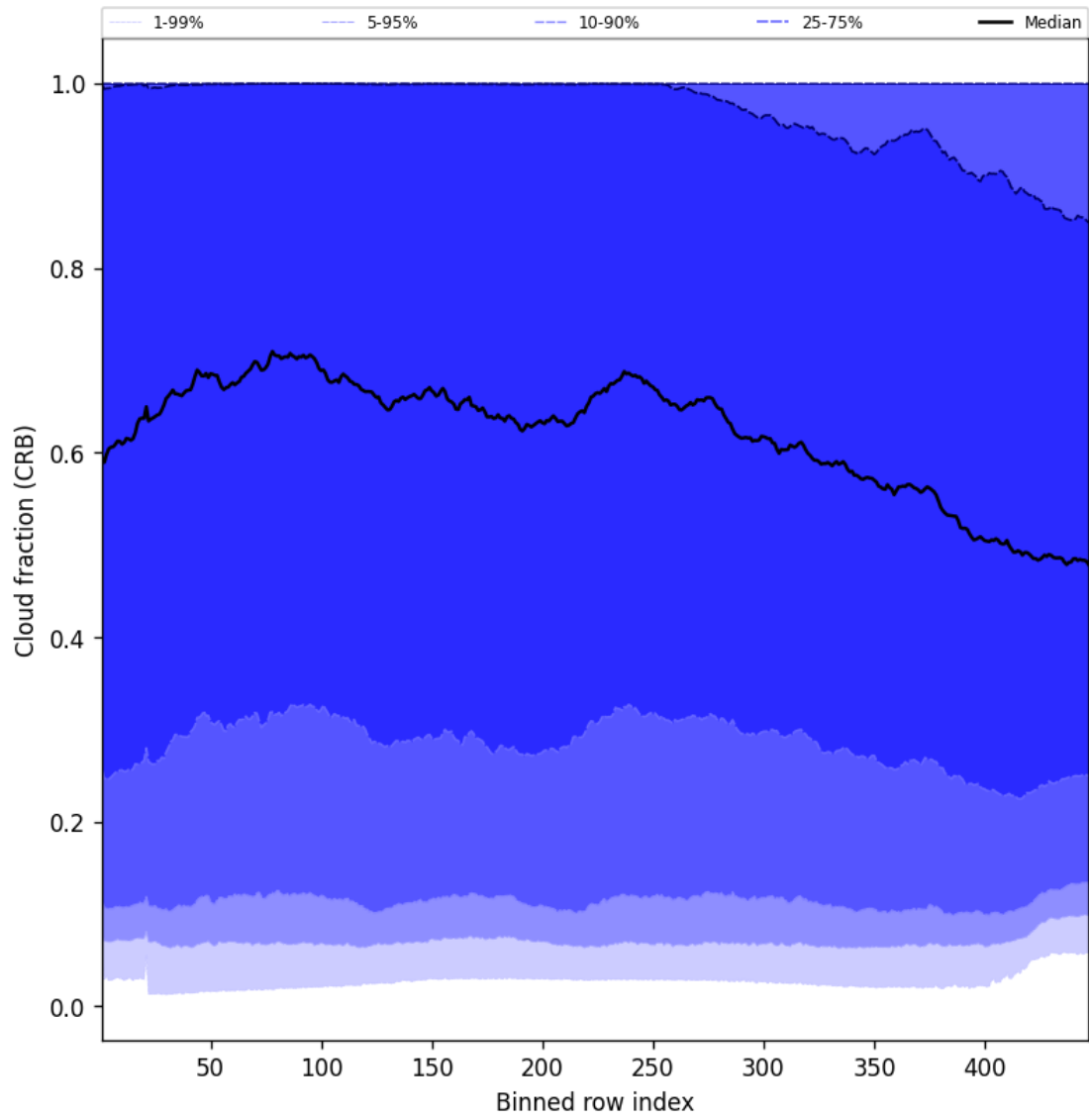
Figure 56: Along track statistics of “Cloud fraction (CRB)” for 2025-07-29 to 2025-07-30
