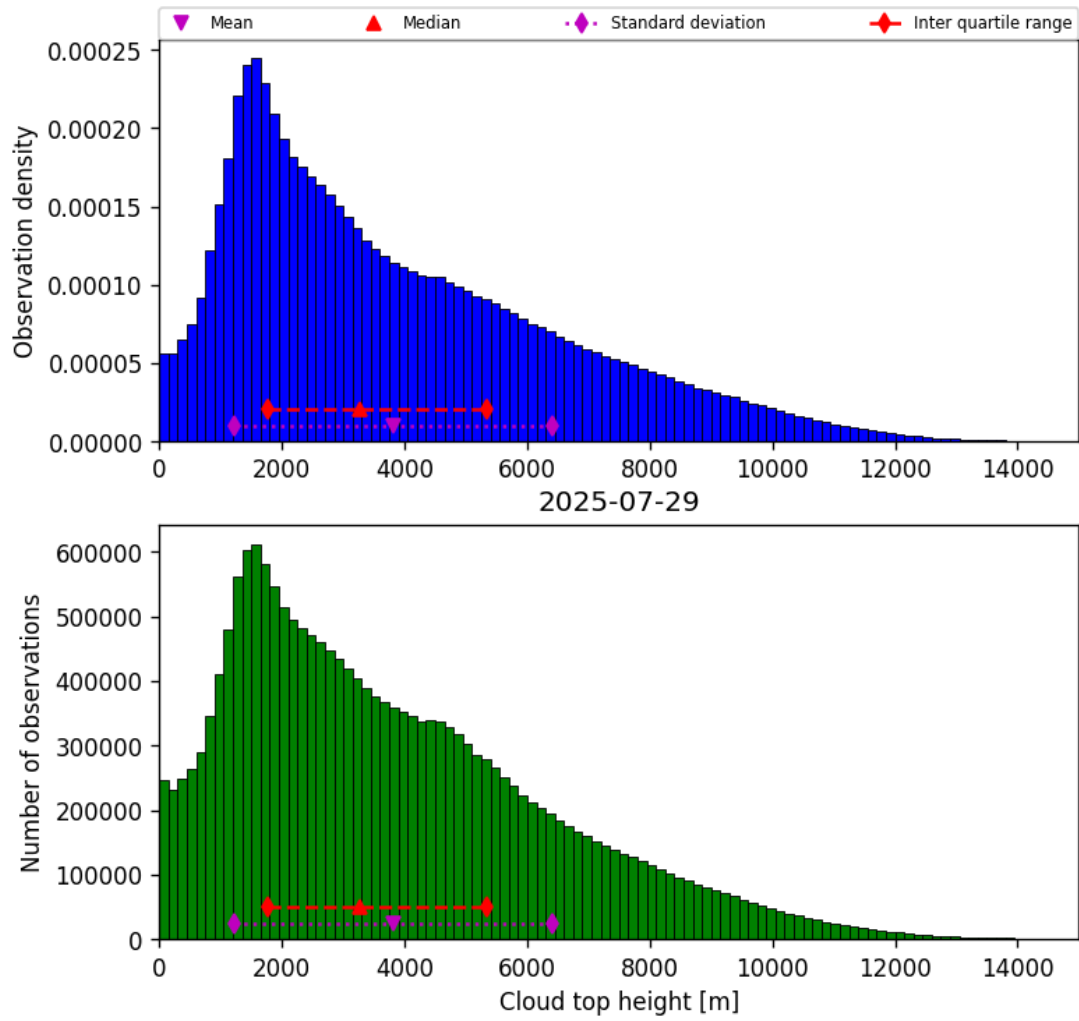
Figure 38: Histogram of “Cloud top height” for 2025-07-29 to 2025-07-30
