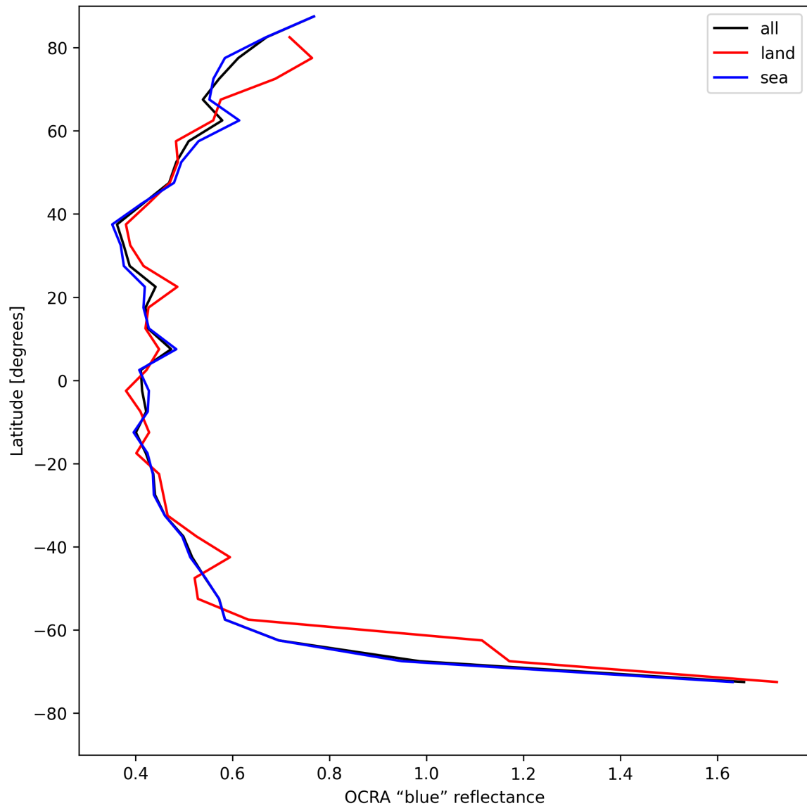
Figure 33: Zonal average of “OCRA “blue” reflectance” for 2025-07-29 to 2025-07-30.
