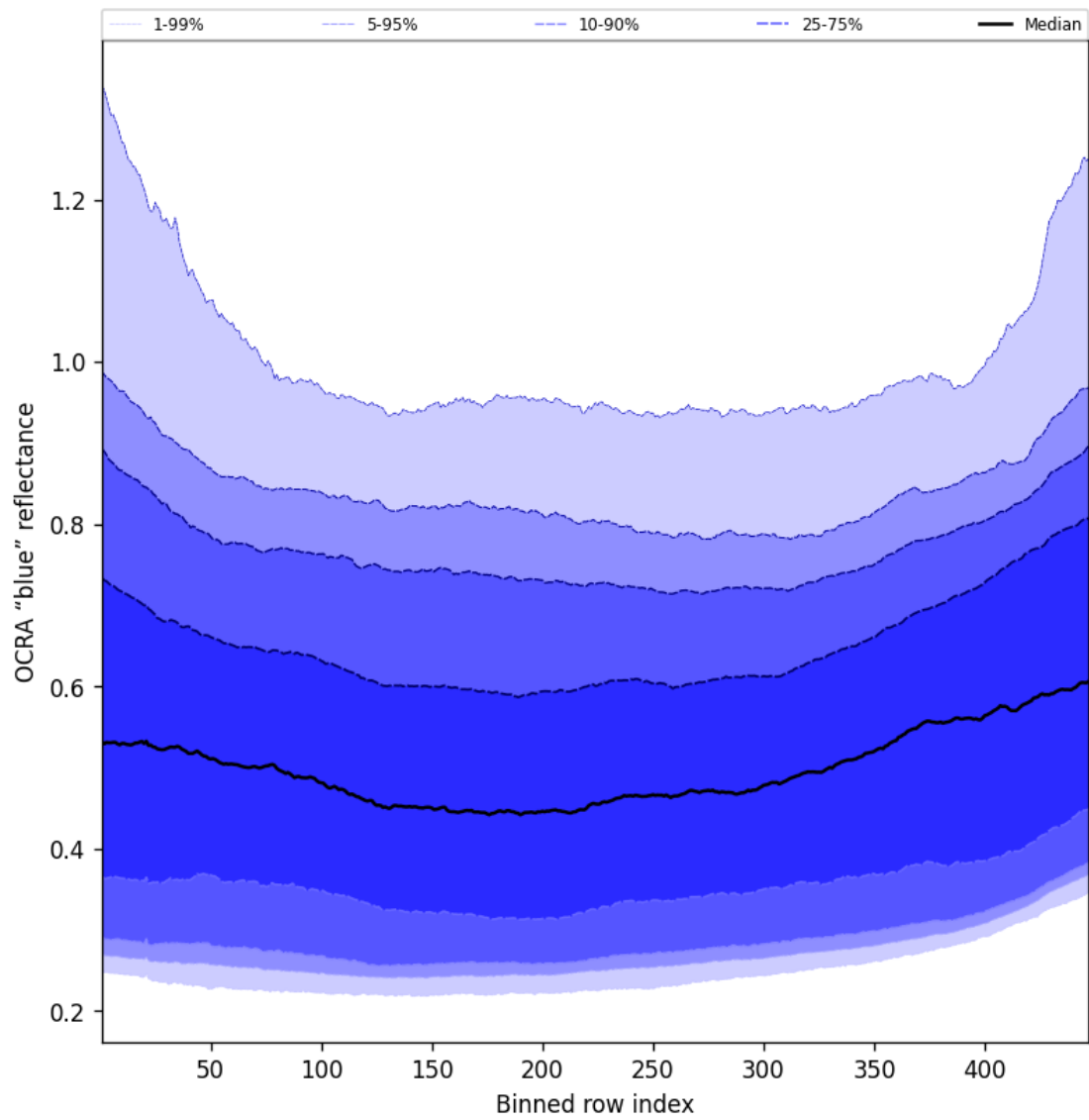
Figure 65: Along track statistics of “OCRA “blue” reflectance” for 2025-07-29 to 2025-07-30
