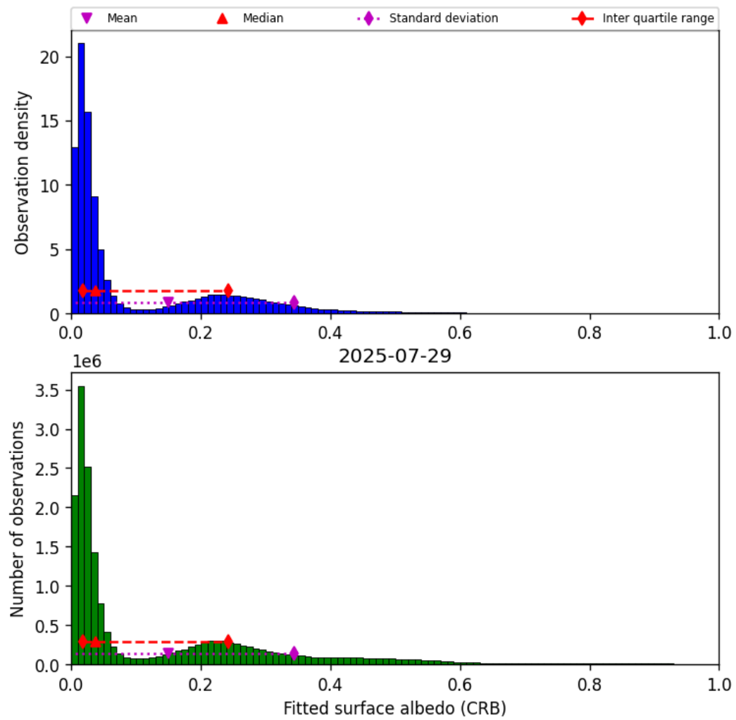
Figure 44: Histogram of “Fitted surface albedo (CRB)” for 2025-07-29 to 2025-07-30
