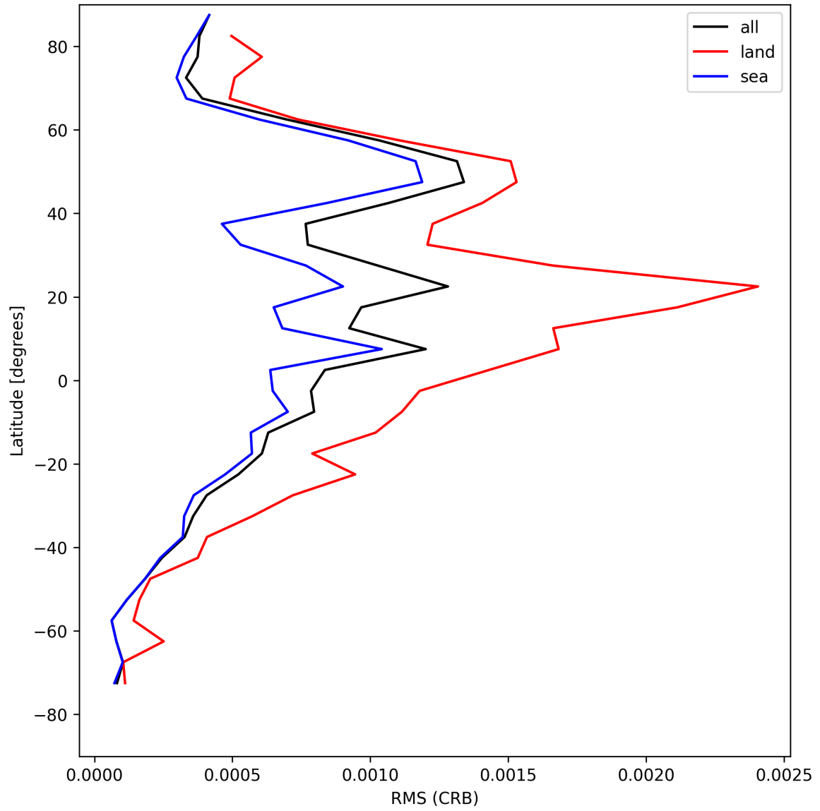
Figure 30: Zonal average of “RMS (CRB)” for 2025-07-29 to 2025-07-30.
