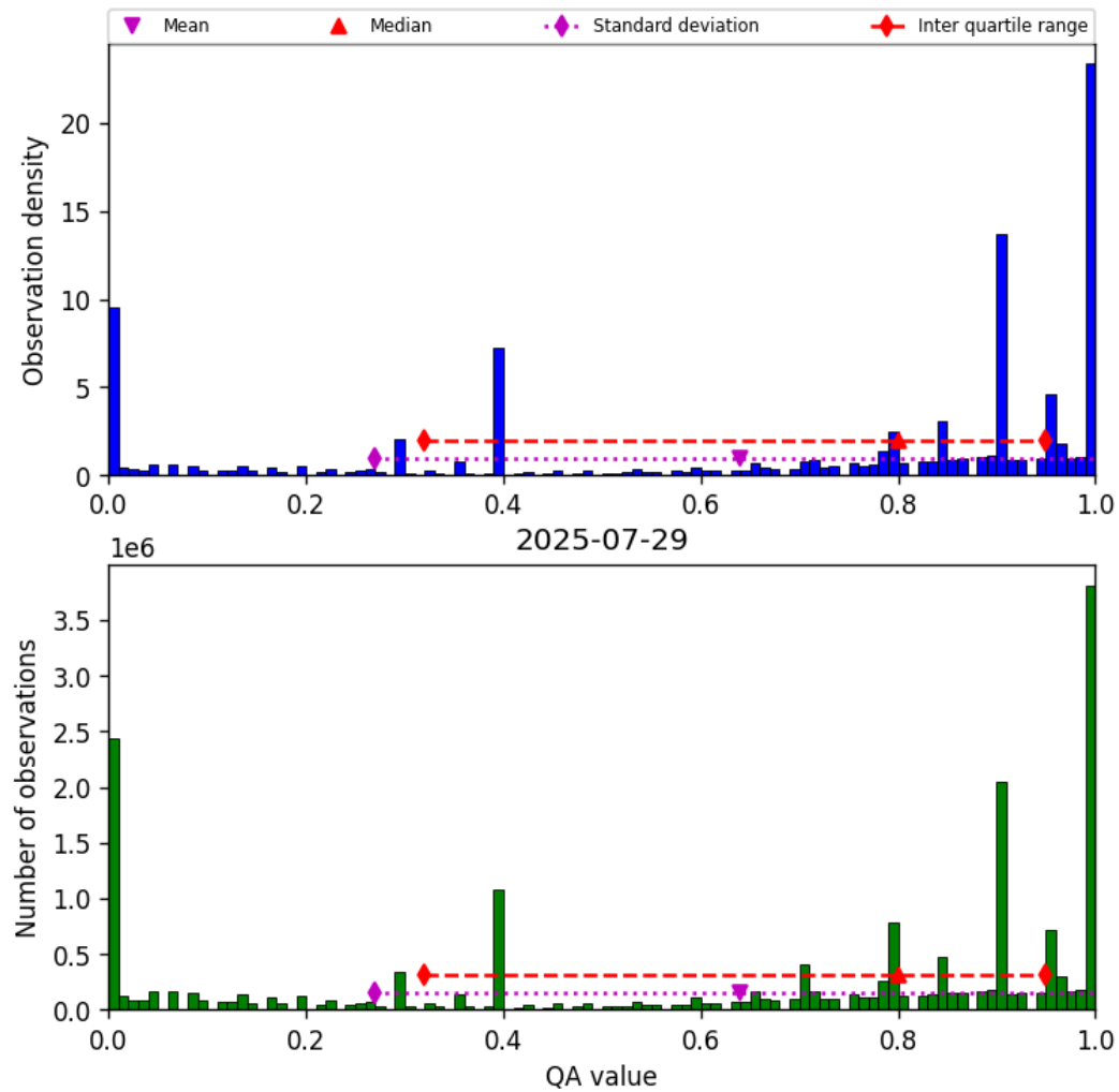
Figure 36: Histogram of “QA value” for 2025-07-29 to 2025-07-30
