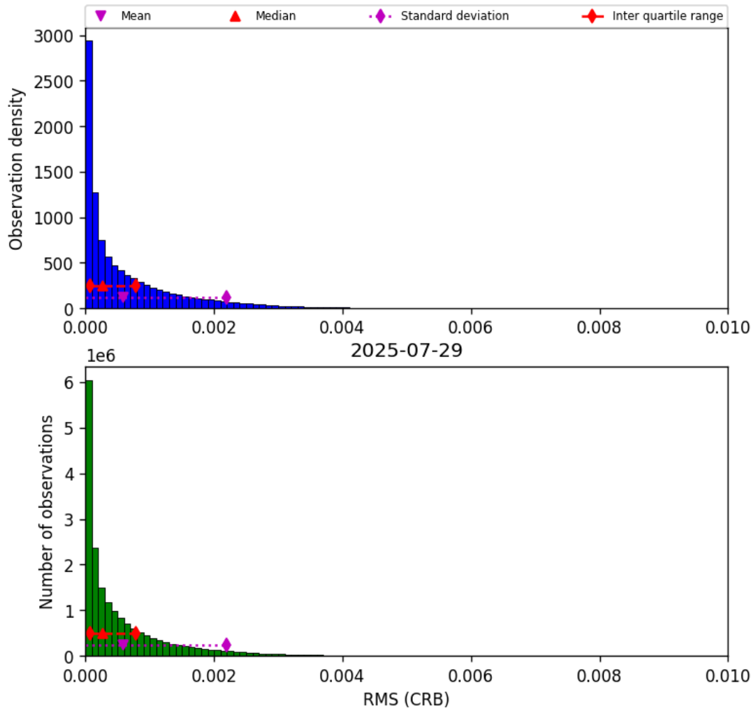
Figure 46: Histogram of “RMS (CRB)” for 2025-07-29 to 2025-07-30
