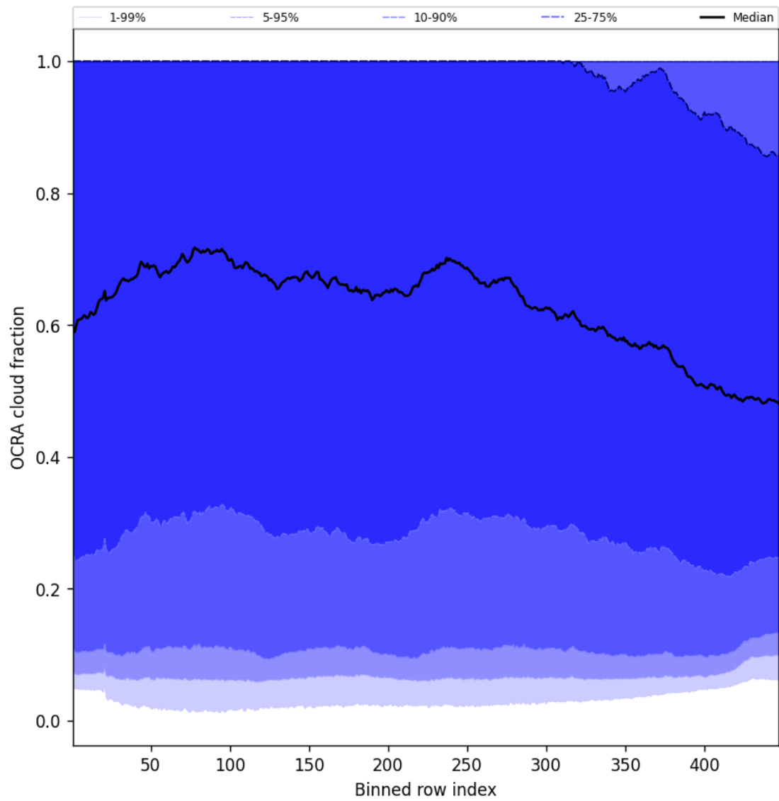
Figure 64: Along track statistics of “OCRA cloud fraction” for 2025-07-29 to 2025-07-30
