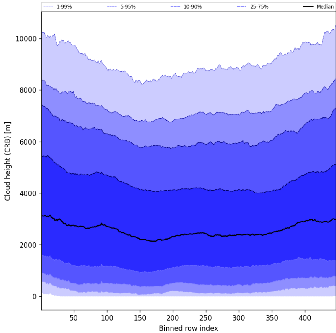
Figure 57: Along track statistics of “Cloud height (CRB)” for 2025-07-29 to 2025-07-30
