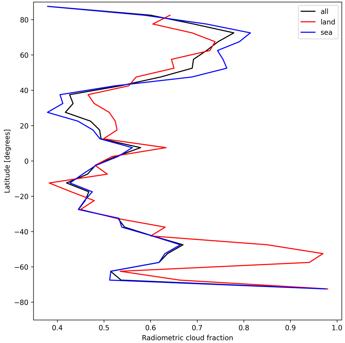
Figure 21: Zonal average of “Radiometric cloud fraction” for 2025-07-30 to 2025-07-31.
