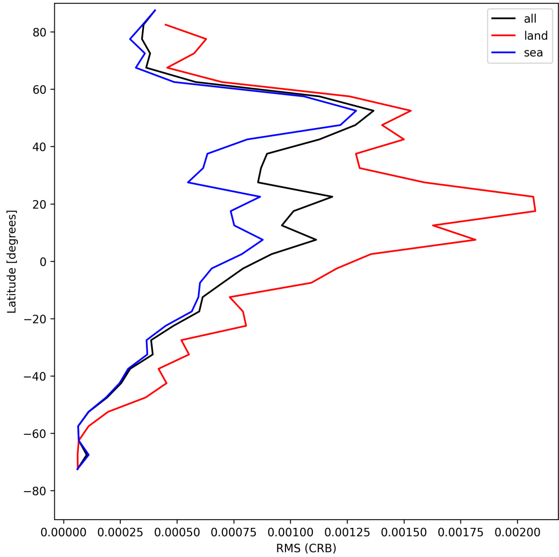
Figure 30: Zonal average of “RMS (CRB)” for 2025-07-30 to 2025-07-31.
