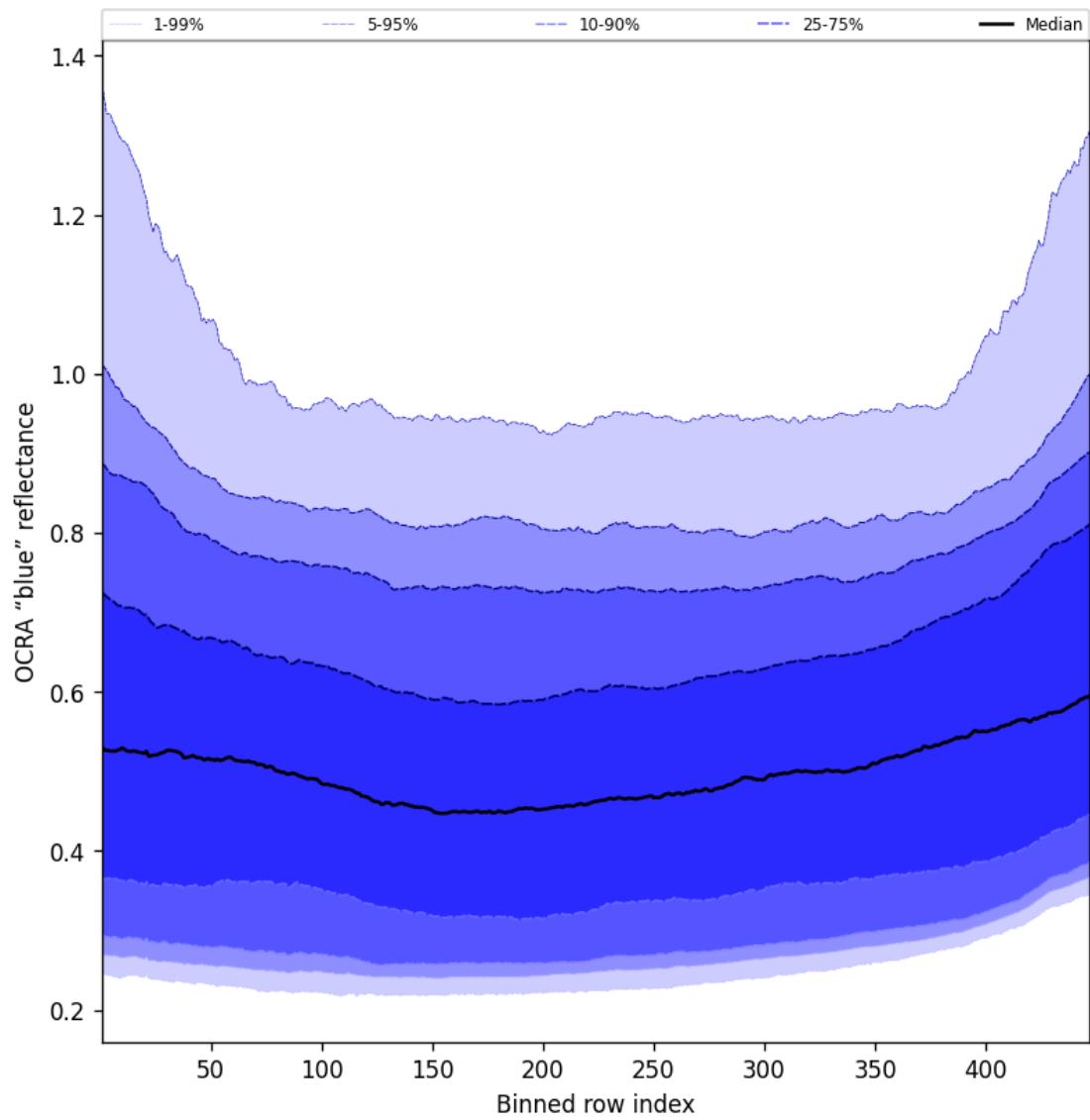
Figure 65: Along track statistics of “OCRA “blue” reflectance” for 2025-07-30 to 2025-07-31
