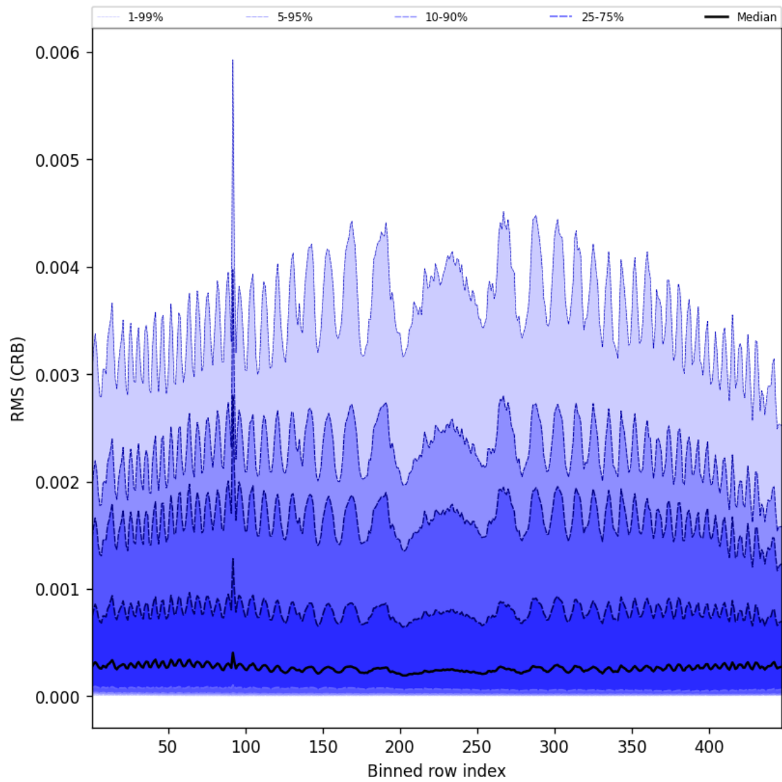
Figure 62: Along track statistics of “RMS (CRB)” for 2025-07-30 to 2025-07-31
