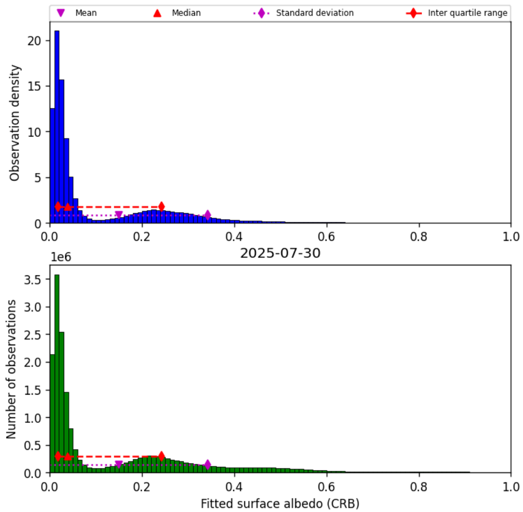
Figure 44: Histogram of "Fitted surface albedo (CRB)" for 2025-07-30 to 2025-07-31
