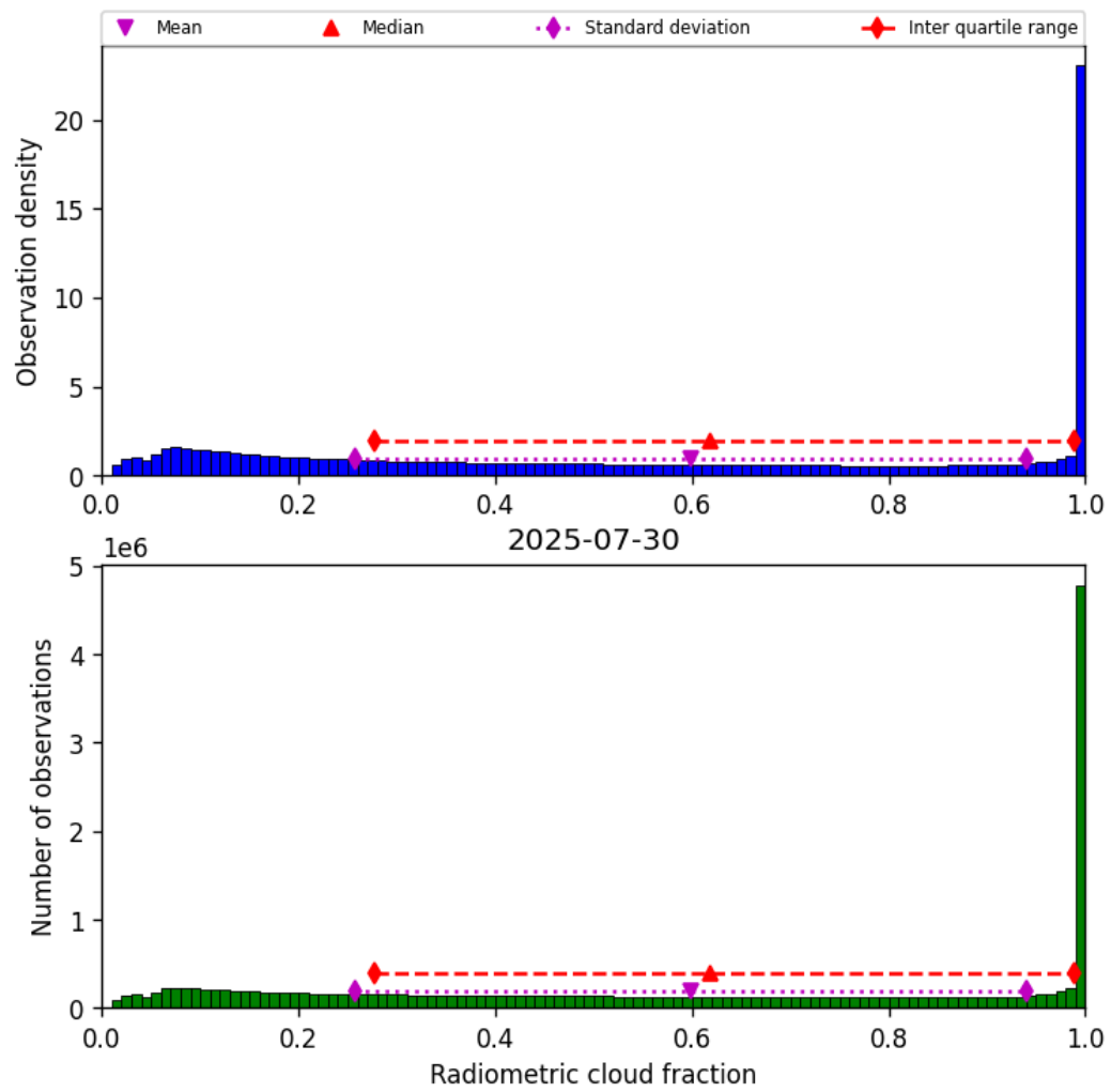
Figure 37: Histogram of “Radiometric cloud fraction” for 2025-07-30 to 2025-07-31
