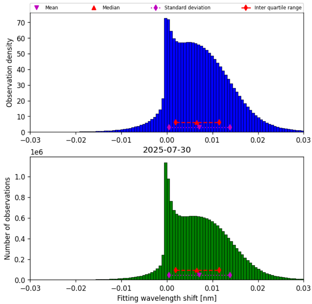
Figure 47: Histogram of “Fitting wavelength shift” for 2025-07-30 to 2025-07-31
