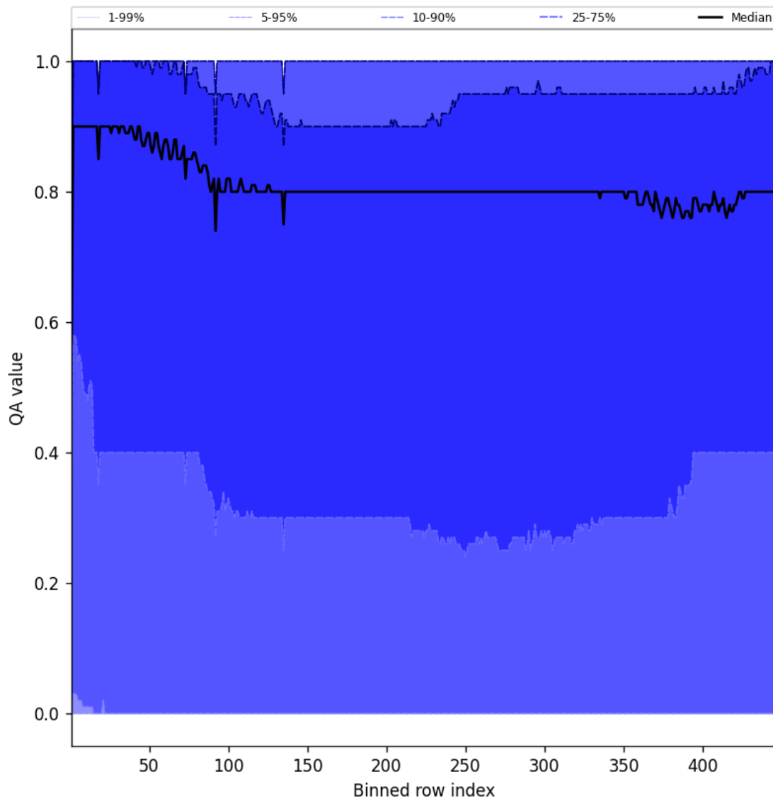
Figure 52: Along track statistics of “QA value” for 2025-07-30 to 2025-07-31
