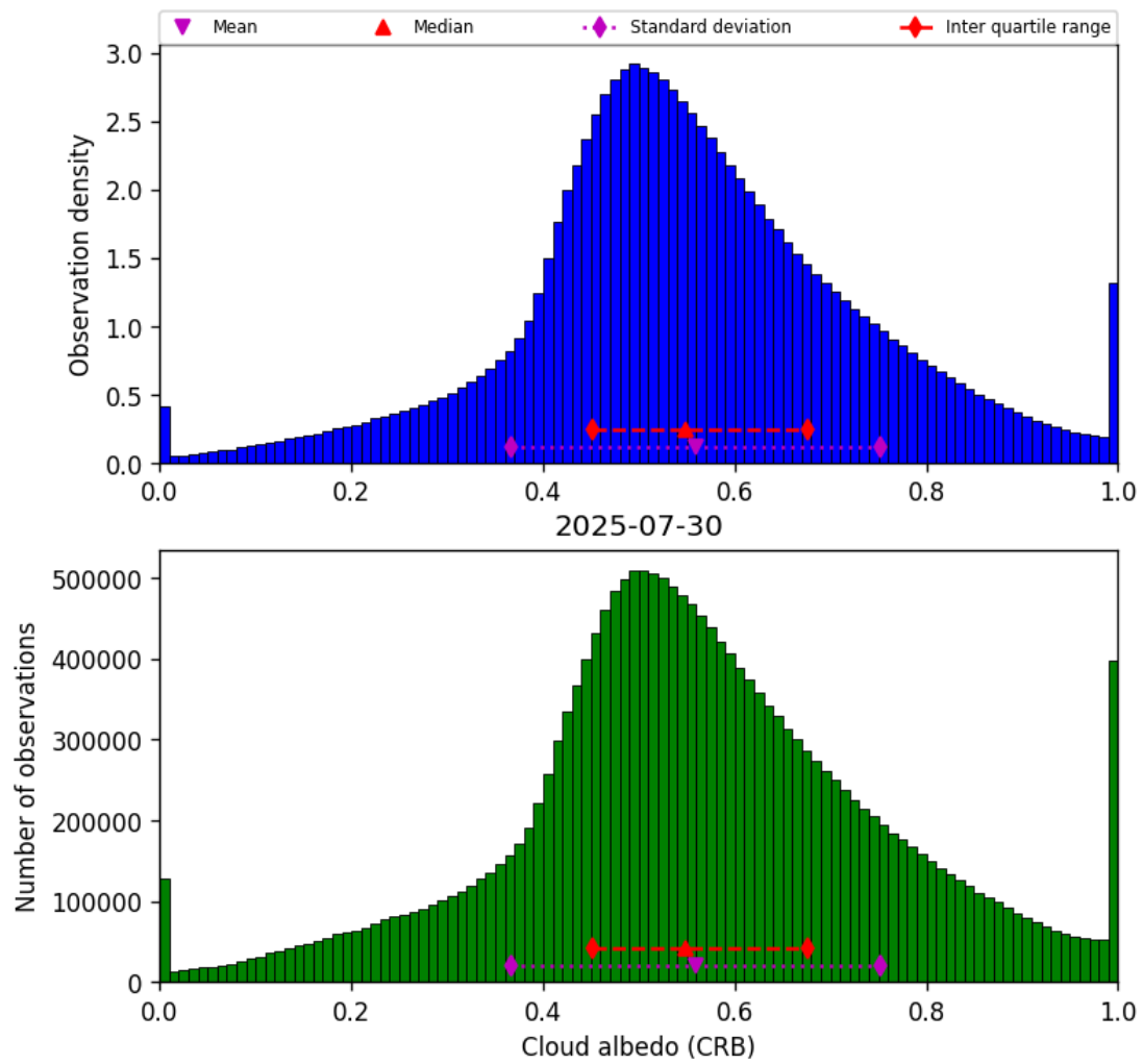
Figure 42: Histogram of “Cloud albedo (CRB)” for 2025-07-30 to 2025-07-31
