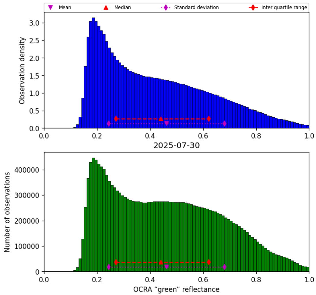
Figure 50: Histogram of “OCRA “green” reflectance” for 2025-07-30 to 2025-07-31
