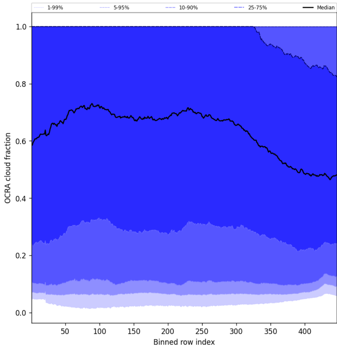
Figure 64: Along track statistics of “OCRA cloud fraction” for 2025-07-30 to 2025-07-31
