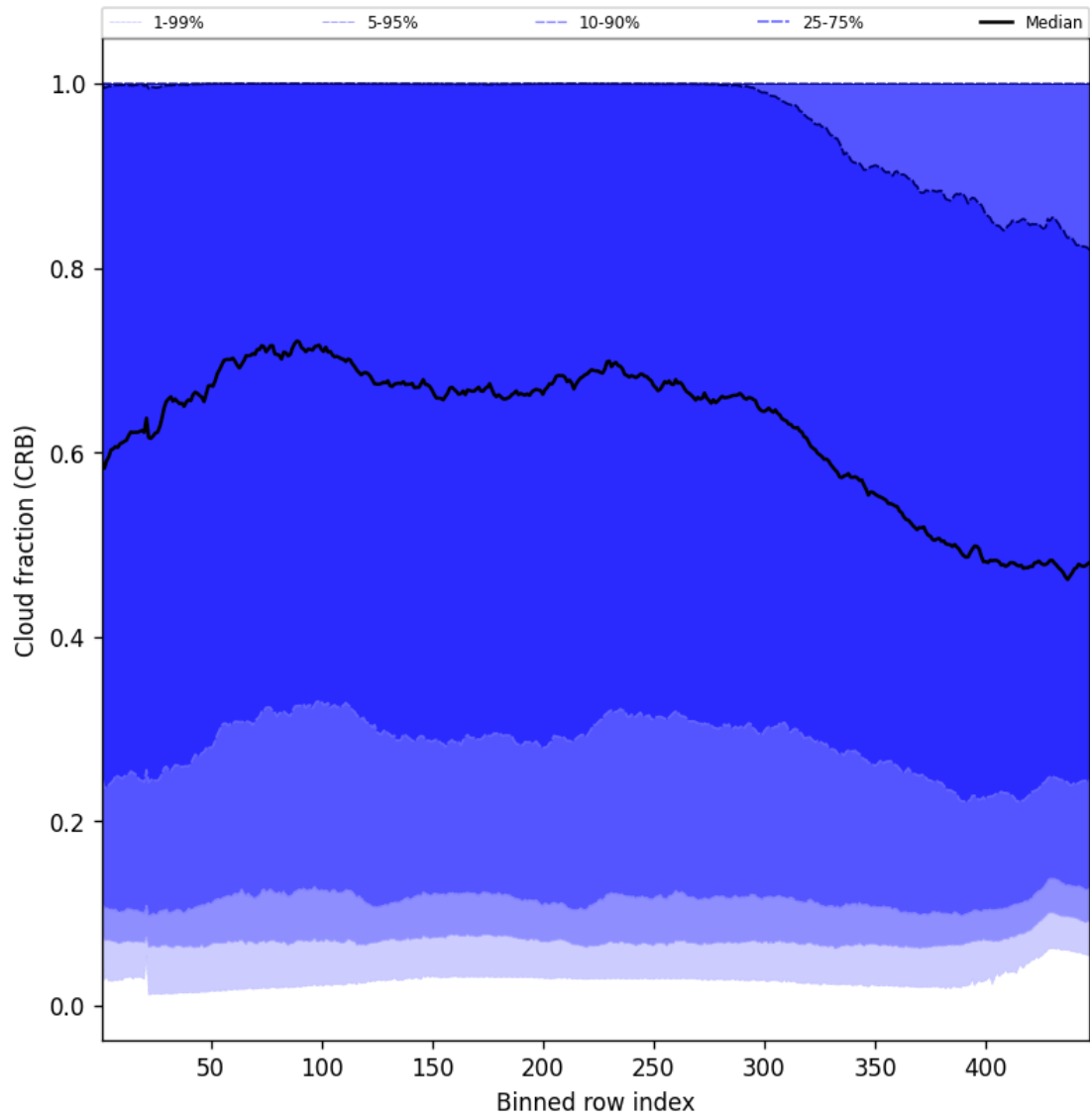
Figure 56: Along track statistics of “Cloud fraction (CRB)” for 2025-07-30 to 2025-07-31
