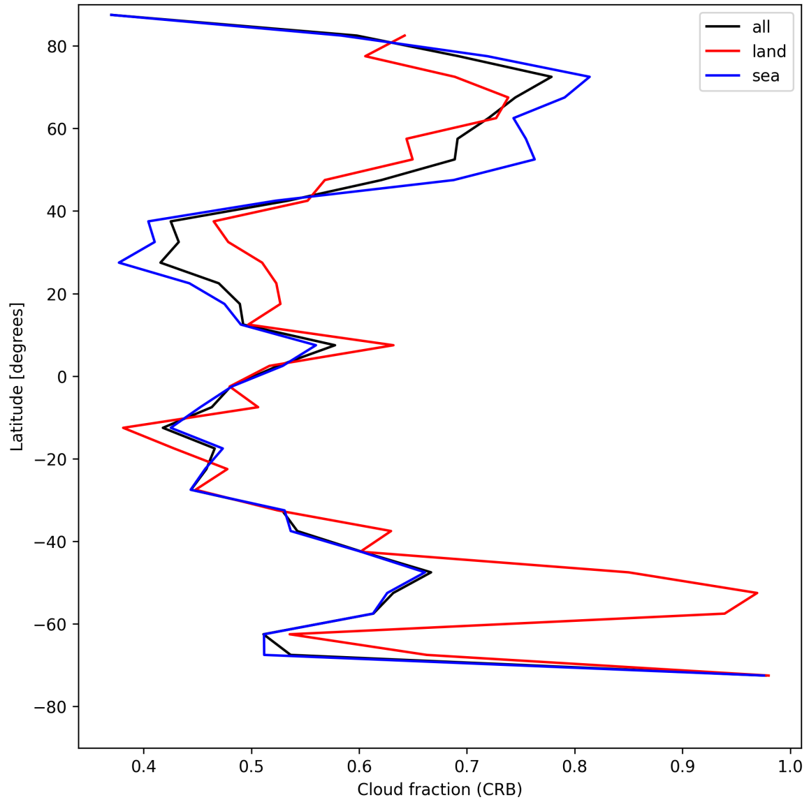
Figure 24: Zonal average of “Cloud fraction (CRB)” for 2025-07-30 to 2025-07-31.
