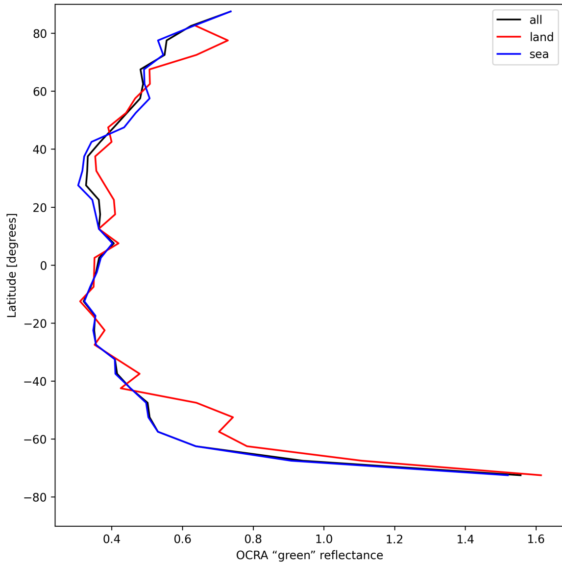
Figure 34: Zonal average of “OCRA “green” reflectance” for 2025-07-30 to 2025-07-31.
