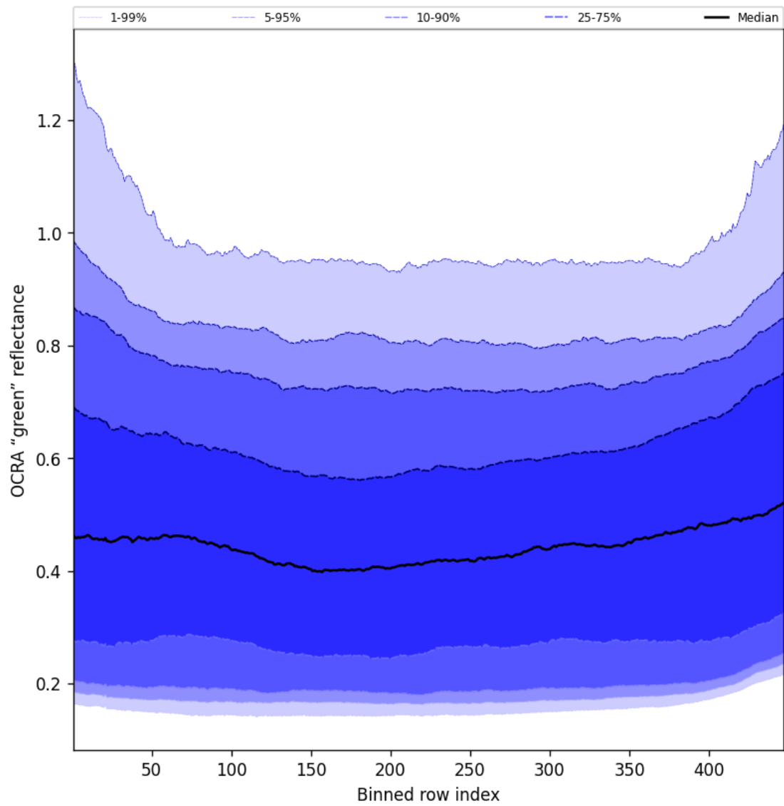
Figure 66: Along track statistics of "OCRA "green" reflectance" for 2025-07-30 to 2025-07-31
