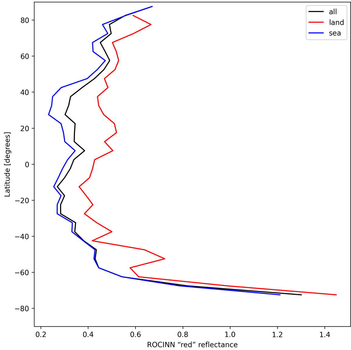
Figure 35: Zonal average of “ROCINN “red” reflectance” for 2025-07-30 to 2025-07-31.
