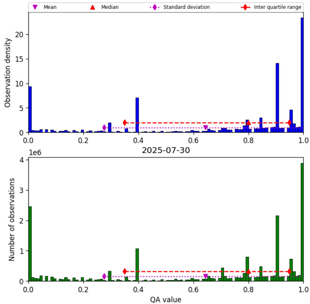
Figure 36: Histogram of “QA value” for 2025-07-30 to 2025-07-31
