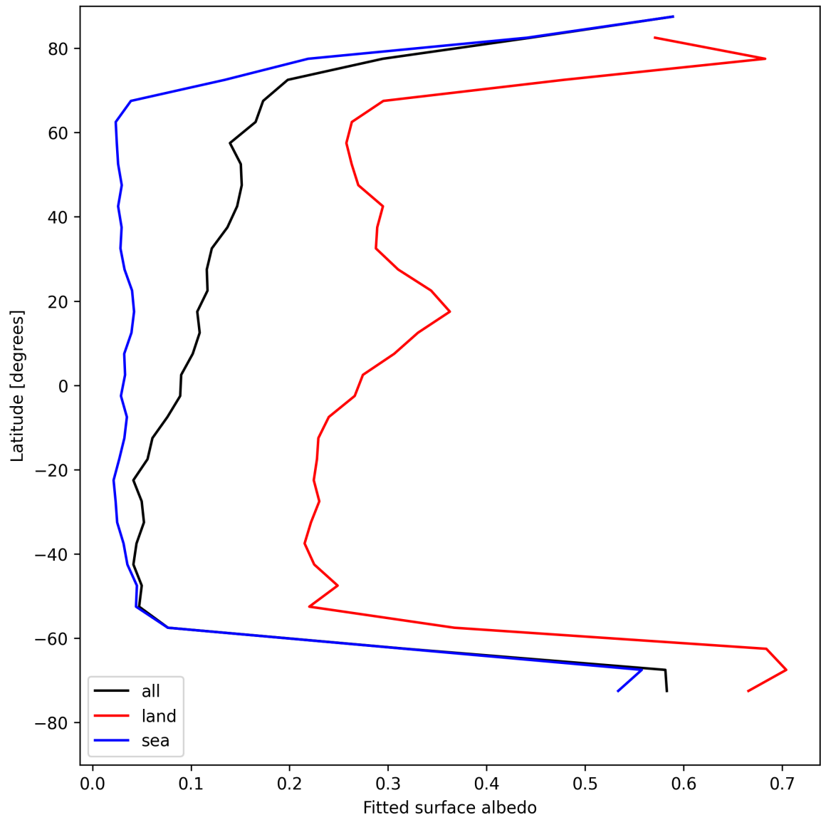
Figure 27: Zonal average of “Fitted surface albedo” for 2025-07-30 to 2025-07-31.
