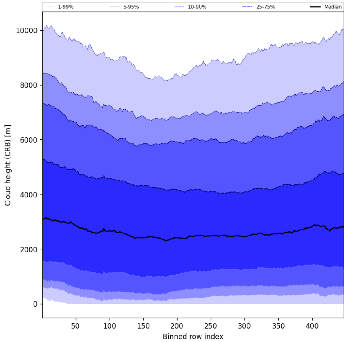
Figure 57: Along track statistics of “Cloud height (CRB)” for 2025-07-30 to 2025-07-31
