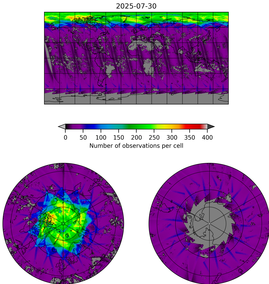
Figure 19: Map of the number of observations for 2025-07-30 to 2025-07-31
