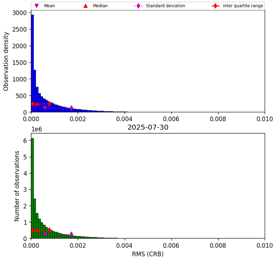
Figure 46: Histogram of “RMS (CRB)” for 2025-07-30 to 2025-07-31
