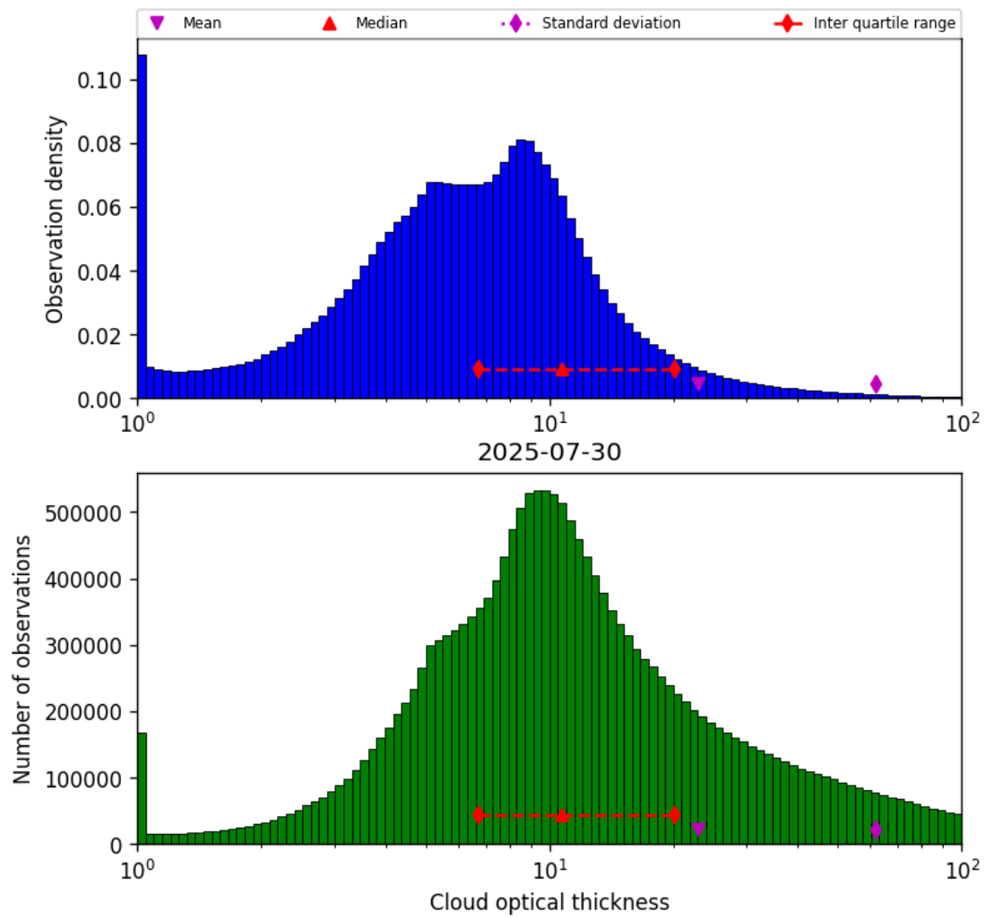
Figure 39: Histogram of “Cloud optical thickness” for 2025-07-30 to 2025-07-31
