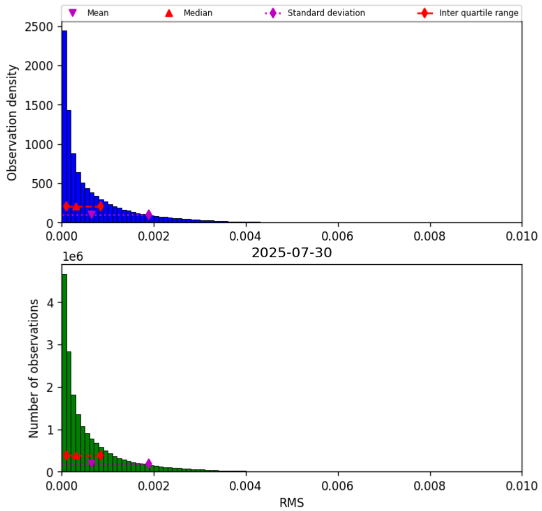
Figure 45: Histogram of “RMS” for 2025-07-30 to 2025-07-31
