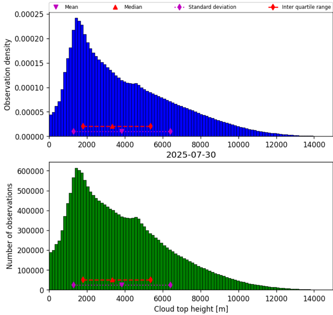
Figure 38: Histogram of “Cloud top height” for 2025-07-30 to 2025-07-31
