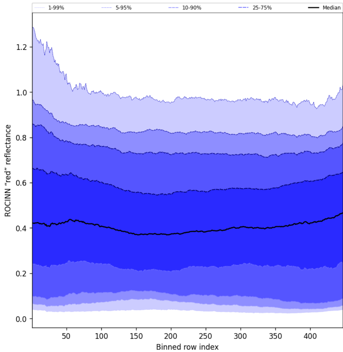
Figure 67: Along track statistics of "ROCINN "red" reflectance" for 2025-07-30 to 2025-07-31
