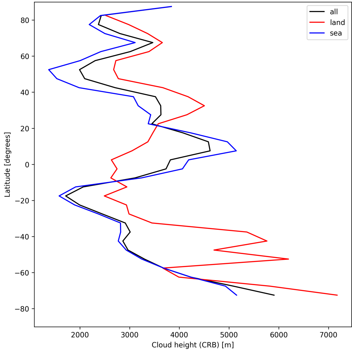
Figure 25: Zonal average of “Cloud height (CRB)” for 2025-07-30 to 2025-07-31.
