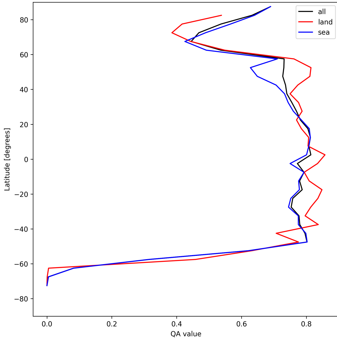
Figure 20: Zonal average of “QA value” for 2025-07-30 to 2025-07-31.
