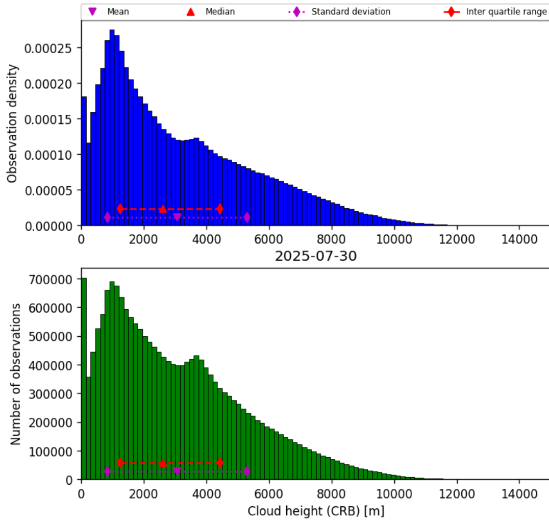
Figure 41: Histogram of “Cloud height (CRB)” for 2025-07-30 to 2025-07-31
