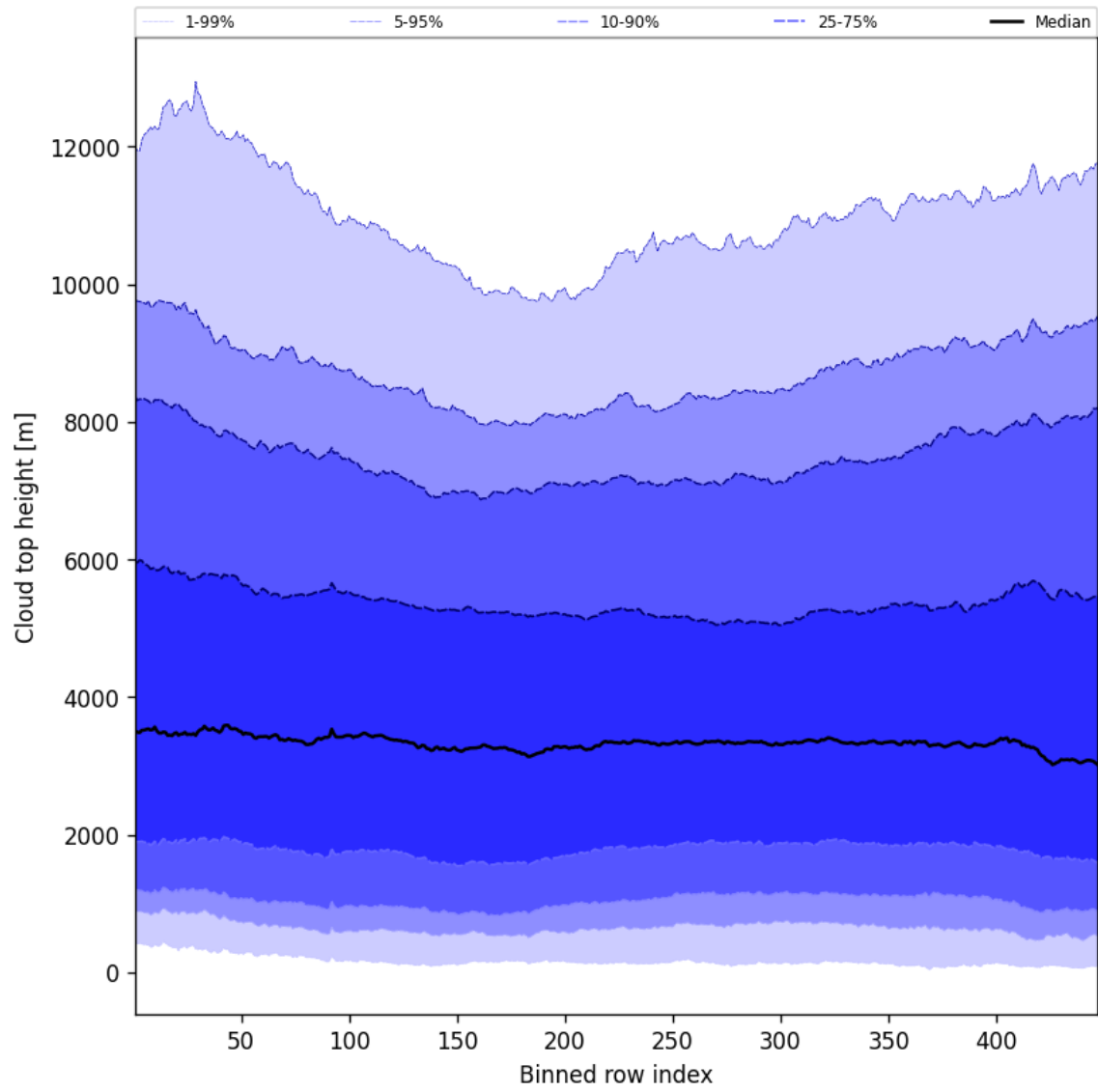
Figure 54: Along track statistics of “Cloud top height” for 2025-07-30 to 2025-07-31
