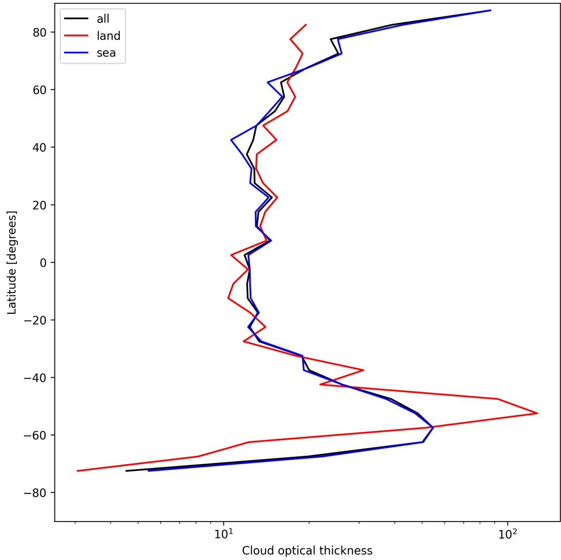
Figure 23: Zonal average of “Cloud optical thickness” for 2025-07-30 to 2025-07-31.
