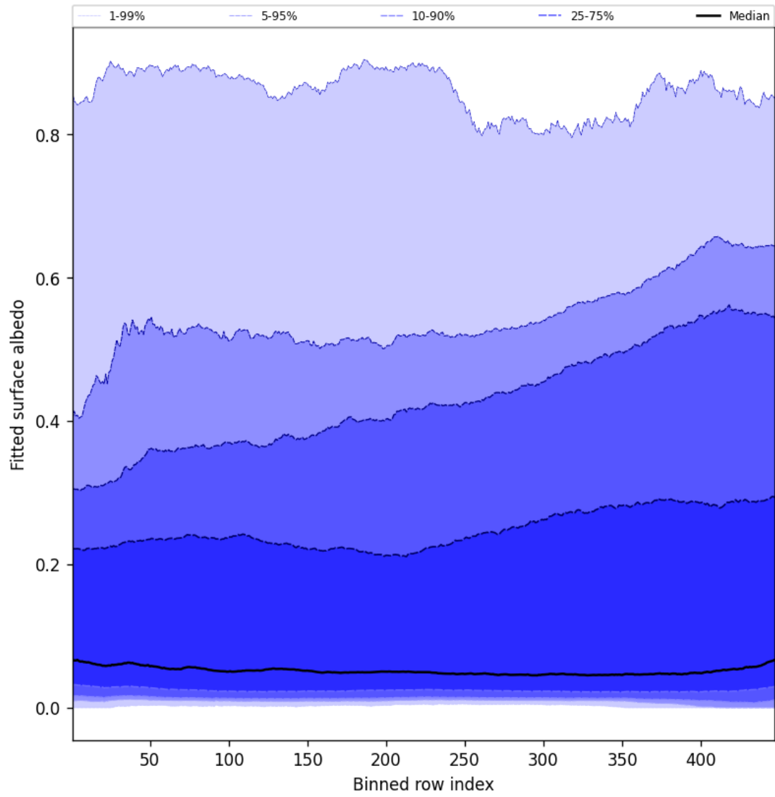
Figure 59: Along track statistics of “Fitted surface albedo” for 2025-07-30 to 2025-07-31
