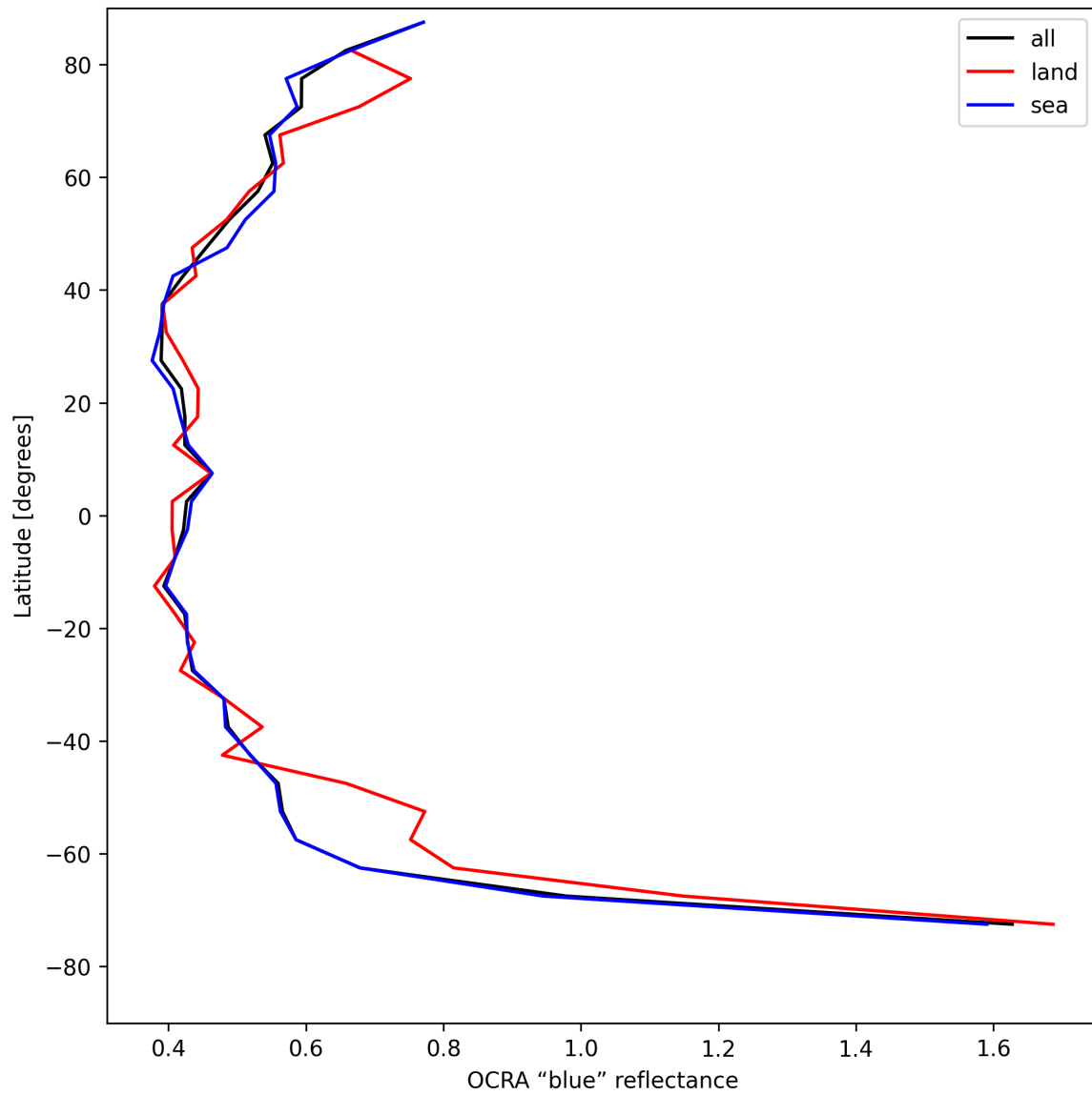
Figure 33: Zonal average of “OCRA “blue” reflectance” for 2025-07-30 to 2025-07-31.
