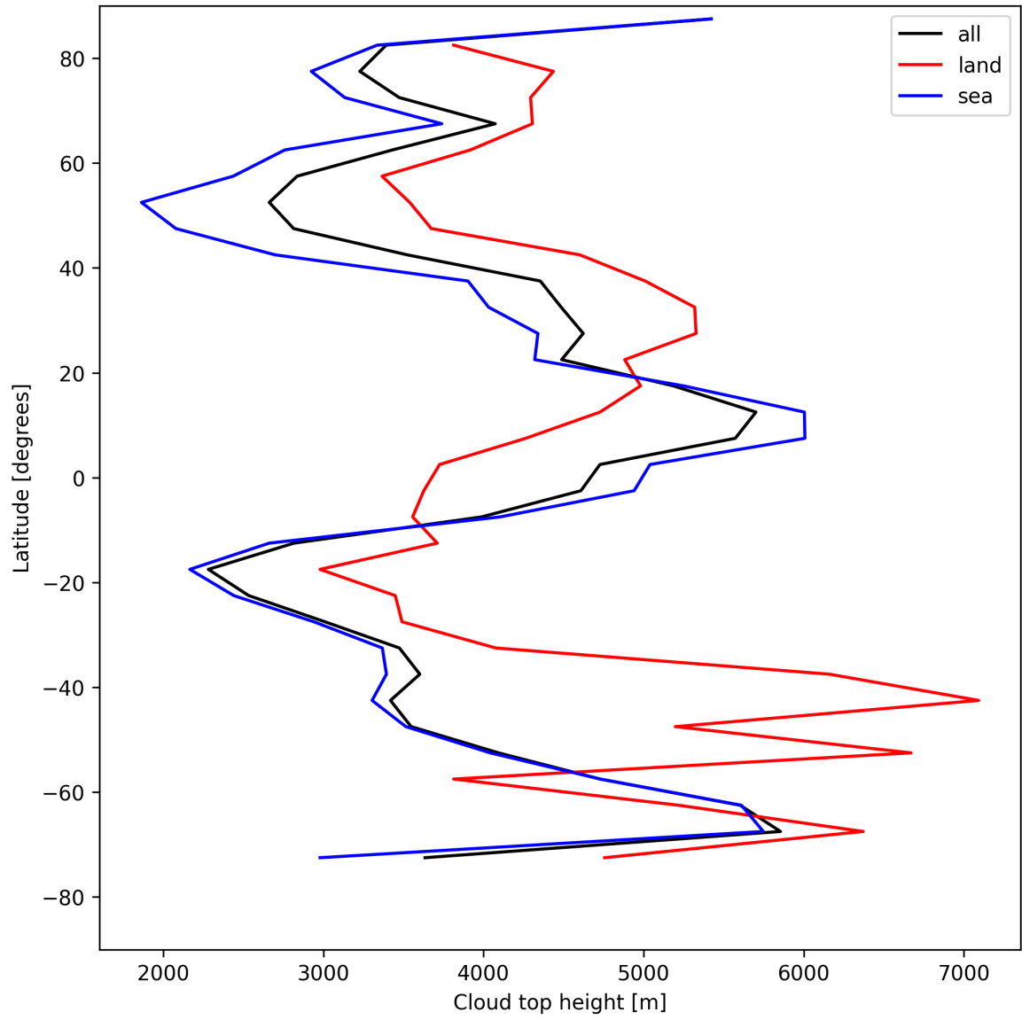
Figure 22: Zonal average of “Cloud top height” for 2025-07-30 to 2025-07-31.
