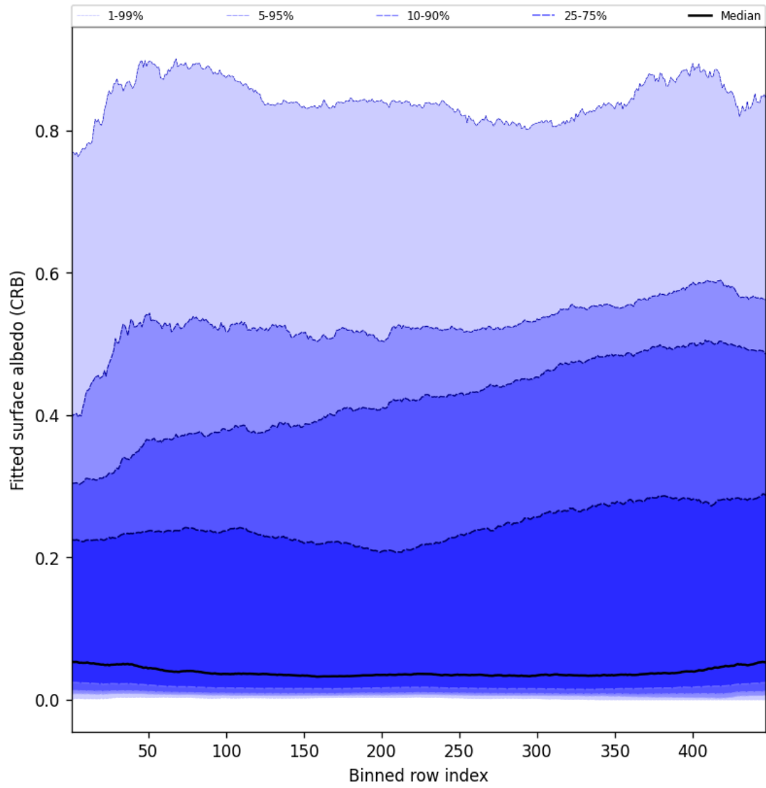
Figure 60: Along track statistics of “Fitted surface albedo (CRB)” for 2025-07-30 to 2025-07-31
