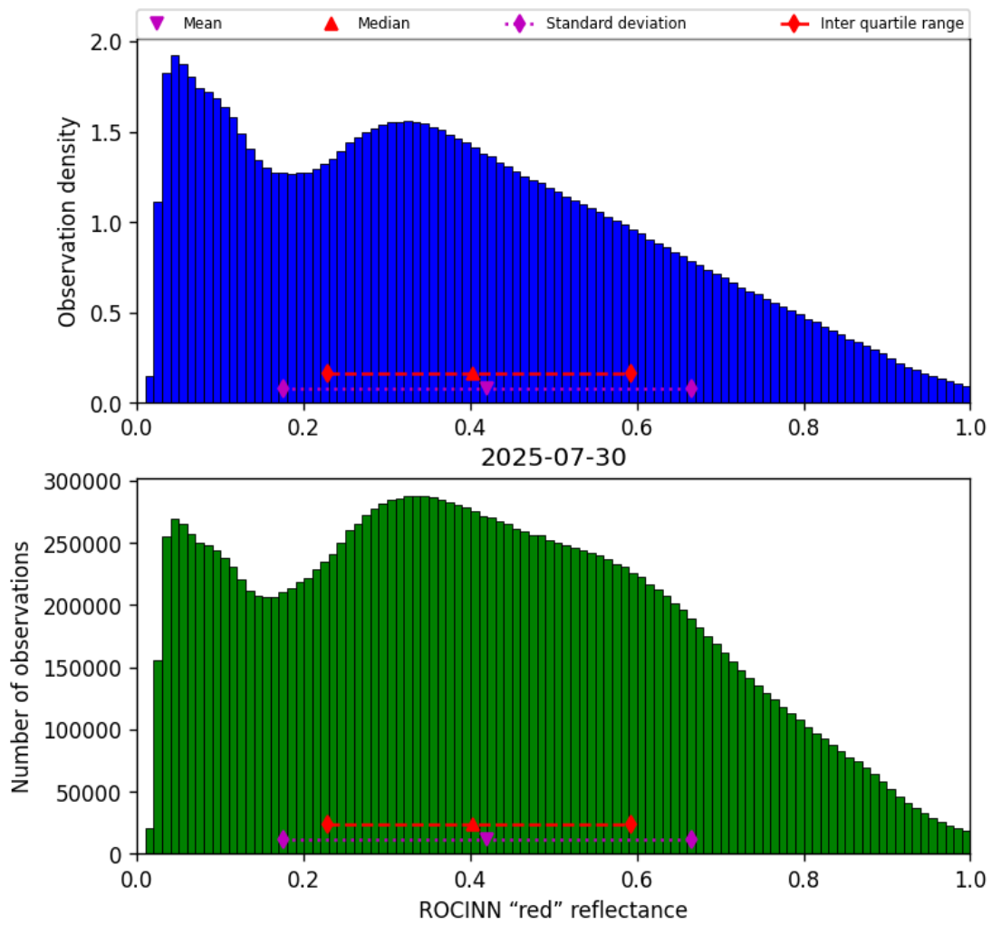
Figure 51: Histogram of “ROCINN “red” reflectance” for 2025-07-30 to 2025-07-31
