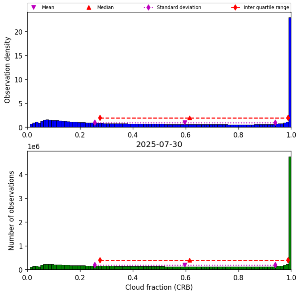
Figure 40: Histogram of “Cloud fraction (CRB)” for 2025-07-30 to 2025-07-31
