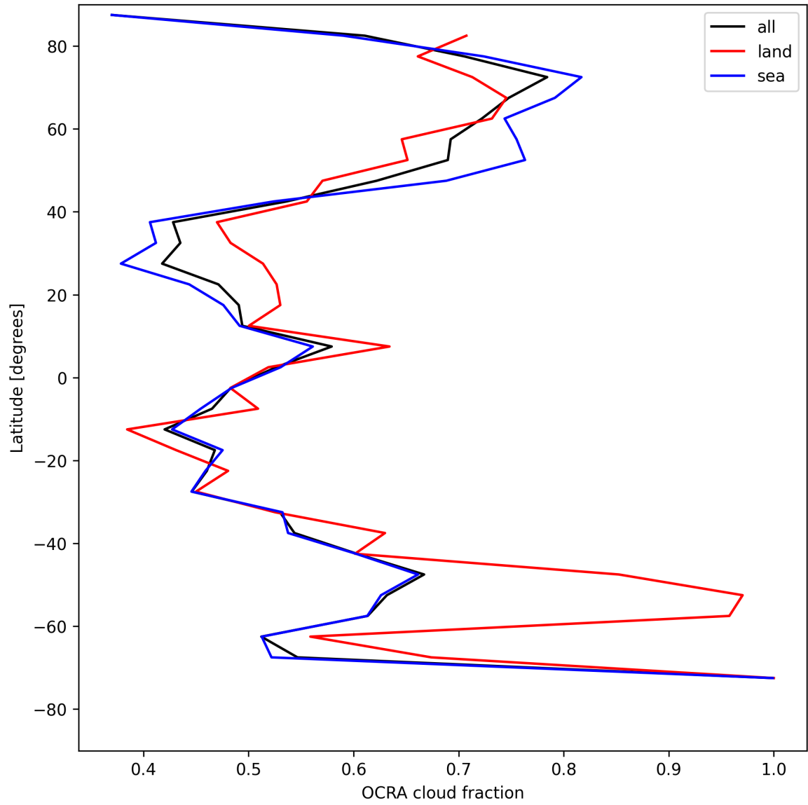
Figure 32: Zonal average of “OCRA cloud fraction” for 2025-07-30 to 2025-07-31.
