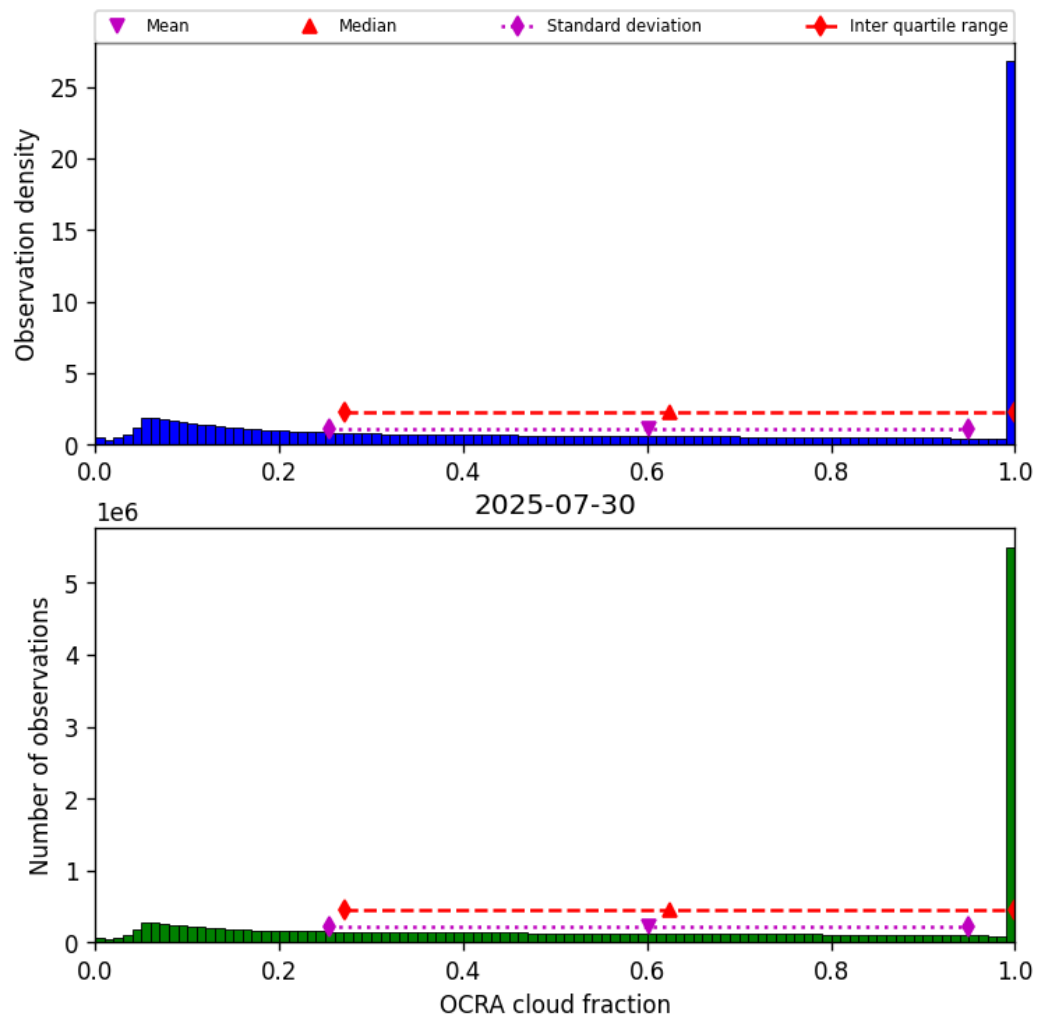
Figure 48: Histogram of “OCRA cloud fraction” for 2025-07-30 to 2025-07-31
