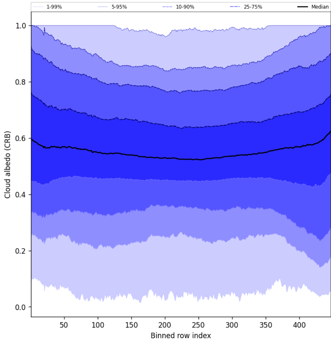
Figure 58: Along track statistics of “Cloud albedo (CRB)” for 2025-07-30 to 2025-07-31
