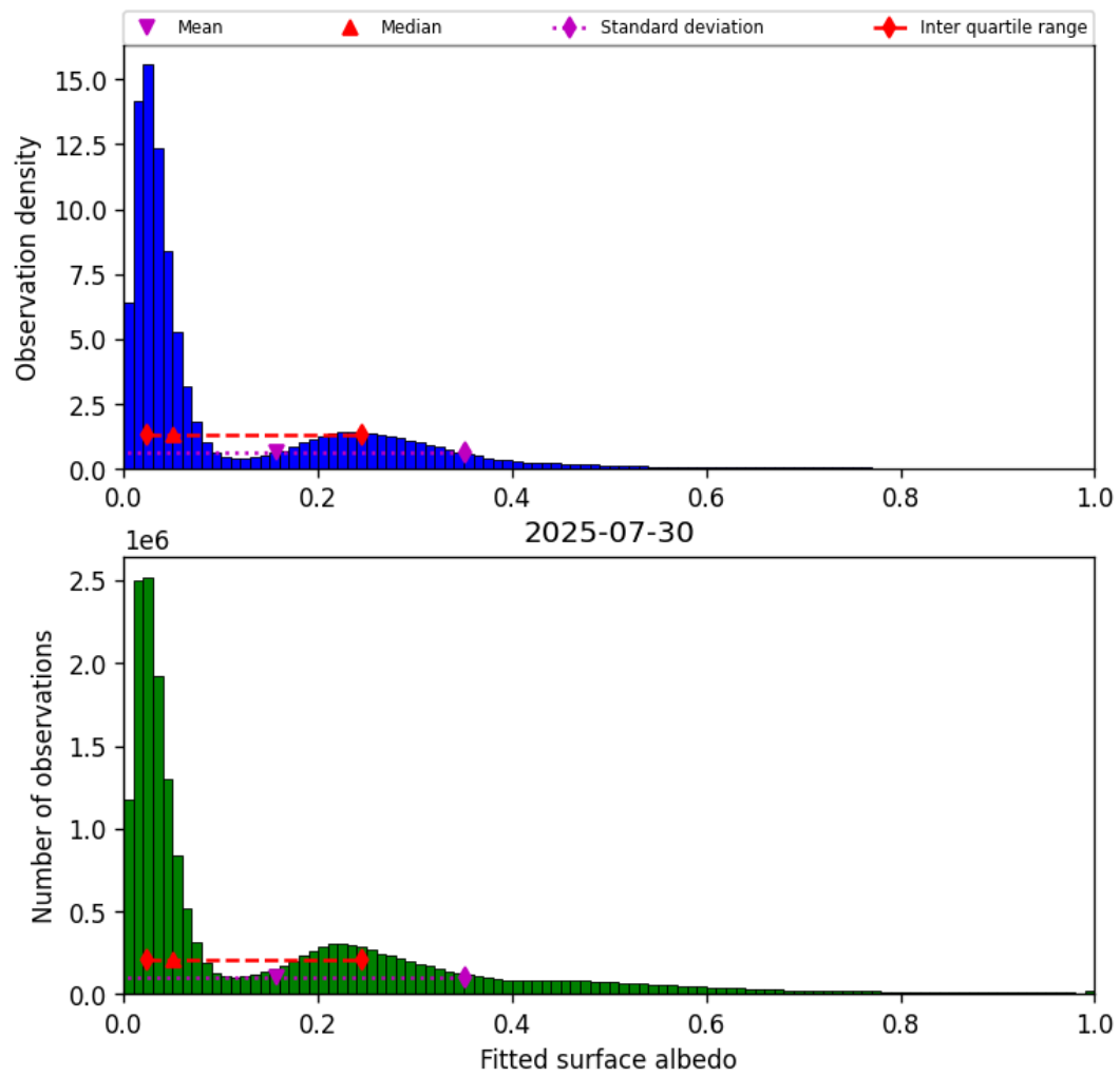
Figure 43: Histogram of “Fitted surface albedo” for 2025-07-30 to 2025-07-31
