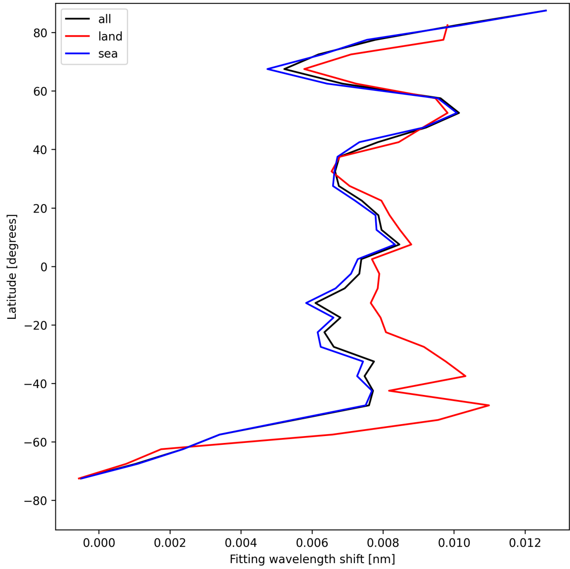
Figure 31: Zonal average of “Fitting wavelength shift” for 2025-07-30 to 2025-07-31.
