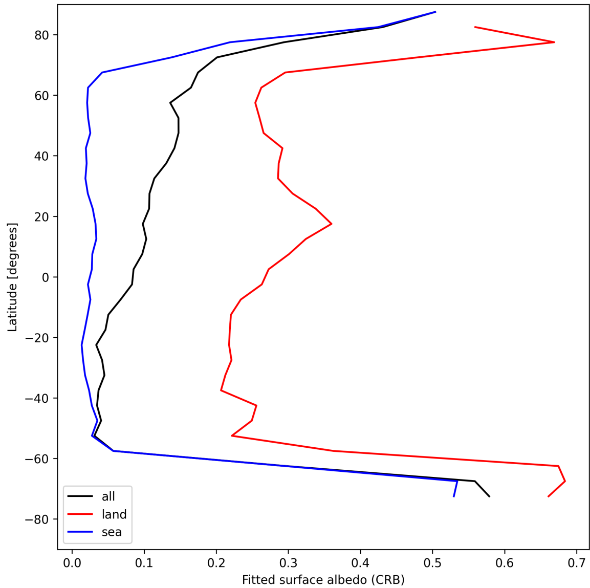
Figure 28: Zonal average of “Fitted surface albedo (CRB)” for 2025-07-30 to 2025-07-31.
