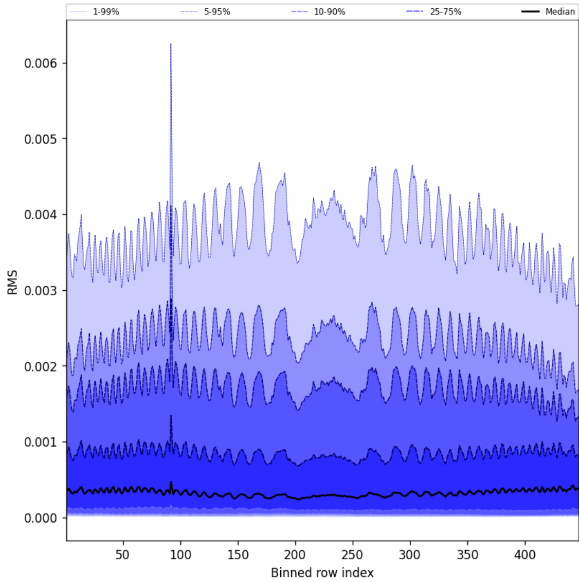
Figure 61: Along track statistics of “RMS” for 2025-07-30 to 2025-07-31
