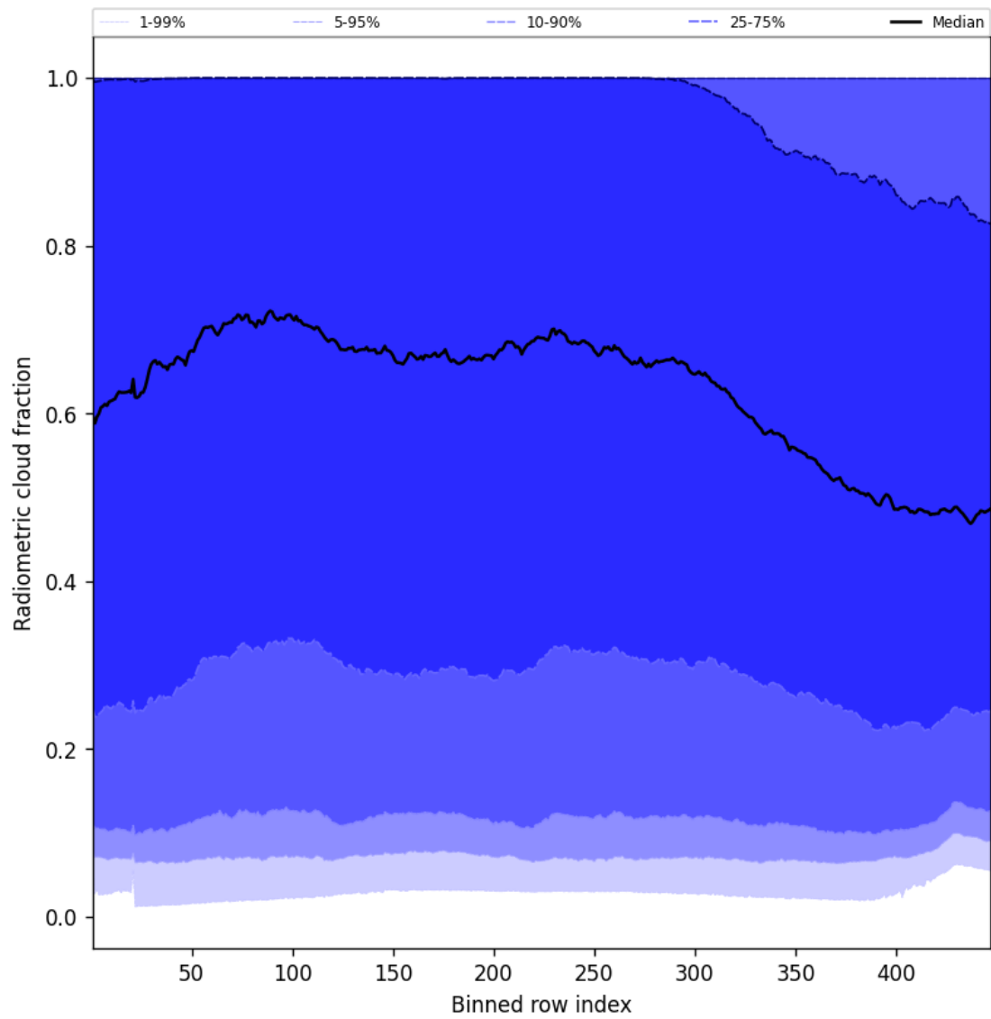
Figure 53: Along track statistics of “Radiometric cloud fraction” for 2025-07-30 to 2025-07-31
