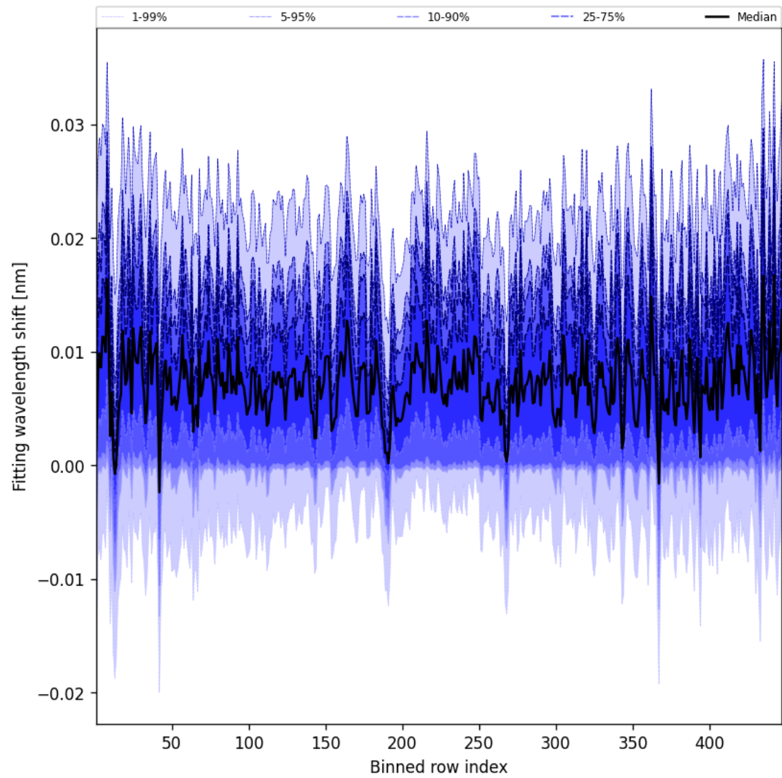
Figure 63: Along track statistics of “Fitting wavelength shift” for 2025-07-30 to 2025-07-31
