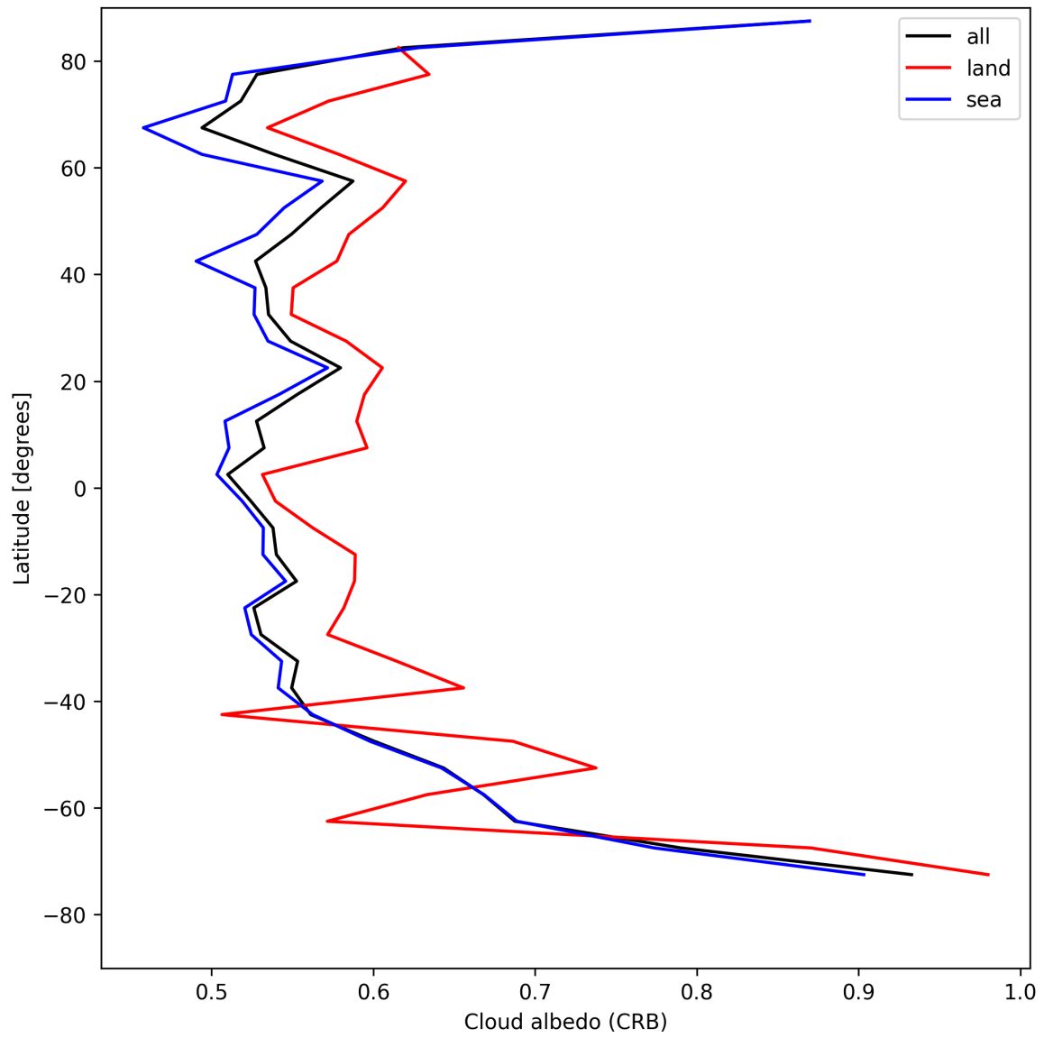
Figure 26: Zonal average of “Cloud albedo (CRB)” for 2025-07-30 to 2025-07-31.
