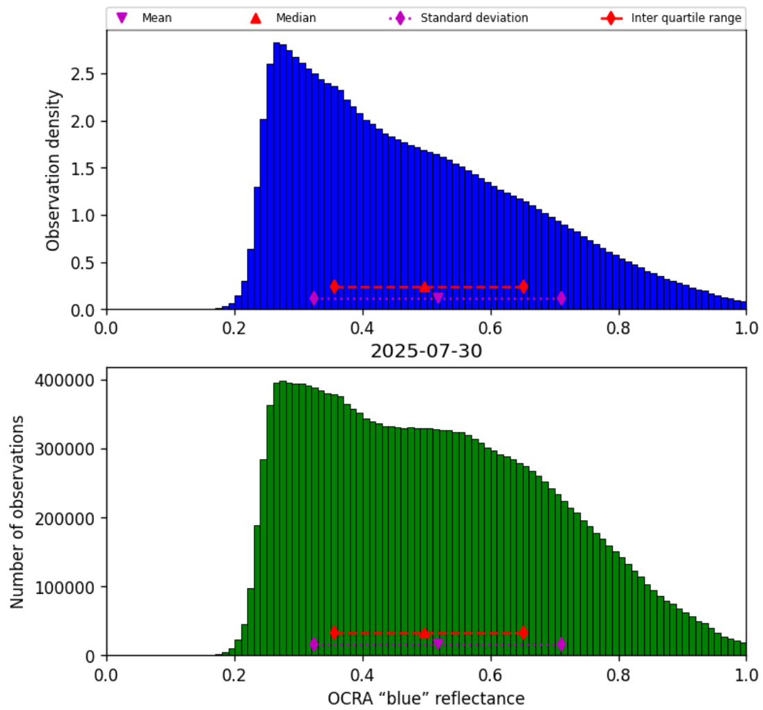
Figure 49: Histogram of “OCRA “blue” reflectance” for 2025-07-30 to 2025-07-31
