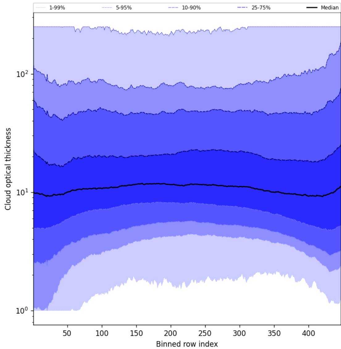
Figure 55: Along track statistics of “Cloud optical thickness” for 2025-07-30 to 2025-07-31
