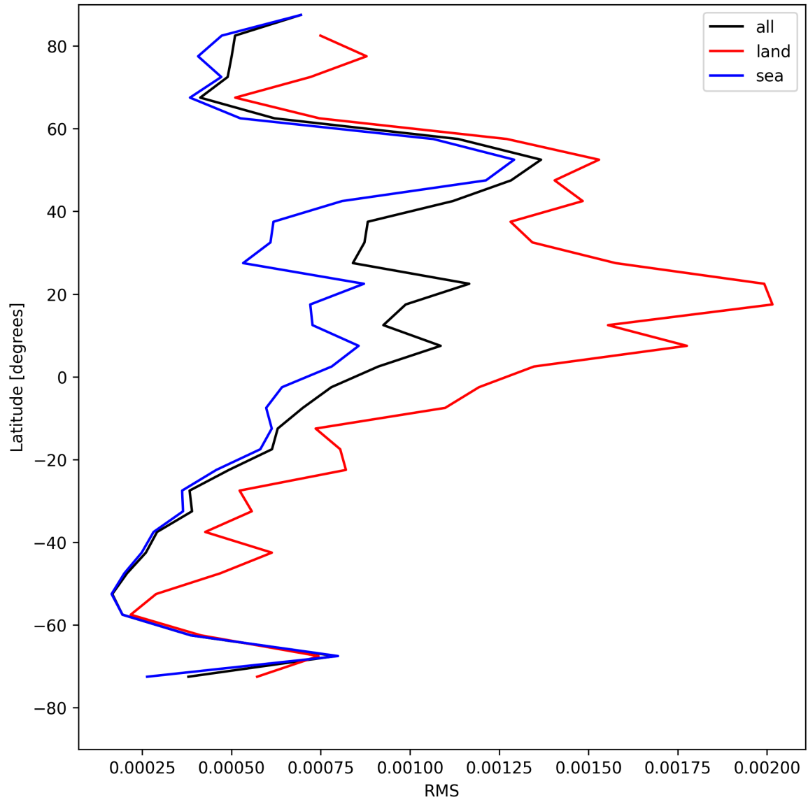
Figure 29: Zonal average of “RMS” for 2025-07-30 to 2025-07-31.
