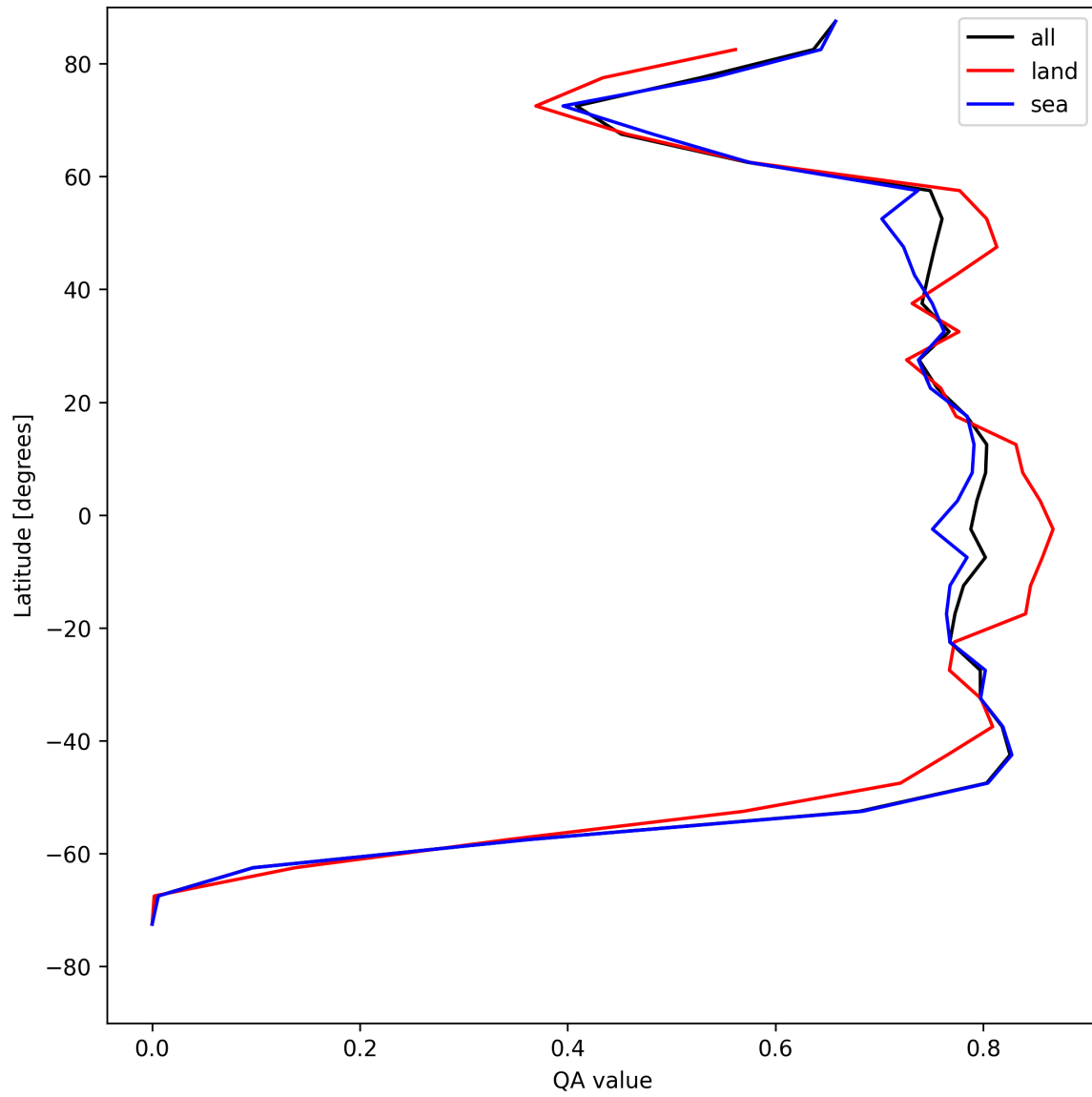
Figure 20: Zonal average of “QA value” for 2025-08-01 to 2025-08-01.
