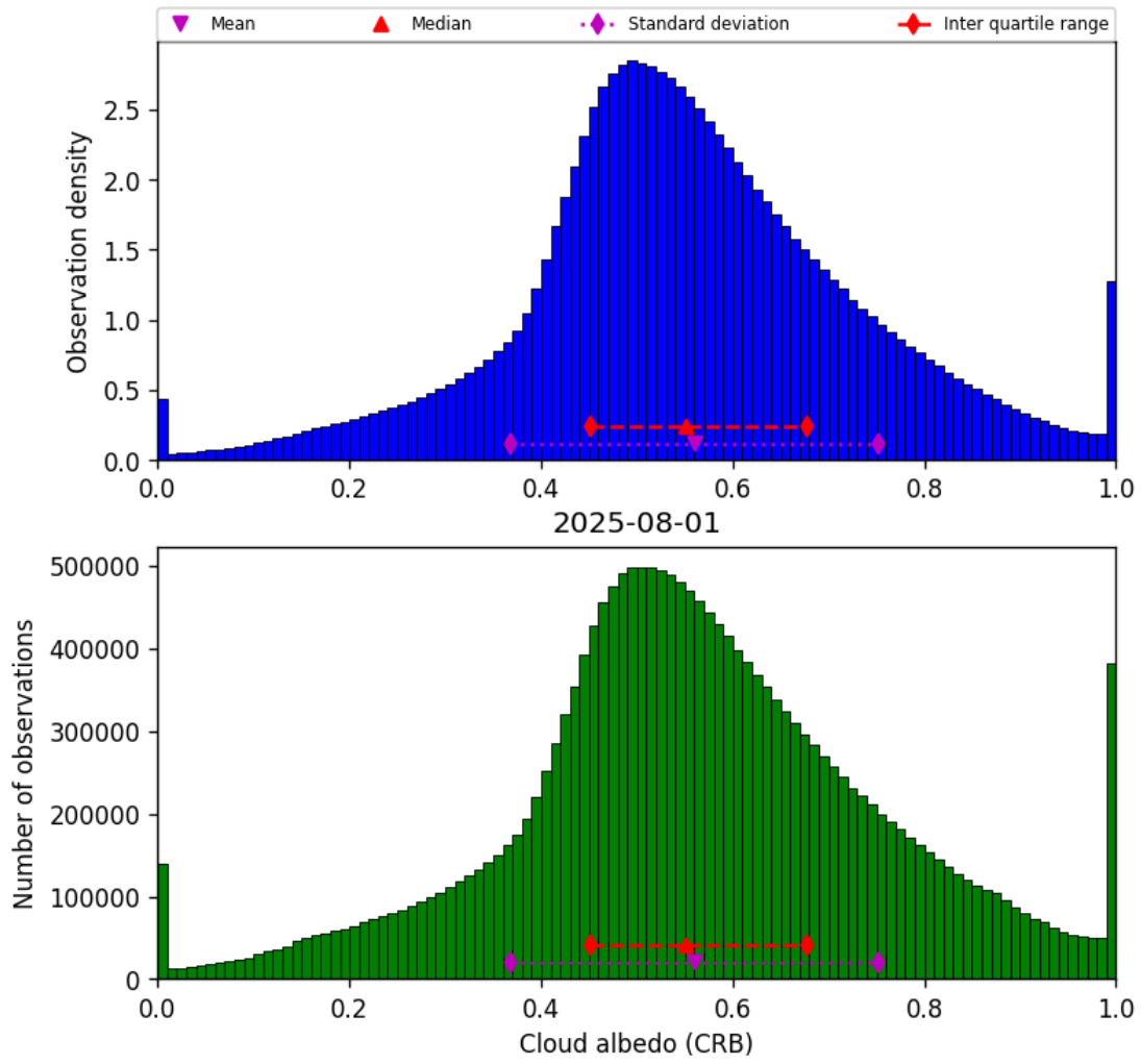
Figure 42: Histogram of “Cloud albedo (CRB)” for 2025-08-01 to 2025-08-01
