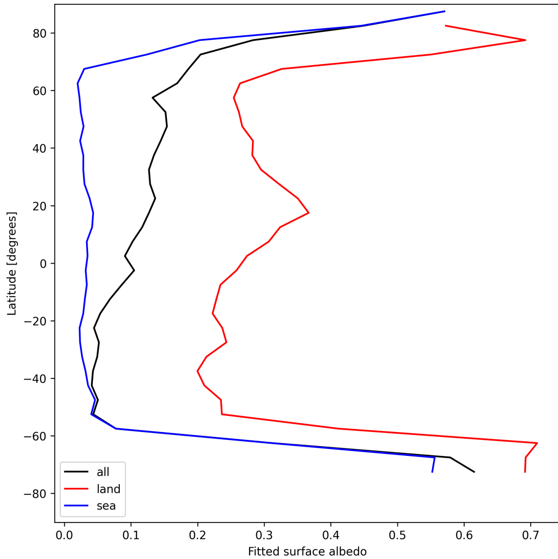
Figure 27: Zonal average of “Fitted surface albedo” for 2025-08-01 to 2025-08-01.
