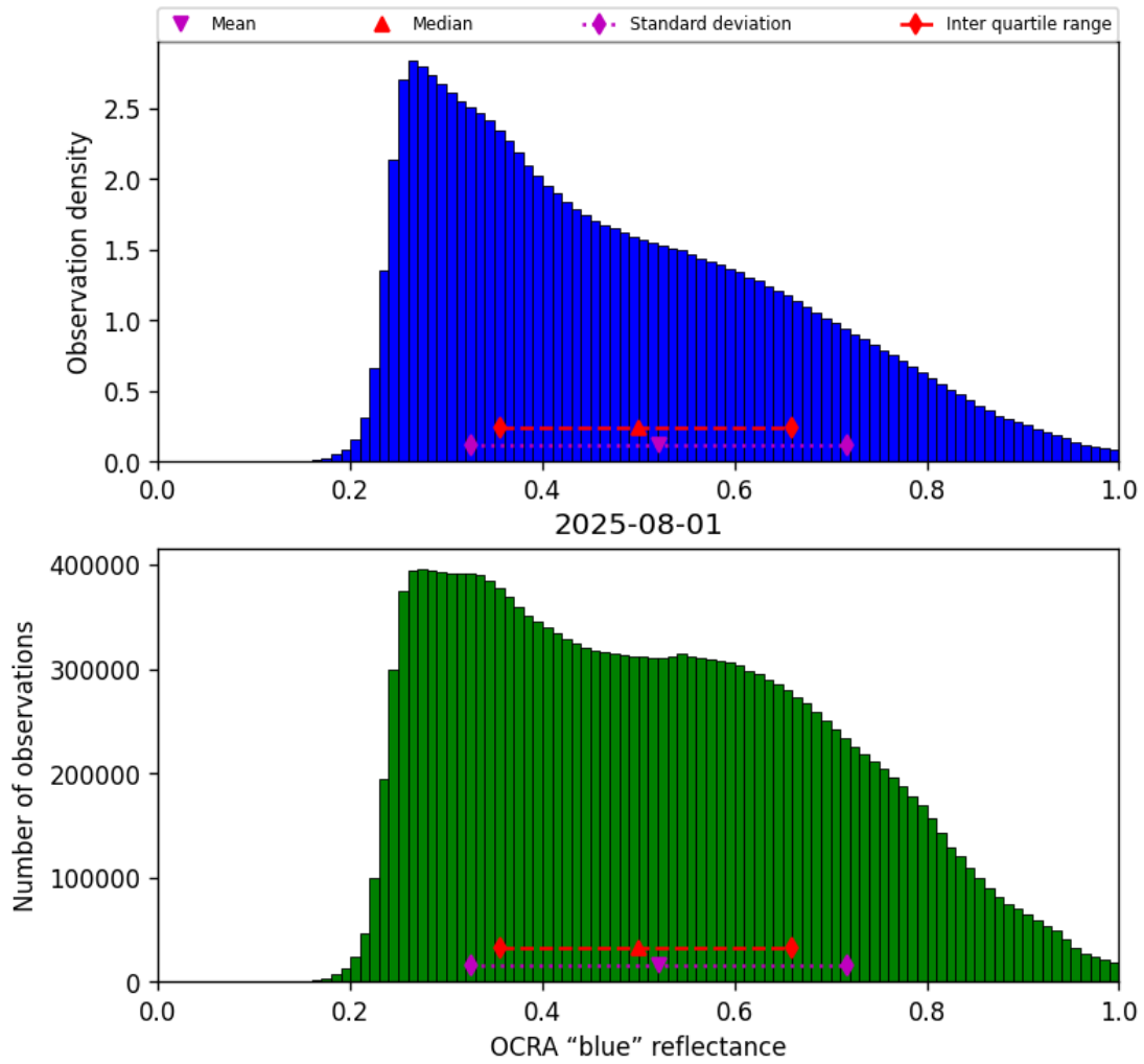
Figure 49: Histogram of “OCRA “blue” reflectance” for 2025-08-01 to 2025-08-01
