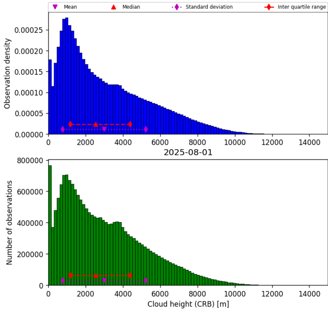
Figure 41: Histogram of “Cloud height (CRB)” for 2025-08-01 to 2025-08-01
