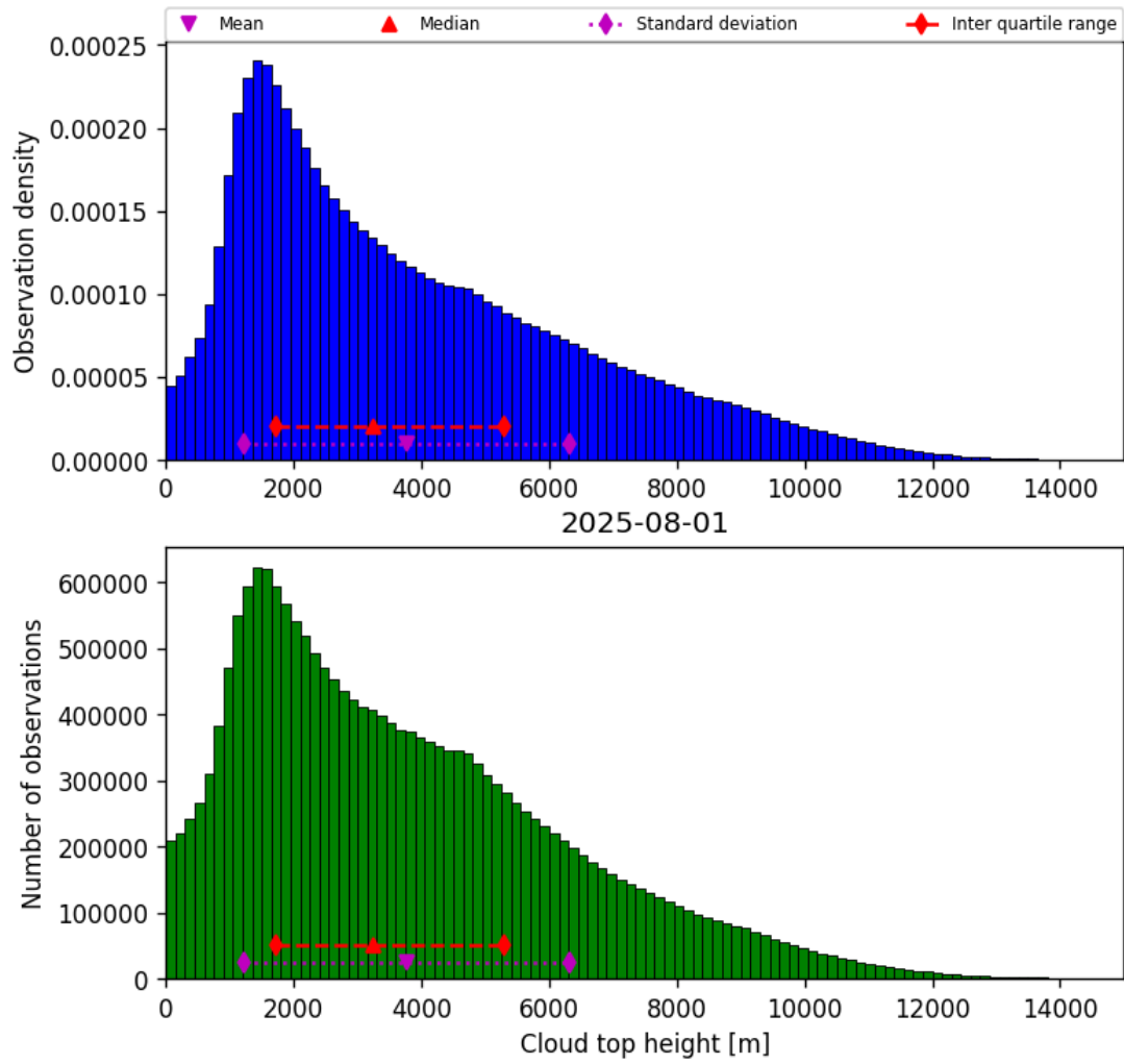
Figure 38: Histogram of “Cloud top height” for 2025-08-01 to 2025-08-01
