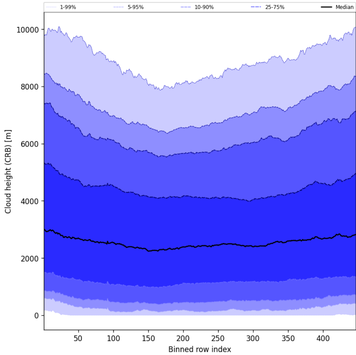
Figure 57: Along track statistics of “Cloud height (CRB)” for 2025-08-01 to 2025-08-01
