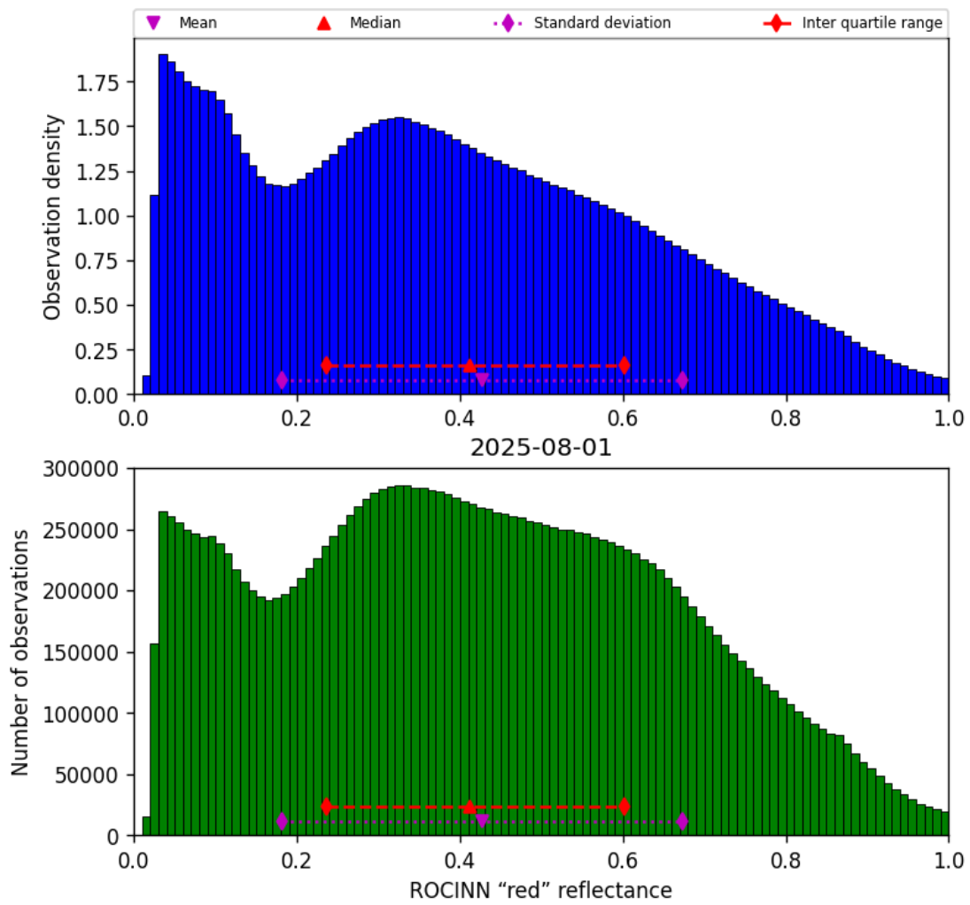
Figure 51: Histogram of “ROCINN “red” reflectance” for 2025-08-01 to 2025-08-01
