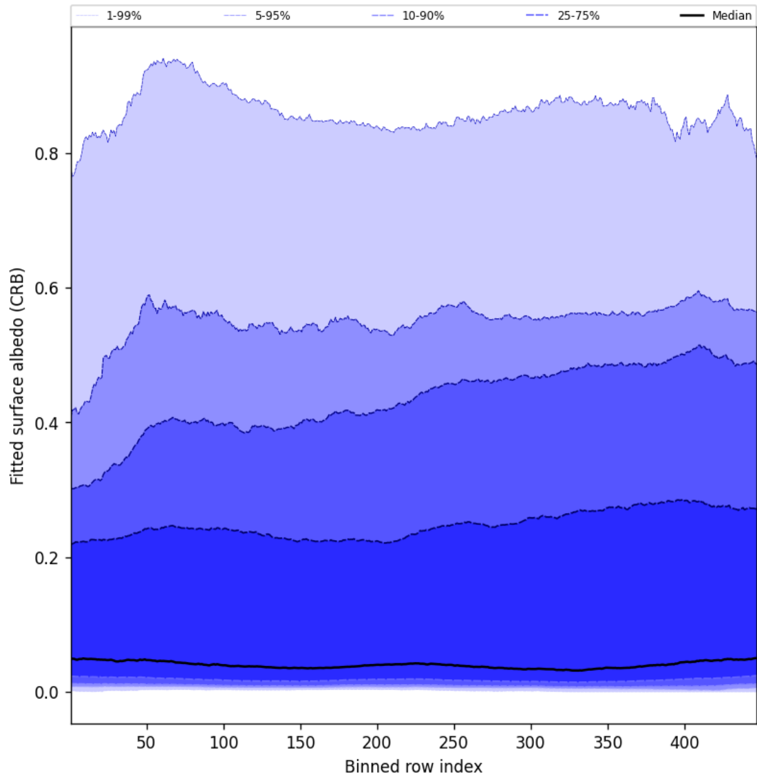
Figure 60: Along track statistics of “Fitted surface albedo (CRB)” for 2025-08-01 to 2025-08-01
