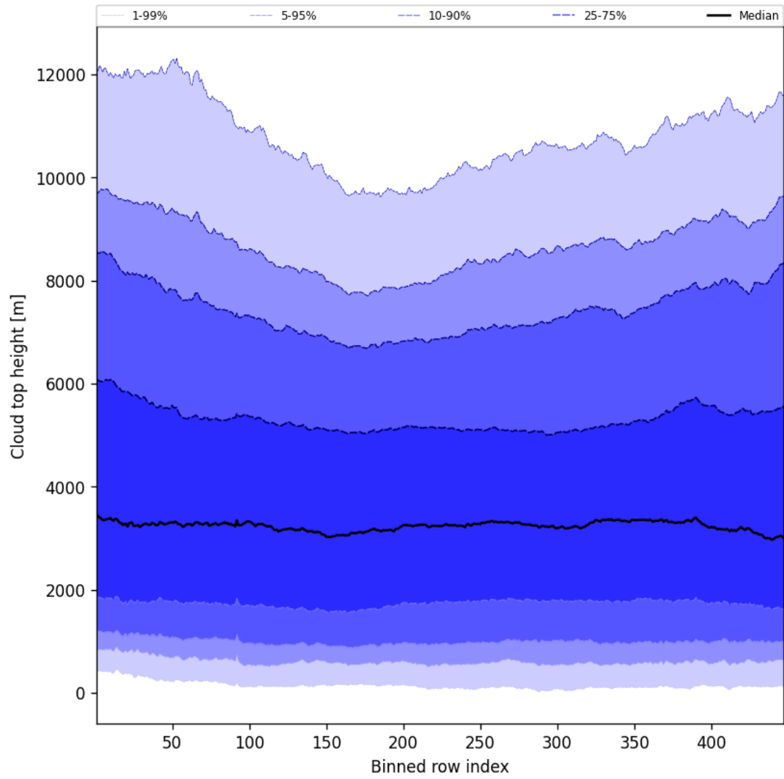
Figure 54: Along track statistics of “Cloud top height” for 2025-08-01 to 2025-08-01
