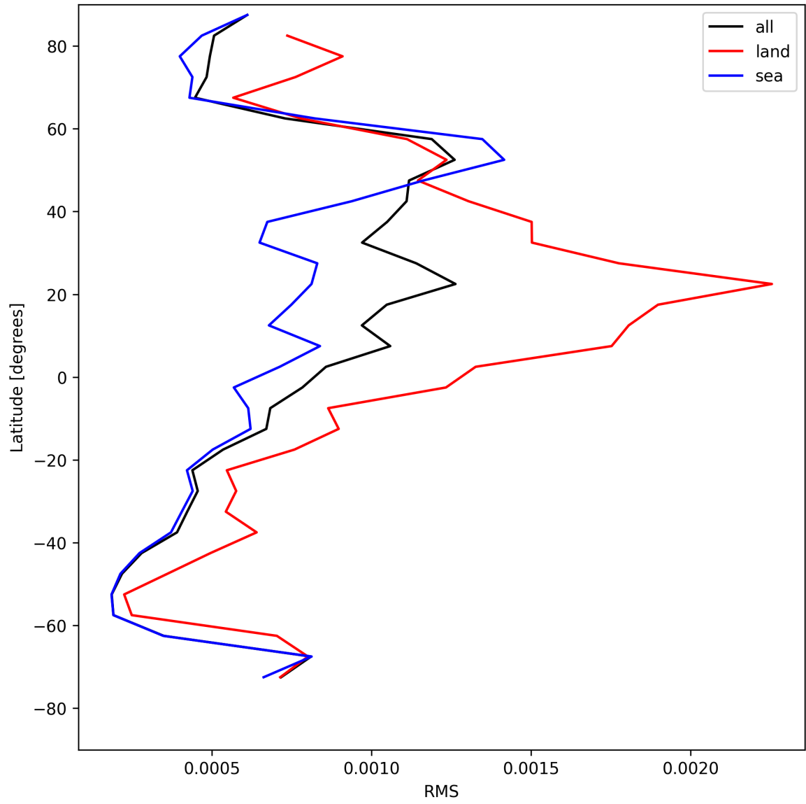
Figure 29: Zonal average of “RMS” for 2025-08-01 to 2025-08-01.
