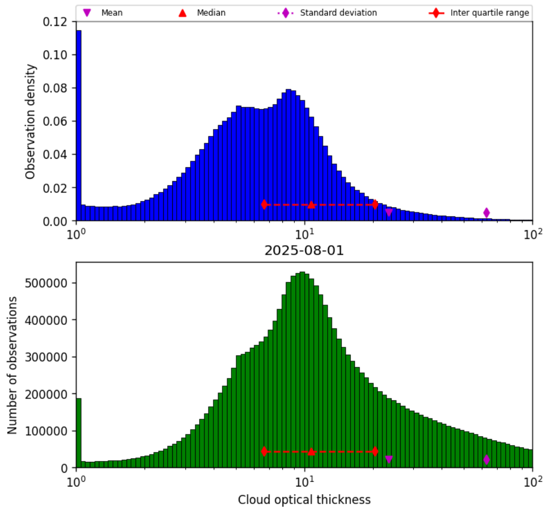
Figure 39: Histogram of “Cloud optical thickness” for 2025-08-01 to 2025-08-01
