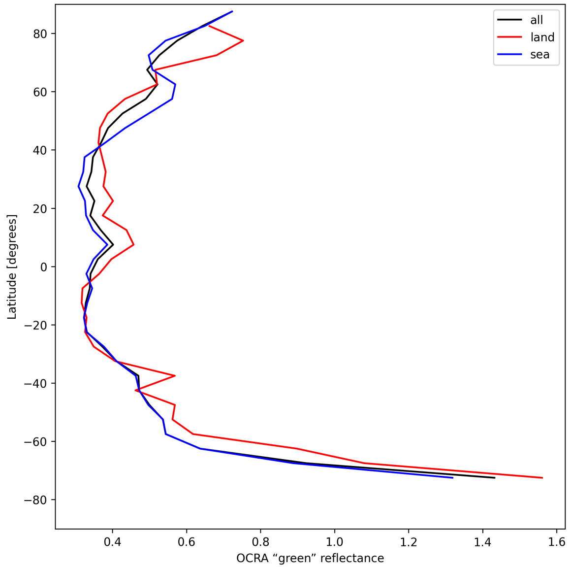
Figure 34: Zonal average of “OCRA “green” reflectance” for 2025-08-01 to 2025-08-01.
