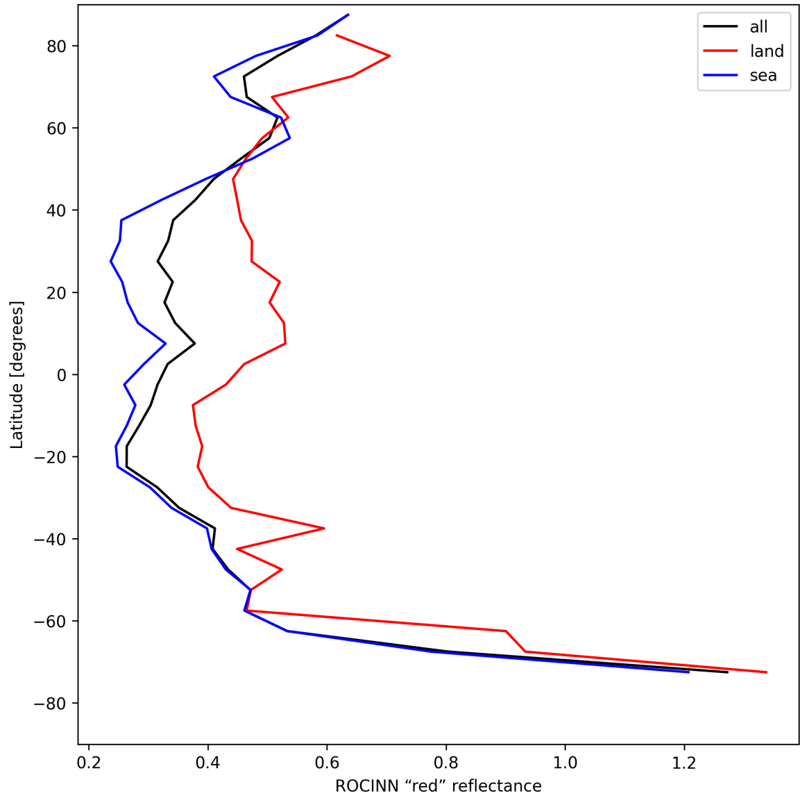
Figure 35: Zonal average of “ROCINN “red” reflectance” for 2025-08-01 to 2025-08-01.
