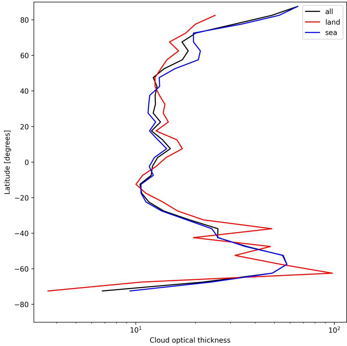
Figure 23: Zonal average of “Cloud optical thickness” for 2025-08-01 to 2025-08-01.
