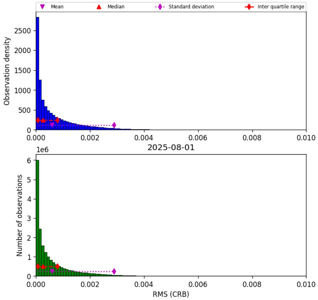
Figure 46: Histogram of “RMS (CRB)” for 2025-08-01 to 2025-08-01
