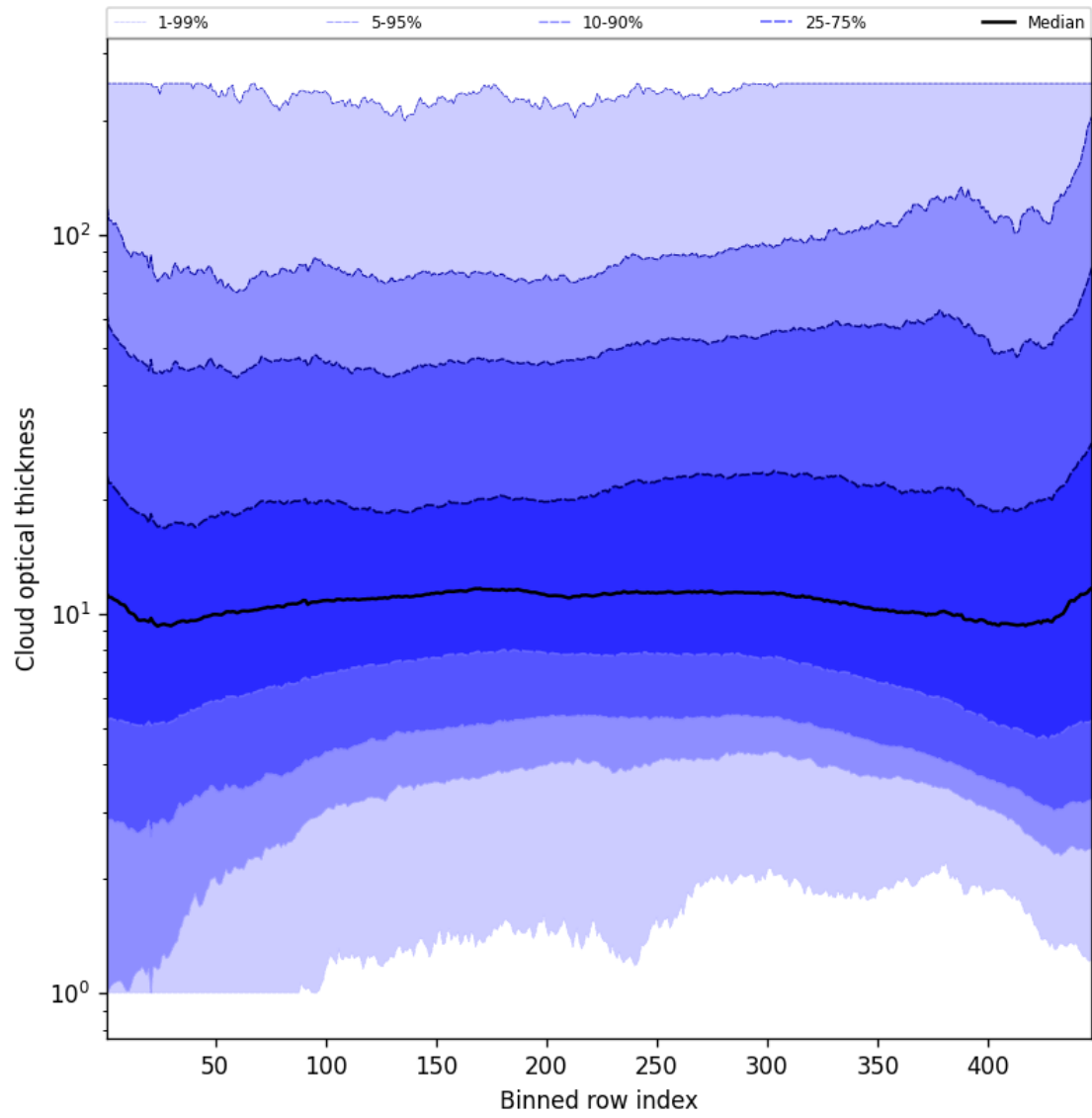
Figure 55: Along track statistics of “Cloud optical thickness” for 2025-08-01 to 2025-08-01
