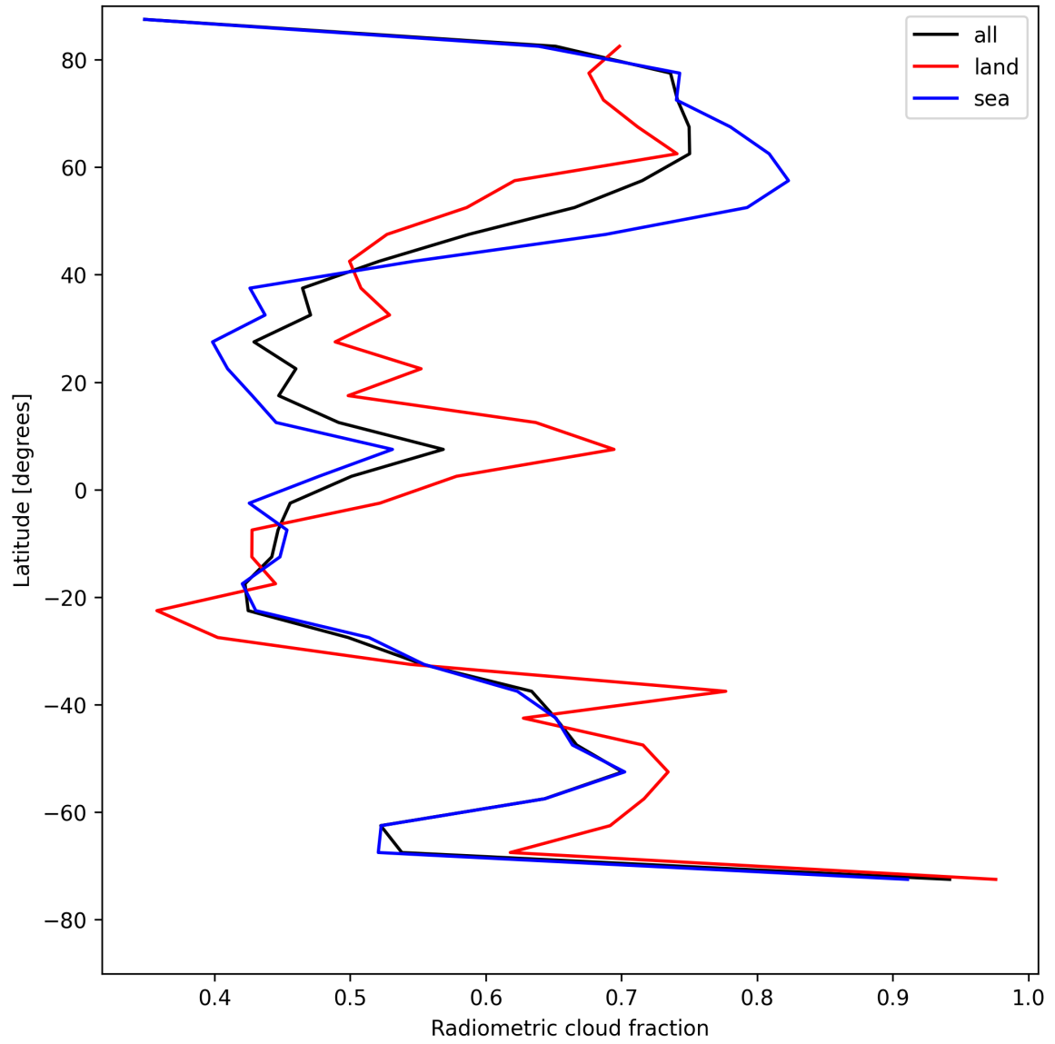
Figure 21: Zonal average of “Radiometric cloud fraction” for 2025-08-01 to 2025-08-01.
