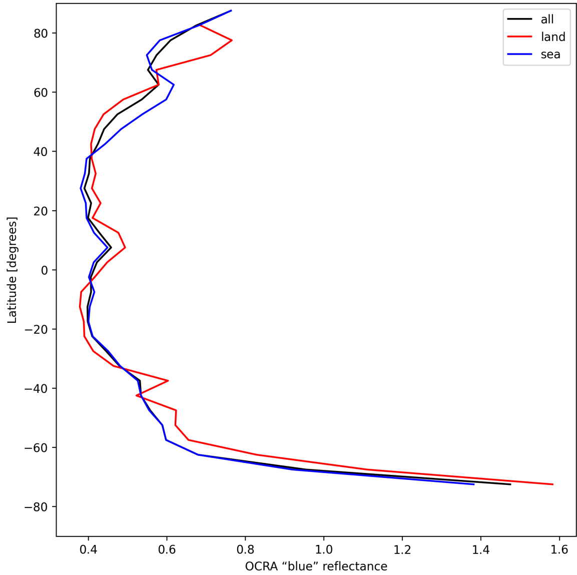
Figure 33: Zonal average of “OCRA “blue” reflectance” for 2025-08-01 to 2025-08-01.
