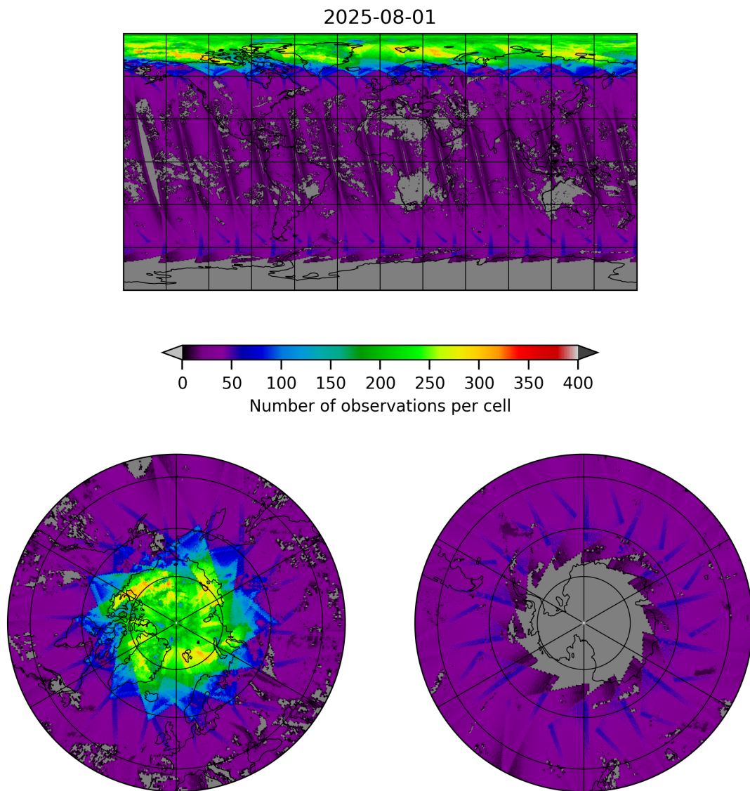
Figure 19: Map of the number of observations for 2025-08-01 to 2025-08-01
