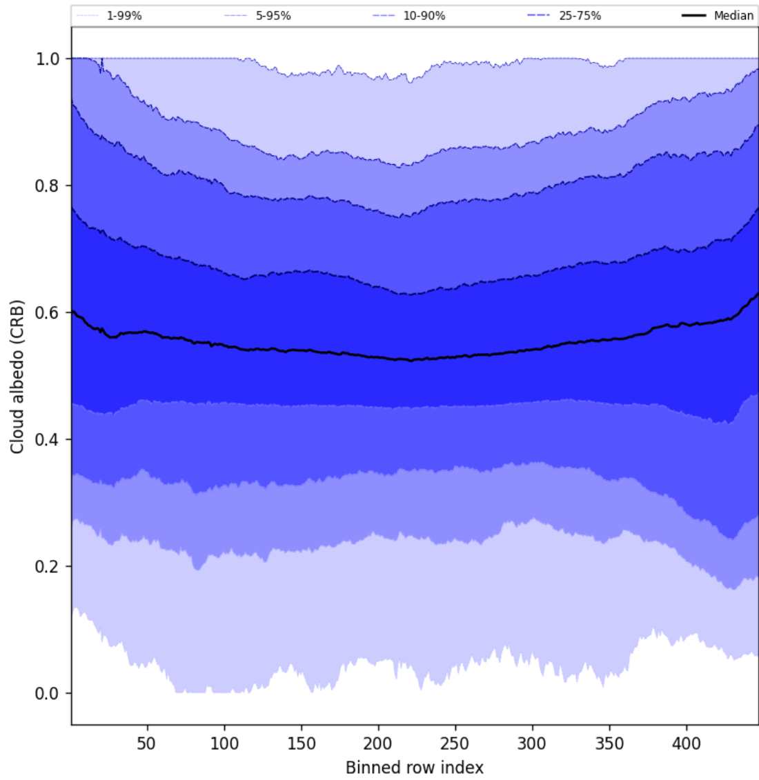
Figure 58: Along track statistics of “Cloud albedo (CRB)” for 2025-08-01 to 2025-08-01
