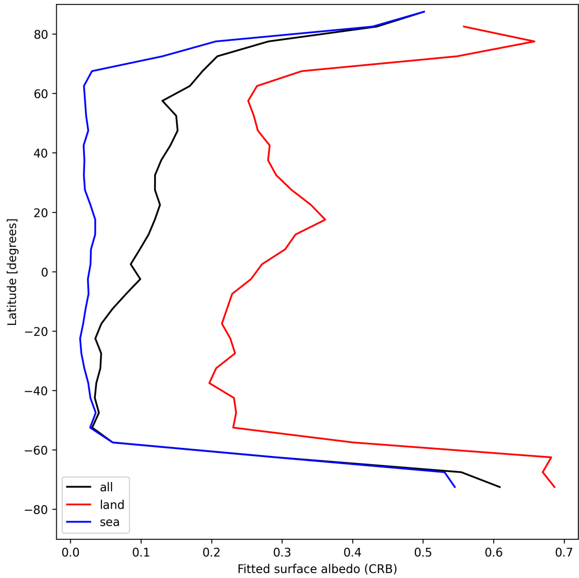
Figure 28: Zonal average of “Fitted surface albedo (CRB)” for 2025-08-01 to 2025-08-01.
