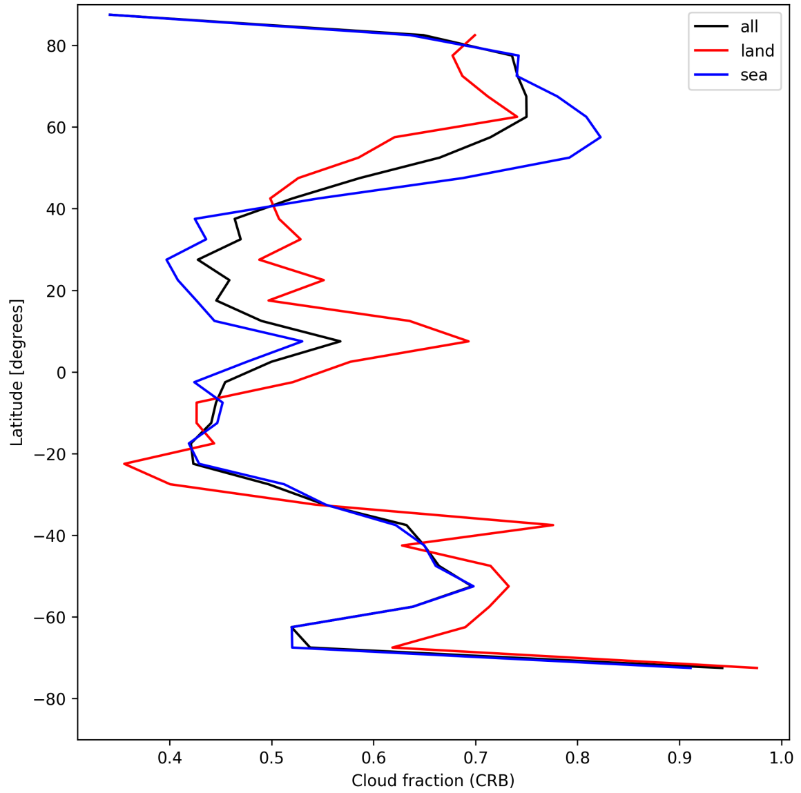
Figure 24: Zonal average of “Cloud fraction (CRB)” for 2025-08-01 to 2025-08-01.
