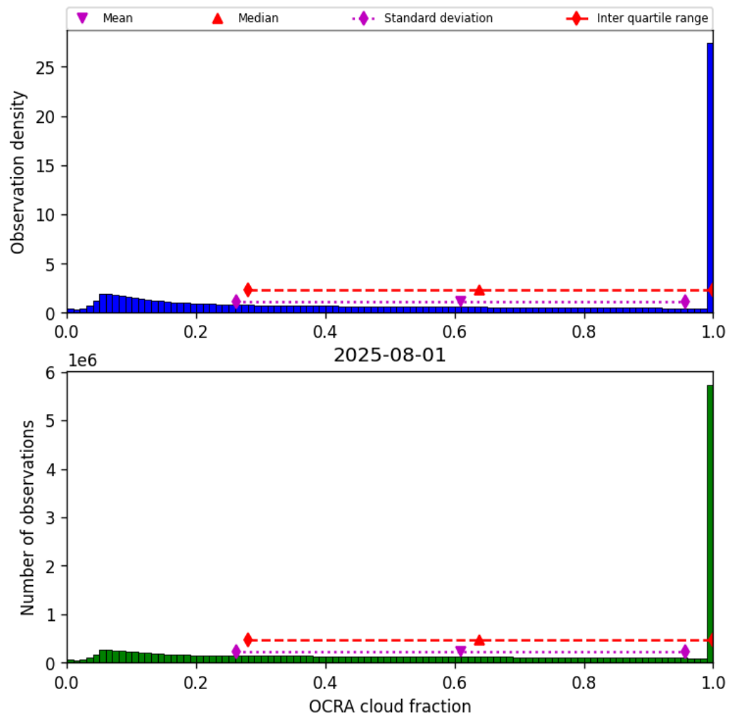
Figure 48: Histogram of “OCRA cloud fraction” for 2025-08-01 to 2025-08-01
