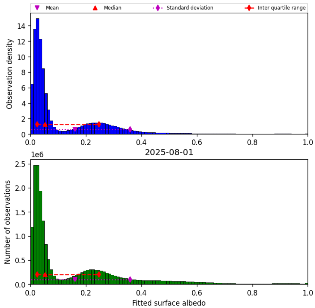
Figure 43: Histogram of “Fitted surface albedo” for 2025-08-01 to 2025-08-01
