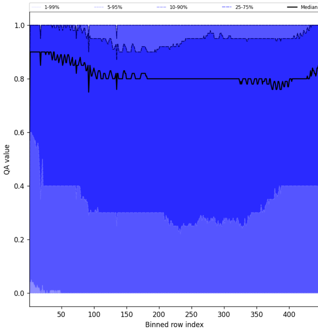
Figure 52: Along track statistics of “QA value” for 2025-08-01 to 2025-08-01
