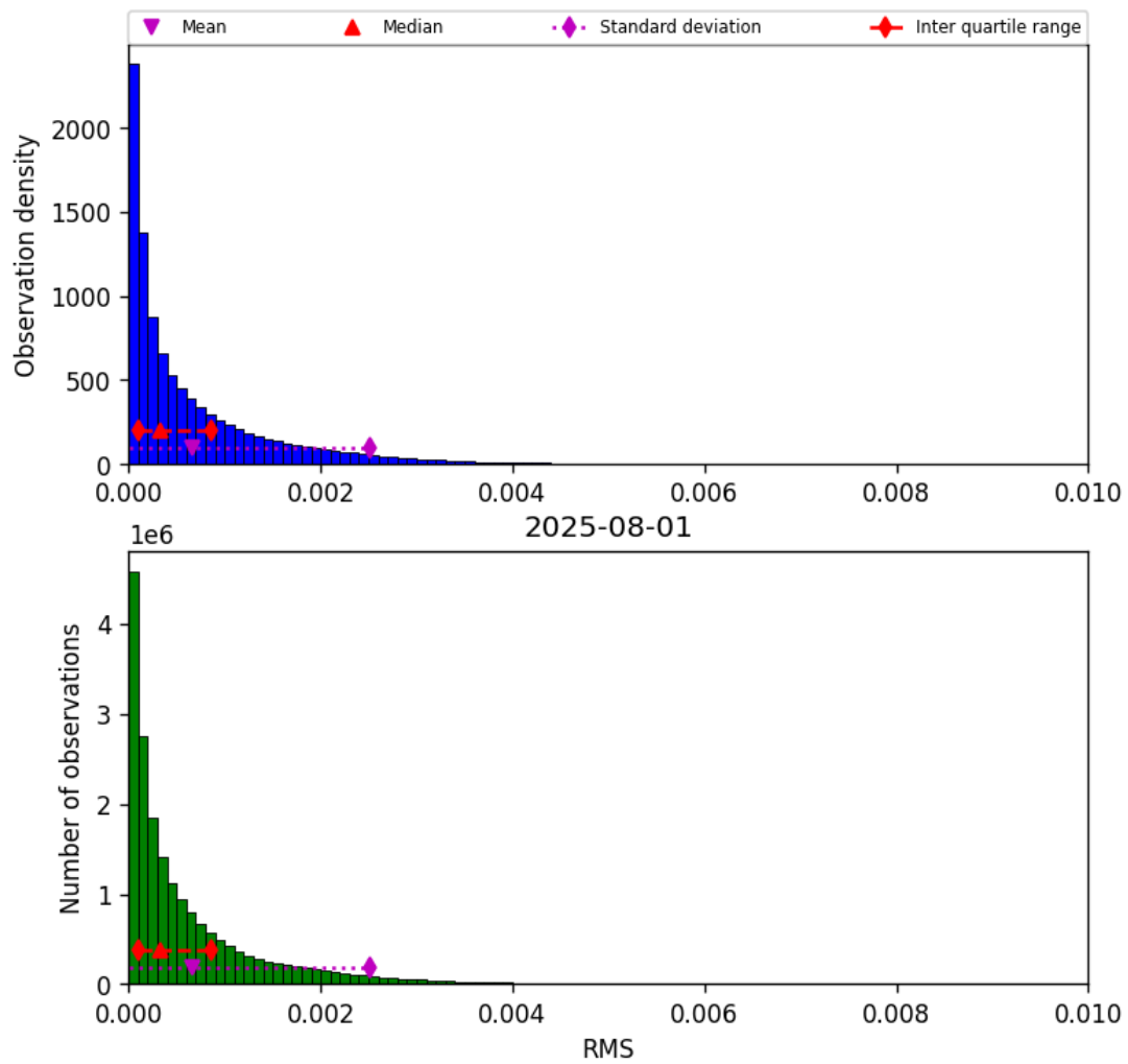
Figure 45: Histogram of “RMS” for 2025-08-01 to 2025-08-01
