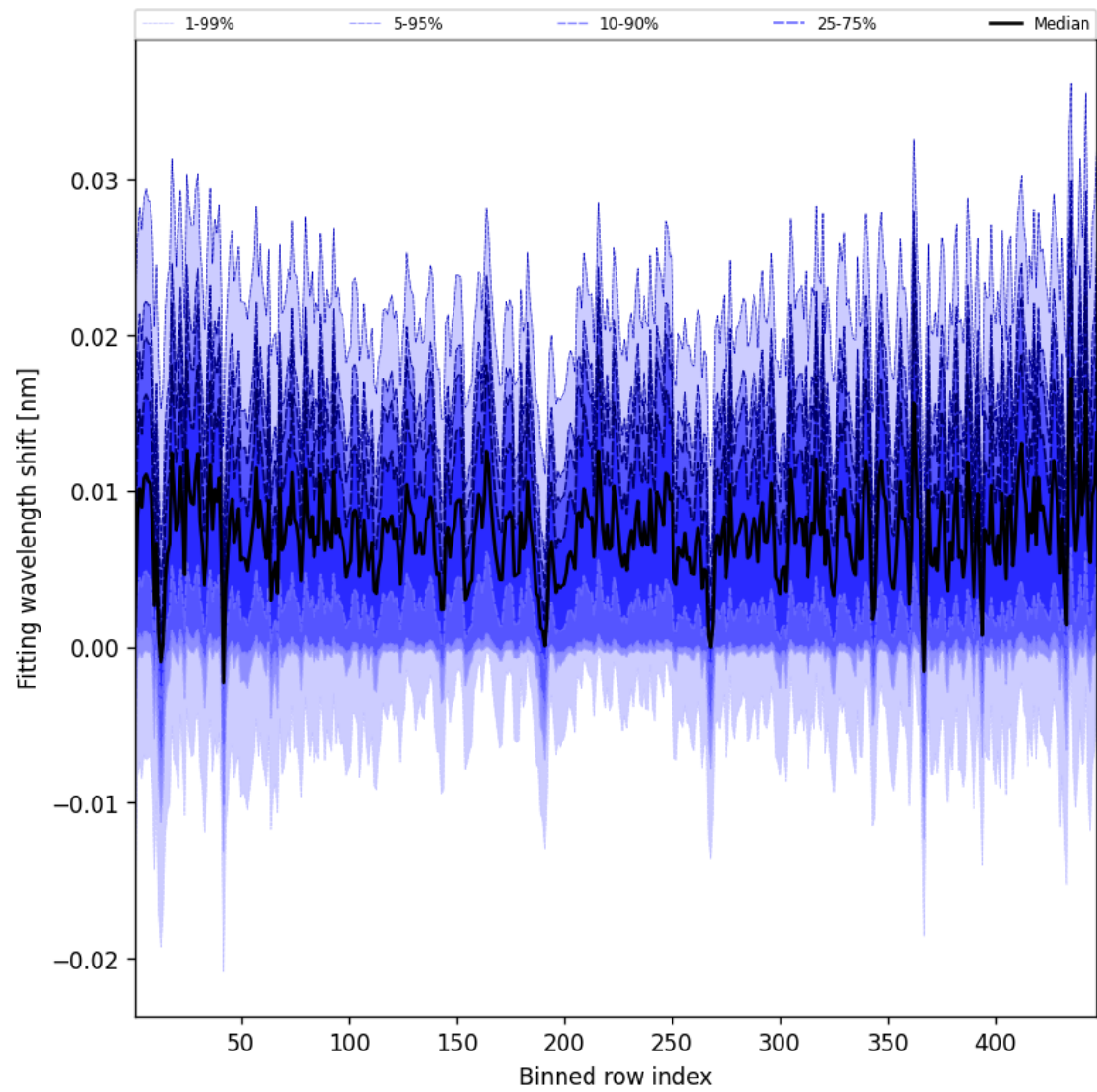
Figure 63: Along track statistics of “Fitting wavelength shift” for 2025-08-01 to 2025-08-01
