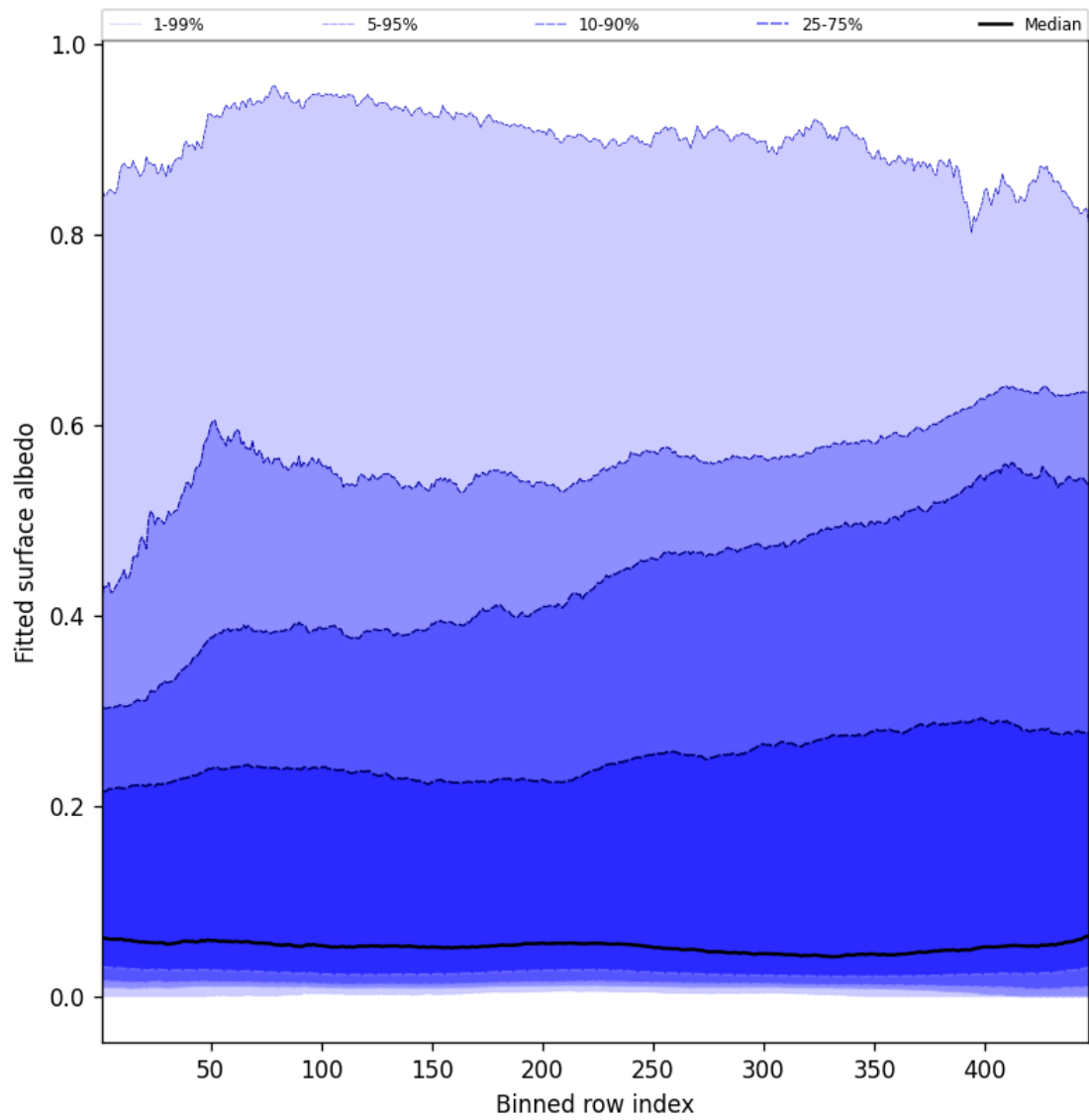
Figure 59: Along track statistics of “Fitted surface albedo” for 2025-08-01 to 2025-08-01
