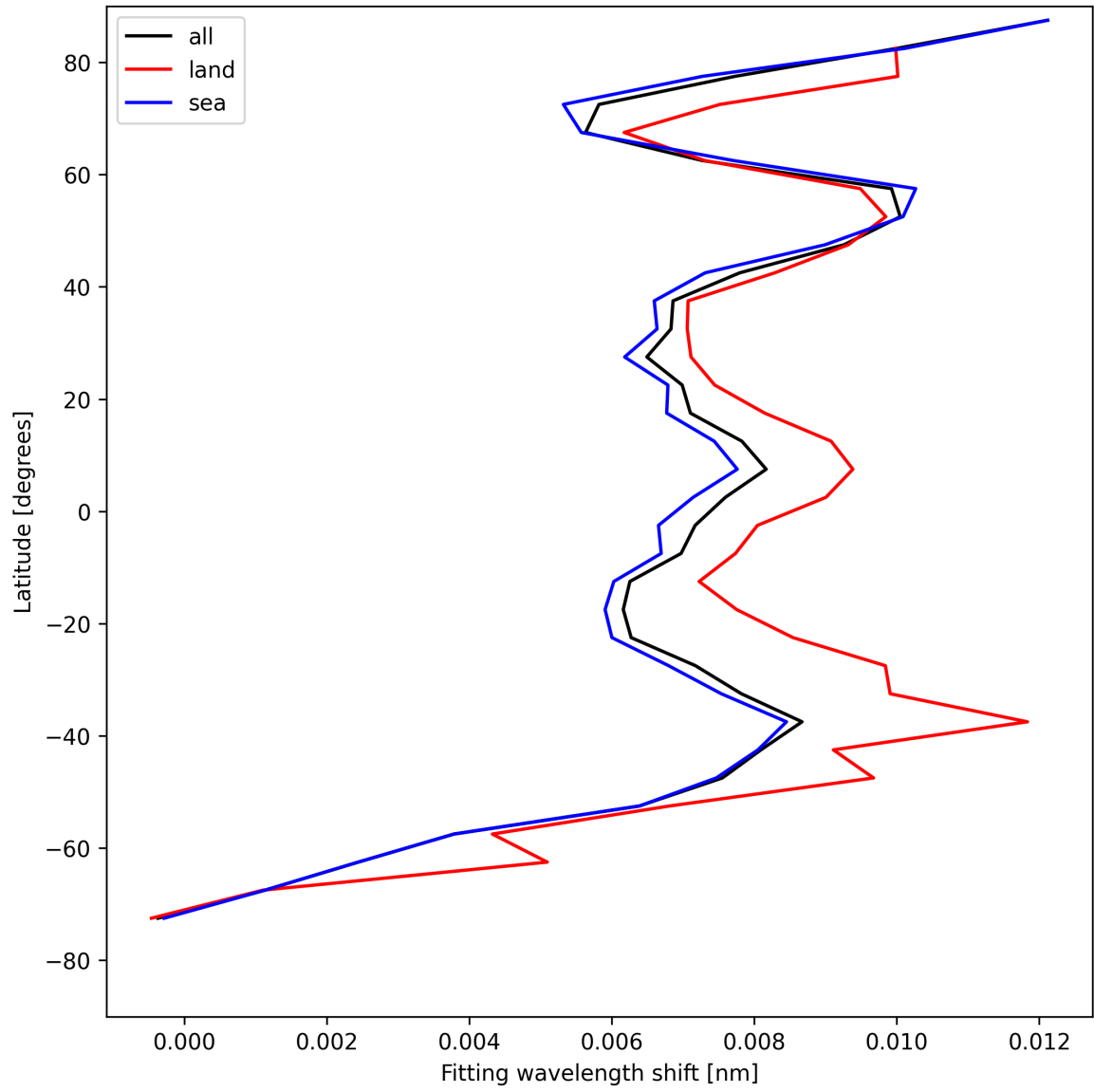
Figure 31: Zonal average of “Fitting wavelength shift” for 2025-08-01 to 2025-08-01.
