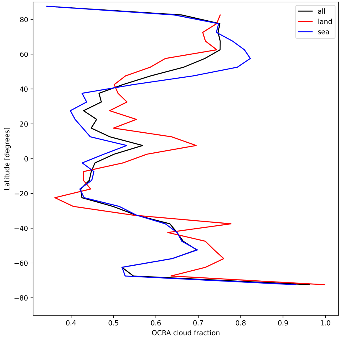
Figure 32: Zonal average of “OCRA cloud fraction” for 2025-08-01 to 2025-08-01.
