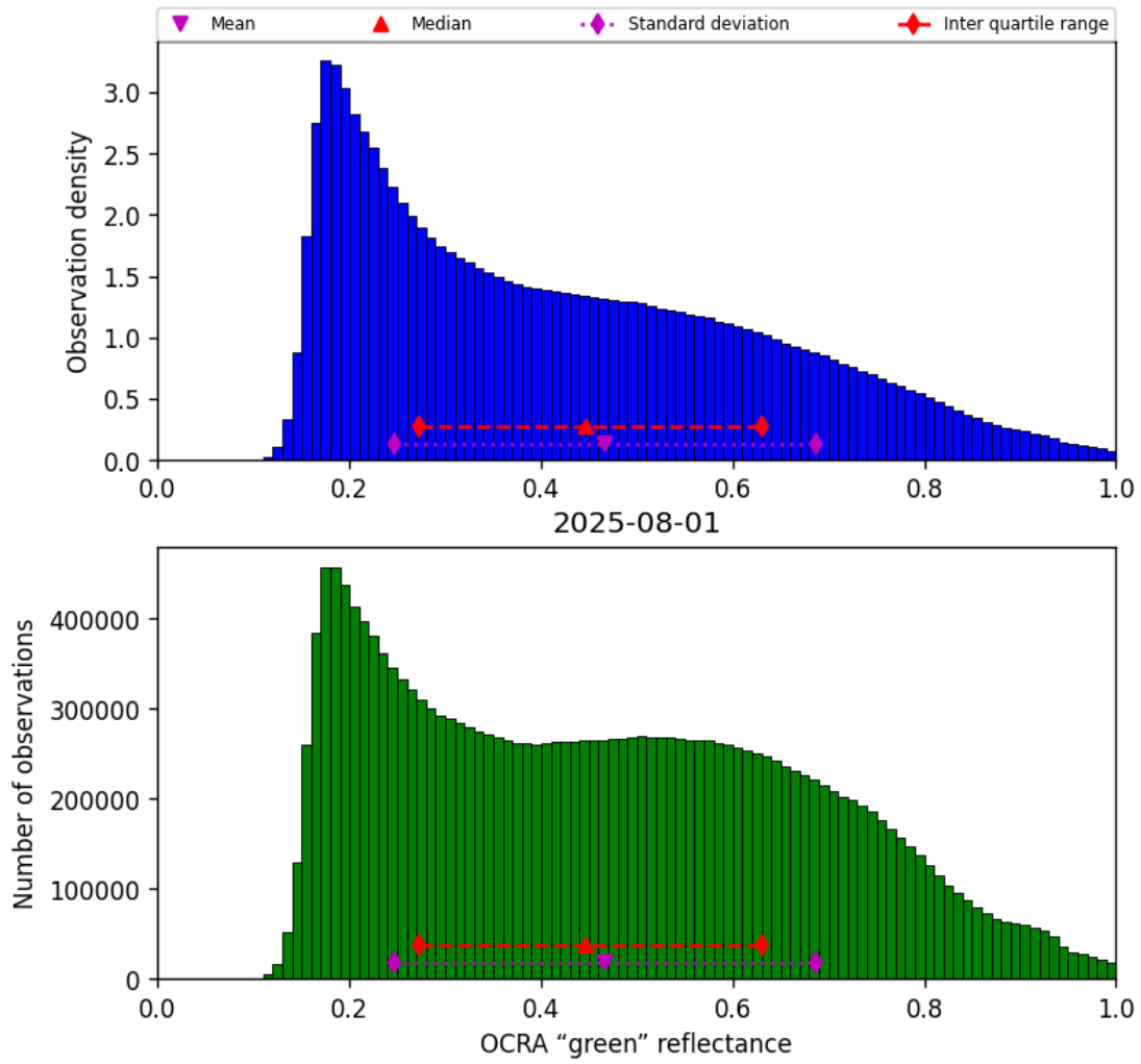
Figure 50: Histogram of “OCRA “green” reflectance” for 2025-08-01 to 2025-08-01
