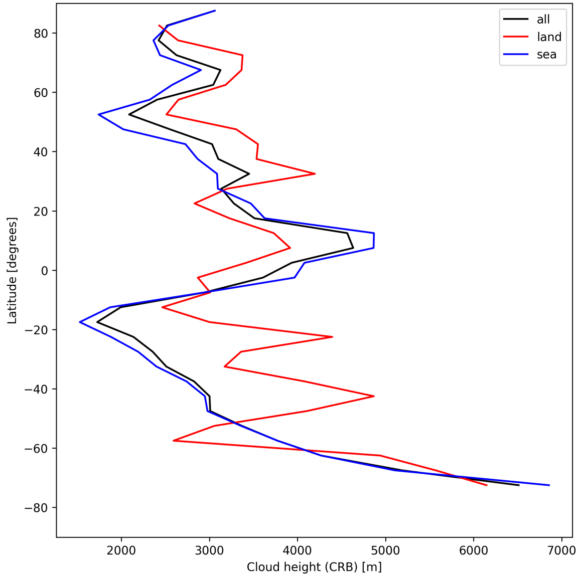
Figure 25: Zonal average of “Cloud height (CRB)” for 2025-08-01 to 2025-08-01.
