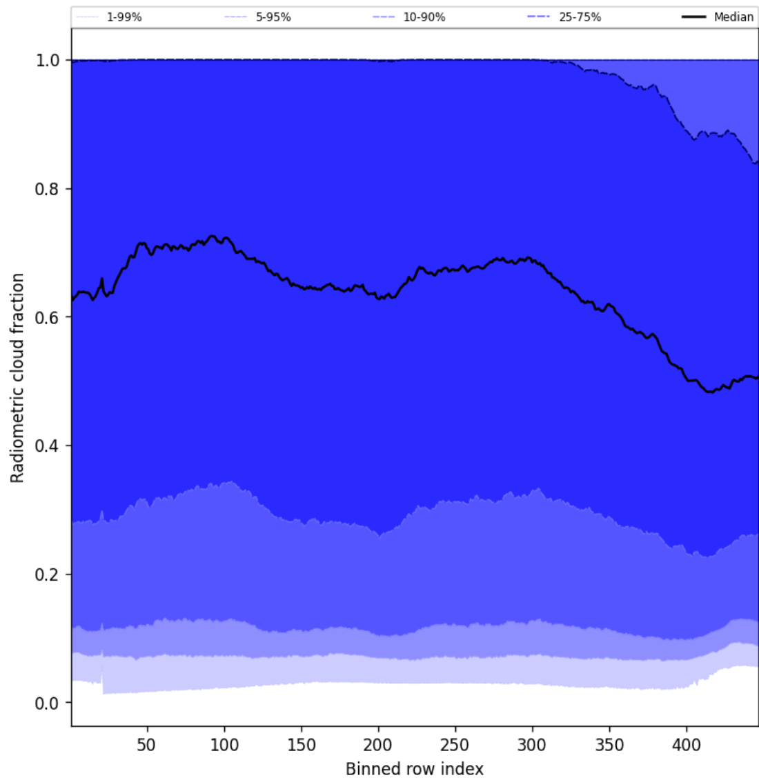
Figure 53: Along track statistics of “Radiometric cloud fraction” for 2025-08-01 to 2025-08-01
