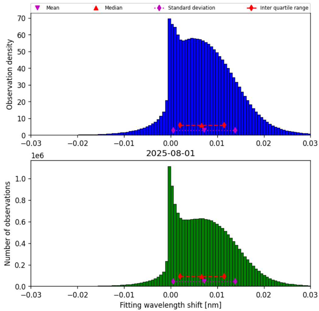
Figure 47: Histogram of “Fitting wavelength shift” for 2025-08-01 to 2025-08-01
