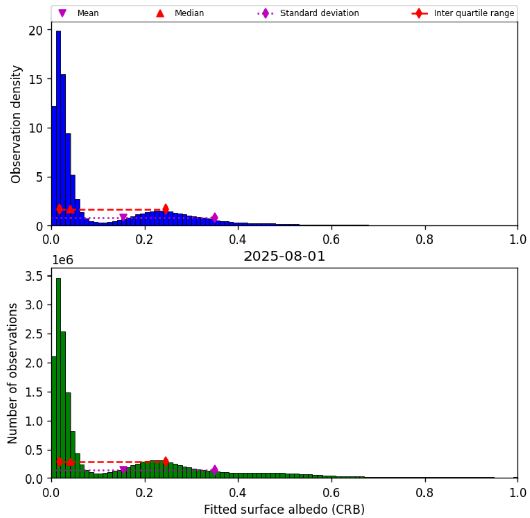
Figure 44: Histogram of “Fitted surface albedo (CRB)” for 2025-08-01 to 2025-08-01
