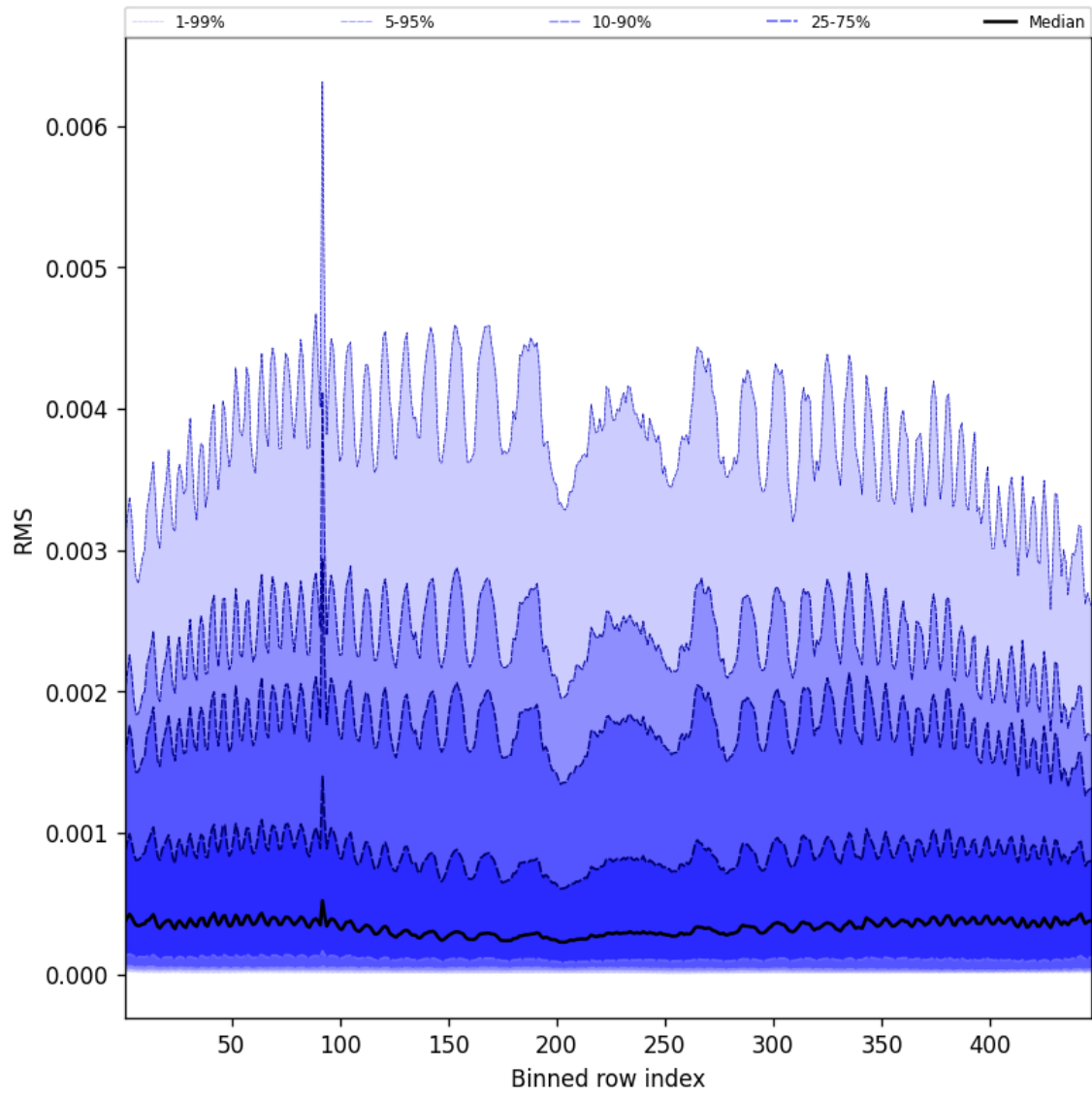
Figure 61: Along track statistics of “RMS” for 2025-08-01 to 2025-08-01
