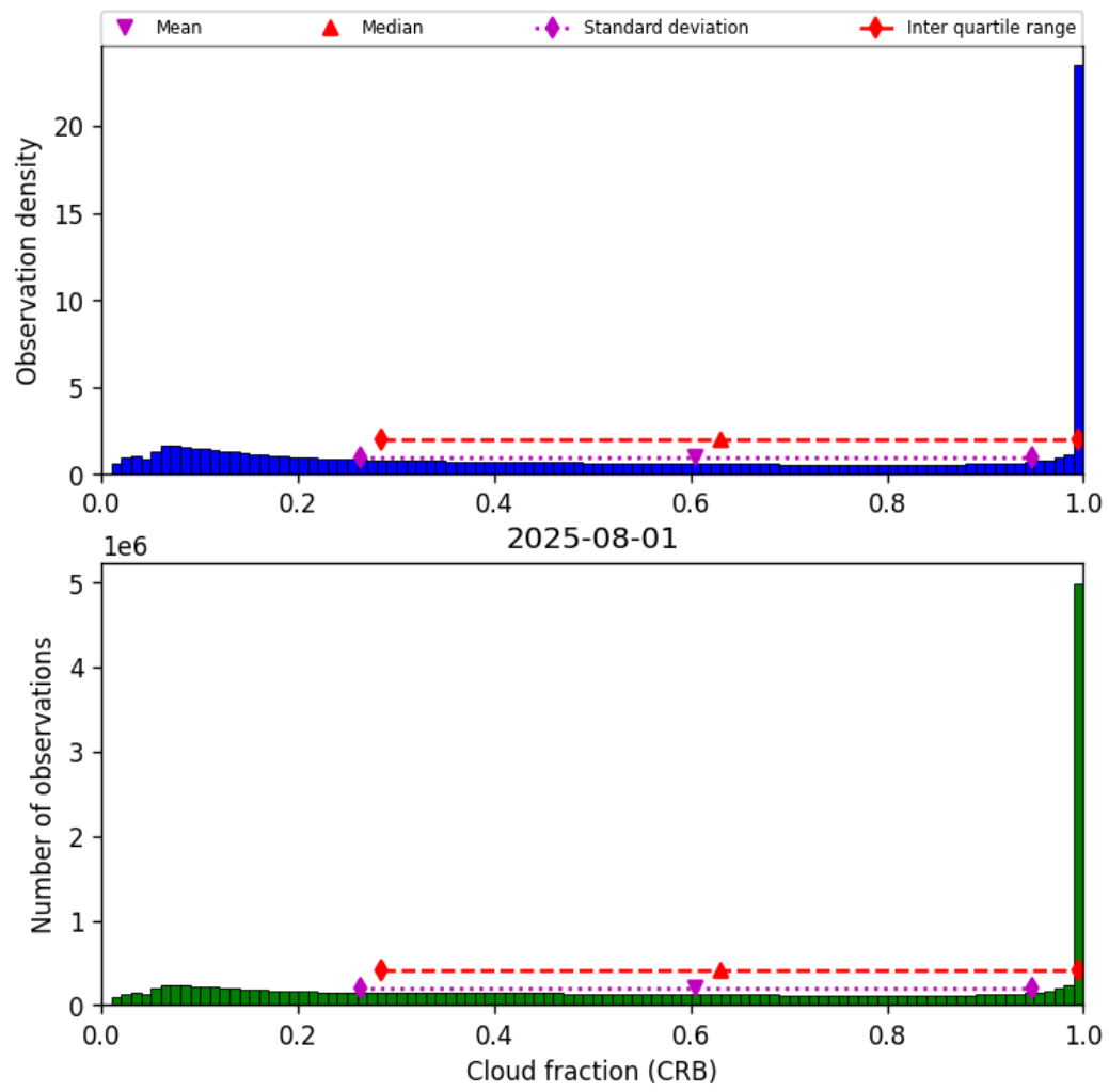
Figure 40: Histogram of “Cloud fraction (CRB)” for 2025-08-01 to 2025-08-01
