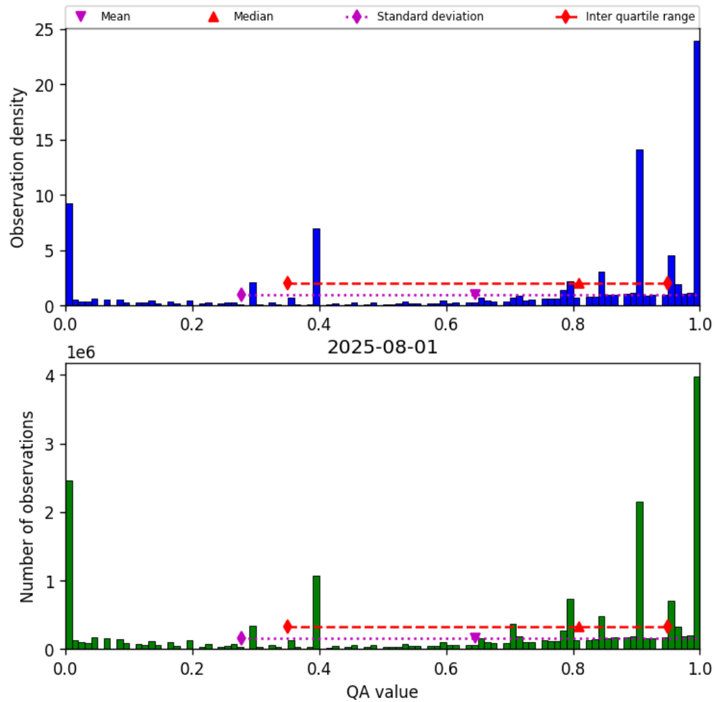
Figure 36: Histogram of “QA value” for 2025-08-01 to 2025-08-01
