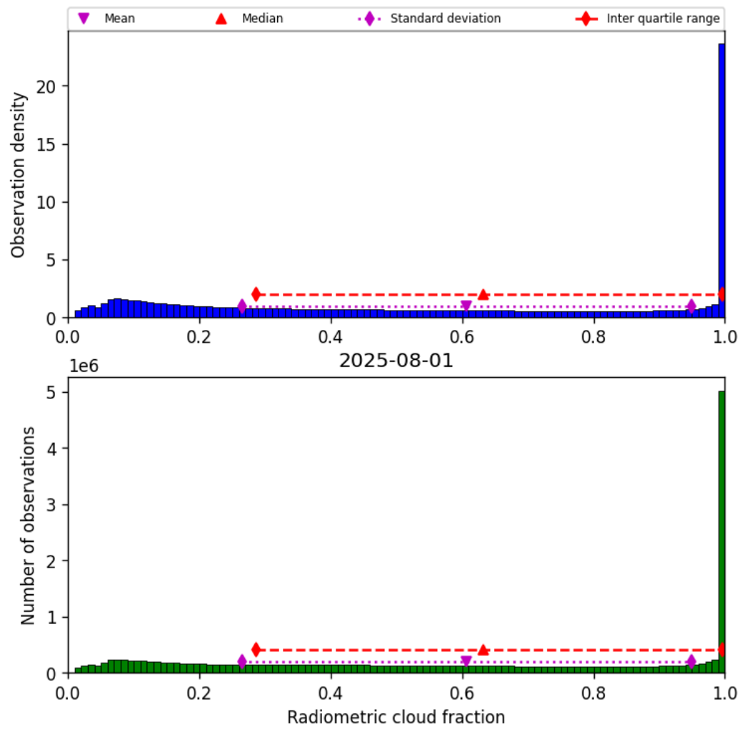
Figure 37: Histogram of “Radiometric cloud fraction” for 2025-08-01 to 2025-08-01
