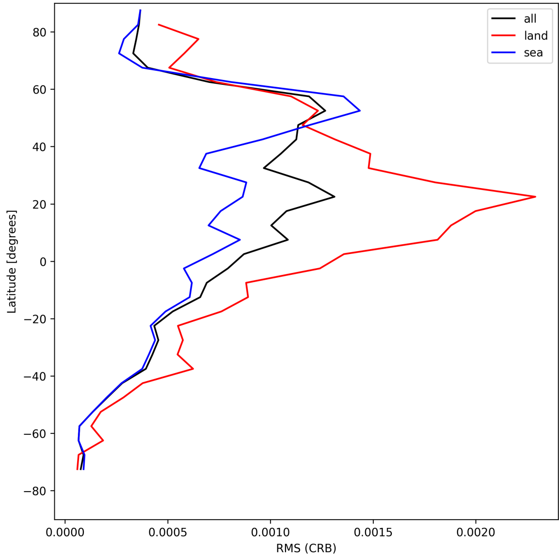
Figure 30: Zonal average of “RMS (CRB)” for 2025-08-01 to 2025-08-01.
