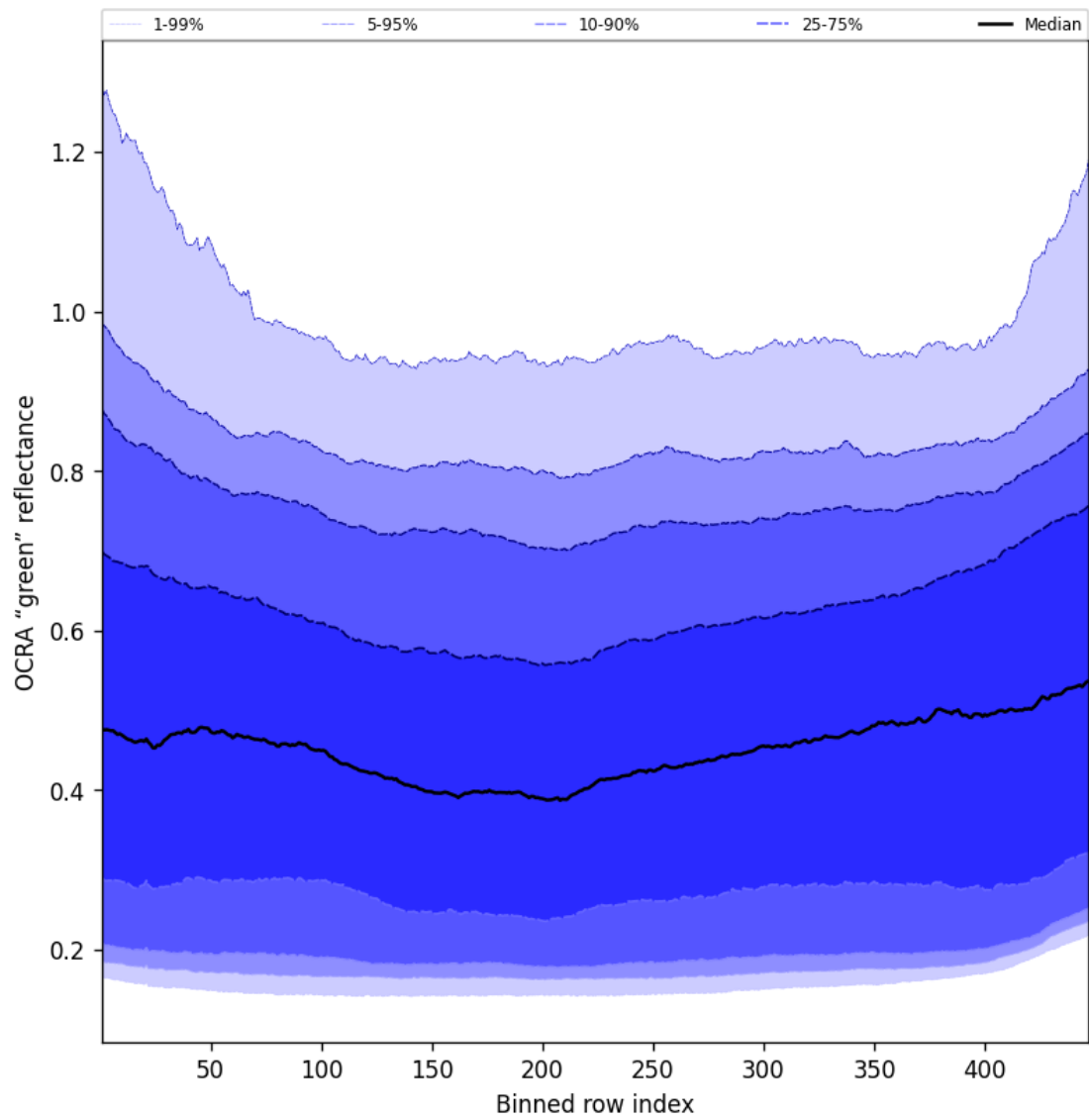
Figure 66: Along track statistics of “OCRA “green” reflectance” for 2025-08-01 to 2025-08-01
