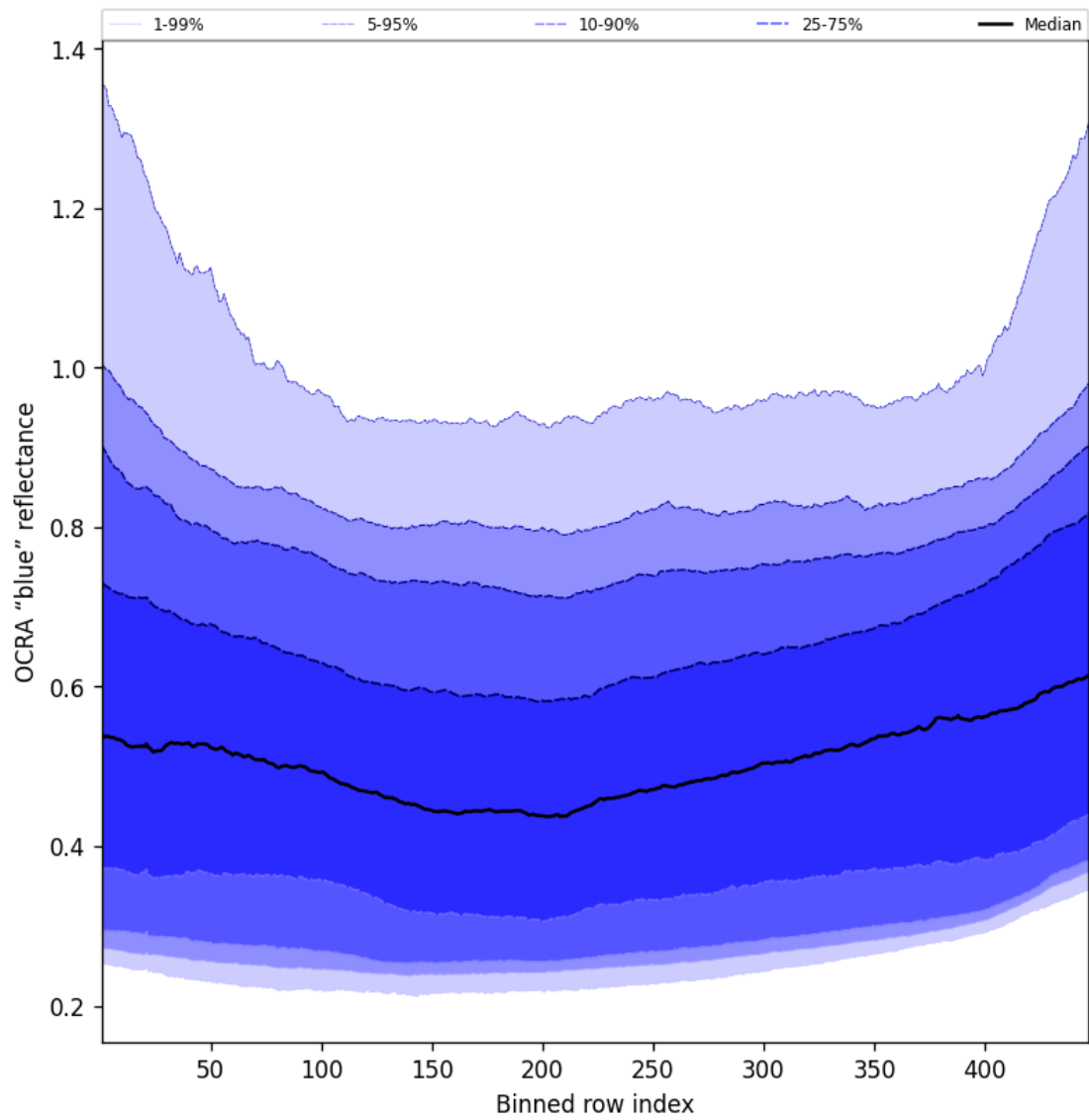
Figure 65: Along track statistics of “OCRA “blue” reflectance” for 2025-08-01 to 2025-08-01
