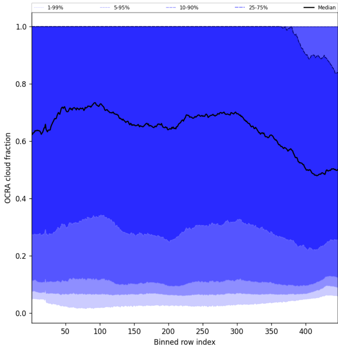
Figure 64: Along track statistics of “OCRA cloud fraction” for 2025-08-01 to 2025-08-01
