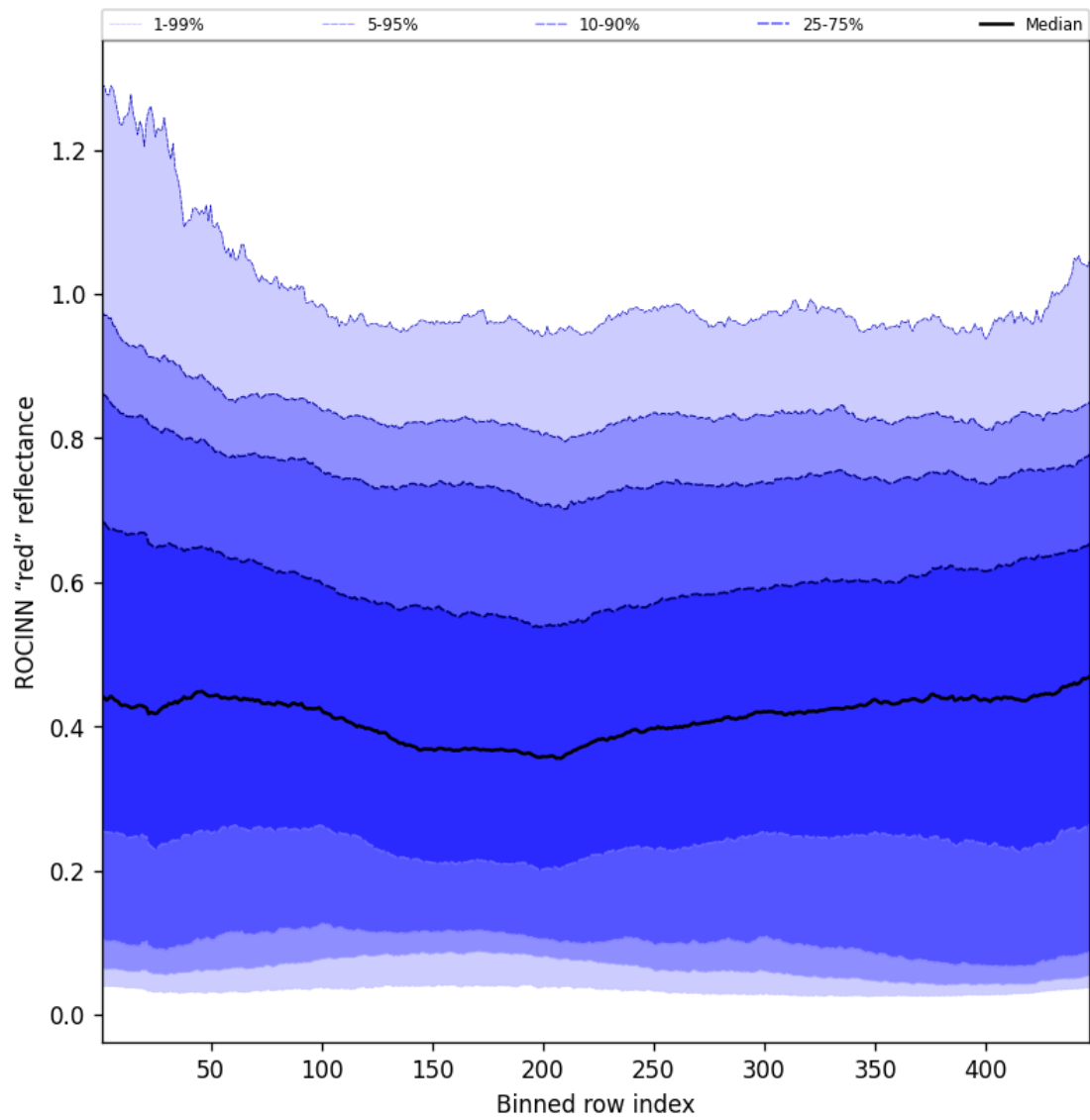
Figure 67: Along track statistics of "ROCINN "red" reflectance" for 2025-08-01 to 2025-08-01
