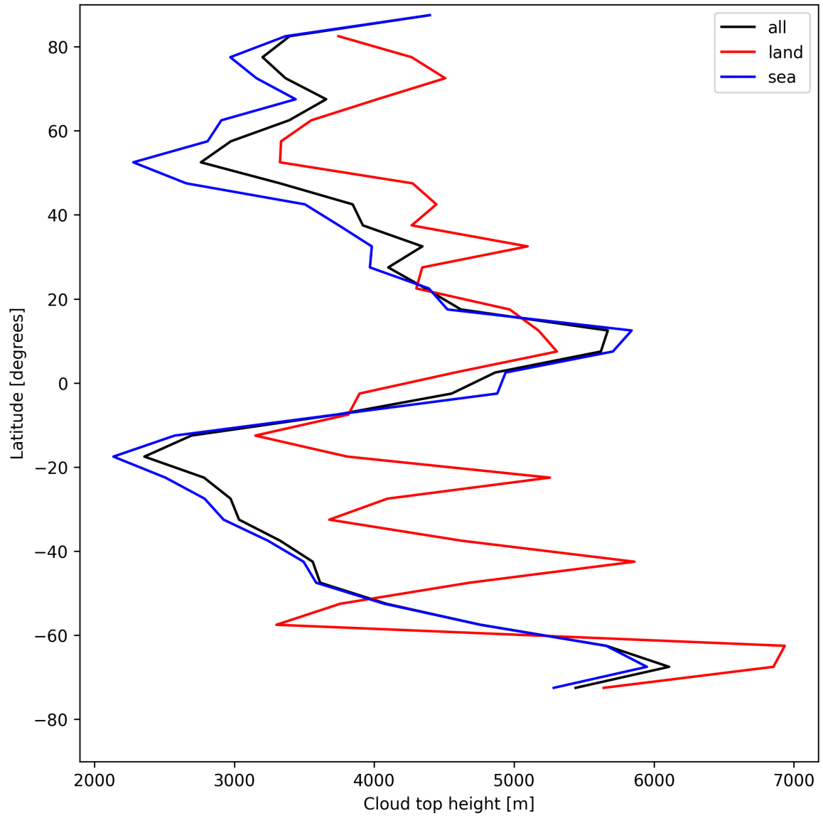
Figure 22: Zonal average of “Cloud top height” for 2025-08-01 to 2025-08-01.
