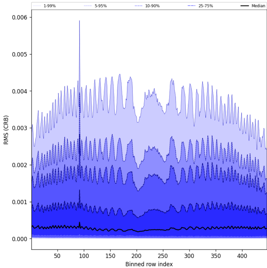
Figure 62: Along track statistics of “RMS (CRB)” for 2025-08-01 to 2025-08-01
