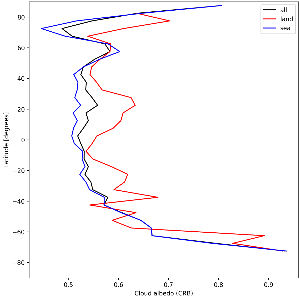
Figure 26: Zonal average of “Cloud albedo (CRB)” for 2025-08-01 to 2025-08-01.
