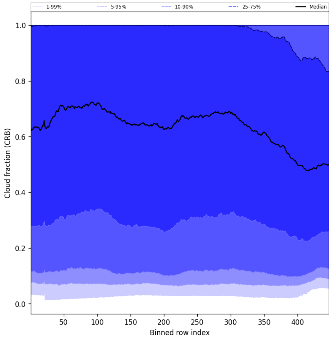
Figure 56: Along track statistics of “Cloud fraction (CRB)” for 2025-08-01 to 2025-08-01
