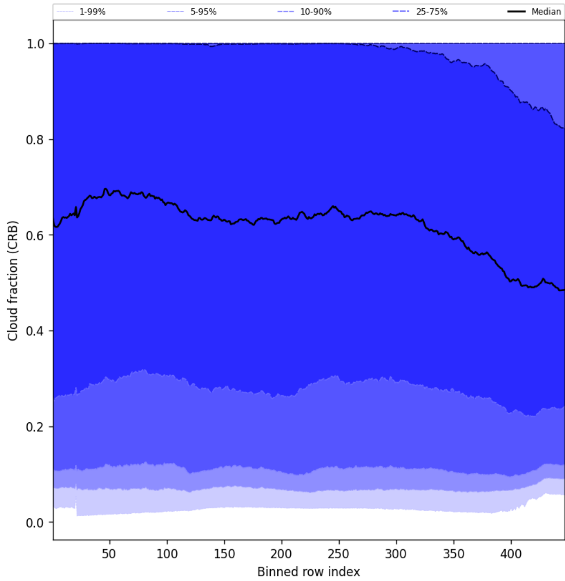
Figure 56: Along track statistics of “Cloud fraction (CRB)” for 2025-08-02 to 2025-08-03
