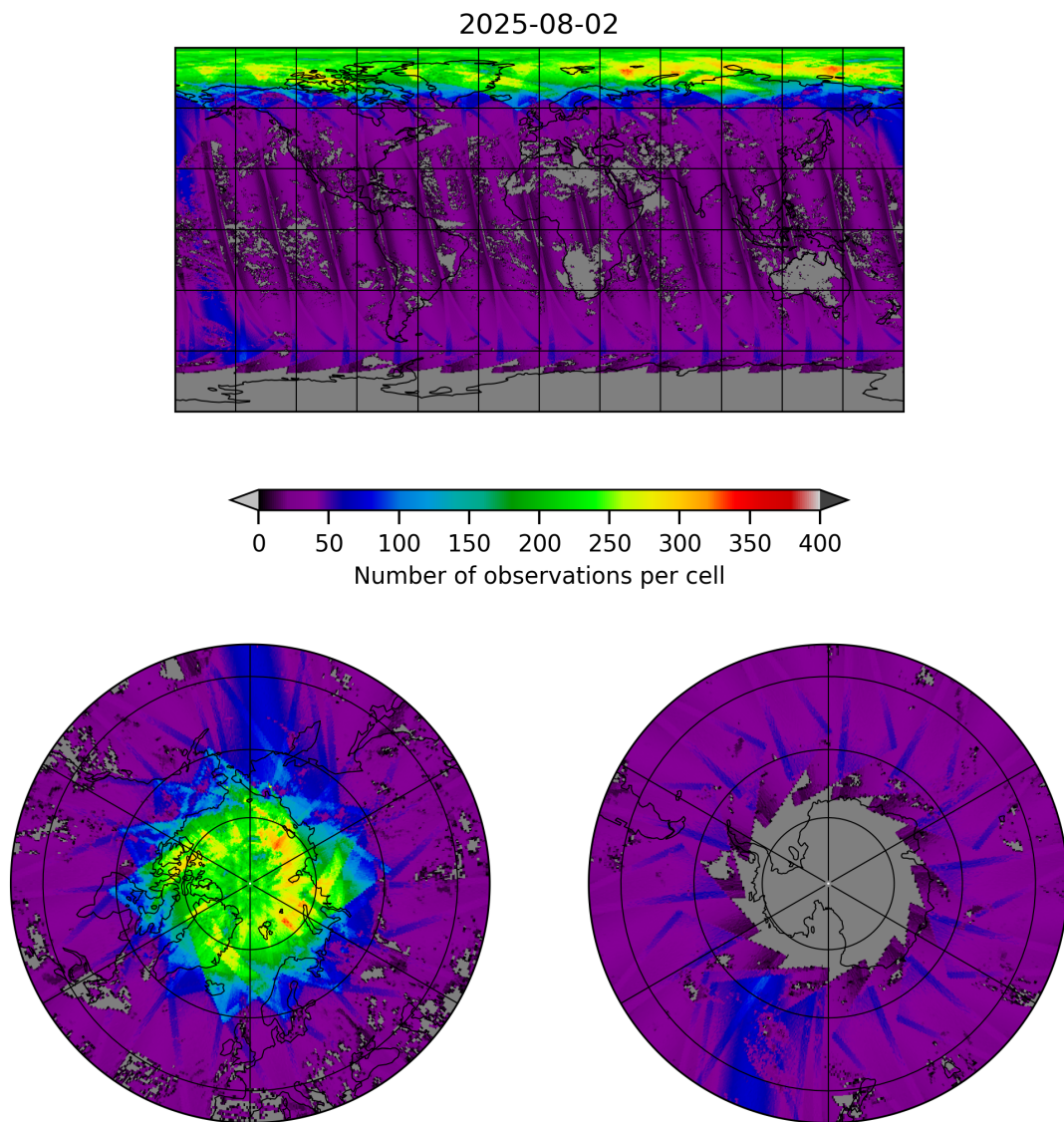
Figure 19: Map of the number of observations for 2025-08-02 to 2025-08-03
