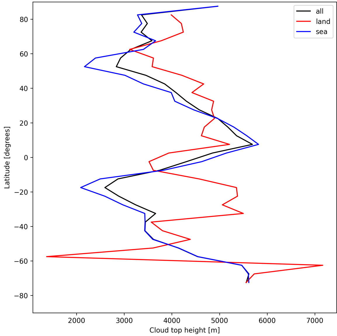
Figure 22: Zonal average of “Cloud top height” for 2025-08-02 to 2025-08-03.
