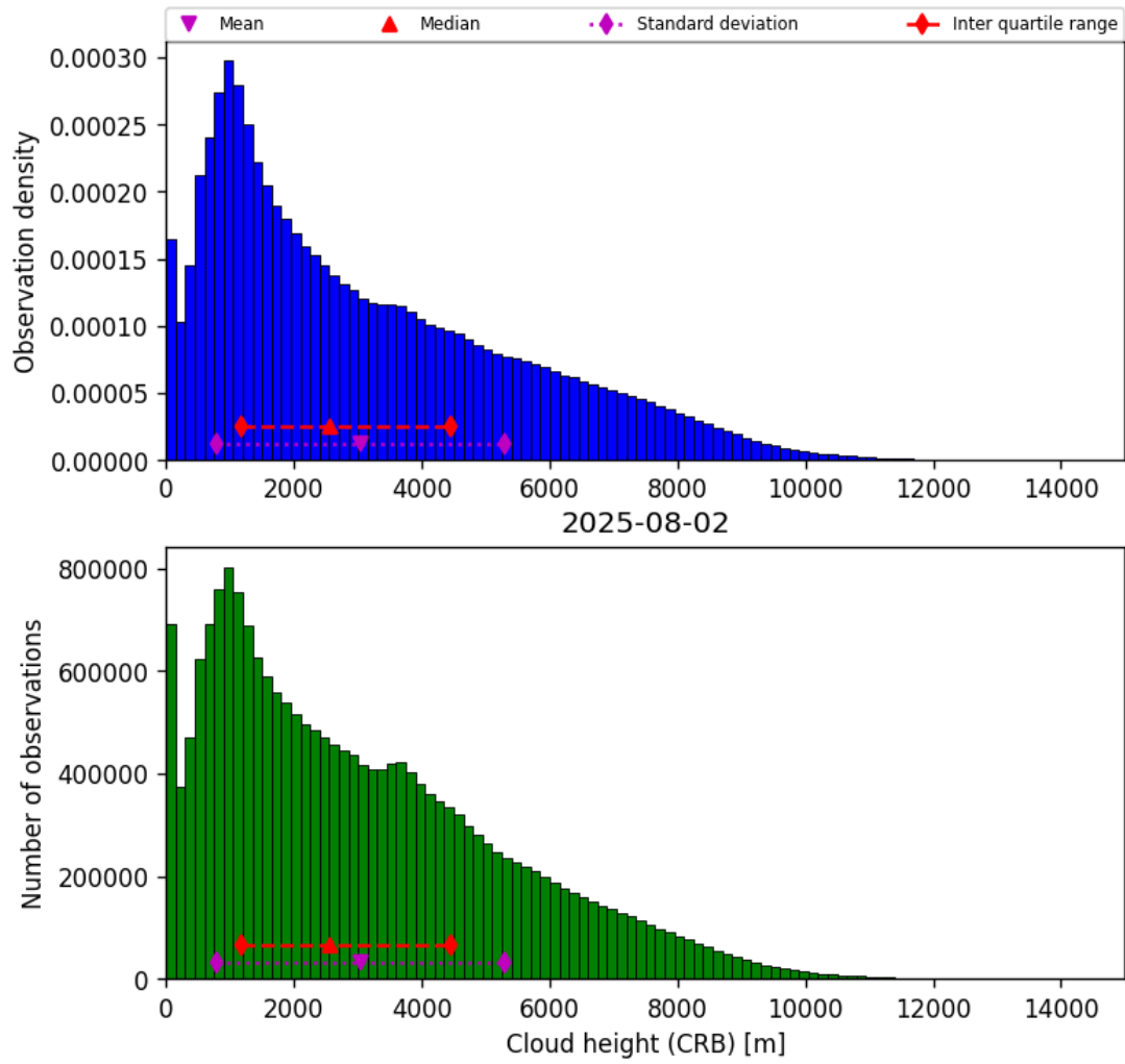
Figure 41: Histogram of “Cloud height (CRB)” for 2025-08-02 to 2025-08-03
