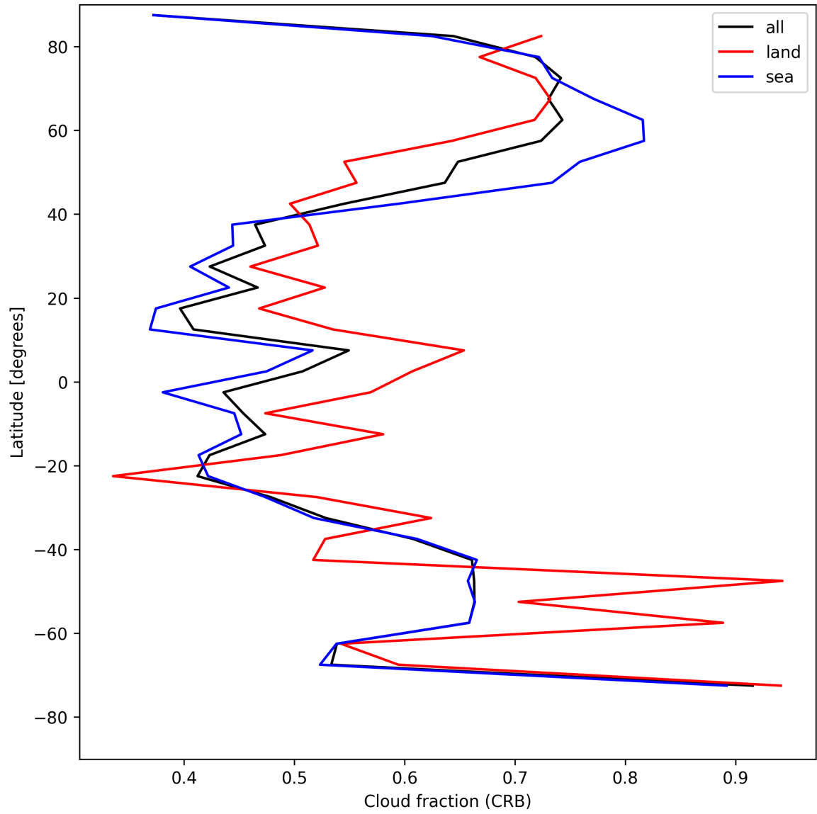
Figure 24: Zonal average of “Cloud fraction (CRB)” for 2025-08-02 to 2025-08-03.
