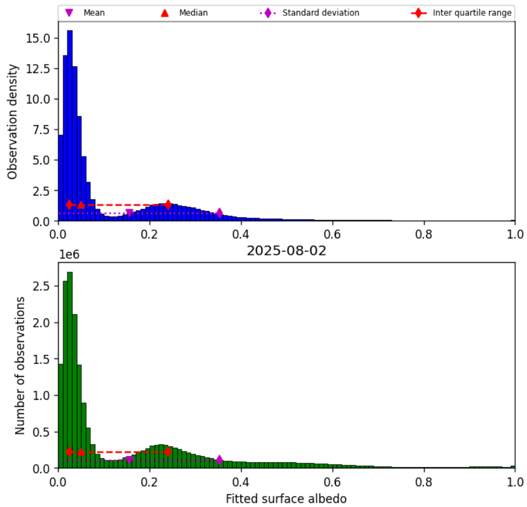
Figure 43: Histogram of “Fitted surface albedo” for 2025-08-02 to 2025-08-03
