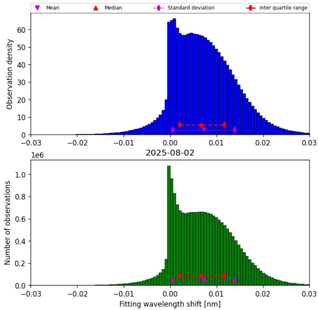
Figure 47: Histogram of “Fitting wavelength shift” for 2025-08-02 to 2025-08-03
