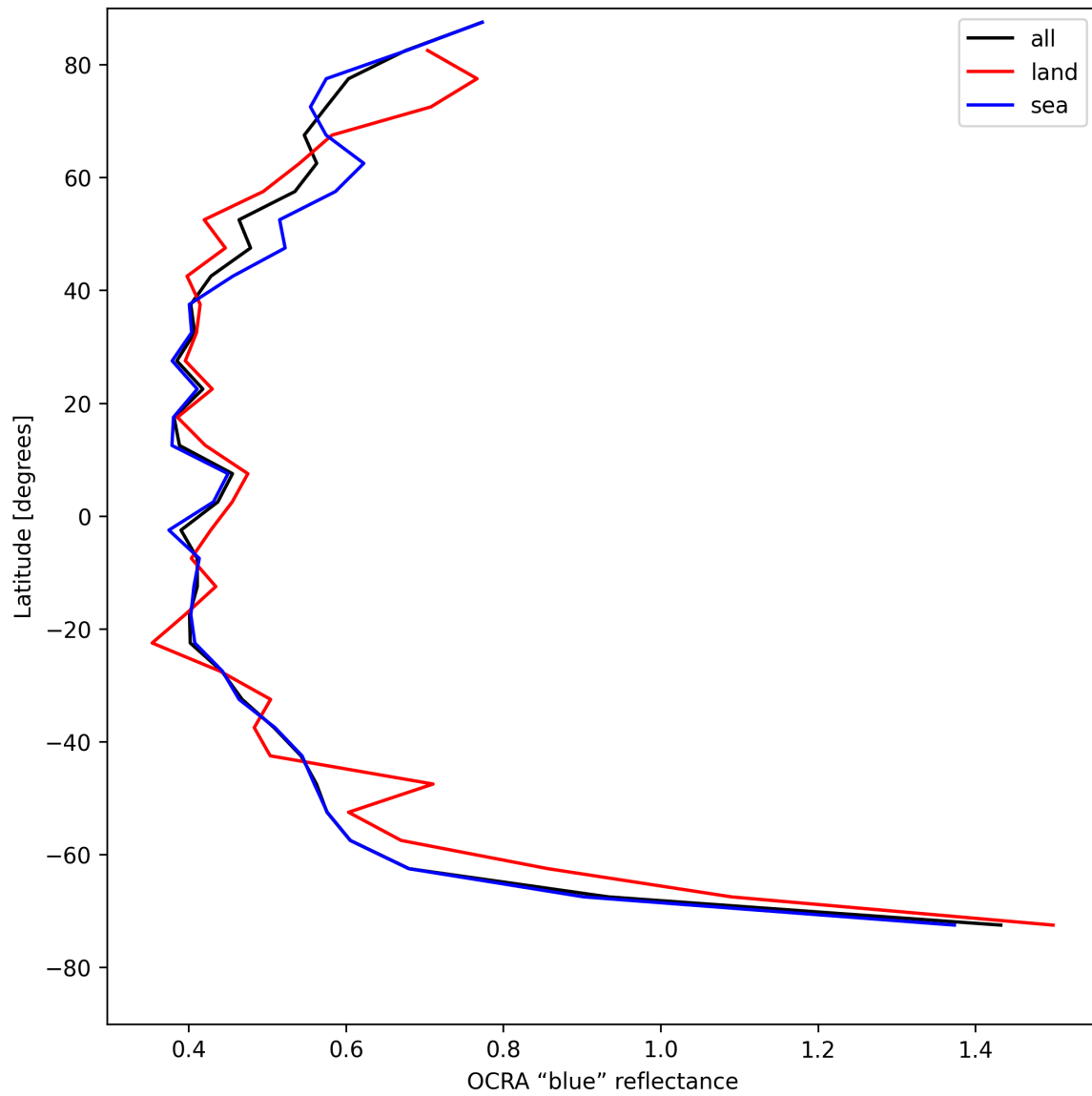
Figure 33: Zonal average of “OCRA “blue” reflectance” for 2025-08-02 to 2025-08-03.
