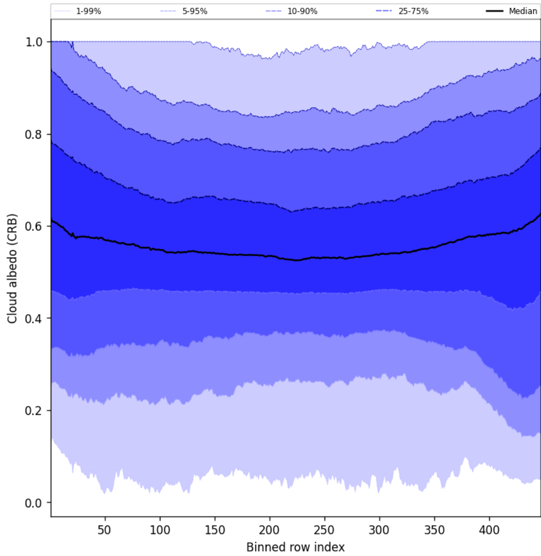
Figure 58: Along track statistics of “Cloud albedo (CRB)” for 2025-08-02 to 2025-08-03
