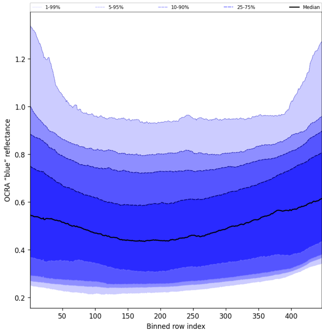
Figure 65: Along track statistics of “OCRA “blue” reflectance” for 2025-08-02 to 2025-08-03
