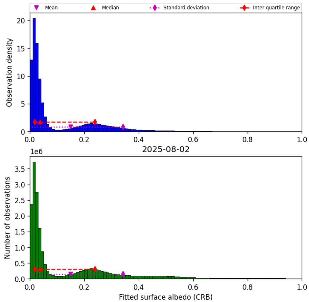
Figure 44: Histogram of “Fitted surface albedo (CRB)” for 2025-08-02 to 2025-08-03
