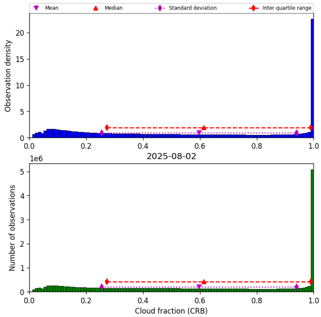
Figure 40: Histogram of “Cloud fraction (CRB)” for 2025-08-02 to 2025-08-03
