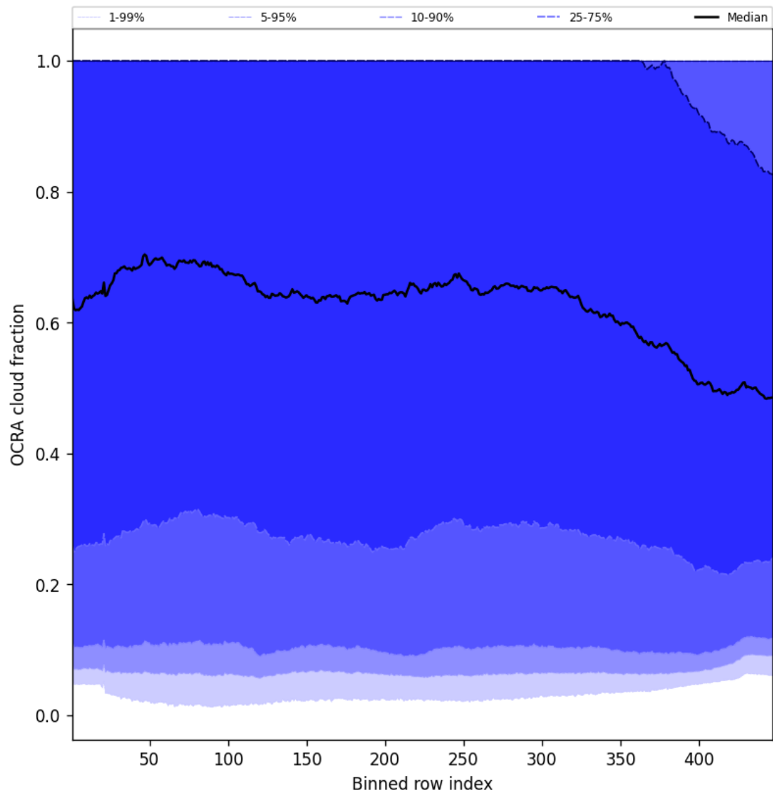
Figure 64: Along track statistics of “OCRA cloud fraction” for 2025-08-02 to 2025-08-03
