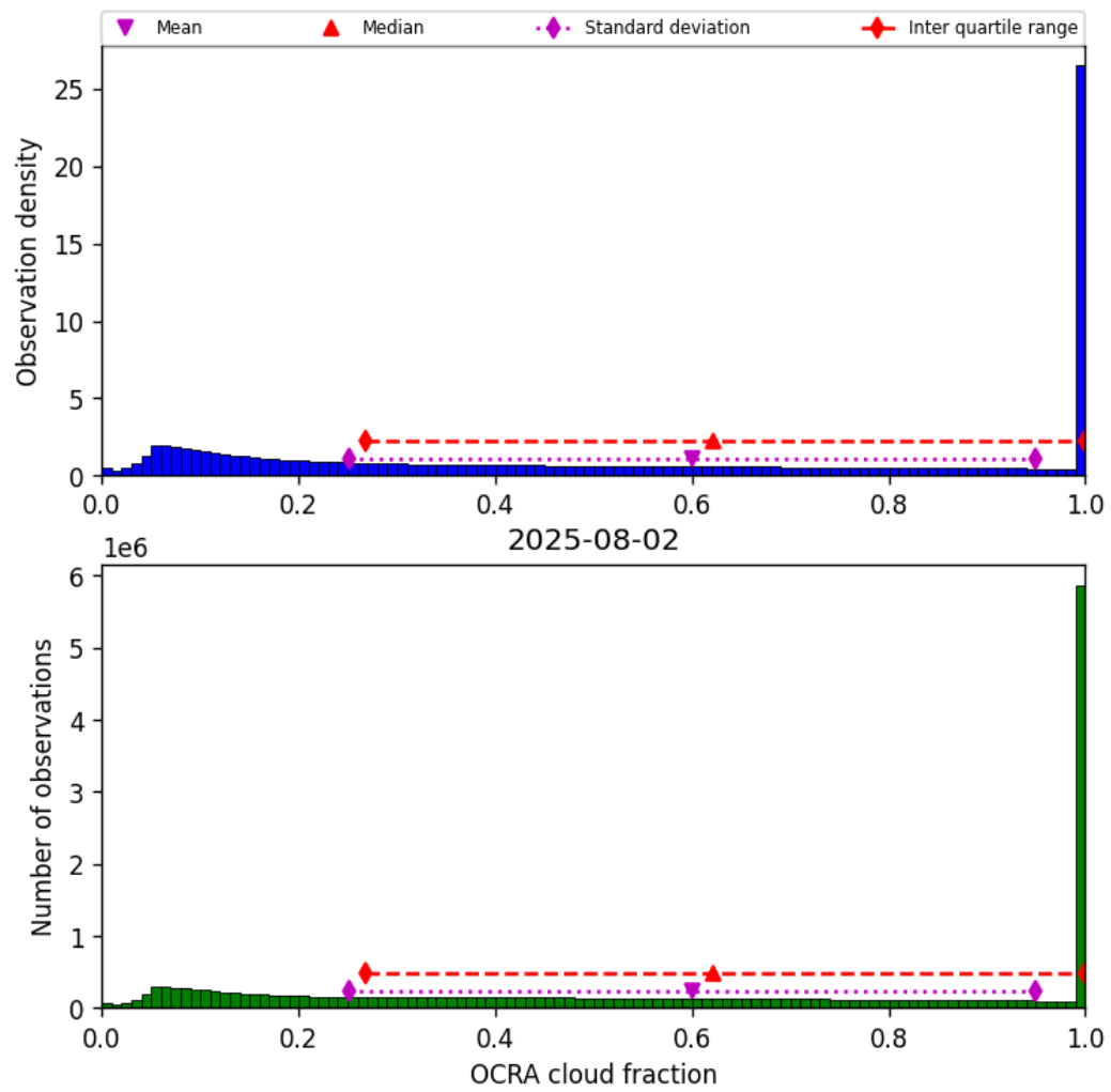
Figure 48: Histogram of “OCRA cloud fraction” for 2025-08-02 to 2025-08-03
