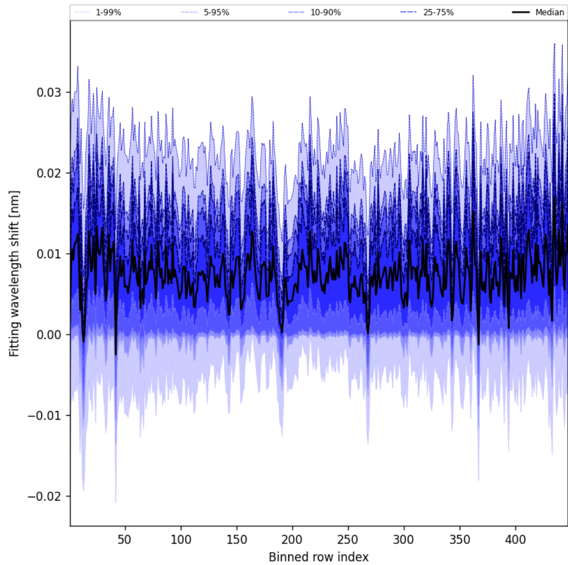
Figure 63: Along track statistics of “Fitting wavelength shift” for 2025-08-02 to 2025-08-03
