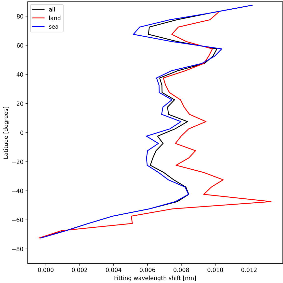
Figure 31: Zonal average of “Fitting wavelength shift” for 2025-08-02 to 2025-08-03.
