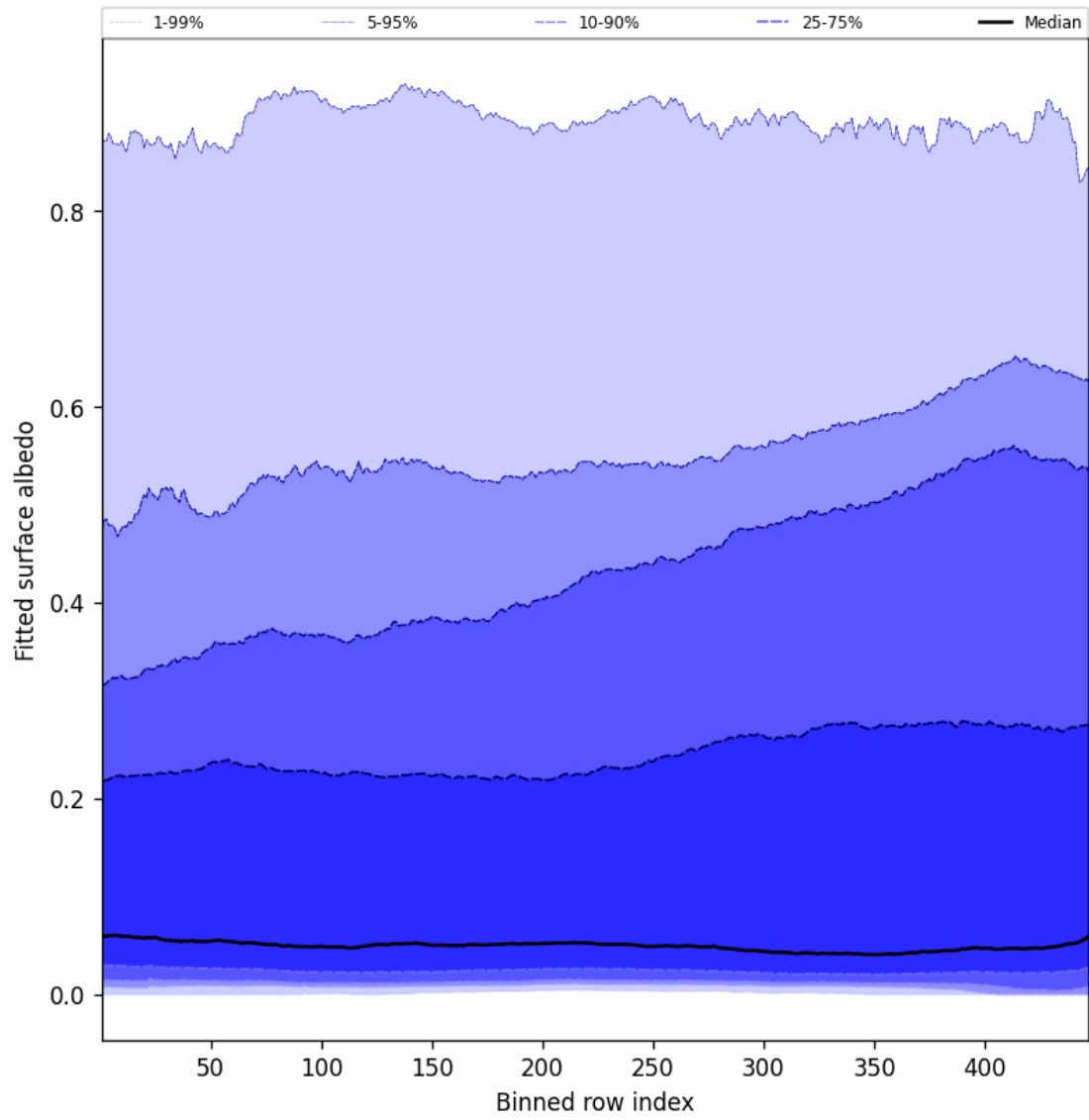
Figure 59: Along track statistics of “Fitted surface albedo” for 2025-08-02 to 2025-08-03
