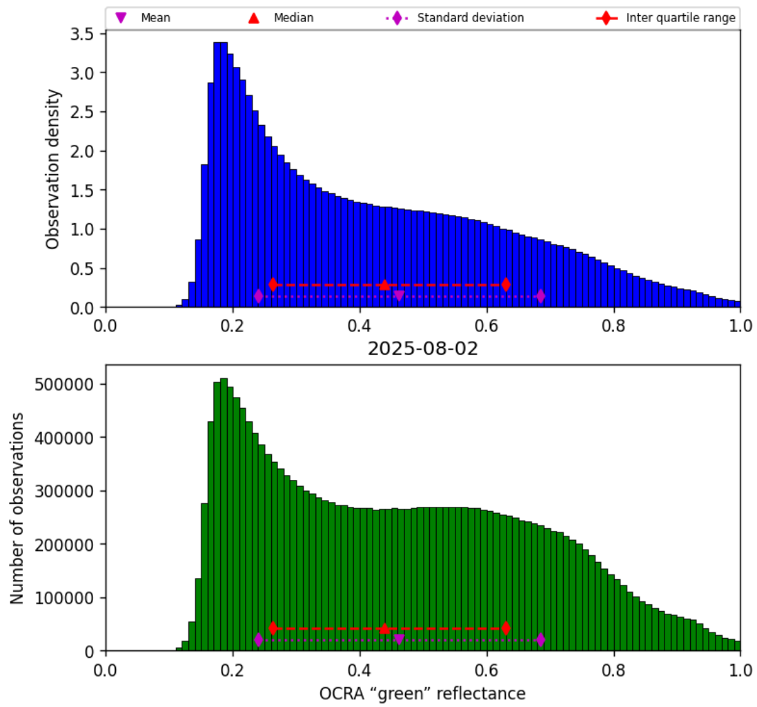
Figure 50: Histogram of “OCRA “green” reflectance” for 2025-08-02 to 2025-08-03
