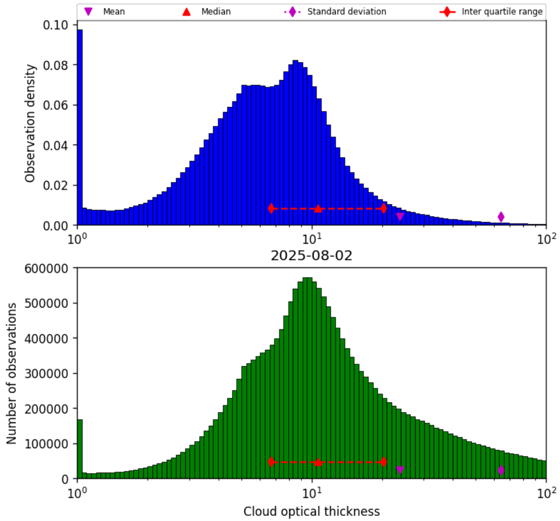
Figure 39: Histogram of “Cloud optical thickness” for 2025-08-02 to 2025-08-03
