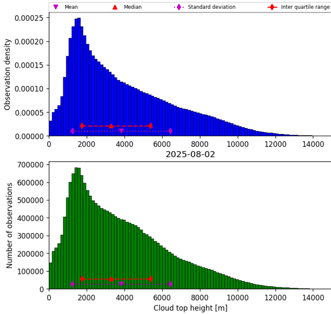
Figure 38: Histogram of “Cloud top height” for 2025-08-02 to 2025-08-03
