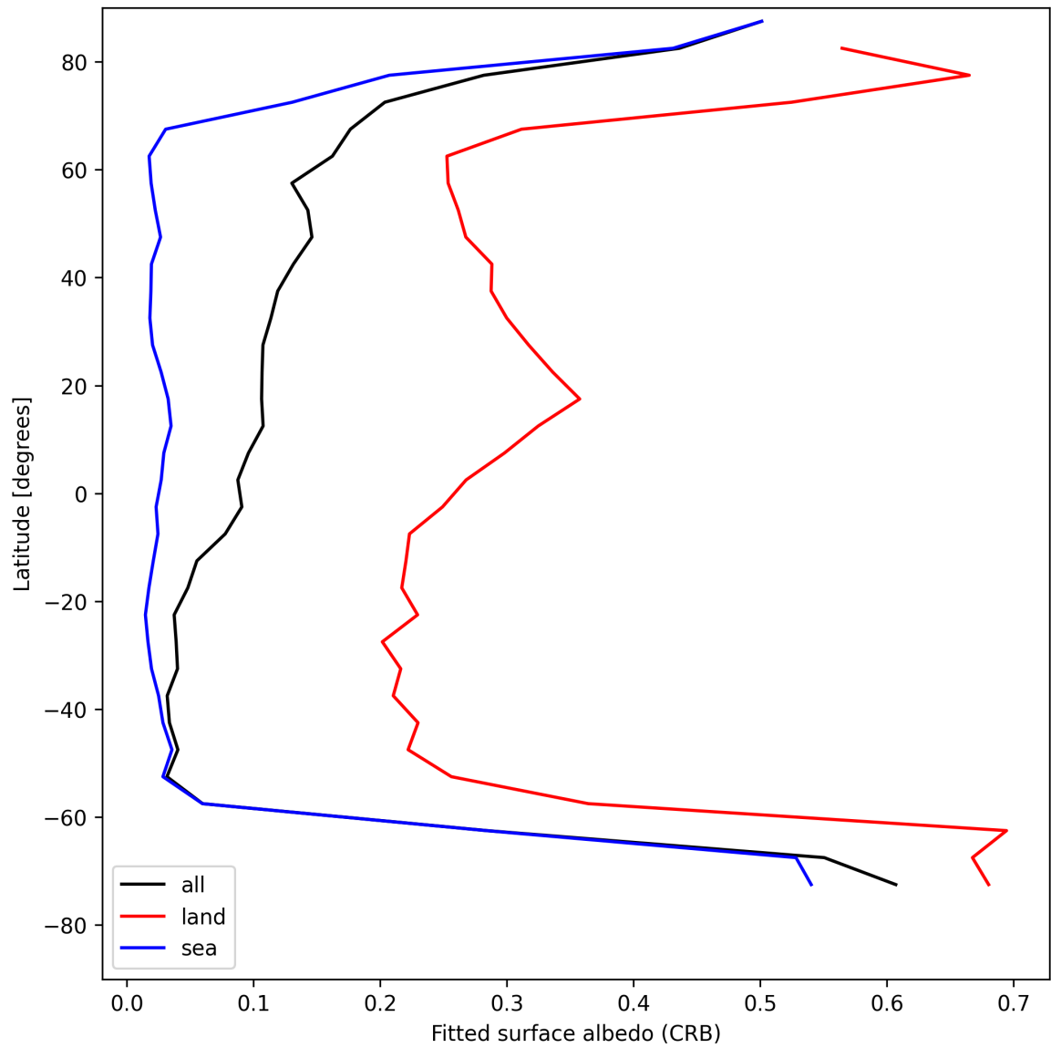
Figure 28: Zonal average of “Fitted surface albedo (CRB)” for 2025-08-02 to 2025-08-03.
