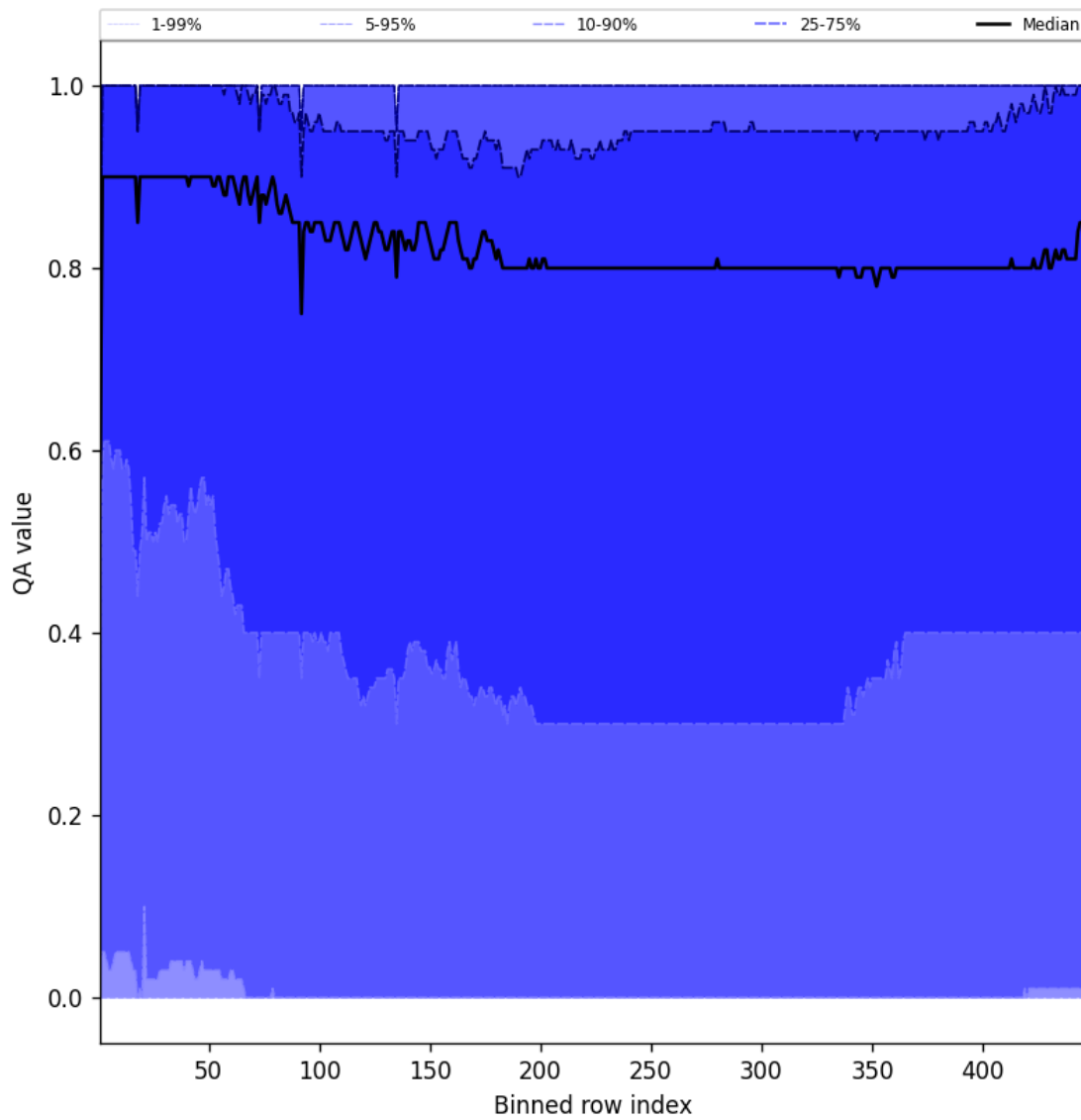
Figure 52: Along track statistics of “QA value” for 2025-08-02 to 2025-08-03
