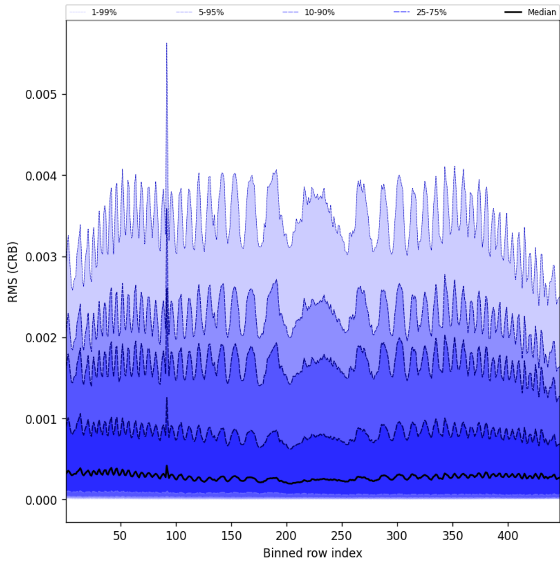
Figure 62: Along track statistics of “RMS (CRB)” for 2025-08-02 to 2025-08-03
