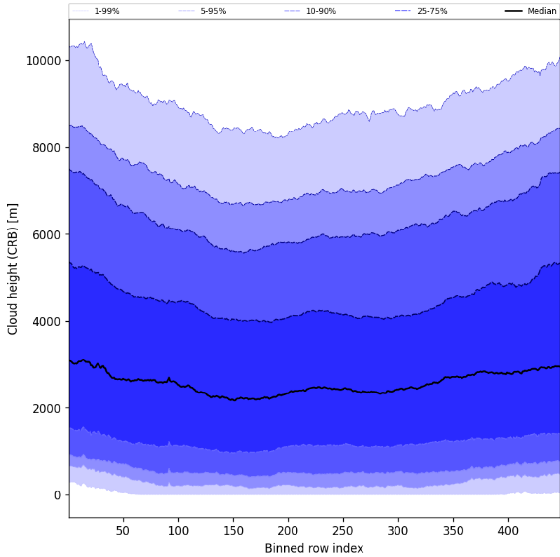
Figure 57: Along track statistics of “Cloud height (CRB)” for 2025-08-02 to 2025-08-03
