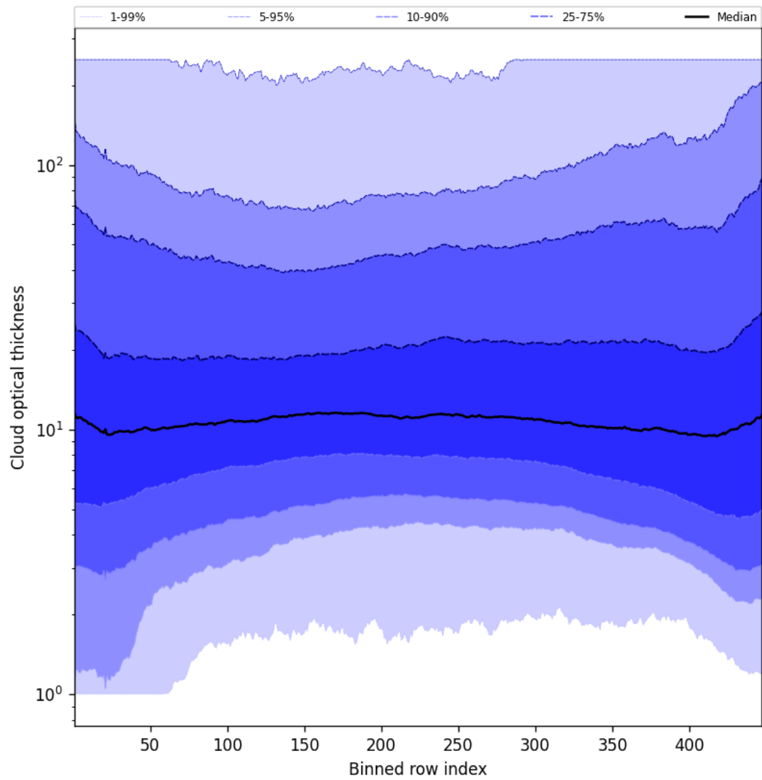
Figure 55: Along track statistics of “Cloud optical thickness” for 2025-08-02 to 2025-08-03
