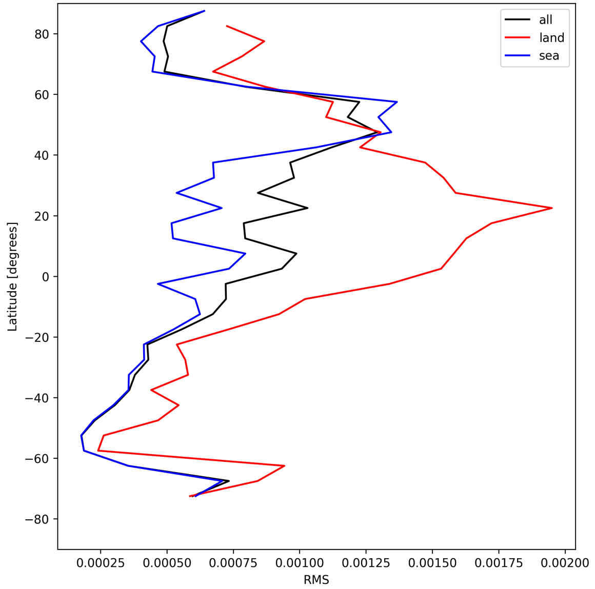
Figure 29: Zonal average of “RMS” for 2025-08-02 to 2025-08-03.
