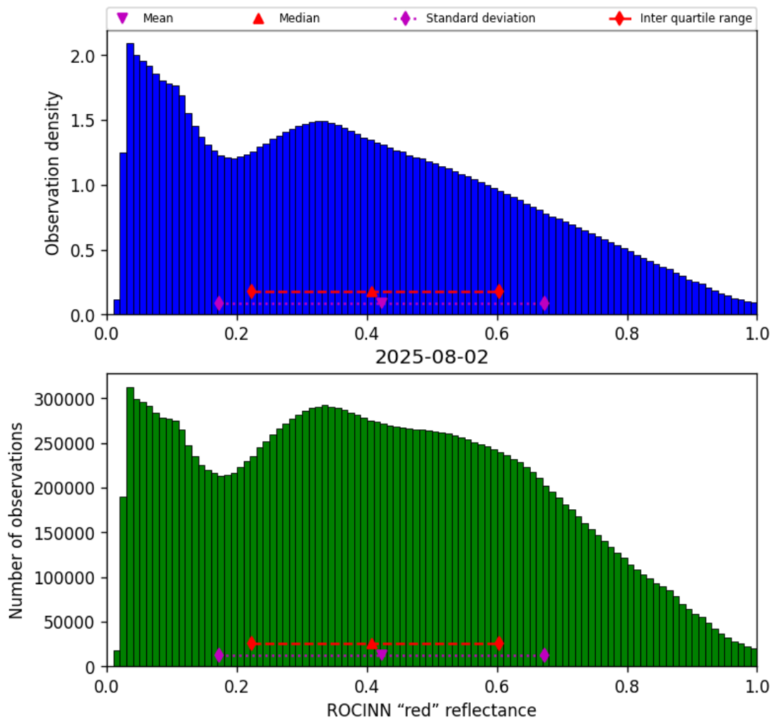
Figure 51: Histogram of “ROCINN “red” reflectance” for 2025-08-02 to 2025-08-03
