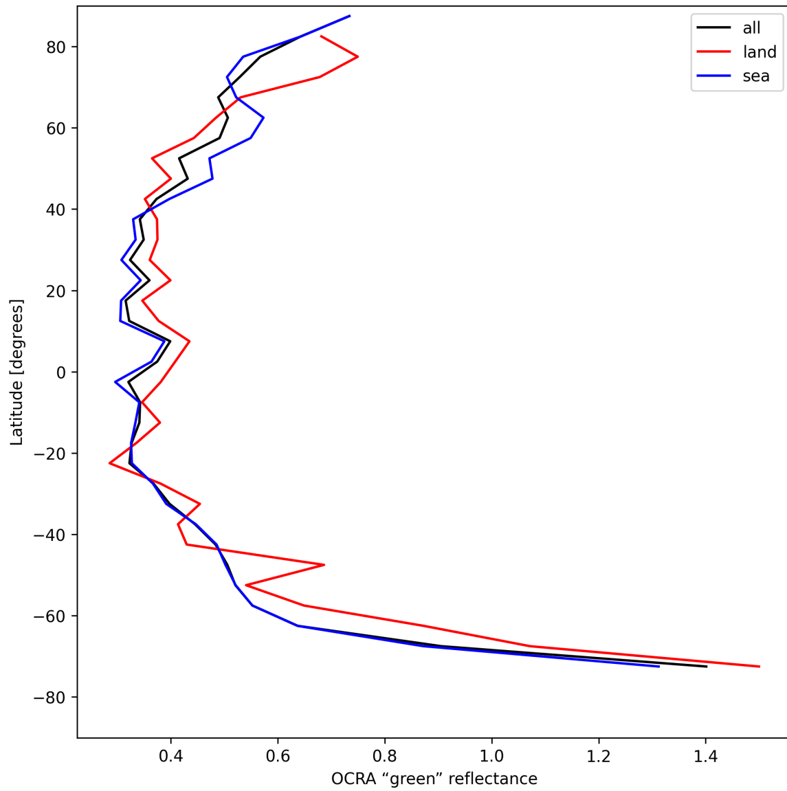
Figure 34: Zonal average of “OCRA “green” reflectance” for 2025-08-02 to 2025-08-03.
