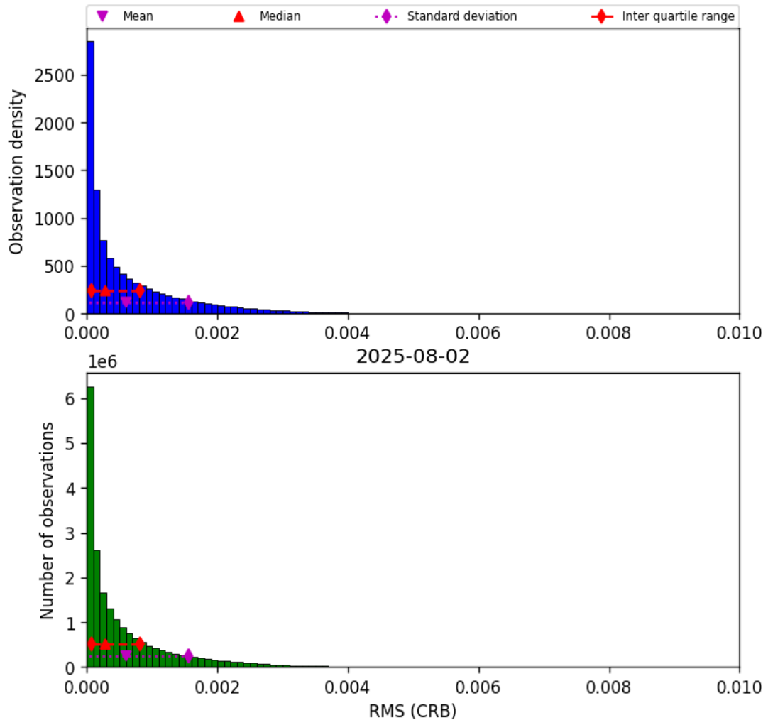
Figure 46: Histogram of “RMS (CRB)” for 2025-08-02 to 2025-08-03
