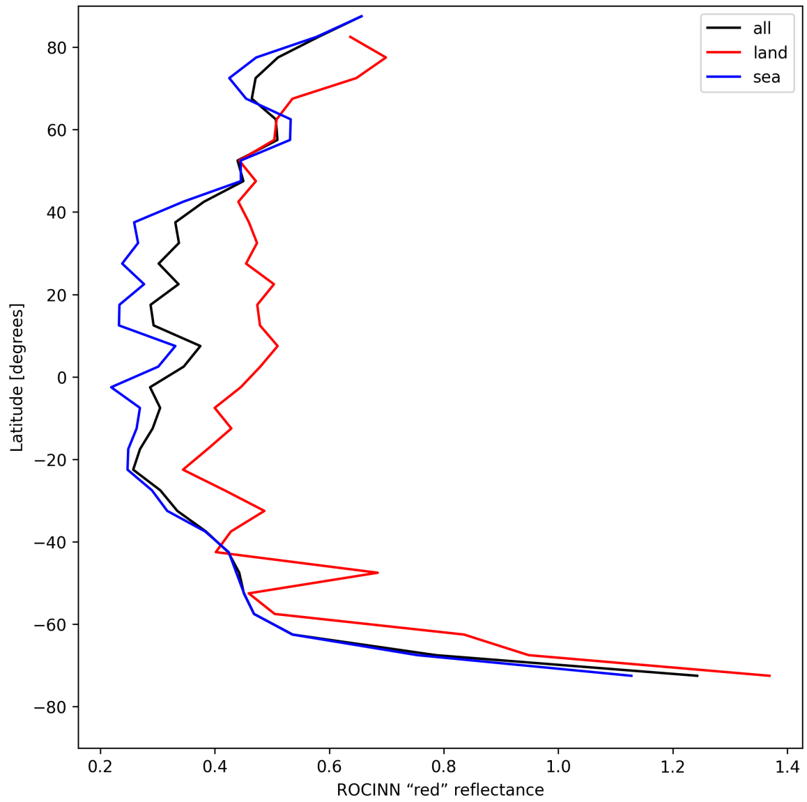
Figure 35: Zonal average of “ROCINN “red” reflectance” for 2025-08-02 to 2025-08-03.
