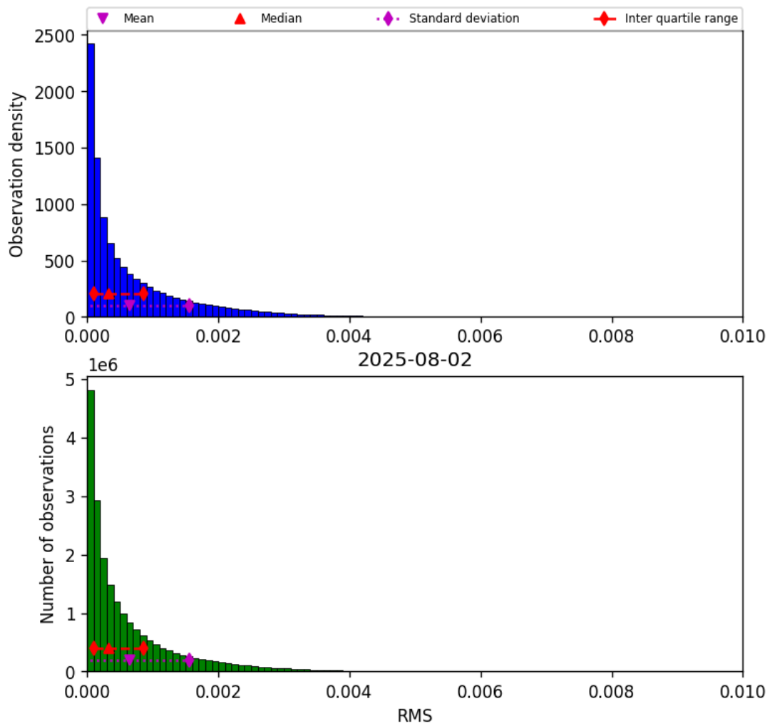
Figure 45: Histogram of “RMS” for 2025-08-02 to 2025-08-03
