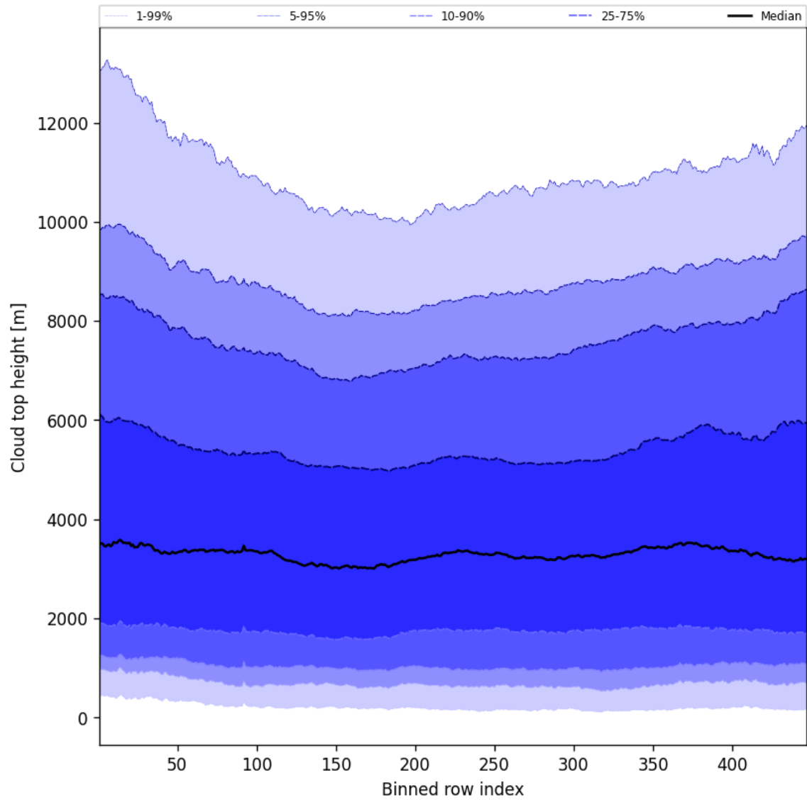
Figure 54: Along track statistics of “Cloud top height” for 2025-08-02 to 2025-08-03
