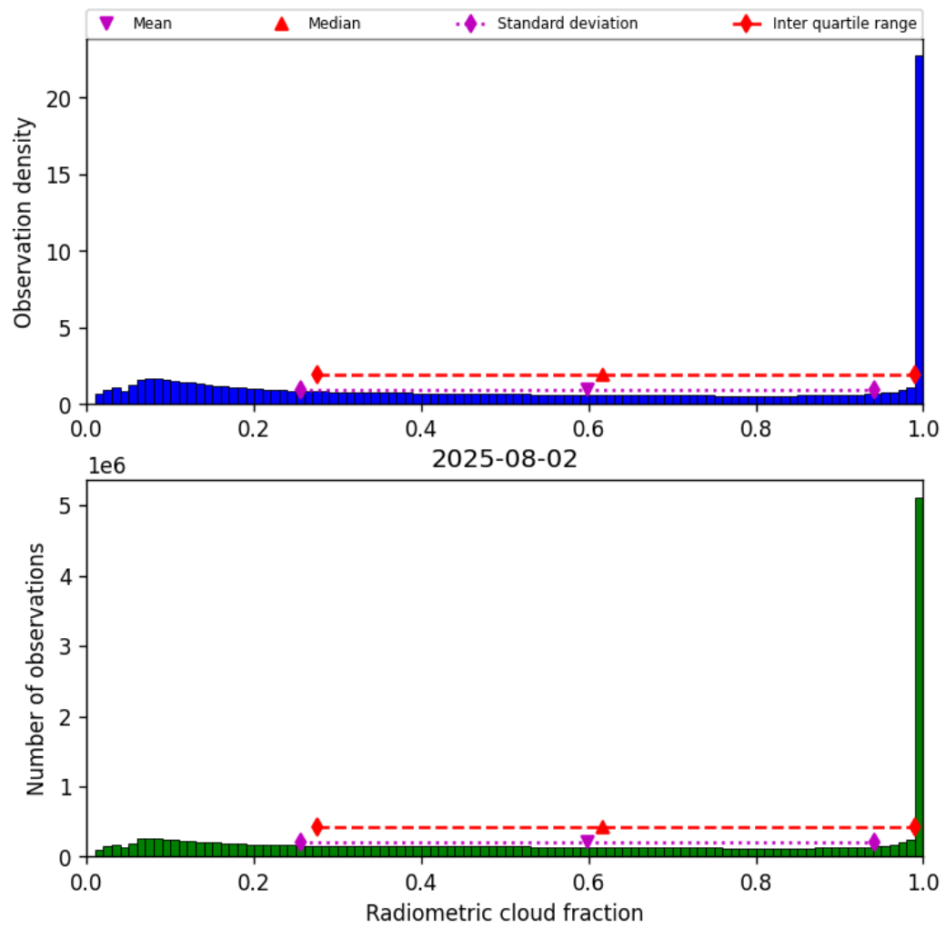
Figure 37: Histogram of “Radiometric cloud fraction” for 2025-08-02 to 2025-08-03
