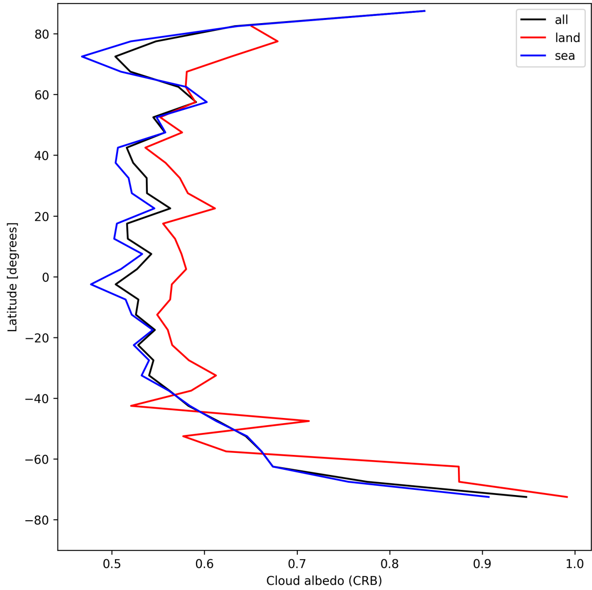
Figure 26: Zonal average of “Cloud albedo (CRB)” for 2025-08-02 to 2025-08-03.
