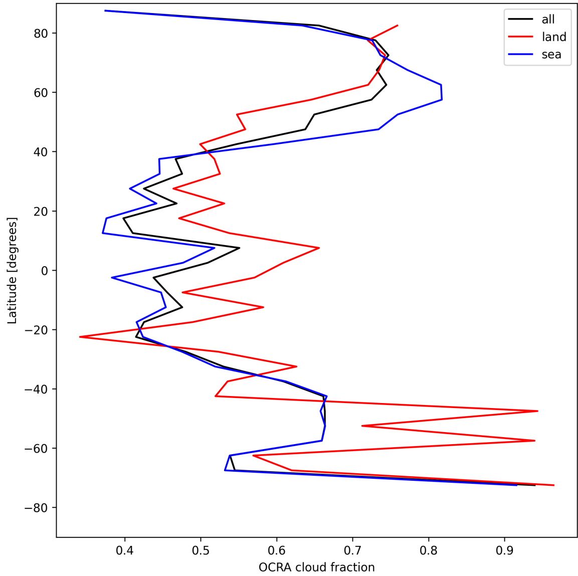
Figure 32: Zonal average of “OCRA cloud fraction” for 2025-08-02 to 2025-08-03.
