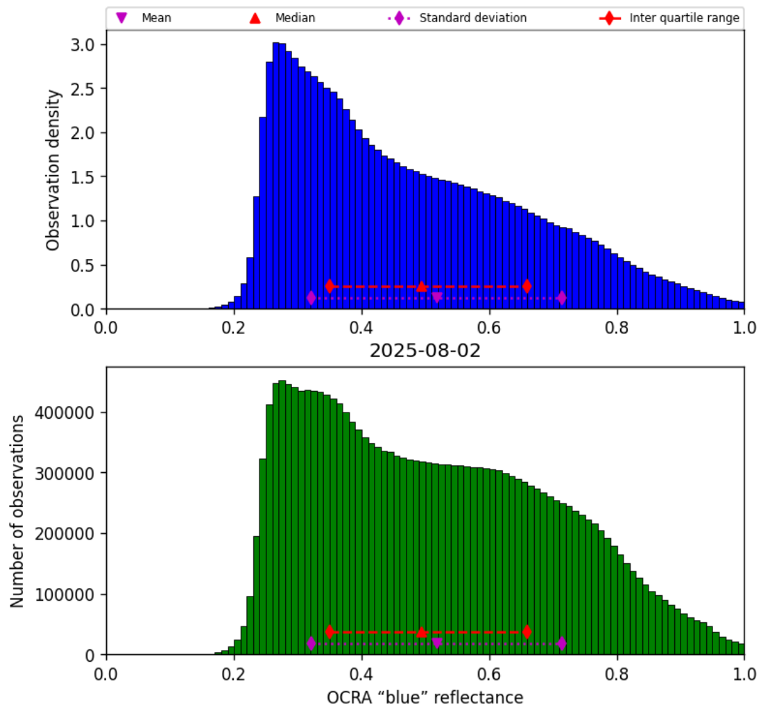
Figure 49: Histogram of “OCRA “blue” reflectance” for 2025-08-02 to 2025-08-03
