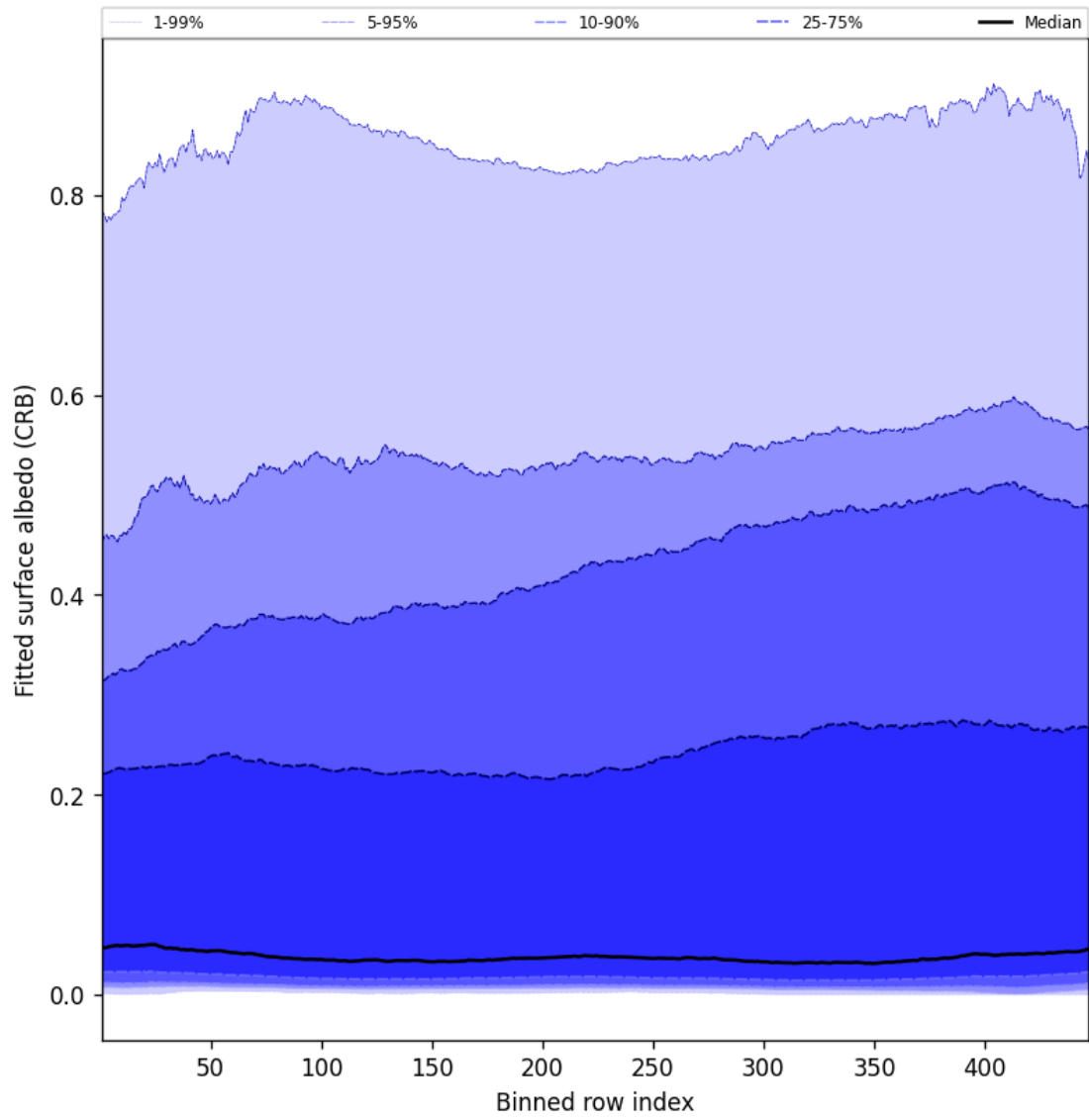
Figure 60: Along track statistics of “Fitted surface albedo (CRB)” for 2025-08-02 to 2025-08-03
