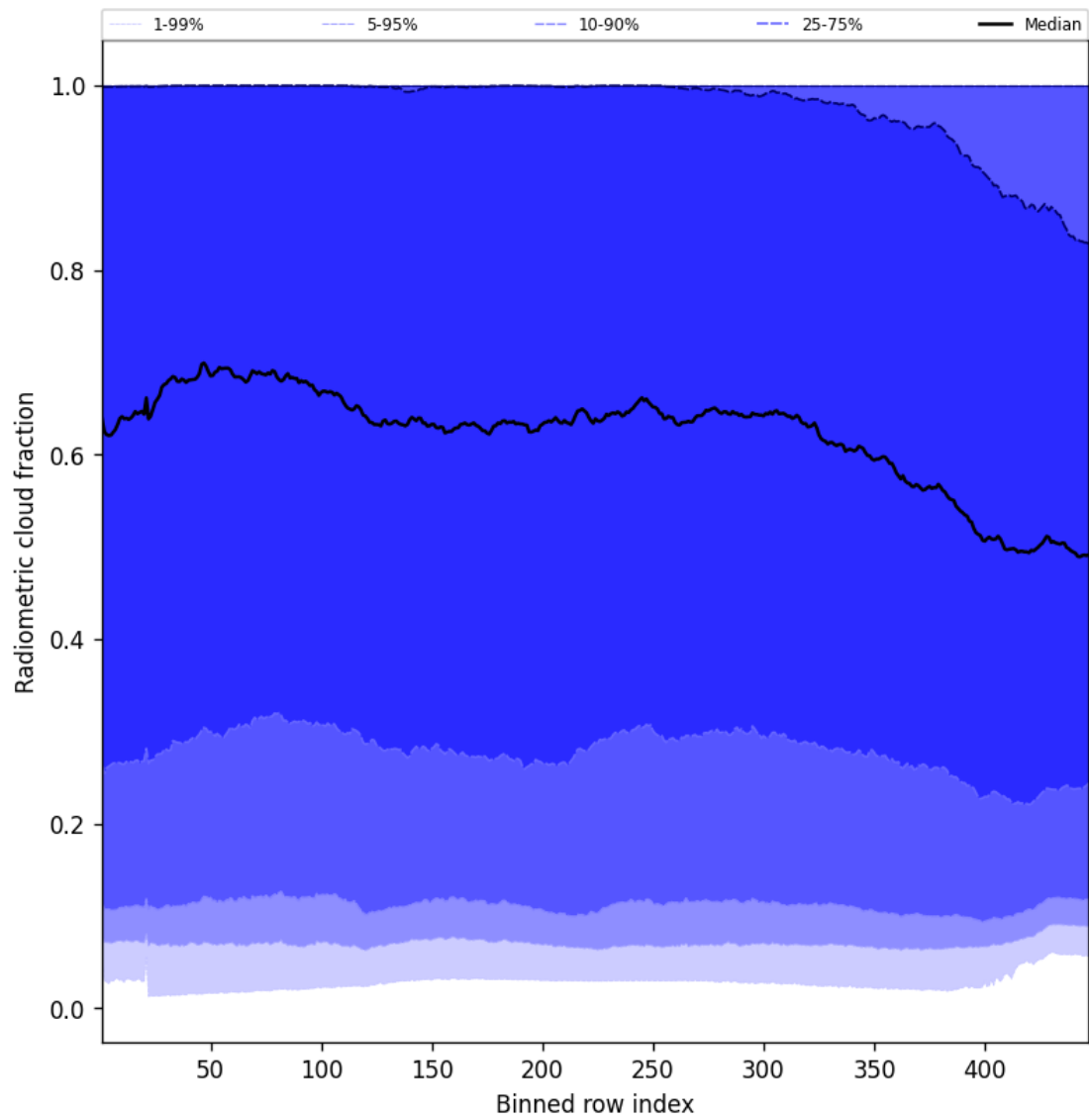
Figure 53: Along track statistics of “Radiometric cloud fraction” for 2025-08-02 to 2025-08-03
