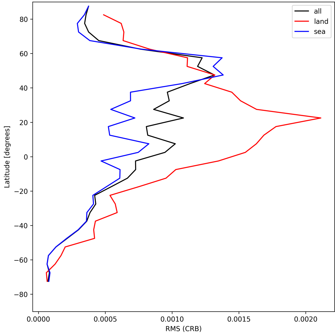
Figure 30: Zonal average of “RMS (CRB)” for 2025-08-02 to 2025-08-03.
