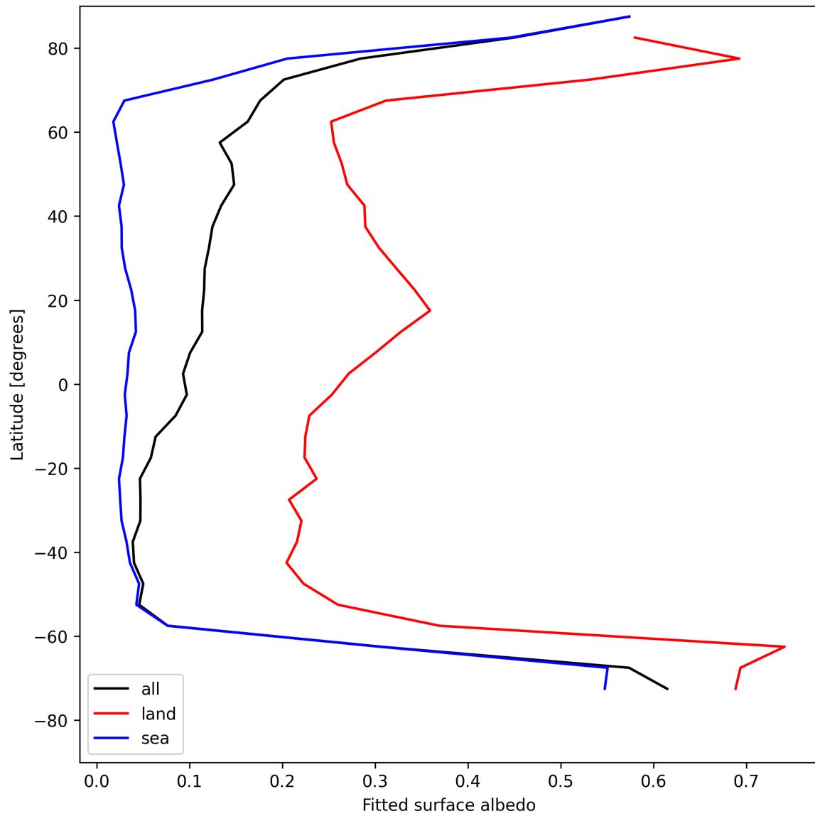
Figure 27: Zonal average of “Fitted surface albedo” for 2025-08-02 to 2025-08-03.
