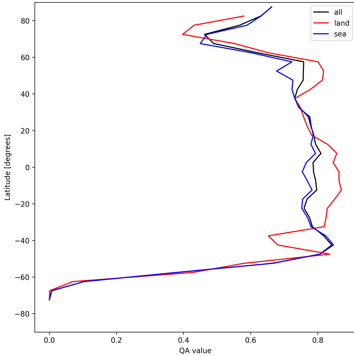
Figure 20: Zonal average of “QA value” for 2025-08-02 to 2025-08-03.
