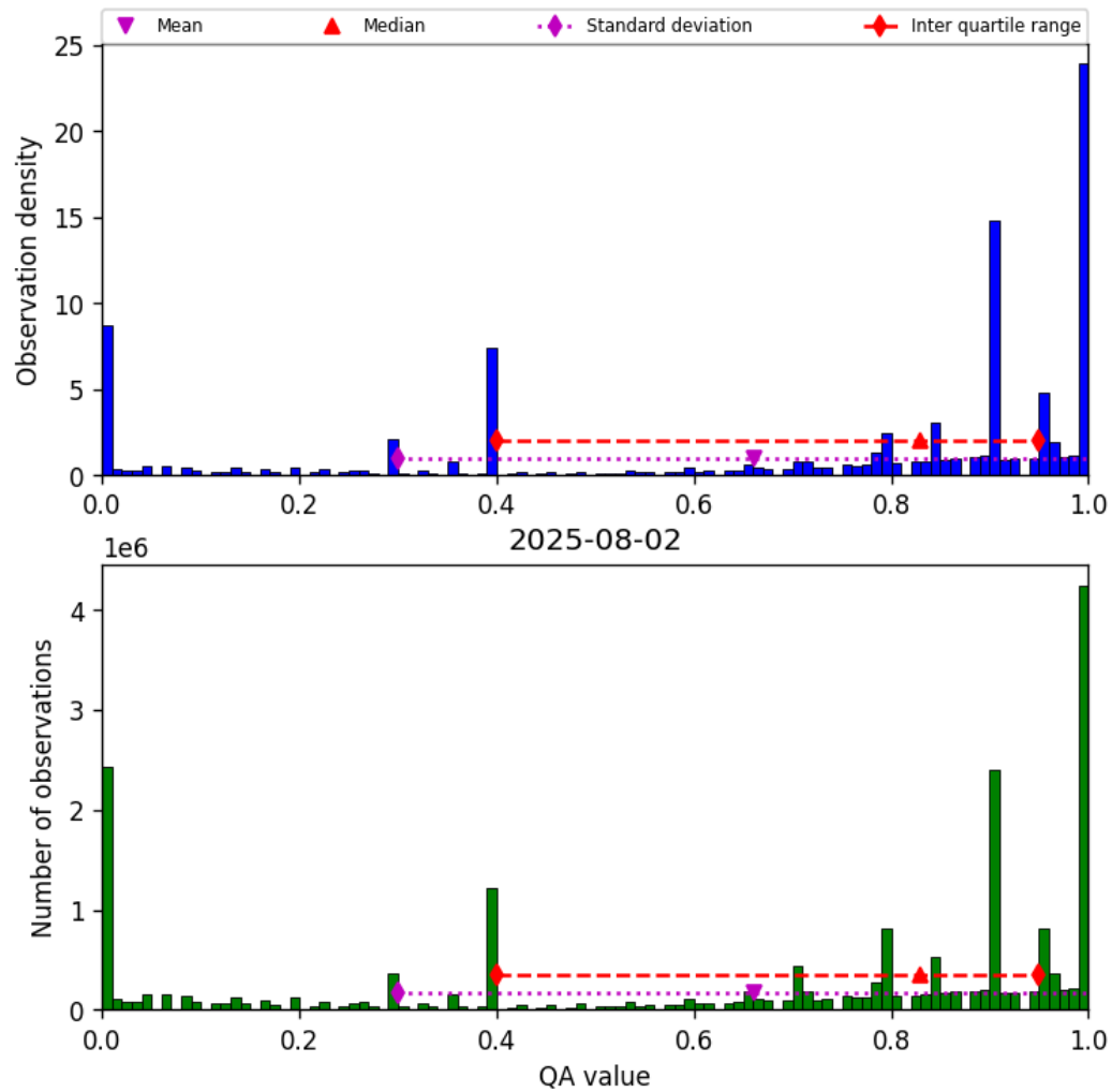
Figure 36: Histogram of “QA value” for 2025-08-02 to 2025-08-03
