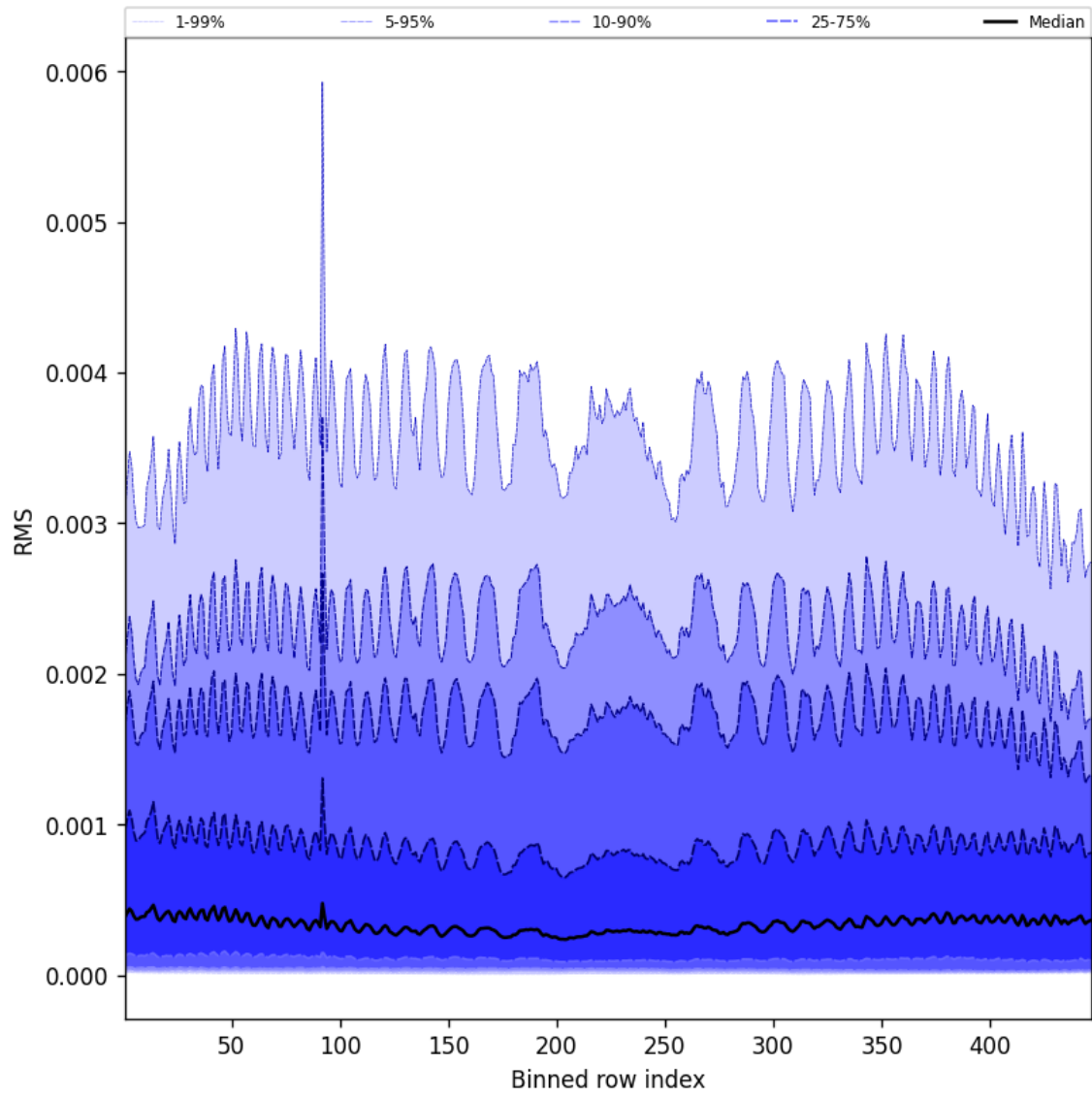
Figure 61: Along track statistics of “RMS” for 2025-08-02 to 2025-08-03
