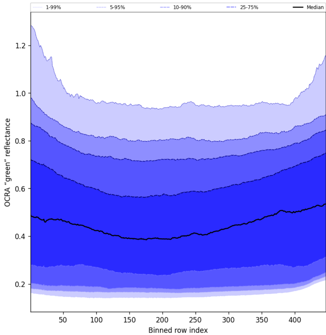
Figure 66: Along track statistics of “OCRA “green” reflectance” for 2025-08-02 to 2025-08-03
