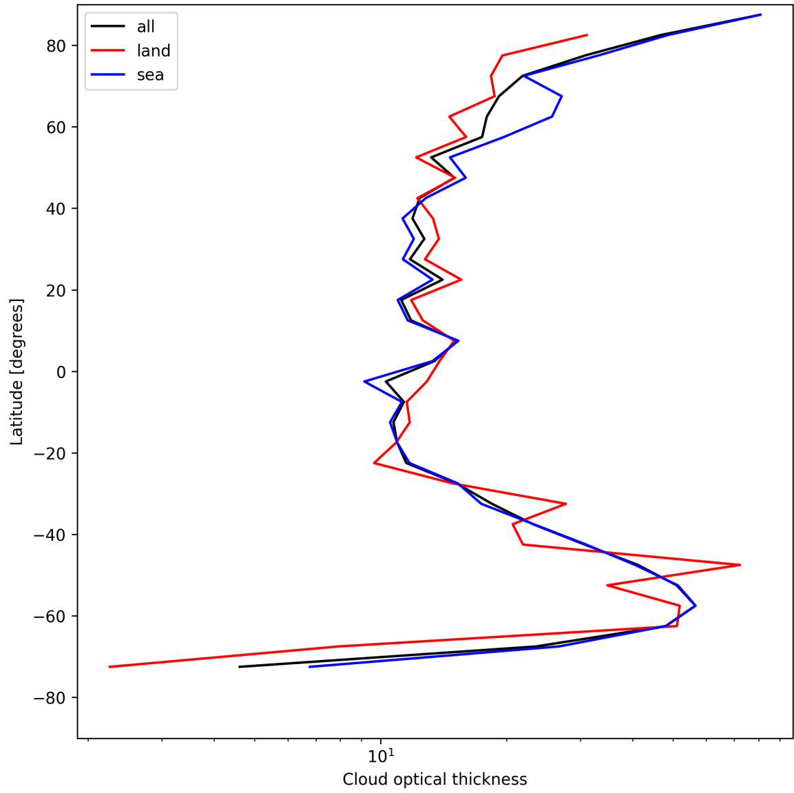
Figure 23: Zonal average of “Cloud optical thickness” for 2025-08-02 to 2025-08-03.
