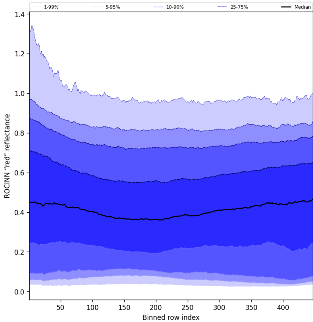
Figure 67: Along track statistics of “ROCINN “red” reflectance” for 2025-08-02 to 2025-08-03
