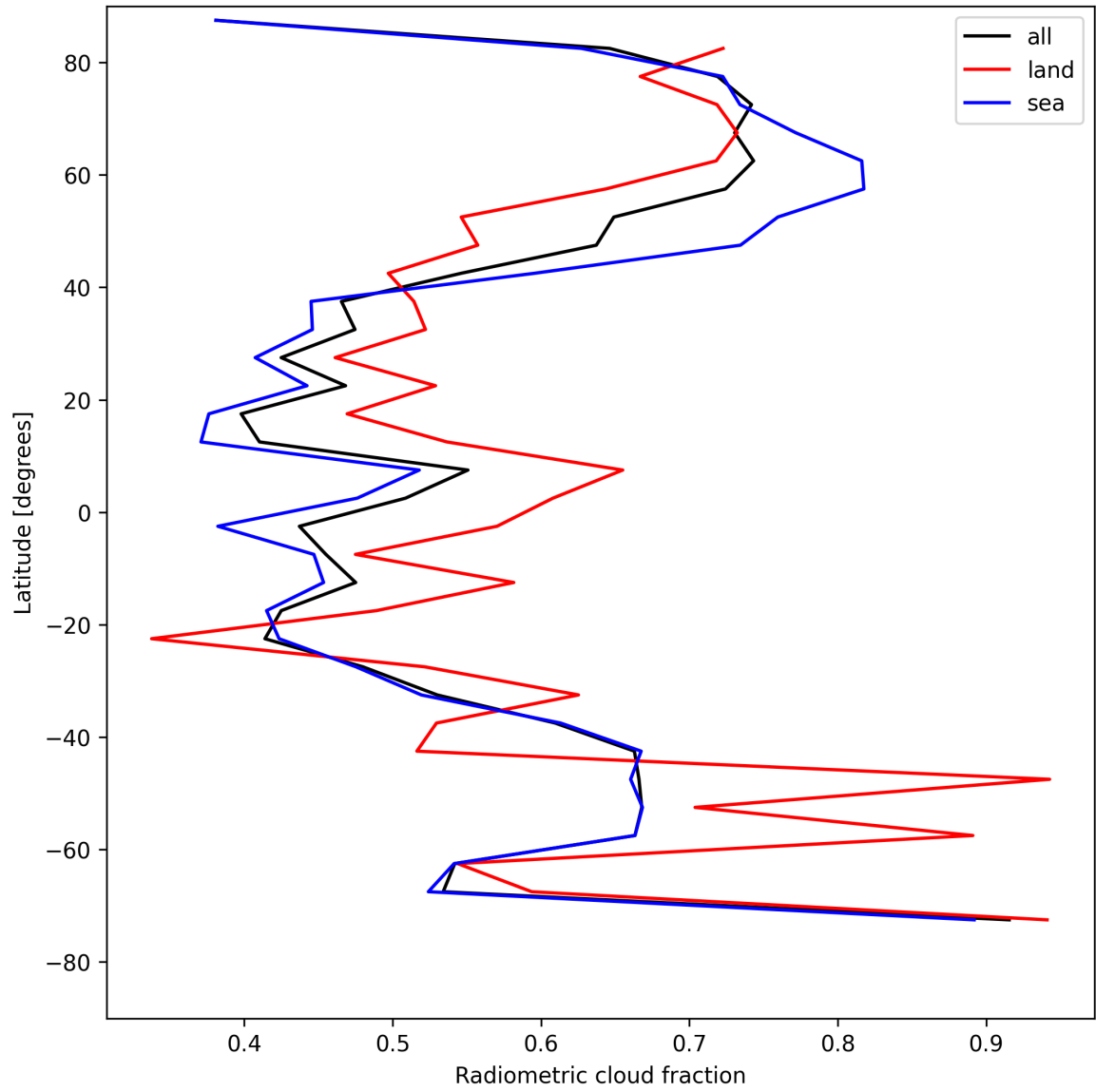
Figure 21: Zonal average of “Radiometric cloud fraction” for 2025-08-02 to 2025-08-03.
