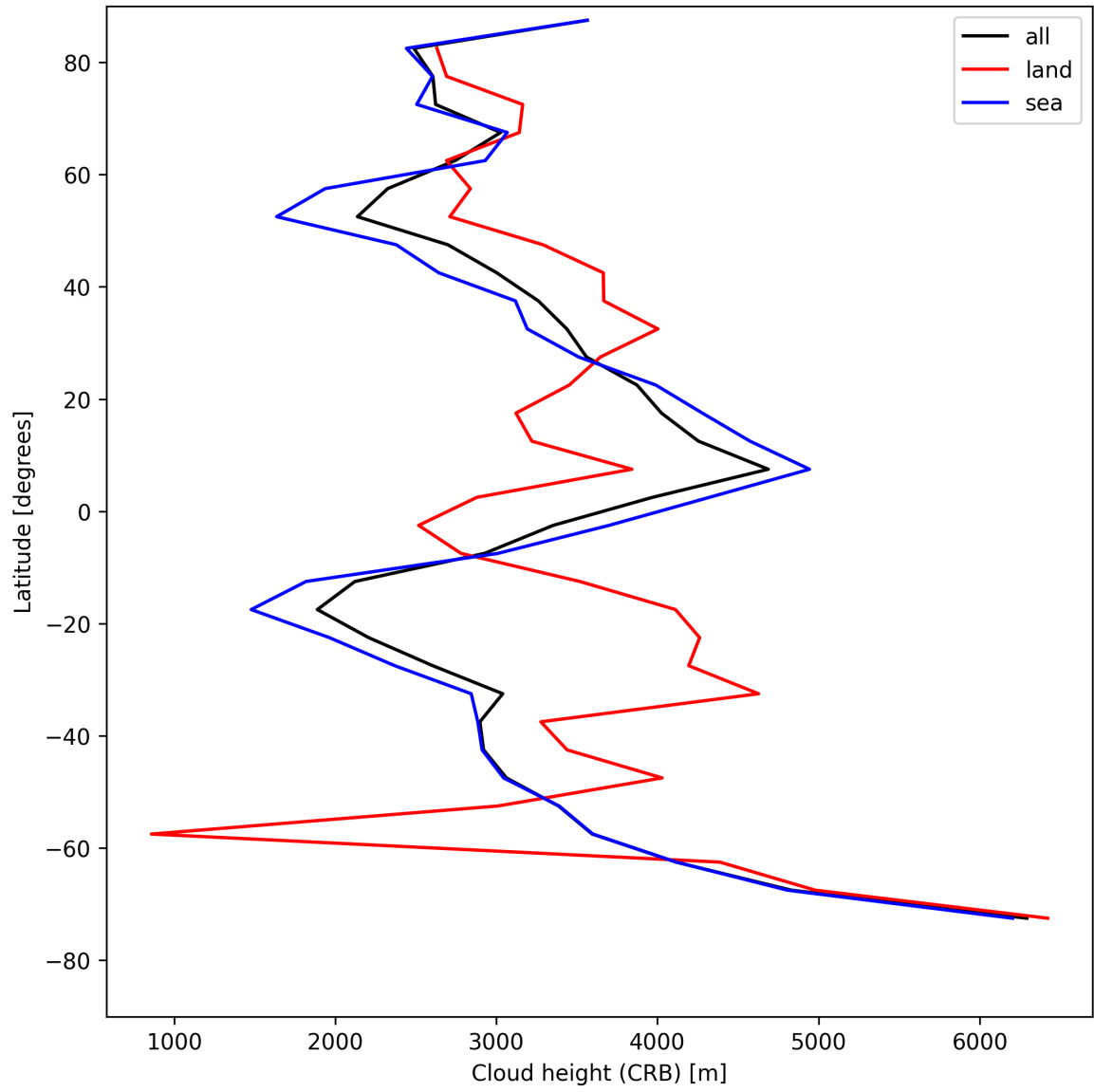
Figure 25: Zonal average of “Cloud height (CRB)” for 2025-08-02 to 2025-08-03.
