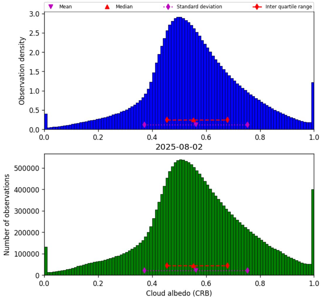
Figure 42: Histogram of “Cloud albedo (CRB)” for 2025-08-02 to 2025-08-03
