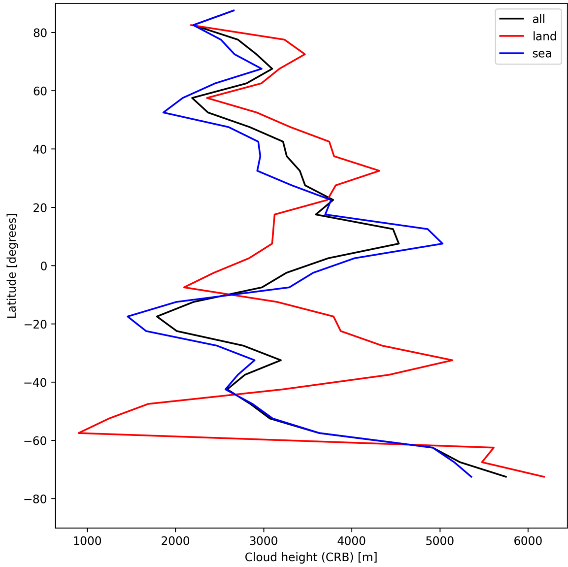
Figure 25: Zonal average of “Cloud height (CRB)” for 2025-08-03 to 2025-08-04.
