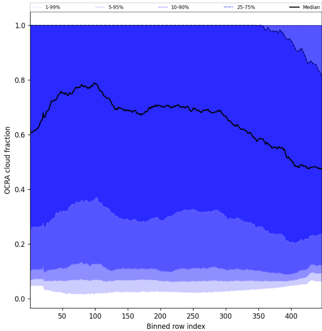
Figure 64: Along track statistics of “OCRA cloud fraction” for 2025-08-03 to 2025-08-04
