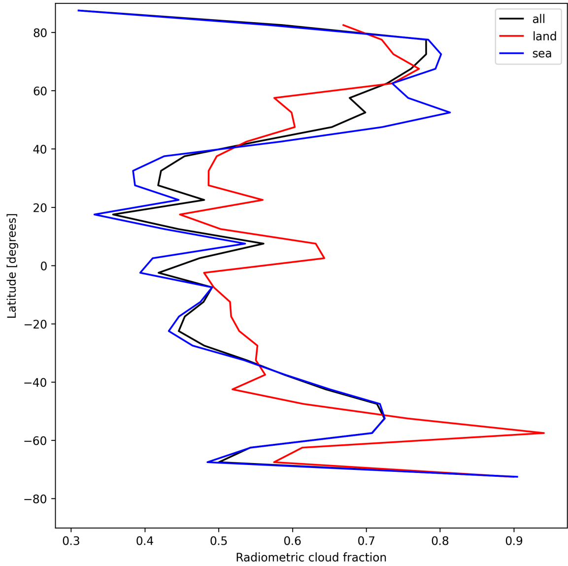
Figure 21: Zonal average of “Radiometric cloud fraction” for 2025-08-03 to 2025-08-04.
