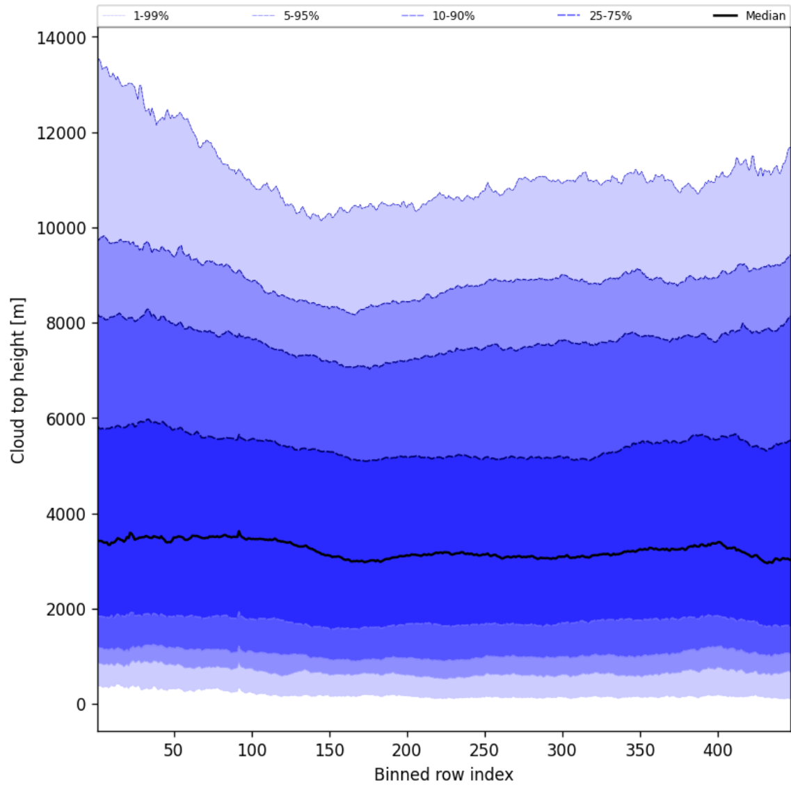
Figure 54: Along track statistics of “Cloud top height” for 2025-08-03 to 2025-08-04
