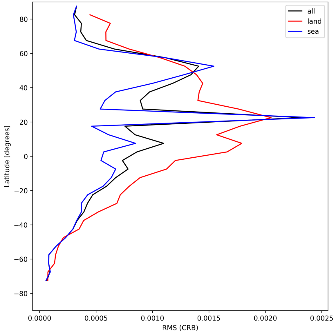
Figure 30: Zonal average of “RMS (CRB)” for 2025-08-03 to 2025-08-04.
