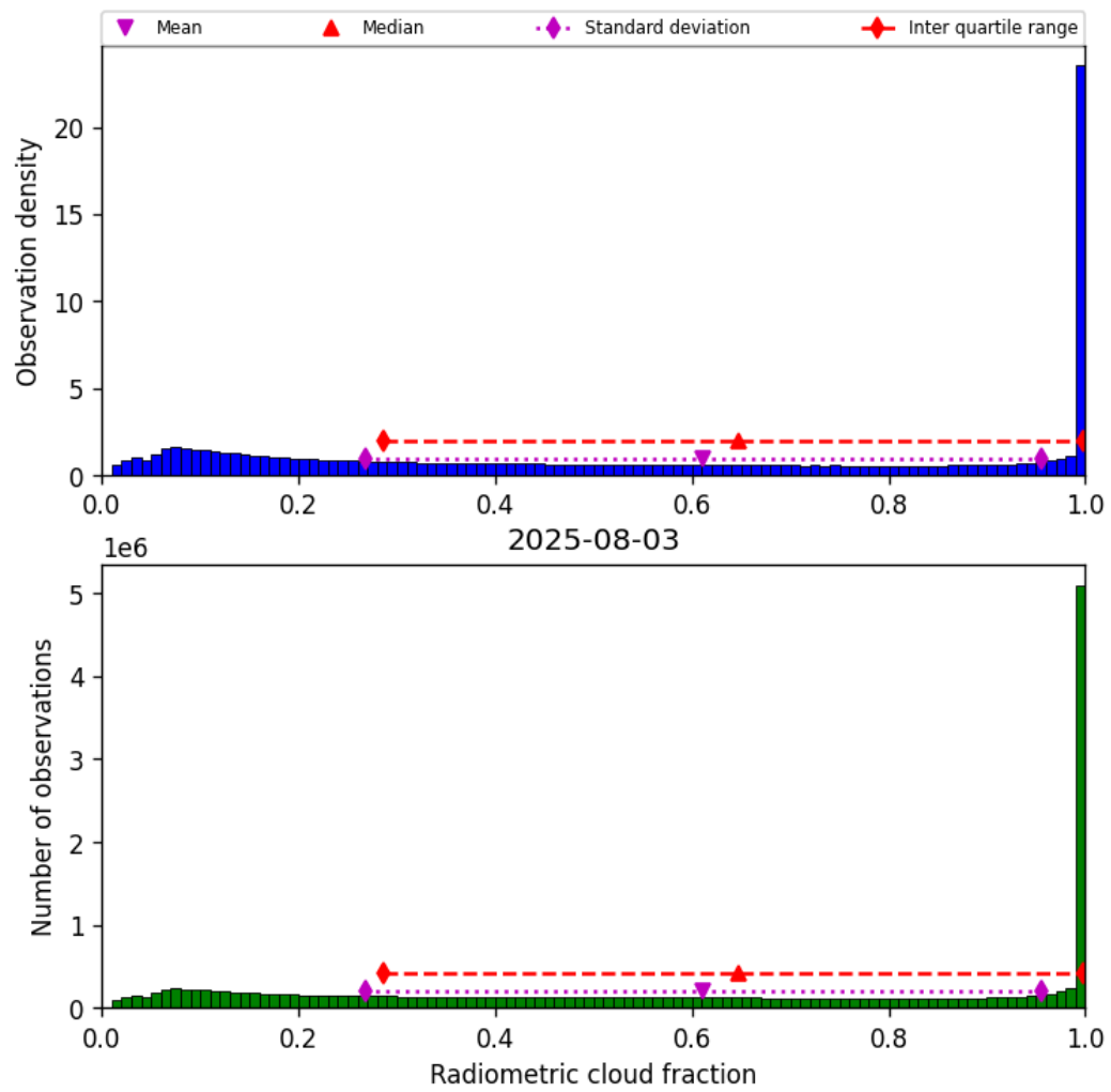
Figure 37: Histogram of “Radiometric cloud fraction” for 2025-08-03 to 2025-08-04
