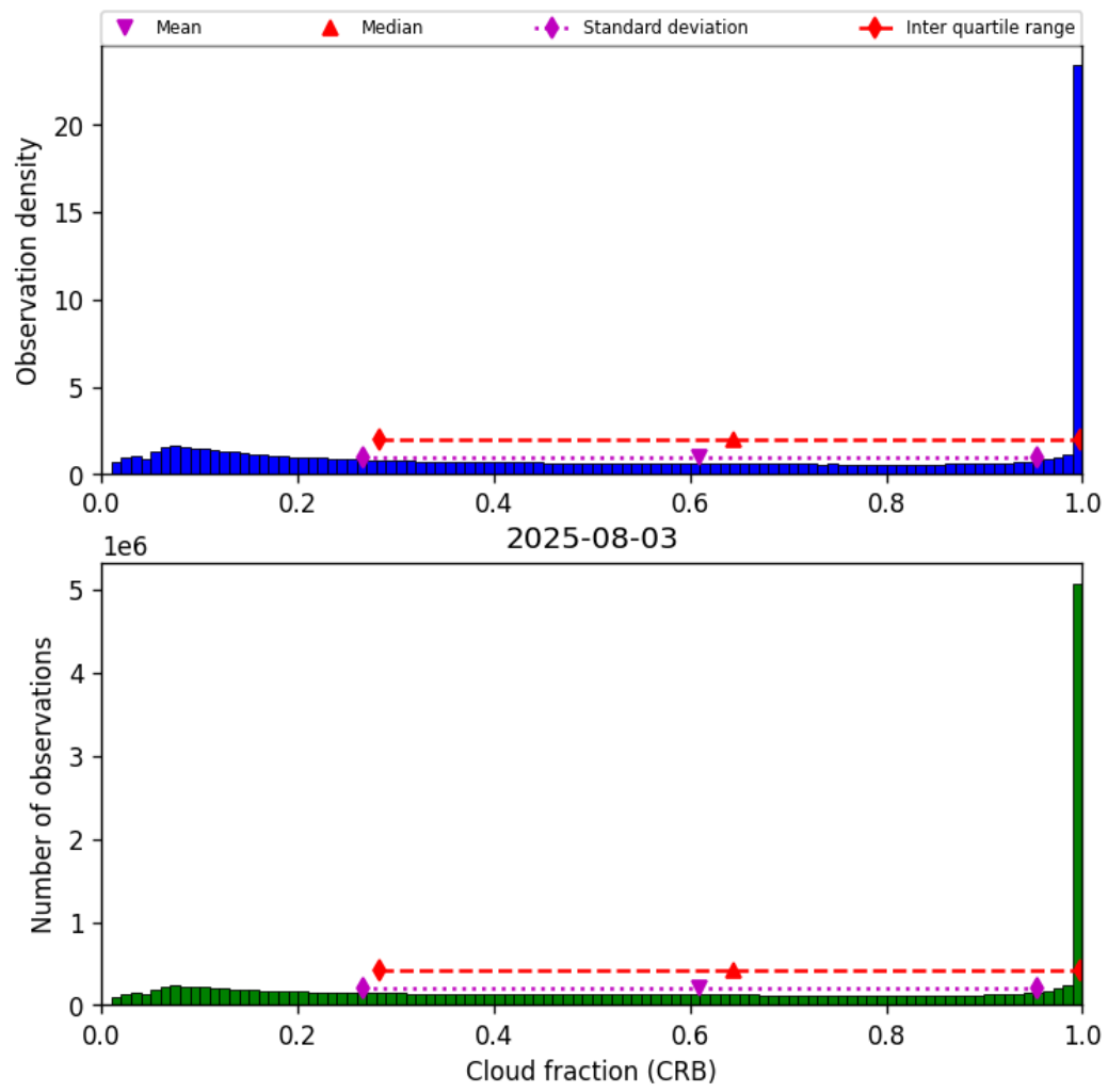
Figure 40: Histogram of “Cloud fraction (CRB)” for 2025-08-03 to 2025-08-04
