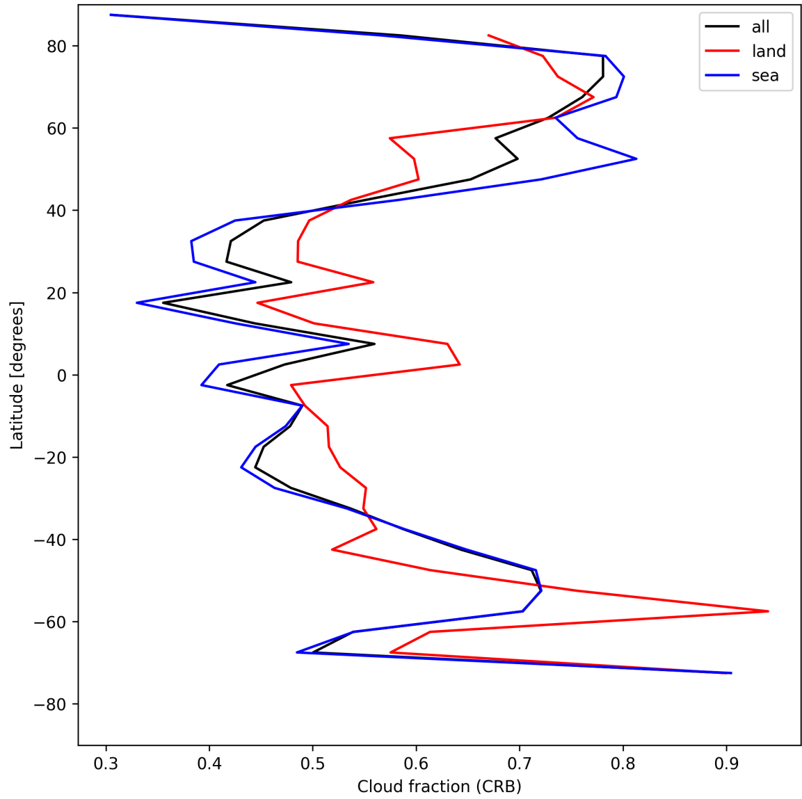
Figure 24: Zonal average of “Cloud fraction (CRB)” for 2025-08-03 to 2025-08-04.
