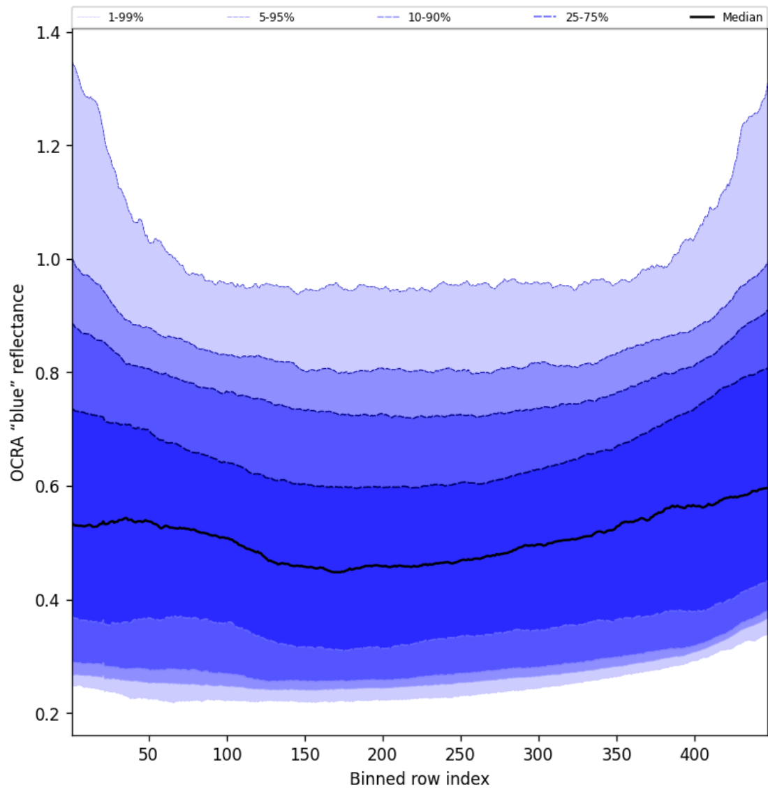
Figure 65: Along track statistics of “OCRA “blue” reflectance” for 2025-08-03 to 2025-08-04
