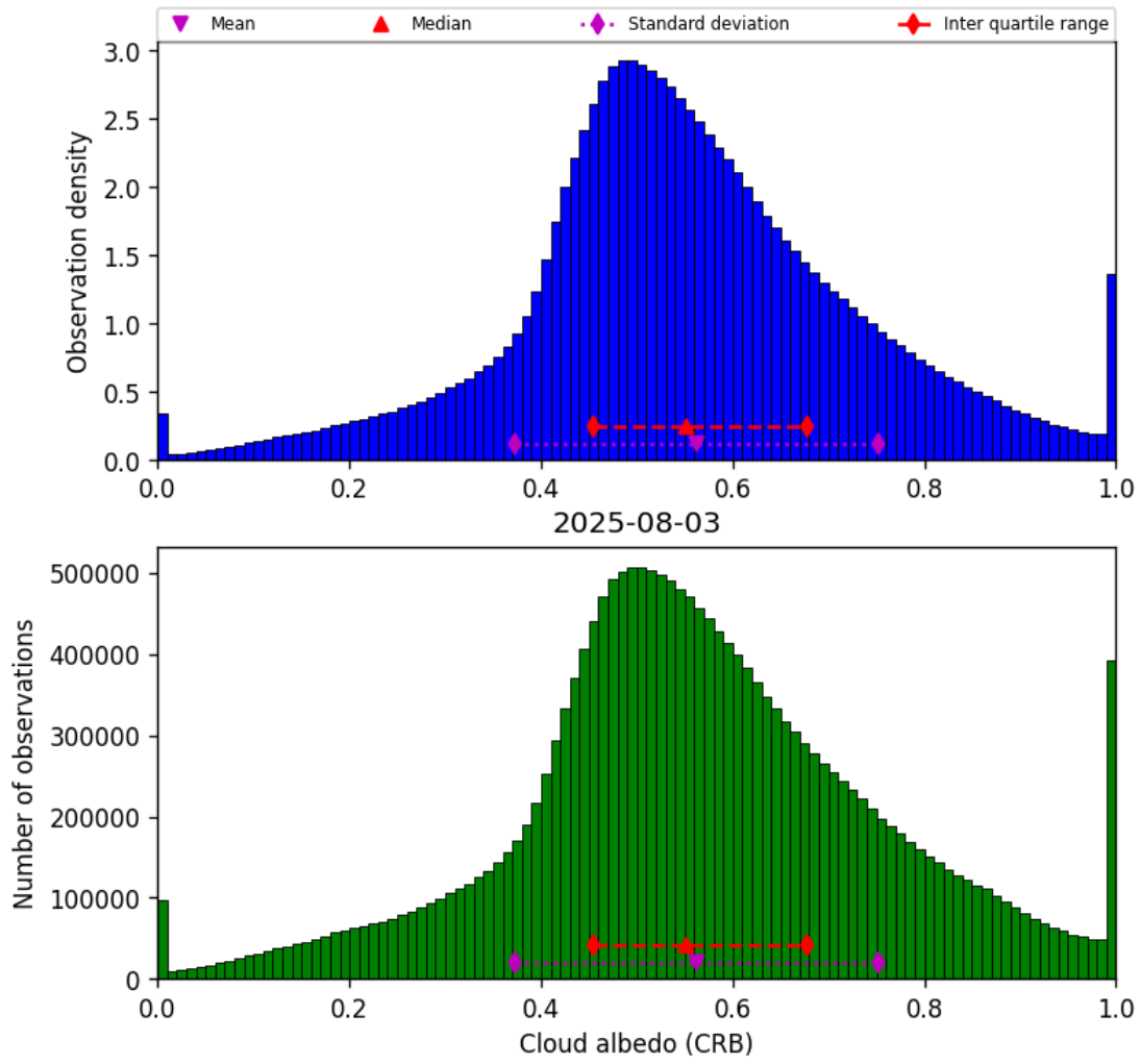
Figure 42: Histogram of “Cloud albedo (CRB)” for 2025-08-03 to 2025-08-04
