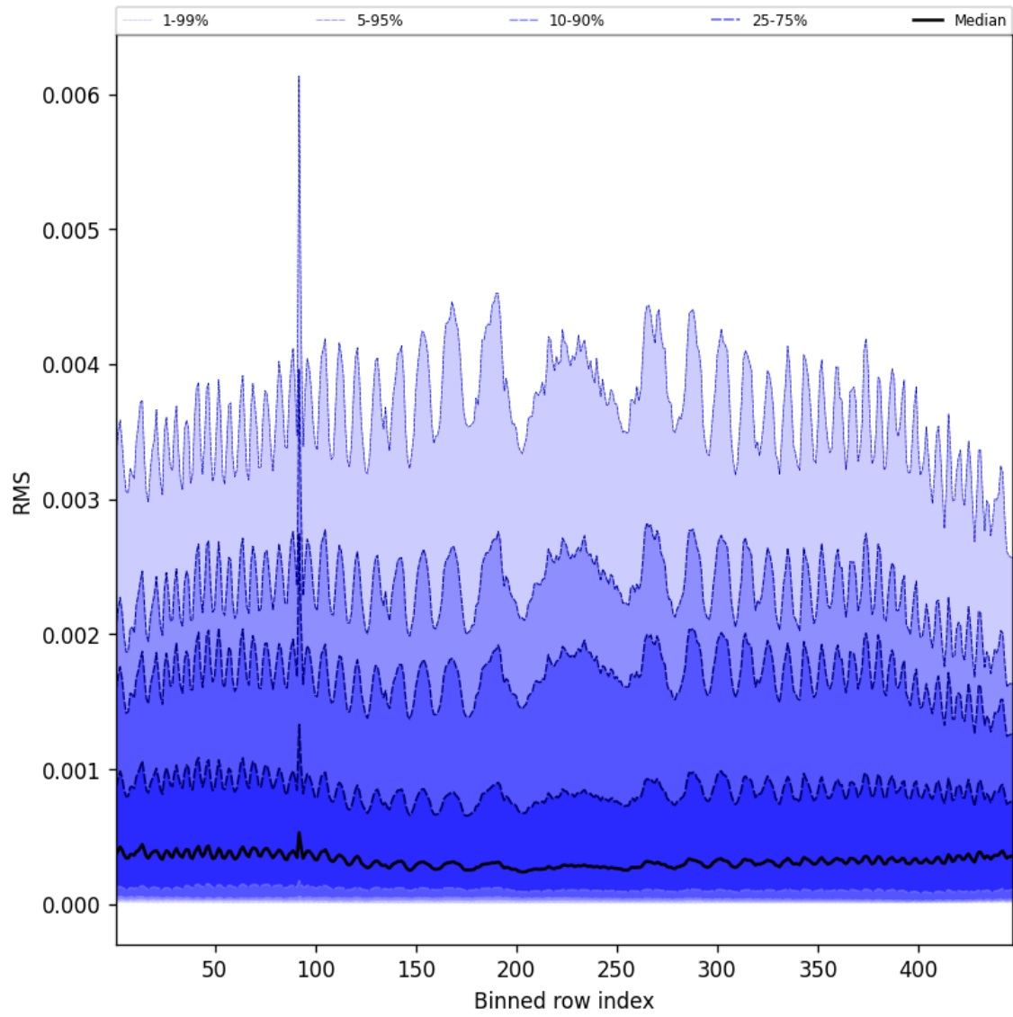
Figure 61: Along track statistics of “RMS” for 2025-08-03 to 2025-08-04
