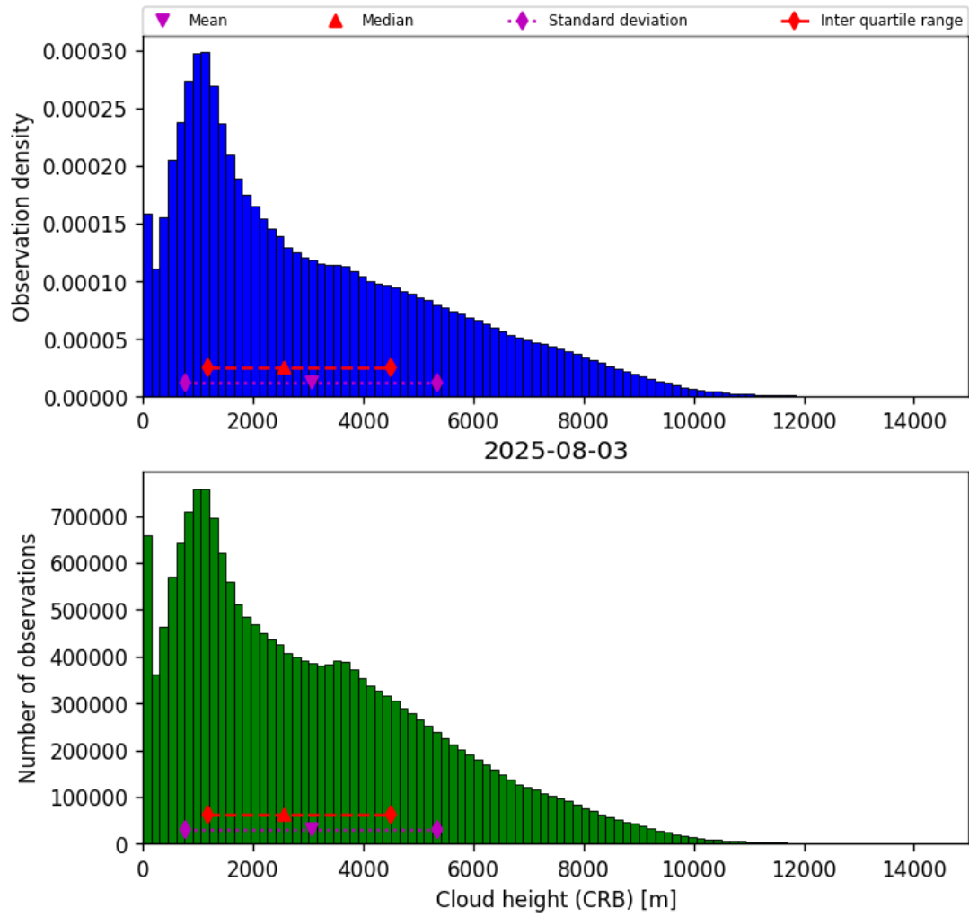
Figure 41: Histogram of “Cloud height (CRB)” for 2025-08-03 to 2025-08-04
