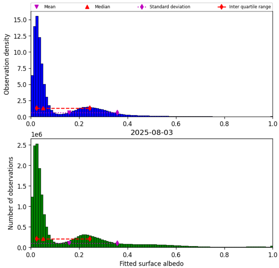
Figure 43: Histogram of “Fitted surface albedo” for 2025-08-03 to 2025-08-04
