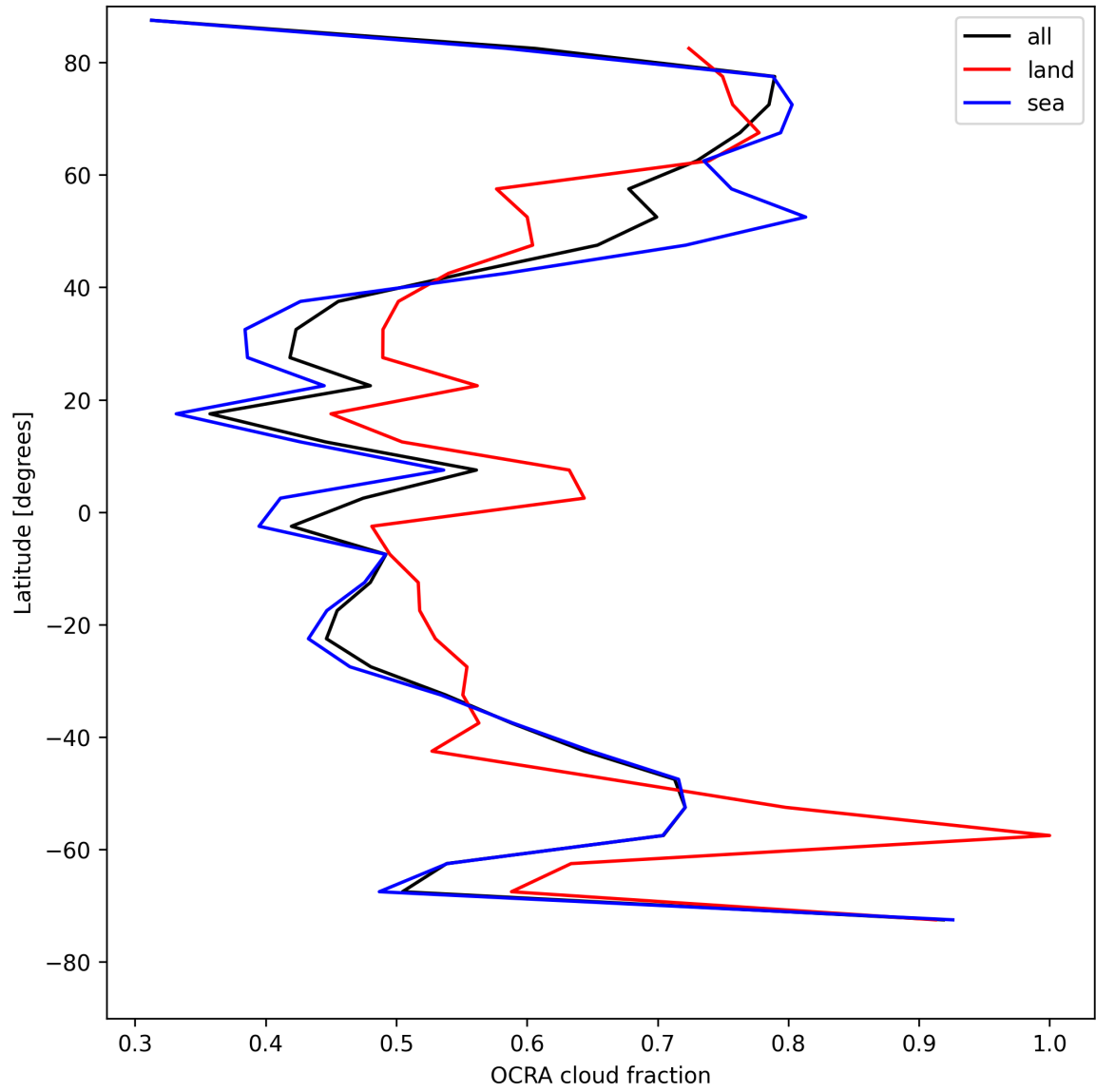
Figure 32: Zonal average of “OCRA cloud fraction” for 2025-08-03 to 2025-08-04.
