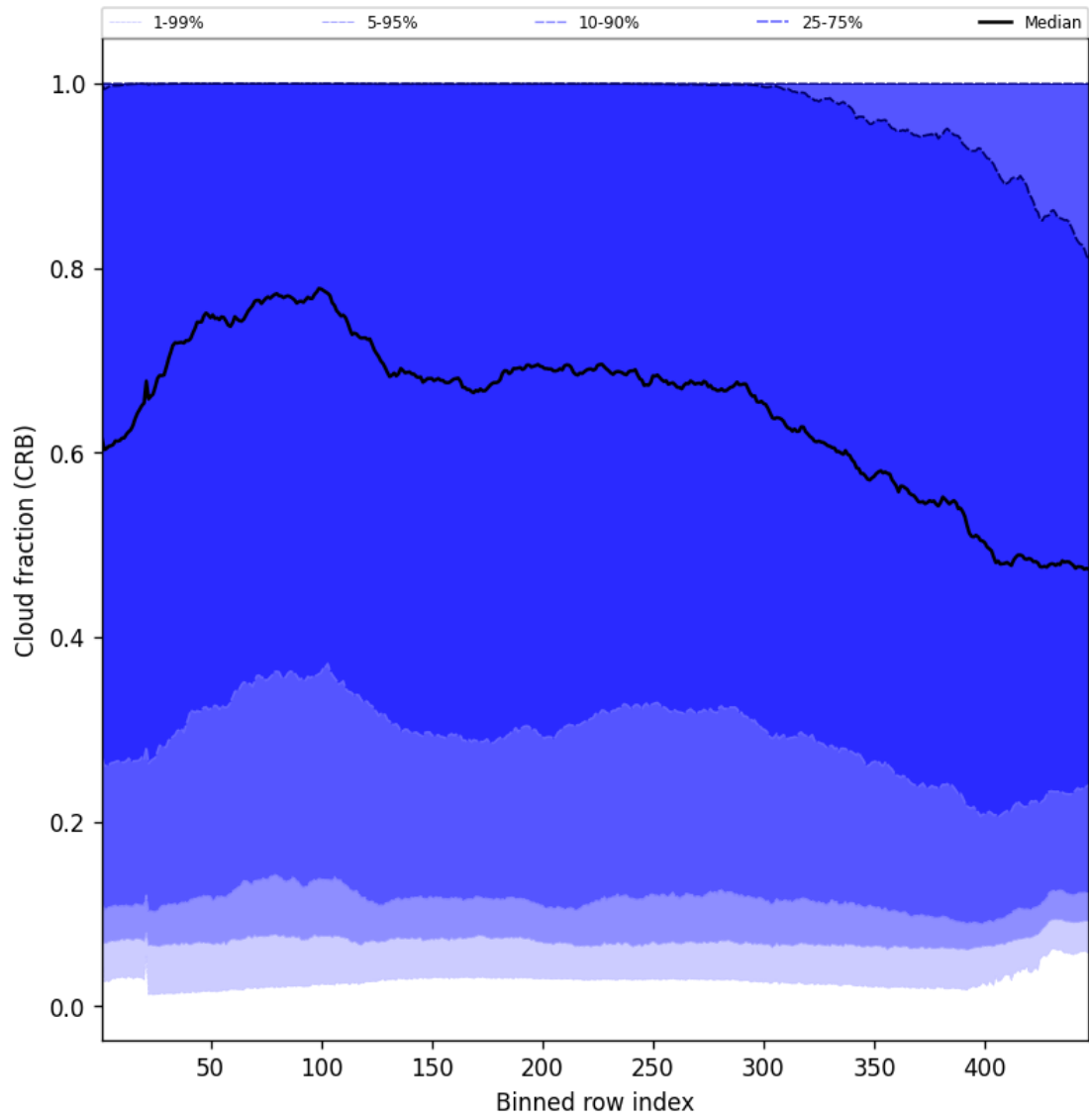
Figure 56: Along track statistics of “Cloud fraction (CRB)” for 2025-08-03 to 2025-08-04
