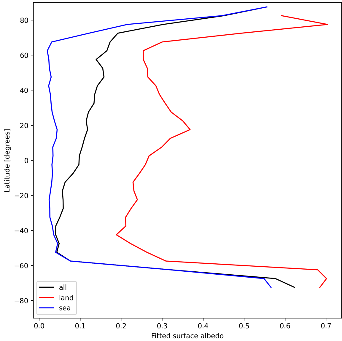
Figure 27: Zonal average of “Fitted surface albedo” for 2025-08-03 to 2025-08-04.
