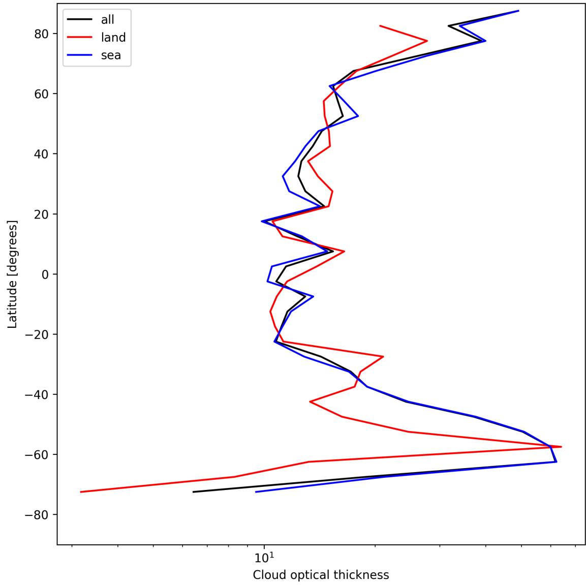
Figure 23: Zonal average of “Cloud optical thickness” for 2025-08-03 to 2025-08-04.
