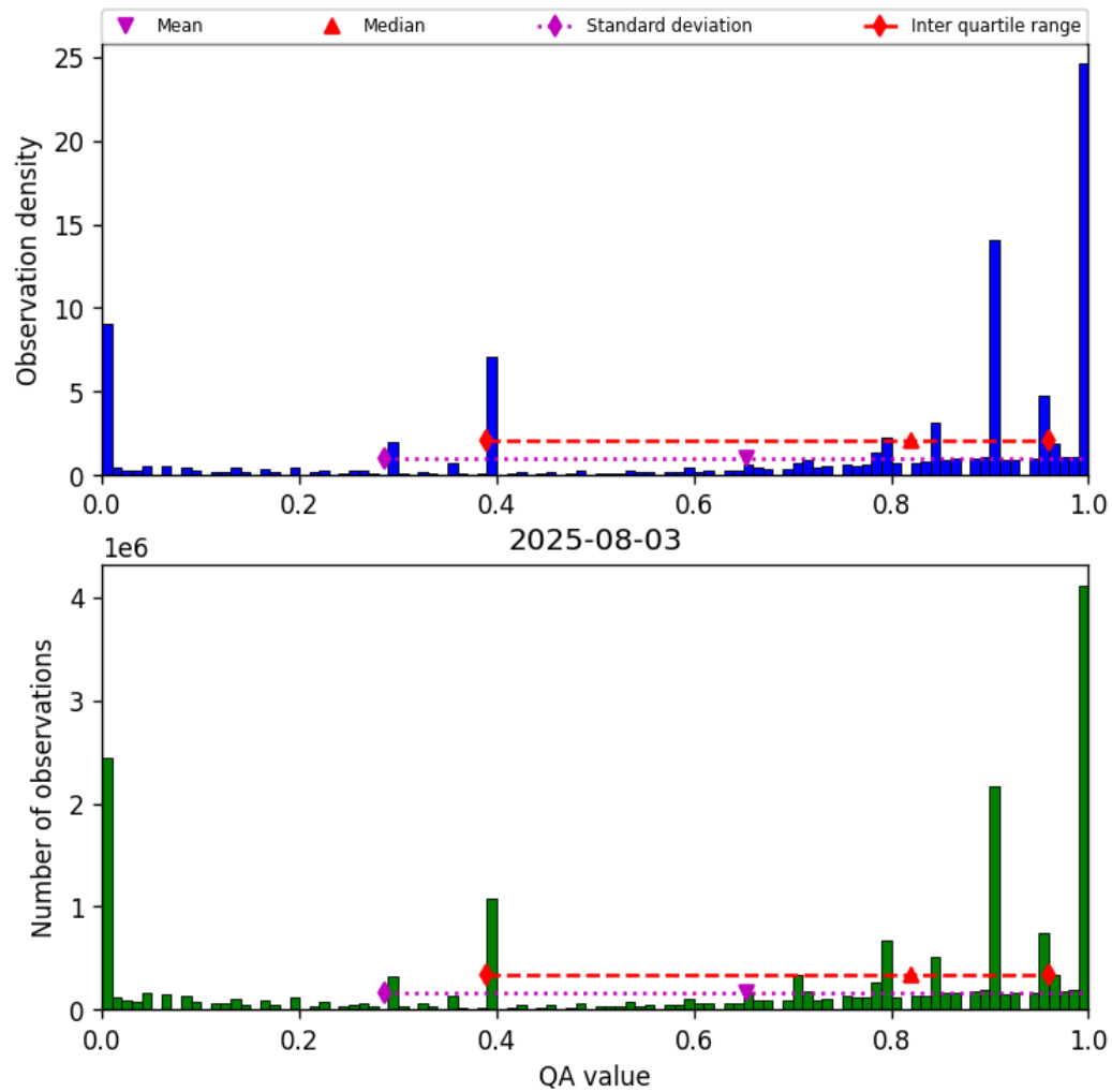
Figure 36: Histogram of “QA value” for 2025-08-03 to 2025-08-04
