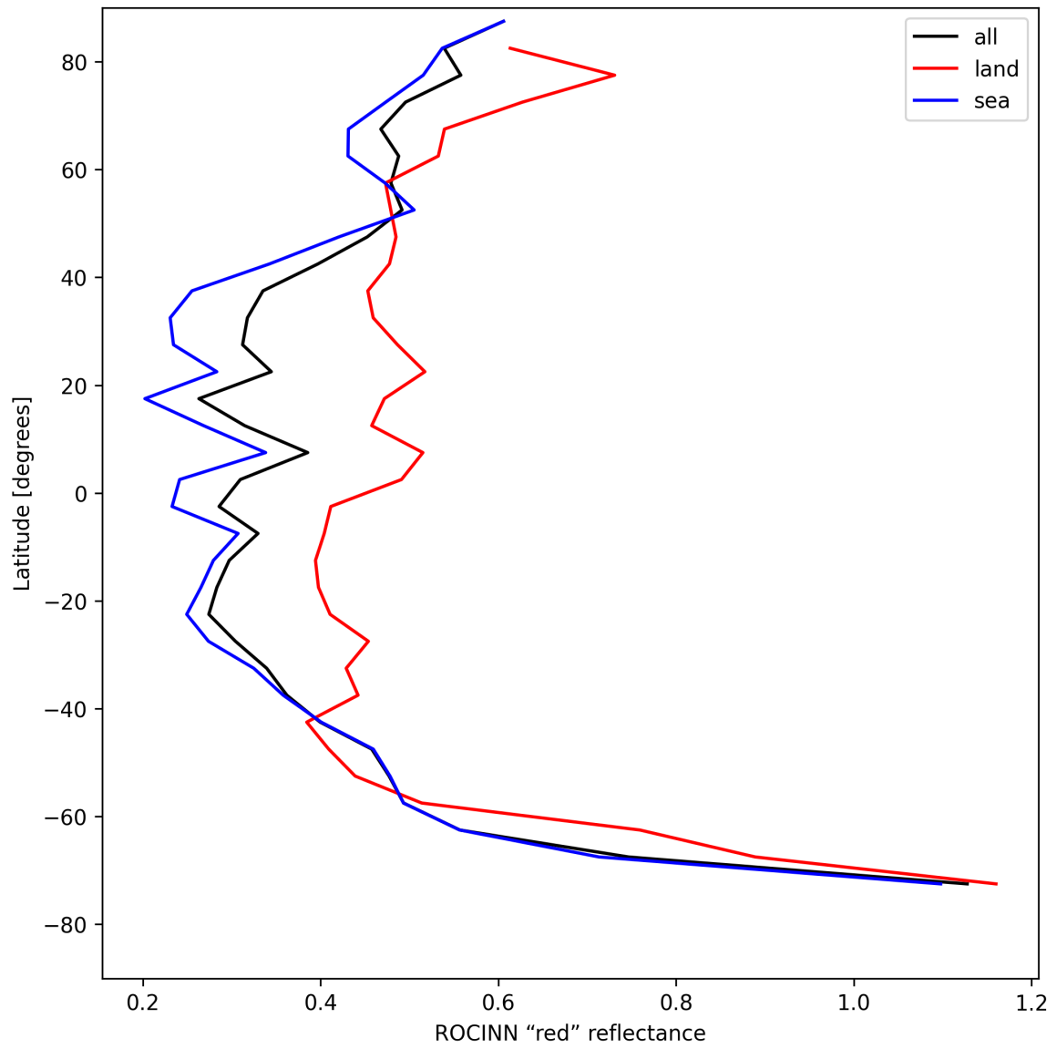
Figure 35: Zonal average of “ROCINN “red” reflectance” for 2025-08-03 to 2025-08-04.
