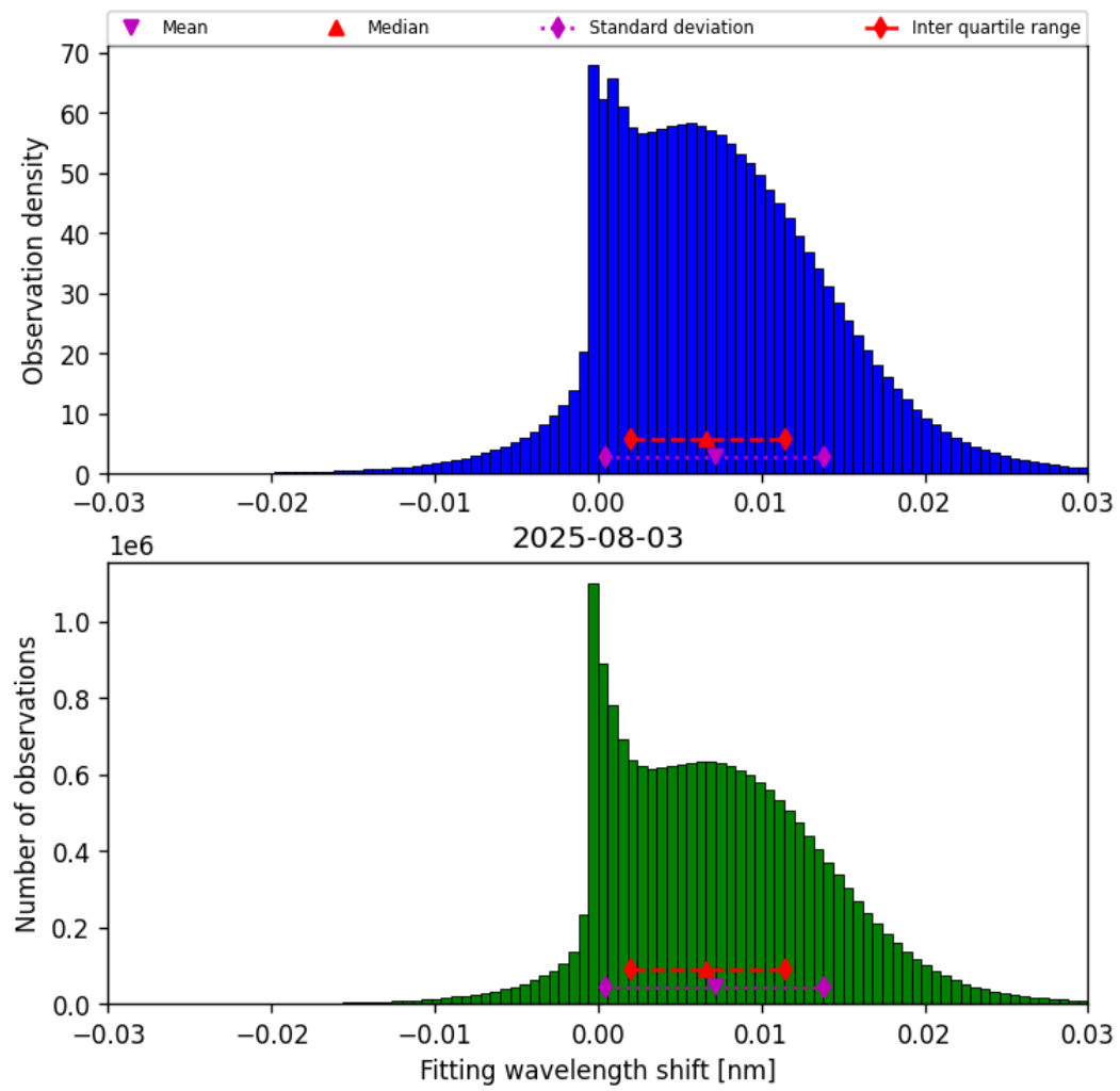
Figure 47: Histogram of “Fitting wavelength shift” for 2025-08-03 to 2025-08-04
