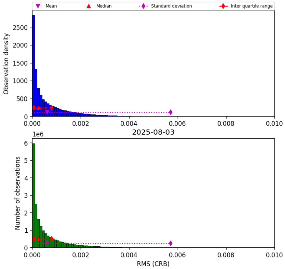
Figure 46: Histogram of "RMS (CRB)" for 2025-08-03 to 2025-08-04
