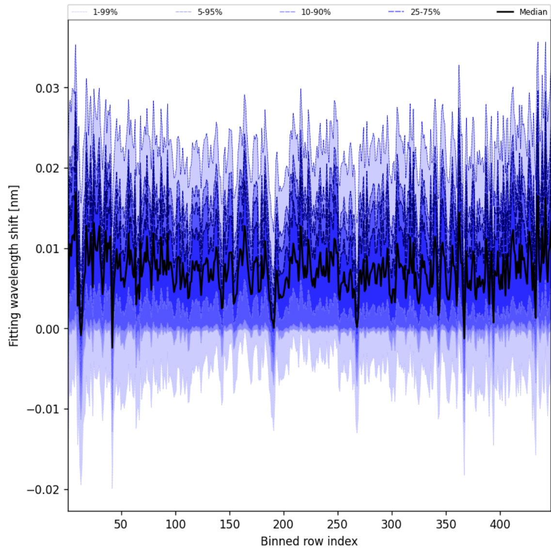
Figure 63: Along track statistics of “Fitting wavelength shift” for 2025-08-03 to 2025-08-04
