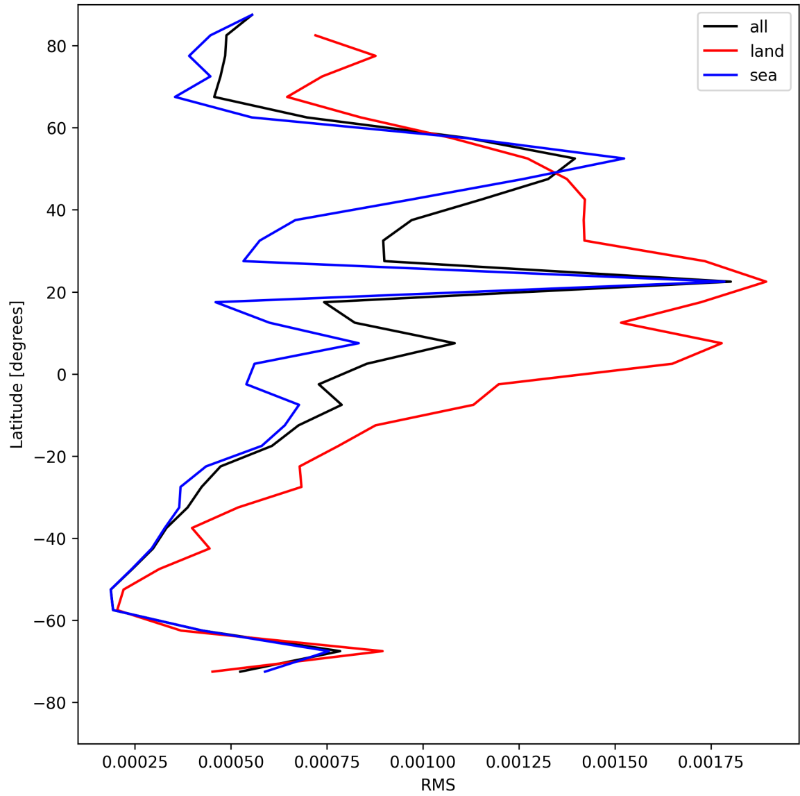
Figure 29: Zonal average of “RMS” for 2025-08-03 to 2025-08-04.
