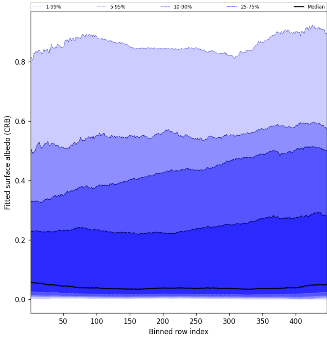
Figure 60: Along track statistics of “Fitted surface albedo (CRB)” for 2025-08-03 to 2025-08-04
