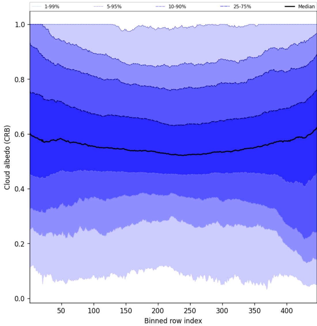
Figure 58: Along track statistics of “Cloud albedo (CRB)” for 2025-08-03 to 2025-08-04
