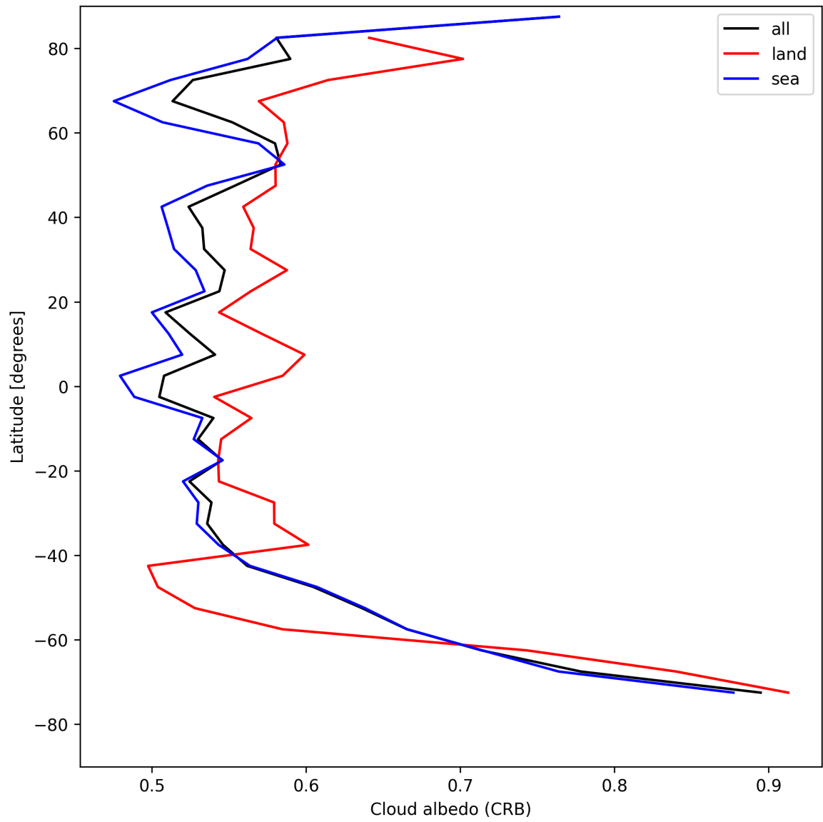
Figure 26: Zonal average of “Cloud albedo (CRB)” for 2025-08-03 to 2025-08-04.
