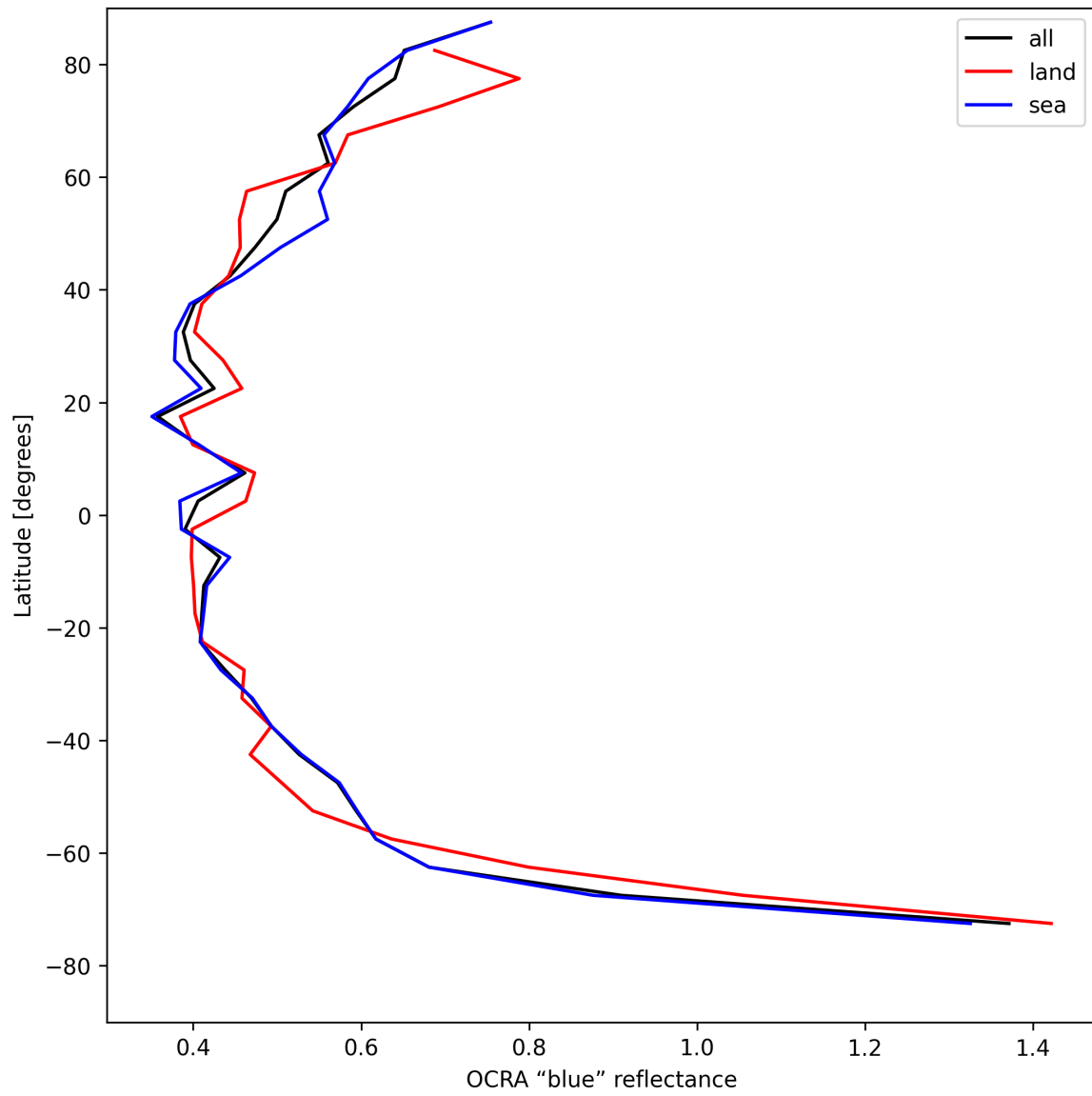
Figure 33: Zonal average of “OCRA “blue” reflectance” for 2025-08-03 to 2025-08-04.
