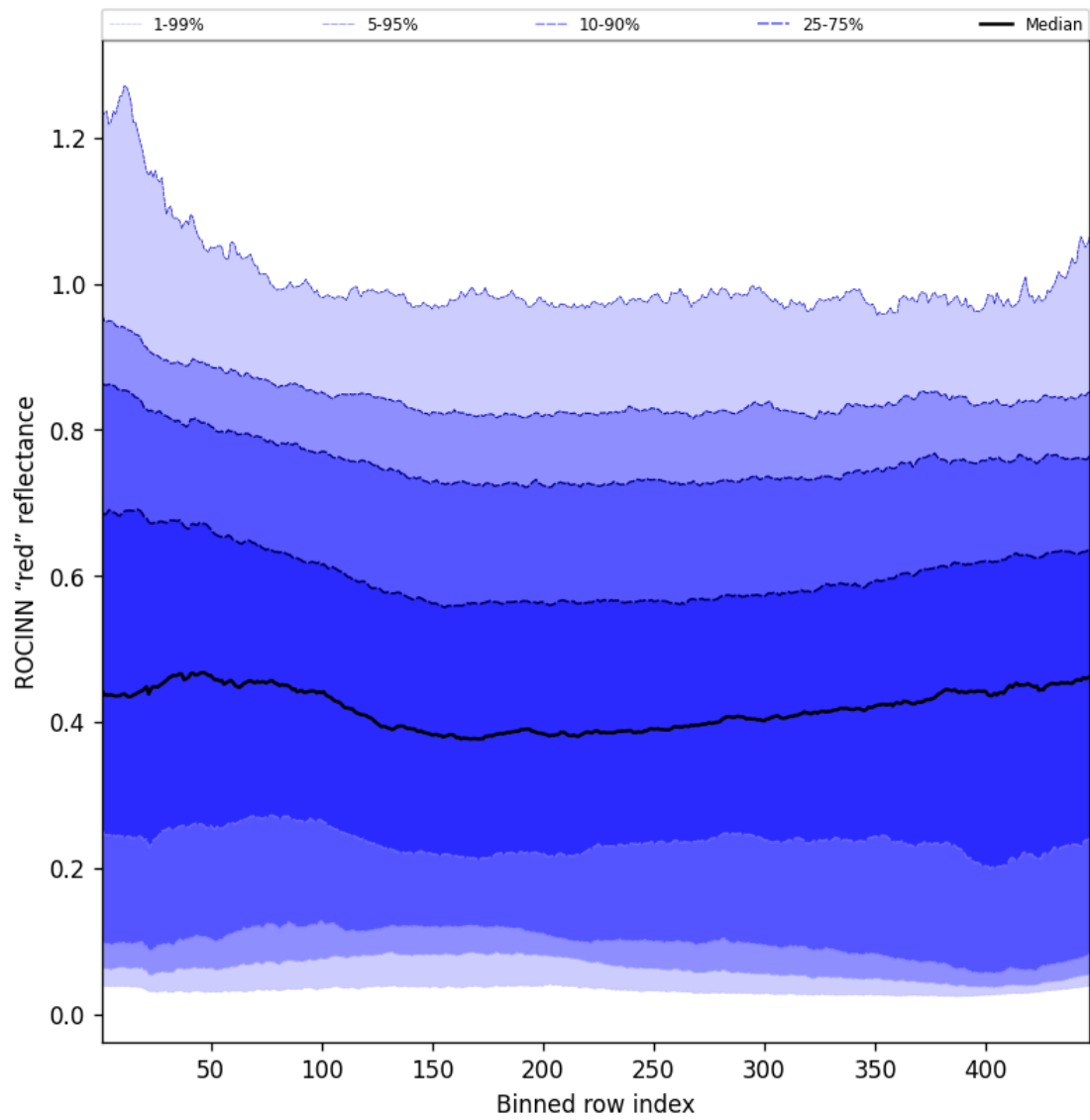
Figure 67: Along track statistics of “ROCINN “red” reflectance” for 2025-08-03 to 2025-08-04
