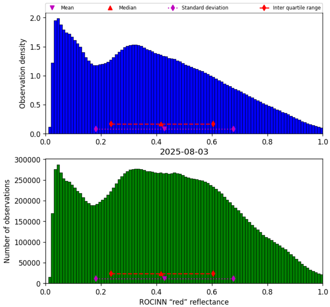
Figure 51: Histogram of “ROCINN “red” reflectance” for 2025-08-03 to 2025-08-04
