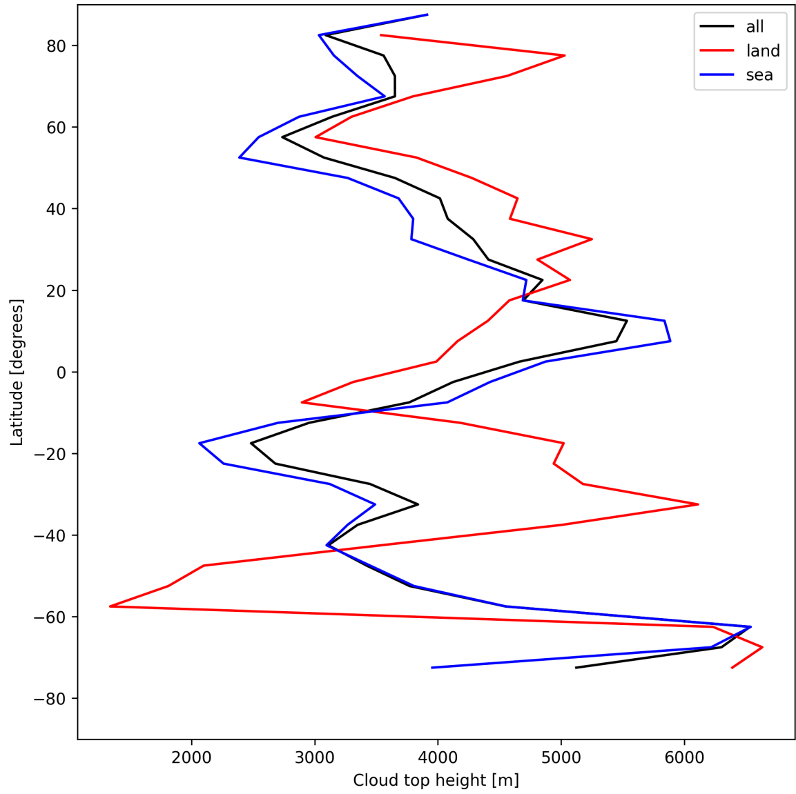
Figure 22: Zonal average of “Cloud top height” for 2025-08-03 to 2025-08-04.
