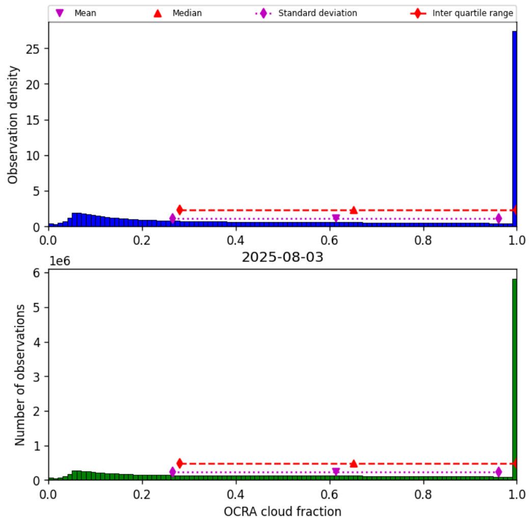
Figure 48: Histogram of “OCRA cloud fraction” for 2025-08-03 to 2025-08-04
