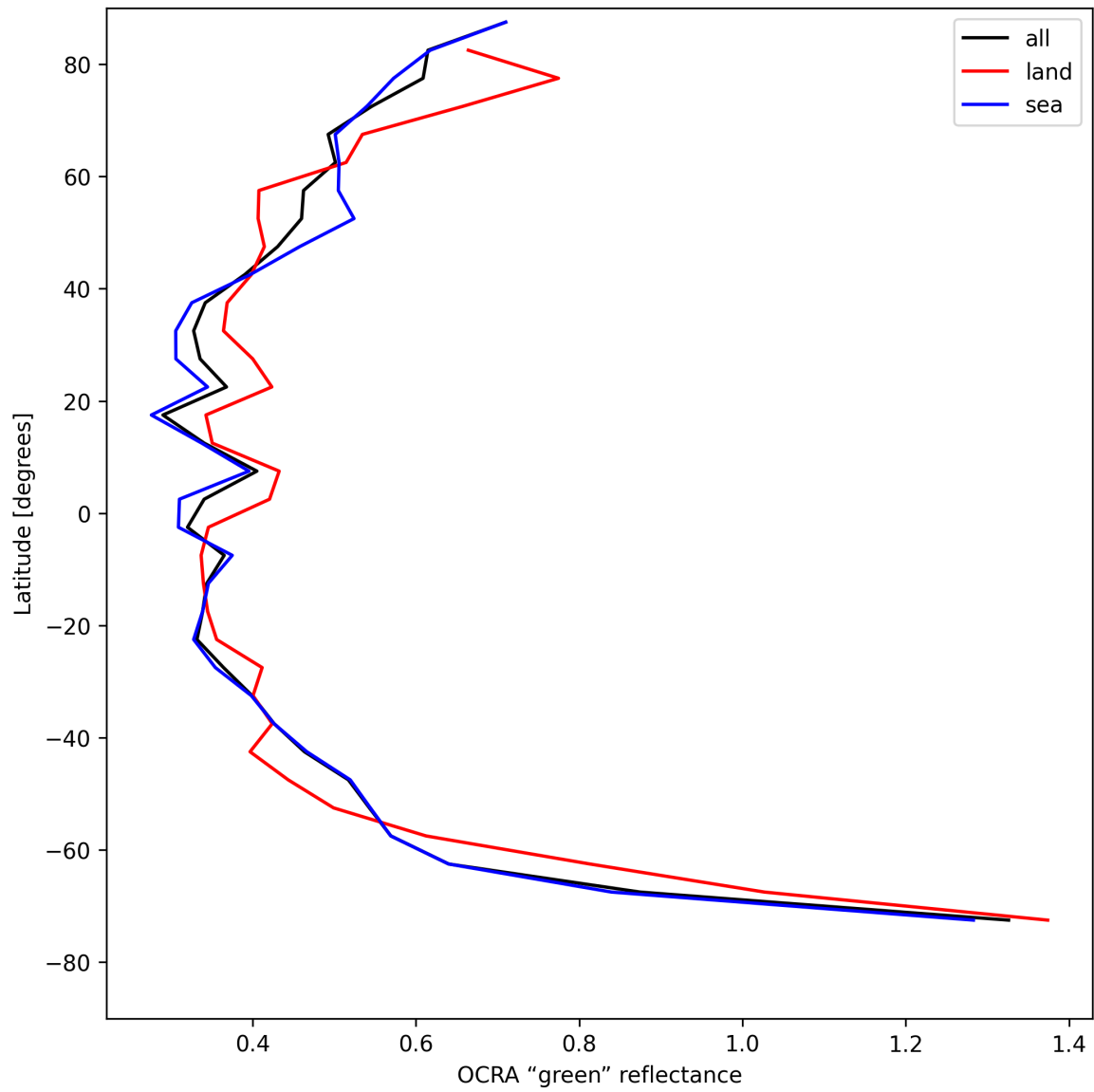
Figure 34: Zonal average of “OCRA “green” reflectance” for 2025-08-03 to 2025-08-04.
