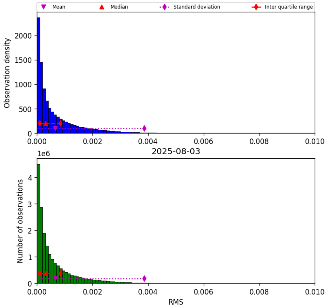
Figure 45: Histogram of “RMS” for 2025-08-03 to 2025-08-04
