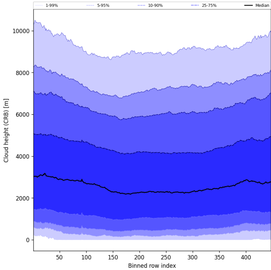
Figure 57: Along track statistics of “Cloud height (CRB)” for 2025-08-03 to 2025-08-04
