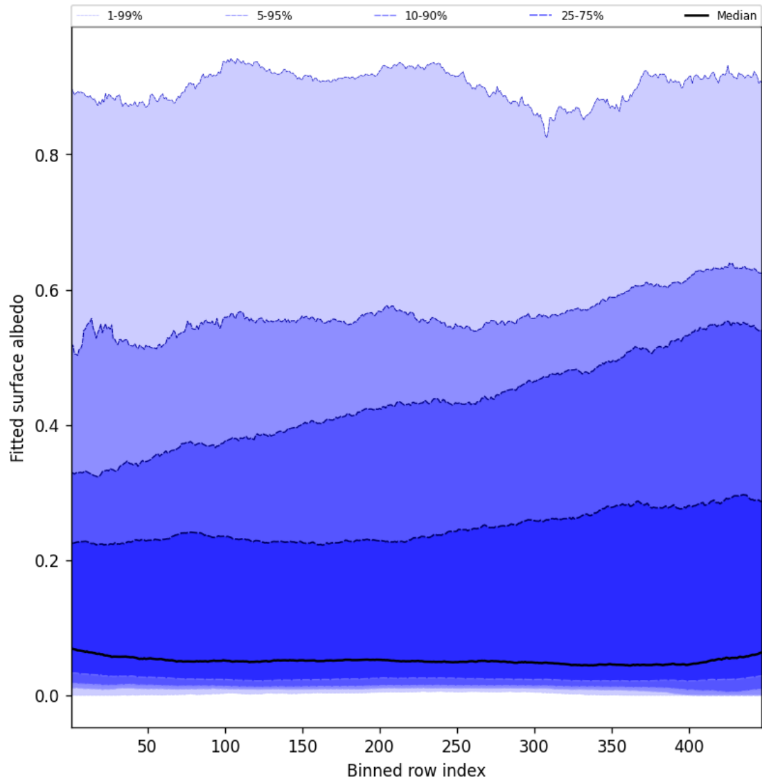
Figure 59: Along track statistics of “Fitted surface albedo” for 2025-08-03 to 2025-08-04
