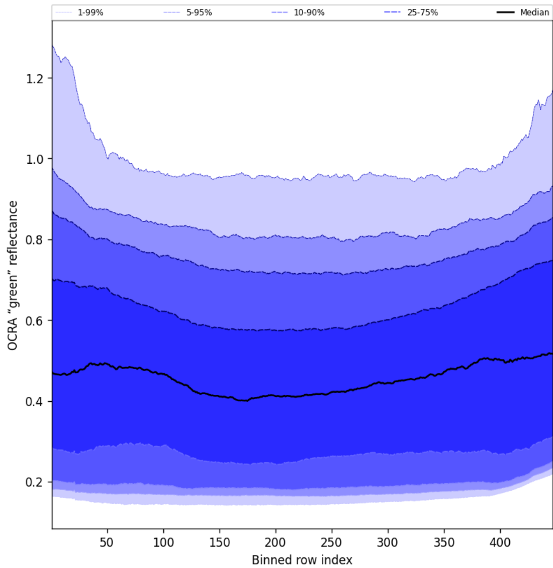
Figure 66: Along track statistics of “OCRA “green” reflectance” for 2025-08-03 to 2025-08-04
