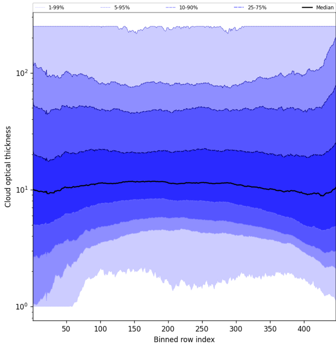
Figure 55: Along track statistics of “Cloud optical thickness” for 2025-08-03 to 2025-08-04
