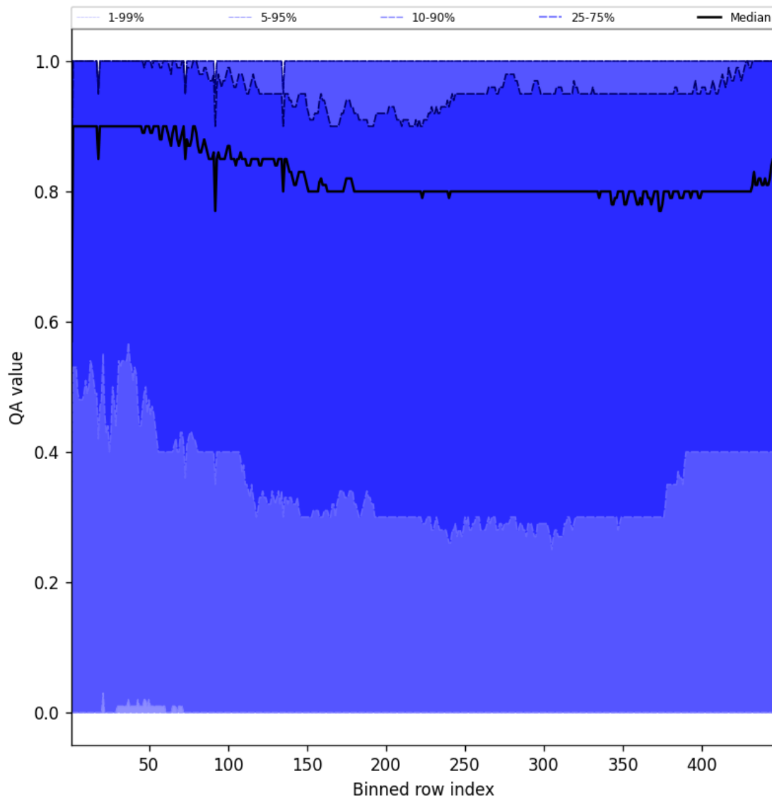
Figure 52: Along track statistics of “QA value” for 2025-08-03 to 2025-08-04
