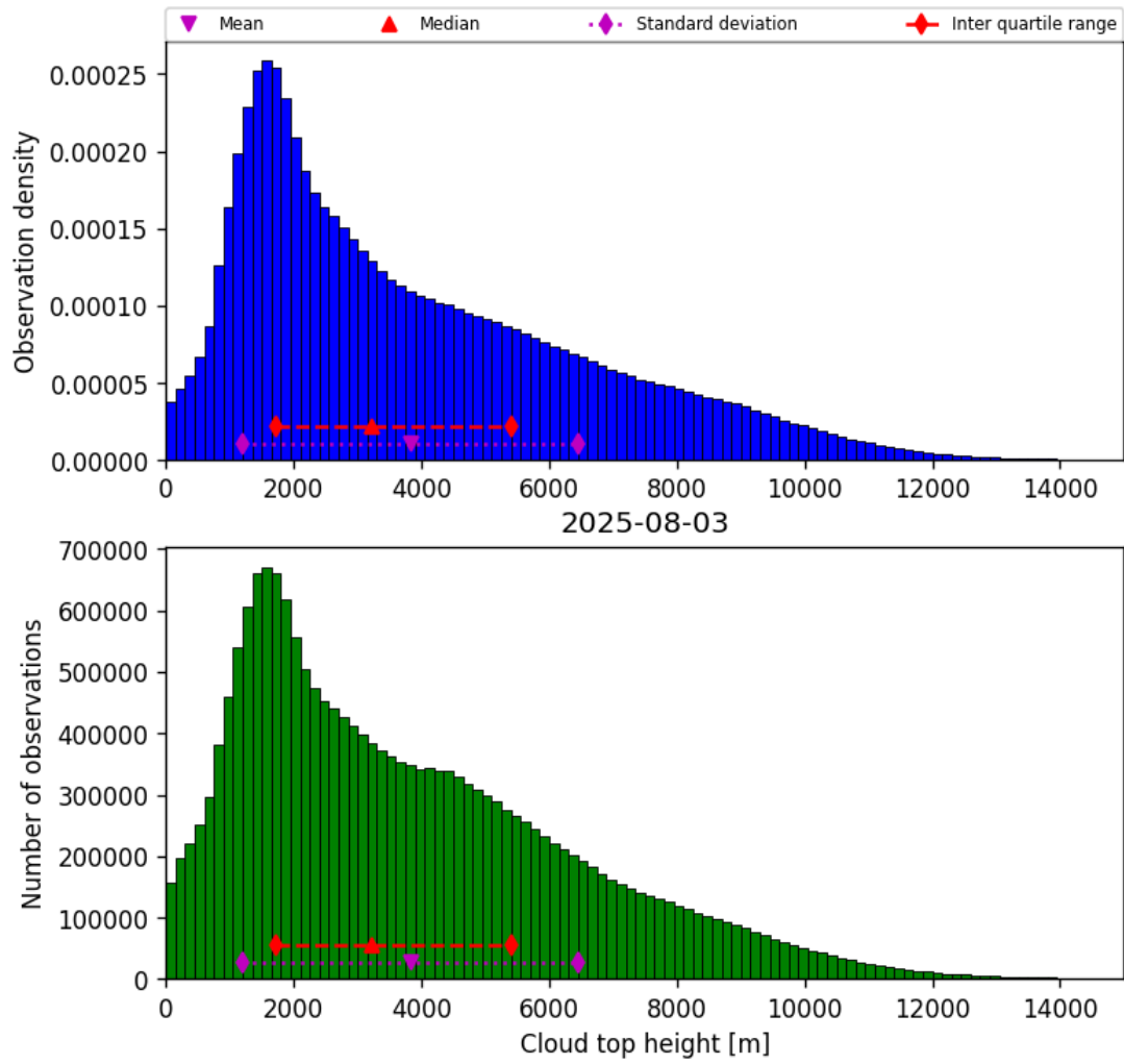
Figure 38: Histogram of “Cloud top height” for 2025-08-03 to 2025-08-04
