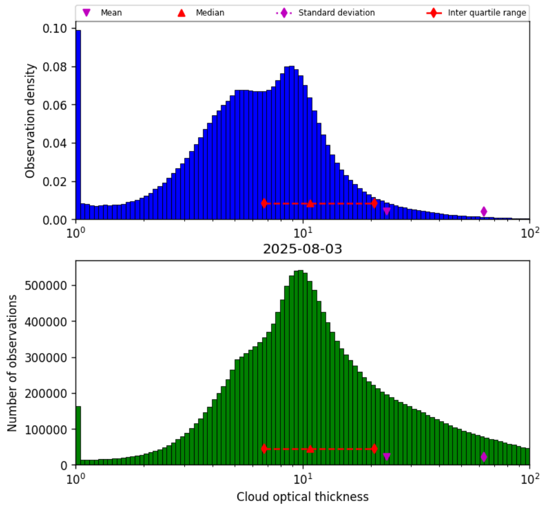
Figure 39: Histogram of “Cloud optical thickness” for 2025-08-03 to 2025-08-04
