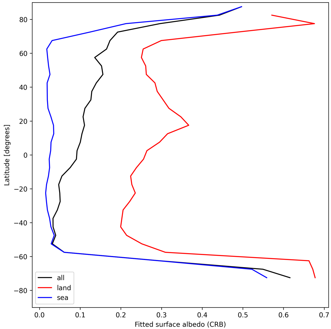
Figure 28: Zonal average of “Fitted surface albedo (CRB)” for 2025-08-03 to 2025-08-04.
