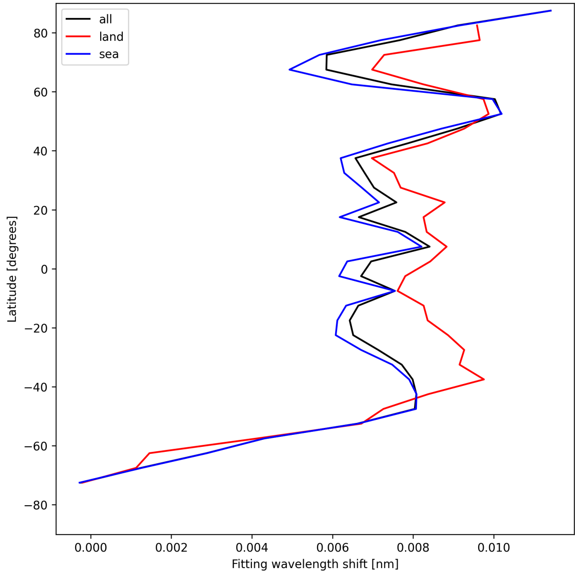
Figure 31: Zonal average of “Fitting wavelength shift” for 2025-08-03 to 2025-08-04.
