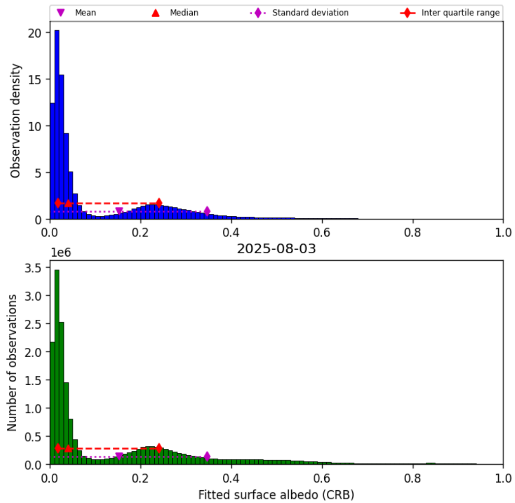
Figure 44: Histogram of “Fitted surface albedo (CRB)” for 2025-08-03 to 2025-08-04
