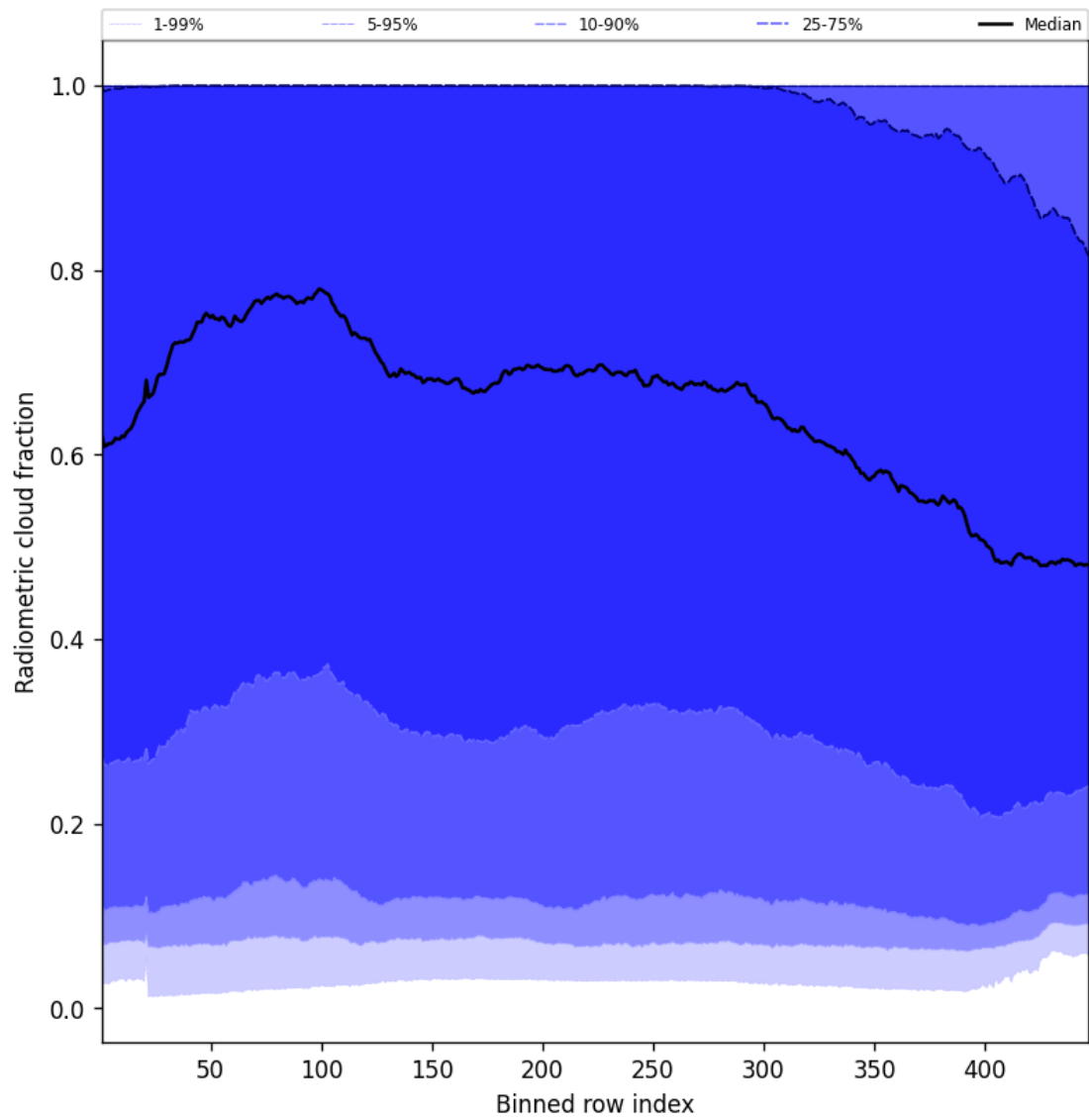
Figure 53: Along track statistics of “Radiometric cloud fraction” for 2025-08-03 to 2025-08-04
