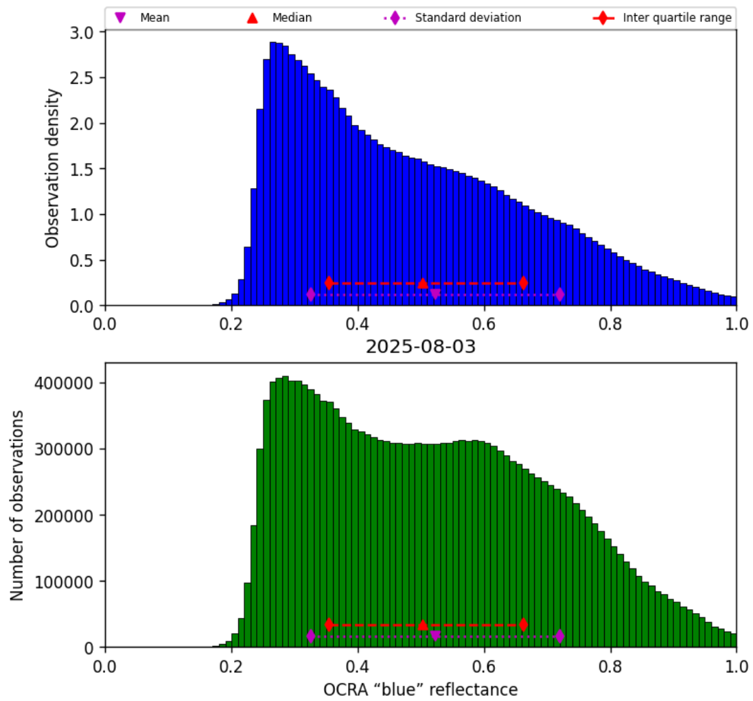
Figure 49: Histogram of “OCRA “blue” reflectance” for 2025-08-03 to 2025-08-04
