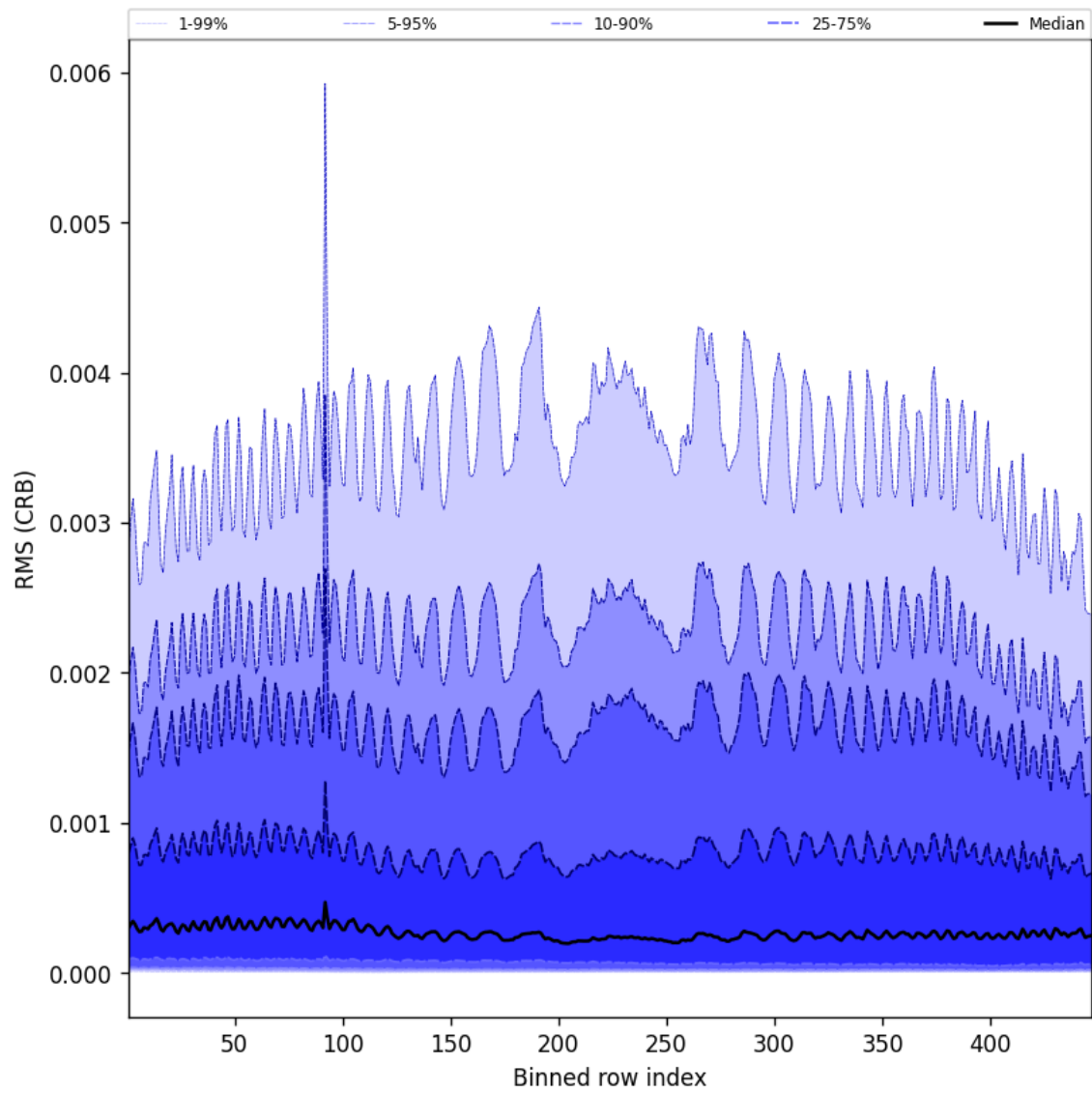
Figure 62: Along track statistics of “RMS (CRB)” for 2025-08-03 to 2025-08-04
