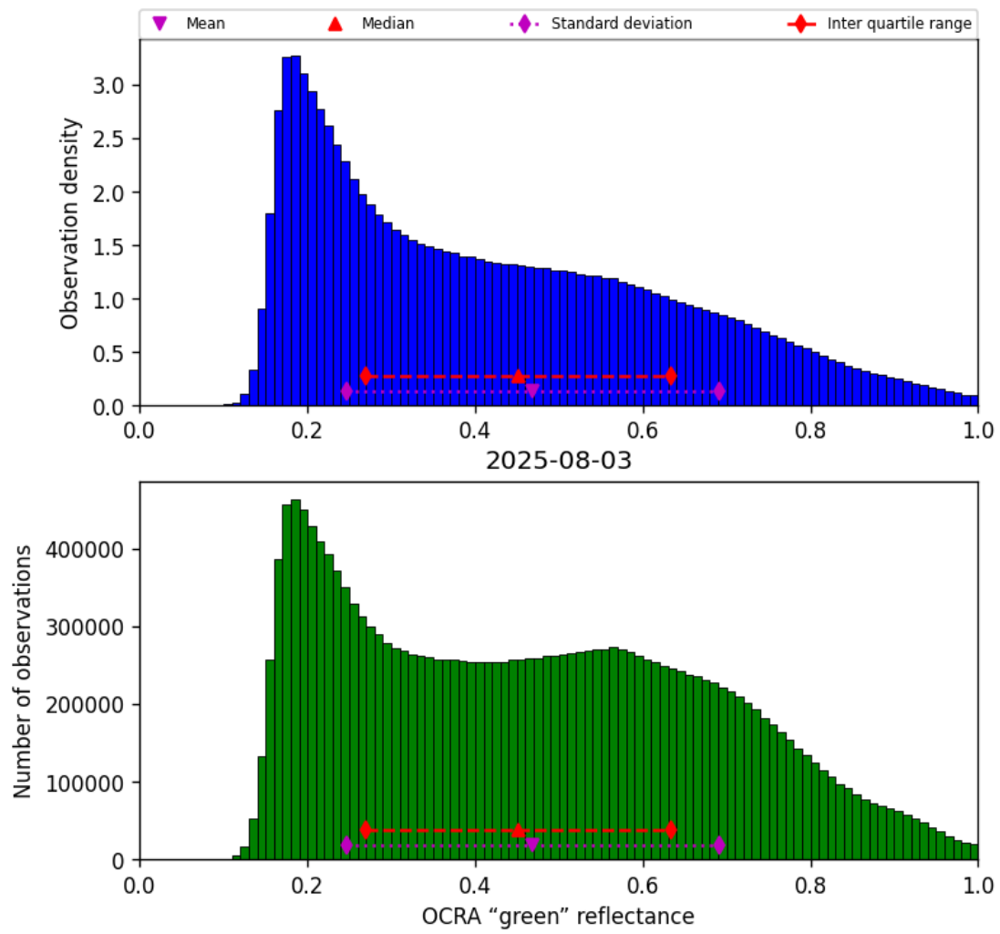
Figure 50: Histogram of “OCRA “green” reflectance” for 2025-08-03 to 2025-08-04
