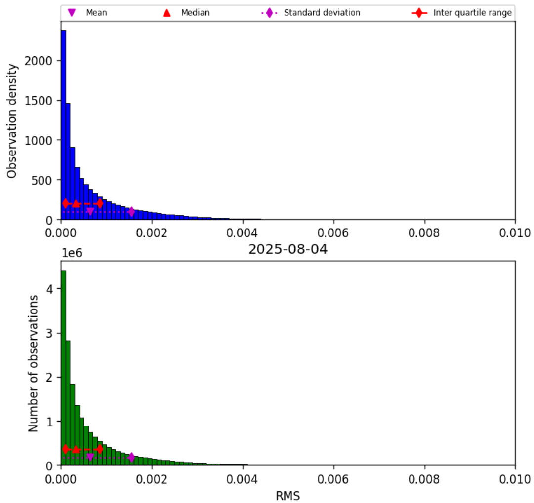
Figure 45: Histogram of “RMS” for 2025-08-04 to 2025-08-05
