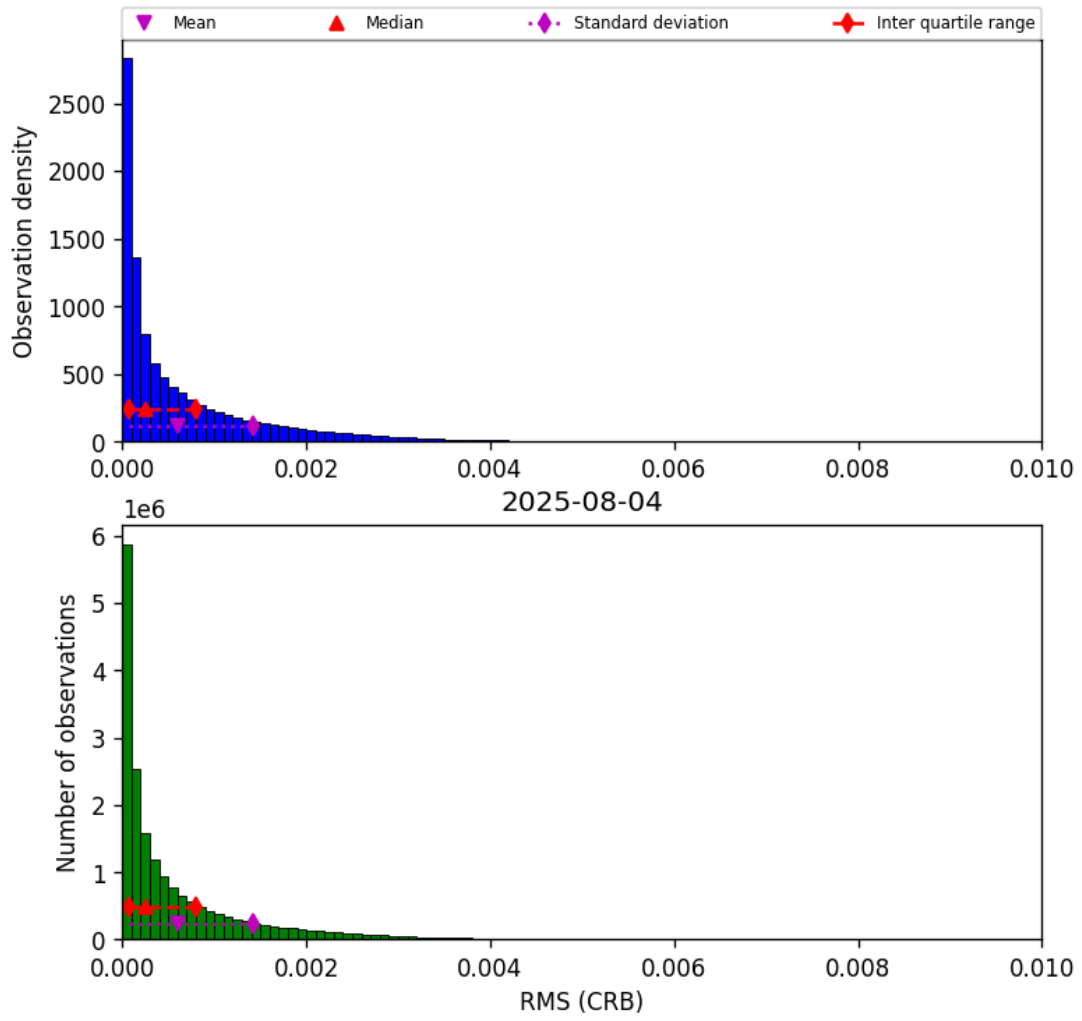
Figure 46: Histogram of “RMS (CRB)” for 2025-08-04 to 2025-08-05
