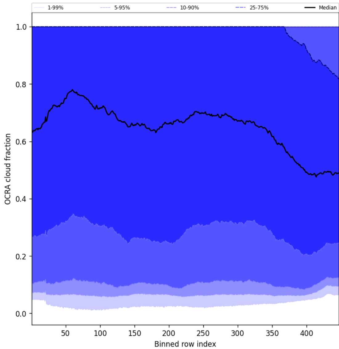
Figure 64: Along track statistics of “OCRA cloud fraction” for 2025-08-04 to 2025-08-05
