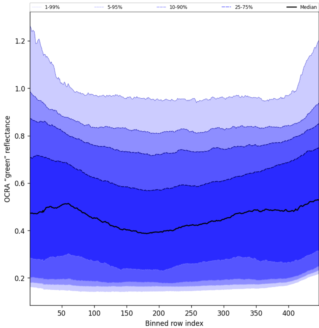
Figure 66: Along track statistics of “OCRA “green” reflectance” for 2025-08-04 to 2025-08-05
