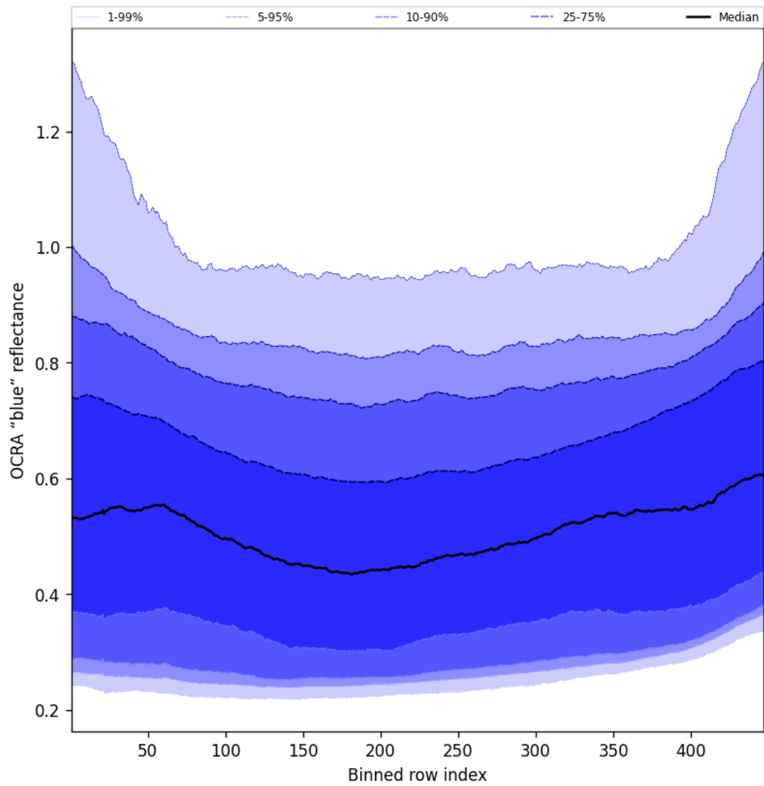
Figure 65: Along track statistics of “OCRA “blue” reflectance” for 2025-08-04 to 2025-08-05
