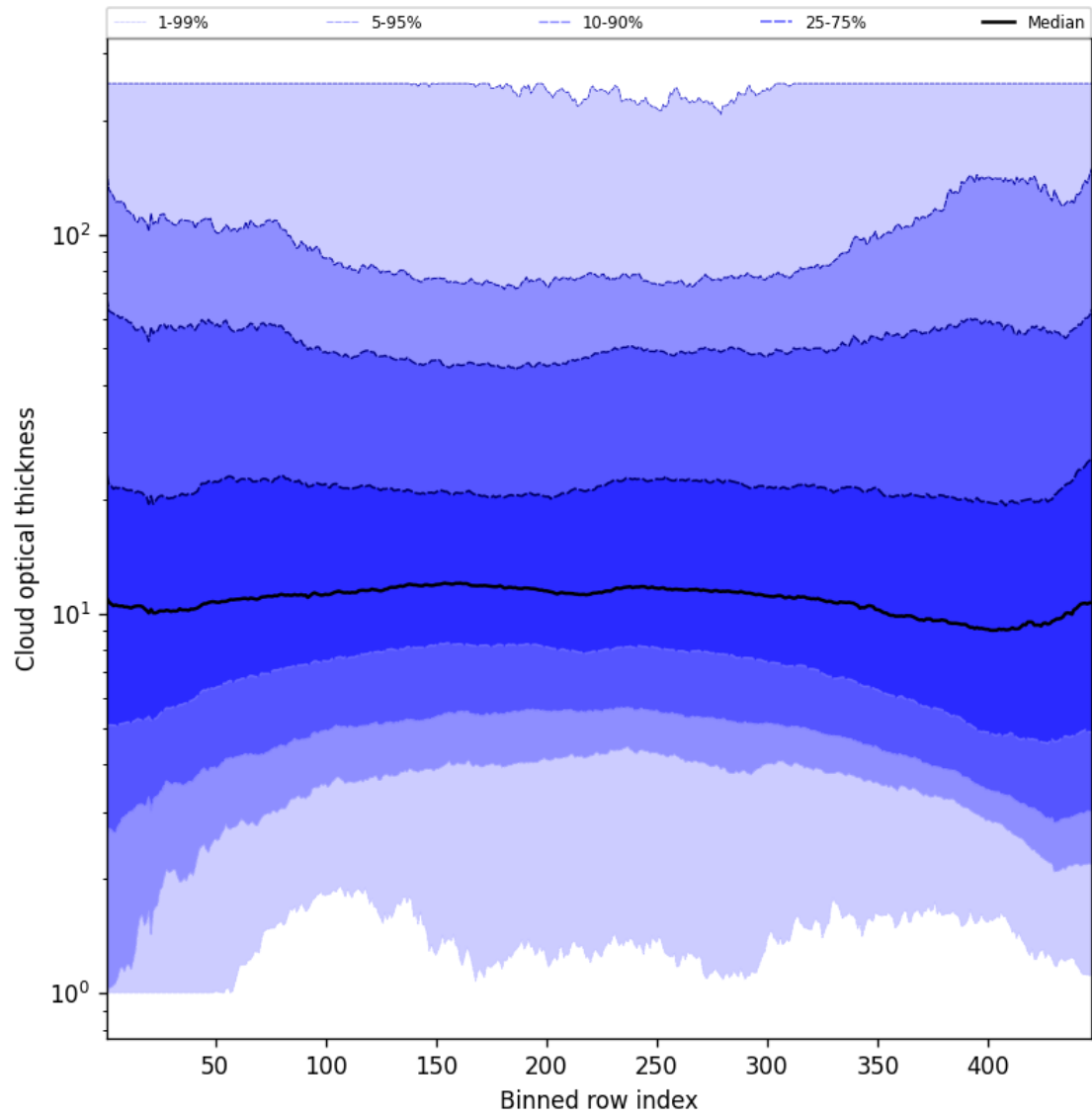
Figure 55: Along track statistics of “Cloud optical thickness” for 2025-08-04 to 2025-08-05
