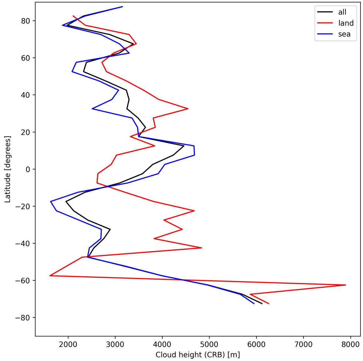
Figure 25: Zonal average of “Cloud height (CRB)” for 2025-08-04 to 2025-08-05.
