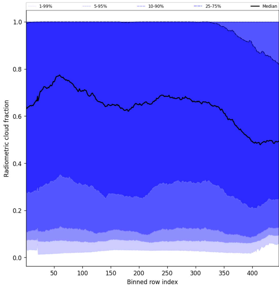
Figure 53: Along track statistics of “Radiometric cloud fraction” for 2025-08-04 to 2025-08-05
