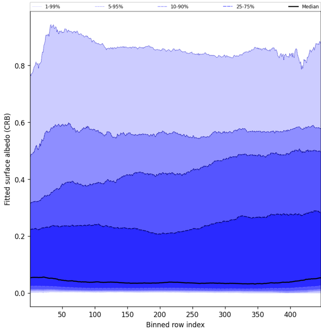
Figure 60: Along track statistics of “Fitted surface albedo (CRB)” for 2025-08-04 to 2025-08-05
