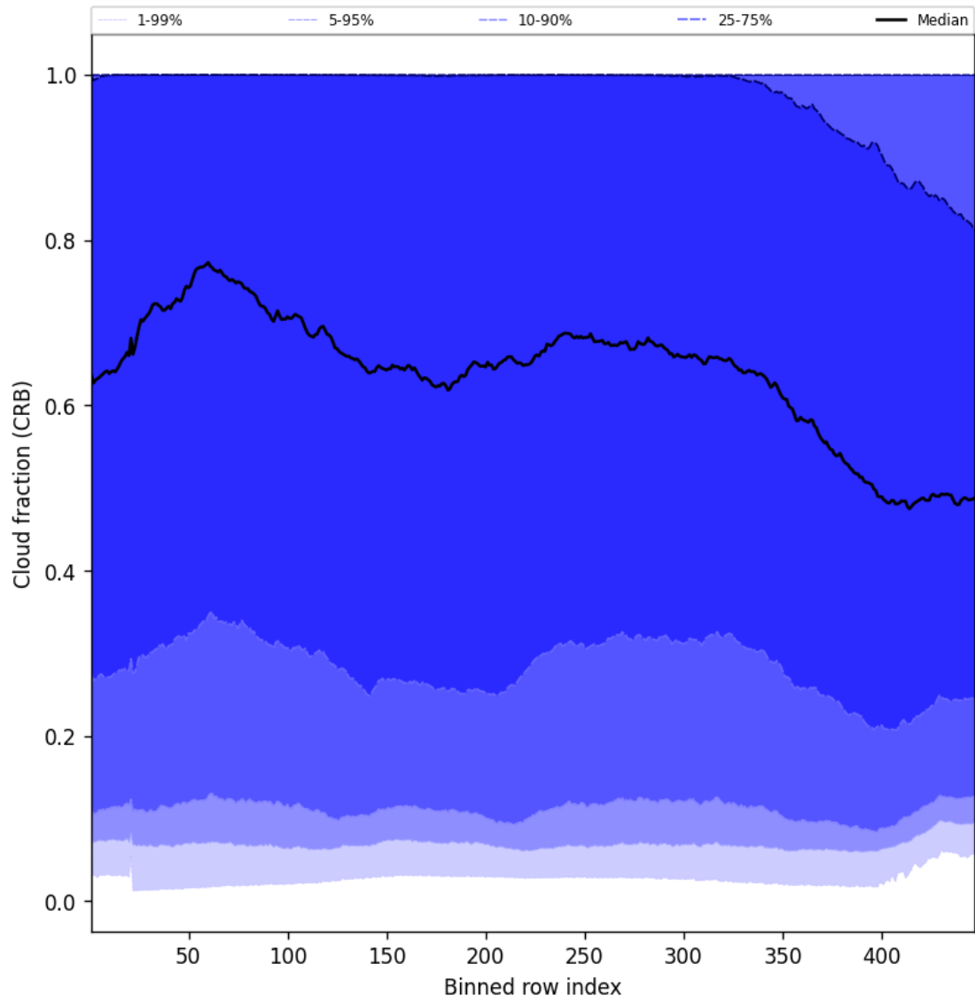
Figure 56: Along track statistics of “Cloud fraction (CRB)” for 2025-08-04 to 2025-08-05
