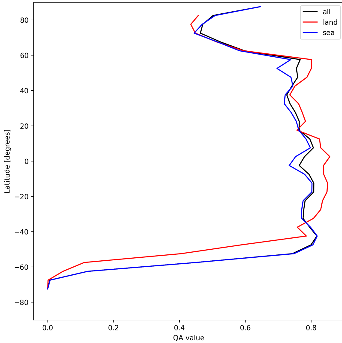
Figure 20: Zonal average of “QA value” for 2025-08-04 to 2025-08-05.
