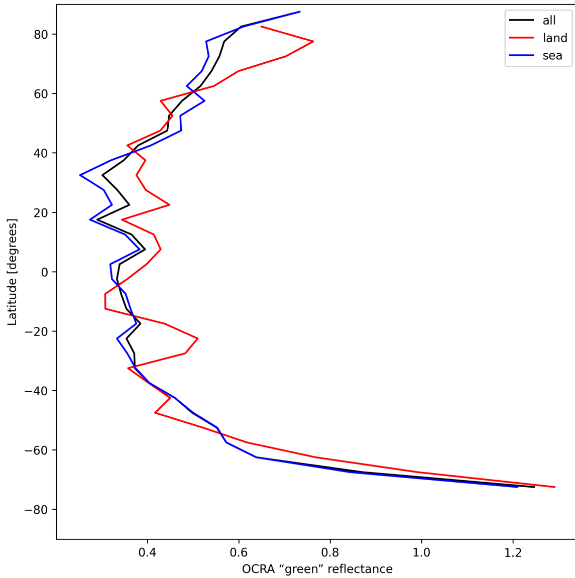
Figure 34: Zonal average of “OCRA “green” reflectance” for 2025-08-04 to 2025-08-05.
