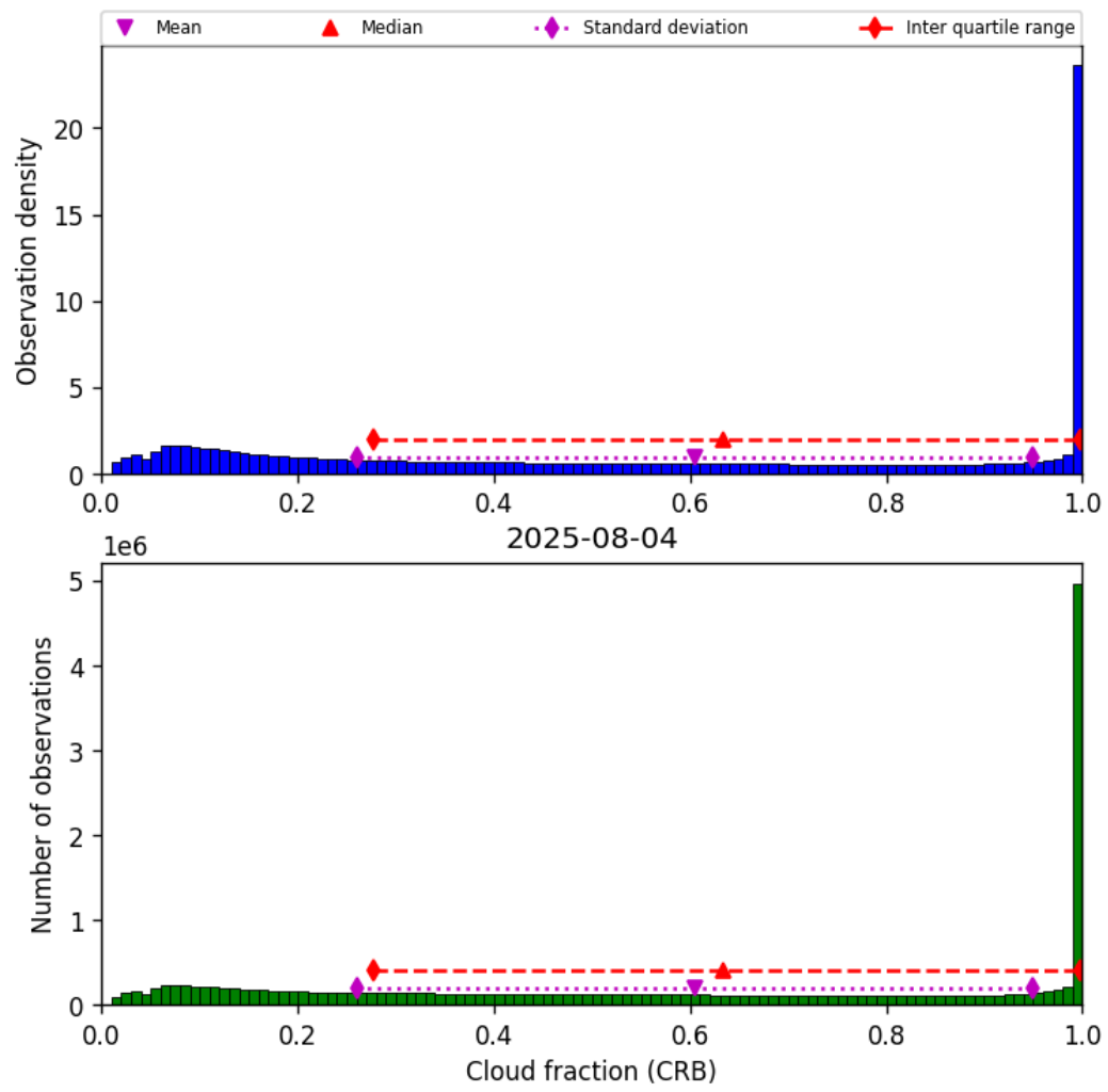
Figure 40: Histogram of “Cloud fraction (CRB)” for 2025-08-04 to 2025-08-05
