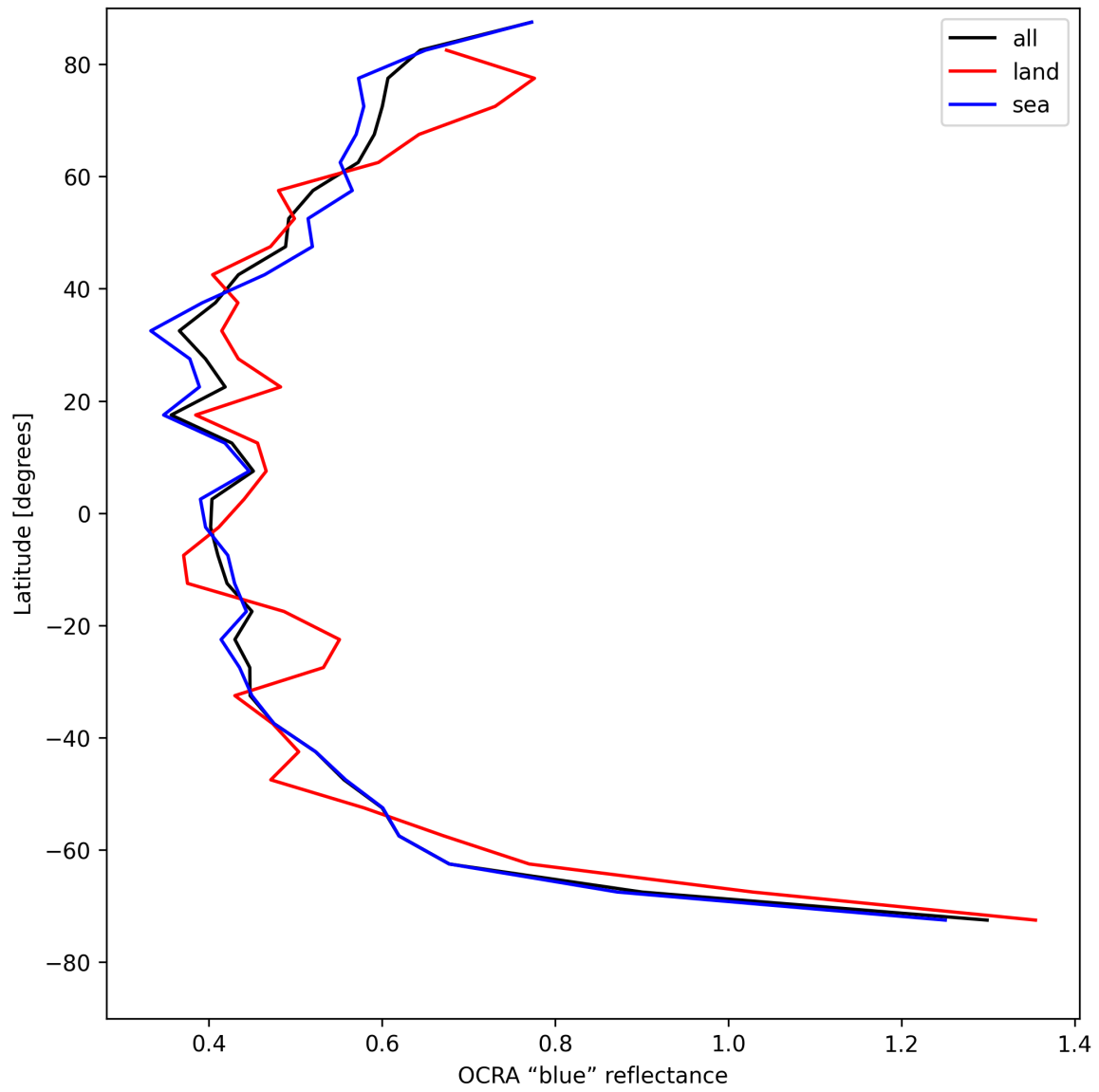
Figure 33: Zonal average of “OCRA “blue” reflectance” for 2025-08-04 to 2025-08-05.
