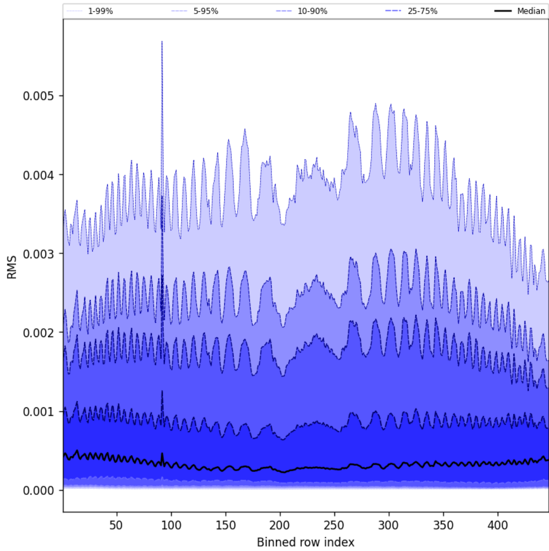
Figure 61: Along track statistics of “RMS” for 2025-08-04 to 2025-08-05
