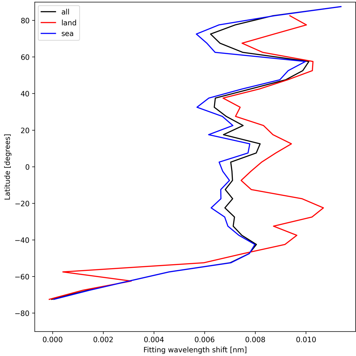
Figure 31: Zonal average of “Fitting wavelength shift” for 2025-08-04 to 2025-08-05.
