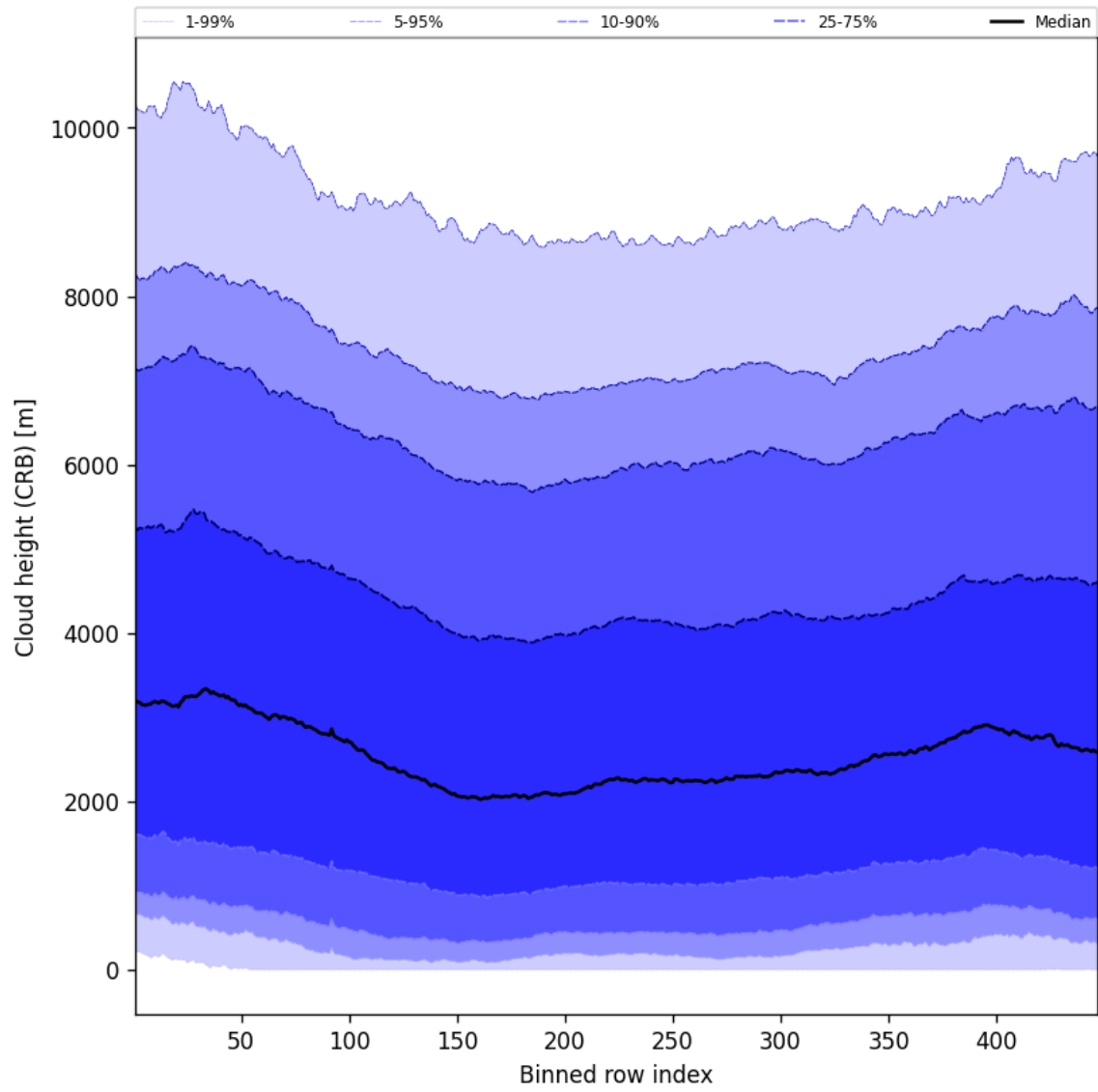
Figure 57: Along track statistics of “Cloud height (CRB)” for 2025-08-04 to 2025-08-05
