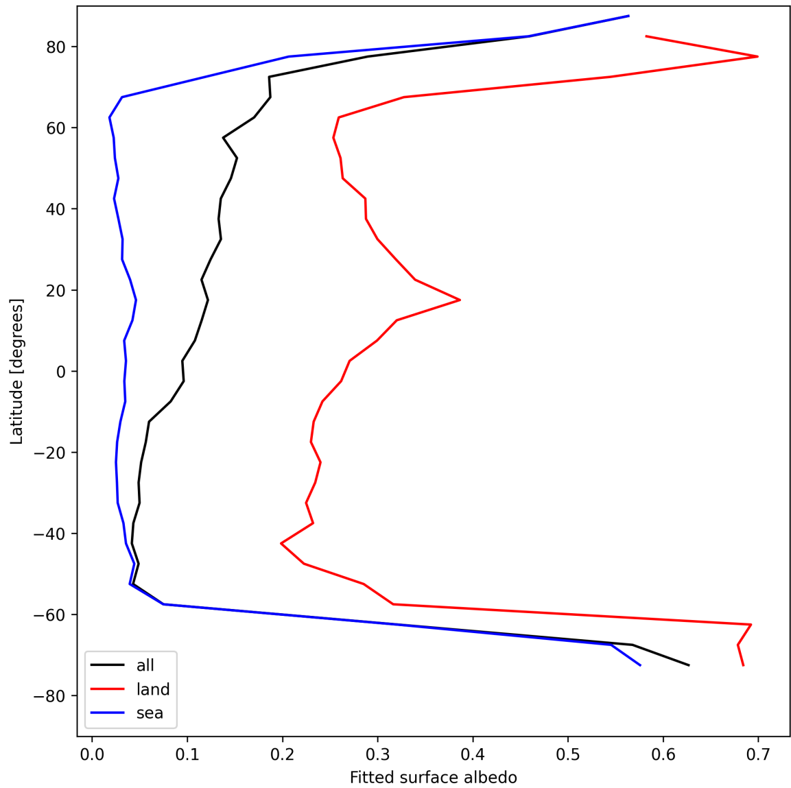
Figure 27: Zonal average of “Fitted surface albedo” for 2025-08-04 to 2025-08-05.
