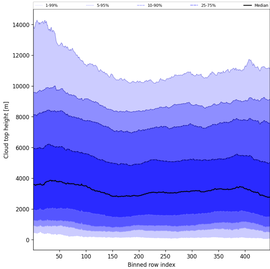
Figure 54: Along track statistics of “Cloud top height” for 2025-08-04 to 2025-08-05
