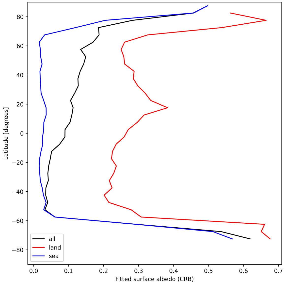
Figure 28: Zonal average of “Fitted surface albedo (CRB)” for 2025-08-04 to 2025-08-05.
