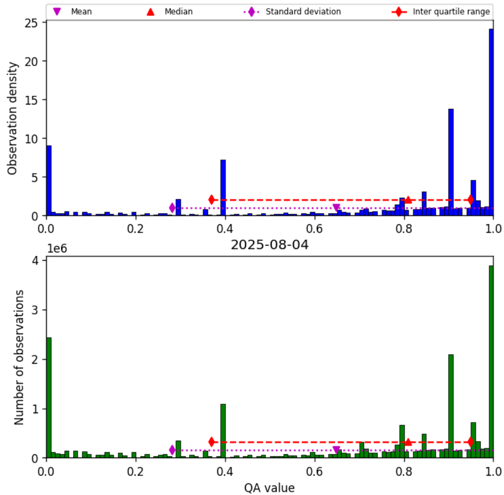
Figure 36: Histogram of “QA value” for 2025-08-04 to 2025-08-05
