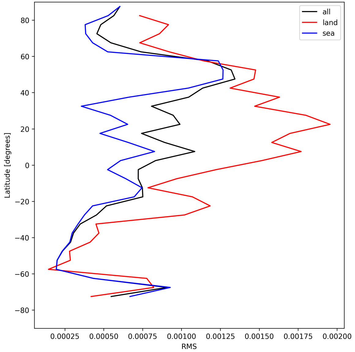
Figure 29: Zonal average of “RMS” for 2025-08-04 to 2025-08-05.
