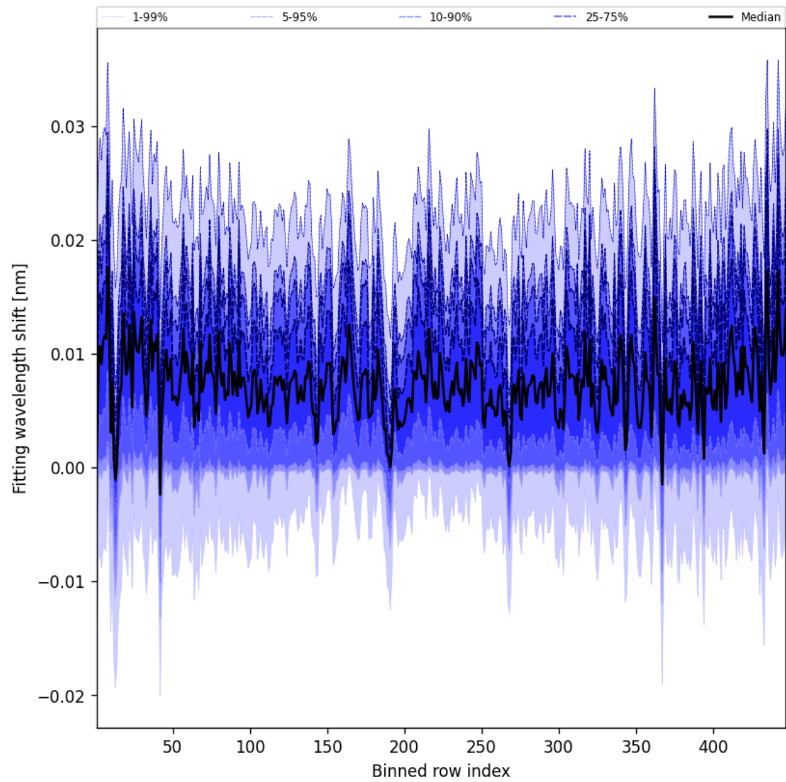
Figure 63: Along track statistics of “Fitting wavelength shift” for 2025-08-04 to 2025-08-05
