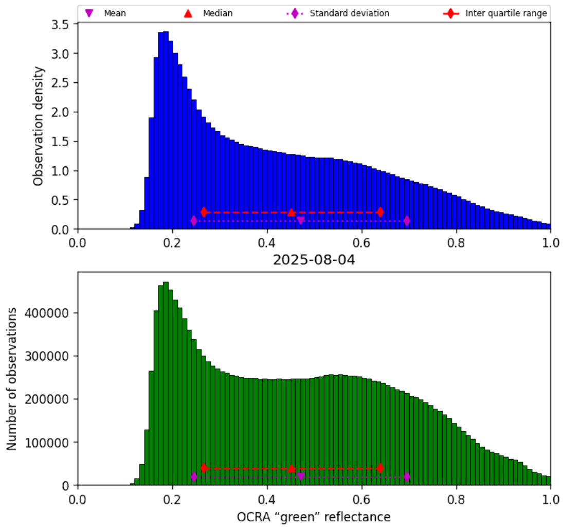
Figure 50: Histogram of “OCRA “green” reflectance” for 2025-08-04 to 2025-08-05
