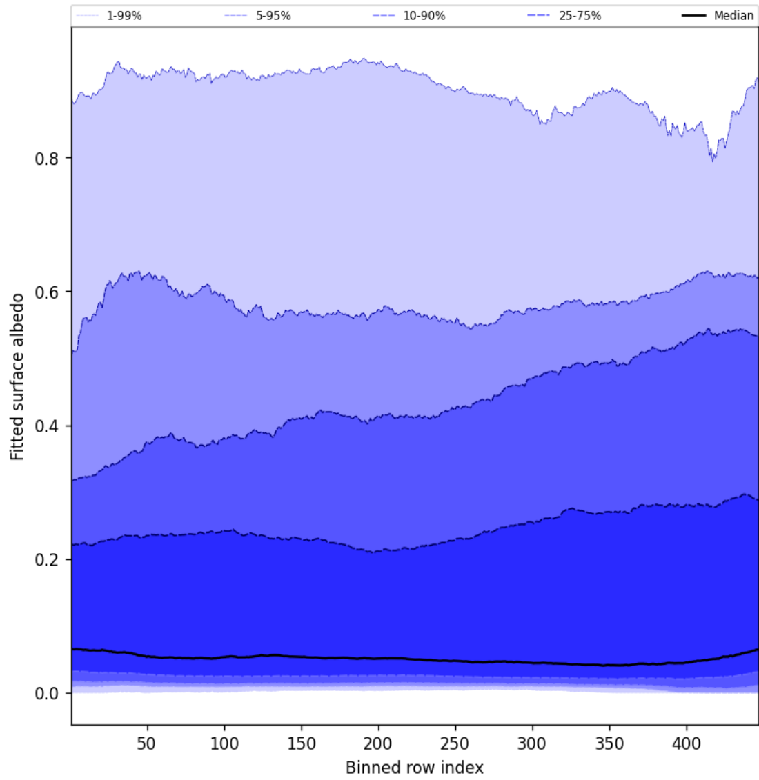
Figure 59: Along track statistics of “Fitted surface albedo” for 2025-08-04 to 2025-08-05
