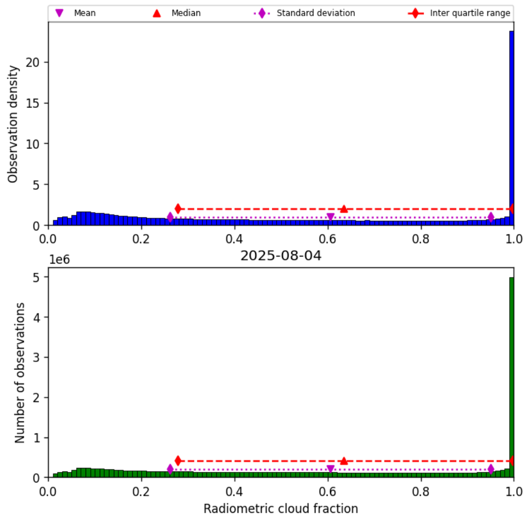
Figure 37: Histogram of “Radiometric cloud fraction” for 2025-08-04 to 2025-08-05
