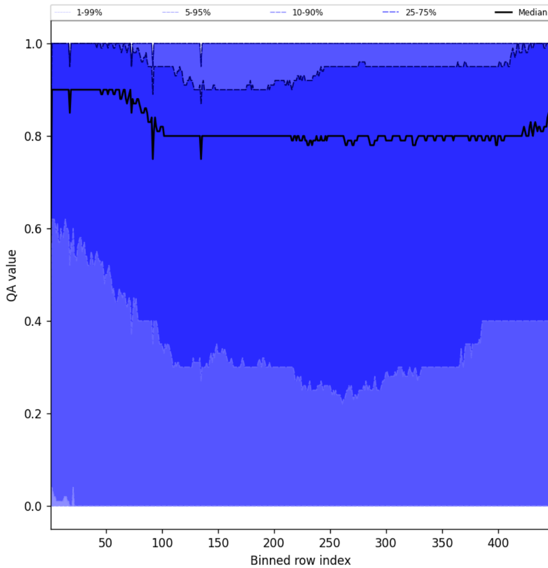
Figure 52: Along track statistics of “QA value” for 2025-08-04 to 2025-08-05
