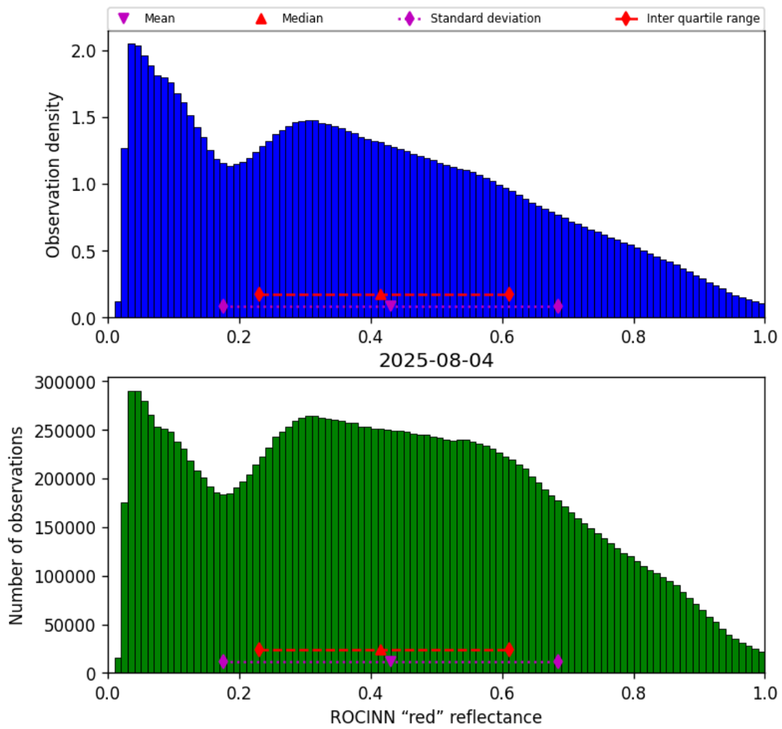
Figure 51: Histogram of “ROCINN “red” reflectance” for 2025-08-04 to 2025-08-05
