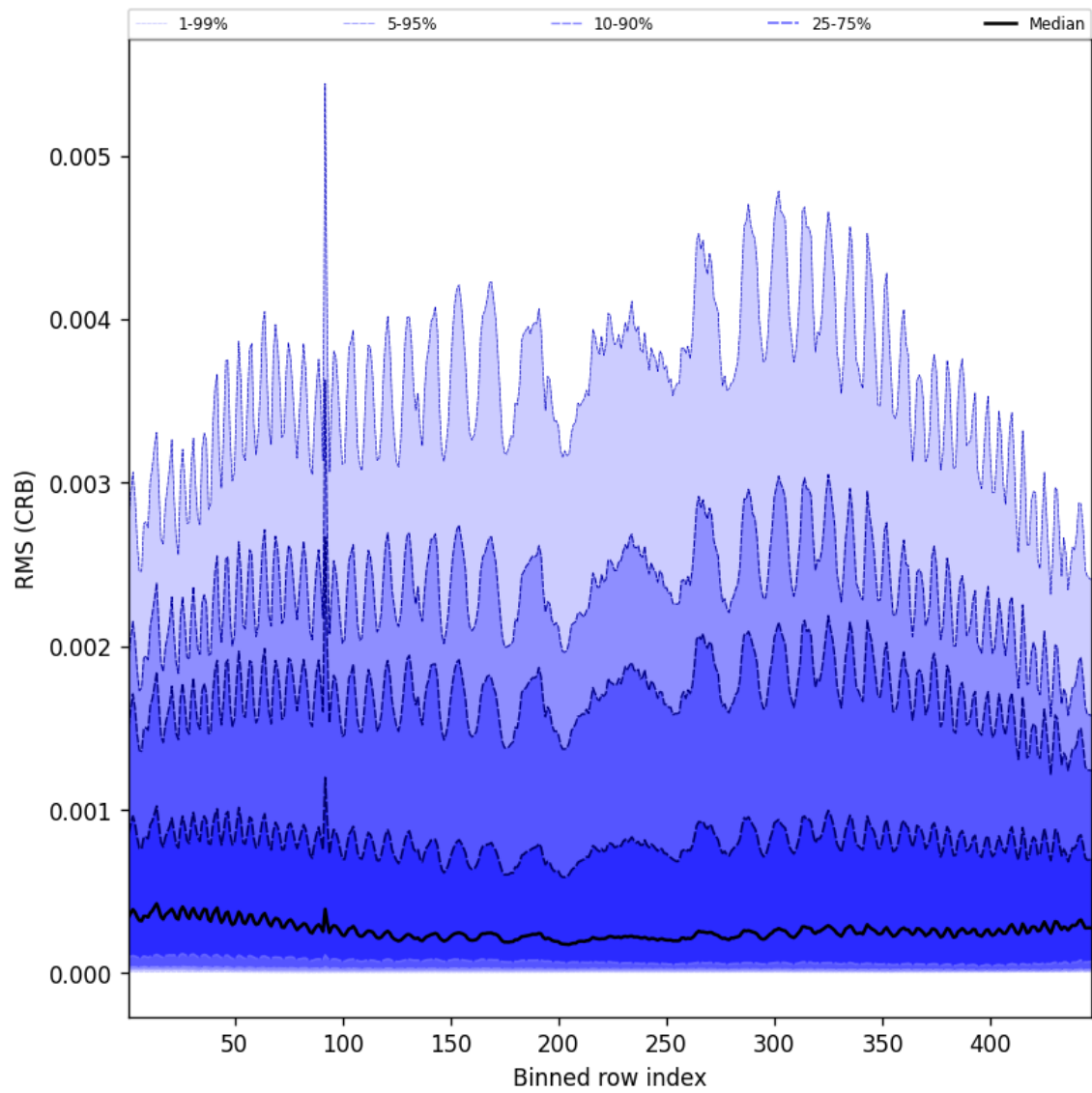
Figure 62: Along track statistics of “RMS (CRB)” for 2025-08-04 to 2025-08-05
