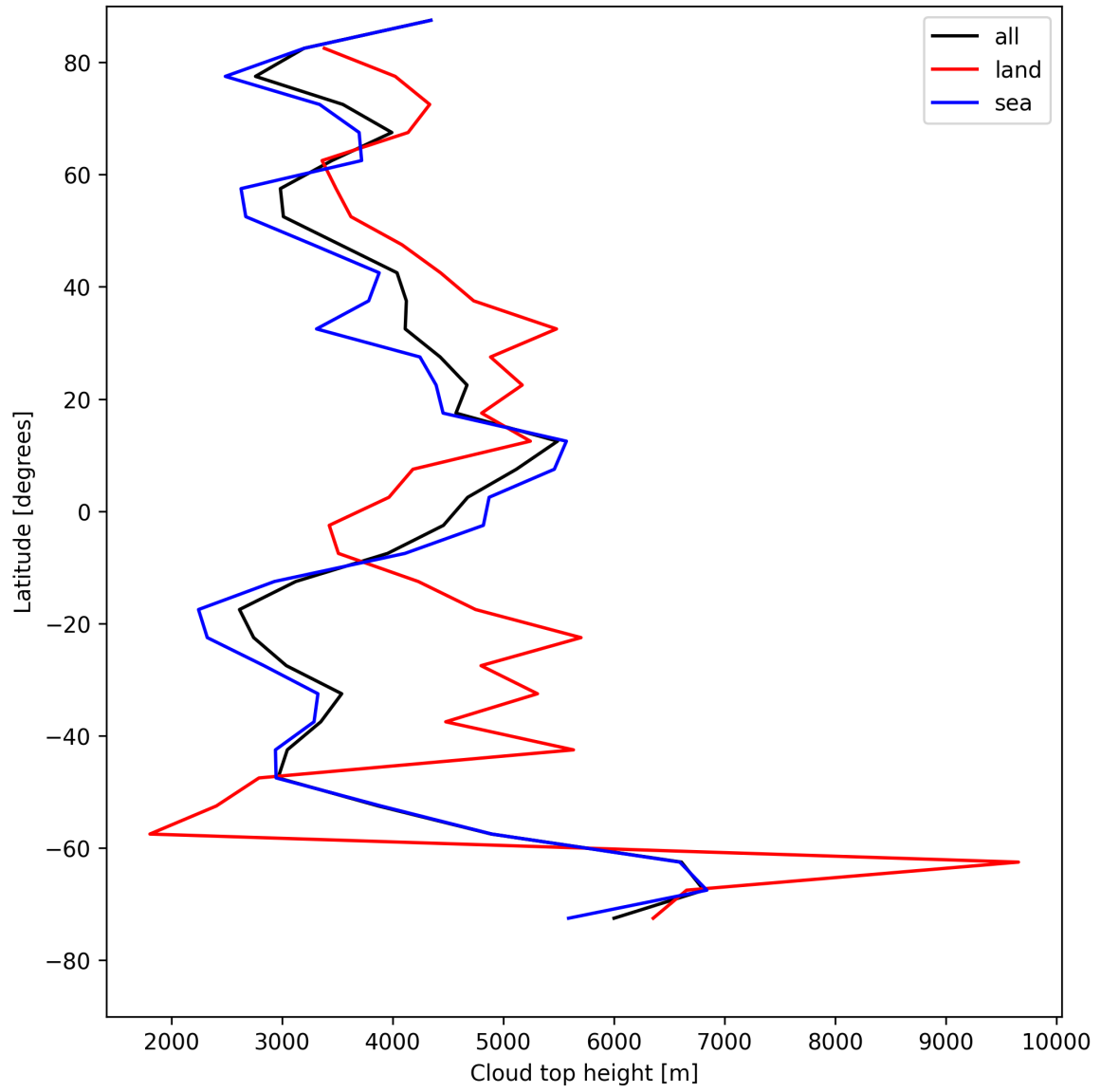
Figure 22: Zonal average of “Cloud top height” for 2025-08-04 to 2025-08-05.
