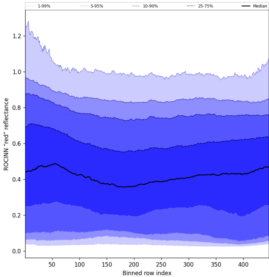
Figure 67: Along track statistics of "ROCINN "red" reflectance" for 2025-08-04 to 2025-08-05
