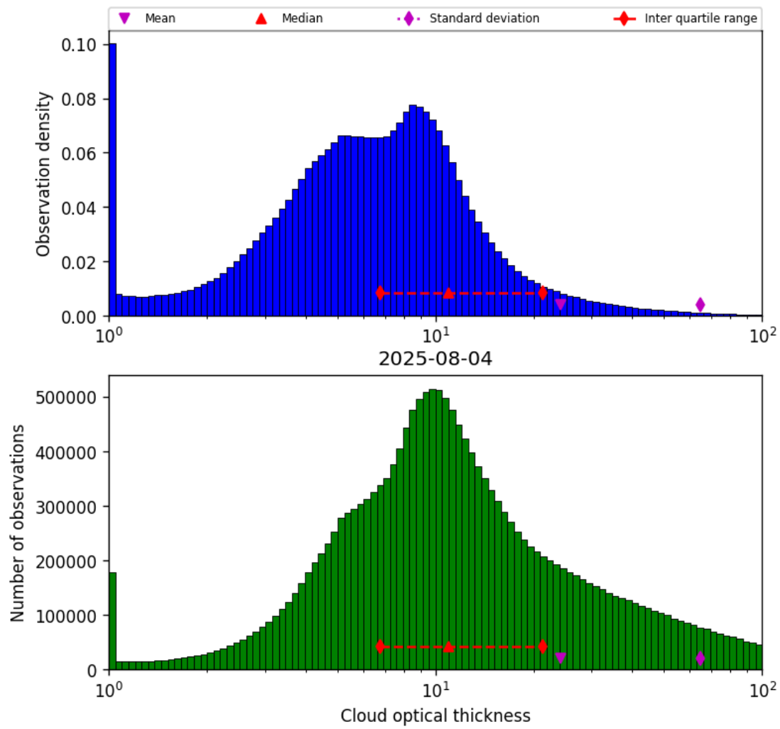
Figure 39: Histogram of “Cloud optical thickness” for 2025-08-04 to 2025-08-05
