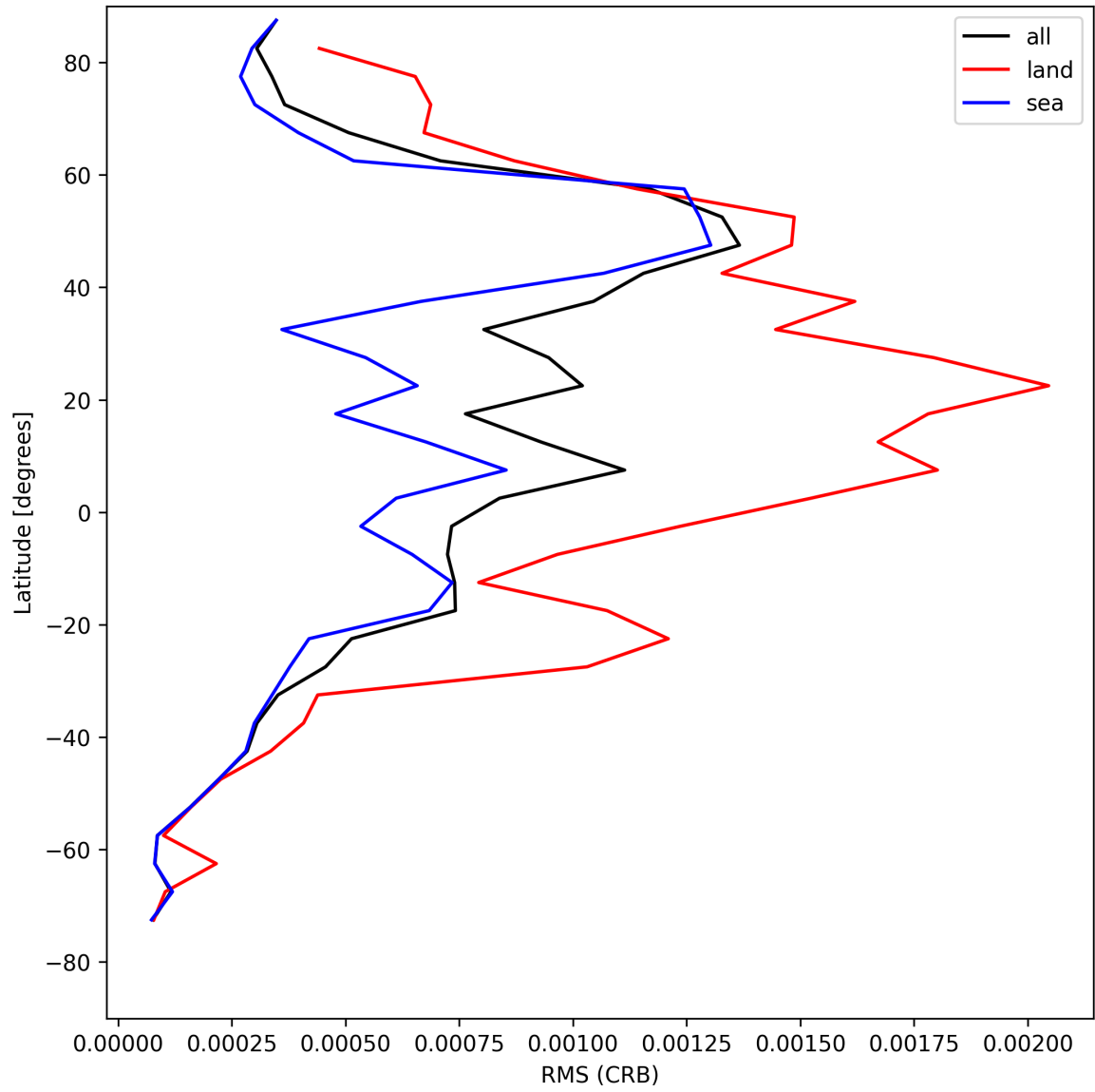
Figure 30: Zonal average of “RMS (CRB)” for 2025-08-04 to 2025-08-05.
