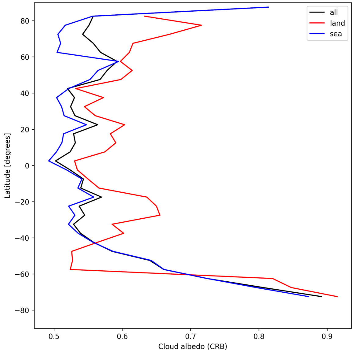
Figure 26: Zonal average of “Cloud albedo (CRB)” for 2025-08-04 to 2025-08-05.
