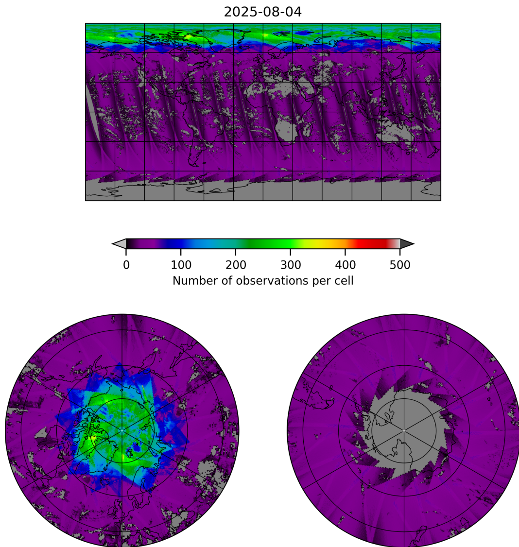
Figure 19: Map of the number of observations for 2025-08-04 to 2025-08-05
