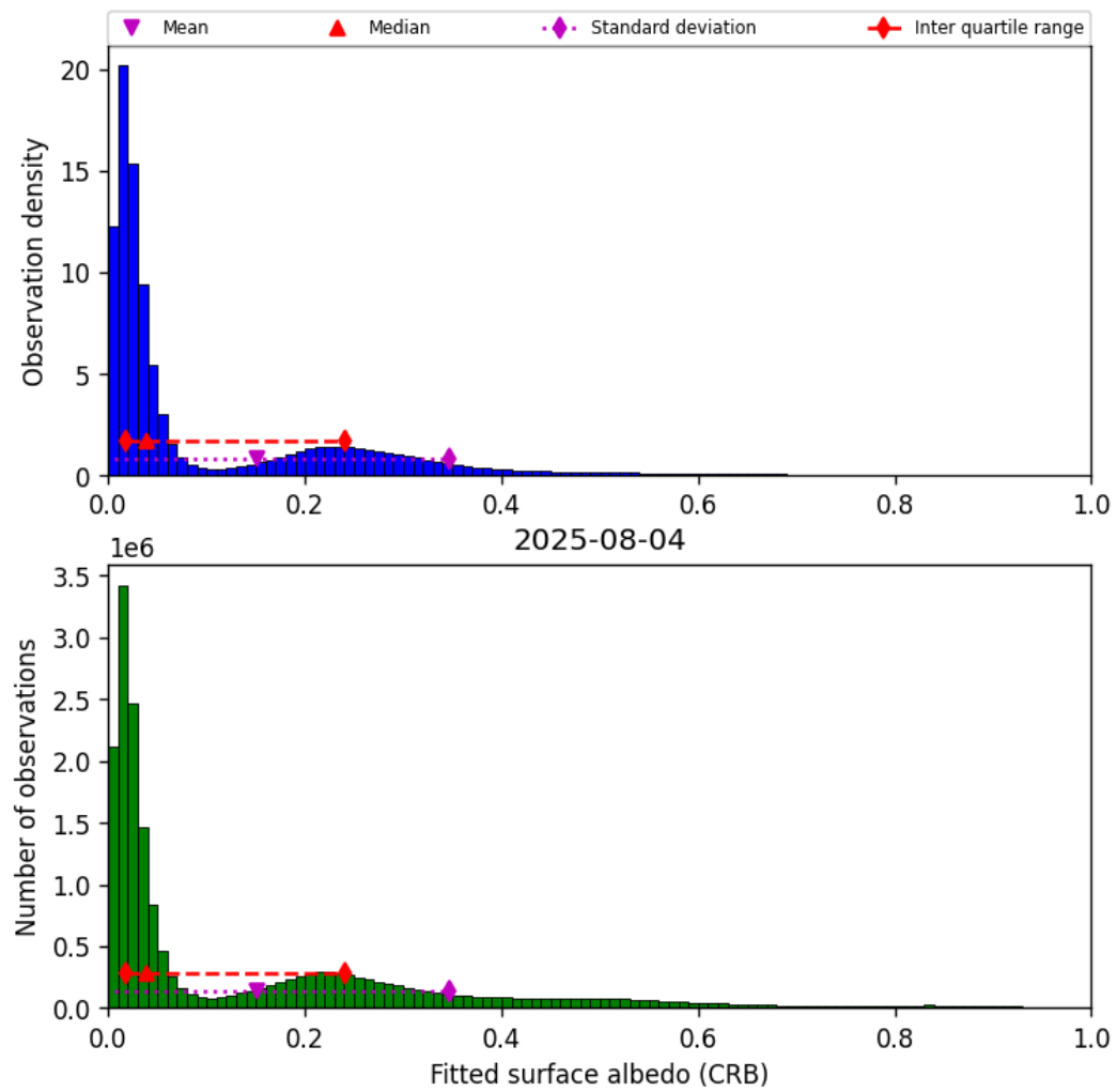
Figure 44: Histogram of “Fitted surface albedo (CRB)” for 2025-08-04 to 2025-08-05
