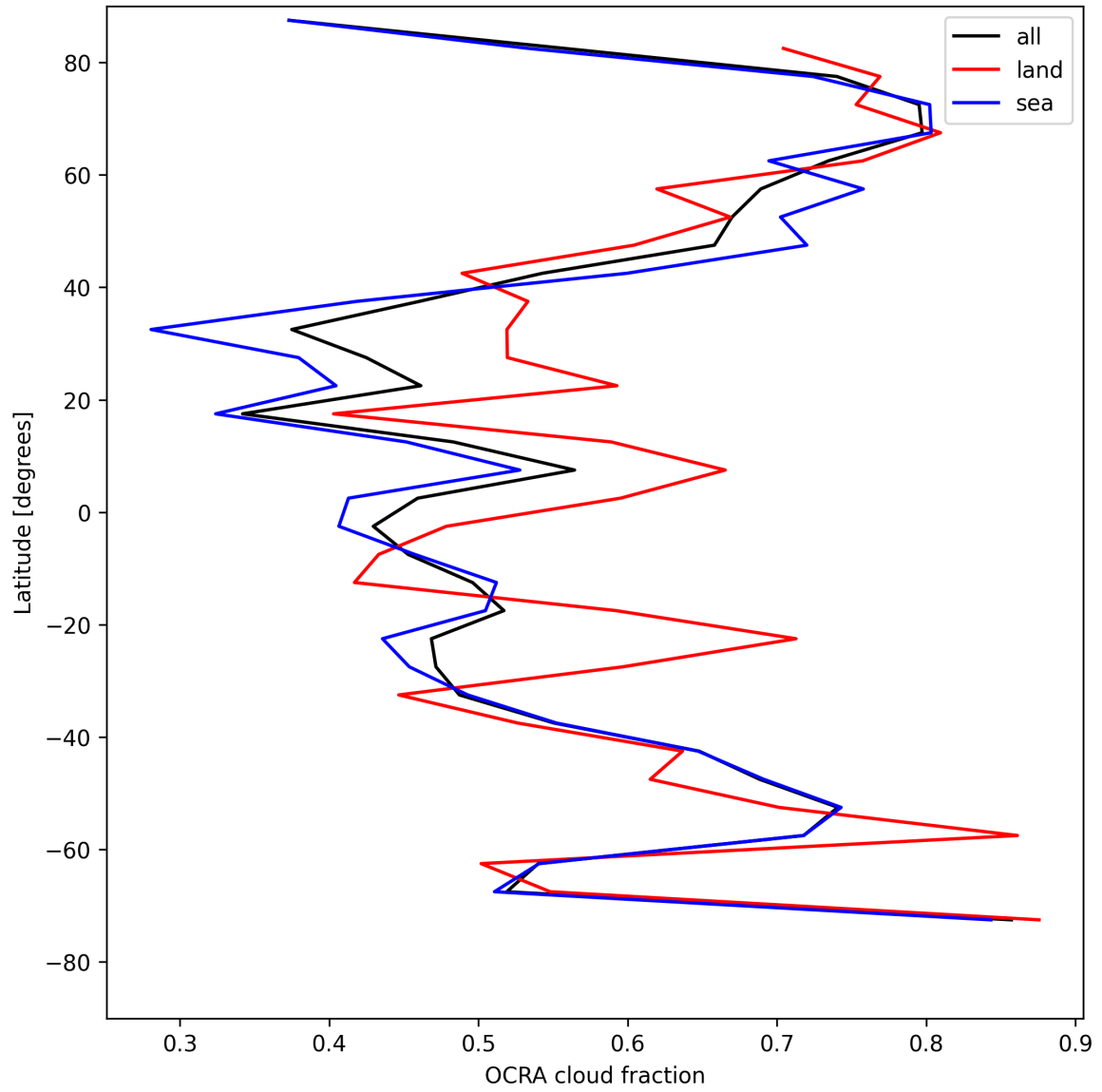
Figure 32: Zonal average of “OCRA cloud fraction” for 2025-08-04 to 2025-08-05.
