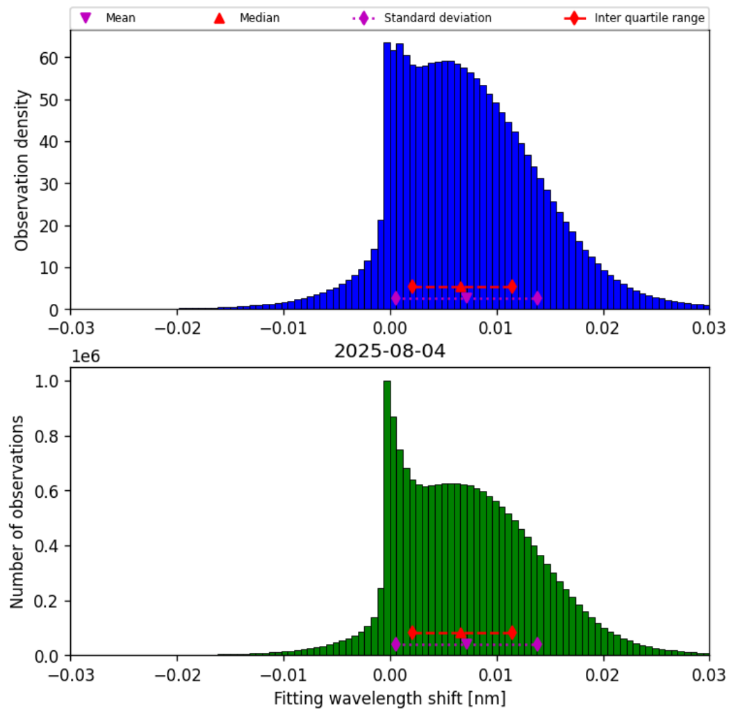
Figure 47: Histogram of “Fitting wavelength shift” for 2025-08-04 to 2025-08-05
