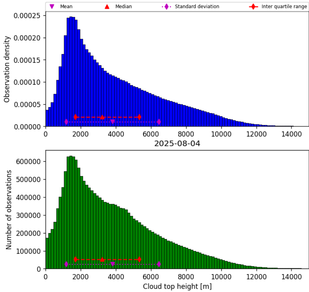
Figure 38: Histogram of “Cloud top height” for 2025-08-04 to 2025-08-05
