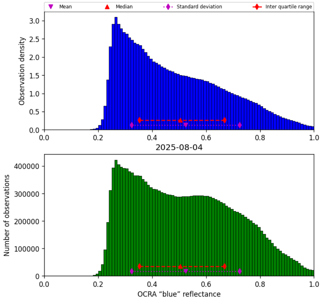
Figure 49: Histogram of “OCRA “blue” reflectance” for 2025-08-04 to 2025-08-05
