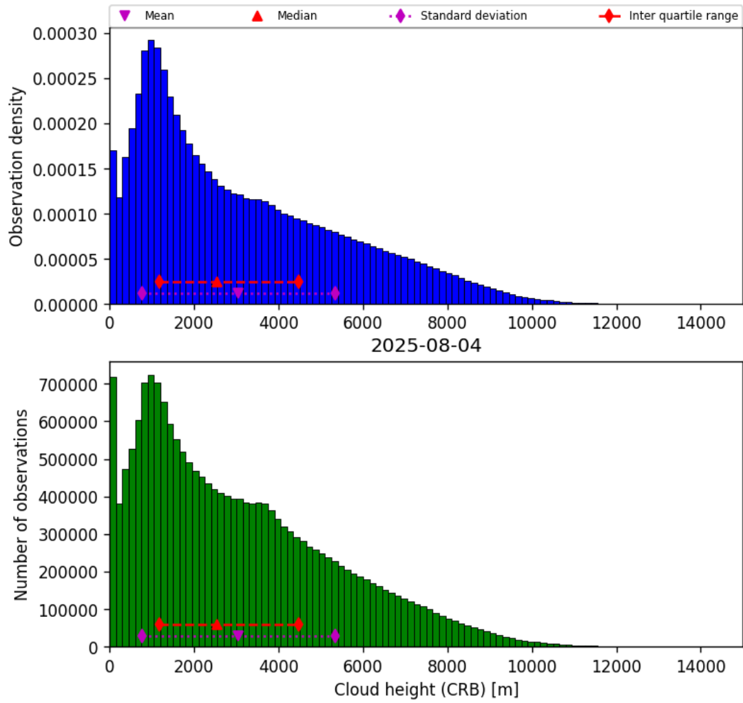
Figure 41: Histogram of “Cloud height (CRB)” for 2025-08-04 to 2025-08-05
