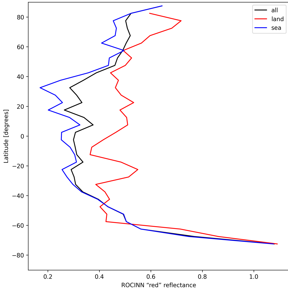
Figure 35: Zonal average of “ROCINN “red” reflectance” for 2025-08-04 to 2025-08-05.
