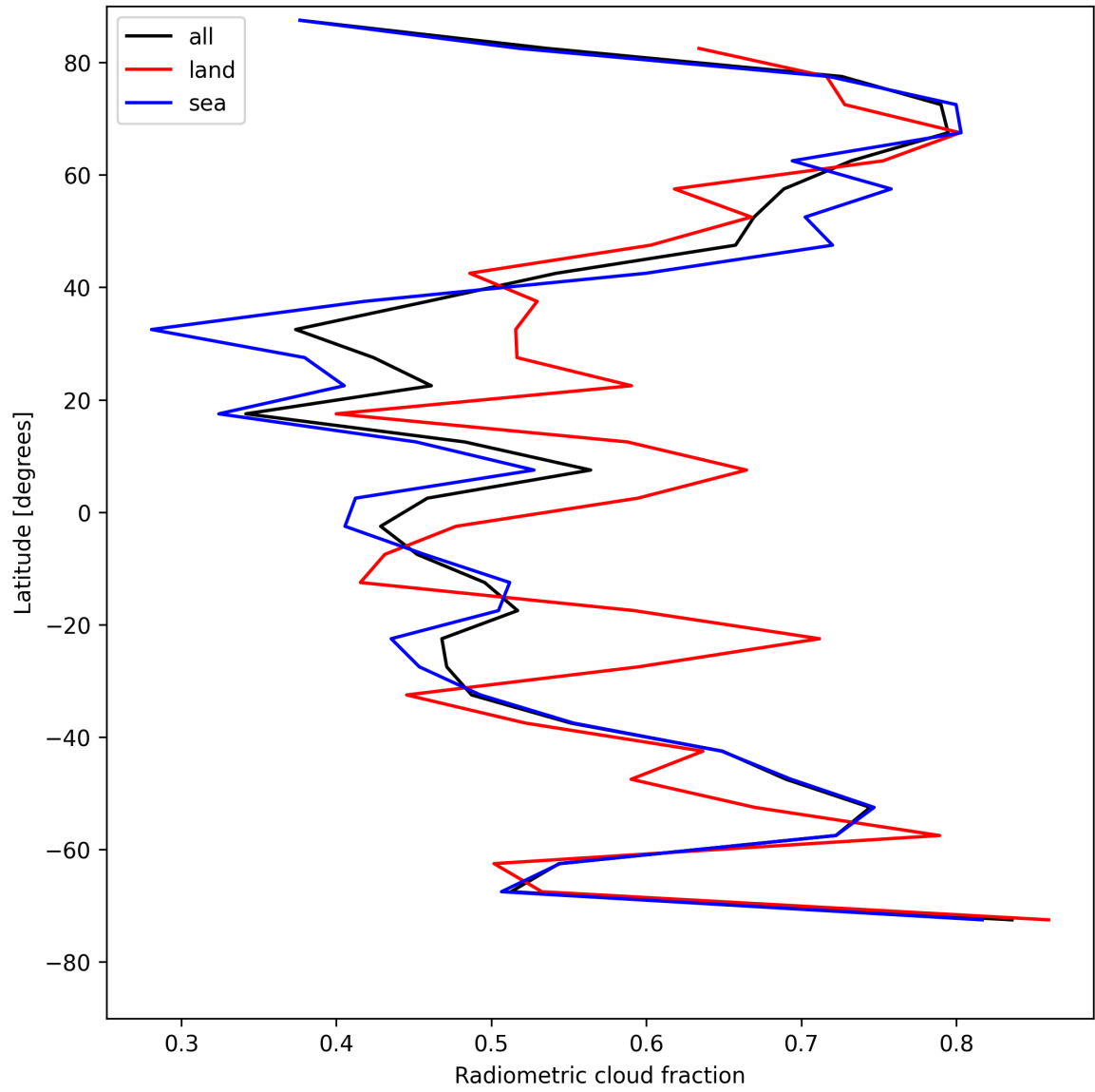
Figure 21: Zonal average of “Radiometric cloud fraction” for 2025-08-04 to 2025-08-05.
