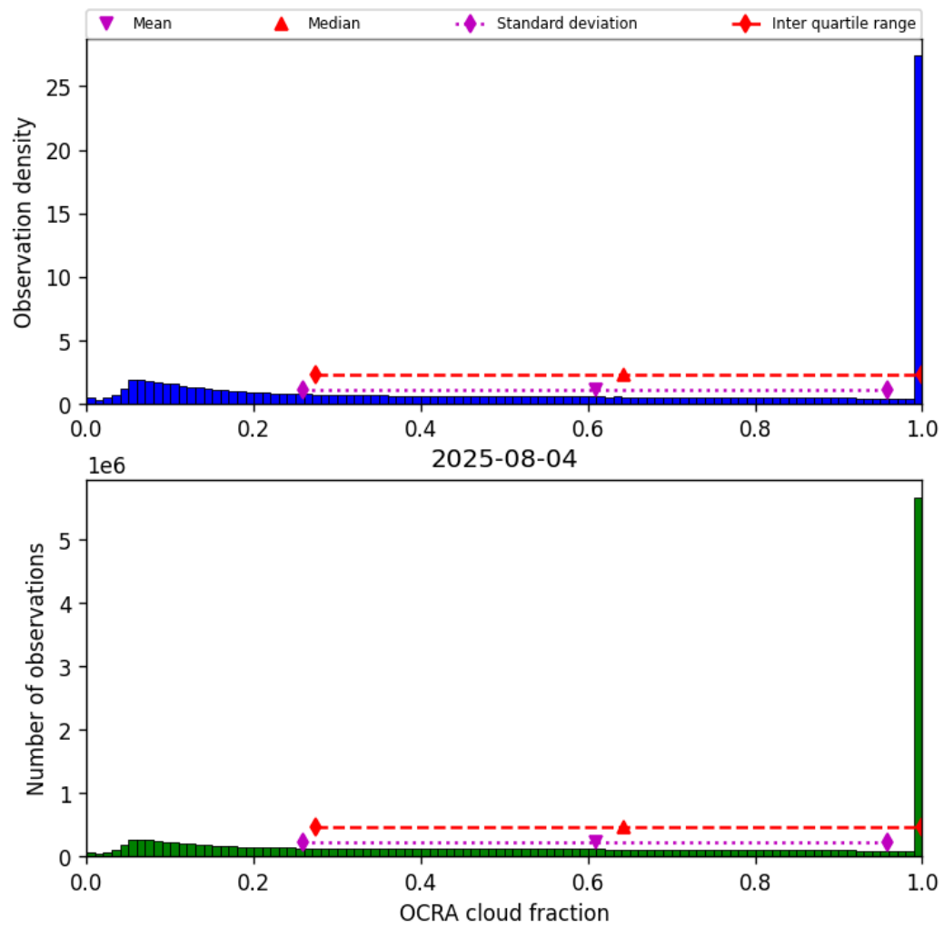
Figure 48: Histogram of “OCRA cloud fraction” for 2025-08-04 to 2025-08-05
