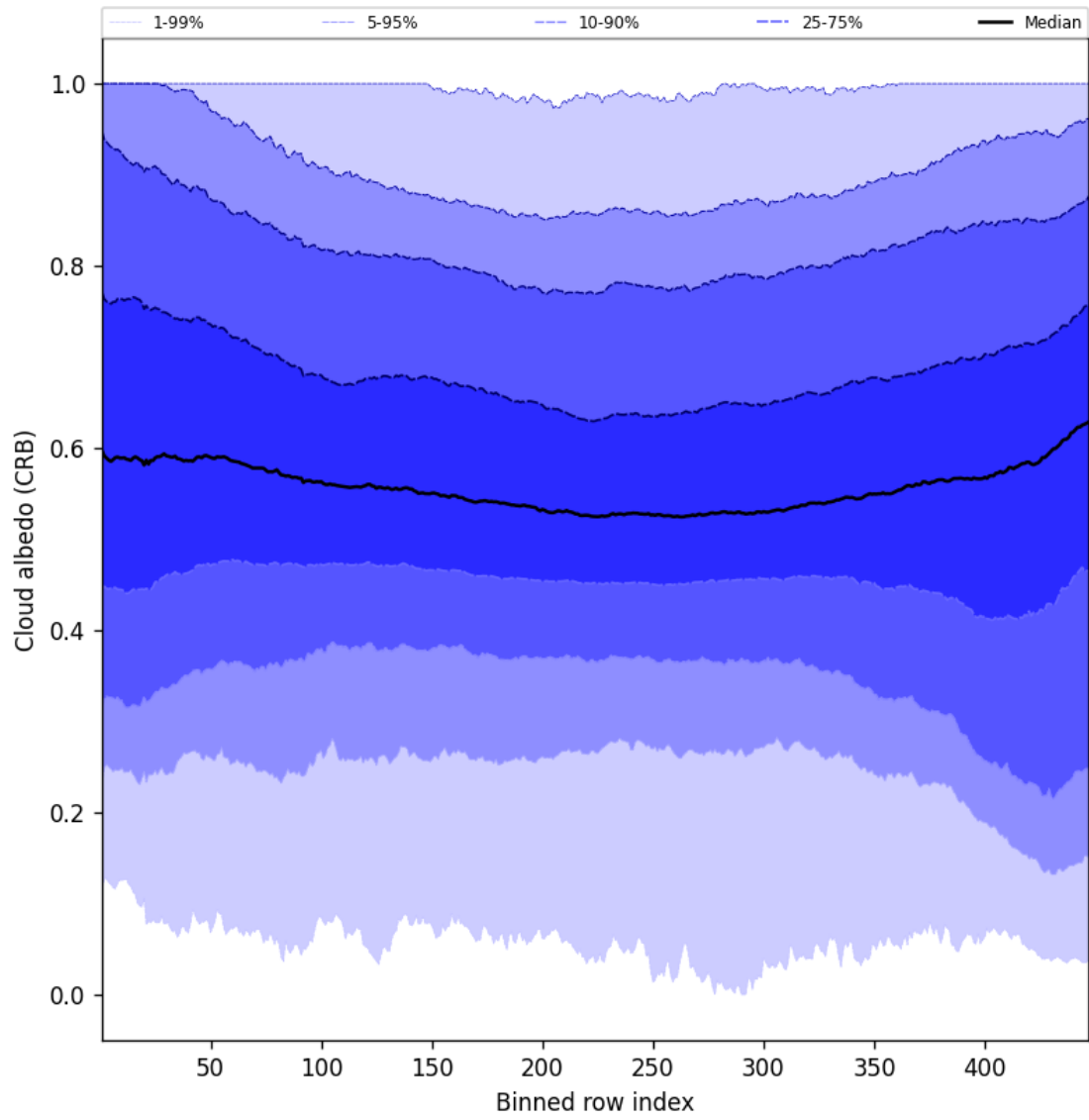
Figure 58: Along track statistics of “Cloud albedo (CRB)” for 2025-08-04 to 2025-08-05
