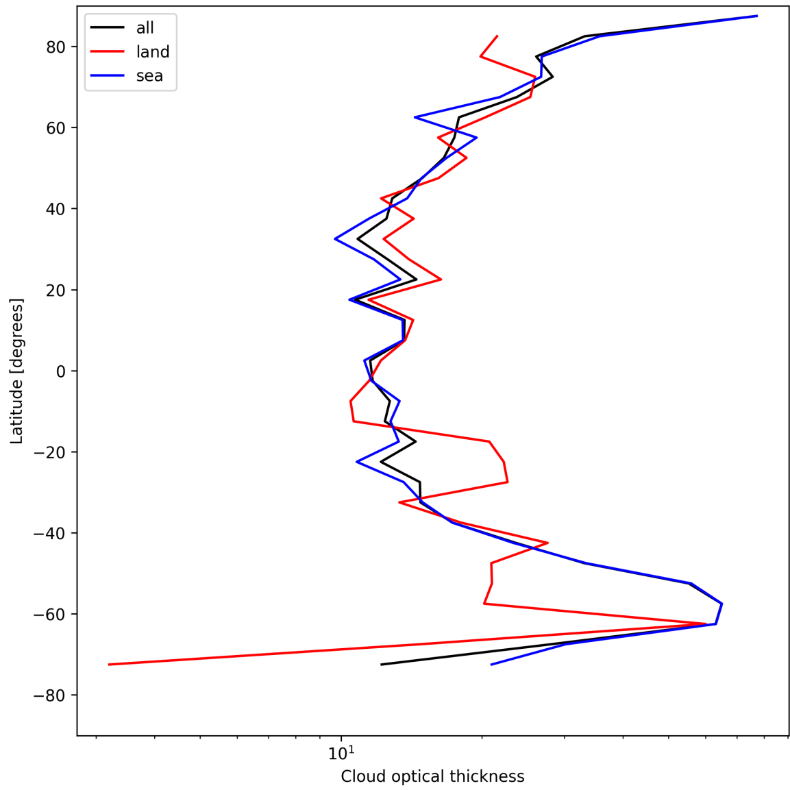
Figure 23: Zonal average of “Cloud optical thickness” for 2025-08-04 to 2025-08-05.
