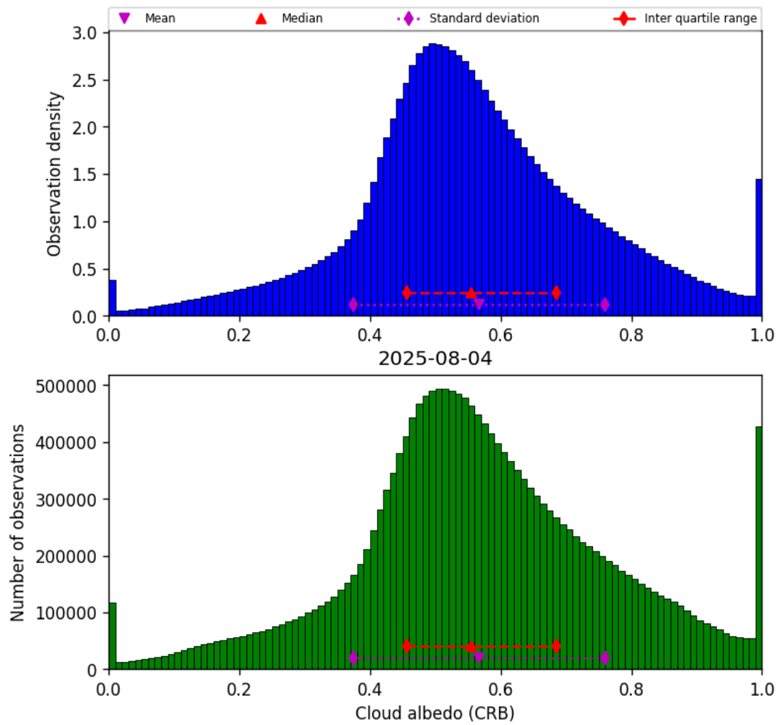
Figure 42: Histogram of “Cloud albedo (CRB)” for 2025-08-04 to 2025-08-05
