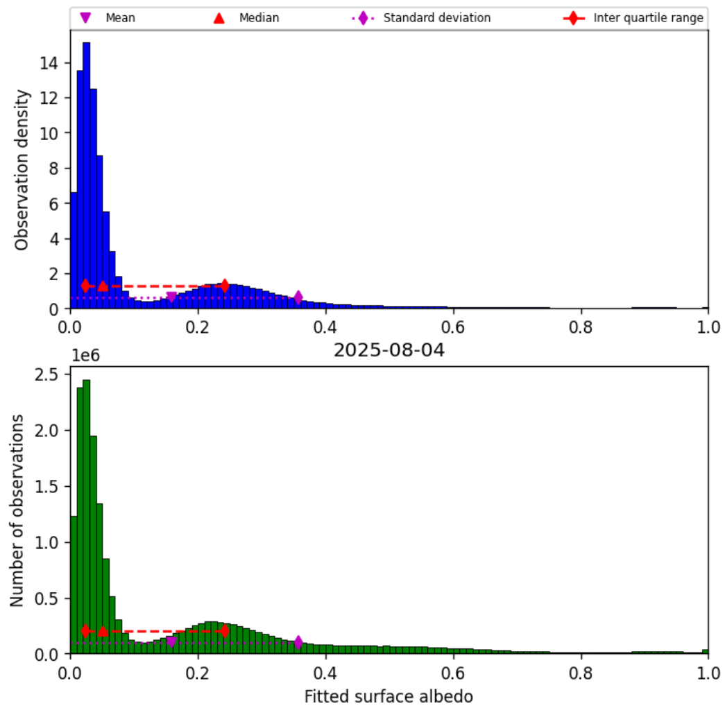
Figure 43: Histogram of “Fitted surface albedo” for 2025-08-04 to 2025-08-05
