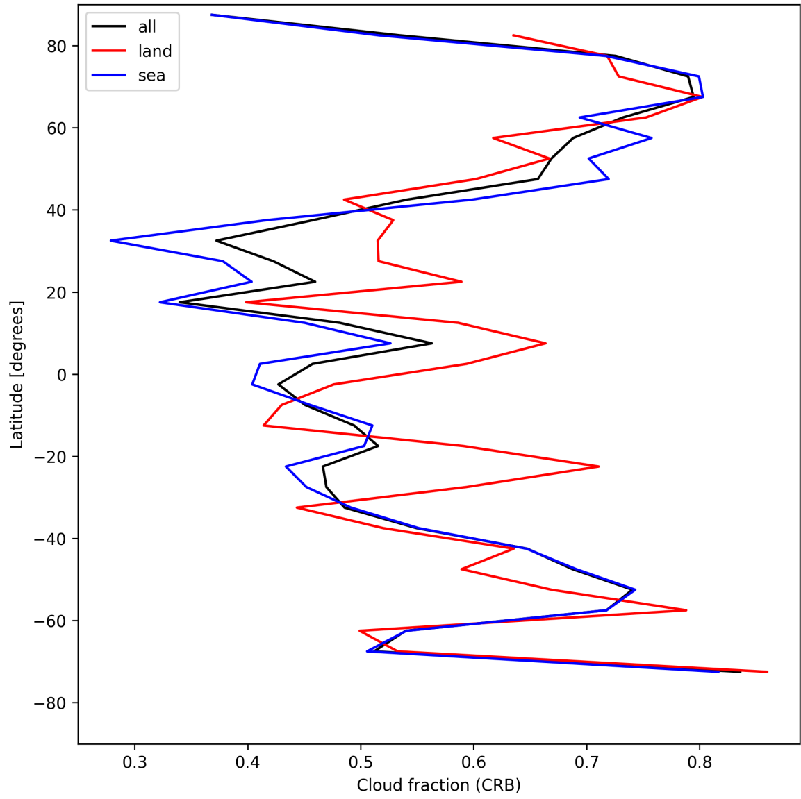
Figure 24: Zonal average of “Cloud fraction (CRB)” for 2025-08-04 to 2025-08-05.
