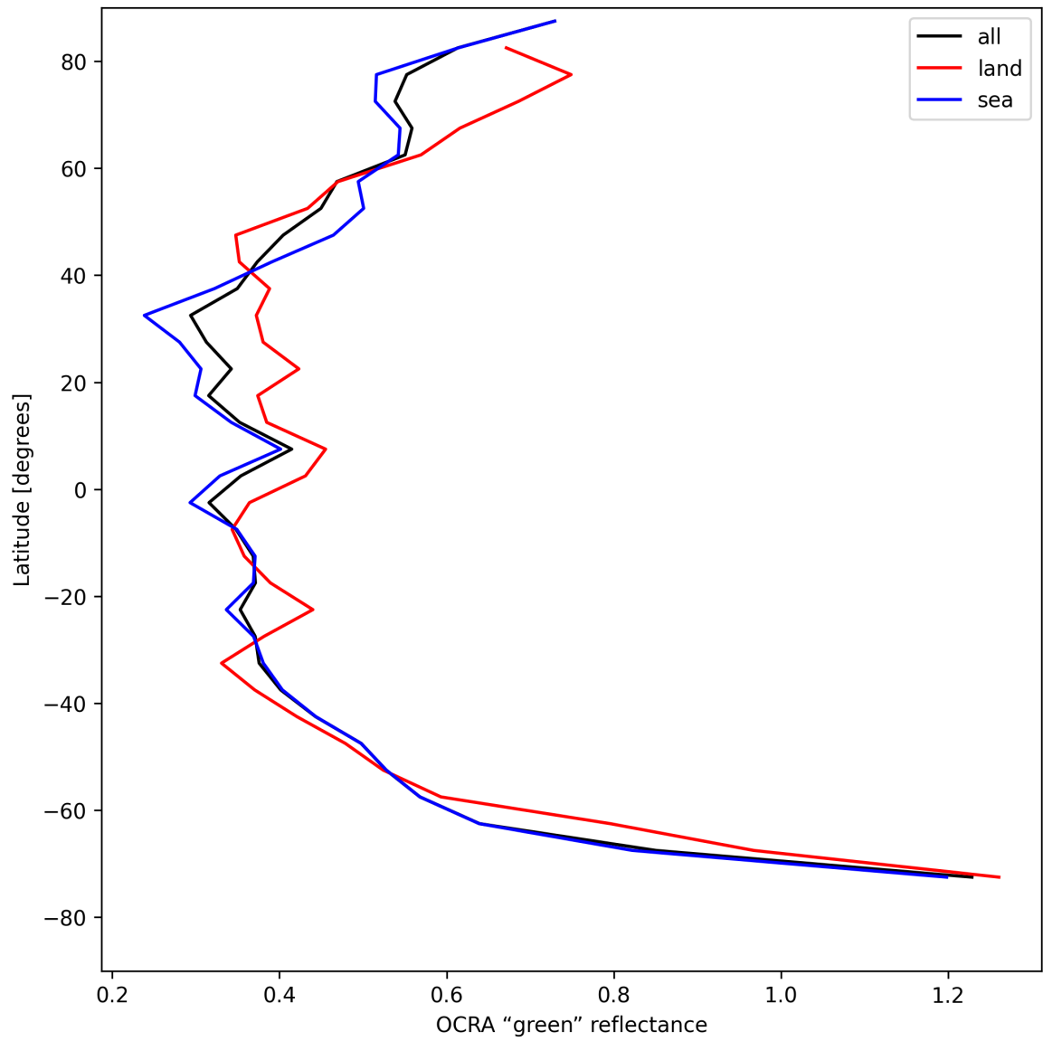
Figure 34: Zonal average of “OCRA “green” reflectance” for 2025-08-05 to 2025-08-06.
