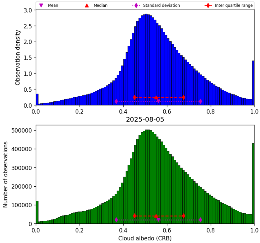
Figure 42: Histogram of “Cloud albedo (CRB)” for 2025-08-05 to 2025-08-06
