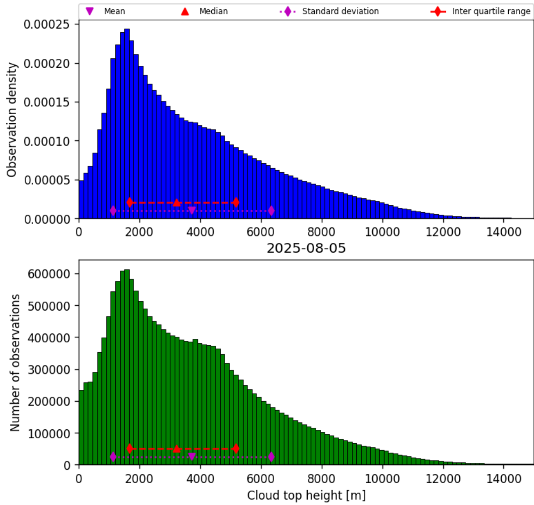
Figure 38: Histogram of “Cloud top height” for 2025-08-05 to 2025-08-06
