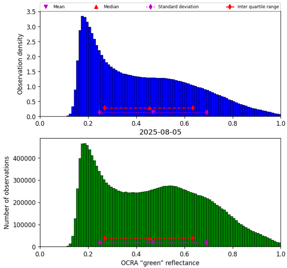
Figure 50: Histogram of “OCRA “green” reflectance” for 2025-08-05 to 2025-08-06
