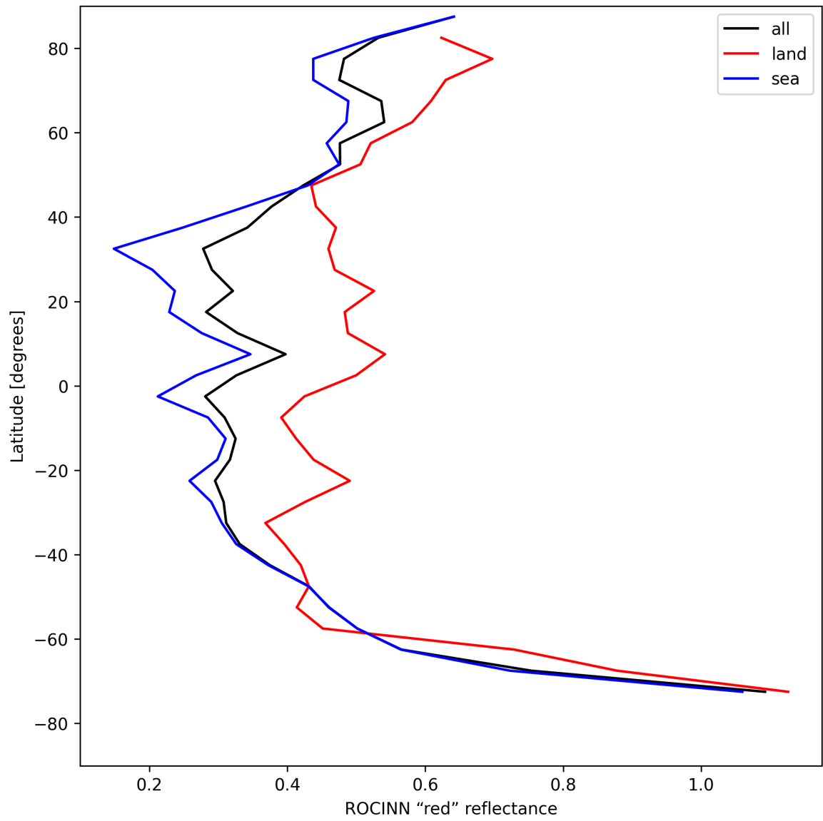
Figure 35: Zonal average of “ROCINN “red” reflectance” for 2025-08-05 to 2025-08-06.
