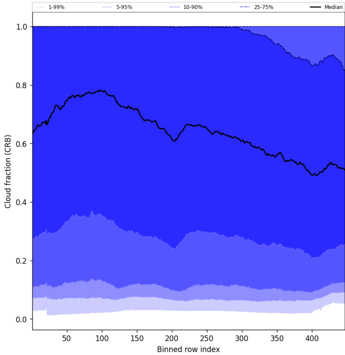
Figure 56: Along track statistics of “Cloud fraction (CRB)” for 2025-08-05 to 2025-08-06
