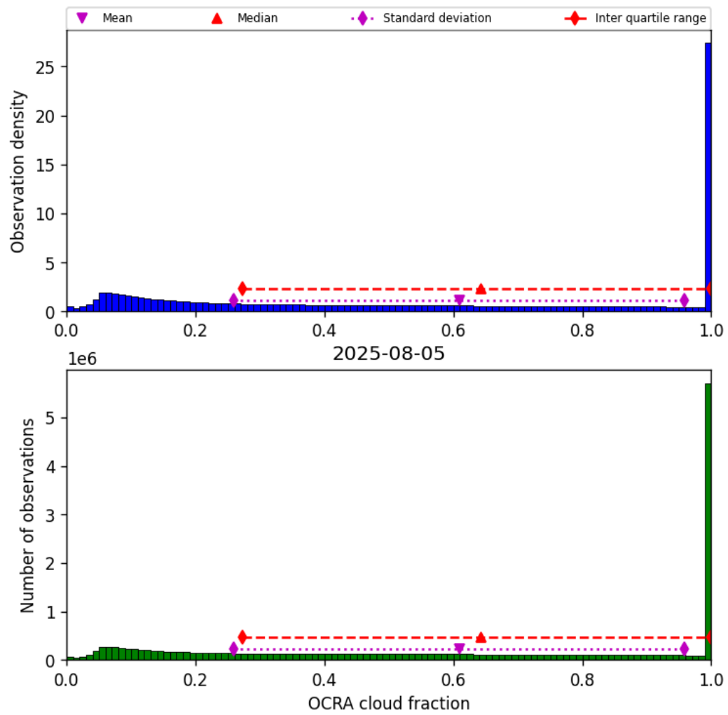
Figure 48: Histogram of “OCRA cloud fraction” for 2025-08-05 to 2025-08-06
