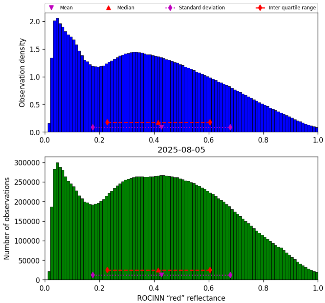
Figure 51: Histogram of "ROCINN "red" reflectance" for 2025-08-05 to 2025-08-06
