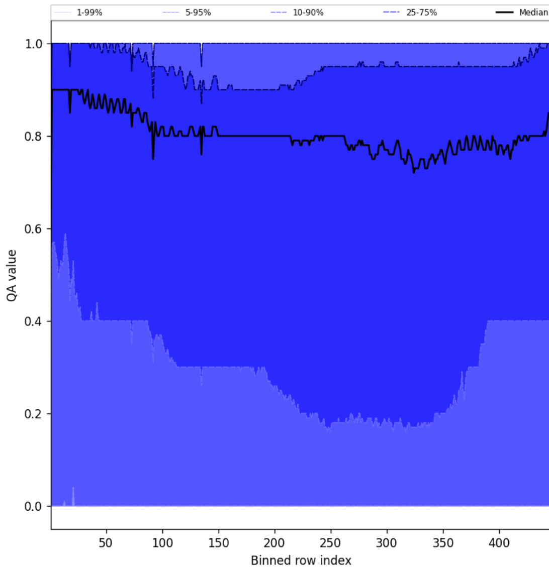
Figure 52: Along track statistics of “QA value” for 2025-08-05 to 2025-08-06
