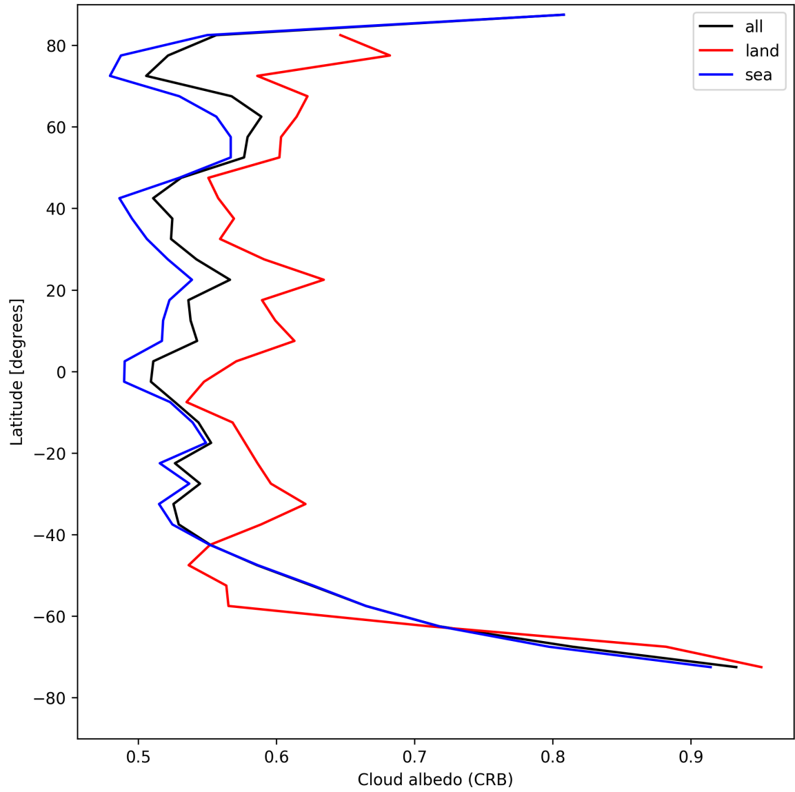
Figure 26: Zonal average of “Cloud albedo (CRB)” for 2025-08-05 to 2025-08-06.
