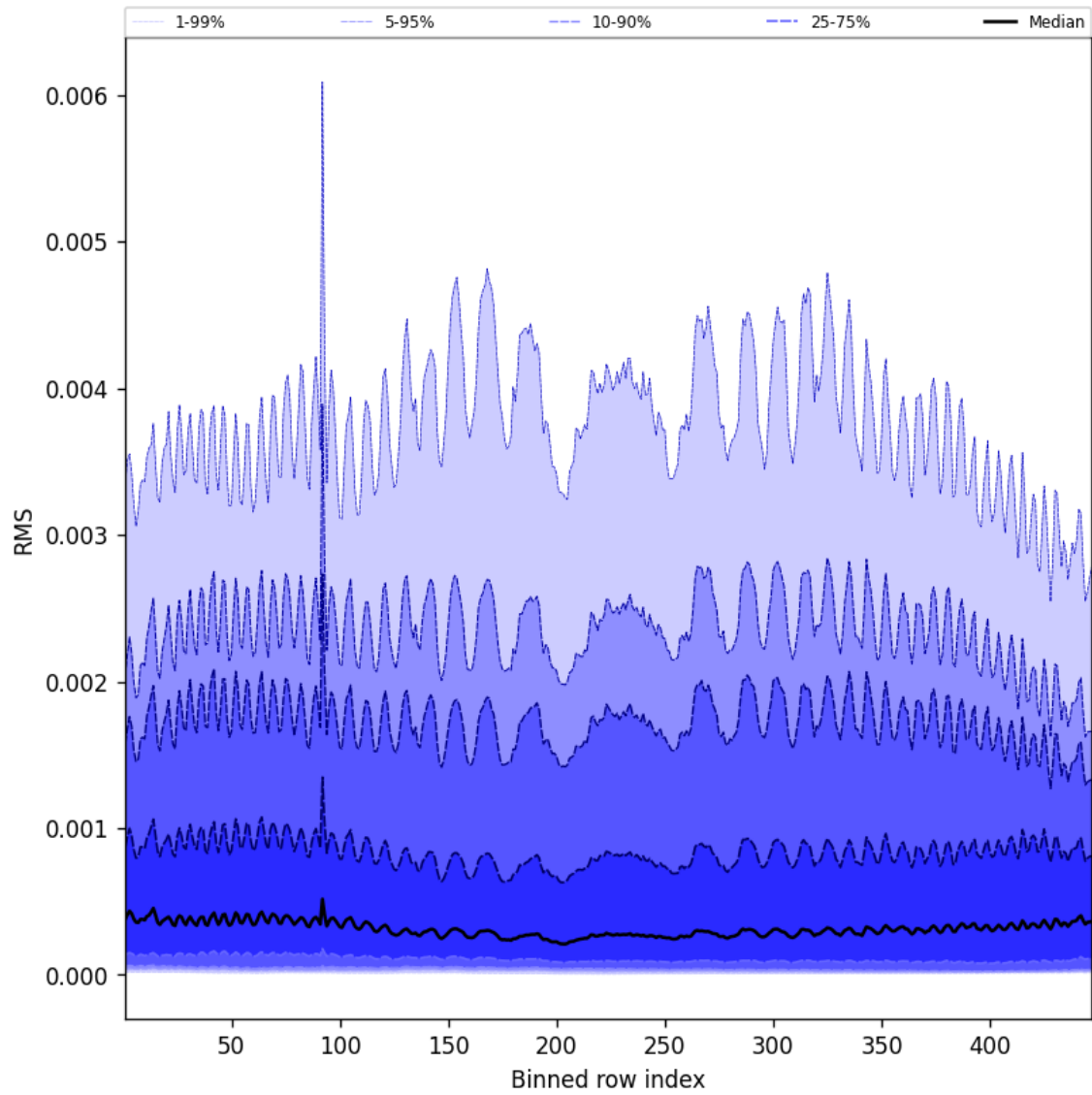
Figure 61: Along track statistics of “RMS” for 2025-08-05 to 2025-08-06
