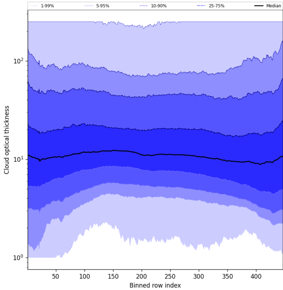
Figure 55: Along track statistics of “Cloud optical thickness” for 2025-08-05 to 2025-08-06
