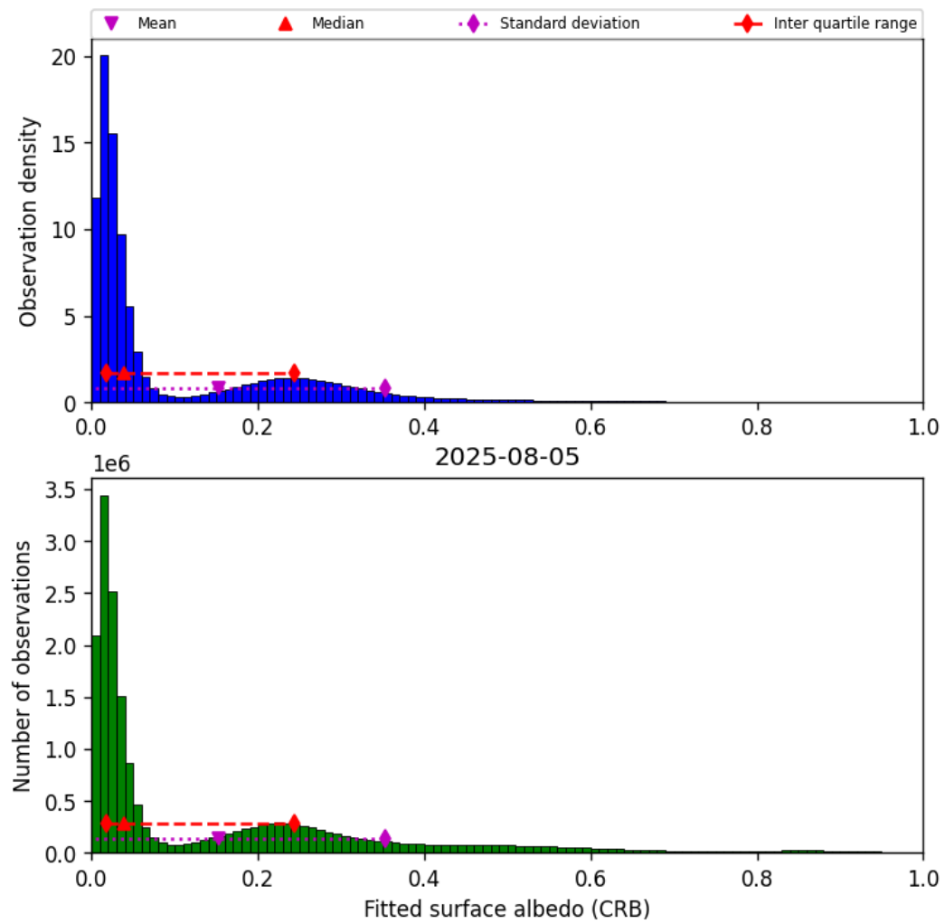
Figure 44: Histogram of “Fitted surface albedo (CRB)” for 2025-08-05 to 2025-08-06
