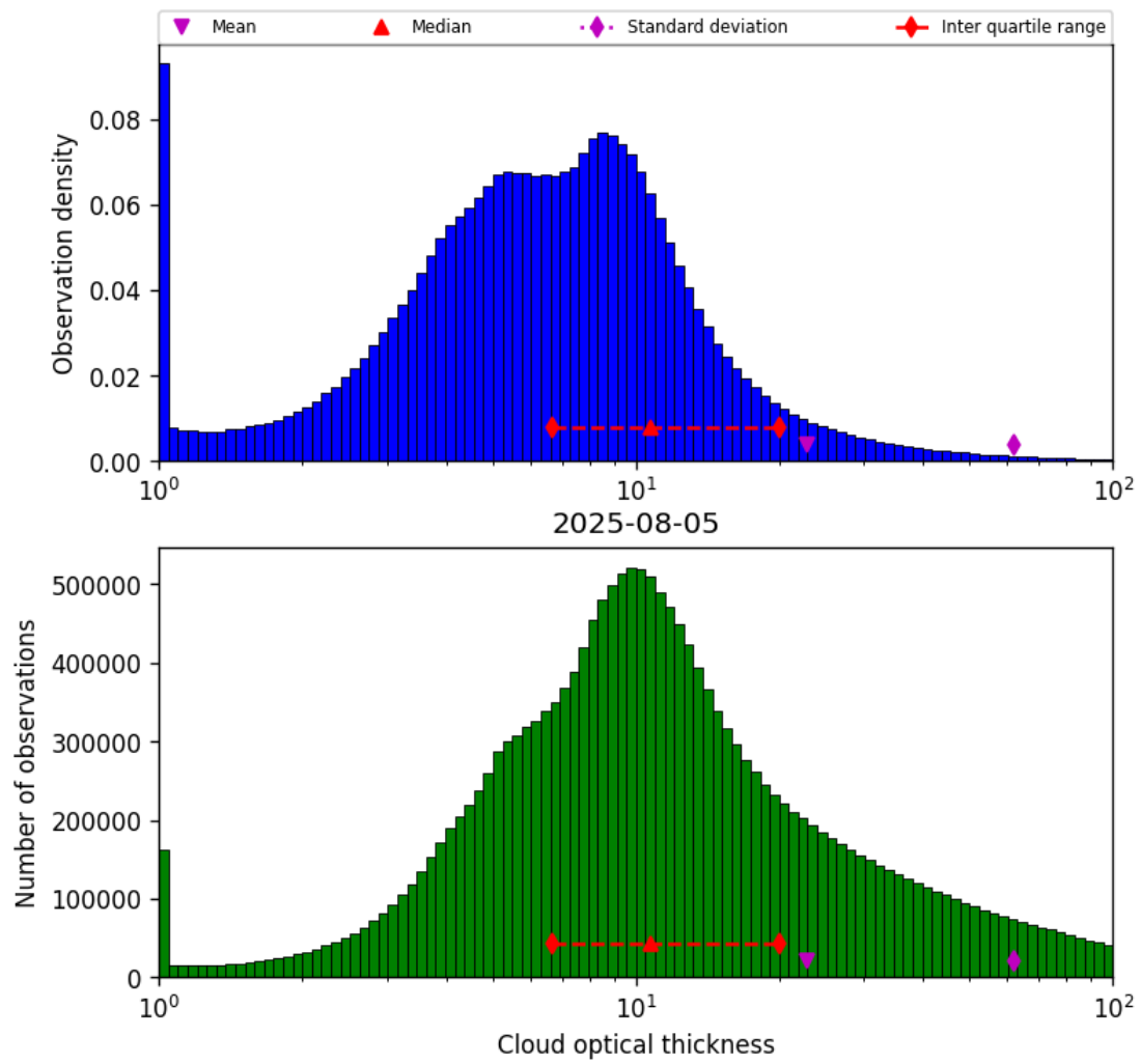
Figure 39: Histogram of “Cloud optical thickness” for 2025-08-05 to 2025-08-06
