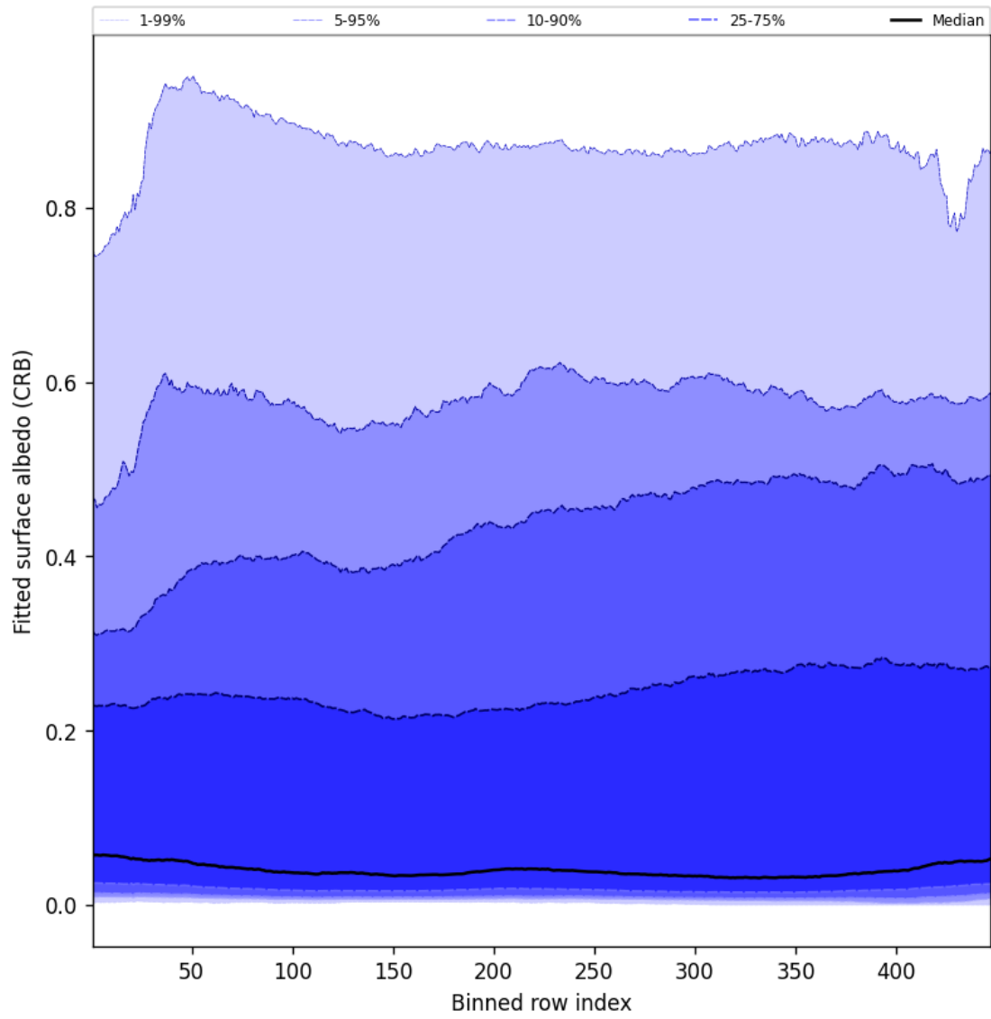
Figure 60: Along track statistics of “Fitted surface albedo (CRB)” for 2025-08-05 to 2025-08-06
