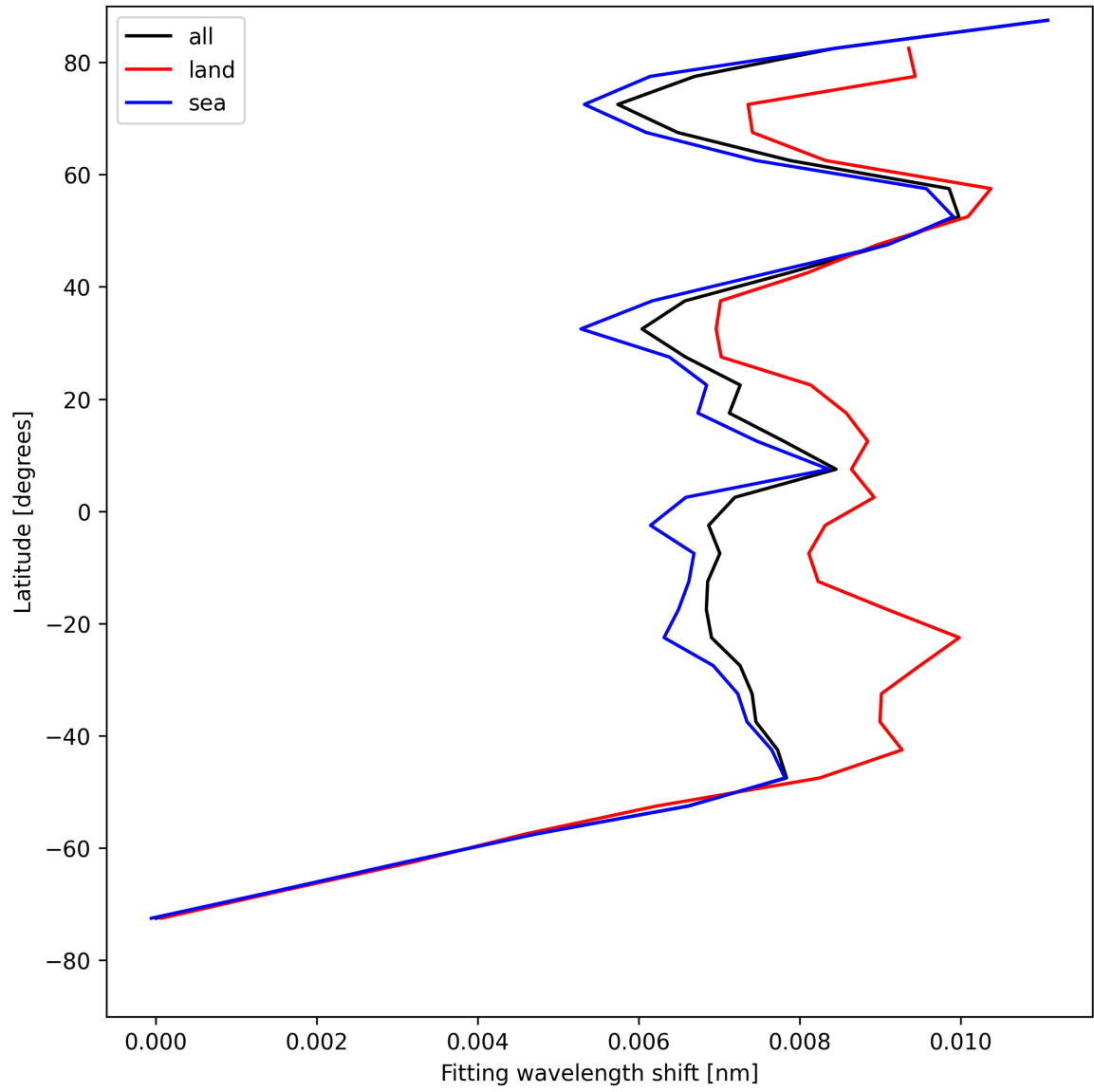
Figure 31: Zonal average of “Fitting wavelength shift” for 2025-08-05 to 2025-08-06.
