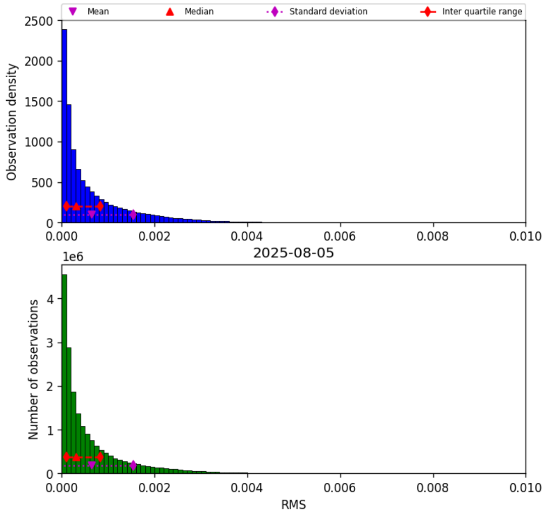
Figure 45: Histogram of “RMS” for 2025-08-05 to 2025-08-06
