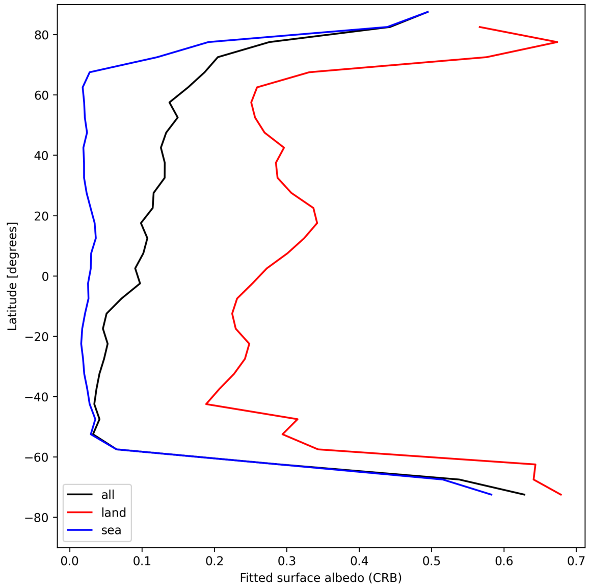
Figure 28: Zonal average of “Fitted surface albedo (CRB)” for 2025-08-05 to 2025-08-06.
