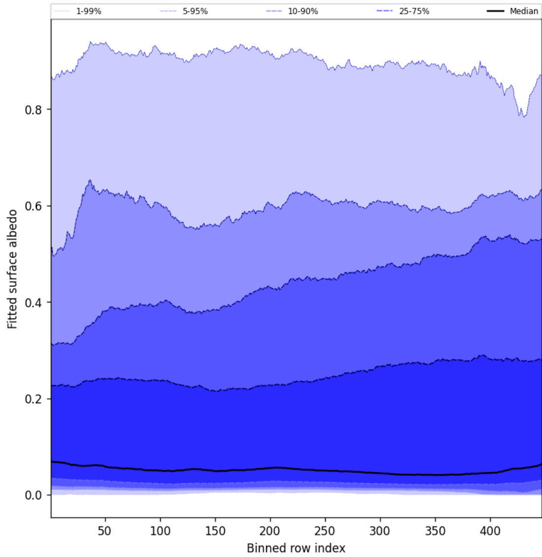
Figure 59: Along track statistics of “Fitted surface albedo” for 2025-08-05 to 2025-08-06
