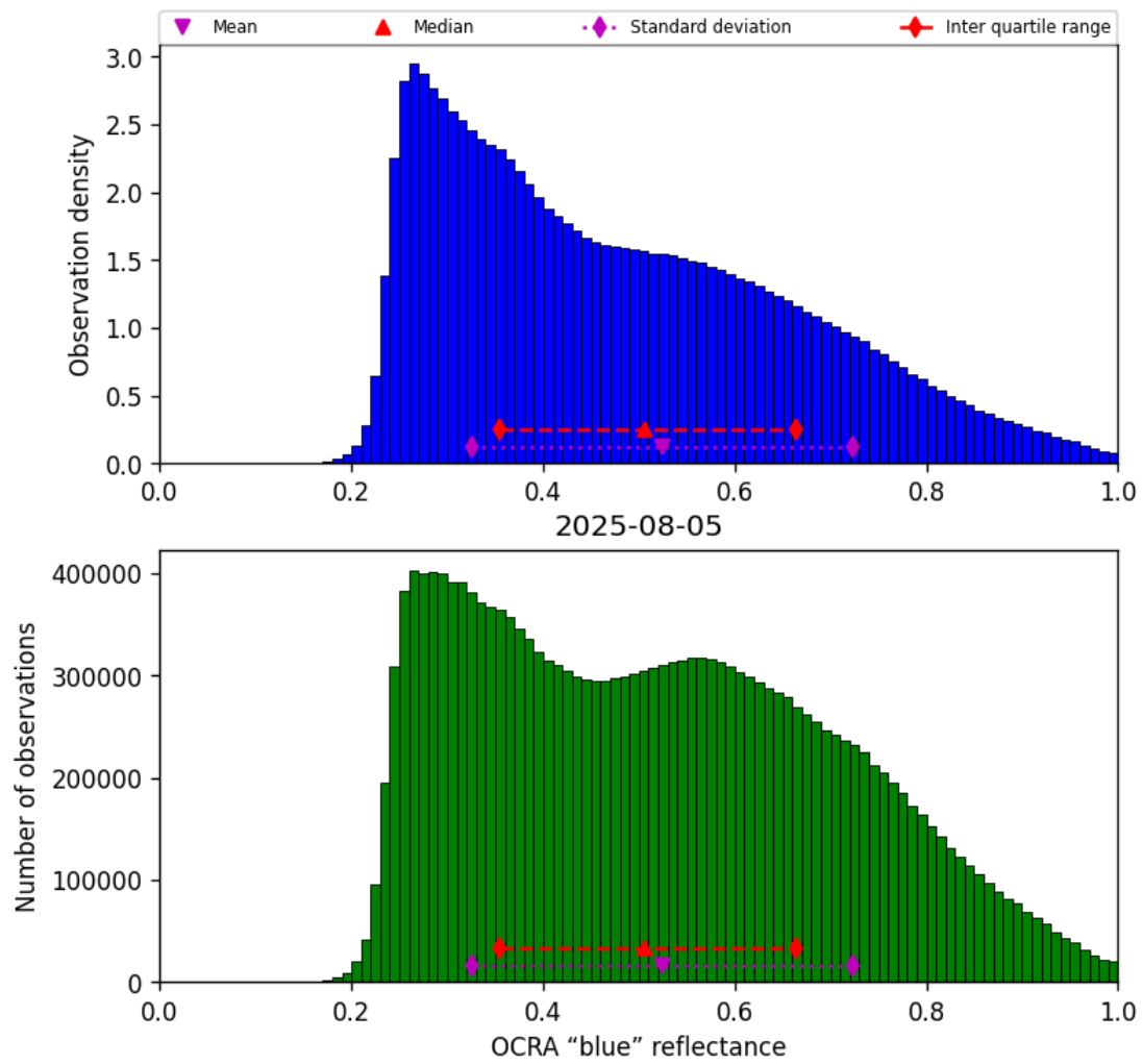
Figure 49: Histogram of “OCRA “blue” reflectance” for 2025-08-05 to 2025-08-06
