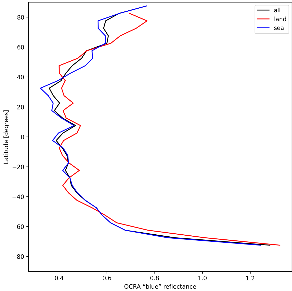
Figure 33: Zonal average of “OCRA “blue” reflectance” for 2025-08-05 to 2025-08-06.
