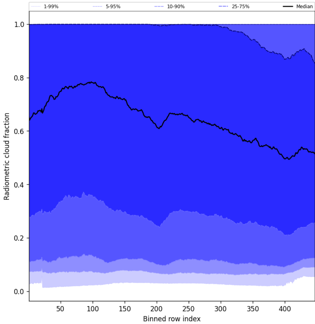
Figure 53: Along track statistics of “Radiometric cloud fraction” for 2025-08-05 to 2025-08-06
