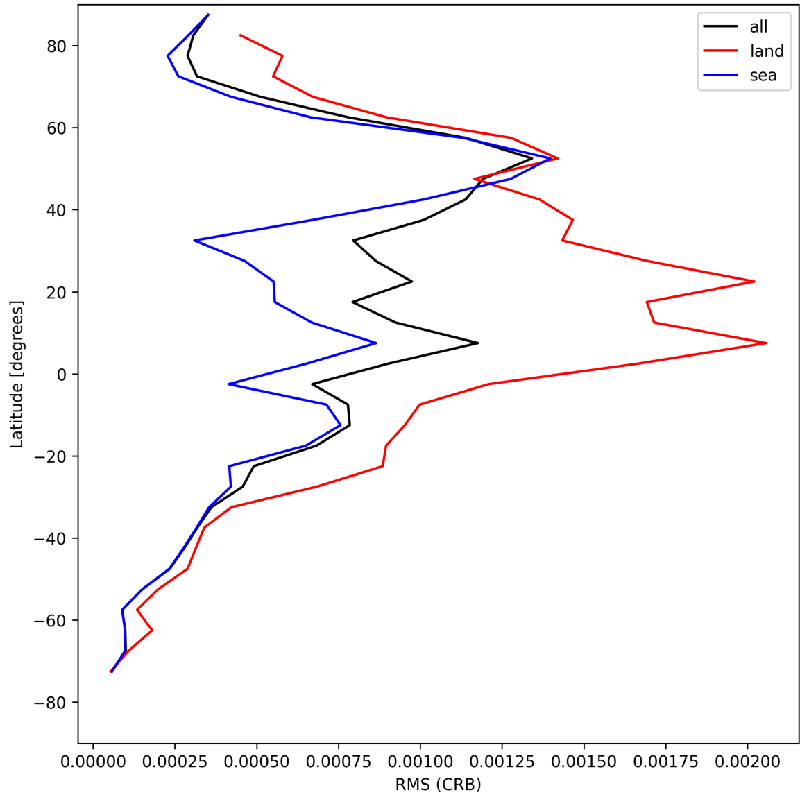
Figure 30: Zonal average of “RMS (CRB)” for 2025-08-05 to 2025-08-06.
