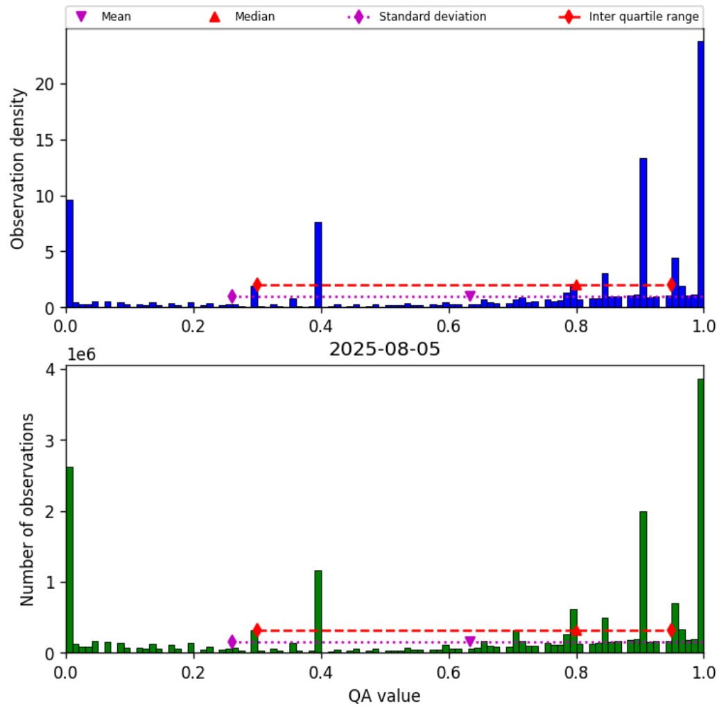
Figure 36: Histogram of “QA value” for 2025-08-05 to 2025-08-06
