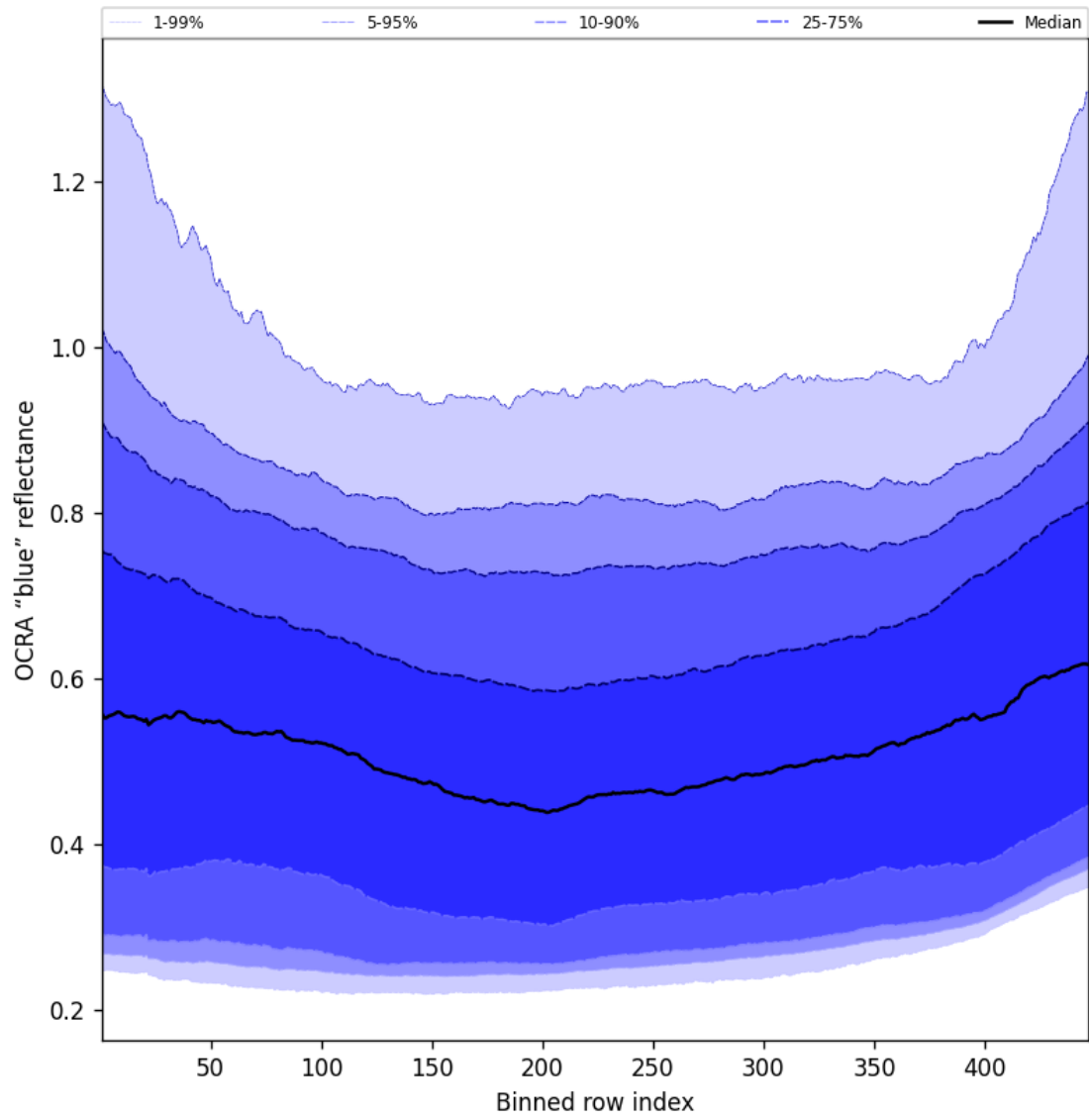
Figure 65: Along track statistics of “OCRA “blue” reflectance” for 2025-08-05 to 2025-08-06
