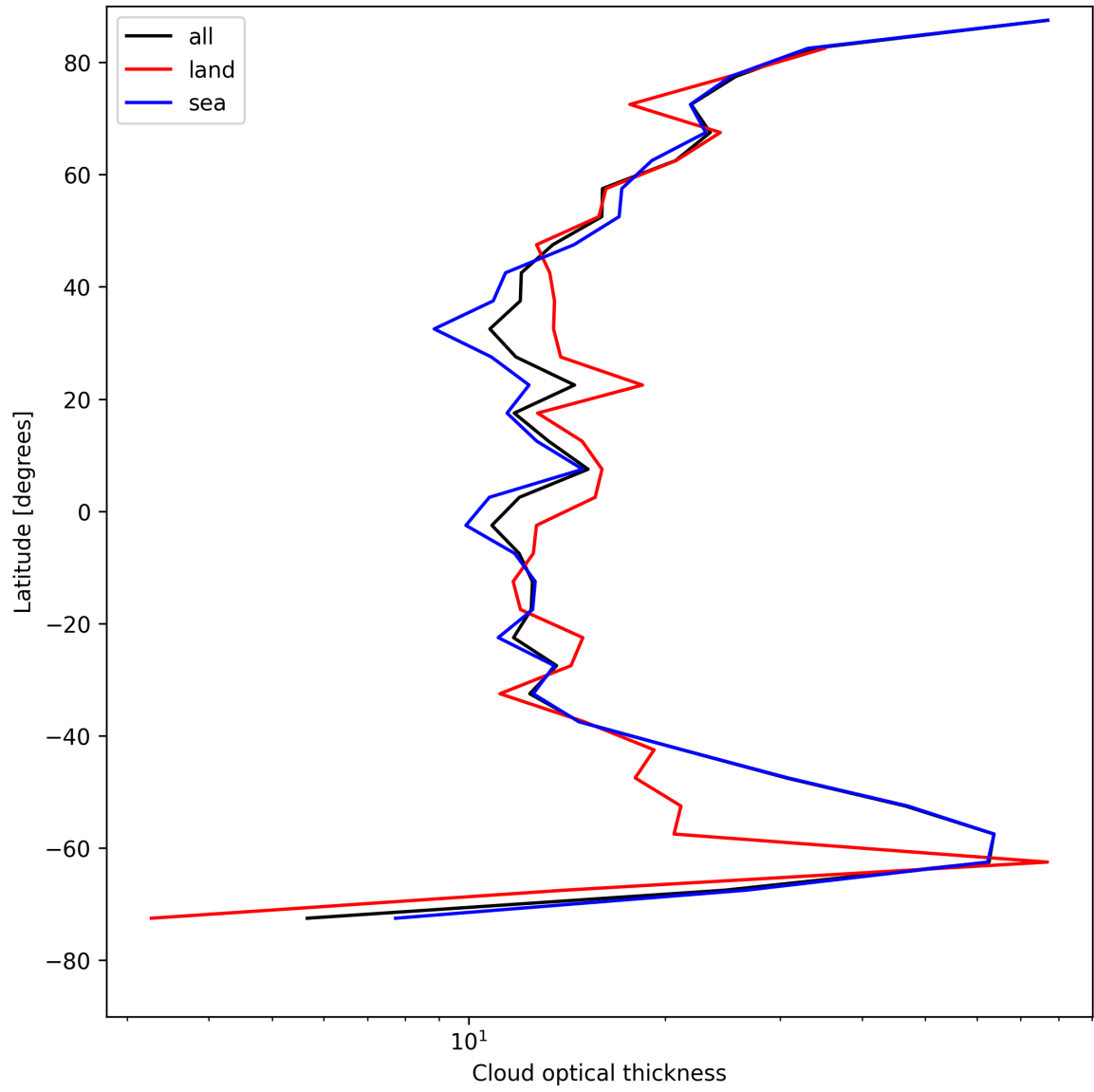
Figure 23: Zonal average of “Cloud optical thickness” for 2025-08-05 to 2025-08-06.
