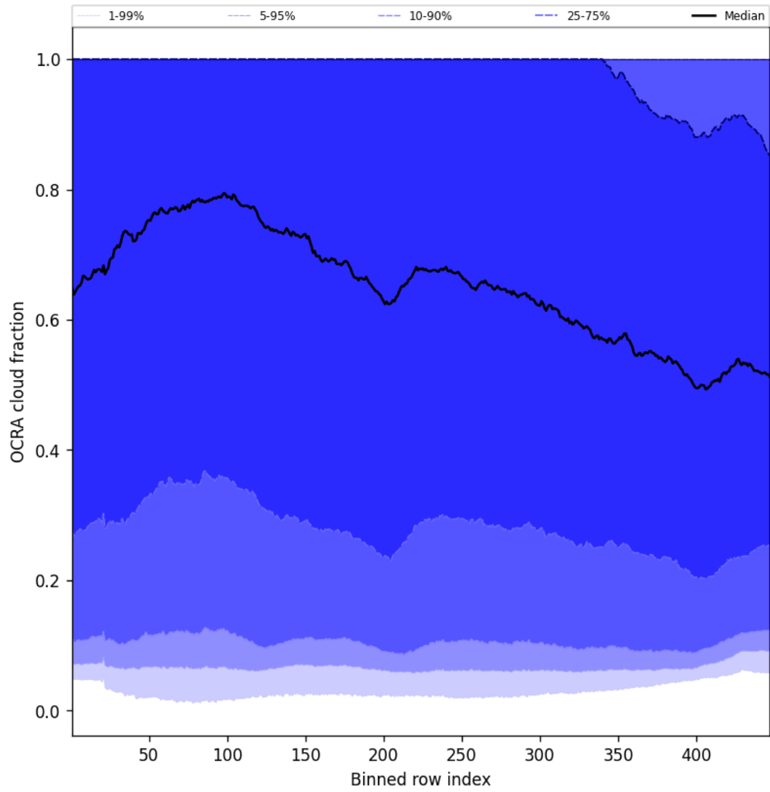
Figure 64: Along track statistics of “OCRA cloud fraction” for 2025-08-05 to 2025-08-06
