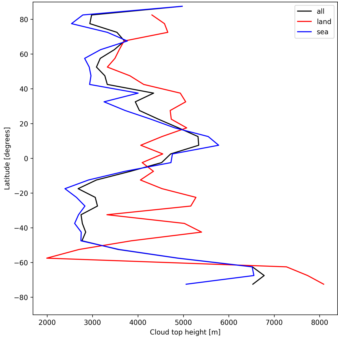
Figure 22: Zonal average of “Cloud top height” for 2025-08-05 to 2025-08-06.
