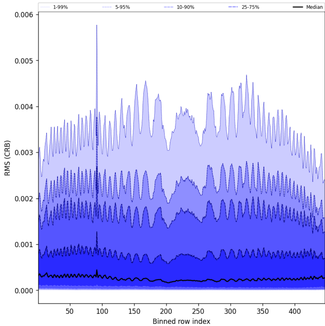
Figure 62: Along track statistics of “RMS (CRB)” for 2025-08-05 to 2025-08-06
