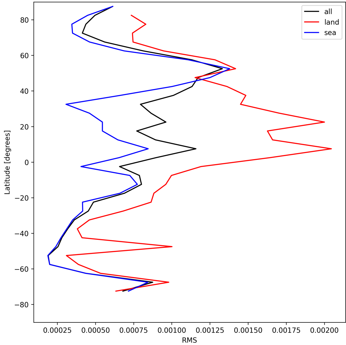
Figure 29: Zonal average of “RMS” for 2025-08-05 to 2025-08-06.
