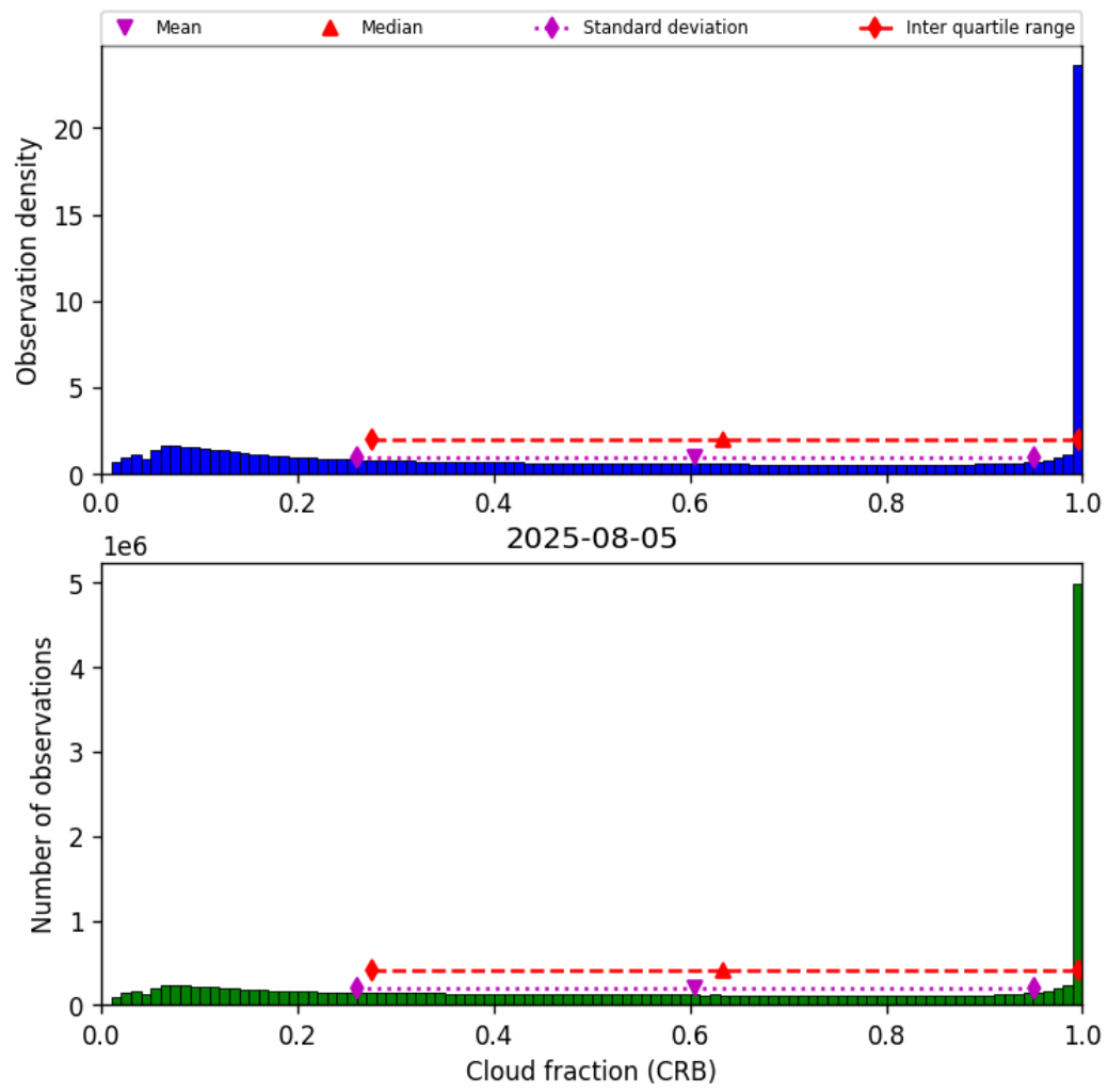
Figure 40: Histogram of “Cloud fraction (CRB)” for 2025-08-05 to 2025-08-06
