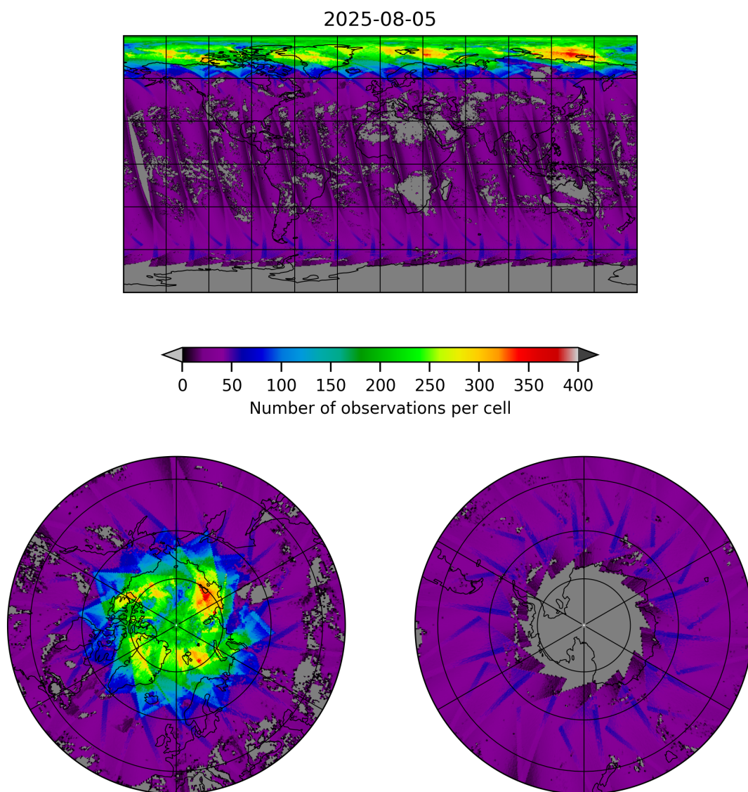
Figure 19: Map of the number of observations for 2025-08-05 to 2025-08-06
