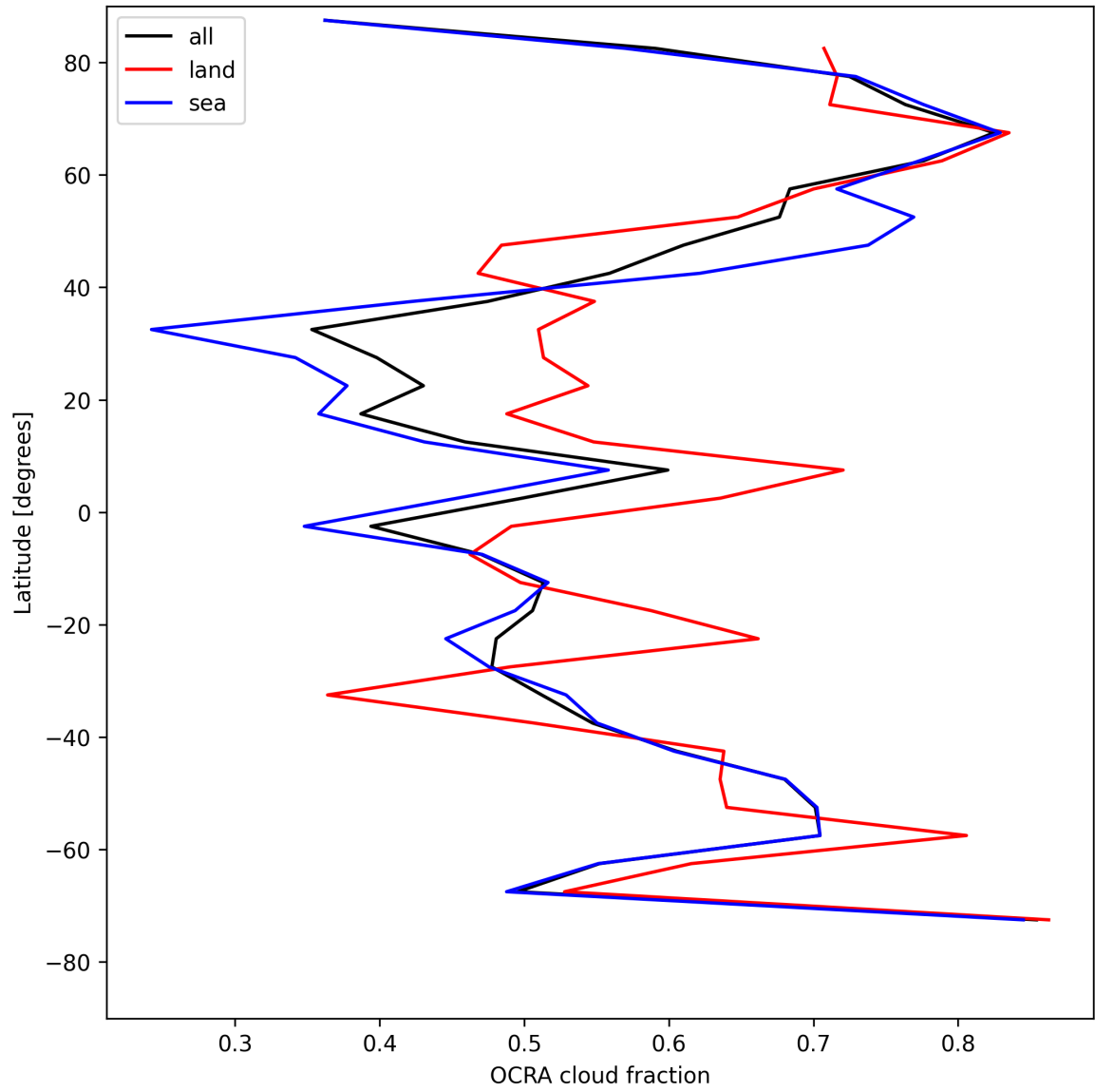
Figure 32: Zonal average of “OCRA cloud fraction” for 2025-08-05 to 2025-08-06.
