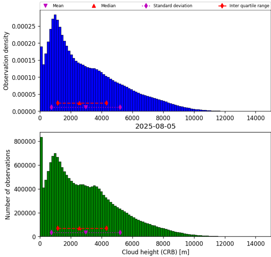
Figure 41: Histogram of “Cloud height (CRB)” for 2025-08-05 to 2025-08-06
