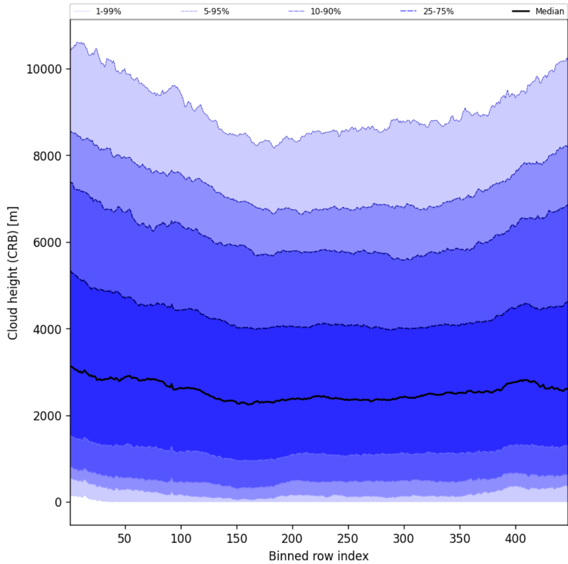
Figure 57: Along track statistics of “Cloud height (CRB)” for 2025-08-05 to 2025-08-06
