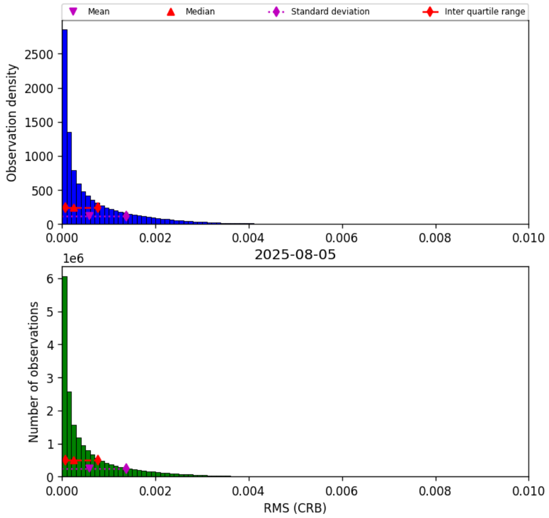
Figure 46: Histogram of “RMS (CRB)” for 2025-08-05 to 2025-08-06
