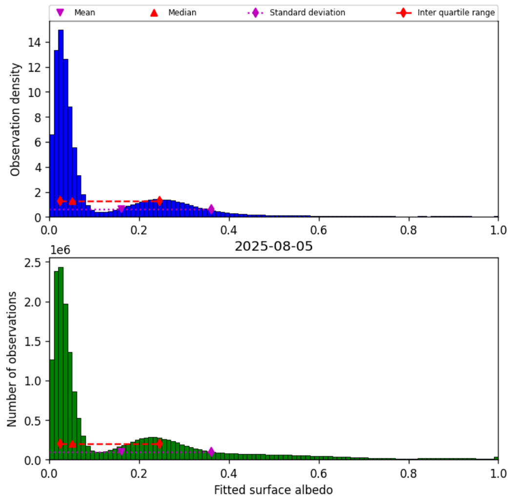
Figure 43: Histogram of “Fitted surface albedo” for 2025-08-05 to 2025-08-06
