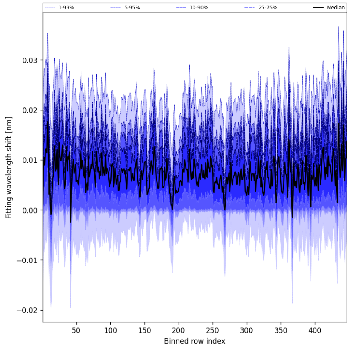
Figure 63: Along track statistics of “Fitting wavelength shift” for 2025-08-05 to 2025-08-06
