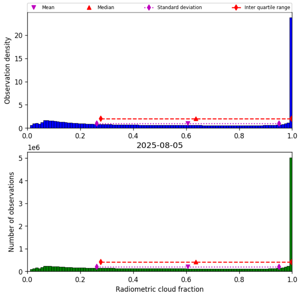
Figure 37: Histogram of “Radiometric cloud fraction” for 2025-08-05 to 2025-08-06
