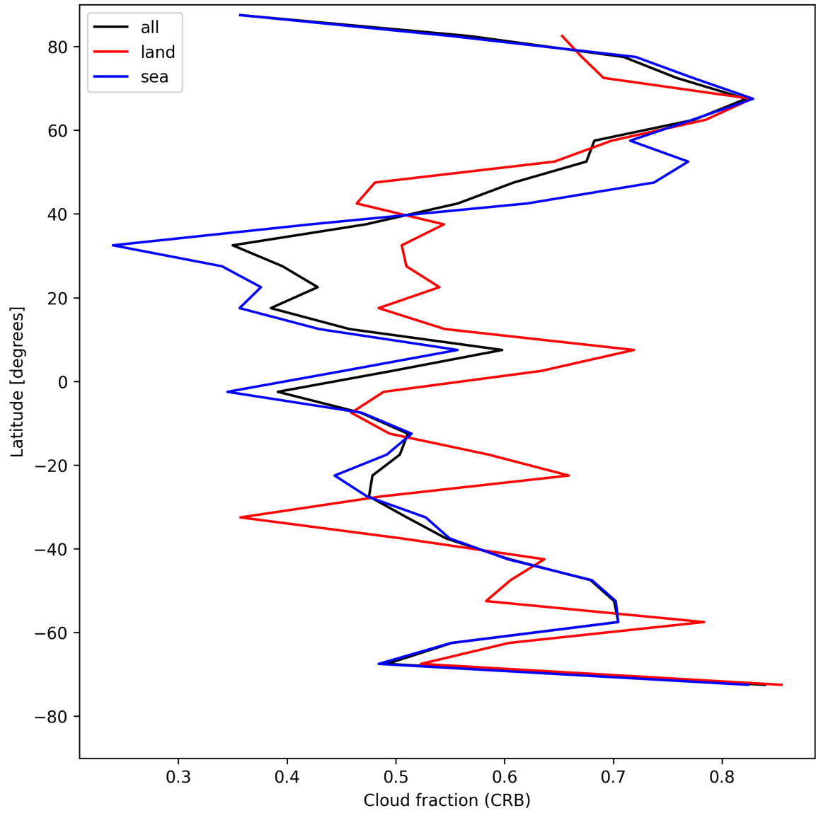
Figure 24: Zonal average of “Cloud fraction (CRB)” for 2025-08-05 to 2025-08-06.
