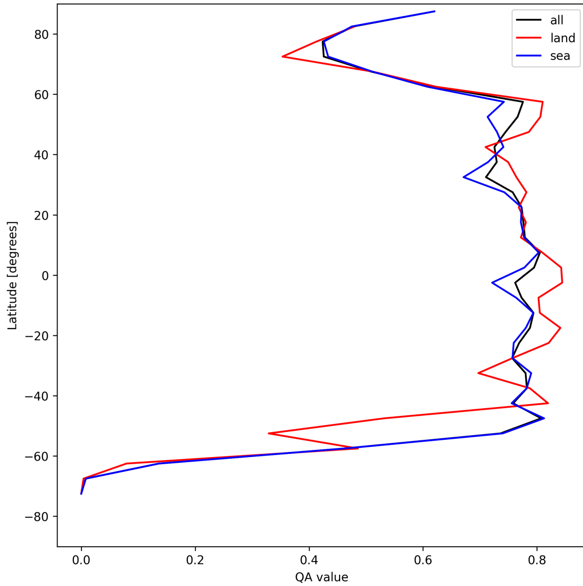
Figure 20: Zonal average of “QA value” for 2025-08-05 to 2025-08-06.
