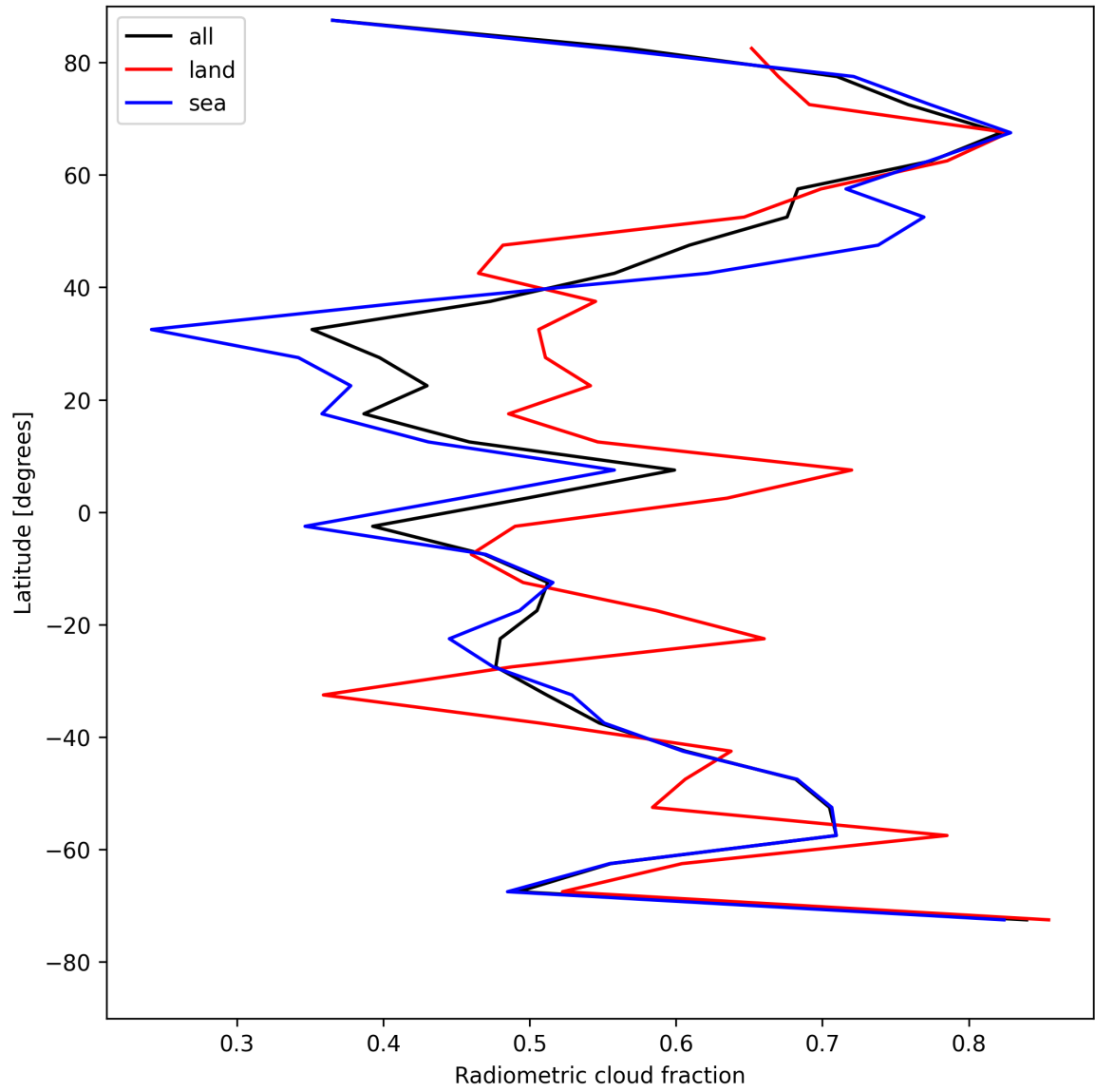
Figure 21: Zonal average of “Radiometric cloud fraction” for 2025-08-05 to 2025-08-06.
