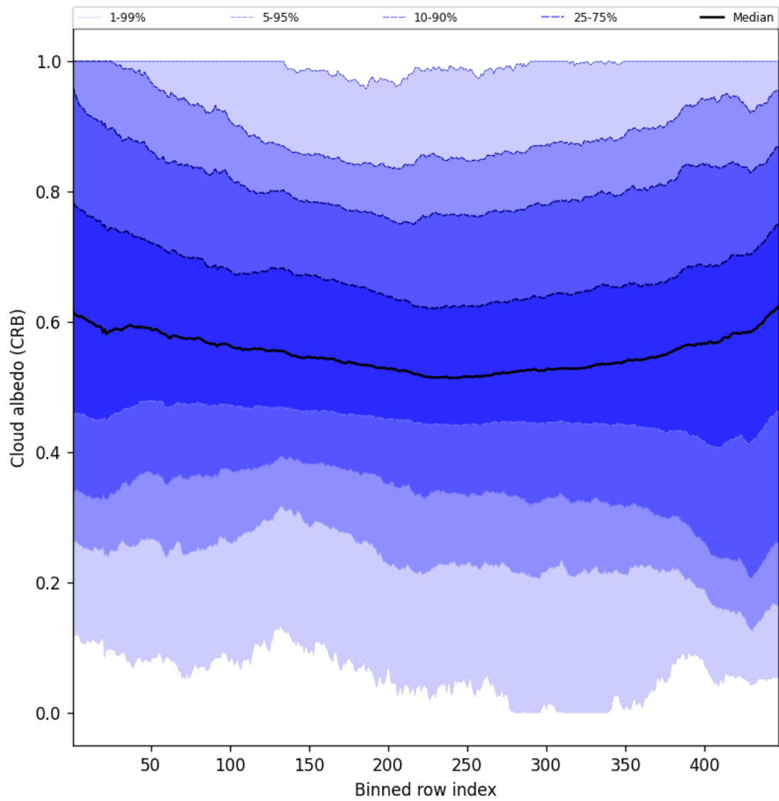
Figure 58: Along track statistics of “Cloud albedo (CRB)” for 2025-08-05 to 2025-08-06
