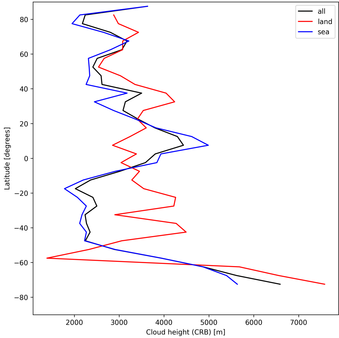
Figure 25: Zonal average of “Cloud height (CRB)” for 2025-08-05 to 2025-08-06.
