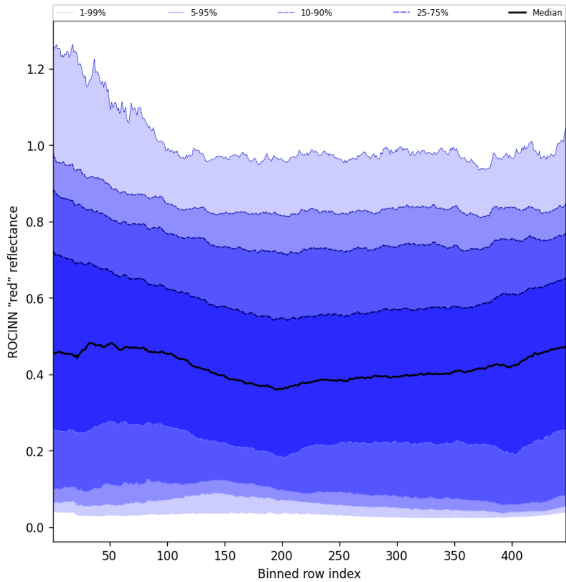
Figure 67: Along track statistics of "ROCINN "red" reflectance" for 2025-08-05 to 2025-08-06
