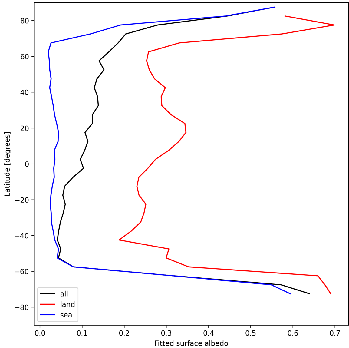
Figure 27: Zonal average of “Fitted surface albedo” for 2025-08-05 to 2025-08-06.
