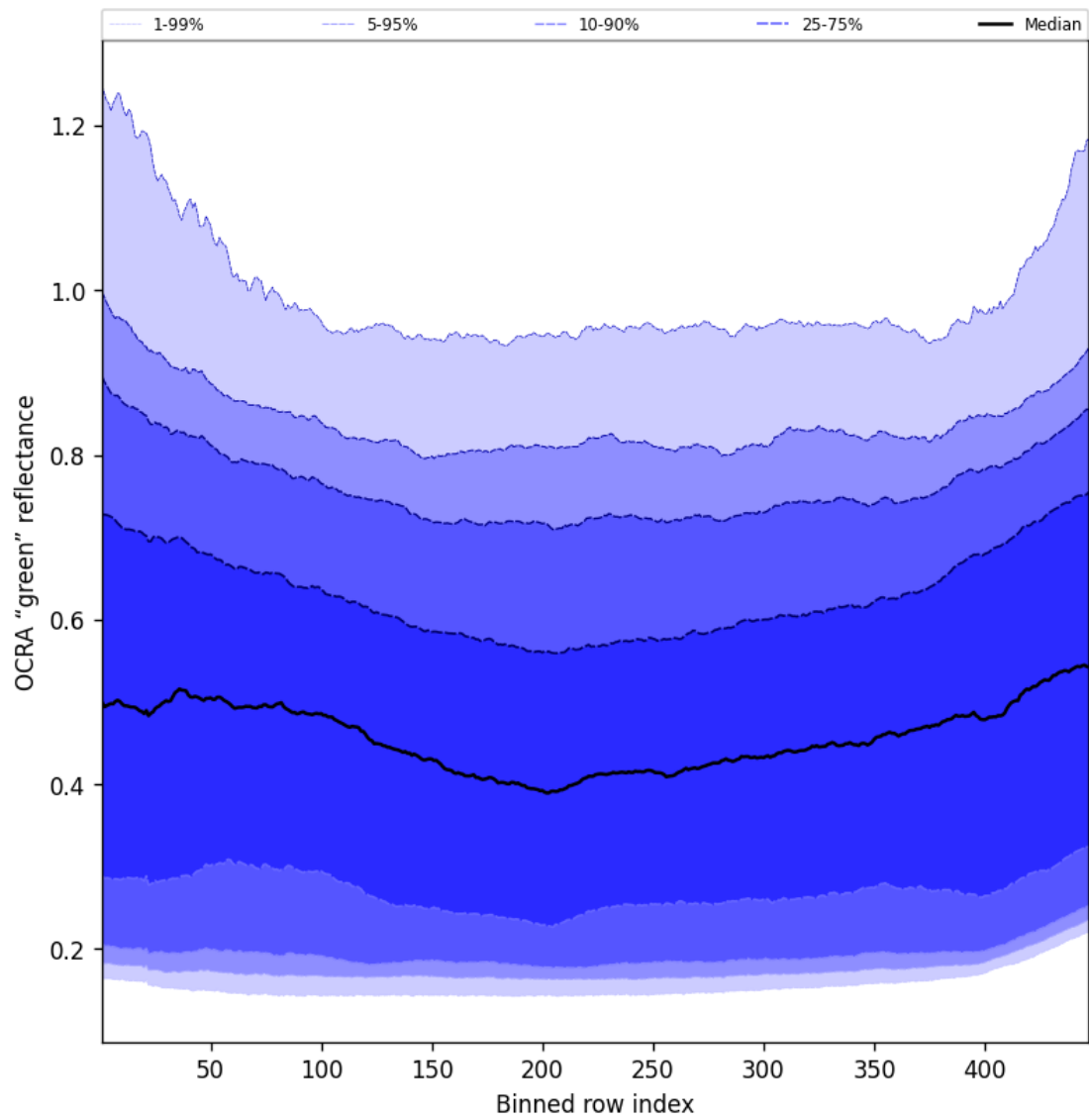
Figure 66: Along track statistics of “OCRA “green” reflectance” for 2025-08-05 to 2025-08-06
