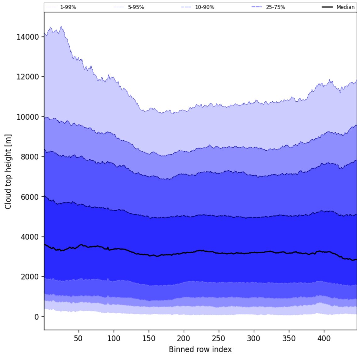
Figure 54: Along track statistics of “Cloud top height” for 2025-08-05 to 2025-08-06
