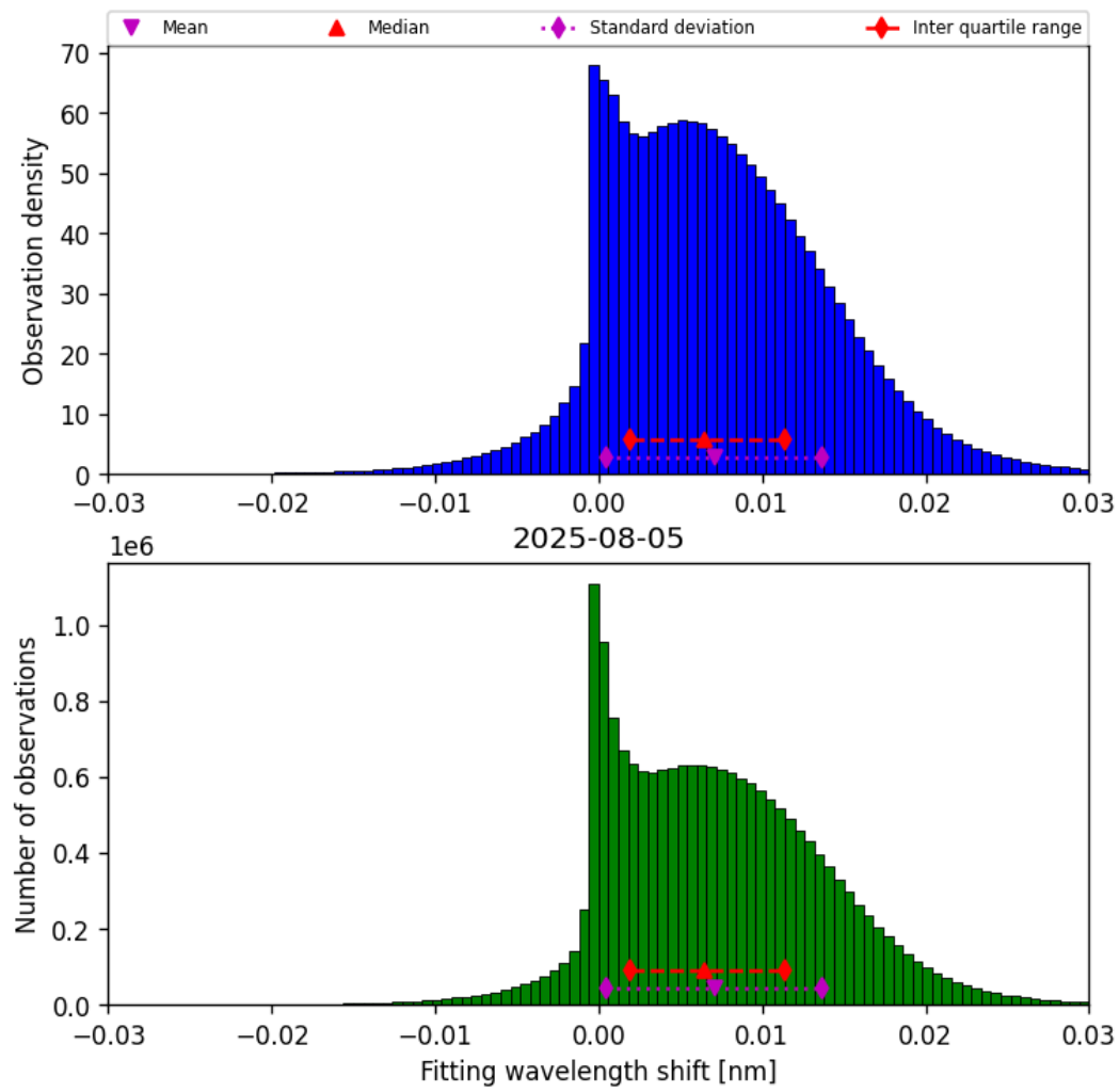
Figure 47: Histogram of “Fitting wavelength shift” for 2025-08-05 to 2025-08-06
