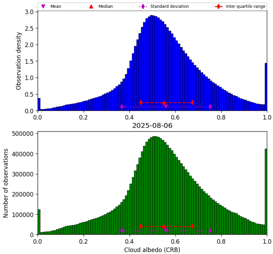
Figure 42: Histogram of “Cloud albedo (CRB)” for 2025-08-06 to 2025-08-07
