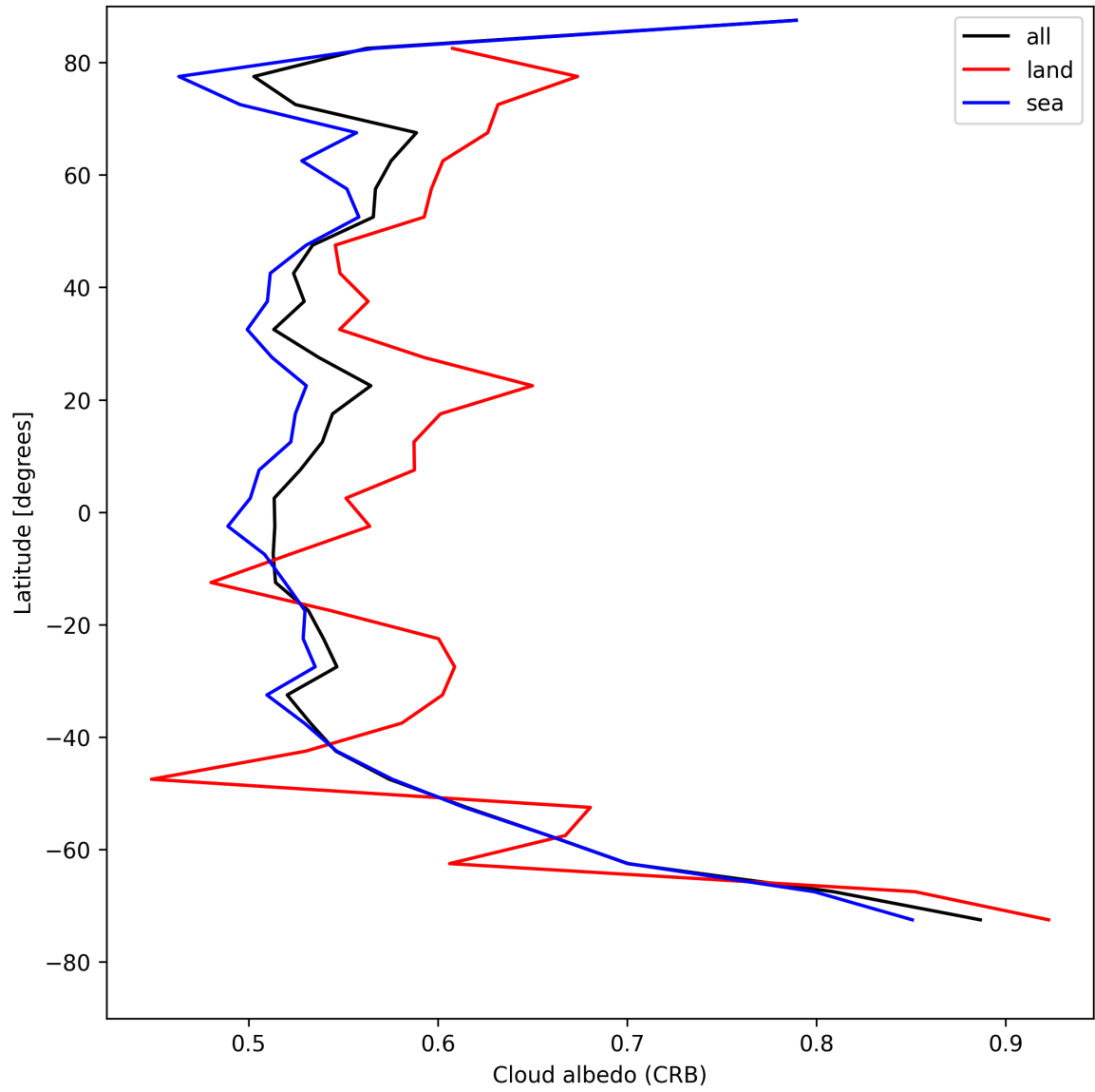
Figure 26: Zonal average of “Cloud albedo (CRB)” for 2025-08-06 to 2025-08-07.
