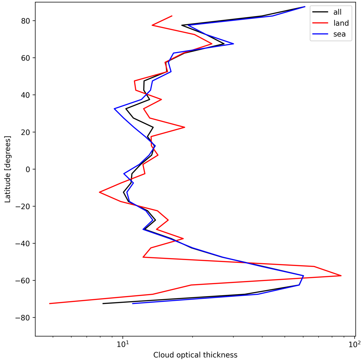
Figure 23: Zonal average of “Cloud optical thickness” for 2025-08-06 to 2025-08-07.
