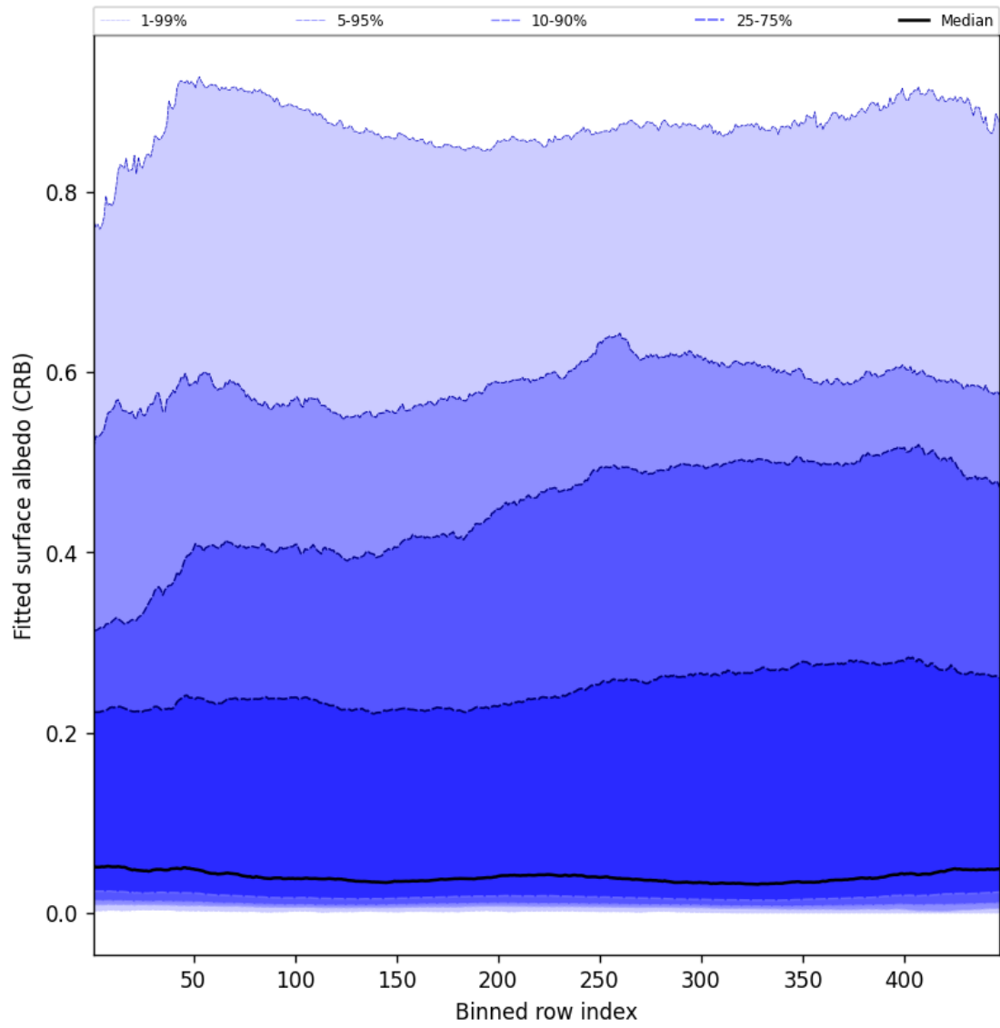
Figure 60: Along track statistics of “Fitted surface albedo (CRB)” for 2025-08-06 to 2025-08-07
