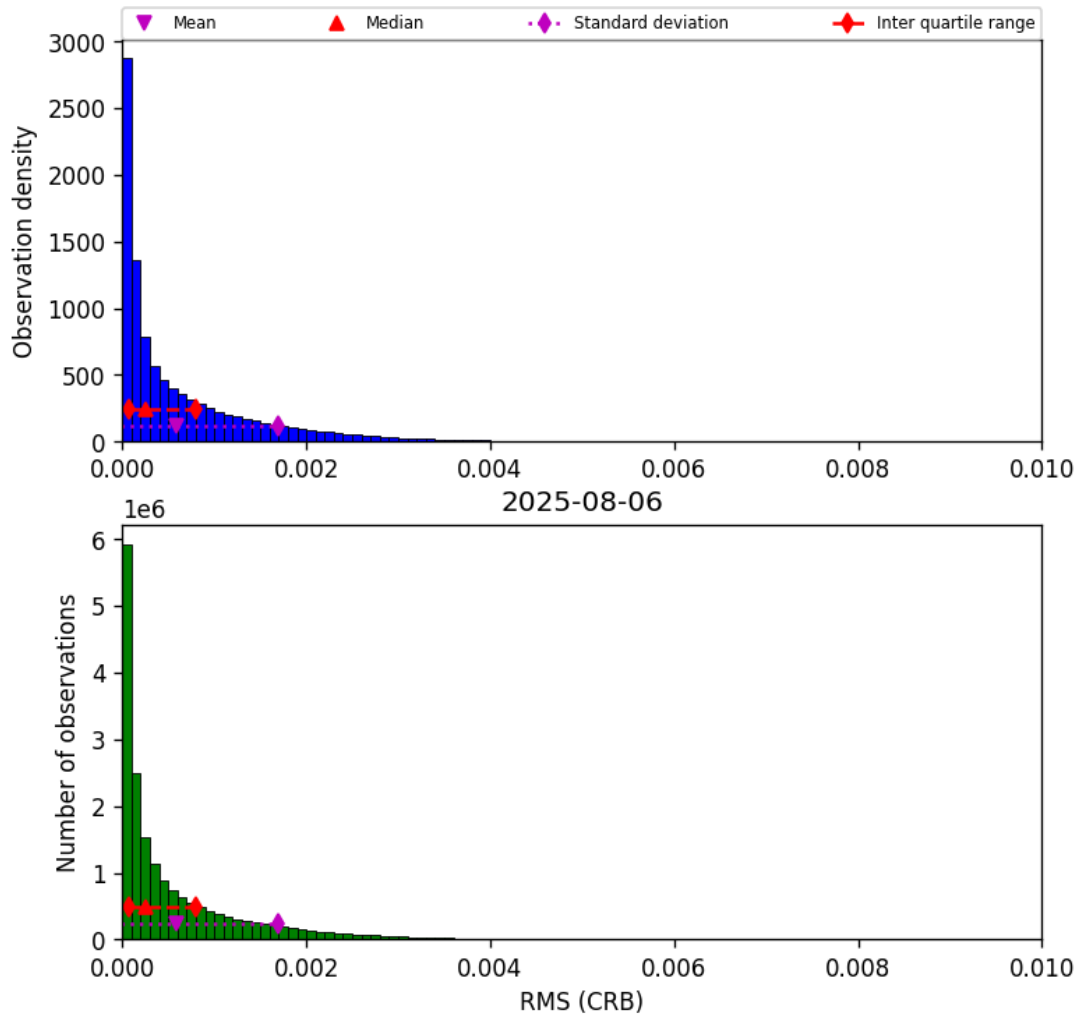
Figure 46: Histogram of “RMS (CRB)” for 2025-08-06 to 2025-08-07
