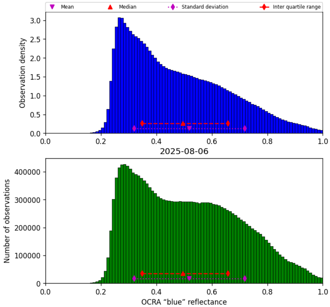
Figure 49: Histogram of “OCRA “blue” reflectance” for 2025-08-06 to 2025-08-07
