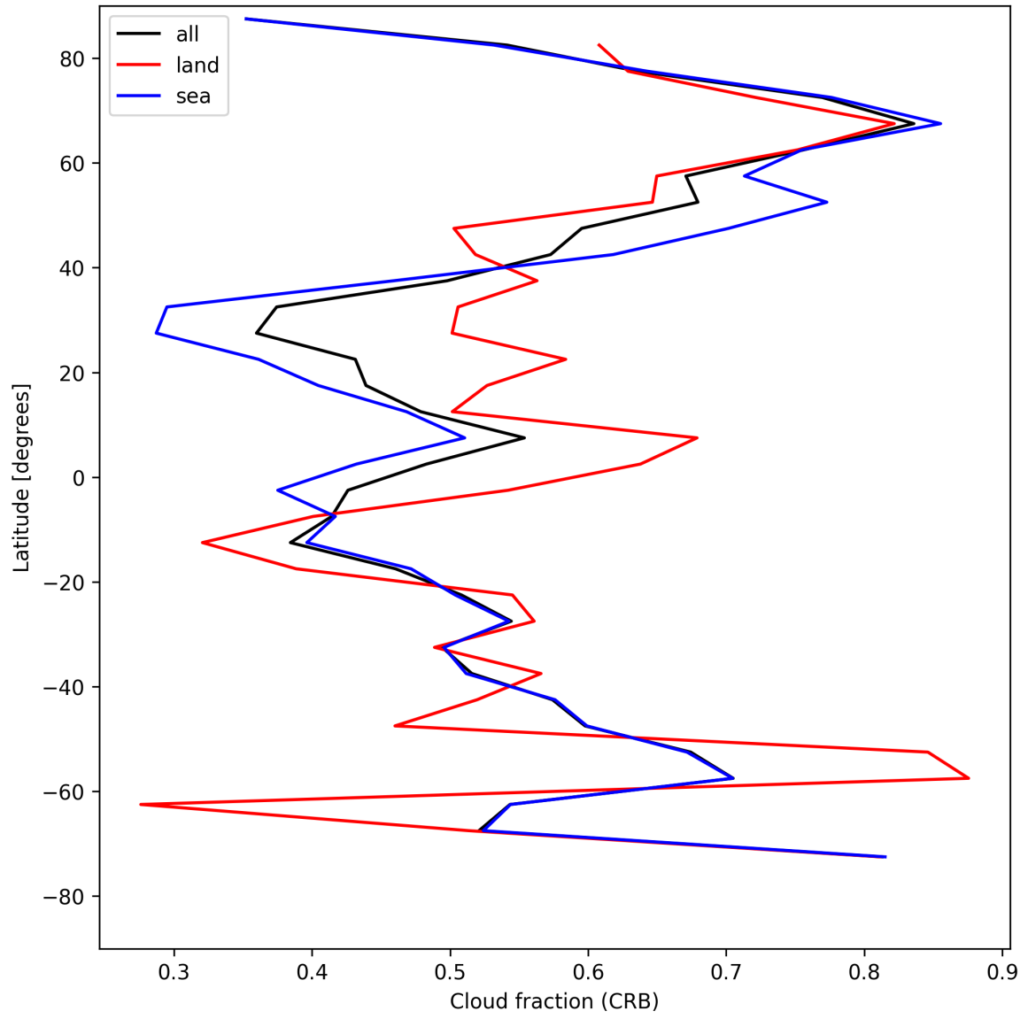
Figure 24: Zonal average of “Cloud fraction (CRB)” for 2025-08-06 to 2025-08-07.
