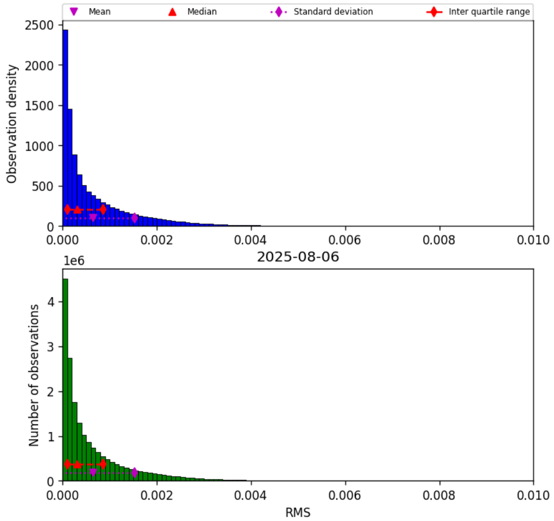
Figure 45: Histogram of “RMS” for 2025-08-06 to 2025-08-07
