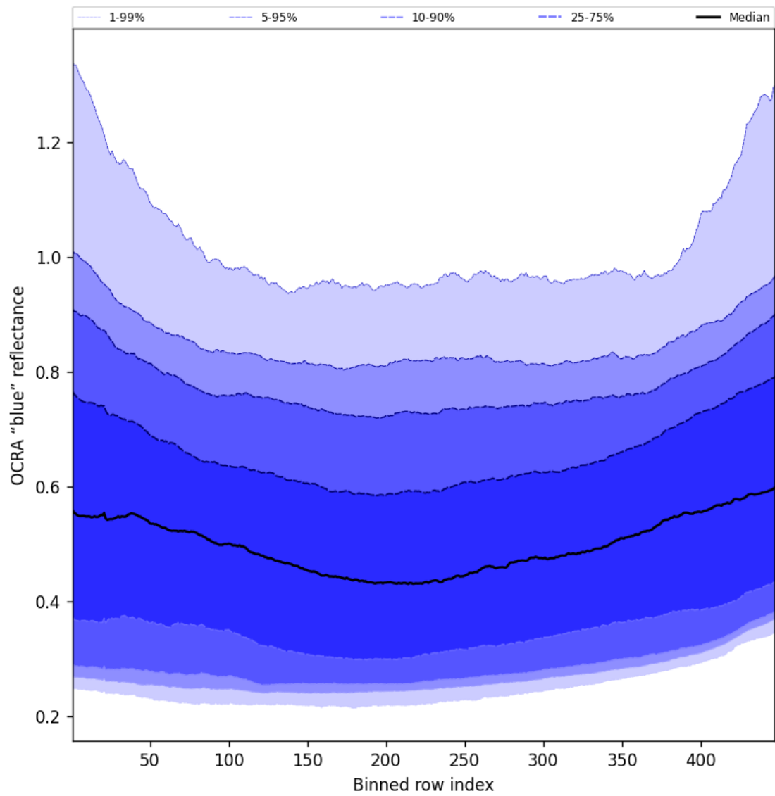
Figure 65: Along track statistics of “OCRA “blue” reflectance” for 2025-08-06 to 2025-08-07
