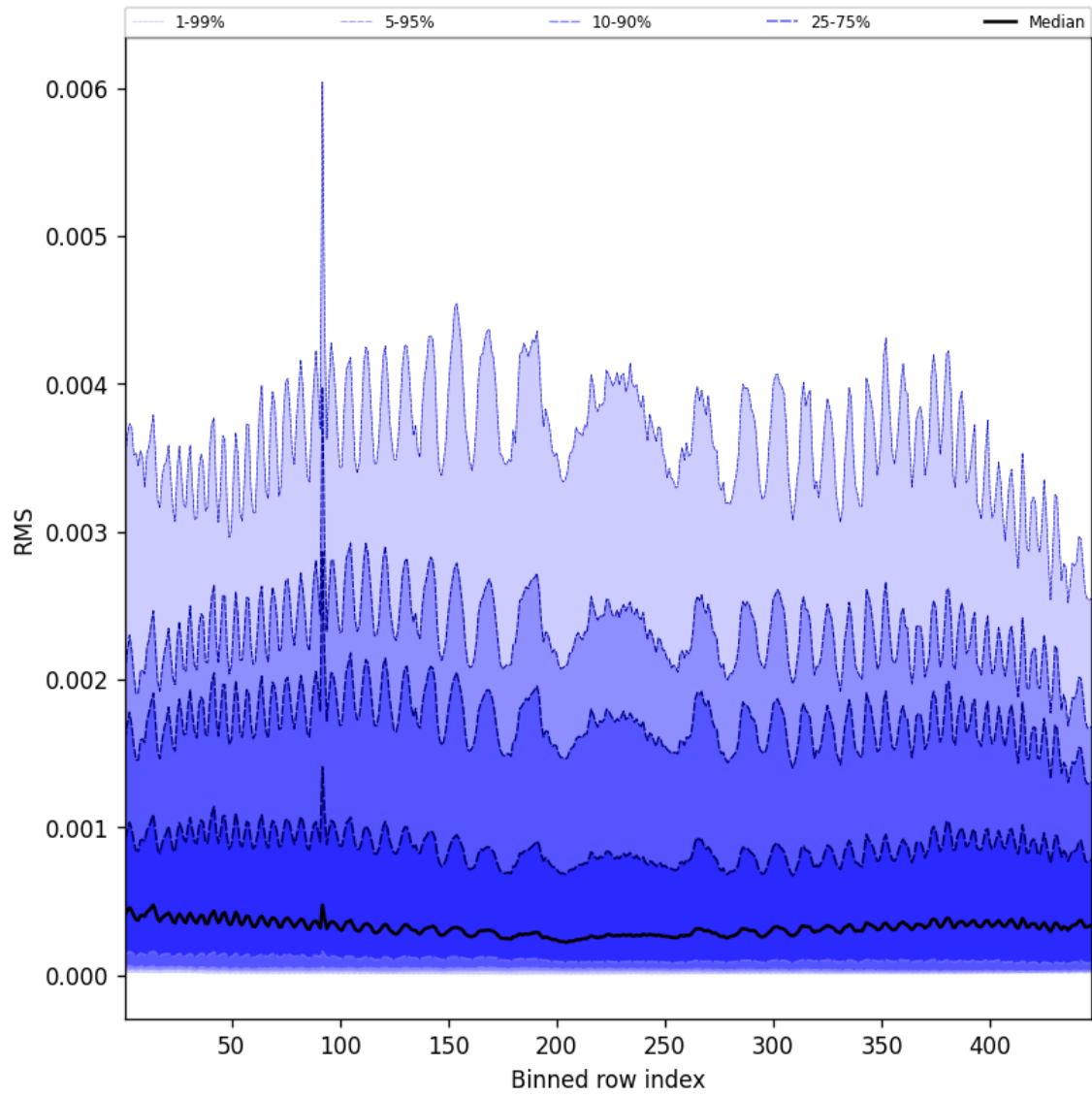
Figure 61: Along track statistics of “RMS” for 2025-08-06 to 2025-08-07
