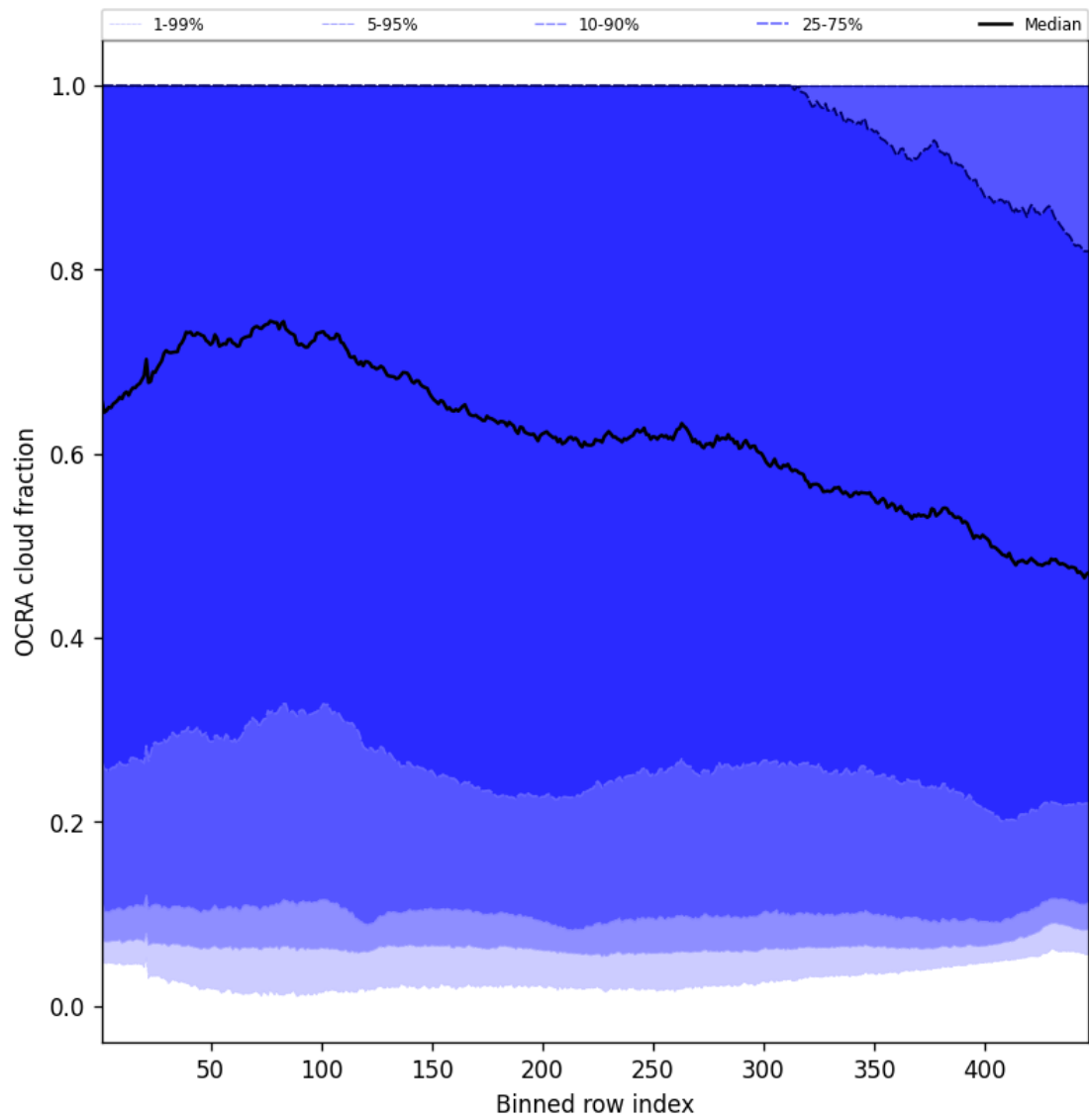
Figure 64: Along track statistics of “OCRA cloud fraction” for 2025-08-06 to 2025-08-07
