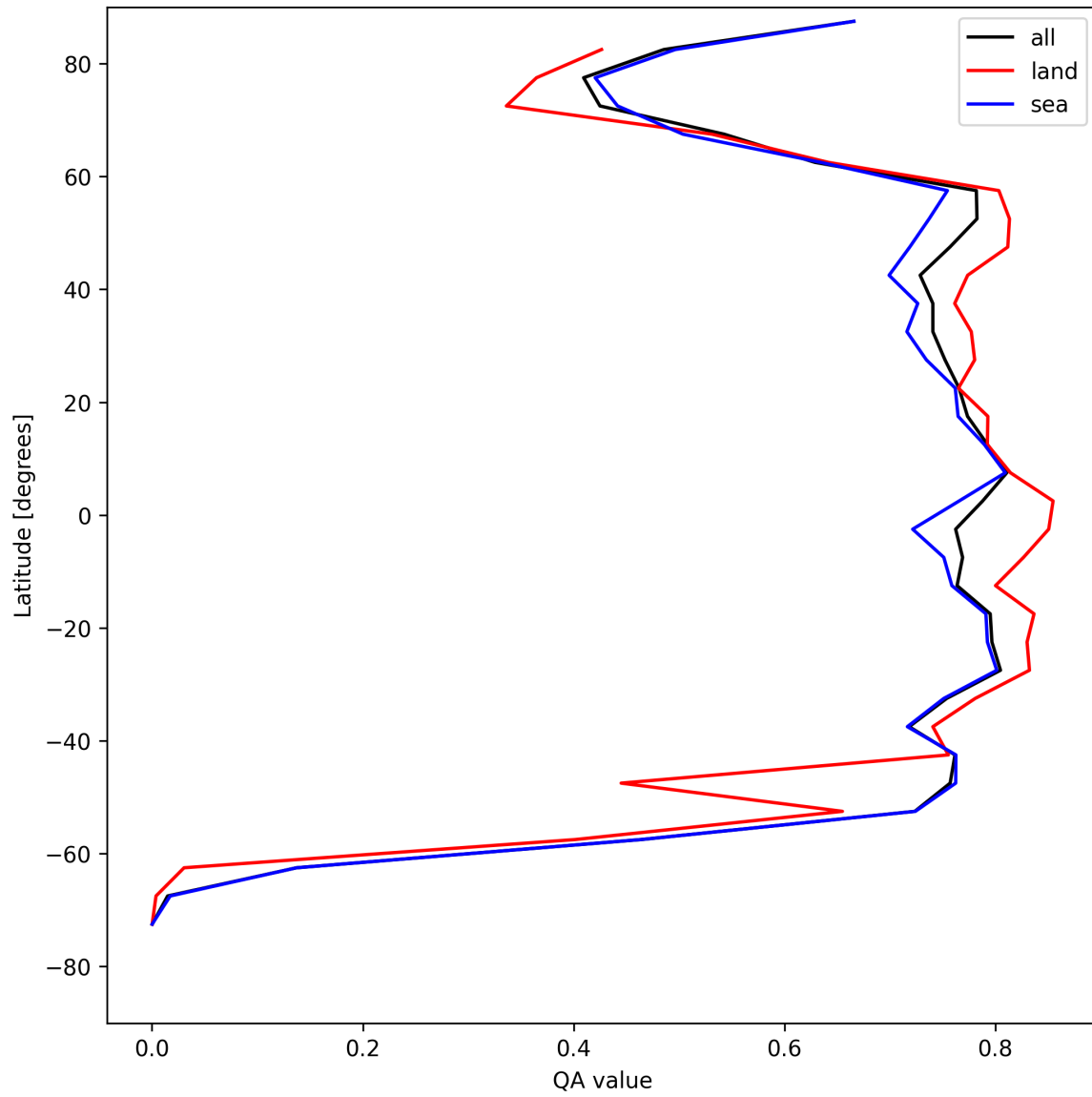
Figure 20: Zonal average of “QA value” for 2025-08-06 to 2025-08-07.
