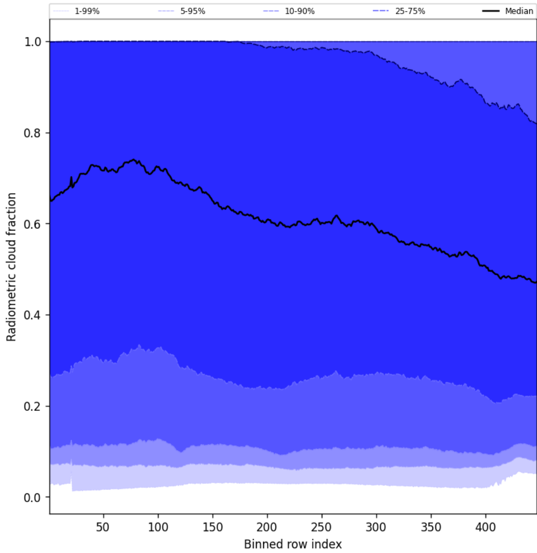
Figure 53: Along track statistics of “Radiometric cloud fraction” for 2025-08-06 to 2025-08-07
