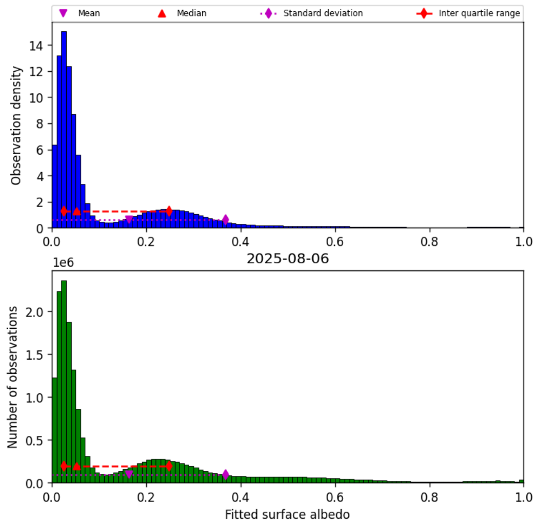
Figure 43: Histogram of “Fitted surface albedo” for 2025-08-06 to 2025-08-07
