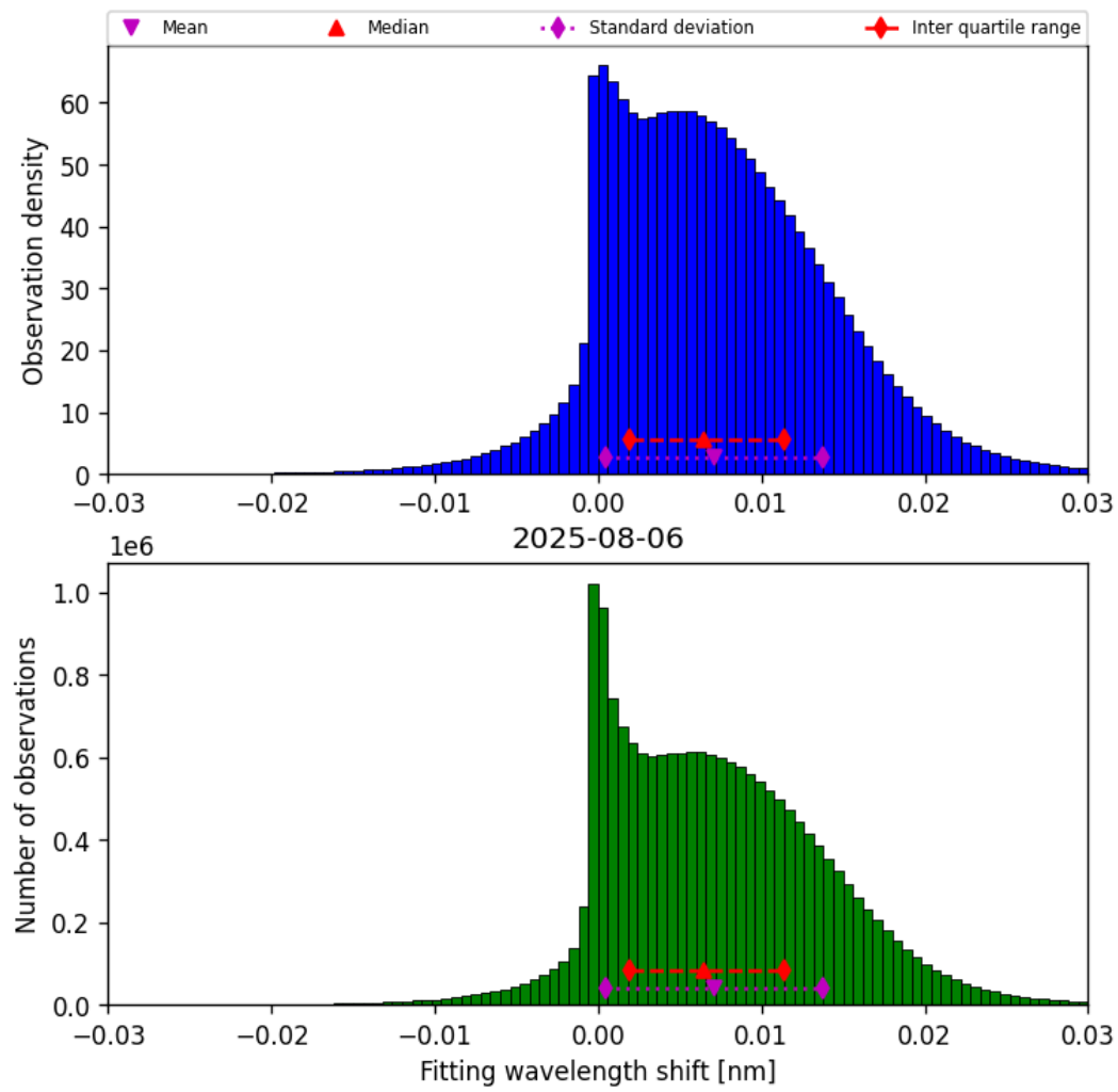
Figure 47: Histogram of “Fitting wavelength shift” for 2025-08-06 to 2025-08-07
