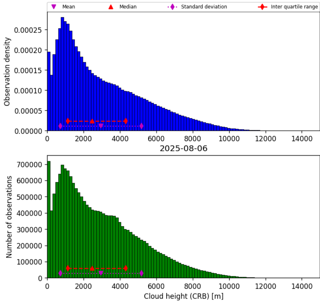
Figure 41: Histogram of “Cloud height (CRB)” for 2025-08-06 to 2025-08-07
