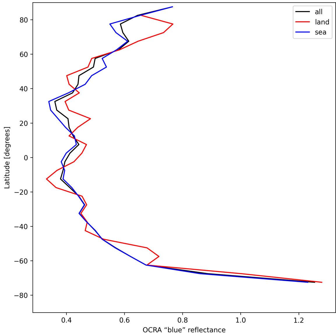
Figure 33: Zonal average of “OCRA “blue” reflectance” for 2025-08-06 to 2025-08-07.
