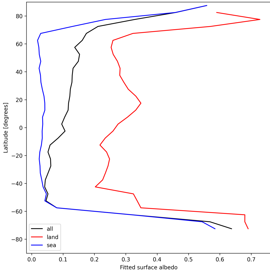
Figure 27: Zonal average of “Fitted surface albedo” for 2025-08-06 to 2025-08-07.
