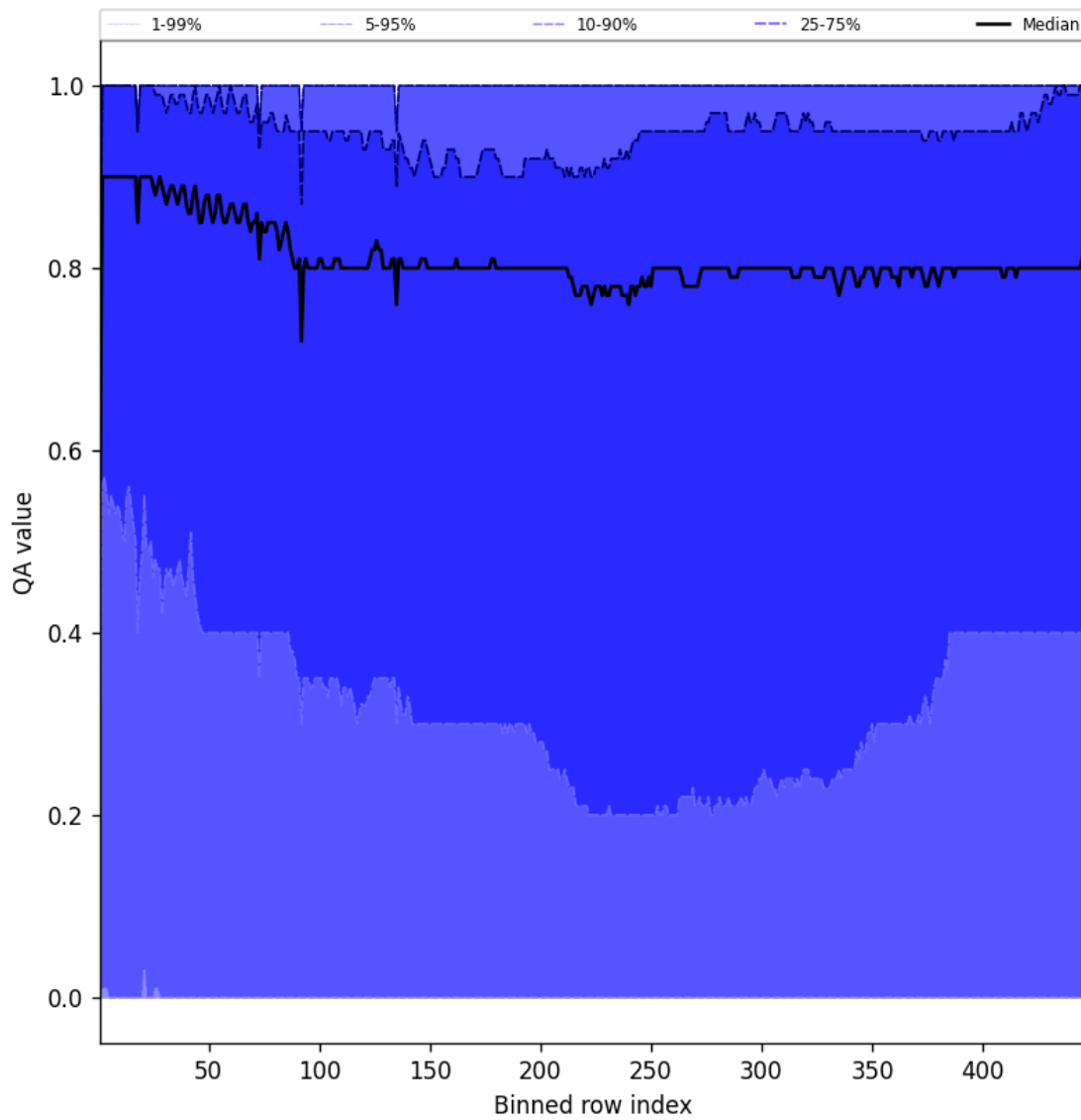
Figure 52: Along track statistics of “QA value” for 2025-08-06 to 2025-08-07
