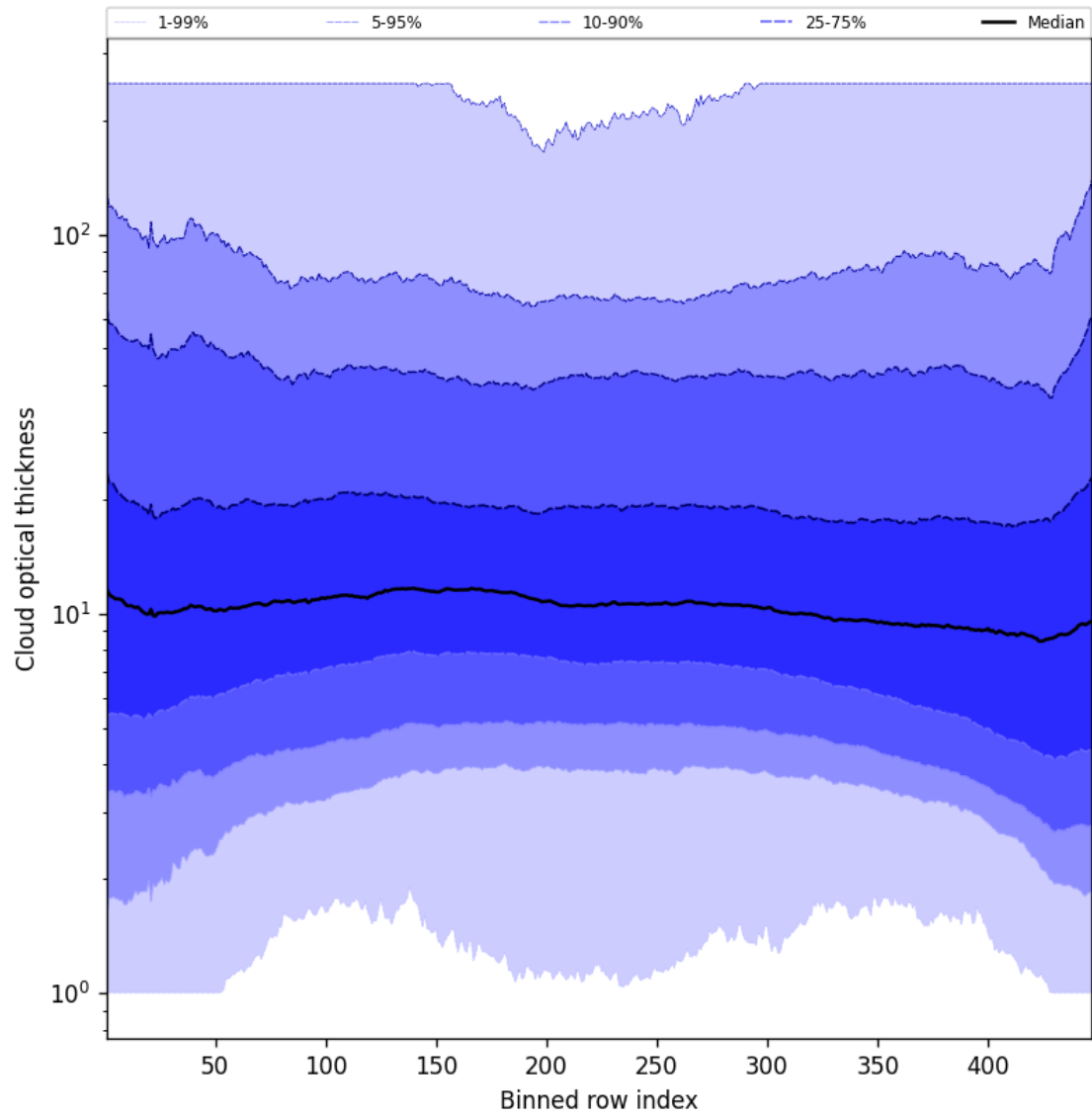
Figure 55: Along track statistics of “Cloud optical thickness” for 2025-08-06 to 2025-08-07
