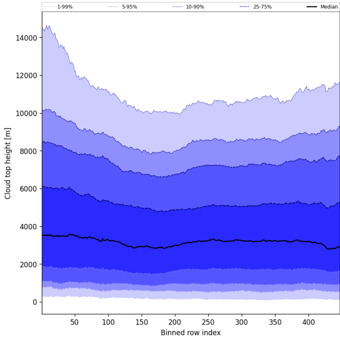
Figure 54: Along track statistics of “Cloud top height” for 2025-08-06 to 2025-08-07
