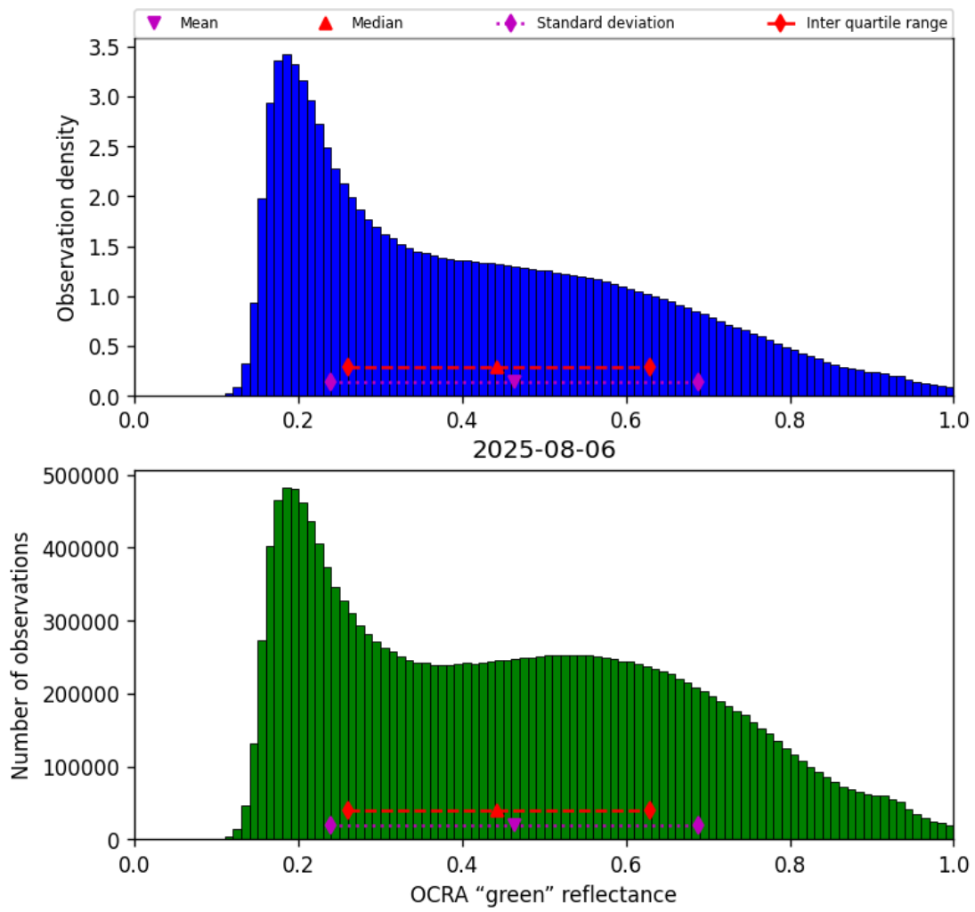
Figure 50: Histogram of “OCRA “green” reflectance” for 2025-08-06 to 2025-08-07
