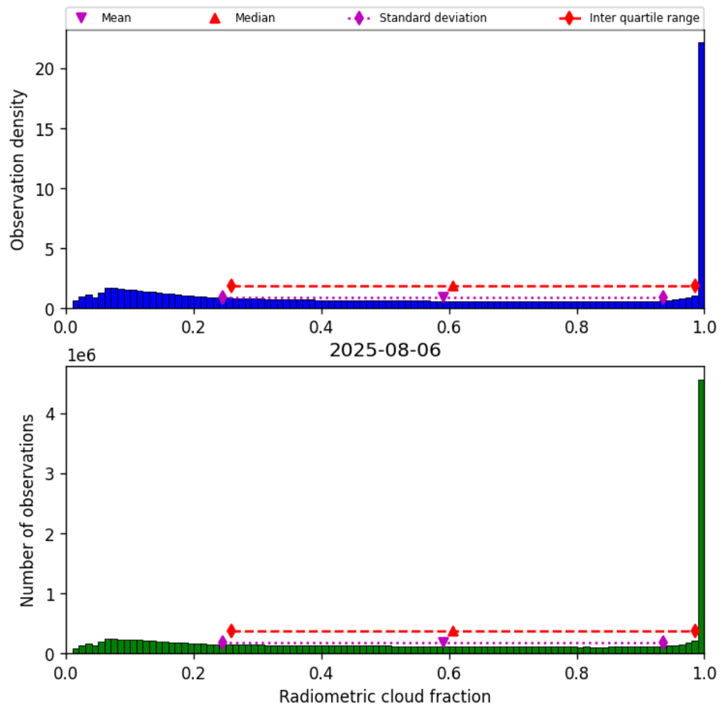
Figure 37: Histogram of “Radiometric cloud fraction” for 2025-08-06 to 2025-08-07
