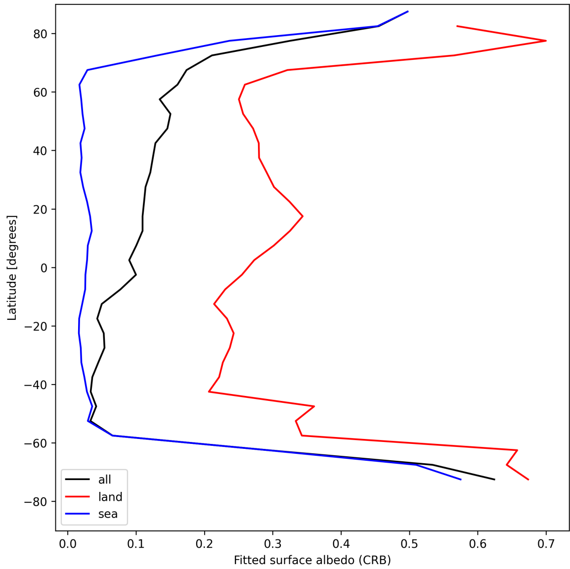
Figure 28: Zonal average of “Fitted surface albedo (CRB)” for 2025-08-06 to 2025-08-07.
