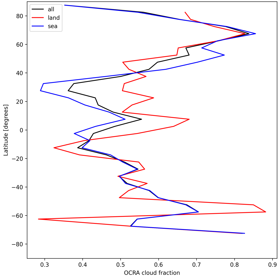
Figure 32: Zonal average of “OCRA cloud fraction” for 2025-08-06 to 2025-08-07.
