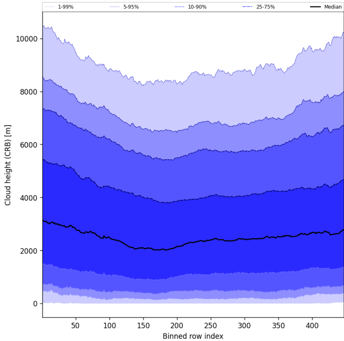
Figure 57: Along track statistics of “Cloud height (CRB)” for 2025-08-06 to 2025-08-07
