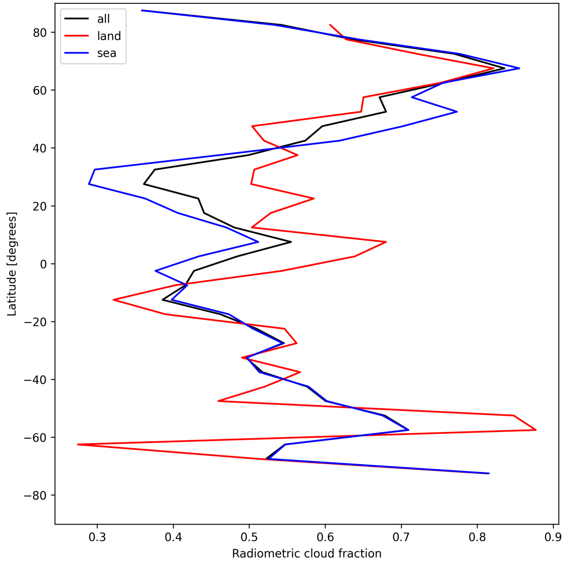
Figure 21: Zonal average of “Radiometric cloud fraction” for 2025-08-06 to 2025-08-07.
