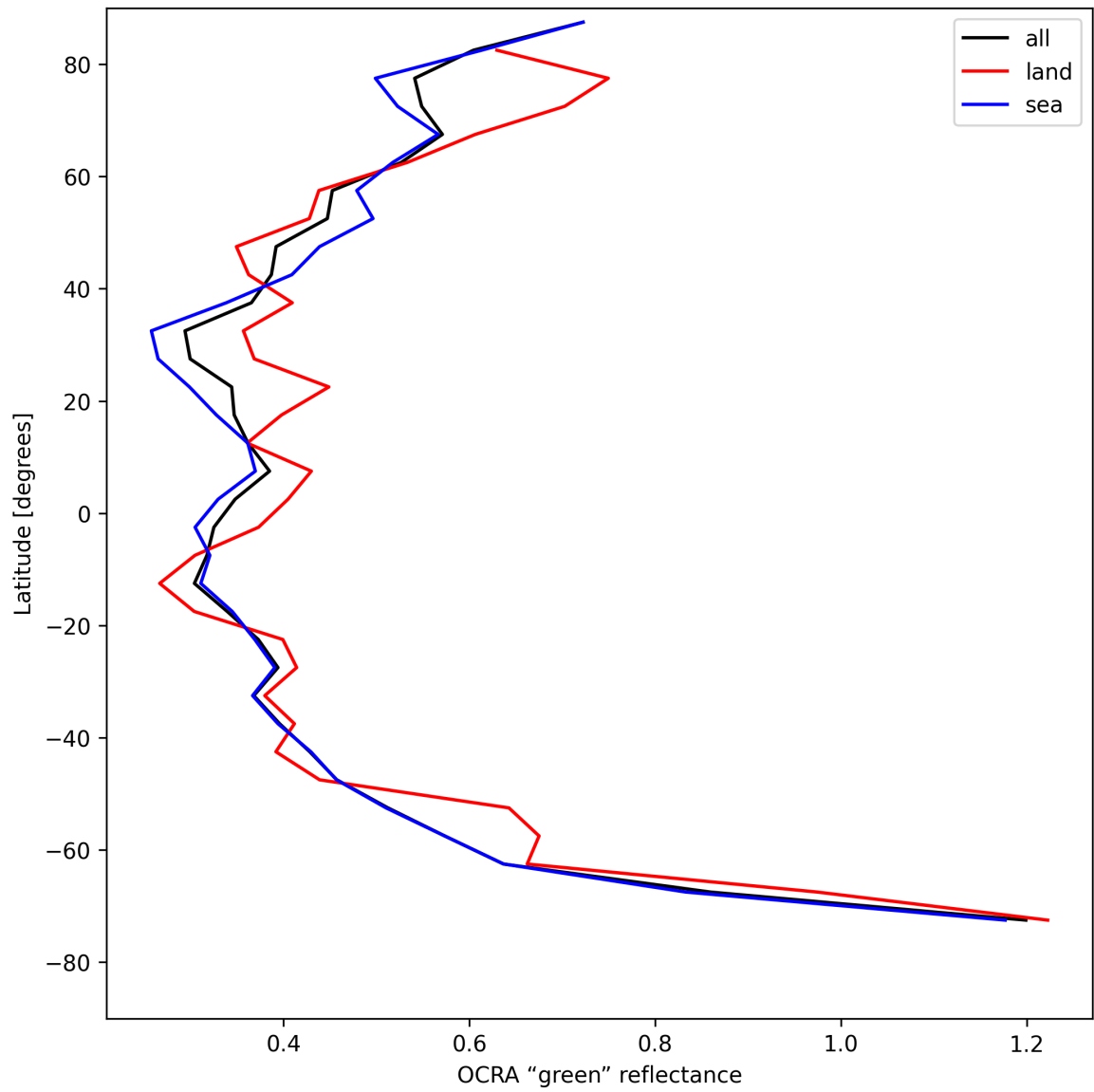
Figure 34: Zonal average of “OCRA “green” reflectance” for 2025-08-06 to 2025-08-07.
