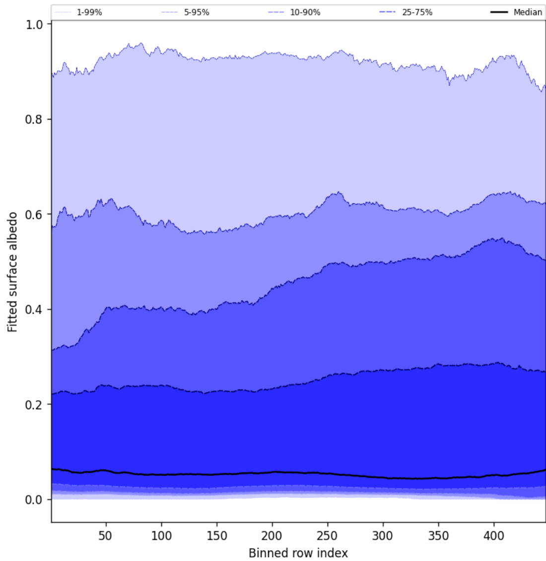
Figure 59: Along track statistics of “Fitted surface albedo” for 2025-08-06 to 2025-08-07
