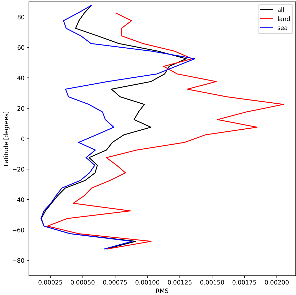
Figure 29: Zonal average of “RMS” for 2025-08-06 to 2025-08-07.
