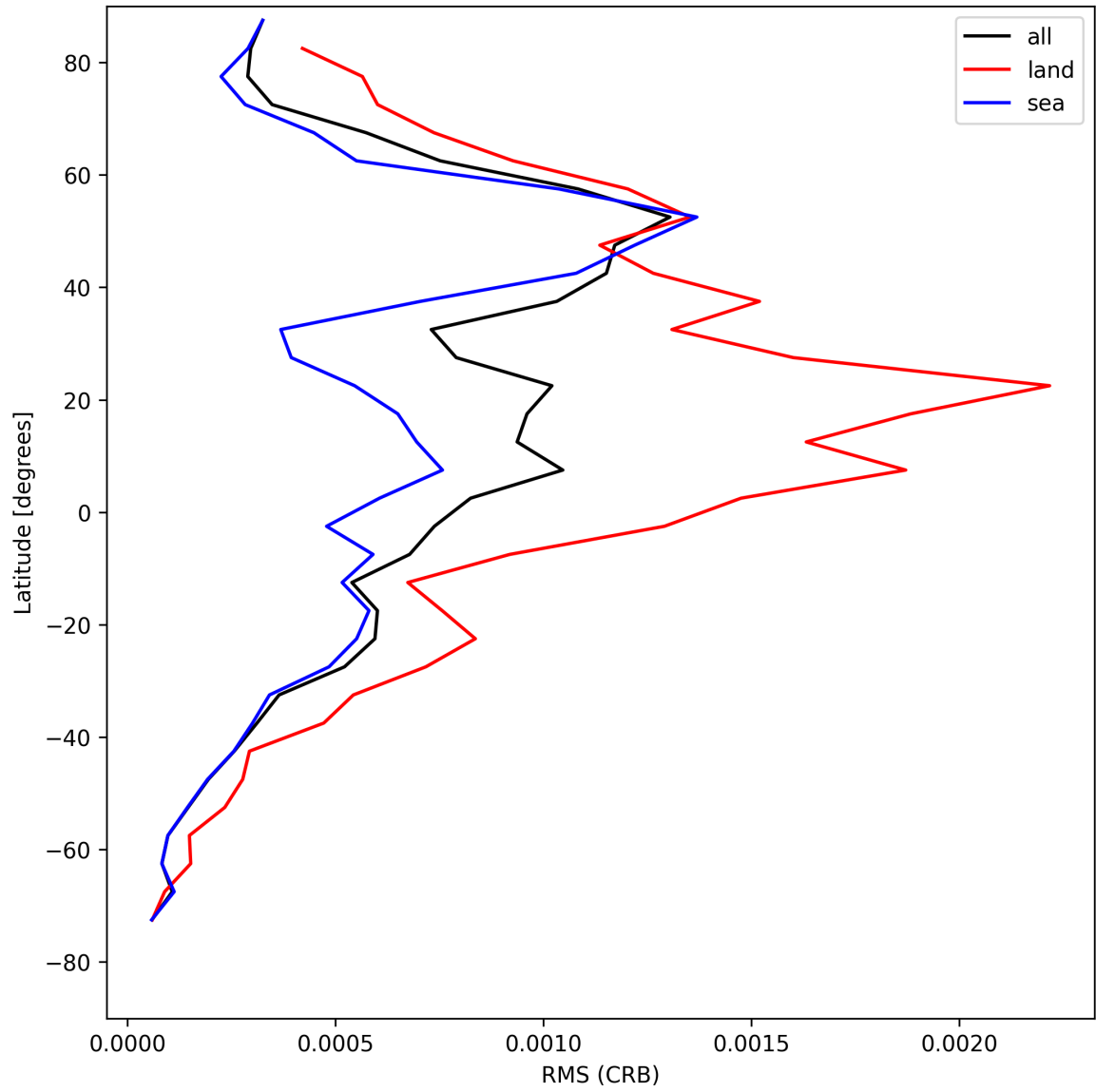
Figure 30: Zonal average of “RMS (CRB)” for 2025-08-06 to 2025-08-07.
