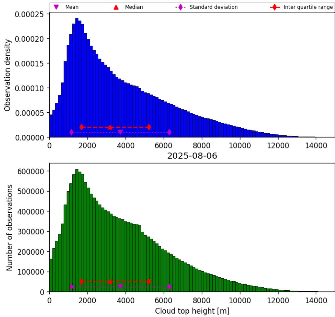
Figure 38: Histogram of “Cloud top height” for 2025-08-06 to 2025-08-07
