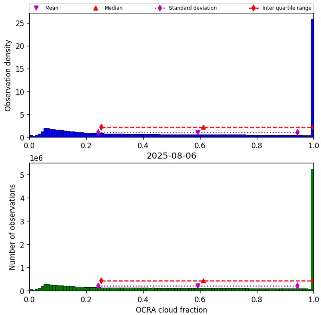
Figure 48: Histogram of “OCRA cloud fraction” for 2025-08-06 to 2025-08-07
