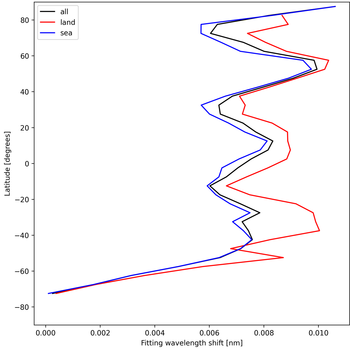
Figure 31: Zonal average of “Fitting wavelength shift” for 2025-08-06 to 2025-08-07.
