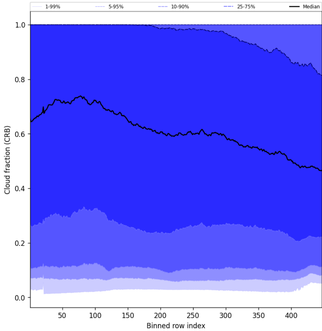
Figure 56: Along track statistics of “Cloud fraction (CRB)” for 2025-08-06 to 2025-08-07
