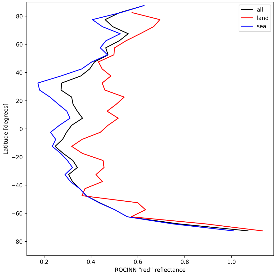
Figure 35: Zonal average of “ROCINN “red” reflectance” for 2025-08-06 to 2025-08-07.
