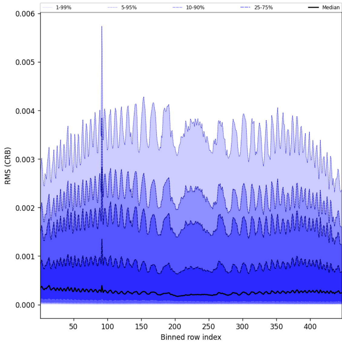
Figure 62: Along track statistics of “RMS (CRB)” for 2025-08-06 to 2025-08-07
