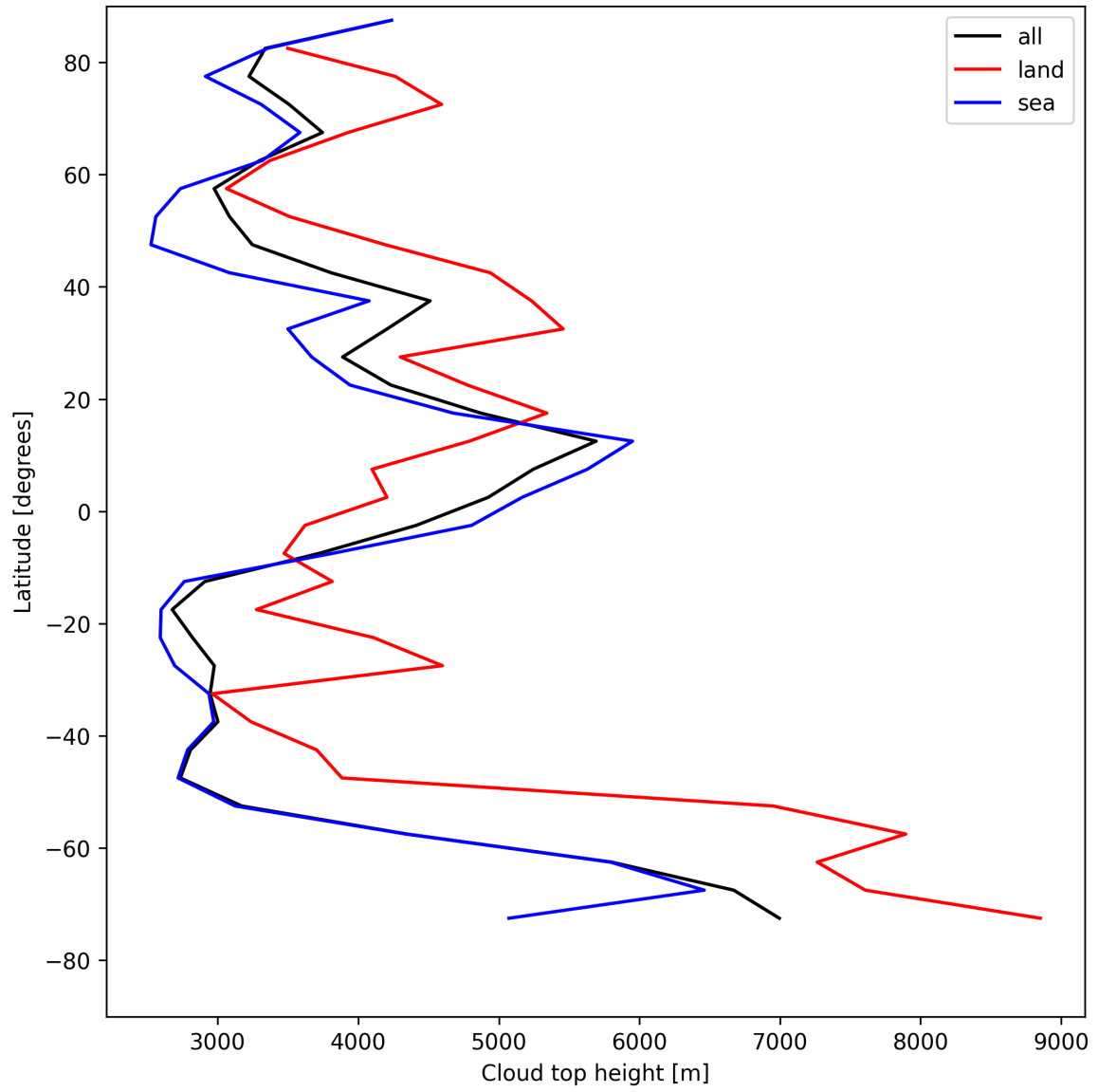
Figure 22: Zonal average of “Cloud top height” for 2025-08-06 to 2025-08-07.
