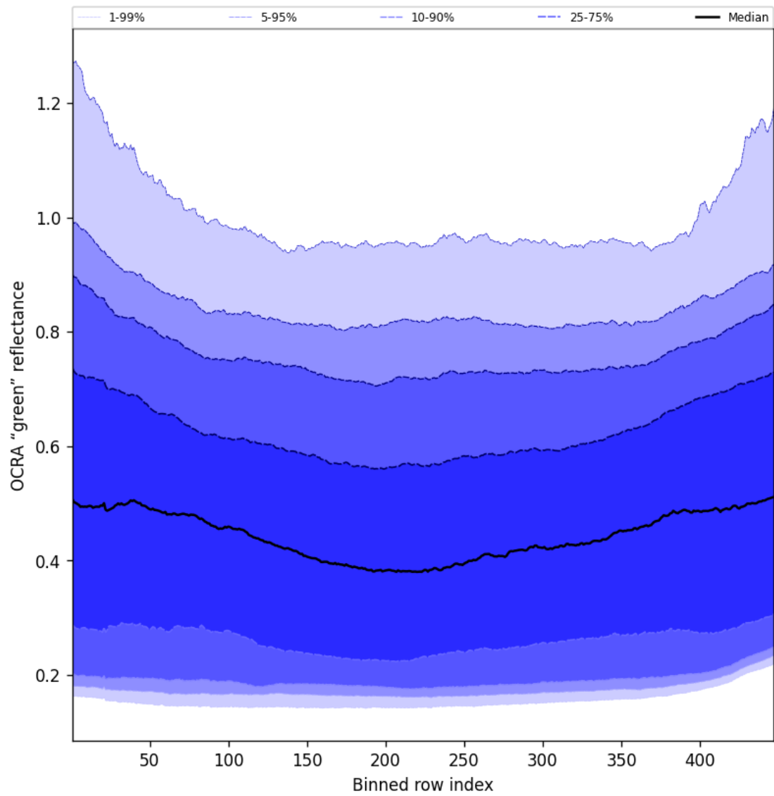
Figure 66: Along track statistics of “OCRA “green” reflectance” for 2025-08-06 to 2025-08-07
