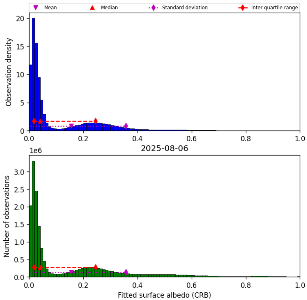
Figure 44: Histogram of “Fitted surface albedo (CRB)” for 2025-08-06 to 2025-08-07
