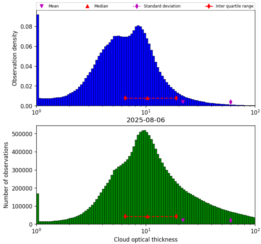
Figure 39: Histogram of “Cloud optical thickness” for 2025-08-06 to 2025-08-07
