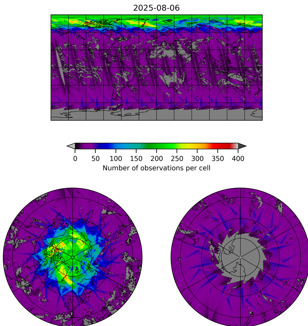
Figure 19: Map of the number of observations for 2025-08-06 to 2025-08-07
