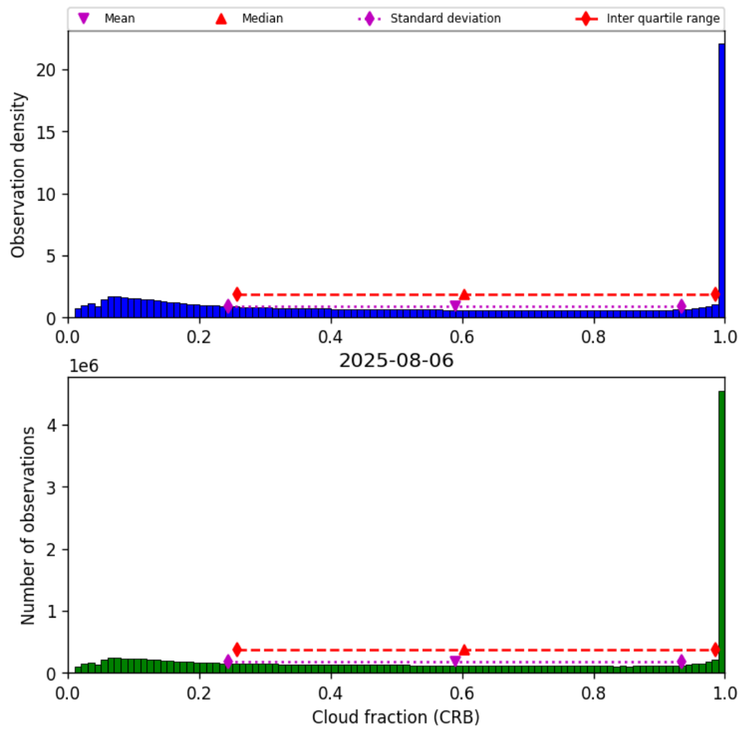
Figure 40: Histogram of “Cloud fraction (CRB)” for 2025-08-06 to 2025-08-07
