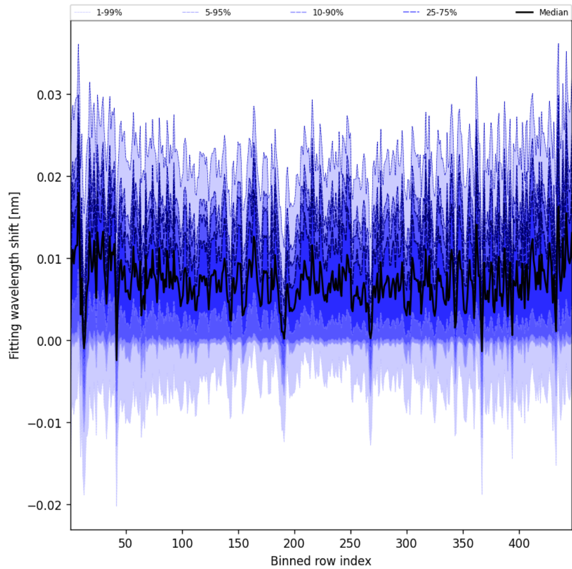
Figure 63: Along track statistics of “Fitting wavelength shift” for 2025-08-06 to 2025-08-07
