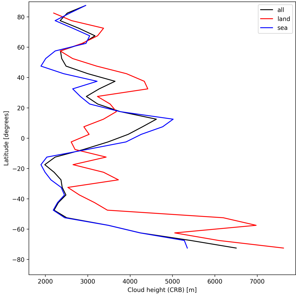
Figure 25: Zonal average of “Cloud height (CRB)” for 2025-08-06 to 2025-08-07.
