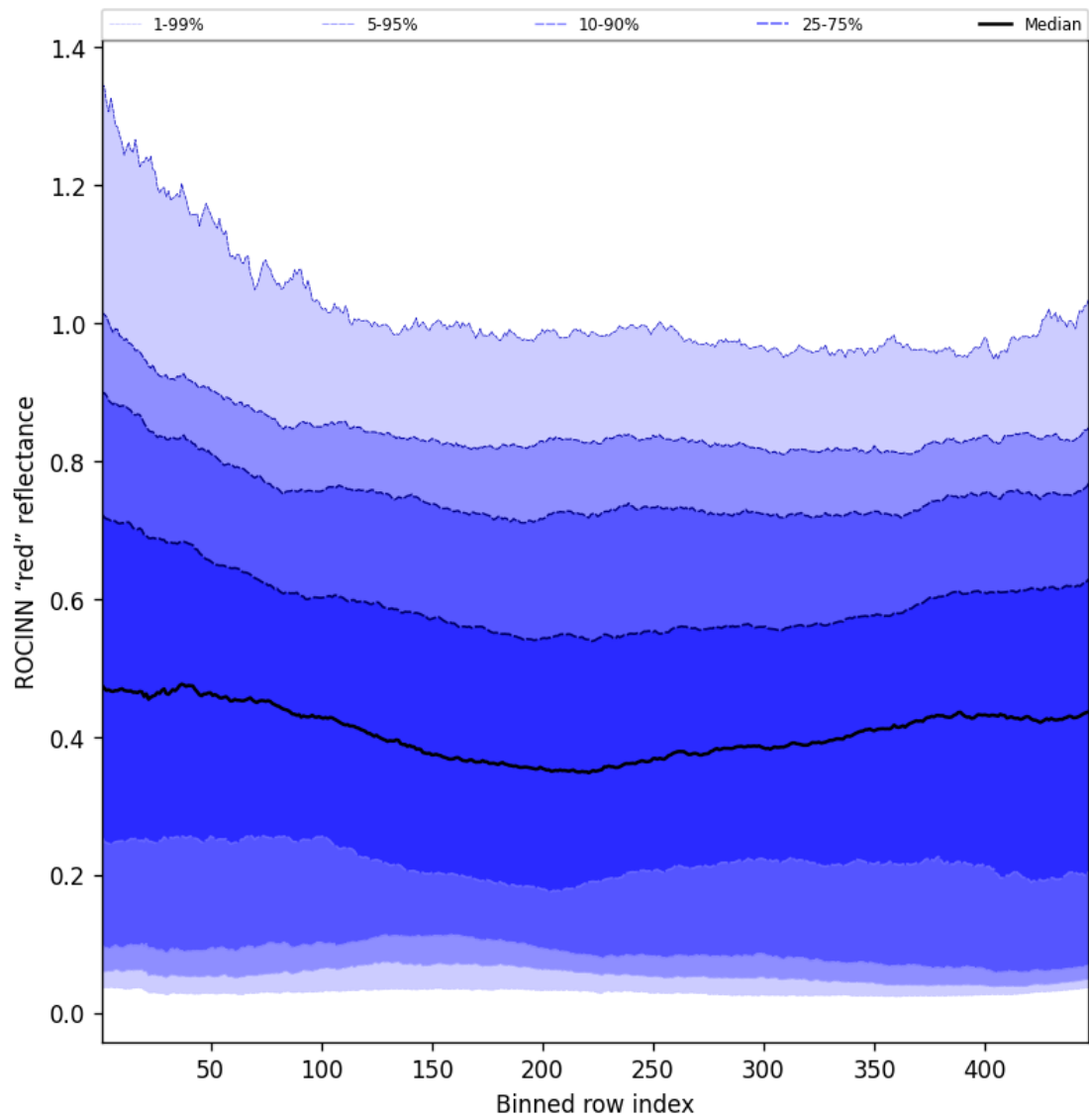
Figure 67: Along track statistics of "ROCINN "red" reflectance" for 2025-08-06 to 2025-08-07
