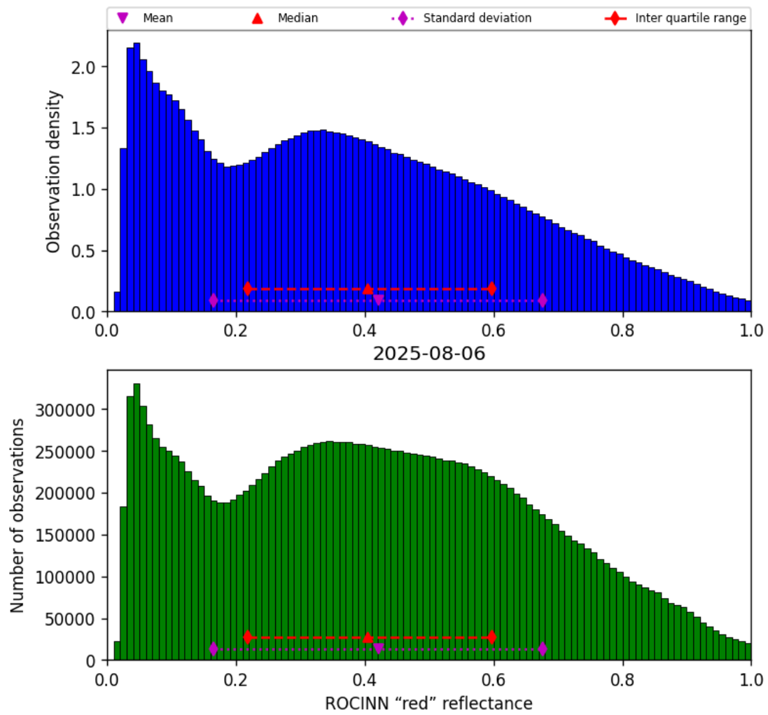
Figure 51: Histogram of “ROCINN “red” reflectance” for 2025-08-06 to 2025-08-07
