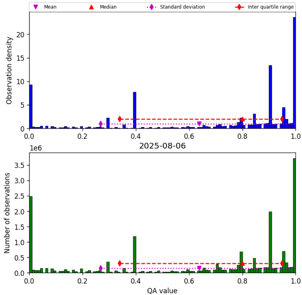
Figure 36: Histogram of “QA value” for 2025-08-06 to 2025-08-07
