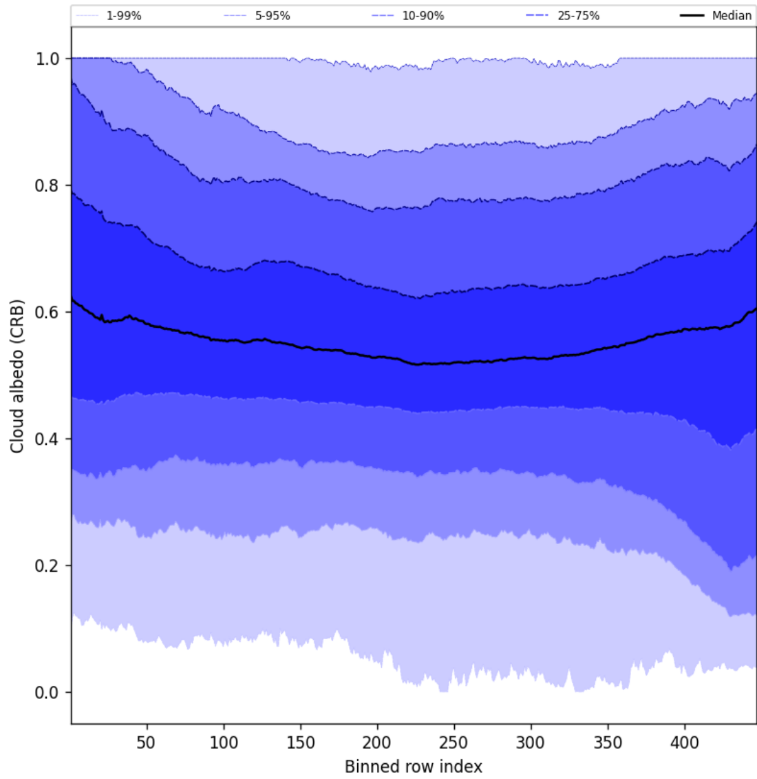
Figure 58: Along track statistics of “Cloud albedo (CRB)” for 2025-08-06 to 2025-08-07
