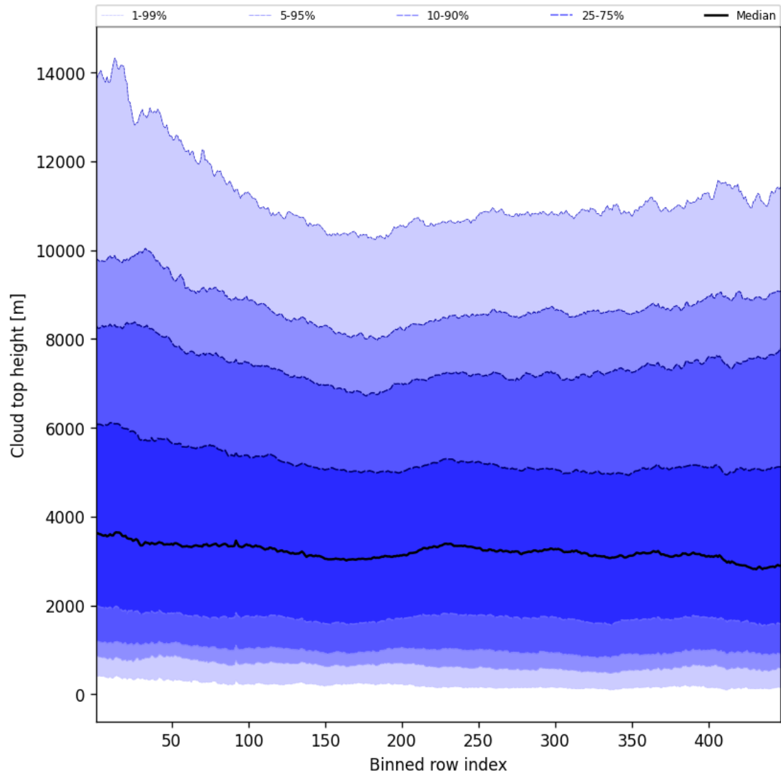
Figure 54: Along track statistics of “Cloud top height” for 2025-08-07 to 2025-08-07
