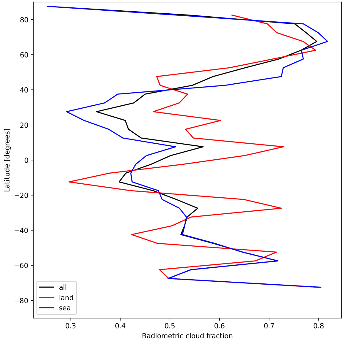
Figure 21: Zonal average of “Radiometric cloud fraction” for 2025-08-07 to 2025-08-07.
