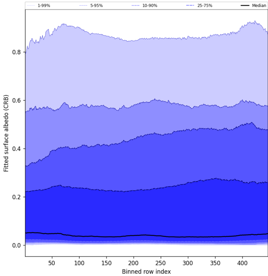
Figure 60: Along track statistics of “Fitted surface albedo (CRB)” for 2025-08-07 to 2025-08-07
