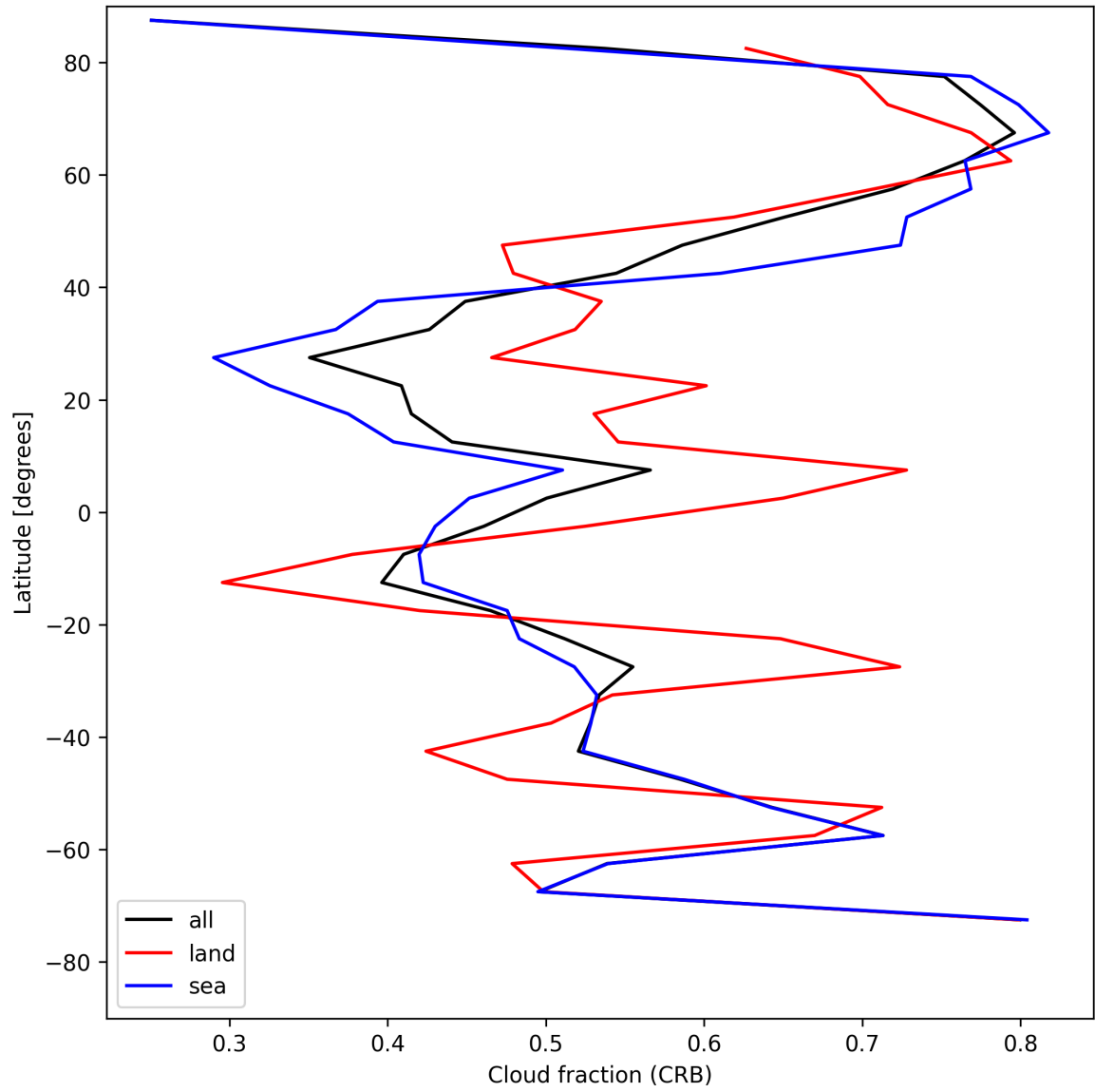
Figure 24: Zonal average of “Cloud fraction (CRB)” for 2025-08-07 to 2025-08-07.
