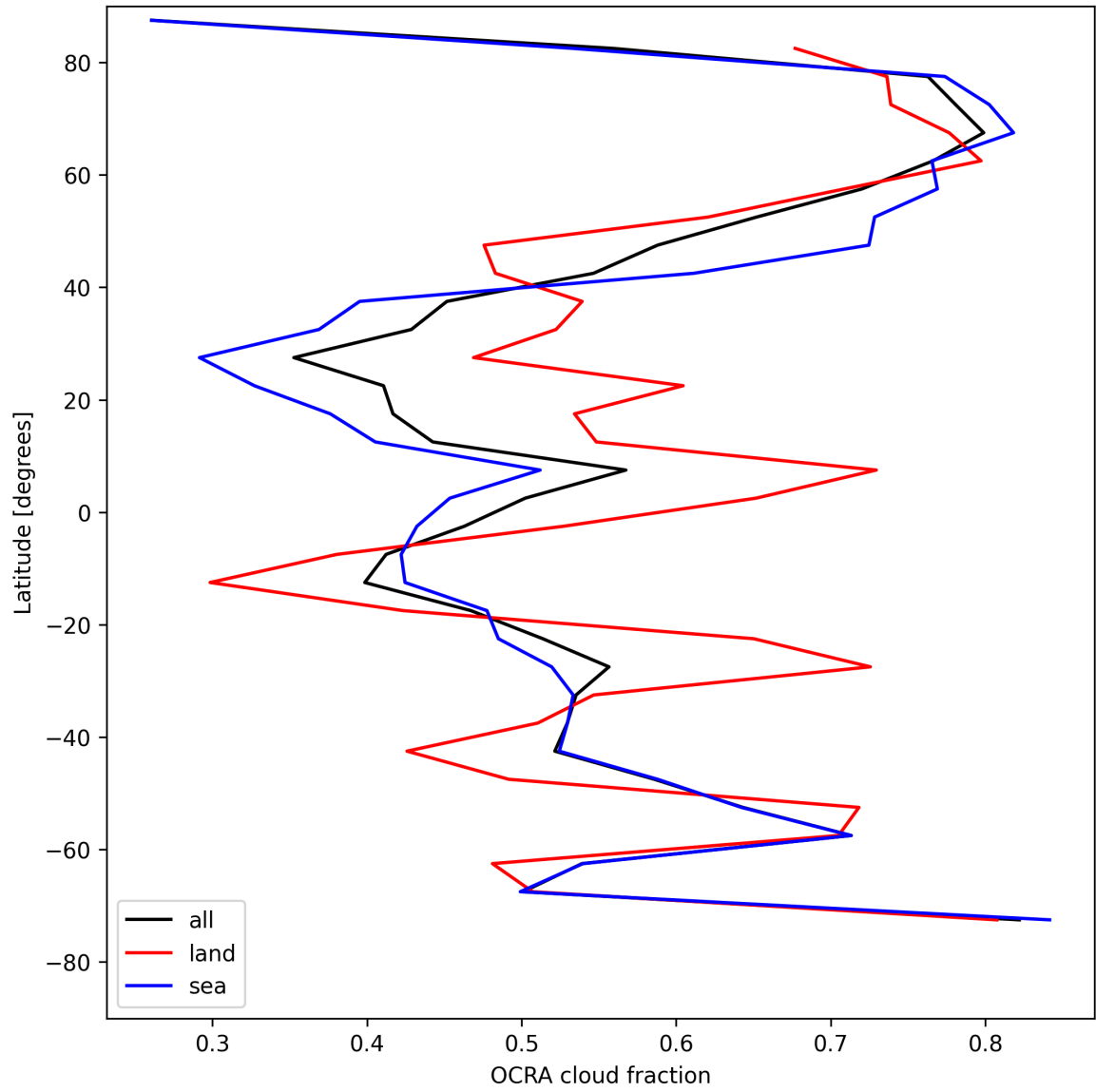
Figure 32: Zonal average of “OCRA cloud fraction” for 2025-08-07 to 2025-08-07.
