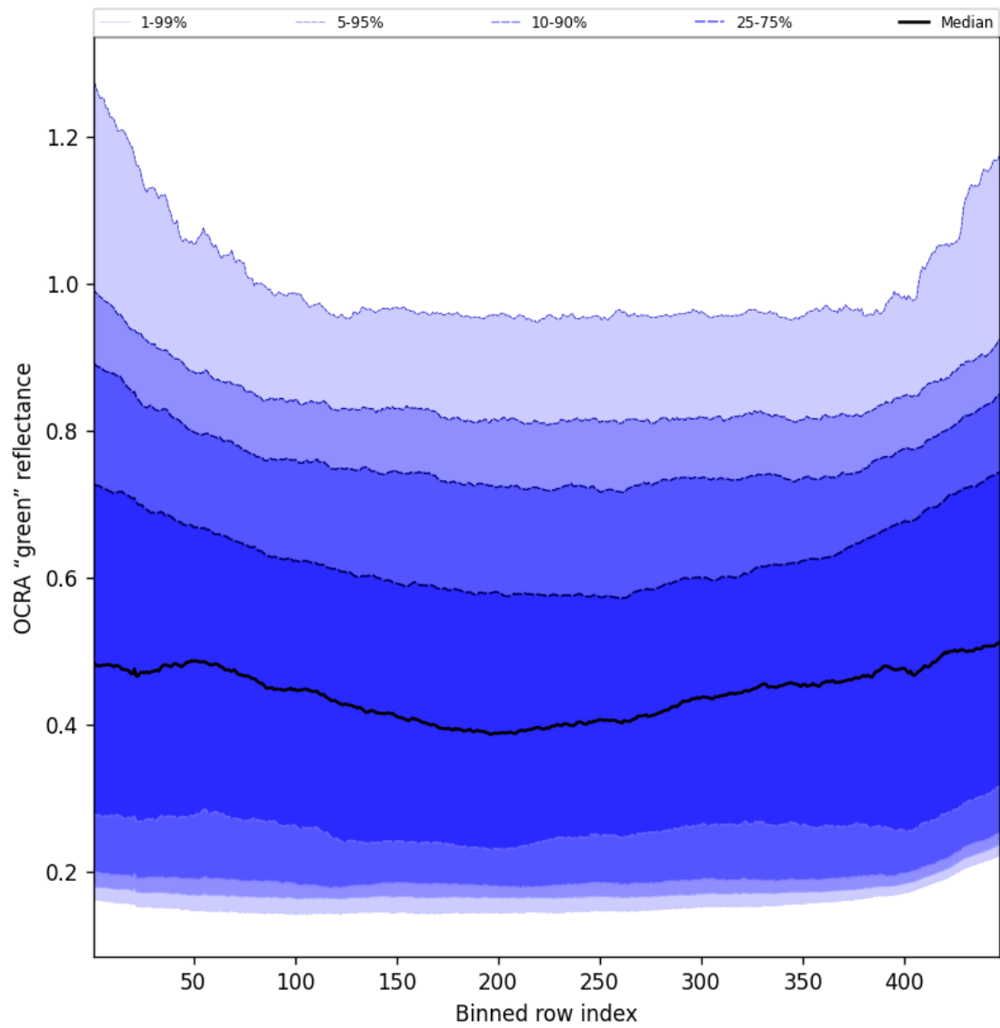
Figure 66: Along track statistics of “OCRA “green” reflectance” for 2025-08-07 to 2025-08-07
