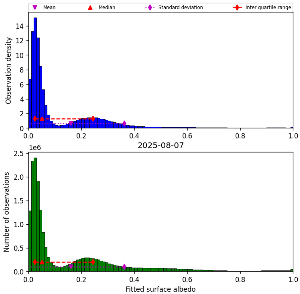
Figure 43: Histogram of “Fitted surface albedo” for 2025-08-07 to 2025-08-07
