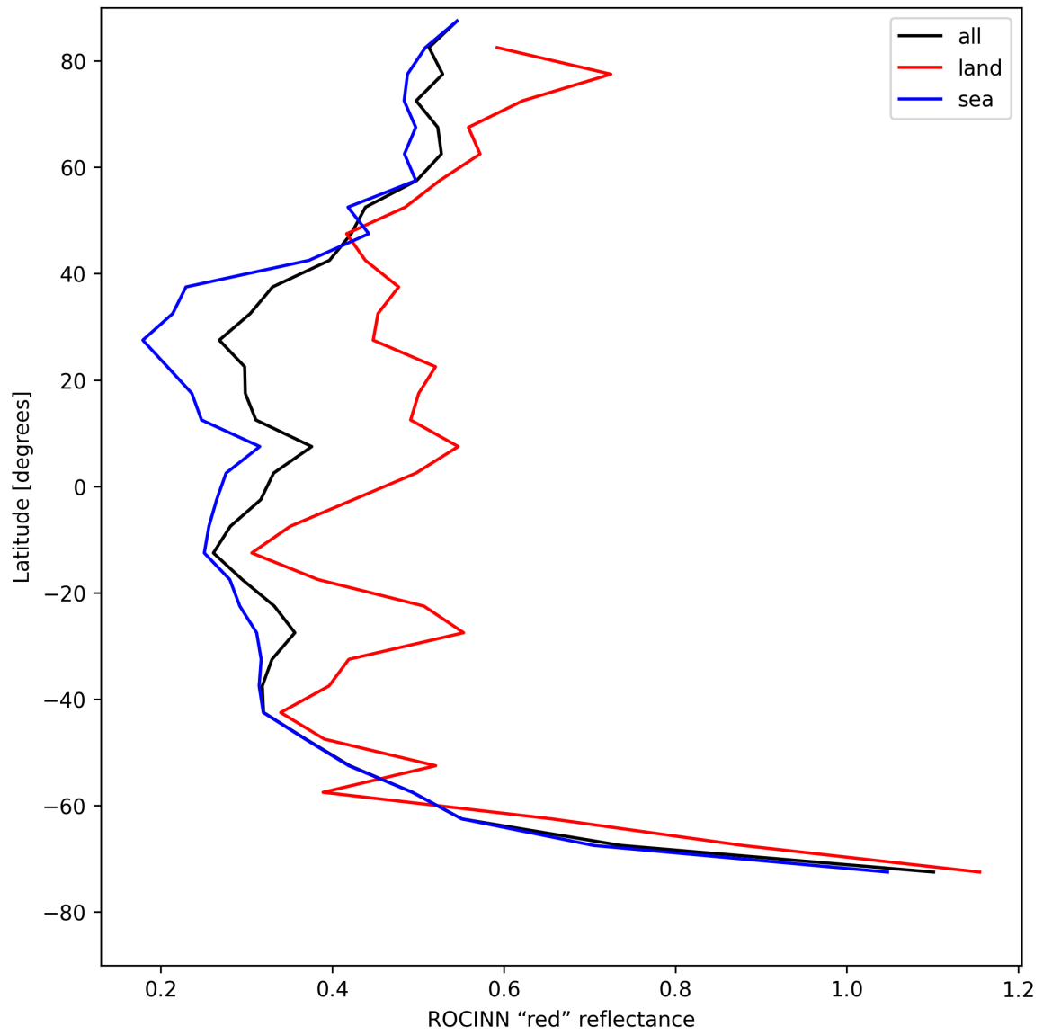
Figure 35: Zonal average of “ROCINN “red” reflectance” for 2025-08-07 to 2025-08-07.
