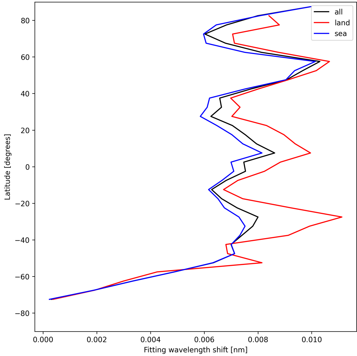
Figure 31: Zonal average of “Fitting wavelength shift” for 2025-08-07 to 2025-08-07.
