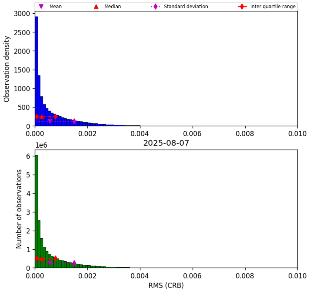
Figure 46: Histogram of “RMS (CRB)” for 2025-08-07 to 2025-08-07
