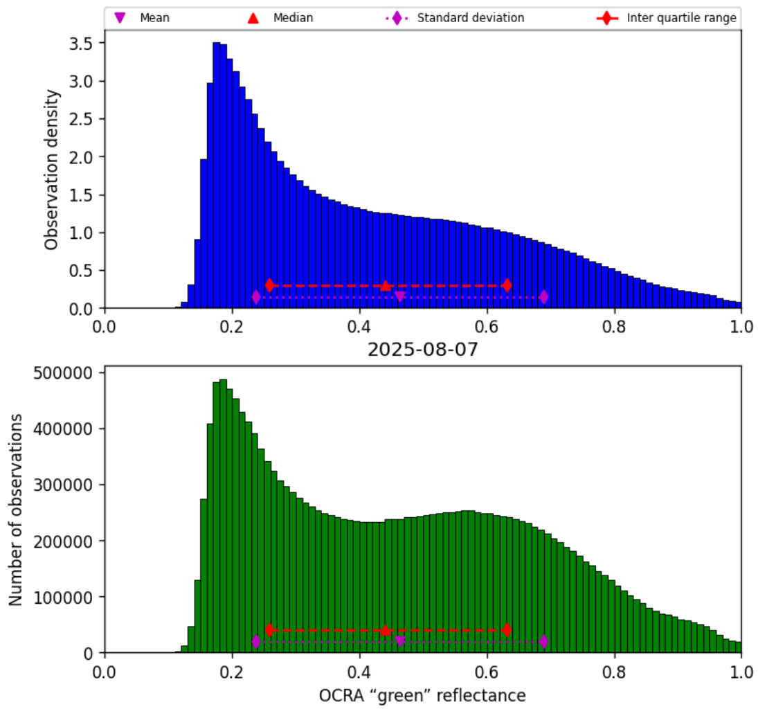
Figure 50: Histogram of “OCRA “green” reflectance” for 2025-08-07 to 2025-08-07
