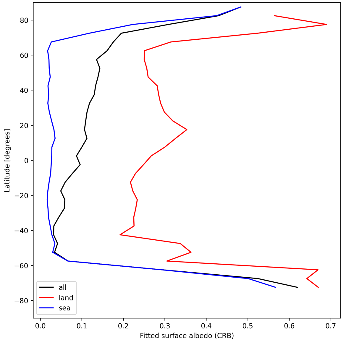
Figure 28: Zonal average of “Fitted surface albedo (CRB)” for 2025-08-07 to 2025-08-07.
