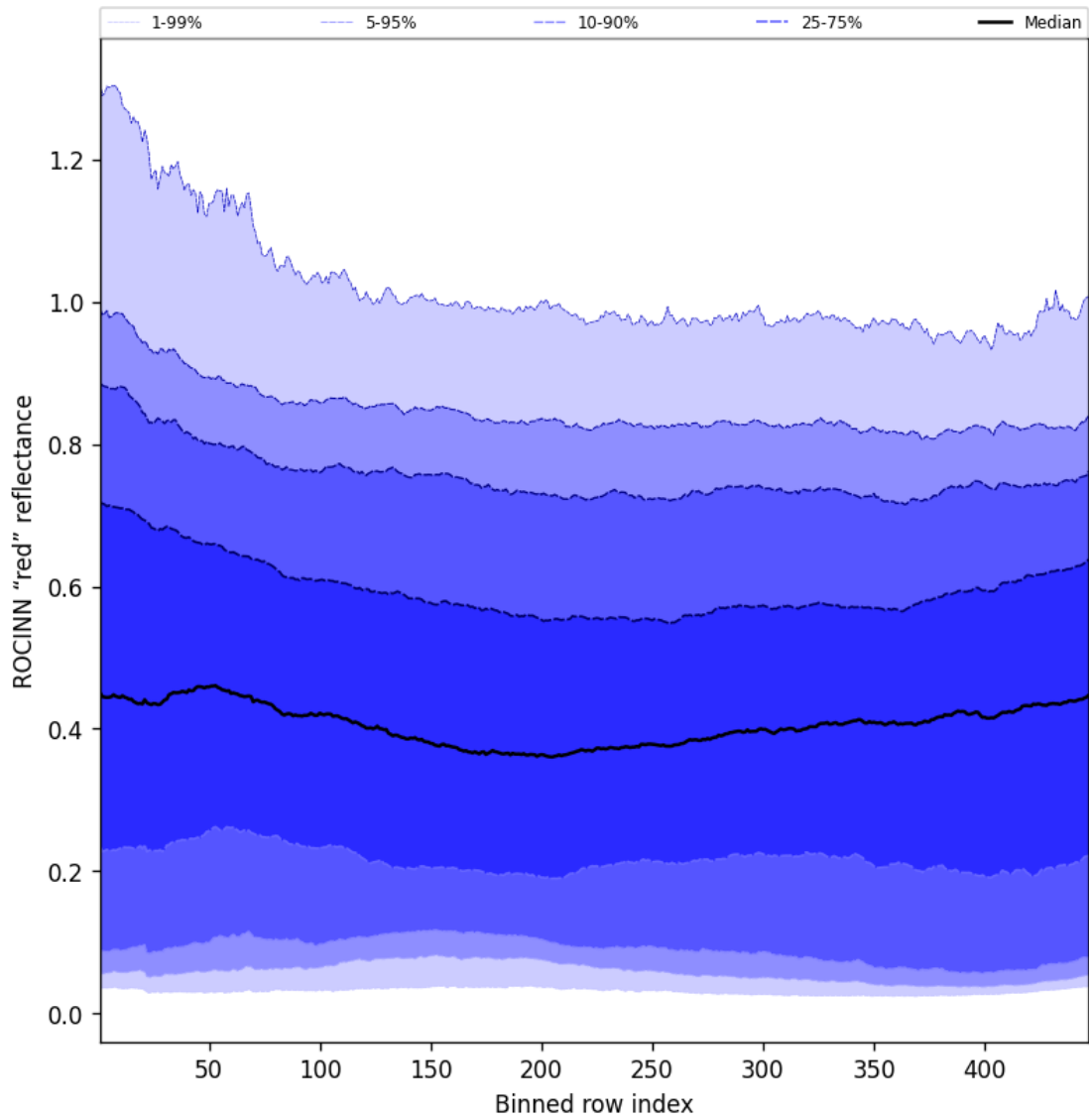
Figure 67: Along track statistics of “ROCINN “red” reflectance” for 2025-08-07 to 2025-08-07
