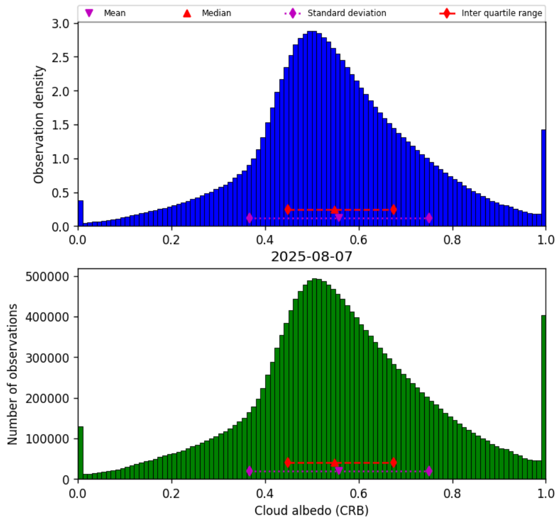
Figure 42: Histogram of “Cloud albedo (CRB)” for 2025-08-07 to 2025-08-07
