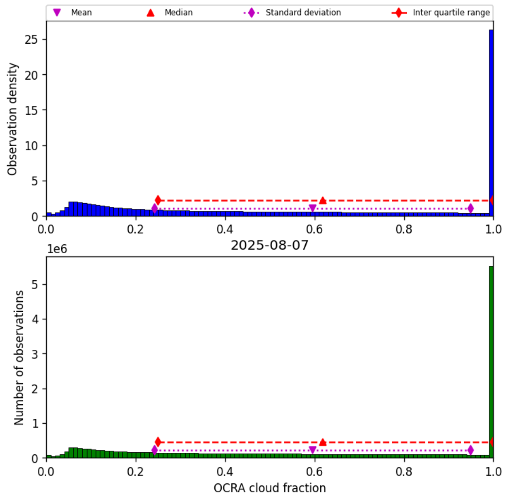
Figure 48: Histogram of “OCRA cloud fraction” for 2025-08-07 to 2025-08-07
