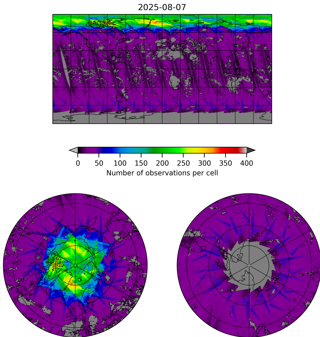
Figure 19: Map of the number of observations for 2025-08-07 to 2025-08-07
