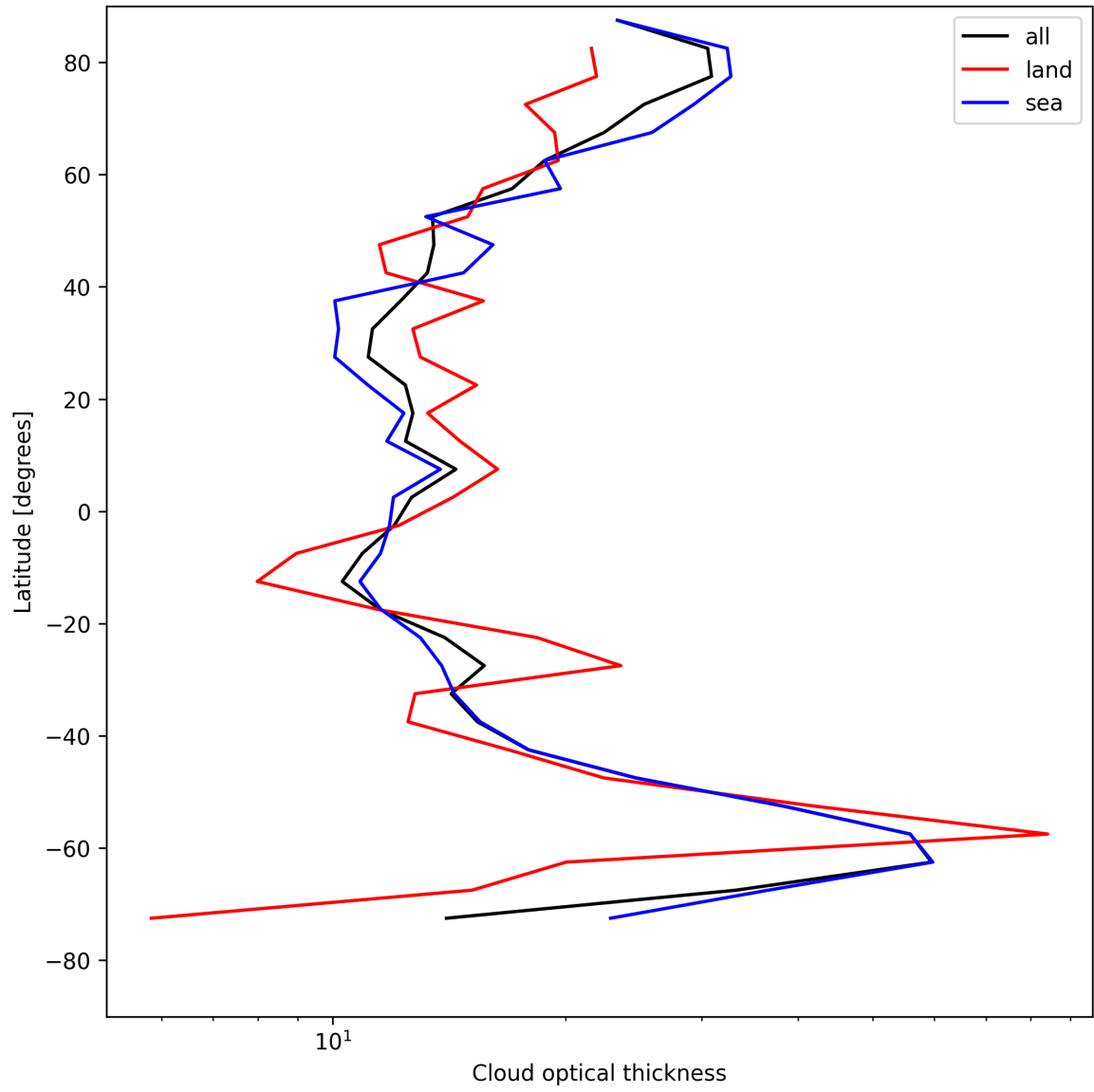
Figure 23: Zonal average of “Cloud optical thickness” for 2025-08-07 to 2025-08-07.
