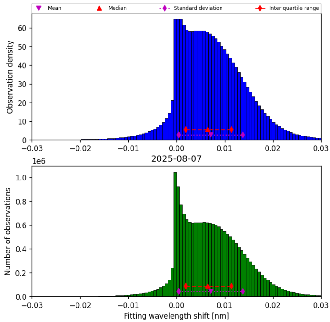
Figure 47: Histogram of “Fitting wavelength shift” for 2025-08-07 to 2025-08-07
