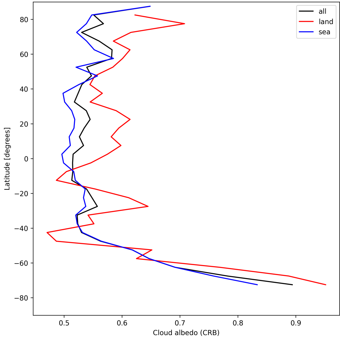
Figure 26: Zonal average of “Cloud albedo (CRB)” for 2025-08-07 to 2025-08-07.
