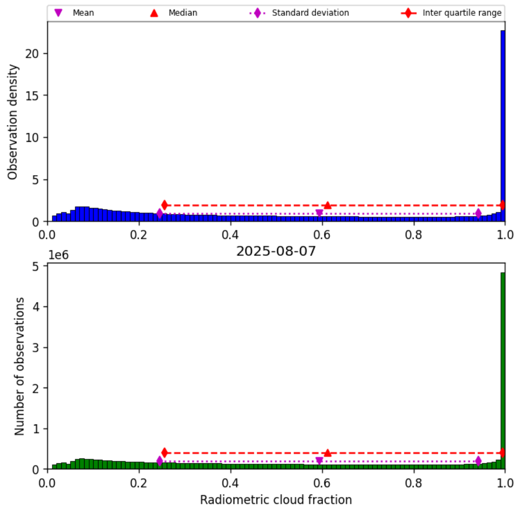
Figure 37: Histogram of “Radiometric cloud fraction” for 2025-08-07 to 2025-08-07
