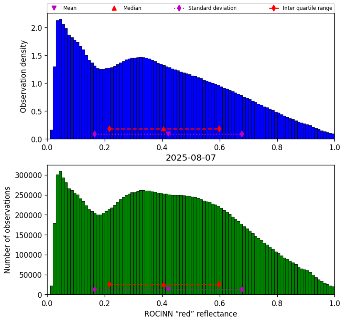
Figure 51: Histogram of “ROCINN “red” reflectance” for 2025-08-07 to 2025-08-07
