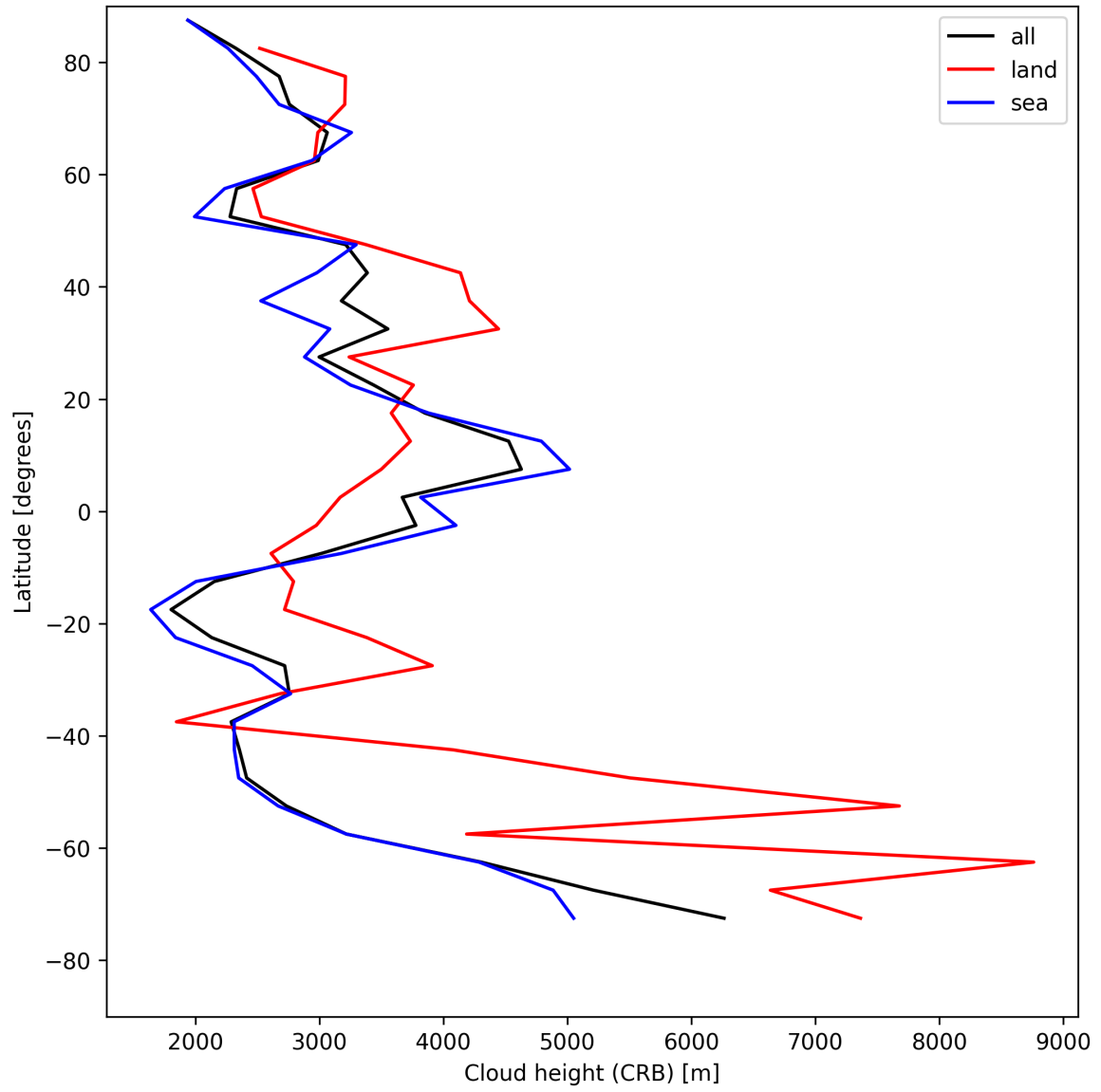
Figure 25: Zonal average of “Cloud height (CRB)” for 2025-08-07 to 2025-08-07.
