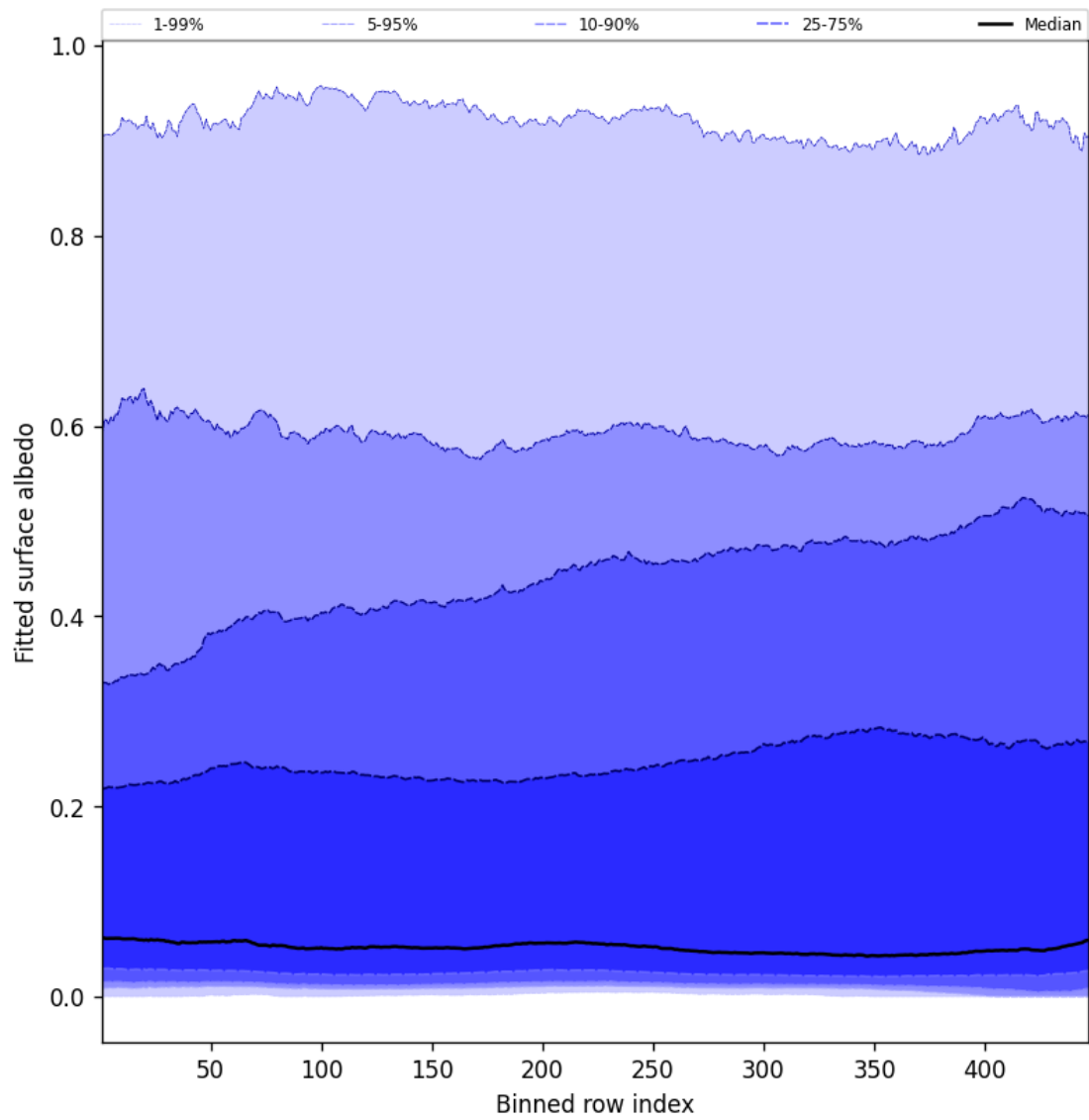
Figure 59: Along track statistics of “Fitted surface albedo” for 2025-08-07 to 2025-08-07
