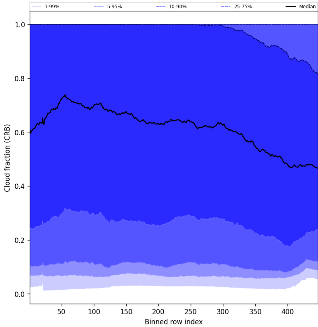
Figure 56: Along track statistics of “Cloud fraction (CRB)” for 2025-08-07 to 2025-08-07
