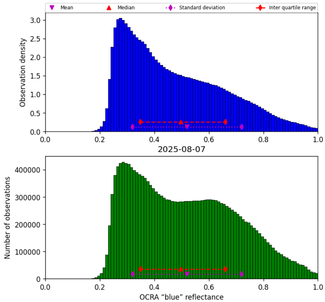
Figure 49: Histogram of “OCRA “blue” reflectance” for 2025-08-07 to 2025-08-07
