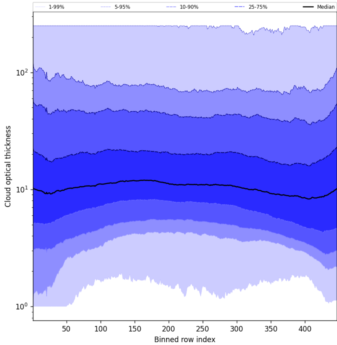
Figure 55: Along track statistics of “Cloud optical thickness” for 2025-08-07 to 2025-08-07
