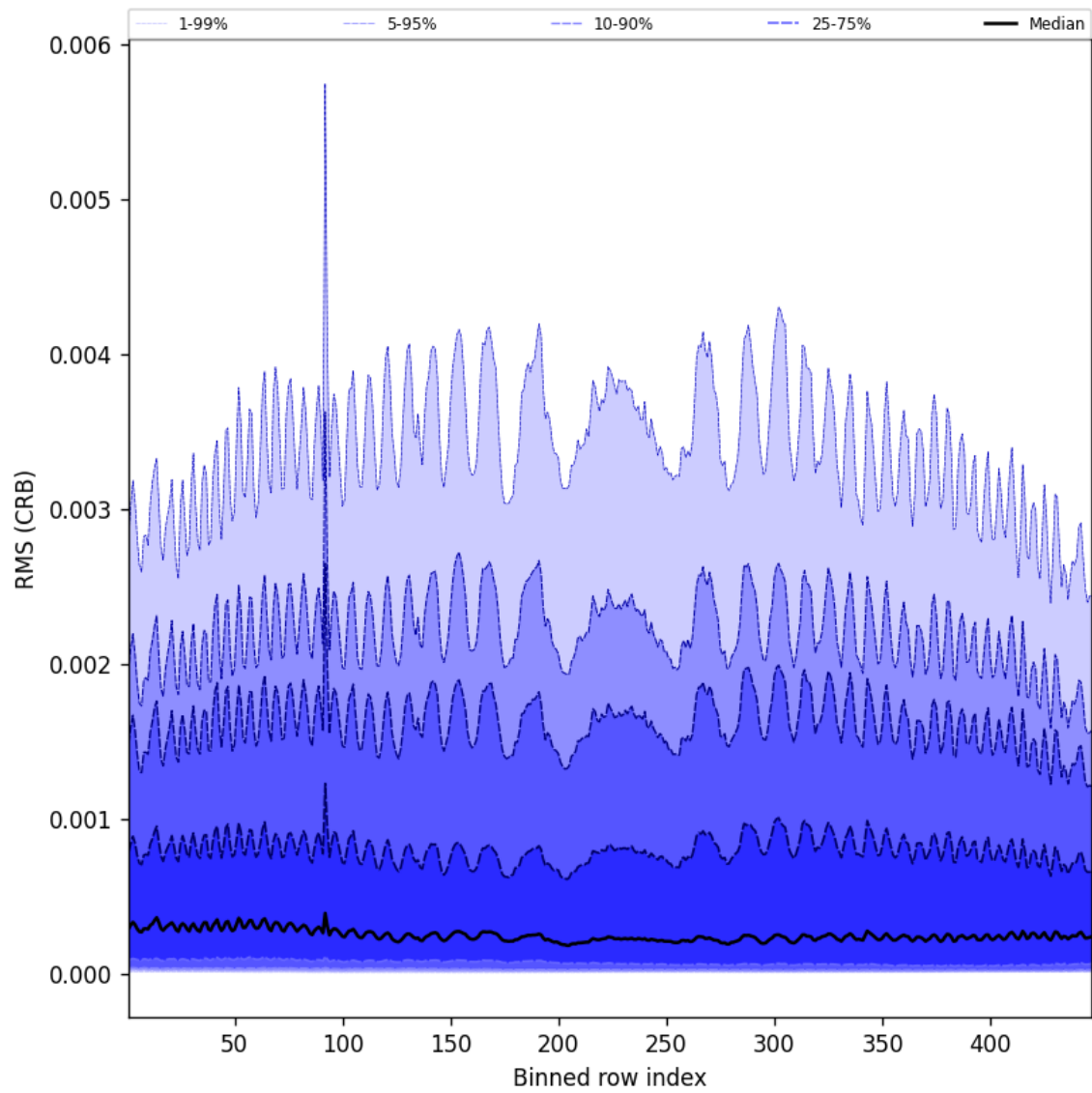
Figure 62: Along track statistics of “RMS (CRB)” for 2025-08-07 to 2025-08-07
