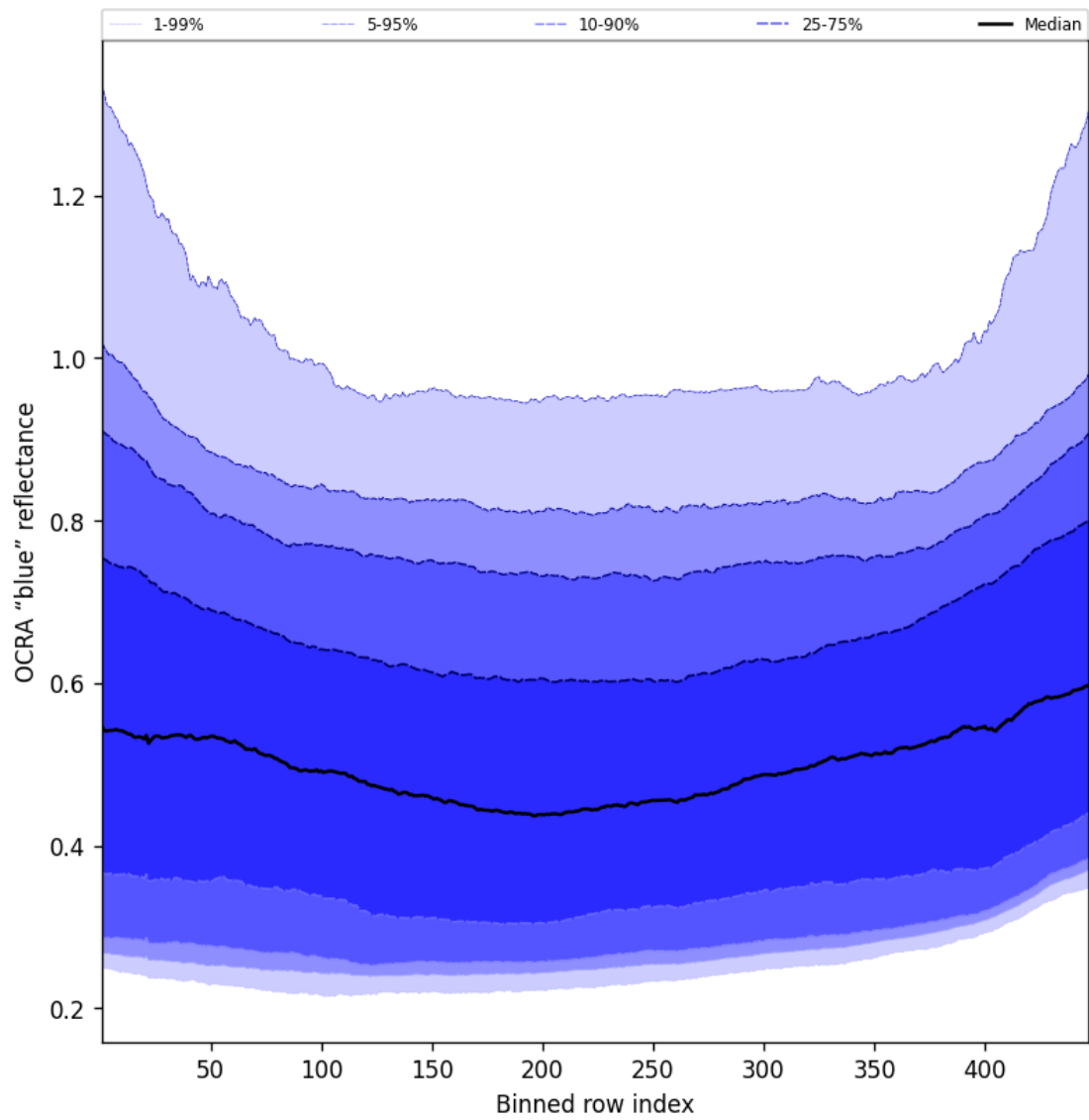
Figure 65: Along track statistics of “OCRA “blue” reflectance” for 2025-08-07 to 2025-08-07
