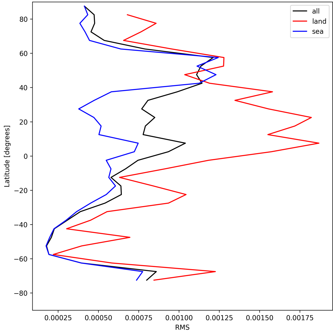
Figure 29: Zonal average of “RMS” for 2025-08-07 to 2025-08-07.
