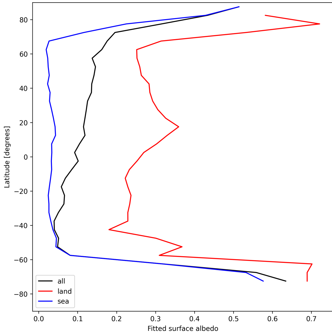
Figure 27: Zonal average of “Fitted surface albedo” for 2025-08-07 to 2025-08-07.
