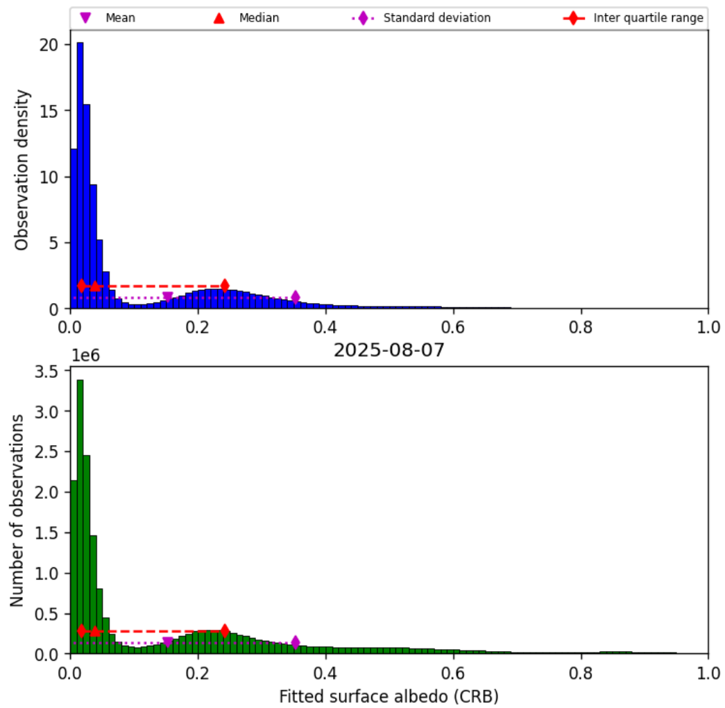
Figure 44: Histogram of “Fitted surface albedo (CRB)” for 2025-08-07 to 2025-08-07
