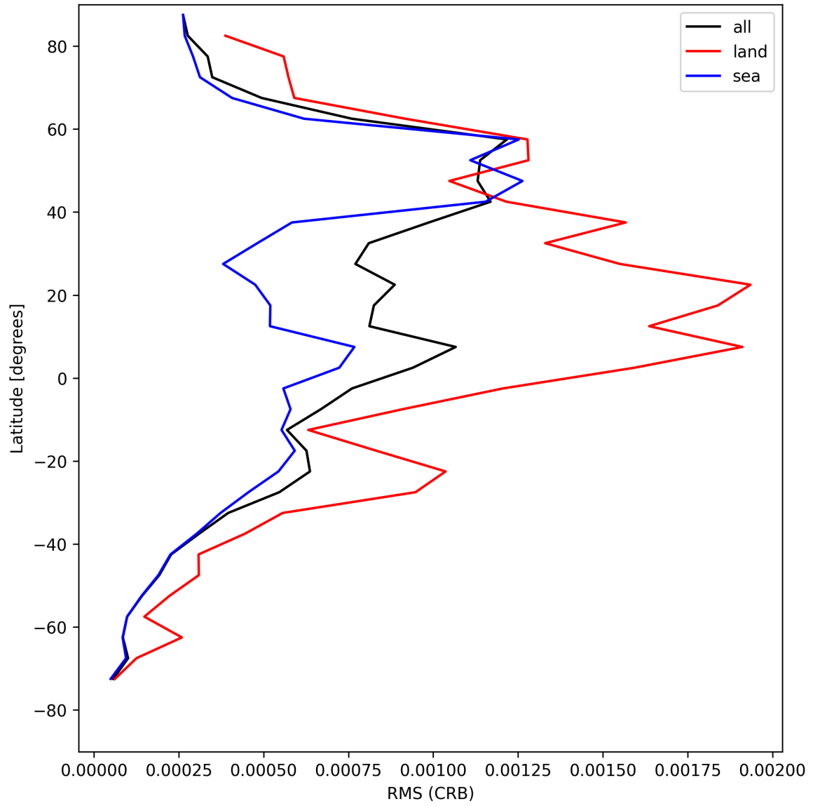
Figure 30: Zonal average of “RMS (CRB)” for 2025-08-07 to 2025-08-07.
