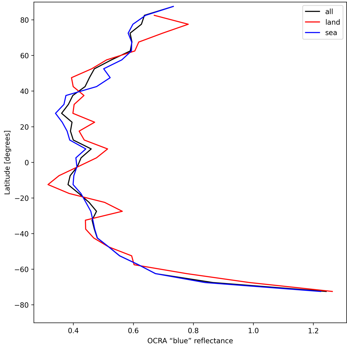
Figure 33: Zonal average of “OCRA “blue” reflectance” for 2025-08-07 to 2025-08-07.
