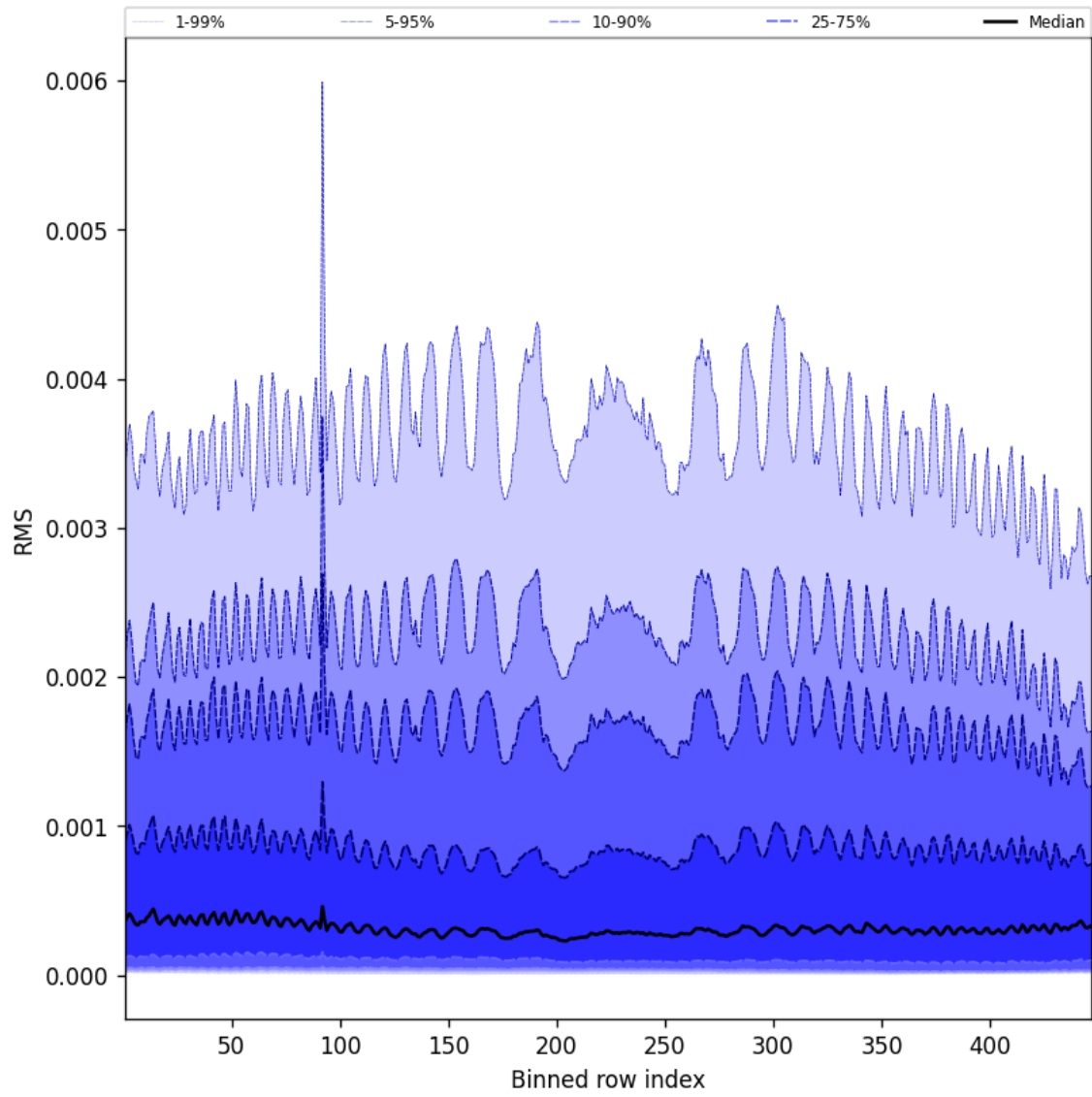
Figure 61: Along track statistics of “RMS” for 2025-08-07 to 2025-08-07
