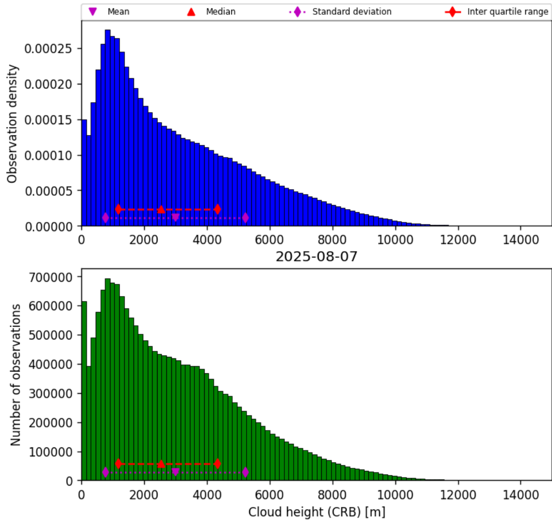
Figure 41: Histogram of “Cloud height (CRB)” for 2025-08-07 to 2025-08-07
