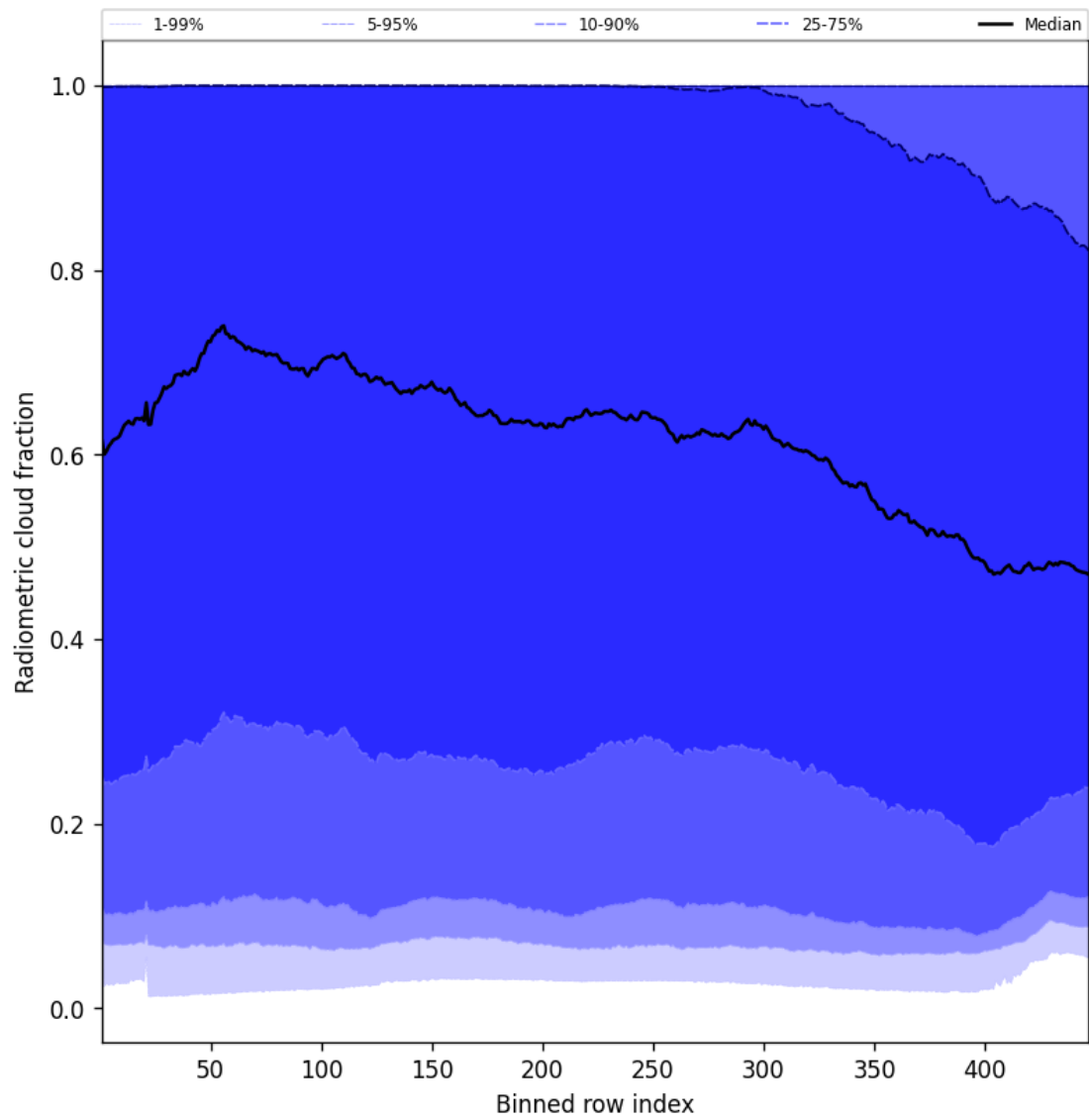
Figure 53: Along track statistics of “Radiometric cloud fraction” for 2025-08-07 to 2025-08-07
