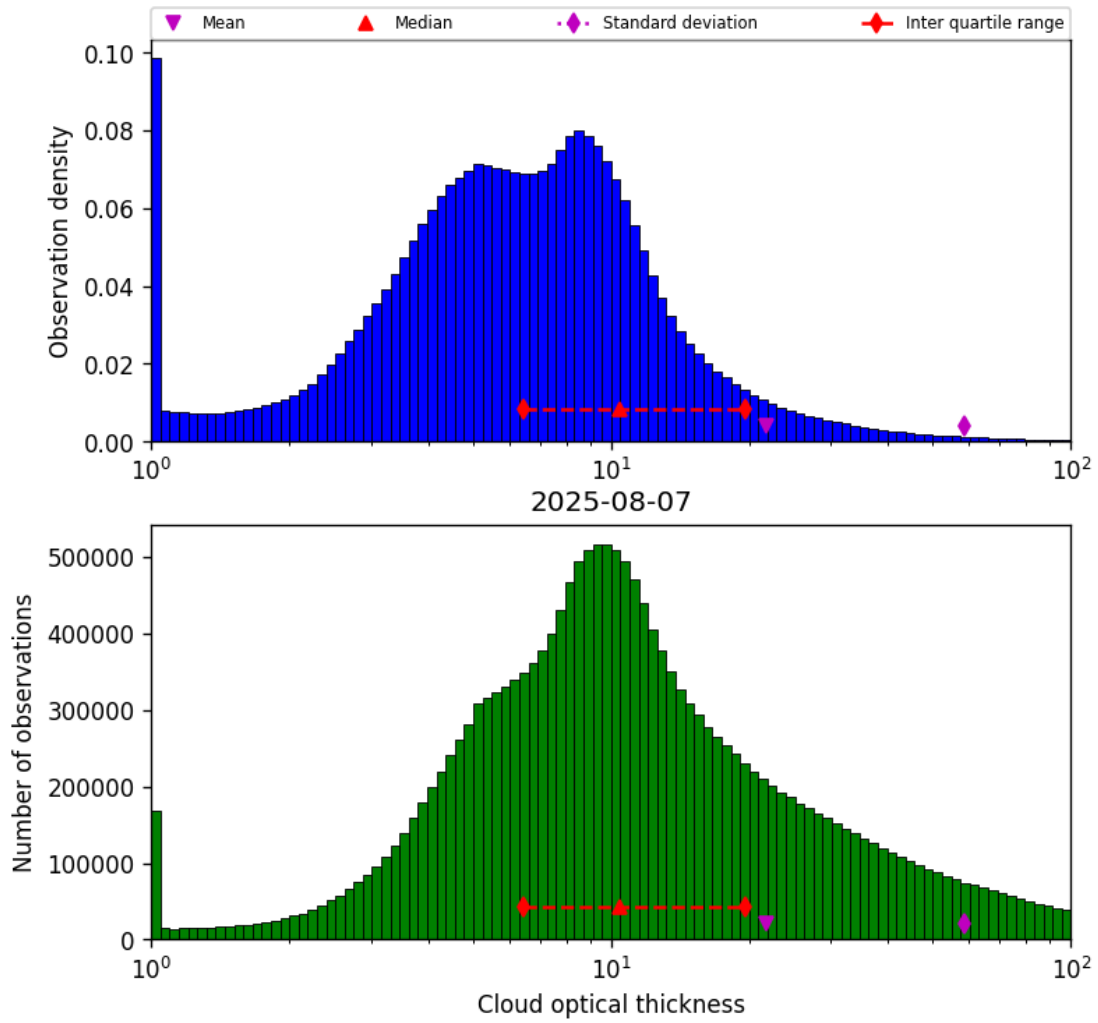
Figure 39: Histogram of “Cloud optical thickness” for 2025-08-07 to 2025-08-07
