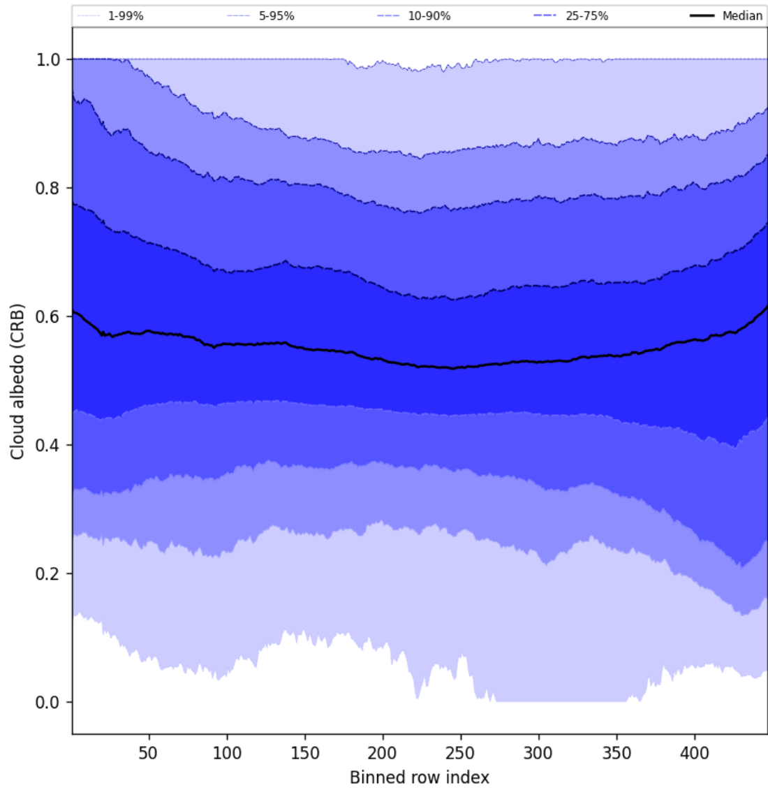
Figure 58: Along track statistics of “Cloud albedo (CRB)” for 2025-08-07 to 2025-08-07
