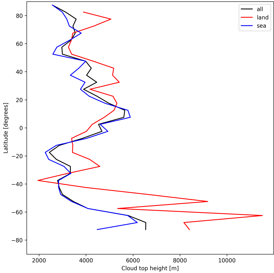
Figure 22: Zonal average of “Cloud top height” for 2025-08-07 to 2025-08-07.
