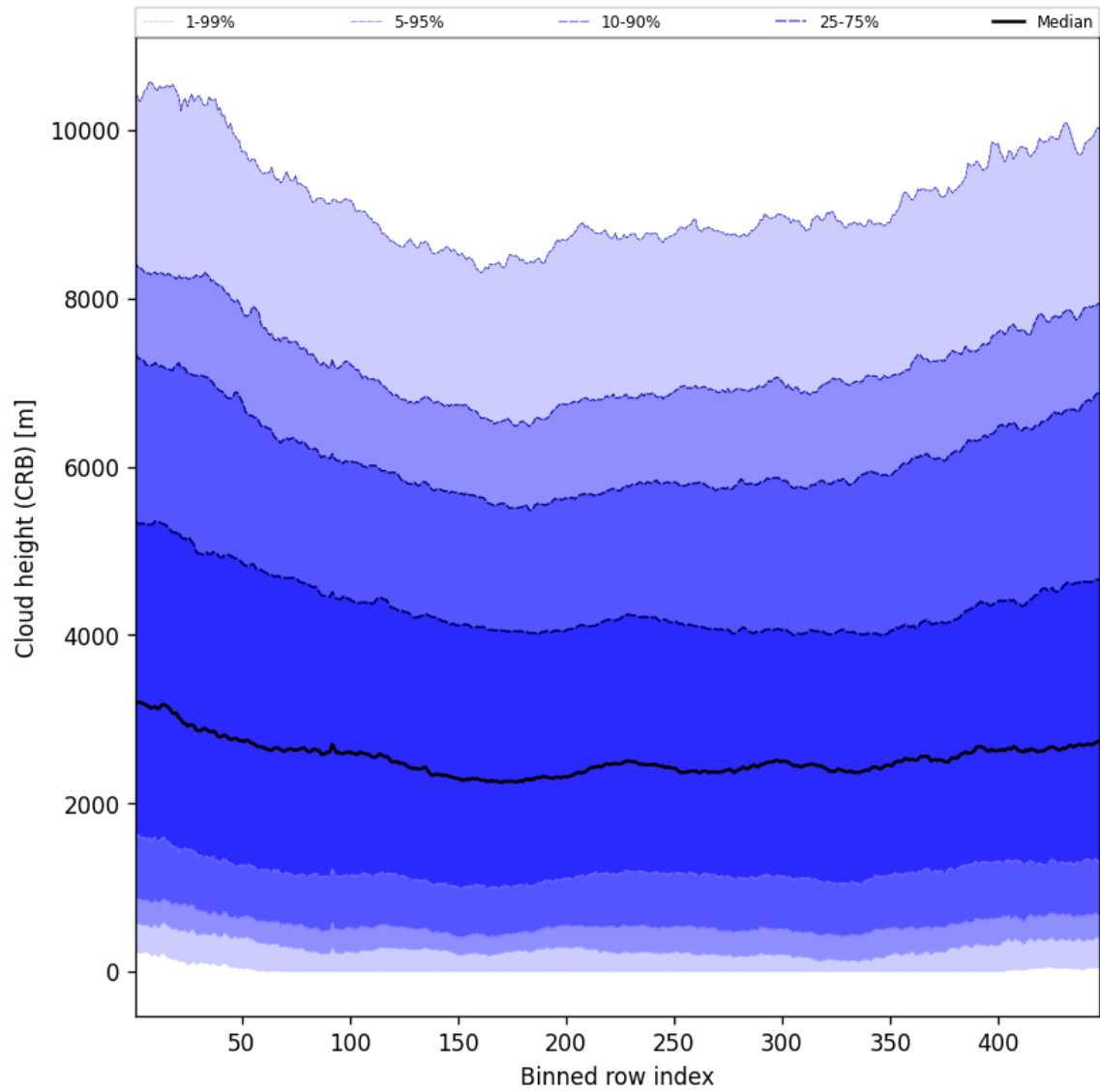
Figure 57: Along track statistics of “Cloud height (CRB)” for 2025-08-07 to 2025-08-07
