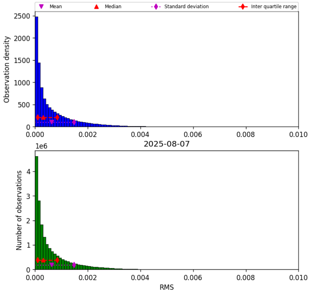
Figure 45: Histogram of “RMS” for 2025-08-07 to 2025-08-07
