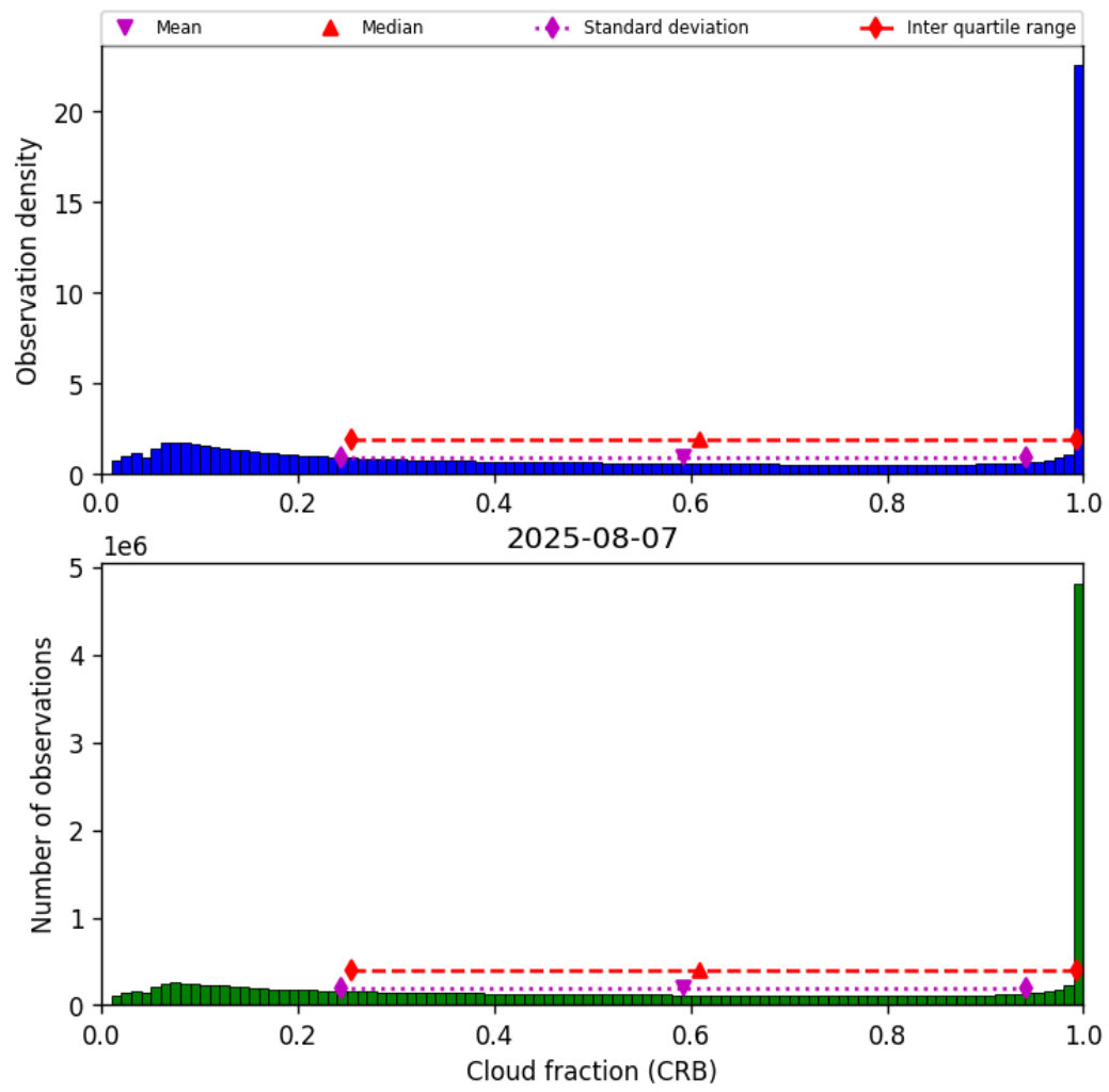
Figure 40: Histogram of “Cloud fraction (CRB)” for 2025-08-07 to 2025-08-07
