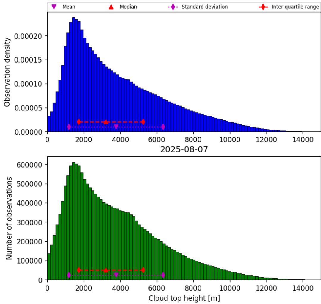
Figure 38: Histogram of “Cloud top height” for 2025-08-07 to 2025-08-07
