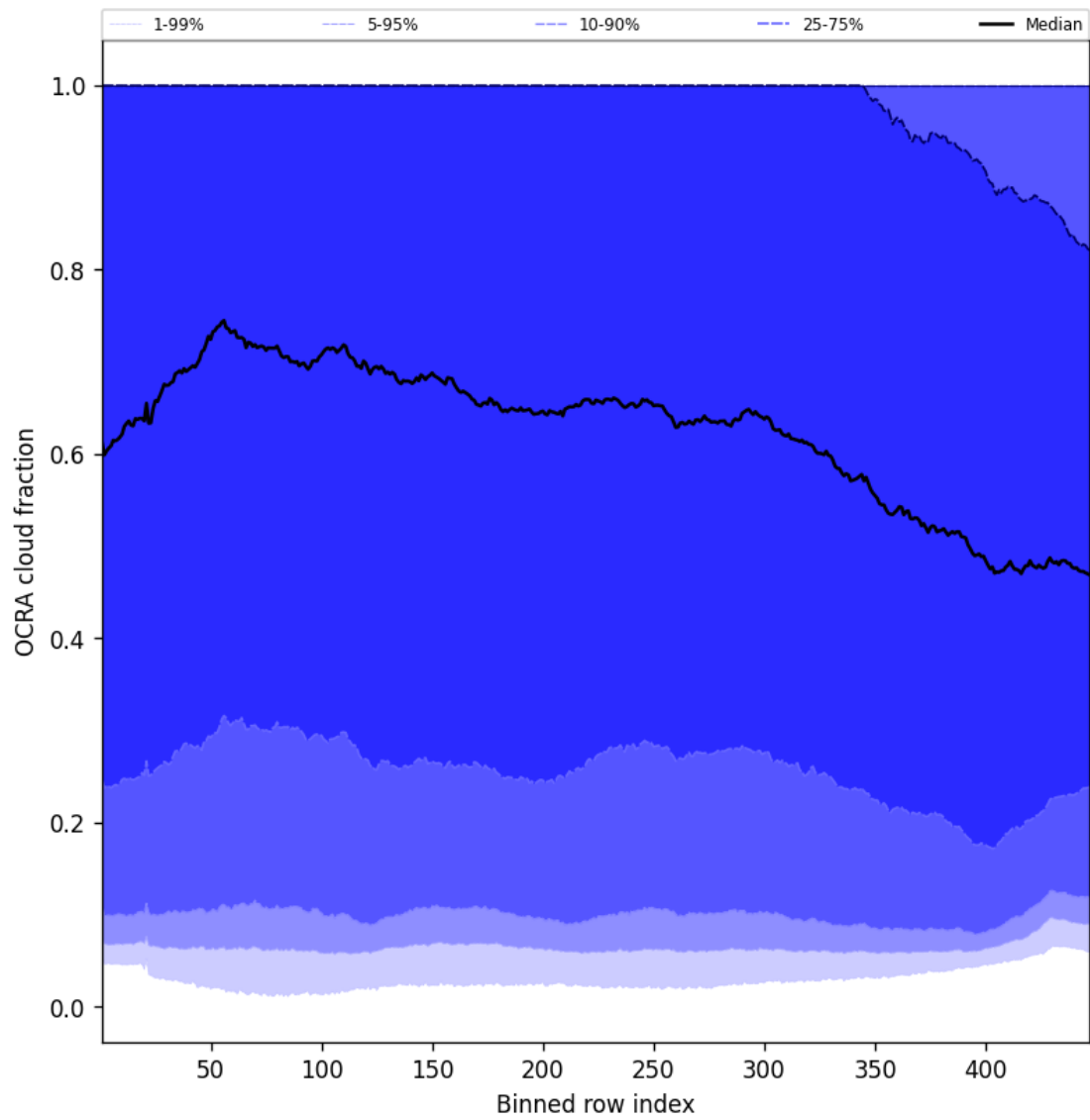
Figure 64: Along track statistics of “OCRA cloud fraction” for 2025-08-07 to 2025-08-07
