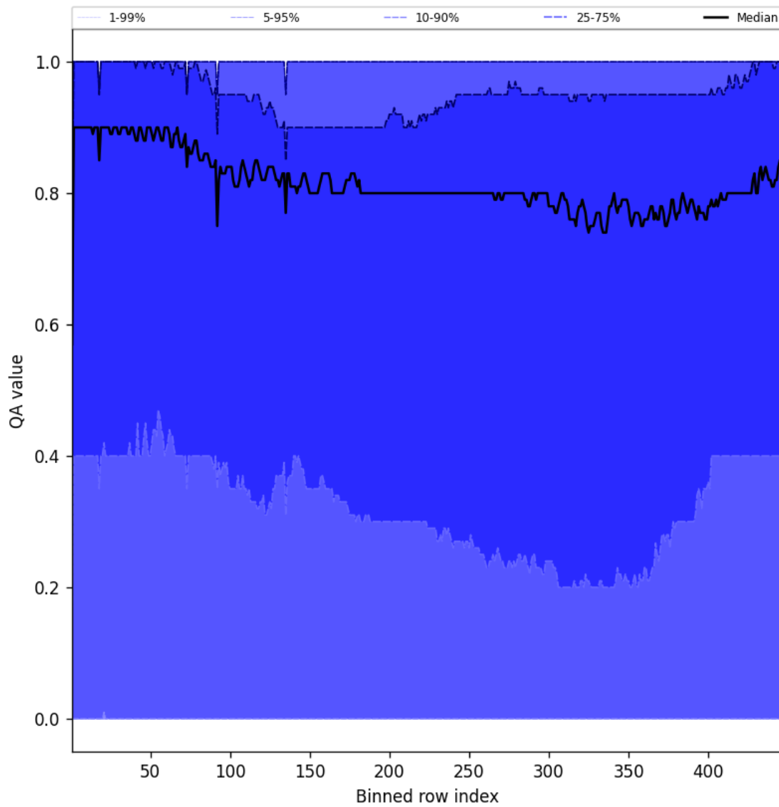
Figure 52: Along track statistics of “QA value” for 2025-08-07 to 2025-08-07
