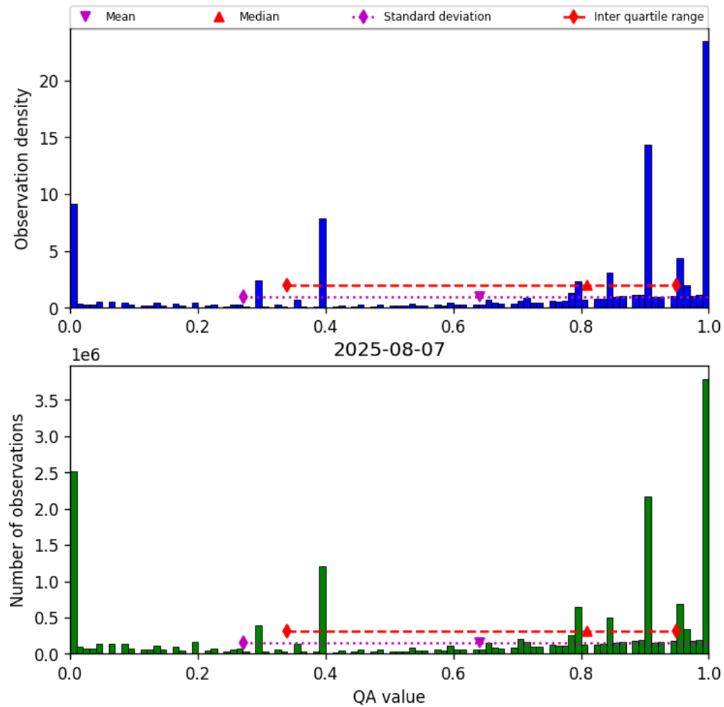
Figure 36: Histogram of “QA value” for 2025-08-07 to 2025-08-07
