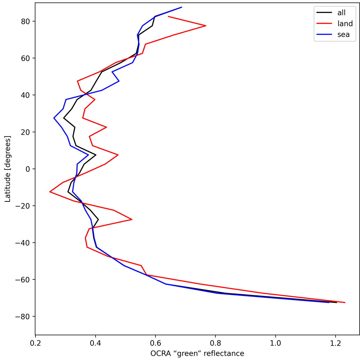
Figure 34: Zonal average of “OCRA “green” reflectance” for 2025-08-07 to 2025-08-07.
