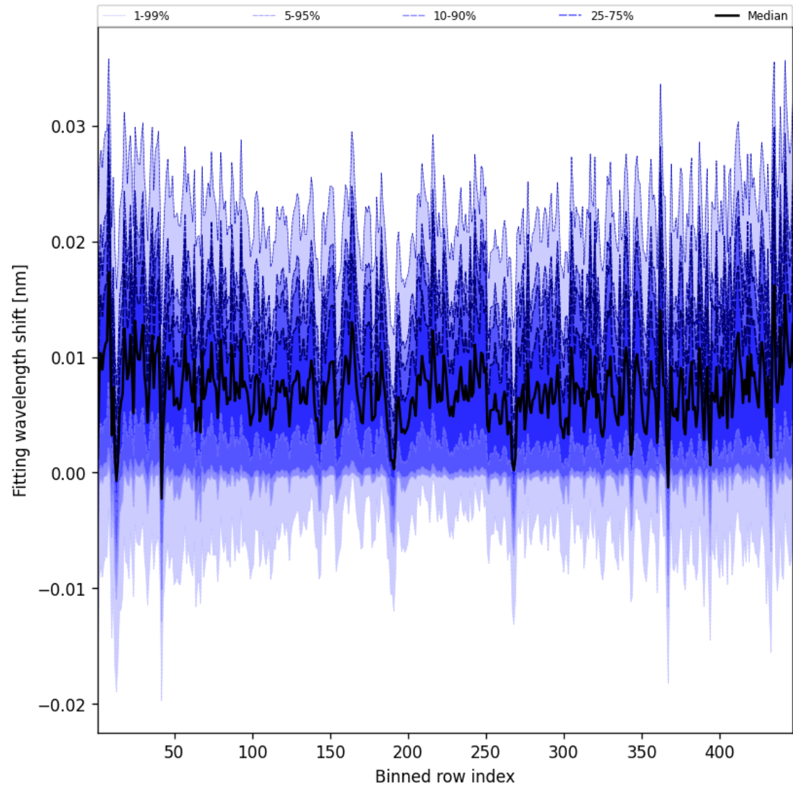
Figure 63: Along track statistics of “Fitting wavelength shift” for 2025-08-07 to 2025-08-07
