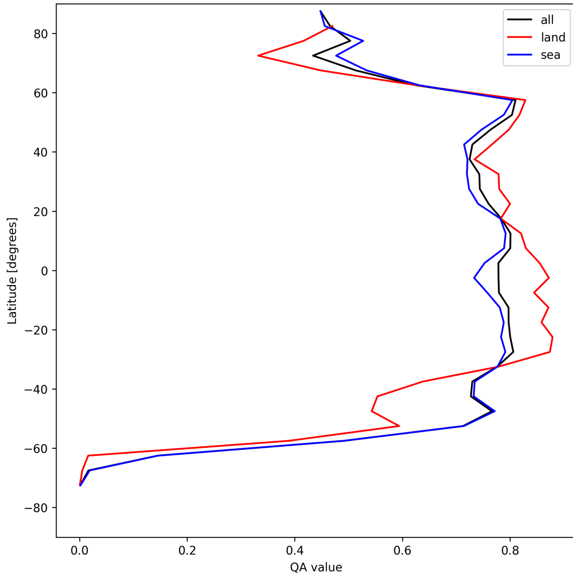
Figure 20: Zonal average of “QA value” for 2025-08-07 to 2025-08-07.
