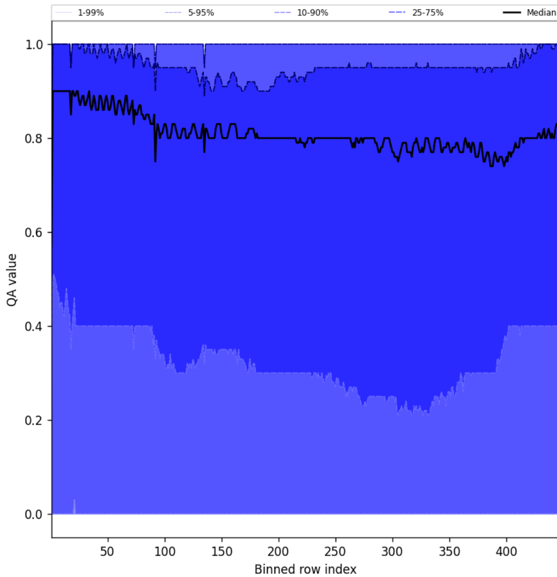
Figure 52: Along track statistics of “QA value” for 2025-08-12 to 2025-08-12
