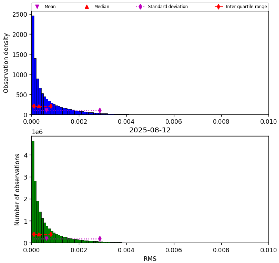
Figure 45: Histogram of “RMS” for 2025-08-12 to 2025-08-12
