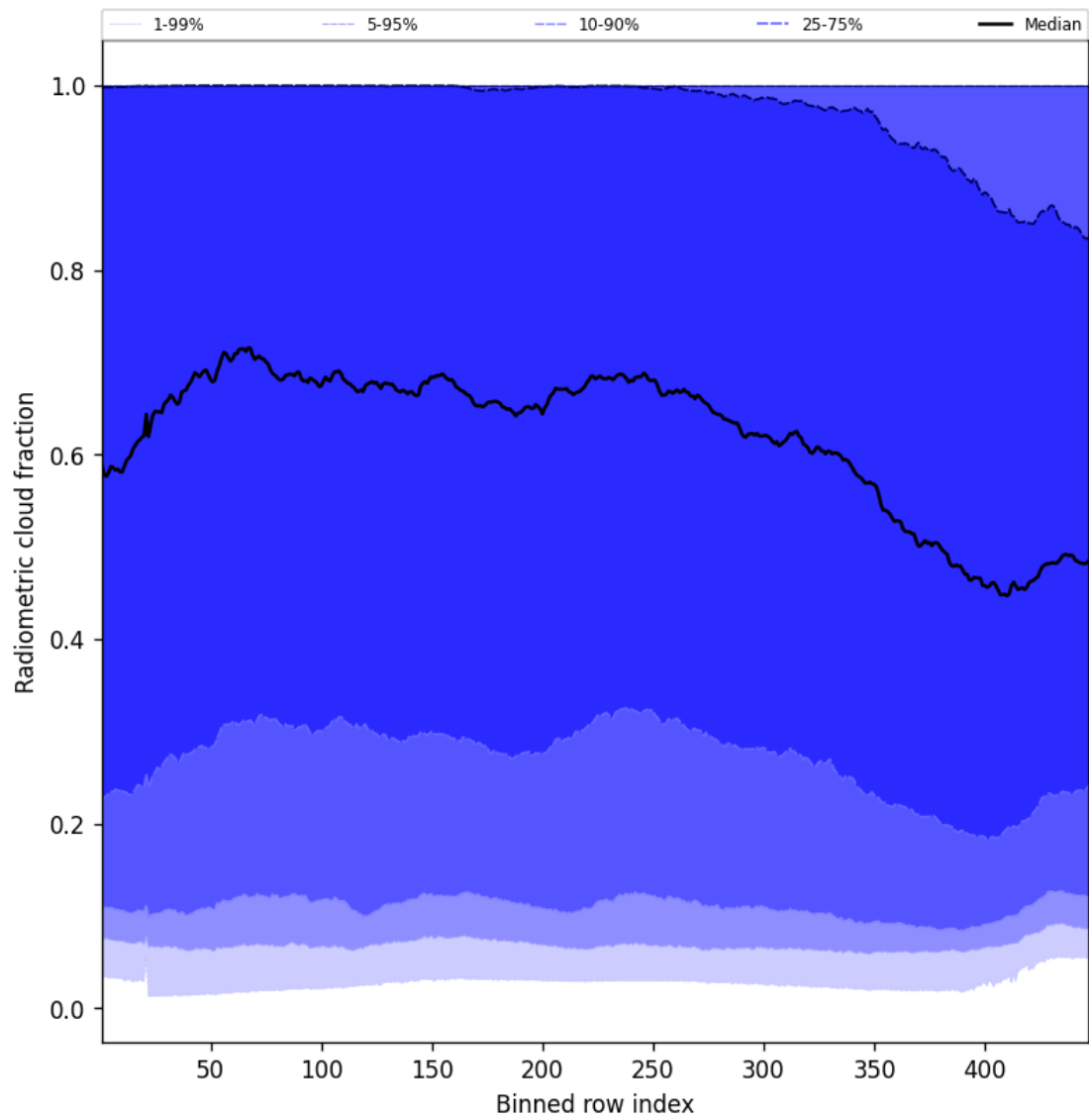
Figure 53: Along track statistics of “Radiometric cloud fraction” for 2025-08-12 to 2025-08-12
