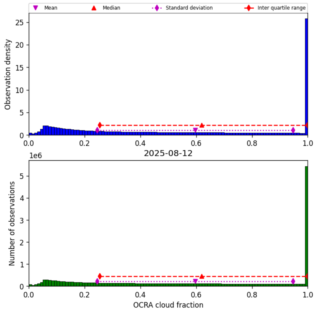
Figure 48: Histogram of “OCRA cloud fraction” for 2025-08-12 to 2025-08-12
