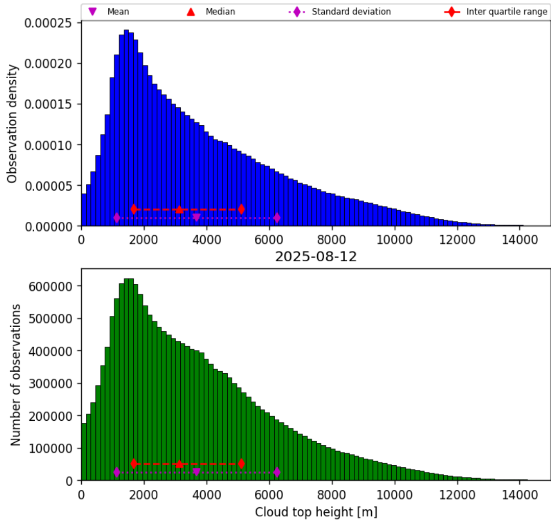
Figure 38: Histogram of “Cloud top height” for 2025-08-12 to 2025-08-12
