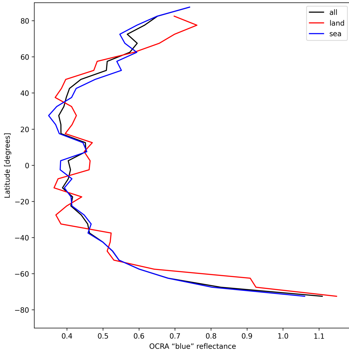
Figure 33: Zonal average of “OCRA “blue” reflectance” for 2025-08-12 to 2025-08-12.
