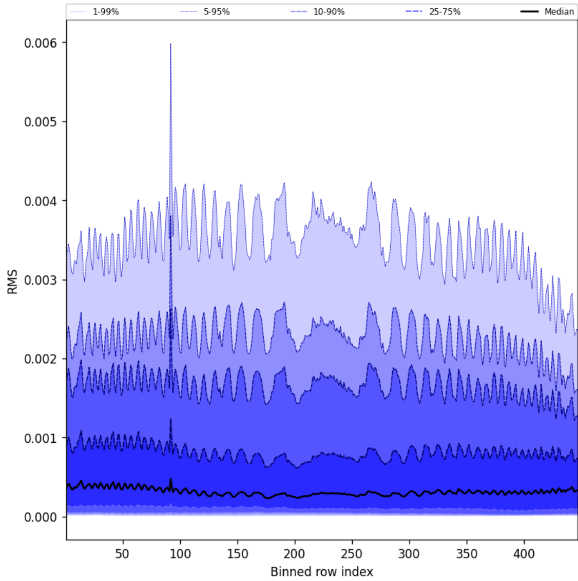
Figure 61: Along track statistics of “RMS” for 2025-08-12 to 2025-08-12
