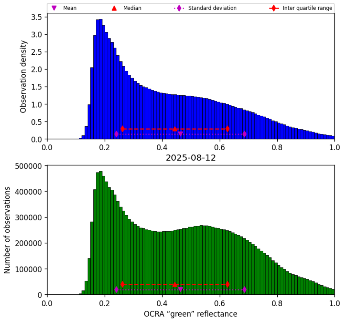
Figure 50: Histogram of “OCRA “green” reflectance” for 2025-08-12 to 2025-08-12
