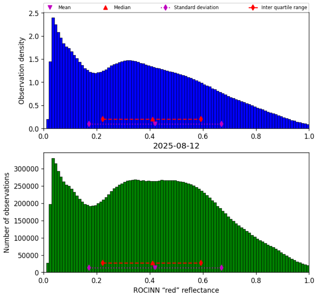
Figure 51: Histogram of “ROCINN “red” reflectance” for 2025-08-12 to 2025-08-12
