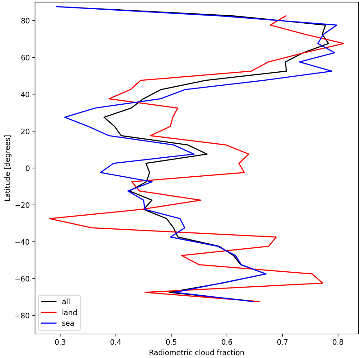
Figure 21: Zonal average of “Radiometric cloud fraction” for 2025-08-12 to 2025-08-12.
