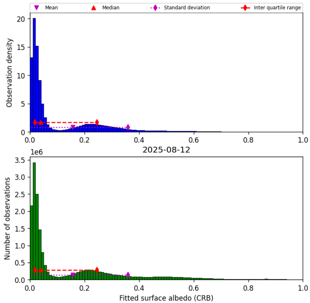
Figure 44: Histogram of “Fitted surface albedo (CRB)” for 2025-08-12 to 2025-08-12
