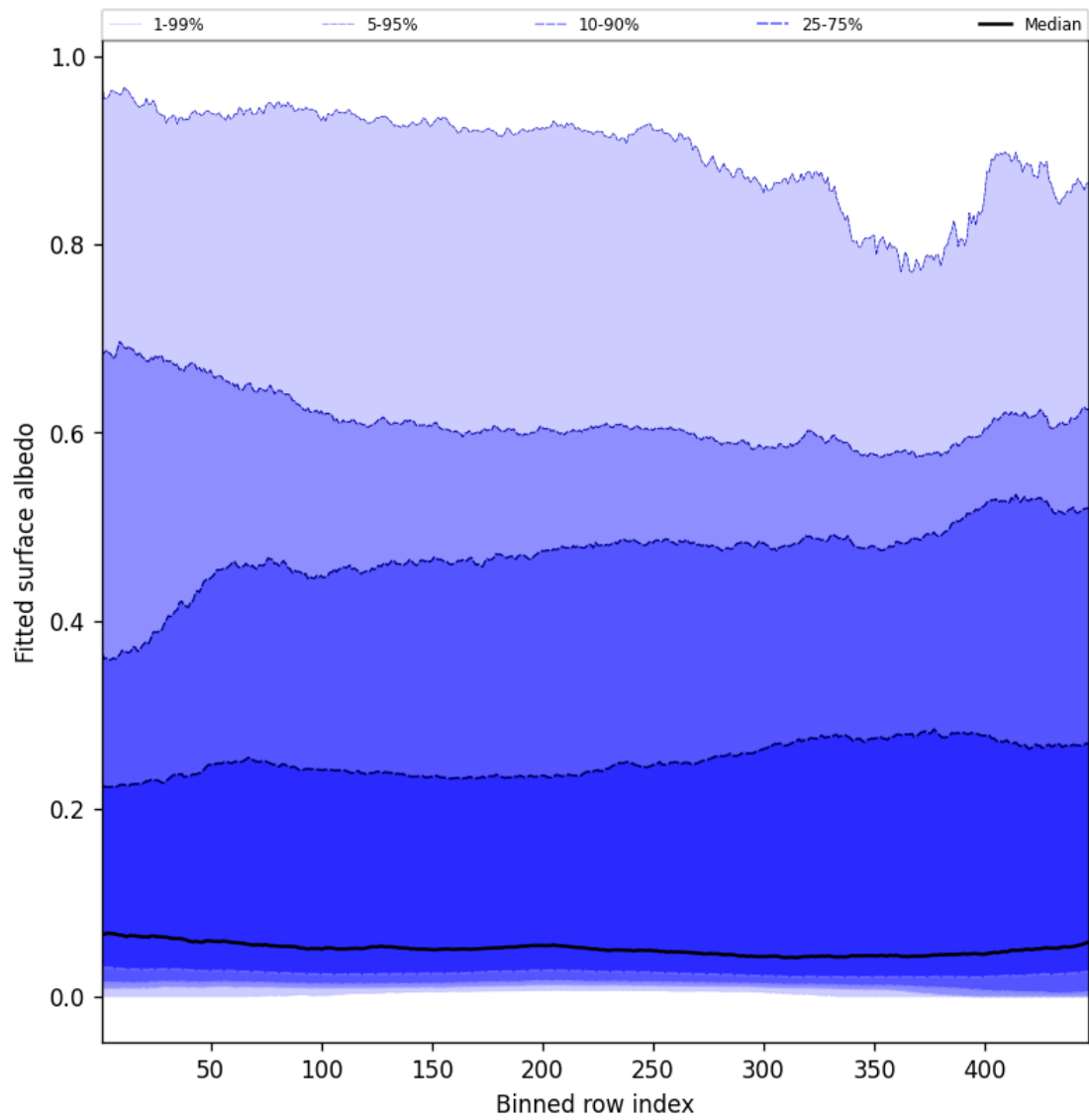
Figure 59: Along track statistics of “Fitted surface albedo” for 2025-08-12 to 2025-08-12
