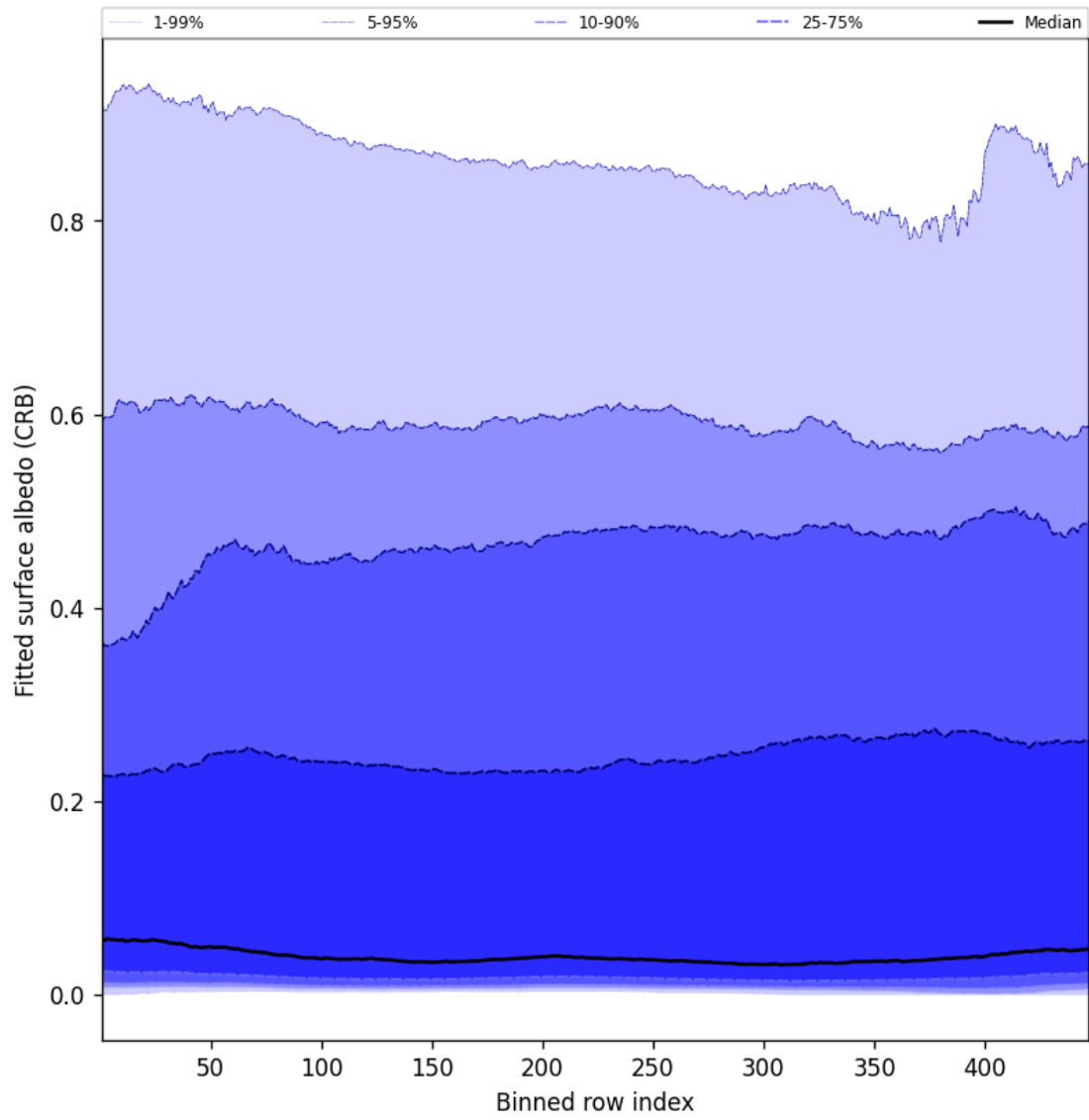
Figure 60: Along track statistics of “Fitted surface albedo (CRB)” for 2025-08-12 to 2025-08-12
