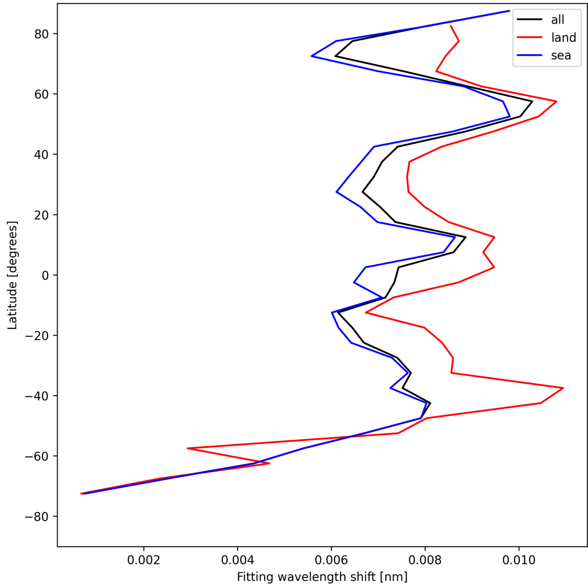
Figure 31: Zonal average of “Fitting wavelength shift” for 2025-08-12 to 2025-08-12.
