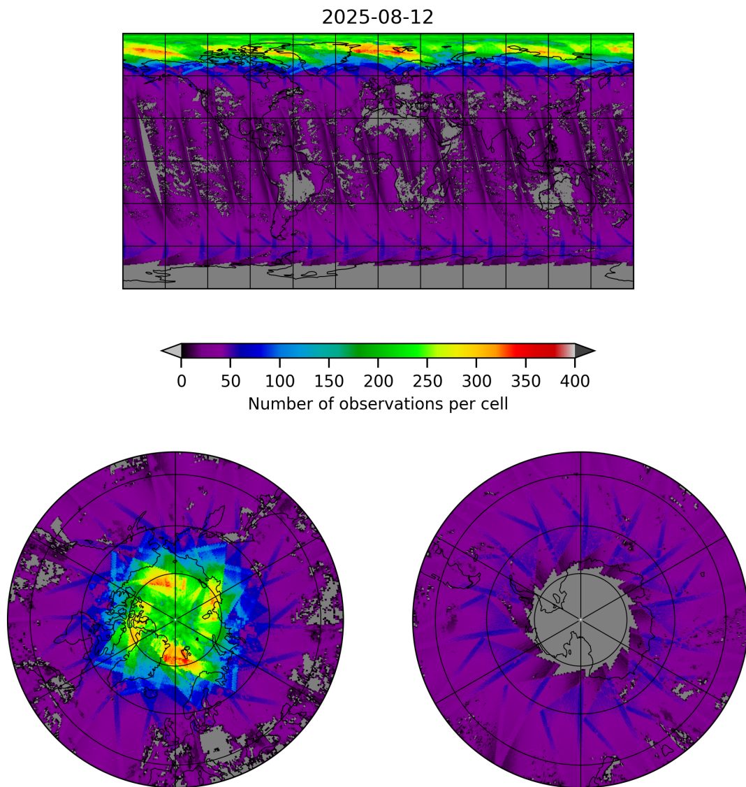
Figure 19: Map of the number of observations for 2025-08-12 to 2025-08-12
