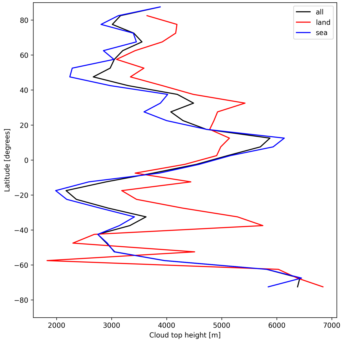
Figure 22: Zonal average of “Cloud top height” for 2025-08-12 to 2025-08-12.
