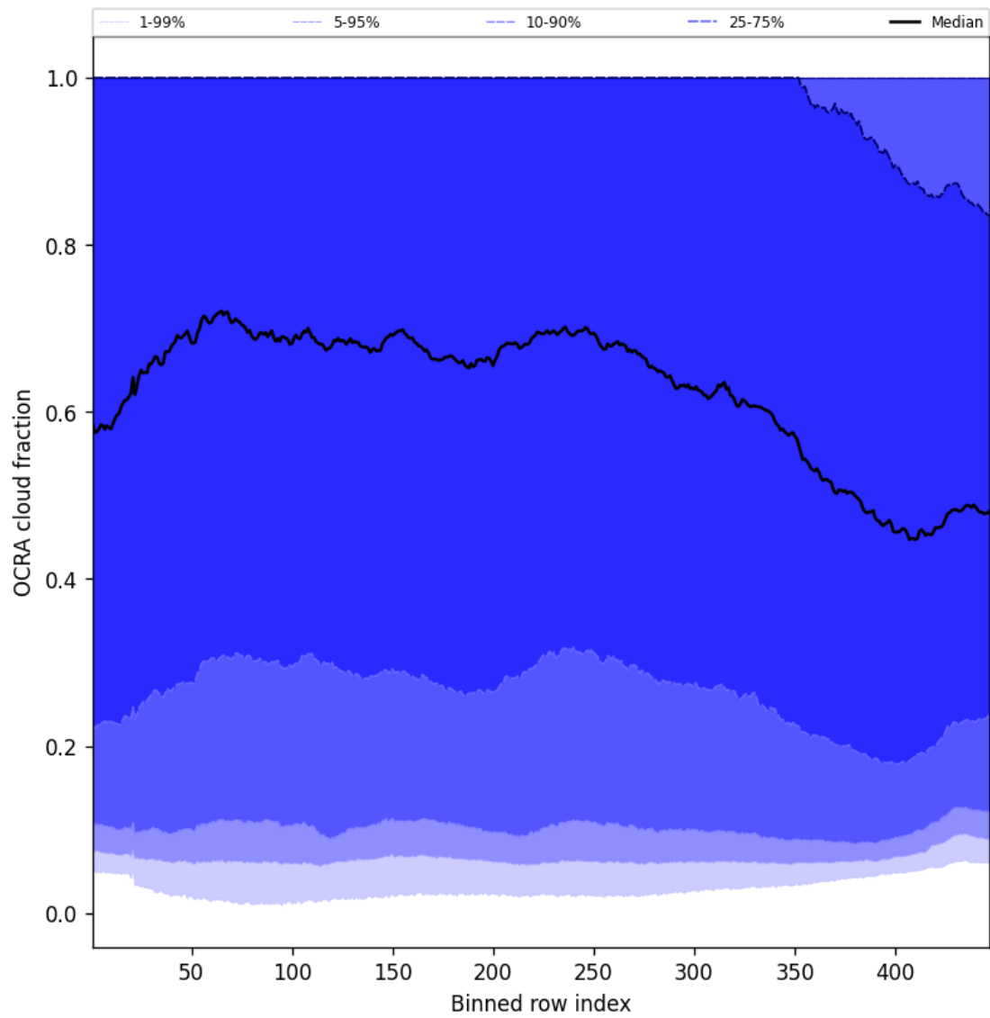
Figure 64: Along track statistics of “OCRA cloud fraction” for 2025-08-12 to 2025-08-12
