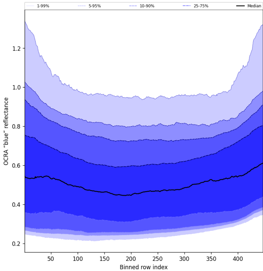
Figure 65: Along track statistics of “OCRA “blue” reflectance” for 2025-08-12 to 2025-08-12
