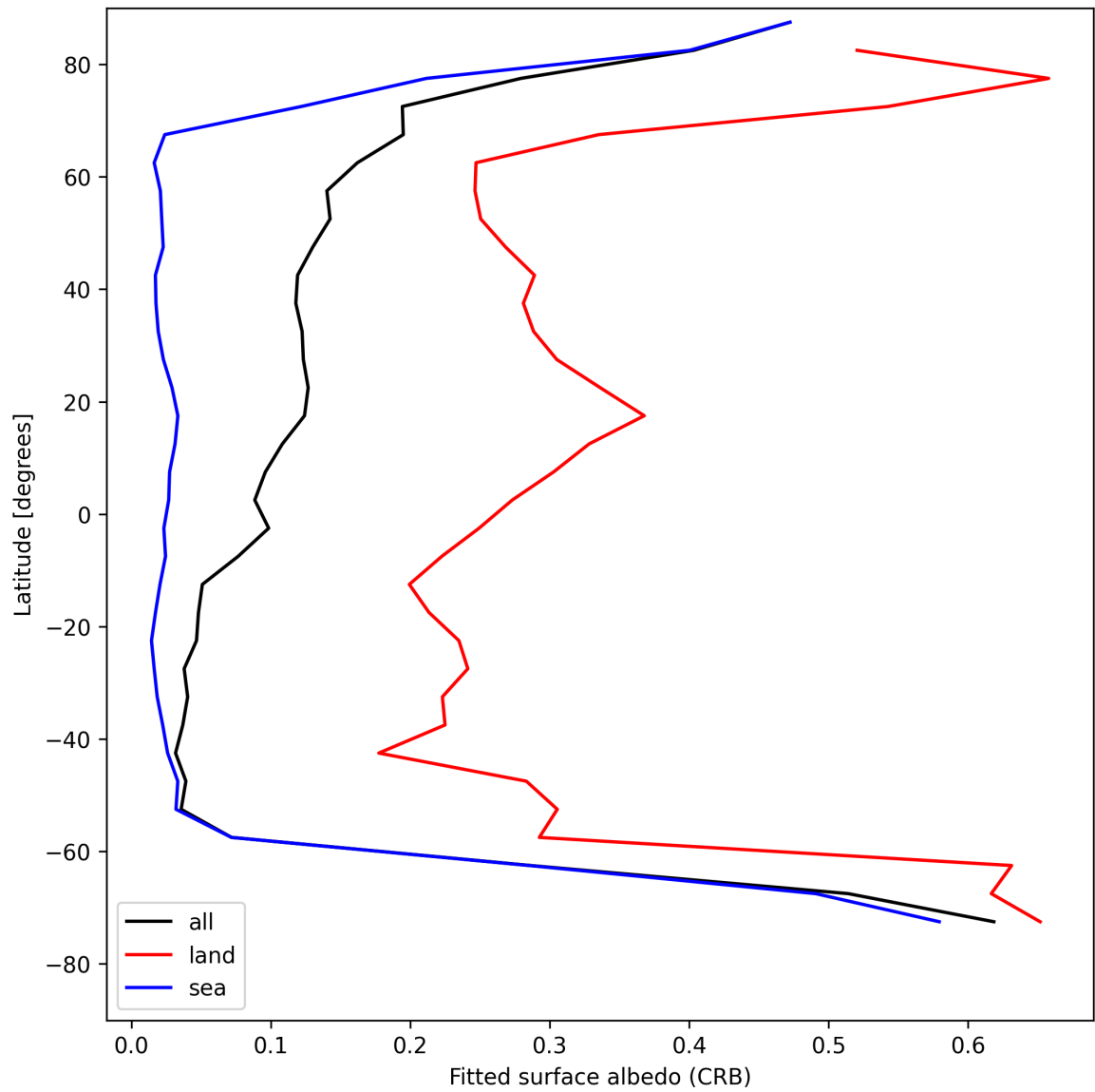
Figure 28: Zonal average of “Fitted surface albedo (CRB)” for 2025-08-12 to 2025-08-12.
