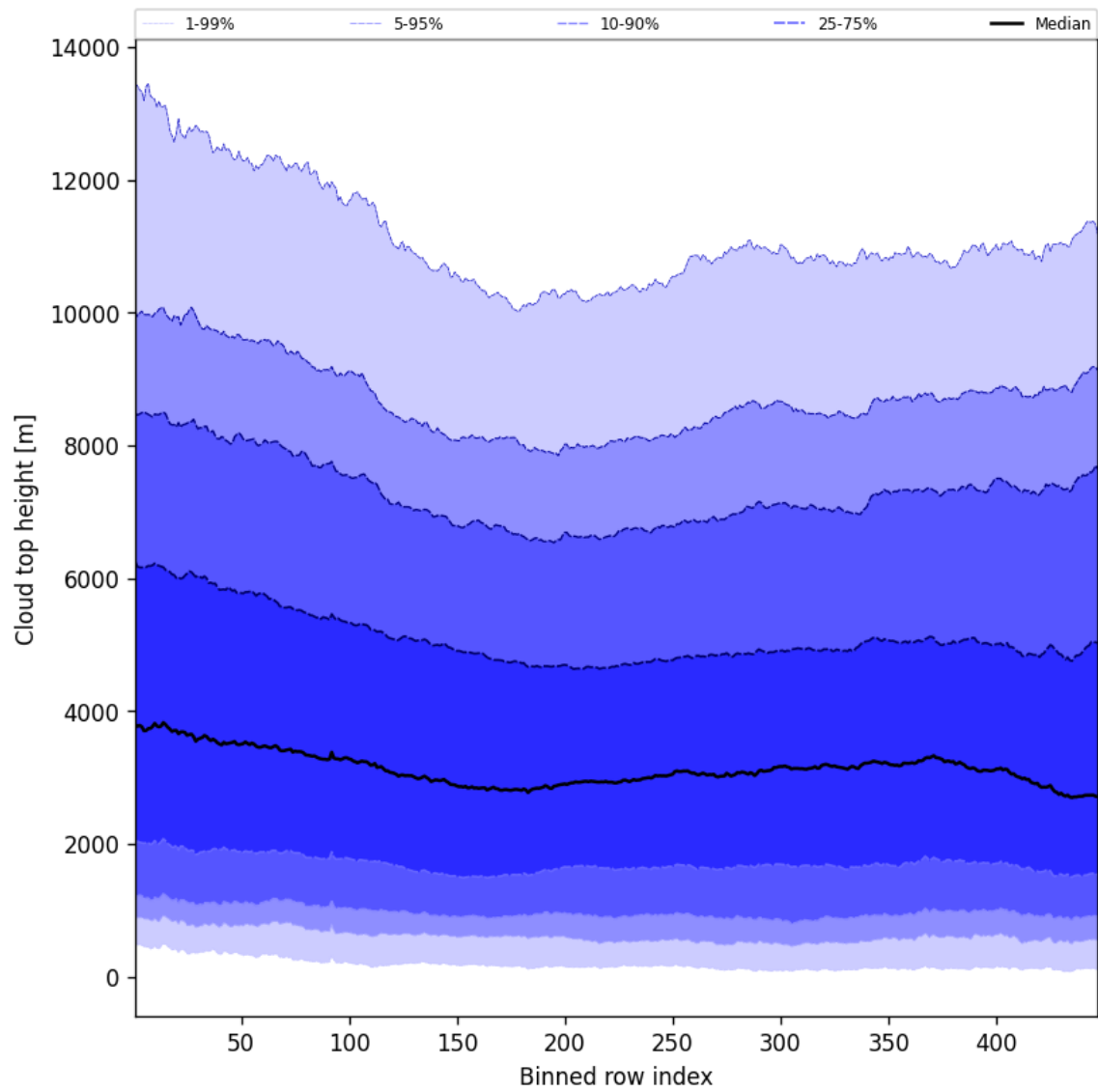
Figure 54: Along track statistics of “Cloud top height” for 2025-08-12 to 2025-08-12
