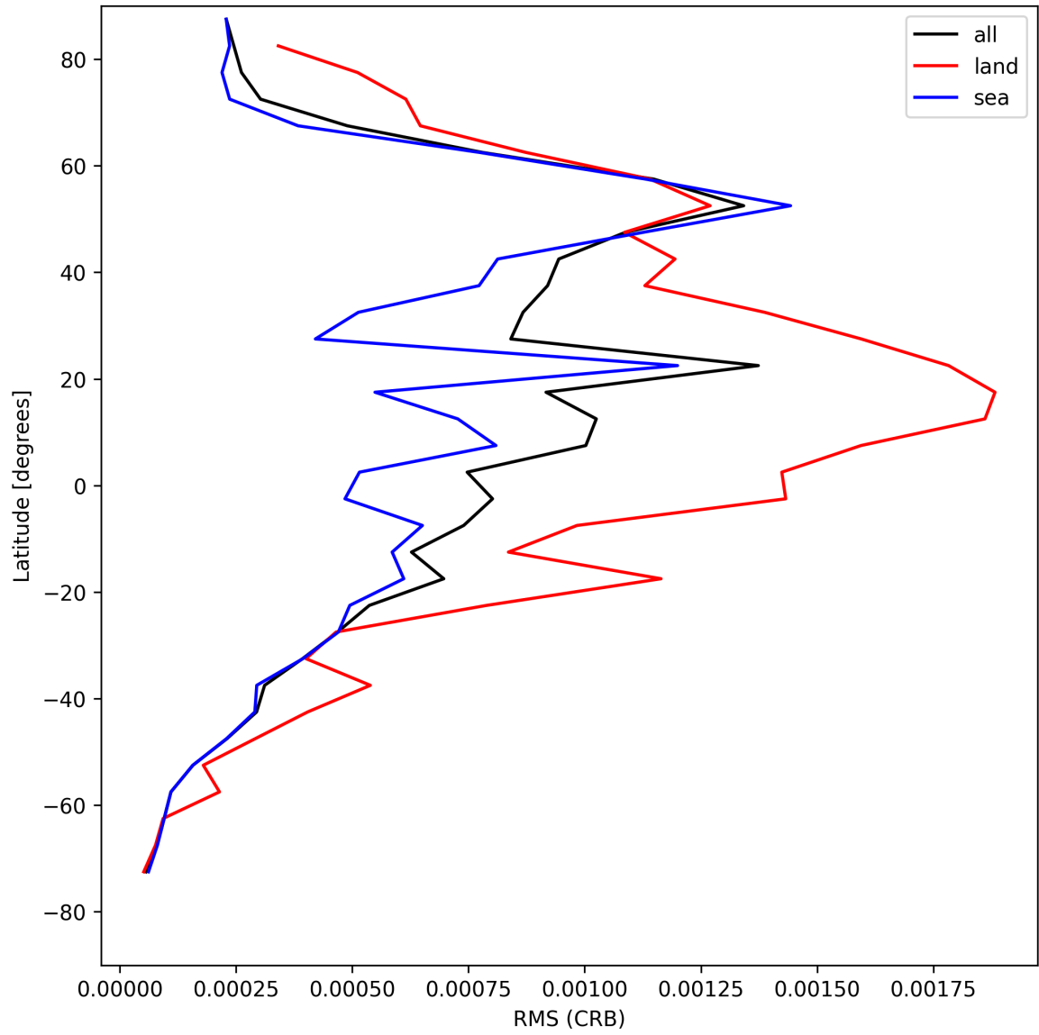
Figure 30: Zonal average of “RMS (CRB)” for 2025-08-12 to 2025-08-12.
