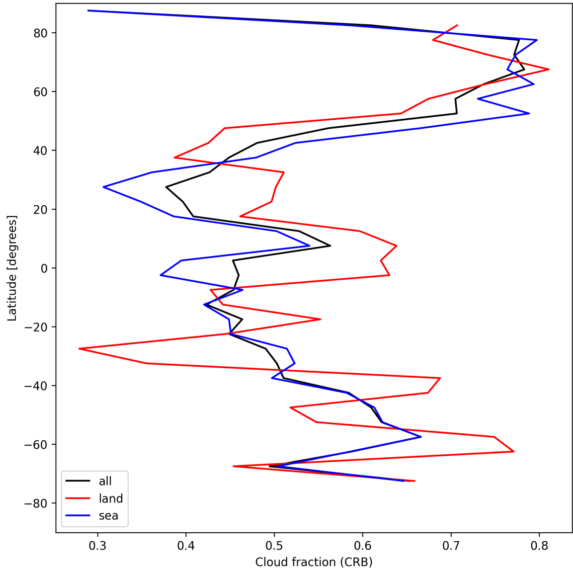
Figure 24: Zonal average of “Cloud fraction (CRB)” for 2025-08-12 to 2025-08-12.
