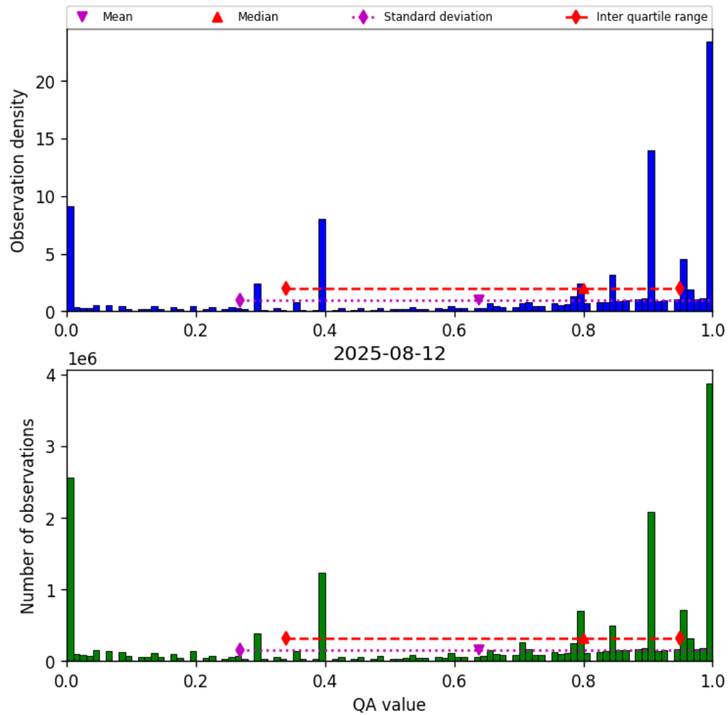
Figure 36: Histogram of “QA value” for 2025-08-12 to 2025-08-12
