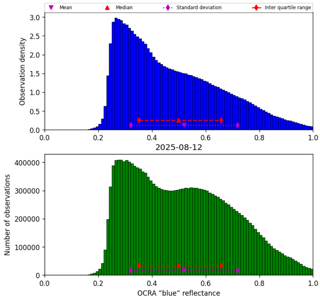
Figure 49: Histogram of “OCRA “blue” reflectance” for 2025-08-12 to 2025-08-12
