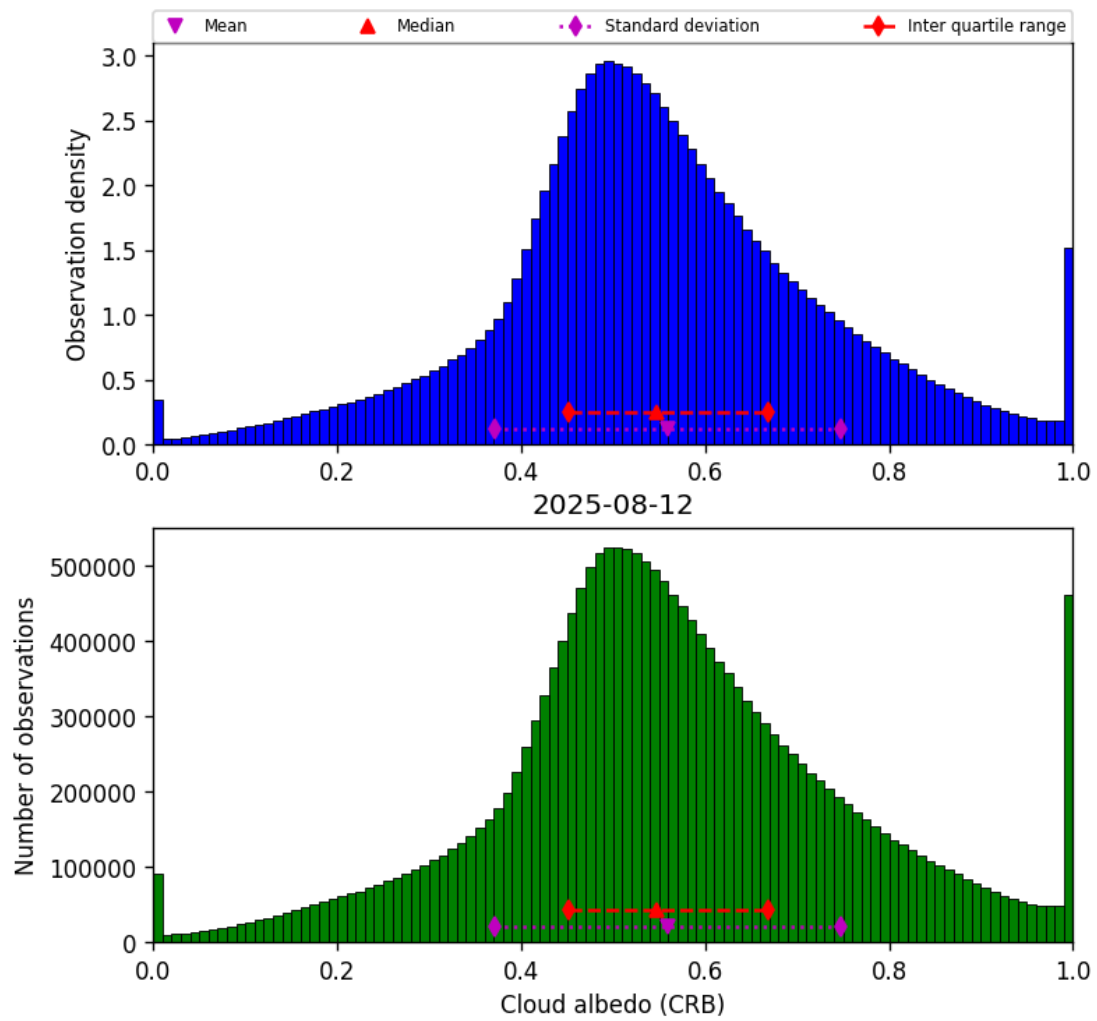
Figure 42: Histogram of “Cloud albedo (CRB)” for 2025-08-12 to 2025-08-12
