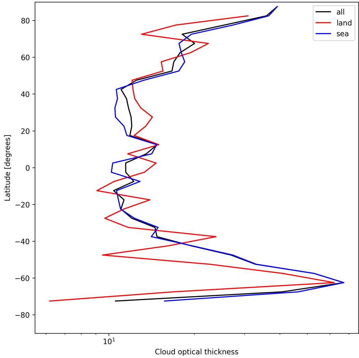
Figure 23: Zonal average of “Cloud optical thickness” for 2025-08-12 to 2025-08-12.
