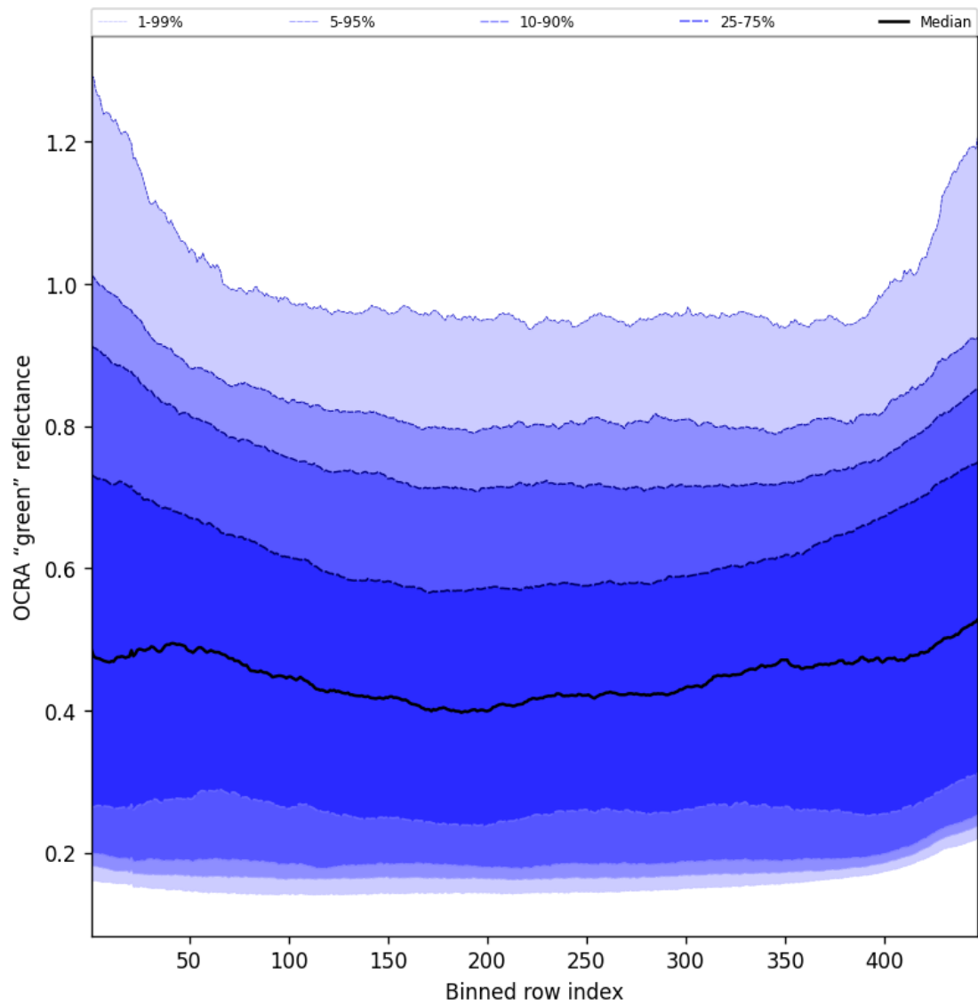
Figure 66: Along track statistics of "OCRA "green" reflectance" for 2025-08-12 to 2025-08-12
