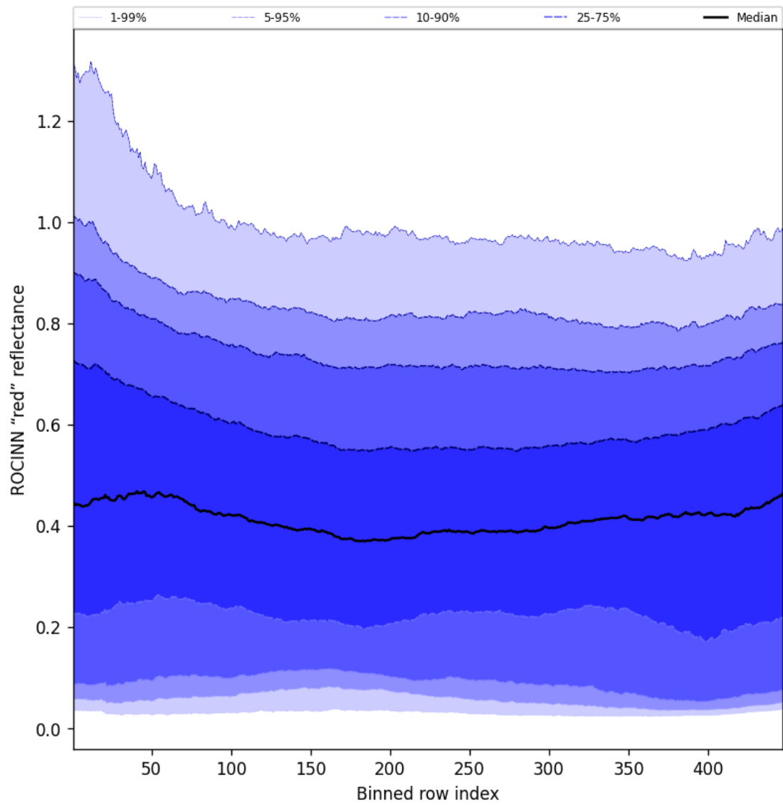
Figure 67: Along track statistics of “ROCINN “red” reflectance” for 2025-08-12 to 2025-08-12
