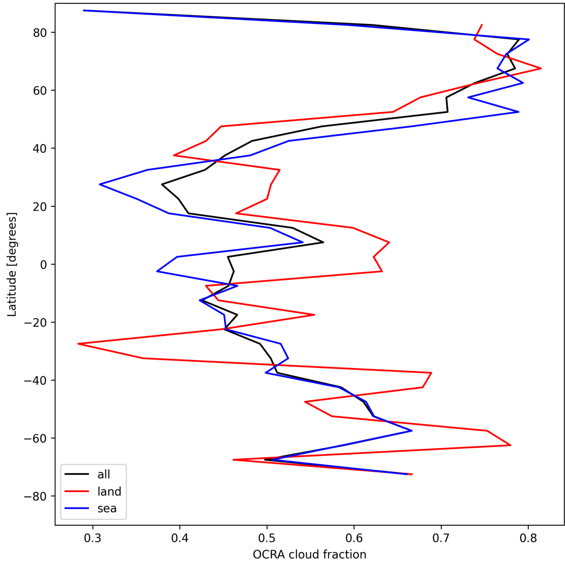
Figure 32: Zonal average of “OCRA cloud fraction” for 2025-08-12 to 2025-08-12.
