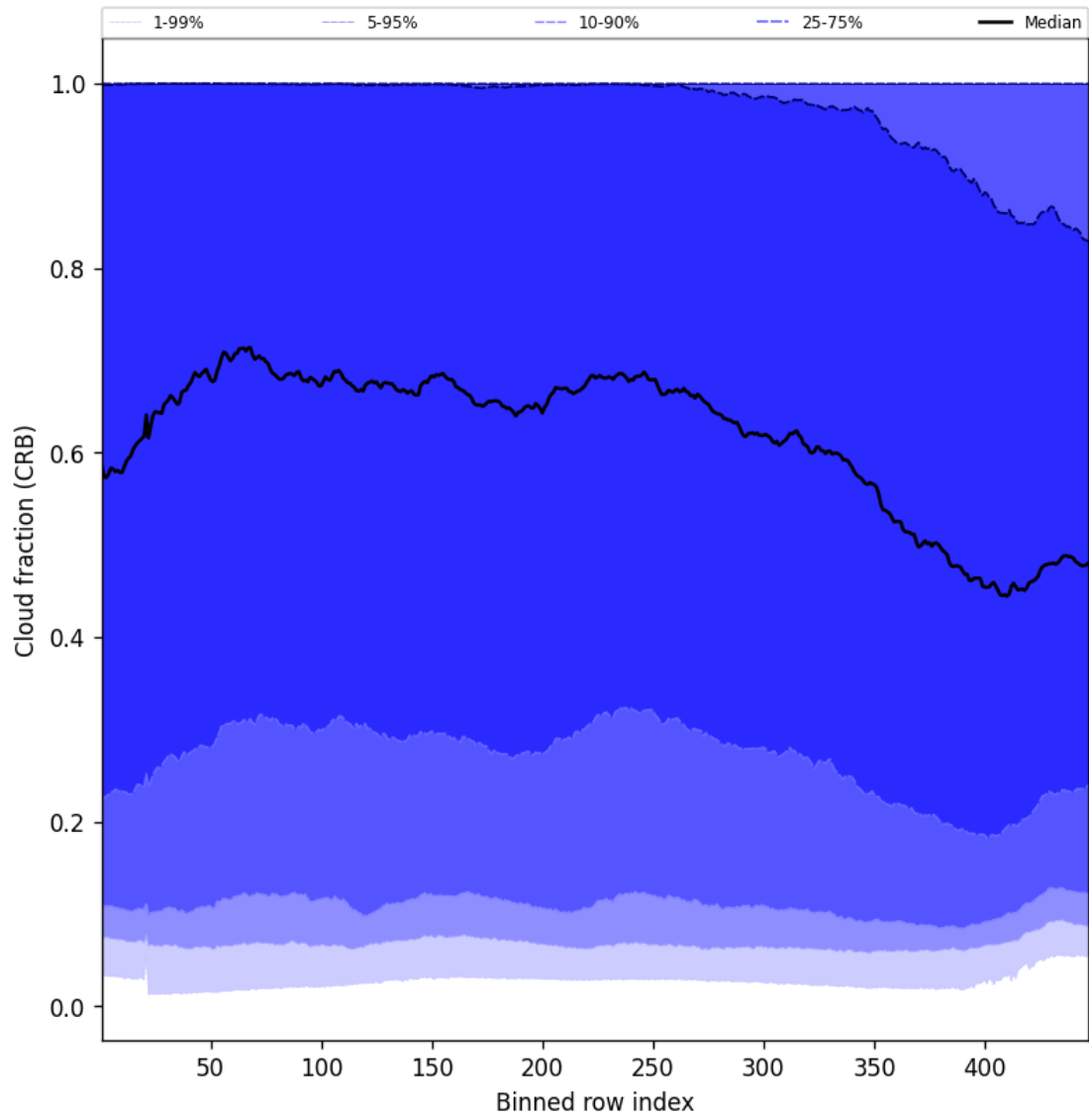
Figure 56: Along track statistics of “Cloud fraction (CRB)” for 2025-08-12 to 2025-08-12
