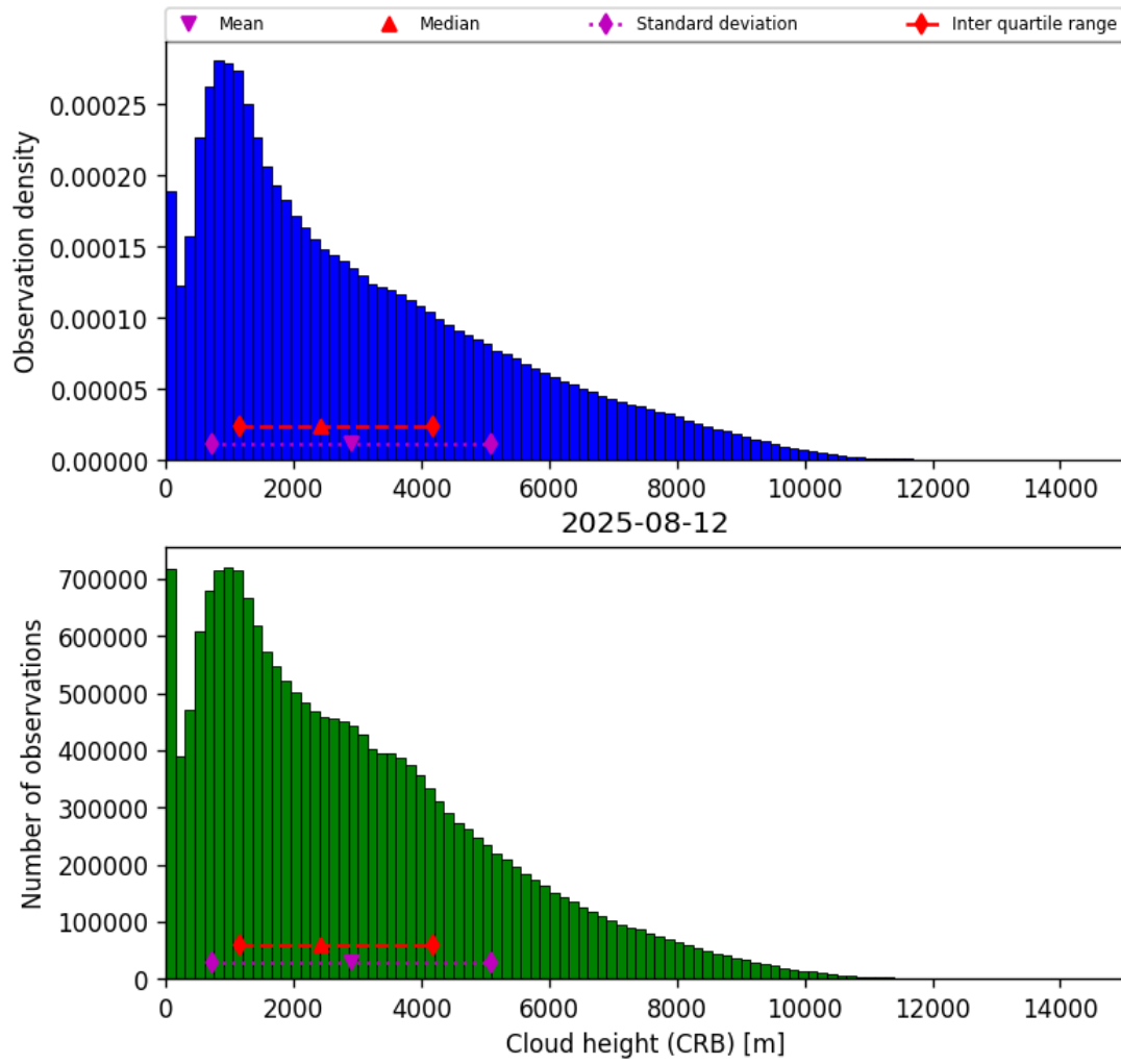
Figure 41: Histogram of “Cloud height (CRB)” for 2025-08-12 to 2025-08-12
