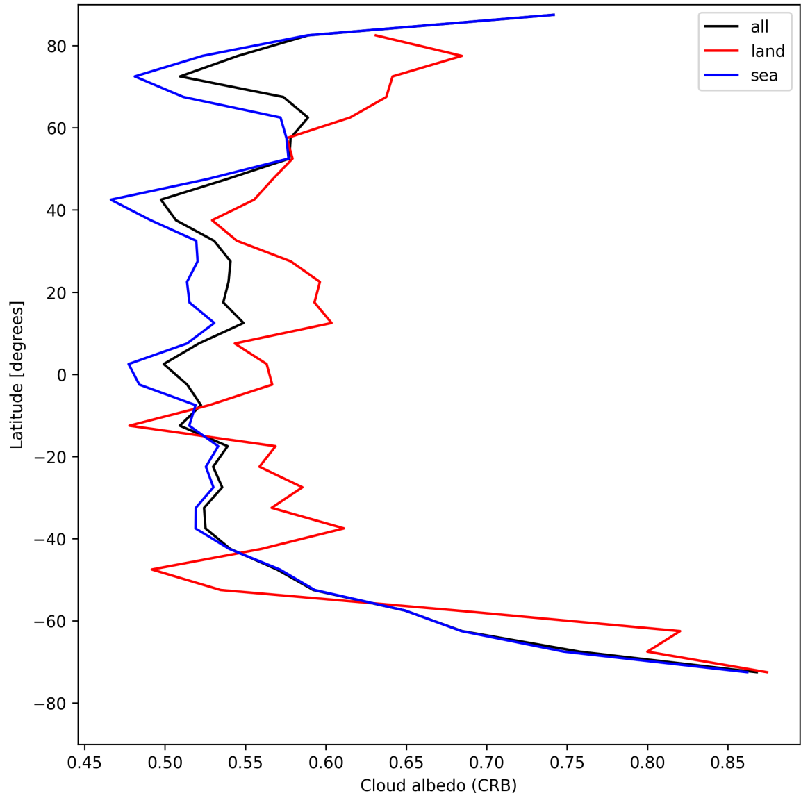
Figure 26: Zonal average of “Cloud albedo (CRB)” for 2025-08-12 to 2025-08-12.
