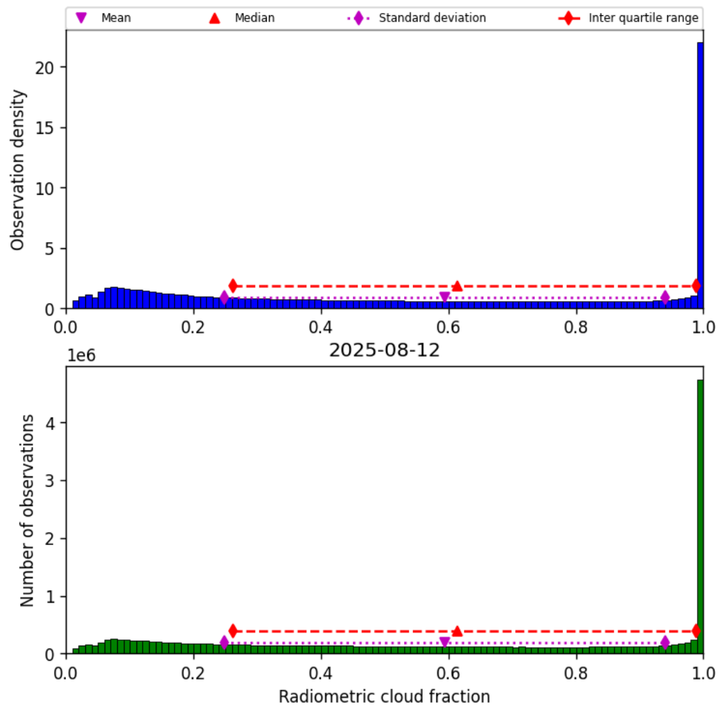
Figure 37: Histogram of “Radiometric cloud fraction” for 2025-08-12 to 2025-08-12
