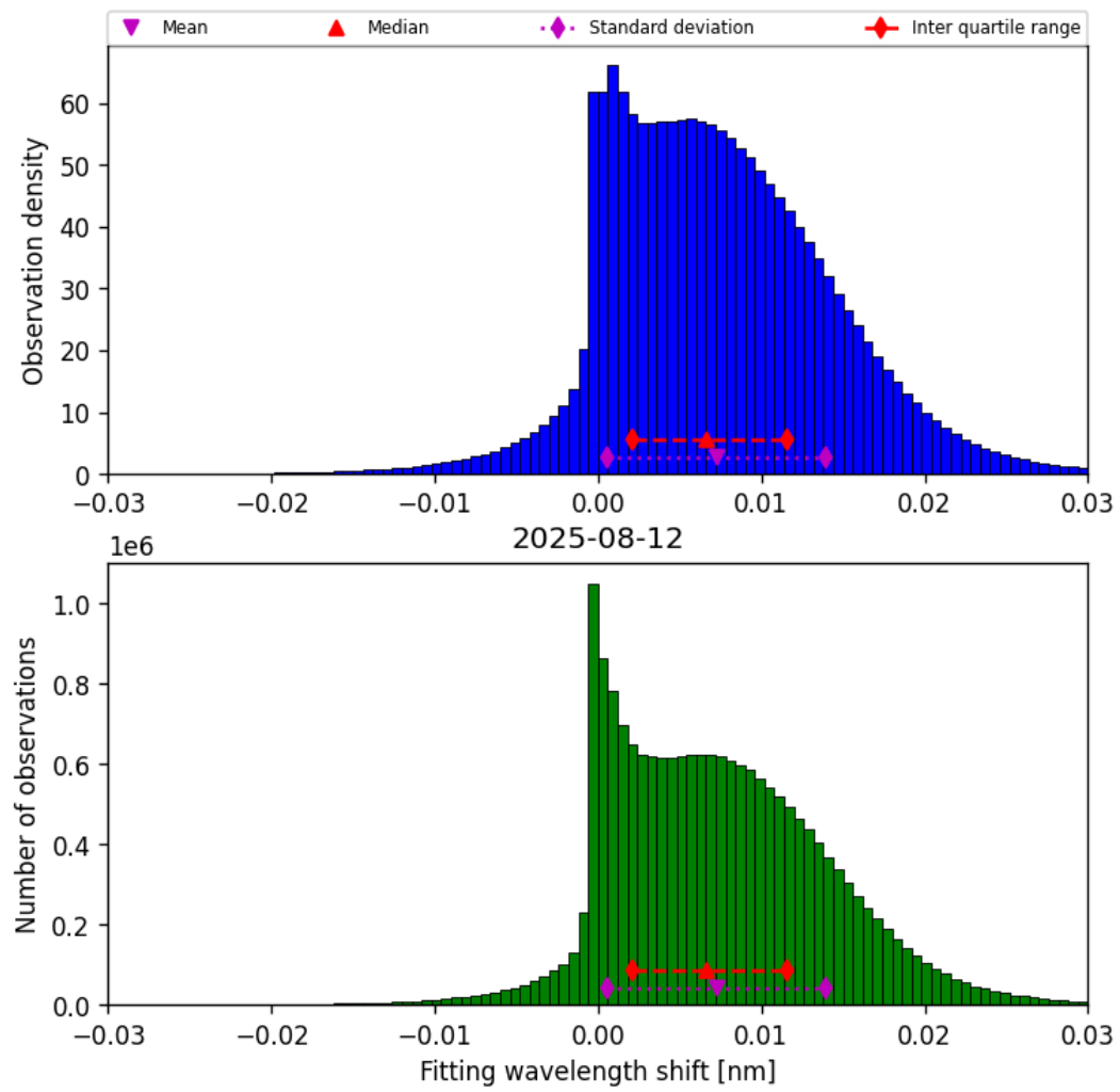
Figure 47: Histogram of “Fitting wavelength shift” for 2025-08-12 to 2025-08-12
