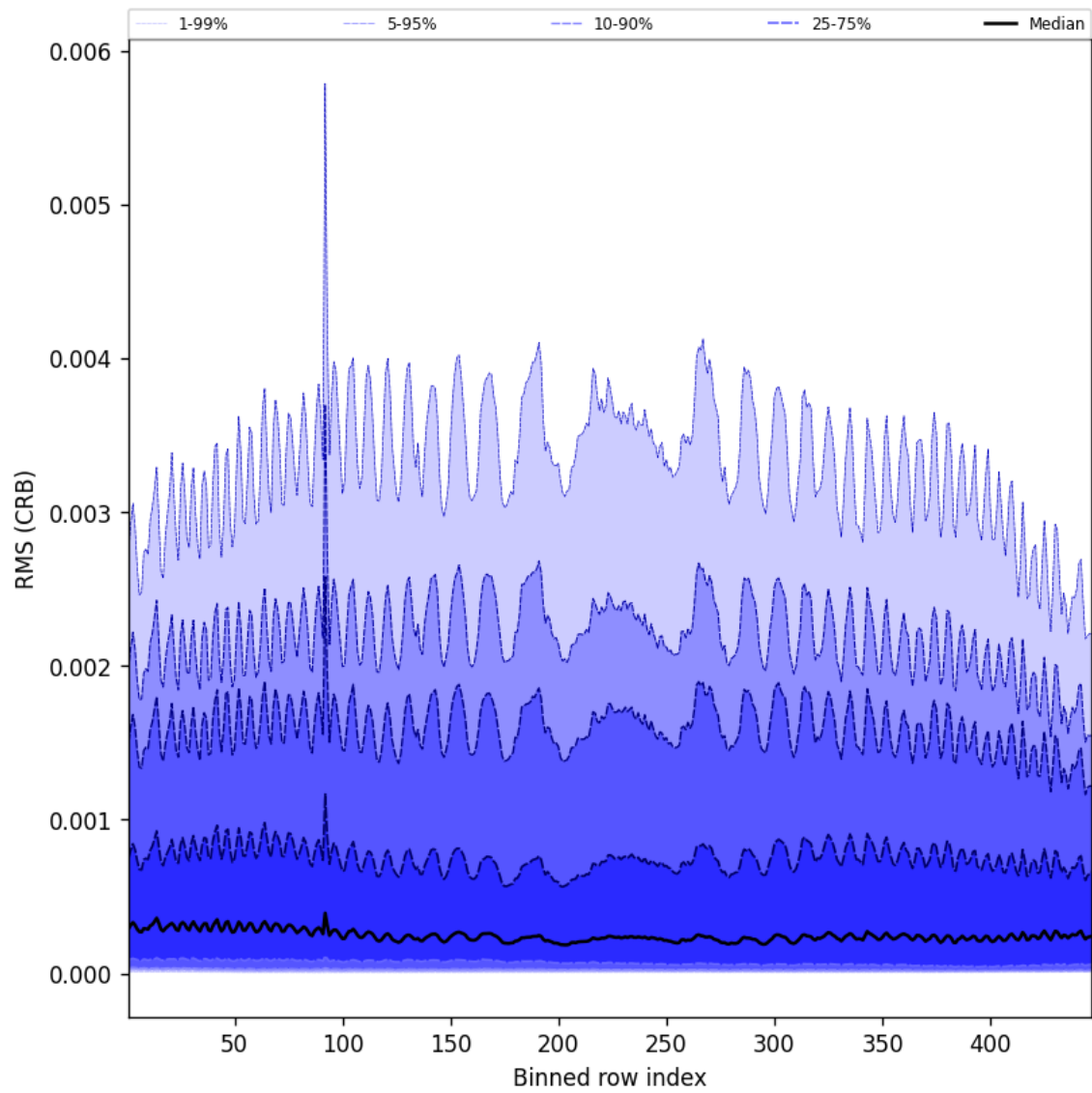
Figure 62: Along track statistics of “RMS (CRB)” for 2025-08-12 to 2025-08-12
