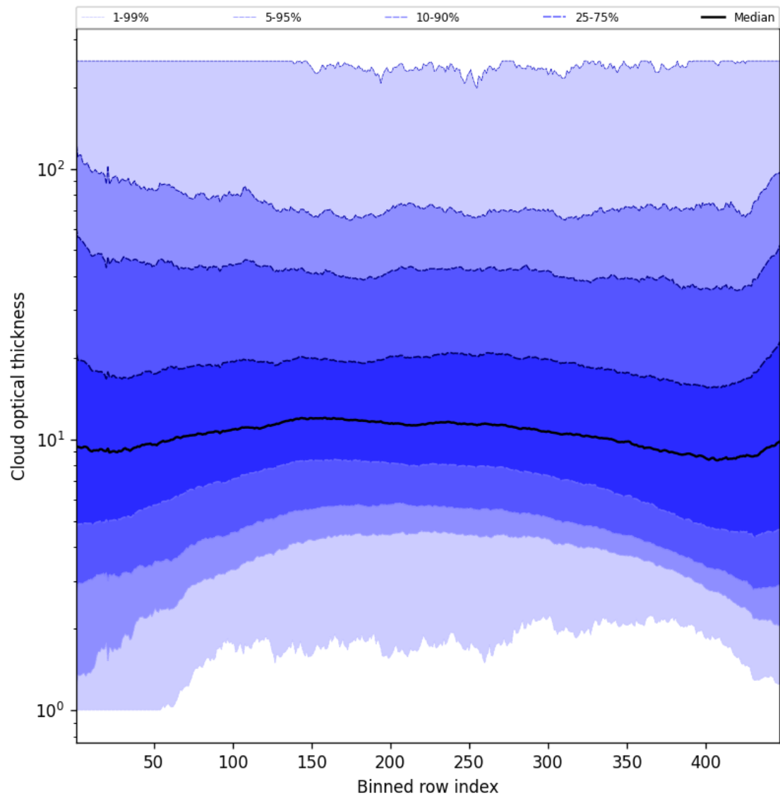
Figure 55: Along track statistics of “Cloud optical thickness” for 2025-08-12 to 2025-08-12
