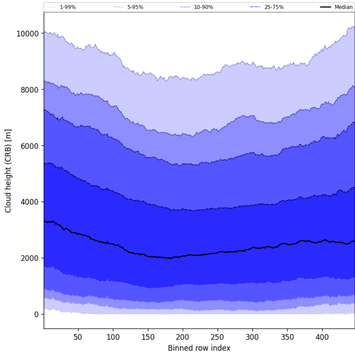
Figure 57: Along track statistics of “Cloud height (CRB)” for 2025-08-12 to 2025-08-12
