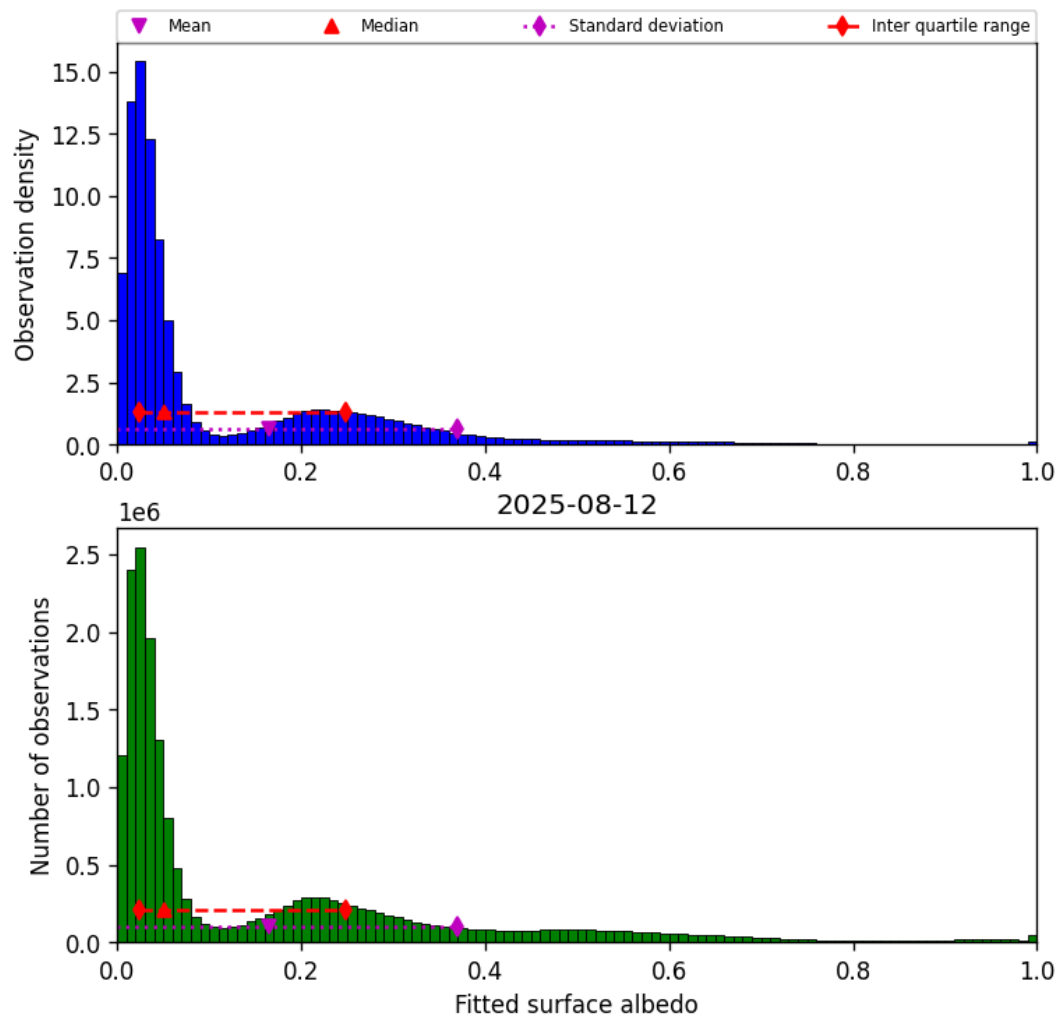
Figure 43: Histogram of “Fitted surface albedo” for 2025-08-12 to 2025-08-12
