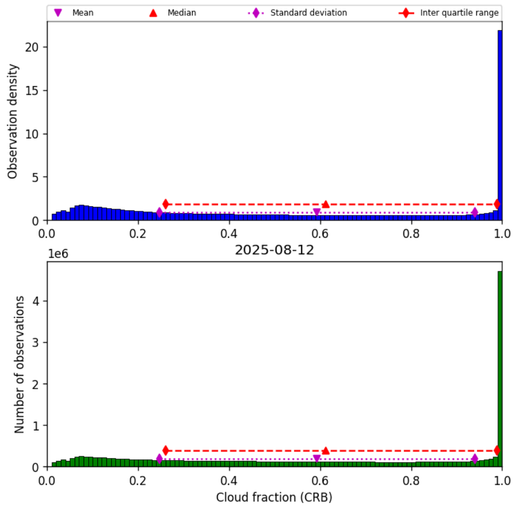
Figure 40: Histogram of “Cloud fraction (CRB)” for 2025-08-12 to 2025-08-12
