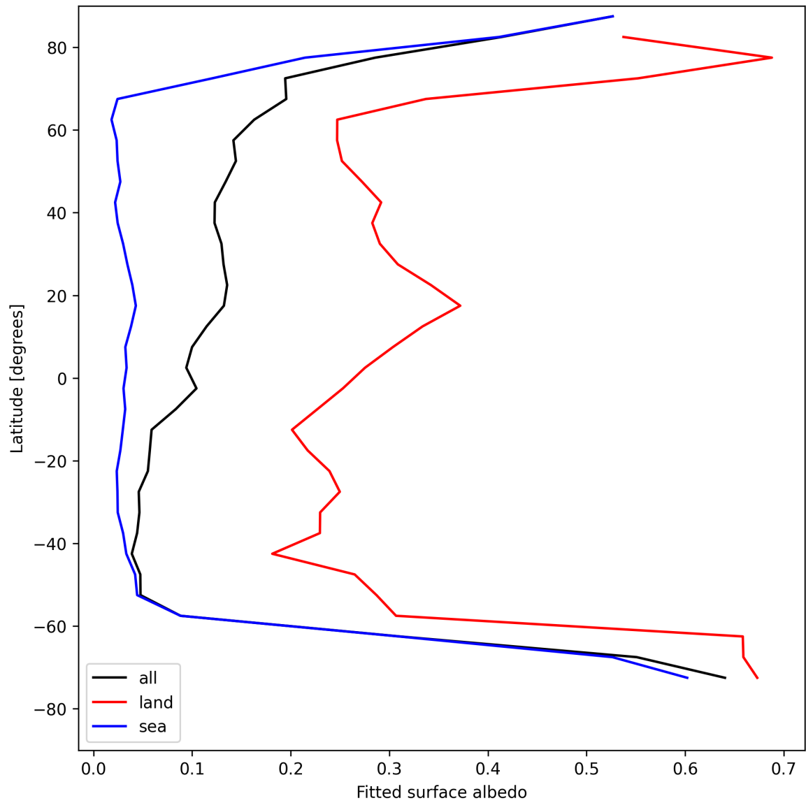
Figure 27: Zonal average of “Fitted surface albedo” for 2025-08-12 to 2025-08-12.
