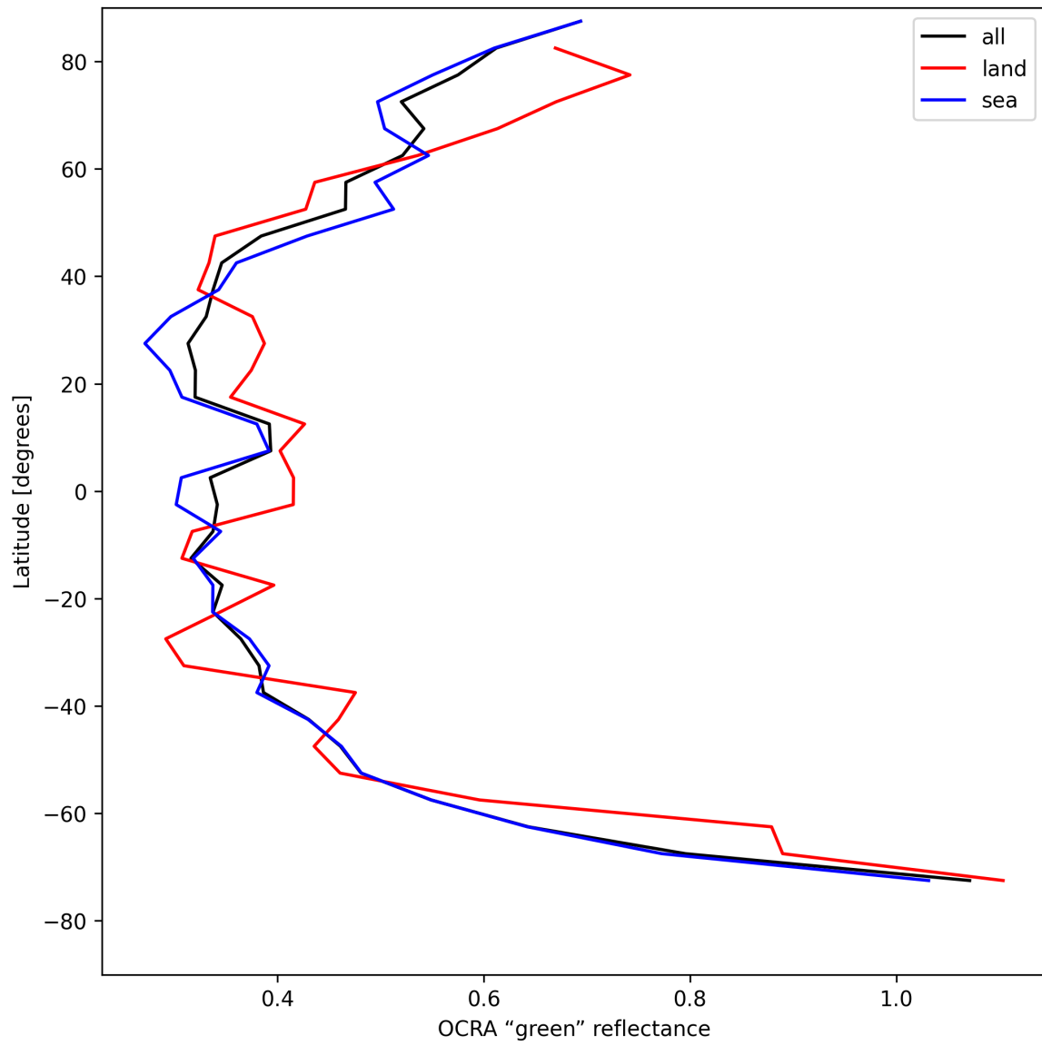
Figure 34: Zonal average of “OCRA “green” reflectance” for 2025-08-12 to 2025-08-12.
