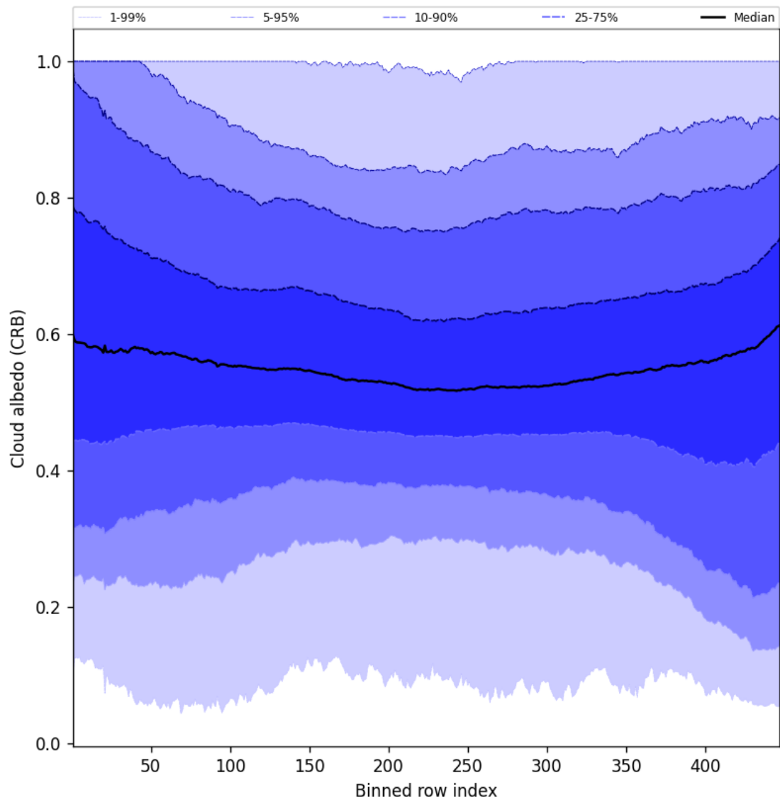
Figure 58: Along track statistics of “Cloud albedo (CRB)” for 2025-08-12 to 2025-08-12
