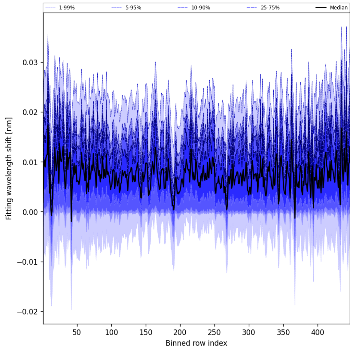
Figure 63: Along track statistics of “Fitting wavelength shift” for 2025-08-12 to 2025-08-12
