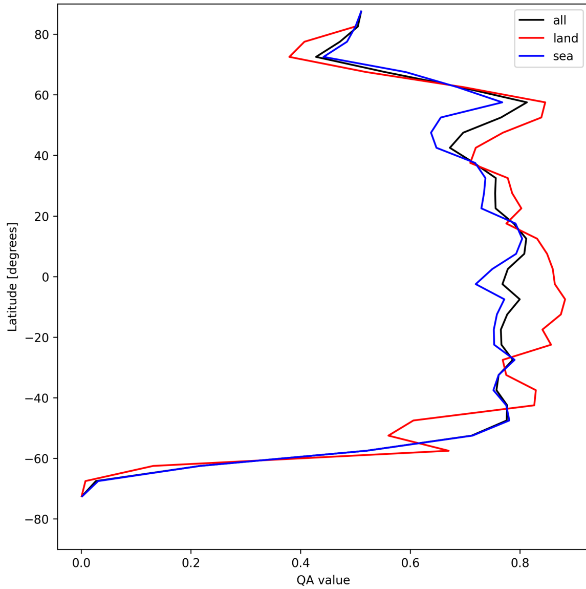
Figure 20: Zonal average of “QA value” for 2025-08-12 to 2025-08-12.
