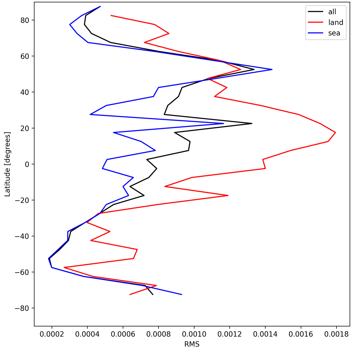
Figure 29: Zonal average of “RMS” for 2025-08-12 to 2025-08-12.
