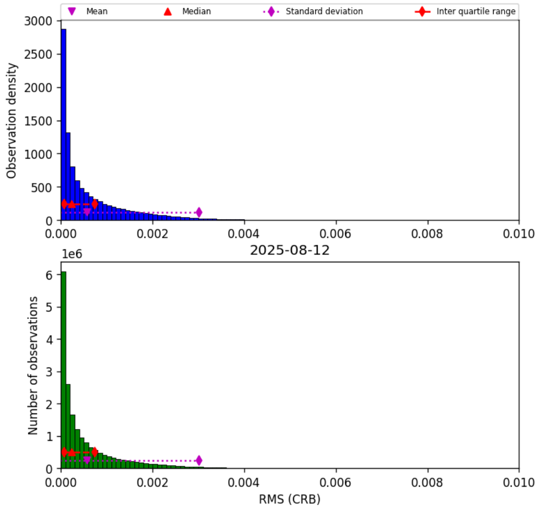
Figure 46: Histogram of “RMS (CRB)” for 2025-08-12 to 2025-08-12
