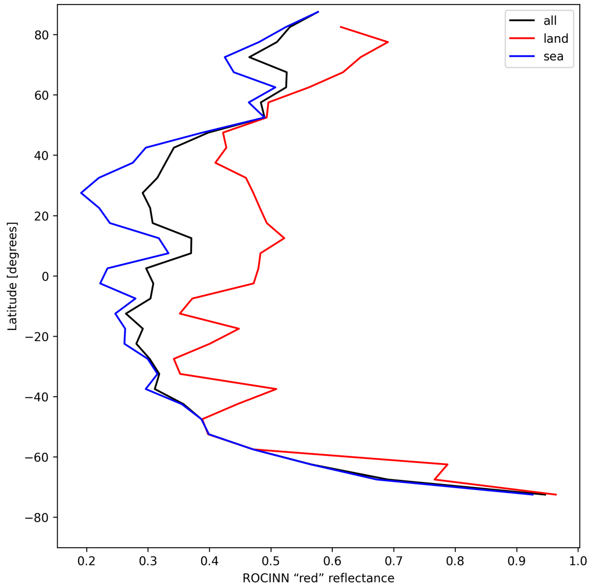
Figure 35: Zonal average of “ROCINN “red” reflectance” for 2025-08-12 to 2025-08-12.
