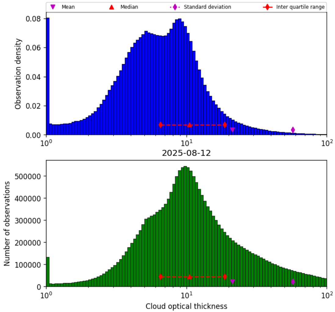
Figure 39: Histogram of “Cloud optical thickness” for 2025-08-12 to 2025-08-12
