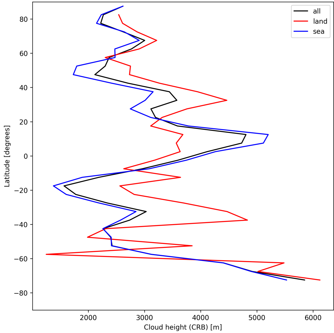
Figure 25: Zonal average of “Cloud height (CRB)” for 2025-08-12 to 2025-08-12.
