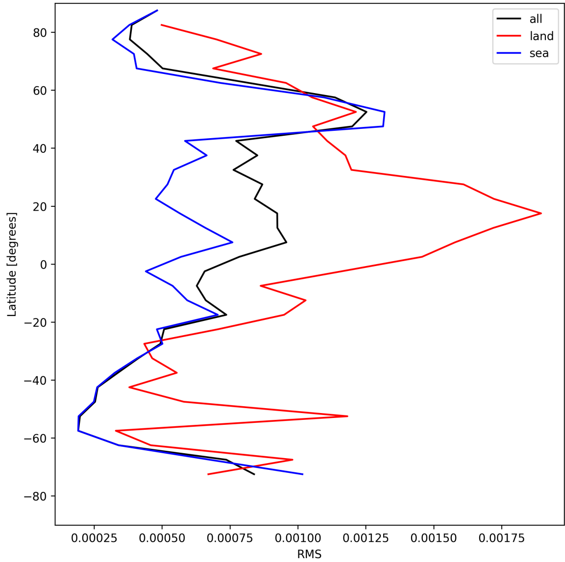
Figure 29: Zonal average of “RMS” for 2025-08-13 to 2025-08-14.
