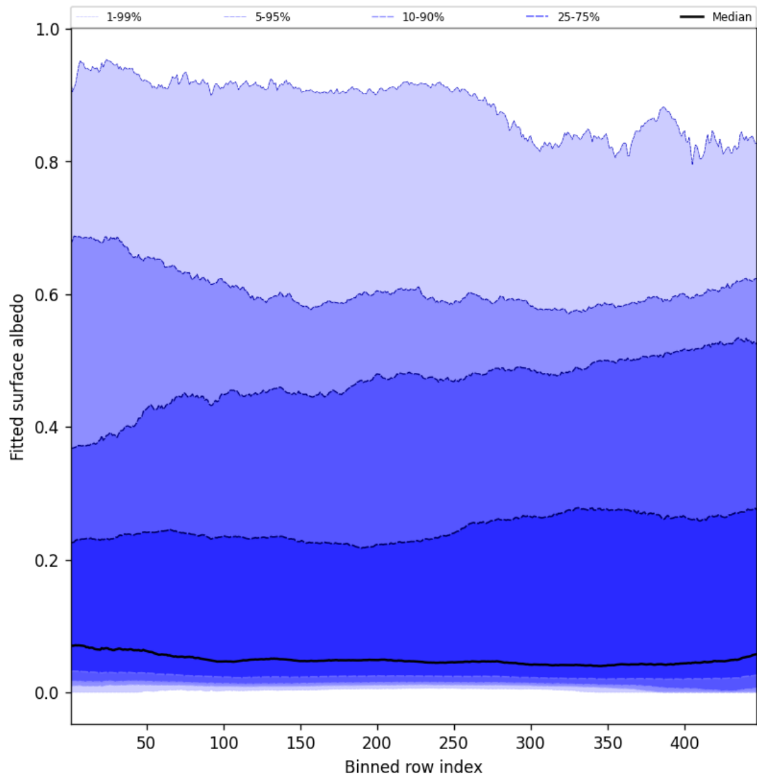
Figure 59: Along track statistics of “Fitted surface albedo” for 2025-08-13 to 2025-08-14
