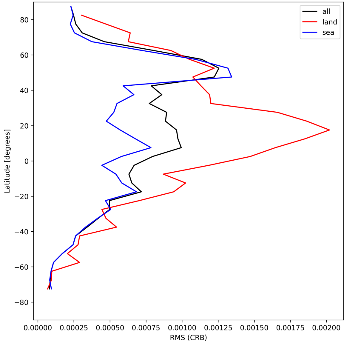
Figure 30: Zonal average of “RMS (CRB)” for 2025-08-13 to 2025-08-14.
