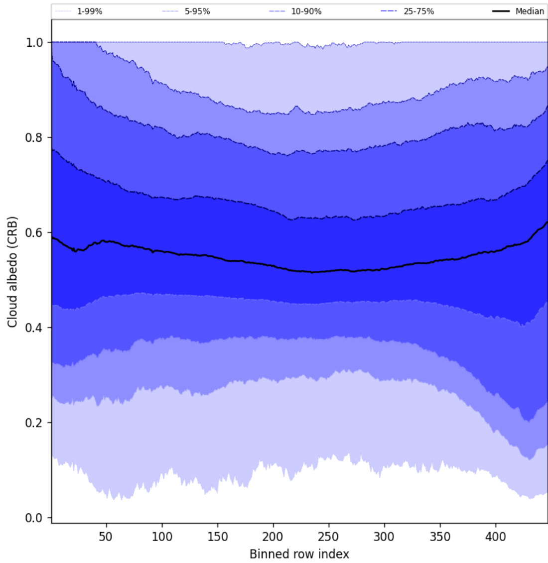
Figure 58: Along track statistics of “Cloud albedo (CRB)” for 2025-08-13 to 2025-08-14
