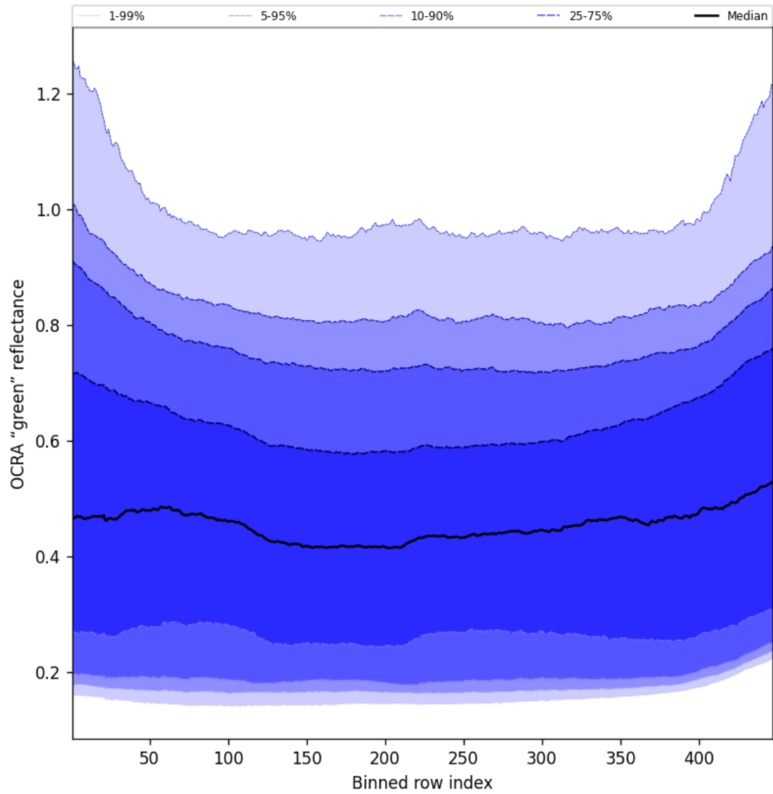
Figure 66: Along track statistics of "OCRA "green" reflectance" for 2025-08-13 to 2025-08-14
