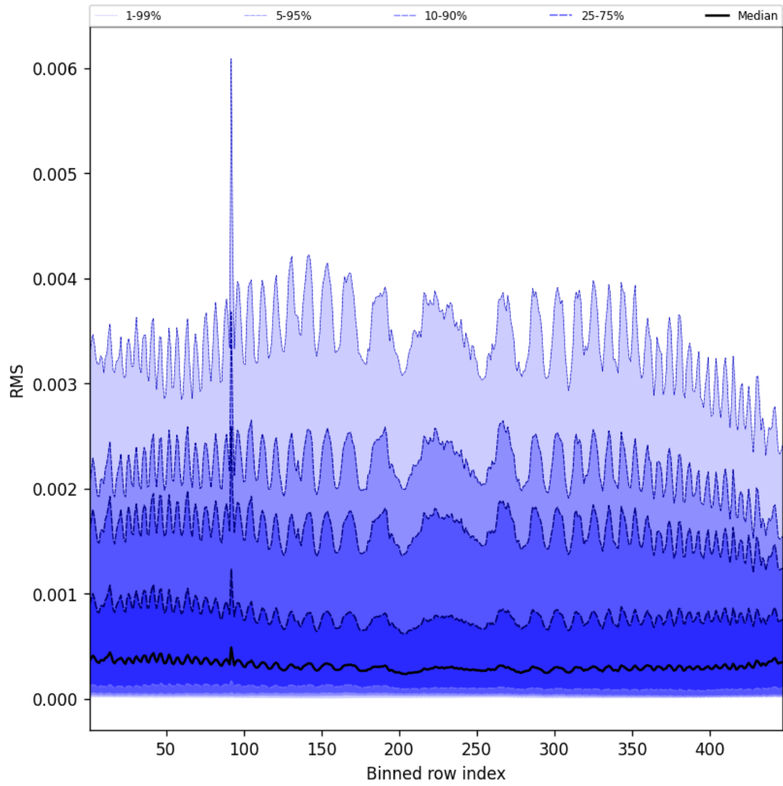
Figure 61: Along track statistics of “RMS” for 2025-08-13 to 2025-08-14
