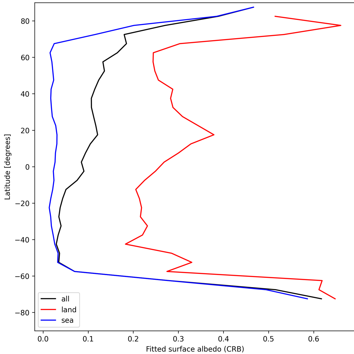
Figure 28: Zonal average of “Fitted surface albedo (CRB)” for 2025-08-13 to 2025-08-14.
