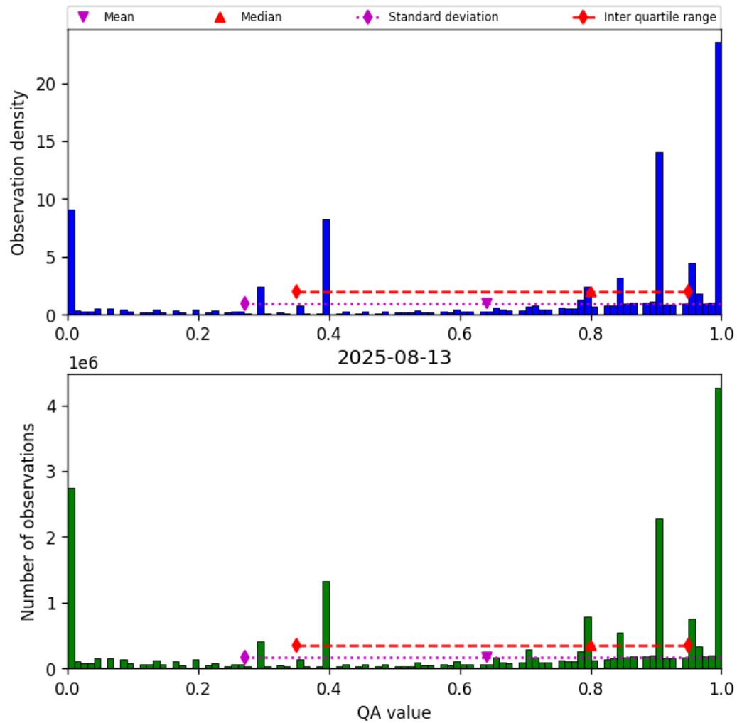
Figure 36: Histogram of “QA value” for 2025-08-13 to 2025-08-14
