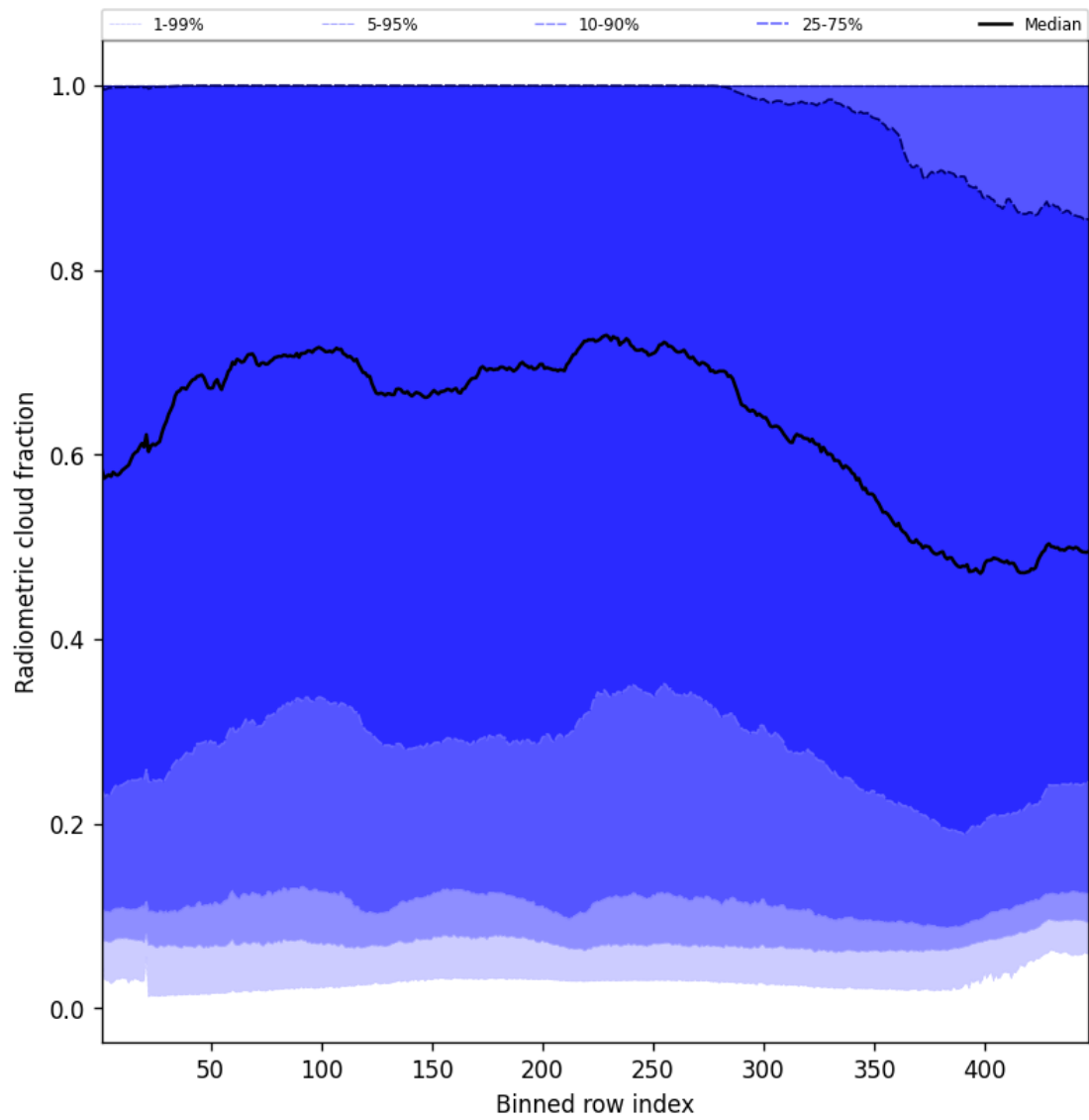
Figure 53: Along track statistics of “Radiometric cloud fraction” for 2025-08-13 to 2025-08-14
