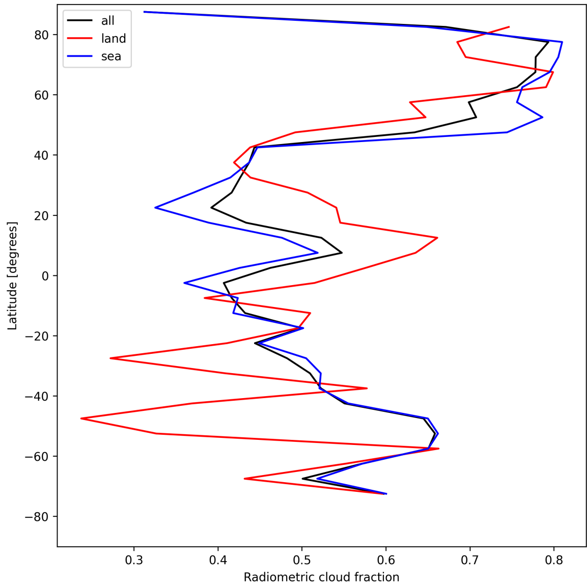
Figure 21: Zonal average of “Radiometric cloud fraction” for 2025-08-13 to 2025-08-14.
