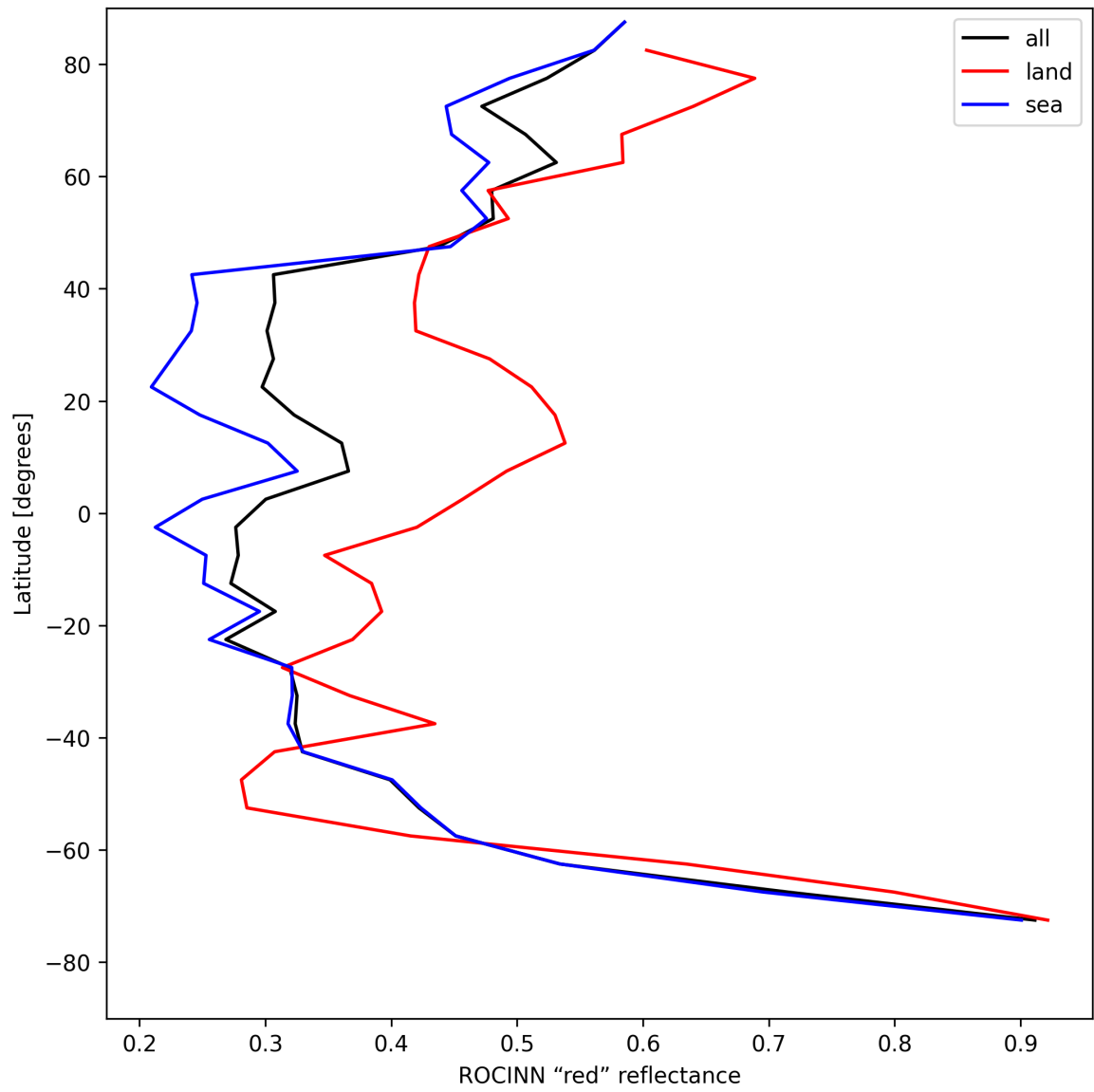
Figure 35: Zonal average of "ROCINN "red" reflectance" for 2025-08-13 to 2025-08-14.
