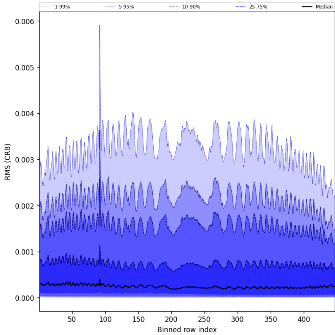
Figure 62: Along track statistics of “RMS (CRB)” for 2025-08-13 to 2025-08-14
