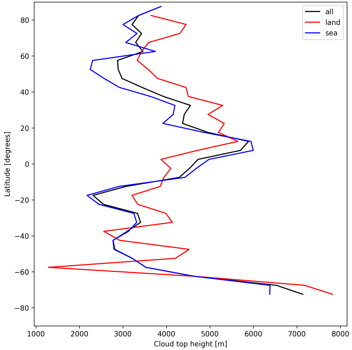
Figure 22: Zonal average of “Cloud top height” for 2025-08-13 to 2025-08-14.
