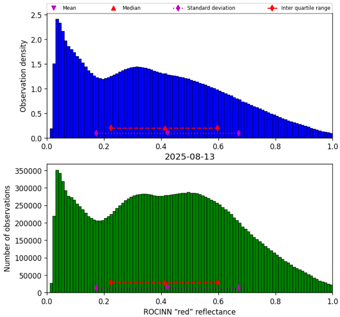
Figure 51: Histogram of “ROCINN “red” reflectance” for 2025-08-13 to 2025-08-14
