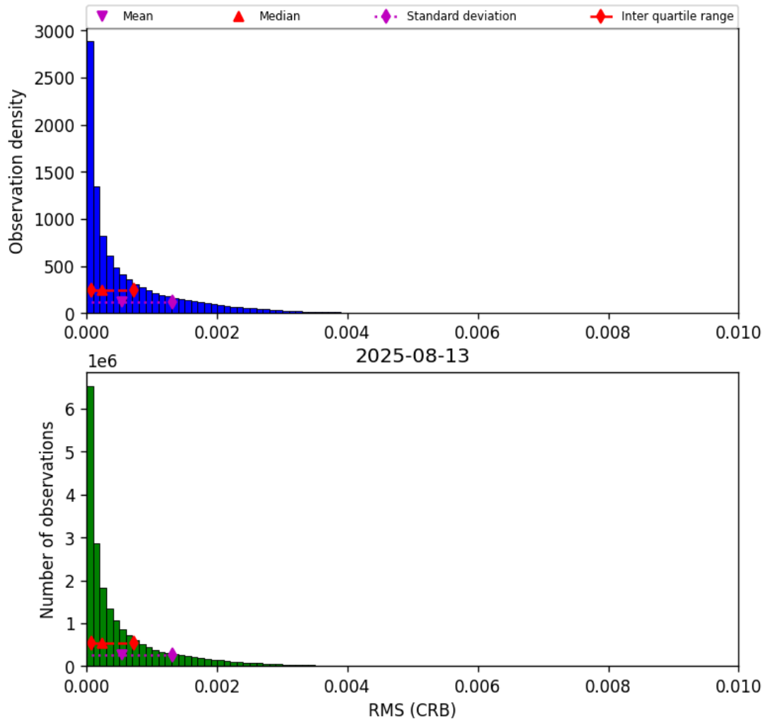
Figure 46: Histogram of “RMS (CRB)” for 2025-08-13 to 2025-08-14
