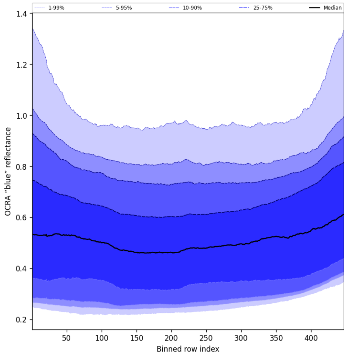
Figure 65: Along track statistics of “OCRA “blue” reflectance” for 2025-08-13 to 2025-08-14
