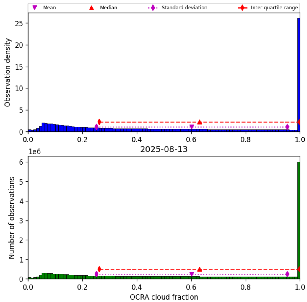
Figure 48: Histogram of “OCRA cloud fraction” for 2025-08-13 to 2025-08-14
