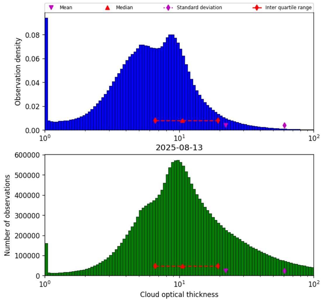
Figure 39: Histogram of “Cloud optical thickness” for 2025-08-13 to 2025-08-14
