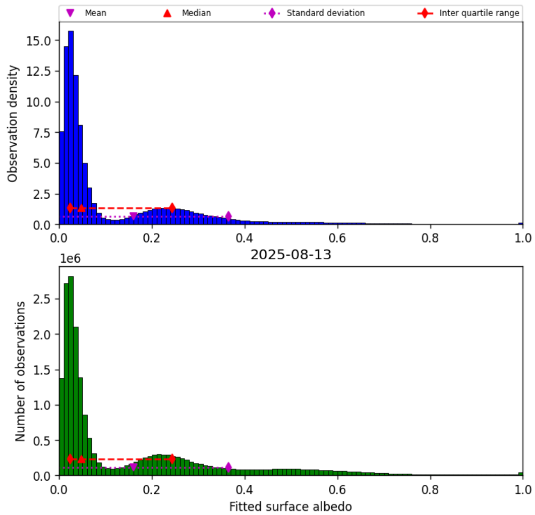
Figure 43: Histogram of “Fitted surface albedo” for 2025-08-13 to 2025-08-14
