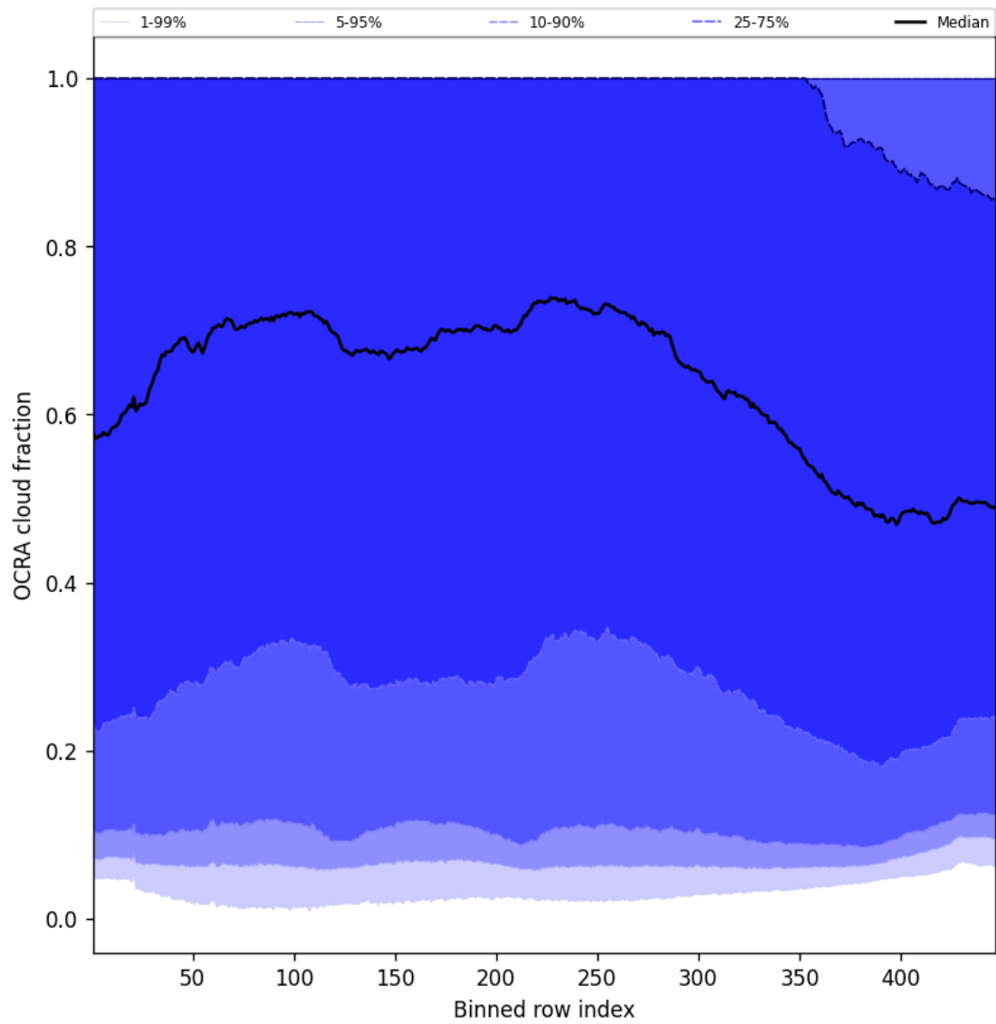
Figure 64: Along track statistics of “OCRA cloud fraction” for 2025-08-13 to 2025-08-14
