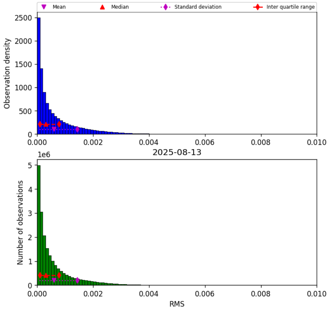
Figure 45: Histogram of “RMS” for 2025-08-13 to 2025-08-14
