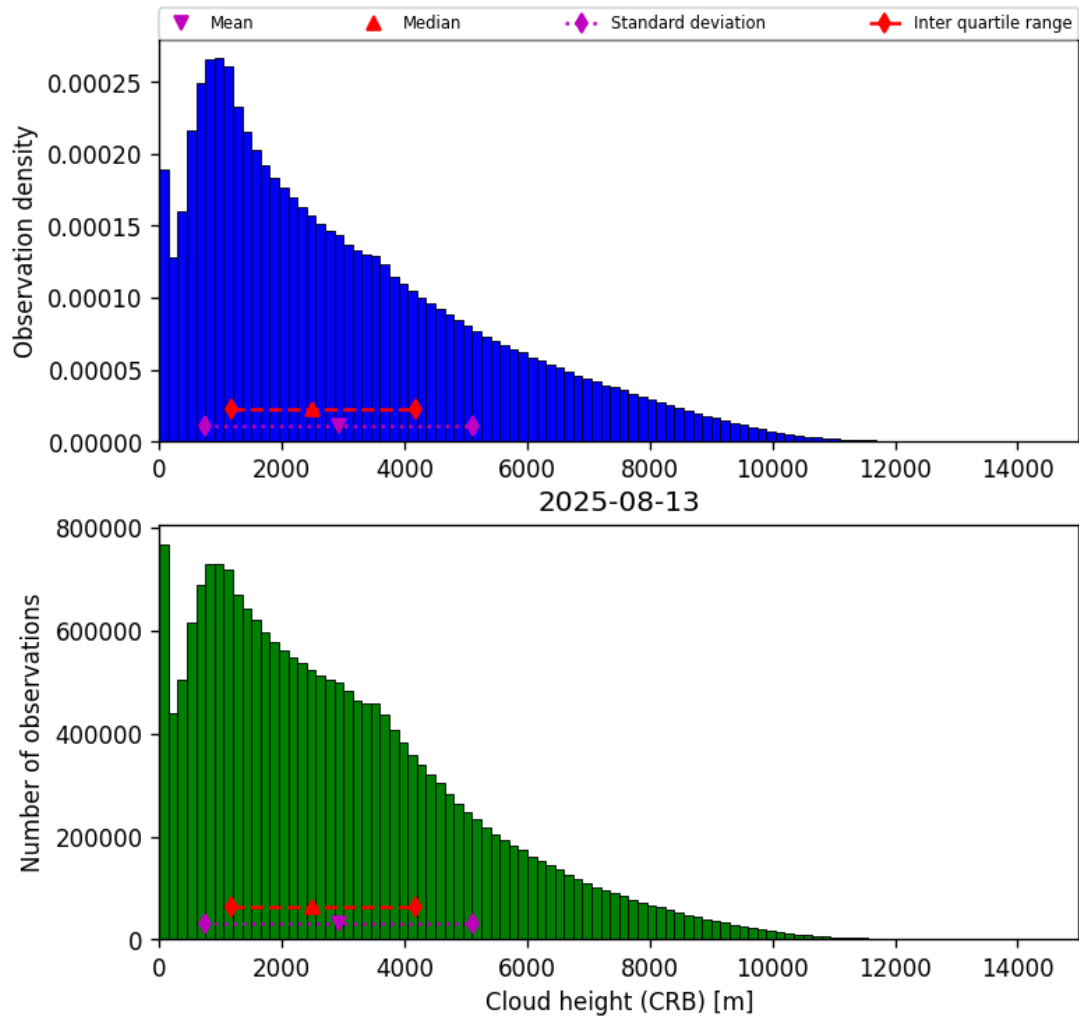
Figure 41: Histogram of “Cloud height (CRB)” for 2025-08-13 to 2025-08-14
