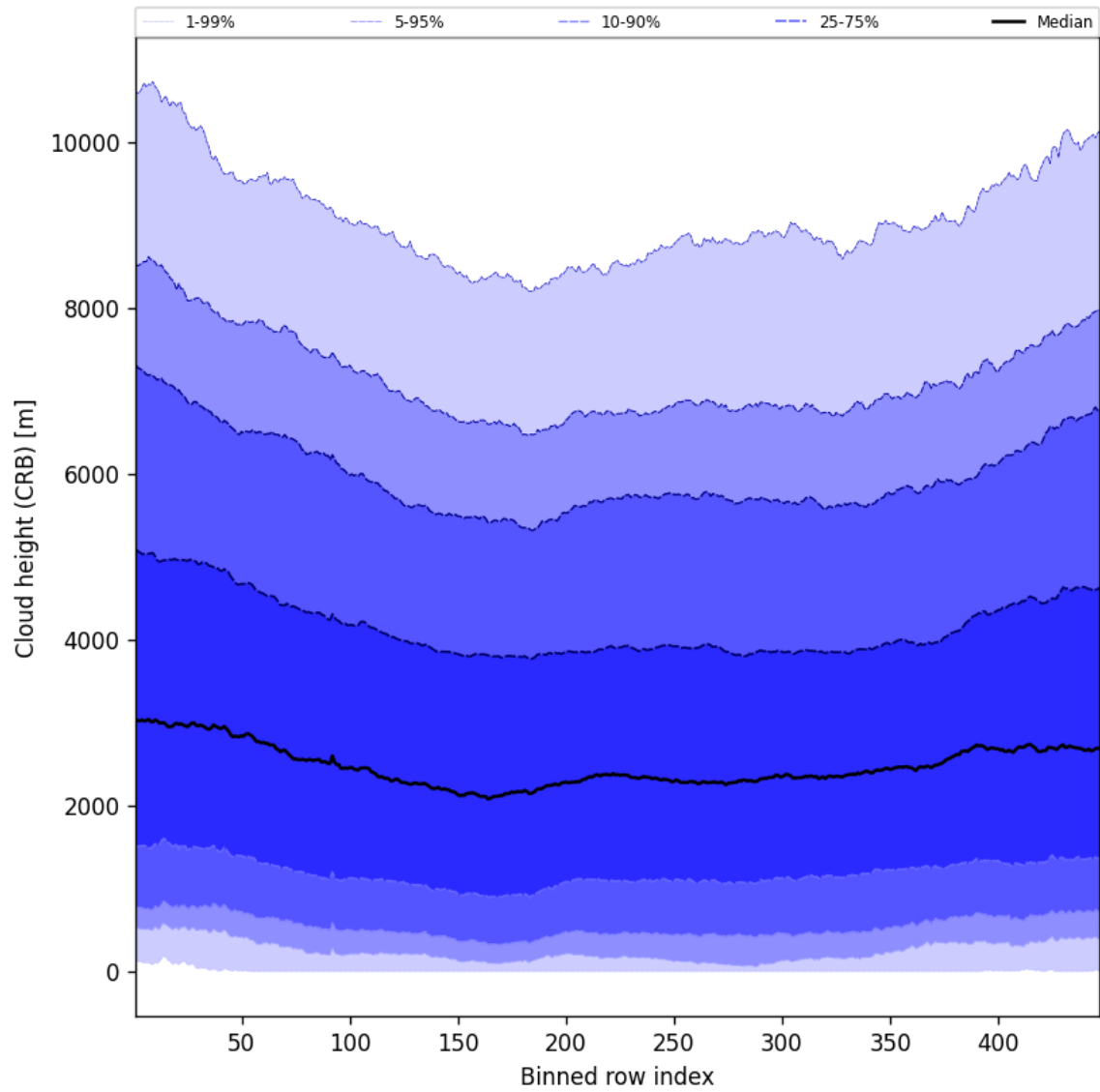
Figure 57: Along track statistics of “Cloud height (CRB)” for 2025-08-13 to 2025-08-14
