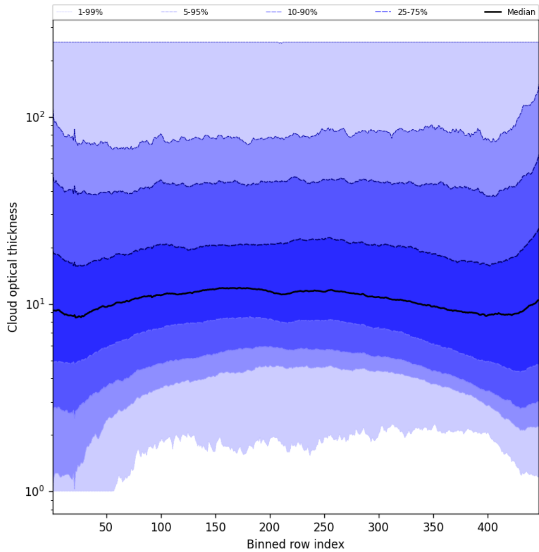
Figure 55: Along track statistics of “Cloud optical thickness” for 2025-08-13 to 2025-08-14
