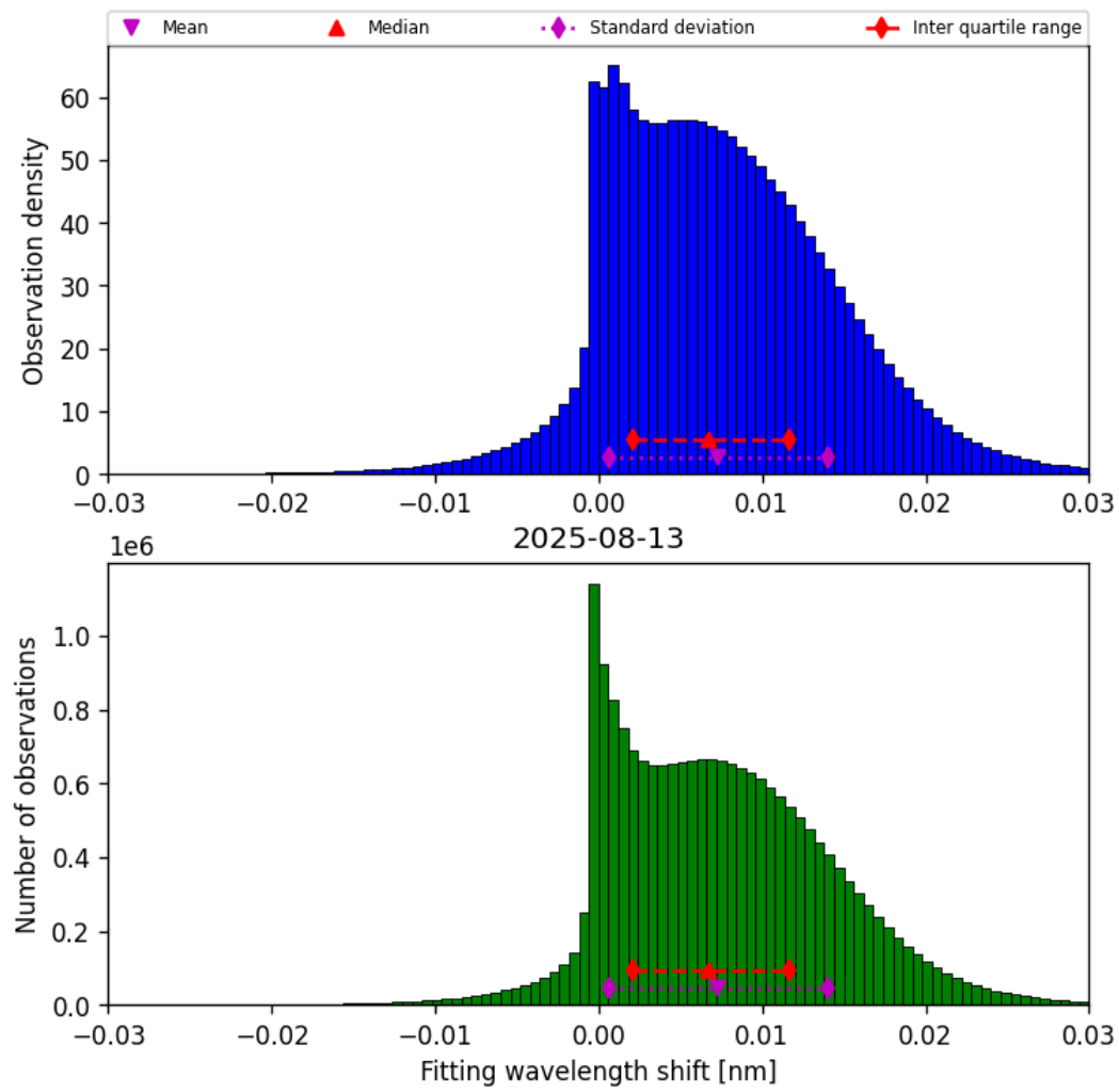
Figure 47: Histogram of “Fitting wavelength shift” for 2025-08-13 to 2025-08-14
