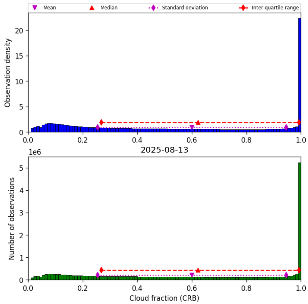
Figure 40: Histogram of “Cloud fraction (CRB)” for 2025-08-13 to 2025-08-14
