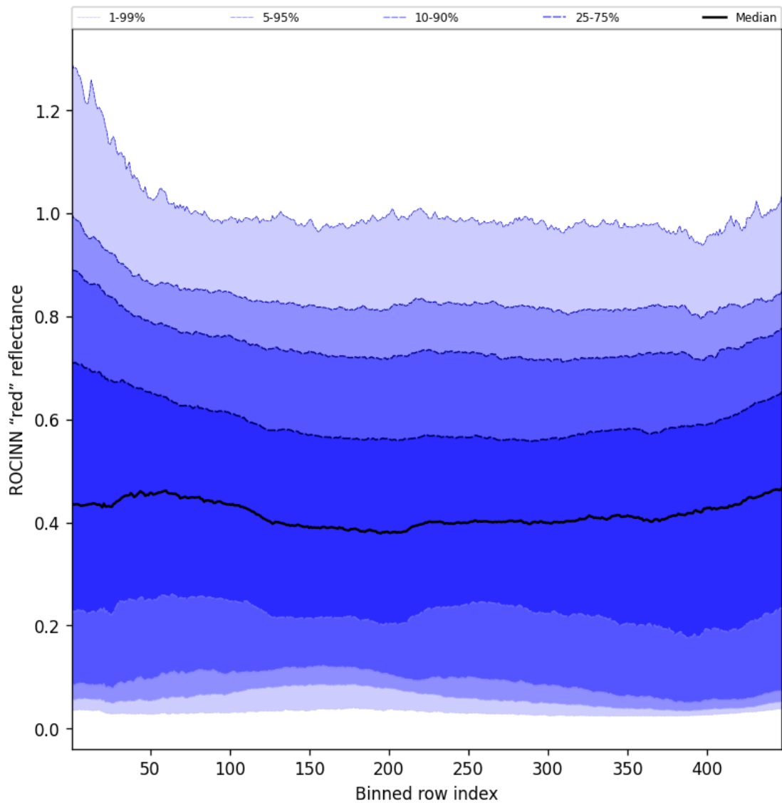
Figure 67: Along track statistics of “ROCINN “red” reflectance” for 2025-08-13 to 2025-08-14
