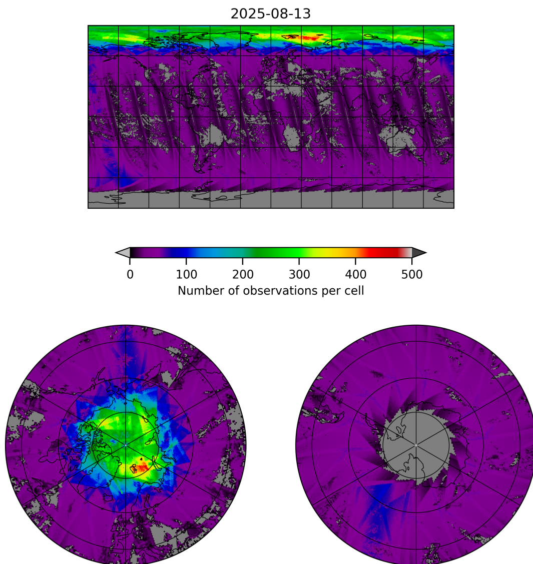
Figure 19: Map of the number of observations for 2025-08-13 to 2025-08-14
