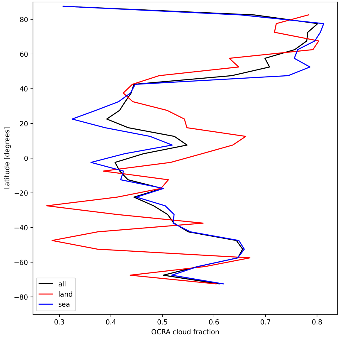
Figure 32: Zonal average of “OCRA cloud fraction” for 2025-08-13 to 2025-08-14.
