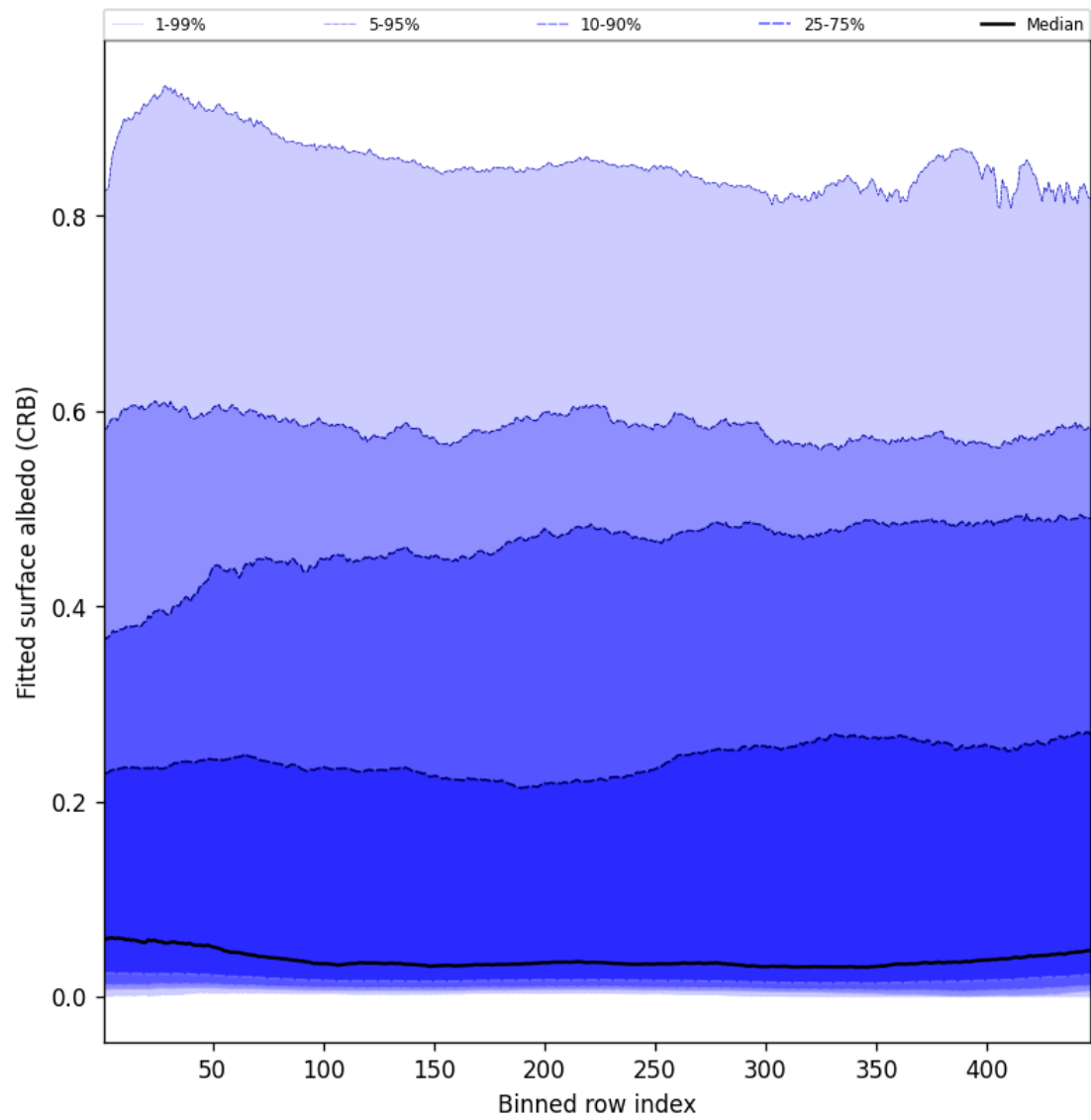
Figure 60: Along track statistics of “Fitted surface albedo (CRB)” for 2025-08-13 to 2025-08-14
