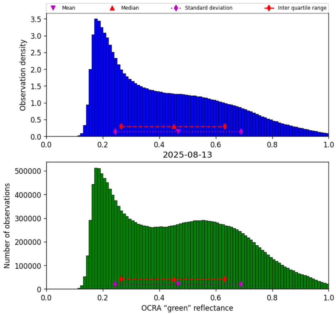
Figure 50: Histogram of “OCRA “green” reflectance” for 2025-08-13 to 2025-08-14
