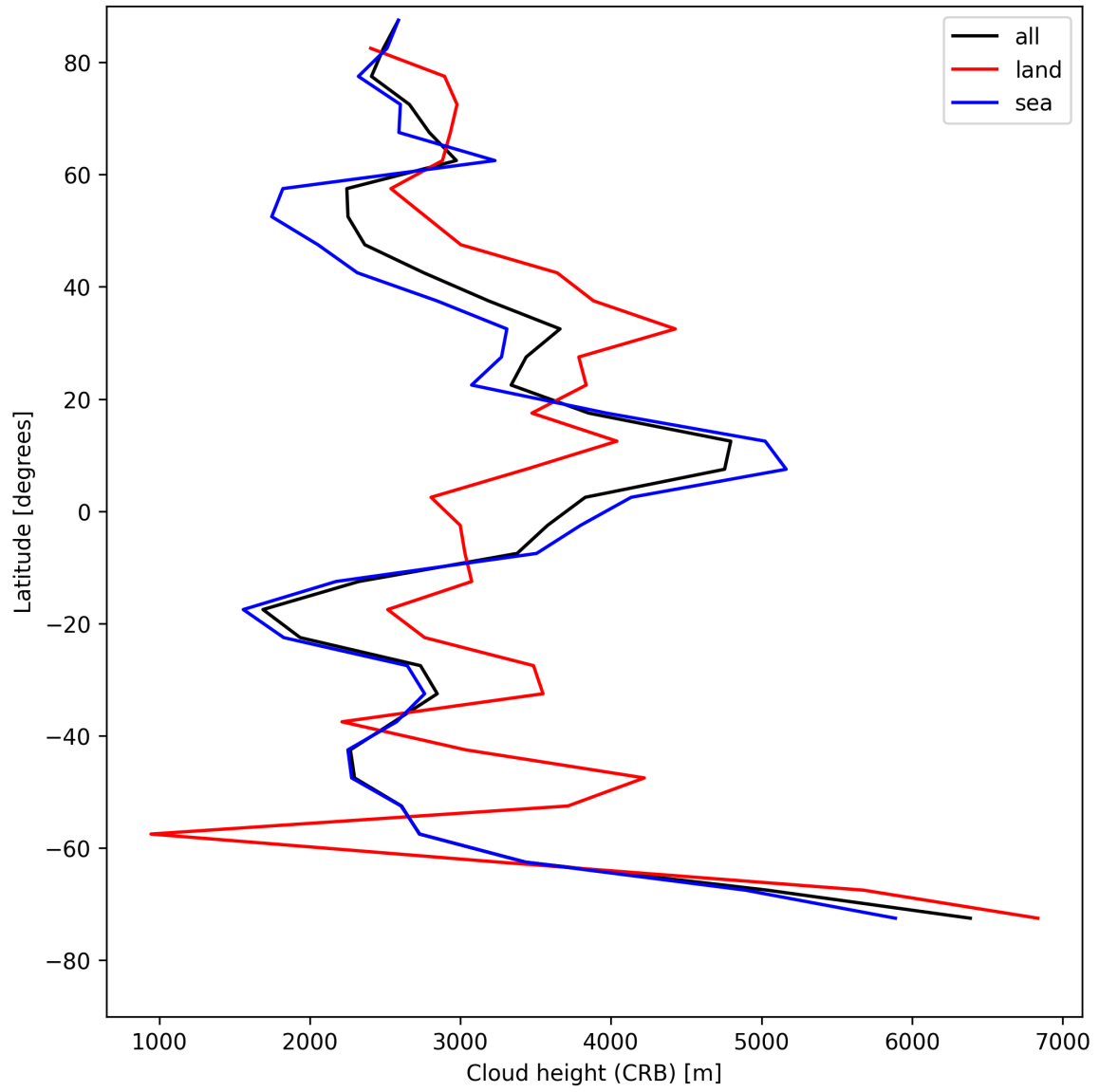
Figure 25: Zonal average of “Cloud height (CRB)” for 2025-08-13 to 2025-08-14.
