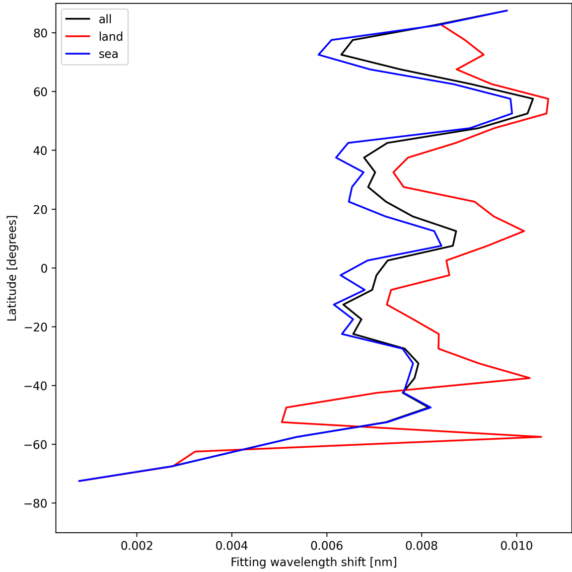
Figure 31: Zonal average of “Fitting wavelength shift” for 2025-08-13 to 2025-08-14.
