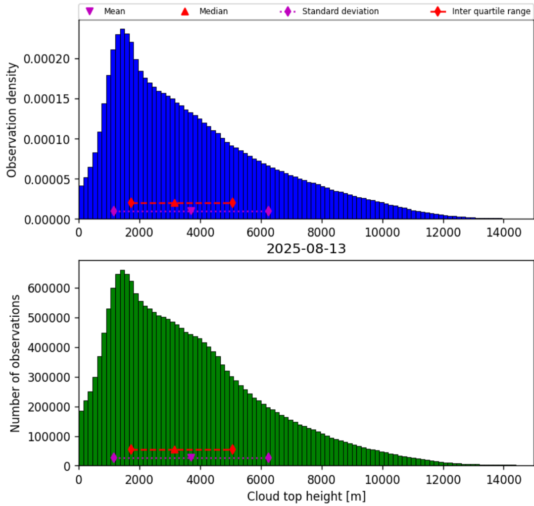
Figure 38: Histogram of “Cloud top height” for 2025-08-13 to 2025-08-14
