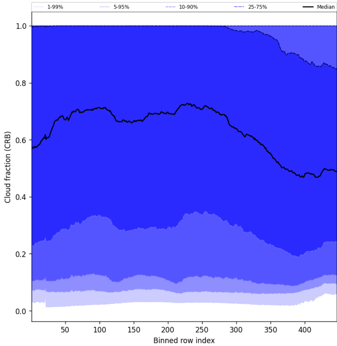
Figure 56: Along track statistics of “Cloud fraction (CRB)” for 2025-08-13 to 2025-08-14
