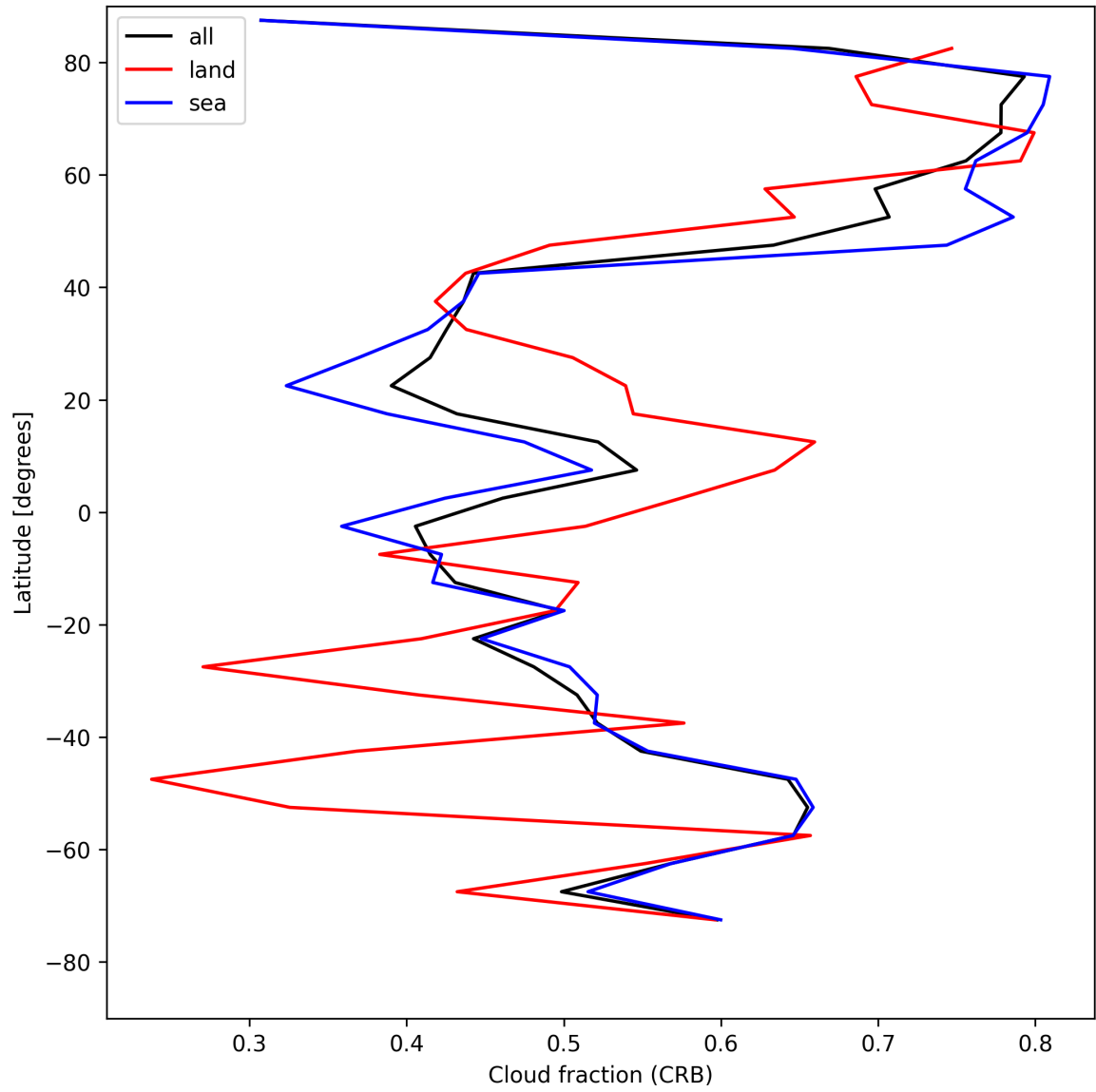
Figure 24: Zonal average of “Cloud fraction (CRB)” for 2025-08-13 to 2025-08-14.
