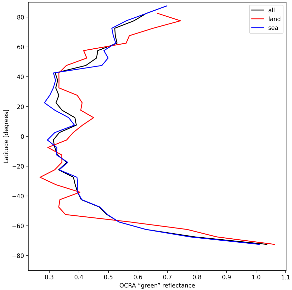
Figure 34: Zonal average of "OCRA "green" reflectance" for 2025-08-13 to 2025-08-14.
