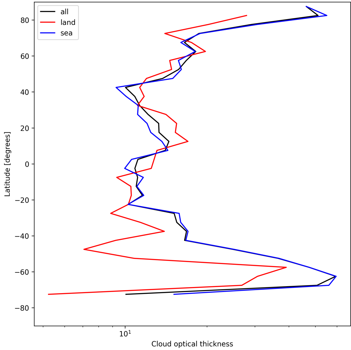
Figure 23: Zonal average of “Cloud optical thickness” for 2025-08-13 to 2025-08-14.
