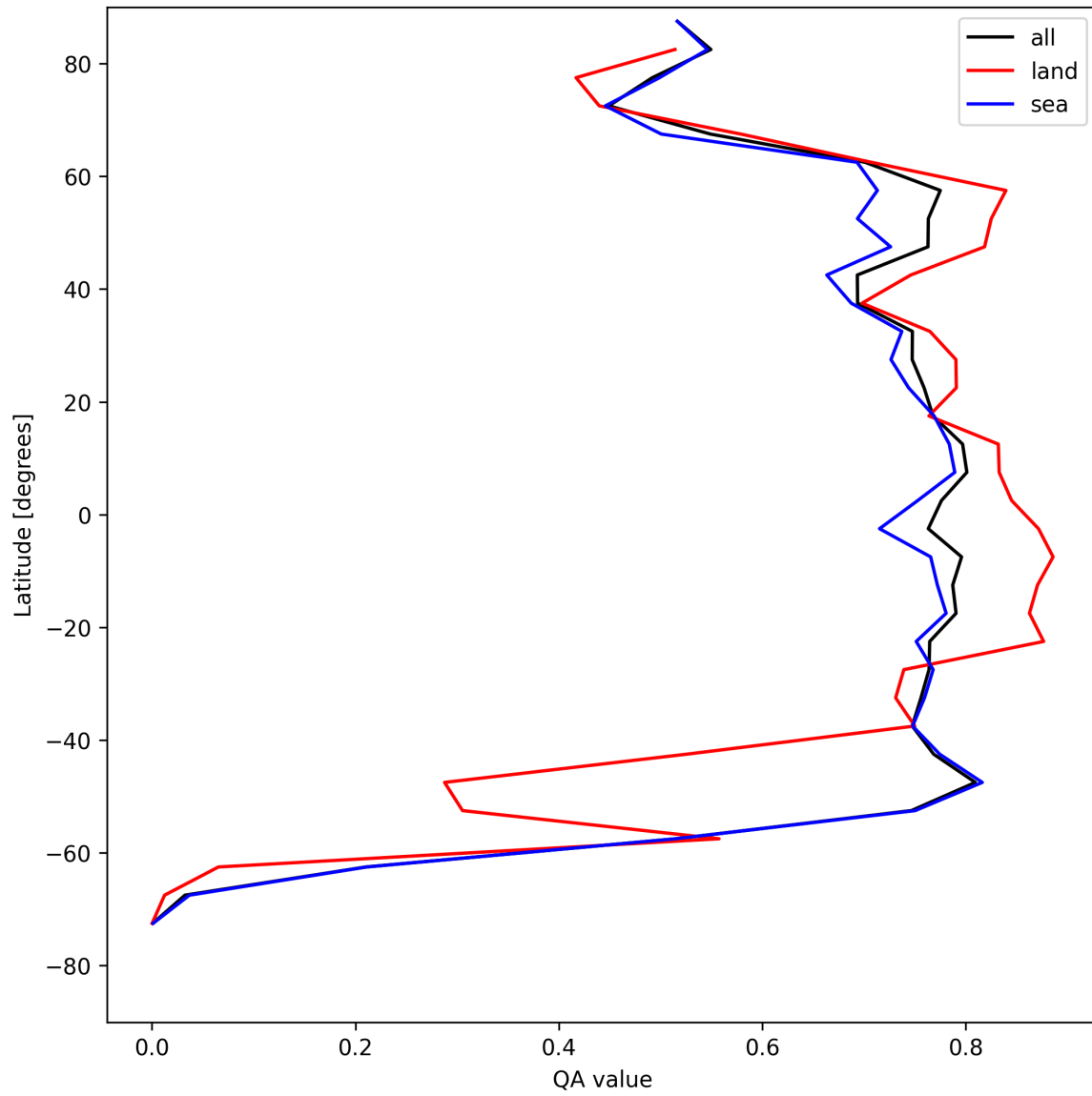
Figure 20: Zonal average of “QA value” for 2025-08-13 to 2025-08-14.
