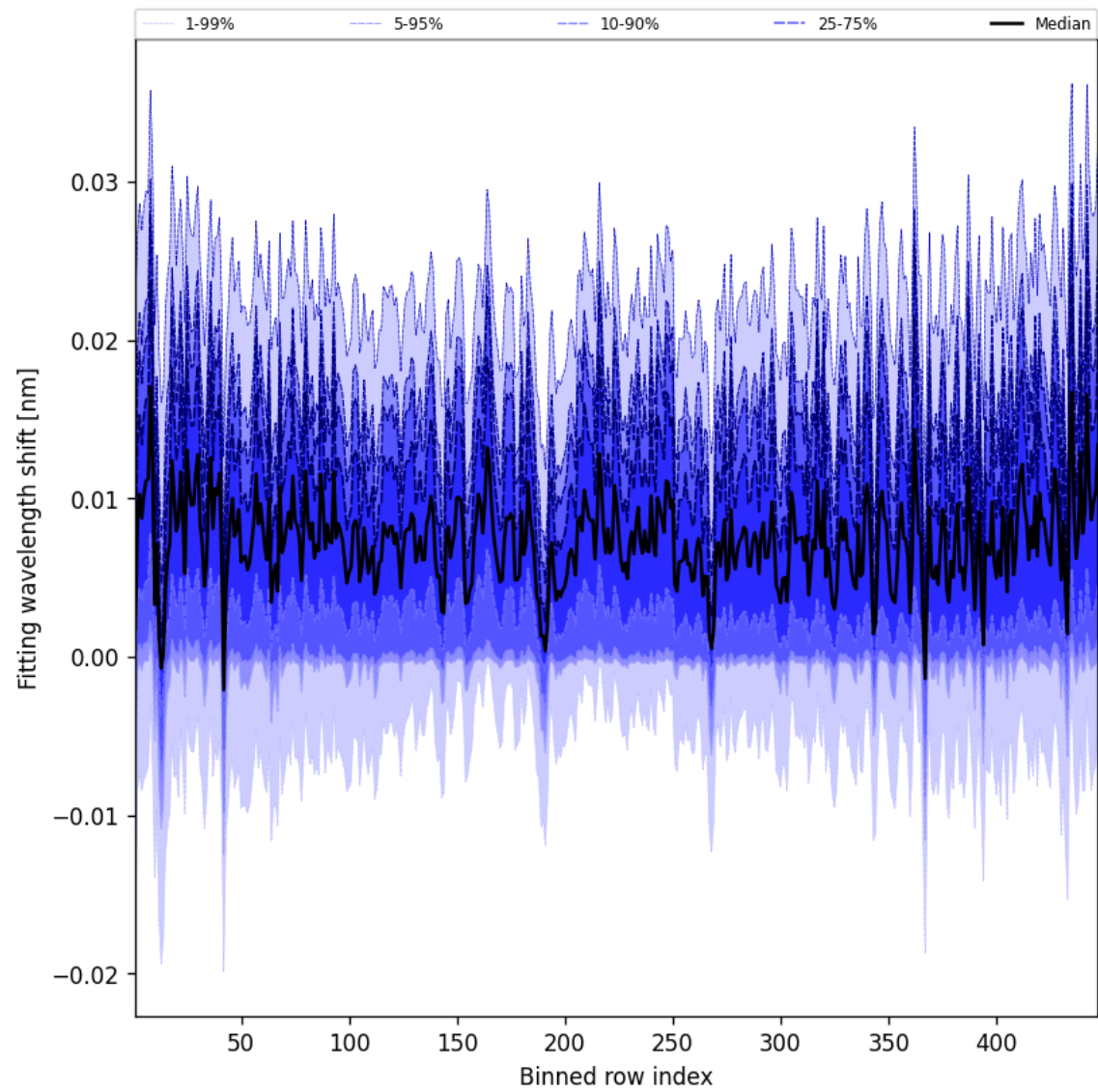
Figure 63: Along track statistics of “Fitting wavelength shift” for 2025-08-13 to 2025-08-14
