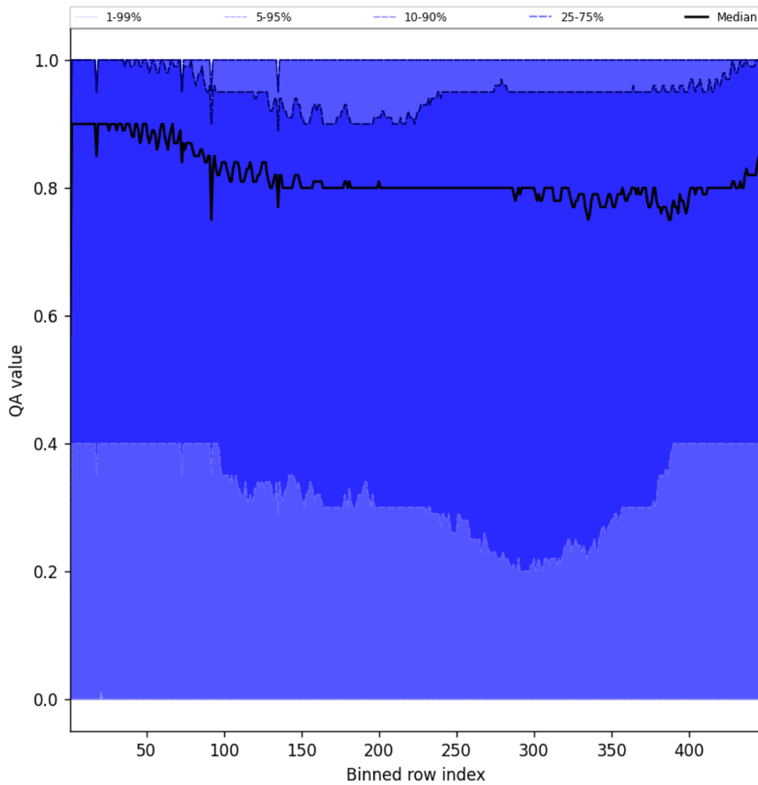
Figure 52: Along track statistics of “QA value” for 2025-08-13 to 2025-08-14
