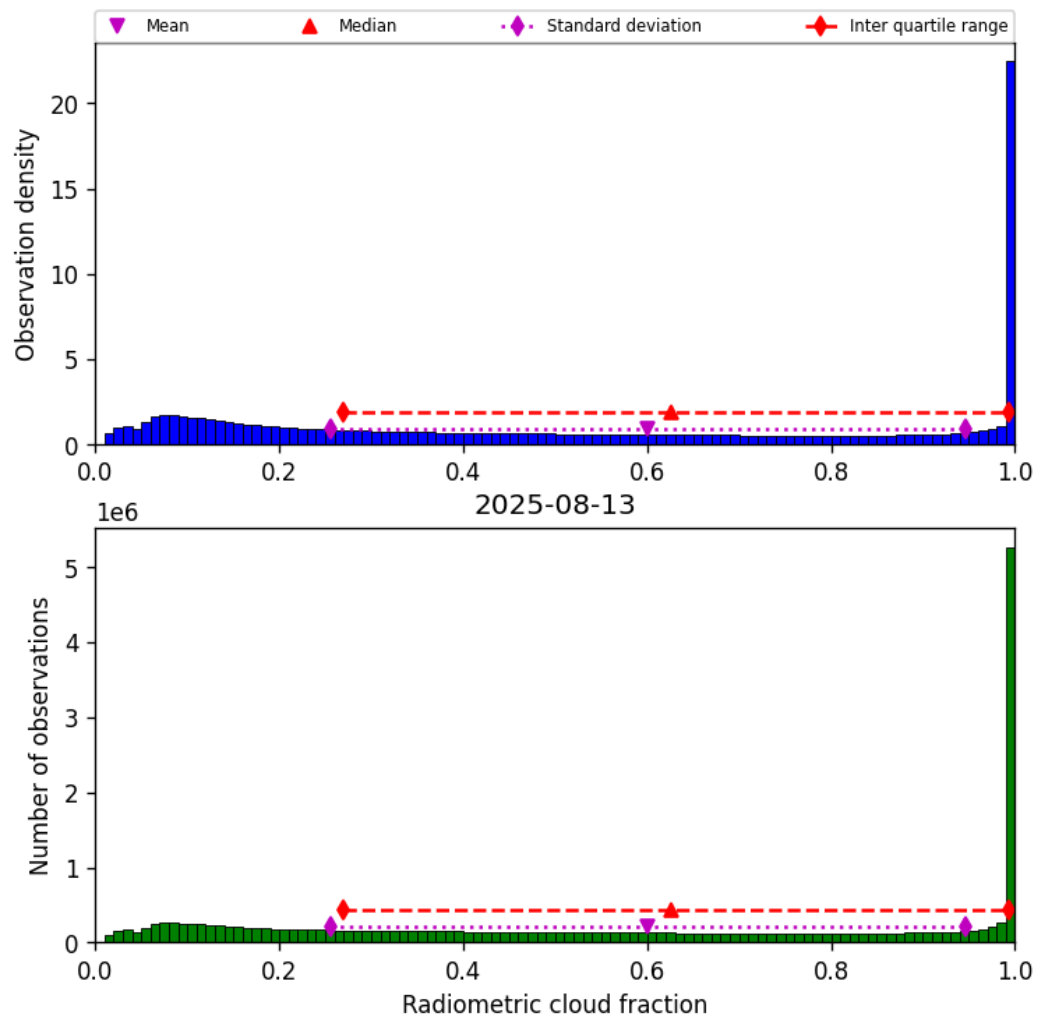
Figure 37: Histogram of “Radiometric cloud fraction” for 2025-08-13 to 2025-08-14
