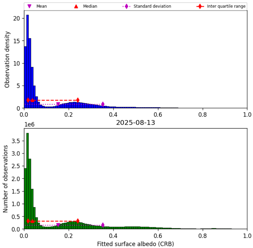
Figure 44: Histogram of “Fitted surface albedo (CRB)” for 2025-08-13 to 2025-08-14
