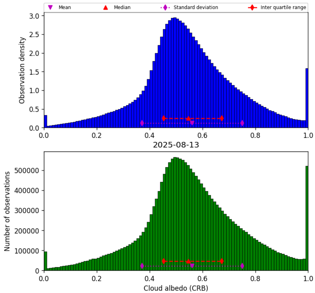
Figure 42: Histogram of “Cloud albedo (CRB)” for 2025-08-13 to 2025-08-14
