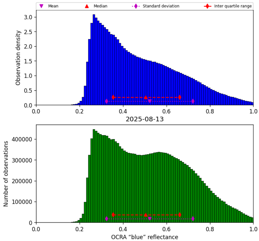
Figure 49: Histogram of “OCRA “blue” reflectance” for 2025-08-13 to 2025-08-14
