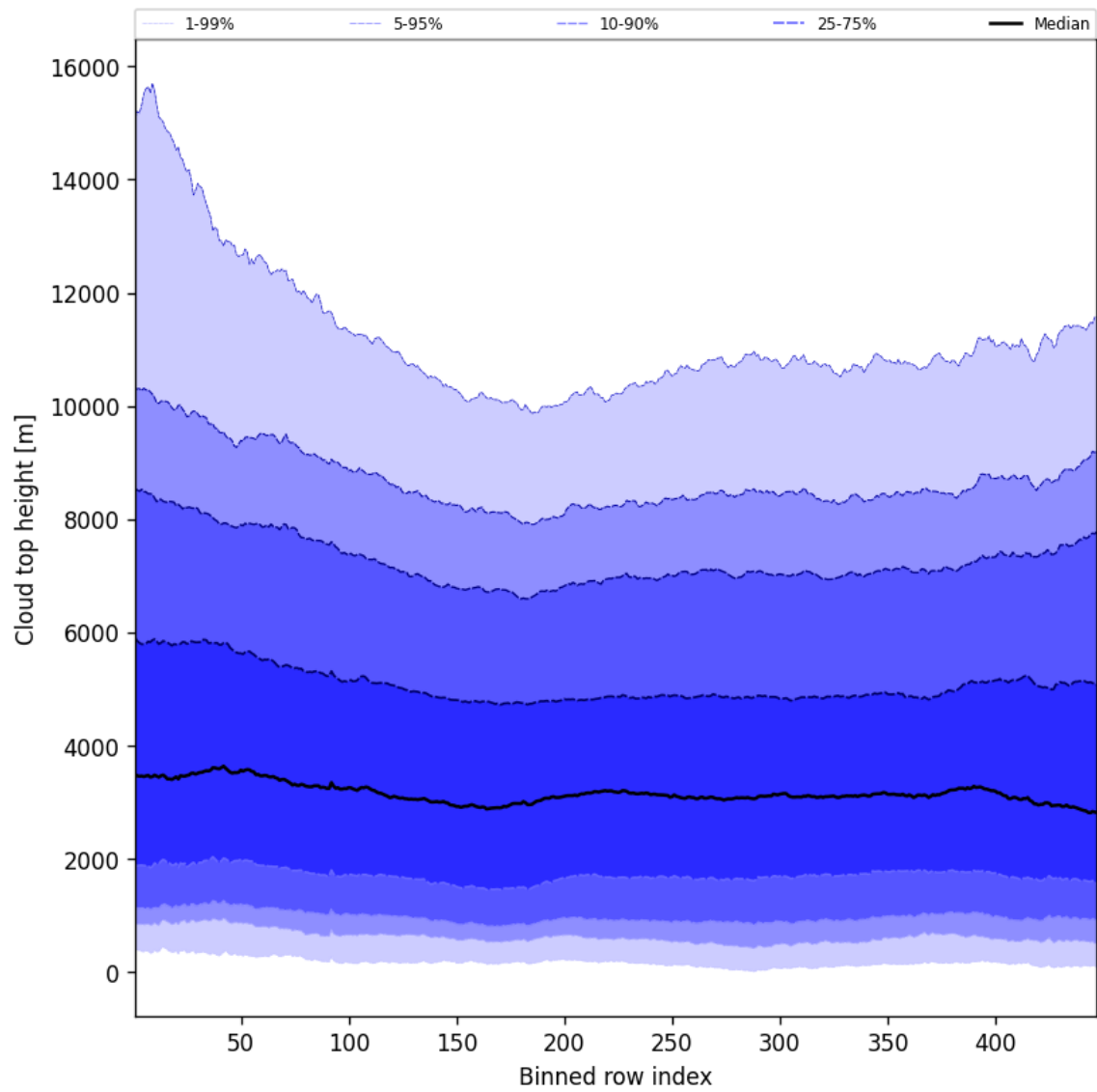
Figure 54: Along track statistics of “Cloud top height” for 2025-08-13 to 2025-08-14
