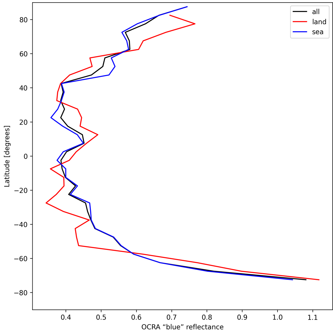
Figure 33: Zonal average of “OCRA “blue” reflectance” for 2025-08-13 to 2025-08-14.
