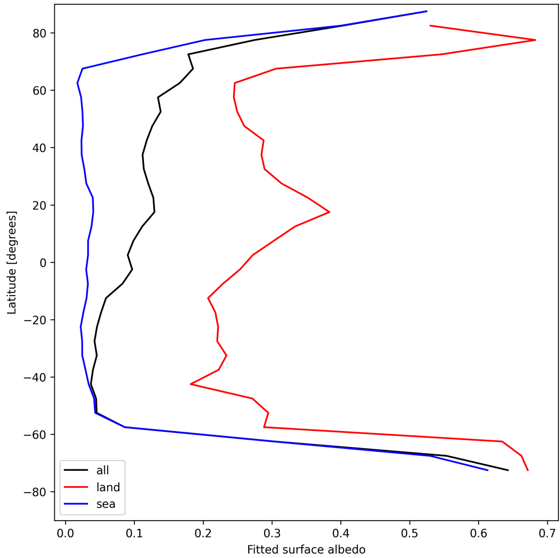
Figure 27: Zonal average of “Fitted surface albedo” for 2025-08-13 to 2025-08-14.
