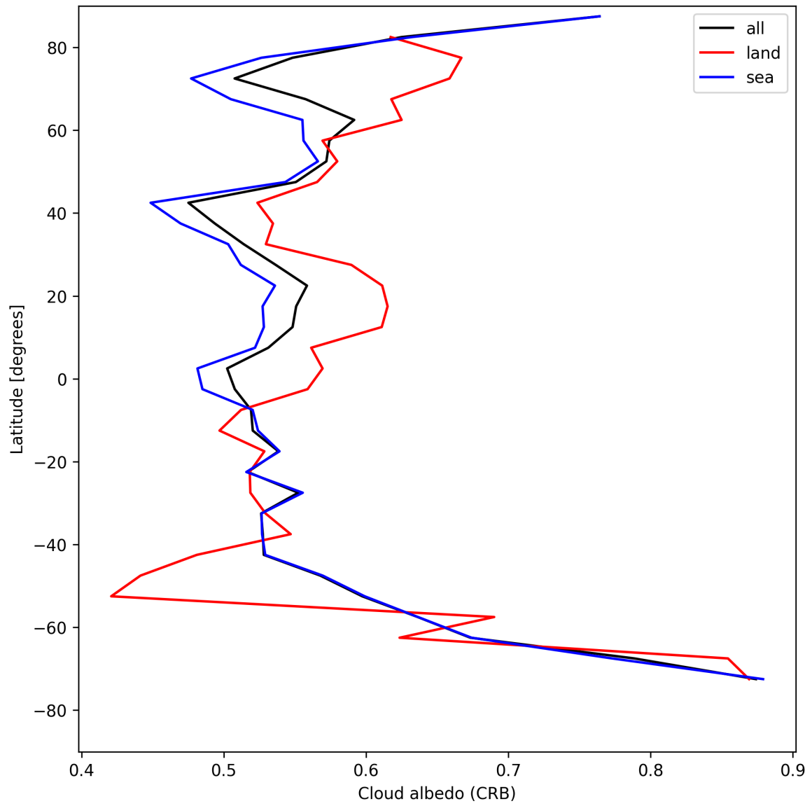
Figure 26: Zonal average of “Cloud albedo (CRB)” for 2025-08-13 to 2025-08-14.
