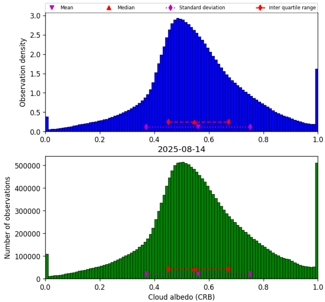
Figure 42: Histogram of “Cloud albedo (CRB)” for 2025-08-14 to 2025-08-15
