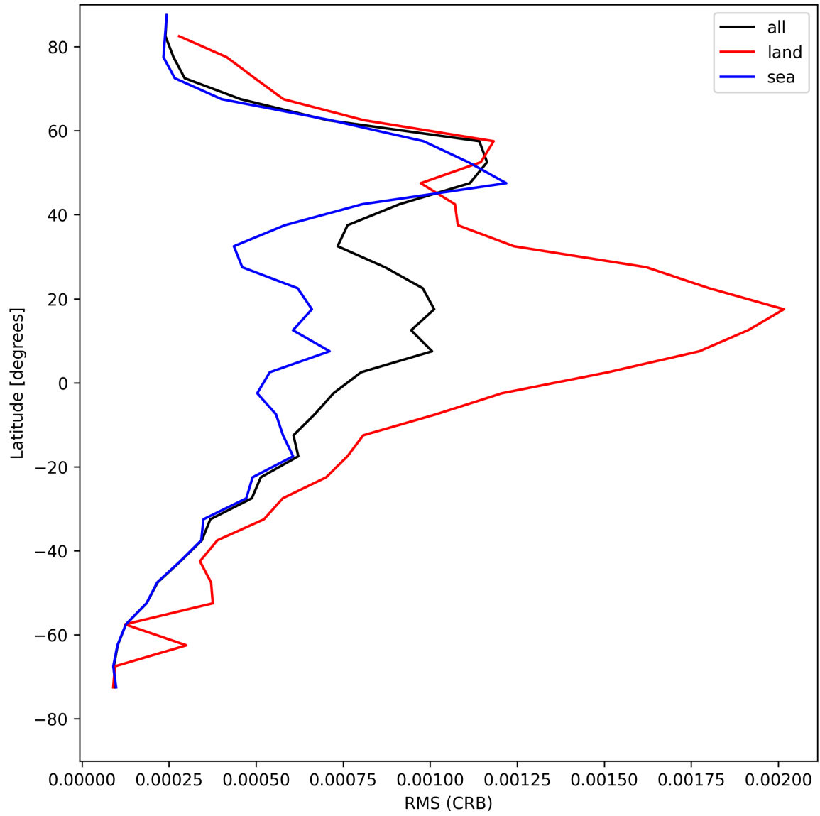
Figure 30: Zonal average of “RMS (CRB)” for 2025-08-14 to 2025-08-15.
