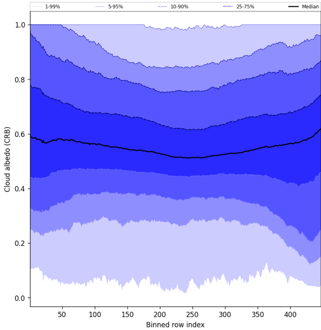
Figure 58: Along track statistics of “Cloud albedo (CRB)” for 2025-08-14 to 2025-08-15
