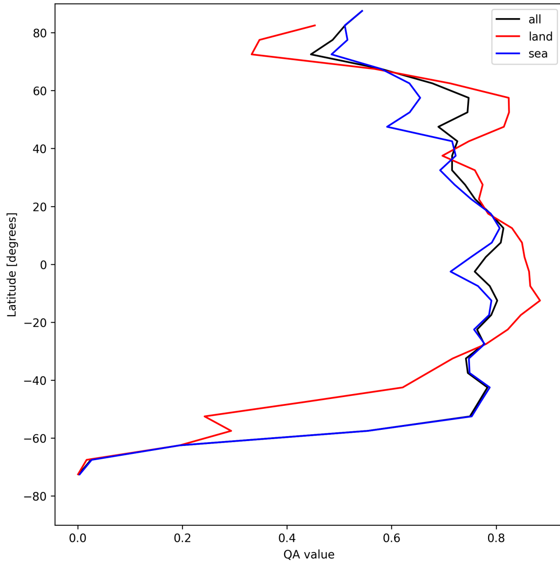
Figure 20: Zonal average of “QA value” for 2025-08-14 to 2025-08-15.
