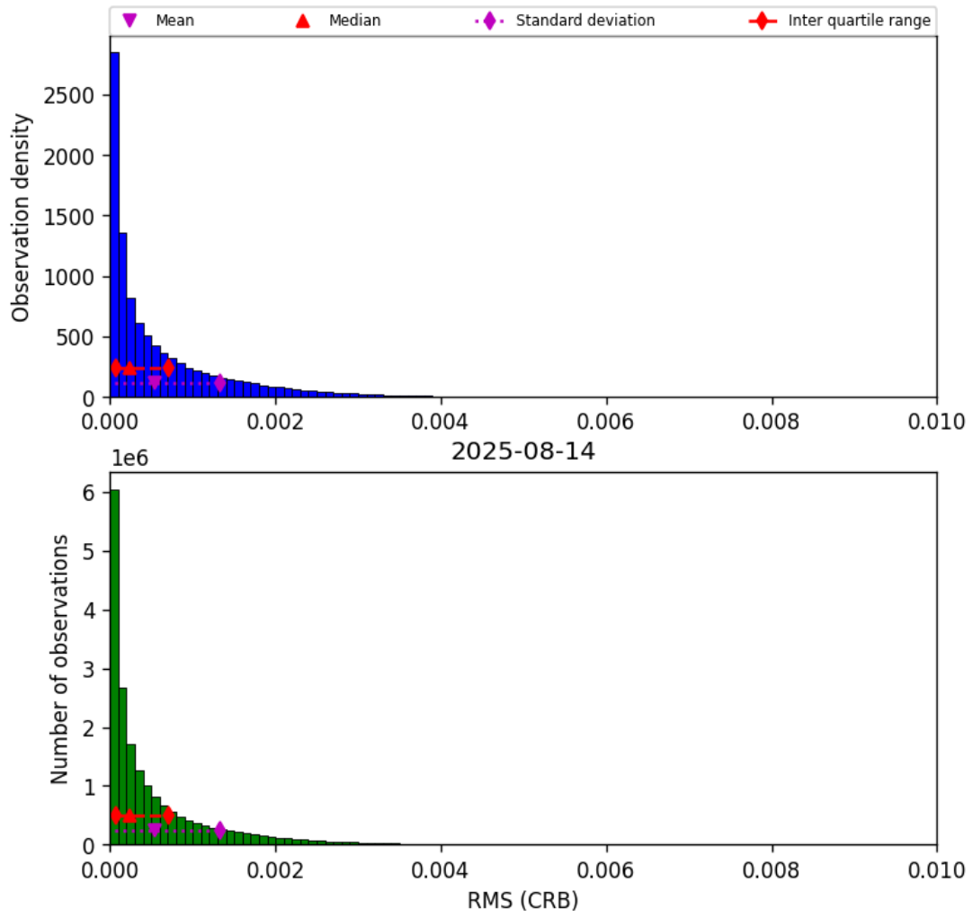
Figure 46: Histogram of “RMS (CRB)” for 2025-08-14 to 2025-08-15
