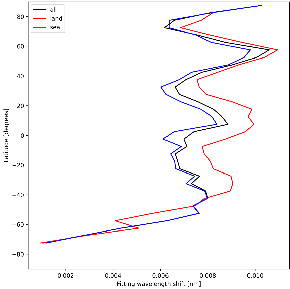
Figure 31: Zonal average of “Fitting wavelength shift” for 2025-08-14 to 2025-08-15.
