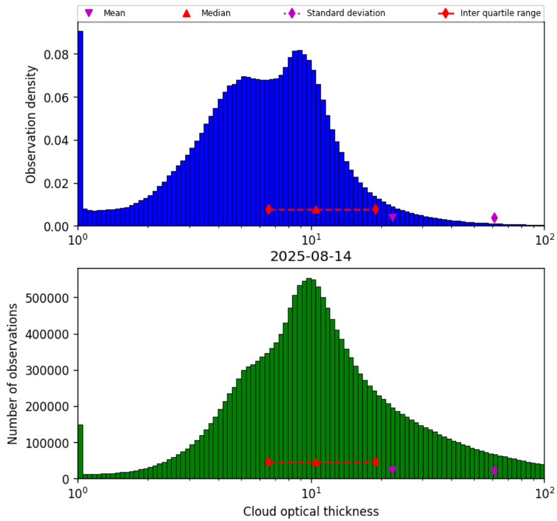
Figure 39: Histogram of “Cloud optical thickness” for 2025-08-14 to 2025-08-15
