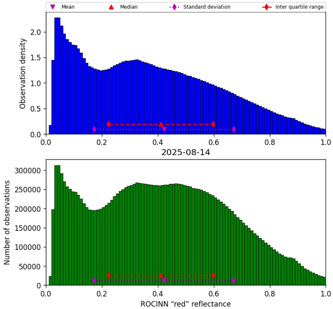
Figure 51: Histogram of “ROCINN “red” reflectance” for 2025-08-14 to 2025-08-15
