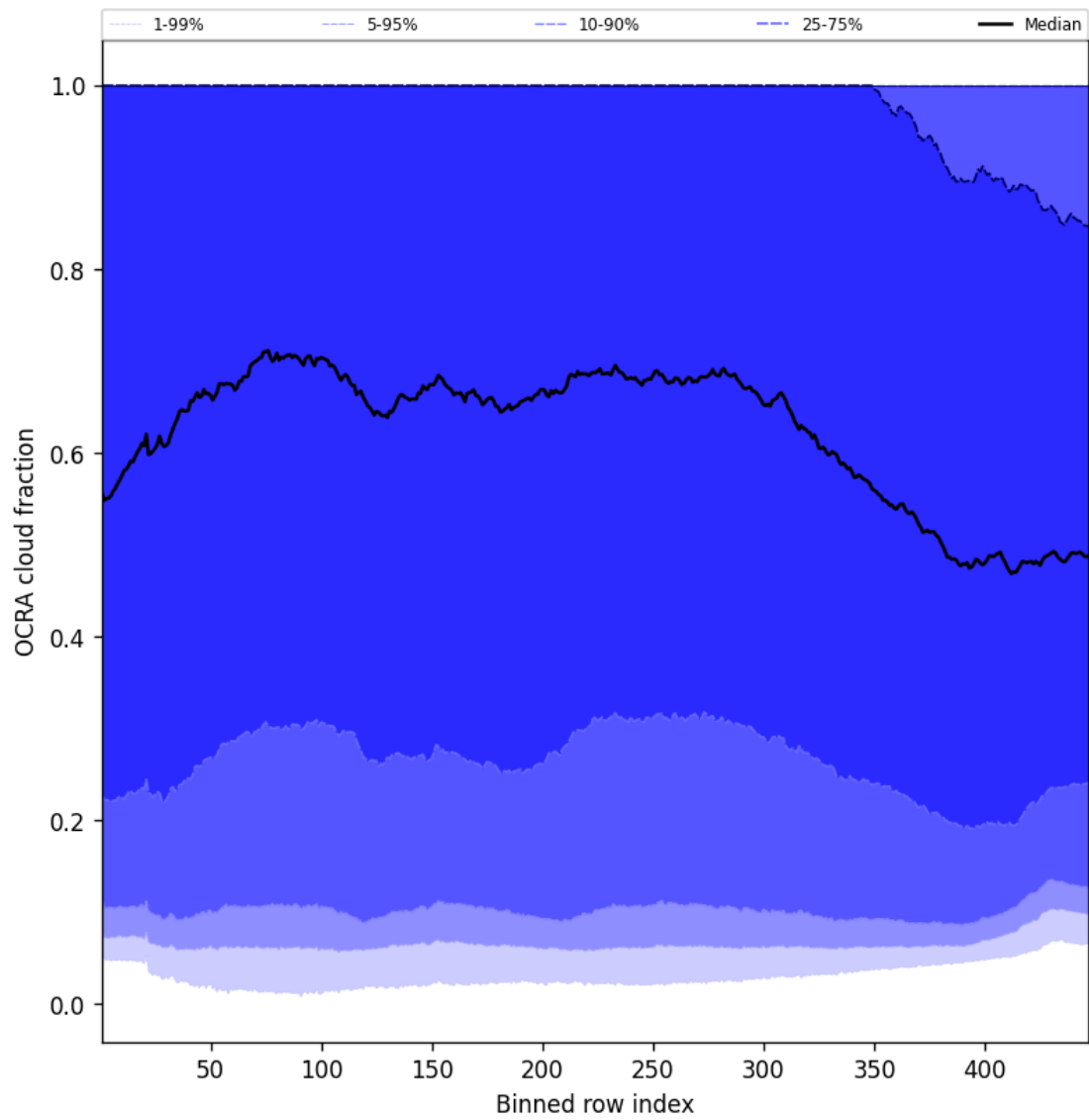
Figure 64: Along track statistics of “OCRA cloud fraction” for 2025-08-14 to 2025-08-15
