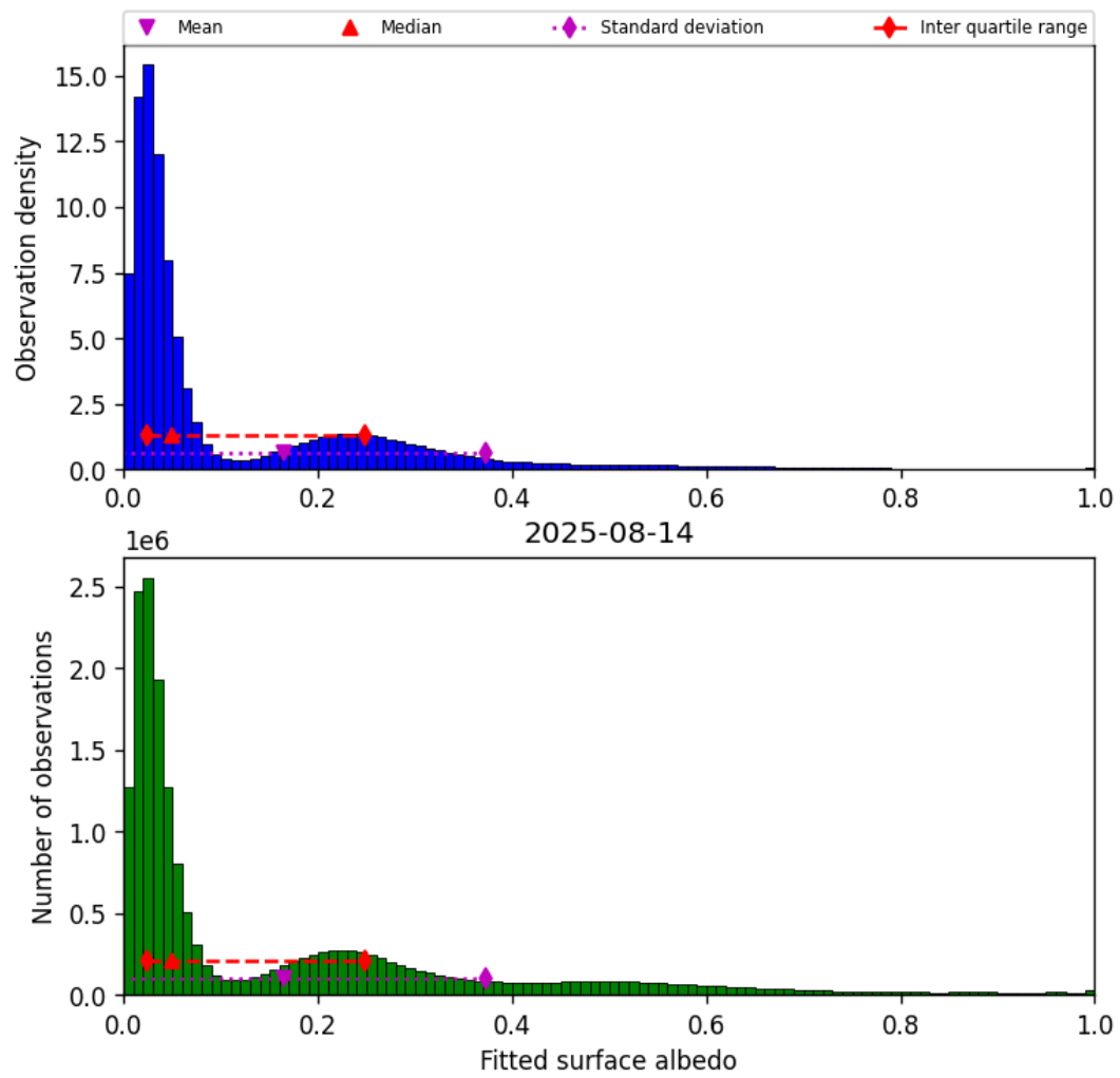
Figure 43: Histogram of “Fitted surface albedo” for 2025-08-14 to 2025-08-15
