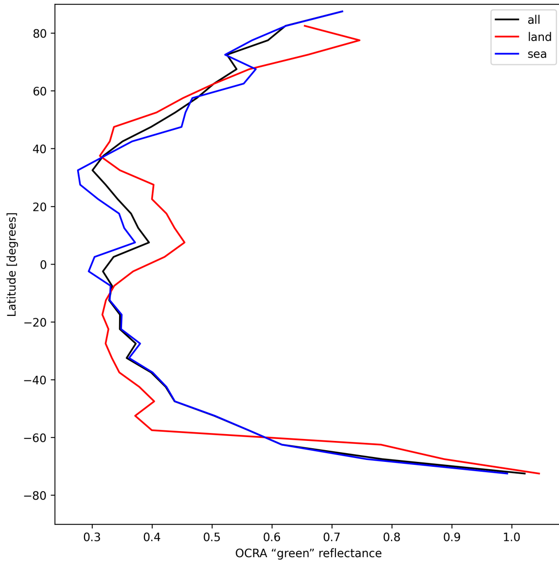
Figure 34: Zonal average of “OCRA “green” reflectance” for 2025-08-14 to 2025-08-15.
