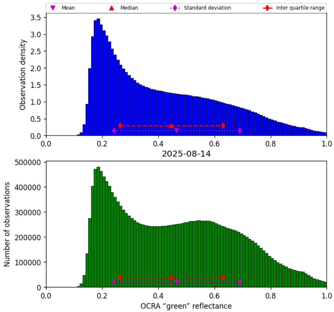
Figure 50: Histogram of “OCRA “green” reflectance” for 2025-08-14 to 2025-08-15
