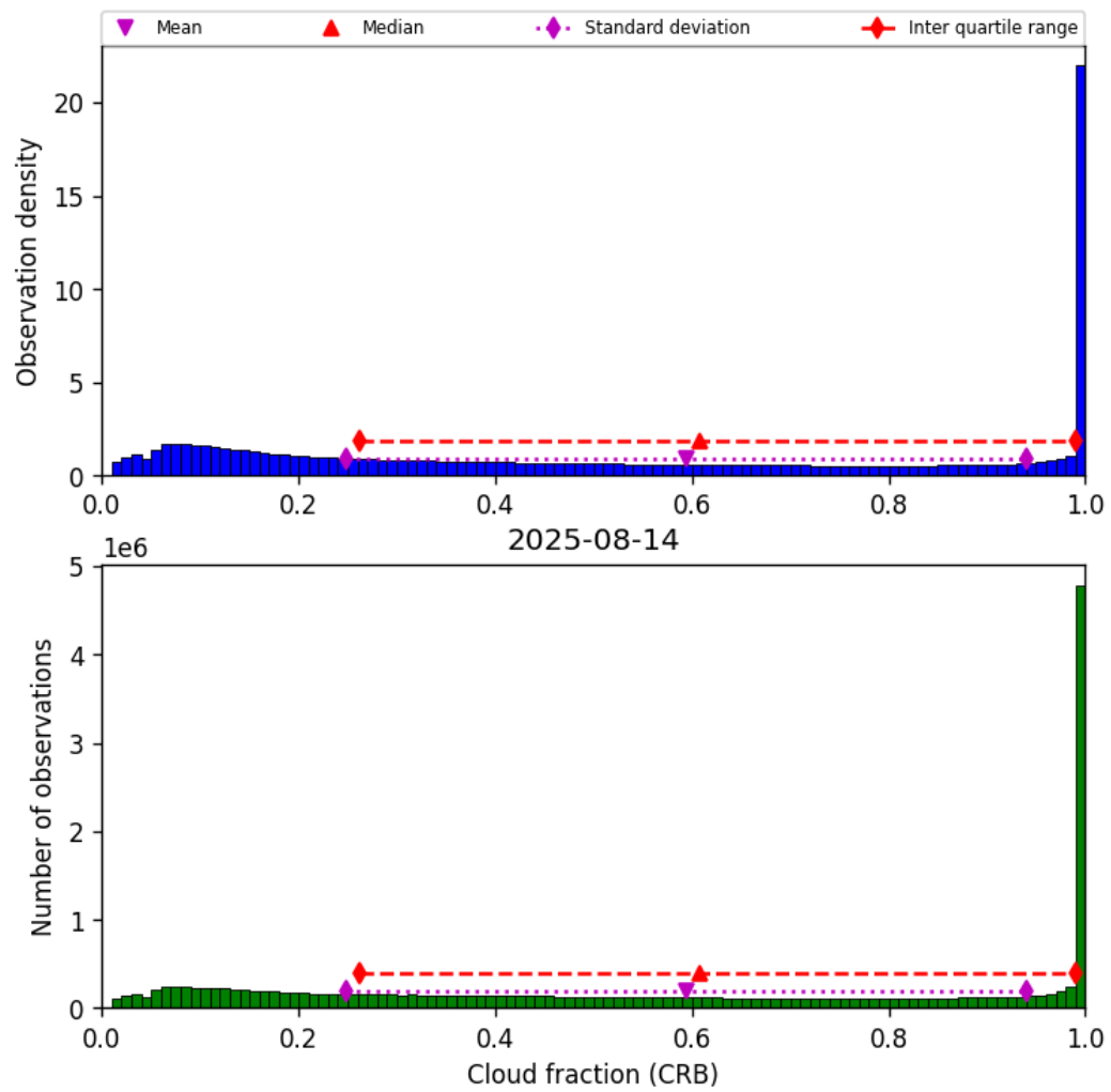
Figure 40: Histogram of “Cloud fraction (CRB)” for 2025-08-14 to 2025-08-15
