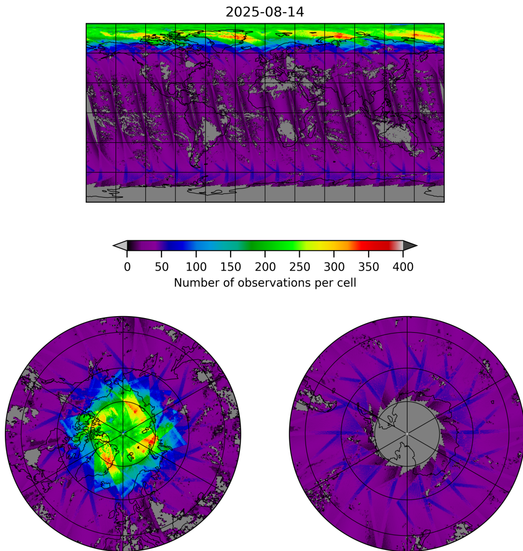
Figure 19: Map of the number of observations for 2025-08-14 to 2025-08-15
