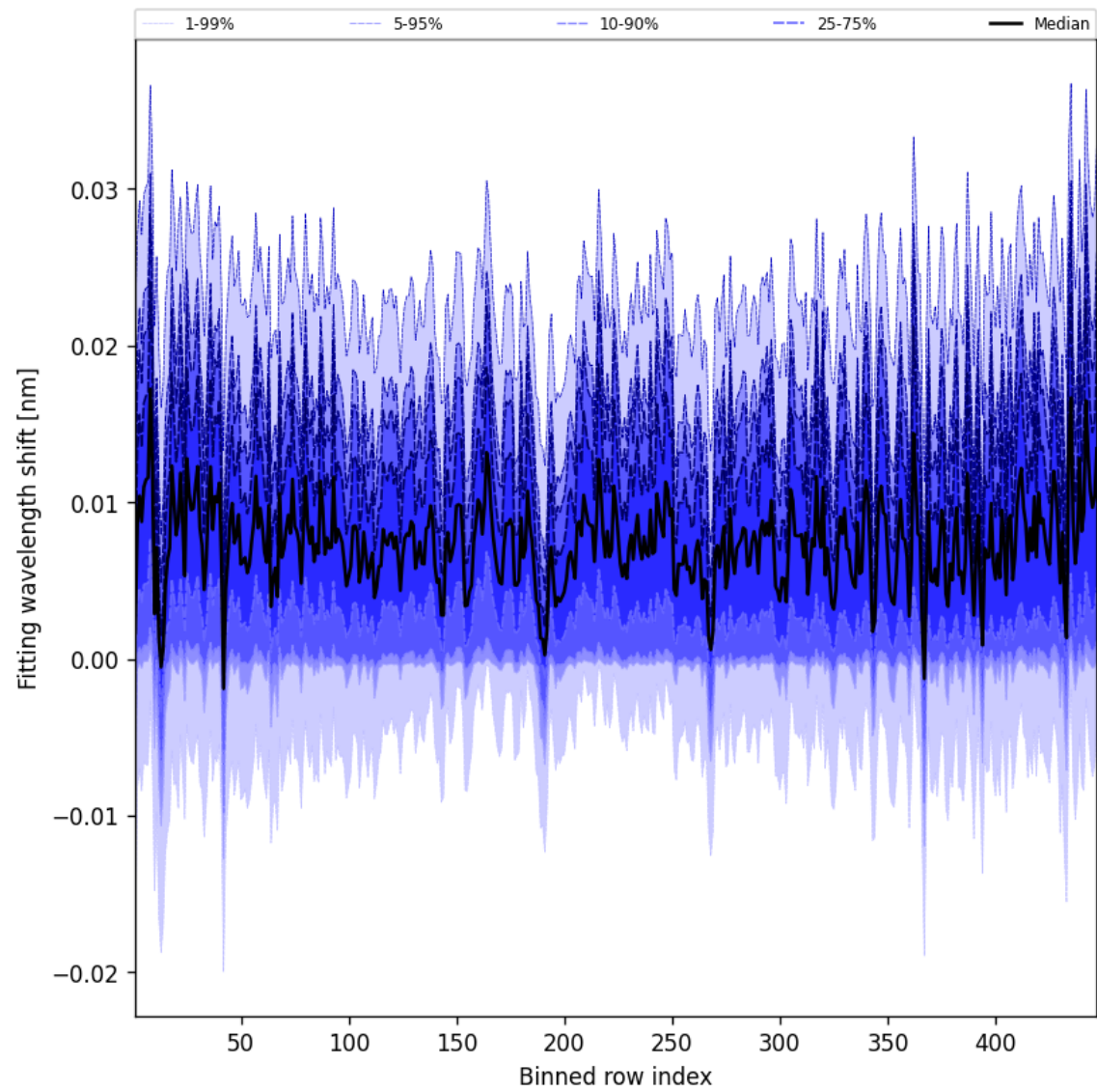
Figure 63: Along track statistics of “Fitting wavelength shift” for 2025-08-14 to 2025-08-15
