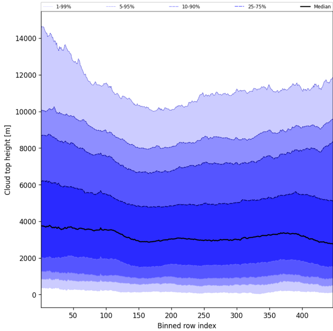
Figure 54: Along track statistics of “Cloud top height” for 2025-08-14 to 2025-08-15
