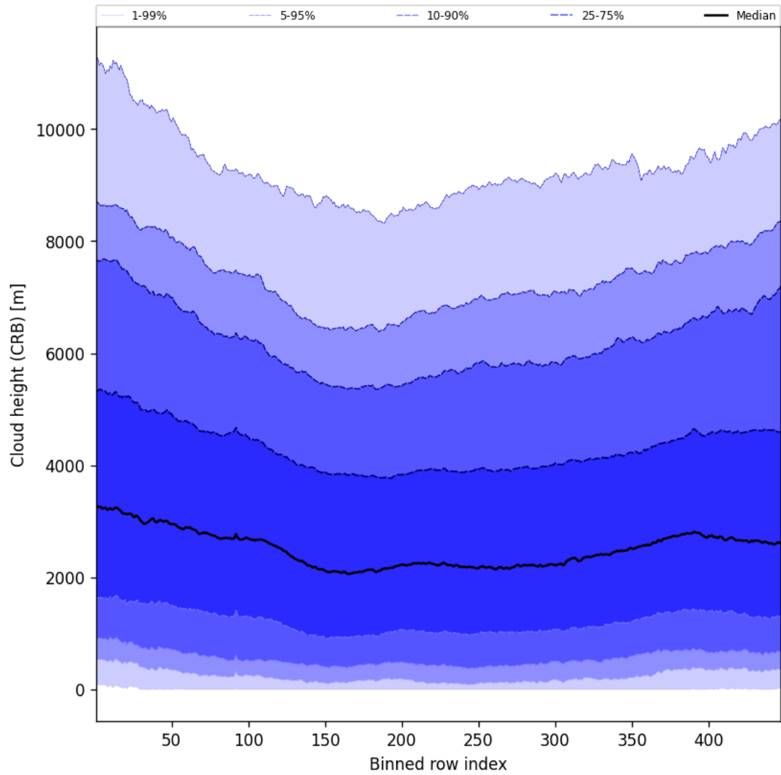
Figure 57: Along track statistics of “Cloud height (CRB)” for 2025-08-14 to 2025-08-15
