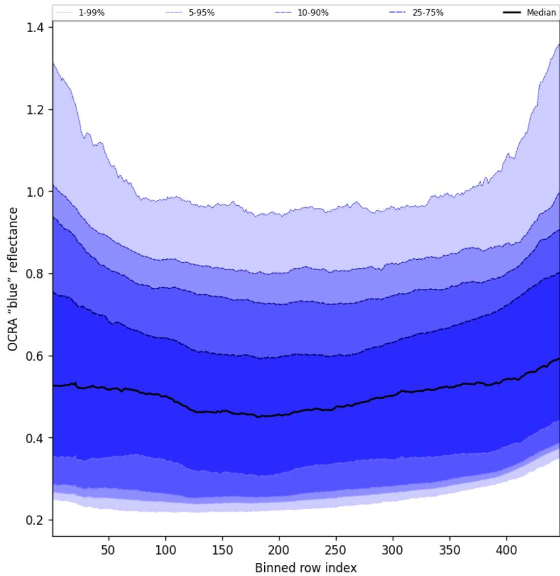
Figure 65: Along track statistics of “OCRA “blue” reflectance” for 2025-08-14 to 2025-08-15
