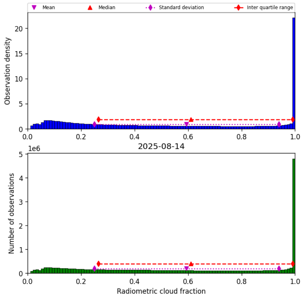
Figure 37: Histogram of “Radiometric cloud fraction” for 2025-08-14 to 2025-08-15
