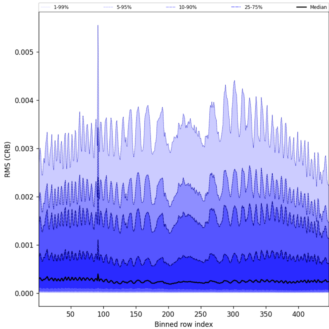
Figure 62: Along track statistics of “RMS (CRB)” for 2025-08-14 to 2025-08-15
