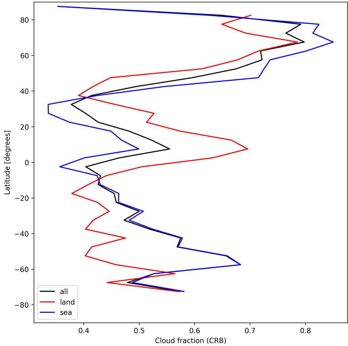
Figure 24: Zonal average of “Cloud fraction (CRB)” for 2025-08-14 to 2025-08-15.
