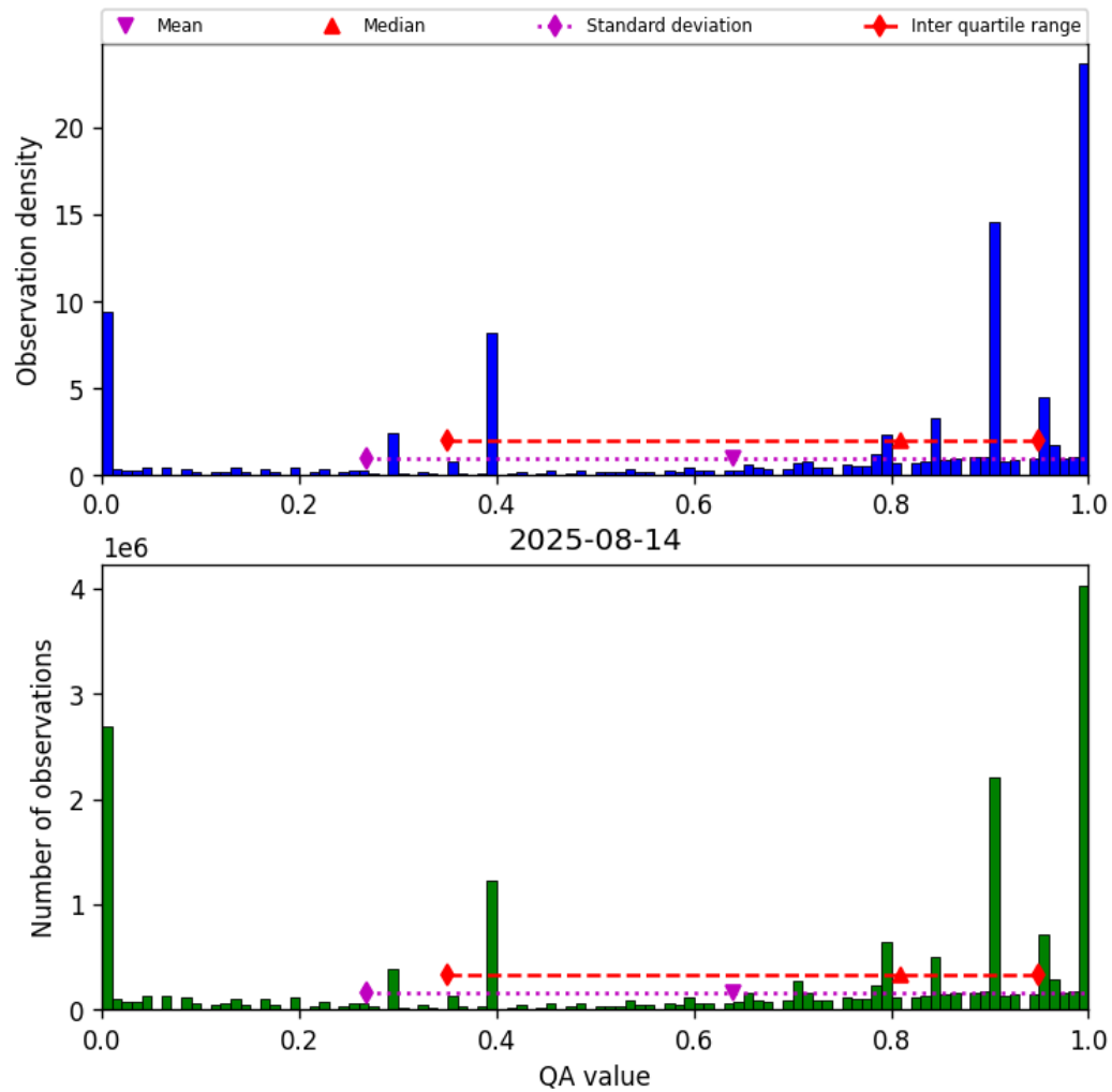
Figure 36: Histogram of “QA value” for 2025-08-14 to 2025-08-15
