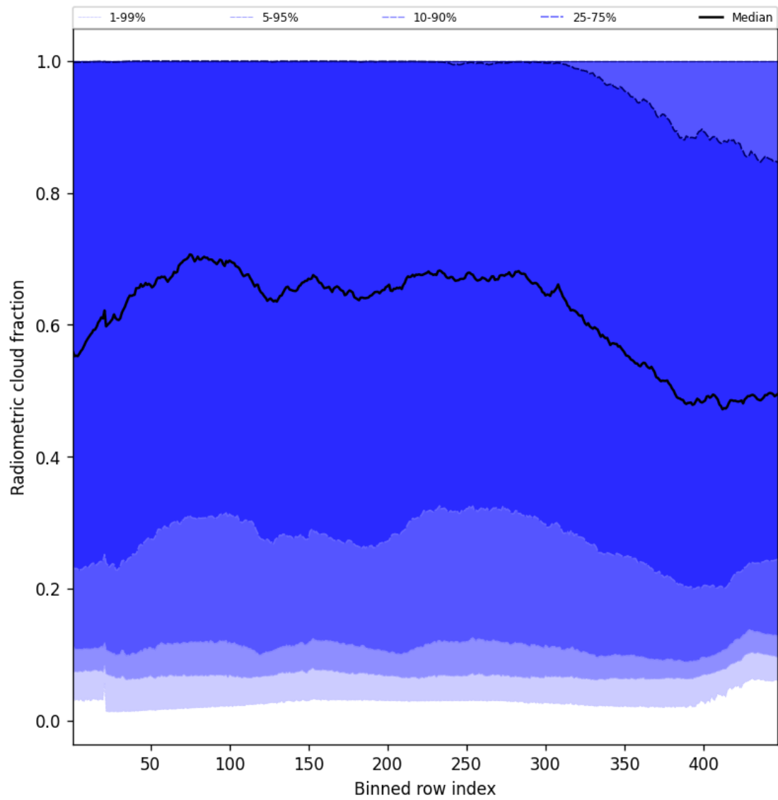
Figure 53: Along track statistics of “Radiometric cloud fraction” for 2025-08-14 to 2025-08-15
