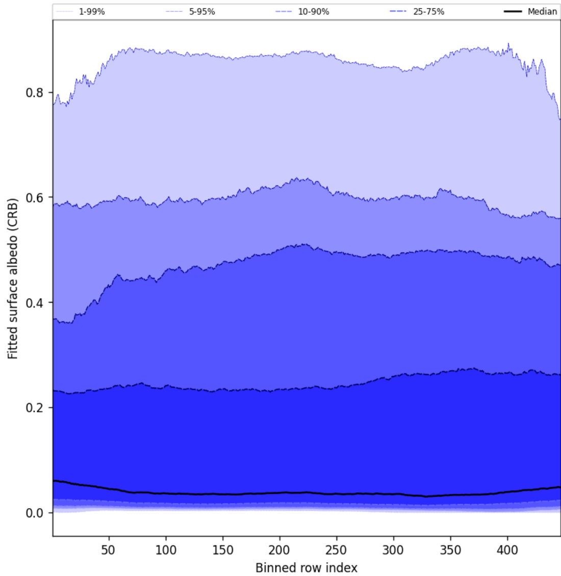
Figure 60: Along track statistics of “Fitted surface albedo (CRB)” for 2025-08-14 to 2025-08-15
