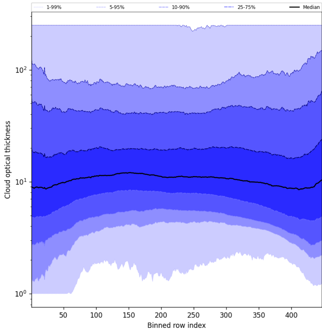
Figure 55: Along track statistics of “Cloud optical thickness” for 2025-08-14 to 2025-08-15
