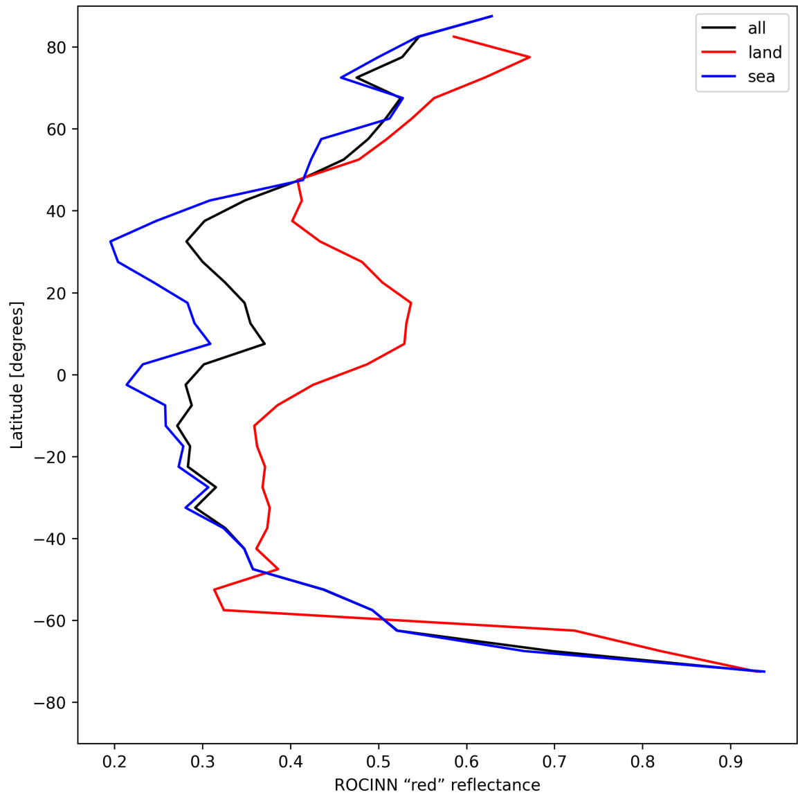
Figure 35: Zonal average of "ROCINN "red" reflectance" for 2025-08-14 to 2025-08-15.
