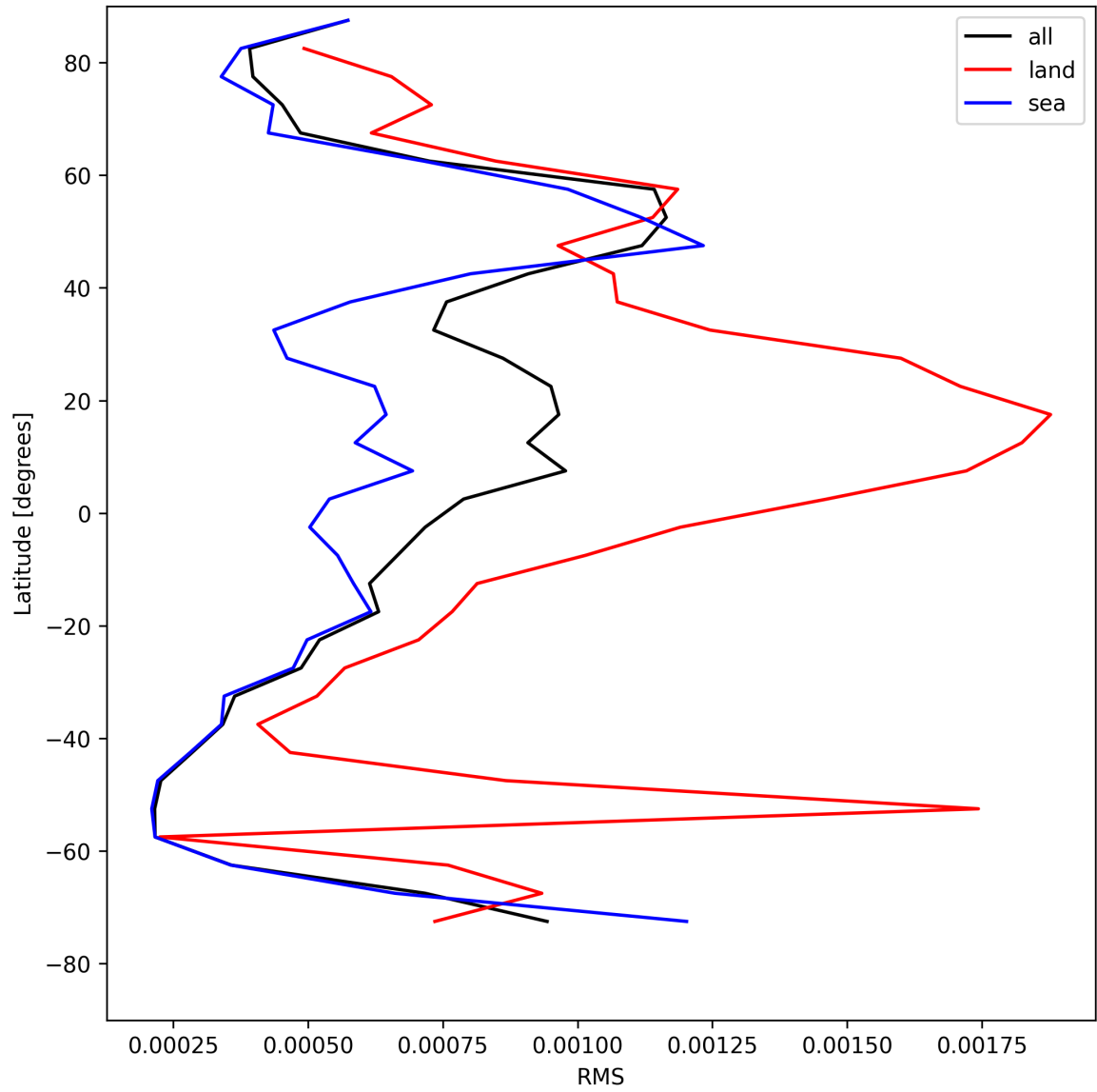
Figure 29: Zonal average of “RMS” for 2025-08-14 to 2025-08-15.
