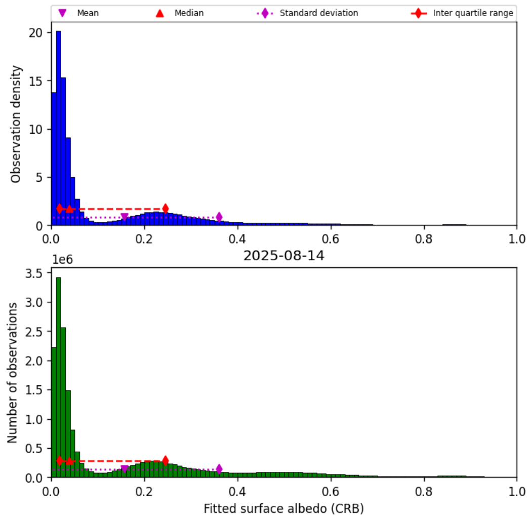
Figure 44: Histogram of “Fitted surface albedo (CRB)” for 2025-08-14 to 2025-08-15
