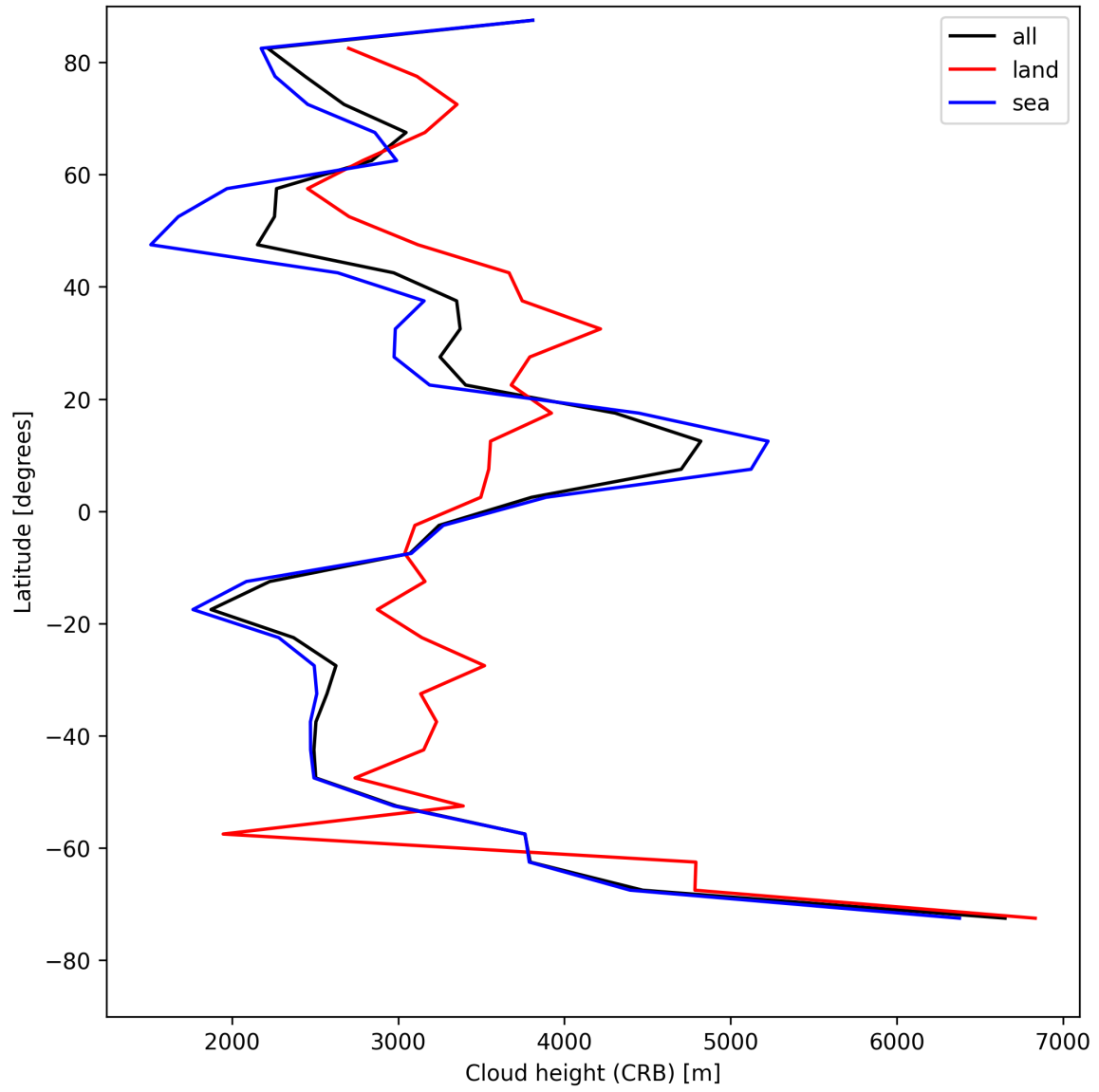
Figure 25: Zonal average of “Cloud height (CRB)” for 2025-08-14 to 2025-08-15.
