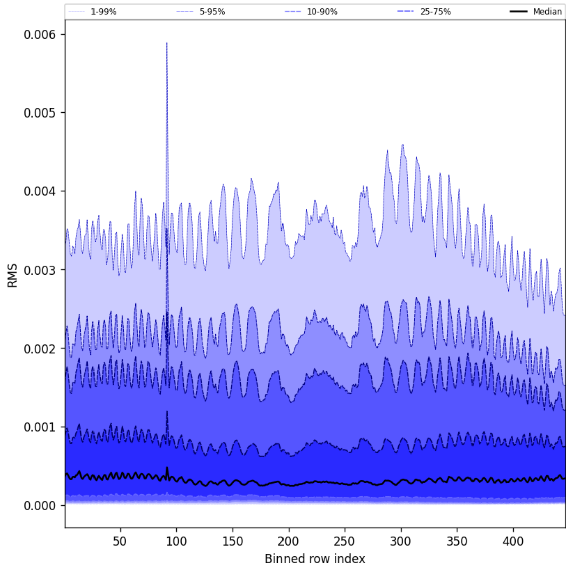
Figure 61: Along track statistics of “RMS” for 2025-08-14 to 2025-08-15
