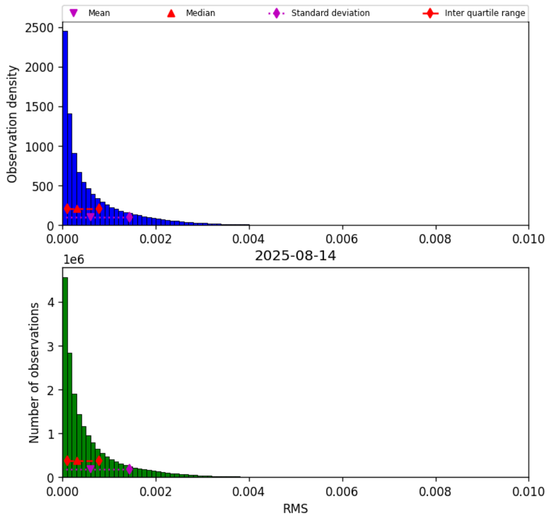
Figure 45: Histogram of “RMS” for 2025-08-14 to 2025-08-15
