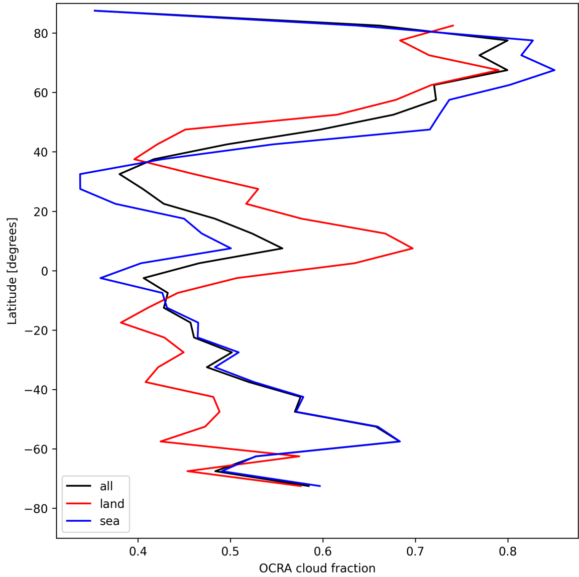
Figure 32: Zonal average of “OCRA cloud fraction” for 2025-08-14 to 2025-08-15.
