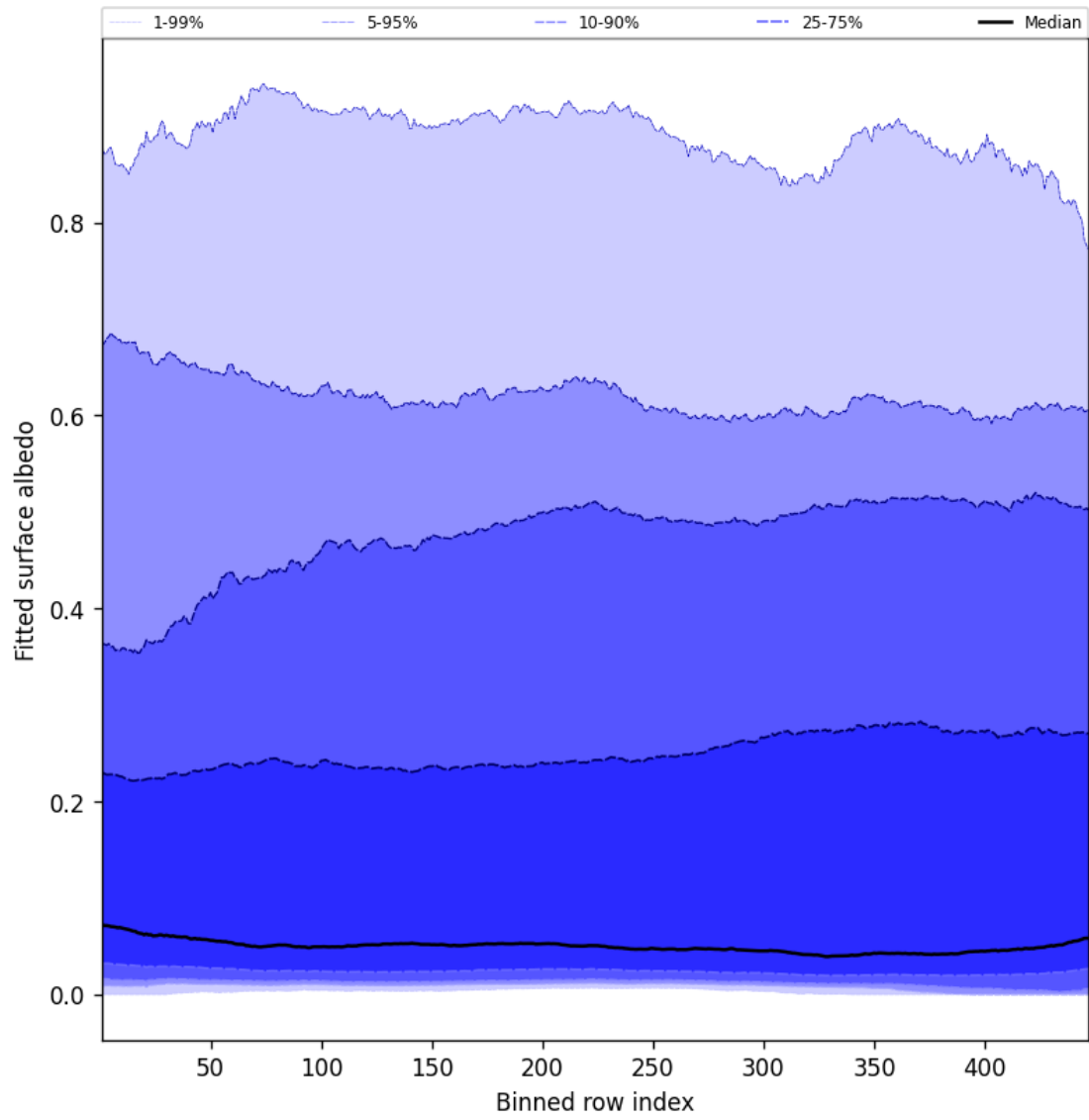
Figure 59: Along track statistics of “Fitted surface albedo” for 2025-08-14 to 2025-08-15
