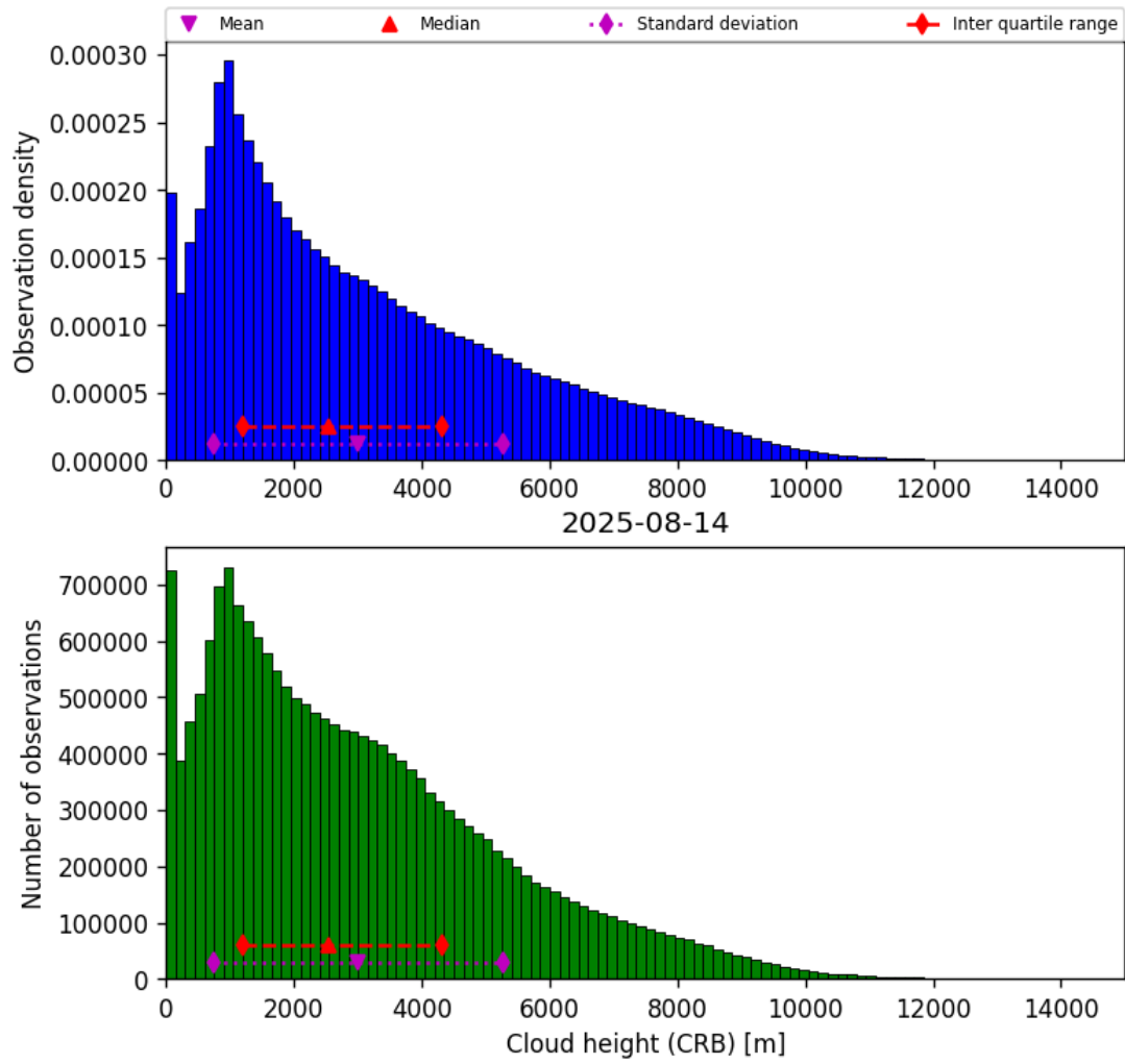
Figure 41: Histogram of “Cloud height (CRB)” for 2025-08-14 to 2025-08-15
