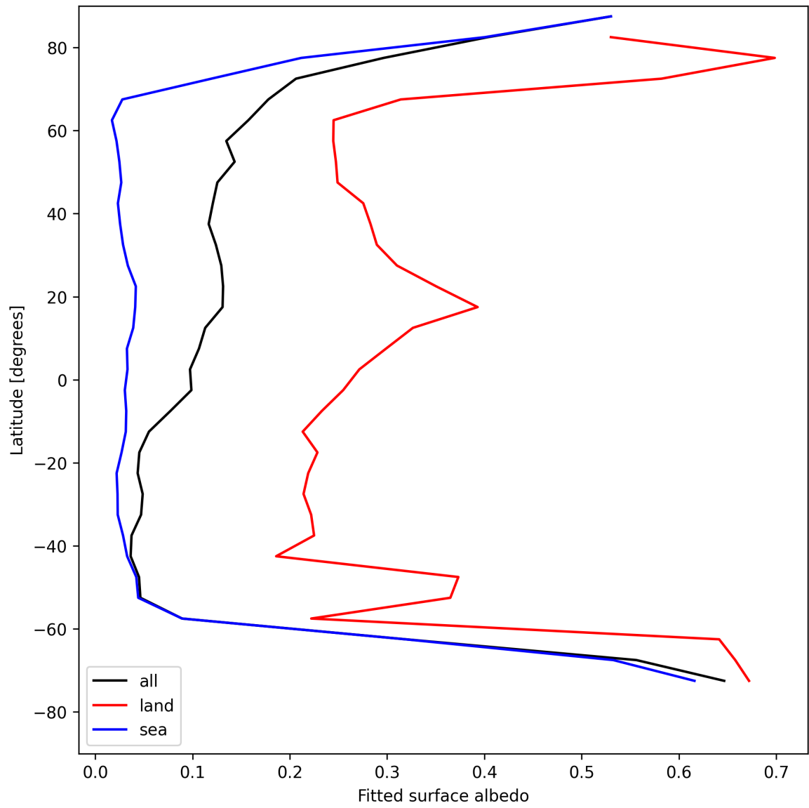
Figure 27: Zonal average of “Fitted surface albedo” for 2025-08-14 to 2025-08-15.
