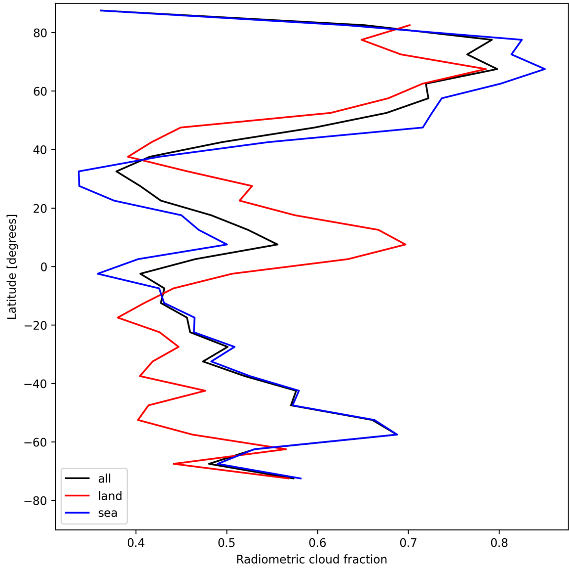
Figure 21: Zonal average of “Radiometric cloud fraction” for 2025-08-14 to 2025-08-15.
