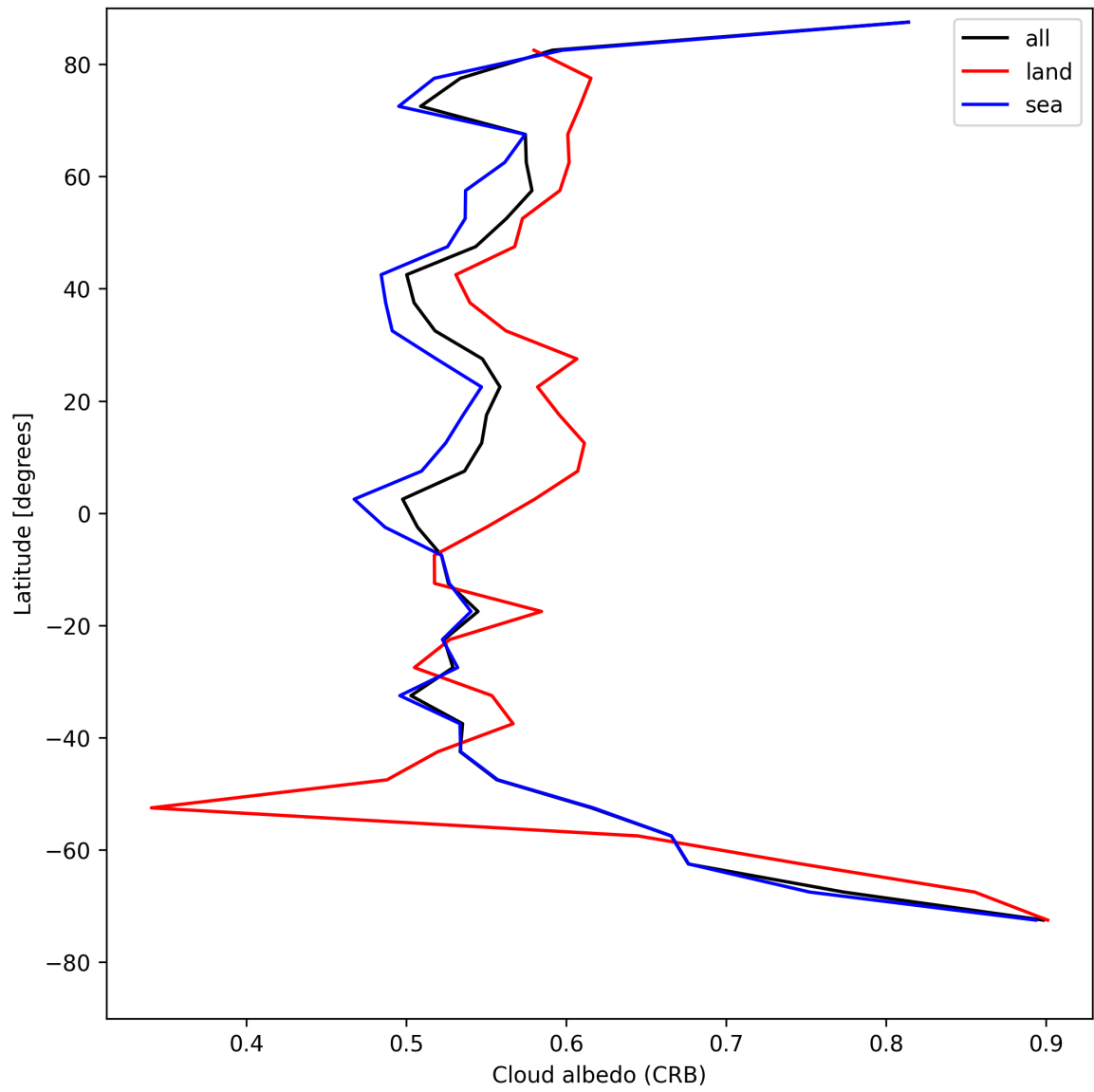
Figure 26: Zonal average of “Cloud albedo (CRB)” for 2025-08-14 to 2025-08-15.
