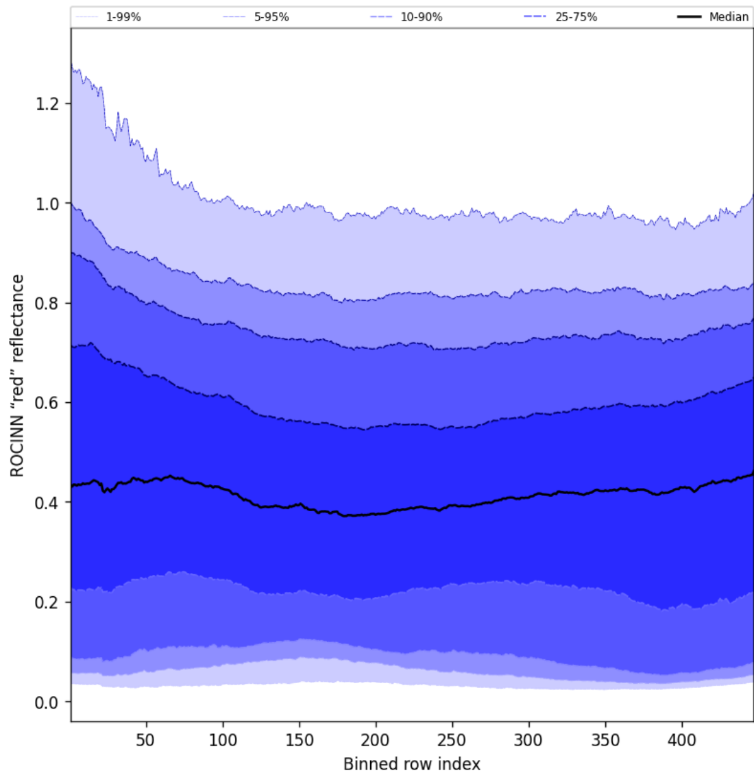
Figure 67: Along track statistics of “ROCINN “red” reflectance” for 2025-08-14 to 2025-08-15
