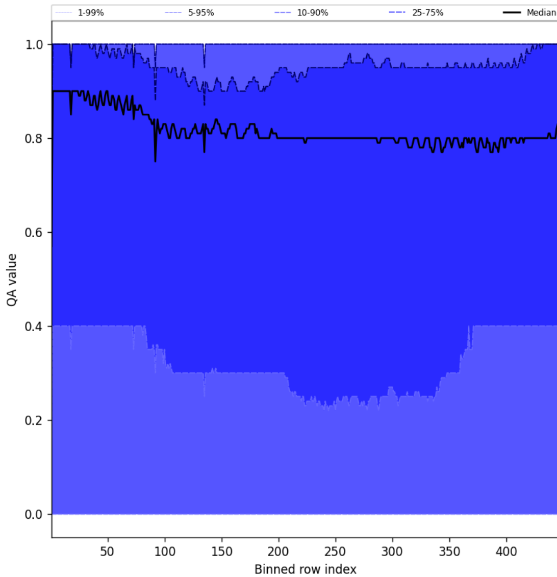
Figure 52: Along track statistics of “QA value” for 2025-08-14 to 2025-08-15
