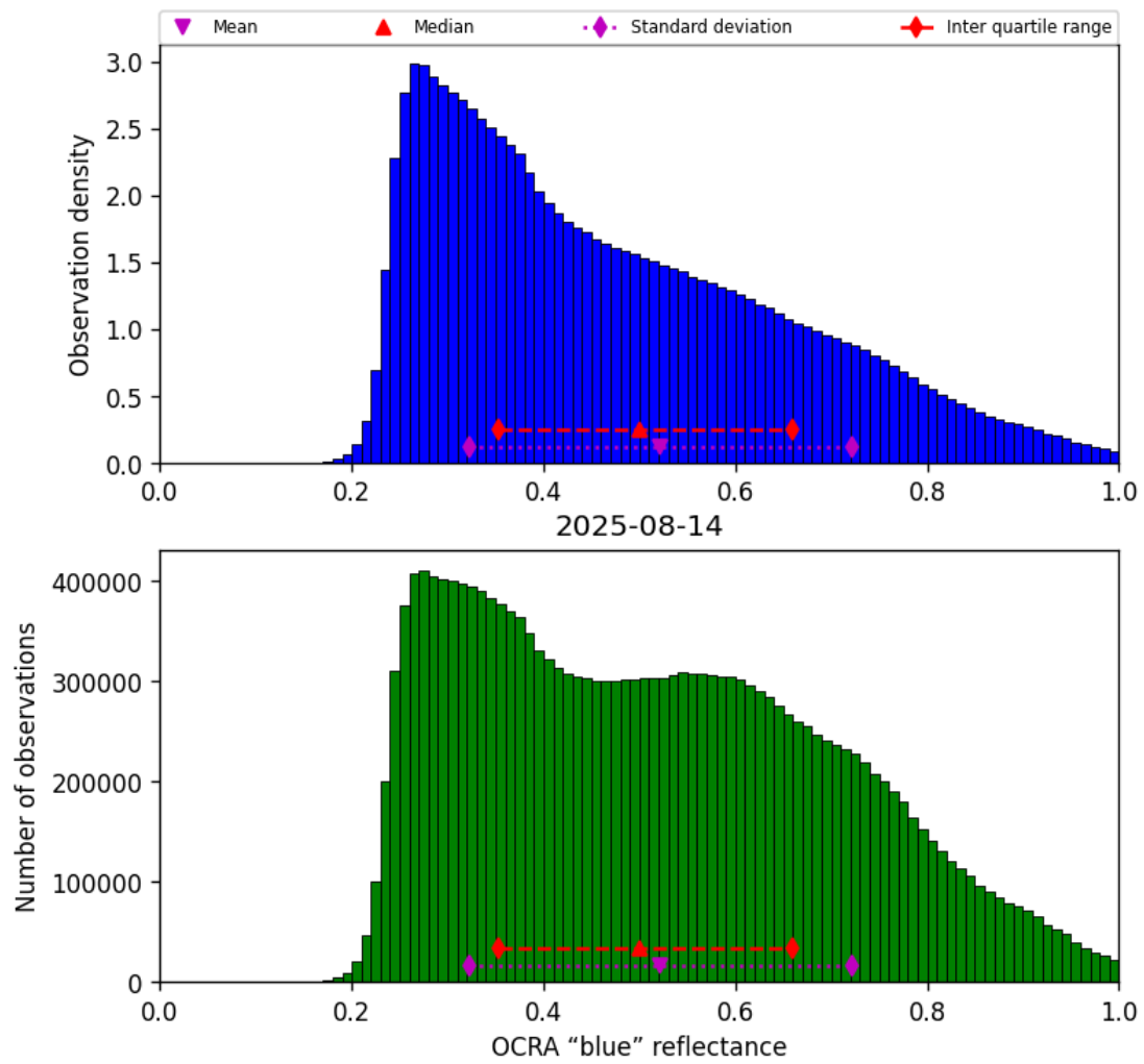
Figure 49: Histogram of “OCRA “blue” reflectance” for 2025-08-14 to 2025-08-15
