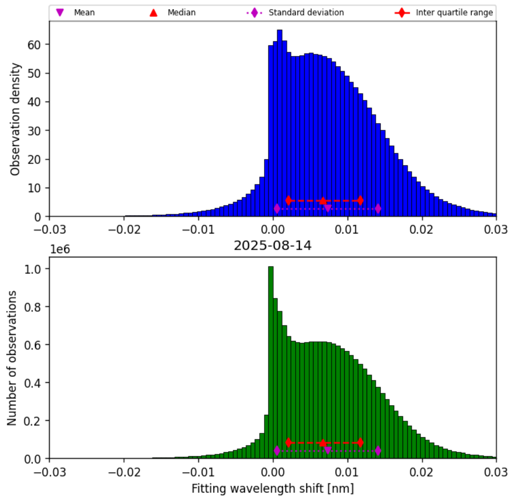
Figure 47: Histogram of “Fitting wavelength shift” for 2025-08-14 to 2025-08-15
