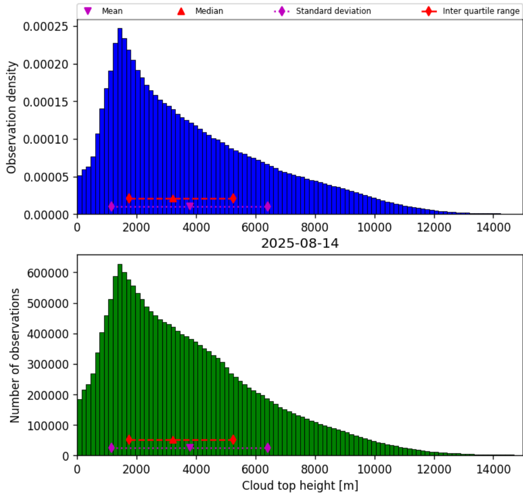
Figure 38: Histogram of “Cloud top height” for 2025-08-14 to 2025-08-15
