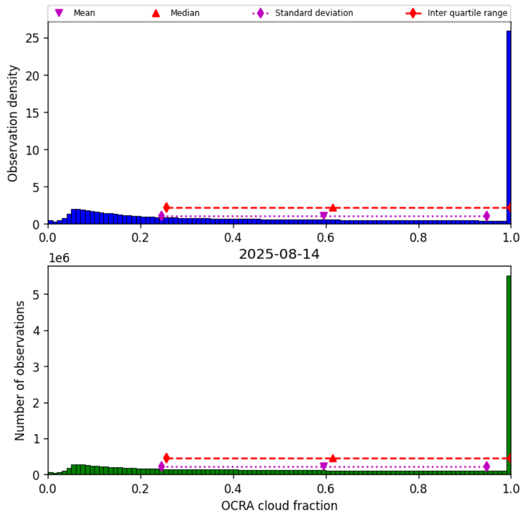
Figure 48: Histogram of “OCRA cloud fraction” for 2025-08-14 to 2025-08-15
