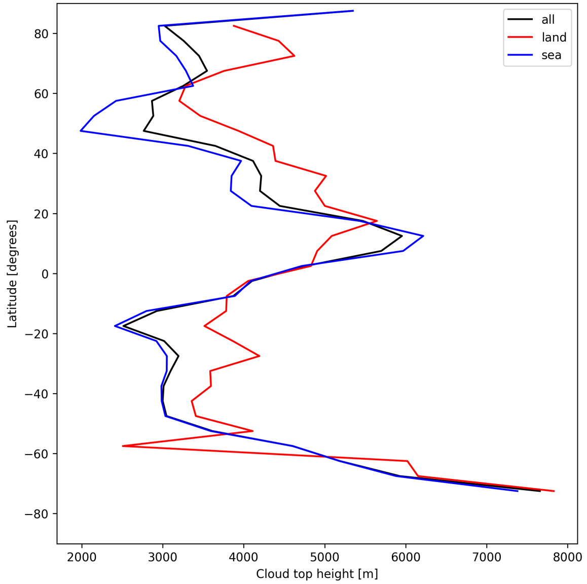
Figure 22: Zonal average of “Cloud top height” for 2025-08-14 to 2025-08-15.
