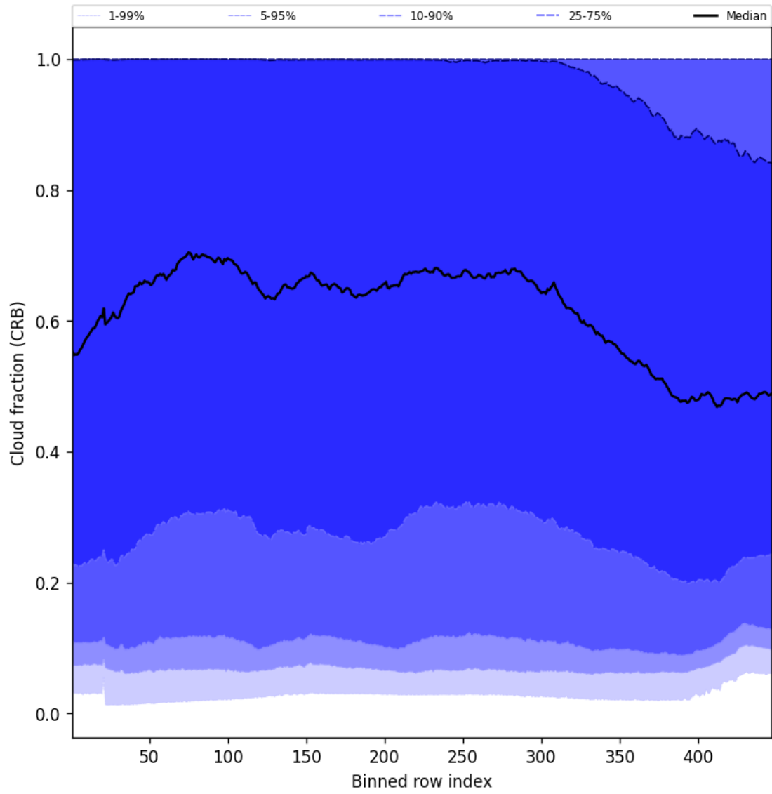
Figure 56: Along track statistics of “Cloud fraction (CRB)” for 2025-08-14 to 2025-08-15
