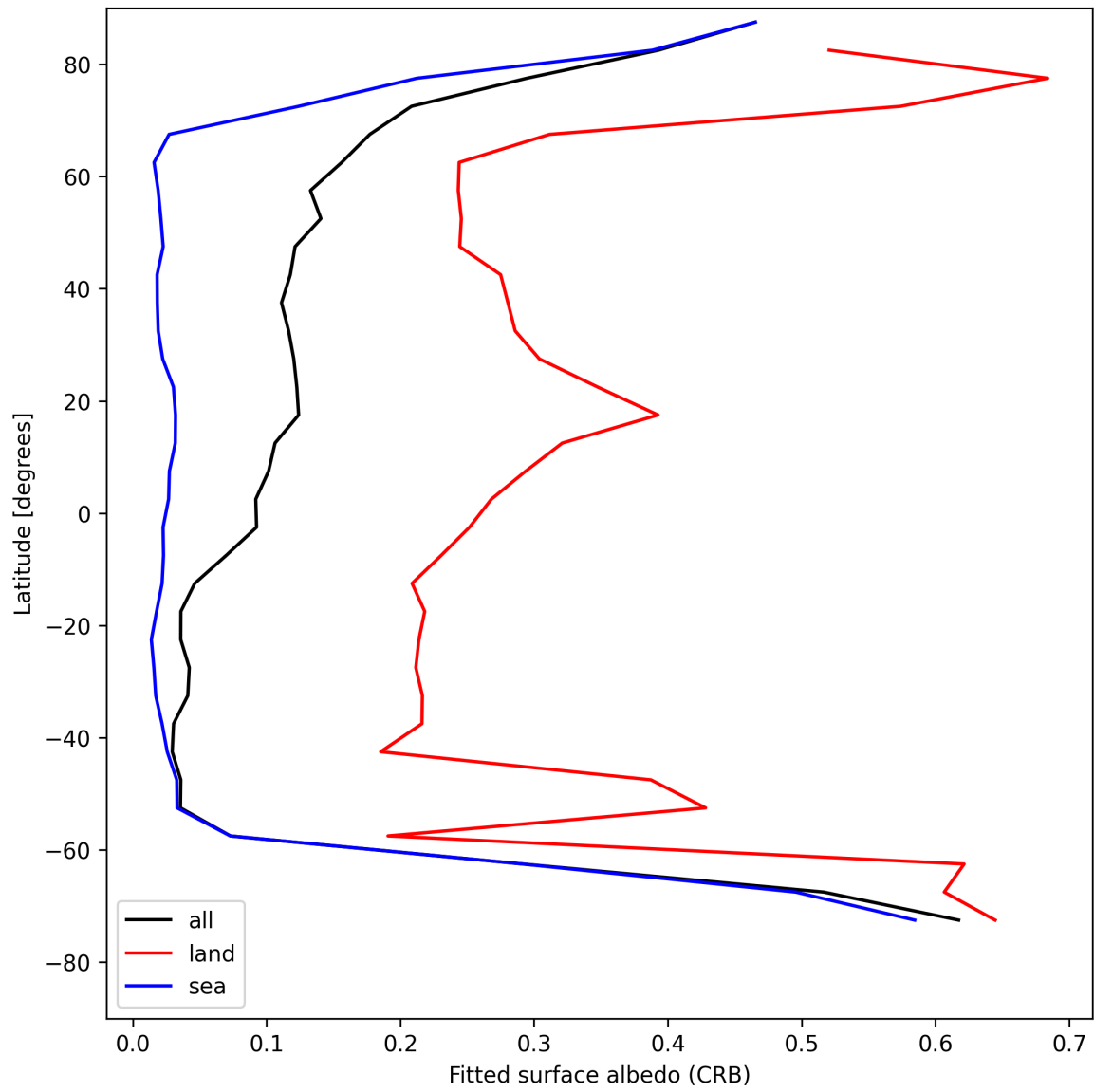
Figure 28: Zonal average of “Fitted surface albedo (CRB)” for 2025-08-14 to 2025-08-15.
