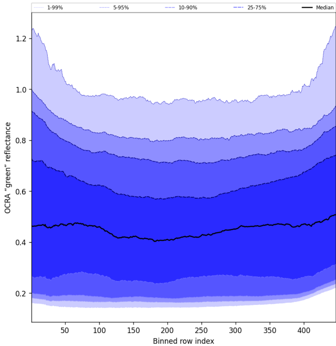
Figure 66: Along track statistics of “OCRA “green” reflectance” for 2025-08-14 to 2025-08-15
