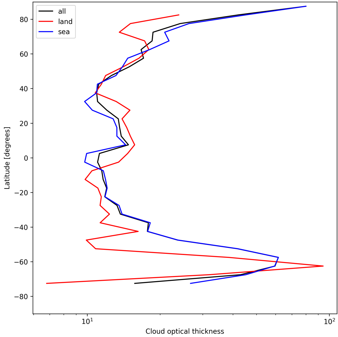
Figure 23: Zonal average of “Cloud optical thickness” for 2025-08-14 to 2025-08-15.
