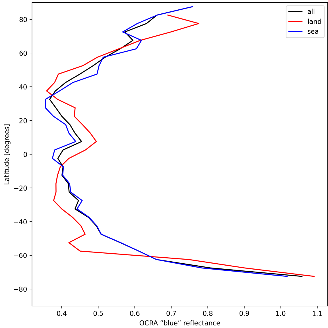
Figure 33: Zonal average of “OCRA “blue” reflectance” for 2025-08-14 to 2025-08-15.
