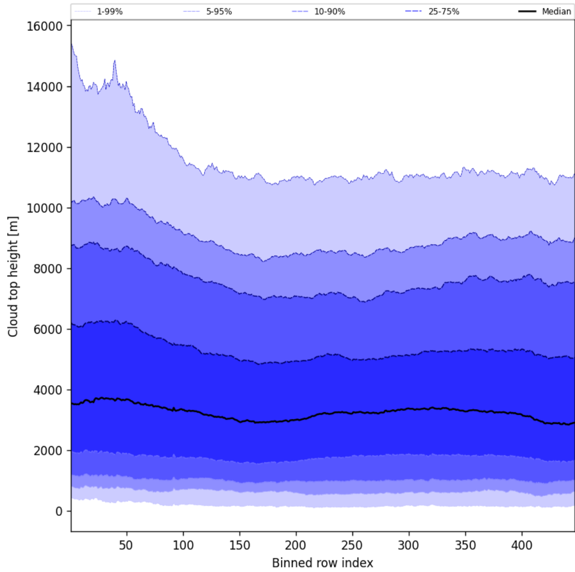
Figure 54: Along track statistics of “Cloud top height” for 2025-08-16 to 2025-08-17
