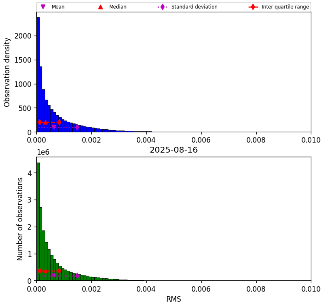
Figure 45: Histogram of “RMS” for 2025-08-16 to 2025-08-17
