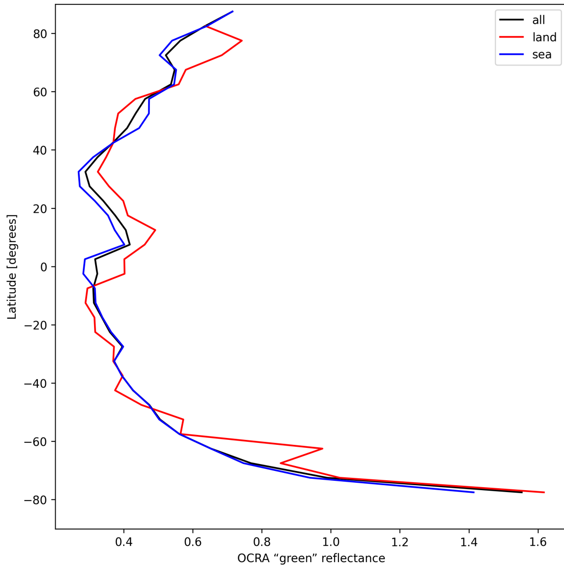
Figure 34: Zonal average of “OCRA “green” reflectance” for 2025-08-16 to 2025-08-17.
