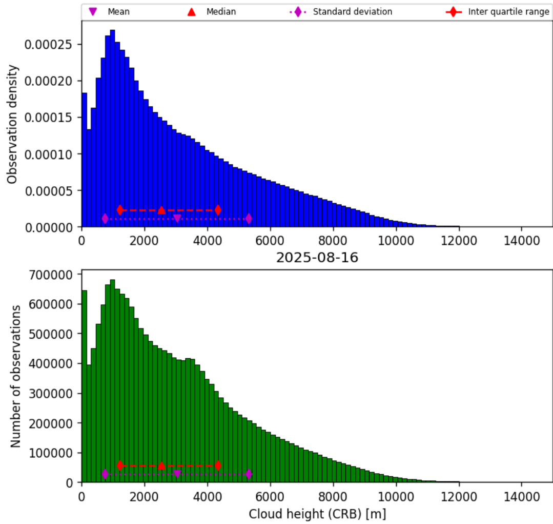
Figure 41: Histogram of “Cloud height (CRB)” for 2025-08-16 to 2025-08-17
