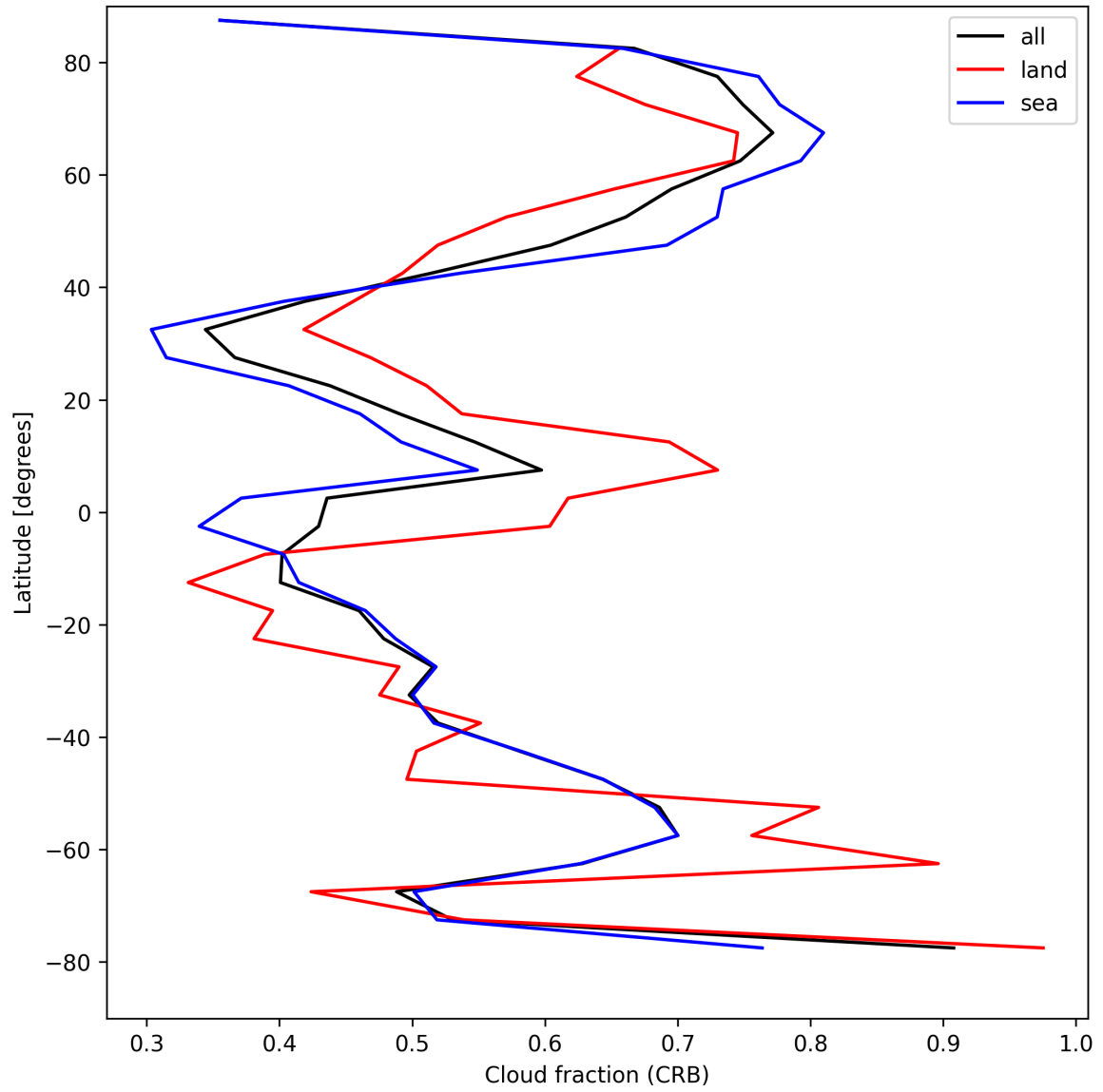
Figure 24: Zonal average of “Cloud fraction (CRB)” for 2025-08-16 to 2025-08-17.
