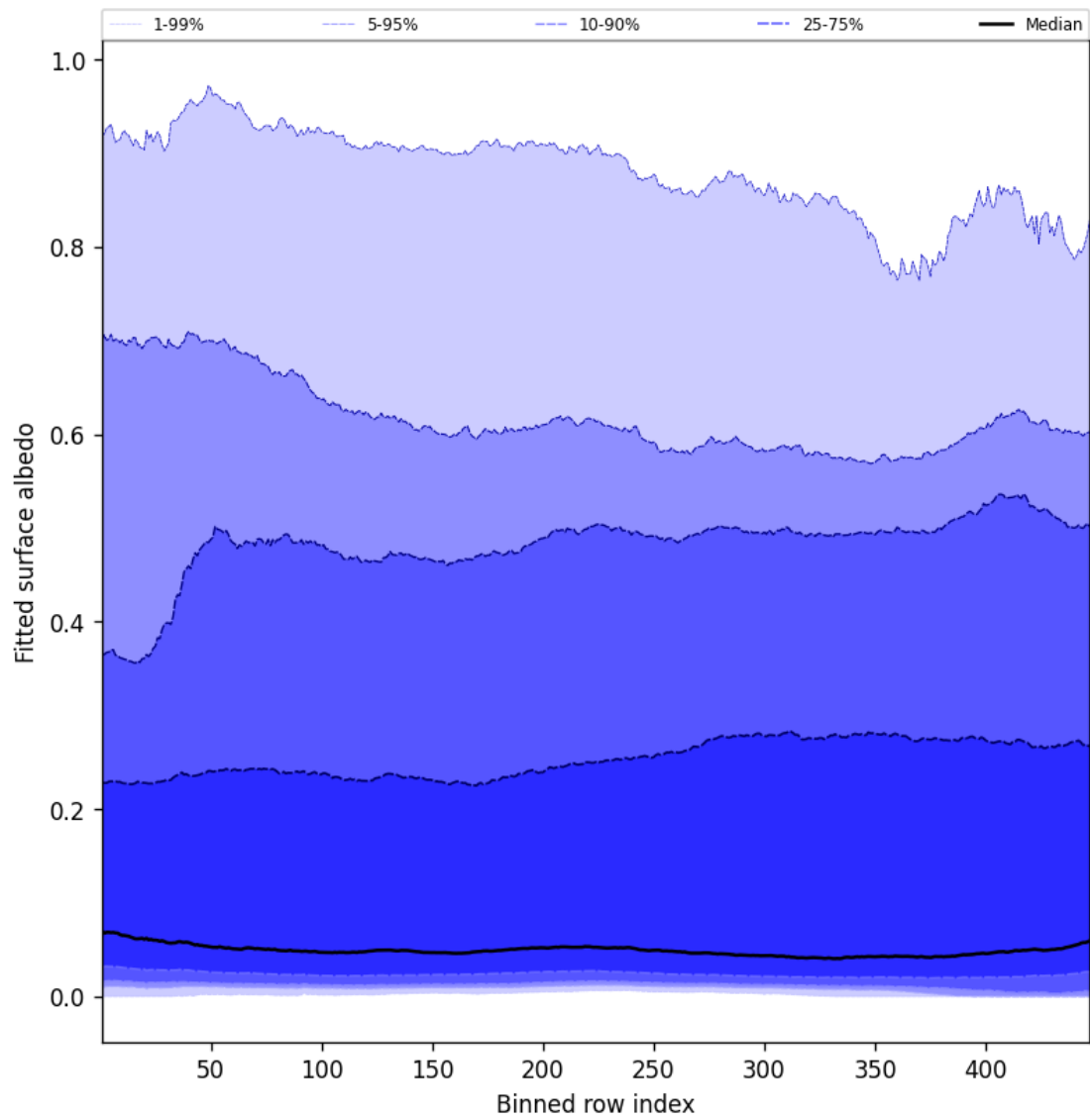
Figure 59: Along track statistics of “Fitted surface albedo” for 2025-08-16 to 2025-08-17
