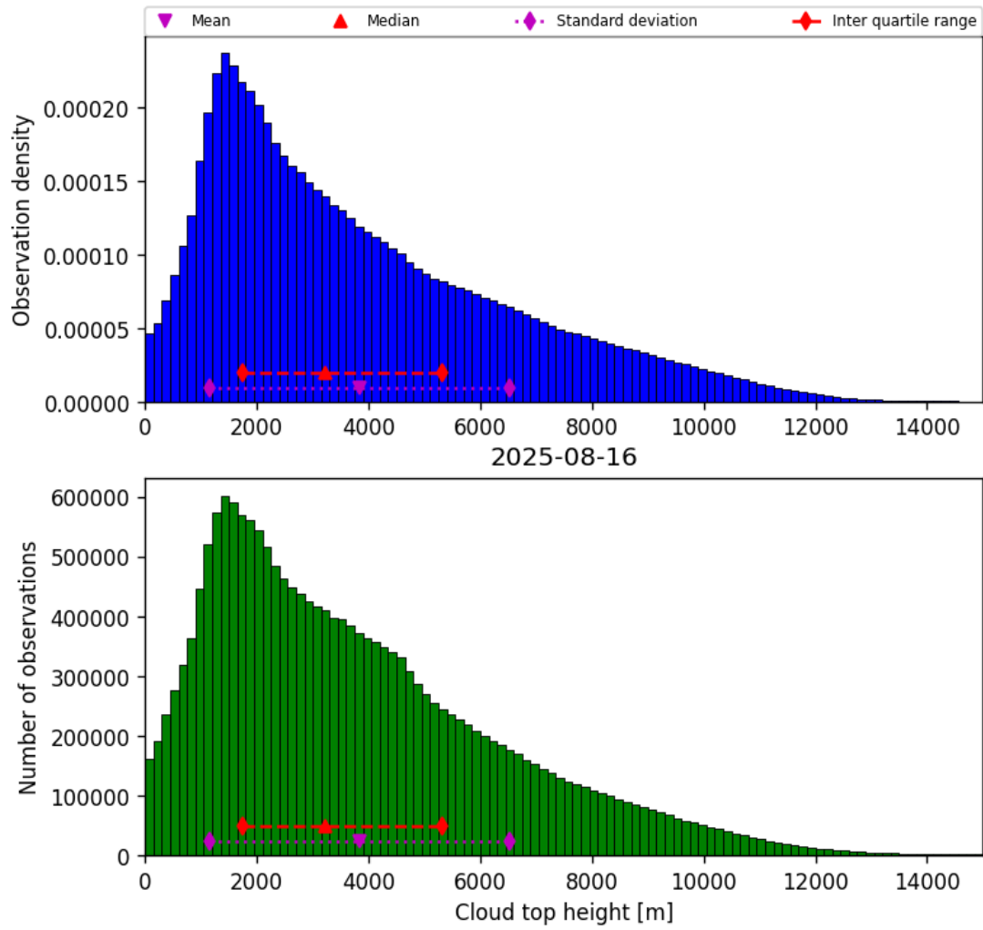
Figure 38: Histogram of “Cloud top height” for 2025-08-16 to 2025-08-17
