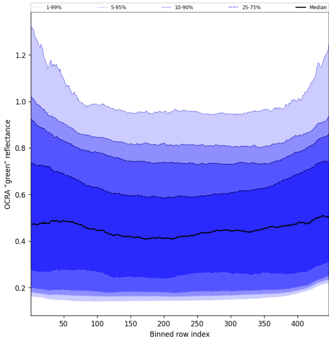
Figure 66: Along track statistics of “OCRA “green” reflectance” for 2025-08-16 to 2025-08-17
