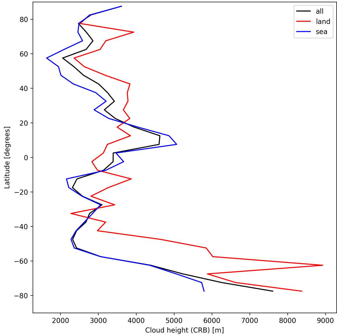
Figure 25: Zonal average of “Cloud height (CRB)” for 2025-08-16 to 2025-08-17.
