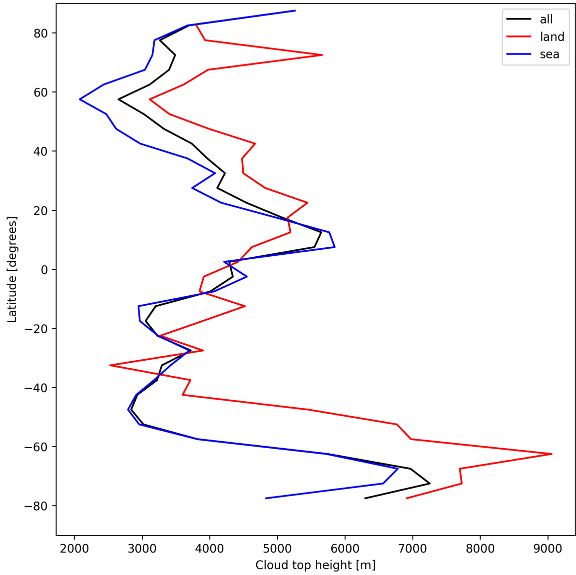
Figure 22: Zonal average of “Cloud top height” for 2025-08-16 to 2025-08-17.
