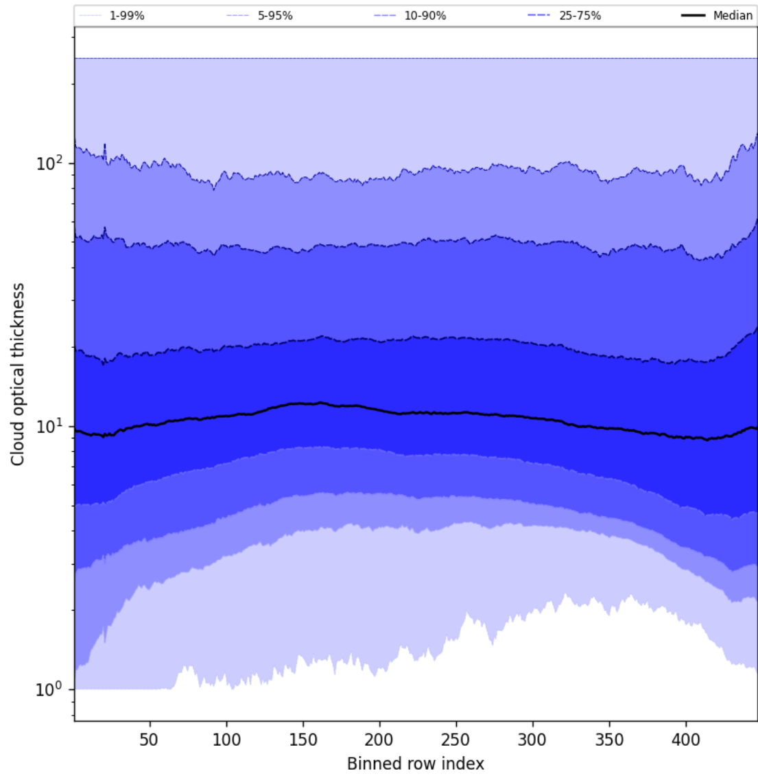
Figure 55: Along track statistics of “Cloud optical thickness” for 2025-08-16 to 2025-08-17
