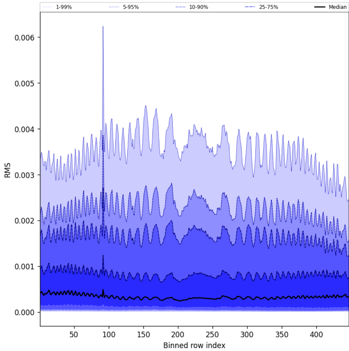
Figure 61: Along track statistics of “RMS” for 2025-08-16 to 2025-08-17
