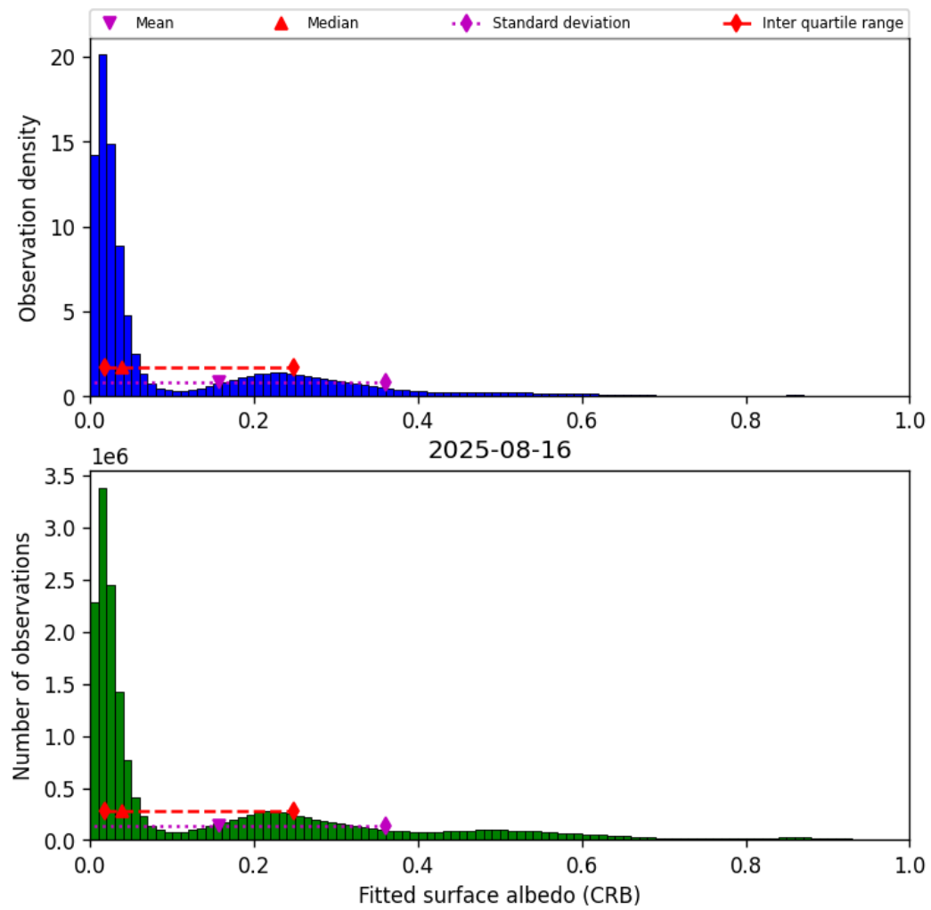
Figure 44: Histogram of “Fitted surface albedo (CRB)” for 2025-08-16 to 2025-08-17
