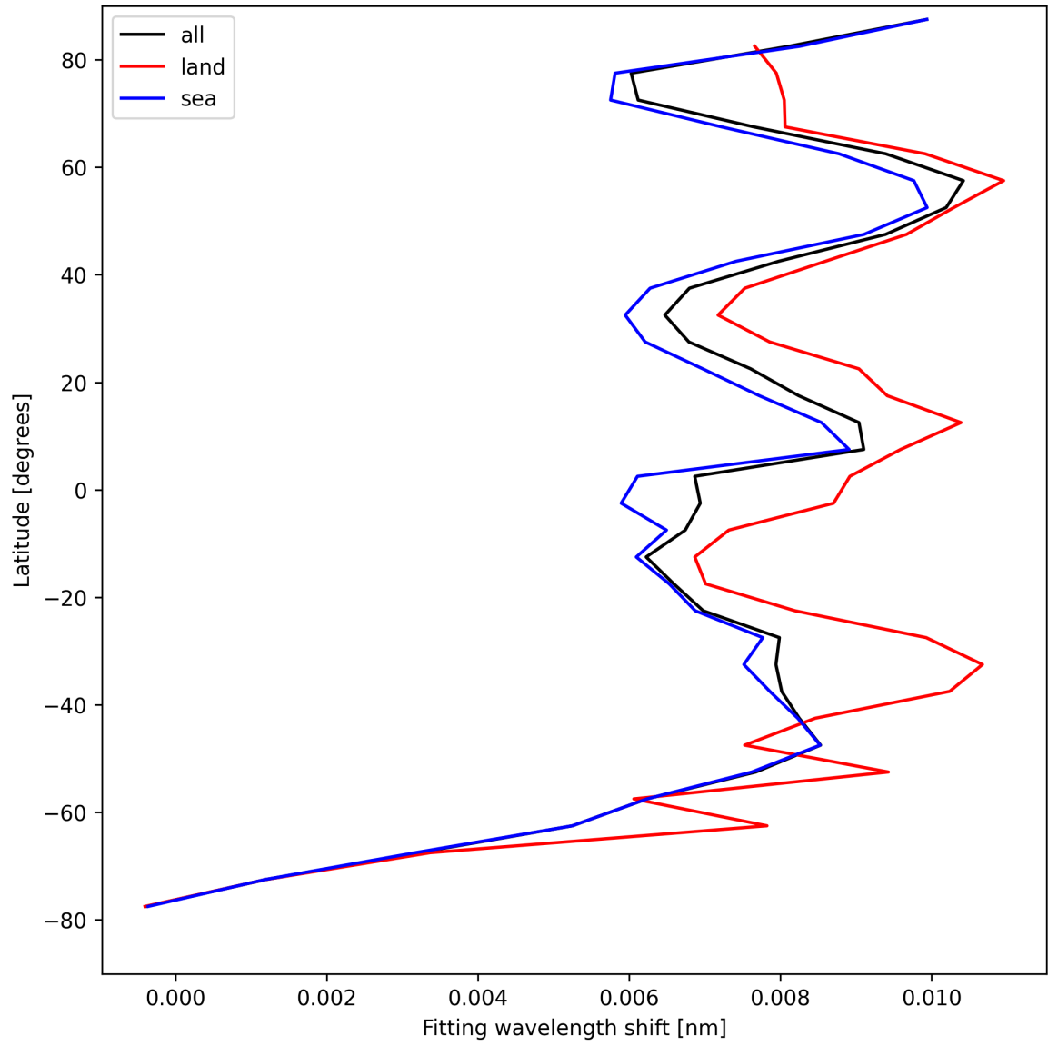
Figure 31: Zonal average of “Fitting wavelength shift” for 2025-08-16 to 2025-08-17.
