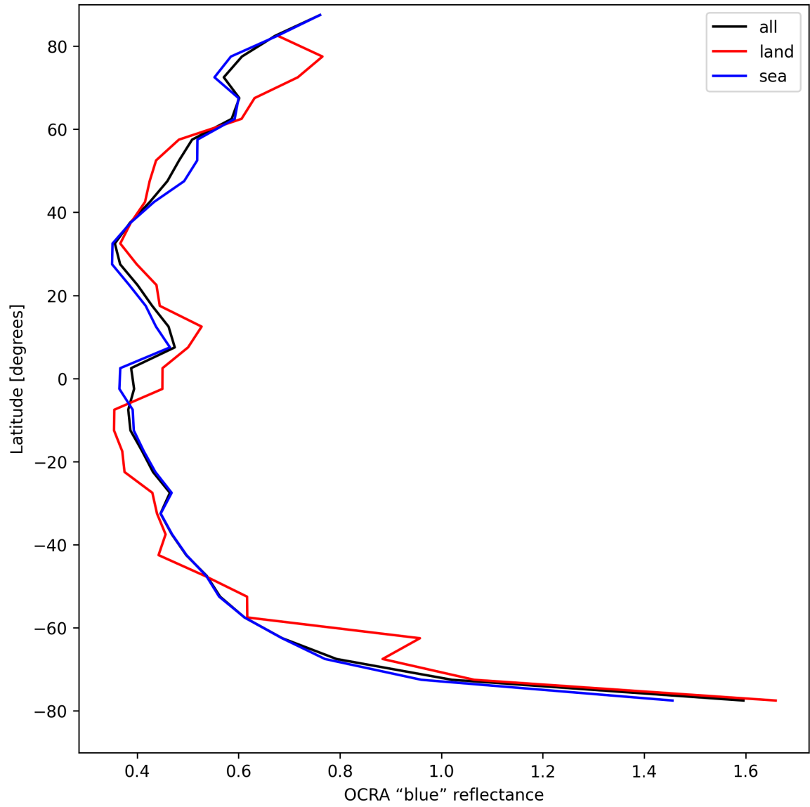
Figure 33: Zonal average of “OCRA “blue” reflectance” for 2025-08-16 to 2025-08-17.
