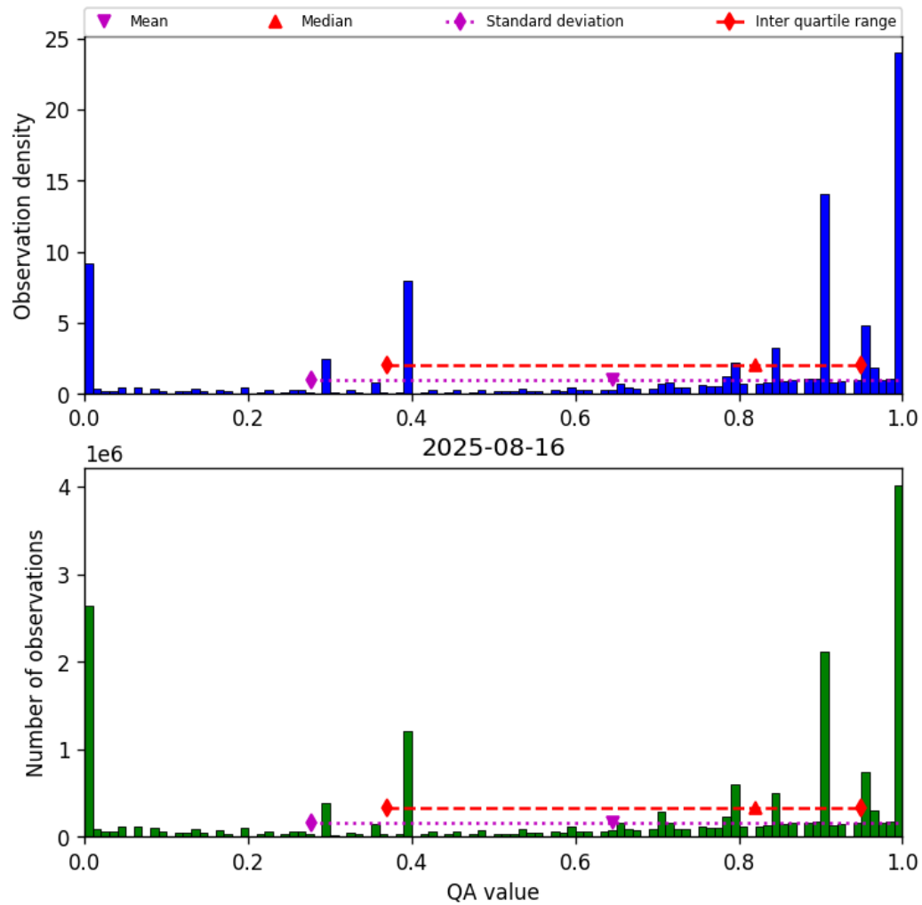
Figure 36: Histogram of “QA value” for 2025-08-16 to 2025-08-17
