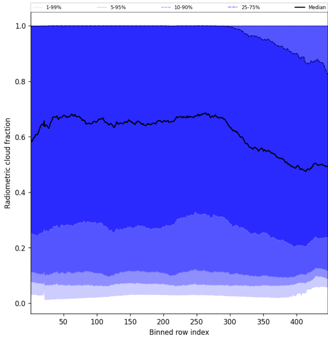
Figure 53: Along track statistics of “Radiometric cloud fraction” for 2025-08-16 to 2025-08-17
