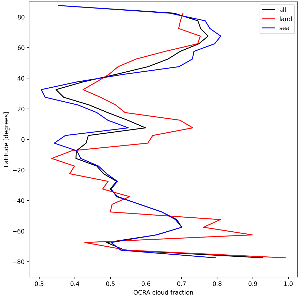
Figure 32: Zonal average of “OCRA cloud fraction” for 2025-08-16 to 2025-08-17.
