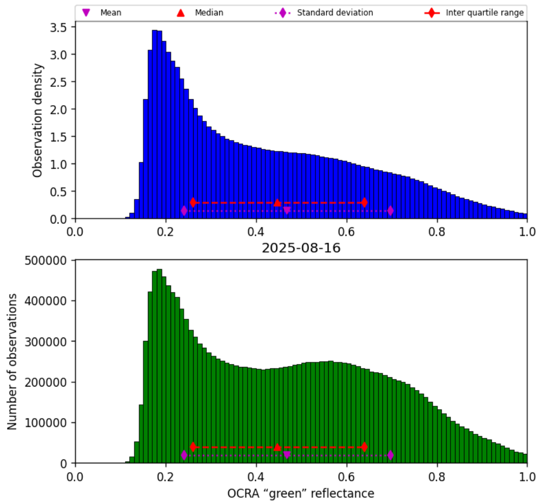
Figure 50: Histogram of “OCRA “green” reflectance” for 2025-08-16 to 2025-08-17
