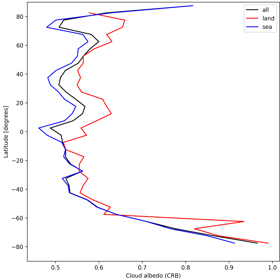
Figure 26: Zonal average of “Cloud albedo (CRB)” for 2025-08-16 to 2025-08-17.
