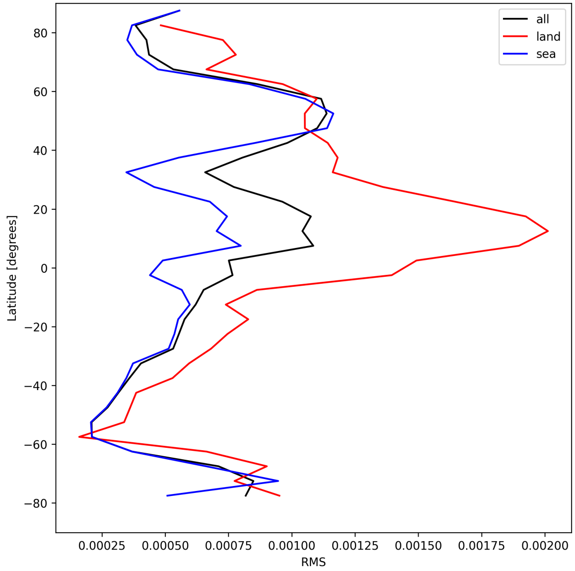
Figure 29: Zonal average of “RMS” for 2025-08-16 to 2025-08-17.
