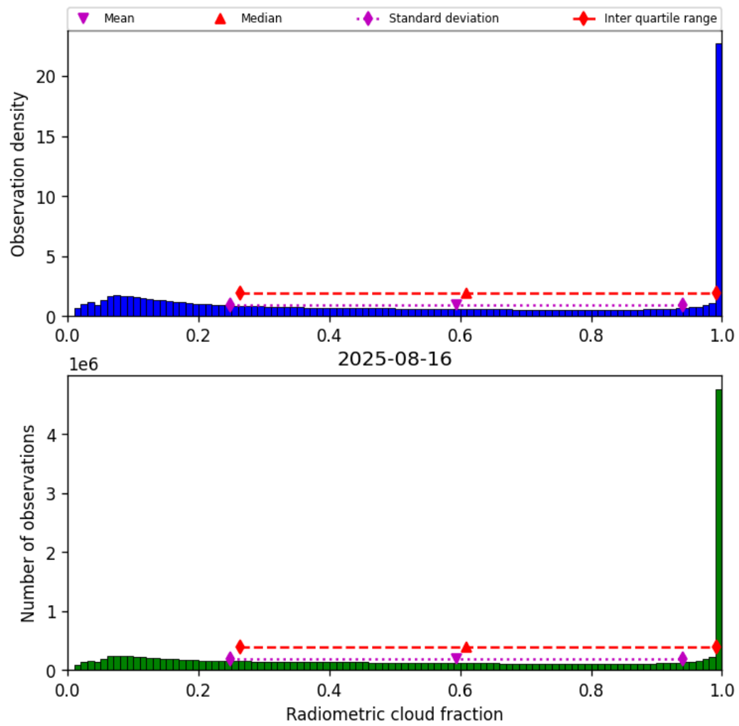
Figure 37: Histogram of “Radiometric cloud fraction” for 2025-08-16 to 2025-08-17
