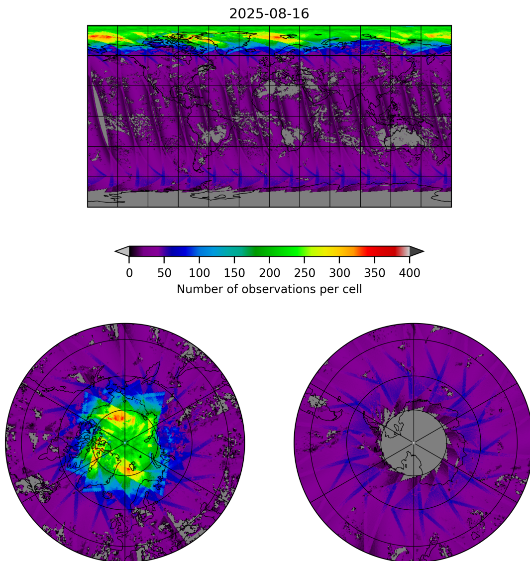
Figure 19: Map of the number of observations for 2025-08-16 to 2025-08-17
