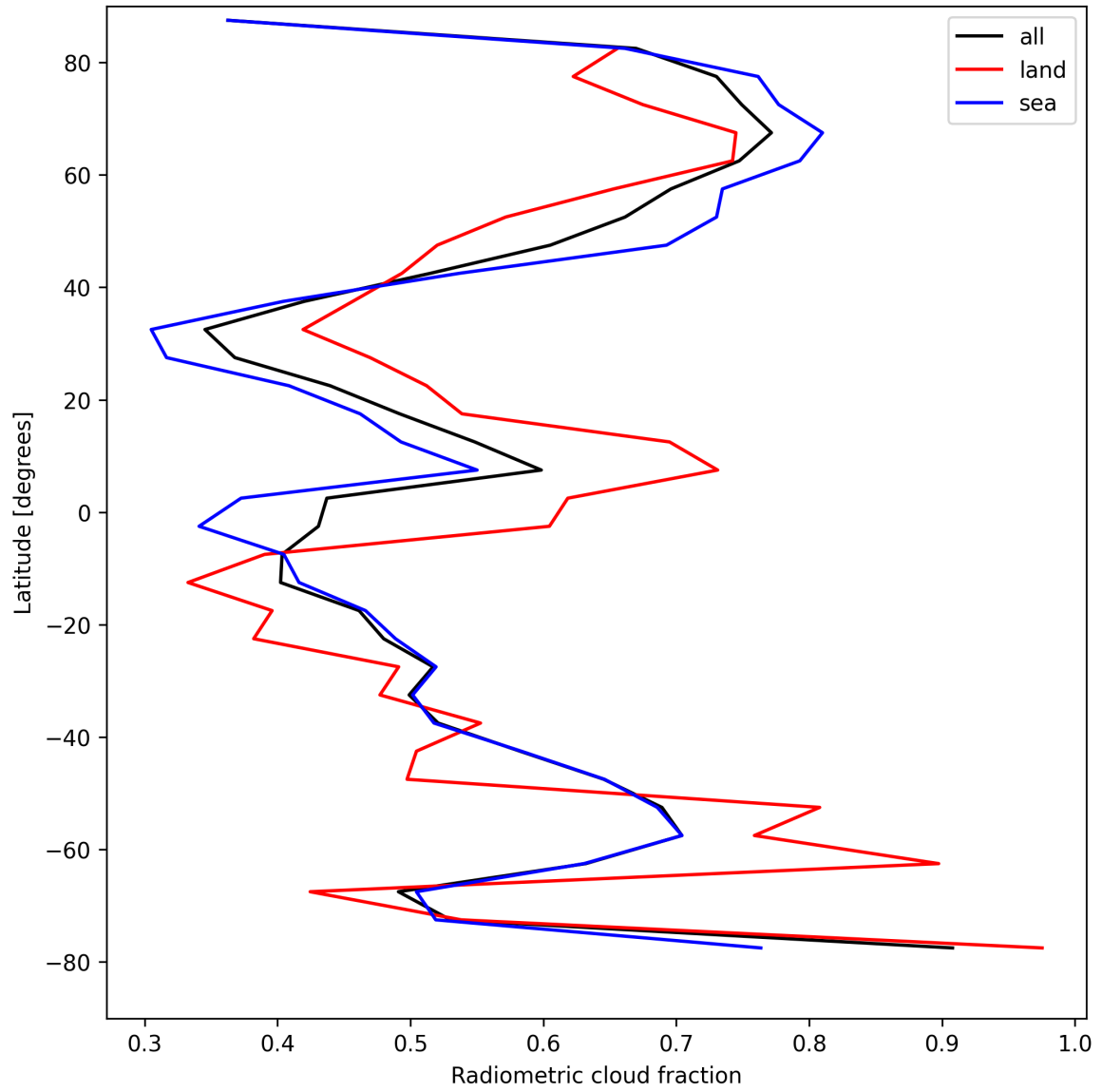
Figure 21: Zonal average of “Radiometric cloud fraction” for 2025-08-16 to 2025-08-17.
