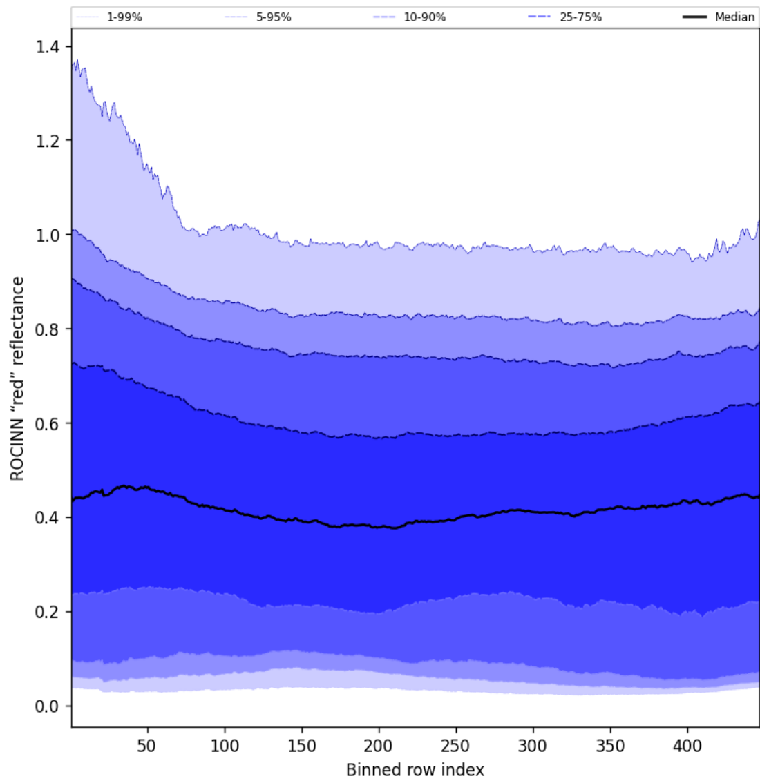
Figure 67: Along track statistics of “ROCINN “red” reflectance” for 2025-08-16 to 2025-08-17
