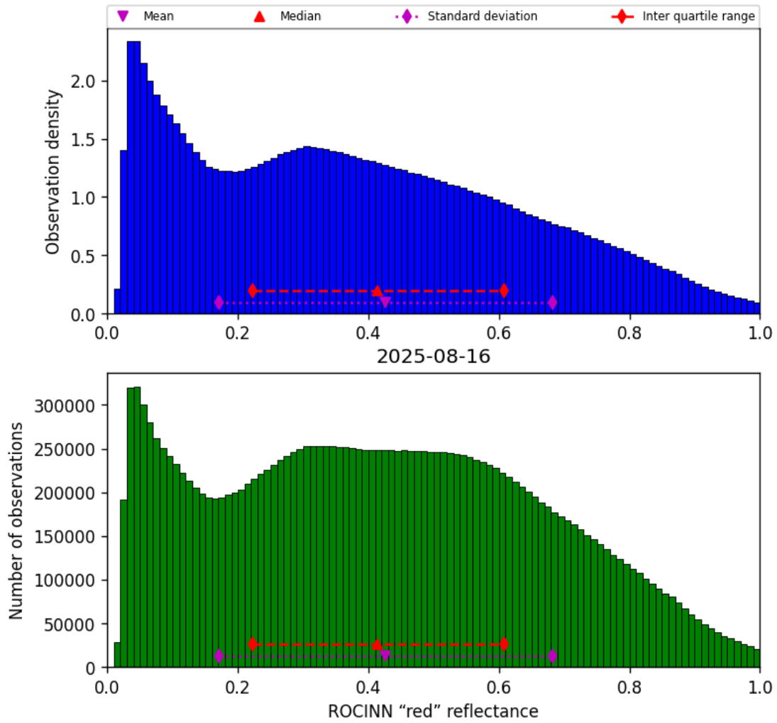
Figure 51: Histogram of “ROCINN “red” reflectance” for 2025-08-16 to 2025-08-17
