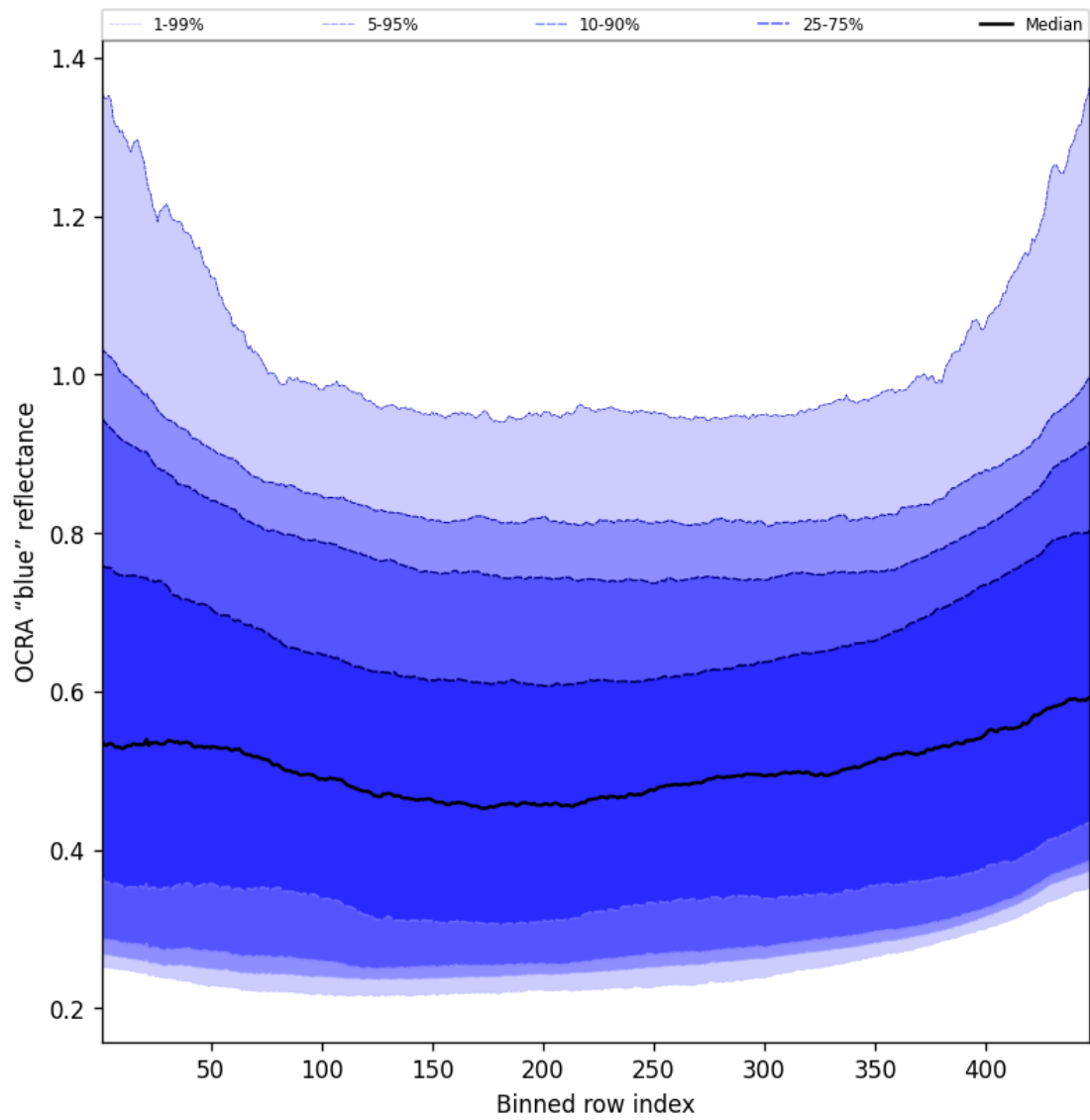
Figure 65: Along track statistics of “OCRA “blue” reflectance” for 2025-08-16 to 2025-08-17
