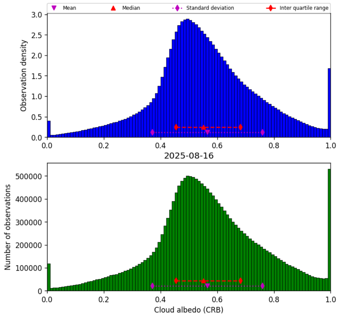
Figure 42: Histogram of “Cloud albedo (CRB)” for 2025-08-16 to 2025-08-17
