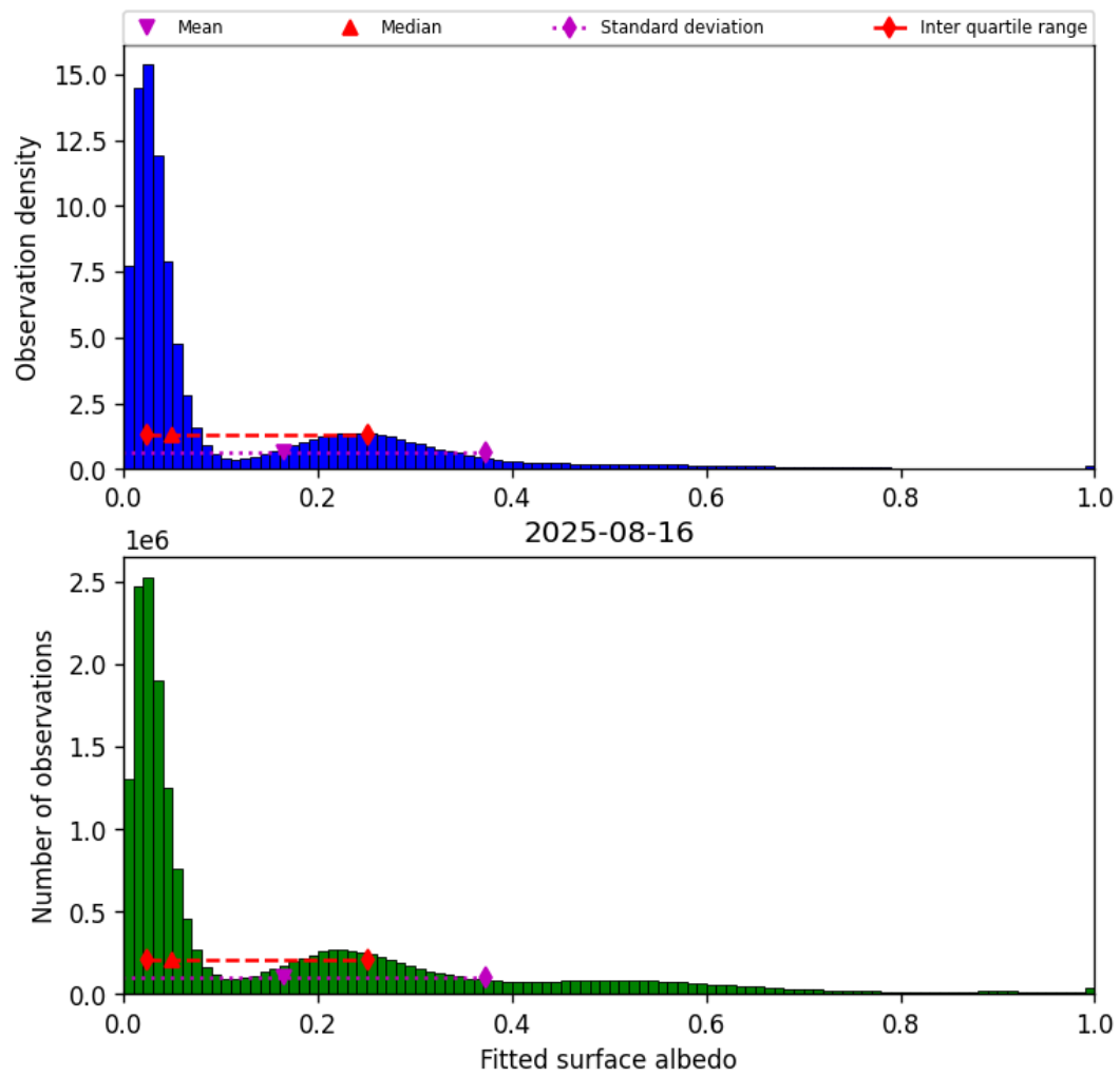
Figure 43: Histogram of “Fitted surface albedo” for 2025-08-16 to 2025-08-17
