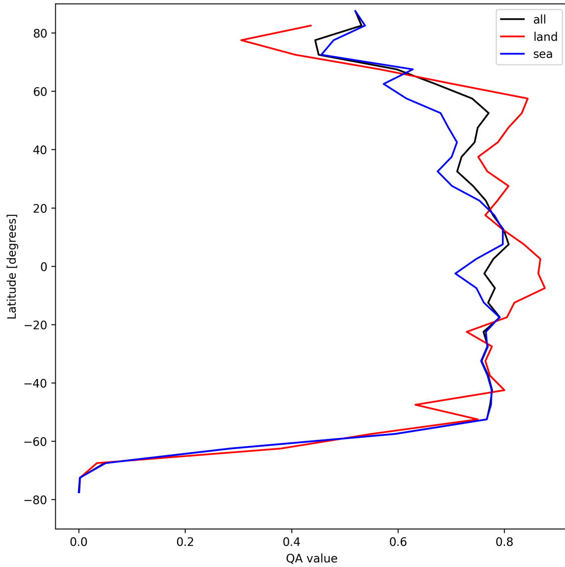
Figure 20: Zonal average of “QA value” for 2025-08-16 to 2025-08-17.
