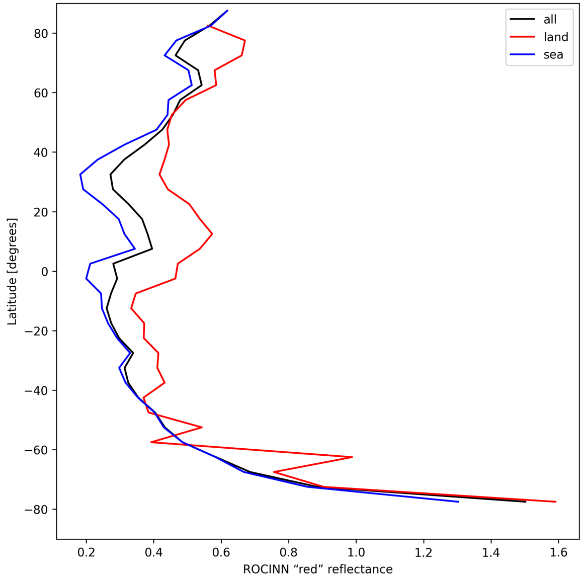
Figure 35: Zonal average of “ROCINN “red” reflectance” for 2025-08-16 to 2025-08-17.
