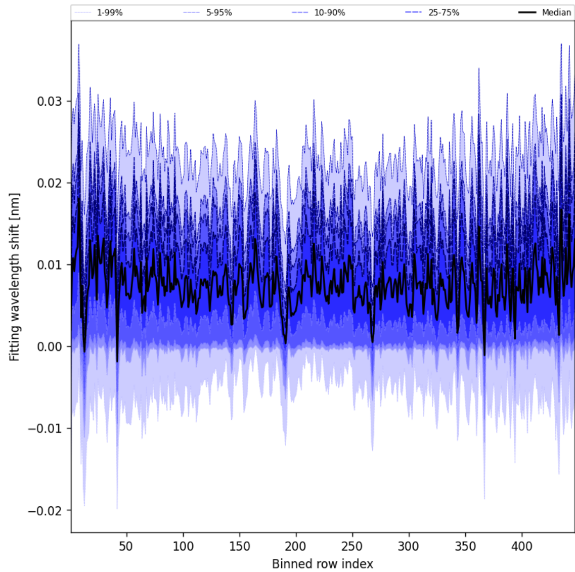
Figure 63: Along track statistics of “Fitting wavelength shift” for 2025-08-16 to 2025-08-17
