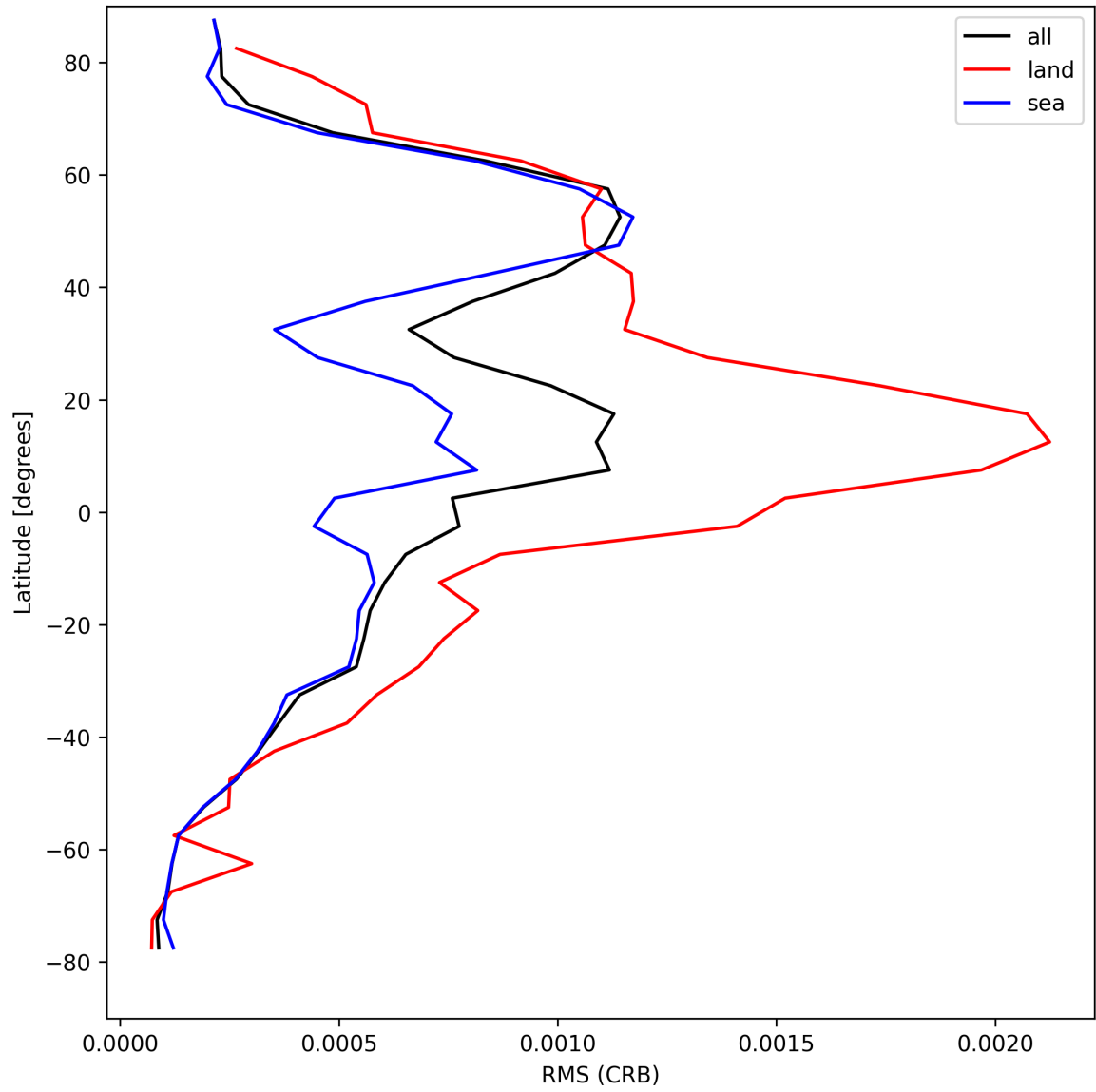
Figure 30: Zonal average of “RMS (CRB)” for 2025-08-16 to 2025-08-17.
