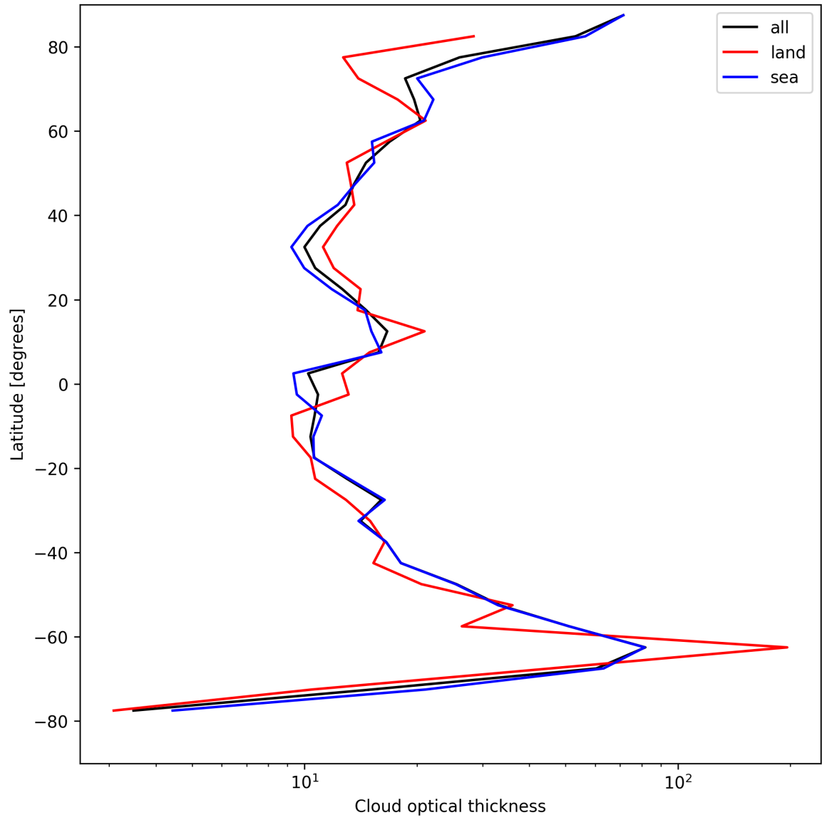
Figure 23: Zonal average of “Cloud optical thickness” for 2025-08-16 to 2025-08-17.
