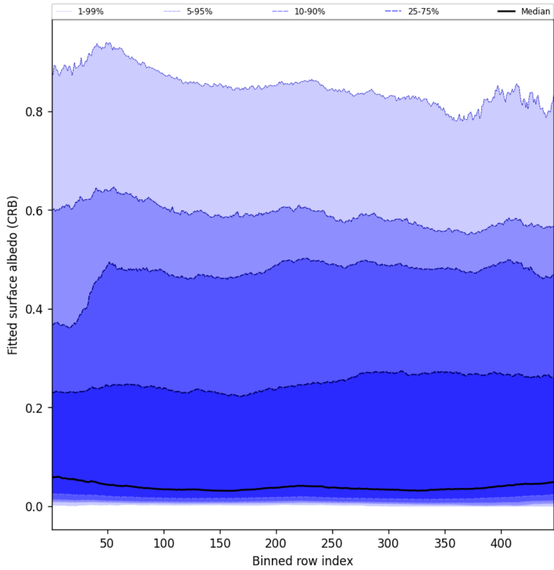
Figure 60: Along track statistics of “Fitted surface albedo (CRB)” for 2025-08-16 to 2025-08-17
