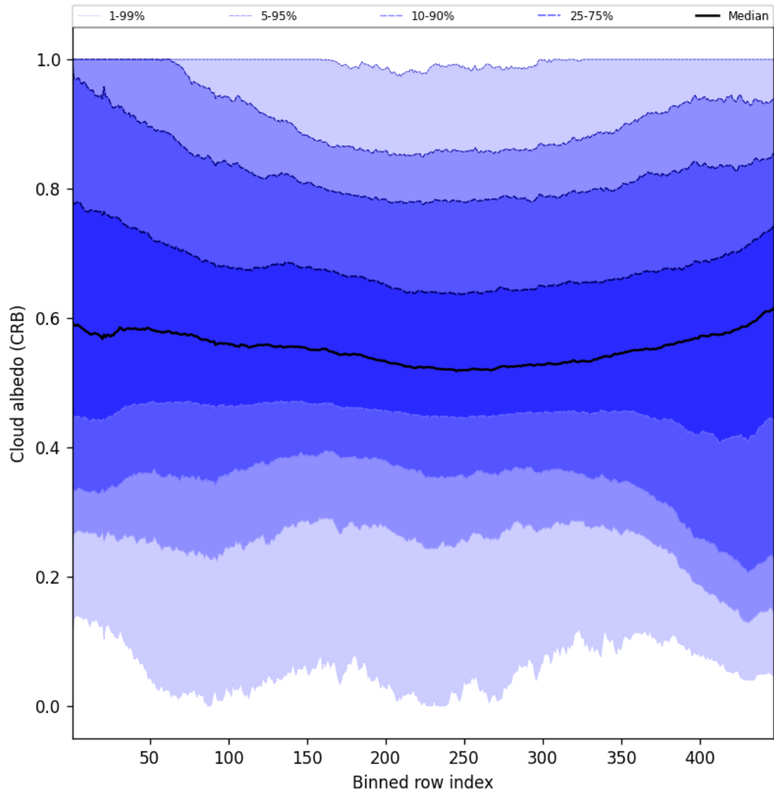
Figure 58: Along track statistics of “Cloud albedo (CRB)” for 2025-08-16 to 2025-08-17
