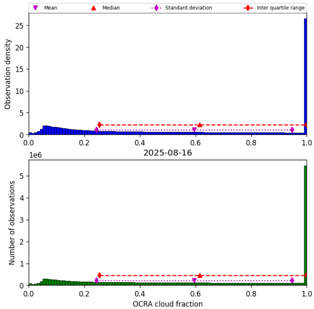
Figure 48: Histogram of “OCRA cloud fraction” for 2025-08-16 to 2025-08-17
