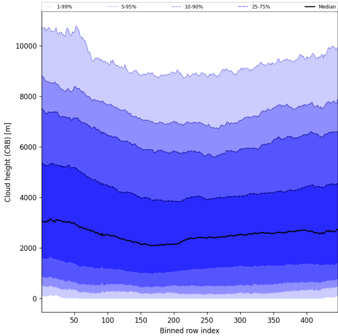
Figure 57: Along track statistics of “Cloud height (CRB)” for 2025-08-16 to 2025-08-17
