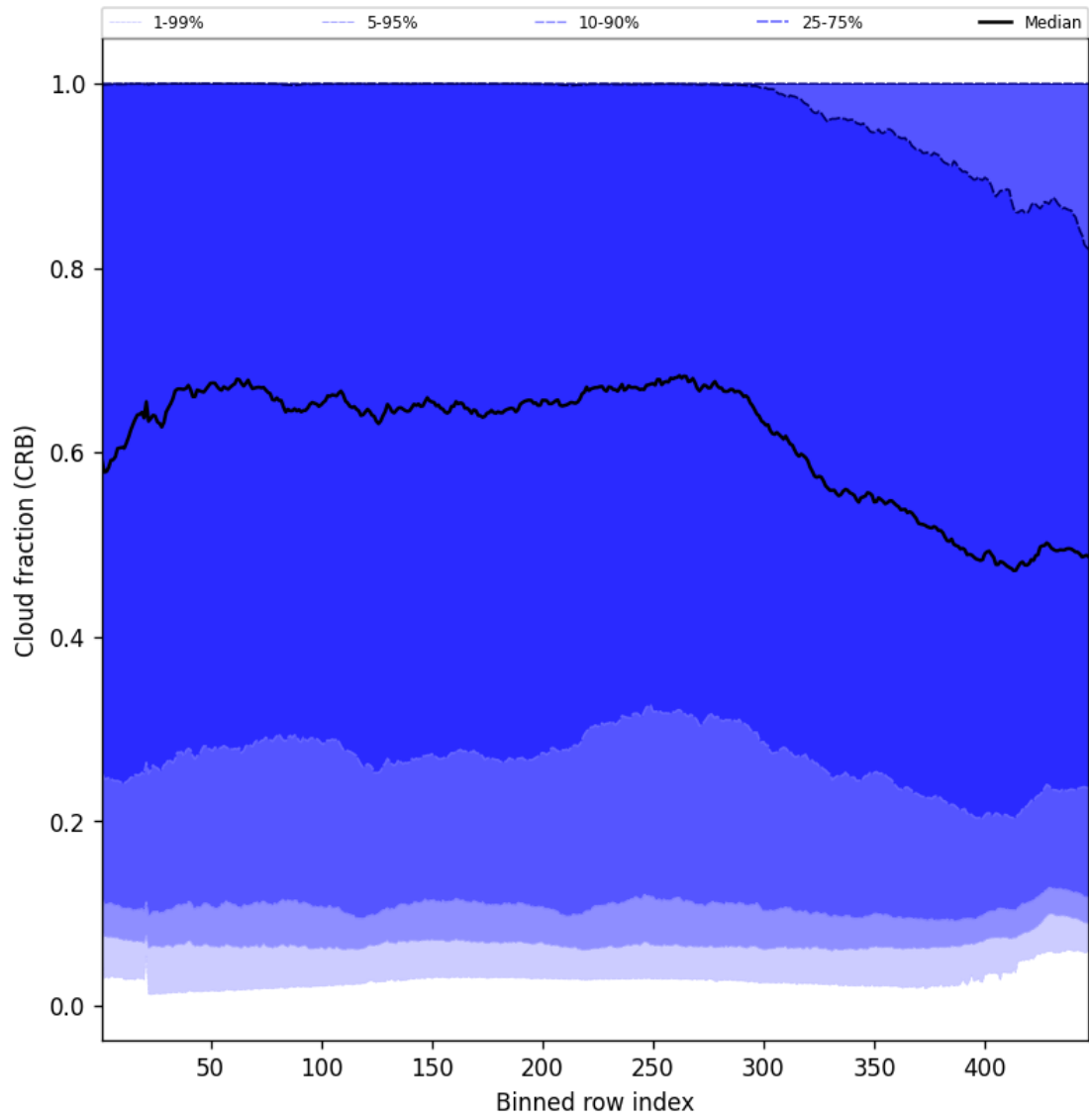
Figure 56: Along track statistics of “Cloud fraction (CRB)” for 2025-08-16 to 2025-08-17
