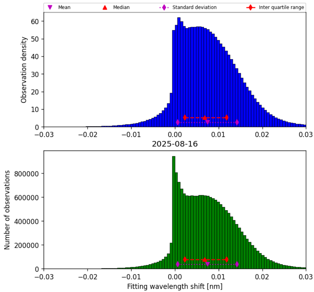
Figure 47: Histogram of “Fitting wavelength shift” for 2025-08-16 to 2025-08-17
