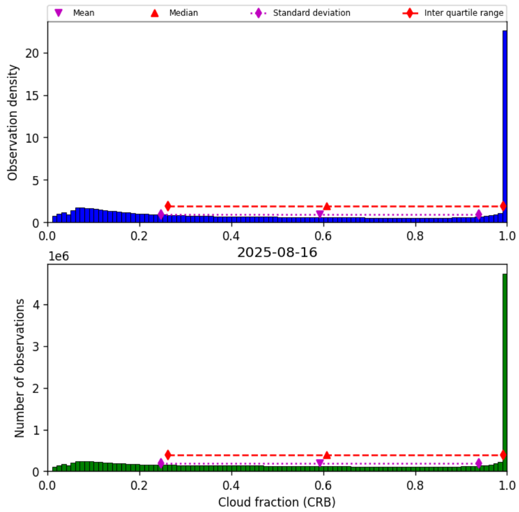
Figure 40: Histogram of “Cloud fraction (CRB)” for 2025-08-16 to 2025-08-17
