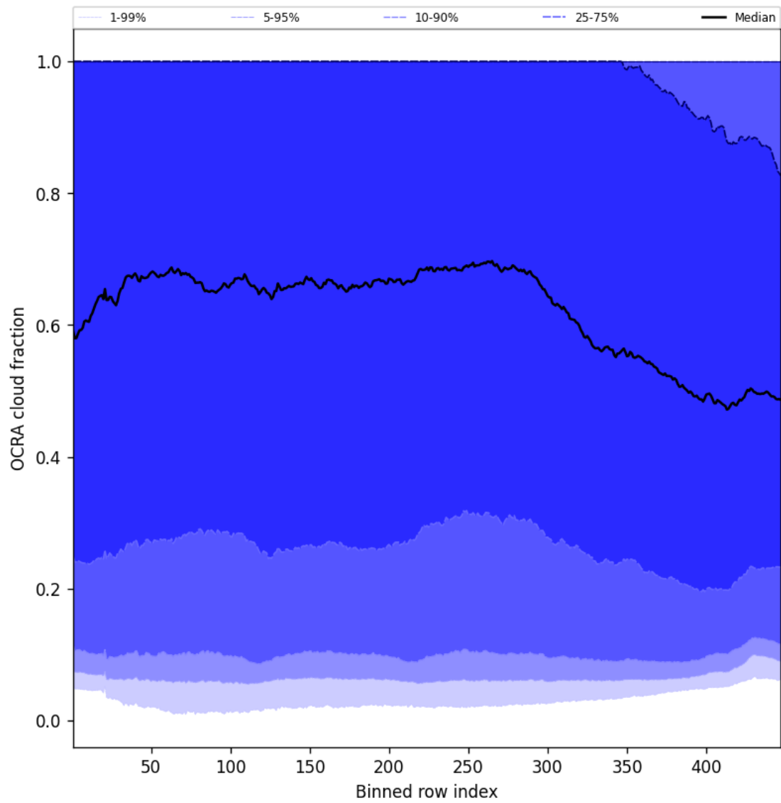
Figure 64: Along track statistics of “OCRA cloud fraction” for 2025-08-16 to 2025-08-17
