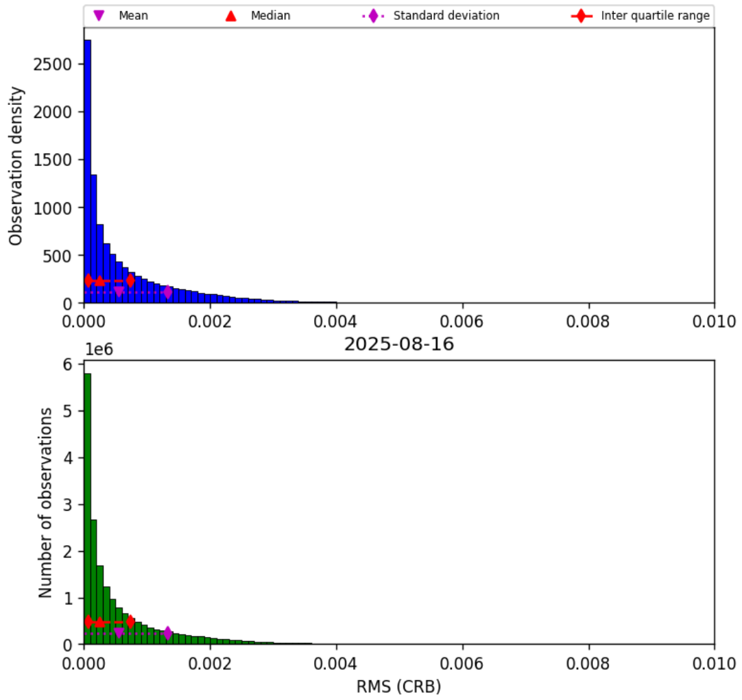
Figure 46: Histogram of “RMS (CRB)” for 2025-08-16 to 2025-08-17
