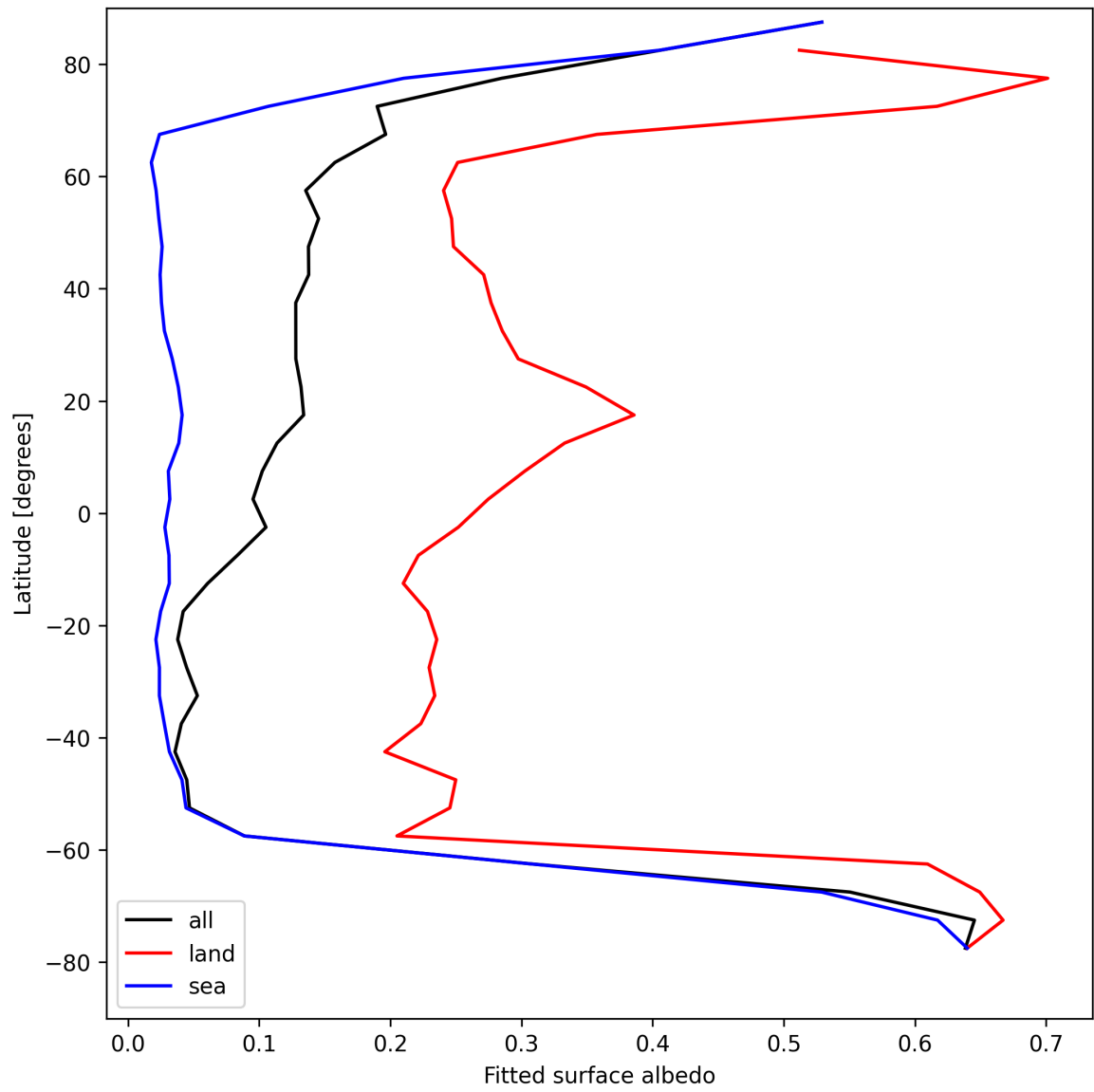
Figure 27: Zonal average of “Fitted surface albedo” for 2025-08-16 to 2025-08-17.
