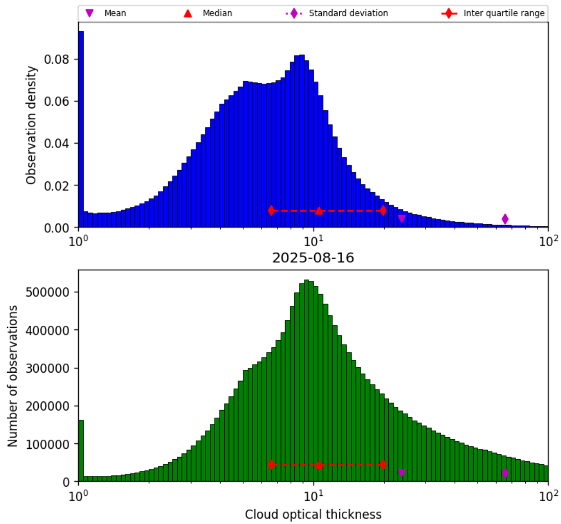
Figure 39: Histogram of “Cloud optical thickness” for 2025-08-16 to 2025-08-17
