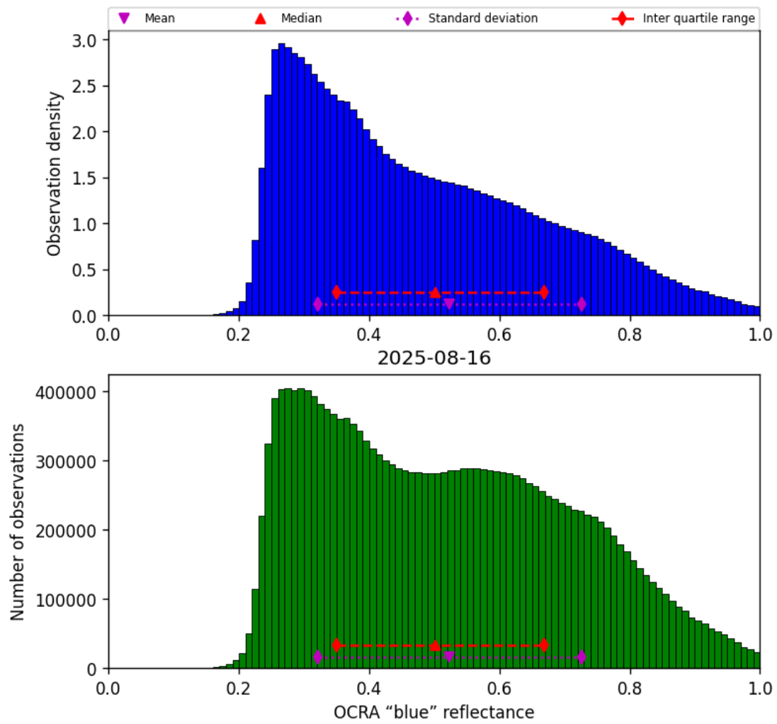
Figure 49: Histogram of “OCRA “blue” reflectance” for 2025-08-16 to 2025-08-17
