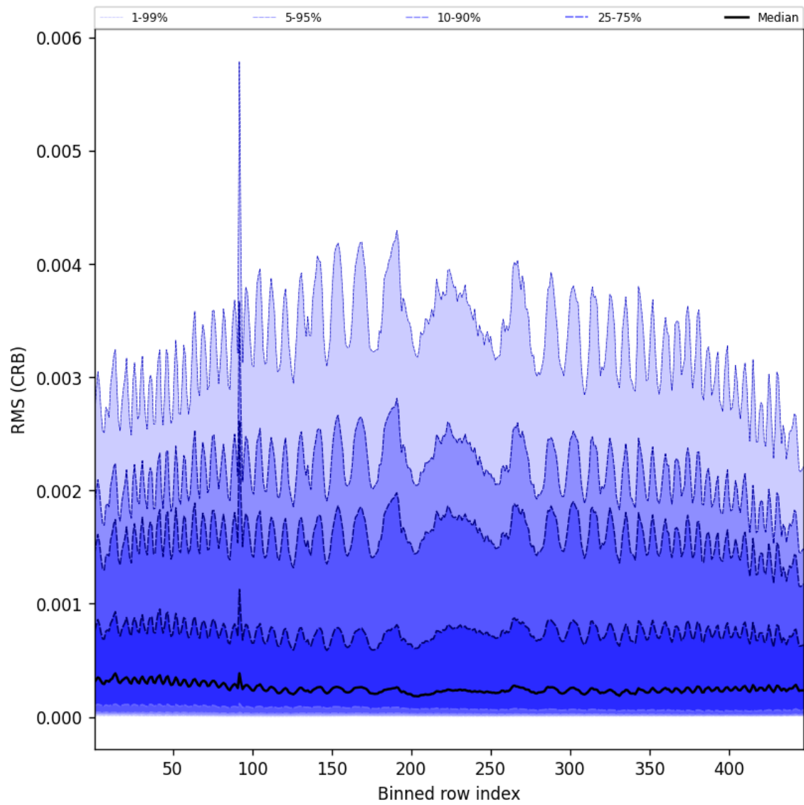
Figure 62: Along track statistics of “RMS (CRB)” for 2025-08-16 to 2025-08-17
