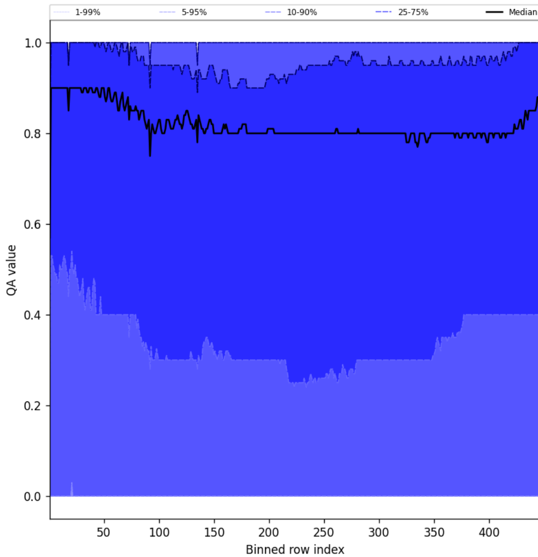
Figure 52: Along track statistics of “QA value” for 2025-08-16 to 2025-08-17
