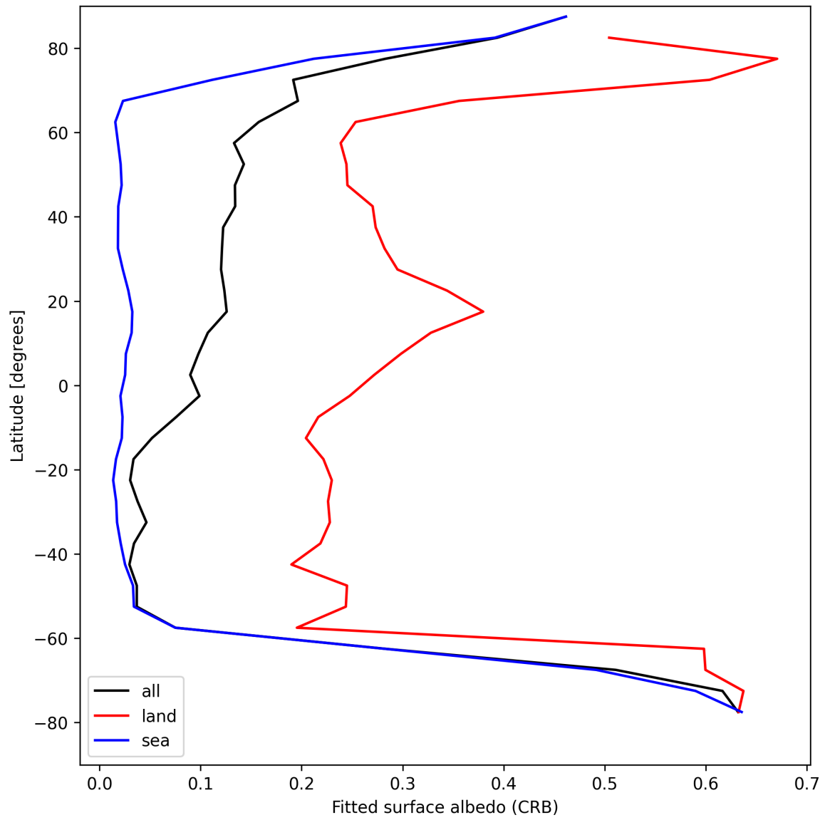
Figure 28: Zonal average of “Fitted surface albedo (CRB)” for 2025-08-16 to 2025-08-17.
