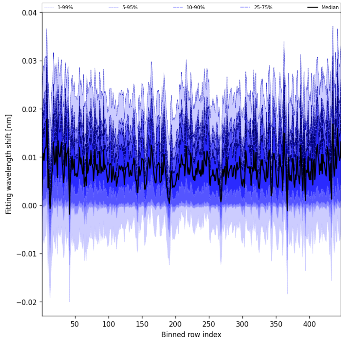
Figure 63: Along track statistics of “Fitting wavelength shift” for 2025-08-17 to 2025-08-17
