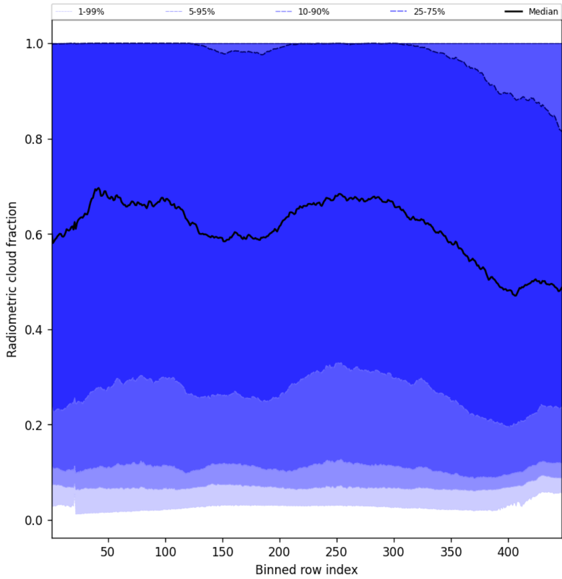
Figure 53: Along track statistics of “Radiometric cloud fraction” for 2025-08-17 to 2025-08-17
