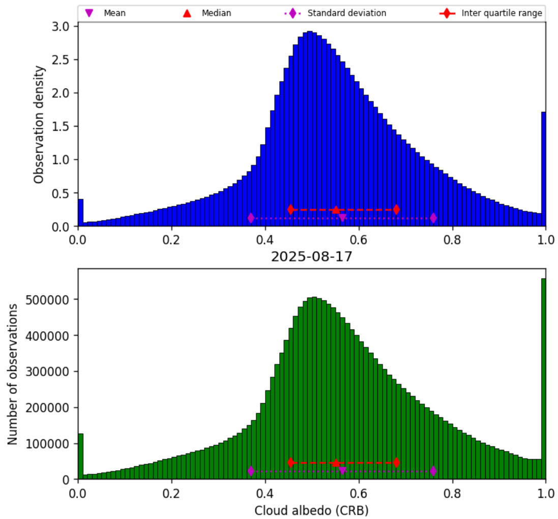
Figure 42: Histogram of “Cloud albedo (CRB)” for 2025-08-17 to 2025-08-17
