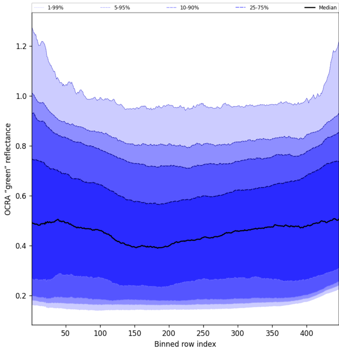
Figure 66: Along track statistics of “OCRA “green” reflectance” for 2025-08-17 to 2025-08-17
