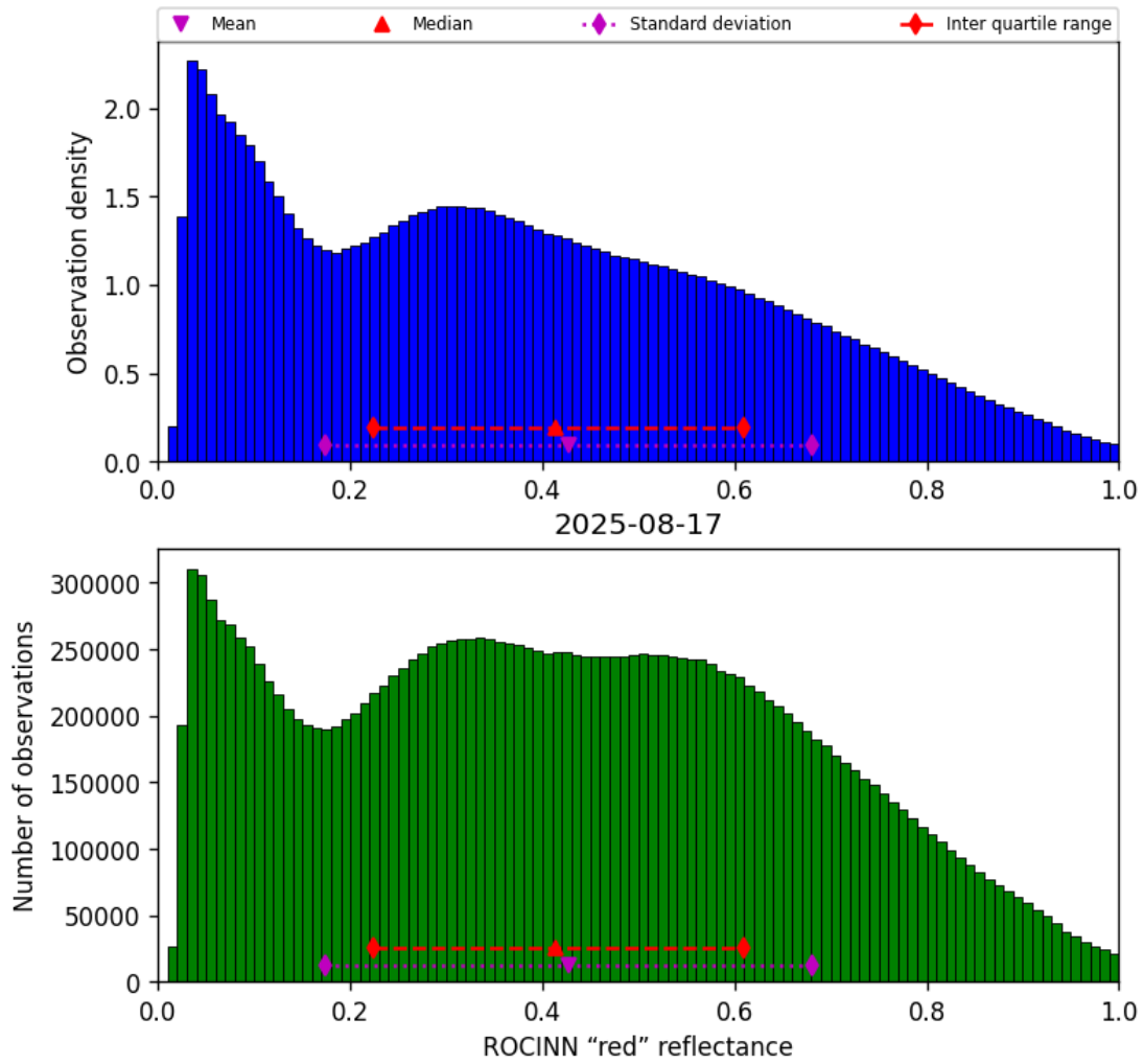
Figure 51: Histogram of “ROCINN “red” reflectance” for 2025-08-17 to 2025-08-17
