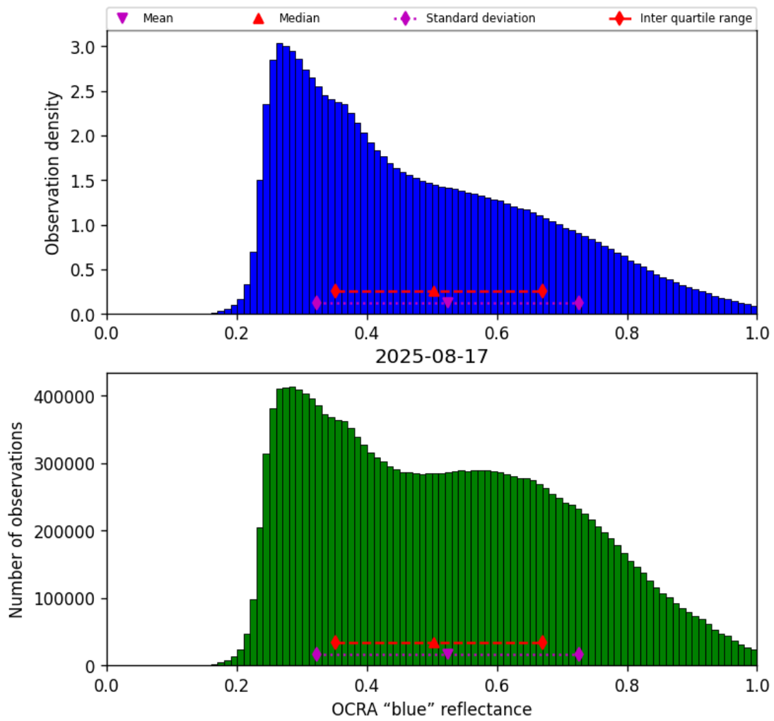
Figure 49: Histogram of “OCRA “blue” reflectance” for 2025-08-17 to 2025-08-17
