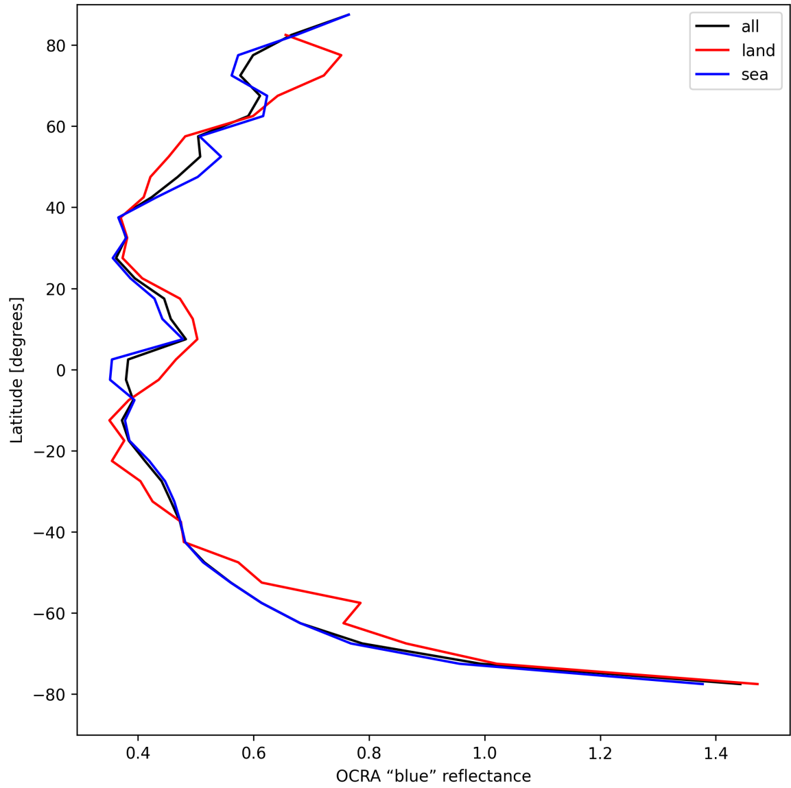
Figure 33: Zonal average of “OCRA “blue” reflectance” for 2025-08-17 to 2025-08-17.
