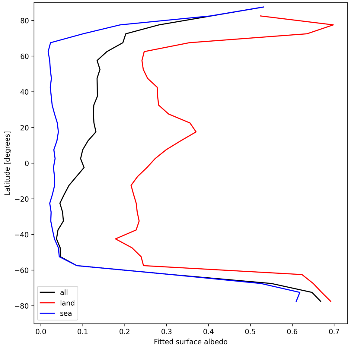
Figure 27: Zonal average of “Fitted surface albedo” for 2025-08-17 to 2025-08-17.
