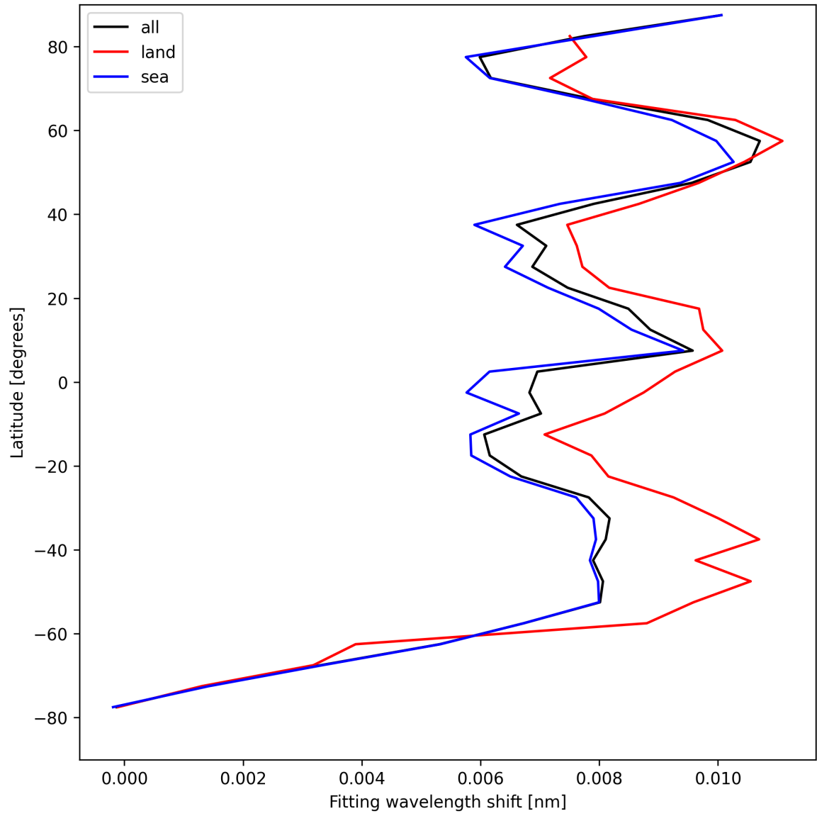
Figure 31: Zonal average of “Fitting wavelength shift” for 2025-08-17 to 2025-08-17.
