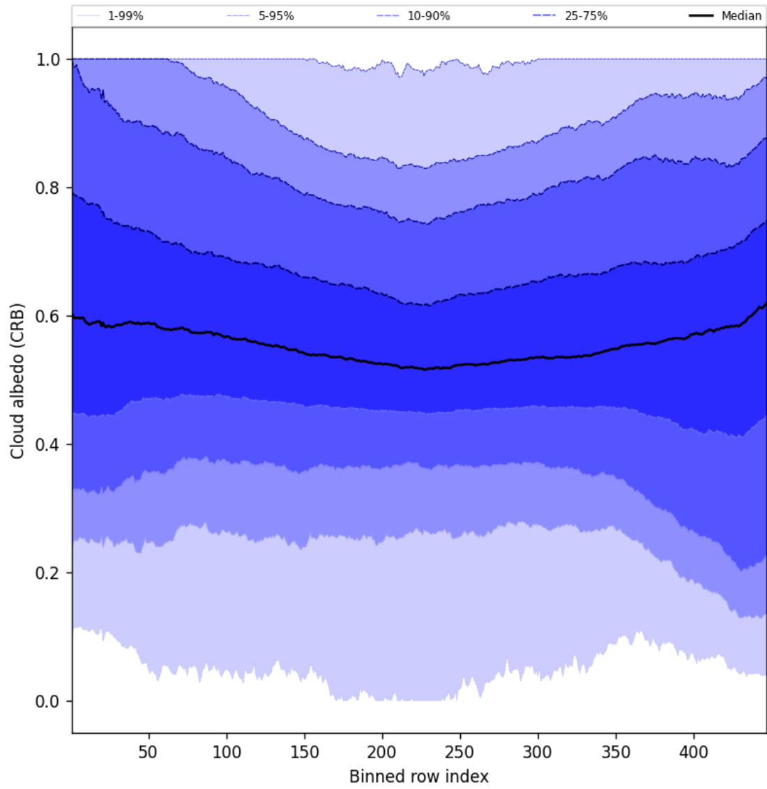
Figure 58: Along track statistics of “Cloud albedo (CRB)” for 2025-08-17 to 2025-08-17
