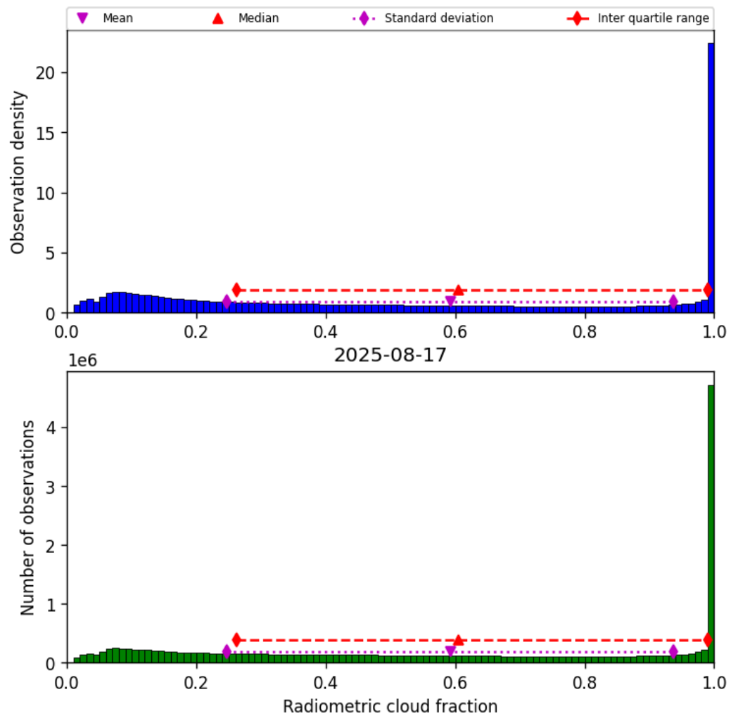
Figure 37: Histogram of “Radiometric cloud fraction” for 2025-08-17 to 2025-08-17
