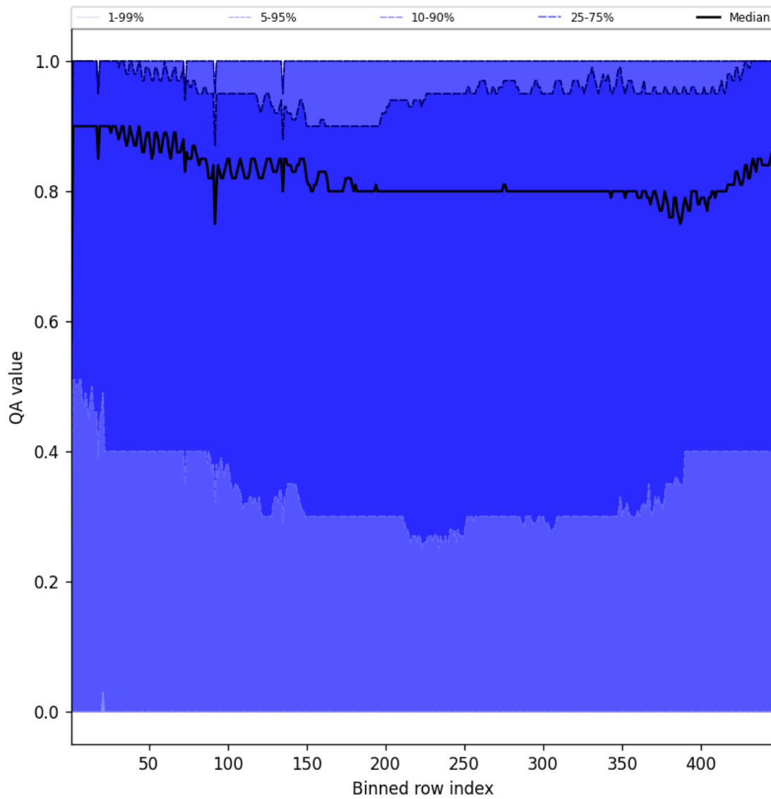
Figure 52: Along track statistics of “QA value” for 2025-08-17 to 2025-08-17
