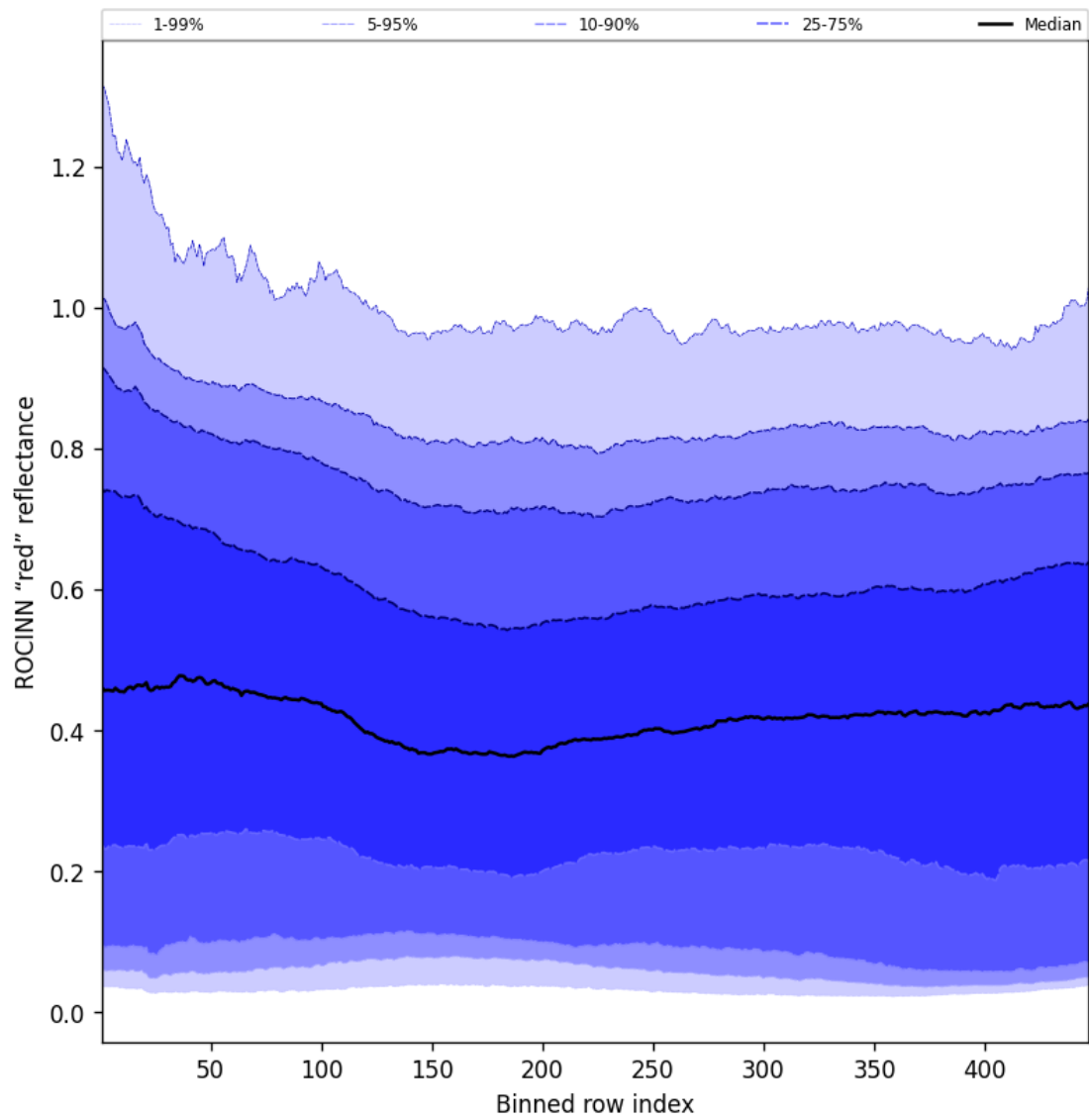
Figure 67: Along track statistics of "ROCINN "red" reflectance" for 2025-08-17 to 2025-08-17
