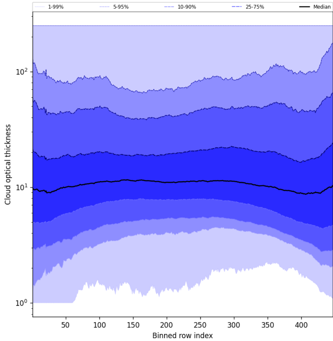
Figure 55: Along track statistics of “Cloud optical thickness” for 2025-08-17 to 2025-08-17
