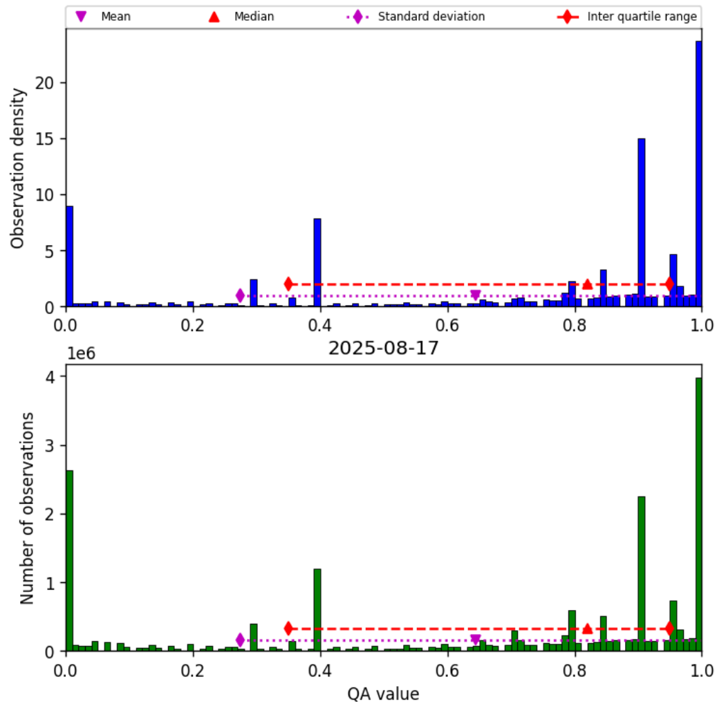
Figure 36: Histogram of “QA value” for 2025-08-17 to 2025-08-17
