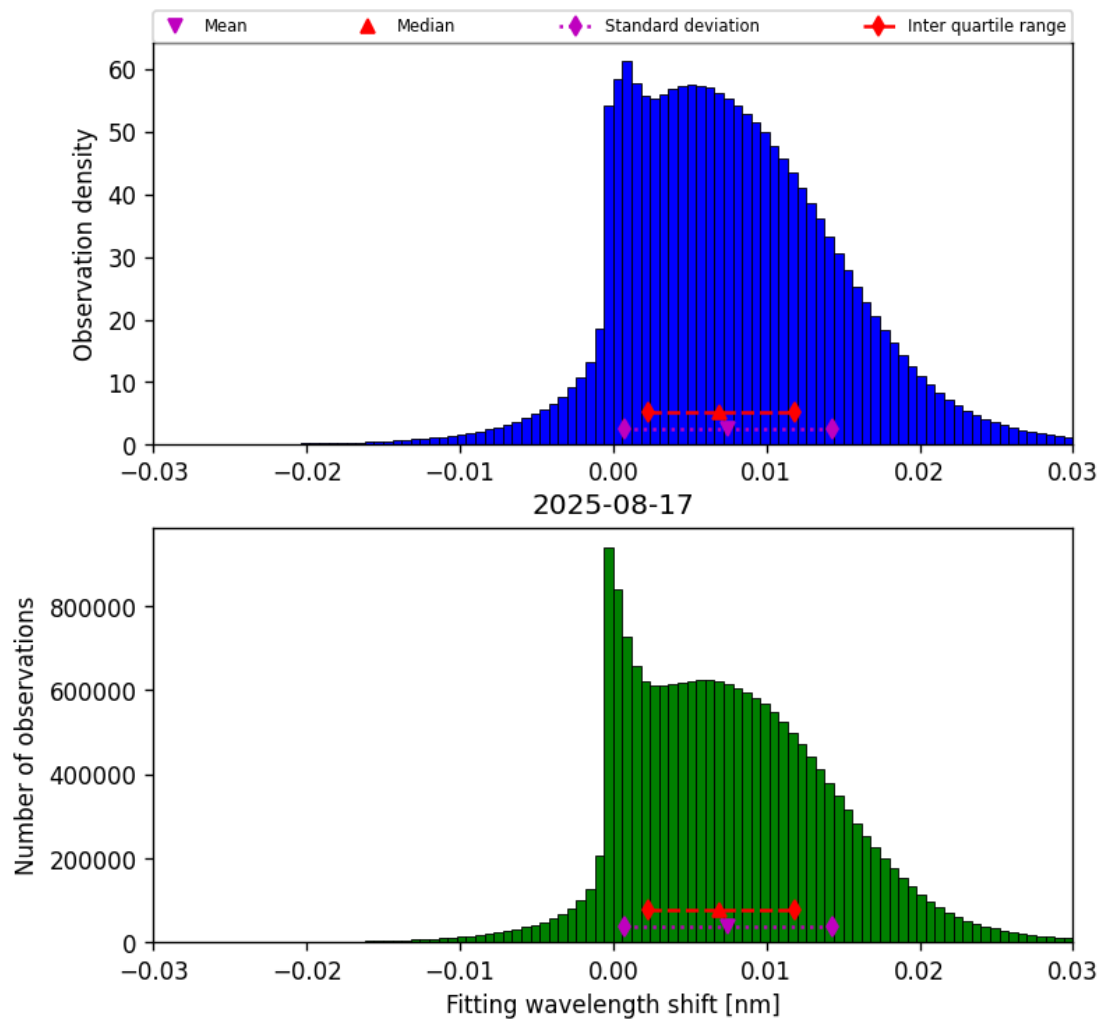
Figure 47: Histogram of “Fitting wavelength shift” for 2025-08-17 to 2025-08-17
