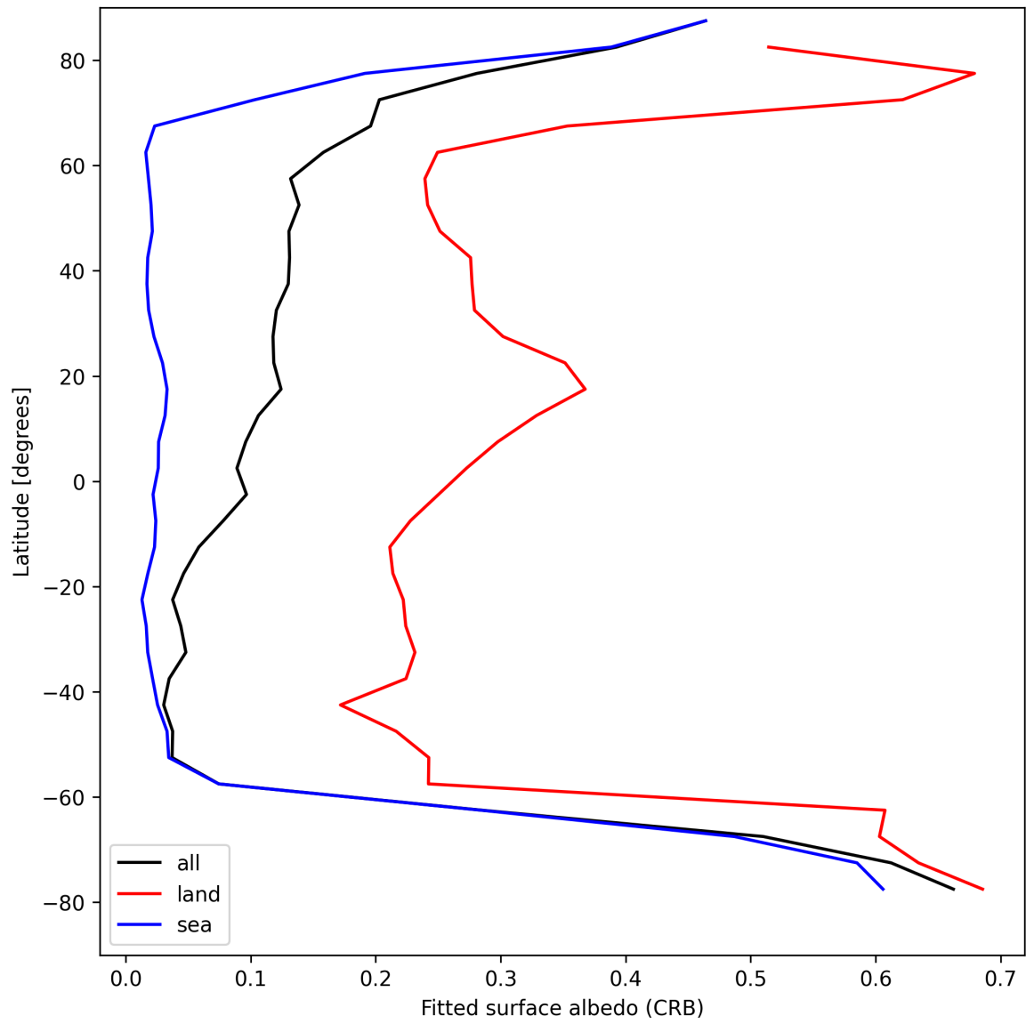
Figure 28: Zonal average of “Fitted surface albedo (CRB)” for 2025-08-17 to 2025-08-17.
