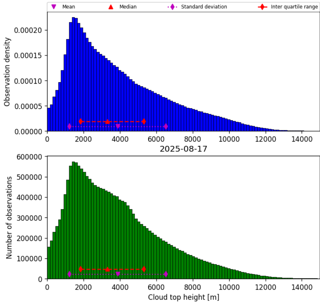
Figure 38: Histogram of “Cloud top height” for 2025-08-17 to 2025-08-17
