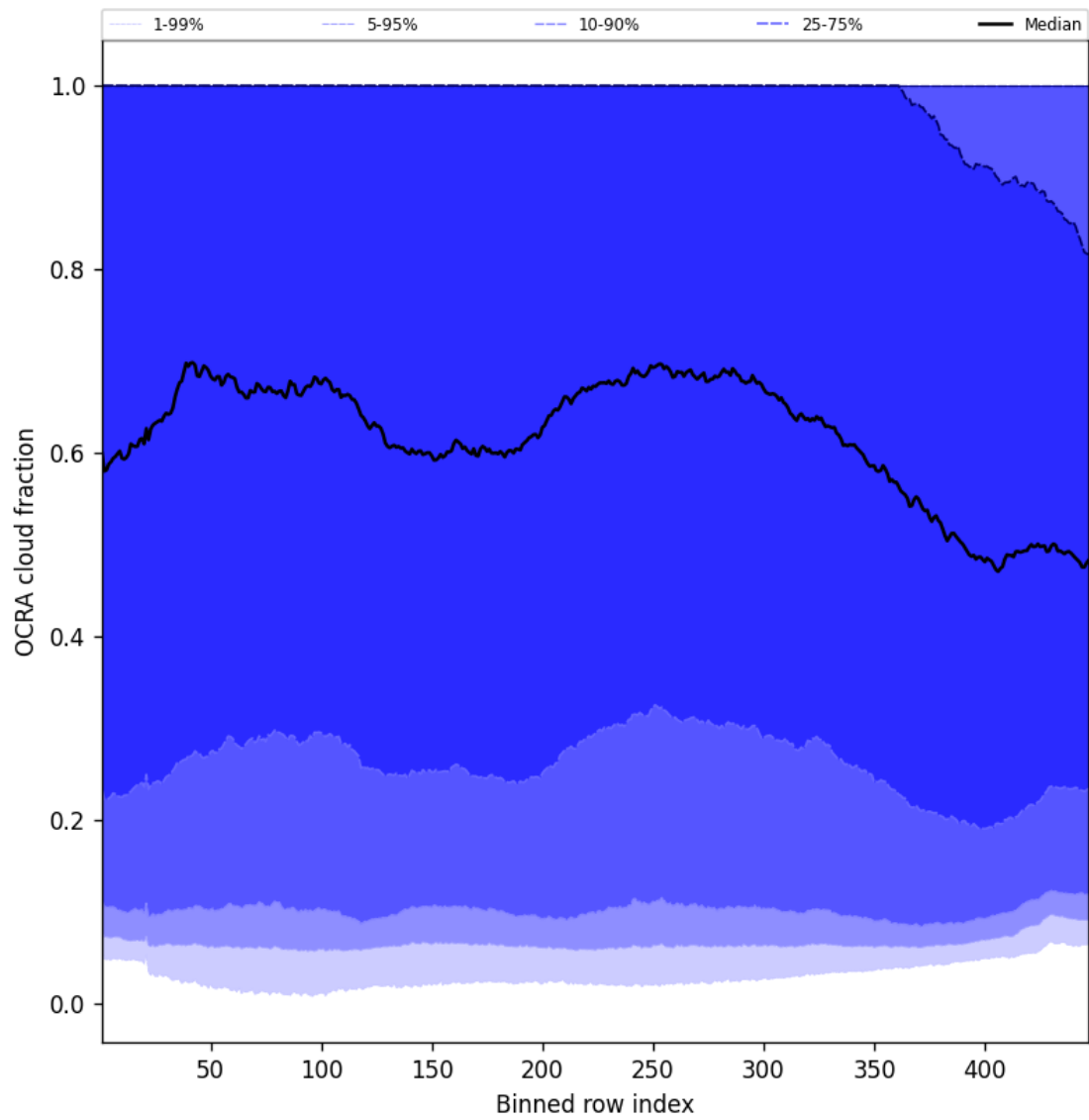
Figure 64: Along track statistics of “OCRA cloud fraction” for 2025-08-17 to 2025-08-17
