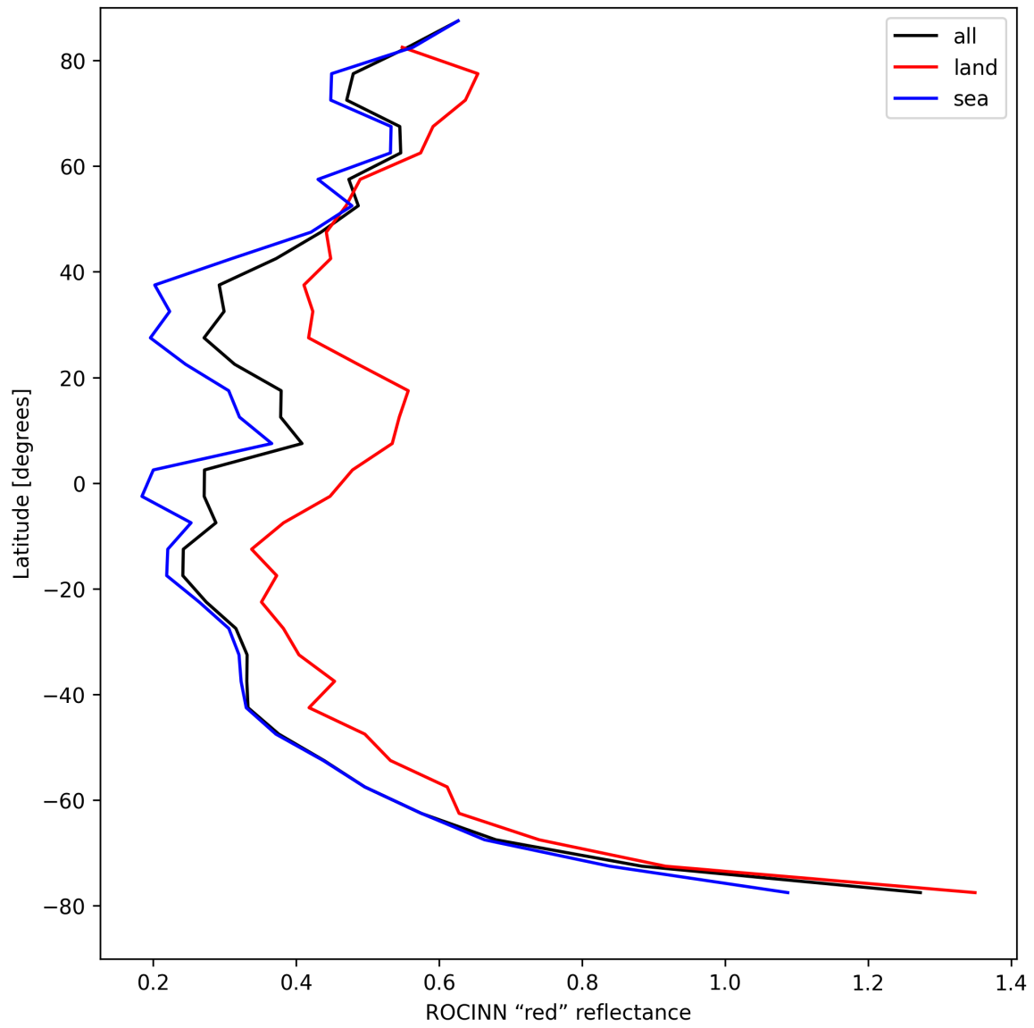
Figure 35: Zonal average of “ROCINN “red” reflectance” for 2025-08-17 to 2025-08-17.
