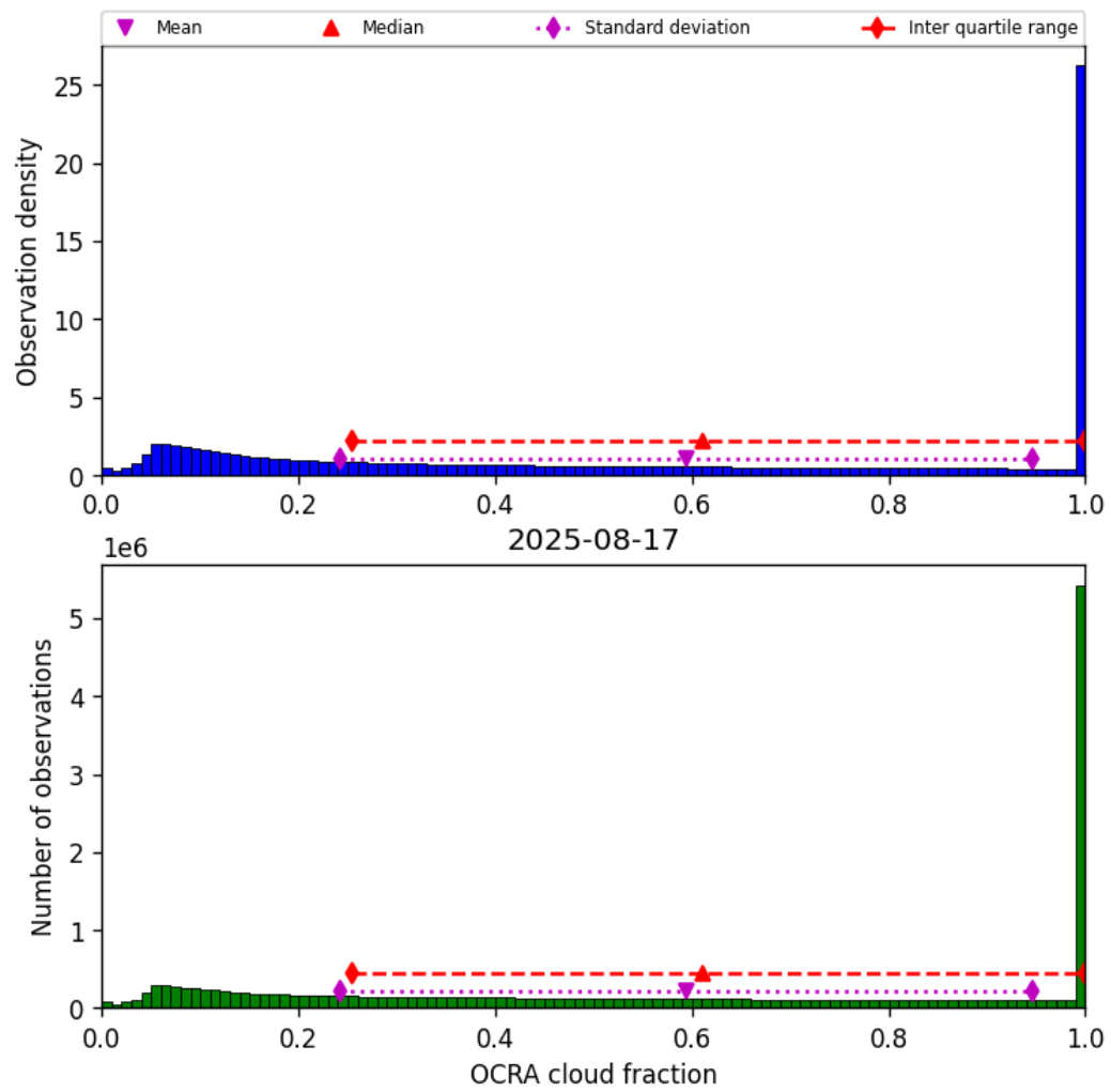
Figure 48: Histogram of “OCRA cloud fraction” for 2025-08-17 to 2025-08-17
