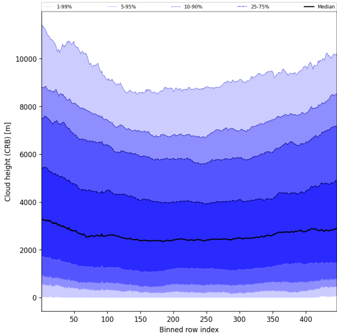
Figure 57: Along track statistics of “Cloud height (CRB)” for 2025-08-17 to 2025-08-17
