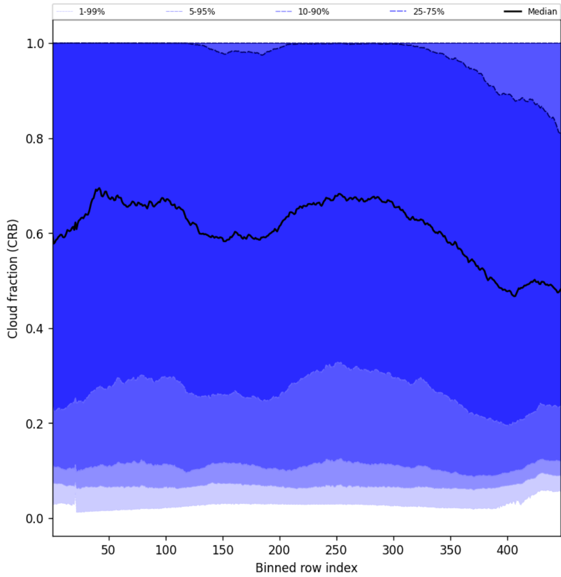
Figure 56: Along track statistics of “Cloud fraction (CRB)” for 2025-08-17 to 2025-08-17
