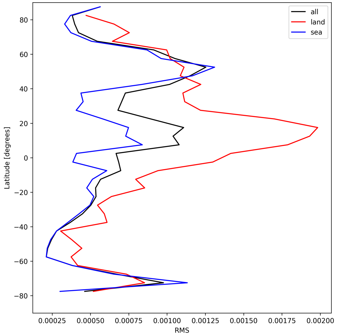
Figure 29: Zonal average of “RMS” for 2025-08-17 to 2025-08-17.
