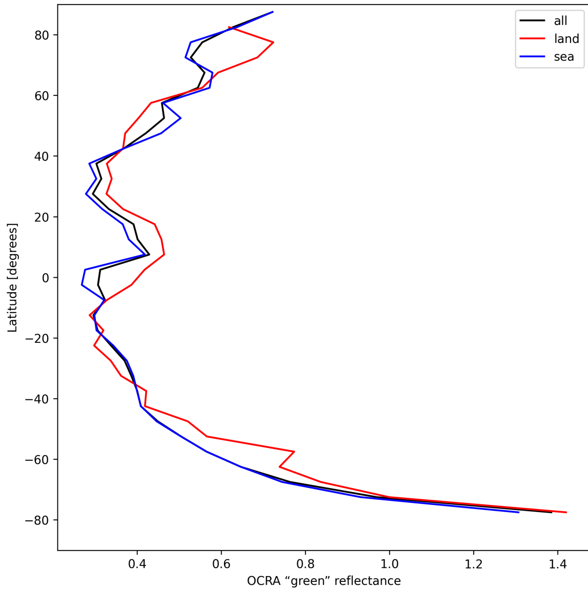
Figure 34: Zonal average of “OCRA “green” reflectance” for 2025-08-17 to 2025-08-17.
