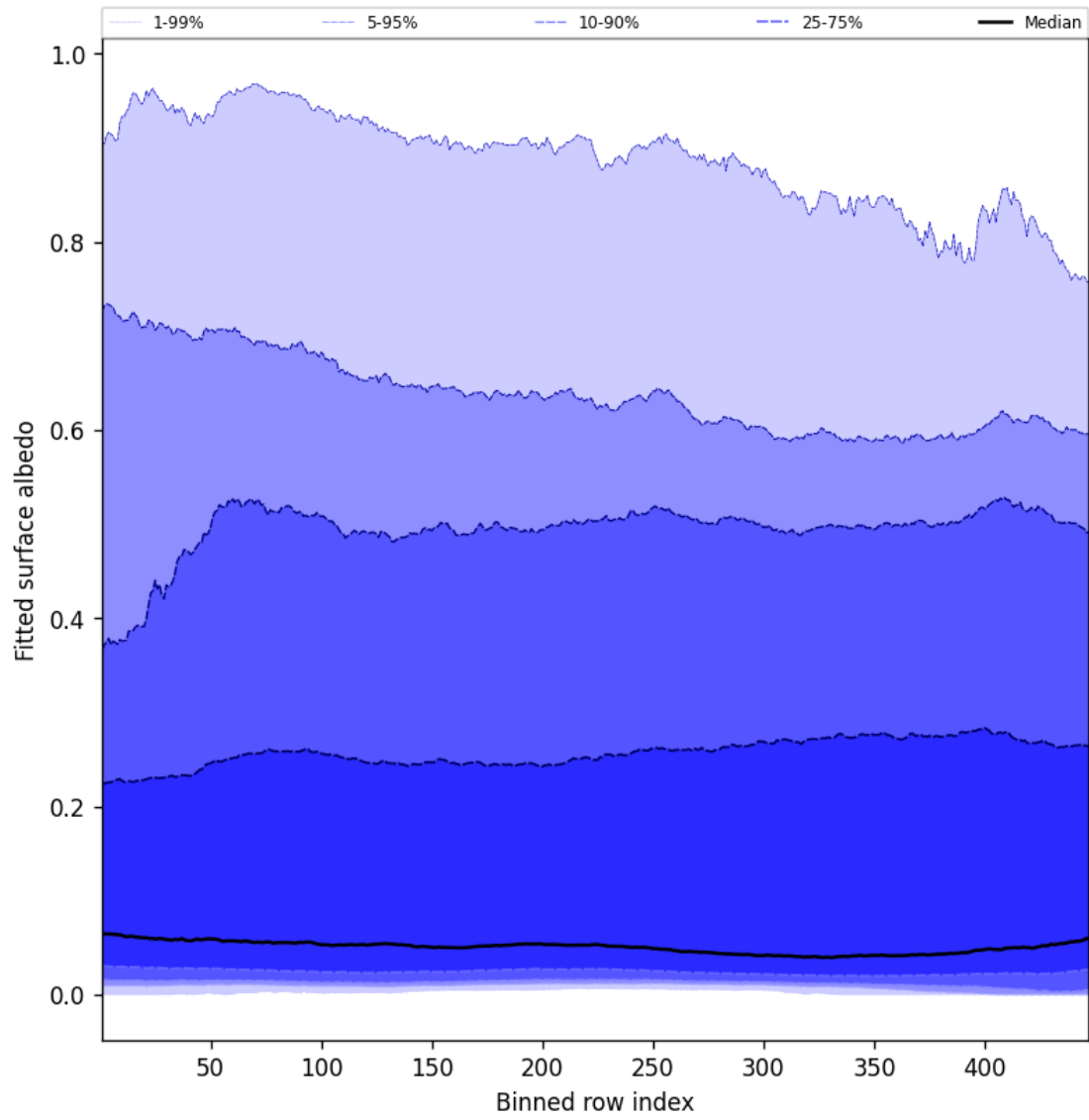
Figure 59: Along track statistics of “Fitted surface albedo” for 2025-08-17 to 2025-08-17
