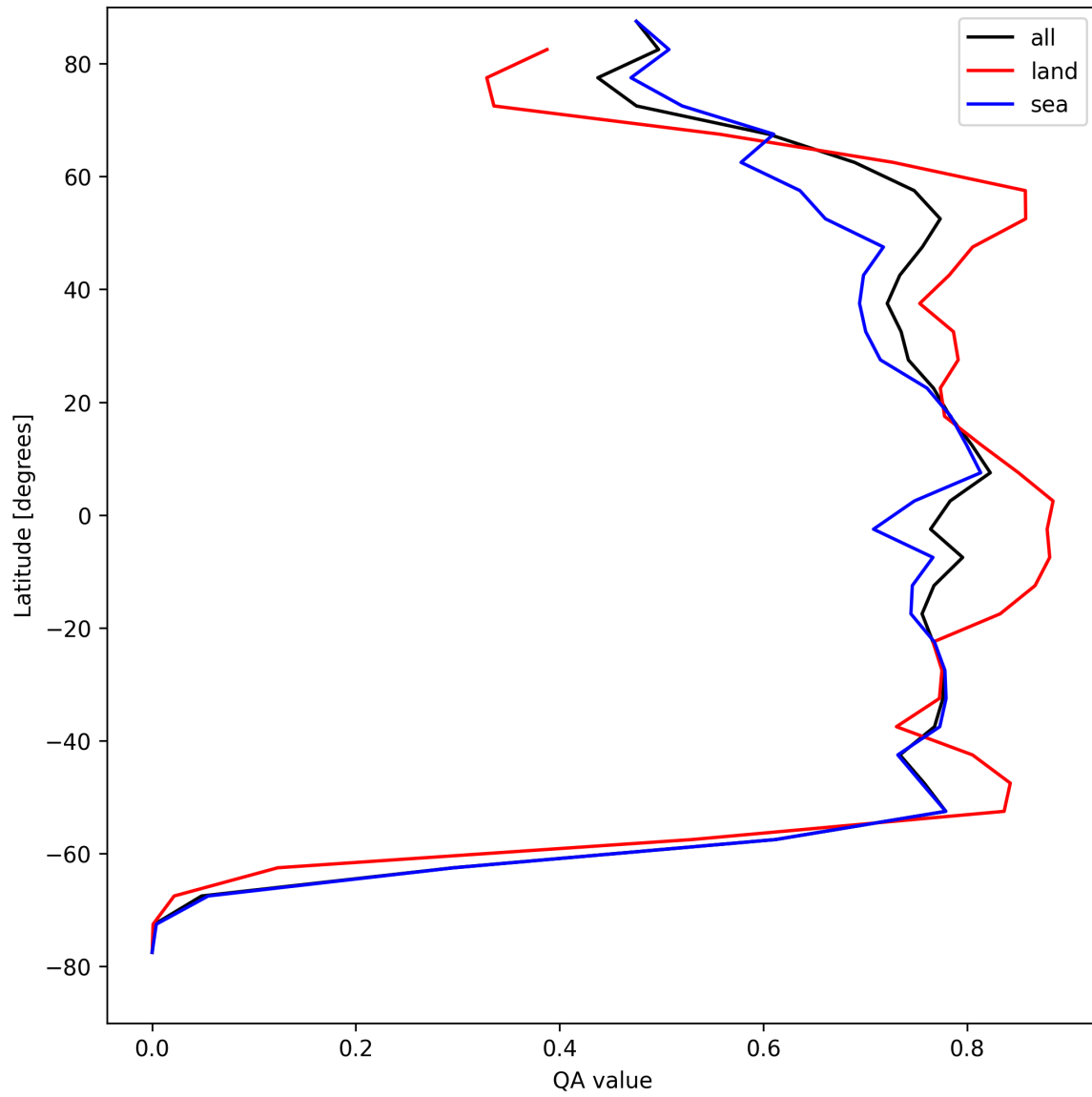
Figure 20: Zonal average of “QA value” for 2025-08-17 to 2025-08-17.
