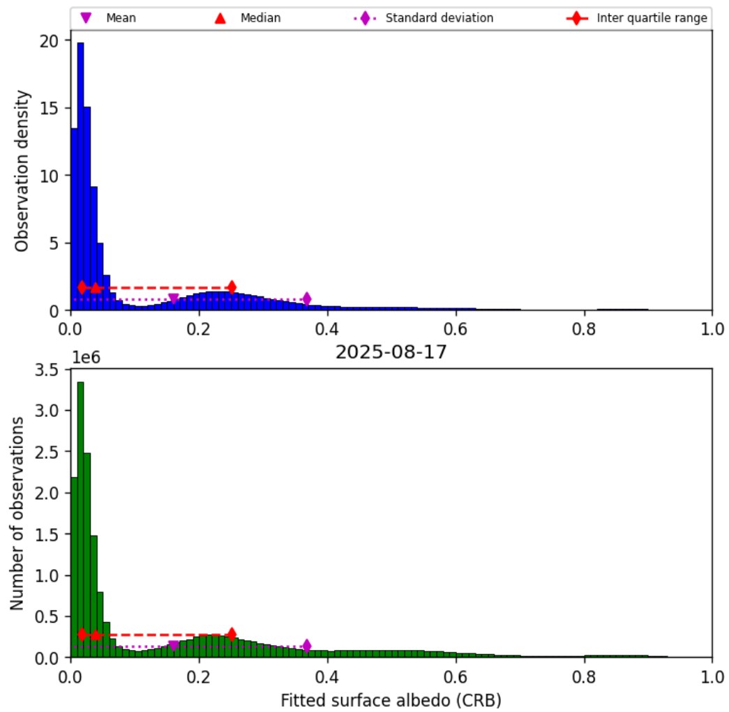
Figure 44: Histogram of “Fitted surface albedo (CRB)” for 2025-08-17 to 2025-08-17
