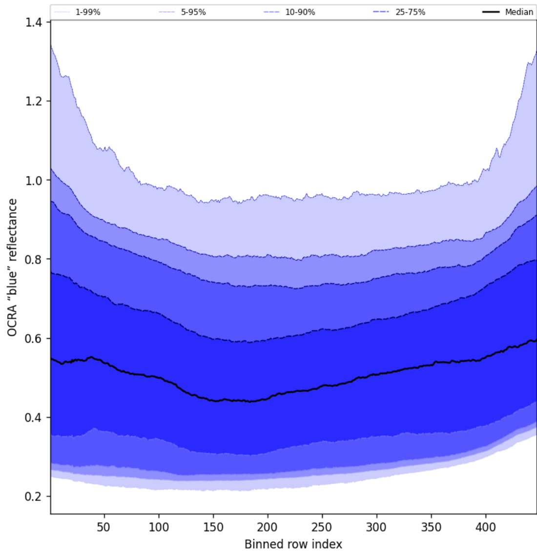
Figure 65: Along track statistics of “OCRA “blue” reflectance” for 2025-08-17 to 2025-08-17
