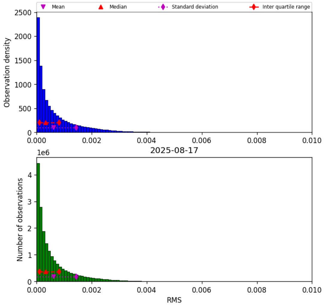
Figure 45: Histogram of “RMS” for 2025-08-17 to 2025-08-17
