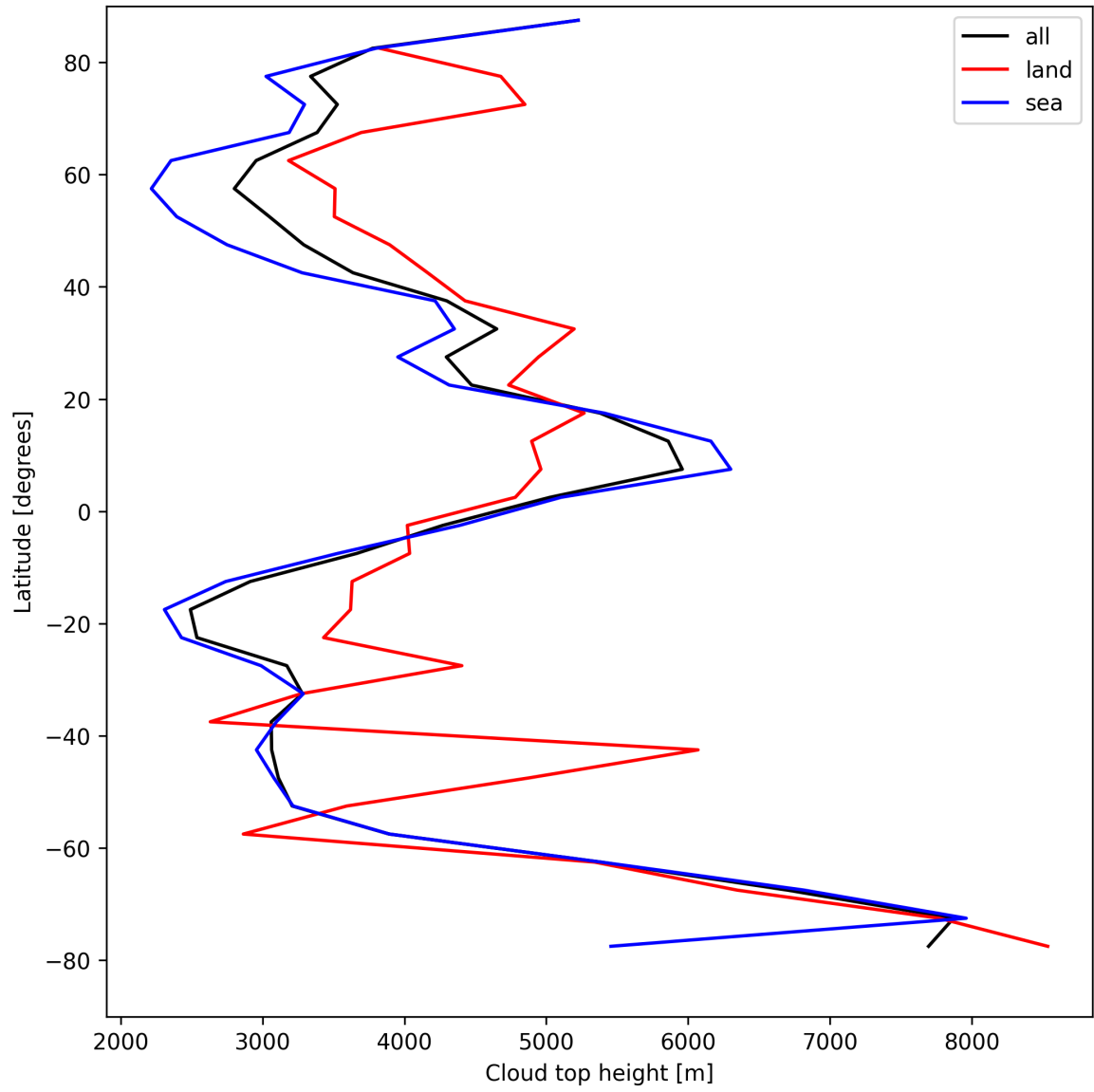
Figure 22: Zonal average of “Cloud top height” for 2025-08-17 to 2025-08-17.
