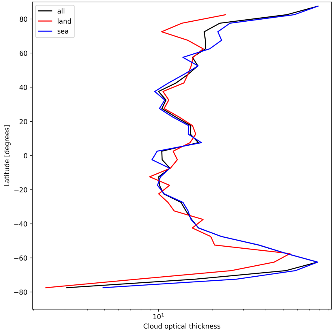
Figure 23: Zonal average of “Cloud optical thickness” for 2025-08-17 to 2025-08-17.
