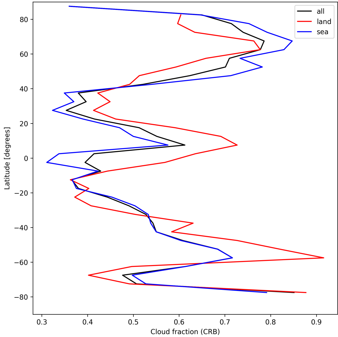
Figure 24: Zonal average of “Cloud fraction (CRB)” for 2025-08-17 to 2025-08-17.
