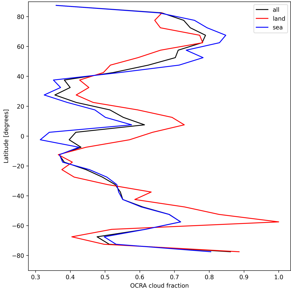
Figure 32: Zonal average of “OCRA cloud fraction” for 2025-08-17 to 2025-08-17.
