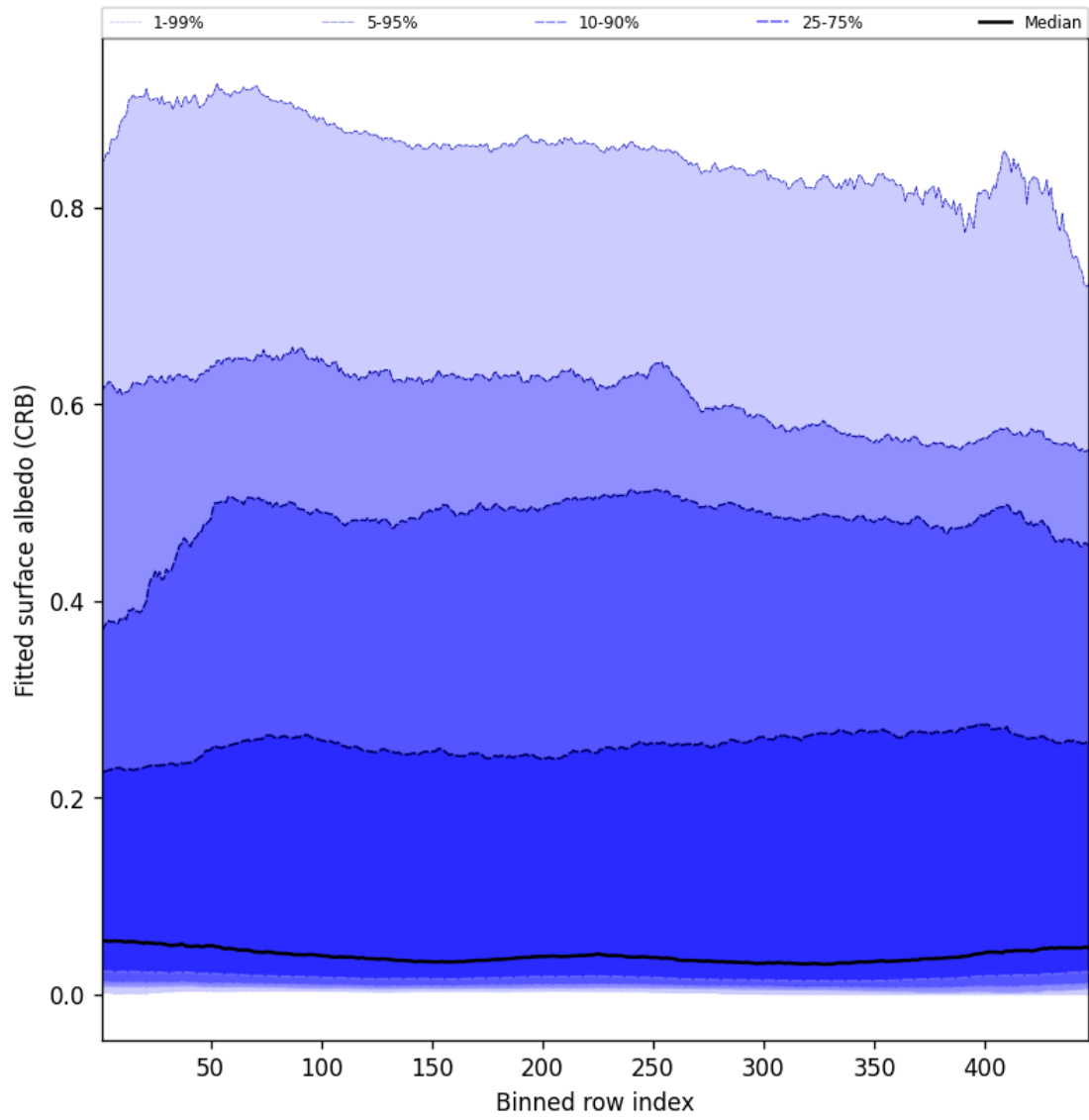
Figure 60: Along track statistics of “Fitted surface albedo (CRB)” for 2025-08-17 to 2025-08-17
