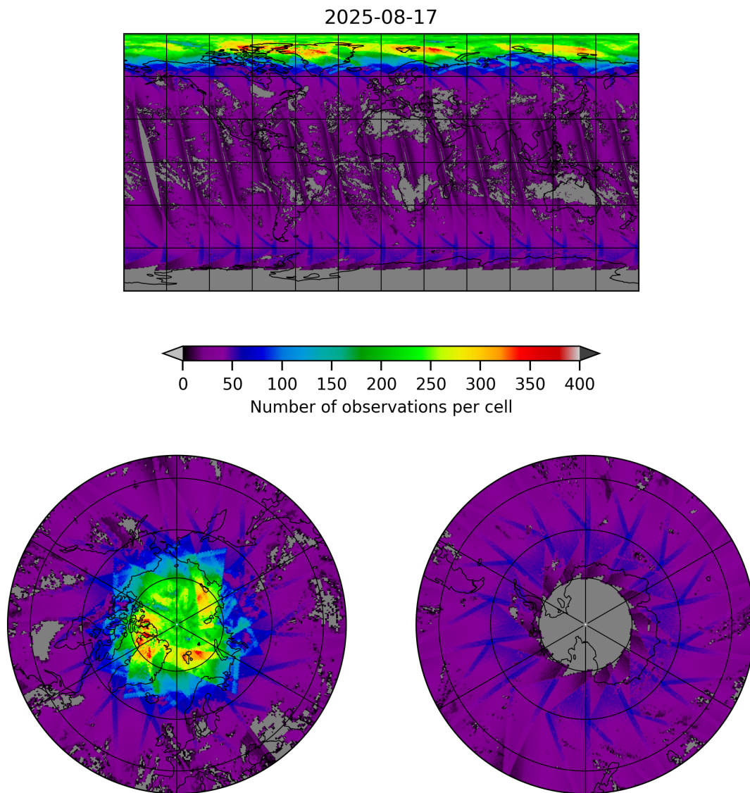
Figure 19: Map of the number of observations for 2025-08-17 to 2025-08-17
