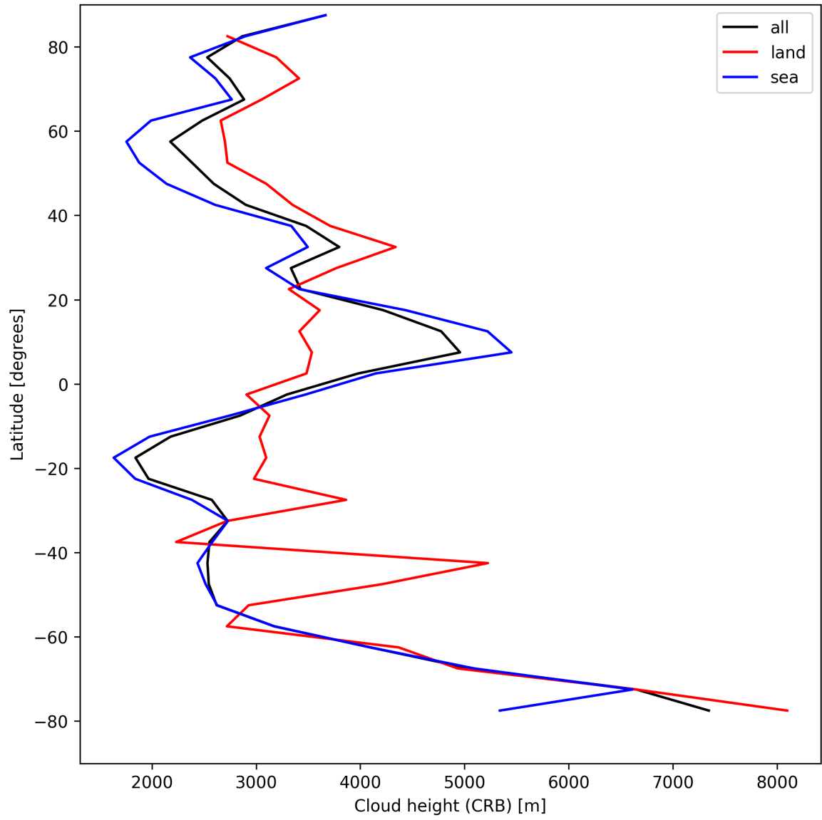
Figure 25: Zonal average of “Cloud height (CRB)” for 2025-08-17 to 2025-08-17.
