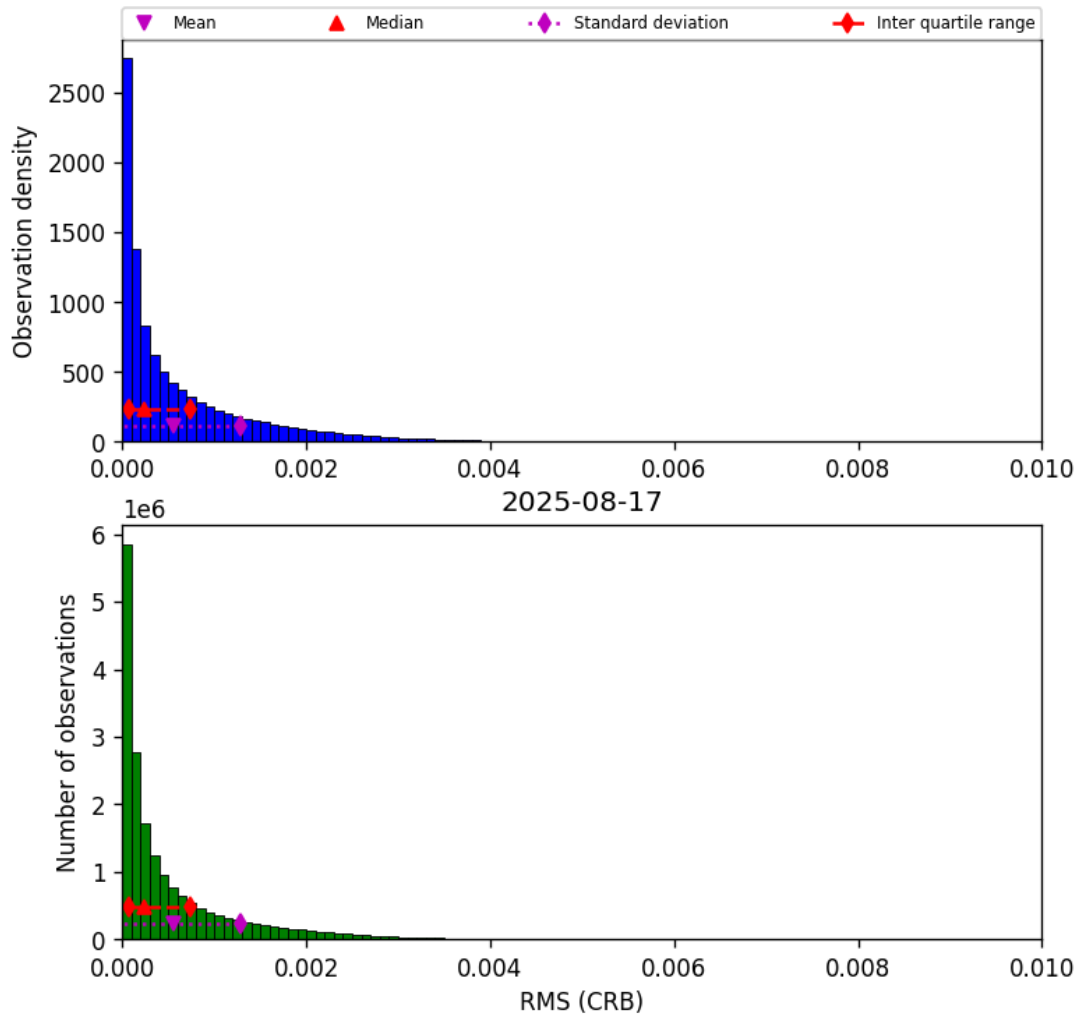
Figure 46: Histogram of “RMS (CRB)” for 2025-08-17 to 2025-08-17
