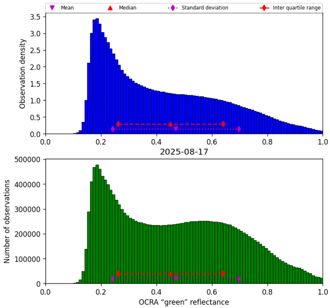
Figure 50: Histogram of “OCRA “green” reflectance” for 2025-08-17 to 2025-08-17
