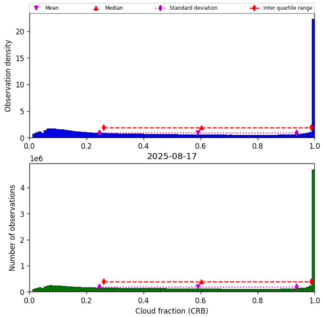
Figure 40: Histogram of “Cloud fraction (CRB)” for 2025-08-17 to 2025-08-17
