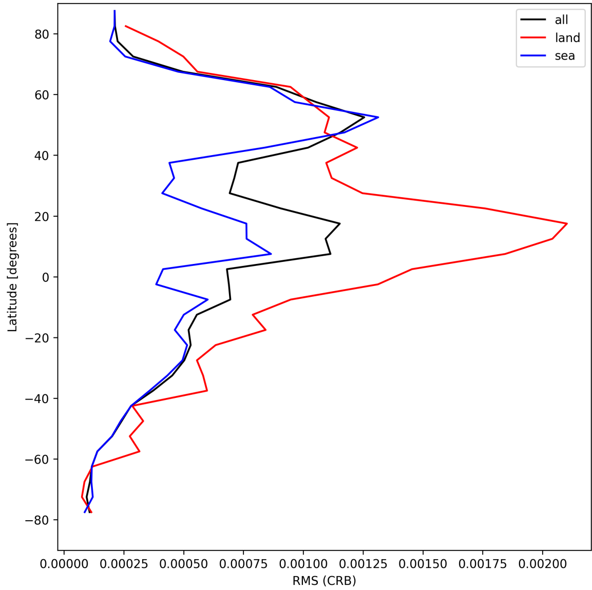
Figure 30: Zonal average of “RMS (CRB)” for 2025-08-17 to 2025-08-17.
