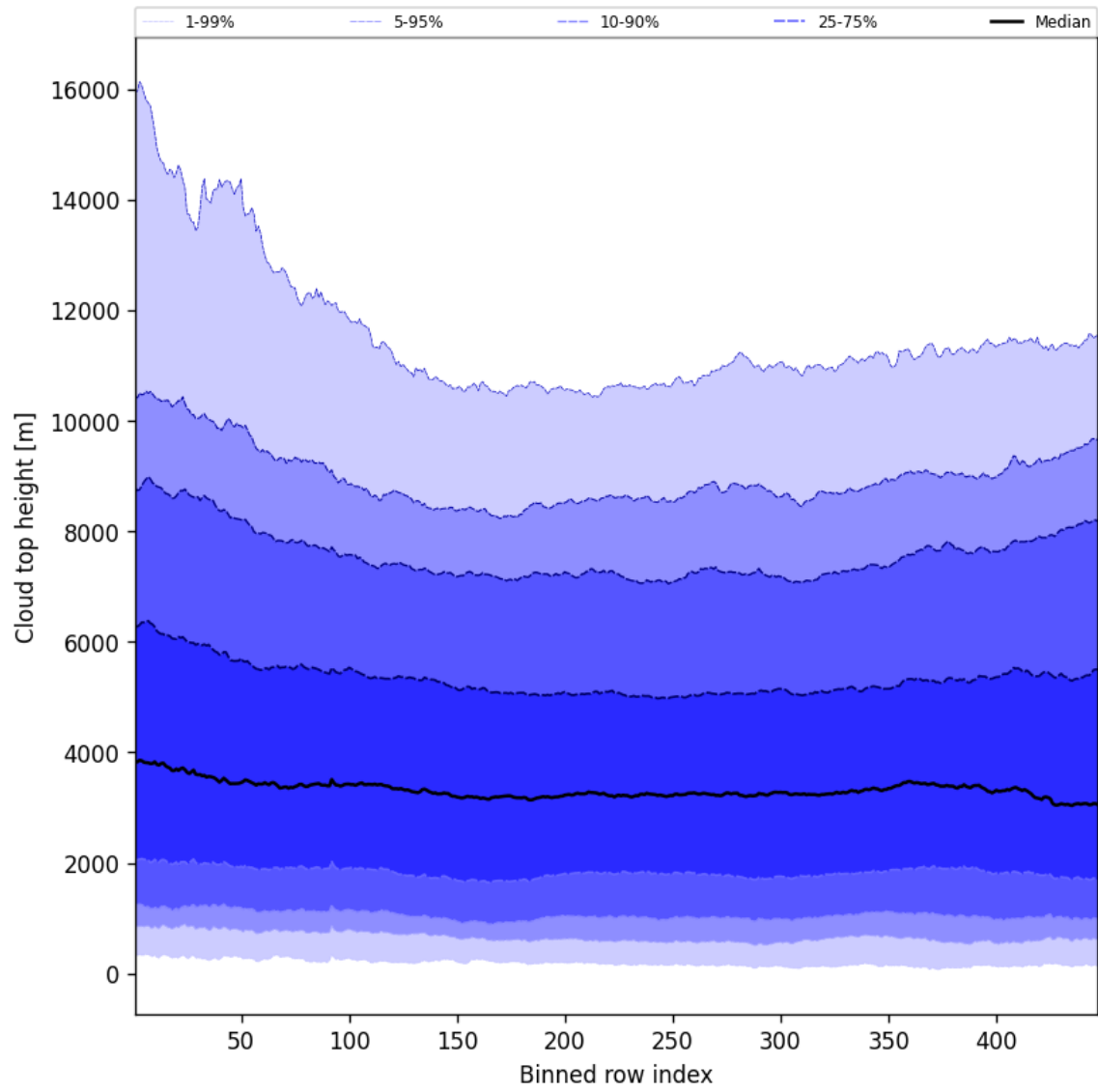
Figure 54: Along track statistics of “Cloud top height” for 2025-08-17 to 2025-08-17
