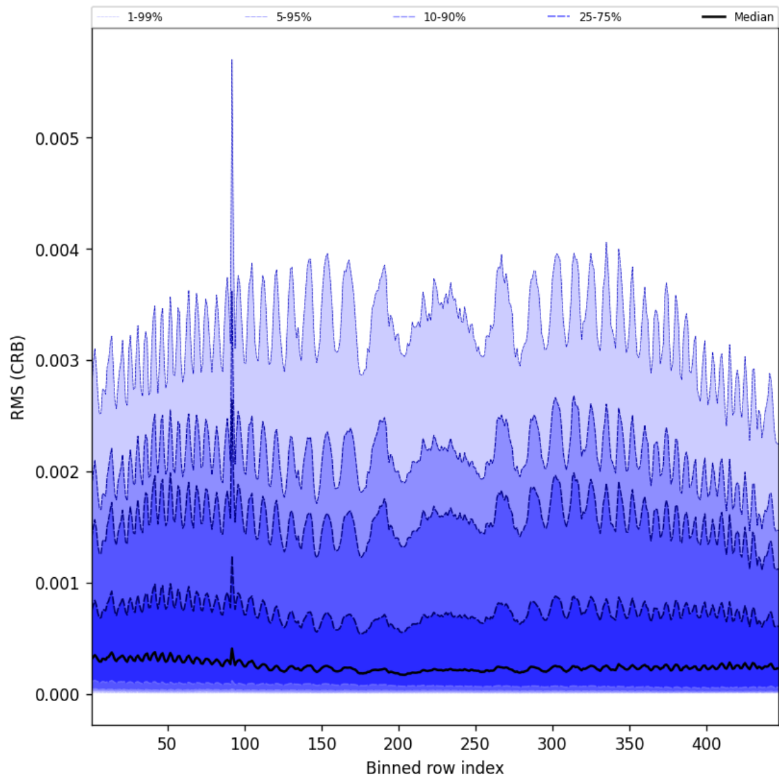
Figure 62: Along track statistics of “RMS (CRB)” for 2025-08-17 to 2025-08-17
