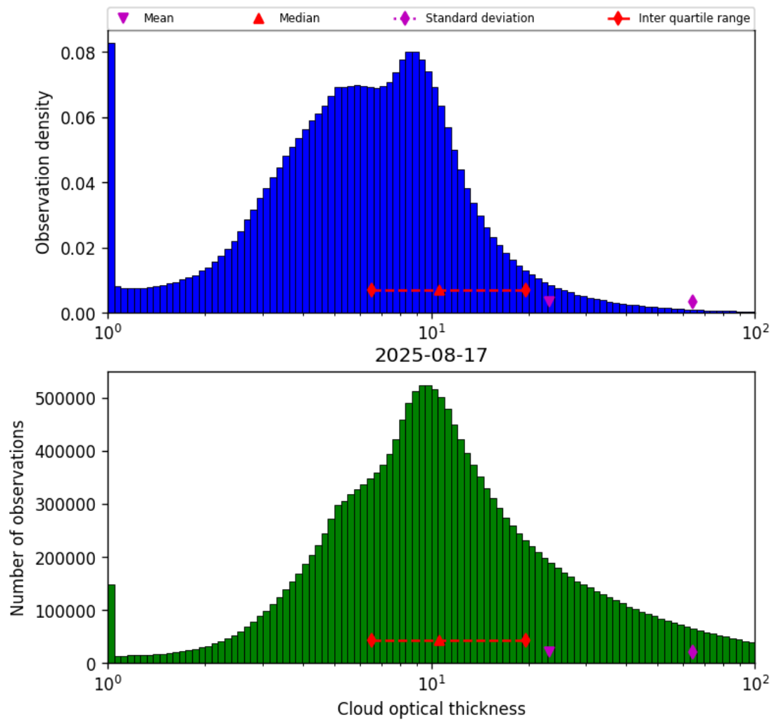
Figure 39: Histogram of “Cloud optical thickness” for 2025-08-17 to 2025-08-17
