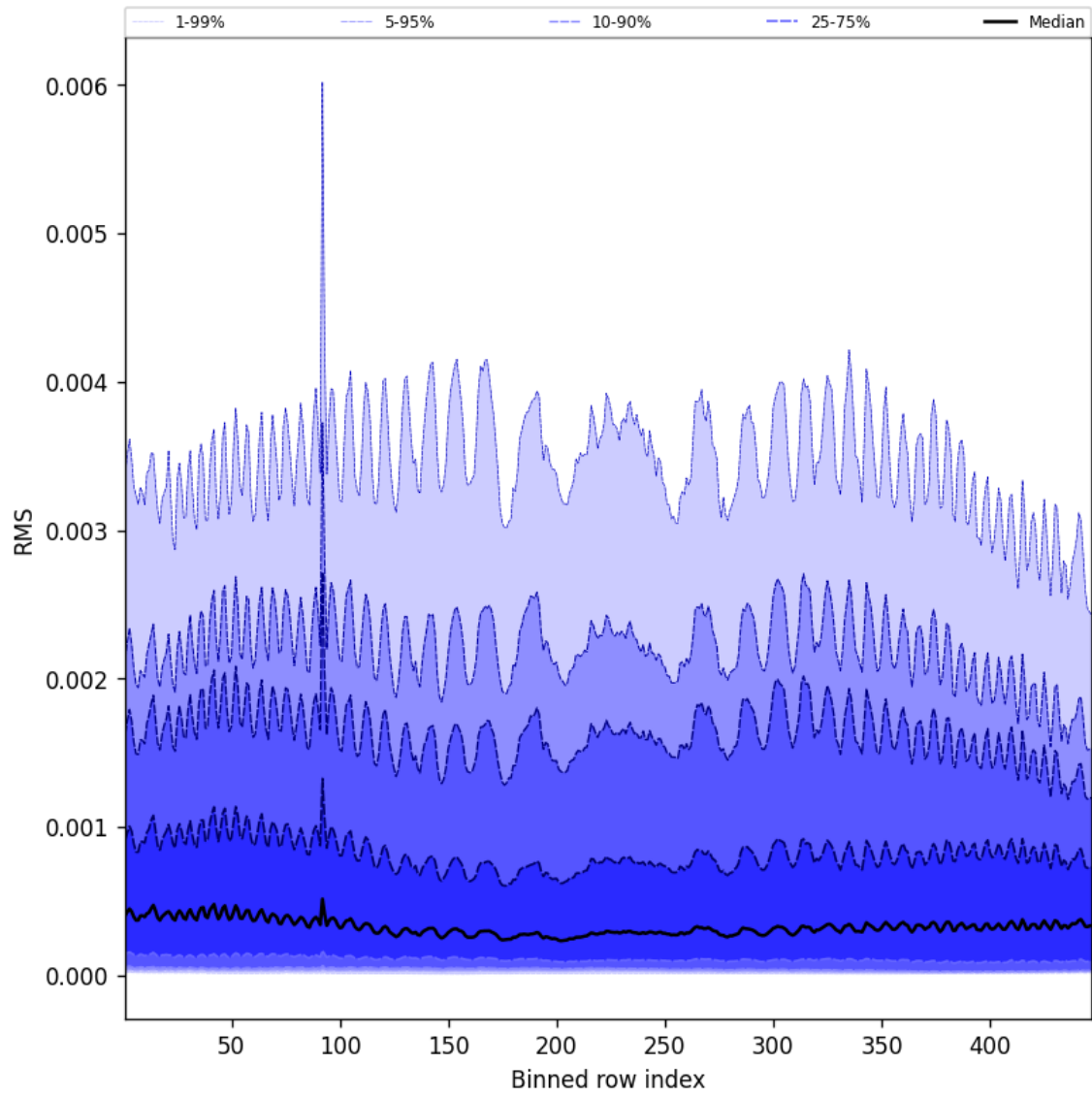
Figure 61: Along track statistics of “RMS” for 2025-08-17 to 2025-08-17
