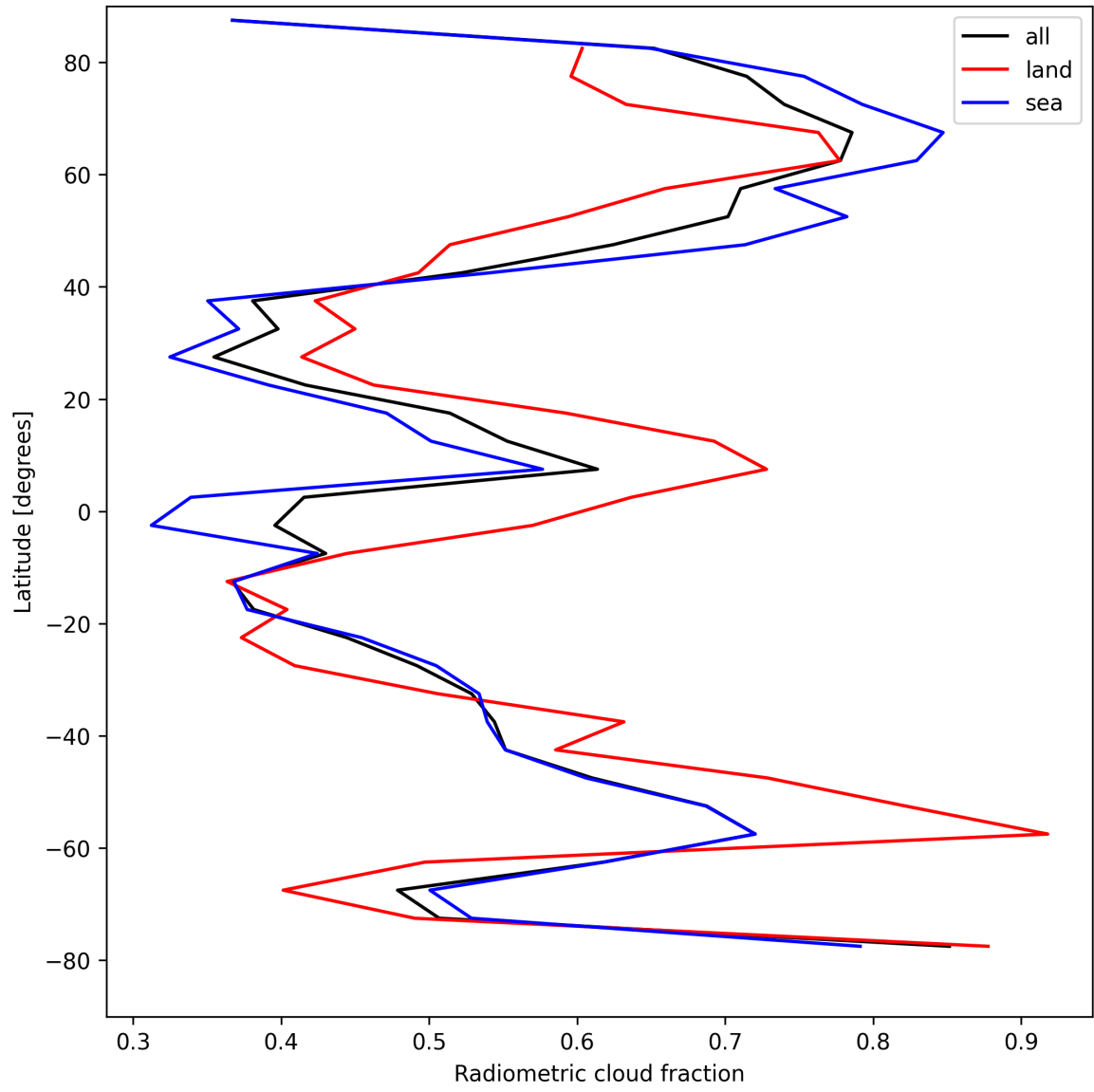
Figure 21: Zonal average of “Radiometric cloud fraction” for 2025-08-17 to 2025-08-17.
