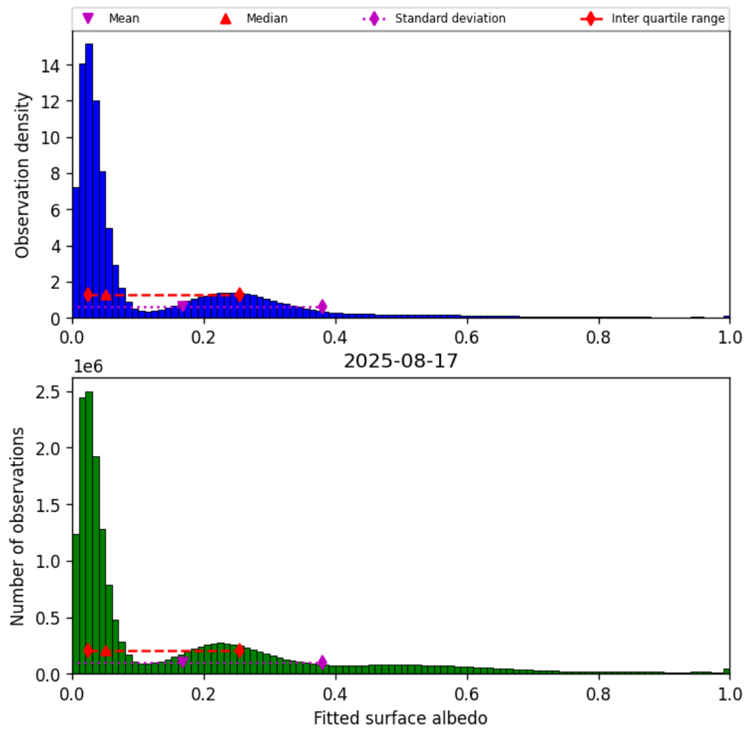
Figure 43: Histogram of “Fitted surface albedo” for 2025-08-17 to 2025-08-17
