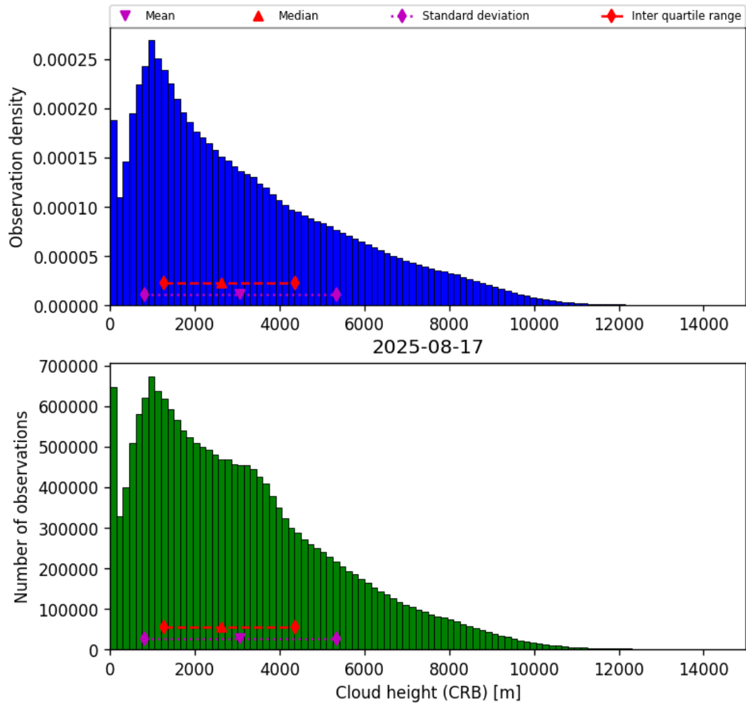
Figure 41: Histogram of “Cloud height (CRB)” for 2025-08-17 to 2025-08-17
