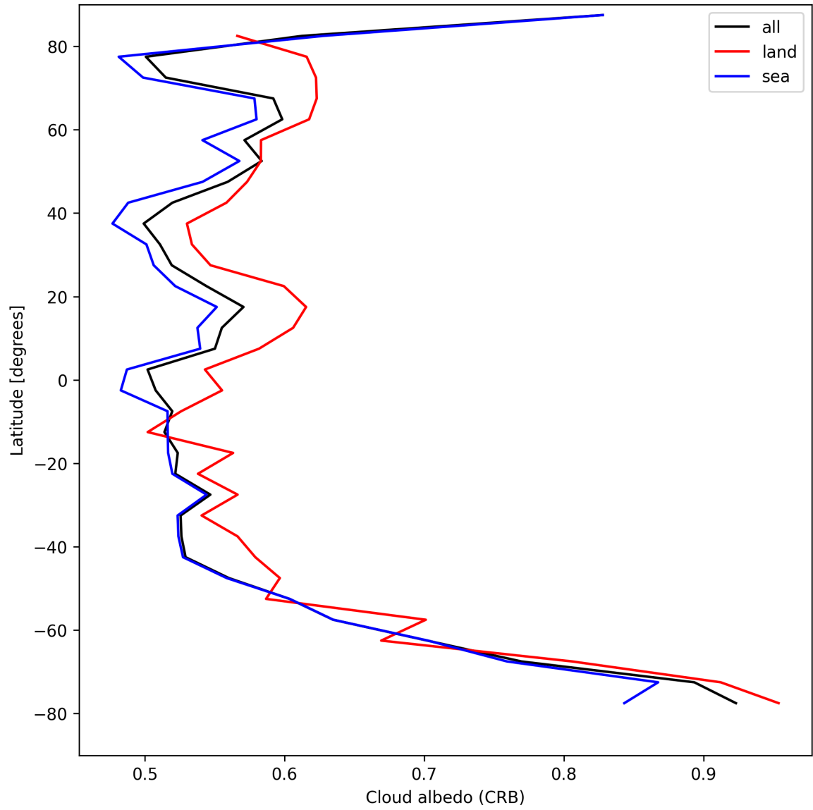
Figure 26: Zonal average of “Cloud albedo (CRB)” for 2025-08-17 to 2025-08-17.
