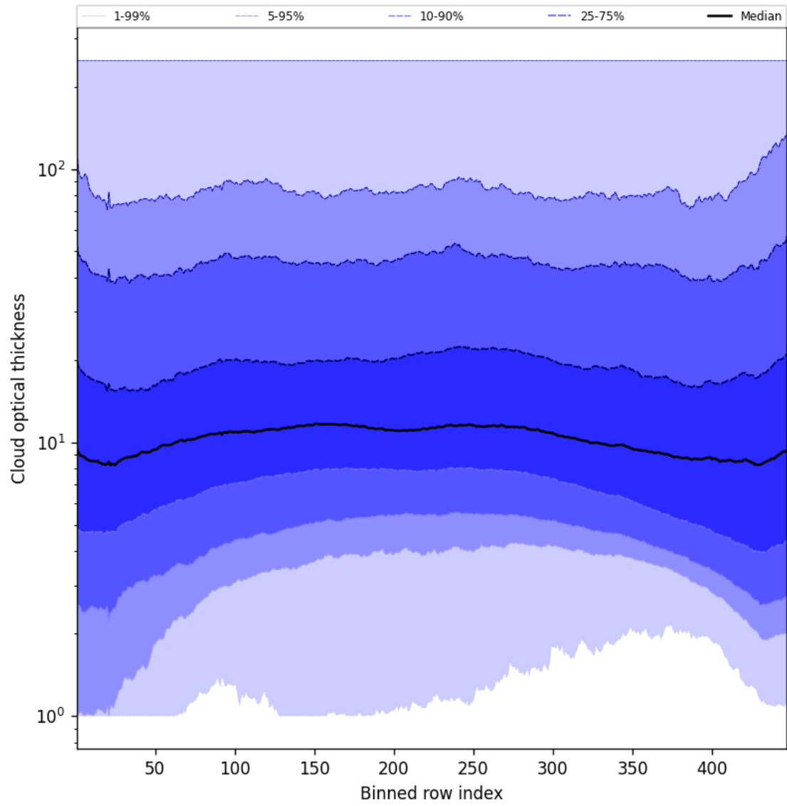
Figure 55: Along track statistics of “Cloud optical thickness” for 2025-08-18 to 2025-08-19
