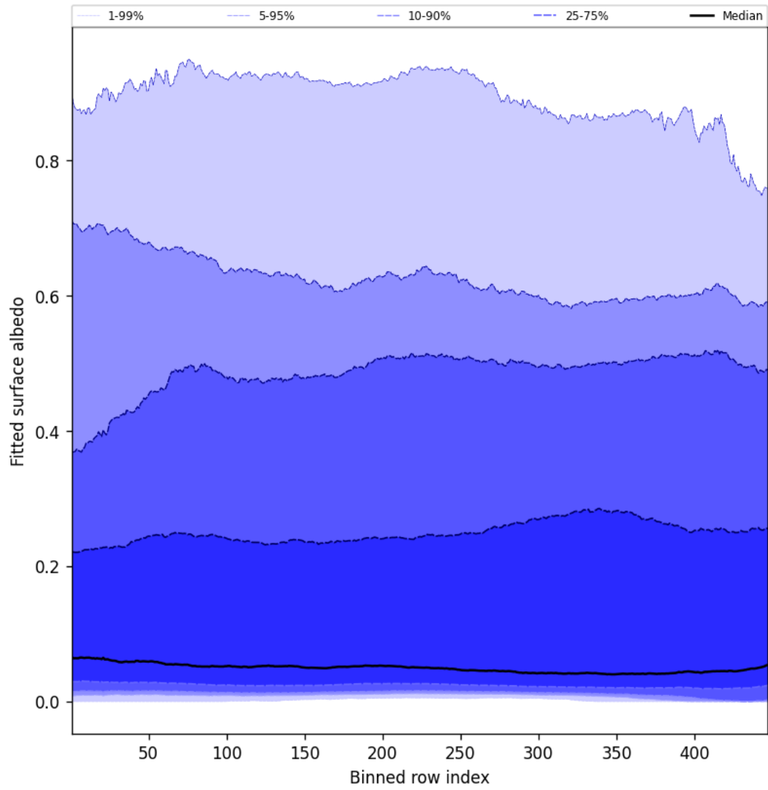
Figure 59: Along track statistics of “Fitted surface albedo” for 2025-08-18 to 2025-08-19
