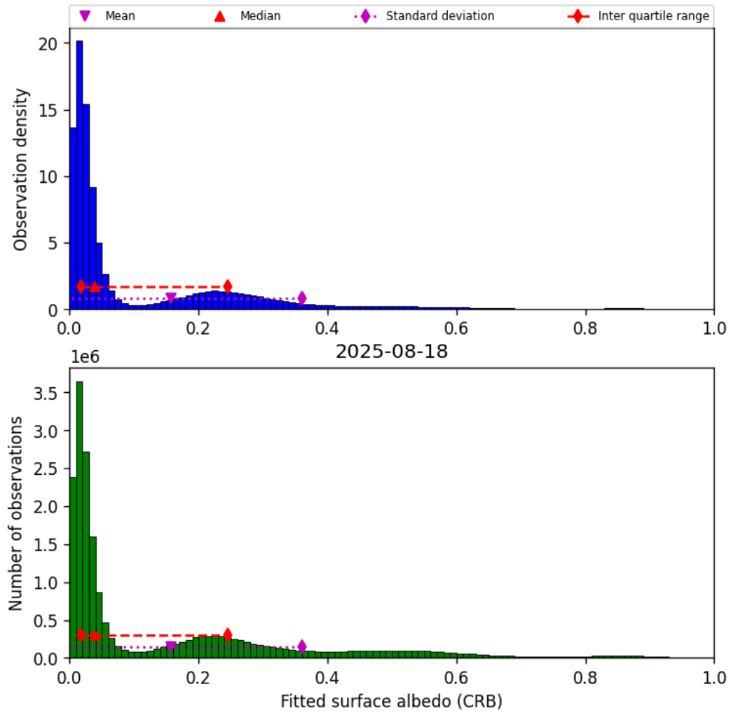
Figure 44: Histogram of “Fitted surface albedo (CRB)” for 2025-08-18 to 2025-08-19
