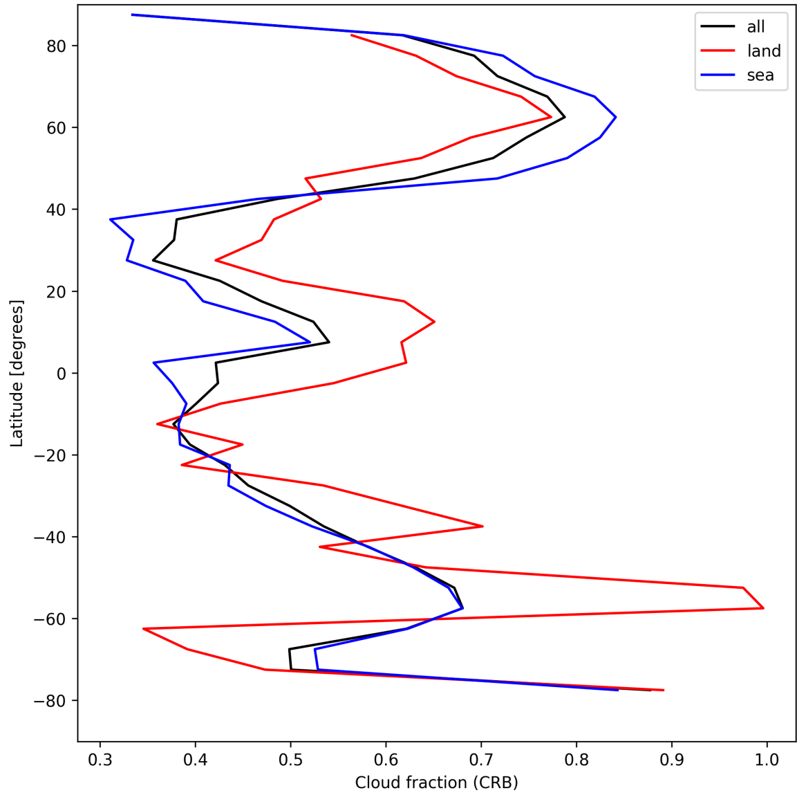
Figure 24: Zonal average of “Cloud fraction (CRB)” for 2025-08-18 to 2025-08-19.
