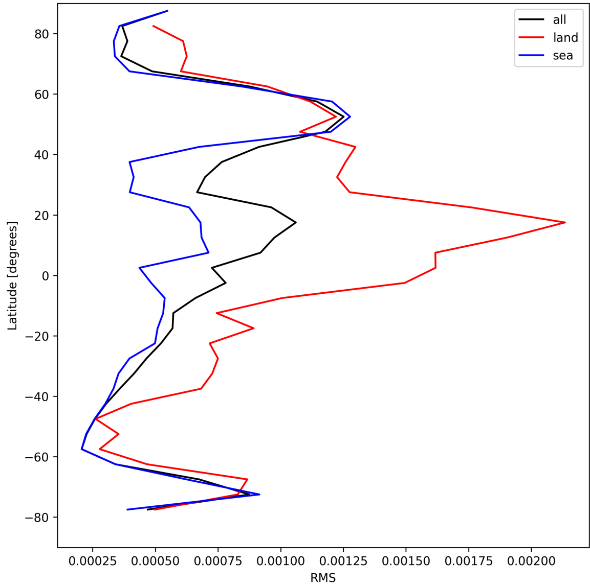
Figure 29: Zonal average of “RMS” for 2025-08-18 to 2025-08-19.
