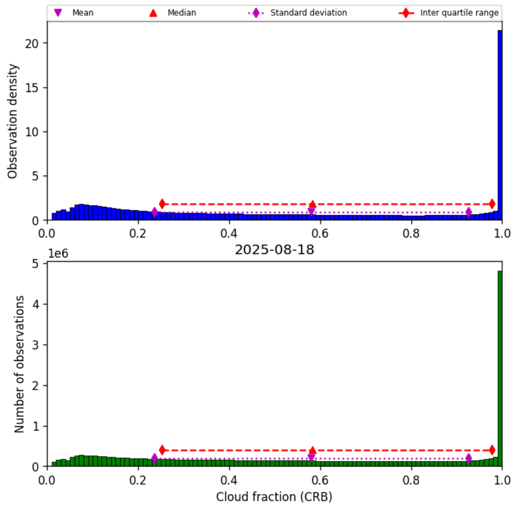
Figure 40: Histogram of "Cloud fraction (CRB)" for 2025-08-18 to 2025-08-19
