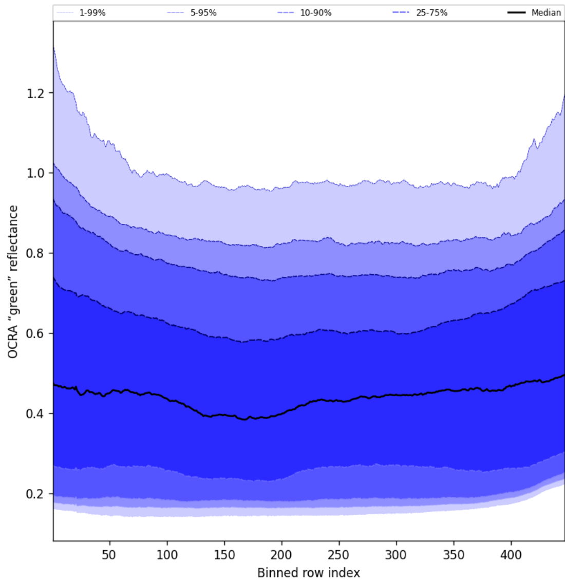
Figure 66: Along track statistics of “OCRA “green” reflectance” for 2025-08-18 to 2025-08-19
