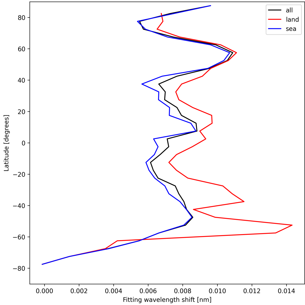
Figure 31: Zonal average of “Fitting wavelength shift” for 2025-08-18 to 2025-08-19.
