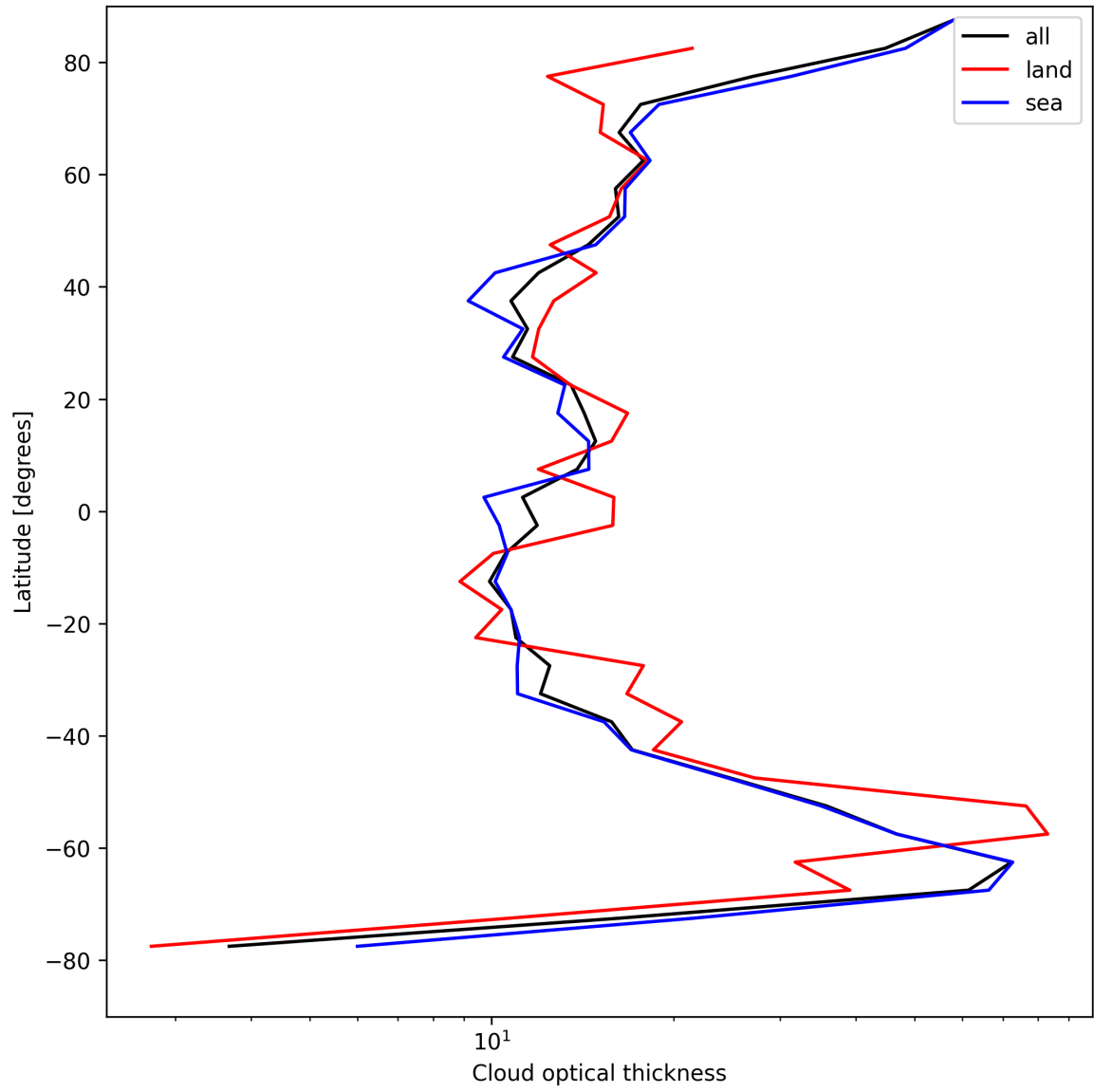
Figure 23: Zonal average of “Cloud optical thickness” for 2025-08-18 to 2025-08-19.
