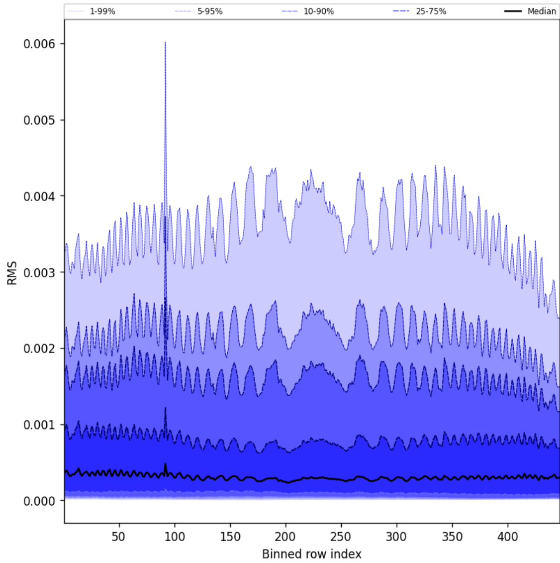
Figure 61: Along track statistics of “RMS” for 2025-08-18 to 2025-08-19
