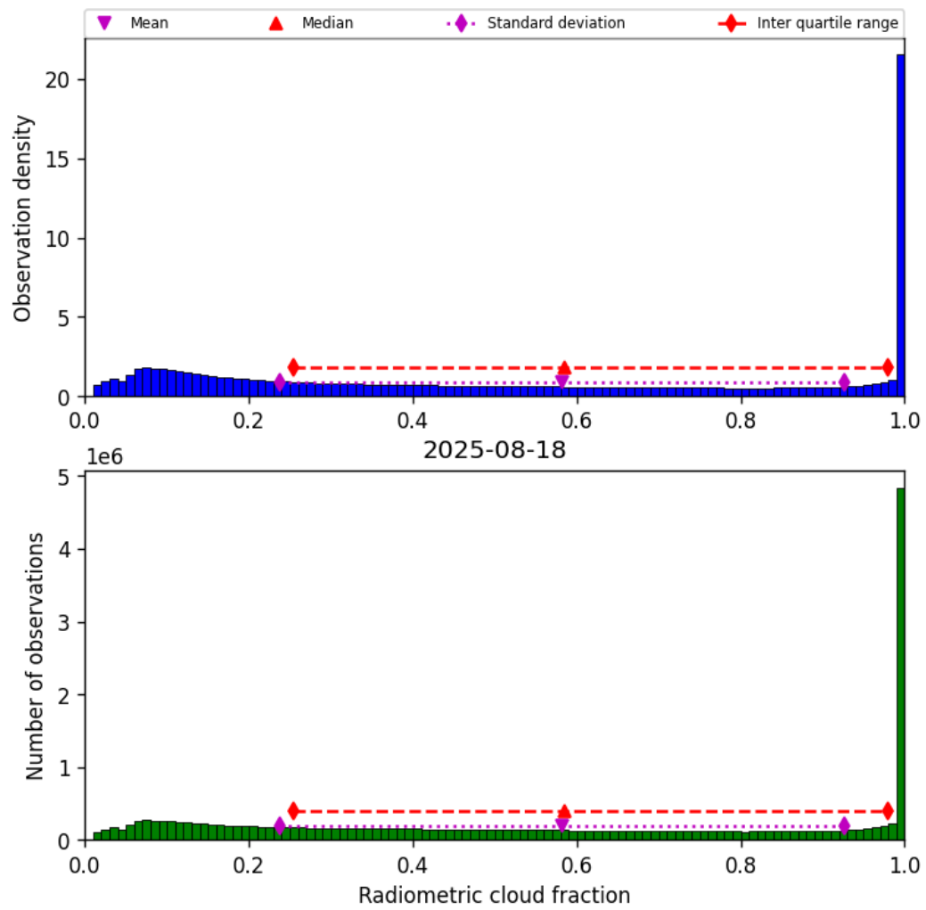
Figure 37: Histogram of “Radiometric cloud fraction” for 2025-08-18 to 2025-08-19
