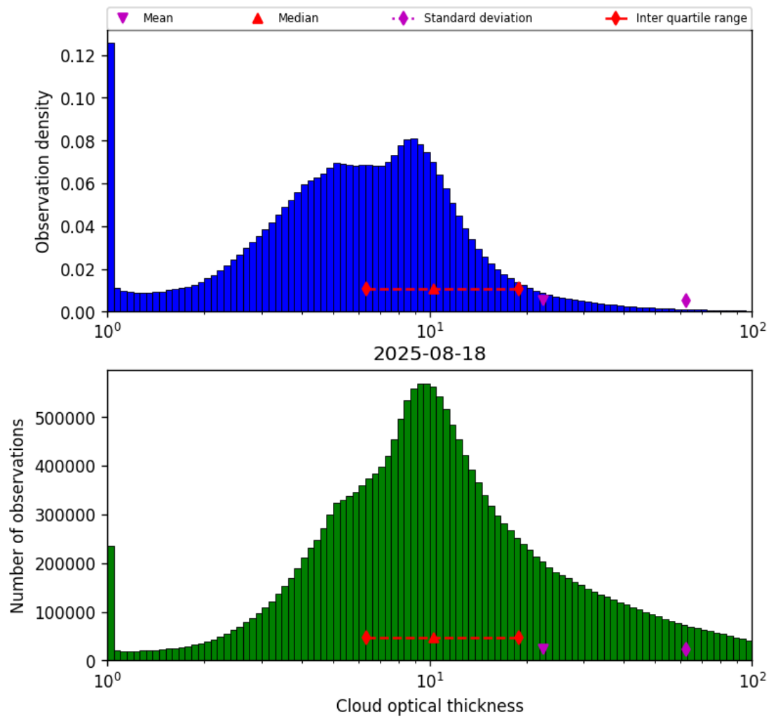
Figure 39: Histogram of “Cloud optical thickness” for 2025-08-18 to 2025-08-19
