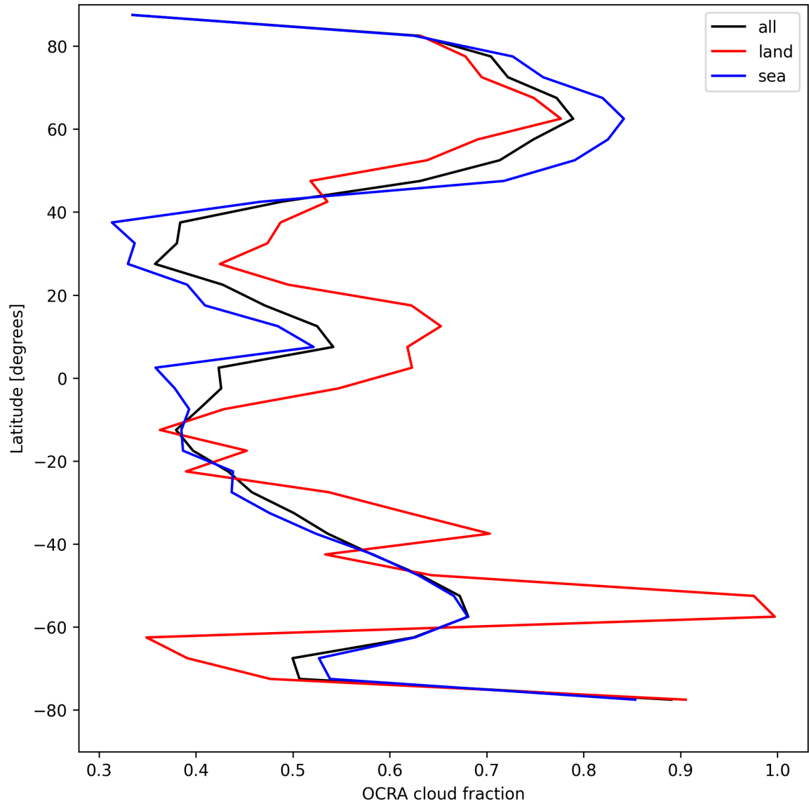
Figure 32: Zonal average of “OCRA cloud fraction” for 2025-08-18 to 2025-08-19.
