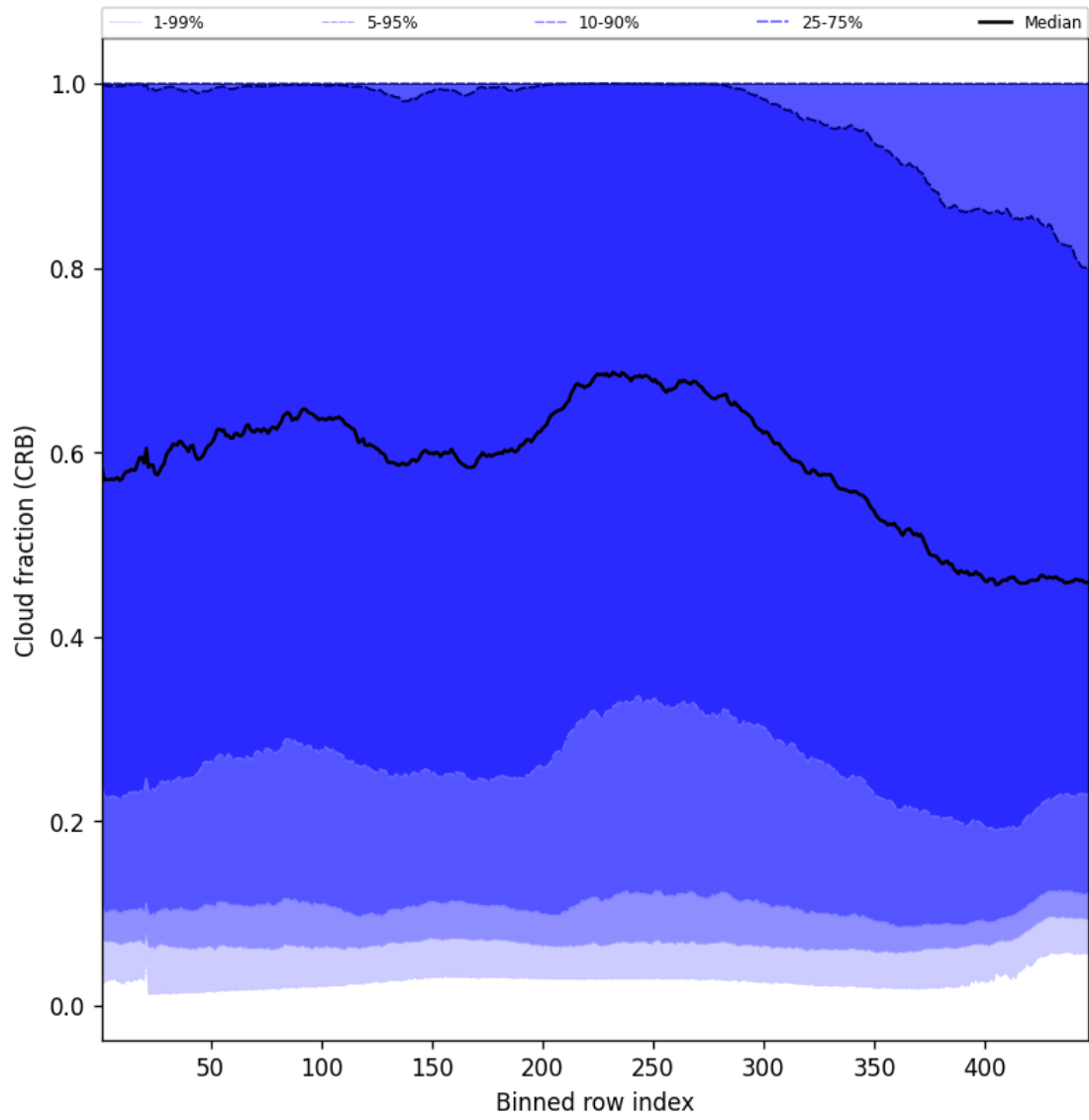
Figure 56: Along track statistics of “Cloud fraction (CRB)” for 2025-08-18 to 2025-08-19
