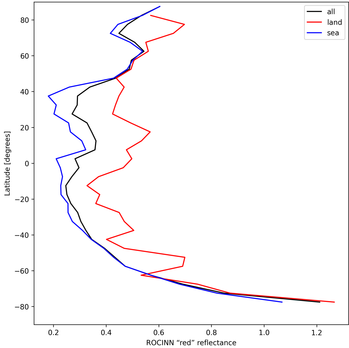
Figure 35: Zonal average of “ROCINN “red” reflectance” for 2025-08-18 to 2025-08-19.
