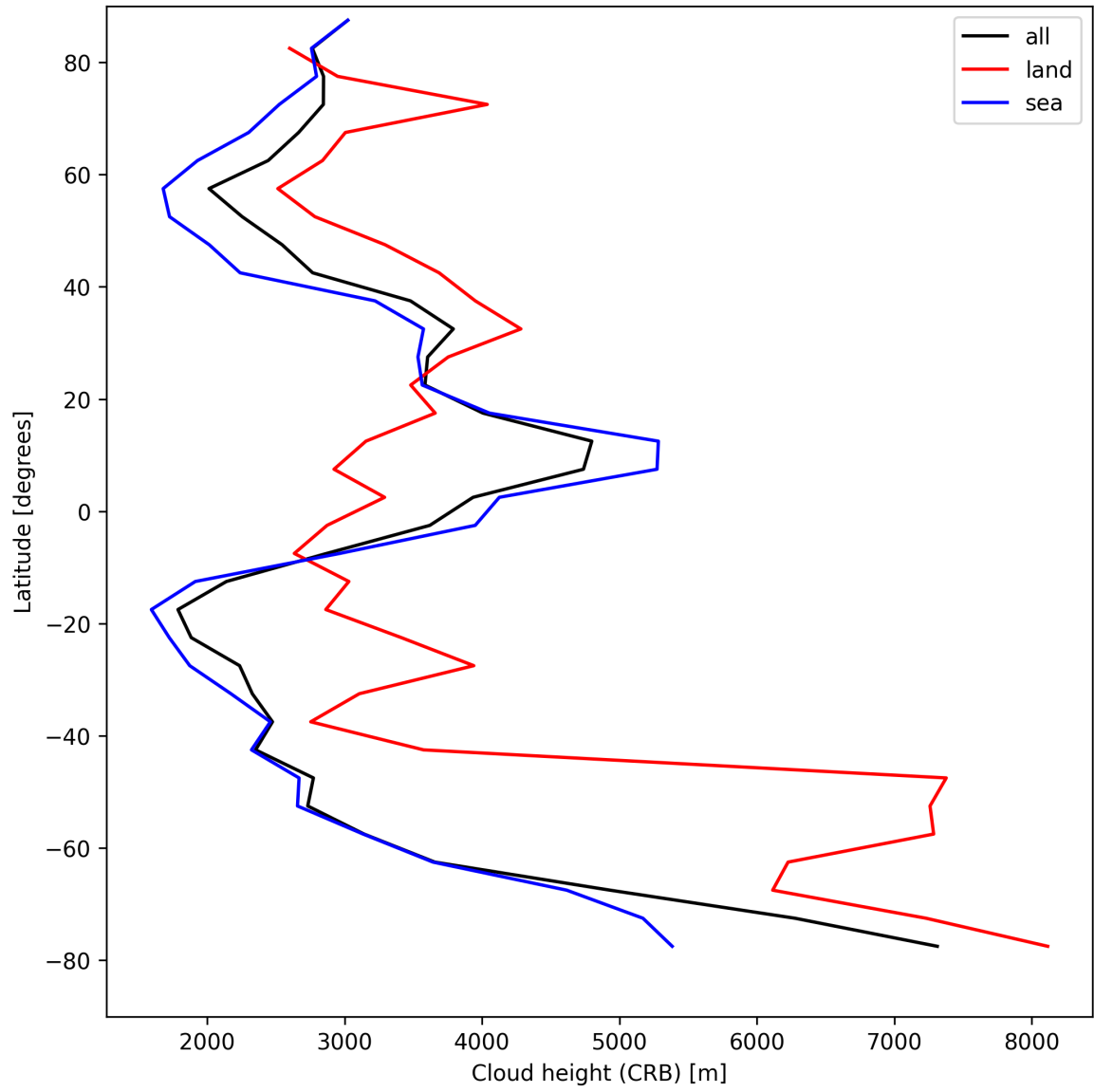
Figure 25: Zonal average of “Cloud height (CRB)” for 2025-08-18 to 2025-08-19.
