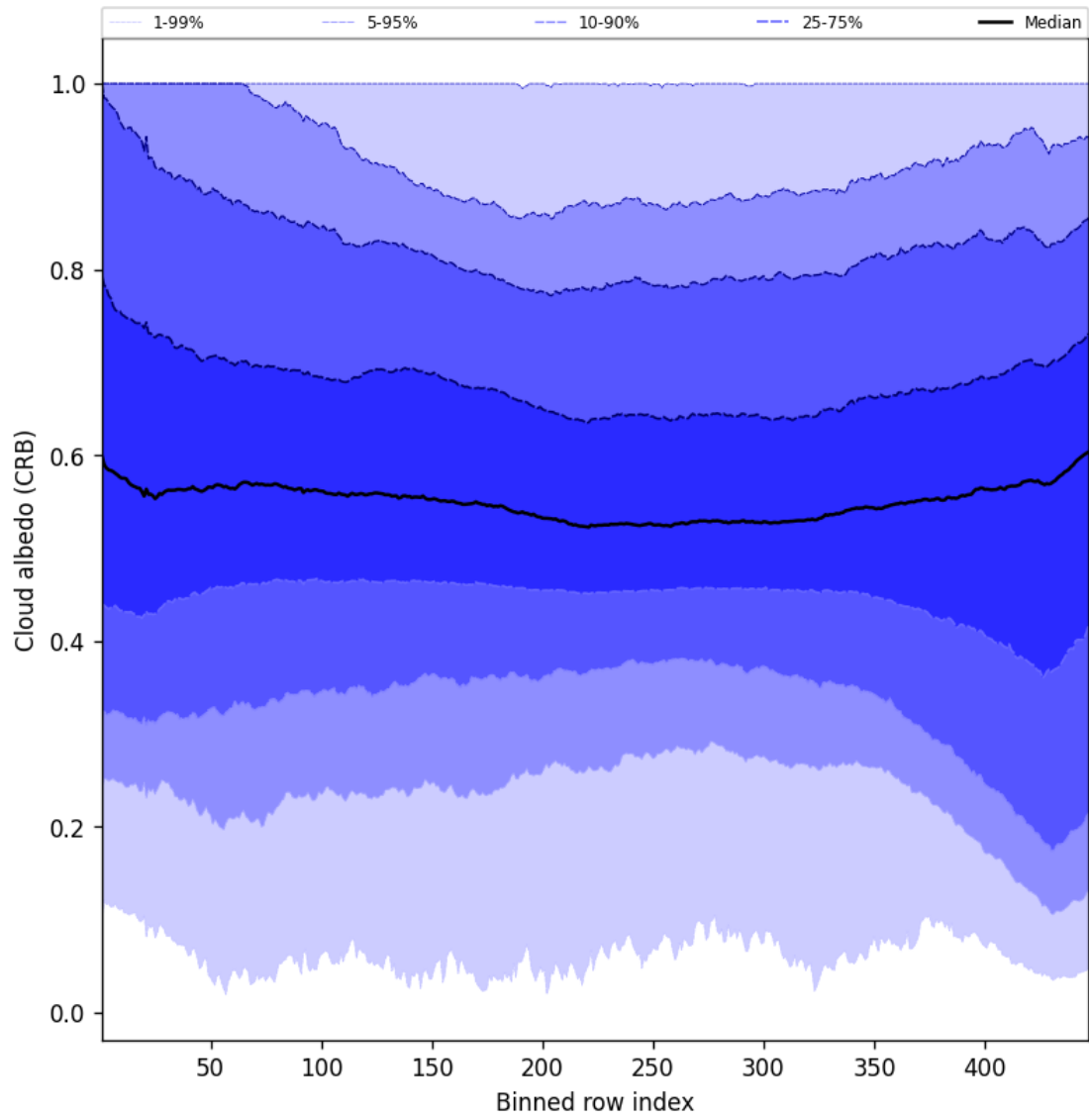
Figure 58: Along track statistics of “Cloud albedo (CRB)” for 2025-08-18 to 2025-08-19
