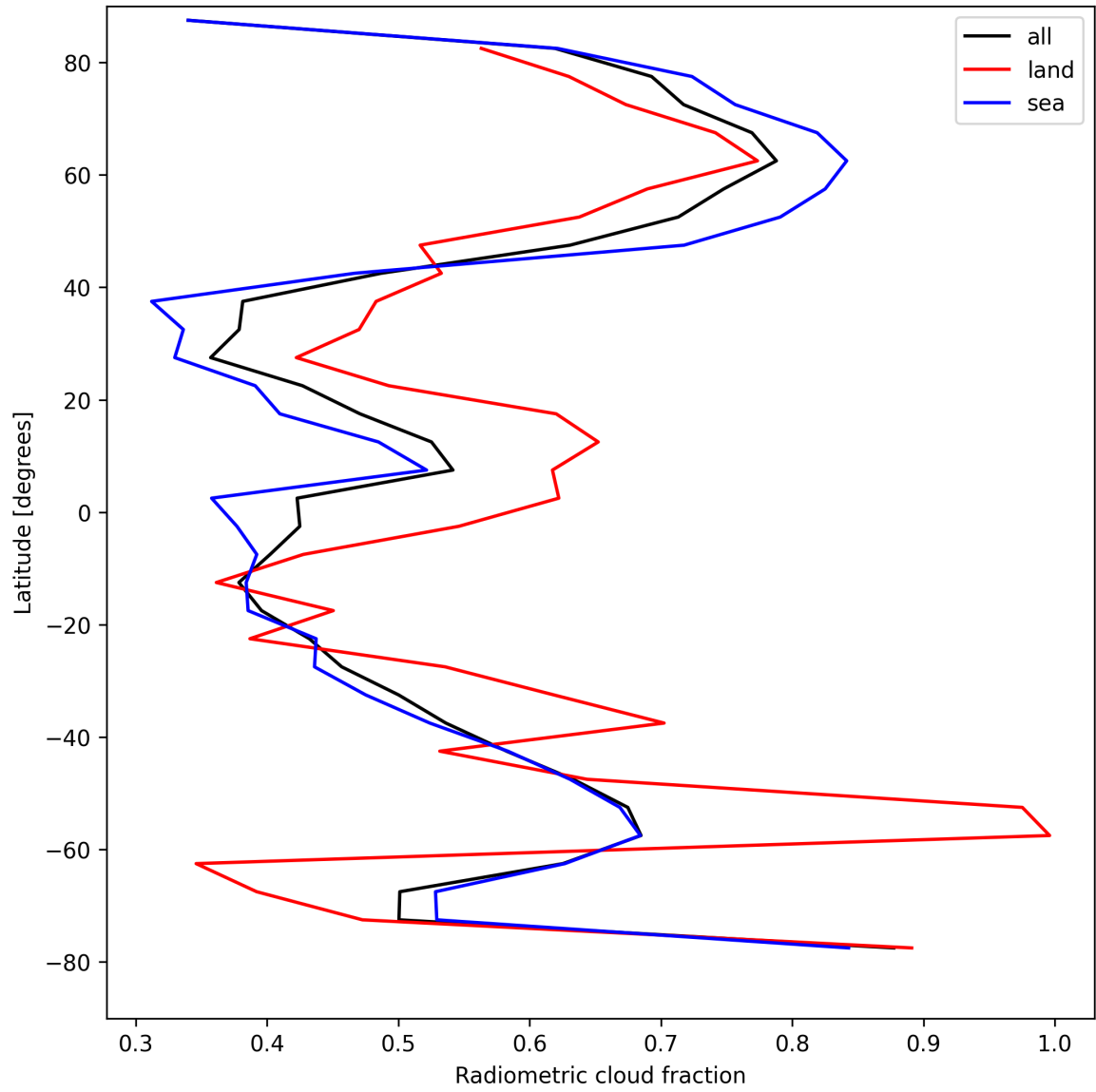
Figure 21: Zonal average of “Radiometric cloud fraction” for 2025-08-18 to 2025-08-19.
