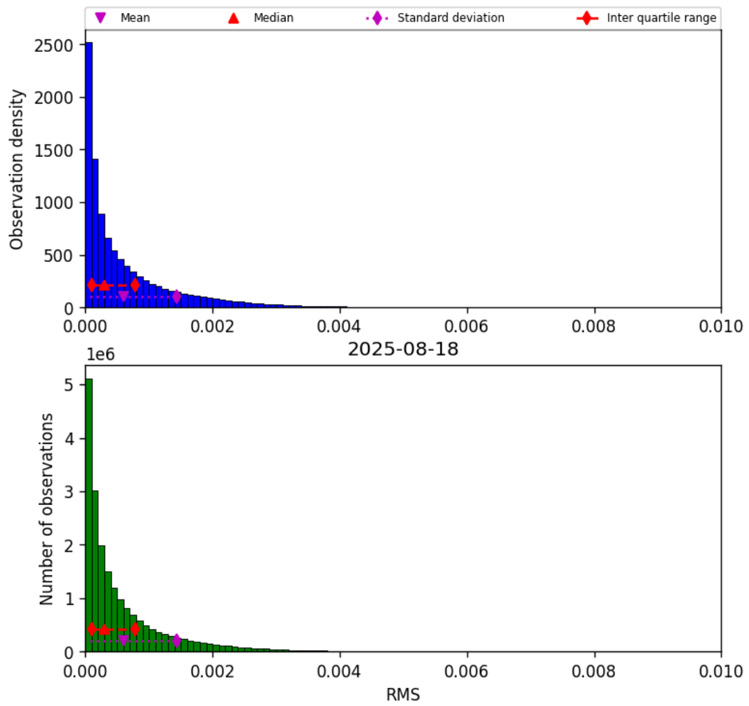
Figure 45: Histogram of “RMS” for 2025-08-18 to 2025-08-19
