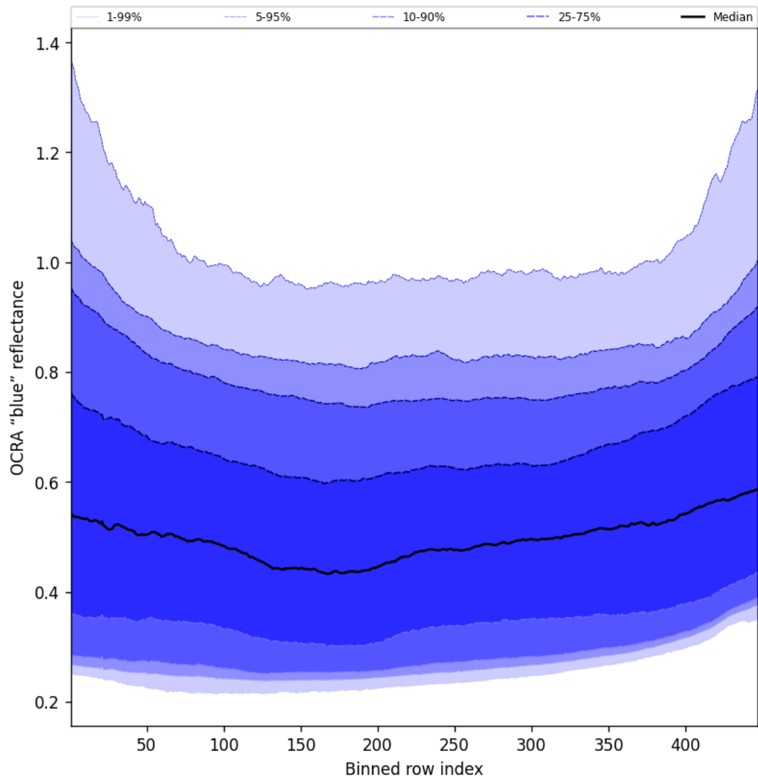
Figure 65: Along track statistics of “OCRA “blue” reflectance” for 2025-08-18 to 2025-08-19
