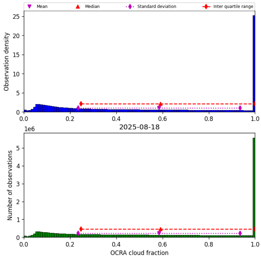
Figure 48: Histogram of “OCRA cloud fraction” for 2025-08-18 to 2025-08-19
