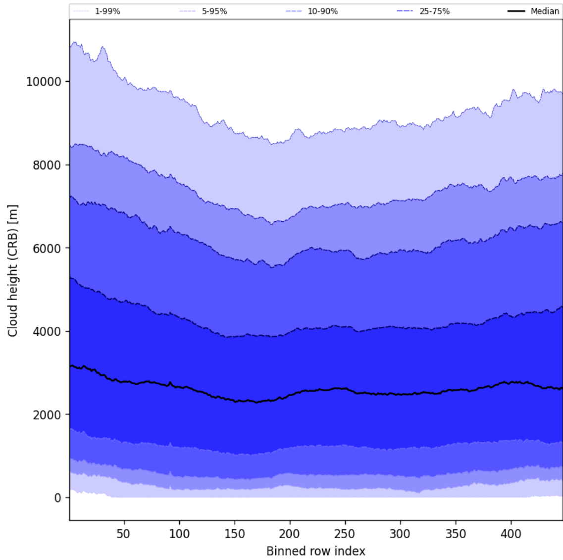
Figure 57: Along track statistics of “Cloud height (CRB)” for 2025-08-18 to 2025-08-19
