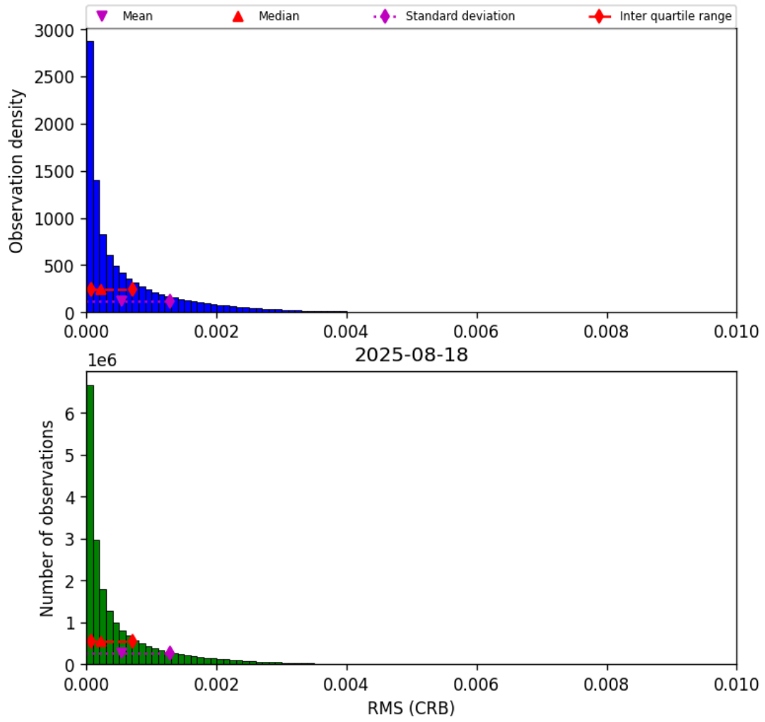
Figure 46: Histogram of “RMS (CRB)” for 2025-08-18 to 2025-08-19
