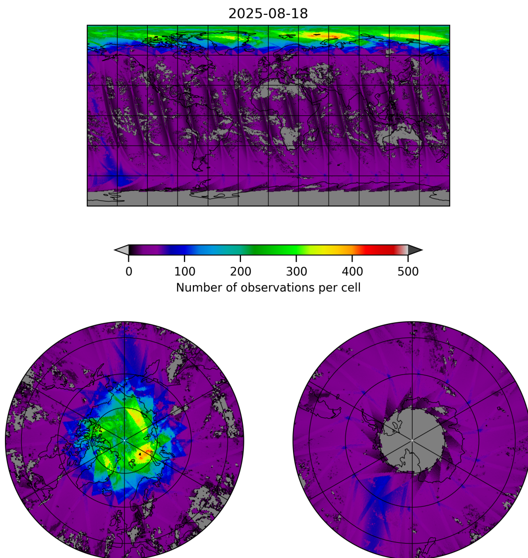
Figure 19: Map of the number of observations for 2025-08-18 to 2025-08-19
