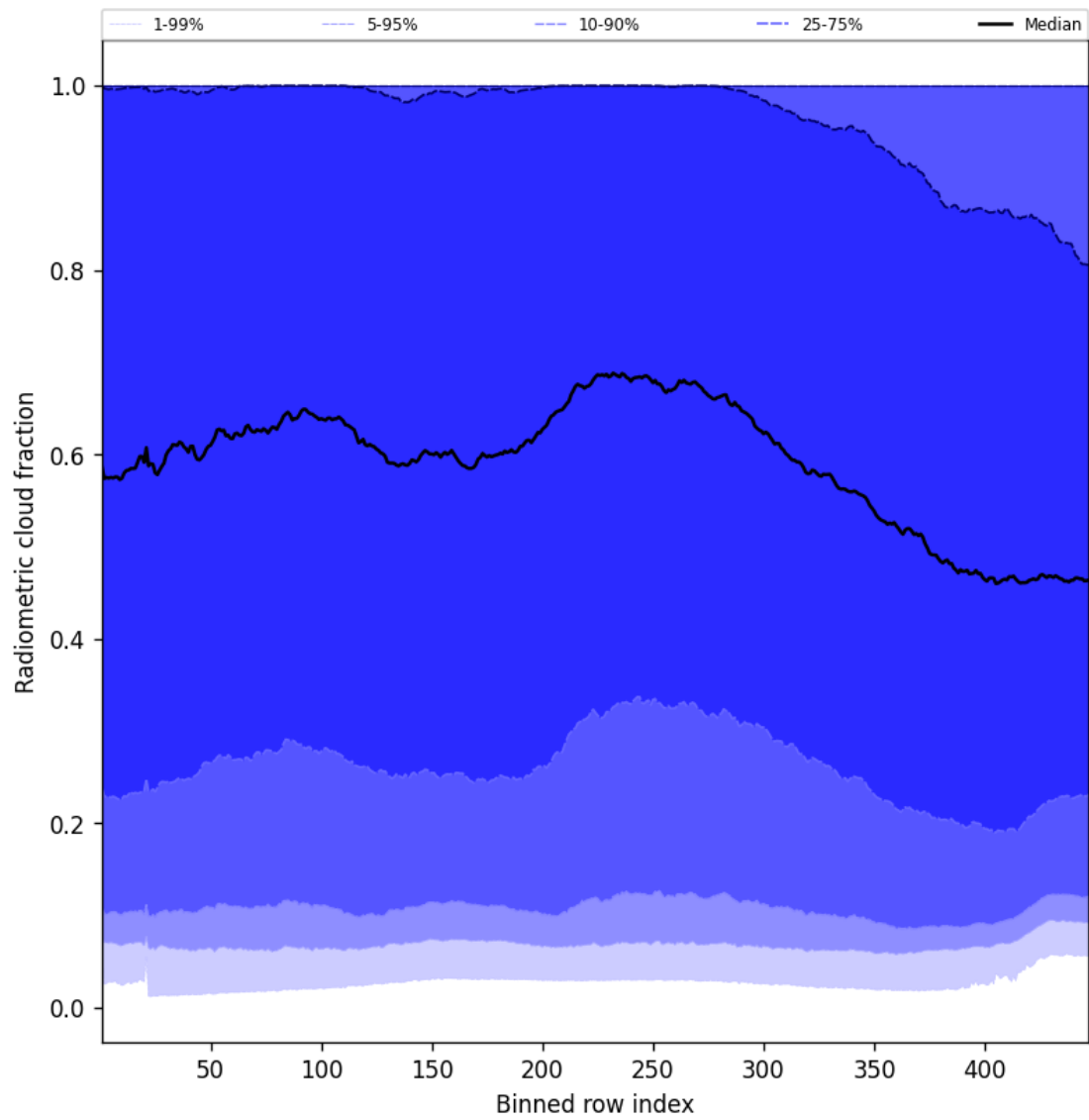
Figure 53: Along track statistics of “Radiometric cloud fraction” for 2025-08-18 to 2025-08-19
