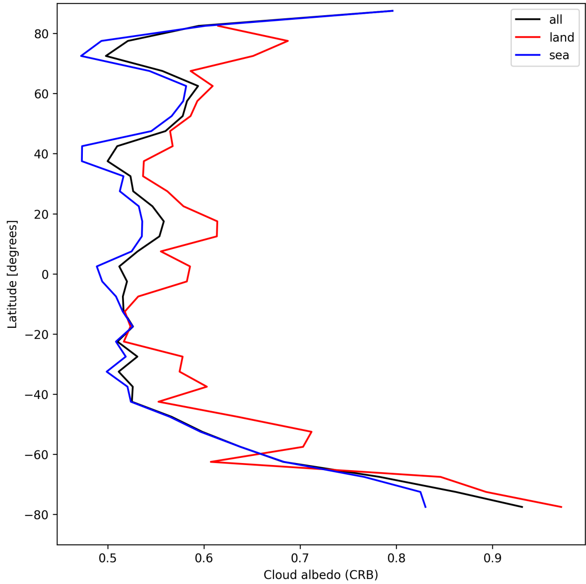
Figure 26: Zonal average of “Cloud albedo (CRB)” for 2025-08-18 to 2025-08-19.
