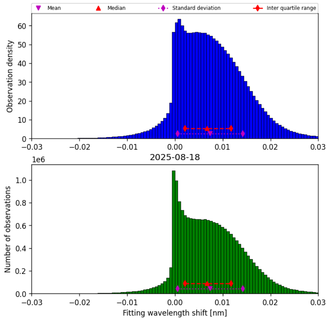
Figure 47: Histogram of “Fitting wavelength shift” for 2025-08-18 to 2025-08-19
