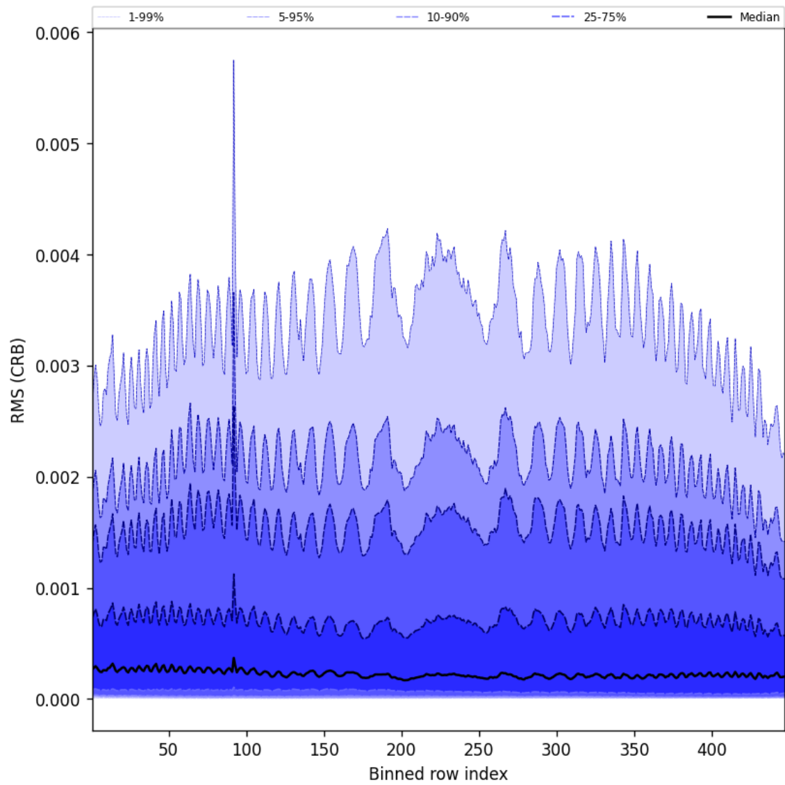
Figure 62: Along track statistics of “RMS (CRB)” for 2025-08-18 to 2025-08-19
