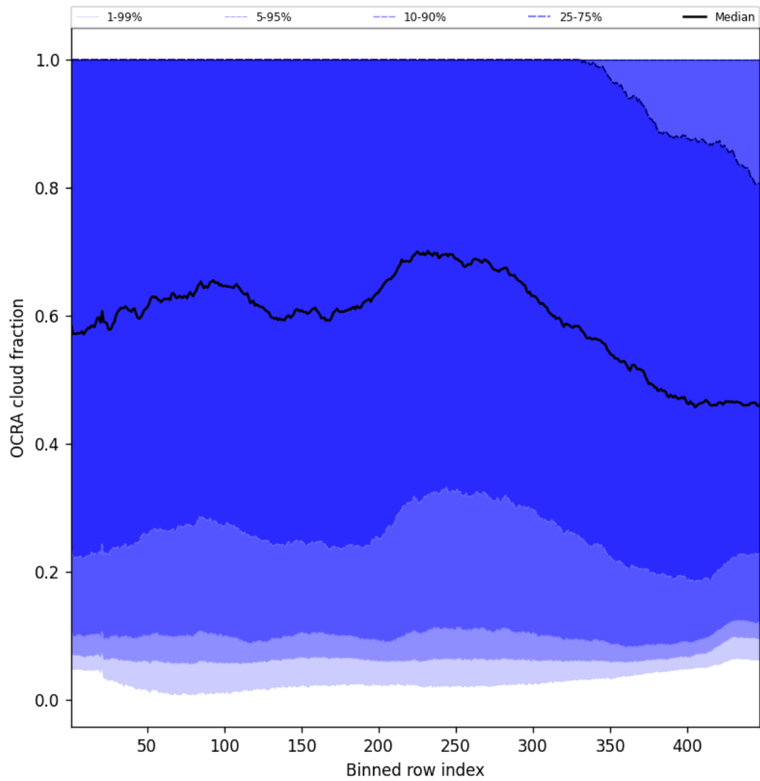
Figure 64: Along track statistics of “OCRA cloud fraction” for 2025-08-18 to 2025-08-19
