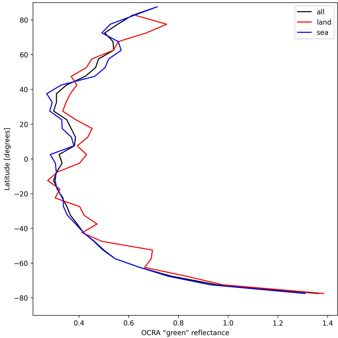
Figure 34: Zonal average of “OCRA “green” reflectance” for 2025-08-18 to 2025-08-19.
