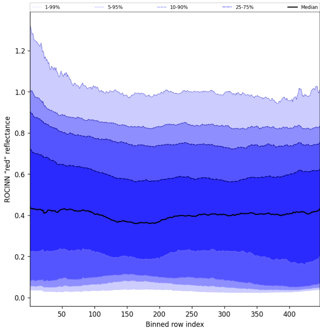
Figure 67: Along track statistics of “ROCINN “red” reflectance” for 2025-08-18 to 2025-08-19
