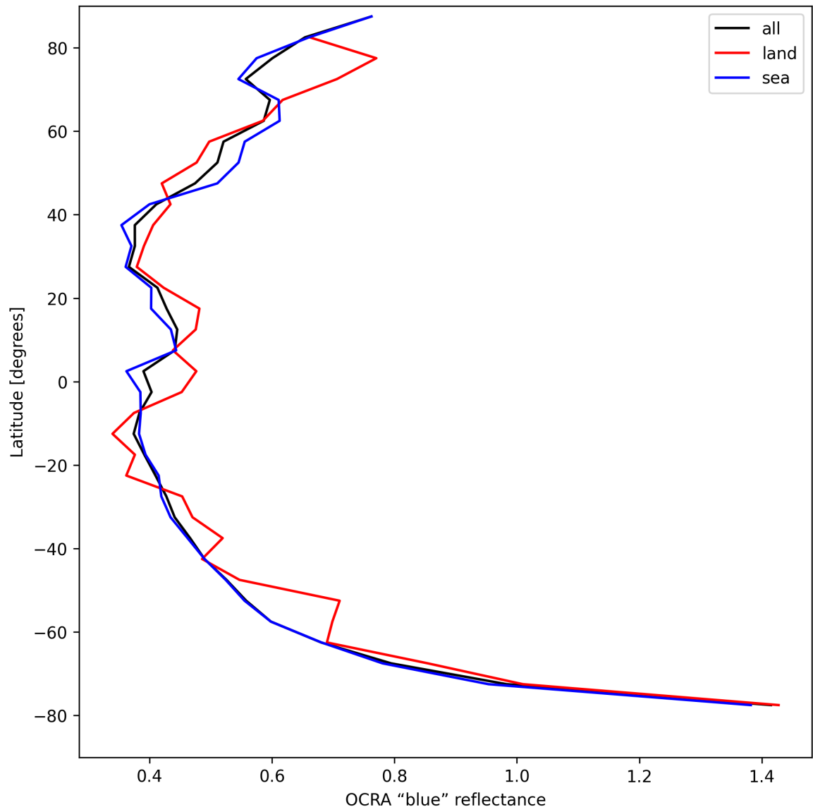
Figure 33: Zonal average of “OCRA “blue” reflectance” for 2025-08-18 to 2025-08-19.
