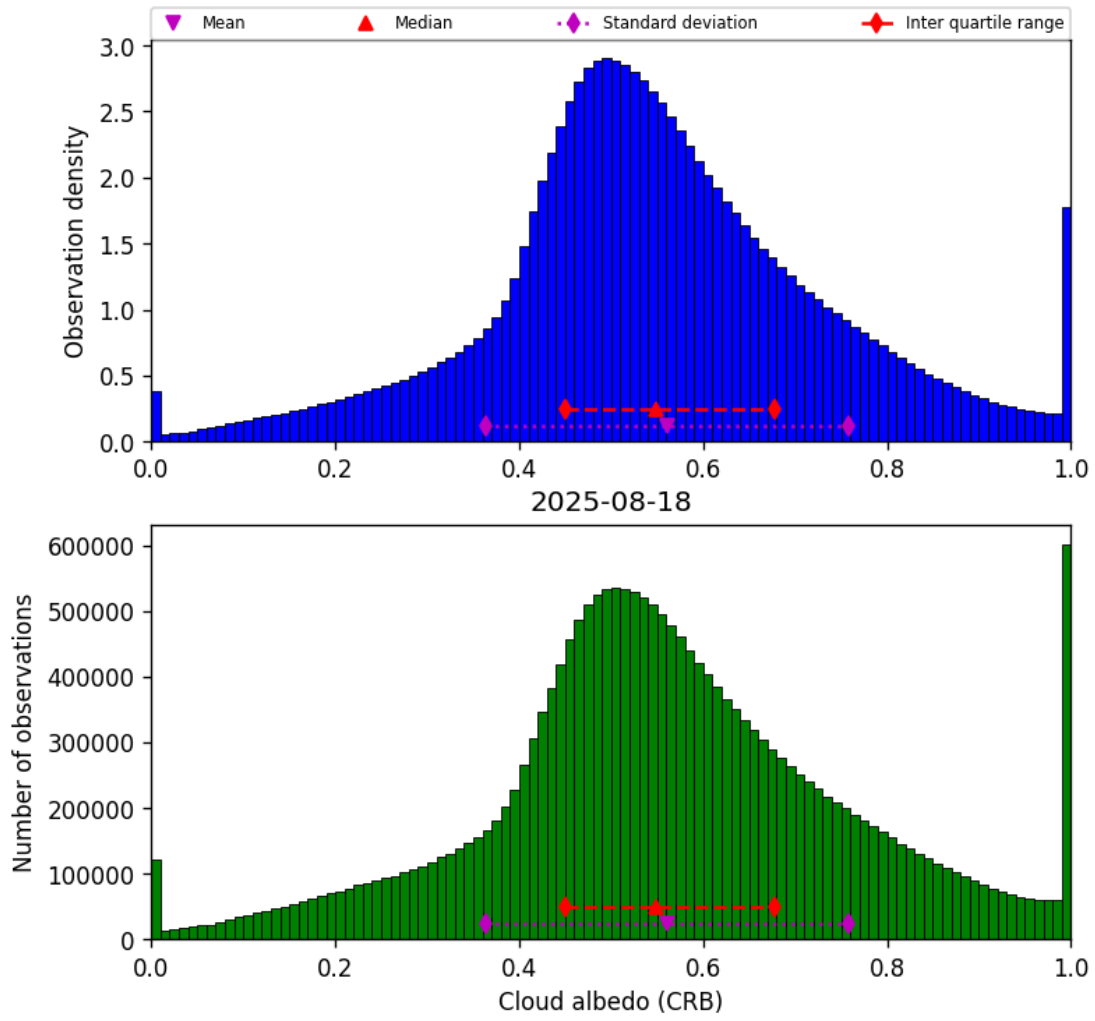
Figure 42: Histogram of “Cloud albedo (CRB)” for 2025-08-18 to 2025-08-19
