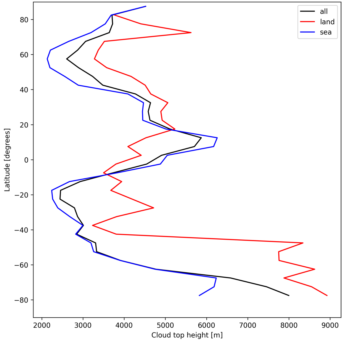
Figure 22: Zonal average of “Cloud top height” for 2025-08-18 to 2025-08-19.
