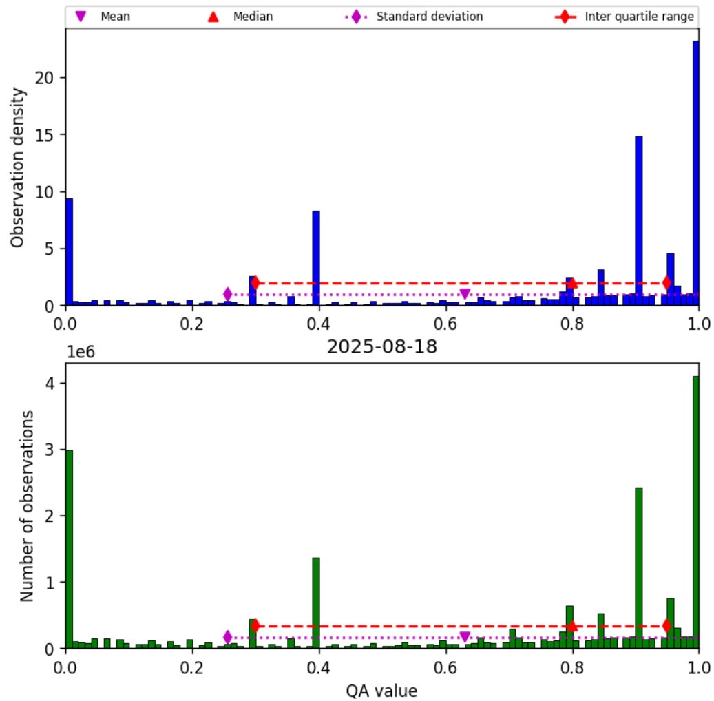
Figure 36: Histogram of “QA value” for 2025-08-18 to 2025-08-19
