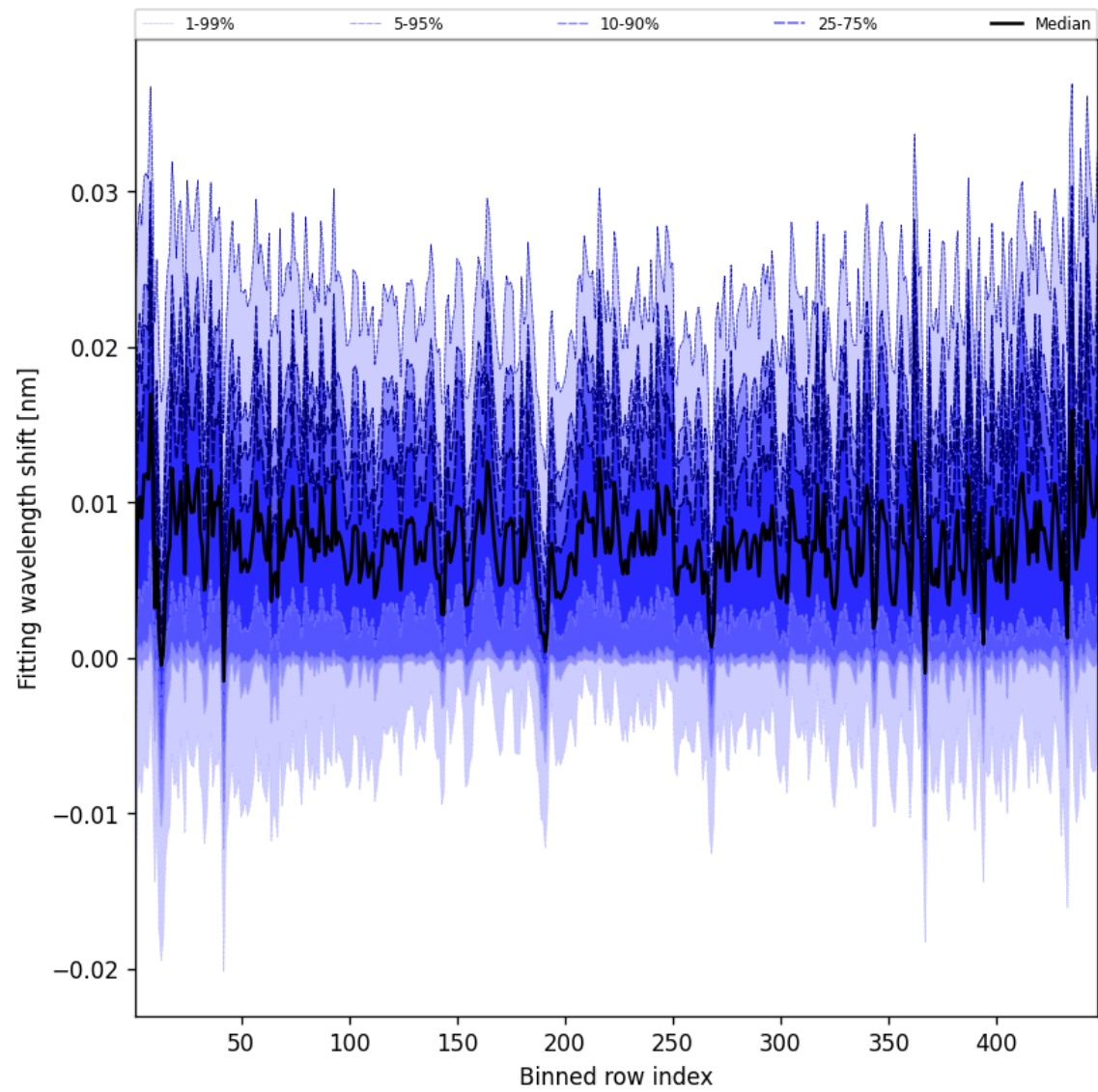
Figure 63: Along track statistics of “Fitting wavelength shift” for 2025-08-18 to 2025-08-19
