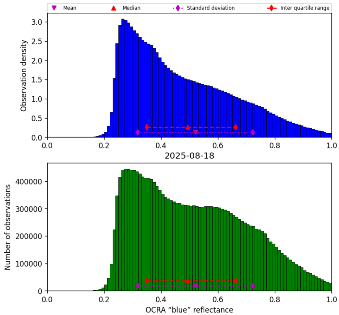
Figure 49: Histogram of “OCRA “blue” reflectance” for 2025-08-18 to 2025-08-19
