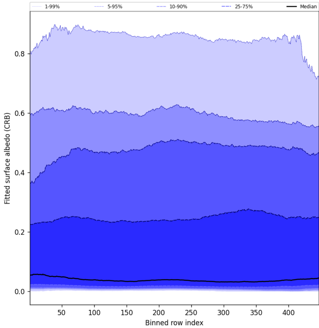
Figure 60: Along track statistics of “Fitted surface albedo (CRB)” for 2025-08-18 to 2025-08-19
