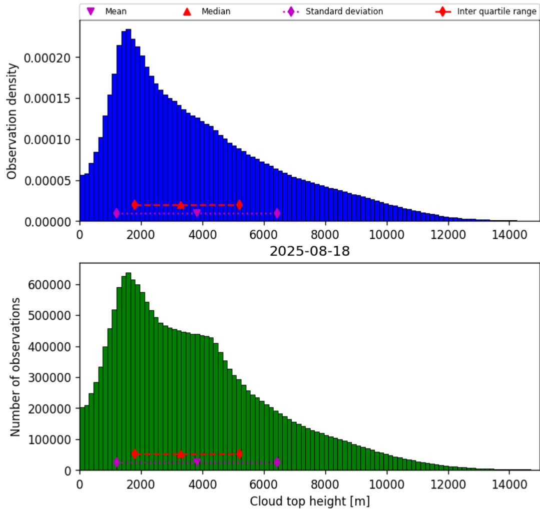
Figure 38: Histogram of “Cloud top height” for 2025-08-18 to 2025-08-19
