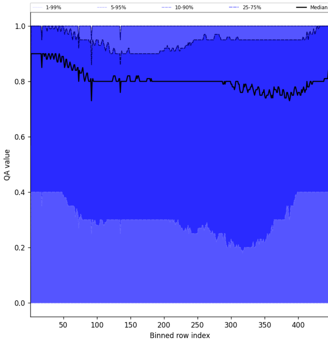
Figure 52: Along track statistics of “QA value” for 2025-08-18 to 2025-08-19
