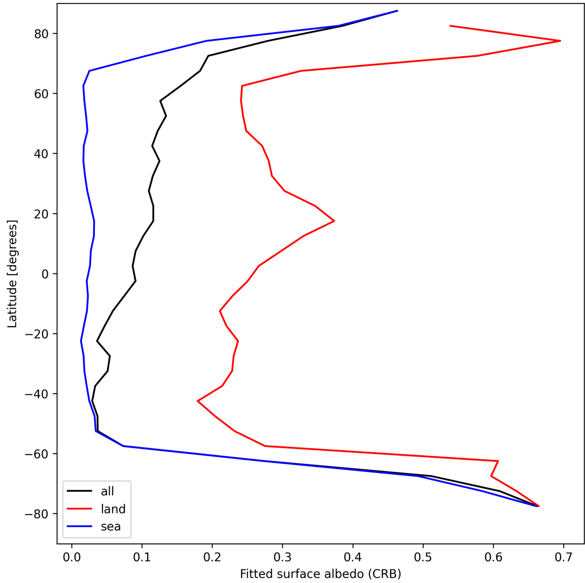
Figure 28: Zonal average of “Fitted surface albedo (CRB)” for 2025-08-18 to 2025-08-19.
