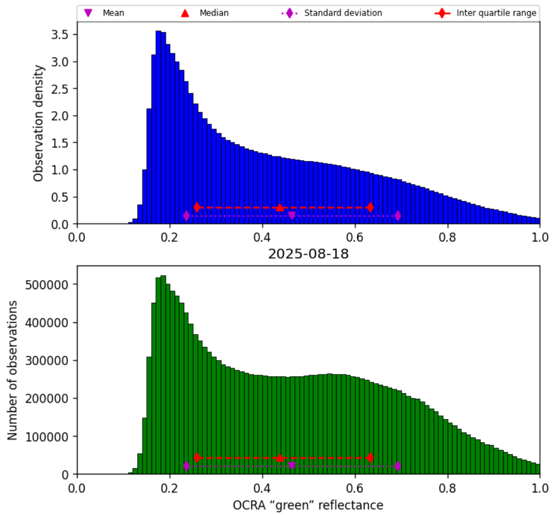
Figure 50: Histogram of “OCRA “green” reflectance” for 2025-08-18 to 2025-08-19
