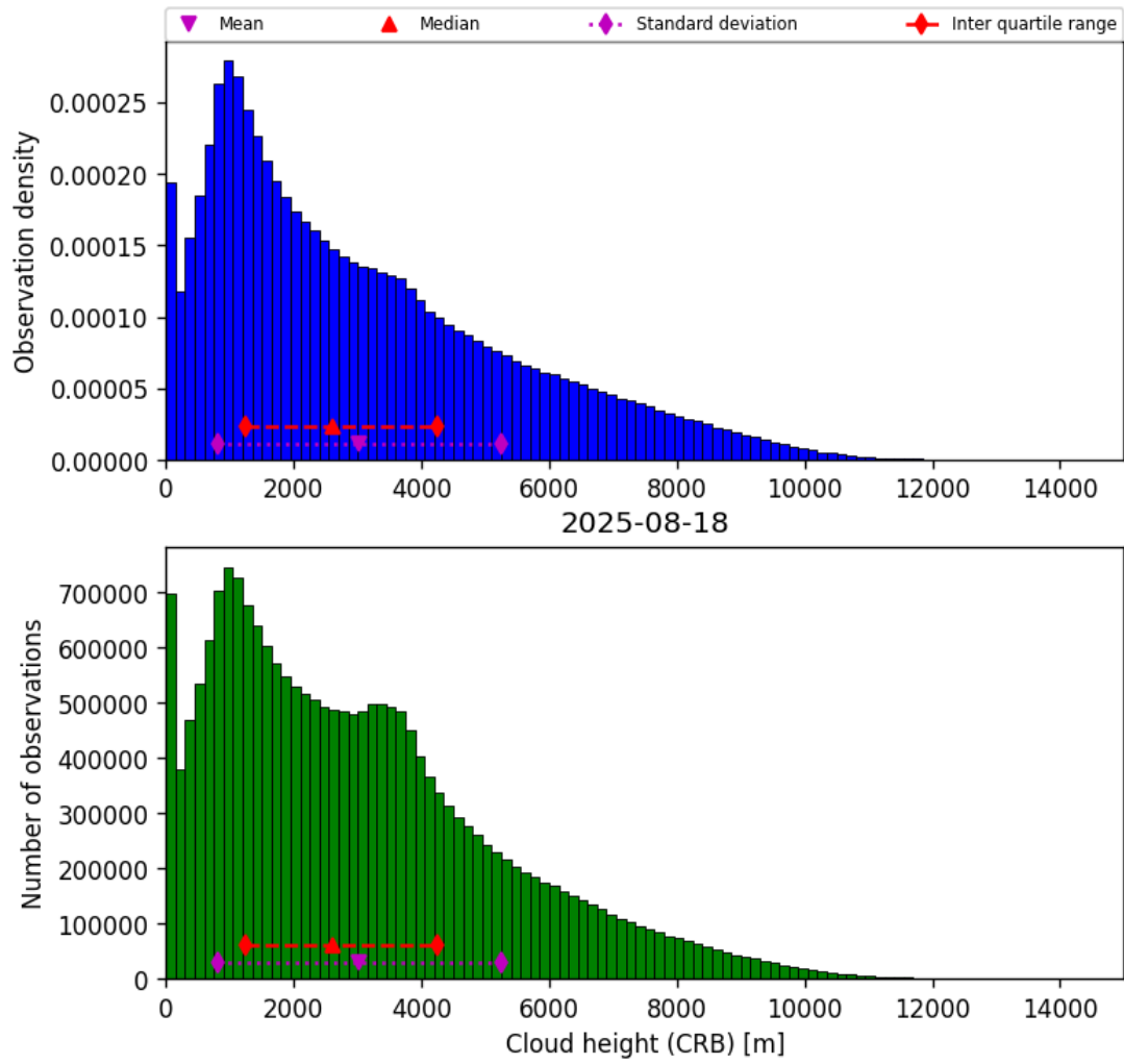
Figure 41: Histogram of “Cloud height (CRB)” for 2025-08-18 to 2025-08-19
