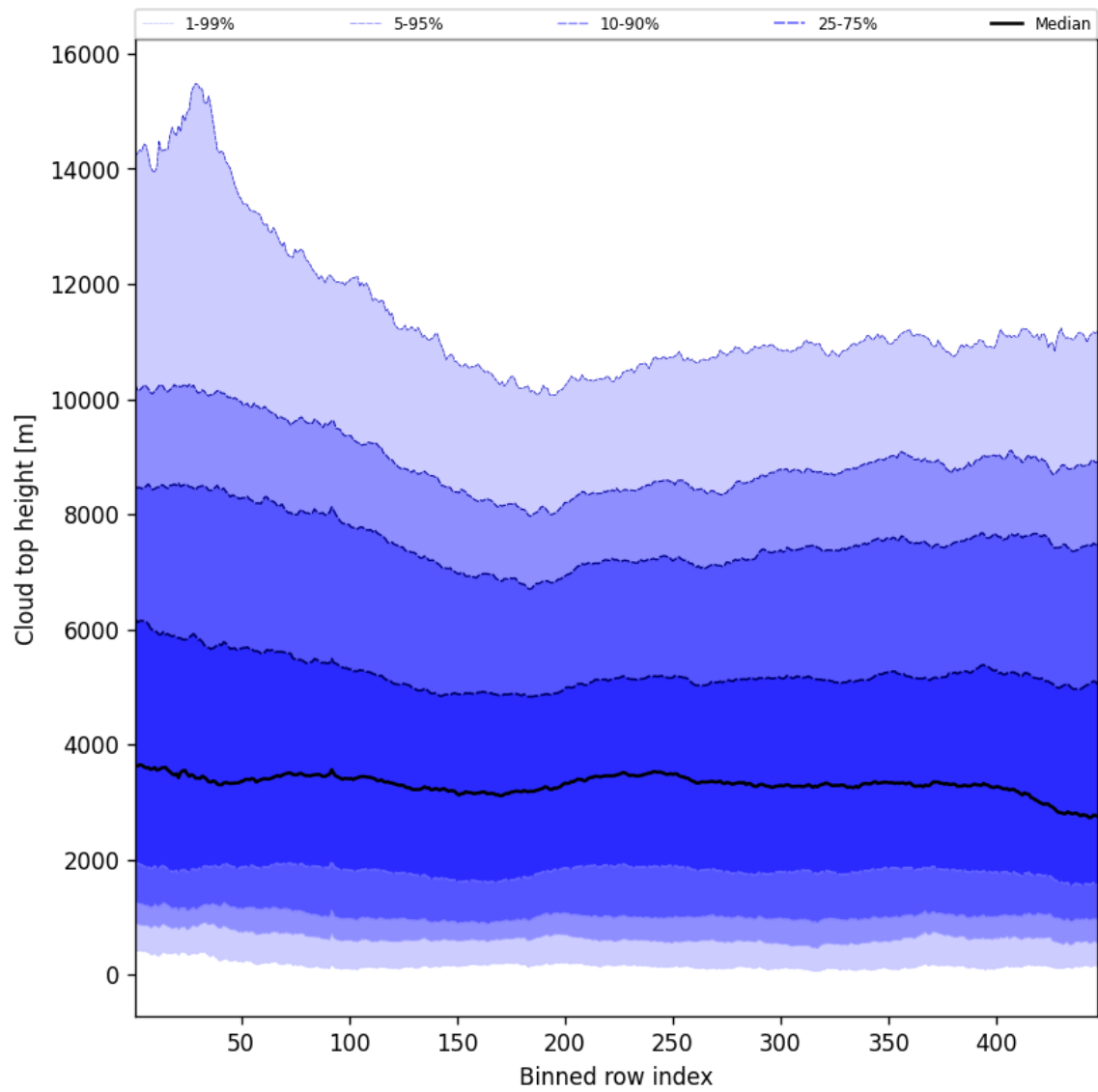
Figure 54: Along track statistics of “Cloud top height” for 2025-08-18 to 2025-08-19
