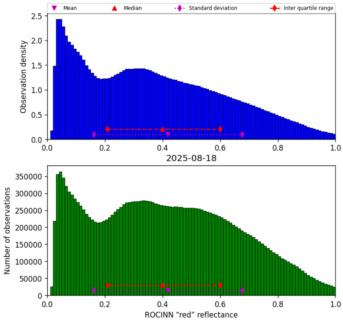
Figure 51: Histogram of "ROCINN "red" reflectance" for 2025-08-18 to 2025-08-19
