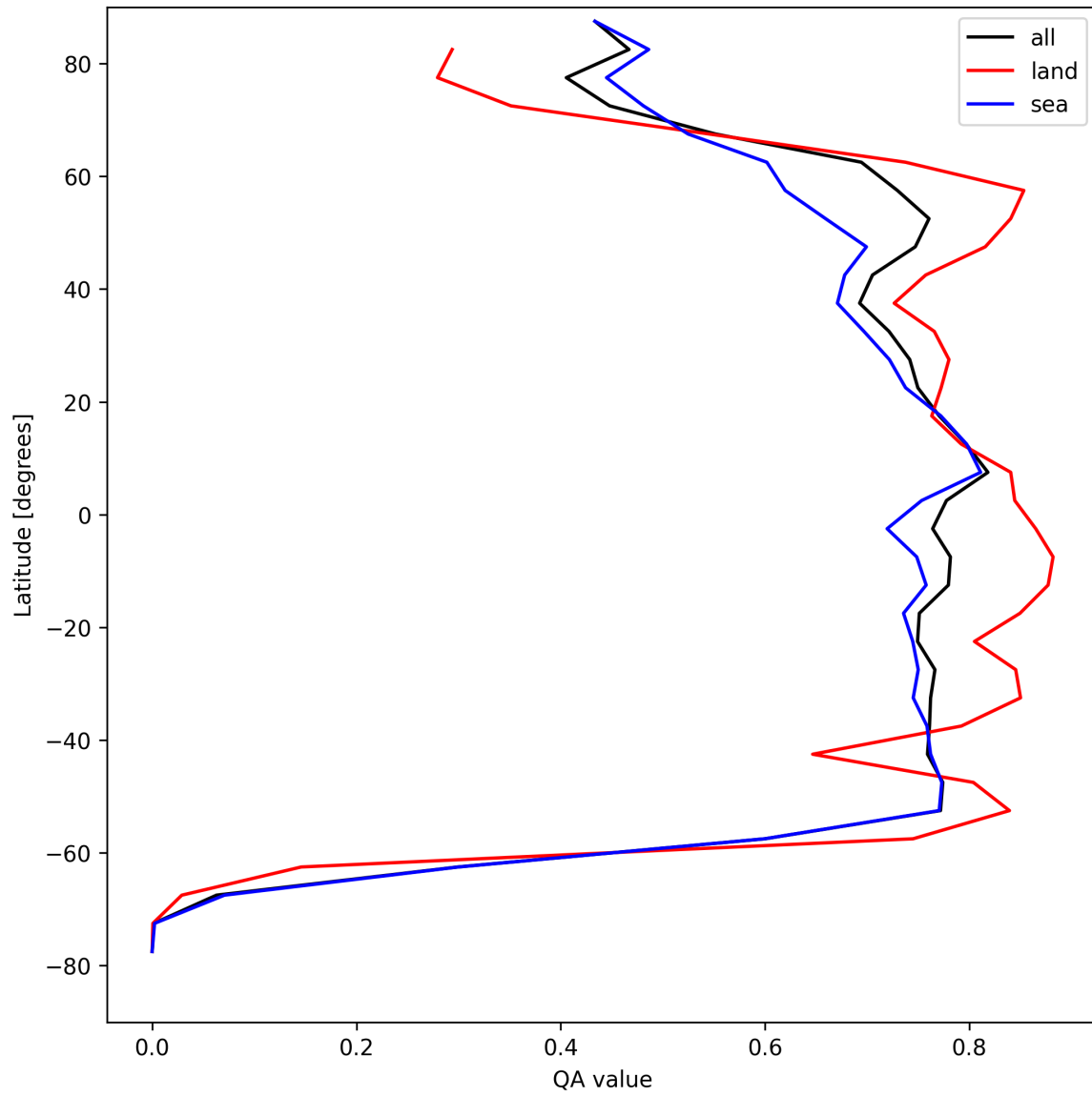
Figure 20: Zonal average of “QA value” for 2025-08-18 to 2025-08-19.
