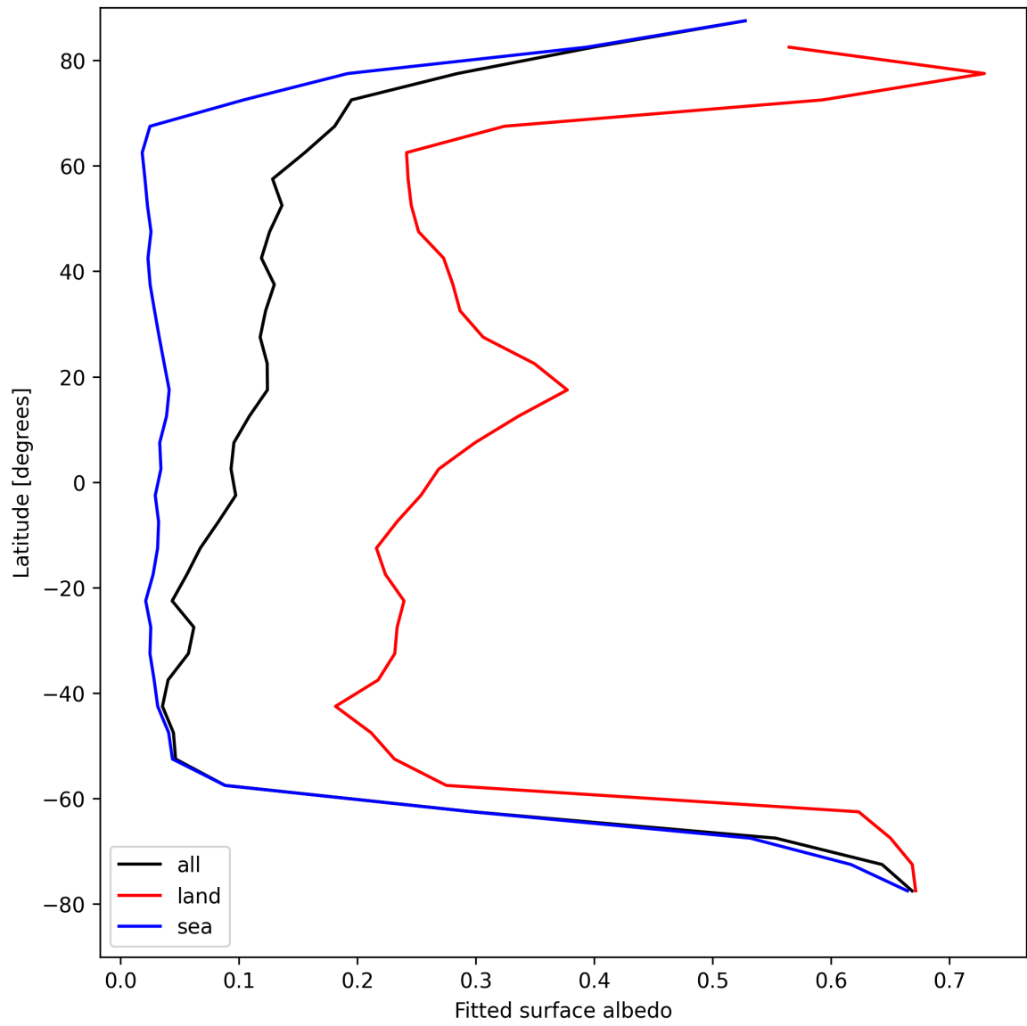
Figure 27: Zonal average of “Fitted surface albedo” for 2025-08-18 to 2025-08-19.
