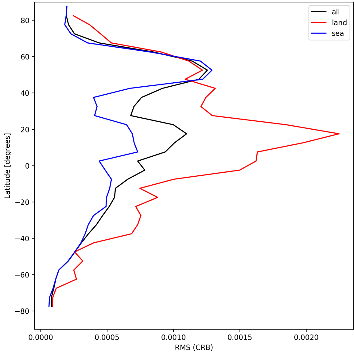
Figure 30: Zonal average of “RMS (CRB)” for 2025-08-18 to 2025-08-19.
