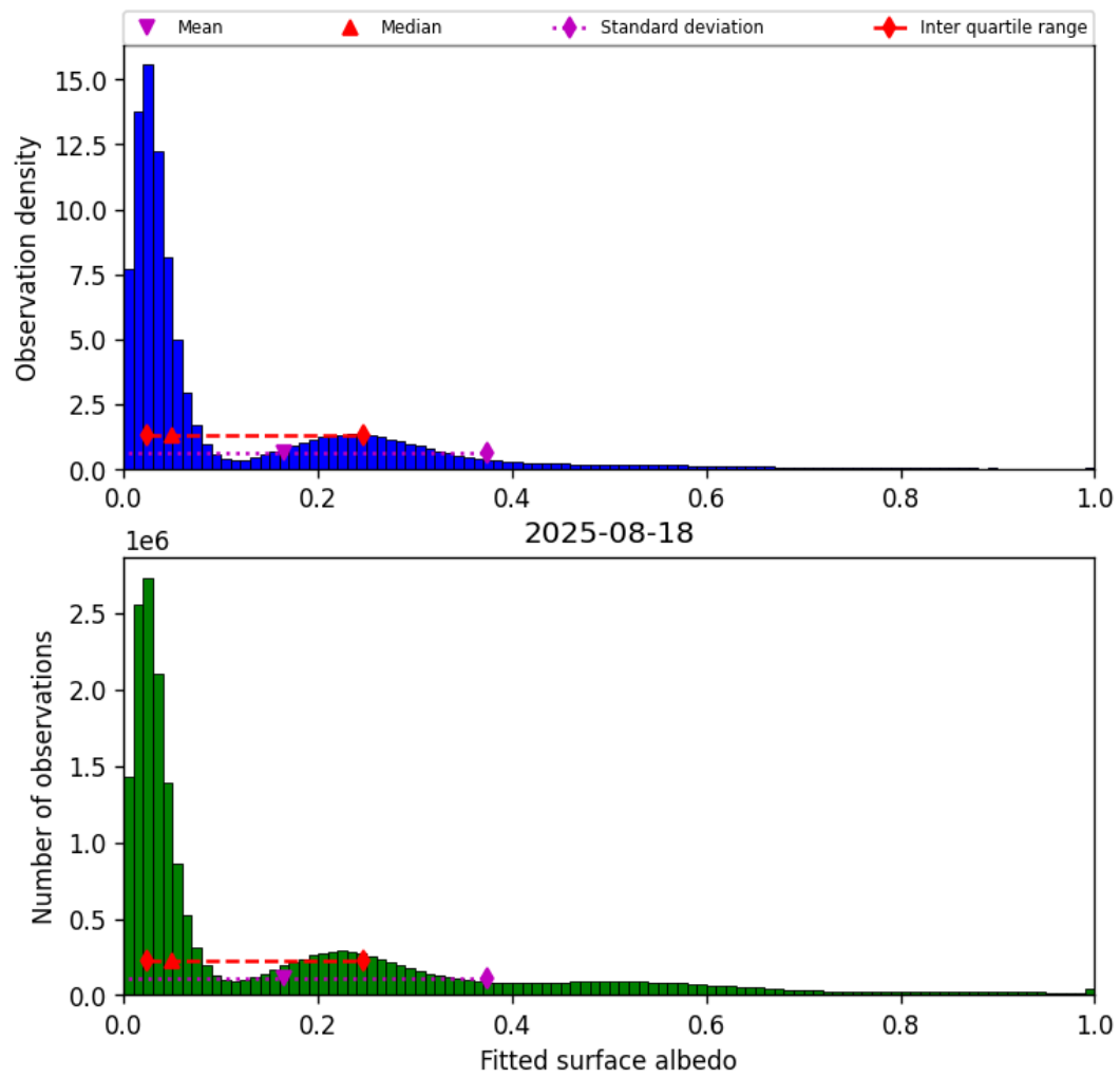
Figure 43: Histogram of “Fitted surface albedo” for 2025-08-18 to 2025-08-19
