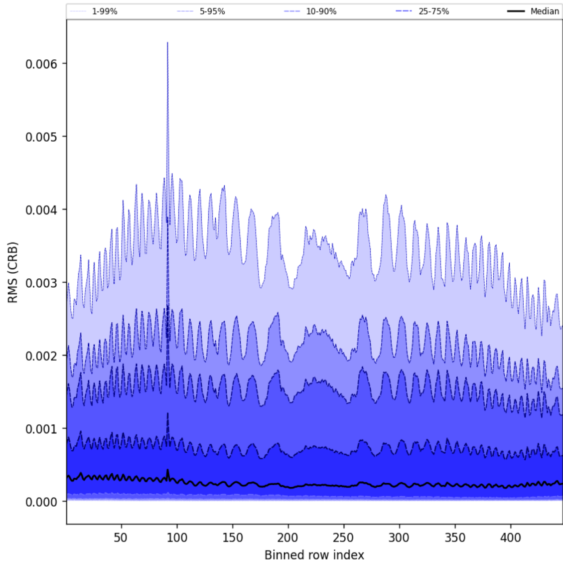
Figure 62: Along track statistics of “RMS (CRB)” for 2025-08-20 to 2025-08-21
