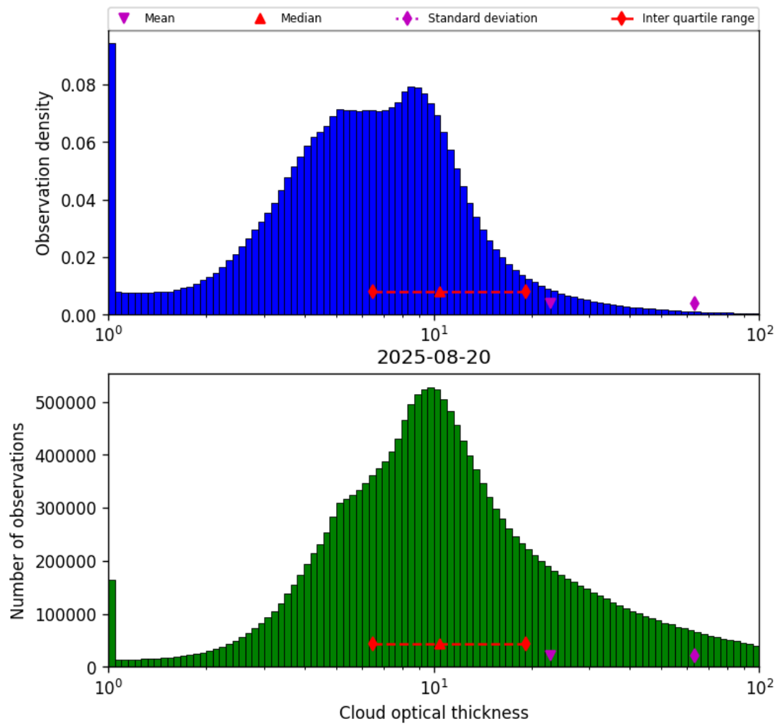
Figure 39: Histogram of “Cloud optical thickness” for 2025-08-20 to 2025-08-21
