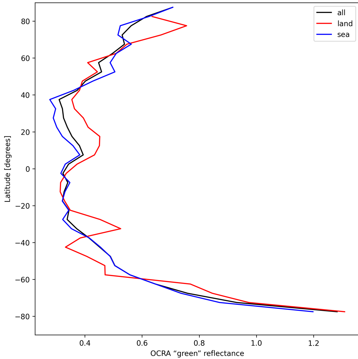
Figure 34: Zonal average of “OCRA “green” reflectance” for 2025-08-20 to 2025-08-21.
