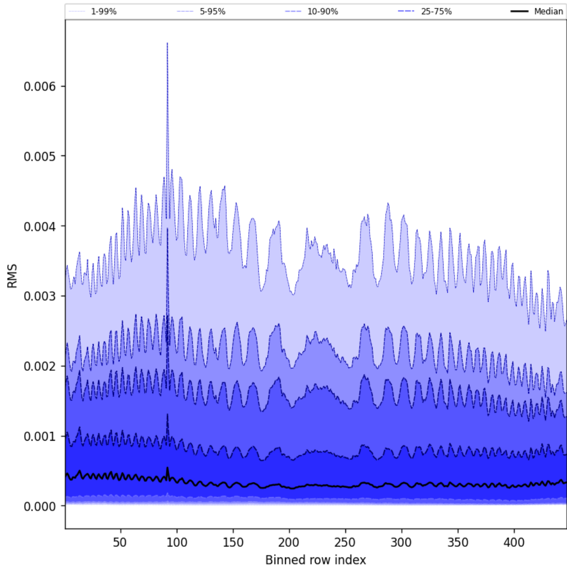
Figure 61: Along track statistics of “RMS” for 2025-08-20 to 2025-08-21
