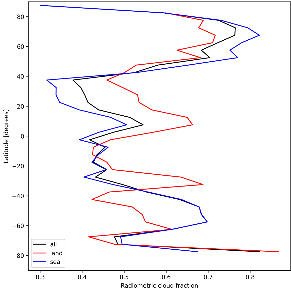
Figure 21: Zonal average of “Radiometric cloud fraction” for 2025-08-20 to 2025-08-21.
