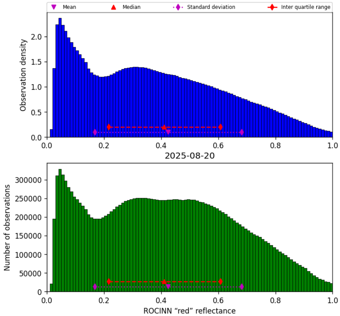
Figure 51: Histogram of “ROCINN “red” reflectance” for 2025-08-20 to 2025-08-21
