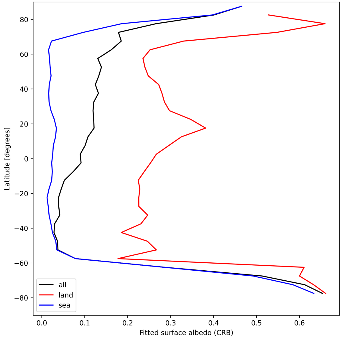
Figure 28: Zonal average of “Fitted surface albedo (CRB)” for 2025-08-20 to 2025-08-21.
