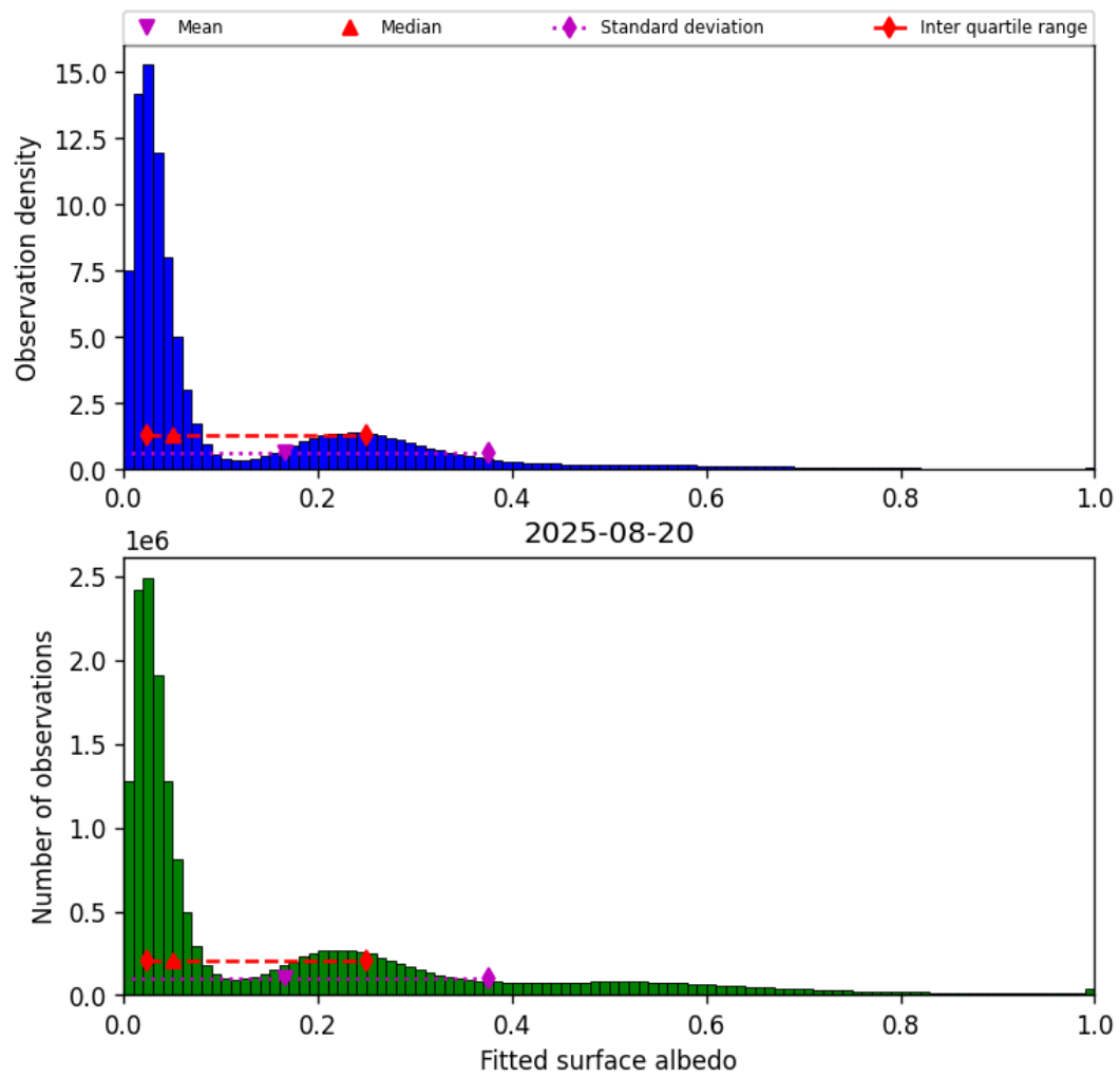
Figure 43: Histogram of “Fitted surface albedo” for 2025-08-20 to 2025-08-21
