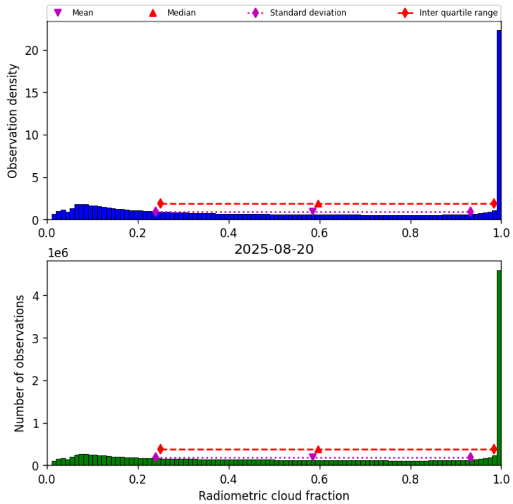
Figure 37: Histogram of “Radiometric cloud fraction” for 2025-08-20 to 2025-08-21
