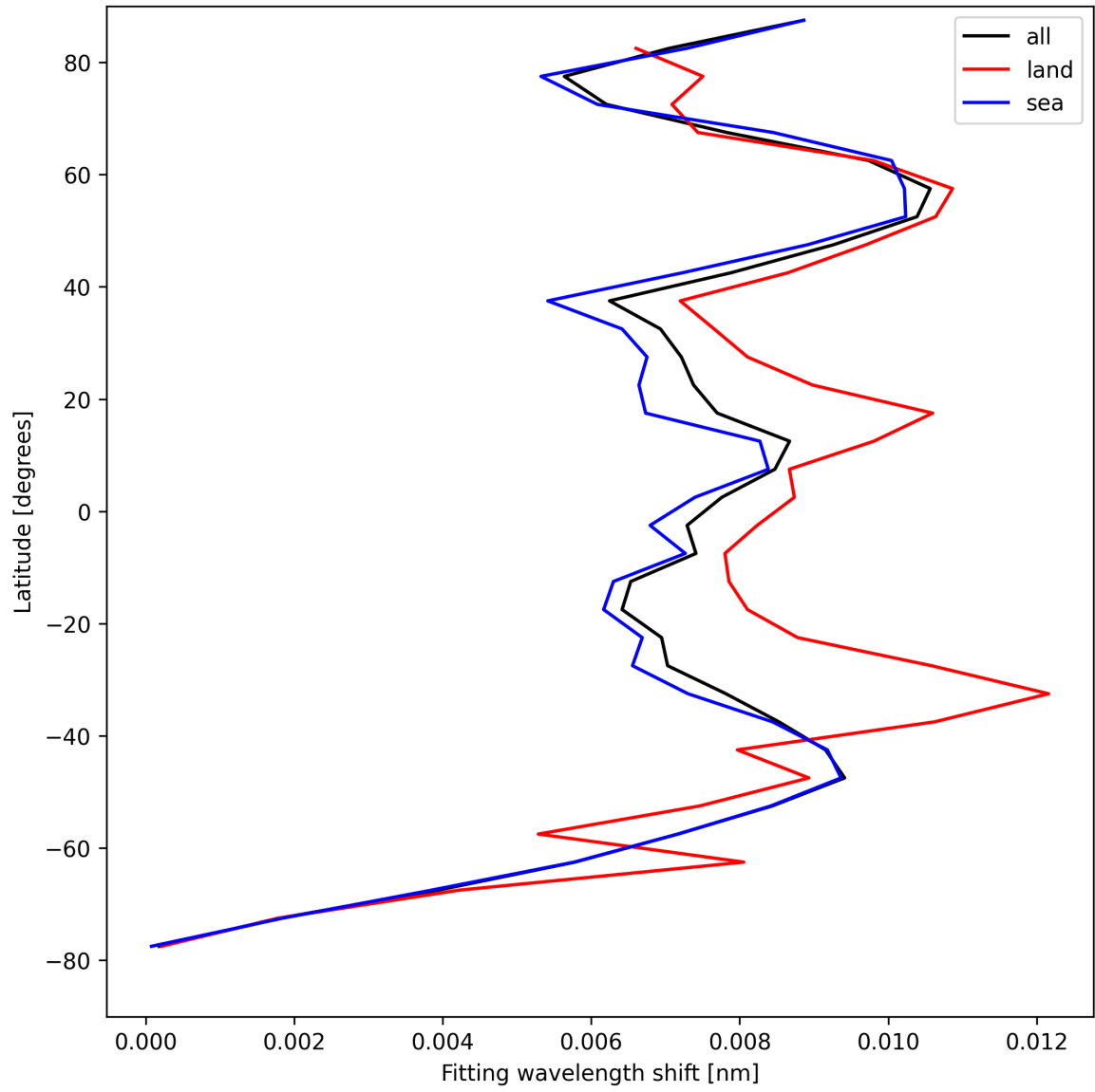
Figure 31: Zonal average of “Fitting wavelength shift” for 2025-08-20 to 2025-08-21.
