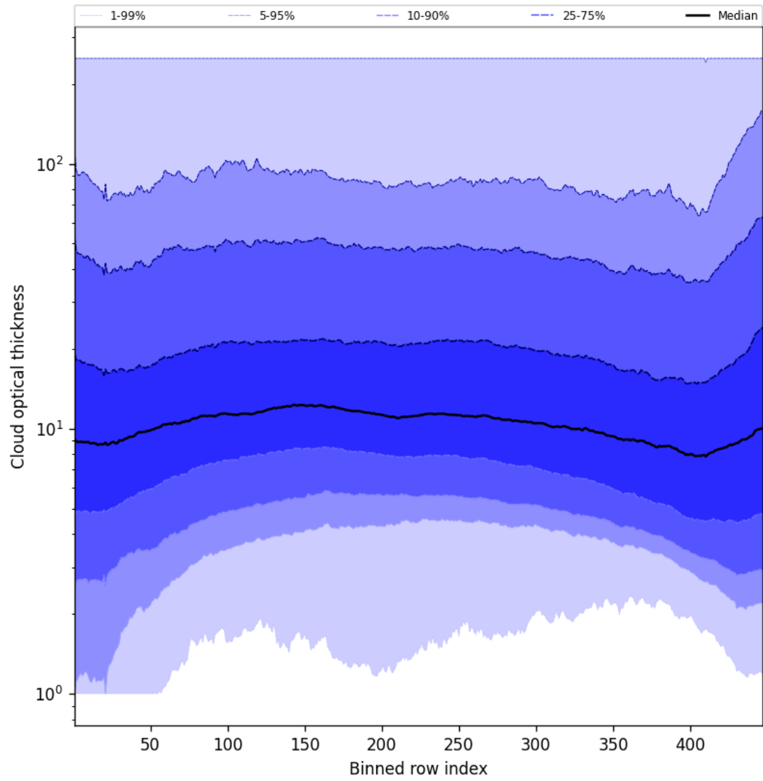
Figure 55: Along track statistics of “Cloud optical thickness” for 2025-08-20 to 2025-08-21
