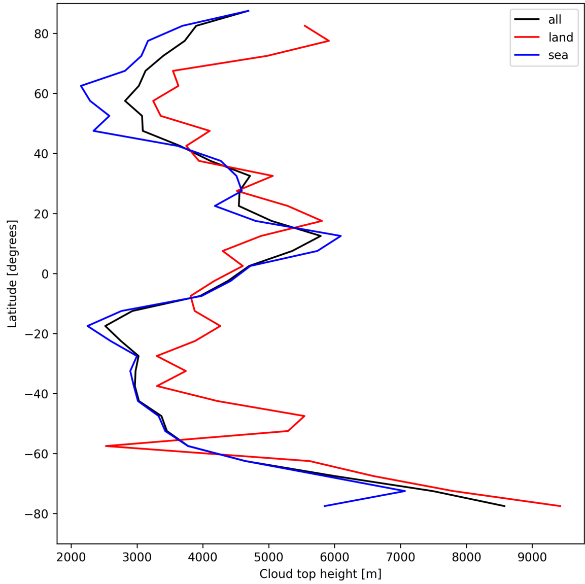
Figure 22: Zonal average of “Cloud top height” for 2025-08-20 to 2025-08-21.
