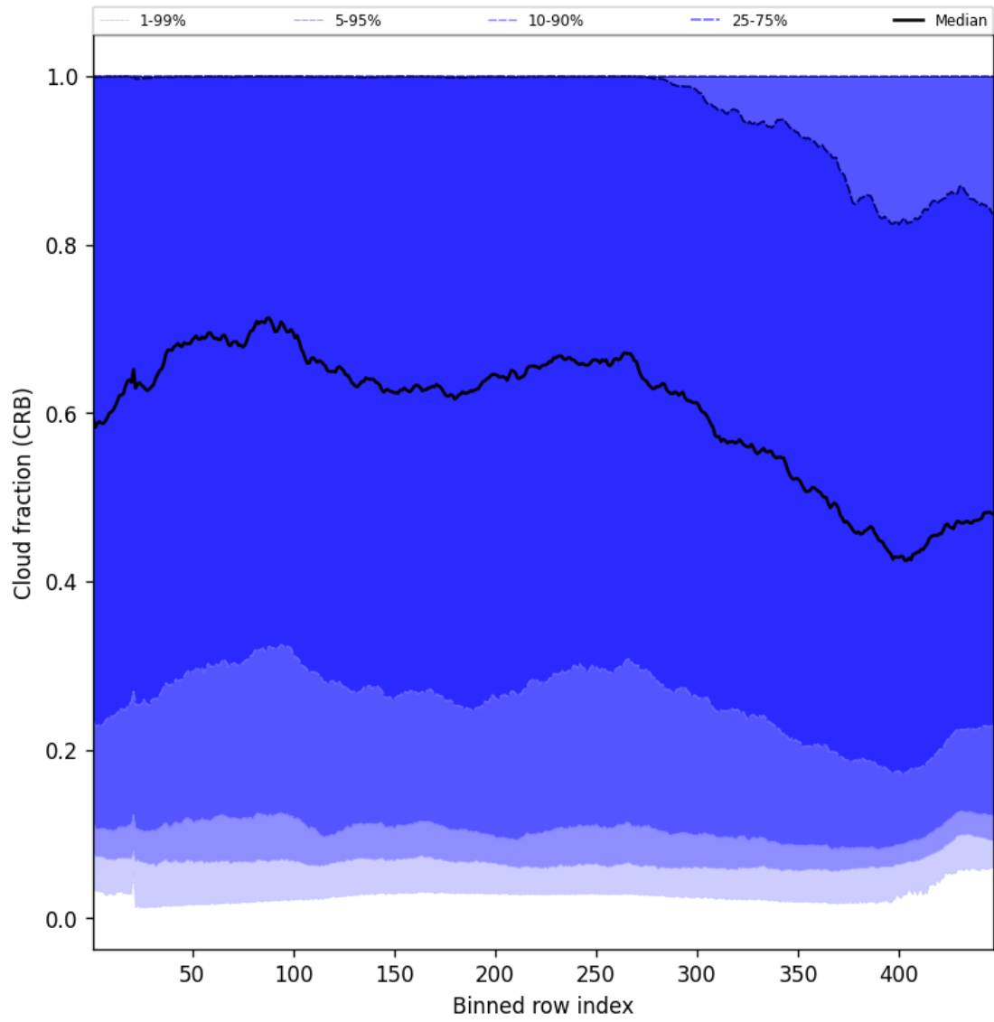
Figure 56: Along track statistics of “Cloud fraction (CRB)” for 2025-08-20 to 2025-08-21
