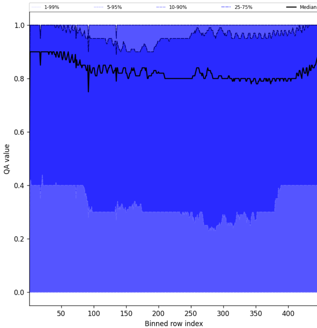
Figure 52: Along track statistics of “QA value” for 2025-08-20 to 2025-08-21
