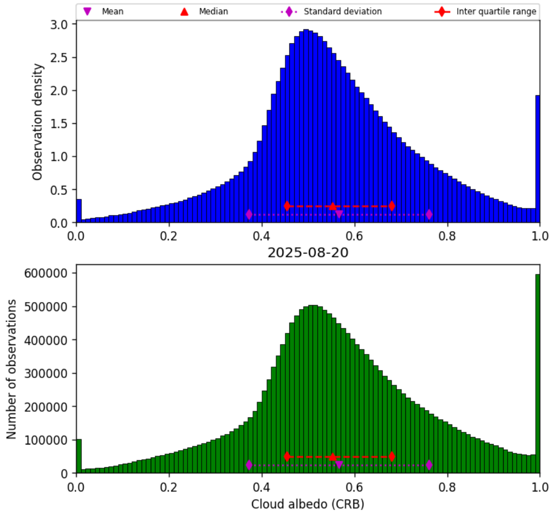
Figure 42: Histogram of “Cloud albedo (CRB)” for 2025-08-20 to 2025-08-21
