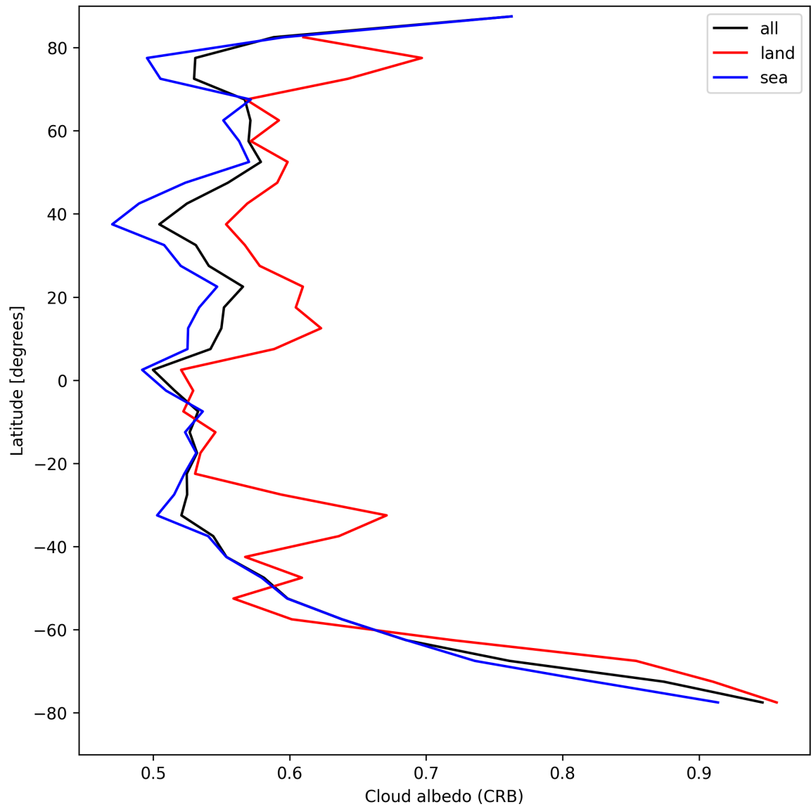
Figure 26: Zonal average of “Cloud albedo (CRB)” for 2025-08-20 to 2025-08-21.
