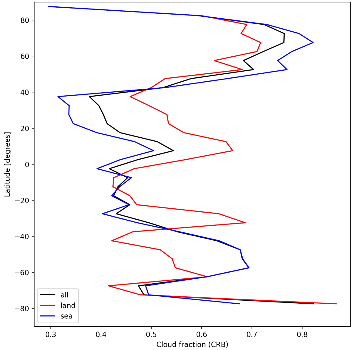
Figure 24: Zonal average of “Cloud fraction (CRB)” for 2025-08-20 to 2025-08-21.
