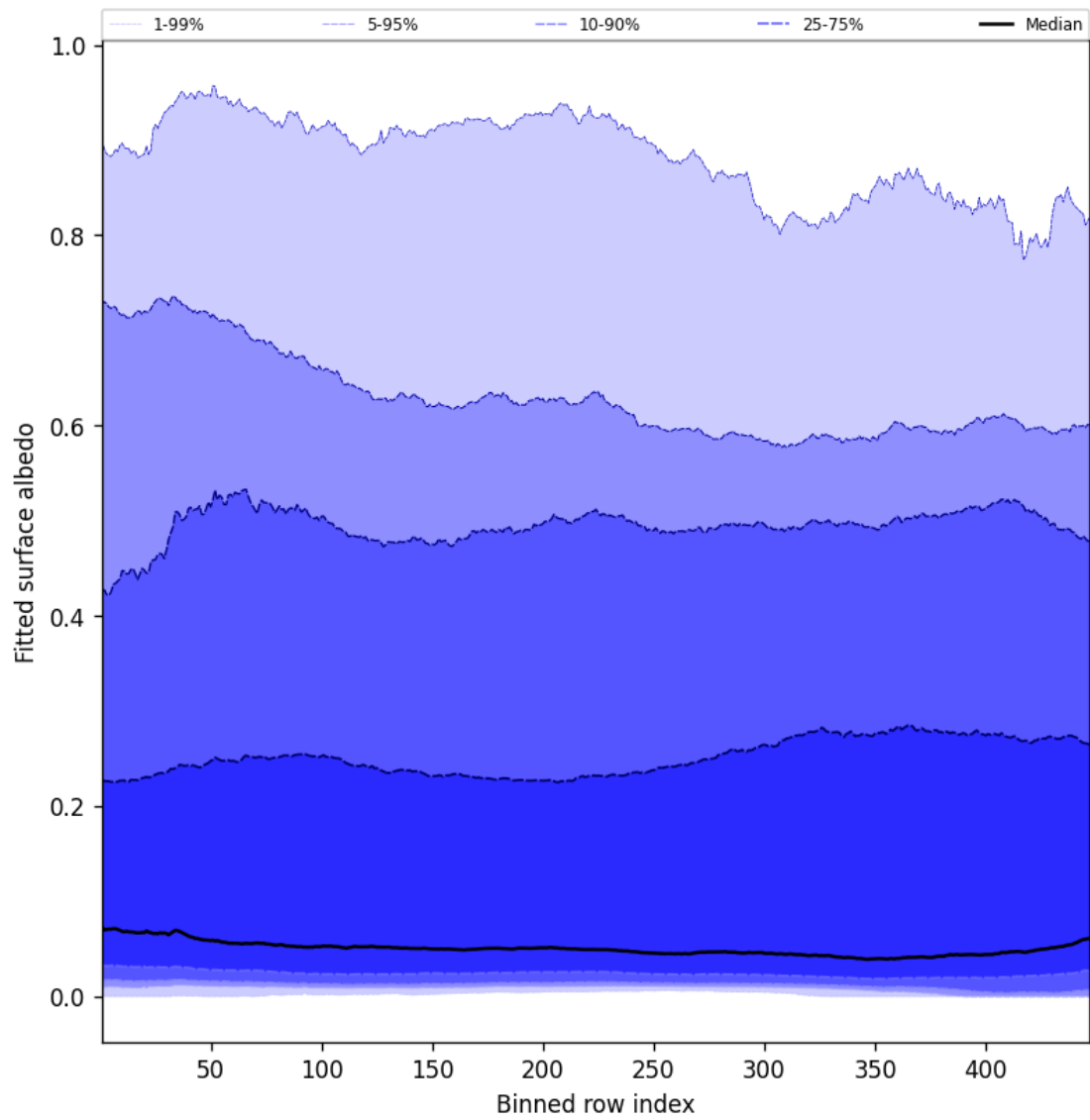
Figure 59: Along track statistics of “Fitted surface albedo” for 2025-08-20 to 2025-08-21
