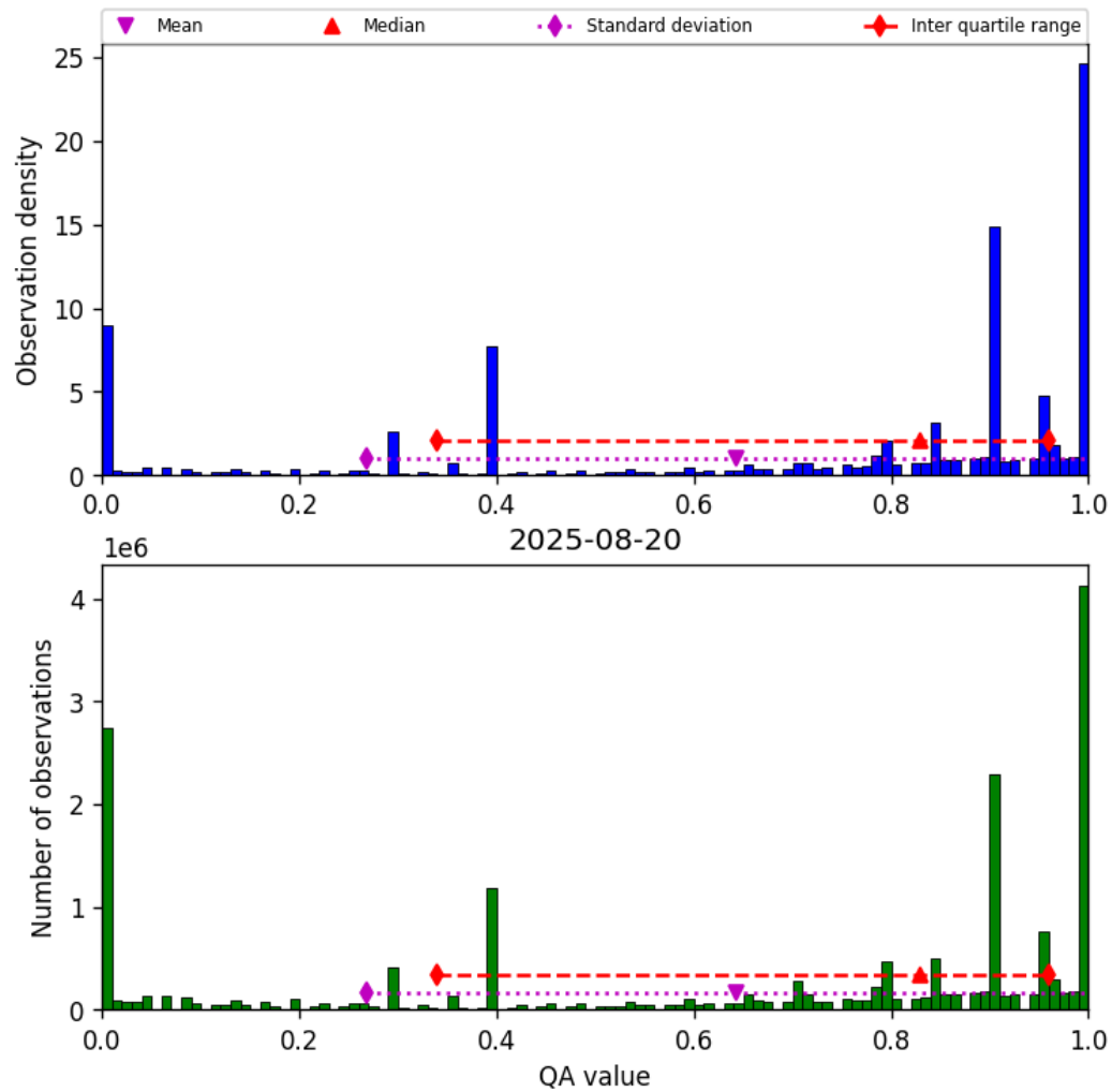
Figure 36: Histogram of “QA value” for 2025-08-20 to 2025-08-21
