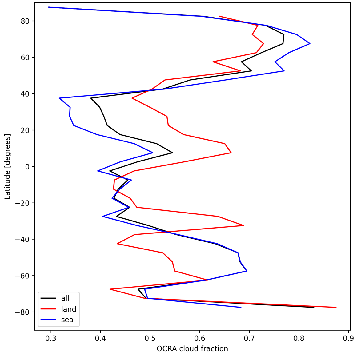
Figure 32: Zonal average of “OCRA cloud fraction” for 2025-08-20 to 2025-08-21.
