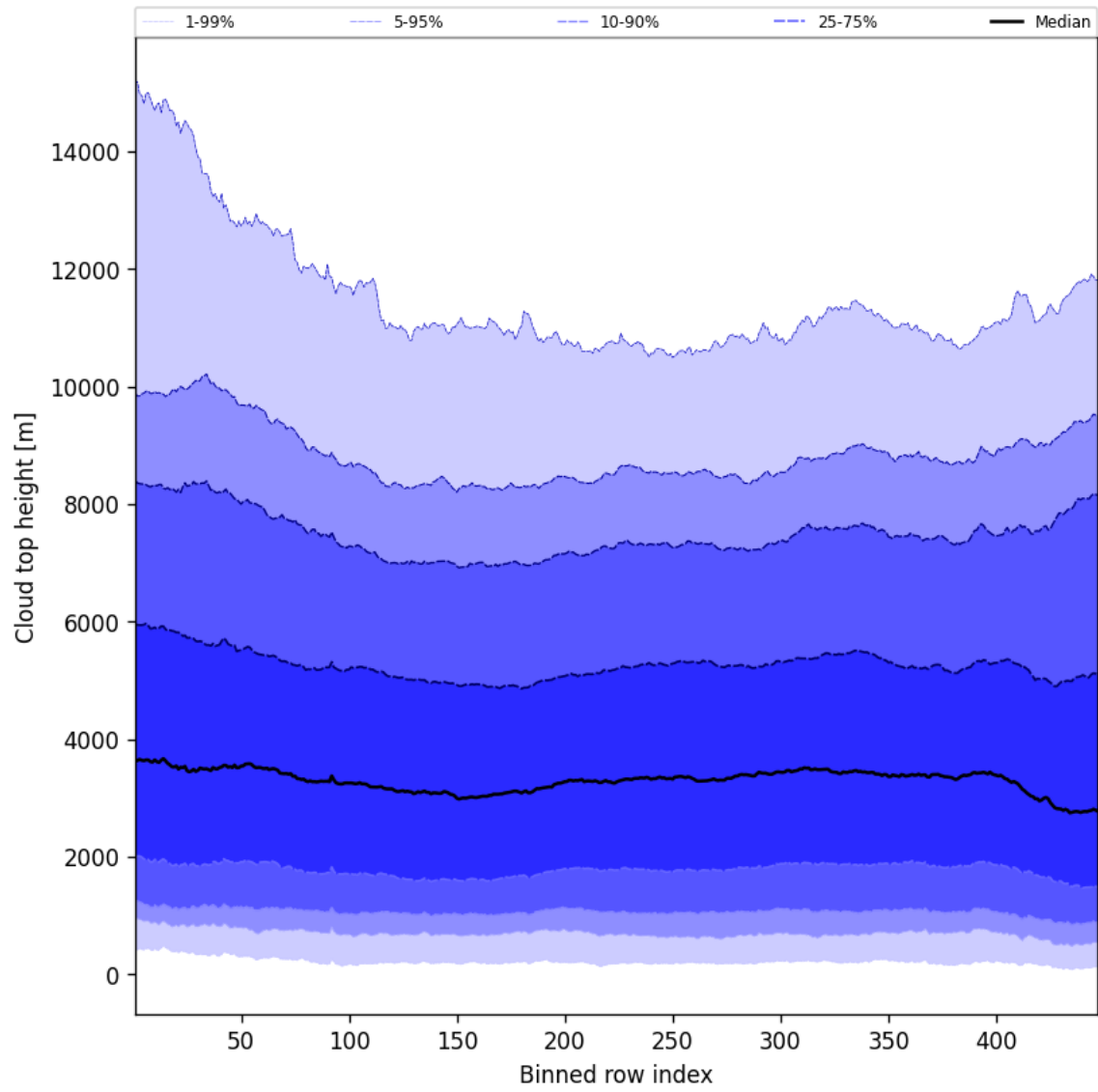
Figure 54: Along track statistics of “Cloud top height” for 2025-08-20 to 2025-08-21
