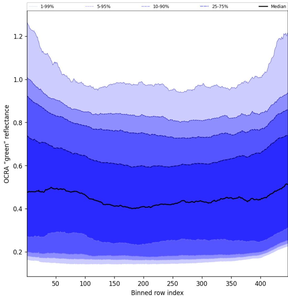
Figure 66: Along track statistics of “OCRA “green” reflectance” for 2025-08-20 to 2025-08-21
