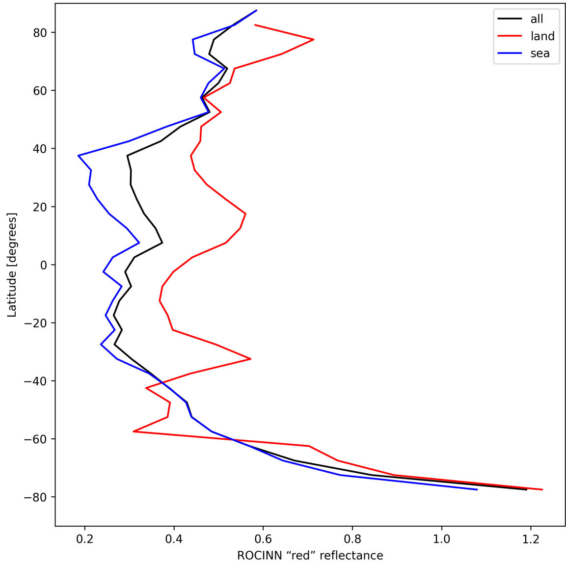
Figure 35: Zonal average of “ROCINN “red” reflectance” for 2025-08-20 to 2025-08-21.
