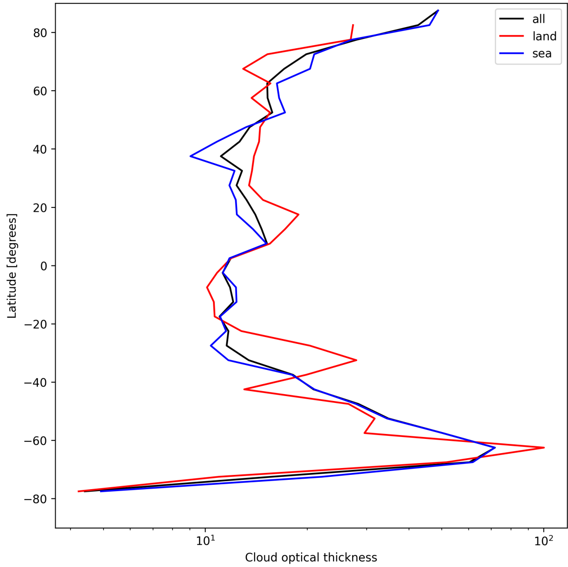
Figure 23: Zonal average of “Cloud optical thickness” for 2025-08-20 to 2025-08-21.
