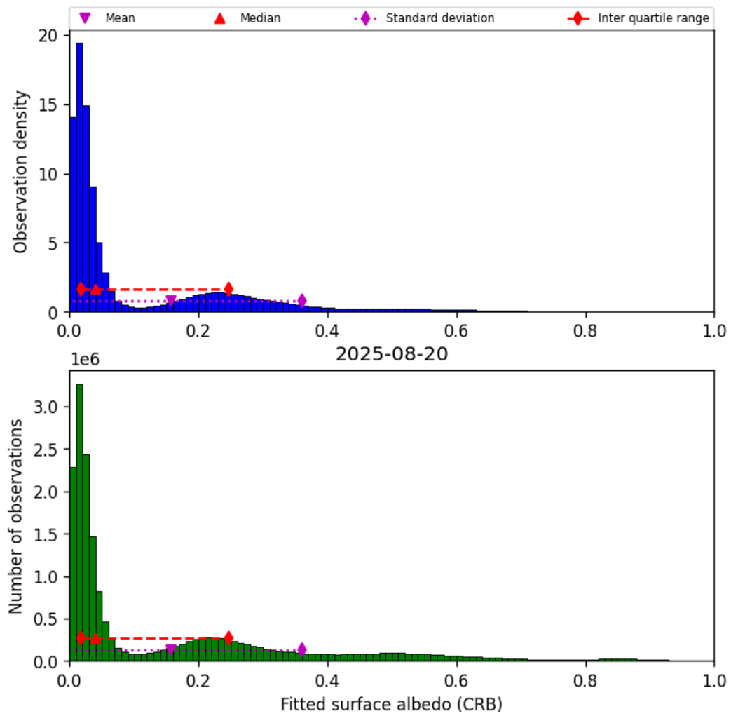
Figure 44: Histogram of “Fitted surface albedo (CRB)” for 2025-08-20 to 2025-08-21
