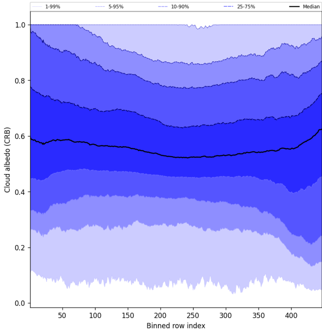
Figure 58: Along track statistics of “Cloud albedo (CRB)” for 2025-08-20 to 2025-08-21
