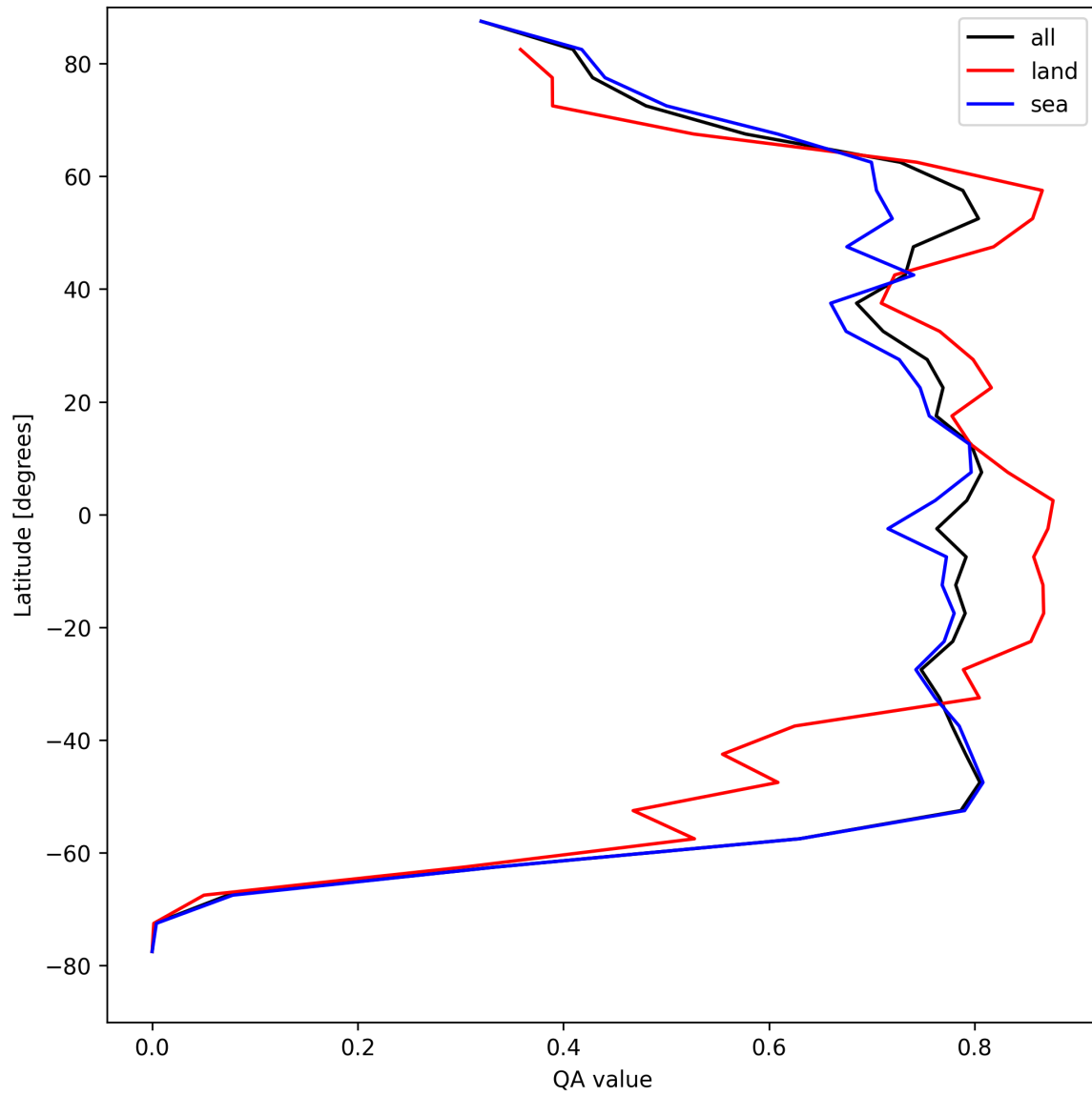
Figure 20: Zonal average of “QA value” for 2025-08-20 to 2025-08-21.
