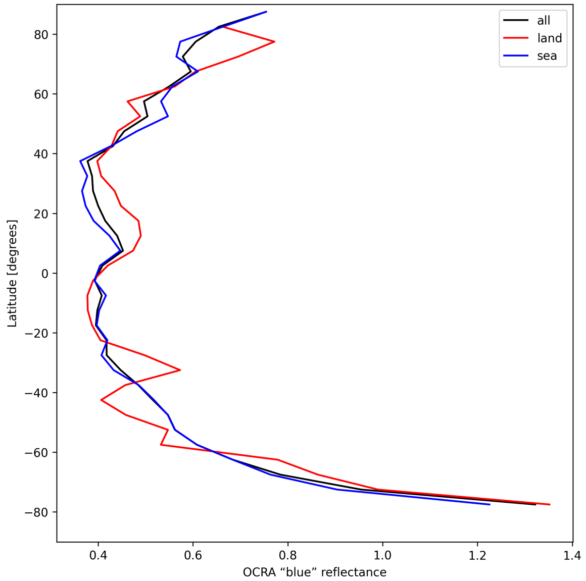
Figure 33: Zonal average of “OCRA “blue” reflectance” for 2025-08-20 to 2025-08-21.
