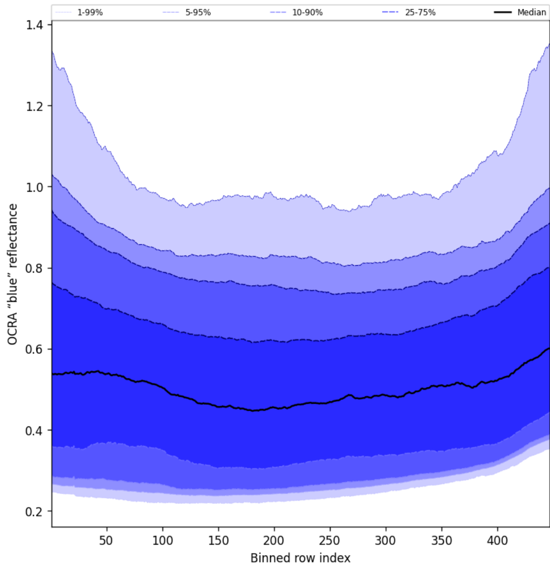
Figure 65: Along track statistics of “OCRA “blue” reflectance” for 2025-08-20 to 2025-08-21
