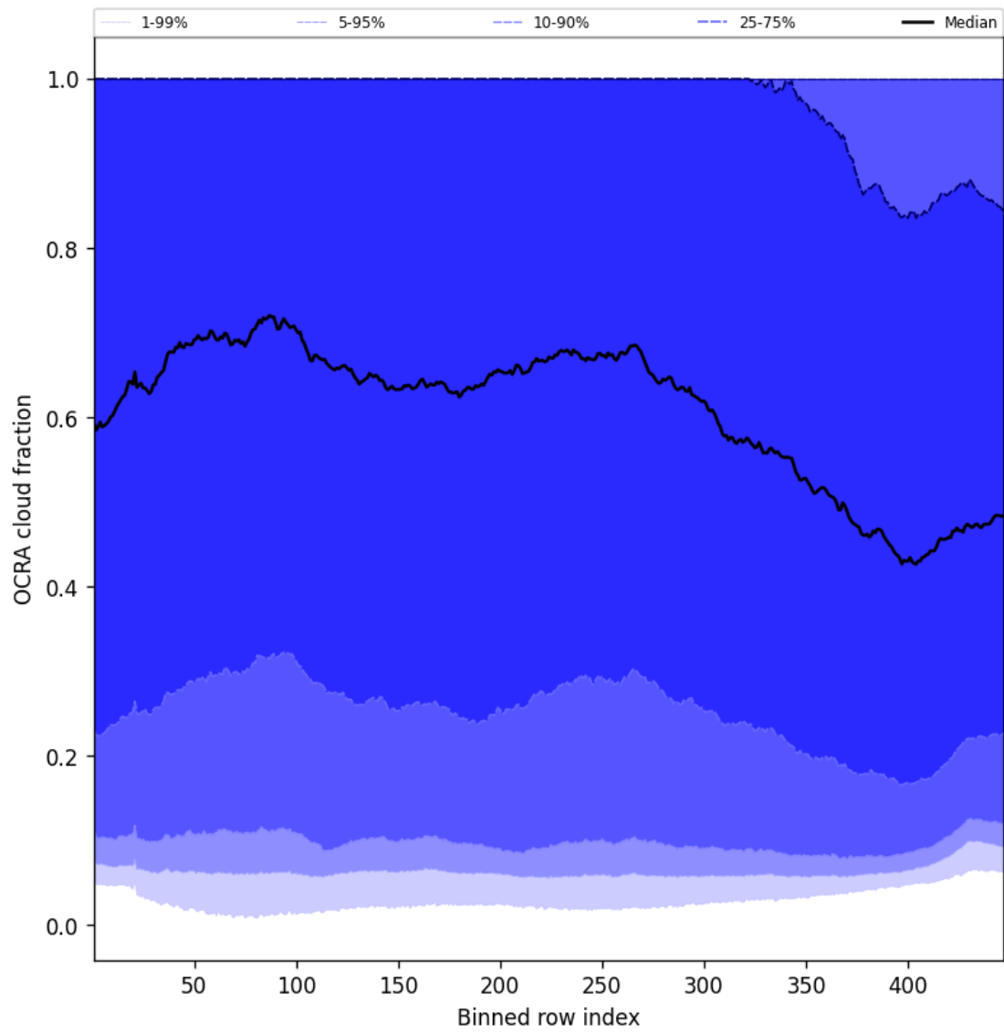
Figure 64: Along track statistics of “OCRA cloud fraction” for 2025-08-20 to 2025-08-21
