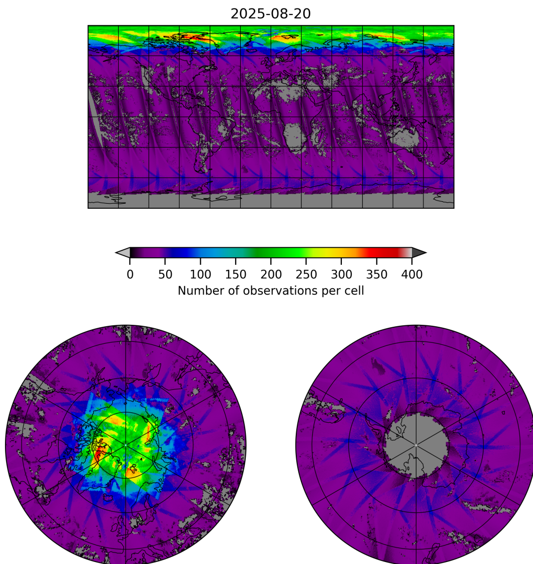
Figure 19: Map of the number of observations for 2025-08-20 to 2025-08-21
