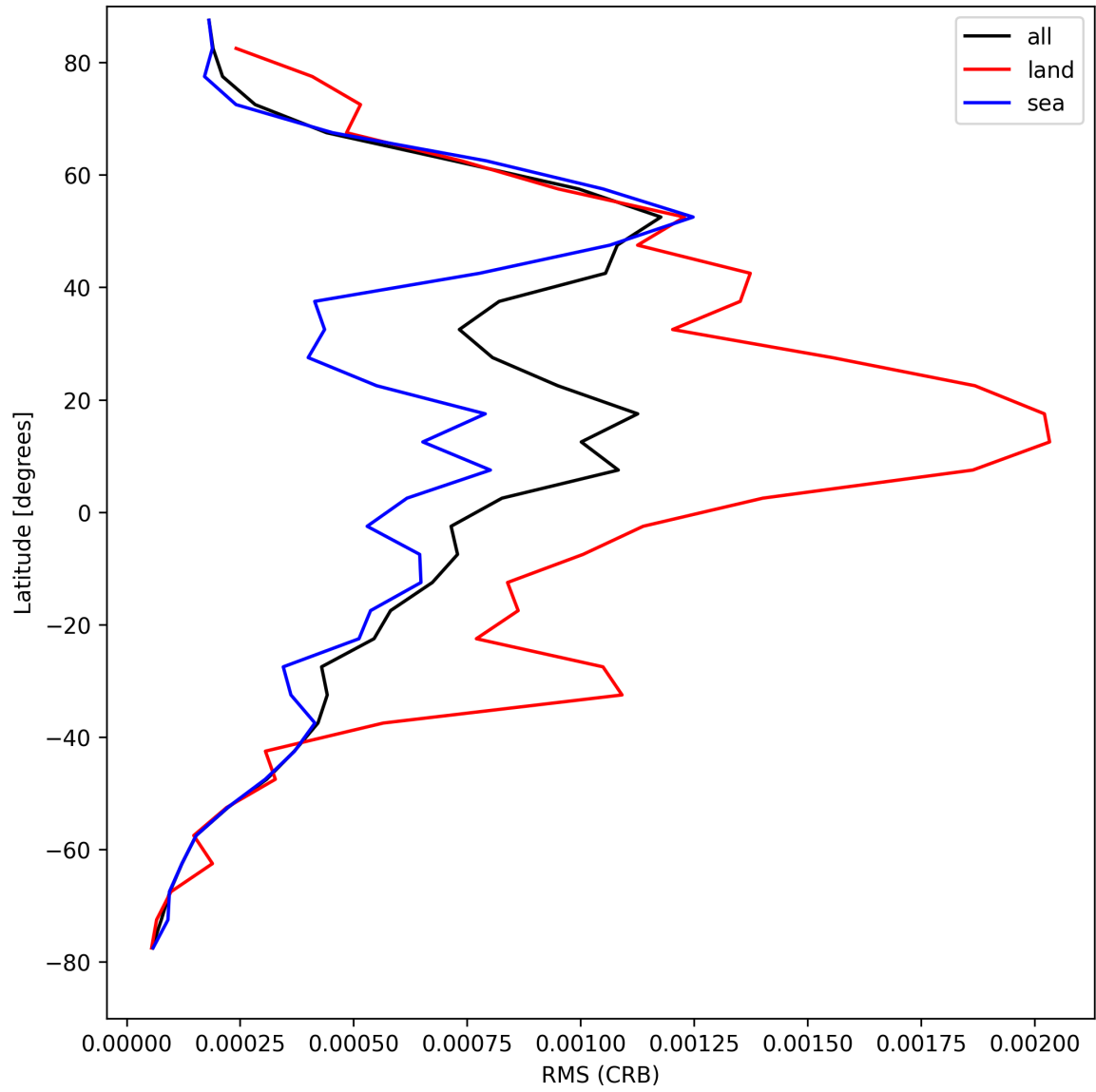
Figure 30: Zonal average of “RMS (CRB)” for 2025-08-20 to 2025-08-21.
