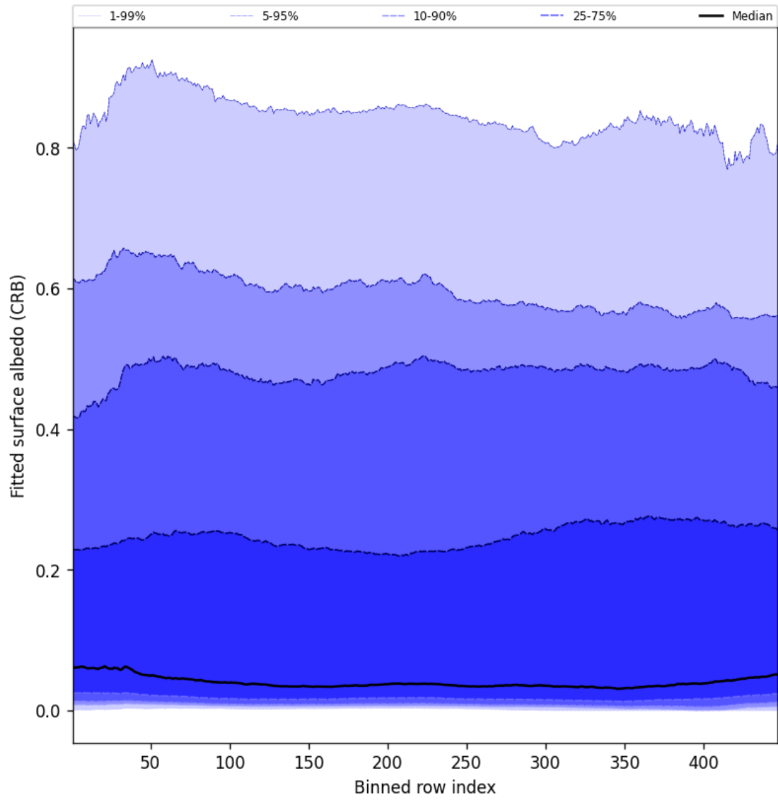
Figure 60: Along track statistics of “Fitted surface albedo (CRB)” for 2025-08-20 to 2025-08-21
