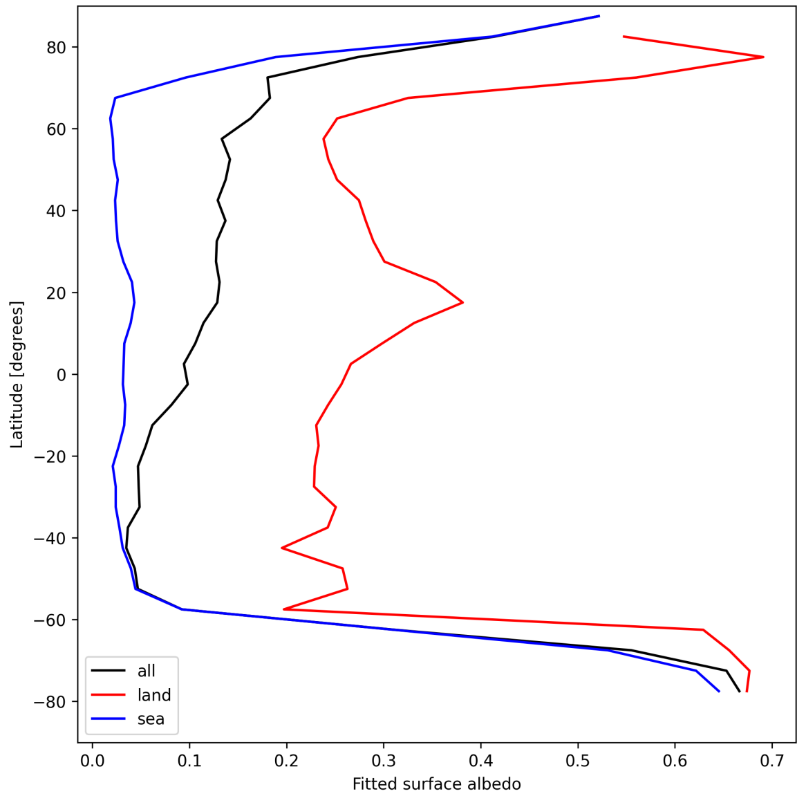
Figure 27: Zonal average of “Fitted surface albedo” for 2025-08-20 to 2025-08-21.
