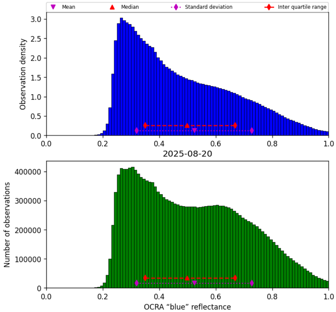
Figure 49: Histogram of “OCRA “blue” reflectance” for 2025-08-20 to 2025-08-21
