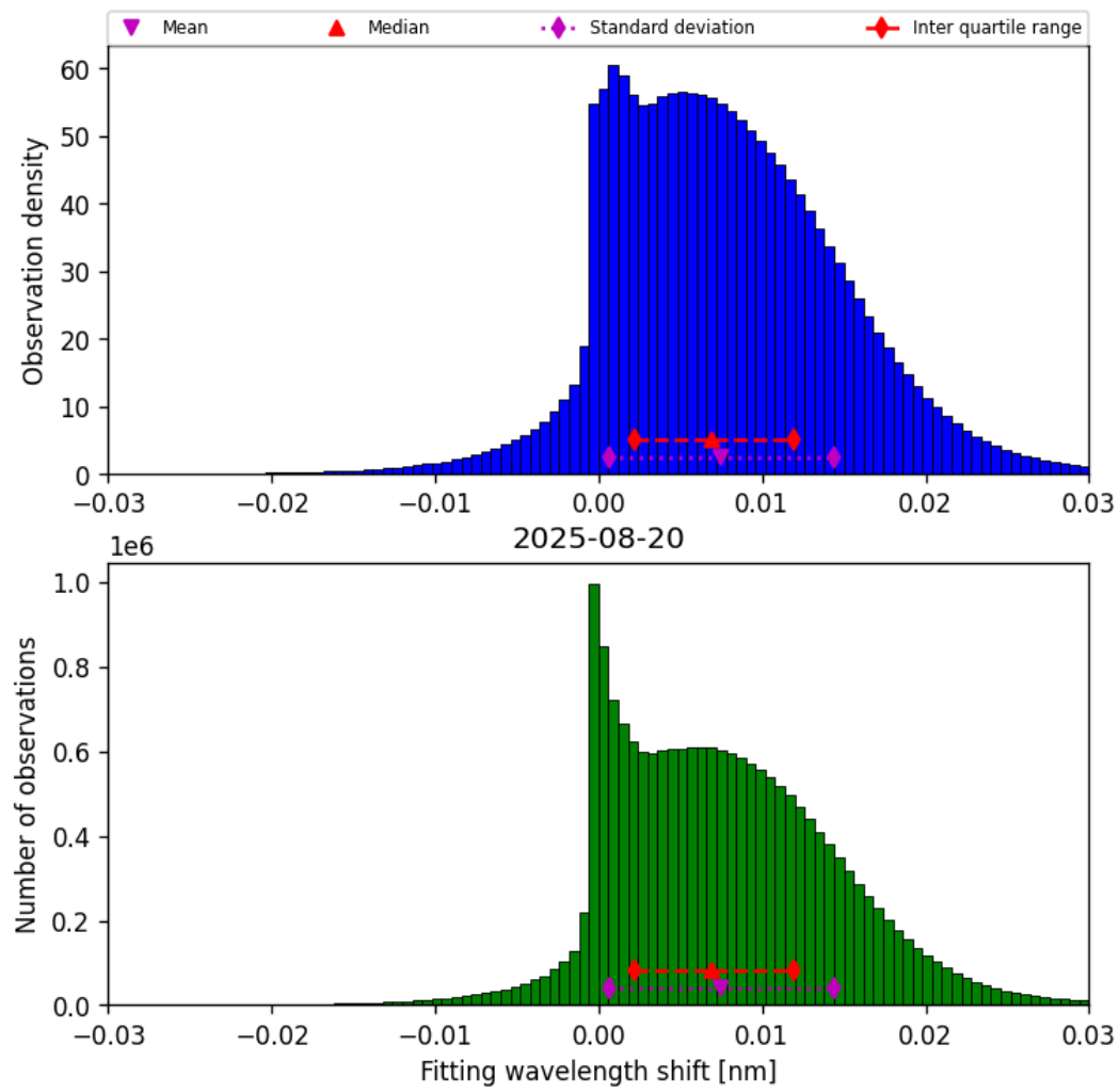
Figure 47: Histogram of “Fitting wavelength shift” for 2025-08-20 to 2025-08-21
