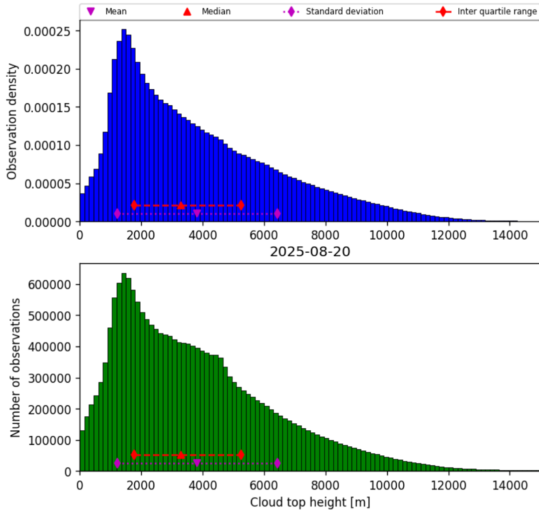
Figure 38: Histogram of “Cloud top height” for 2025-08-20 to 2025-08-21
