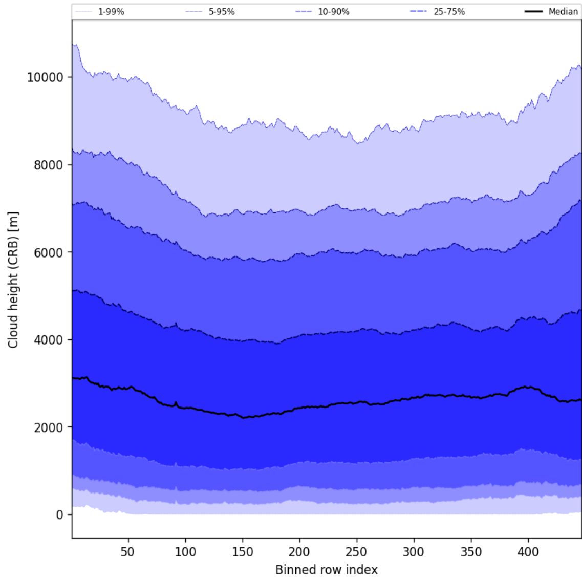
Figure 57: Along track statistics of “Cloud height (CRB)” for 2025-08-20 to 2025-08-21
