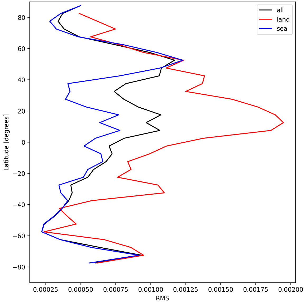
Figure 29: Zonal average of “RMS” for 2025-08-20 to 2025-08-21.
