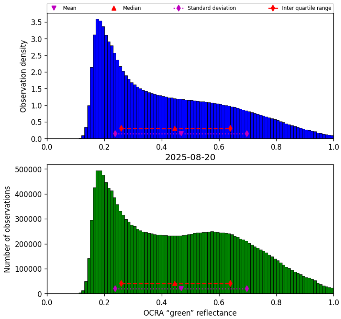
Figure 50: Histogram of “OCRA “green” reflectance” for 2025-08-20 to 2025-08-21
