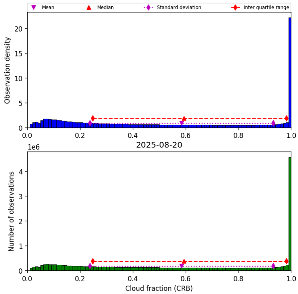
Figure 40: Histogram of “Cloud fraction (CRB)” for 2025-08-20 to 2025-08-21
