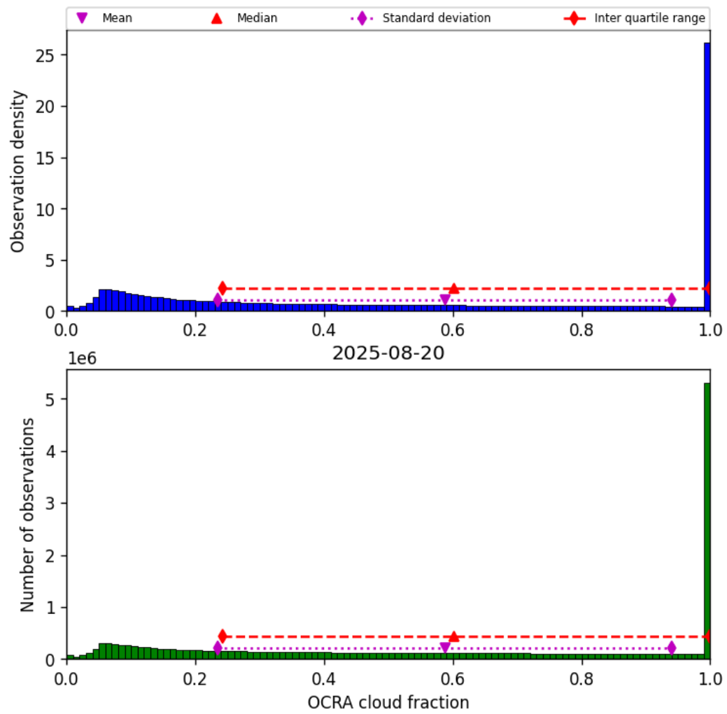
Figure 48: Histogram of “OCRA cloud fraction” for 2025-08-20 to 2025-08-21
