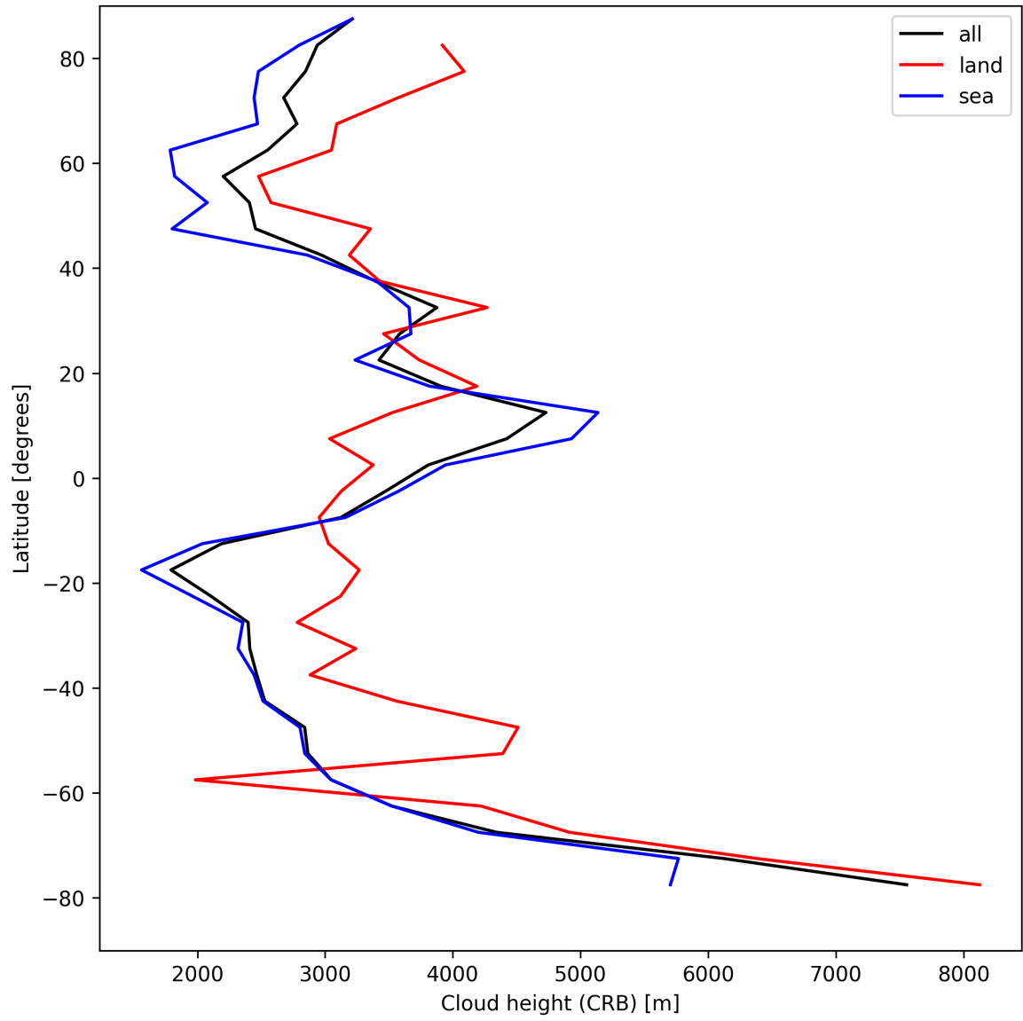
Figure 25: Zonal average of “Cloud height (CRB)” for 2025-08-20 to 2025-08-21.
