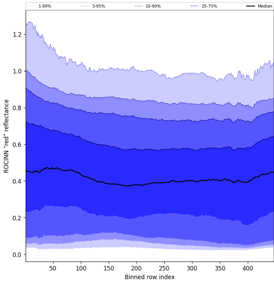
Figure 67: Along track statistics of “ROCINN “red” reflectance” for 2025-08-20 to 2025-08-21
