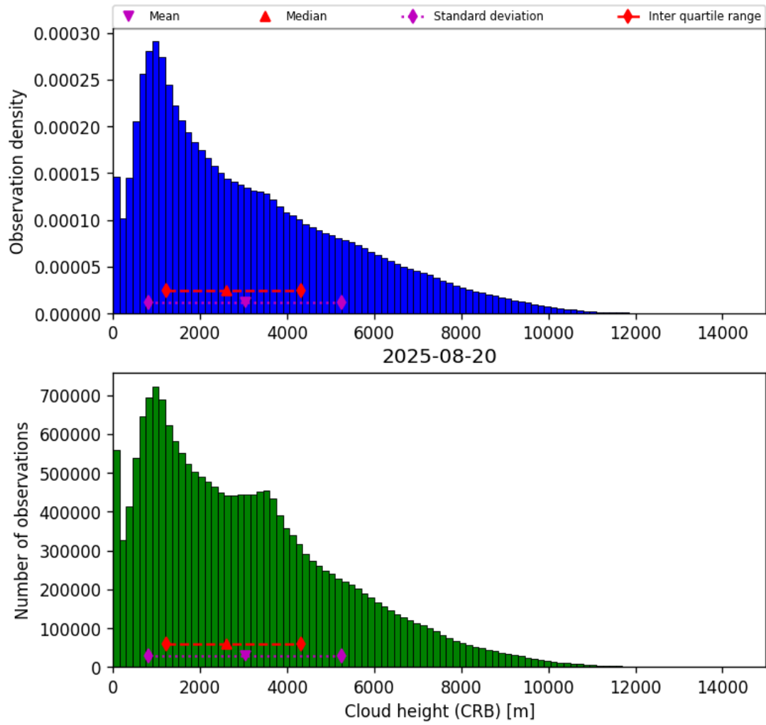
Figure 41: Histogram of “Cloud height (CRB)” for 2025-08-20 to 2025-08-21
