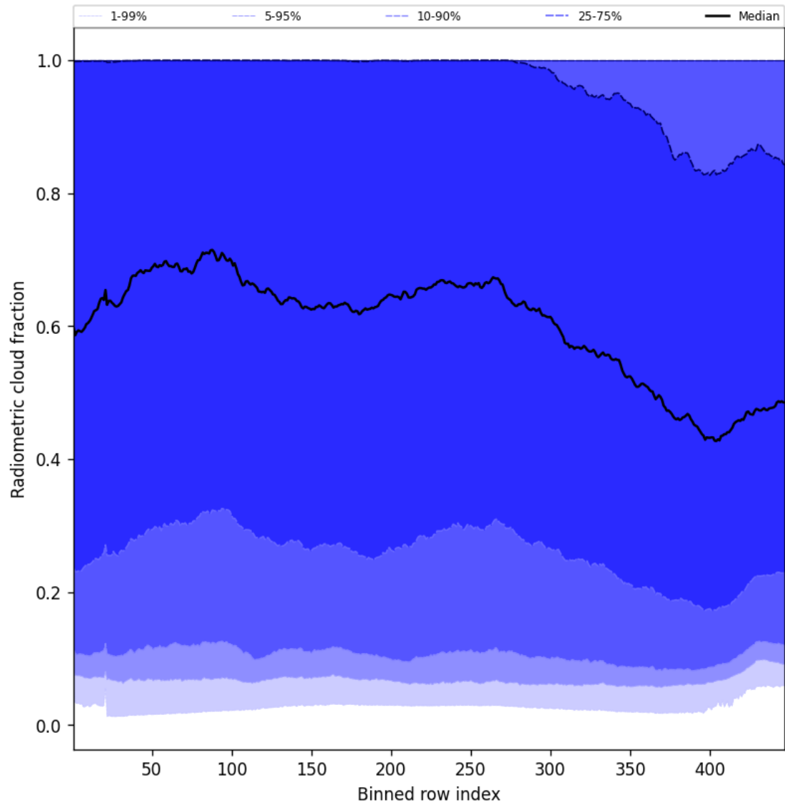
Figure 53: Along track statistics of “Radiometric cloud fraction” for 2025-08-20 to 2025-08-21
