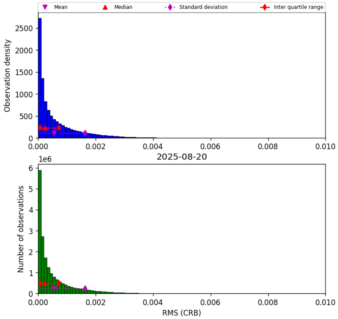
Figure 46: Histogram of “RMS (CRB)” for 2025-08-20 to 2025-08-21
