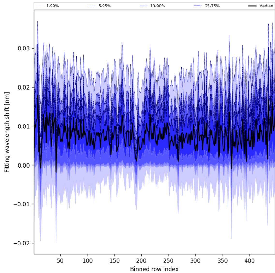
Figure 63: Along track statistics of “Fitting wavelength shift” for 2025-08-20 to 2025-08-21
