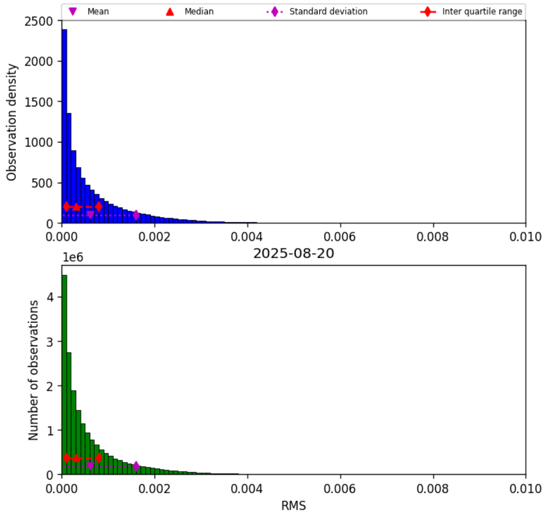
Figure 45: Histogram of “RMS” for 2025-08-20 to 2025-08-21
