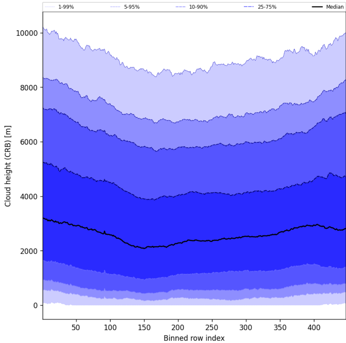
Figure 57: Along track statistics of “Cloud height (CRB)” for 2025-08-21 to 2025-08-22
