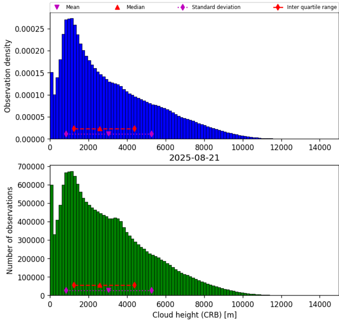
Figure 41: Histogram of “Cloud height (CRB)” for 2025-08-21 to 2025-08-22
