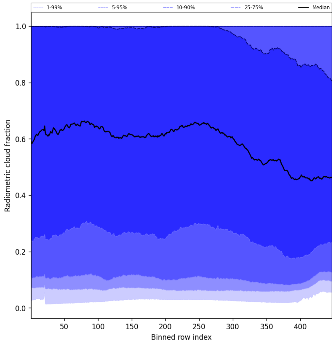
Figure 53: Along track statistics of “Radiometric cloud fraction” for 2025-08-21 to 2025-08-22
