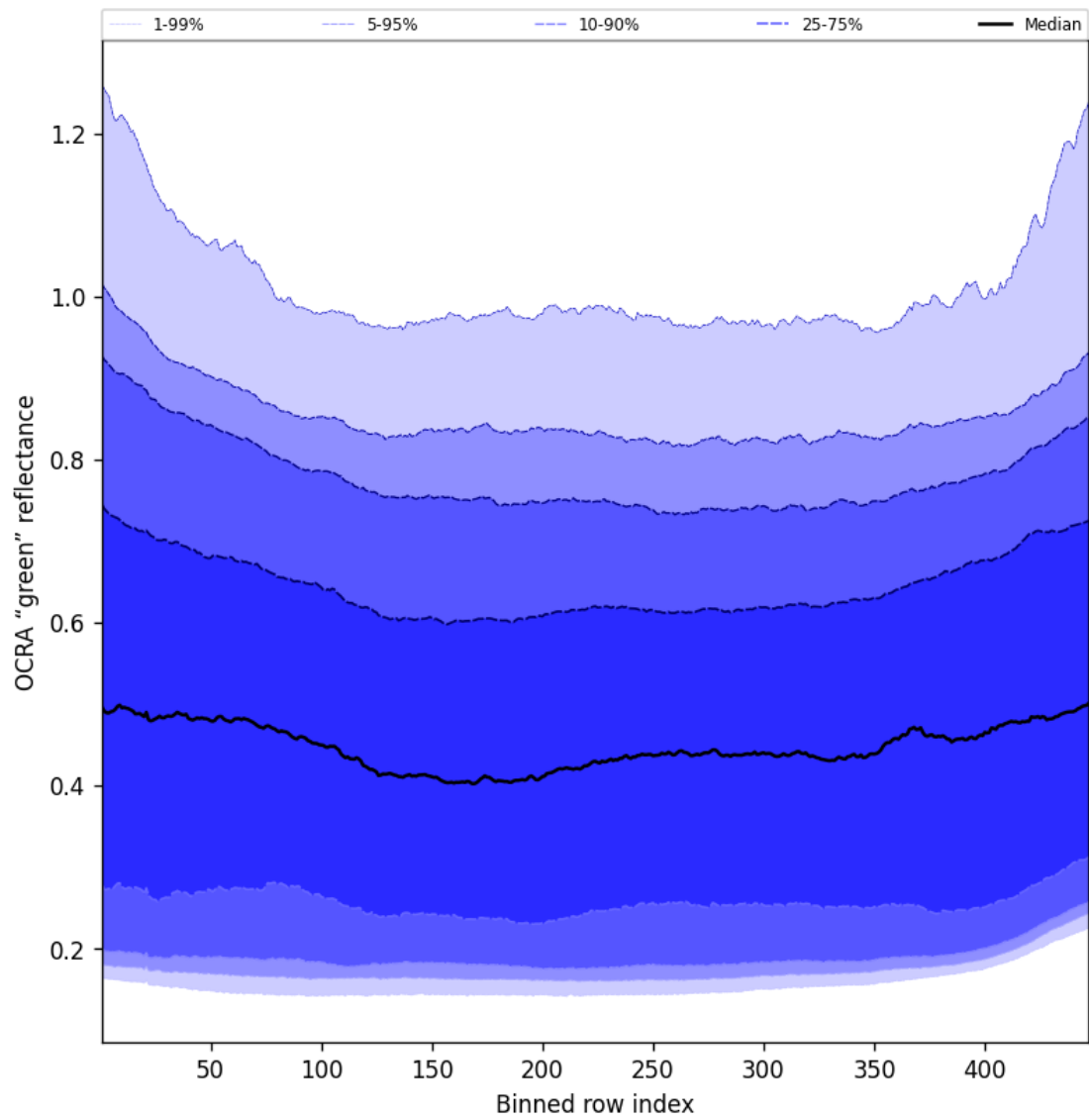
Figure 66: Along track statistics of "OCRA "green" reflectance" for 2025-08-21 to 2025-08-22
