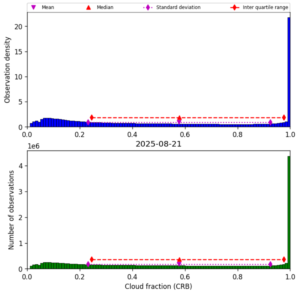
Figure 40: Histogram of “Cloud fraction (CRB)” for 2025-08-21 to 2025-08-22
