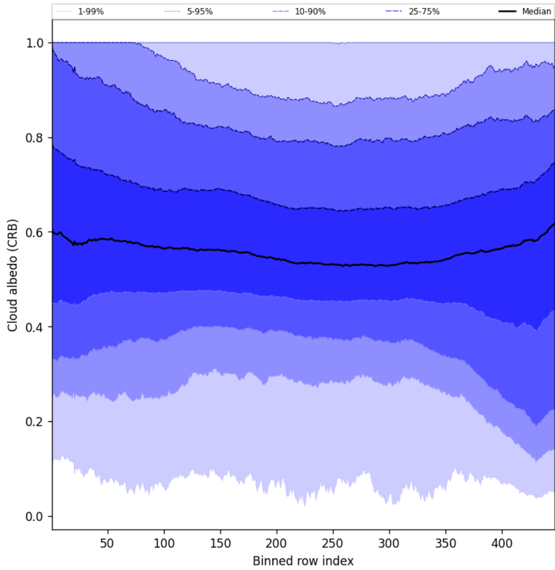
Figure 58: Along track statistics of “Cloud albedo (CRB)” for 2025-08-21 to 2025-08-22
