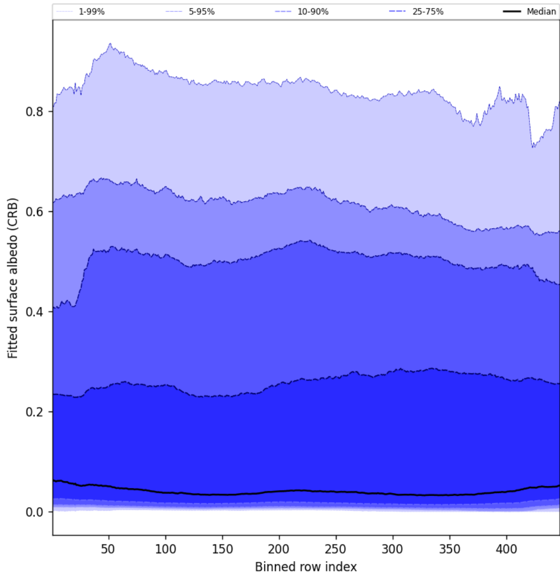
Figure 60: Along track statistics of “Fitted surface albedo (CRB)” for 2025-08-21 to 2025-08-22
