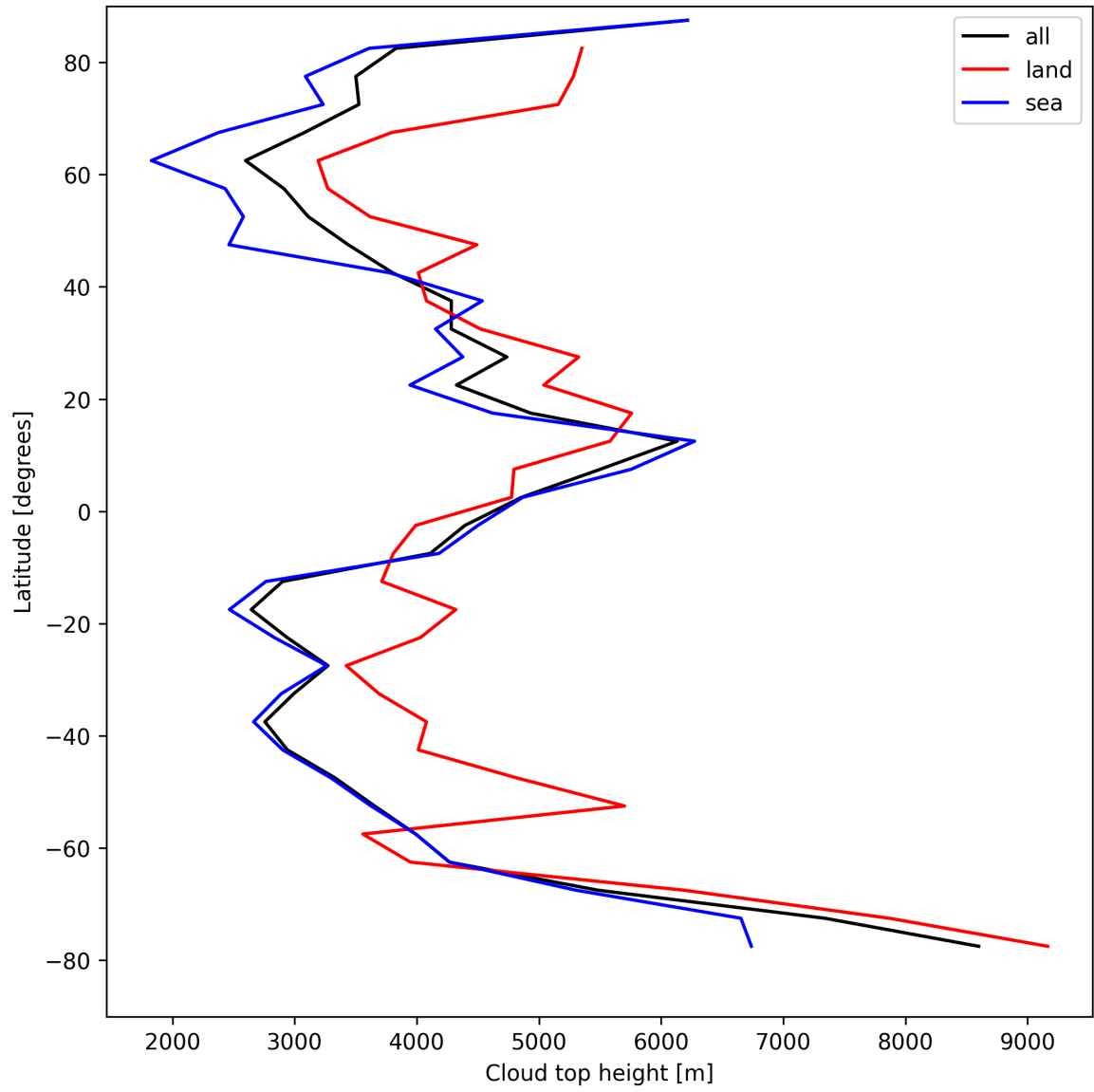
Figure 22: Zonal average of “Cloud top height” for 2025-08-21 to 2025-08-22.
