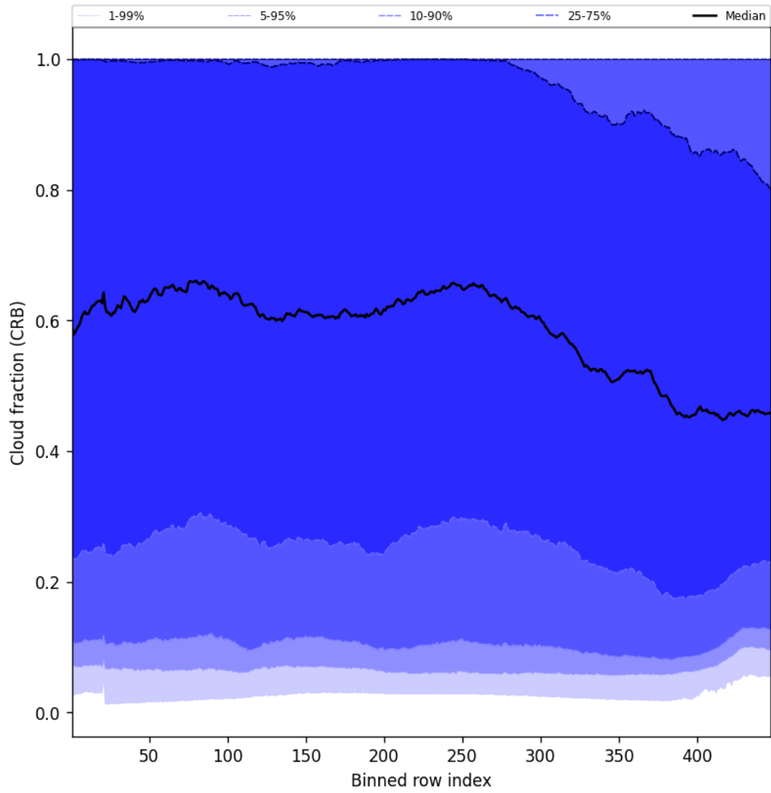
Figure 56: Along track statistics of “Cloud fraction (CRB)” for 2025-08-21 to 2025-08-22
