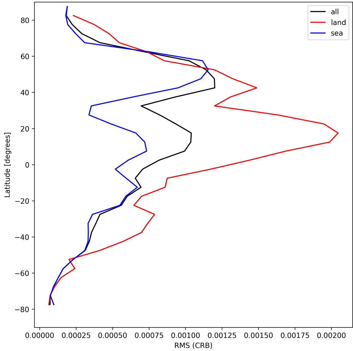
Figure 30: Zonal average of “RMS (CRB)” for 2025-08-21 to 2025-08-22.
