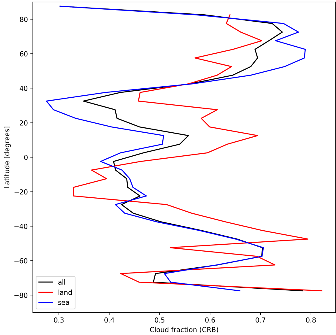
Figure 24: Zonal average of “Cloud fraction (CRB)” for 2025-08-21 to 2025-08-22.
