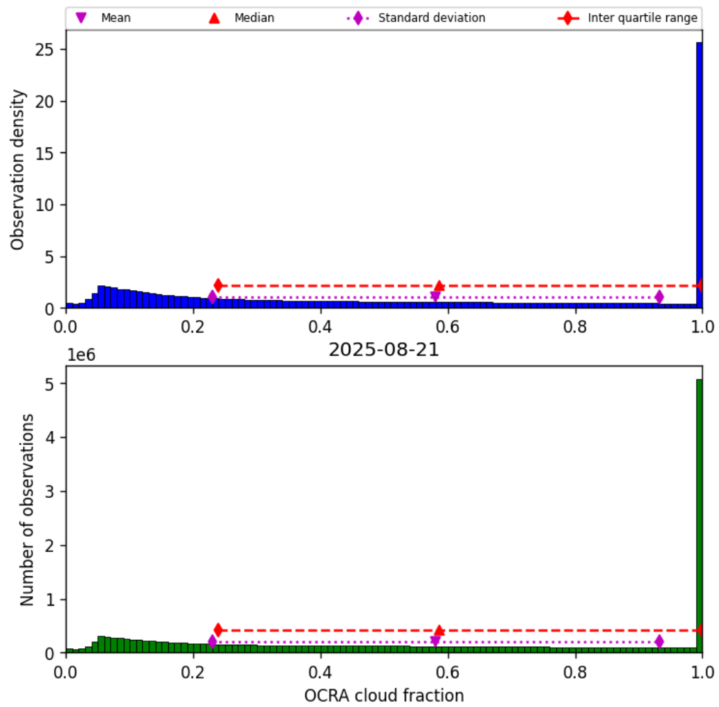
Figure 48: Histogram of “OCRA cloud fraction” for 2025-08-21 to 2025-08-22
