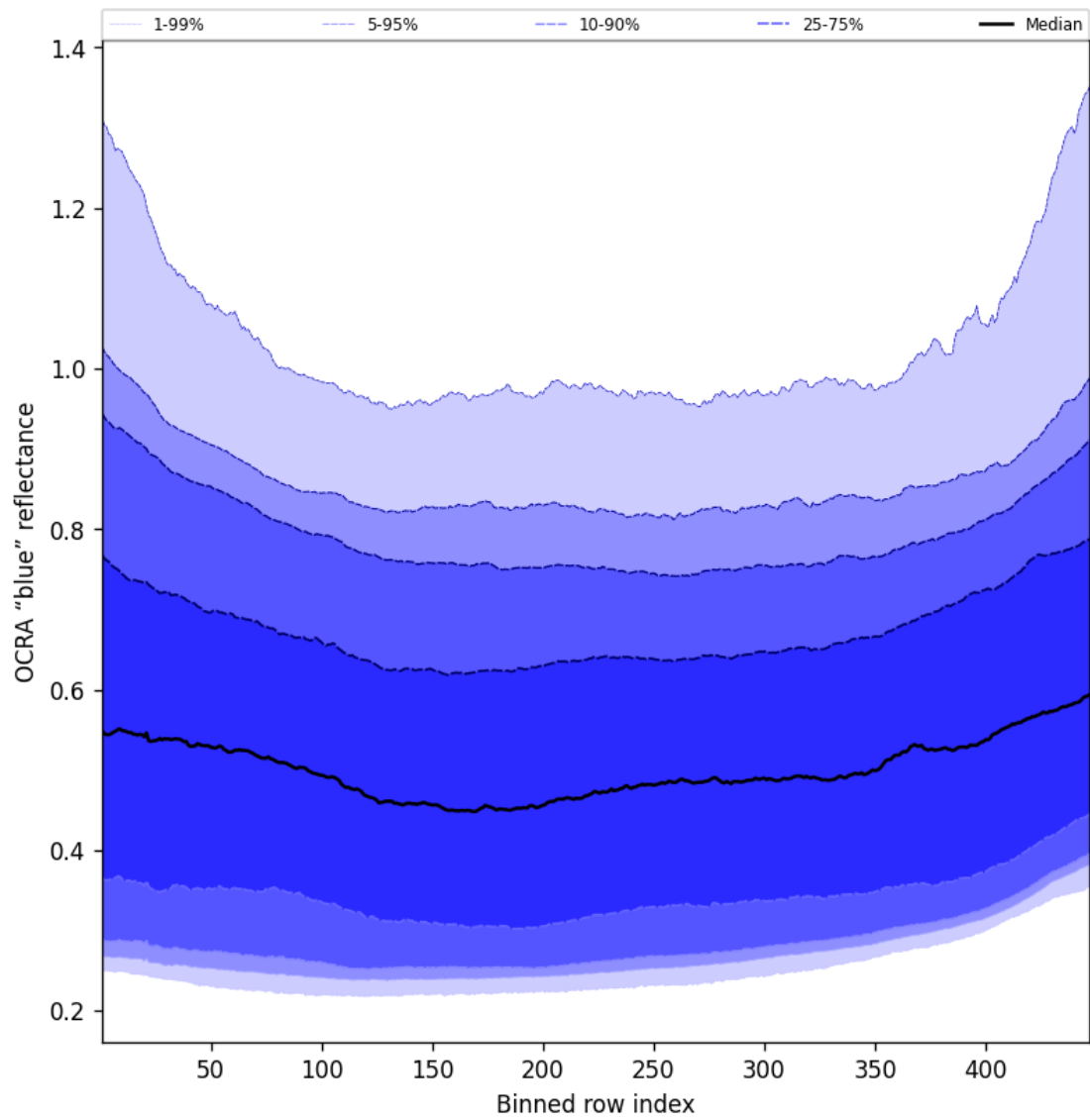
Figure 65: Along track statistics of “OCRA “blue” reflectance” for 2025-08-21 to 2025-08-22
