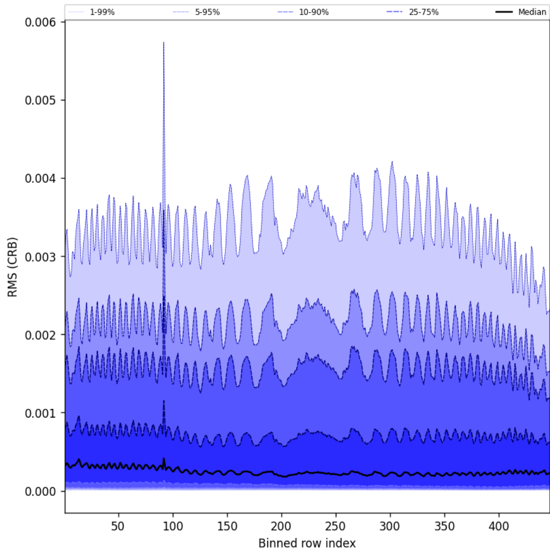
Figure 62: Along track statistics of “RMS (CRB)” for 2025-08-21 to 2025-08-22
