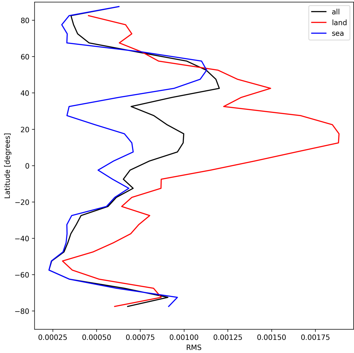
Figure 29: Zonal average of “RMS” for 2025-08-21 to 2025-08-22.
