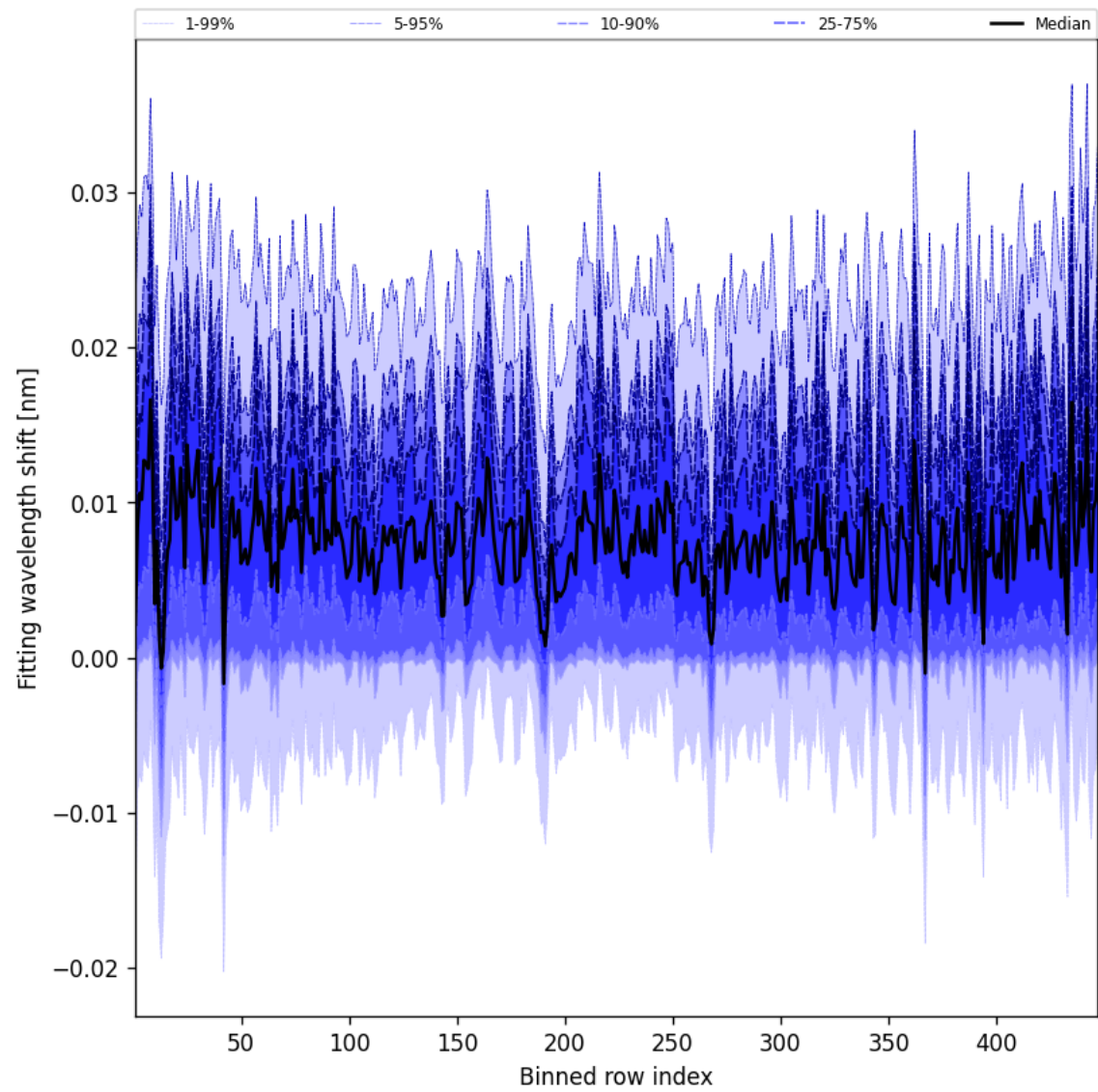
Figure 63: Along track statistics of “Fitting wavelength shift” for 2025-08-21 to 2025-08-22
