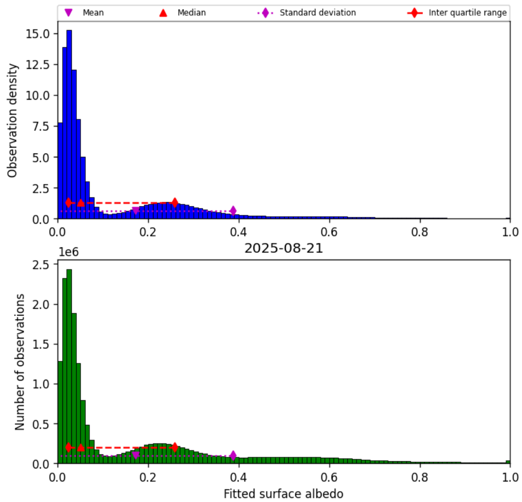
Figure 43: Histogram of “Fitted surface albedo” for 2025-08-21 to 2025-08-22
