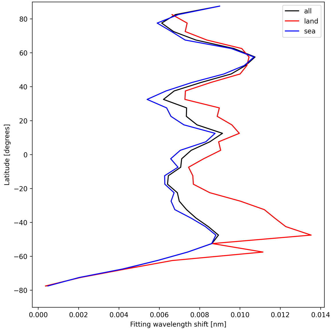
Figure 31: Zonal average of “Fitting wavelength shift” for 2025-08-21 to 2025-08-22.
