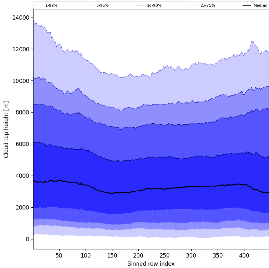
Figure 54: Along track statistics of “Cloud top height” for 2025-08-21 to 2025-08-22
