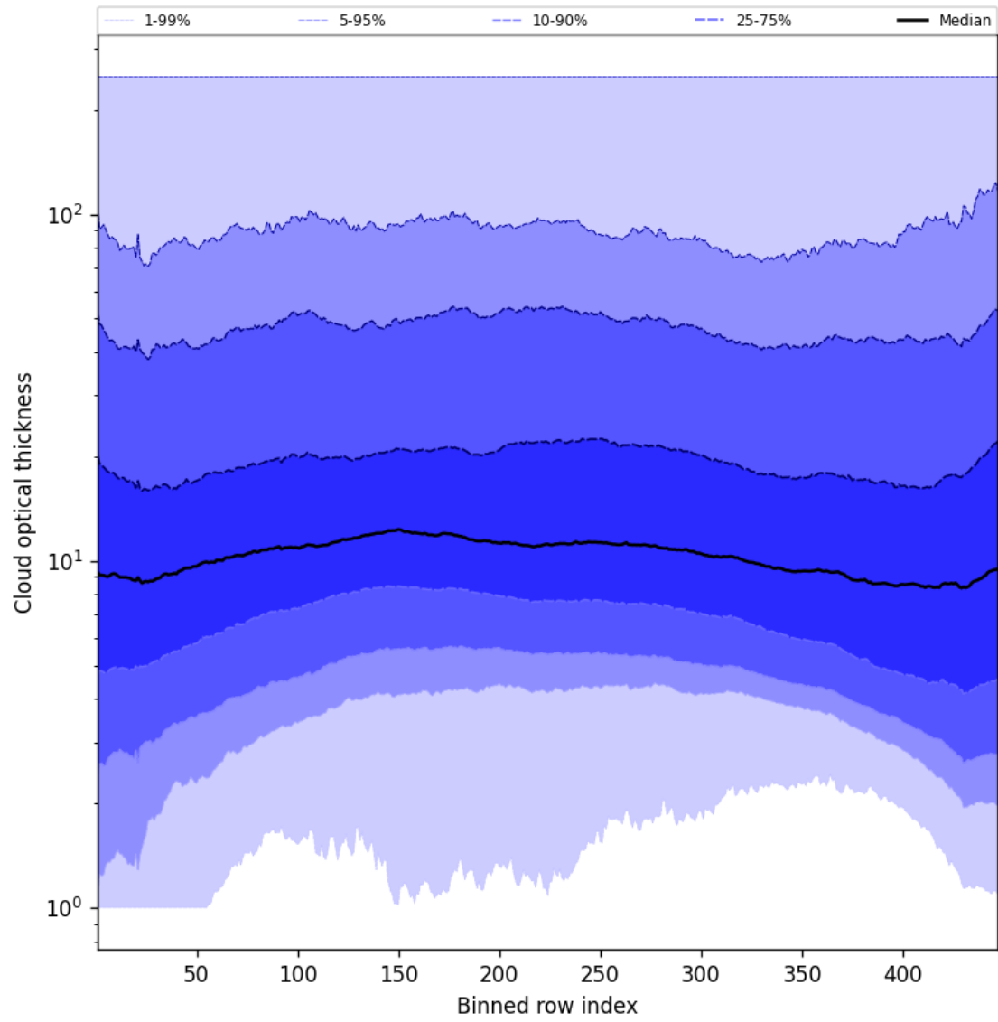
Figure 55: Along track statistics of “Cloud optical thickness” for 2025-08-21 to 2025-08-22
