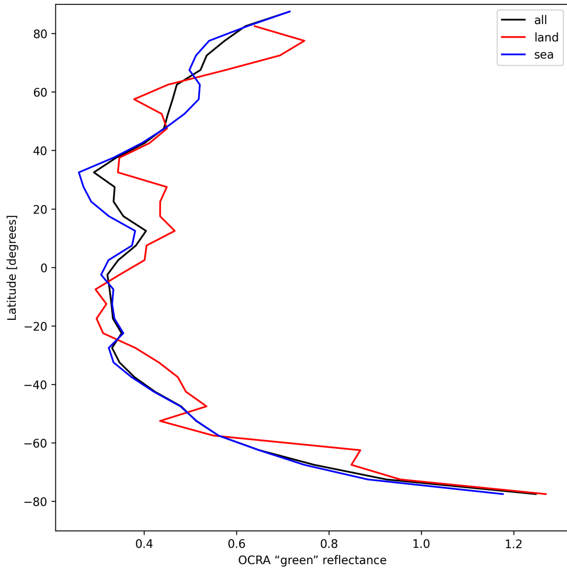
Figure 34: Zonal average of “OCRA “green” reflectance” for 2025-08-21 to 2025-08-22.
