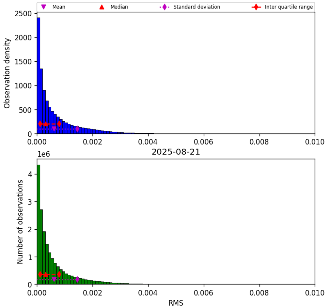
Figure 45: Histogram of “RMS” for 2025-08-21 to 2025-08-22
