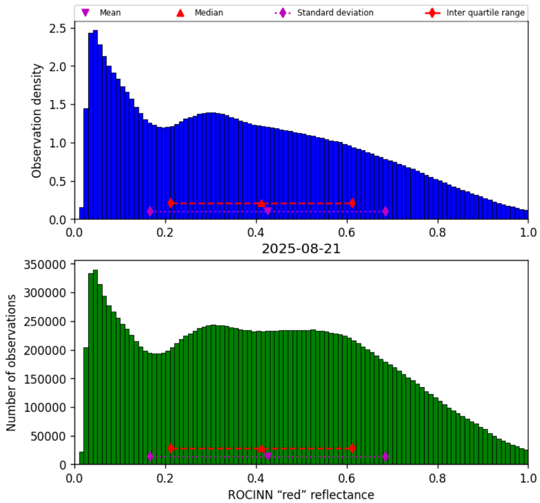
Figure 51: Histogram of “ROCINN “red” reflectance” for 2025-08-21 to 2025-08-22
