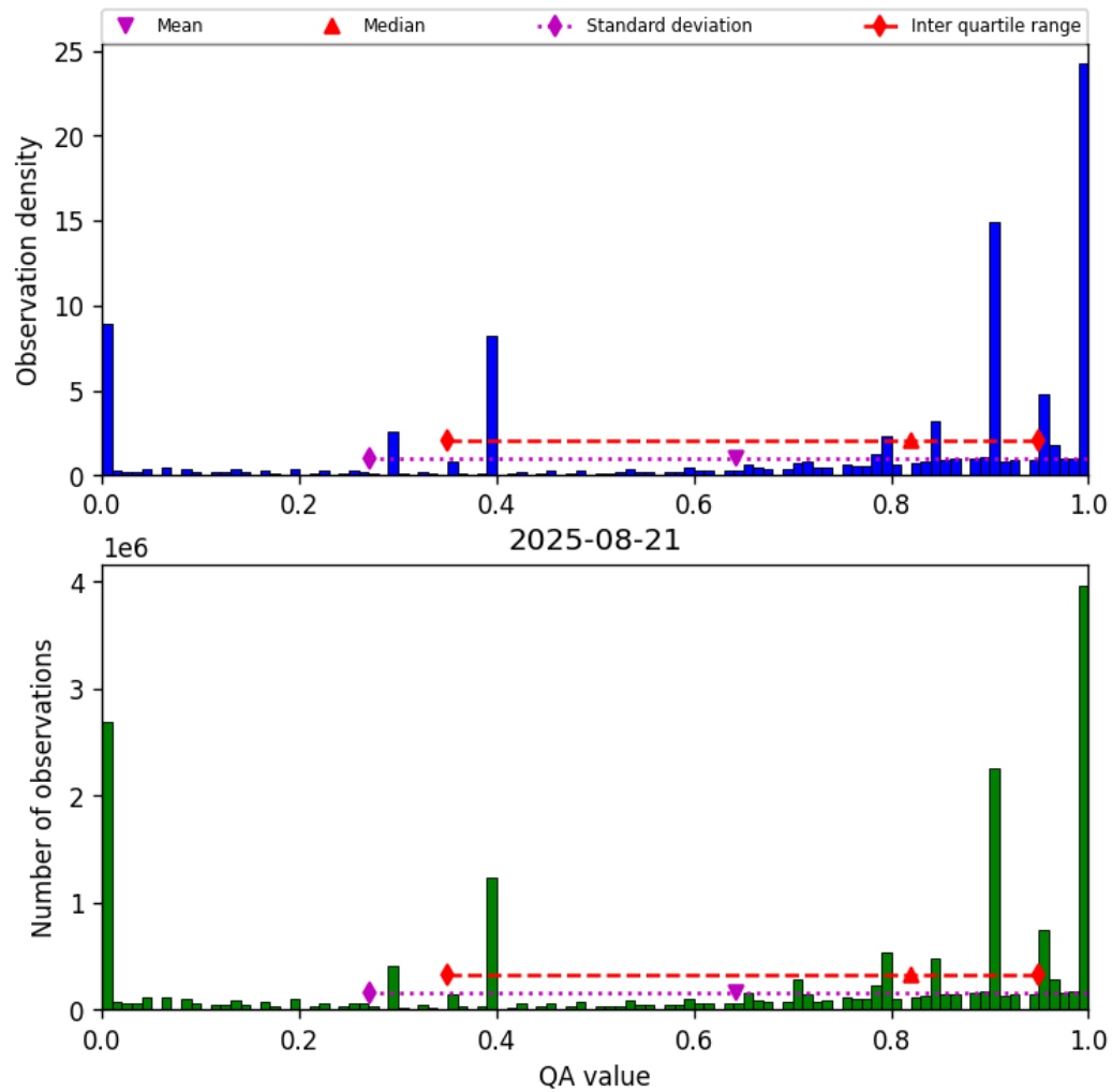
Figure 36: Histogram of “QA value” for 2025-08-21 to 2025-08-22
