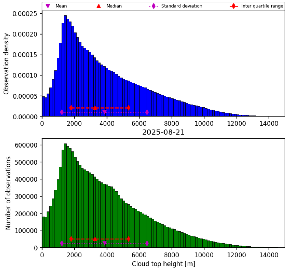
Figure 38: Histogram of “Cloud top height” for 2025-08-21 to 2025-08-22
