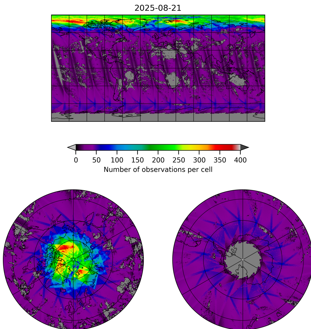
Figure 19: Map of the number of observations for 2025-08-21 to 2025-08-22
