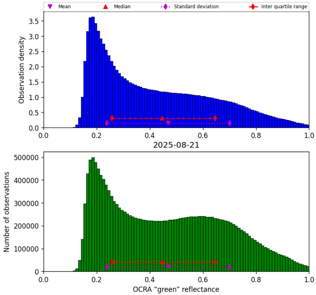
Figure 50: Histogram of “OCRA “green” reflectance” for 2025-08-21 to 2025-08-22
