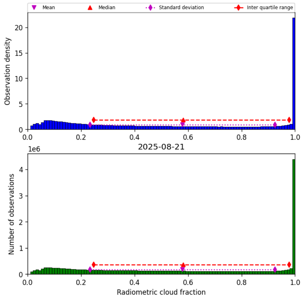
Figure 37: Histogram of “Radiometric cloud fraction” for 2025-08-21 to 2025-08-22
