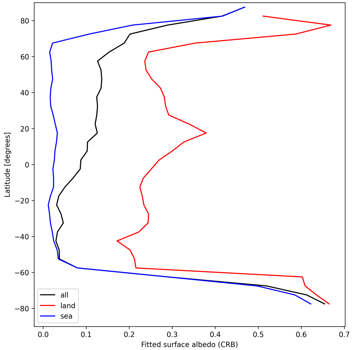
Figure 28: Zonal average of “Fitted surface albedo (CRB)” for 2025-08-21 to 2025-08-22.
