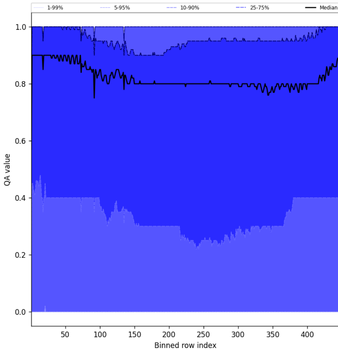
Figure 52: Along track statistics of “QA value” for 2025-08-21 to 2025-08-22
