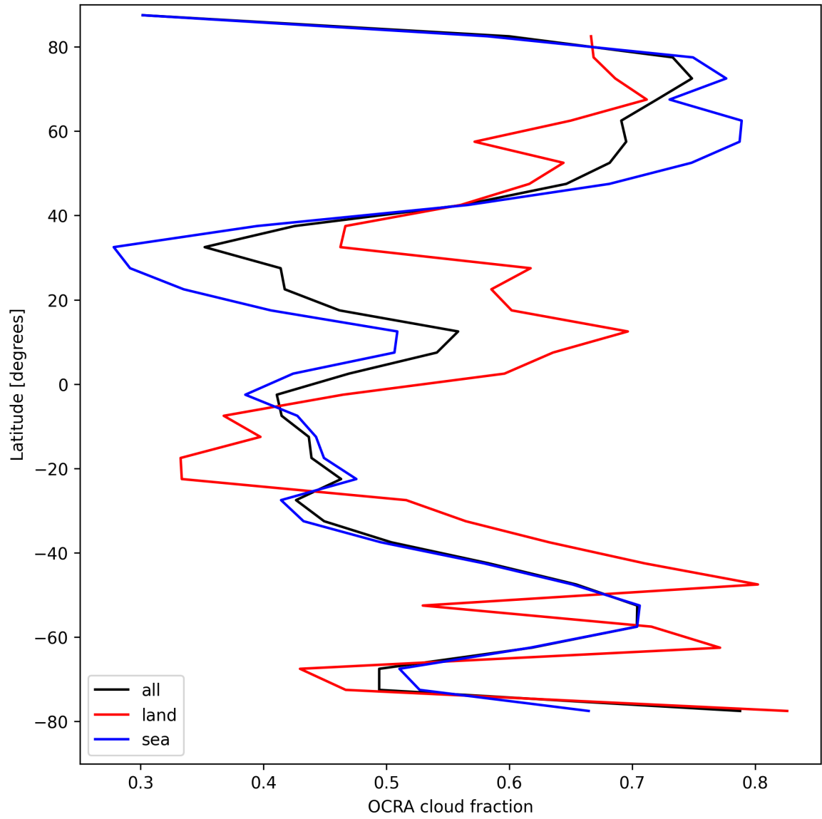
Figure 32: Zonal average of “OCRA cloud fraction” for 2025-08-21 to 2025-08-22.
