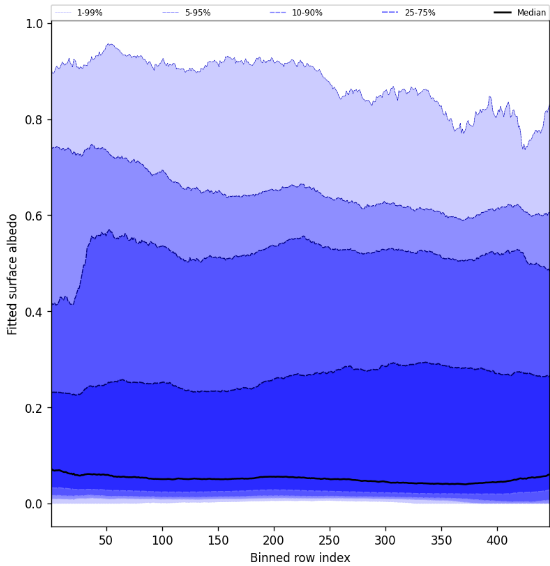
Figure 59: Along track statistics of “Fitted surface albedo” for 2025-08-21 to 2025-08-22
