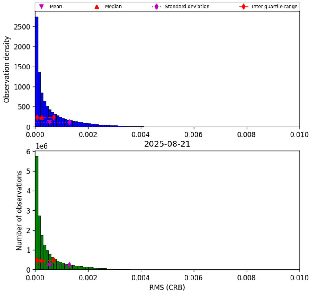
Figure 46: Histogram of “RMS (CRB)” for 2025-08-21 to 2025-08-22
