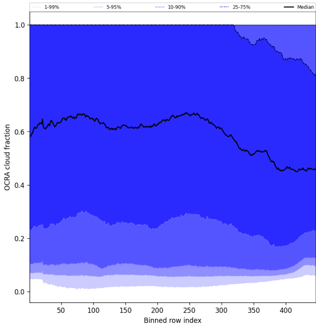
Figure 64: Along track statistics of “OCRA cloud fraction” for 2025-08-21 to 2025-08-22
