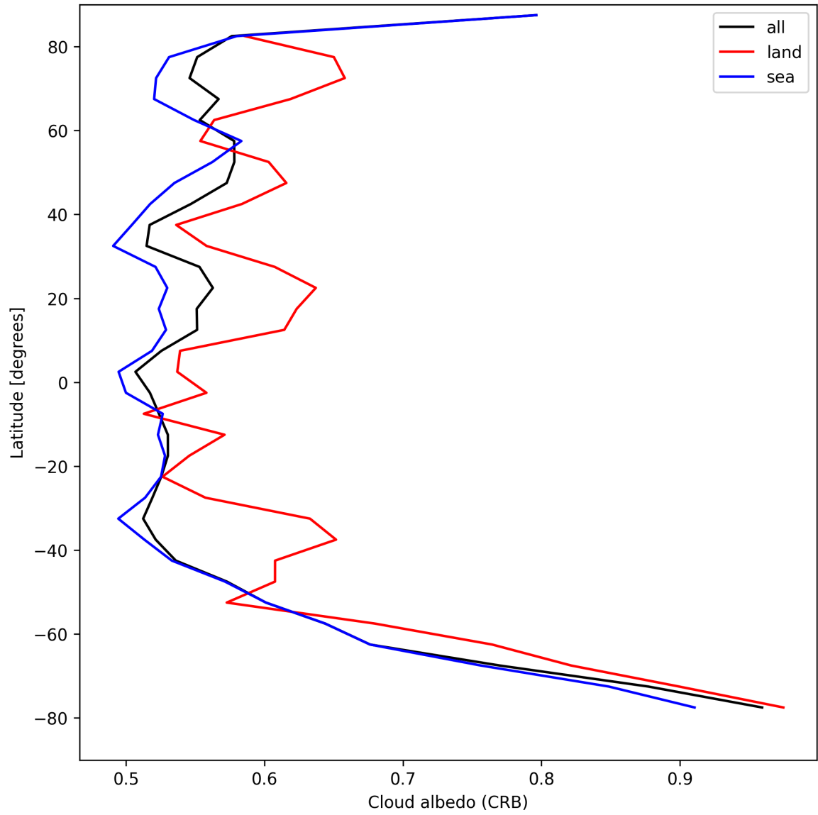
Figure 26: Zonal average of “Cloud albedo (CRB)” for 2025-08-21 to 2025-08-22.
