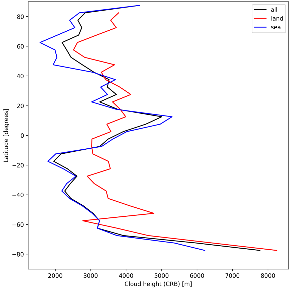
Figure 25: Zonal average of “Cloud height (CRB)” for 2025-08-21 to 2025-08-22.
