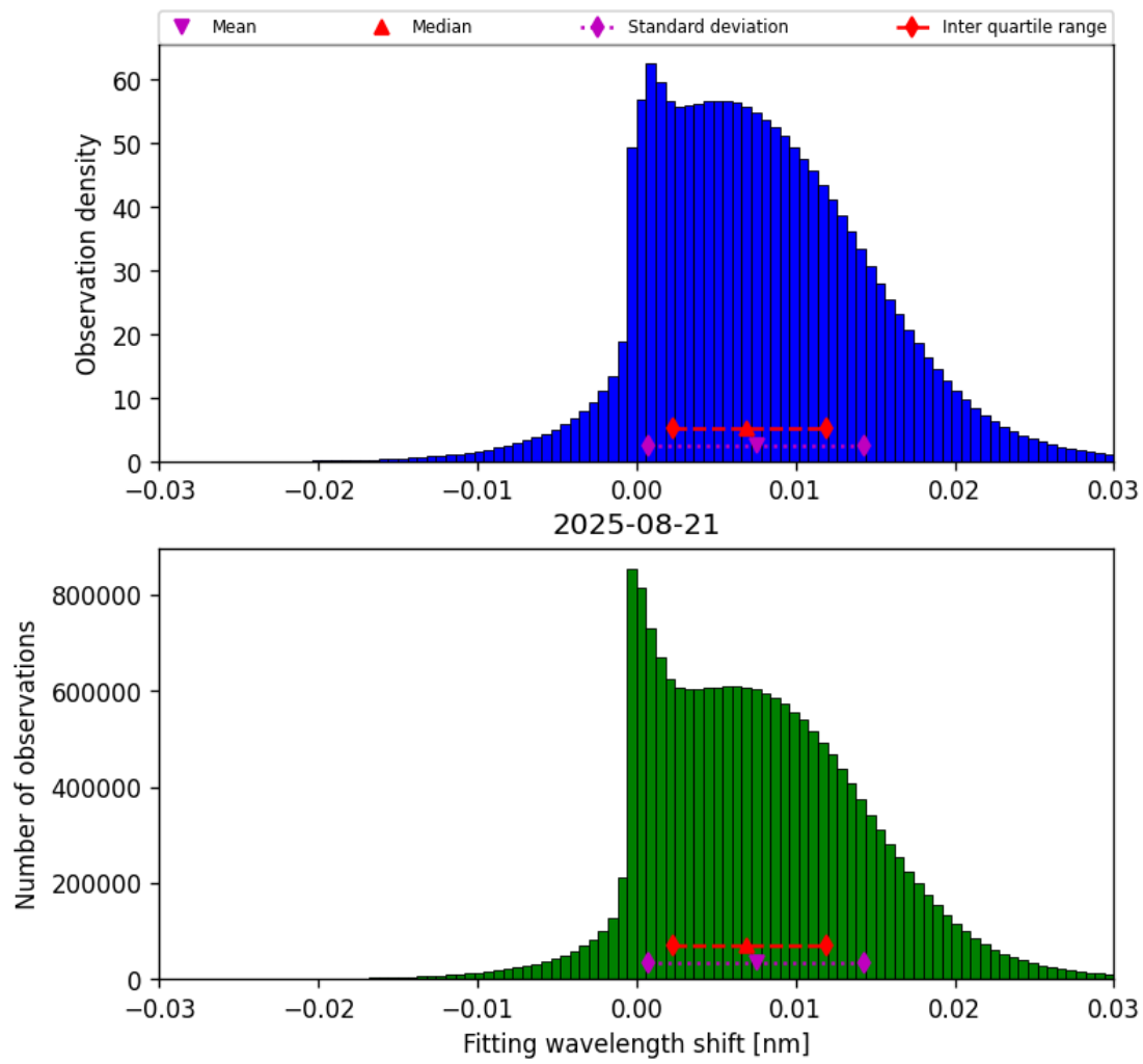
Figure 47: Histogram of “Fitting wavelength shift” for 2025-08-21 to 2025-08-22
