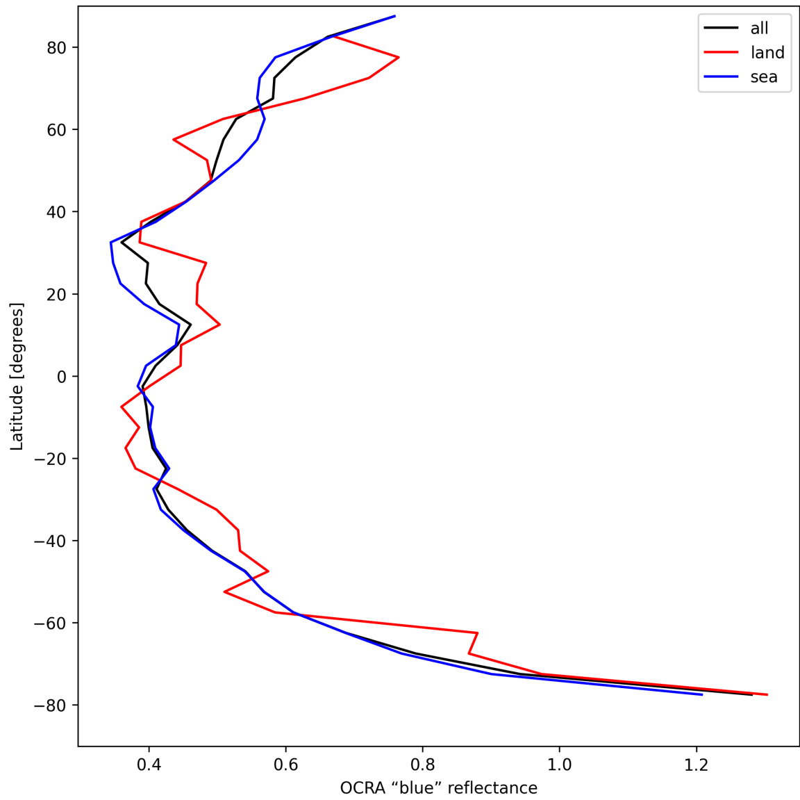
Figure 33: Zonal average of “OCRA “blue” reflectance” for 2025-08-21 to 2025-08-22.
