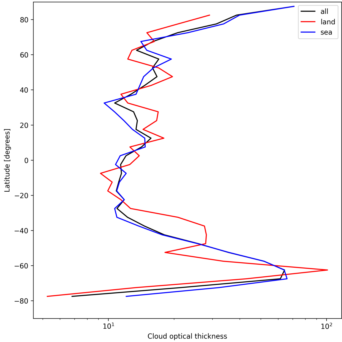
Figure 23: Zonal average of “Cloud optical thickness” for 2025-08-21 to 2025-08-22.
