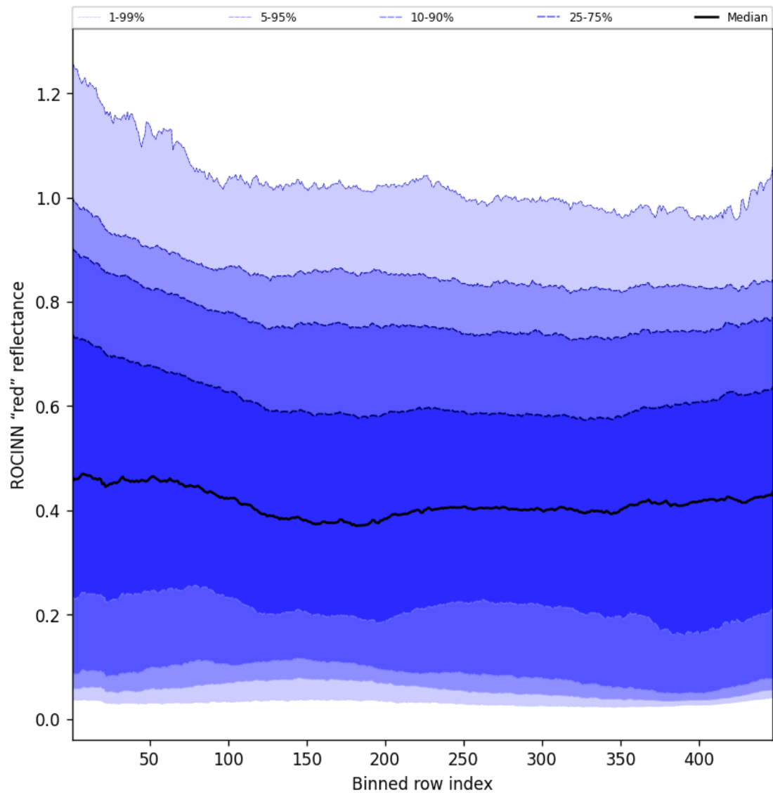
Figure 67: Along track statistics of “ROCINN “red” reflectance” for 2025-08-21 to 2025-08-22
