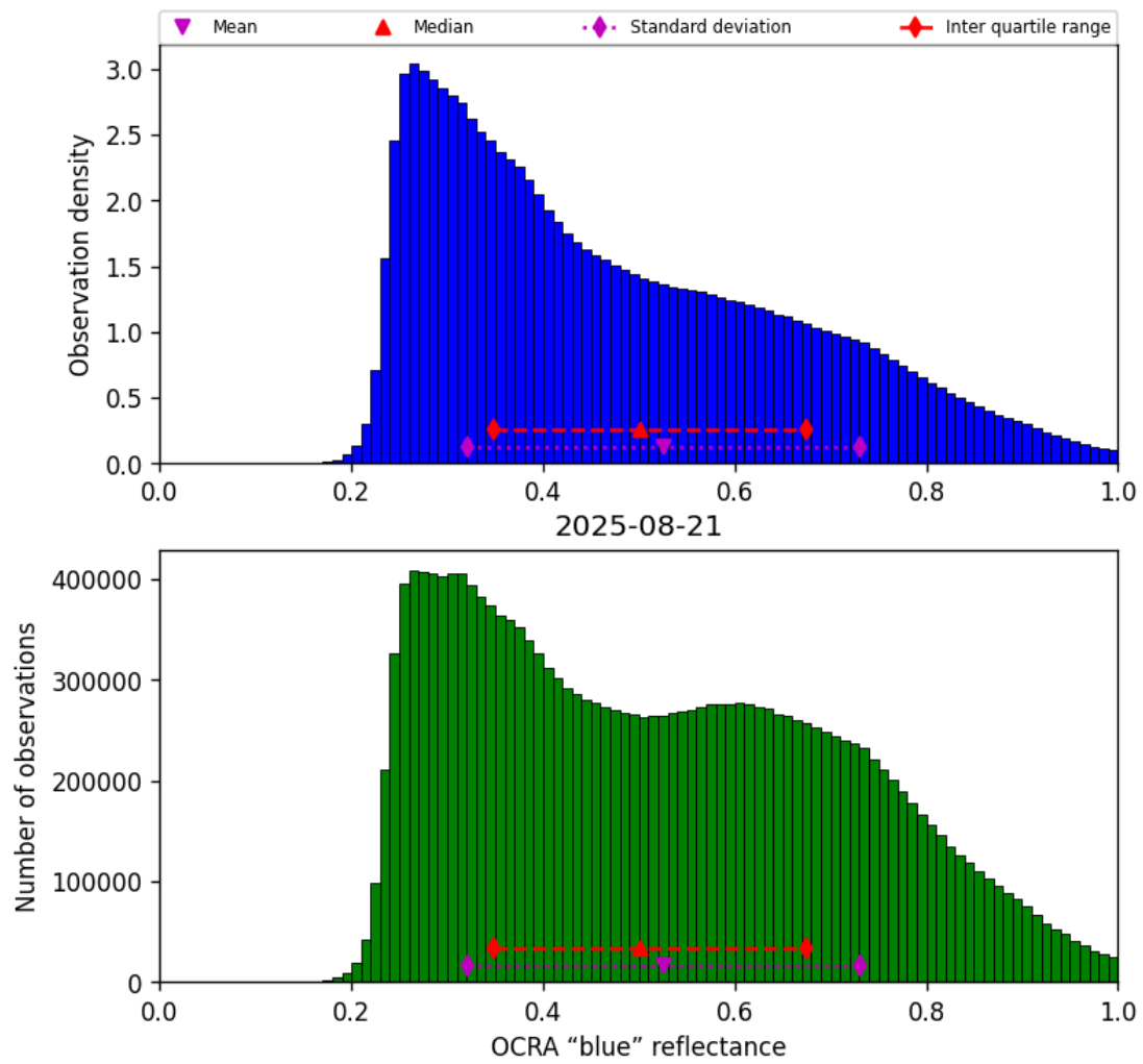
Figure 49: Histogram of “OCRA “blue” reflectance” for 2025-08-21 to 2025-08-22
