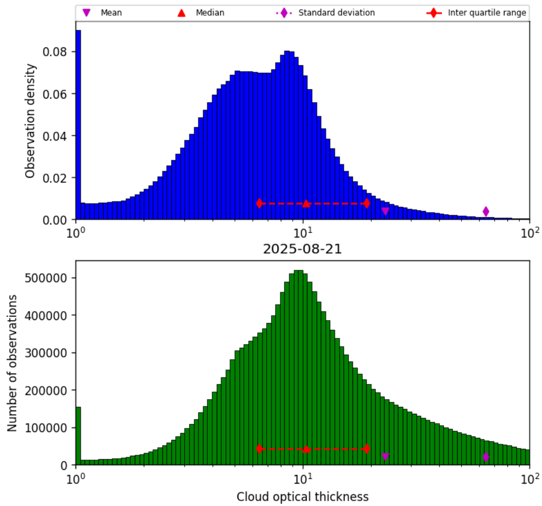
Figure 39: Histogram of “Cloud optical thickness” for 2025-08-21 to 2025-08-22
