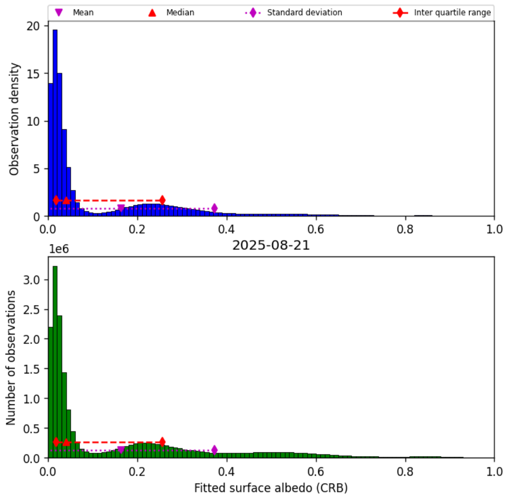
Figure 44: Histogram of “Fitted surface albedo (CRB)” for 2025-08-21 to 2025-08-22
