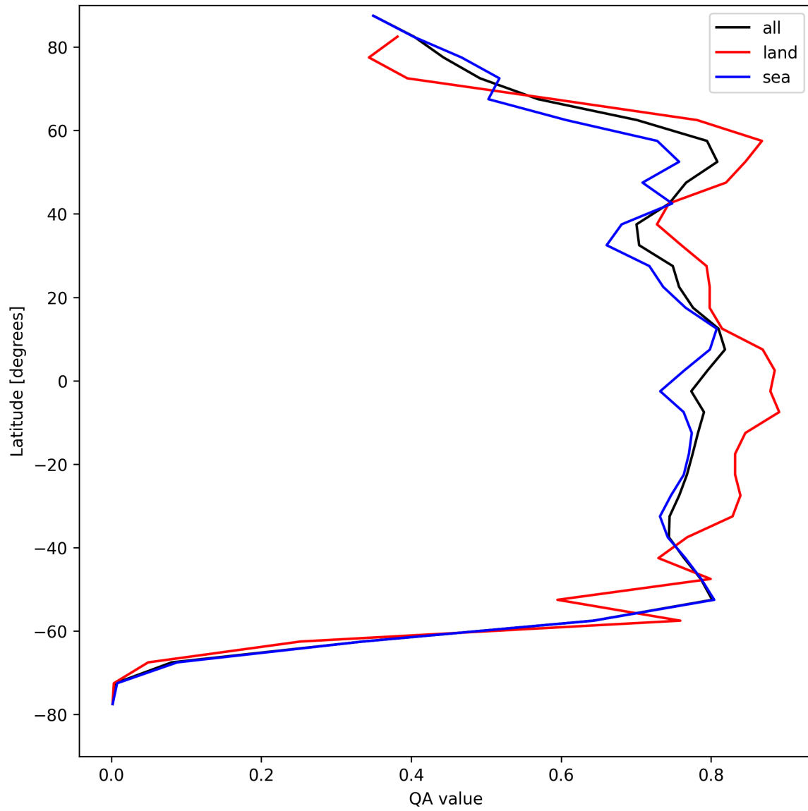
Figure 20: Zonal average of “QA value” for 2025-08-21 to 2025-08-22.
