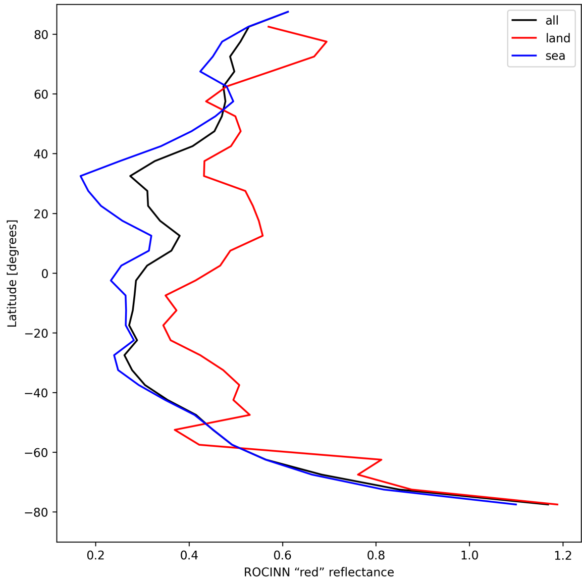
Figure 35: Zonal average of “ROCINN “red” reflectance” for 2025-08-21 to 2025-08-22.
