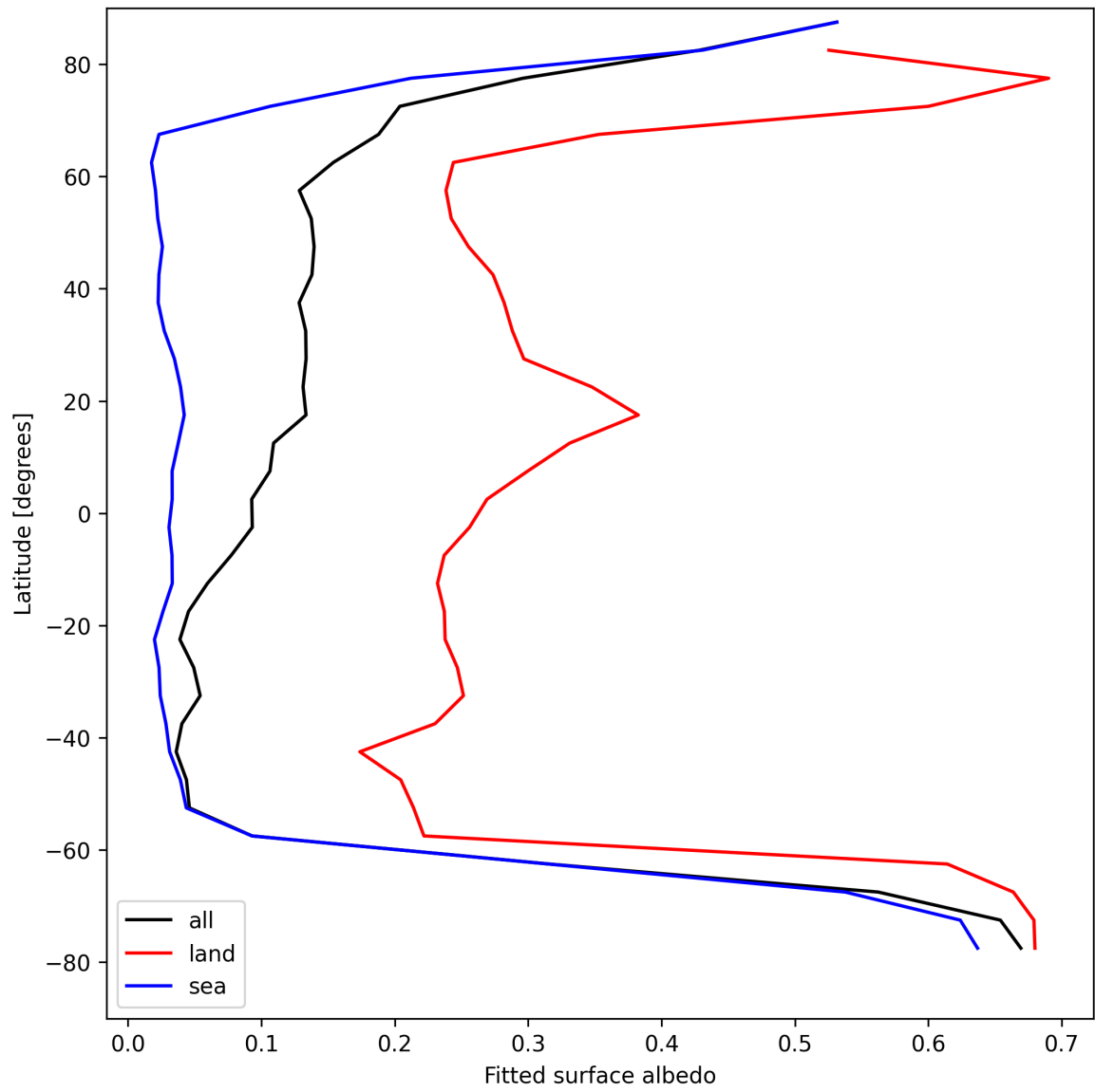
Figure 27: Zonal average of “Fitted surface albedo” for 2025-08-21 to 2025-08-22.
