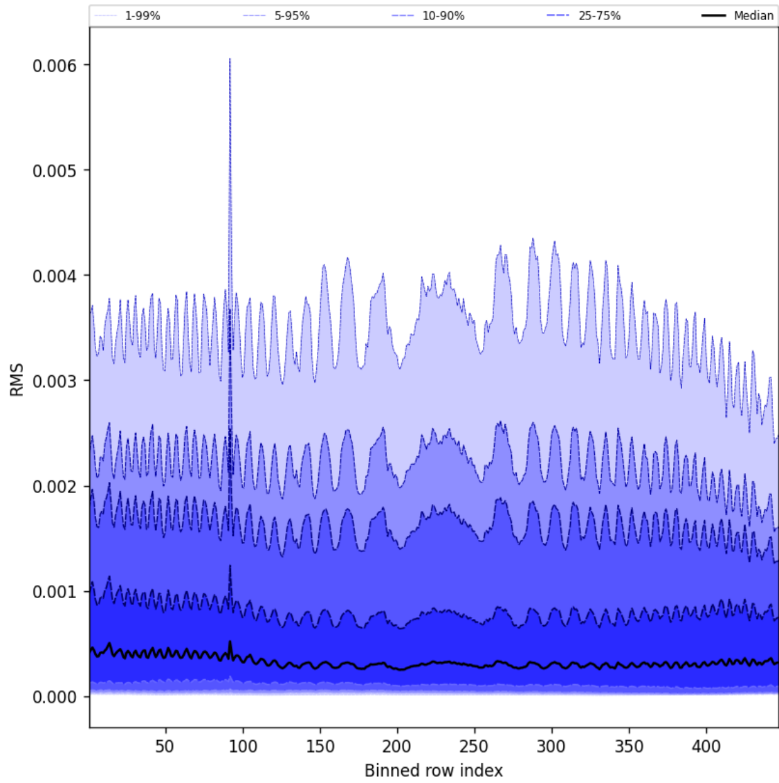
Figure 61: Along track statistics of “RMS” for 2025-08-21 to 2025-08-22
