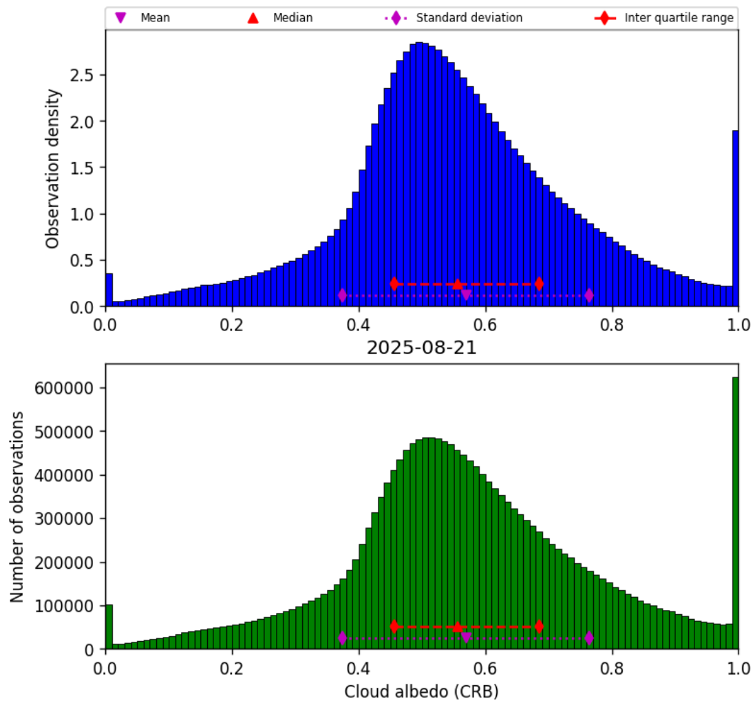
Figure 42: Histogram of “Cloud albedo (CRB)” for 2025-08-21 to 2025-08-22
