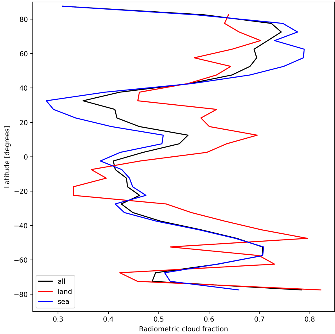
Figure 21: Zonal average of “Radiometric cloud fraction” for 2025-08-21 to 2025-08-22.
