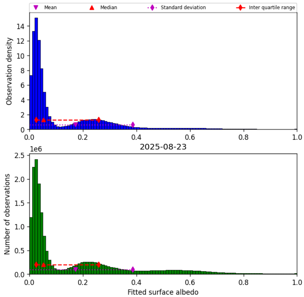
Figure 43: Histogram of “Fitted surface albedo” for 2025-08-23 to 2025-08-23
