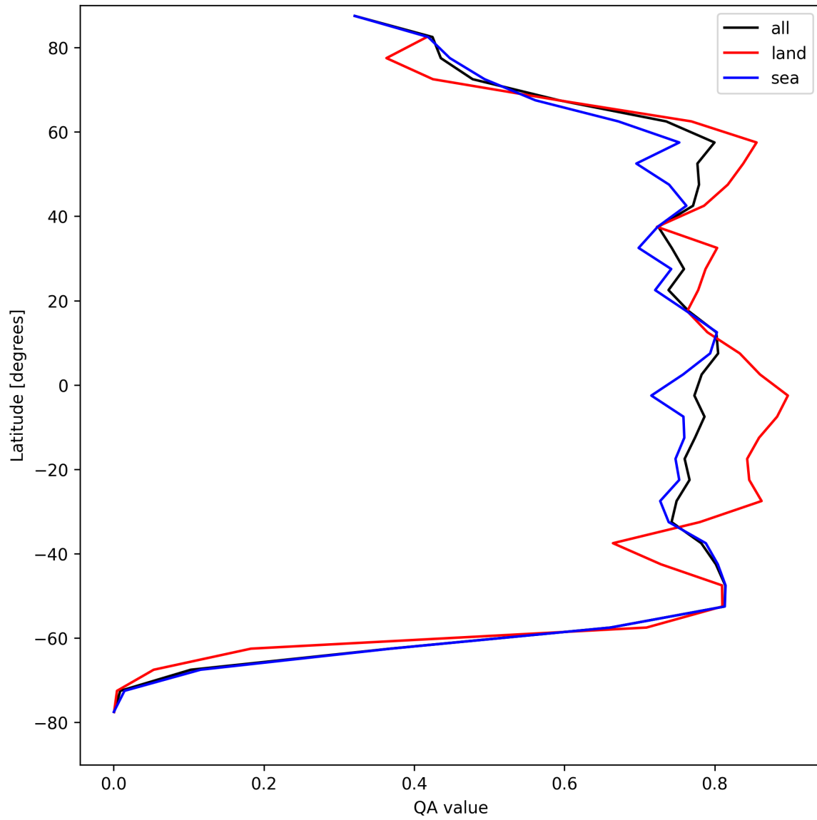
Figure 20: Zonal average of “QA value” for 2025-08-23 to 2025-08-23.
