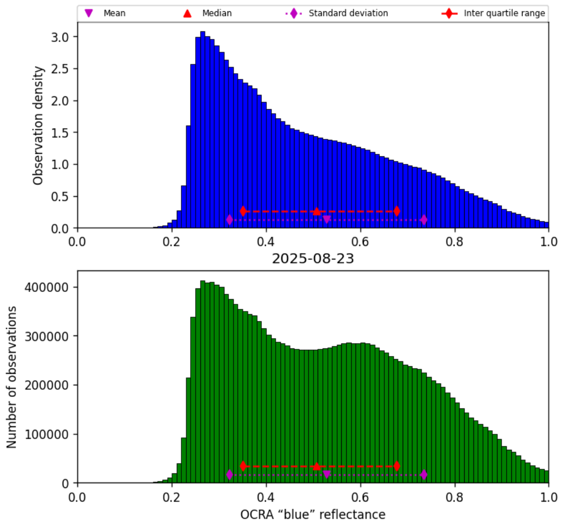
Figure 49: Histogram of “OCRA “blue” reflectance” for 2025-08-23 to 2025-08-23
