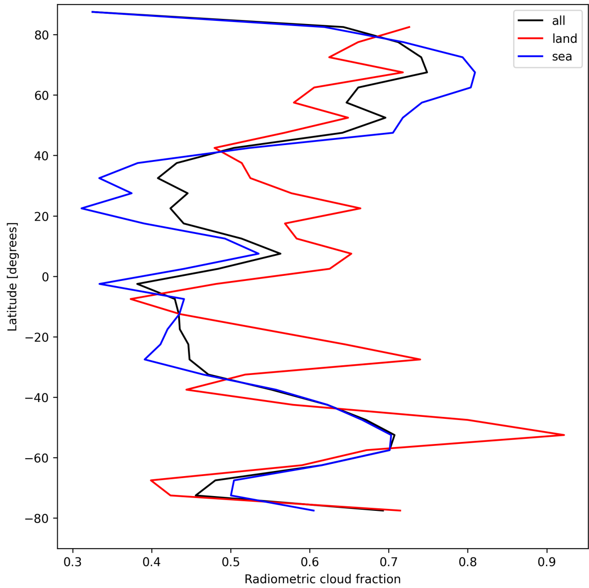
Figure 21: Zonal average of “Radiometric cloud fraction” for 2025-08-23 to 2025-08-23.
