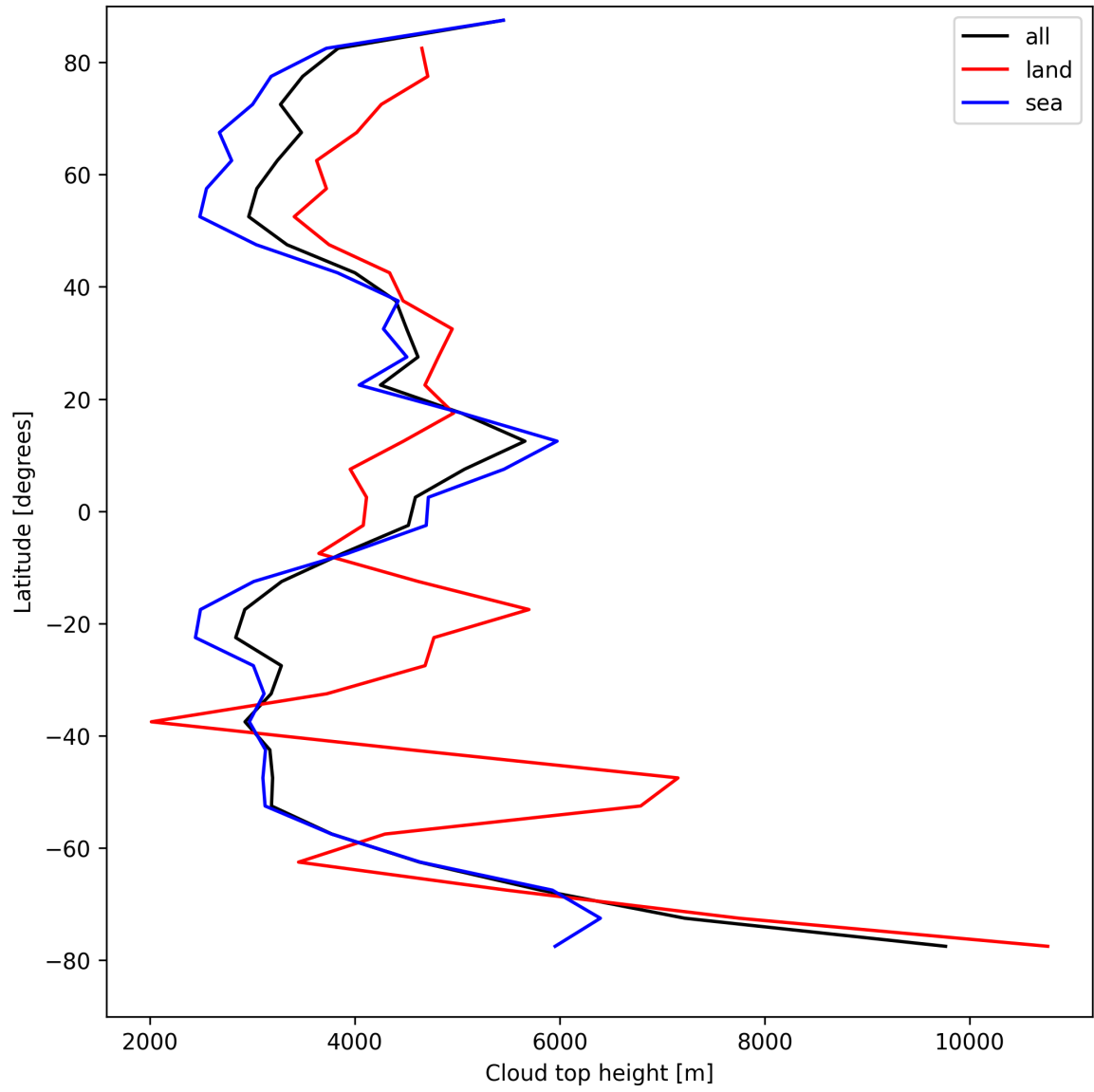
Figure 22: Zonal average of “Cloud top height” for 2025-08-23 to 2025-08-23.
