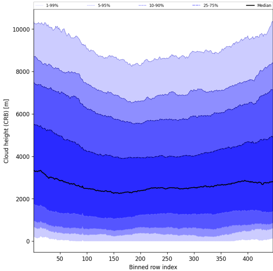
Figure 57: Along track statistics of “Cloud height (CRB)” for 2025-08-23 to 2025-08-23
