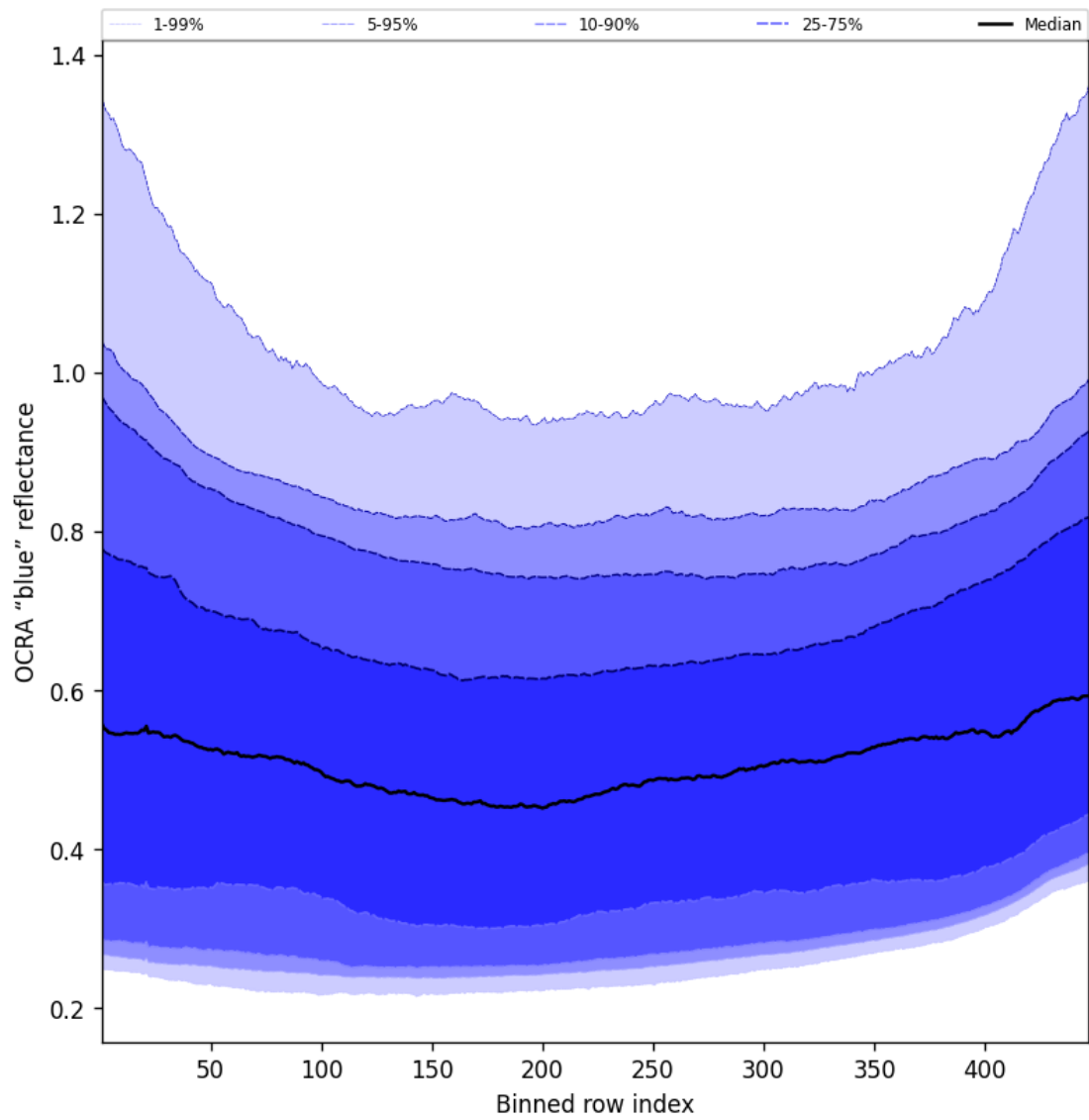
Figure 65: Along track statistics of “OCRA “blue” reflectance” for 2025-08-23 to 2025-08-23
