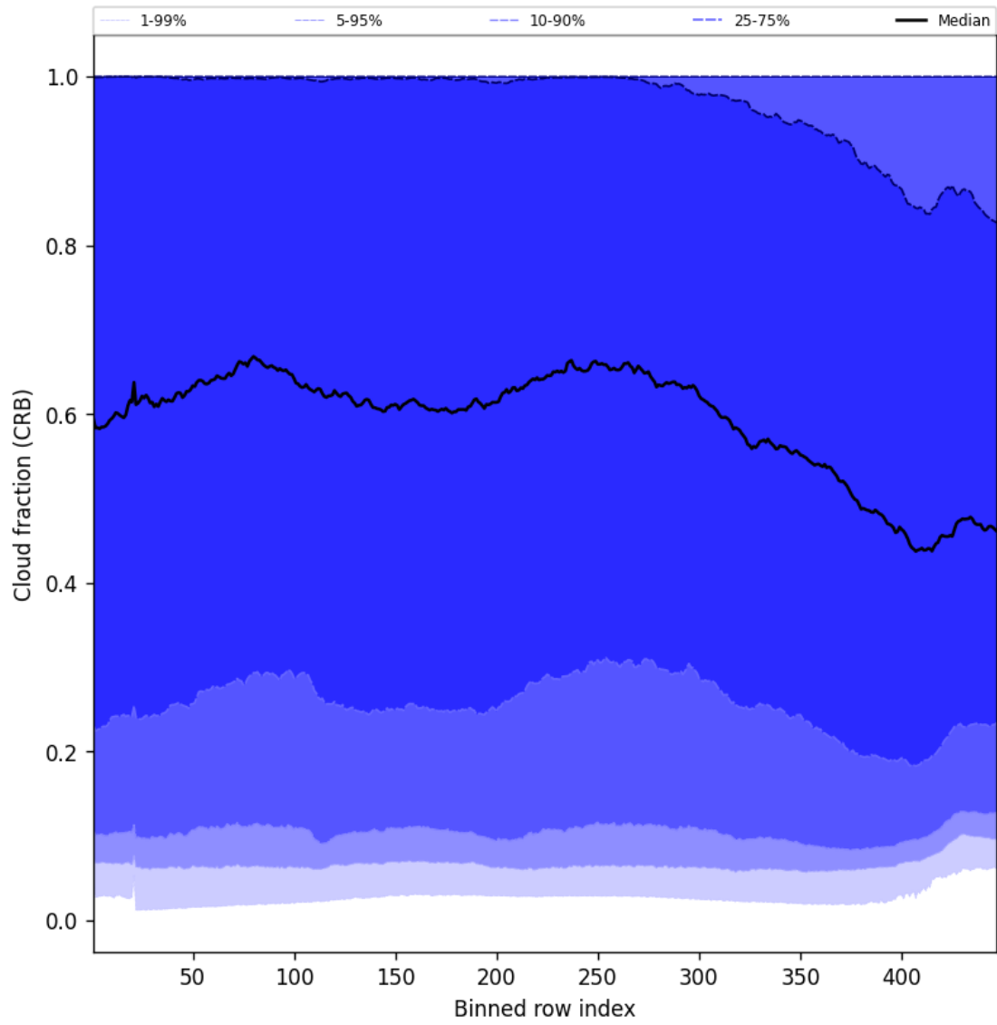
Figure 56: Along track statistics of “Cloud fraction (CRB)” for 2025-08-23 to 2025-08-23
