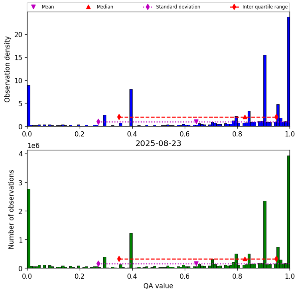
Figure 36: Histogram of “QA value” for 2025-08-23 to 2025-08-23
