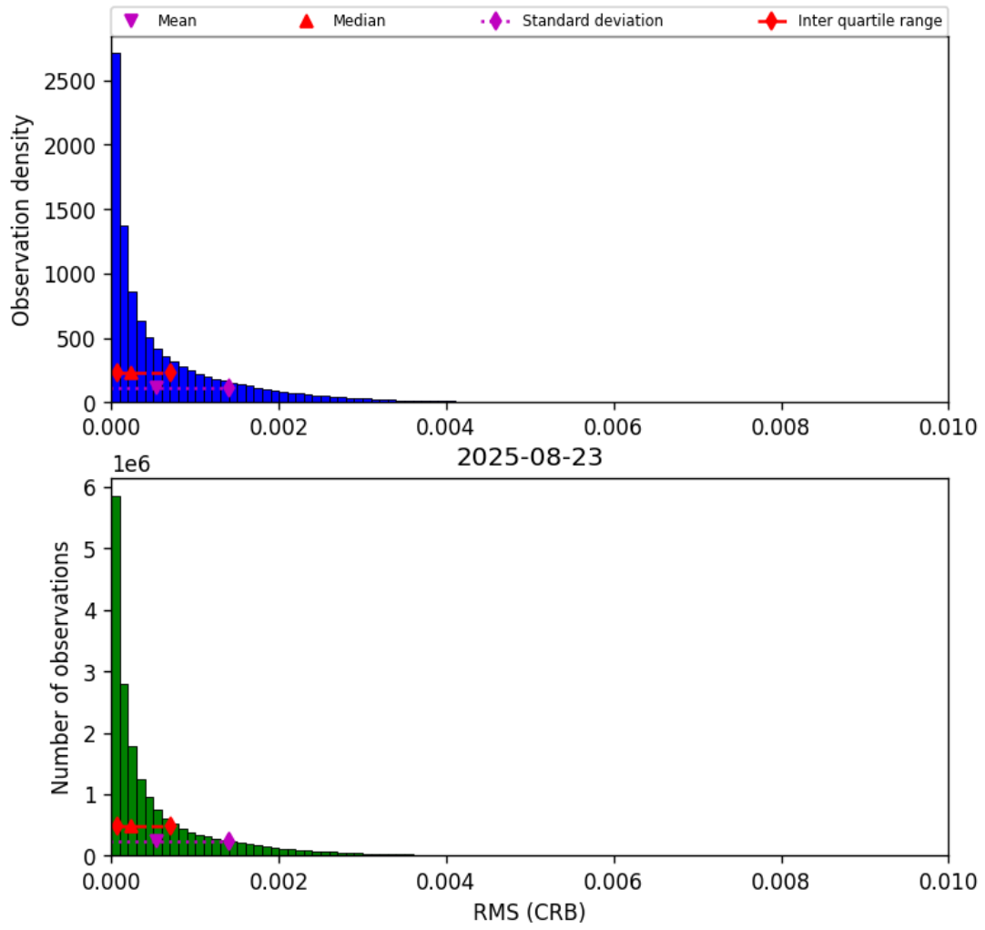
Figure 46: Histogram of “RMS (CRB)” for 2025-08-23 to 2025-08-23
