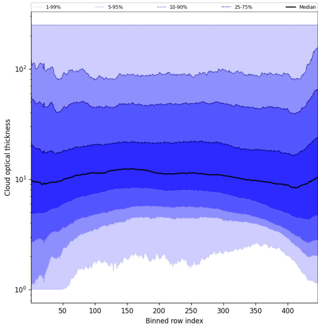
Figure 55: Along track statistics of “Cloud optical thickness” for 2025-08-23 to 2025-08-23
