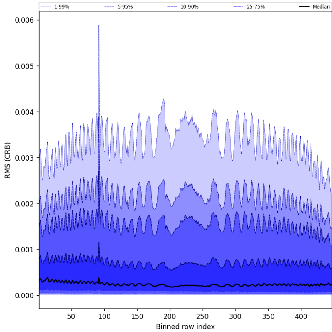
Figure 62: Along track statistics of “RMS (CRB)” for 2025-08-23 to 2025-08-23
