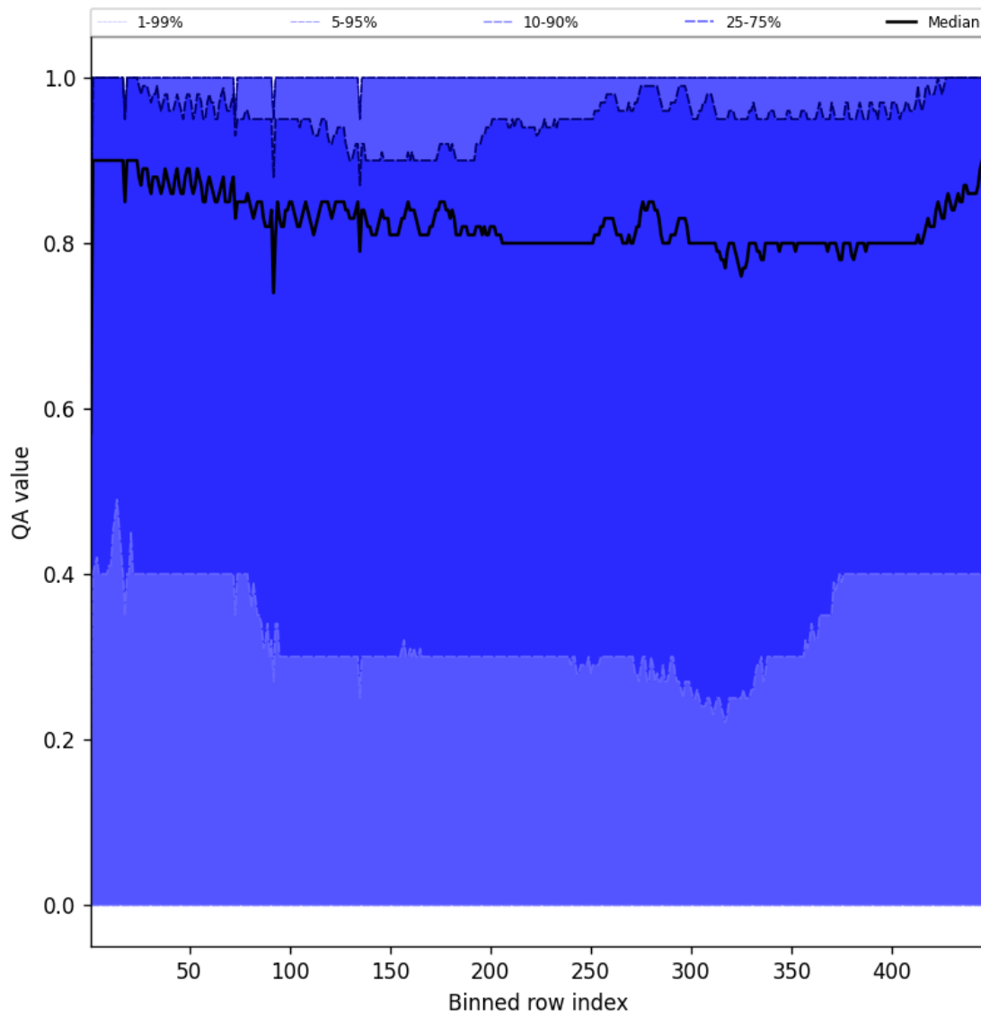
Figure 52: Along track statistics of "QA value" for 2025-08-23 to 2025-08-23
