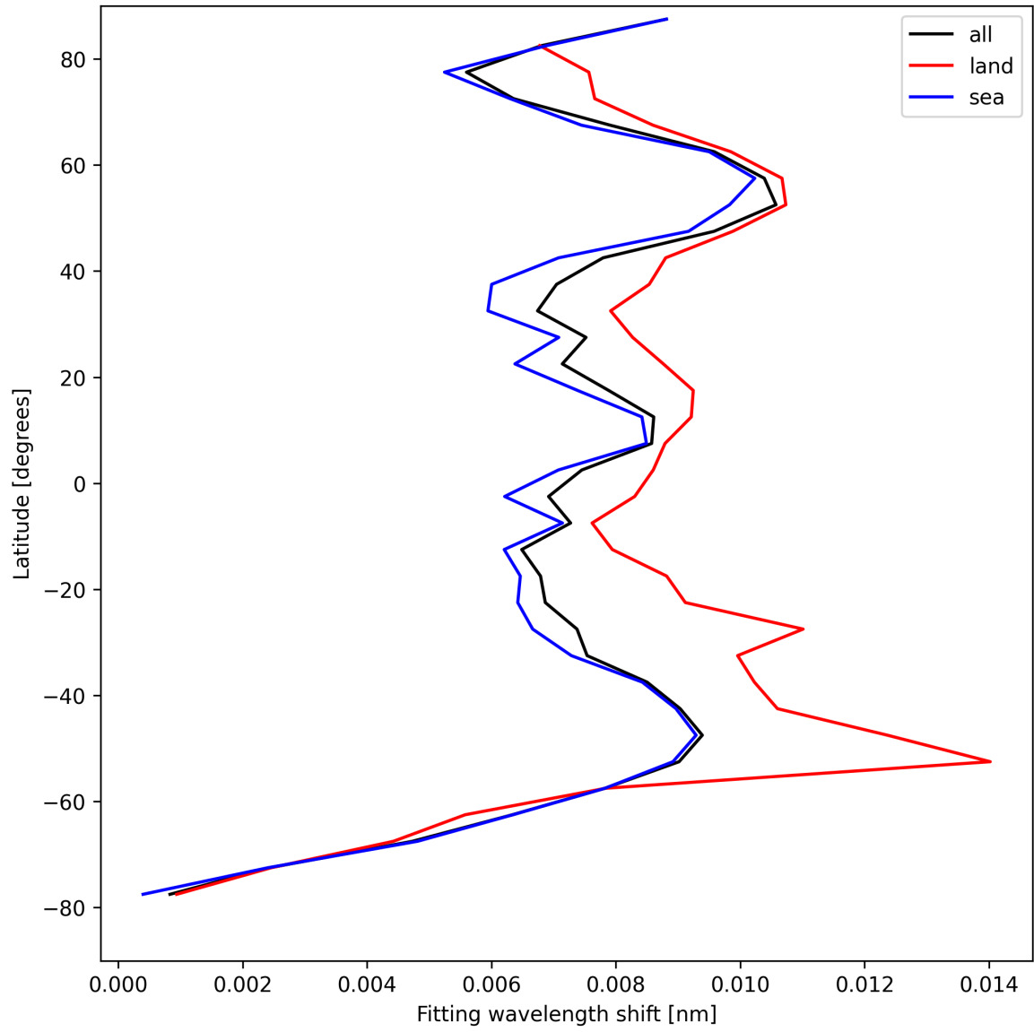
Figure 31: Zonal average of “Fitting wavelength shift” for 2025-08-23 to 2025-08-23.
