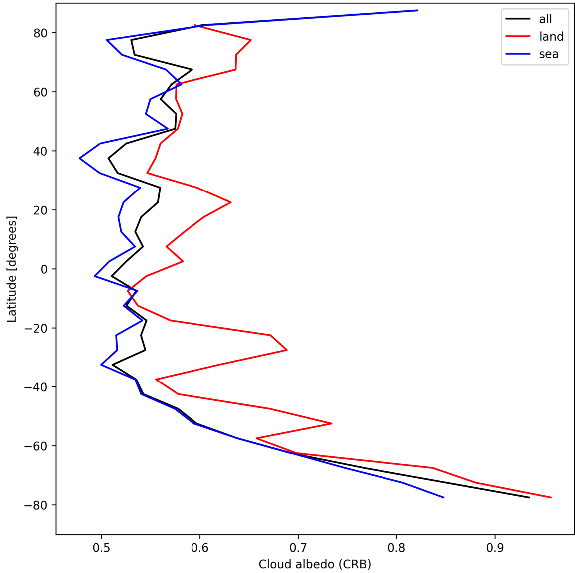
Figure 26: Zonal average of “Cloud albedo (CRB)” for 2025-08-23 to 2025-08-23.
