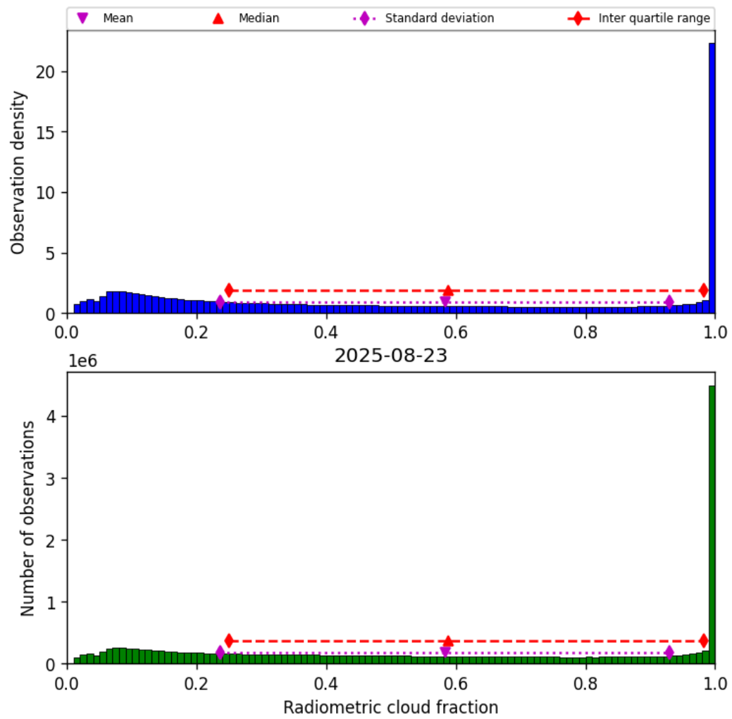
Figure 37: Histogram of “Radiometric cloud fraction” for 2025-08-23 to 2025-08-23
