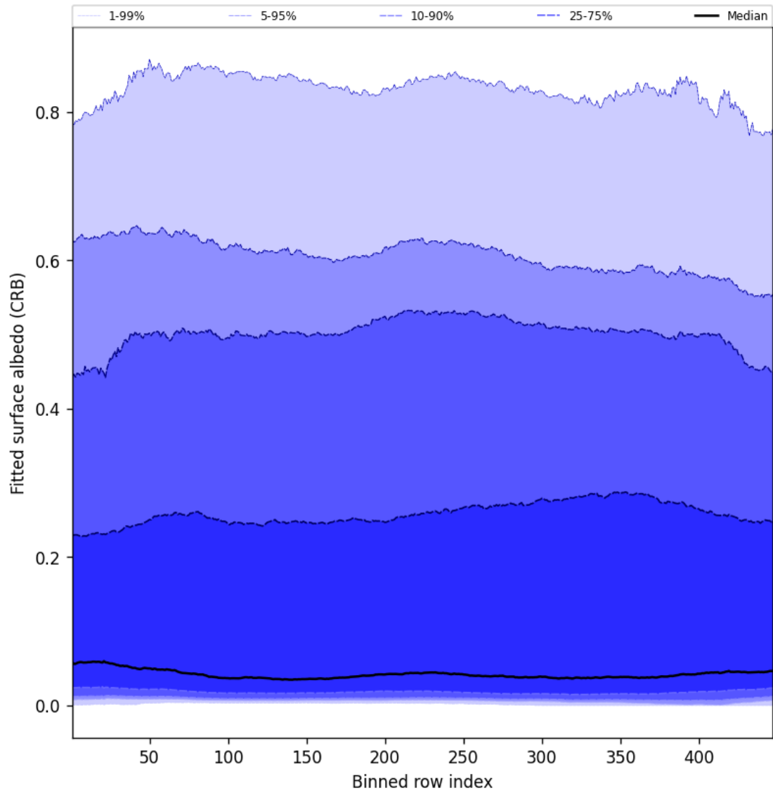
Figure 60: Along track statistics of “Fitted surface albedo (CRB)” for 2025-08-23 to 2025-08-23
