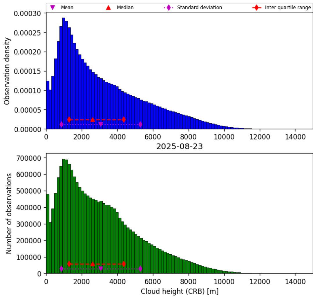
Figure 41: Histogram of “Cloud height (CRB)” for 2025-08-23 to 2025-08-23
