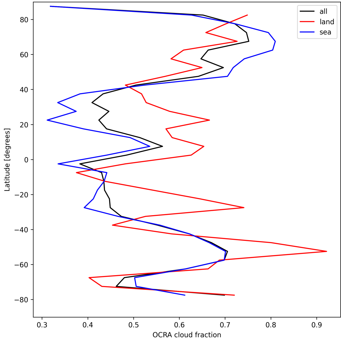
Figure 32: Zonal average of “OCRA cloud fraction” for 2025-08-23 to 2025-08-23.
