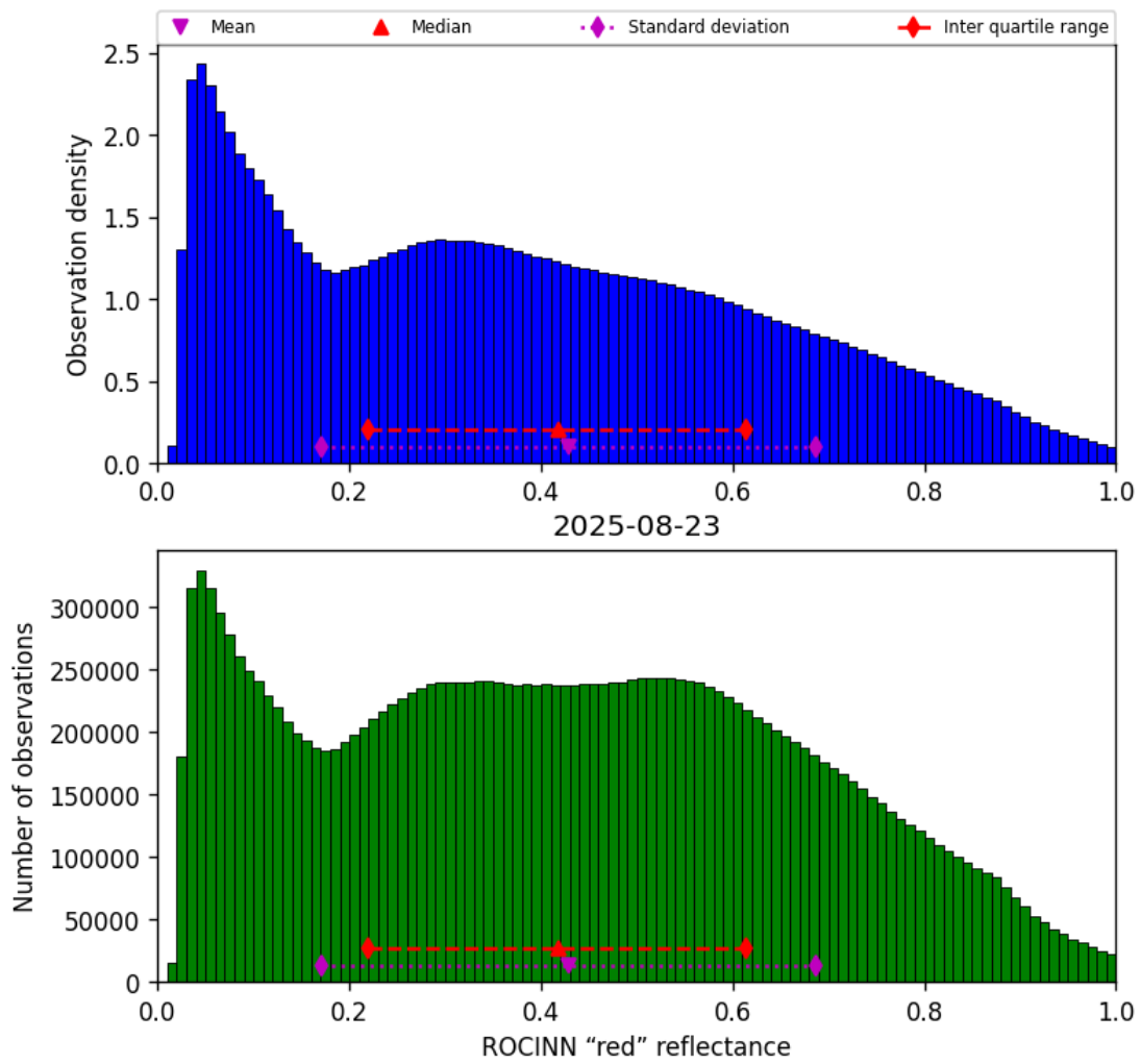
Figure 51: Histogram of “ROCINN “red” reflectance” for 2025-08-23 to 2025-08-23
