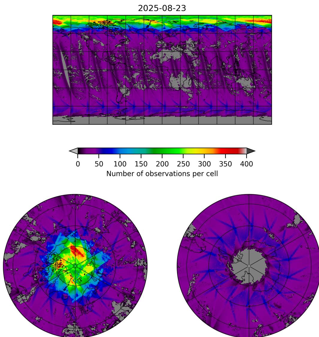
Figure 19: Map of the number of observations for 2025-08-23 to 2025-08-23
