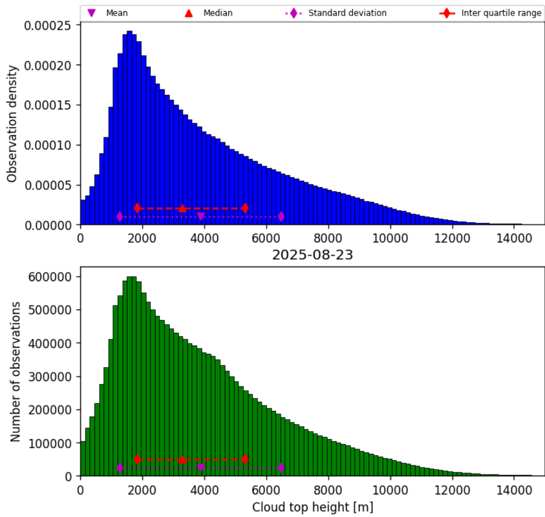
Figure 38: Histogram of “Cloud top height” for 2025-08-23 to 2025-08-23
