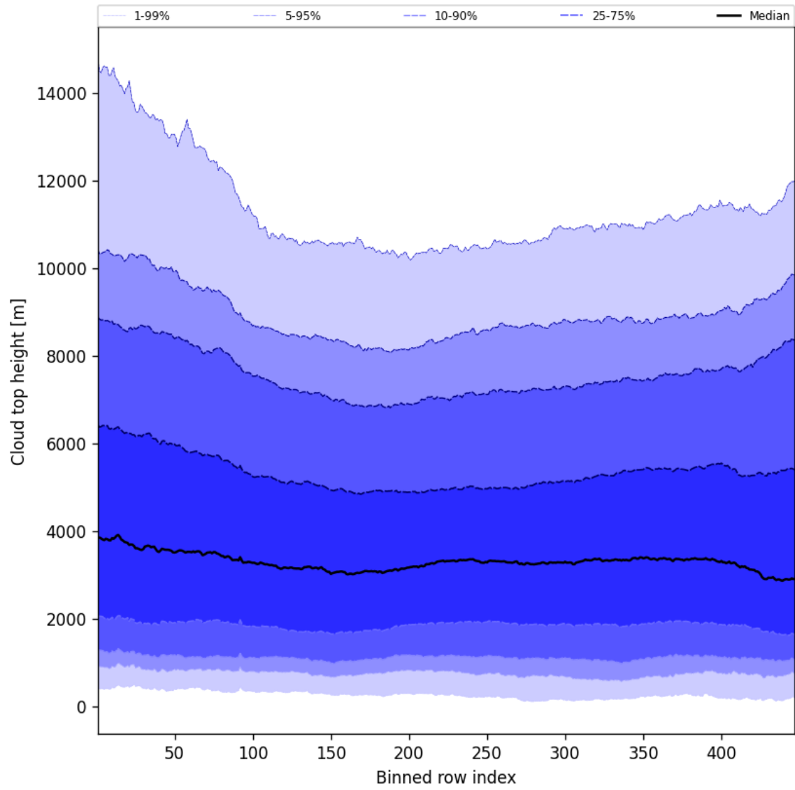
Figure 54: Along track statistics of “Cloud top height” for 2025-08-23 to 2025-08-23
