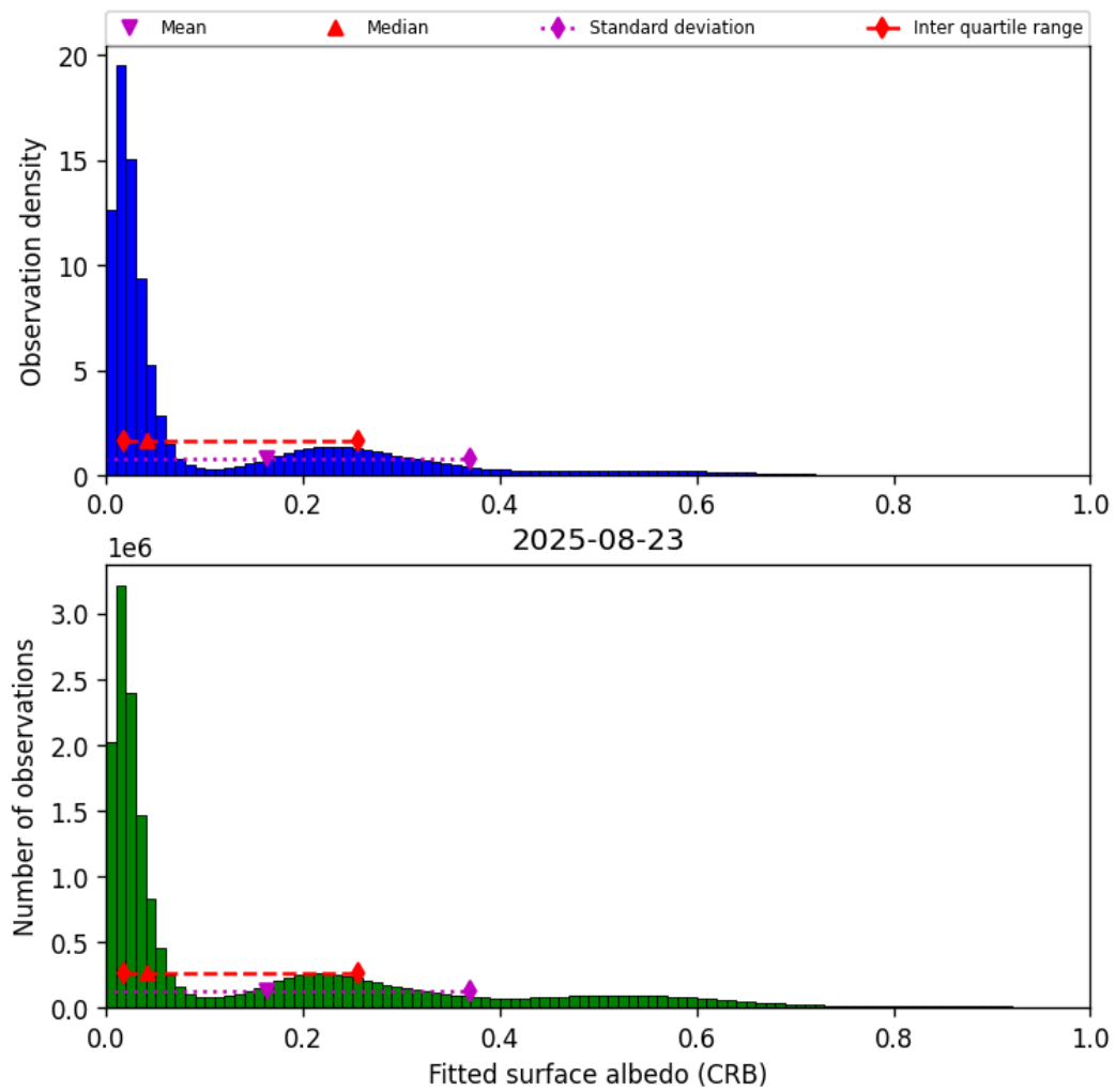
Figure 44: Histogram of “Fitted surface albedo (CRB)” for 2025-08-23 to 2025-08-23
