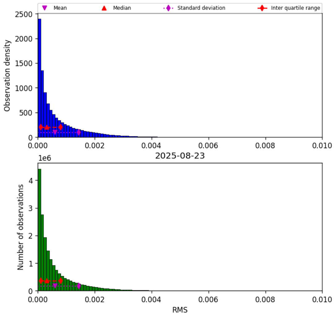
Figure 45: Histogram of “RMS” for 2025-08-23 to 2025-08-23
