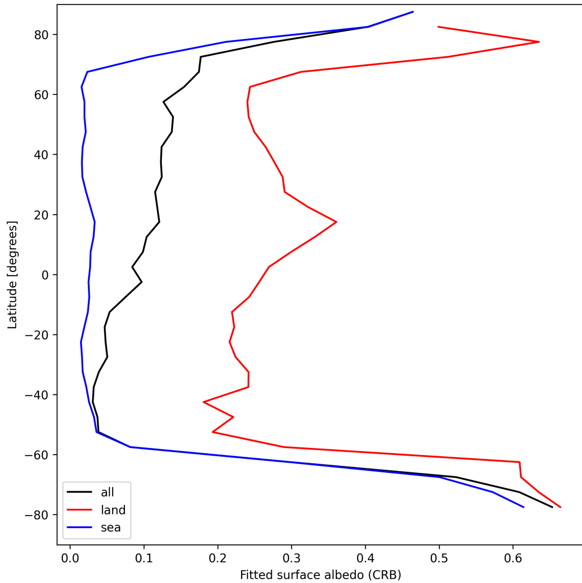
Figure 28: Zonal average of “Fitted surface albedo (CRB)” for 2025-08-23 to 2025-08-23.
