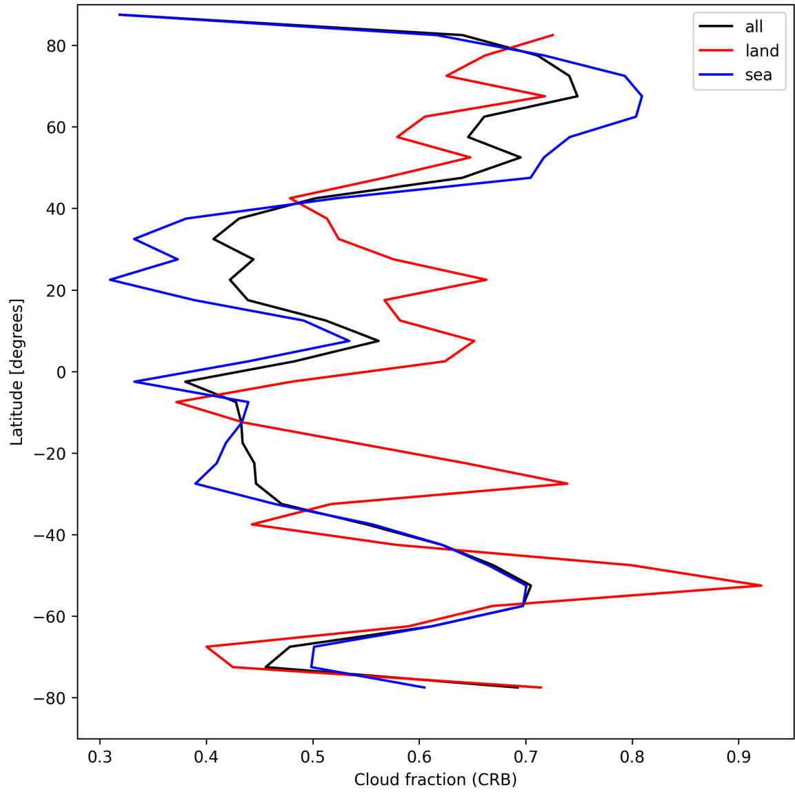
Figure 24: Zonal average of “Cloud fraction (CRB)” for 2025-08-23 to 2025-08-23.
