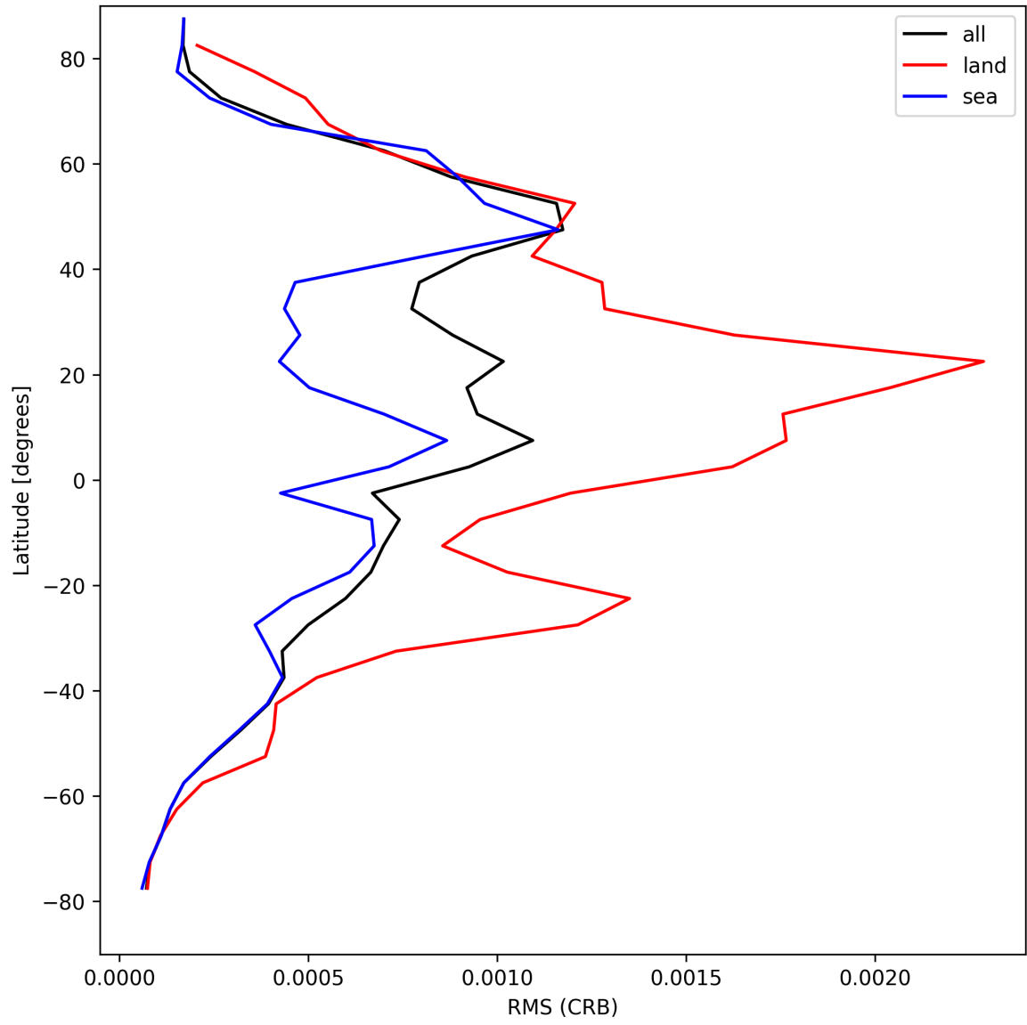
Figure 30: Zonal average of “RMS (CRB)” for 2025-08-23 to 2025-08-23.
