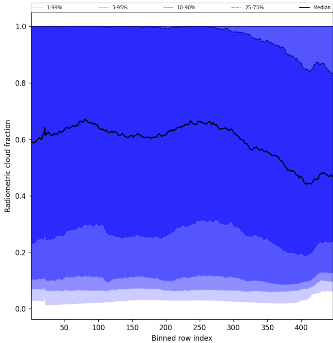
Figure 53: Along track statistics of “Radiometric cloud fraction” for 2025-08-23 to 2025-08-23
