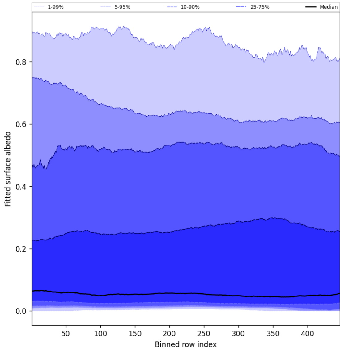
Figure 59: Along track statistics of “Fitted surface albedo” for 2025-08-23 to 2025-08-23
