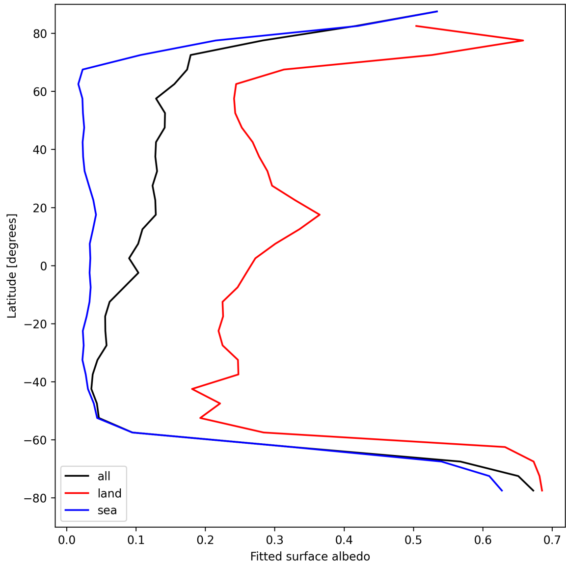
Figure 27: Zonal average of “Fitted surface albedo” for 2025-08-23 to 2025-08-23.
