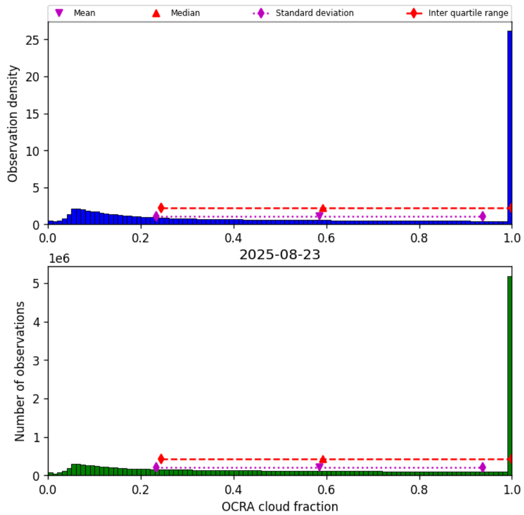
Figure 48: Histogram of “OCRA cloud fraction” for 2025-08-23 to 2025-08-23
