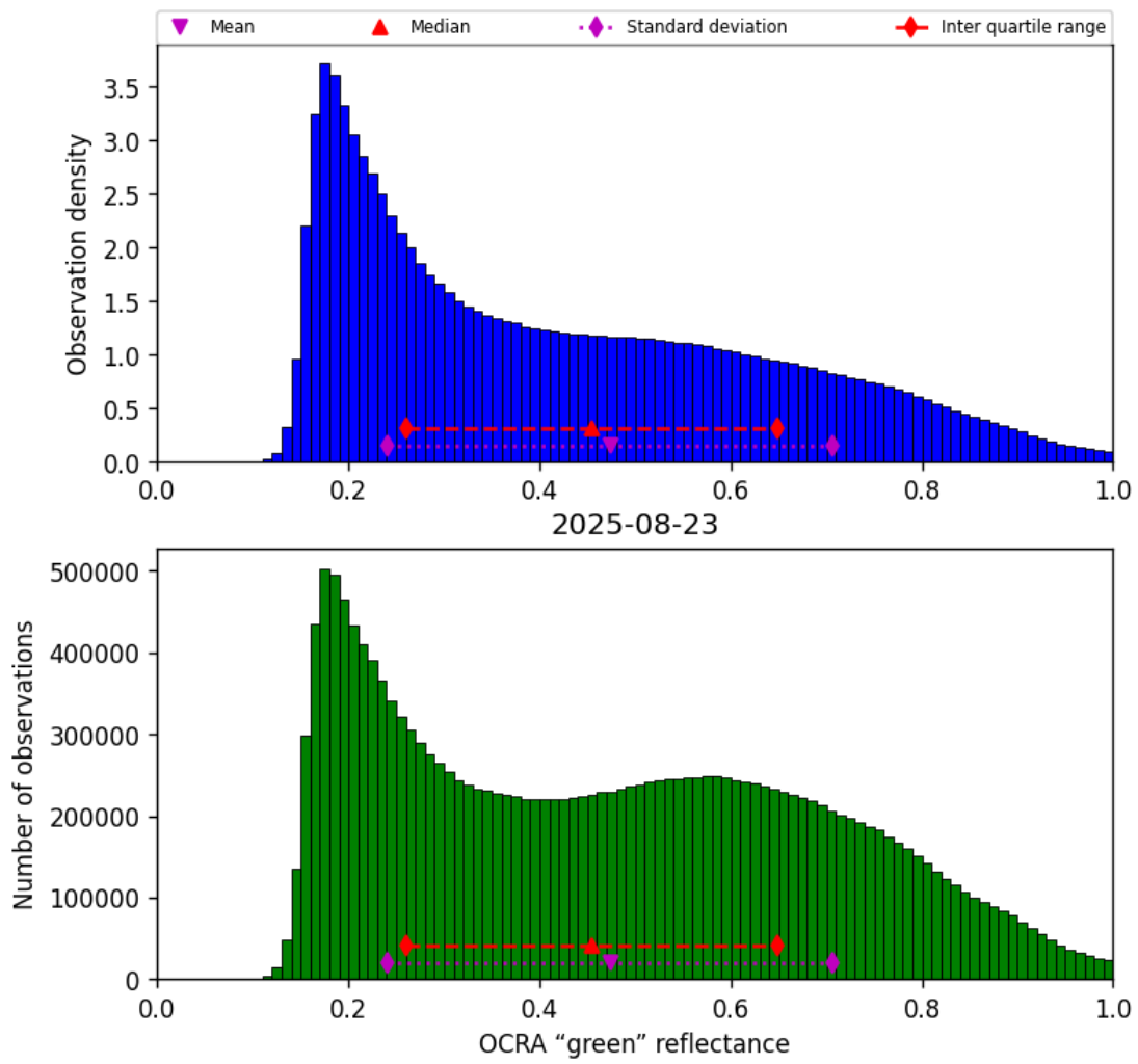
Figure 50: Histogram of “OCRA “green” reflectance” for 2025-08-23 to 2025-08-23
