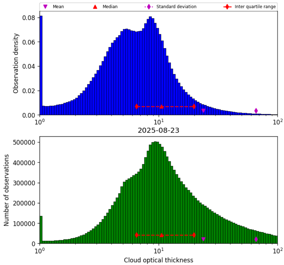
Figure 39: Histogram of “Cloud optical thickness” for 2025-08-23 to 2025-08-23
