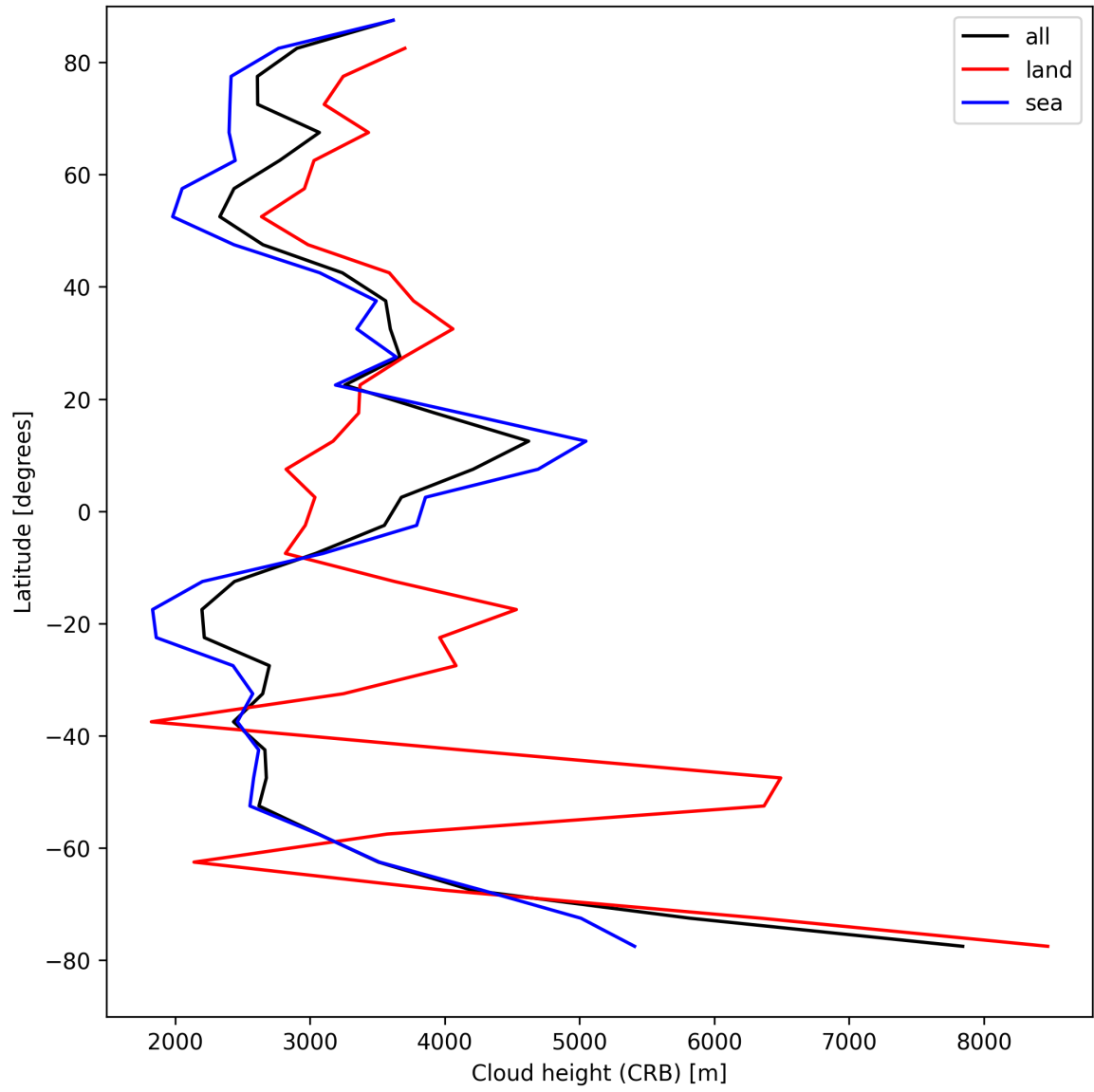
Figure 25: Zonal average of “Cloud height (CRB)” for 2025-08-23 to 2025-08-23.
