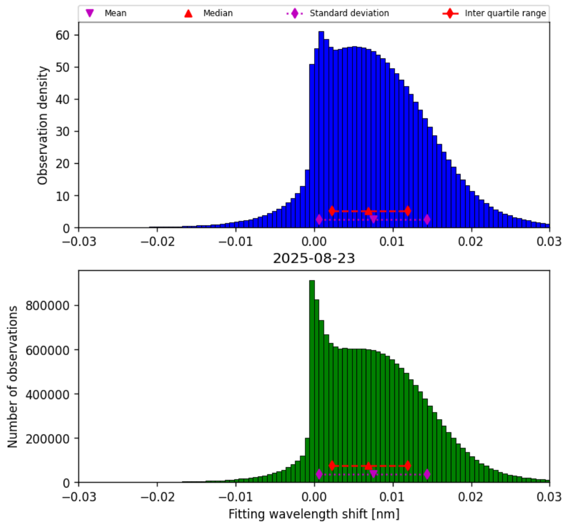
Figure 47: Histogram of “Fitting wavelength shift” for 2025-08-23 to 2025-08-23
