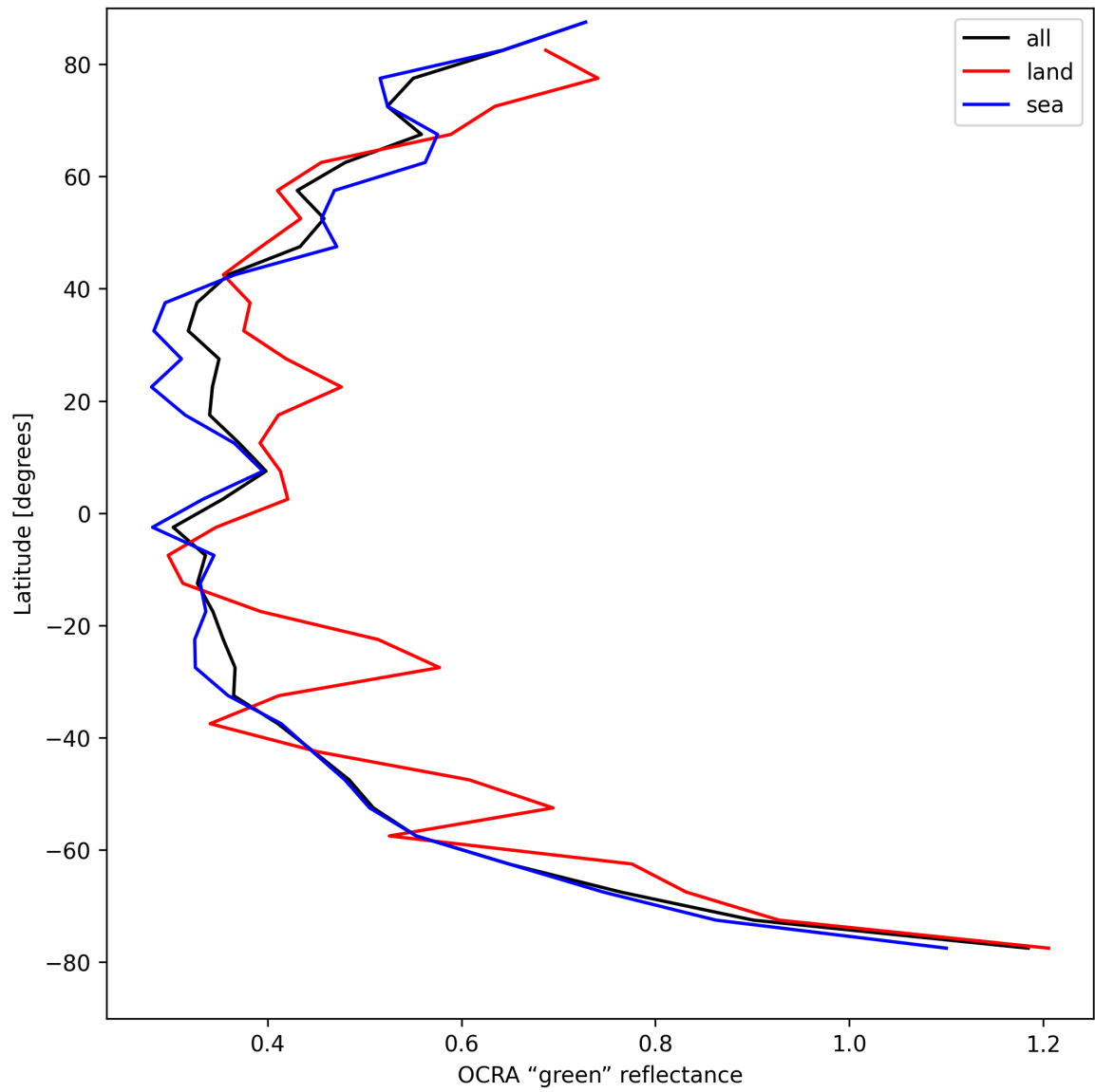
Figure 34: Zonal average of “OCRA “green” reflectance” for 2025-08-23 to 2025-08-23.
