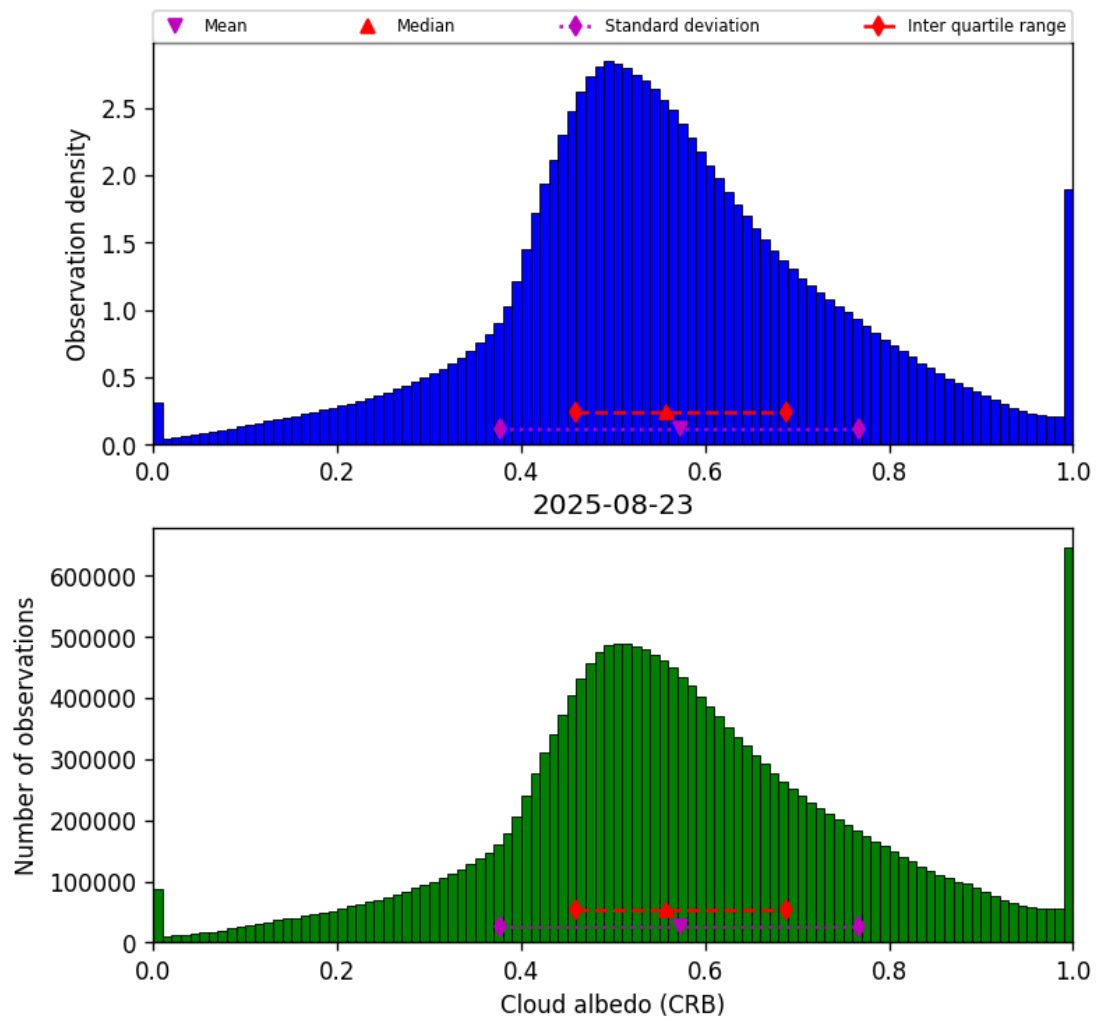
Figure 42: Histogram of “Cloud albedo (CRB)” for 2025-08-23 to 2025-08-23
