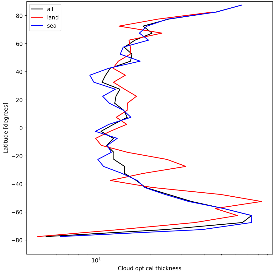
Figure 23: Zonal average of “Cloud optical thickness” for 2025-08-23 to 2025-08-23.
