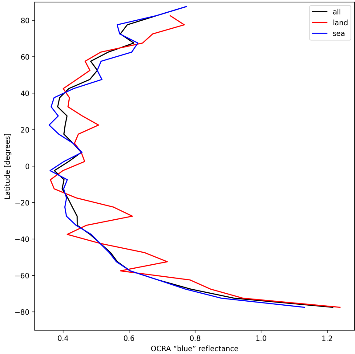
Figure 33: Zonal average of “OCRA “blue” reflectance” for 2025-08-23 to 2025-08-23.
