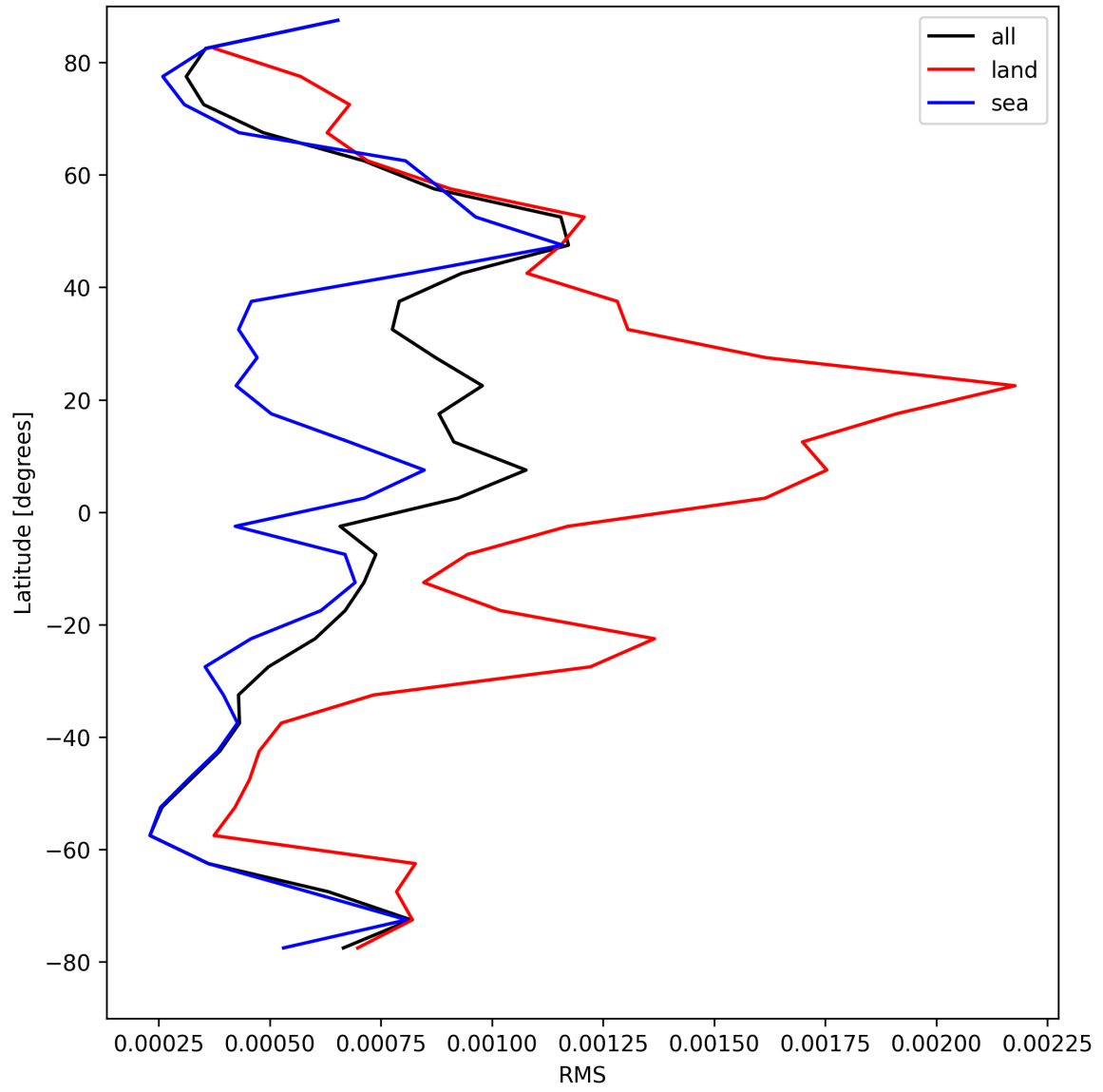
Figure 29: Zonal average of “RMS” for 2025-08-23 to 2025-08-23.
