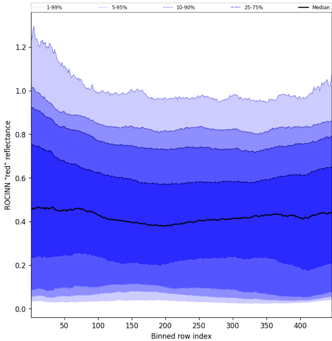
Figure 67: Along track statistics of "ROCINN "red" reflectance" for 2025-08-23 to 2025-08-23
