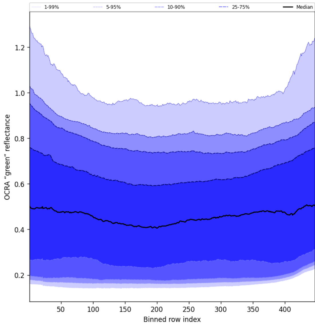
Figure 66: Along track statistics of “OCRA “green” reflectance” for 2025-08-23 to 2025-08-23
