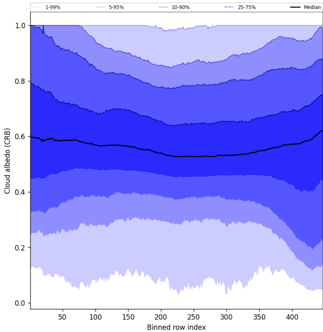
Figure 58: Along track statistics of “Cloud albedo (CRB)” for 2025-08-23 to 2025-08-23
