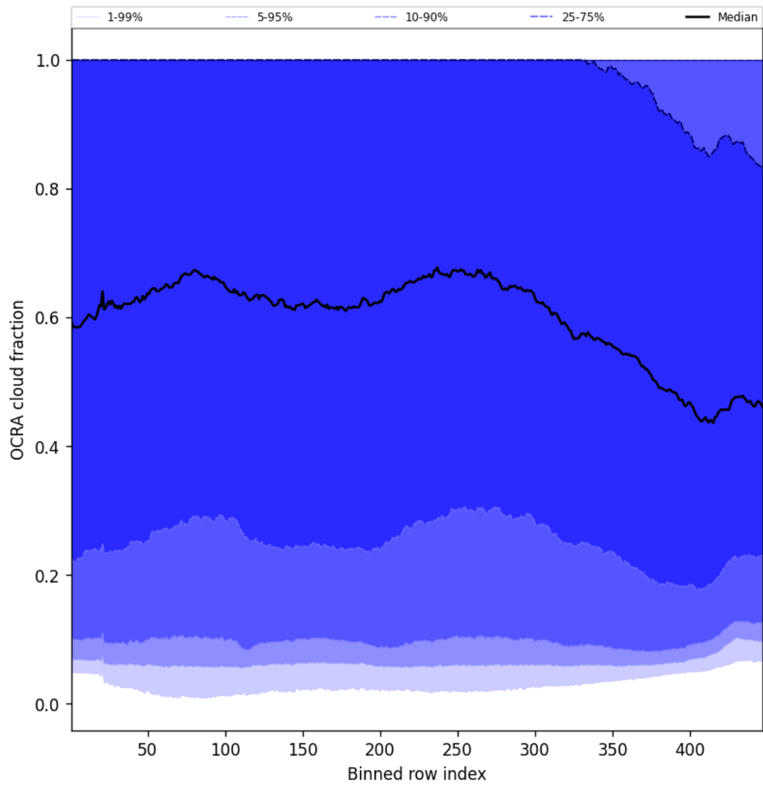
Figure 64: Along track statistics of “OCRA cloud fraction” for 2025-08-23 to 2025-08-23
