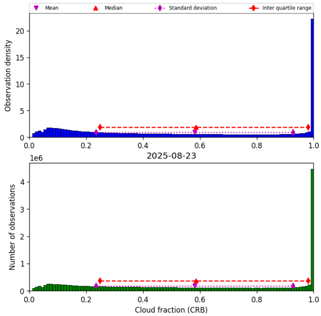
Figure 40: Histogram of “Cloud fraction (CRB)” for 2025-08-23 to 2025-08-23
