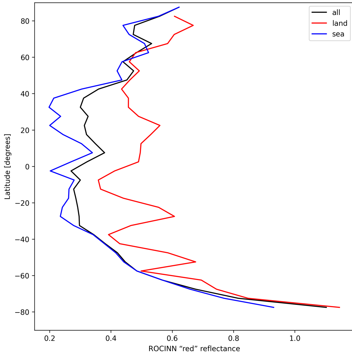
Figure 35: Zonal average of "ROCINN "red" reflectance" for 2025-08-23 to 2025-08-23.
