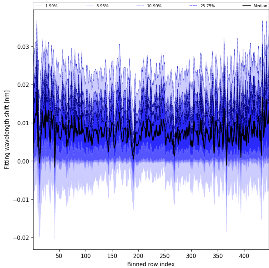
Figure 63: Along track statistics of “Fitting wavelength shift” for 2025-08-23 to 2025-08-23
