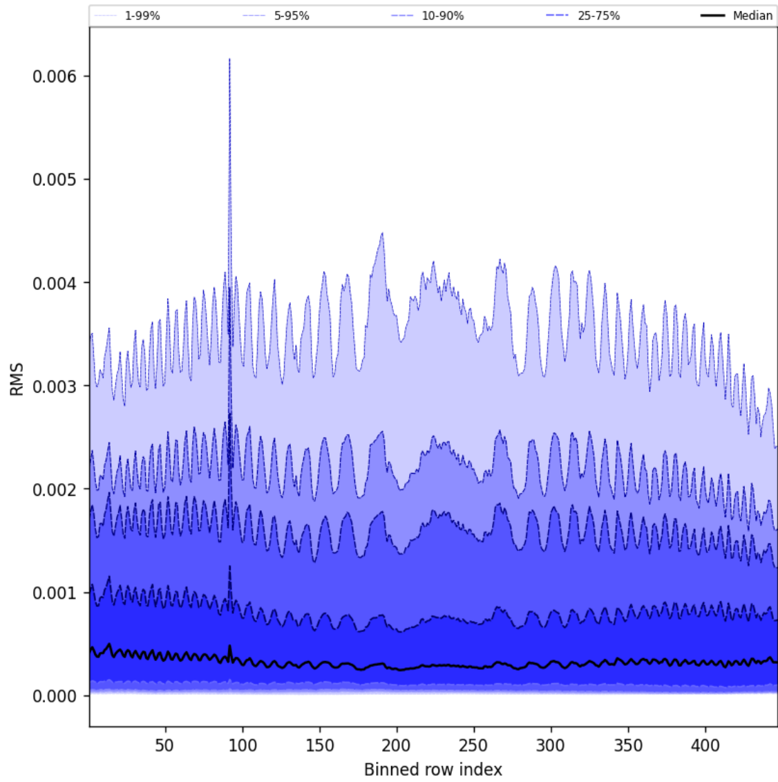
Figure 61: Along track statistics of “RMS” for 2025-08-23 to 2025-08-23
