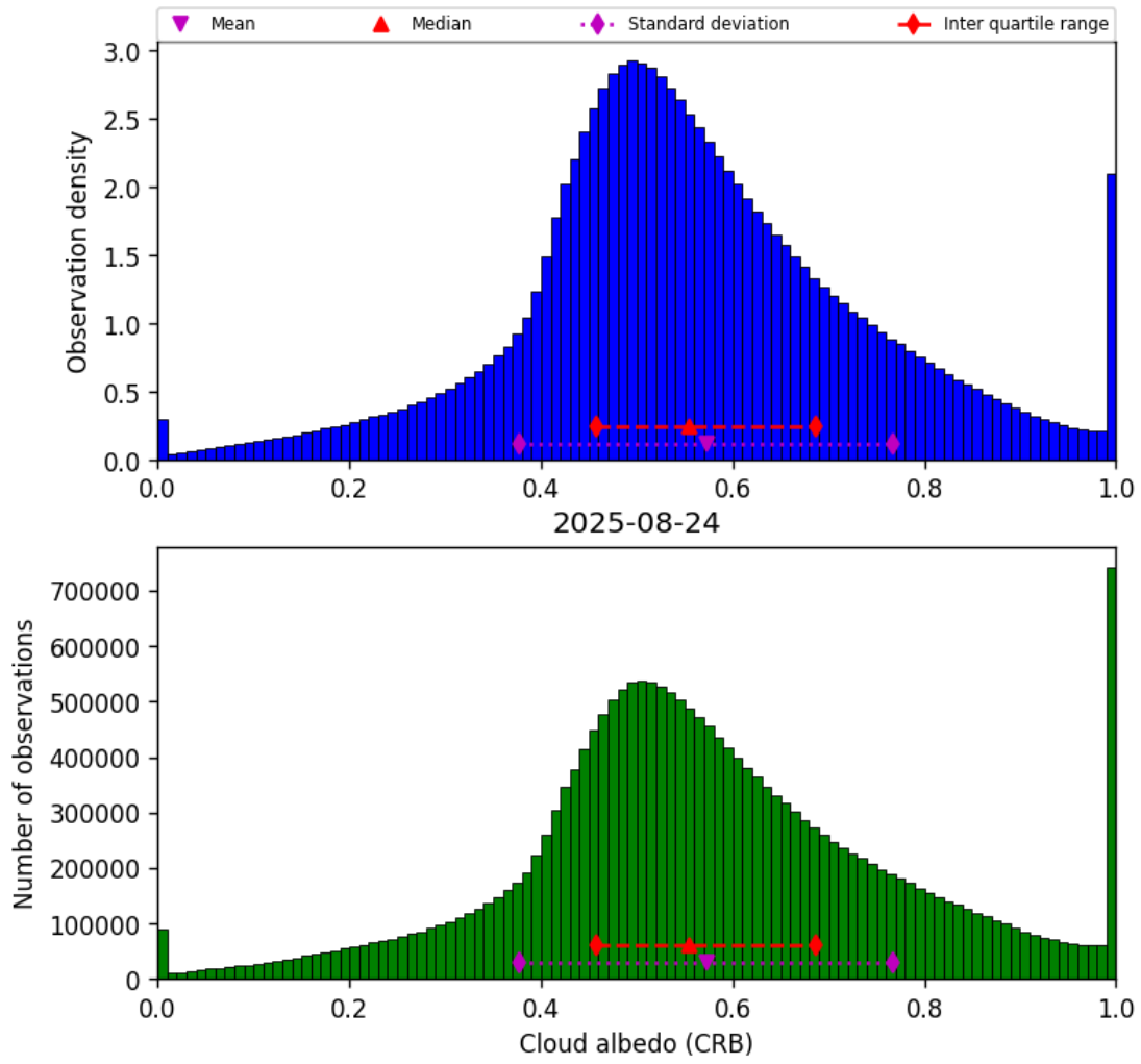
Figure 42: Histogram of “Cloud albedo (CRB)” for 2025-08-24 to 2025-08-25
