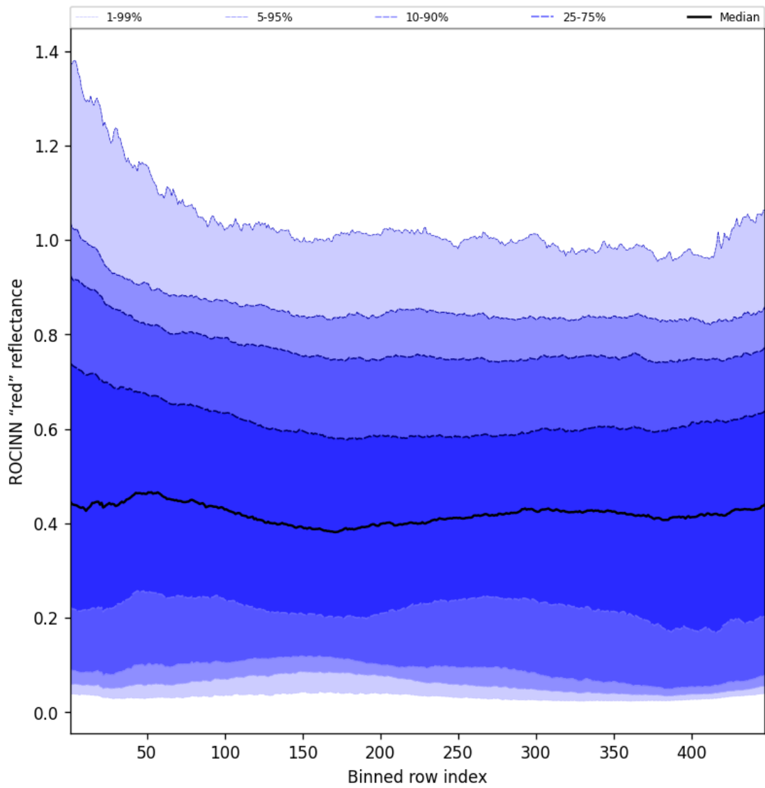
Figure 67: Along track statistics of "ROCINN "red" reflectance" for 2025-08-24 to 2025-08-25
