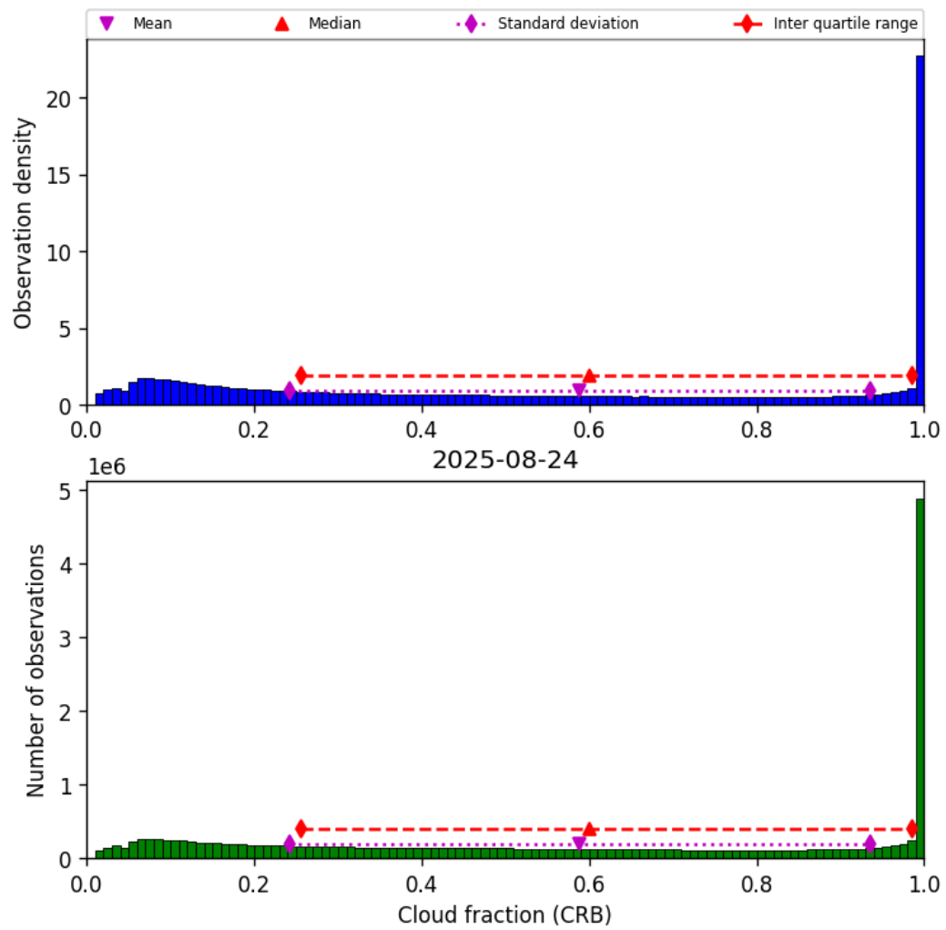
Figure 40: Histogram of “Cloud fraction (CRB)” for 2025-08-24 to 2025-08-25
