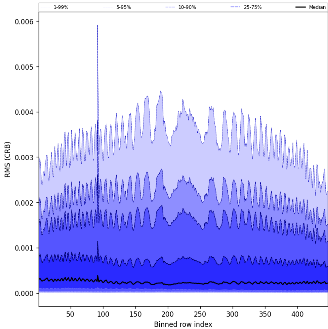
Figure 62: Along track statistics of “RMS (CRB)” for 2025-08-24 to 2025-08-25
