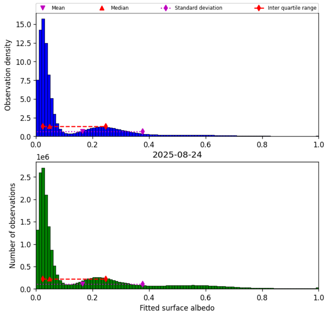
Figure 43: Histogram of “Fitted surface albedo” for 2025-08-24 to 2025-08-25
