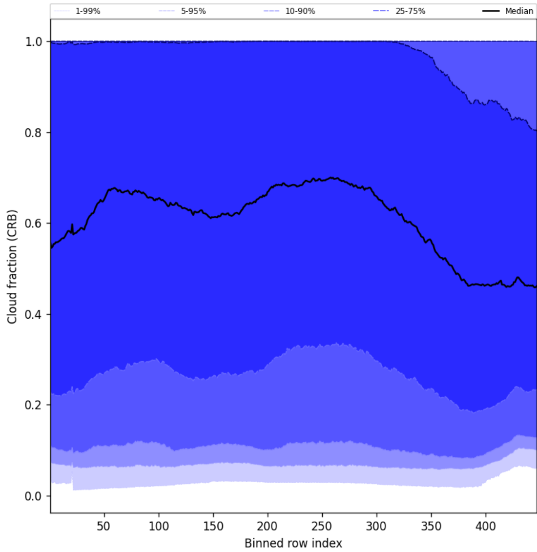
Figure 56: Along track statistics of “Cloud fraction (CRB)” for 2025-08-24 to 2025-08-25
