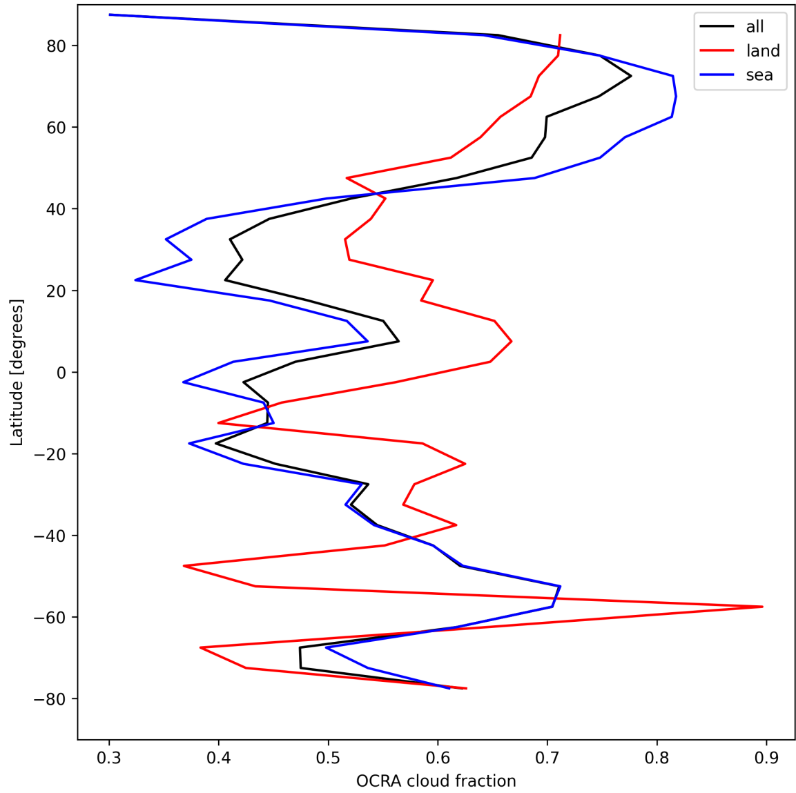
Figure 32: Zonal average of “OCRA cloud fraction” for 2025-08-24 to 2025-08-25.
