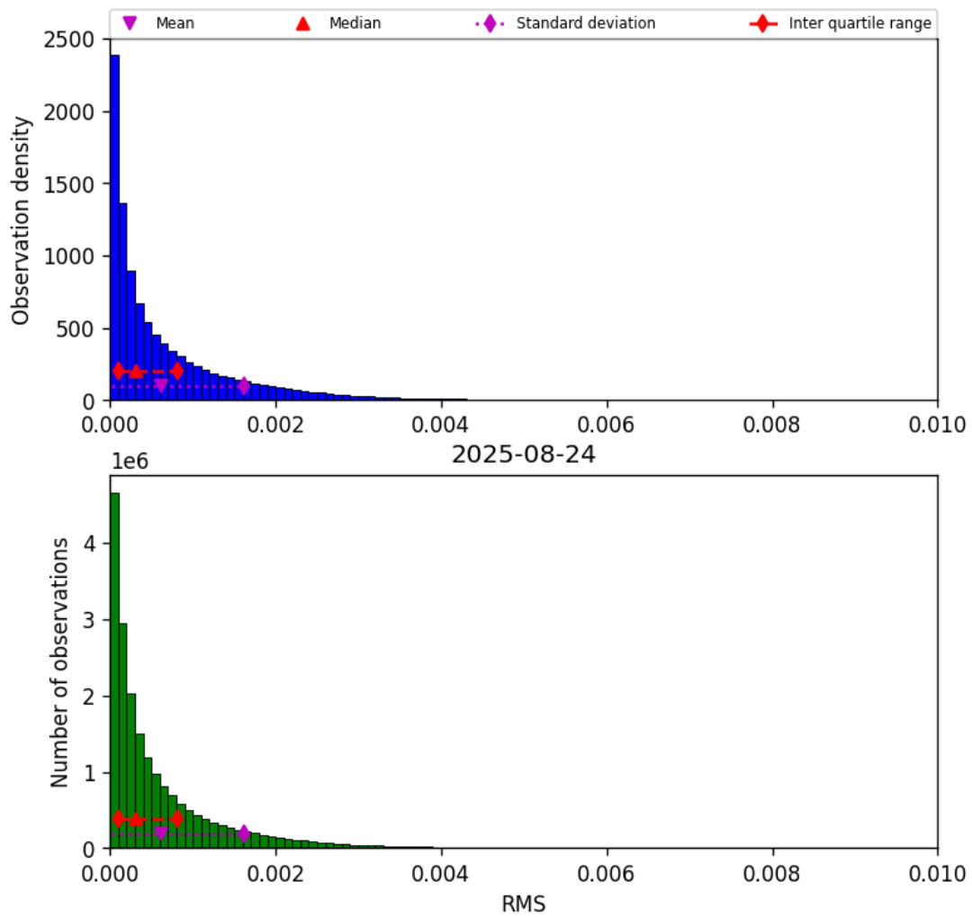
Figure 45: Histogram of “RMS” for 2025-08-24 to 2025-08-25
