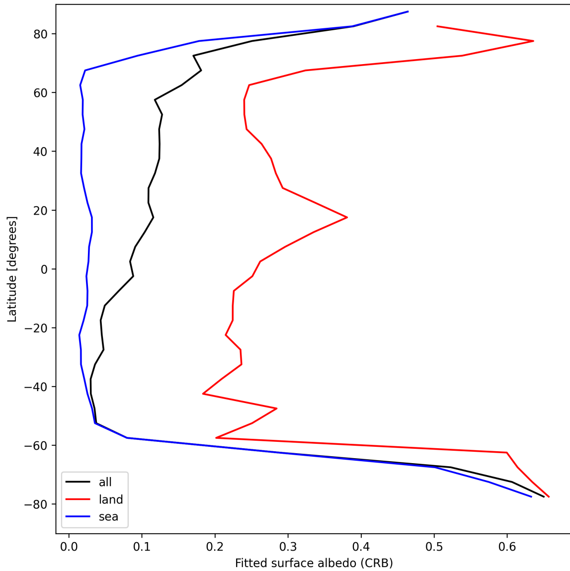
Figure 28: Zonal average of “Fitted surface albedo (CRB)” for 2025-08-24 to 2025-08-25.
