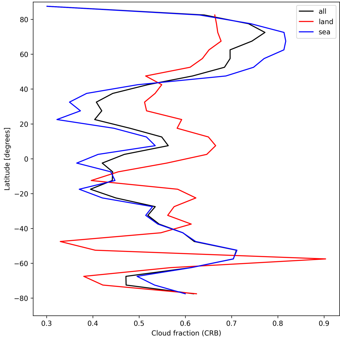
Figure 24: Zonal average of “Cloud fraction (CRB)” for 2025-08-24 to 2025-08-25.
