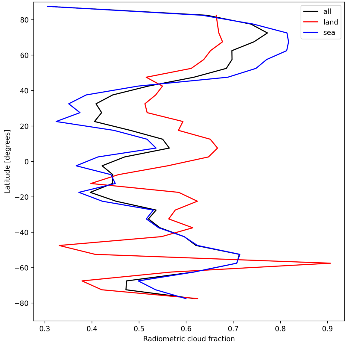
Figure 21: Zonal average of “Radiometric cloud fraction” for 2025-08-24 to 2025-08-25.
