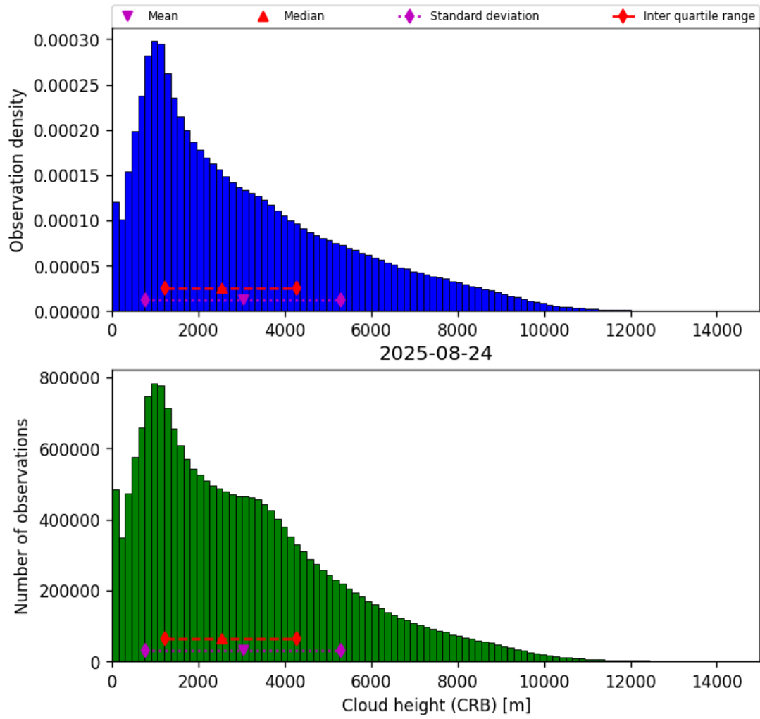
Figure 41: Histogram of “Cloud height (CRB)” for 2025-08-24 to 2025-08-25
