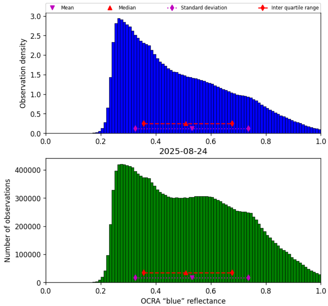
Figure 49: Histogram of “OCRA “blue” reflectance” for 2025-08-24 to 2025-08-25
