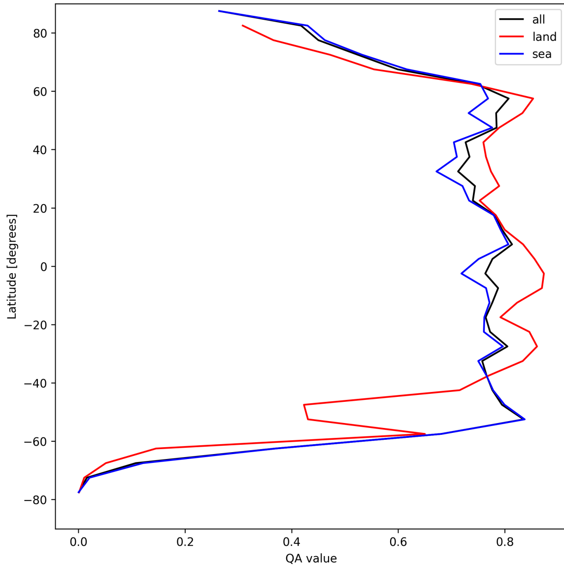
Figure 20: Zonal average of “QA value” for 2025-08-24 to 2025-08-25.
