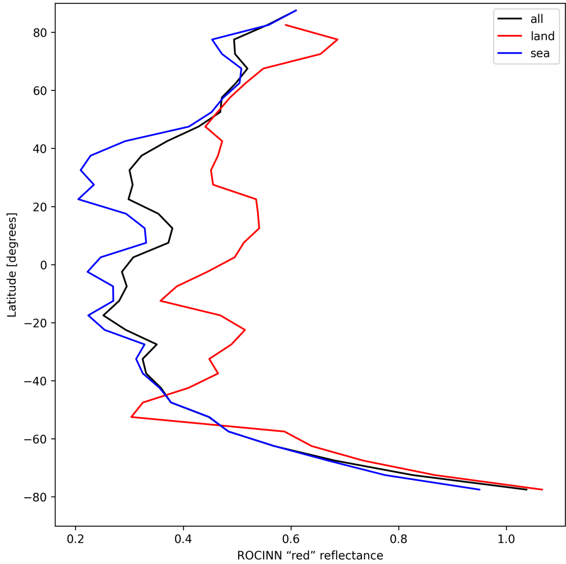
Figure 35: Zonal average of “ROCINN “red” reflectance” for 2025-08-24 to 2025-08-25.
