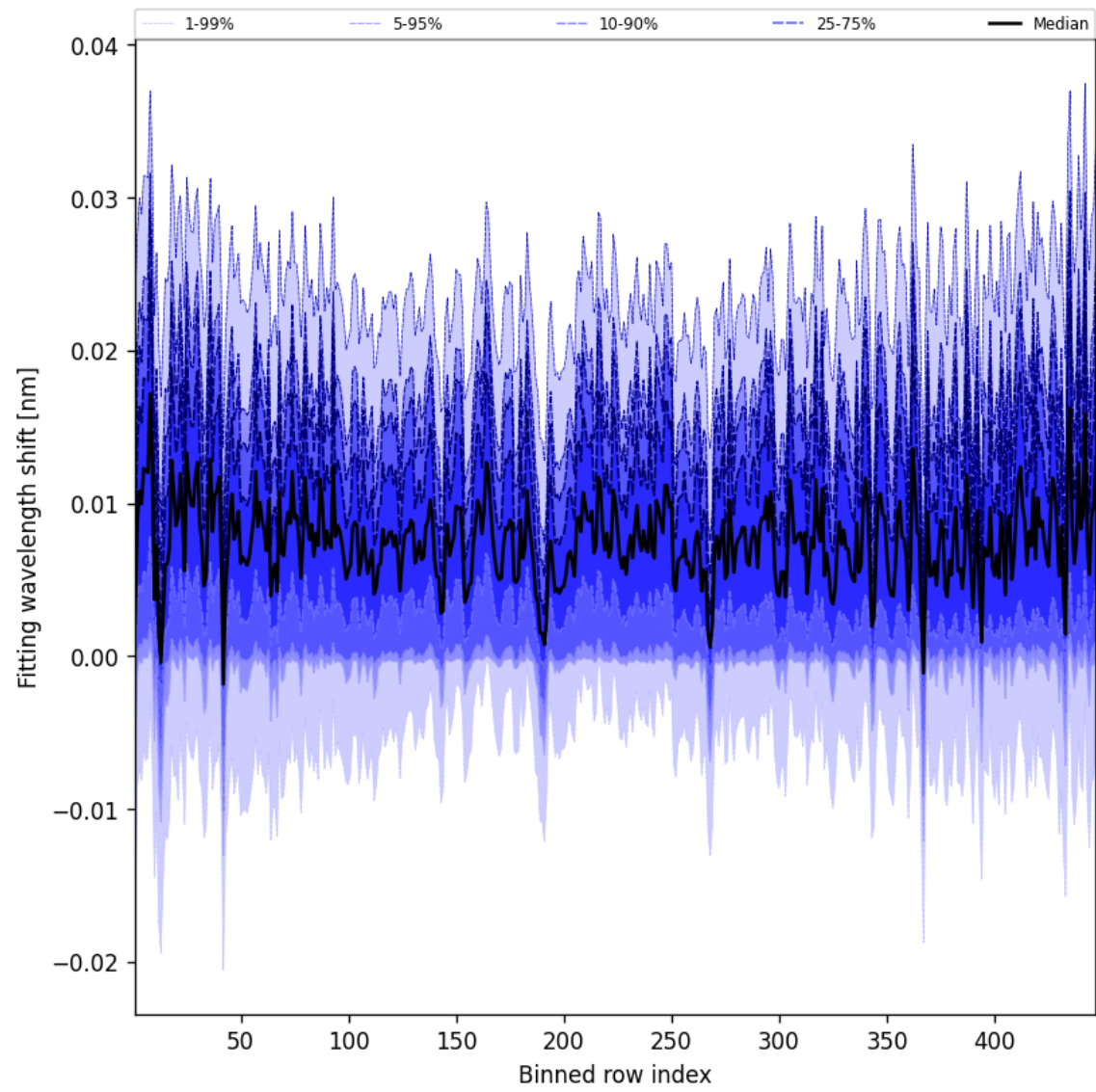
Figure 63: Along track statistics of “Fitting wavelength shift” for 2025-08-24 to 2025-08-25
