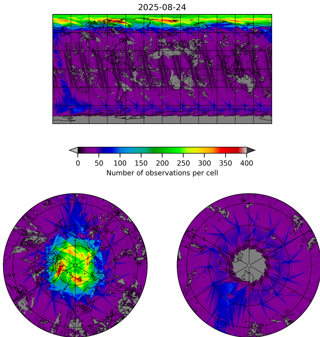
Figure 19: Map of the number of observations for 2025-08-24 to 2025-08-25
