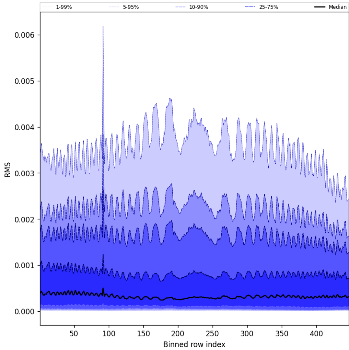
Figure 61: Along track statistics of “RMS” for 2025-08-24 to 2025-08-25
