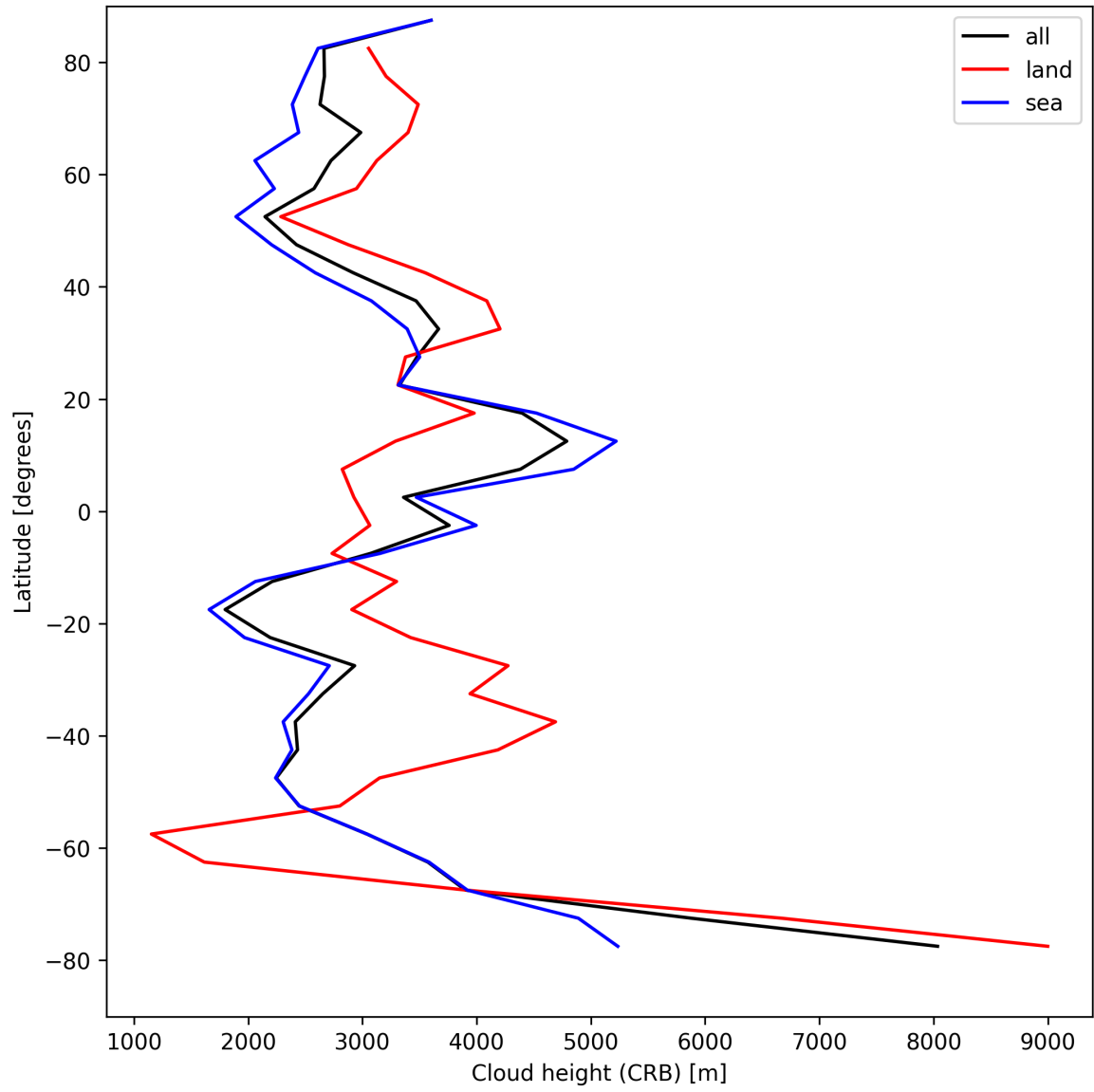
Figure 25: Zonal average of “Cloud height (CRB)” for 2025-08-24 to 2025-08-25.
