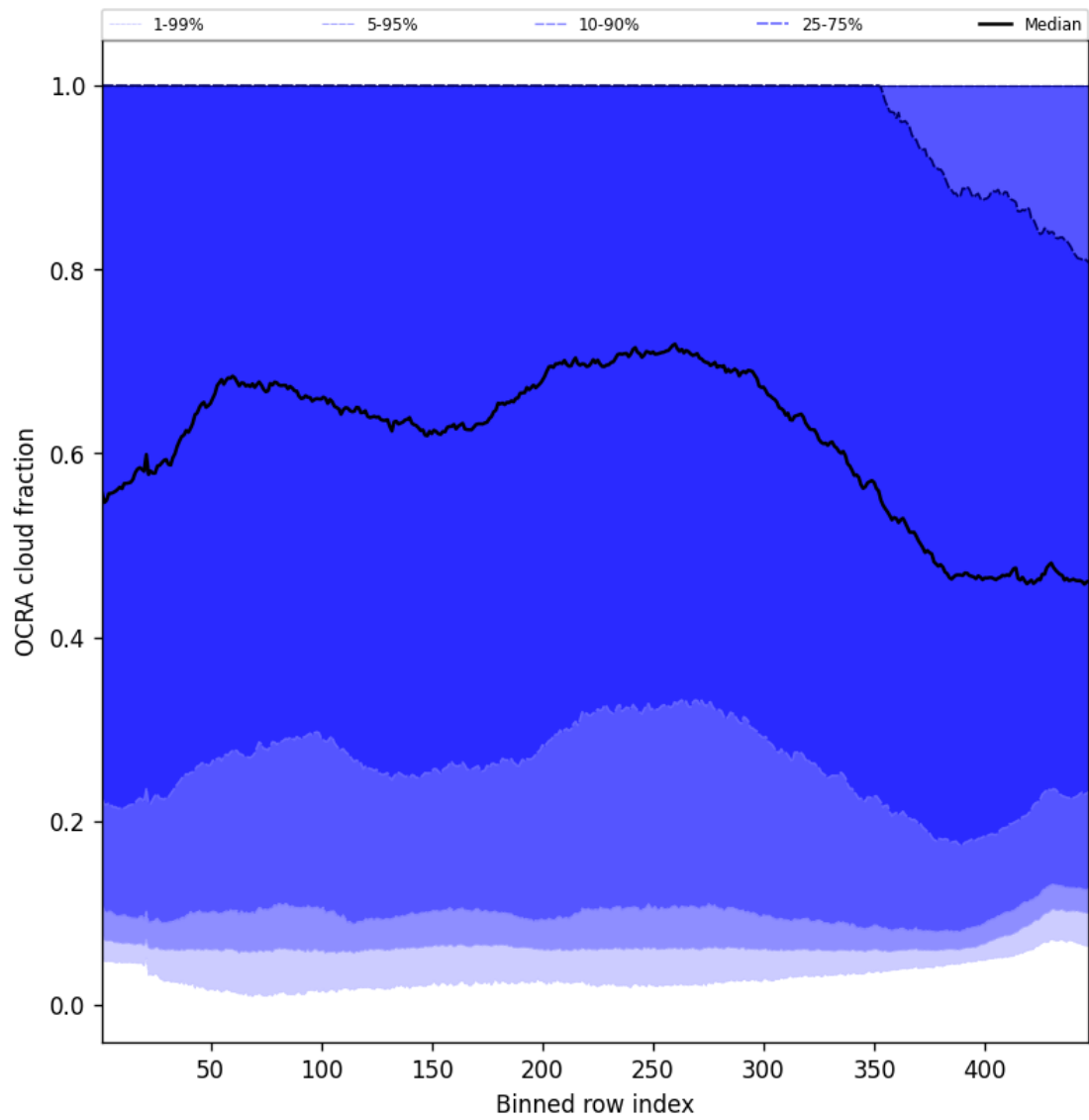
Figure 64: Along track statistics of “OCRA cloud fraction” for 2025-08-24 to 2025-08-25
