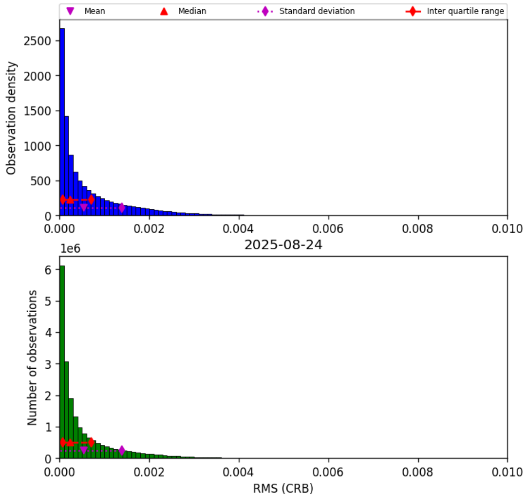
Figure 46: Histogram of “RMS (CRB)” for 2025-08-24 to 2025-08-25
