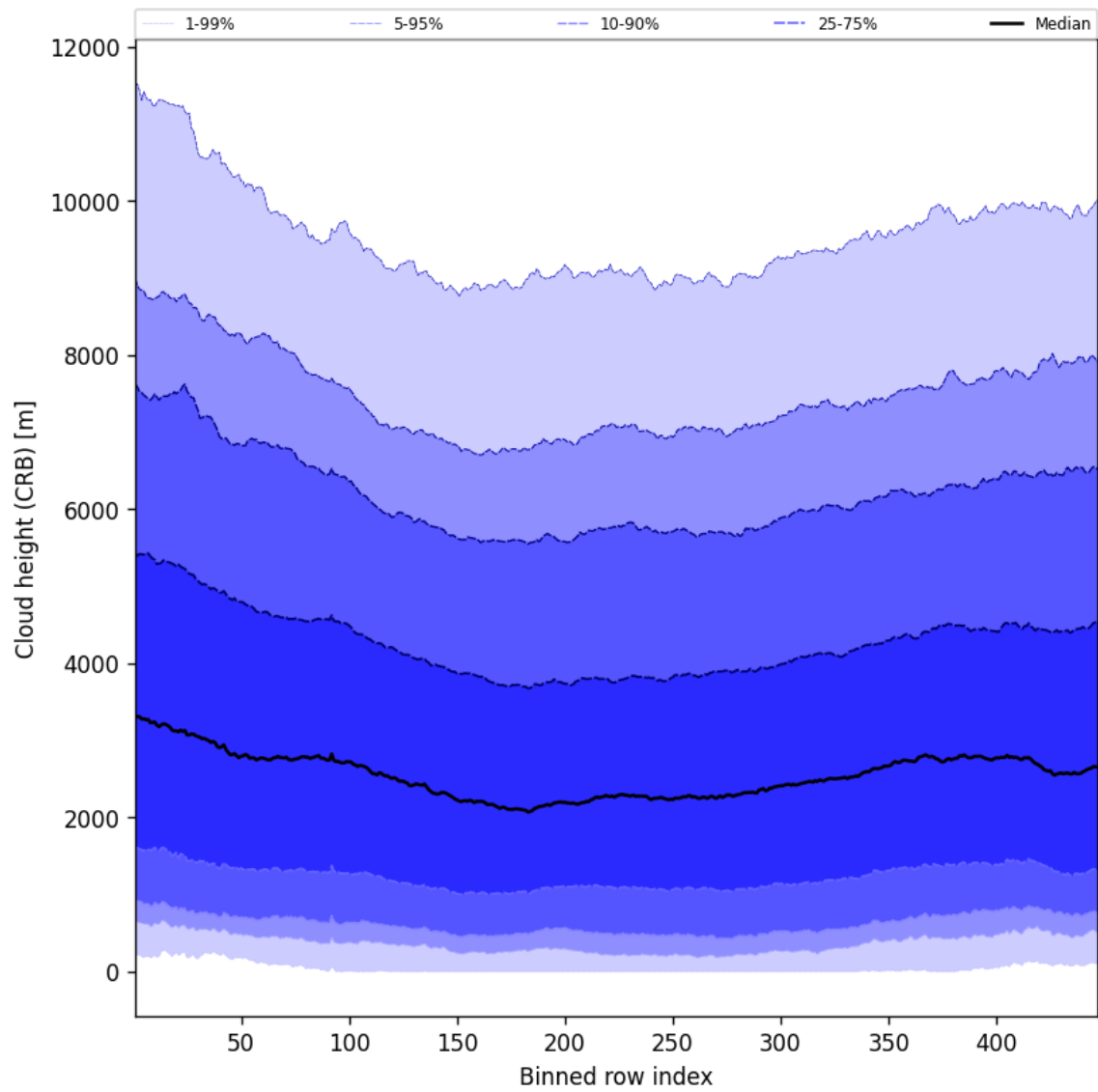
Figure 57: Along track statistics of “Cloud height (CRB)” for 2025-08-24 to 2025-08-25
