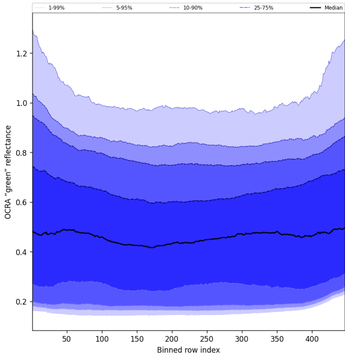
Figure 66: Along track statistics of “OCRA “green” reflectance” for 2025-08-24 to 2025-08-25
