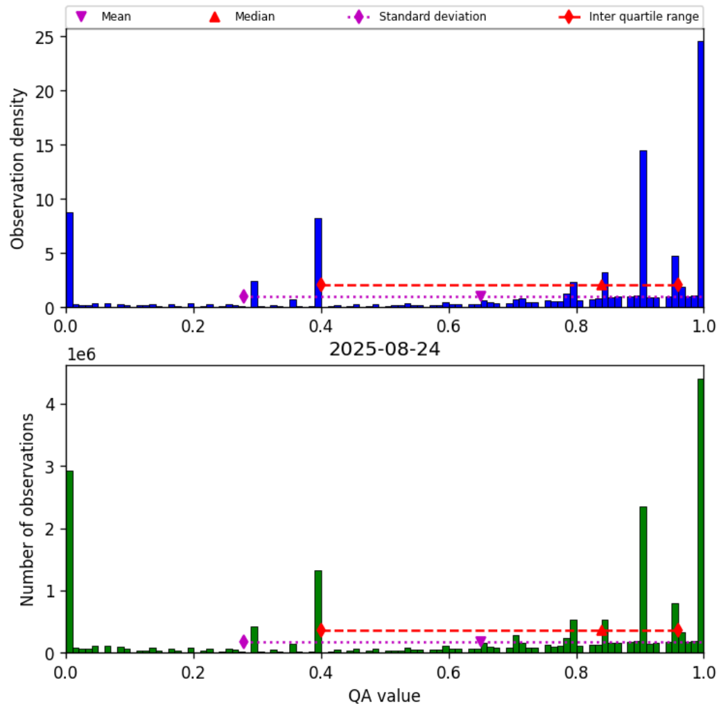
Figure 36: Histogram of “QA value” for 2025-08-24 to 2025-08-25
