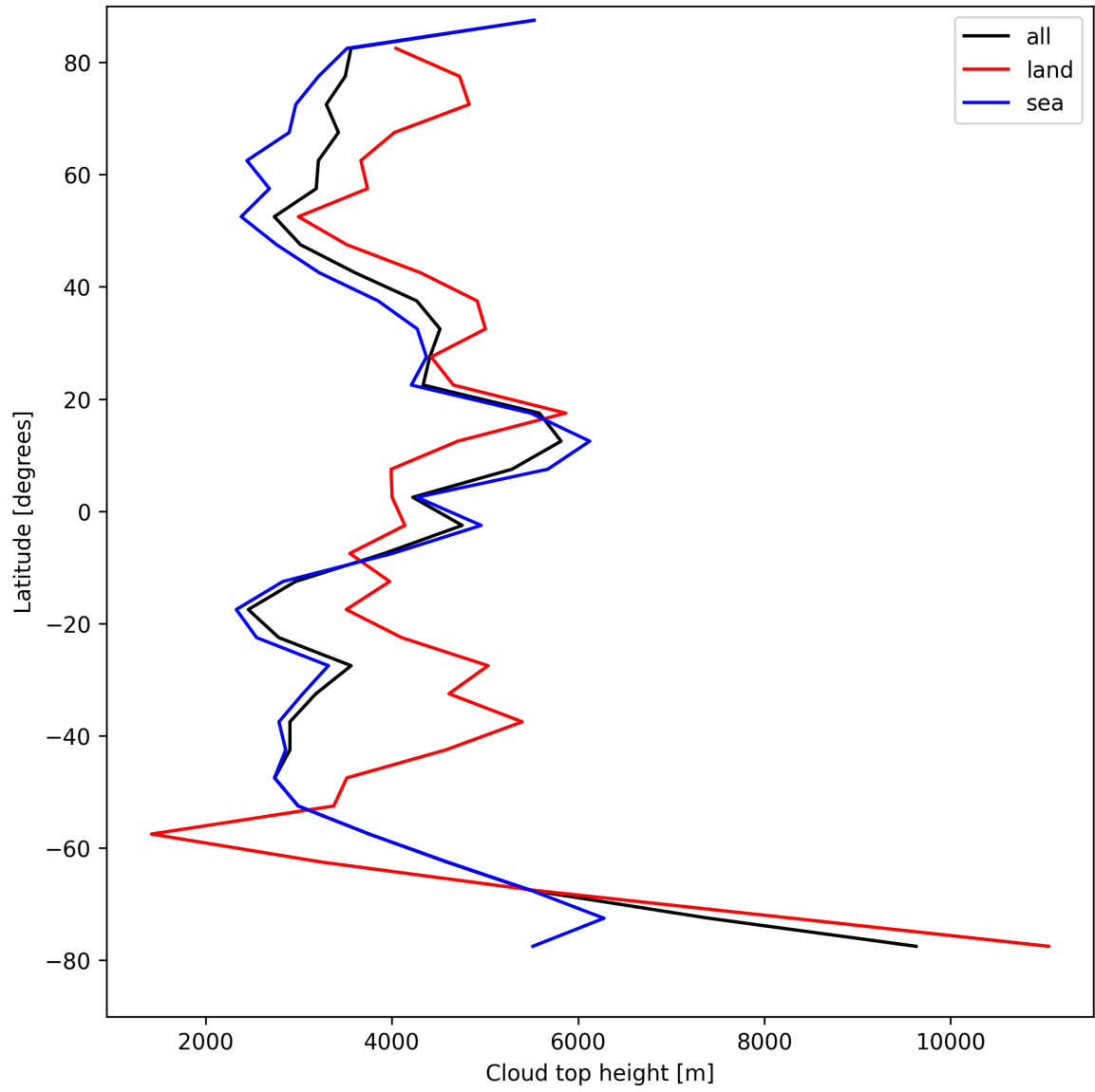
Figure 22: Zonal average of “Cloud top height” for 2025-08-24 to 2025-08-25.
