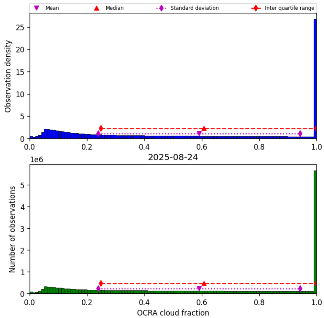
Figure 48: Histogram of “OCRA cloud fraction” for 2025-08-24 to 2025-08-25
