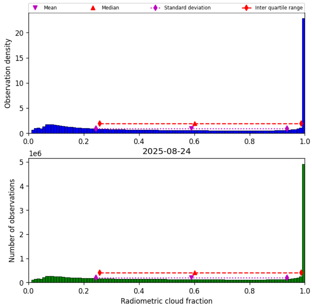
Figure 37: Histogram of “Radiometric cloud fraction” for 2025-08-24 to 2025-08-25
