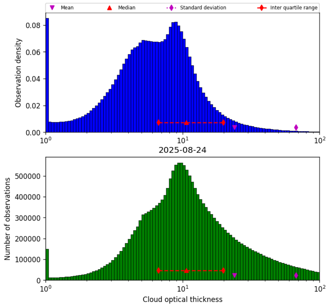
Figure 39: Histogram of “Cloud optical thickness” for 2025-08-24 to 2025-08-25
