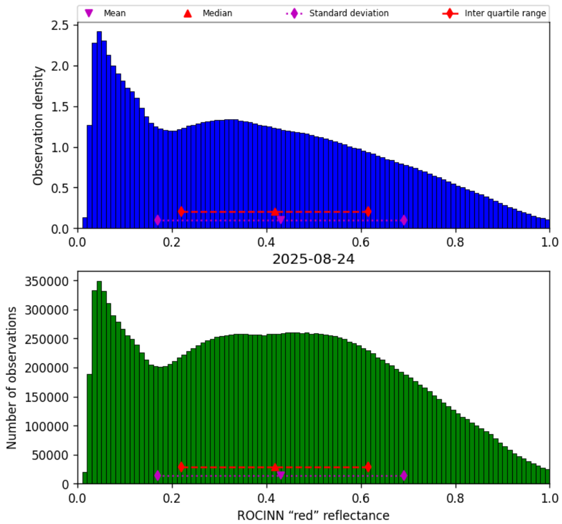
Figure 51: Histogram of “ROCINN “red” reflectance” for 2025-08-24 to 2025-08-25
