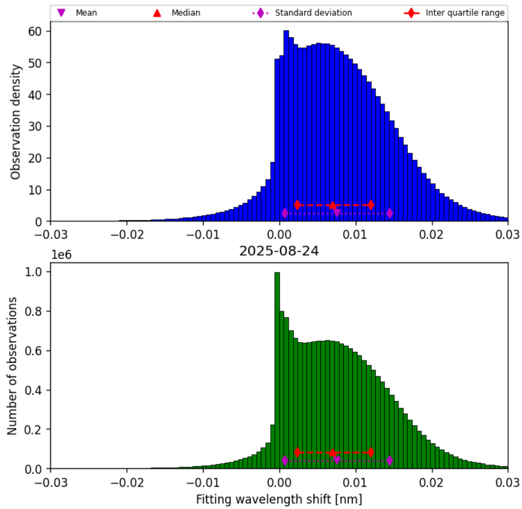
Figure 47: Histogram of “Fitting wavelength shift” for 2025-08-24 to 2025-08-25
