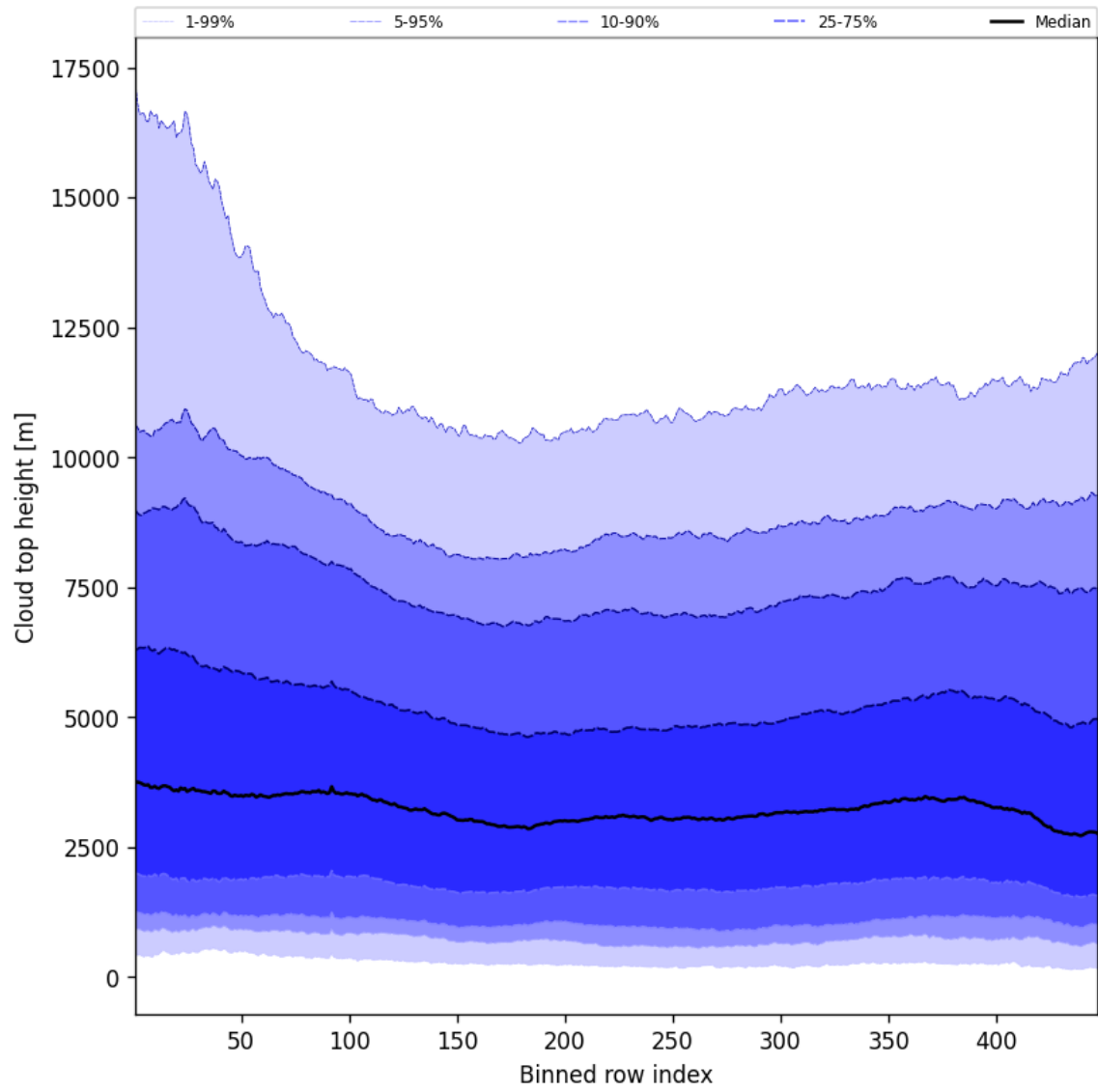
Figure 54: Along track statistics of “Cloud top height” for 2025-08-24 to 2025-08-25
