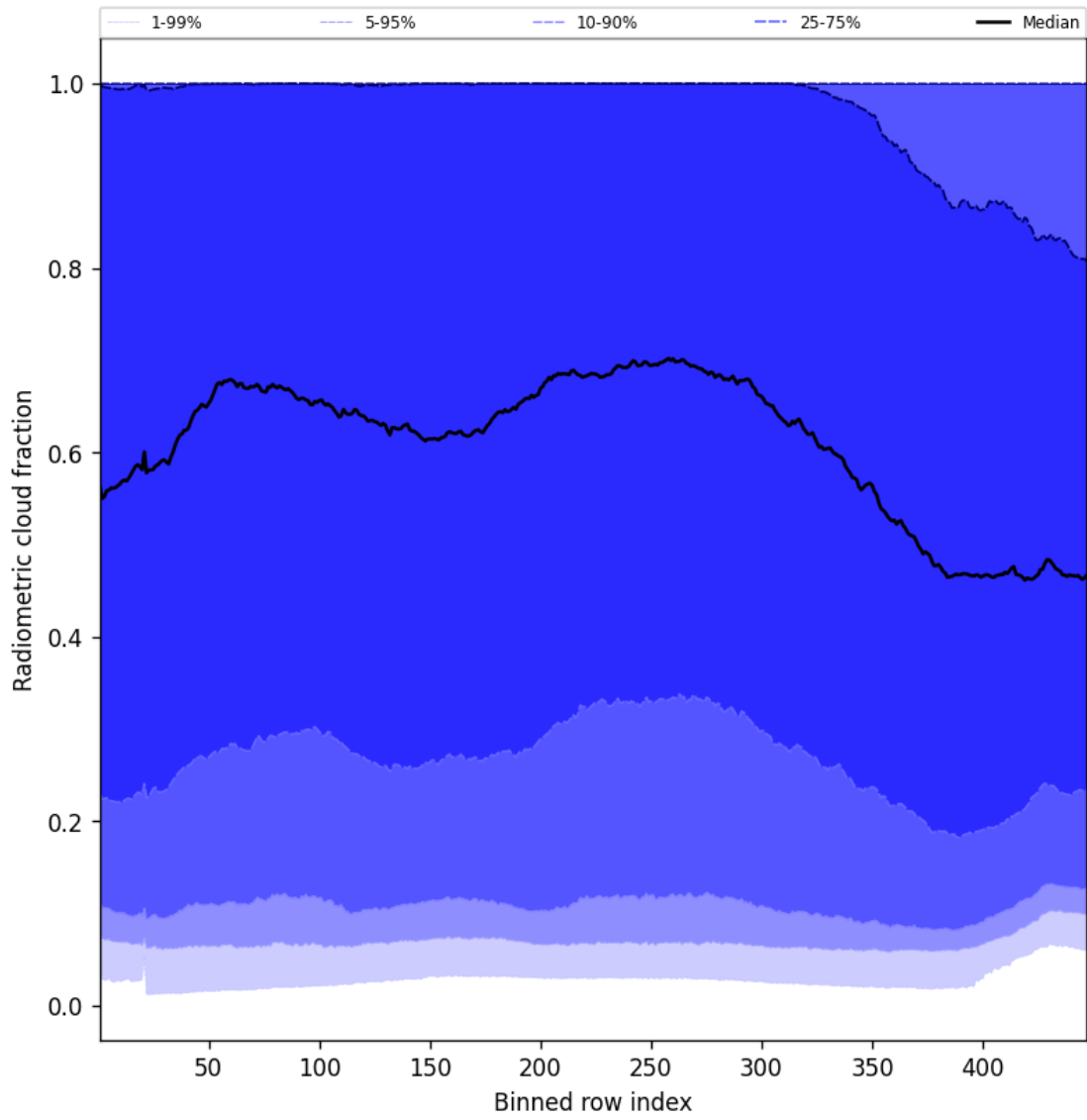
Figure 53: Along track statistics of “Radiometric cloud fraction” for 2025-08-24 to 2025-08-25
