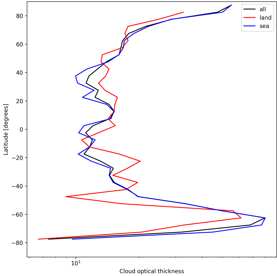
Figure 23: Zonal average of “Cloud optical thickness” for 2025-08-24 to 2025-08-25.
