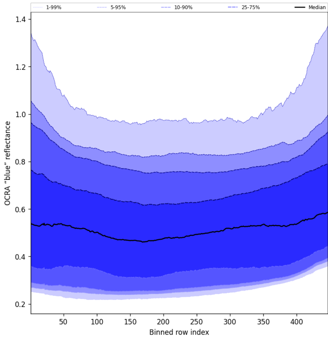
Figure 65: Along track statistics of “OCRA “blue” reflectance” for 2025-08-24 to 2025-08-25
