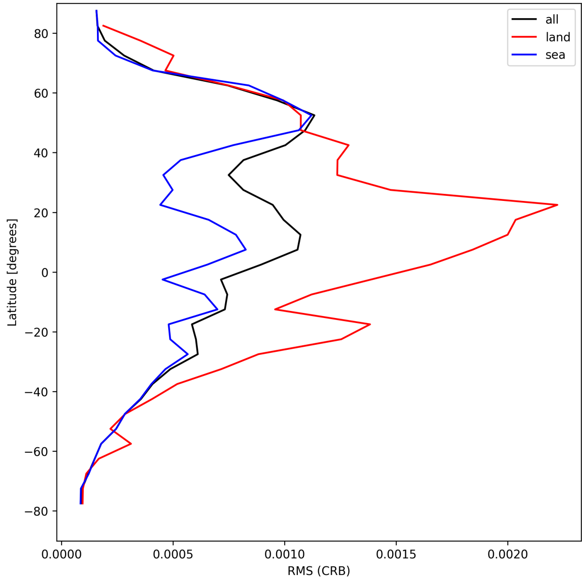
Figure 30: Zonal average of “RMS (CRB)” for 2025-08-24 to 2025-08-25.
