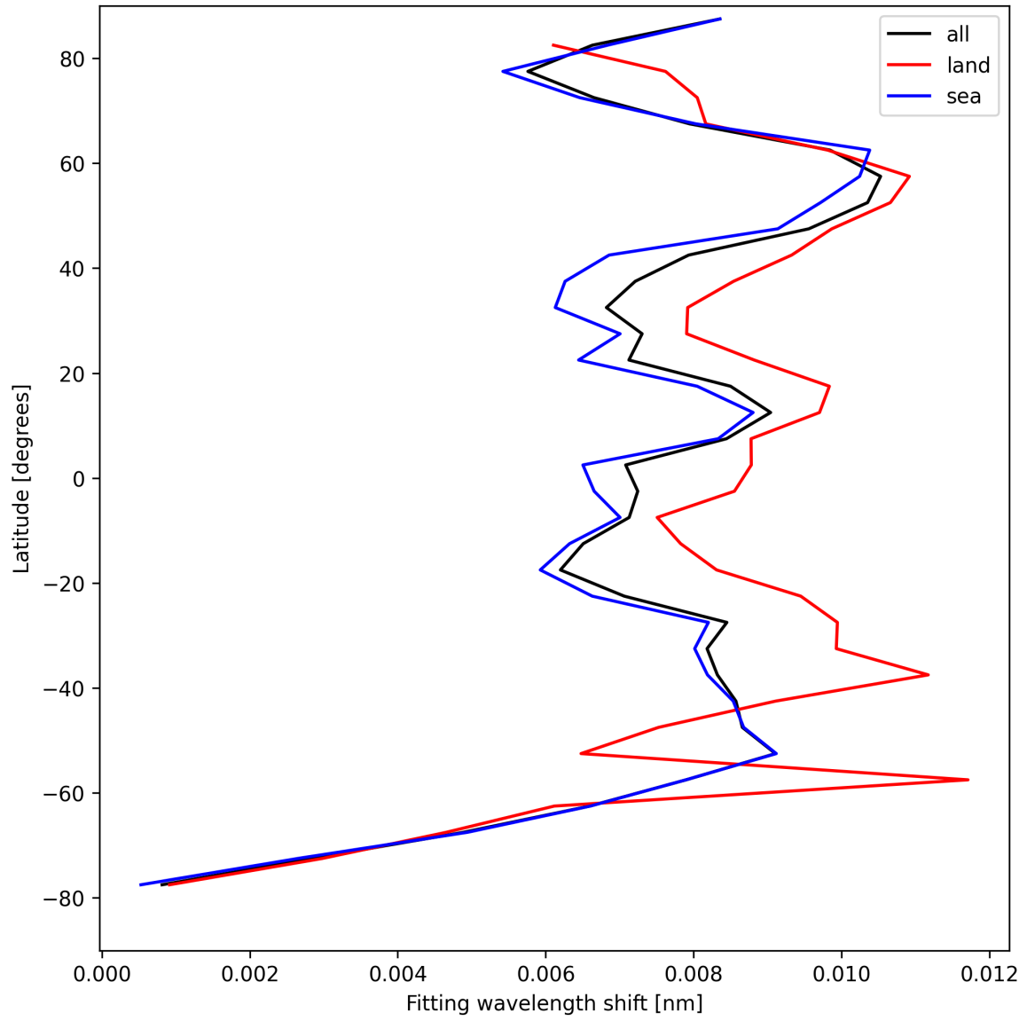
Figure 31: Zonal average of “Fitting wavelength shift” for 2025-08-24 to 2025-08-25.
