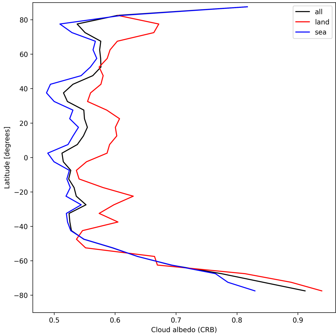
Figure 26: Zonal average of “Cloud albedo (CRB)” for 2025-08-24 to 2025-08-25.
