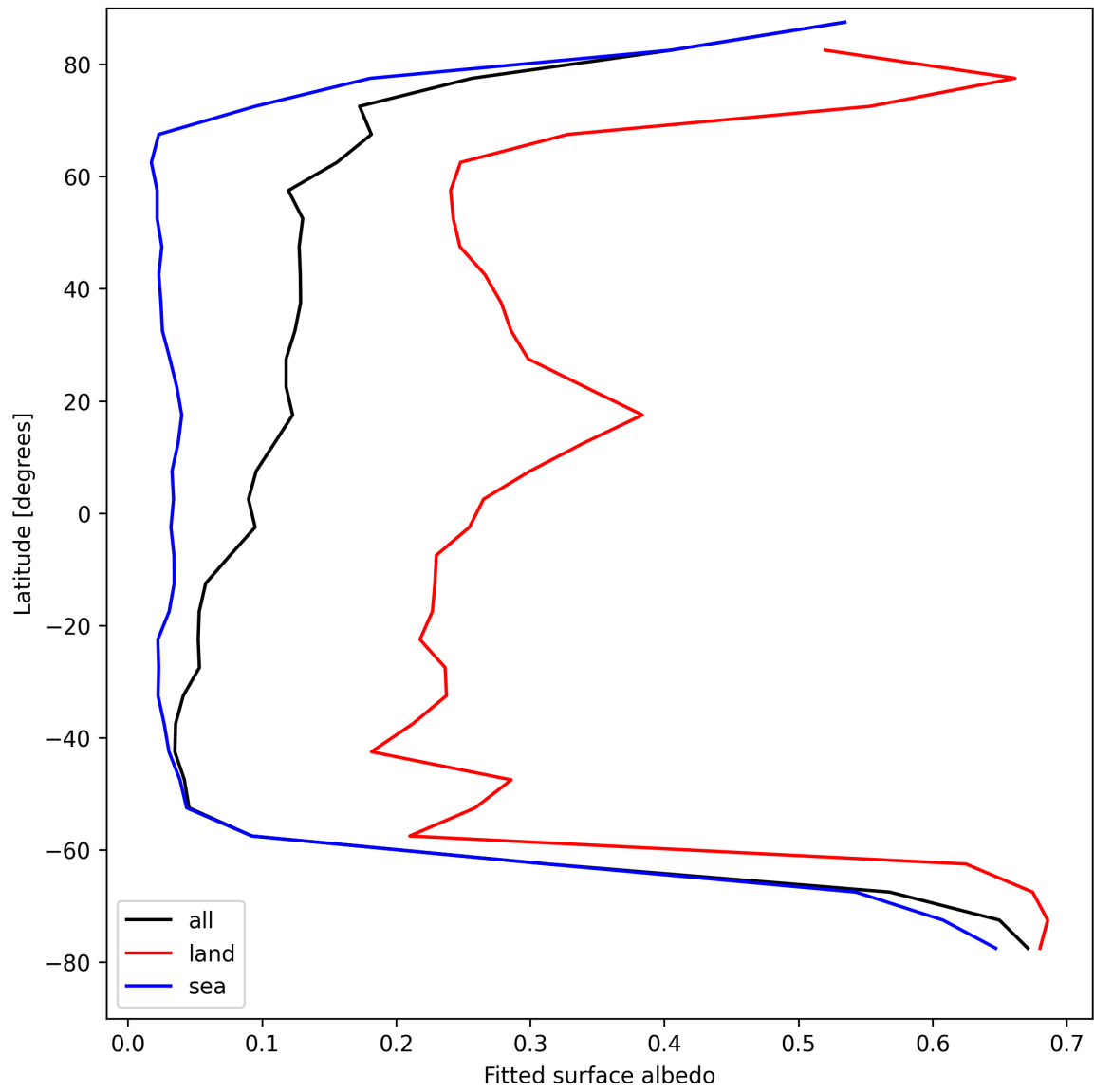
Figure 27: Zonal average of “Fitted surface albedo” for 2025-08-24 to 2025-08-25.
