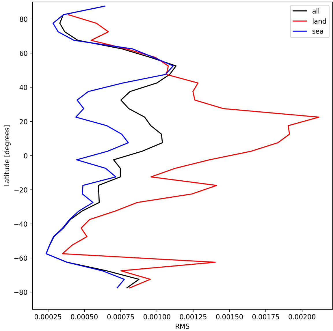
Figure 29: Zonal average of “RMS” for 2025-08-24 to 2025-08-25.
