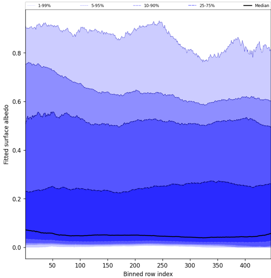
Figure 59: Along track statistics of “Fitted surface albedo” for 2025-08-24 to 2025-08-25
