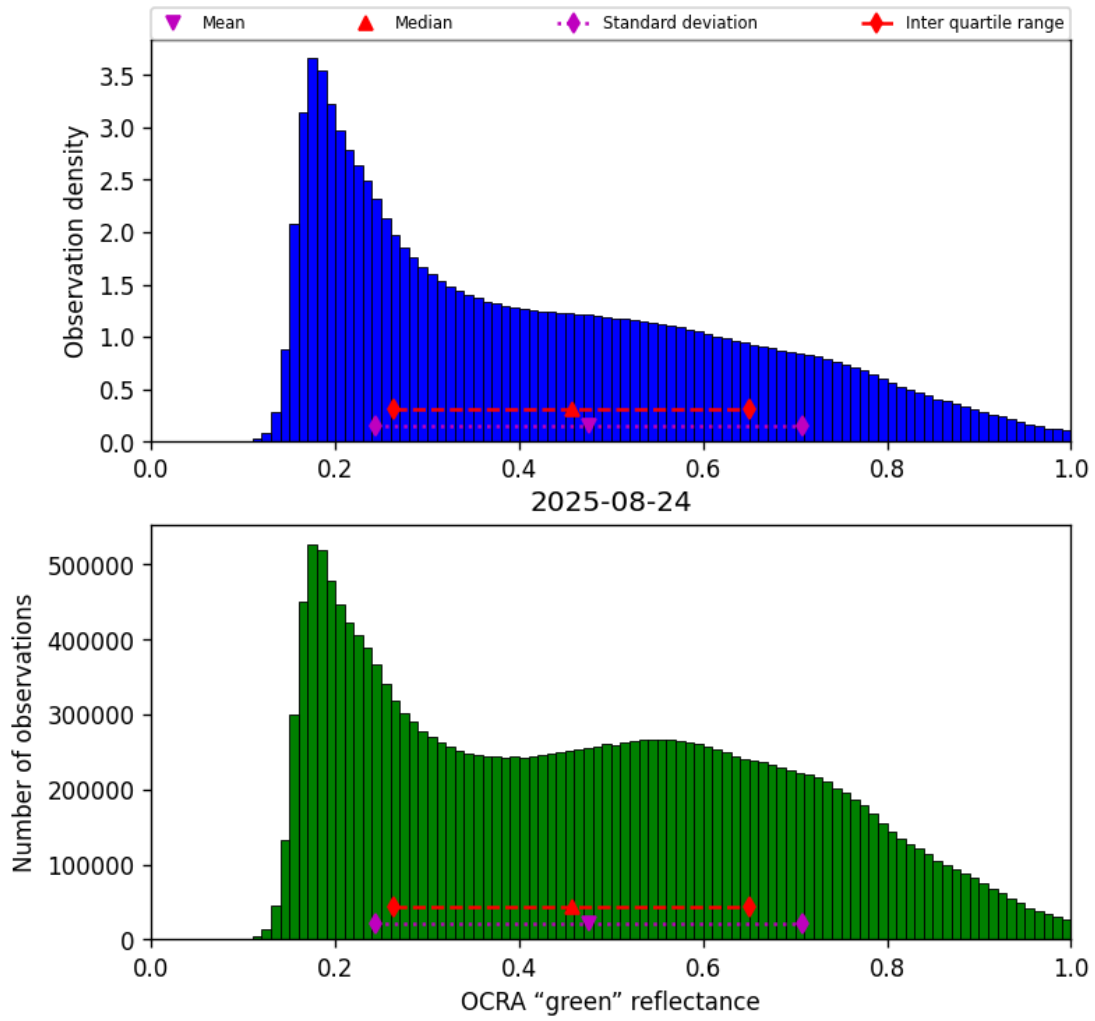
Figure 50: Histogram of “OCRA “green” reflectance” for 2025-08-24 to 2025-08-25
