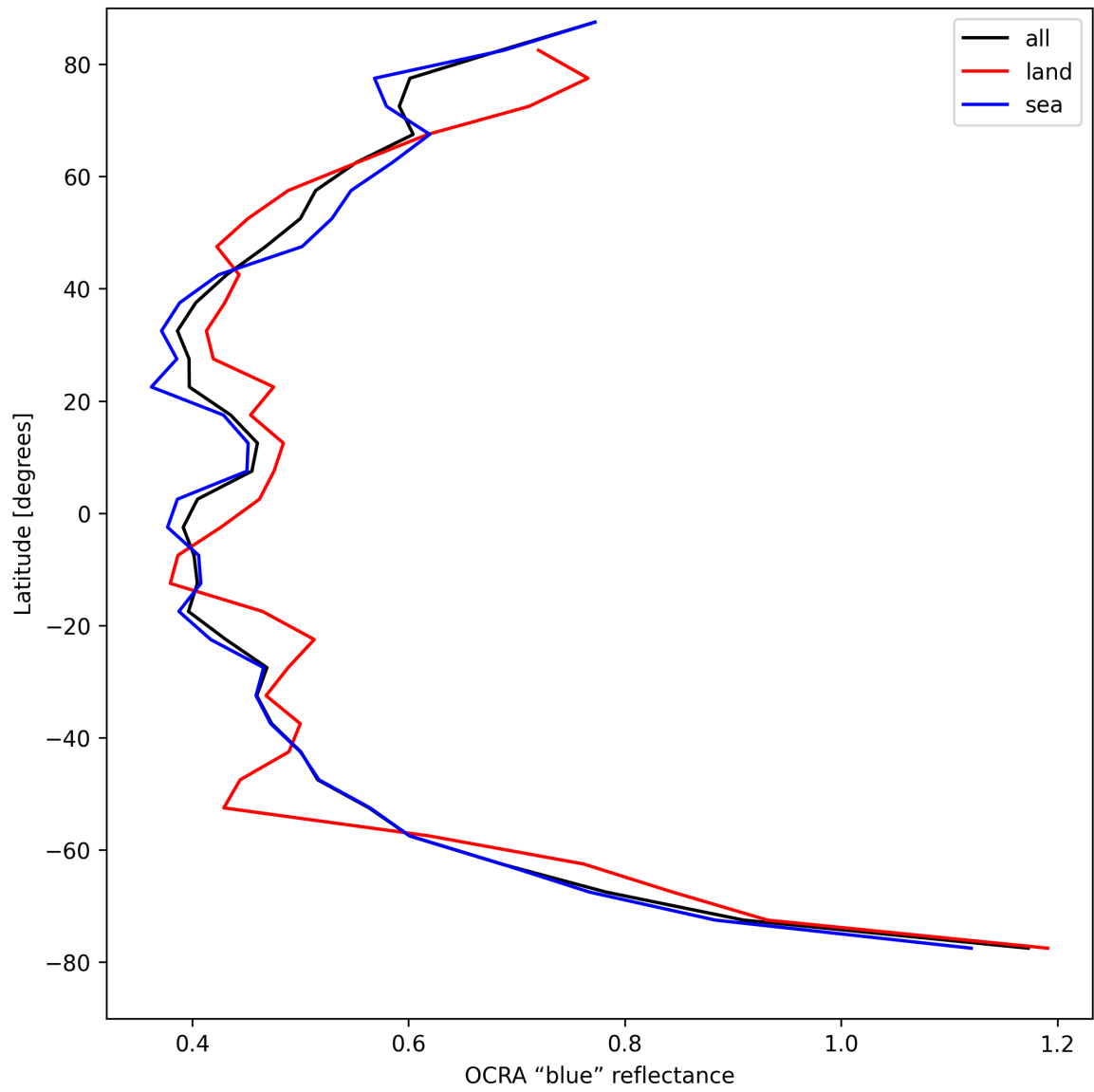
Figure 33: Zonal average of “OCRA “blue” reflectance” for 2025-08-24 to 2025-08-25.
