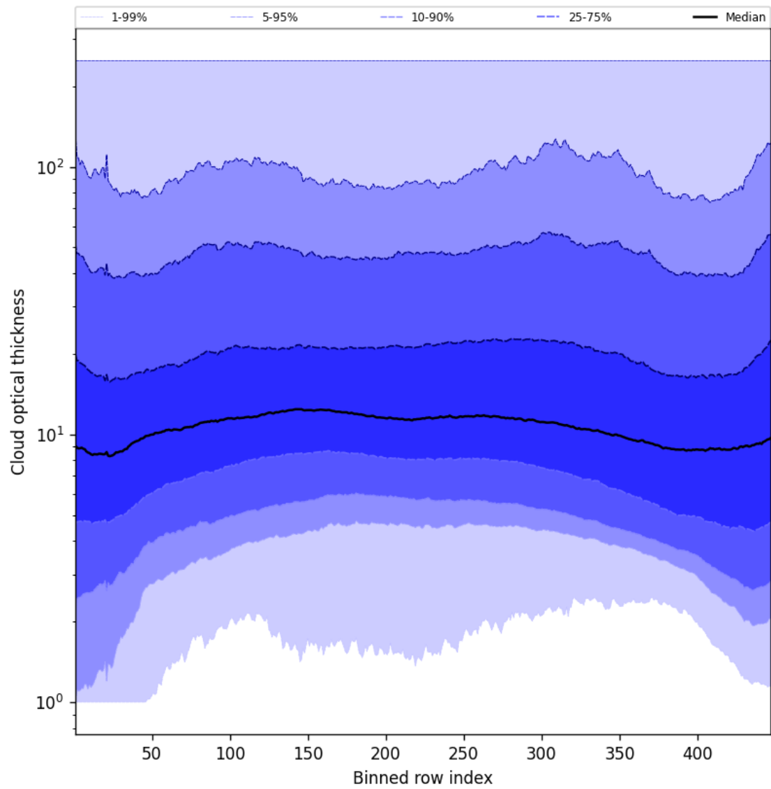
Figure 55: Along track statistics of “Cloud optical thickness” for 2025-08-24 to 2025-08-25
