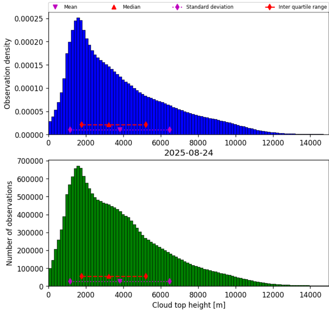
Figure 38: Histogram of “Cloud top height” for 2025-08-24 to 2025-08-25
