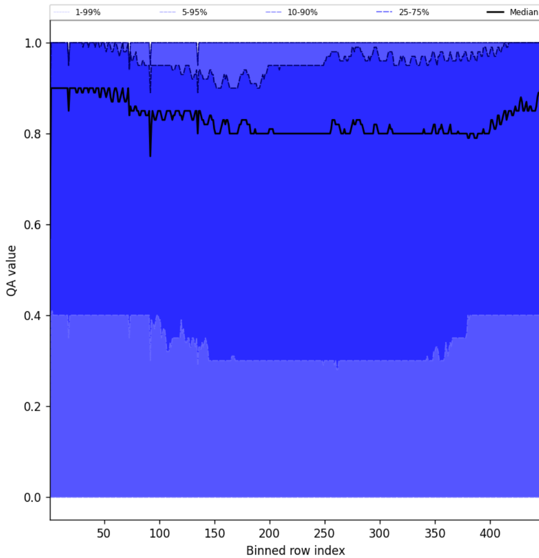
Figure 52: Along track statistics of “QA value” for 2025-08-24 to 2025-08-25
