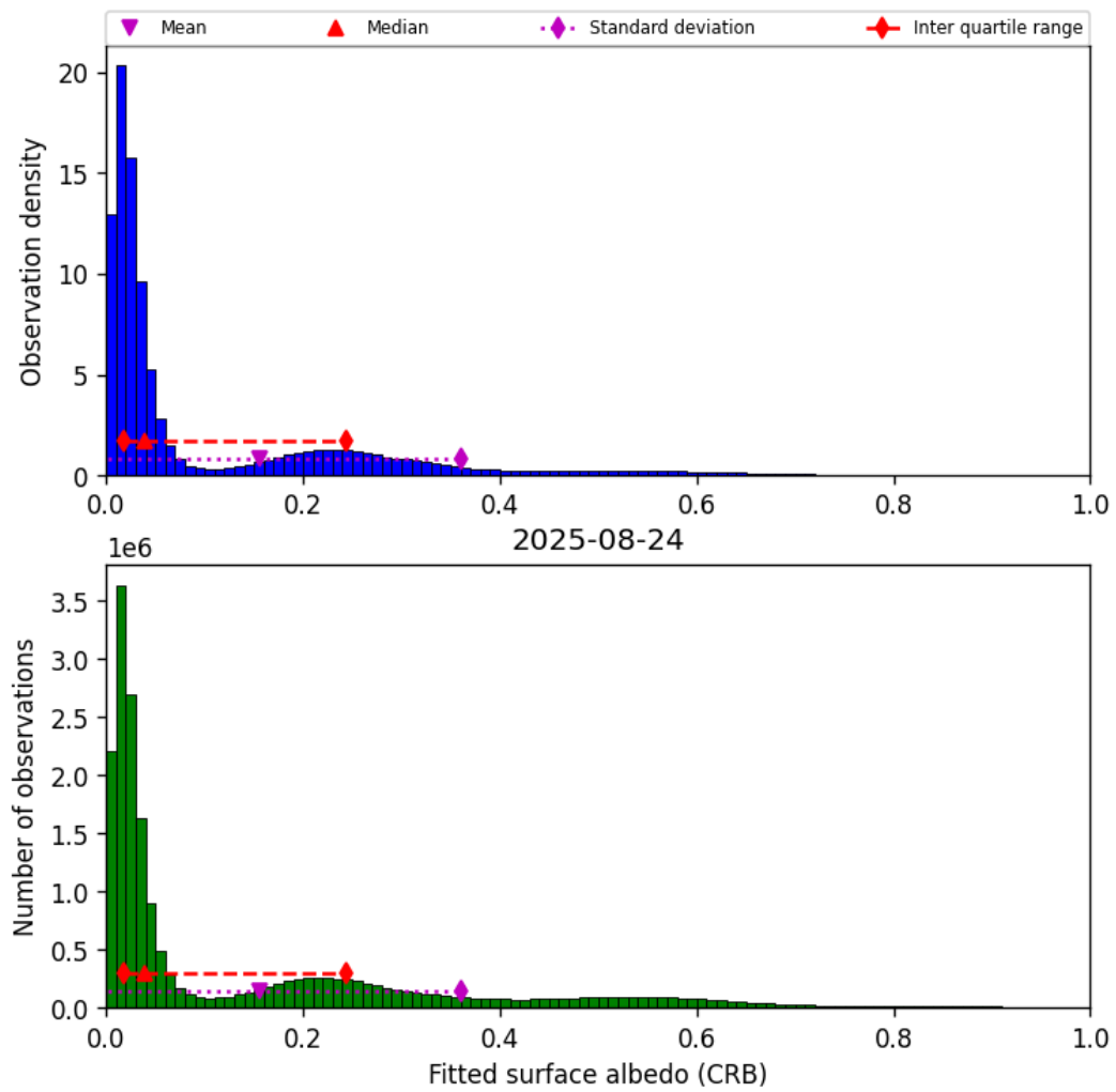
Figure 44: Histogram of “Fitted surface albedo (CRB)” for 2025-08-24 to 2025-08-25
