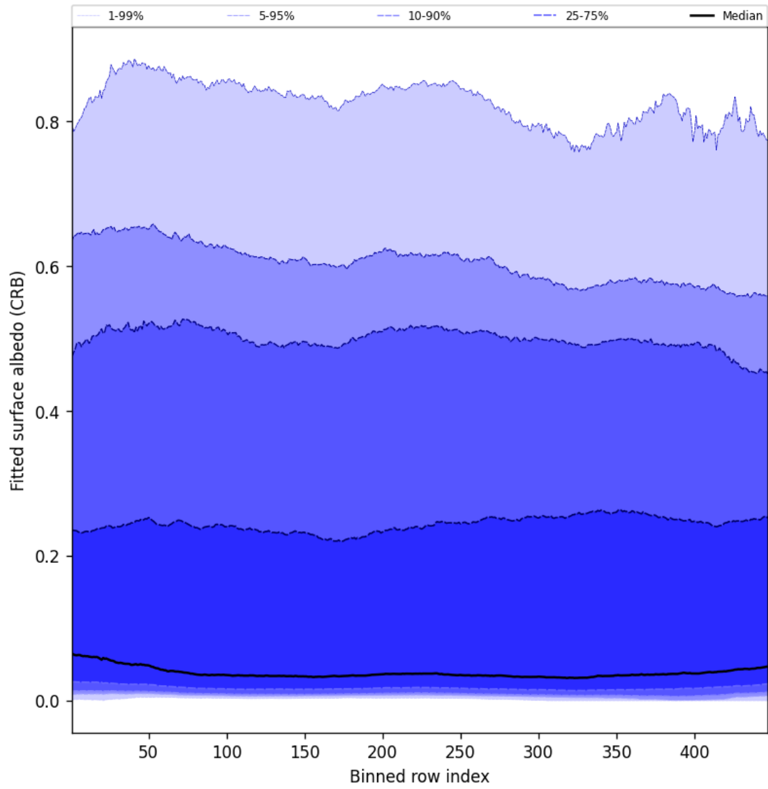
Figure 60: Along track statistics of “Fitted surface albedo (CRB)” for 2025-08-24 to 2025-08-25
