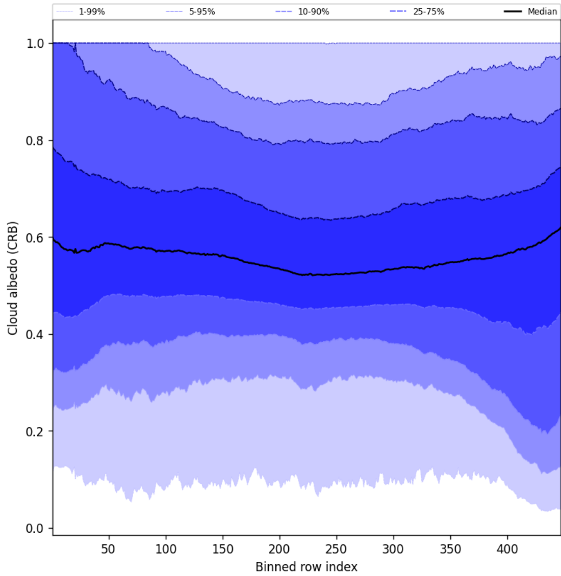
Figure 58: Along track statistics of “Cloud albedo (CRB)” for 2025-08-24 to 2025-08-25
