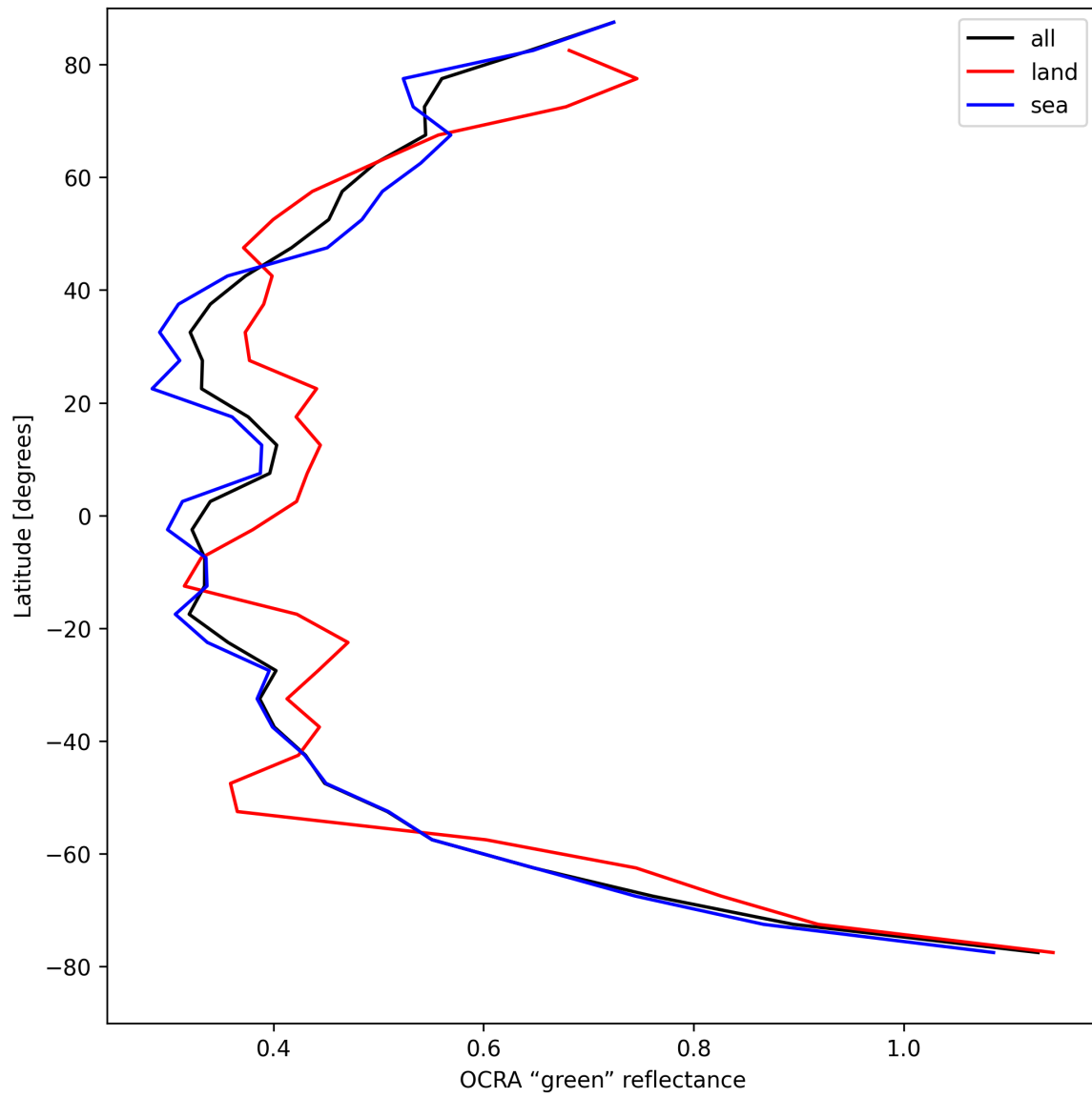
Figure 34: Zonal average of “OCRA “green” reflectance” for 2025-08-24 to 2025-08-25.
