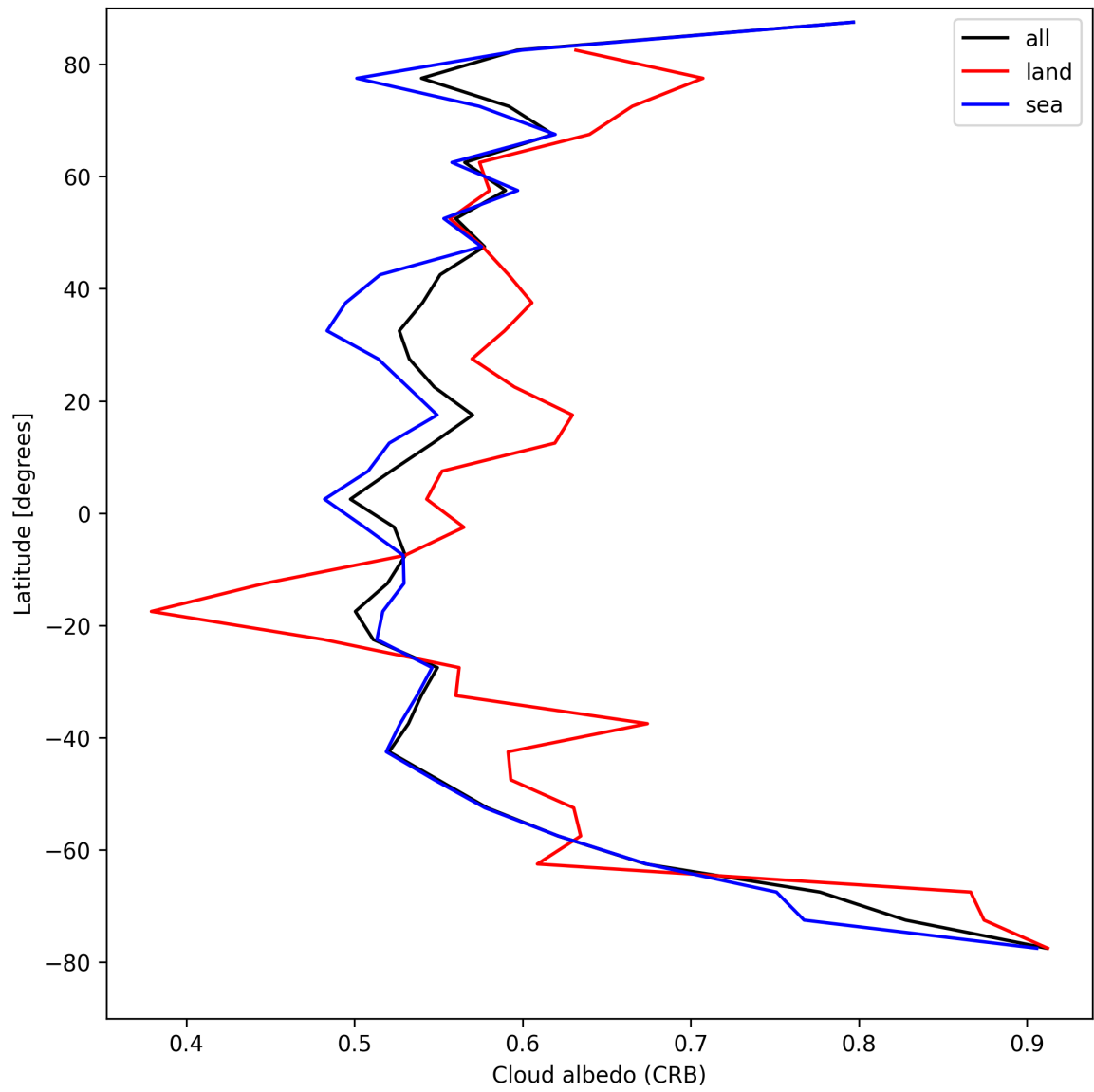
Figure 26: Zonal average of “Cloud albedo (CRB)” for 2025-08-26 to 2025-08-27.
