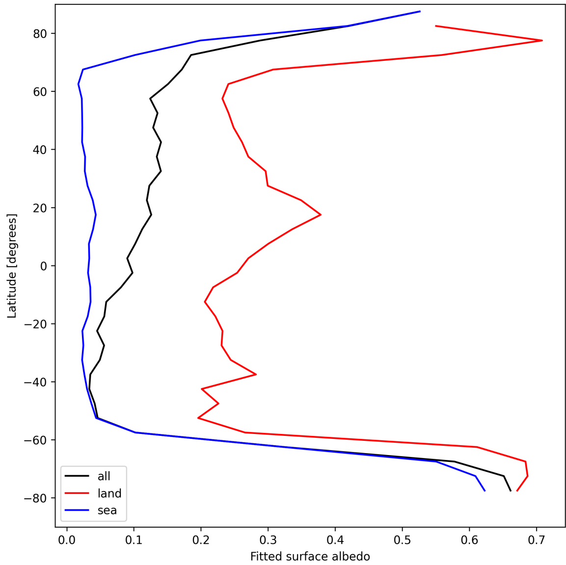
Figure 27: Zonal average of “Fitted surface albedo” for 2025-08-26 to 2025-08-27.
