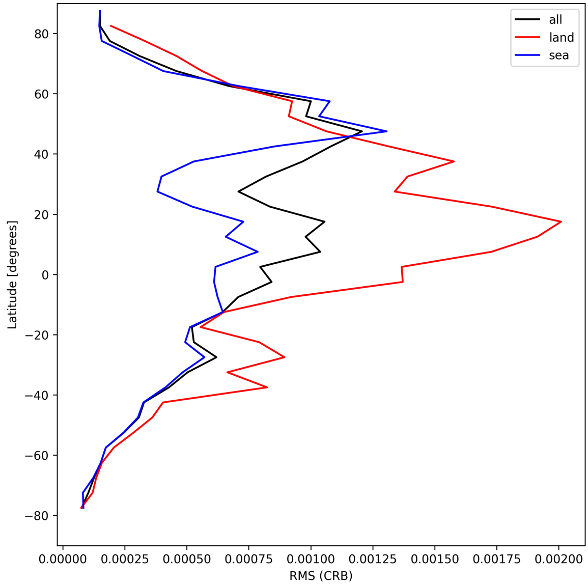
Figure 30: Zonal average of “RMS (CRB)” for 2025-08-26 to 2025-08-27.
