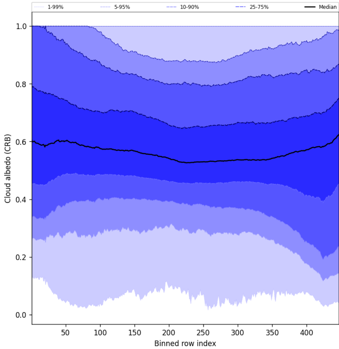
Figure 58: Along track statistics of “Cloud albedo (CRB)” for 2025-08-26 to 2025-08-27
