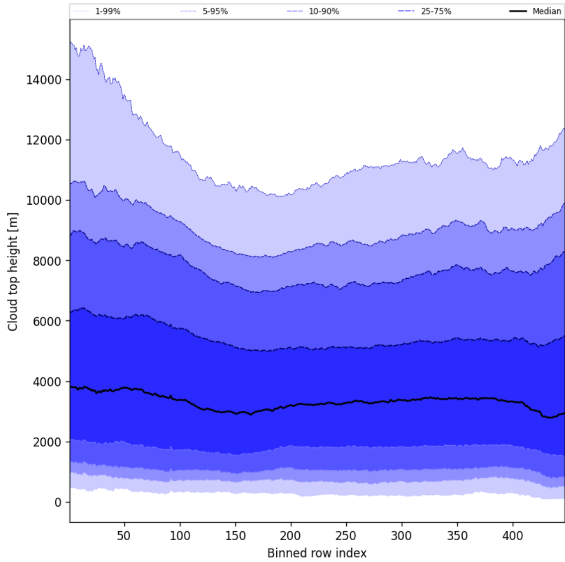
Figure 54: Along track statistics of “Cloud top height” for 2025-08-26 to 2025-08-27
