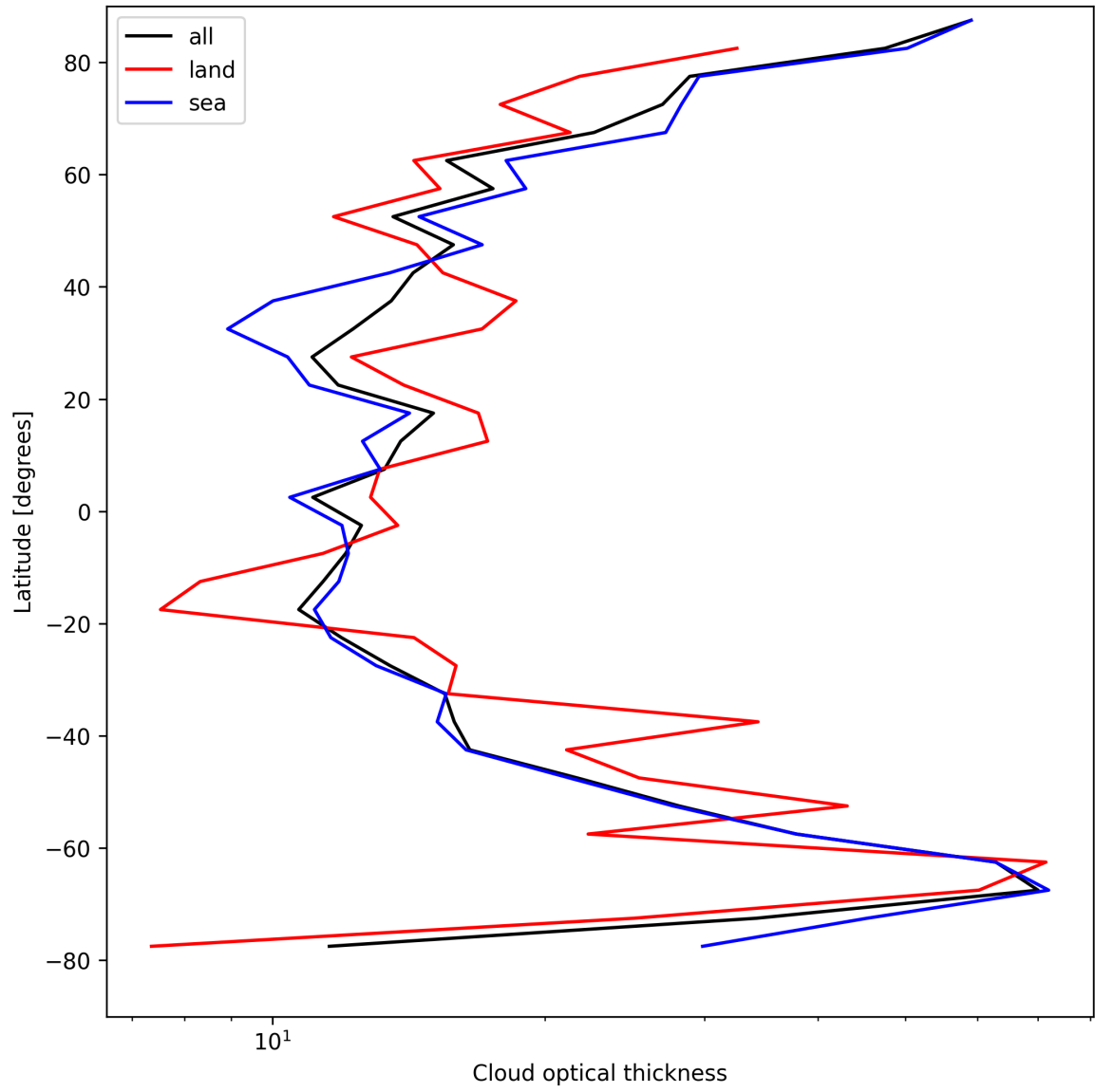
Figure 23: Zonal average of “Cloud optical thickness” for 2025-08-26 to 2025-08-27.
