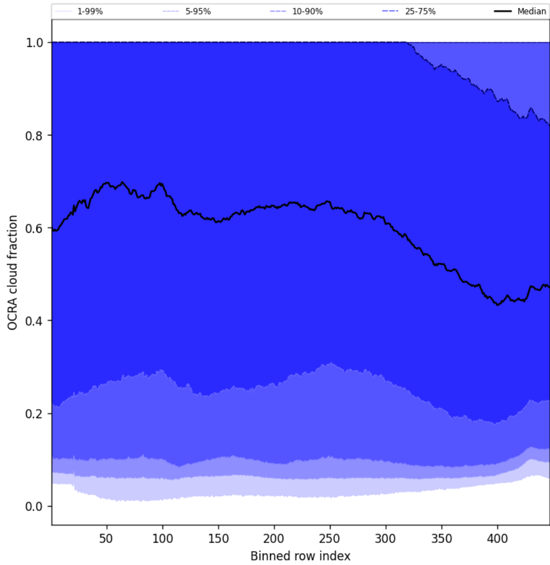
Figure 64: Along track statistics of “OCRA cloud fraction” for 2025-08-26 to 2025-08-27
