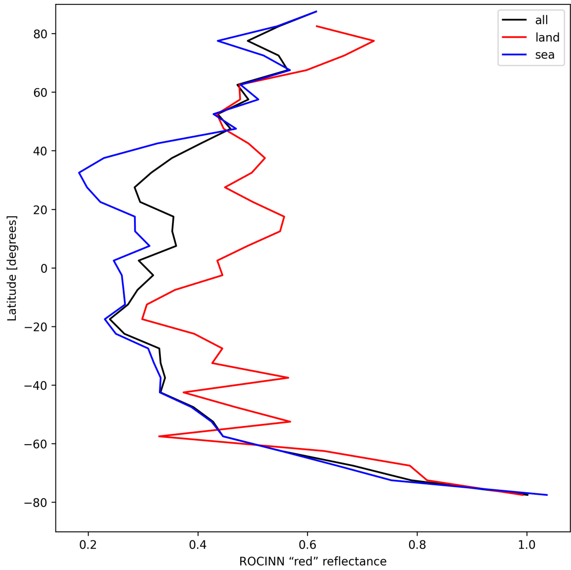
Figure 35: Zonal average of “ROCINN “red” reflectance” for 2025-08-26 to 2025-08-27.
