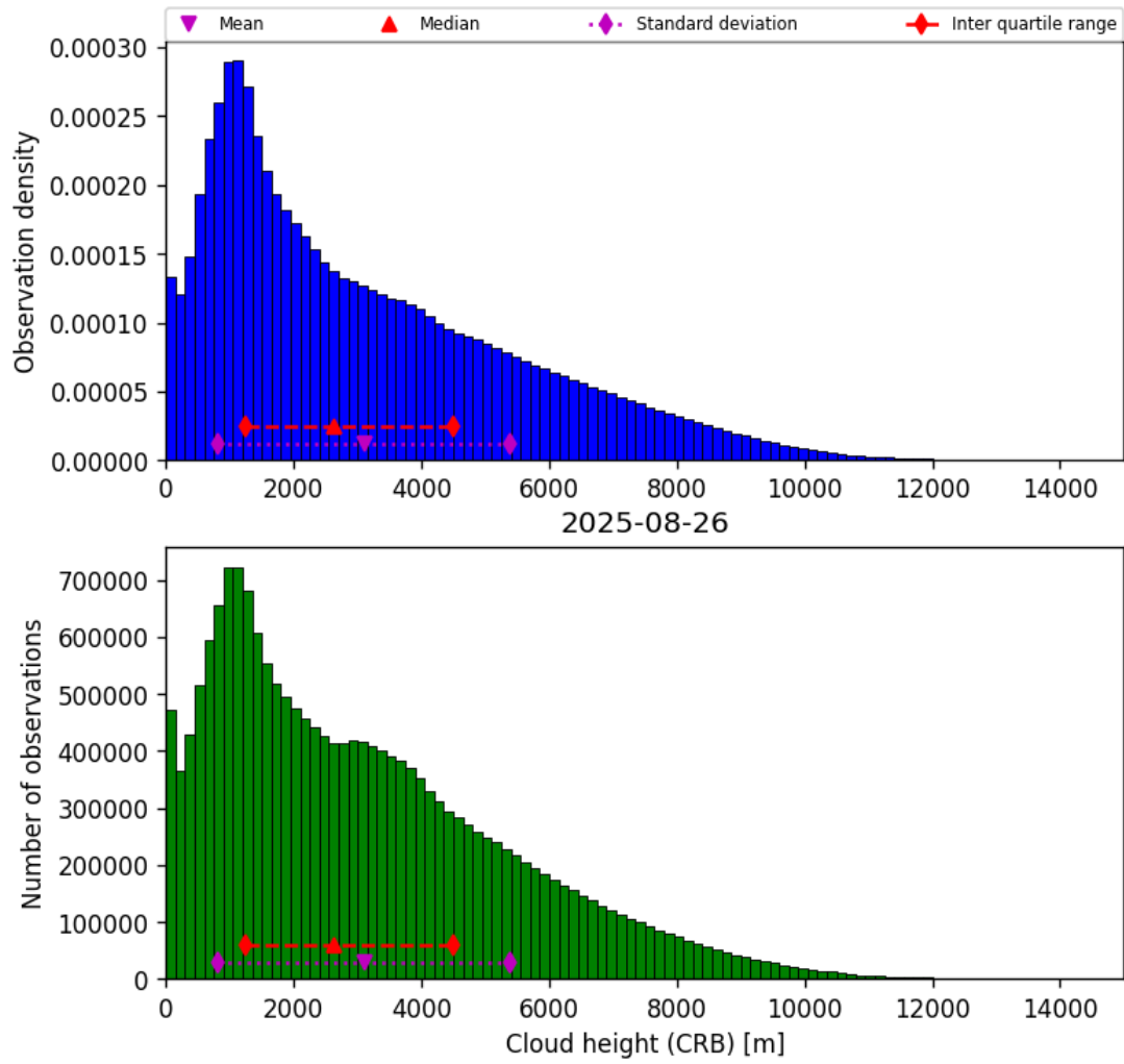
Figure 41: Histogram of “Cloud height (CRB)” for 2025-08-26 to 2025-08-27
