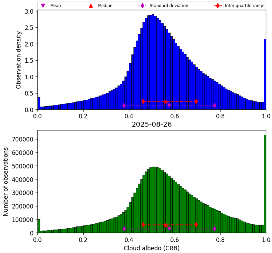
Figure 42: Histogram of “Cloud albedo (CRB)” for 2025-08-26 to 2025-08-27
