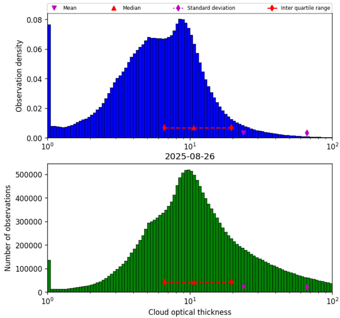
Figure 39: Histogram of “Cloud optical thickness” for 2025-08-26 to 2025-08-27
