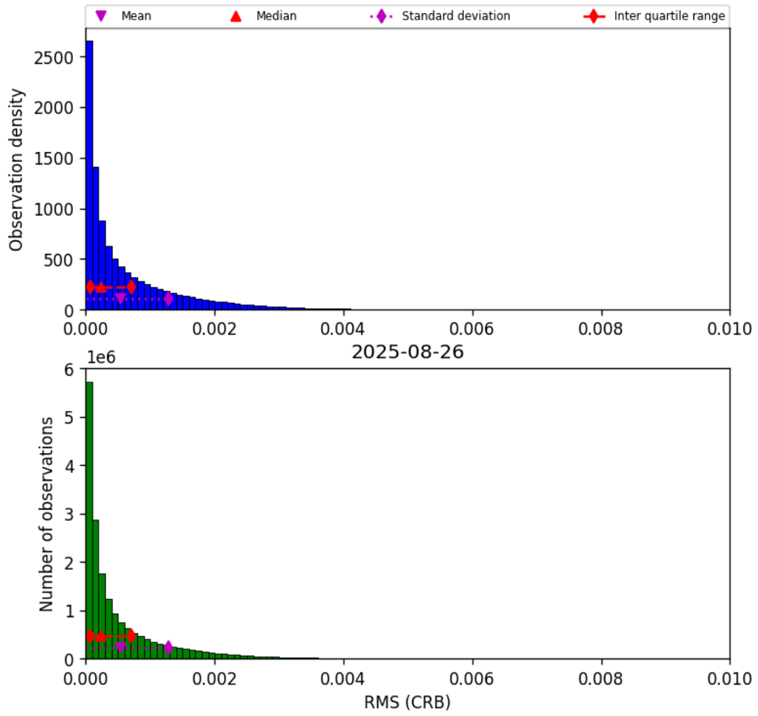
Figure 46: Histogram of “RMS (CRB)” for 2025-08-26 to 2025-08-27
