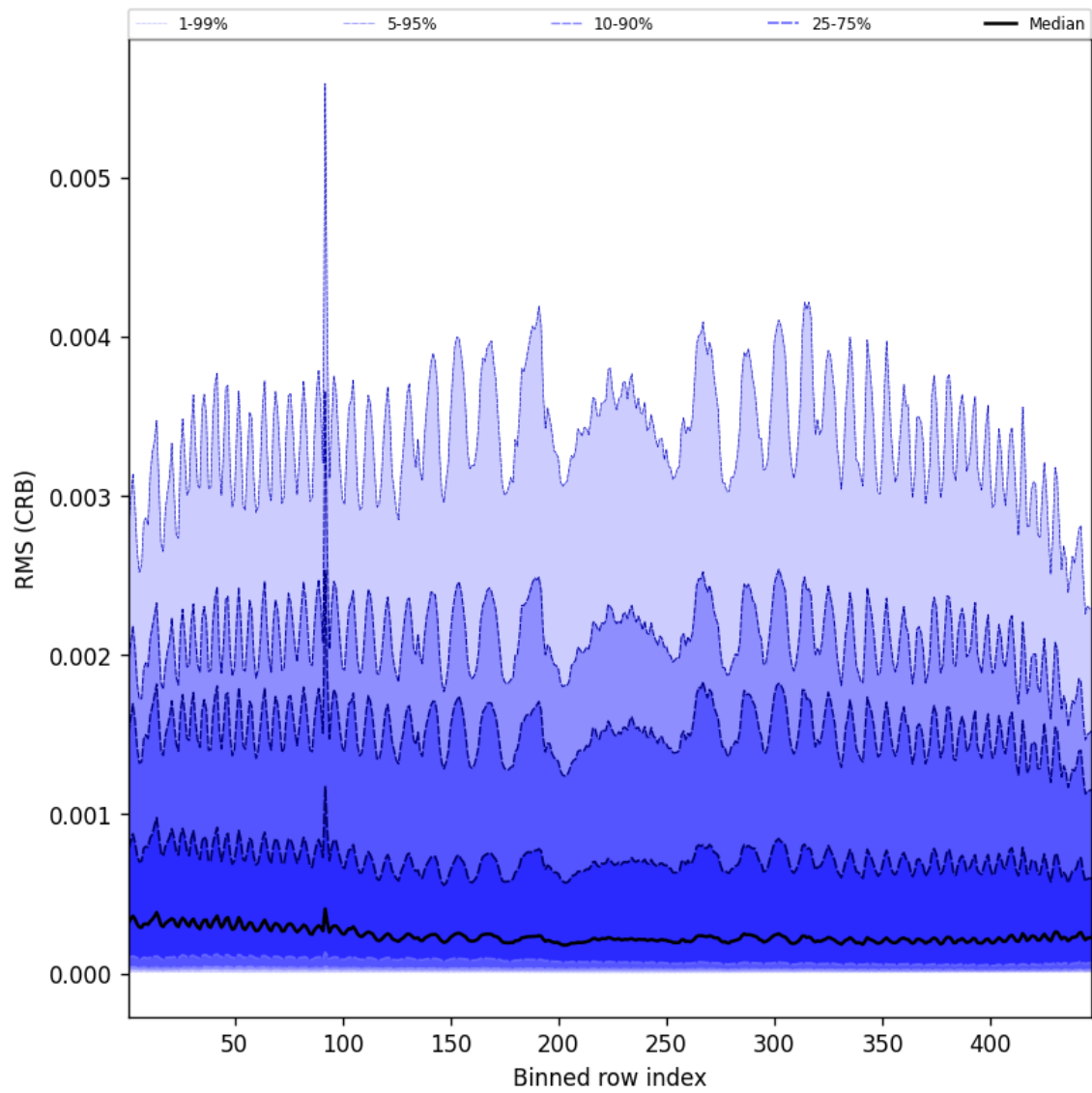
Figure 62: Along track statistics of “RMS (CRB)” for 2025-08-26 to 2025-08-27
