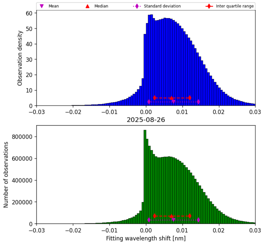
Figure 47: Histogram of “Fitting wavelength shift” for 2025-08-26 to 2025-08-27
