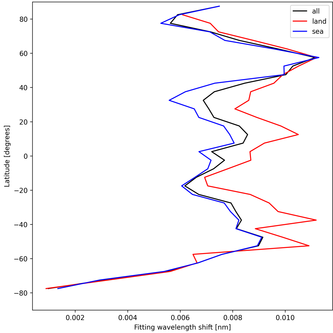
Figure 31: Zonal average of “Fitting wavelength shift” for 2025-08-26 to 2025-08-27.
