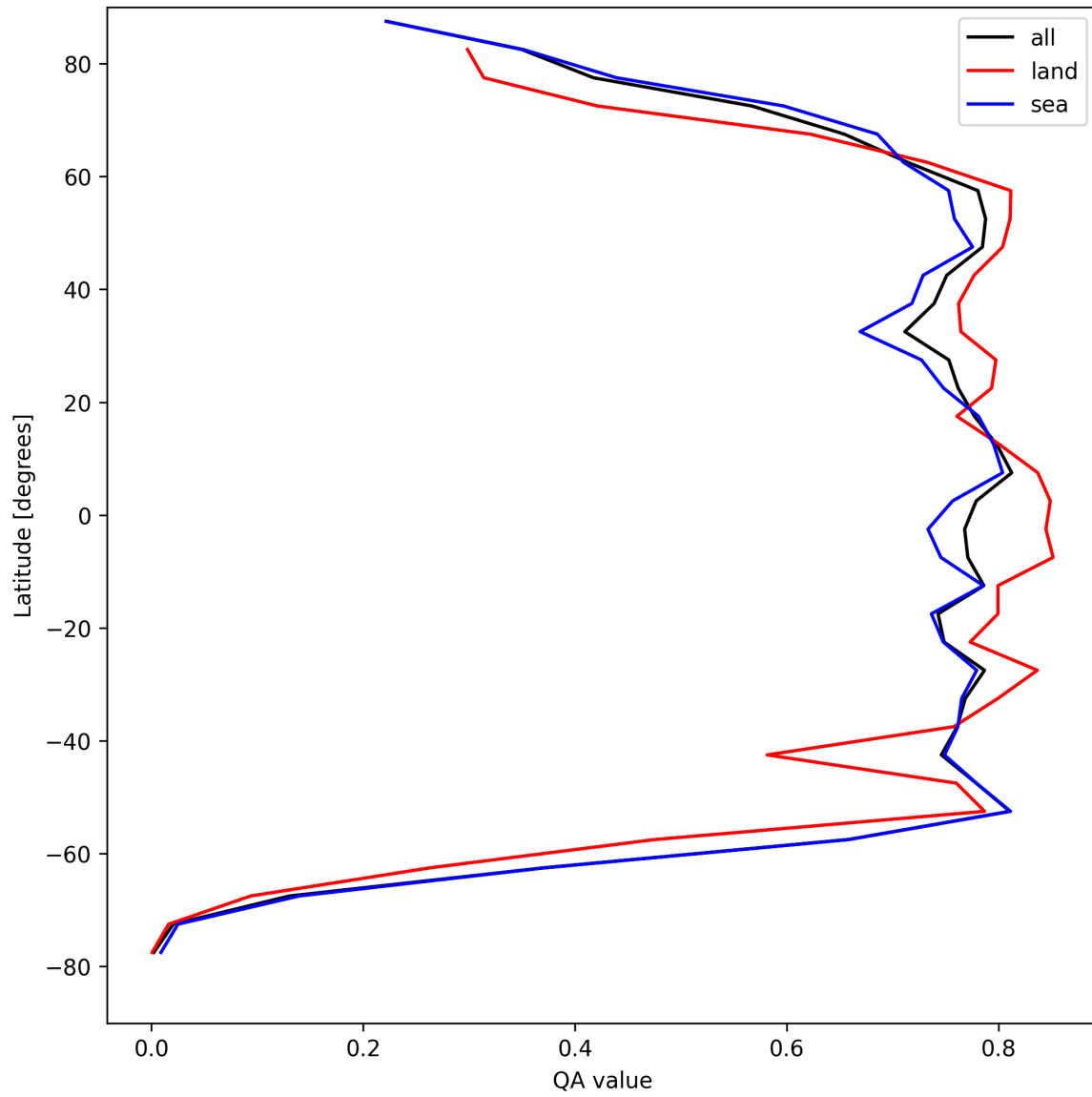
Figure 20: Zonal average of “QA value” for 2025-08-26 to 2025-08-27.
