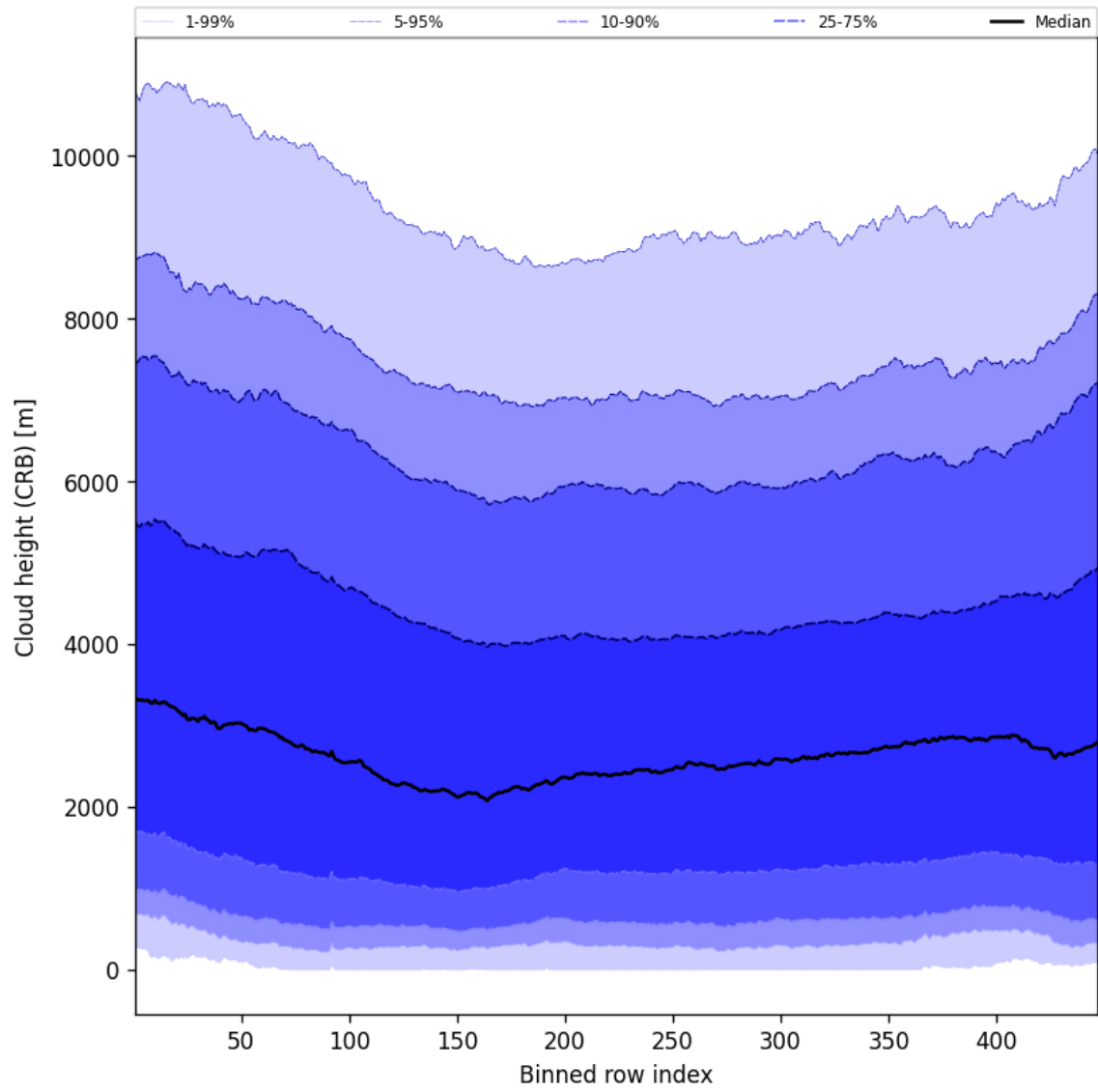
Figure 57: Along track statistics of “Cloud height (CRB)” for 2025-08-26 to 2025-08-27
