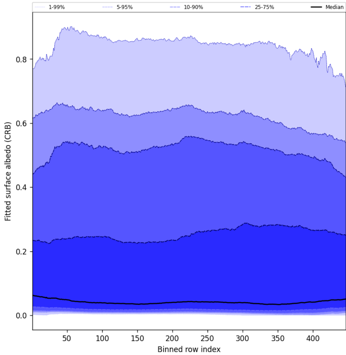
Figure 60: Along track statistics of “Fitted surface albedo (CRB)” for 2025-08-26 to 2025-08-27
