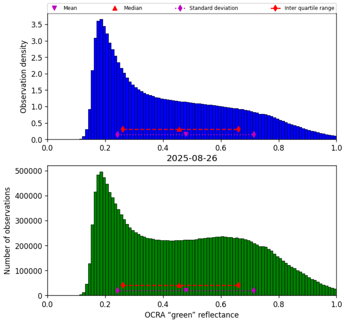
Figure 50: Histogram of “OCRA “green” reflectance” for 2025-08-26 to 2025-08-27
