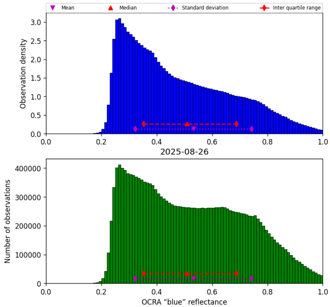
Figure 49: Histogram of “OCRA “blue” reflectance” for 2025-08-26 to 2025-08-27
