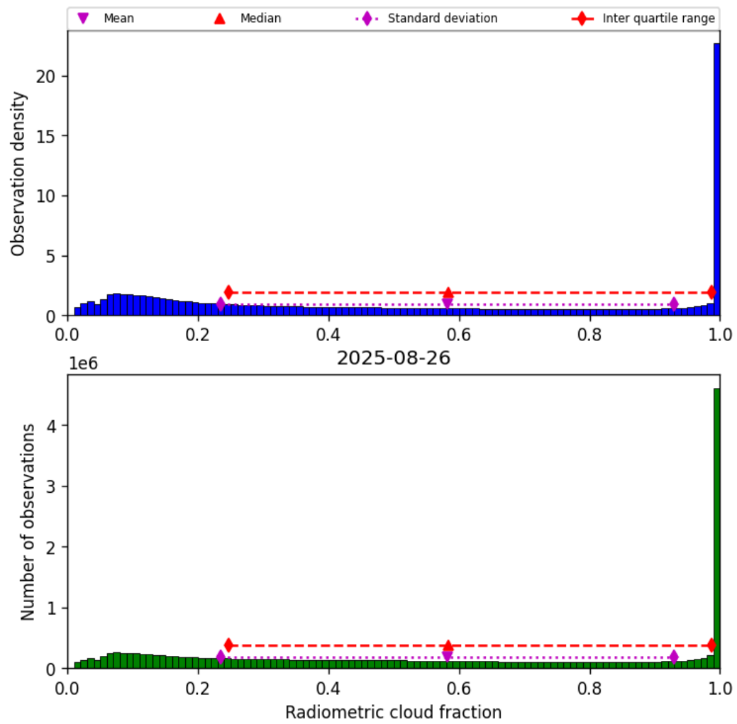
Figure 37: Histogram of “Radiometric cloud fraction” for 2025-08-26 to 2025-08-27
