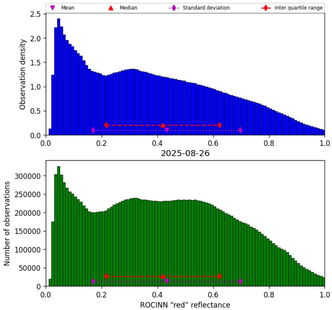
Figure 51: Histogram of "ROCINN "red" reflectance" for 2025-08-26 to 2025-08-27
