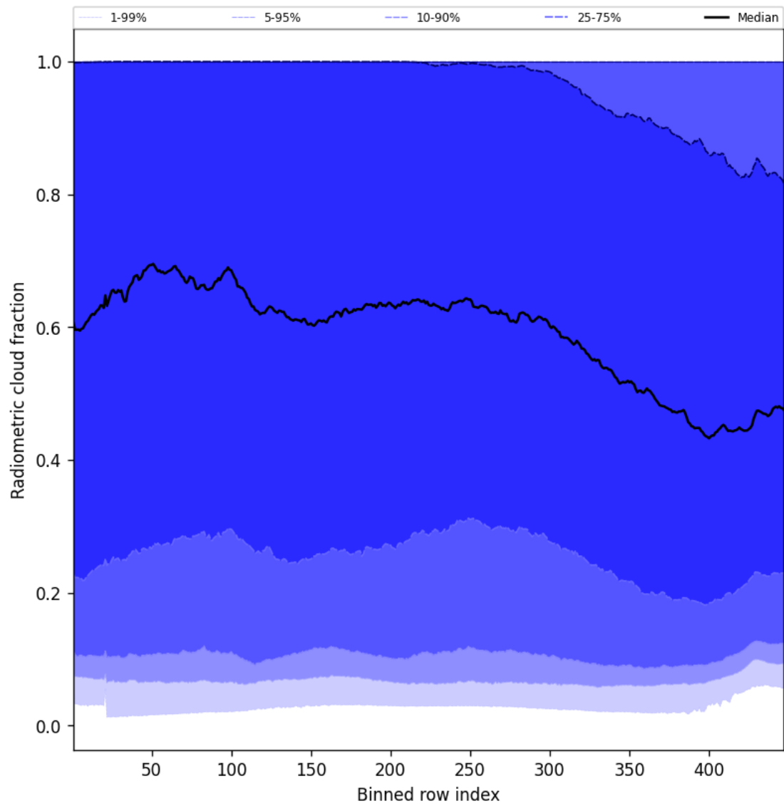
Figure 53: Along track statistics of “Radiometric cloud fraction” for 2025-08-26 to 2025-08-27
