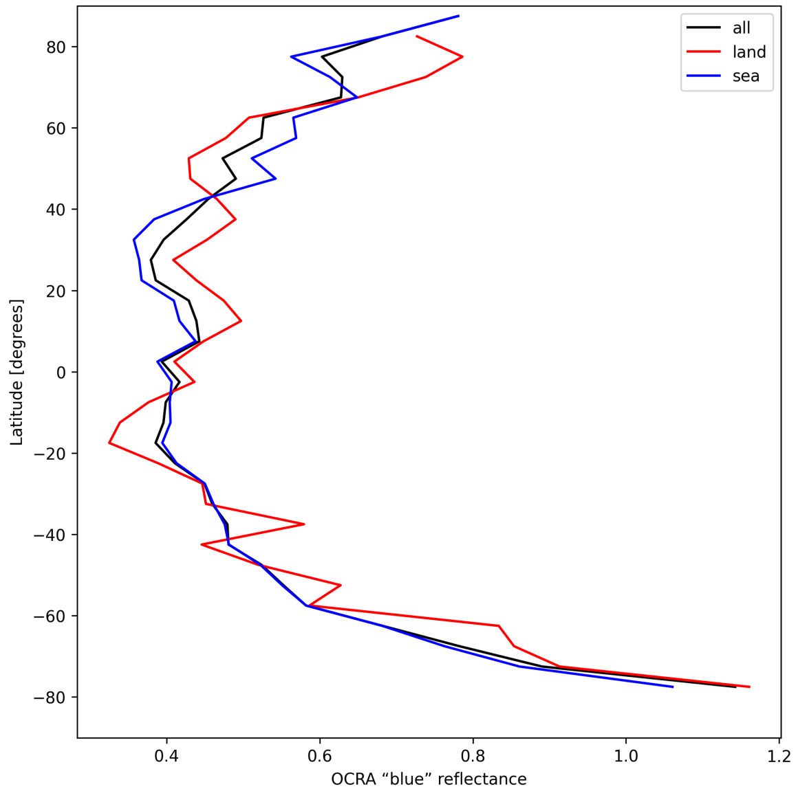
Figure 33: Zonal average of "OCRA "blue" reflectance" for 2025-08-26 to 2025-08-27.
