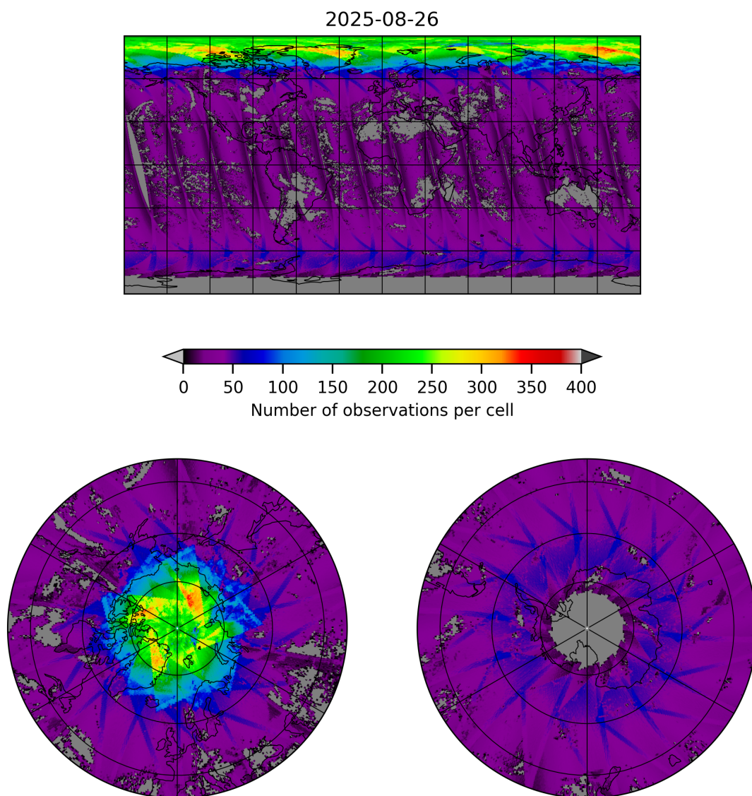
Figure 19: Map of the number of observations for 2025-08-26 to 2025-08-27
