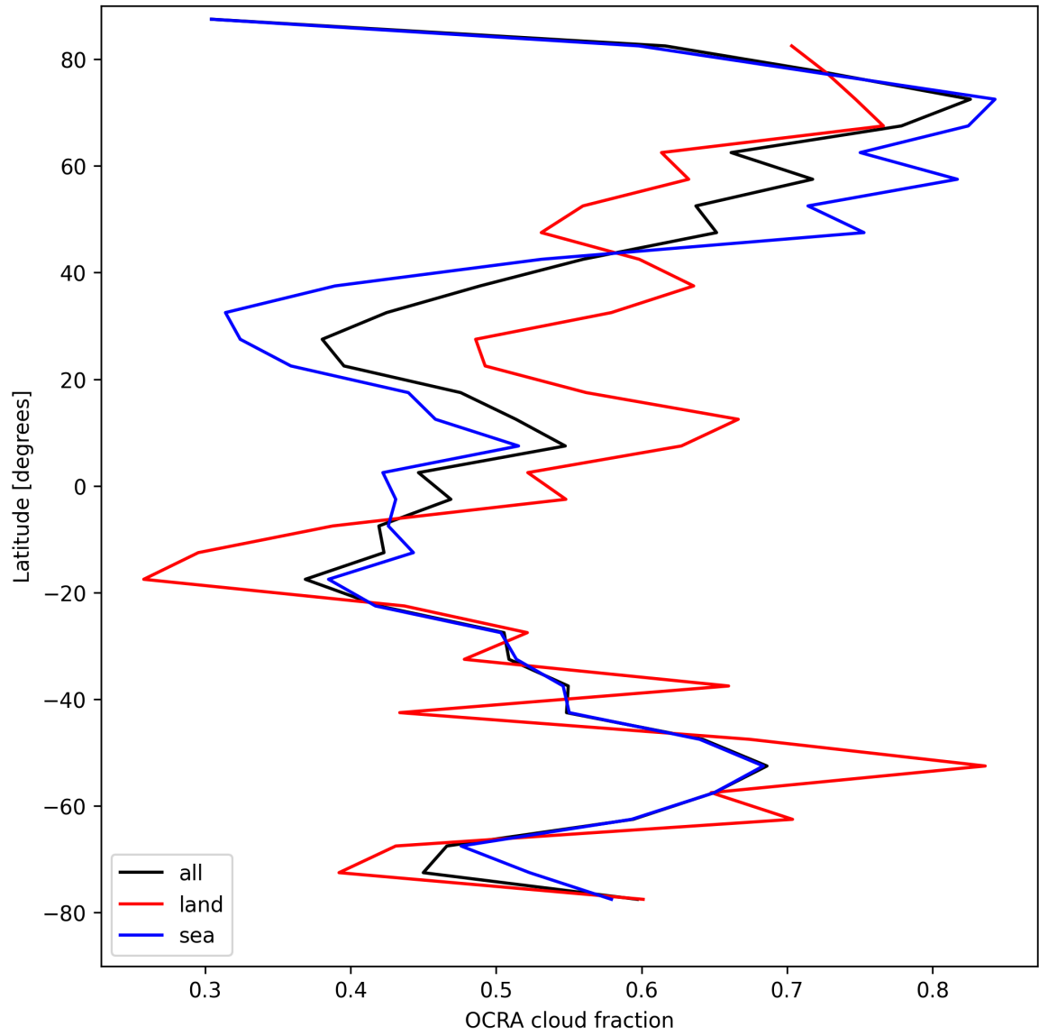
Figure 32: Zonal average of “OCRA cloud fraction” for 2025-08-26 to 2025-08-27.
