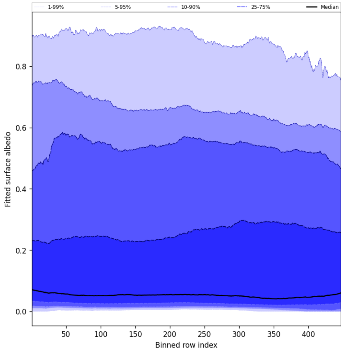
Figure 59: Along track statistics of “Fitted surface albedo” for 2025-08-26 to 2025-08-27
