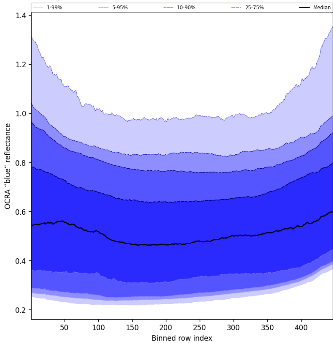
Figure 65: Along track statistics of “OCRA “blue” reflectance” for 2025-08-26 to 2025-08-27
