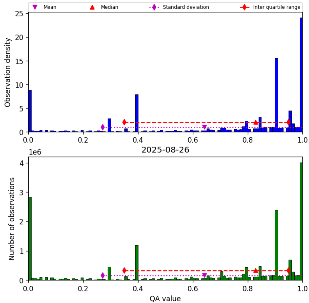
Figure 36: Histogram of “QA value” for 2025-08-26 to 2025-08-27
