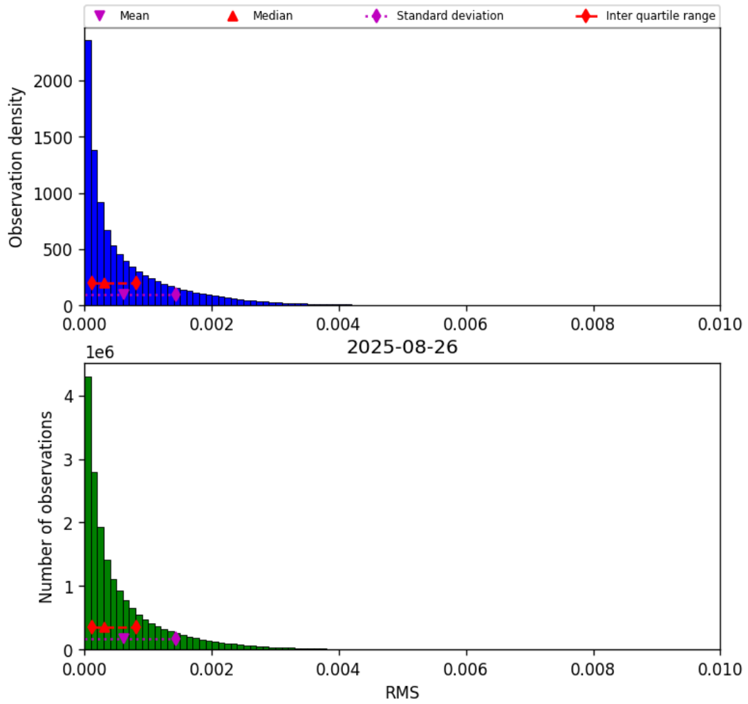
Figure 45: Histogram of “RMS” for 2025-08-26 to 2025-08-27
