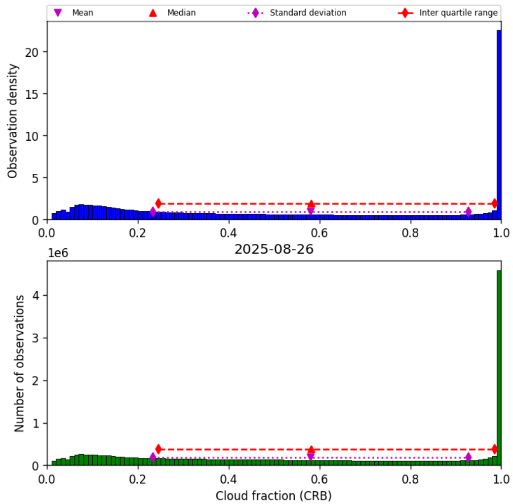
Figure 40: Histogram of “Cloud fraction (CRB)” for 2025-08-26 to 2025-08-27
