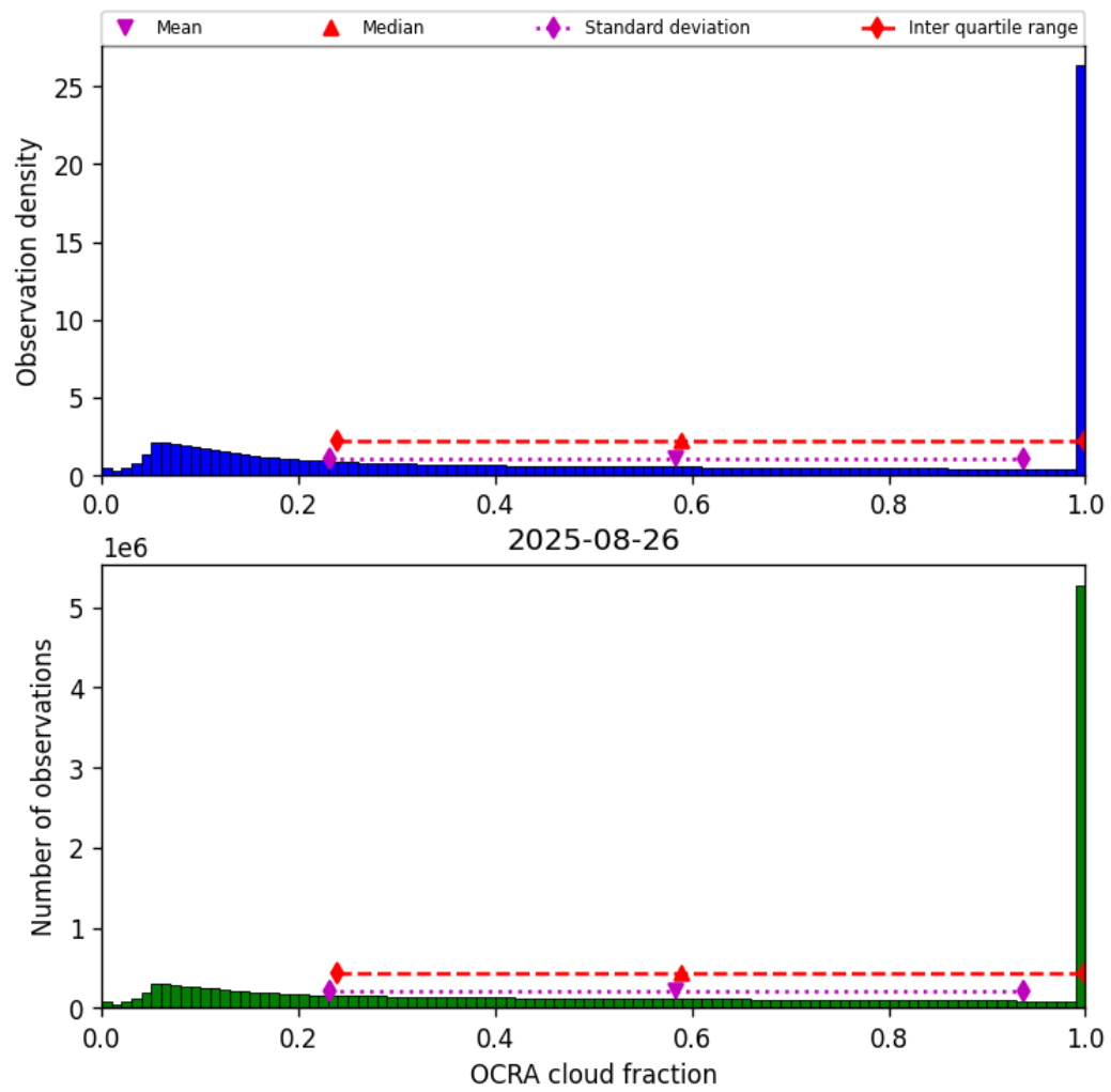
Figure 48: Histogram of “OCRA cloud fraction” for 2025-08-26 to 2025-08-27
