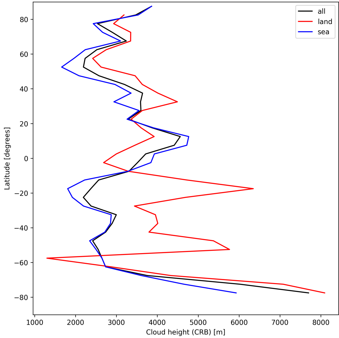
Figure 25: Zonal average of “Cloud height (CRB)” for 2025-08-26 to 2025-08-27.
