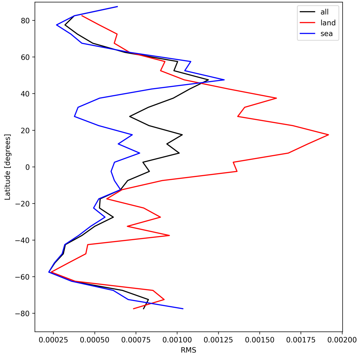
Figure 29: Zonal average of “RMS” for 2025-08-26 to 2025-08-27.
