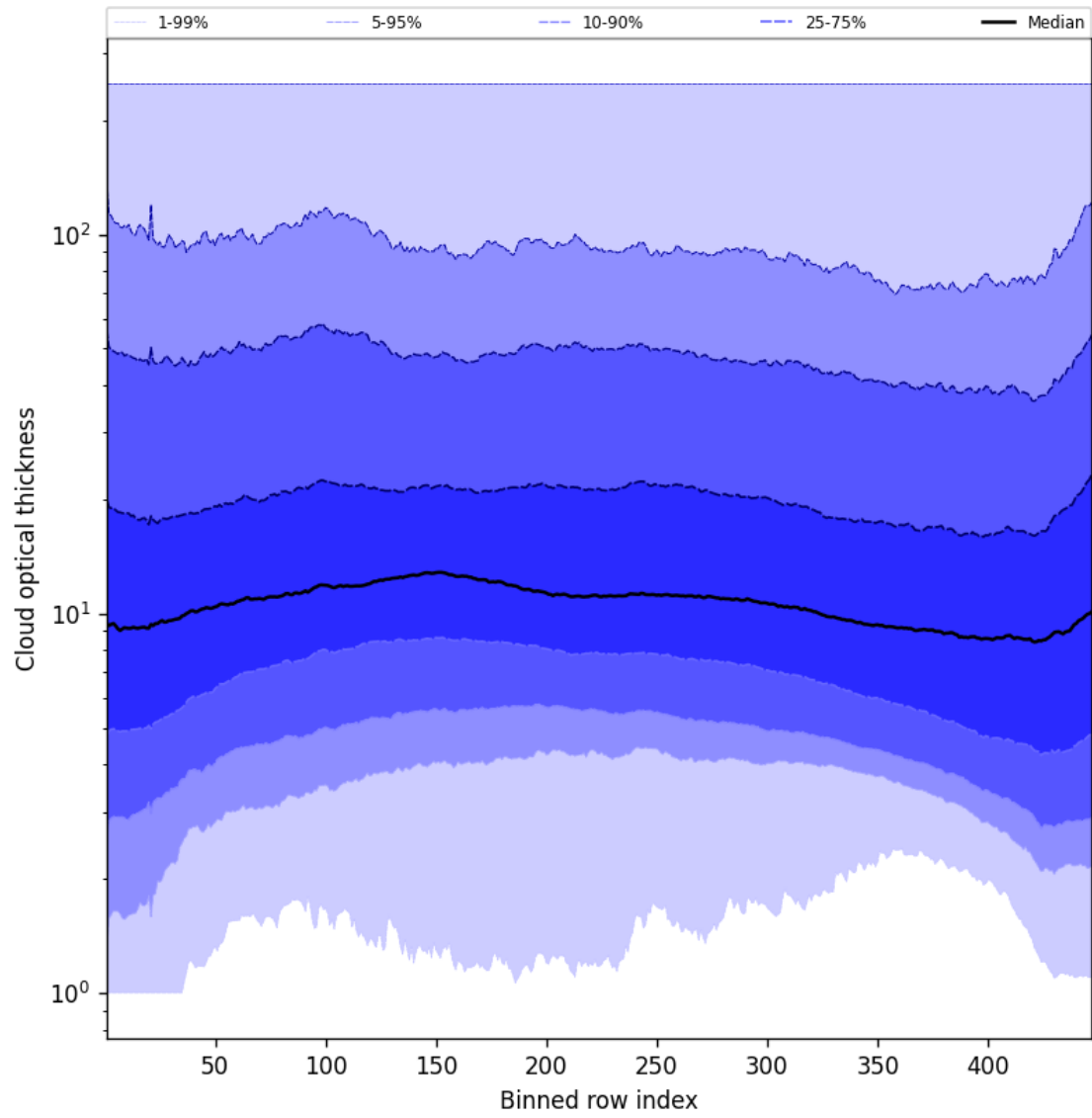
Figure 55: Along track statistics of “Cloud optical thickness” for 2025-08-26 to 2025-08-27
