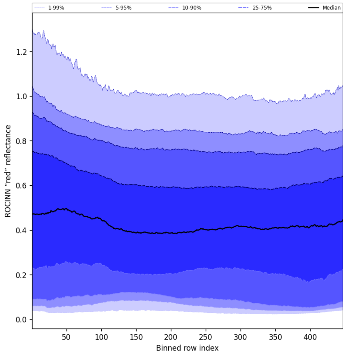
Figure 67: Along track statistics of “ROCINN “red” reflectance” for 2025-08-26 to 2025-08-27
