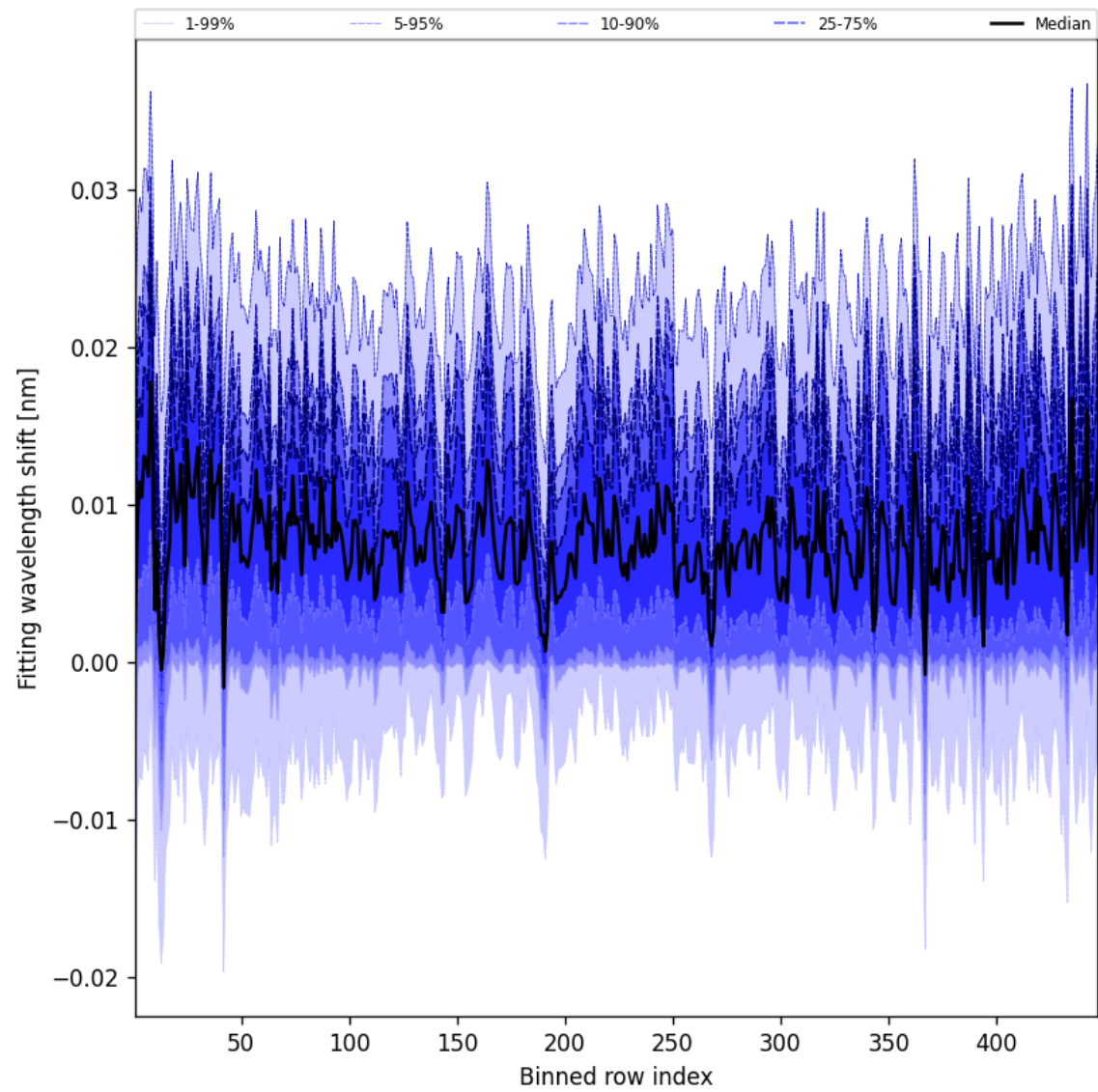
Figure 63: Along track statistics of “Fitting wavelength shift” for 2025-08-26 to 2025-08-27
