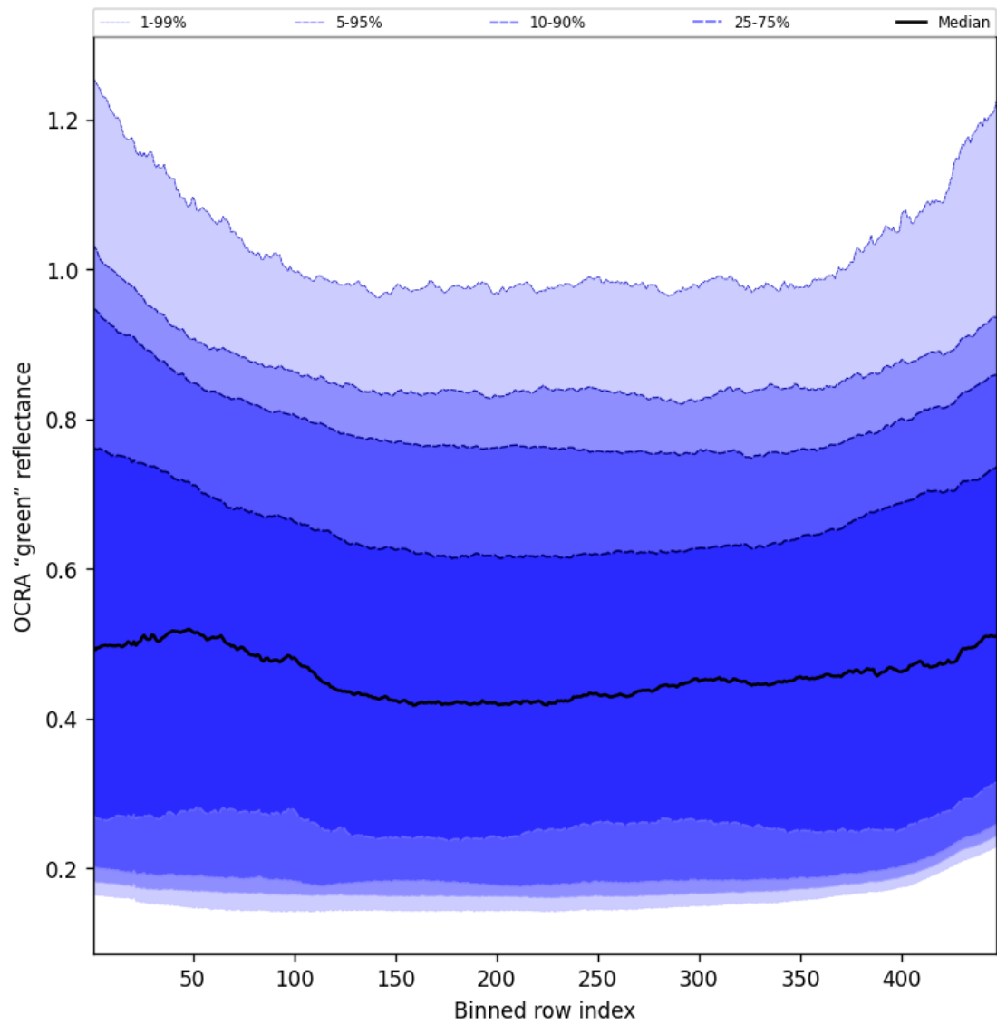
Figure 66: Along track statistics of “OCRA “green” reflectance” for 2025-08-26 to 2025-08-27
