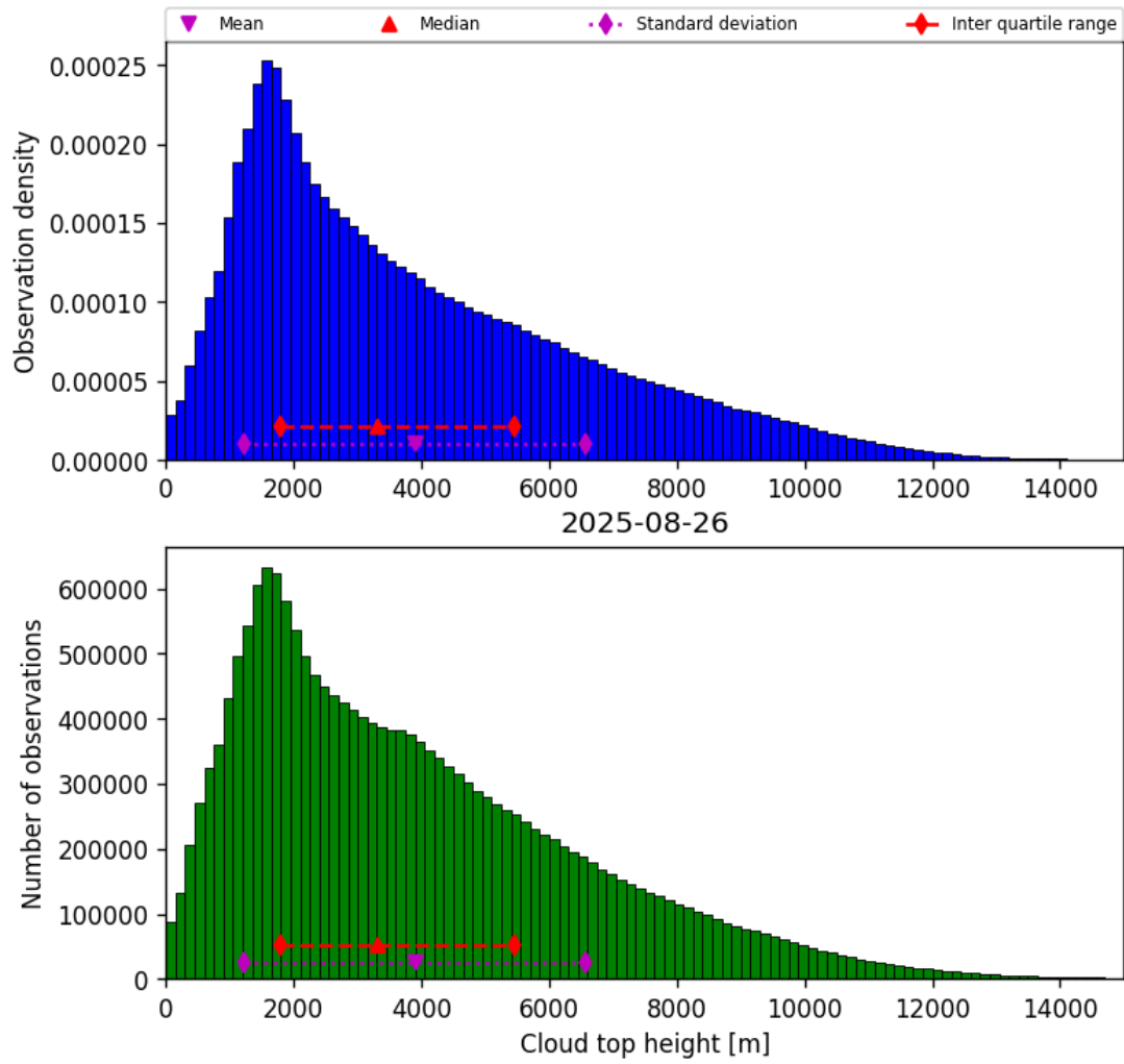
Figure 38: Histogram of “Cloud top height” for 2025-08-26 to 2025-08-27
