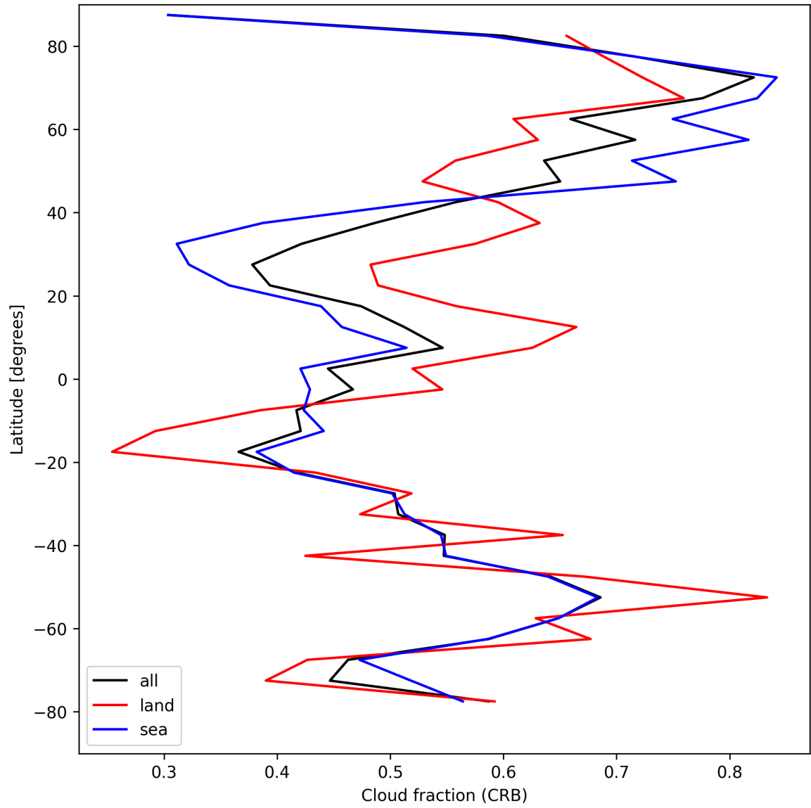
Figure 24: Zonal average of “Cloud fraction (CRB)” for 2025-08-26 to 2025-08-27.
