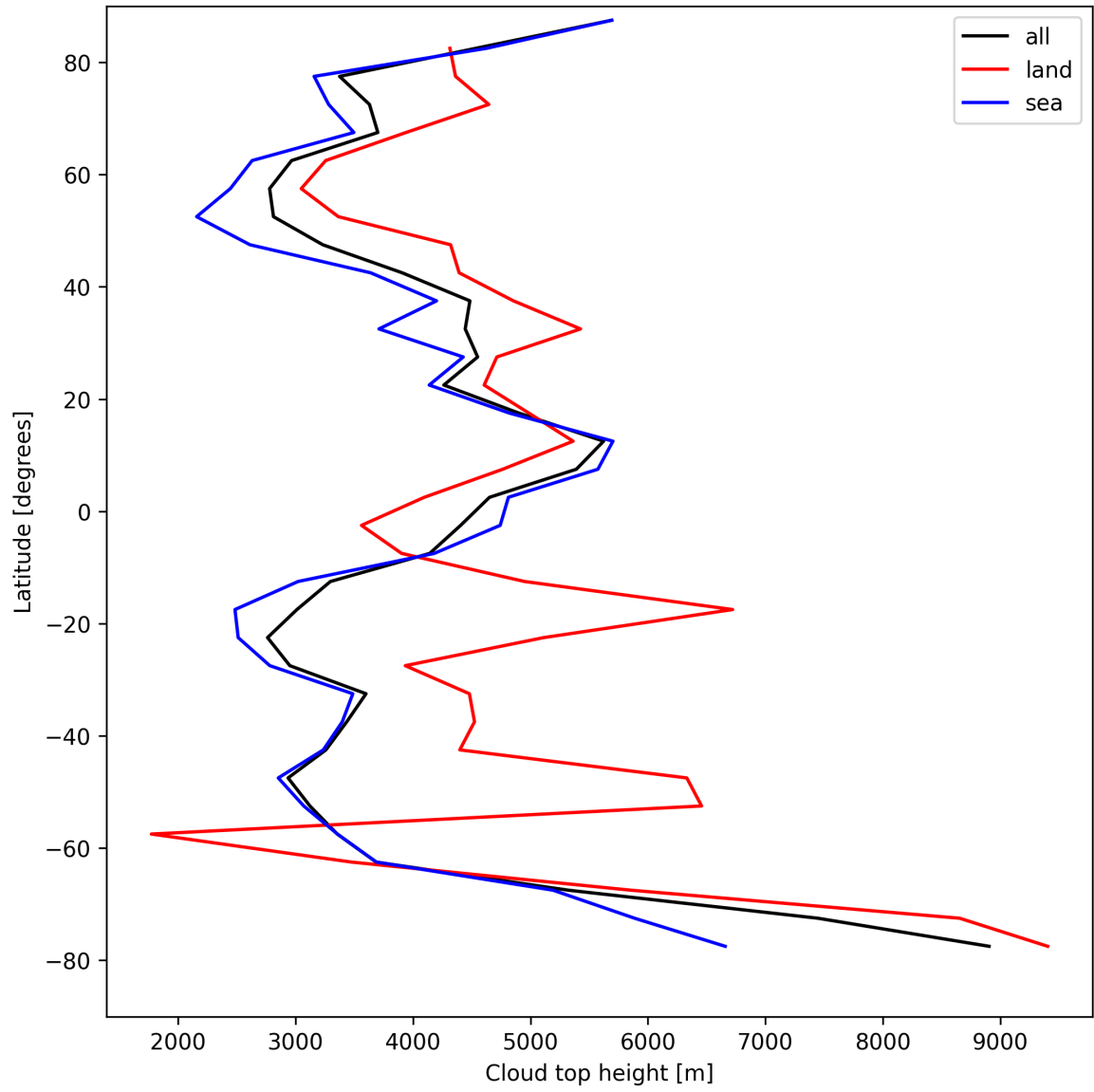
Figure 22: Zonal average of “Cloud top height” for 2025-08-26 to 2025-08-27.
