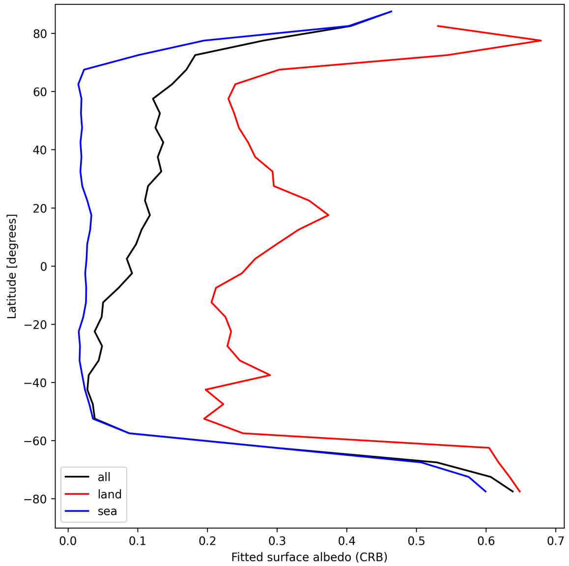
Figure 28: Zonal average of “Fitted surface albedo (CRB)” for 2025-08-26 to 2025-08-27.
