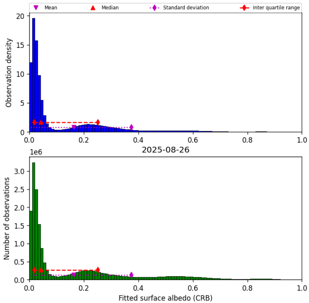
Figure 44: Histogram of “Fitted surface albedo (CRB)” for 2025-08-26 to 2025-08-27
