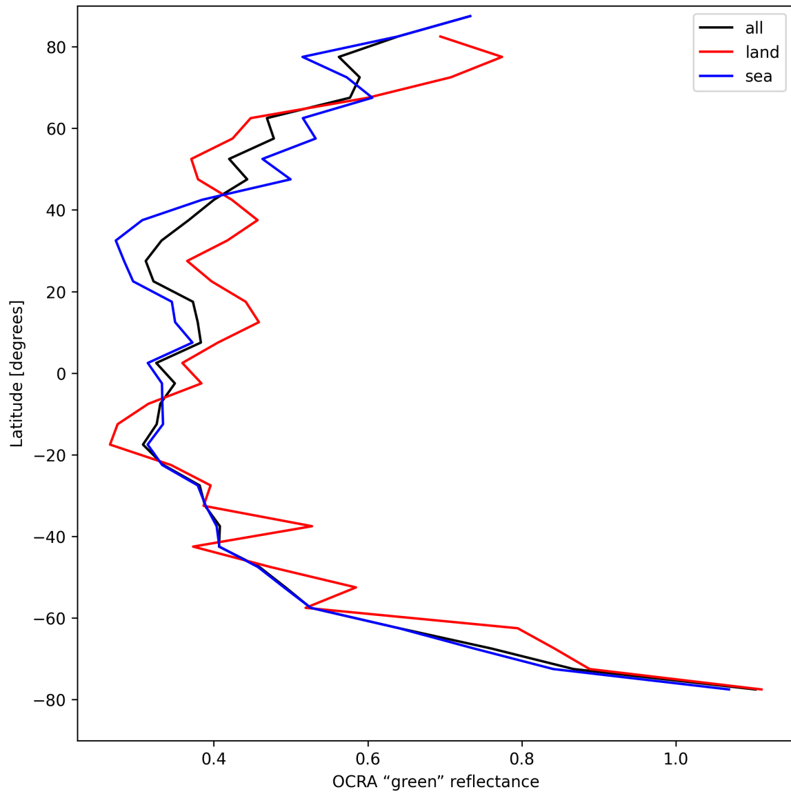
Figure 34: Zonal average of “OCRA “green” reflectance” for 2025-08-26 to 2025-08-27.
