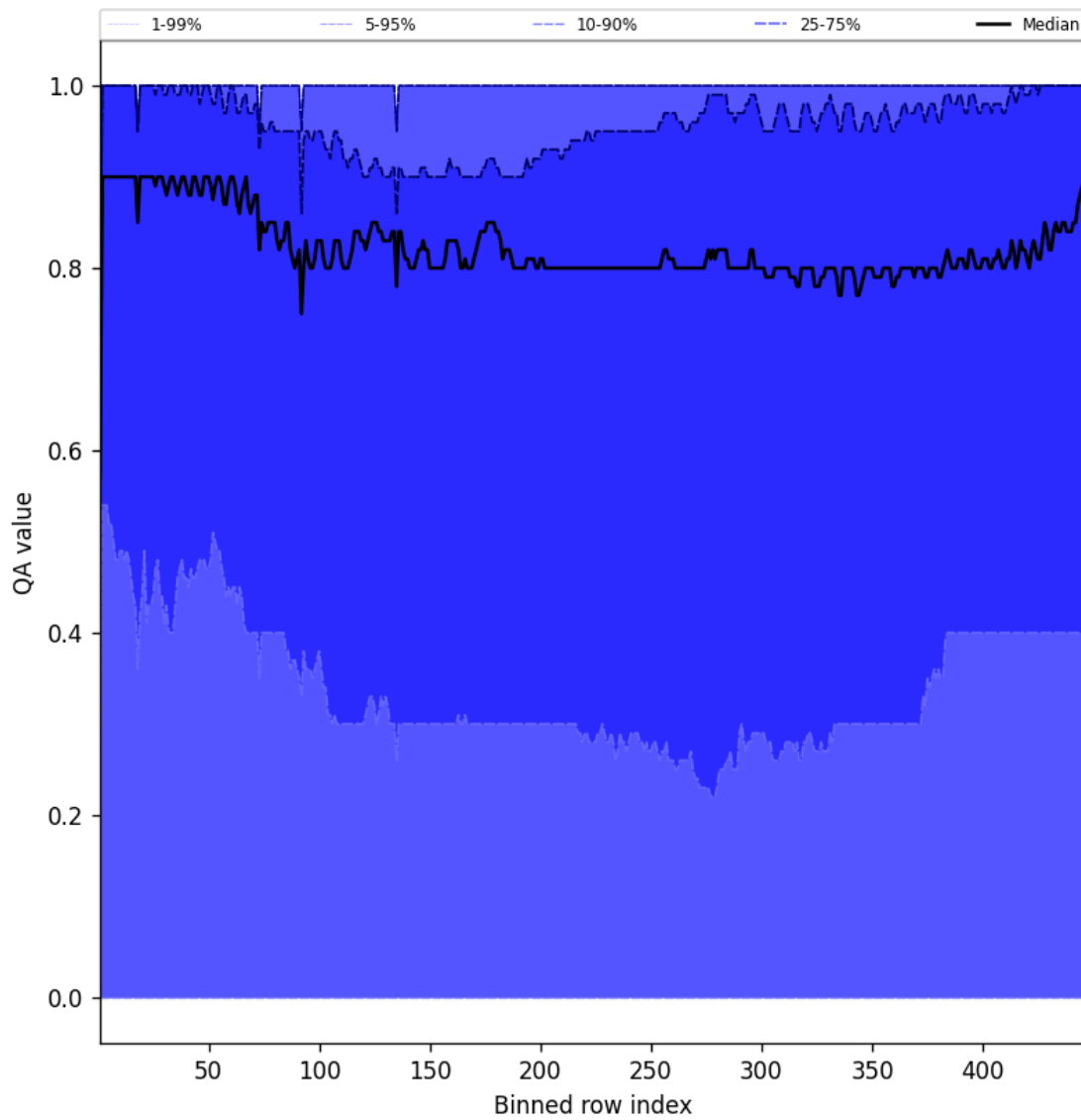
Figure 52: Along track statistics of “QA value” for 2025-08-26 to 2025-08-27
