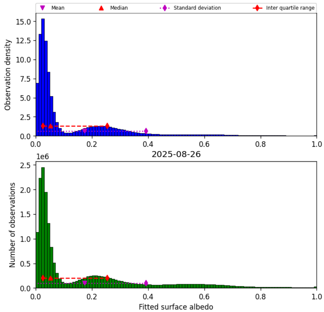
Figure 43: Histogram of “Fitted surface albedo” for 2025-08-26 to 2025-08-27
