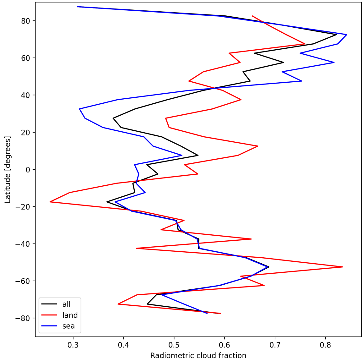
Figure 21: Zonal average of “Radiometric cloud fraction” for 2025-08-26 to 2025-08-27.
