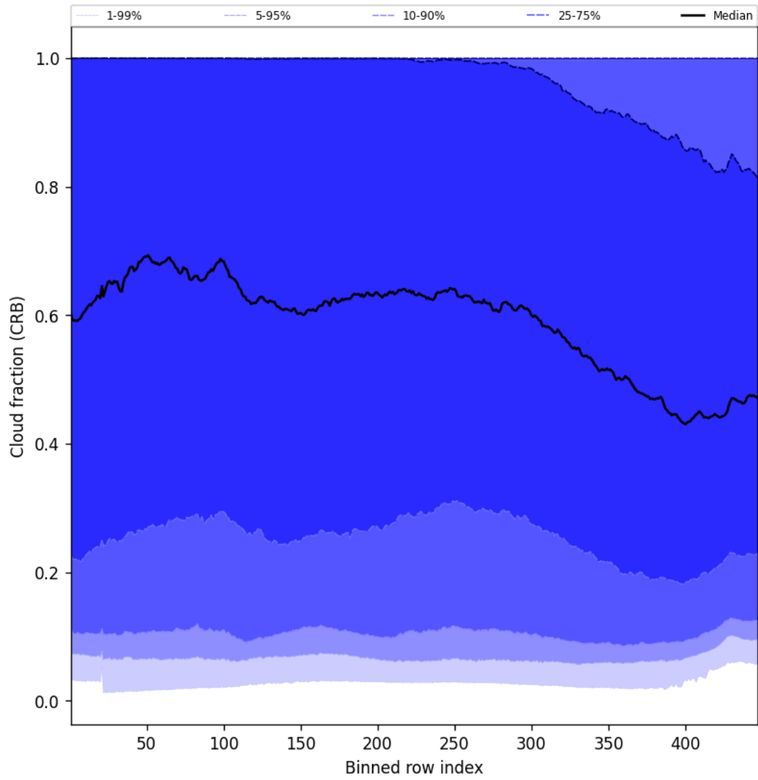
Figure 56: Along track statistics of “Cloud fraction (CRB)” for 2025-08-26 to 2025-08-27
