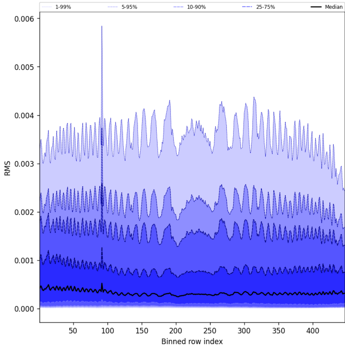
Figure 61: Along track statistics of “RMS” for 2025-08-26 to 2025-08-27
