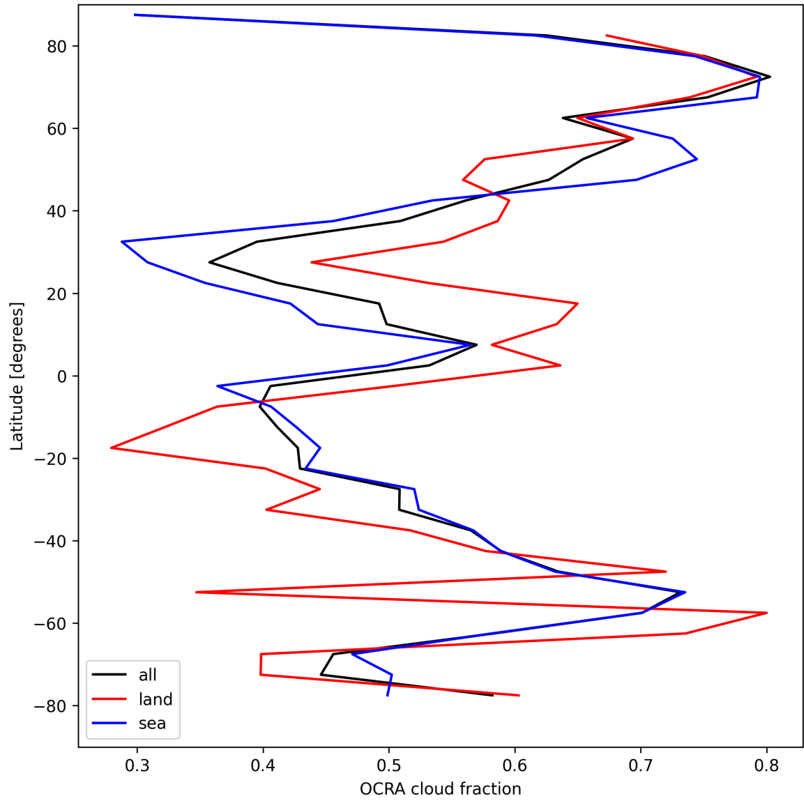
Figure 32: Zonal average of “OCRA cloud fraction” for 2025-08-27 to 2025-08-28.
