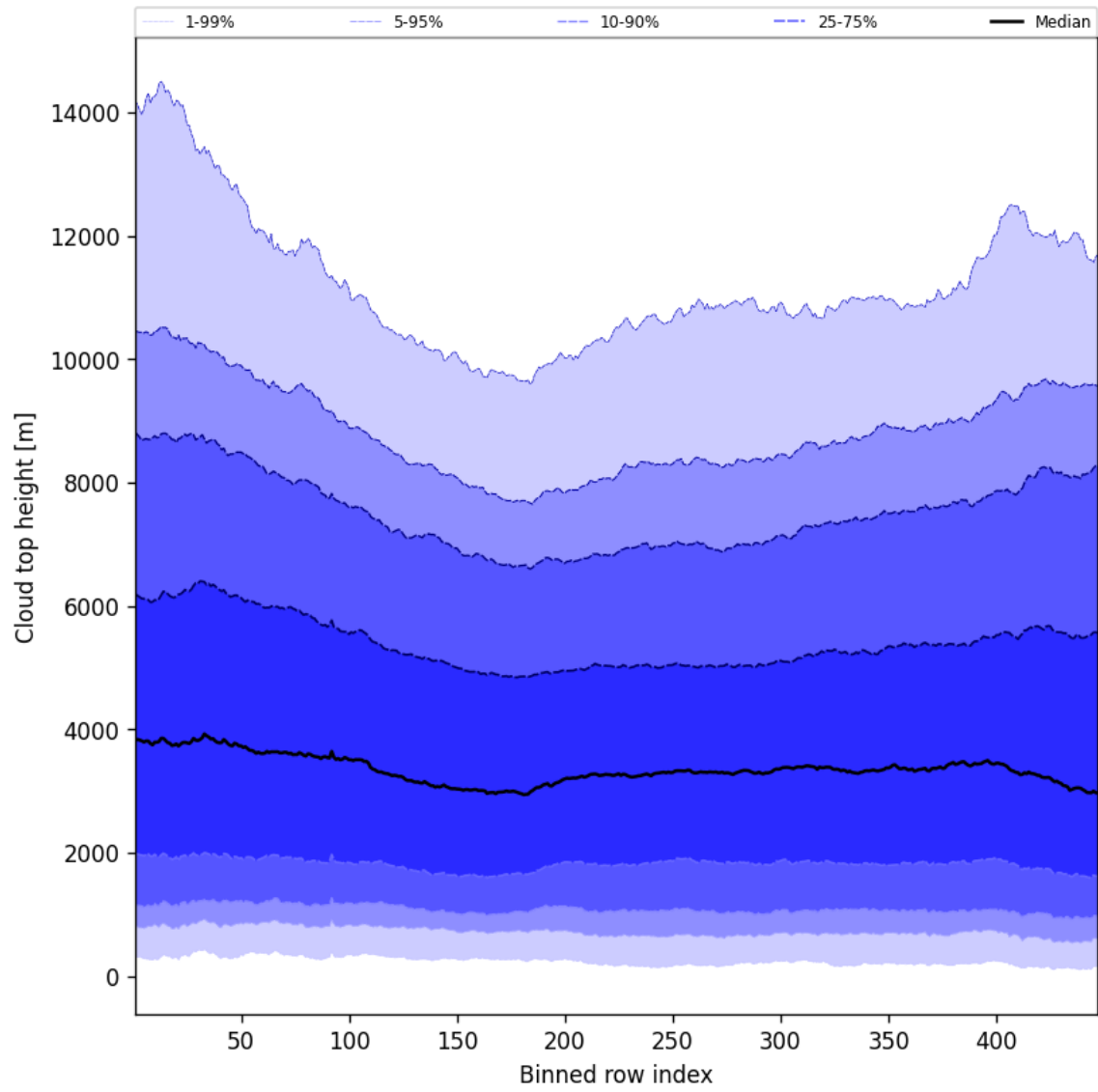
Figure 54: Along track statistics of “Cloud top height” for 2025-08-27 to 2025-08-28
