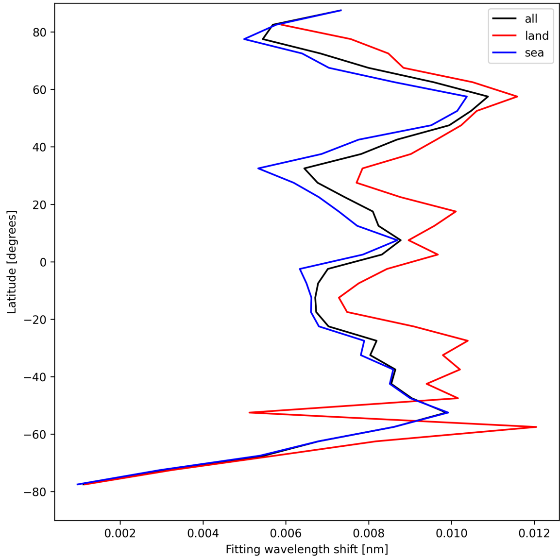
Figure 31: Zonal average of “Fitting wavelength shift” for 2025-08-27 to 2025-08-28.
