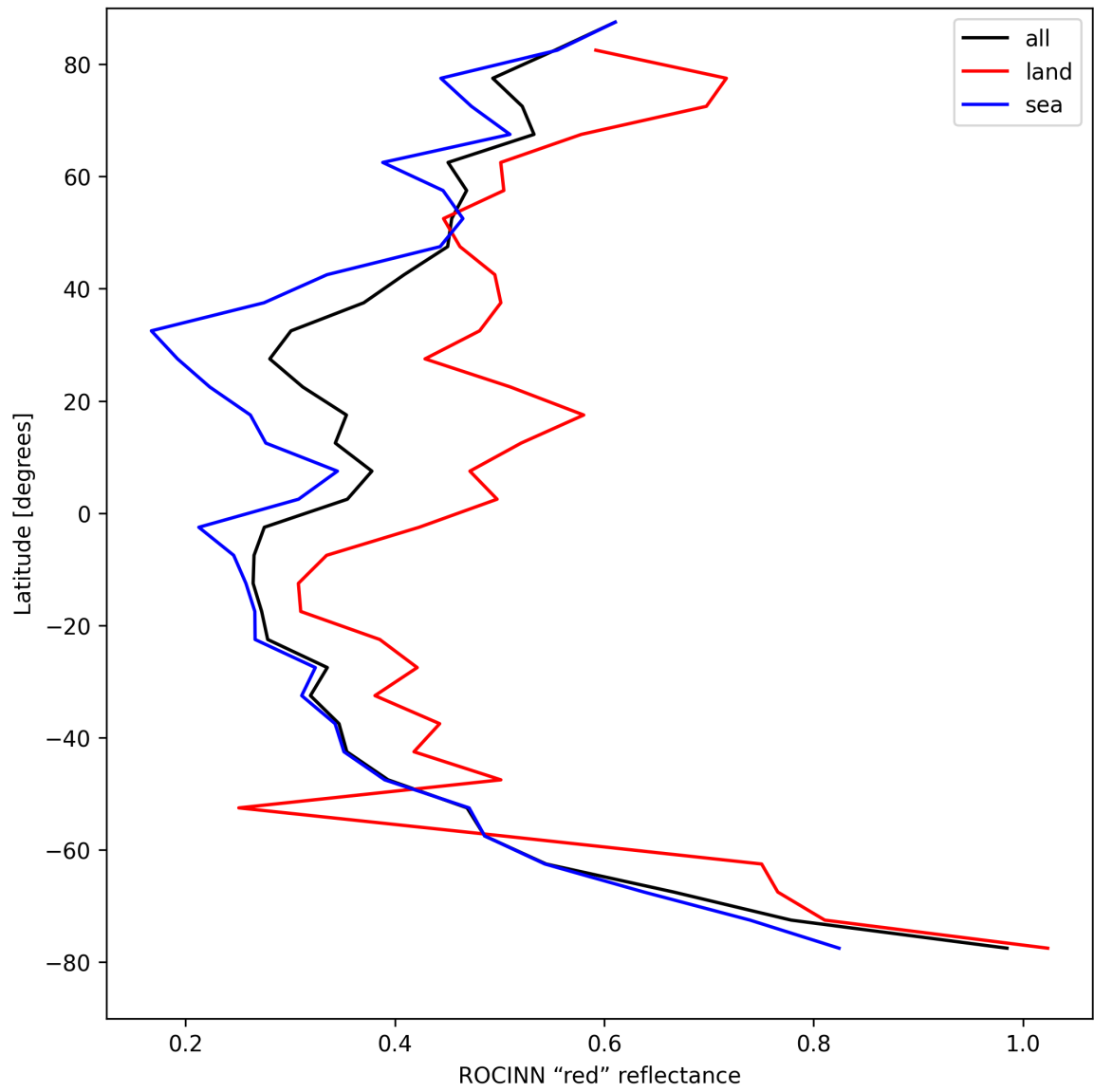
Figure 35: Zonal average of "ROCINN "red" reflectance" for 2025-08-27 to 2025-08-28.
