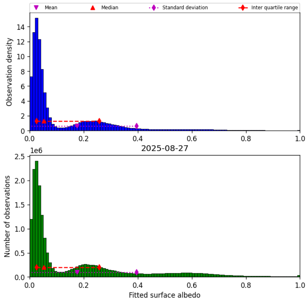
Figure 43: Histogram of “Fitted surface albedo” for 2025-08-27 to 2025-08-28
