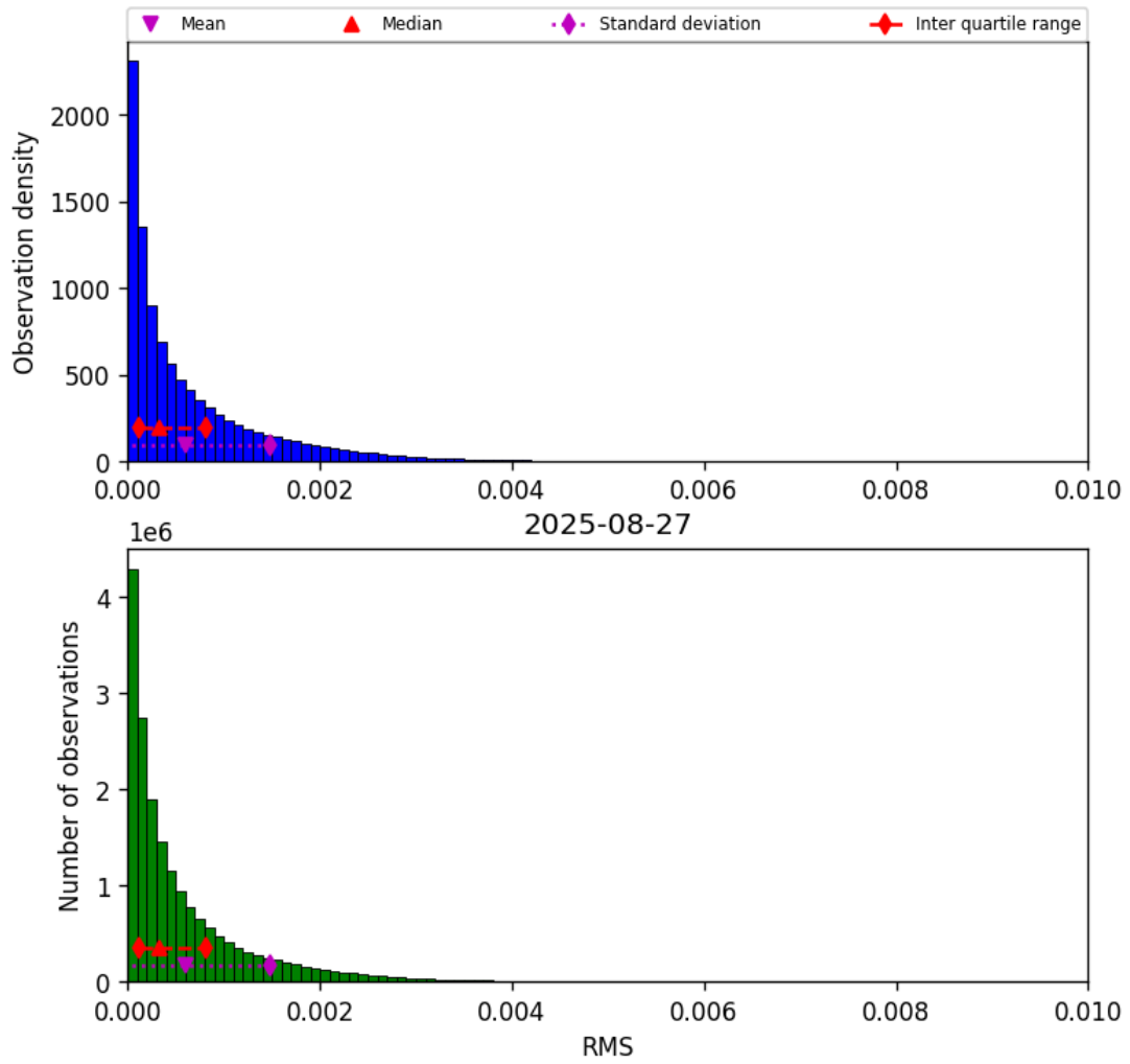
Figure 45: Histogram of “RMS” for 2025-08-27 to 2025-08-28
