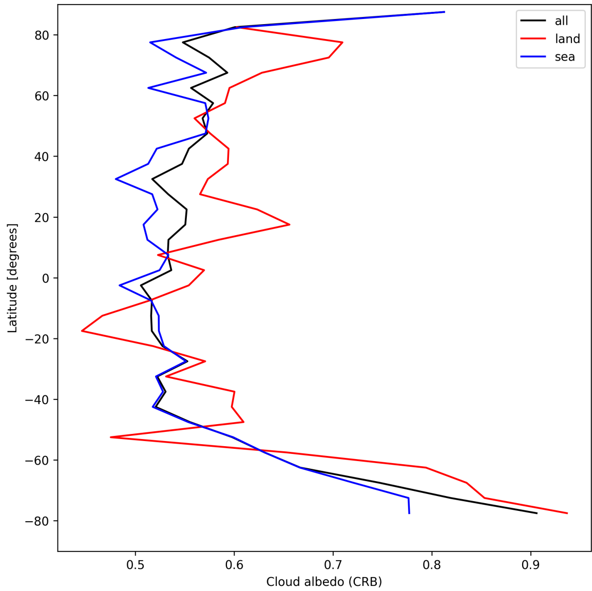
Figure 26: Zonal average of “Cloud albedo (CRB)” for 2025-08-27 to 2025-08-28.
