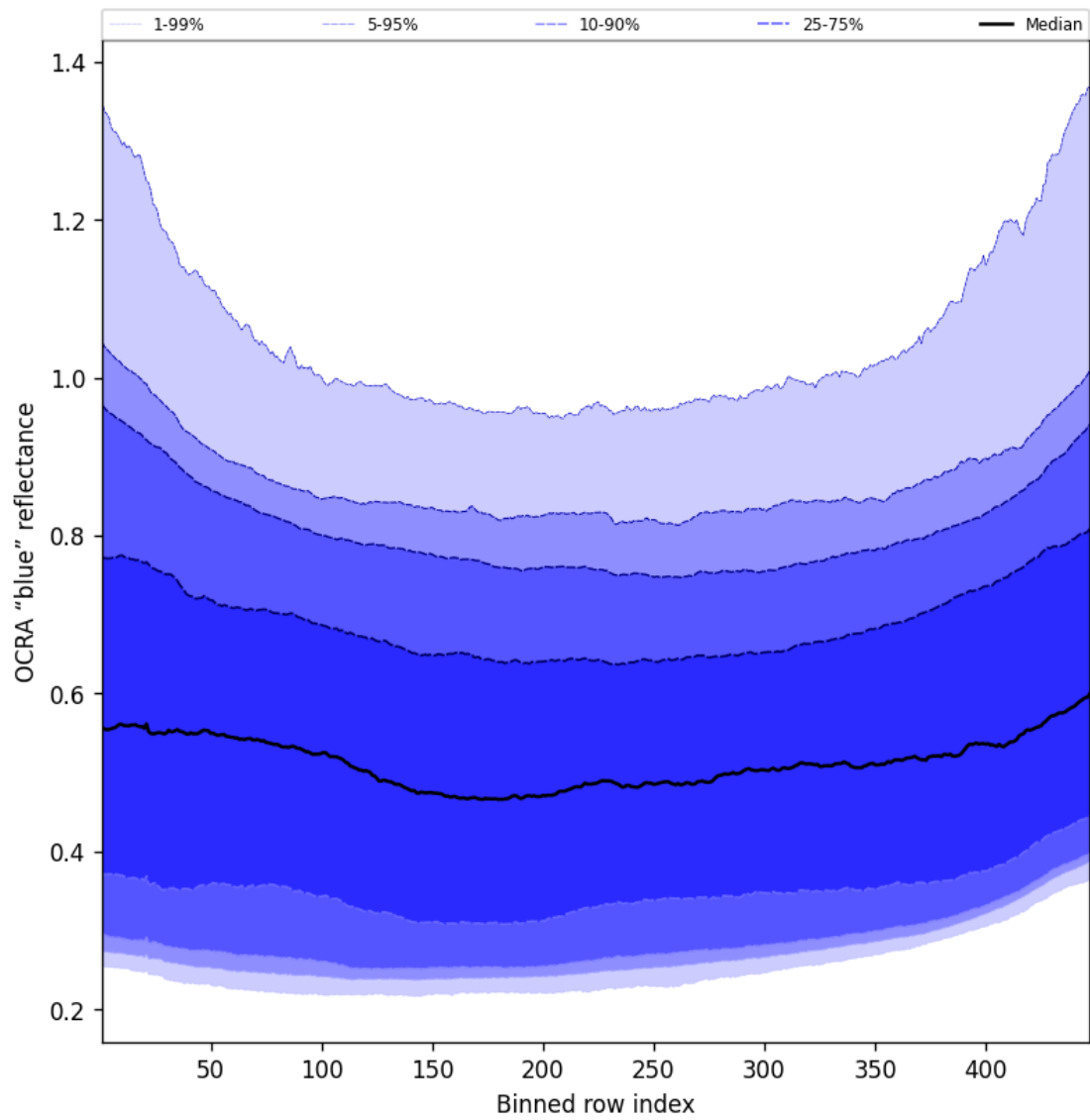
Figure 65: Along track statistics of “OCRA “blue” reflectance” for 2025-08-27 to 2025-08-28
