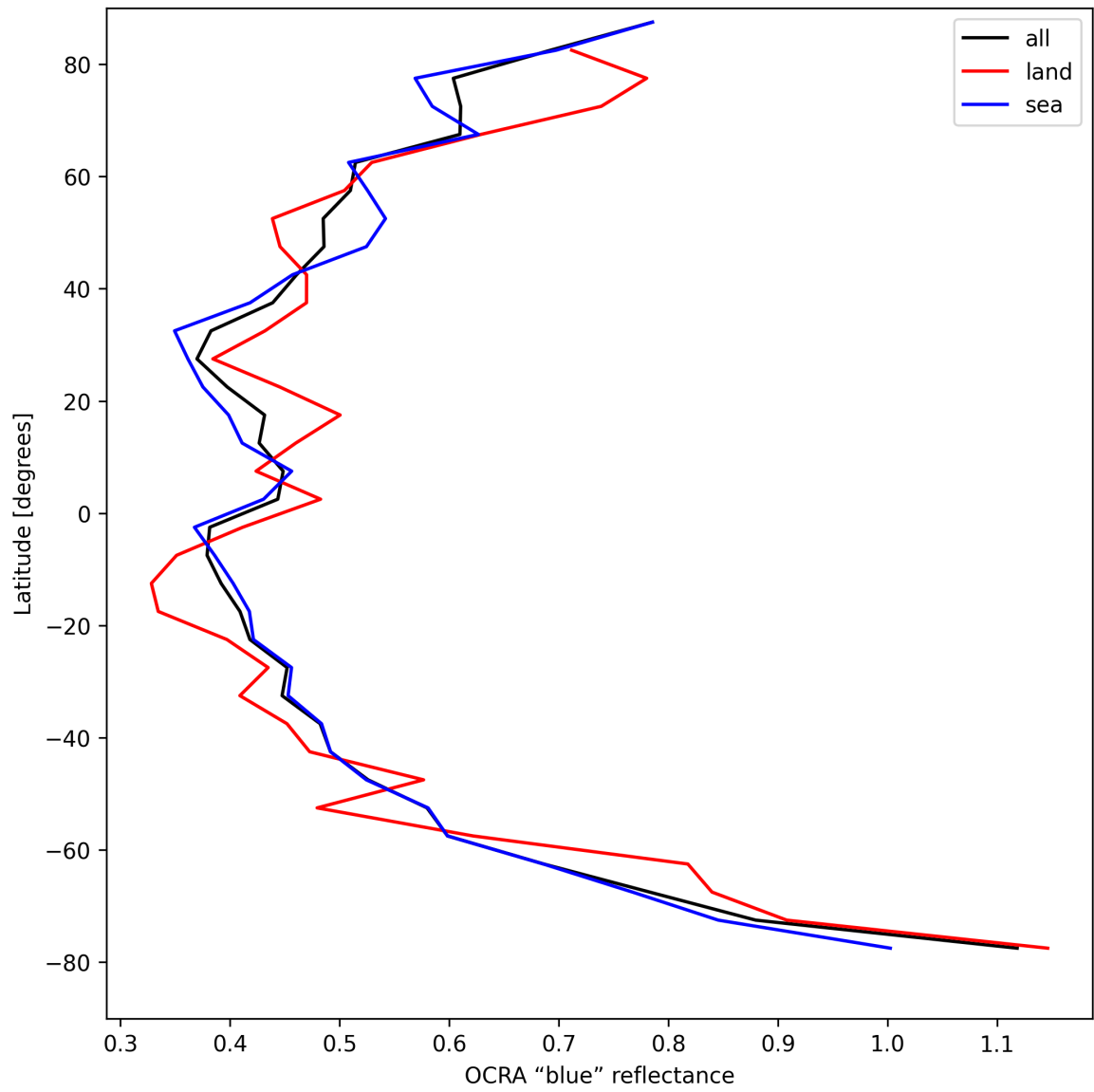
Figure 33: Zonal average of “OCRA “blue” reflectance” for 2025-08-27 to 2025-08-28.
