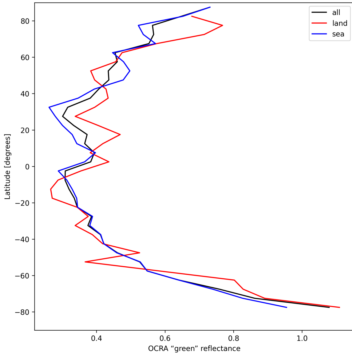
Figure 34: Zonal average of “OCRA “green” reflectance” for 2025-08-27 to 2025-08-28.
