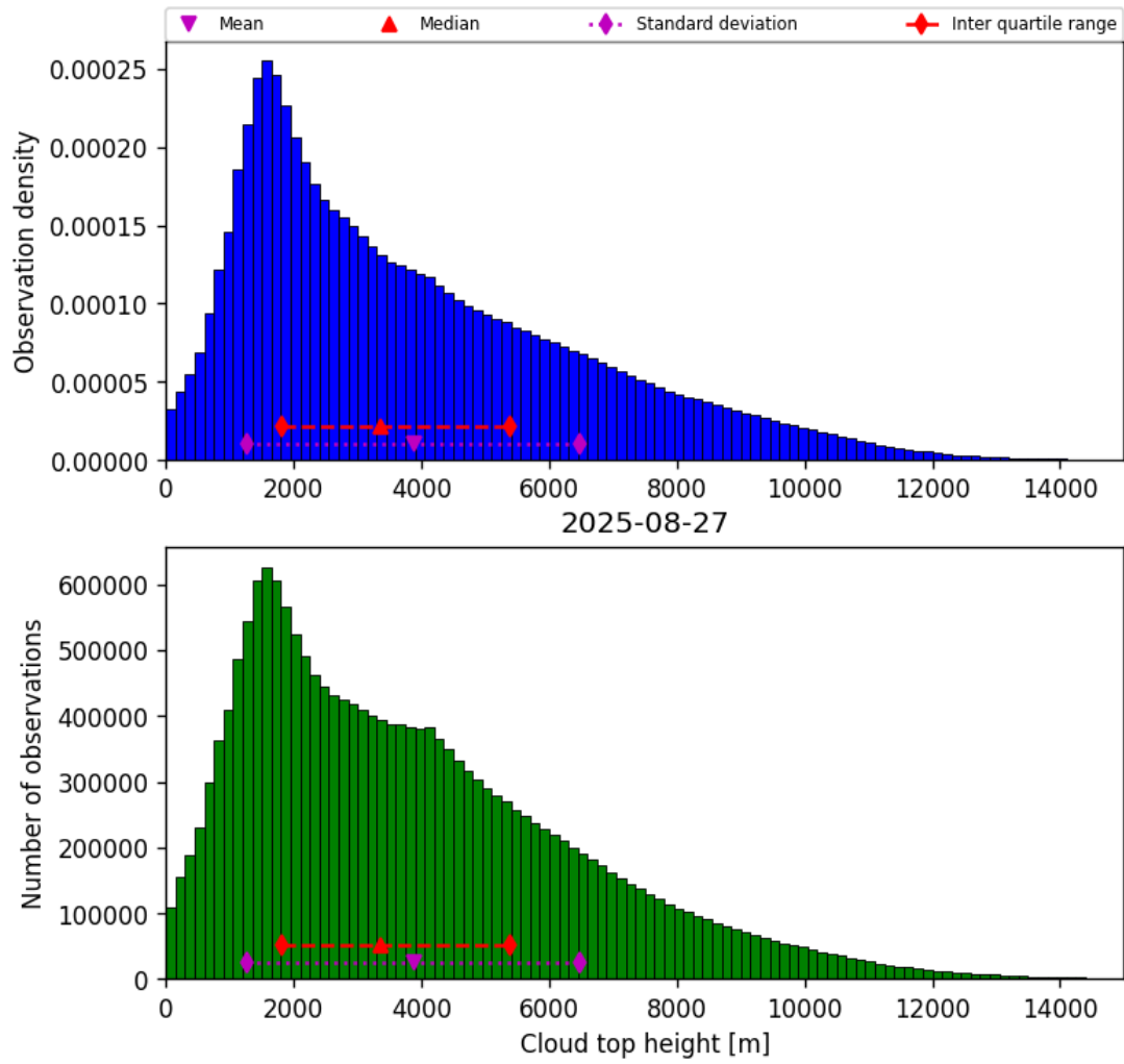
Figure 38: Histogram of “Cloud top height” for 2025-08-27 to 2025-08-28
