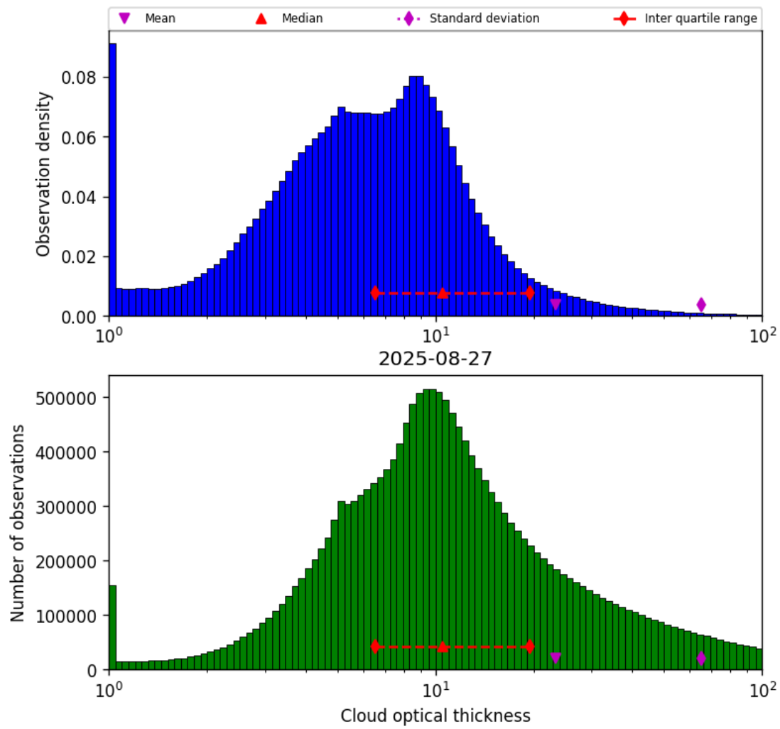
Figure 39: Histogram of “Cloud optical thickness” for 2025-08-27 to 2025-08-28
