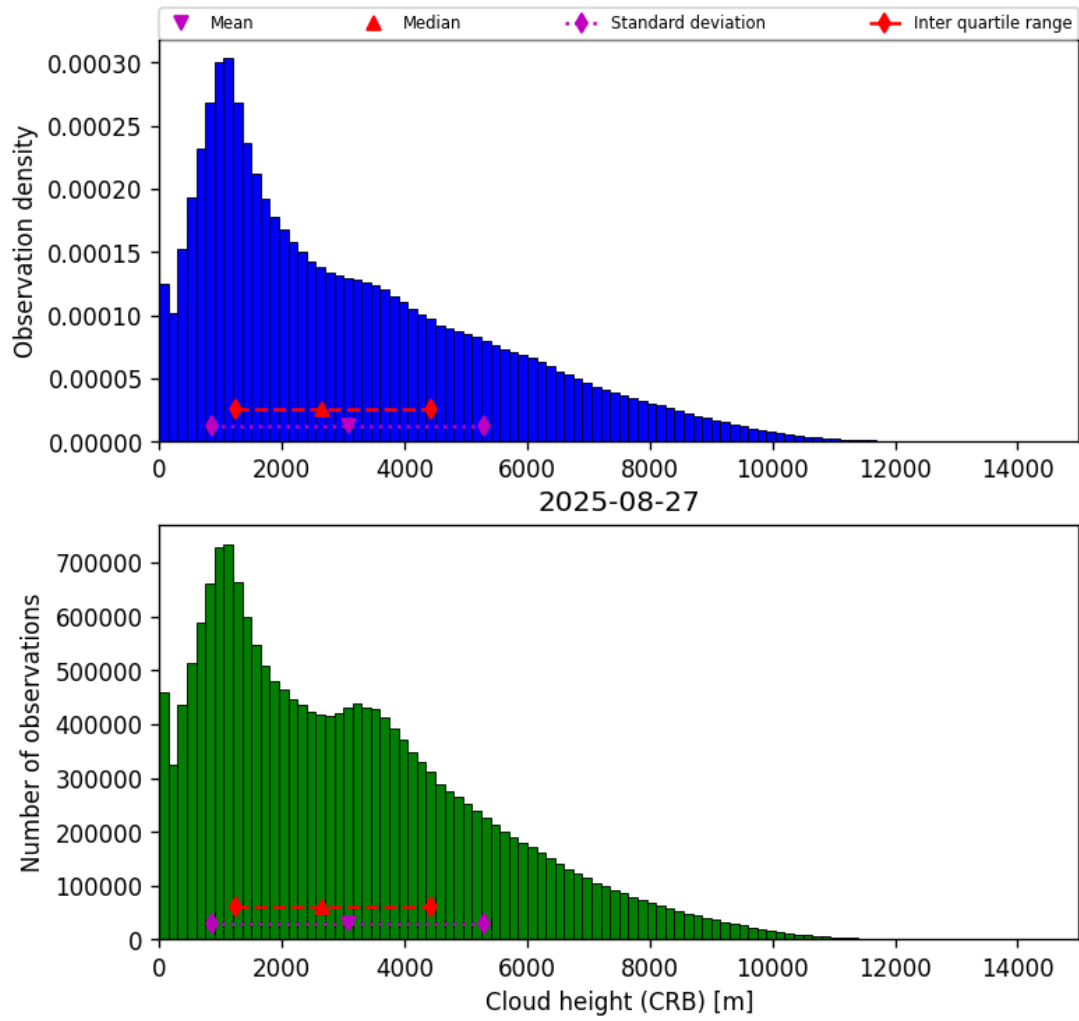
Figure 41: Histogram of “Cloud height (CRB)” for 2025-08-27 to 2025-08-28
