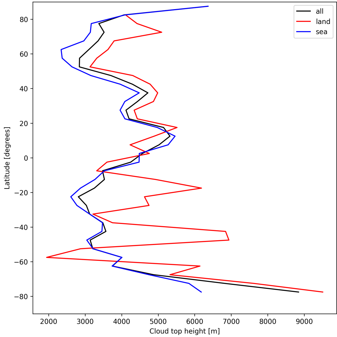
Figure 22: Zonal average of “Cloud top height” for 2025-08-27 to 2025-08-28.
