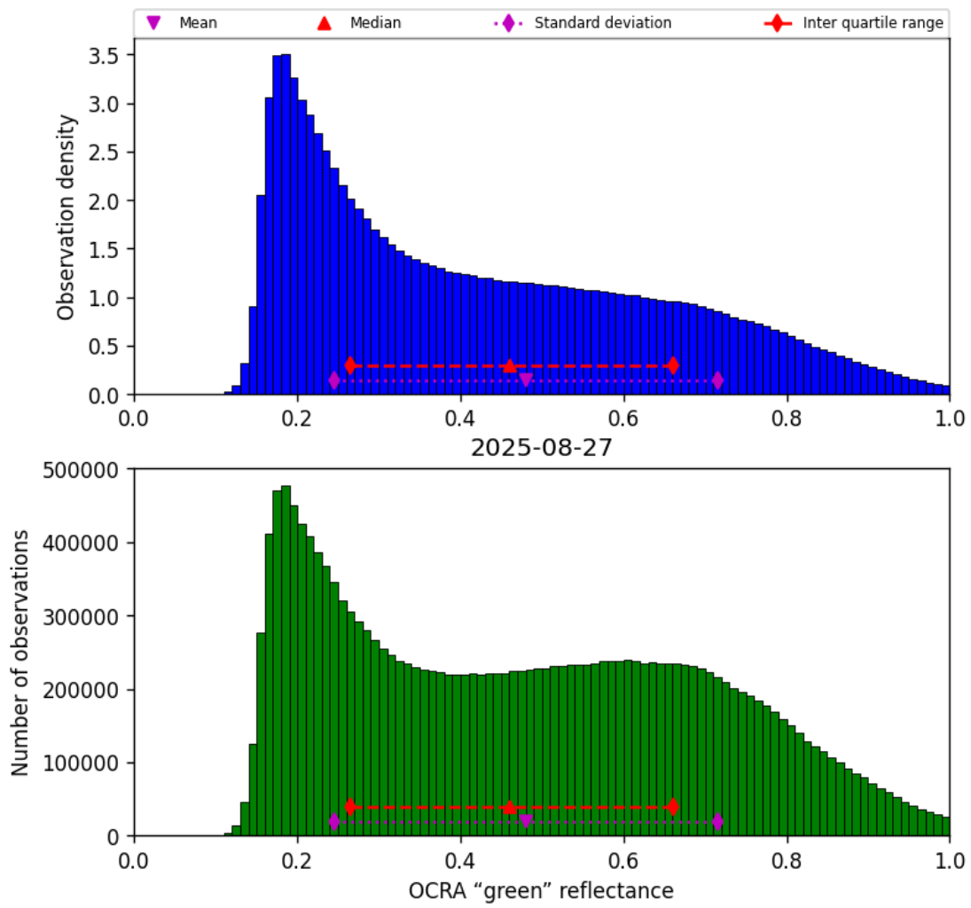
Figure 50: Histogram of “OCRA “green” reflectance” for 2025-08-27 to 2025-08-28
