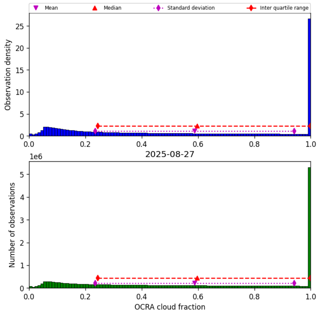
Figure 48: Histogram of “OCRA cloud fraction” for 2025-08-27 to 2025-08-28
