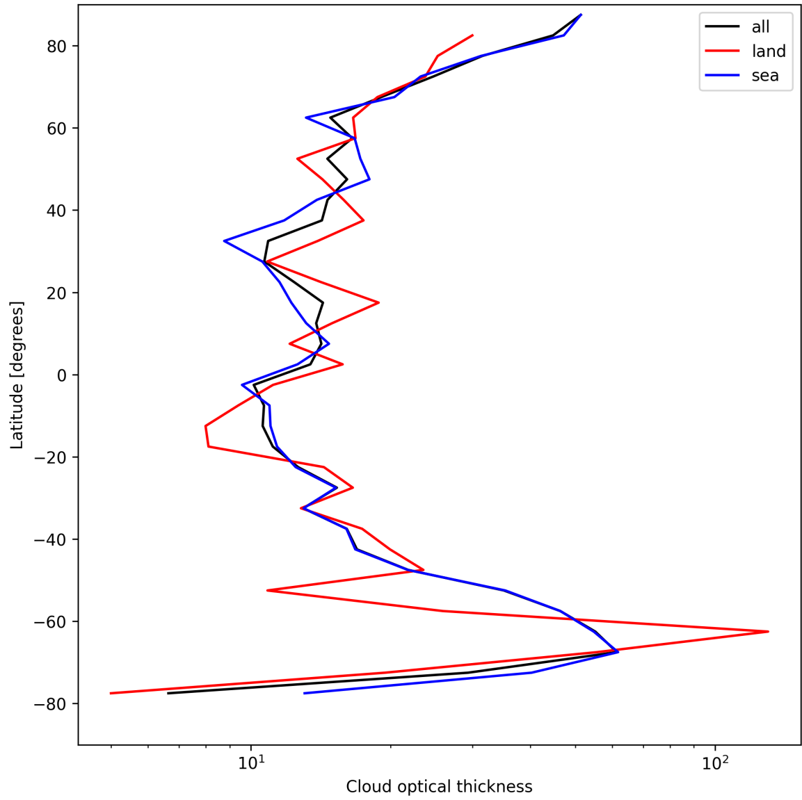
Figure 23: Zonal average of “Cloud optical thickness” for 2025-08-27 to 2025-08-28.
