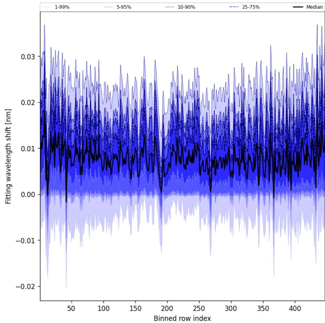
Figure 63: Along track statistics of “Fitting wavelength shift” for 2025-08-27 to 2025-08-28
