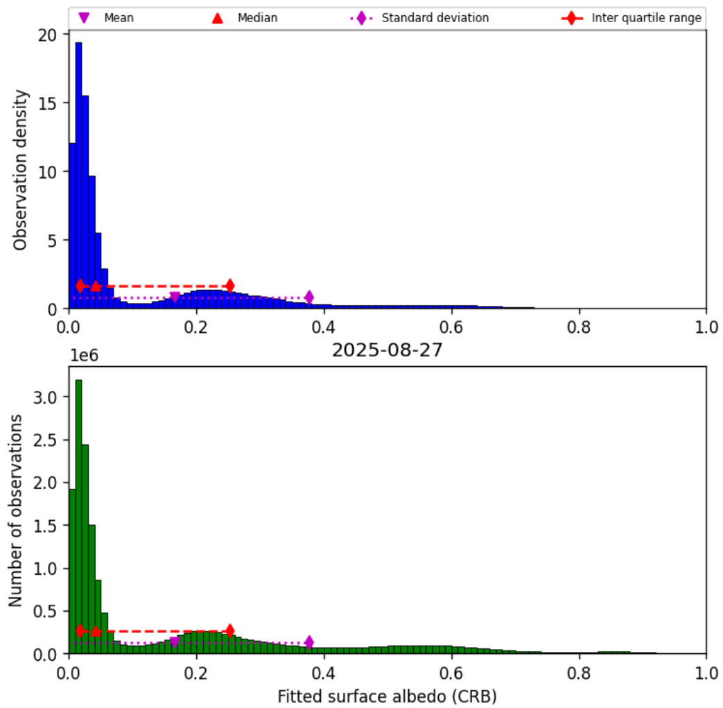
Figure 44: Histogram of “Fitted surface albedo (CRB)” for 2025-08-27 to 2025-08-28
