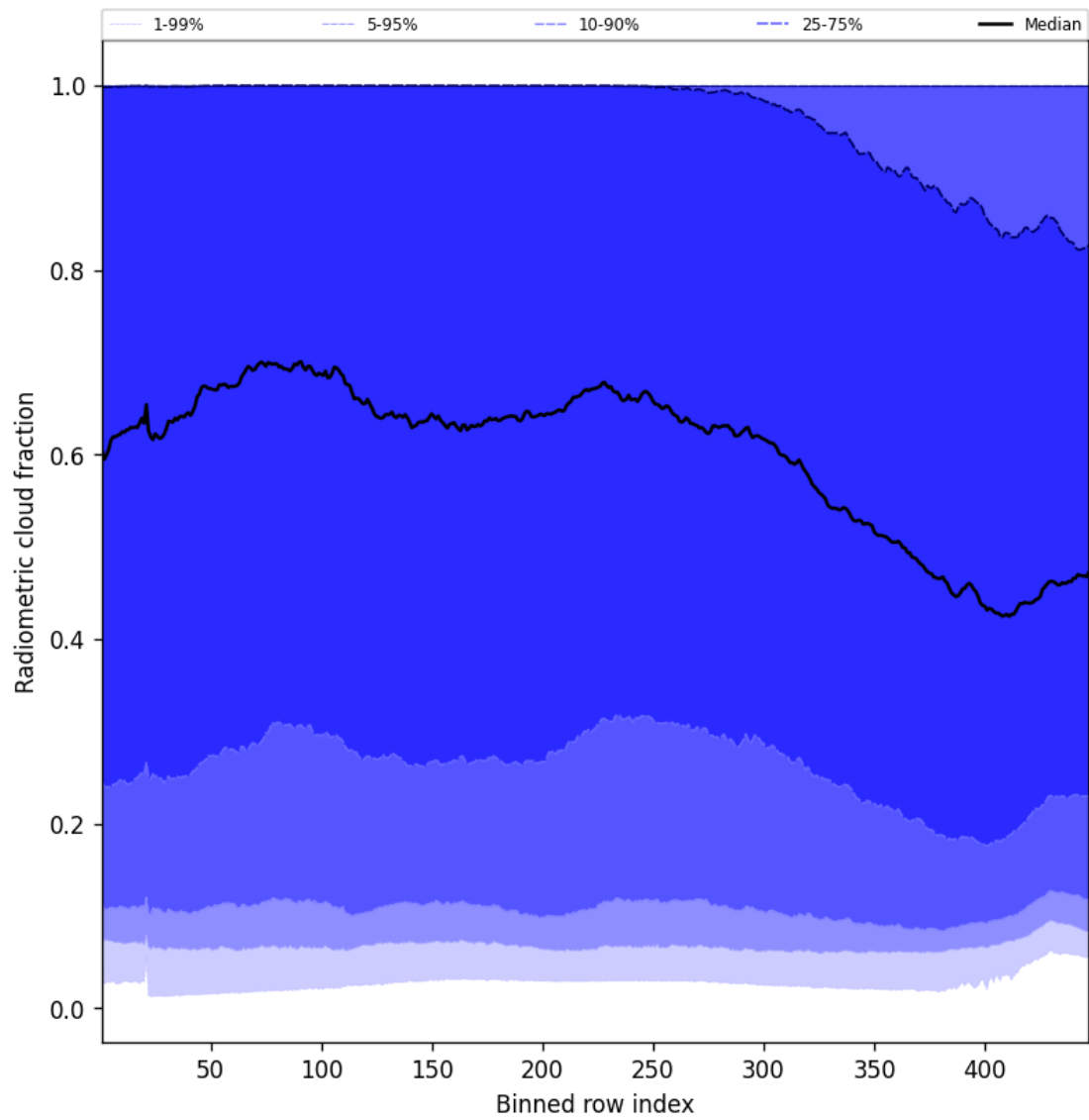
Figure 53: Along track statistics of “Radiometric cloud fraction” for 2025-08-27 to 2025-08-28
