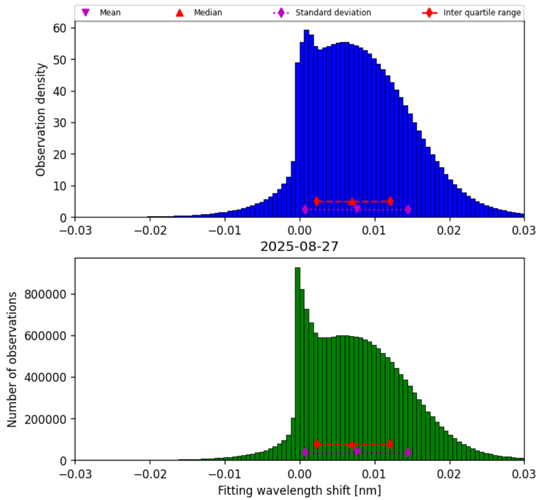
Figure 47: Histogram of “Fitting wavelength shift” for 2025-08-27 to 2025-08-28
