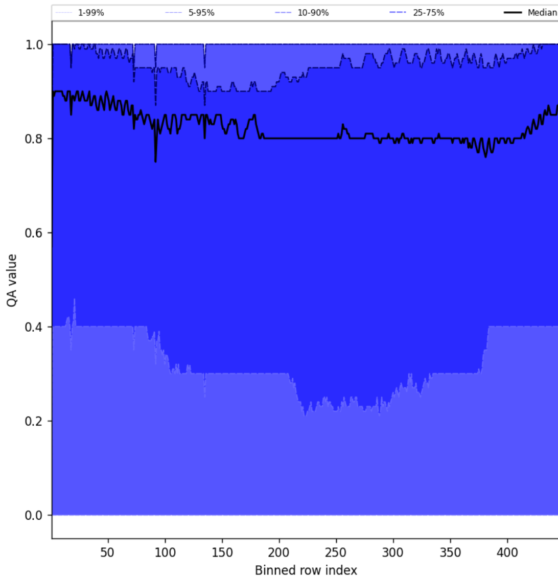
Figure 52: Along track statistics of "QA value" for 2025-08-27 to 2025-08-28
