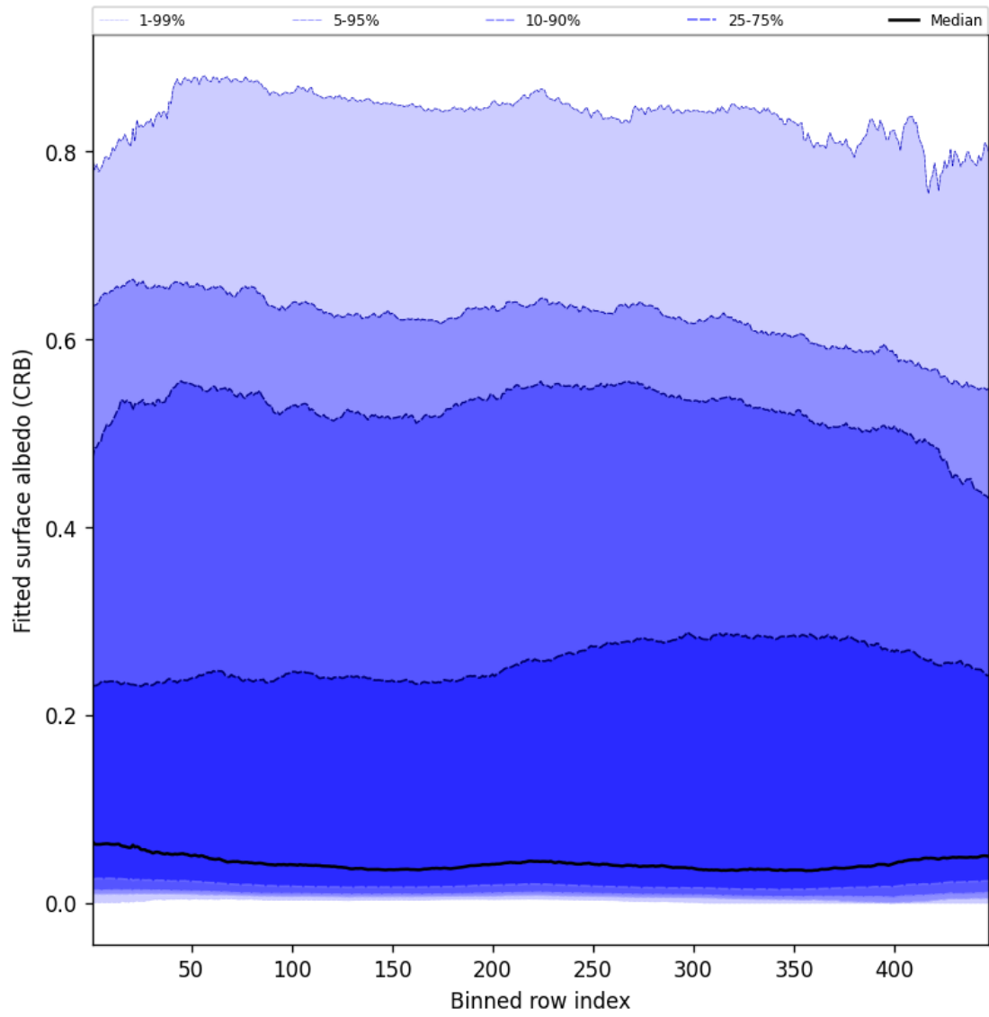
Figure 60: Along track statistics of “Fitted surface albedo (CRB)” for 2025-08-27 to 2025-08-28
