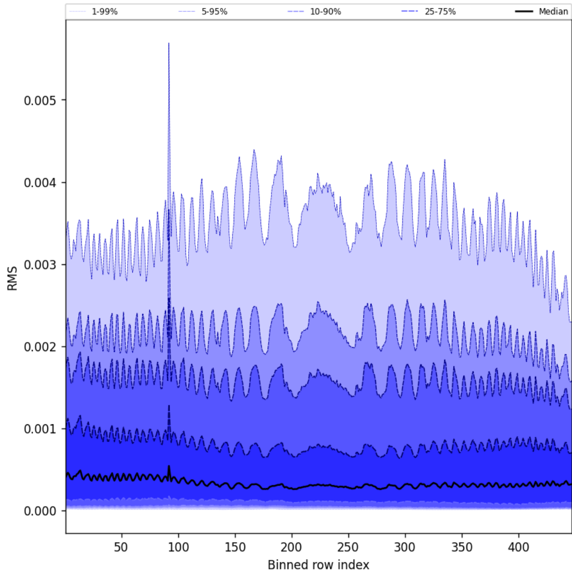
Figure 61: Along track statistics of “RMS” for 2025-08-27 to 2025-08-28
