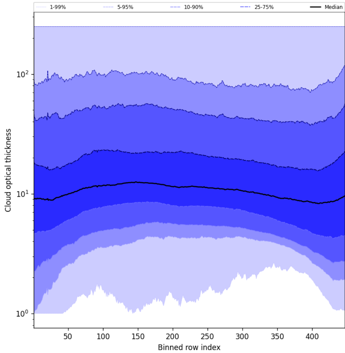
Figure 55: Along track statistics of “Cloud optical thickness” for 2025-08-27 to 2025-08-28
