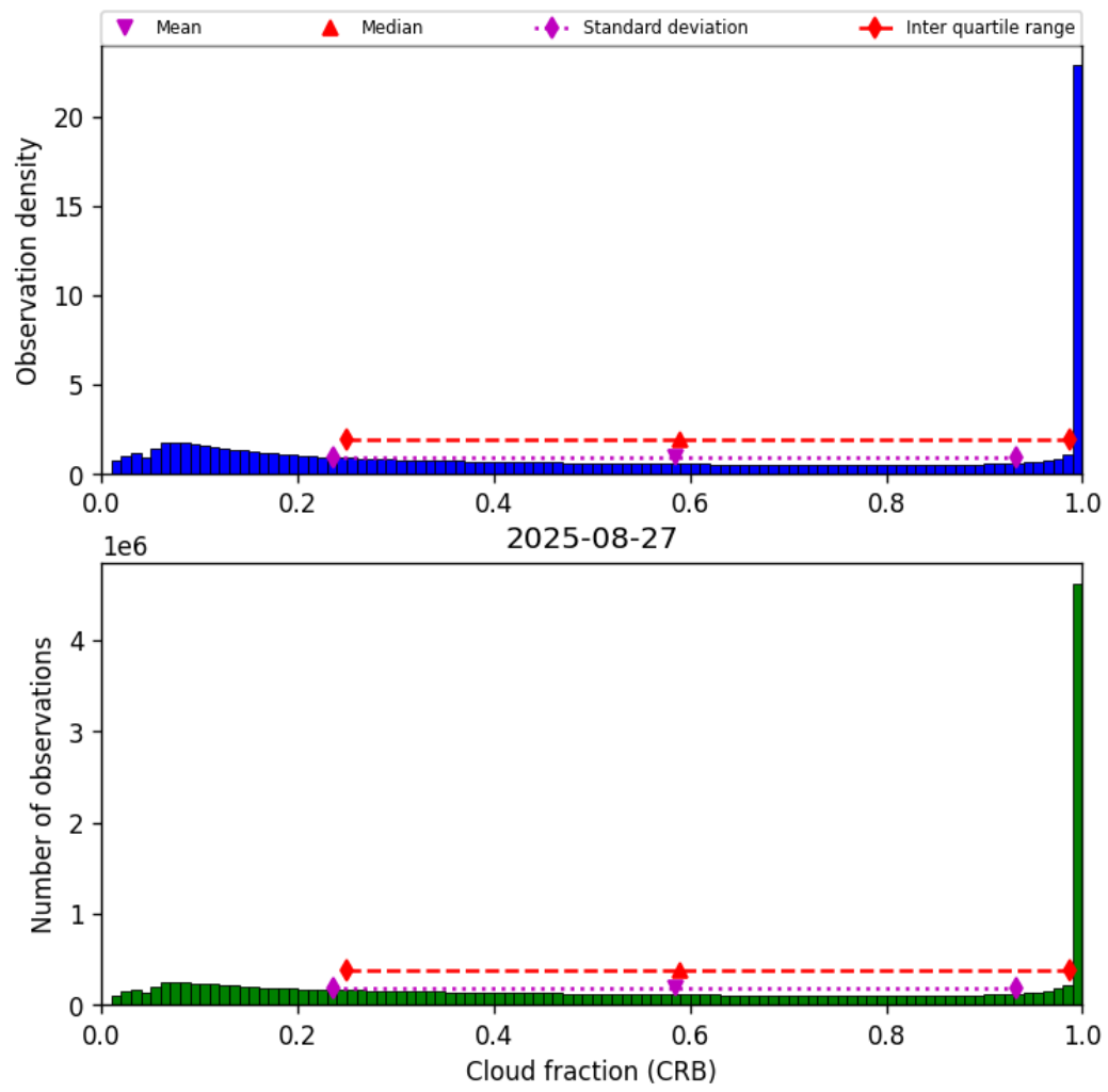
Figure 40: Histogram of “Cloud fraction (CRB)” for 2025-08-27 to 2025-08-28
