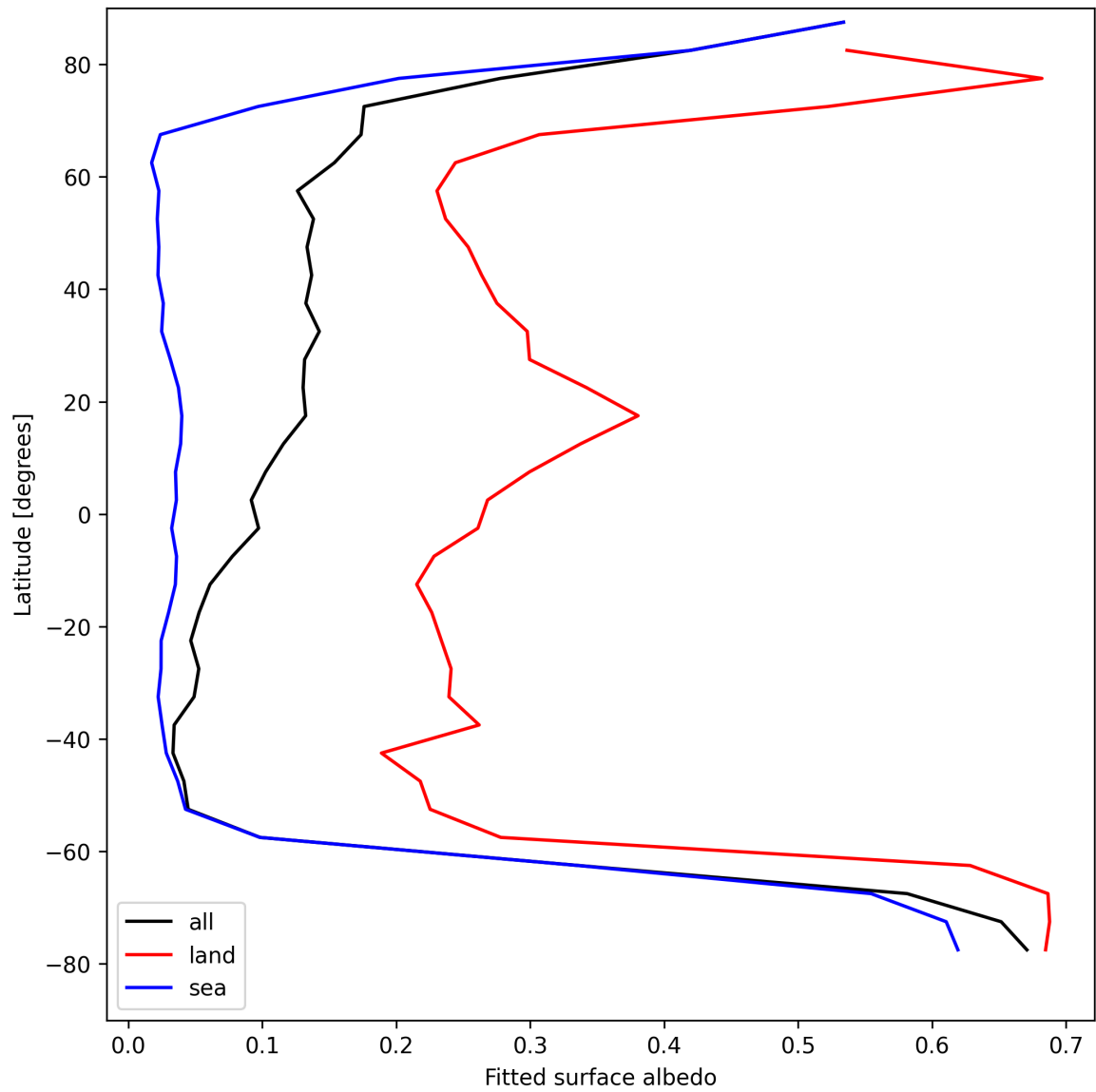
Figure 27: Zonal average of “Fitted surface albedo” for 2025-08-27 to 2025-08-28.
