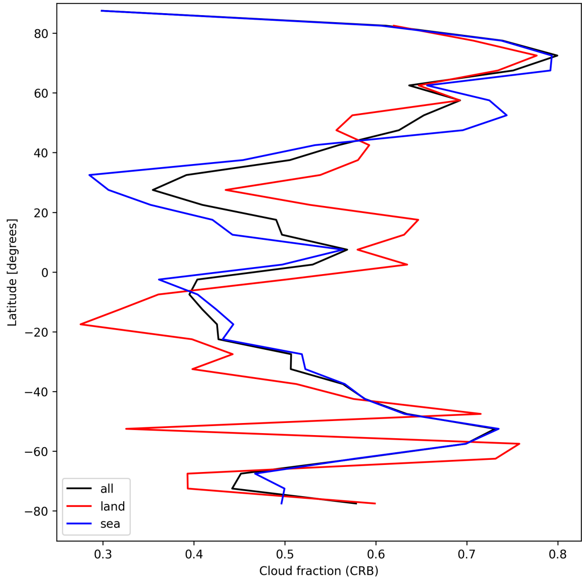
Figure 24: Zonal average of “Cloud fraction (CRB)” for 2025-08-27 to 2025-08-28.
