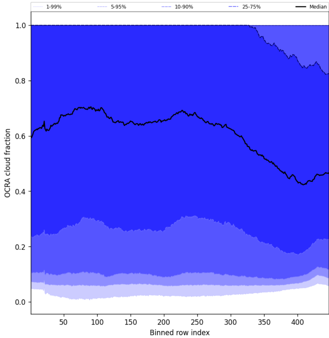
Figure 64: Along track statistics of “OCRA cloud fraction” for 2025-08-27 to 2025-08-28
