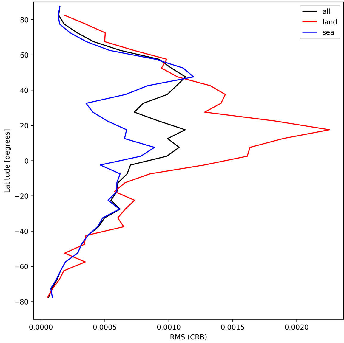
Figure 30: Zonal average of “RMS (CRB)” for 2025-08-27 to 2025-08-28.
