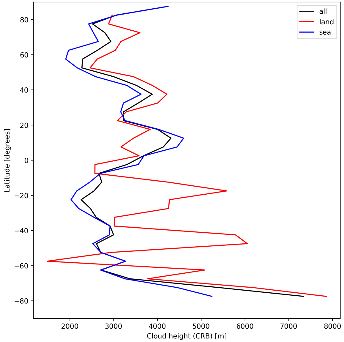
Figure 25: Zonal average of “Cloud height (CRB)” for 2025-08-27 to 2025-08-28.
