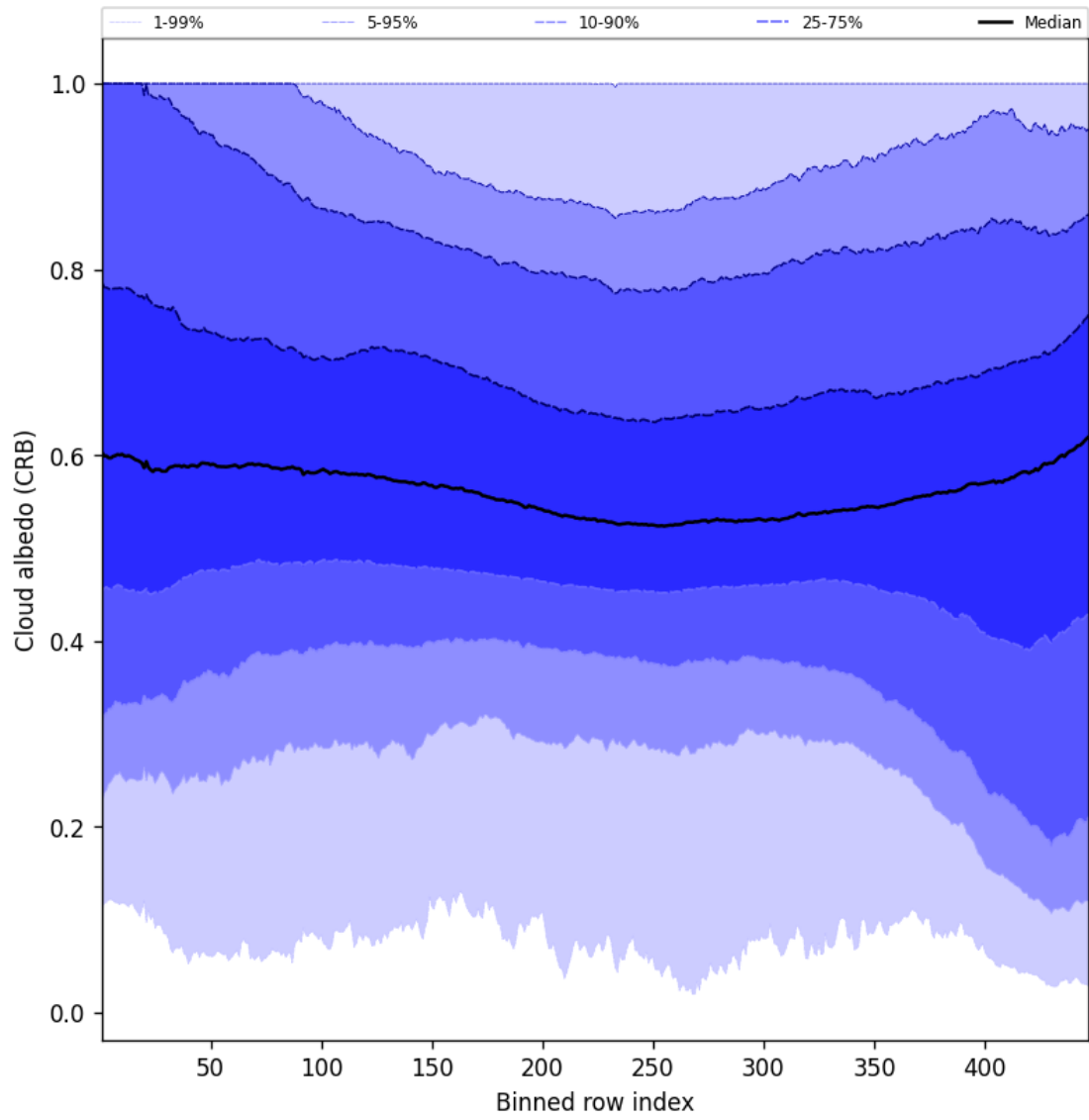
Figure 58: Along track statistics of “Cloud albedo (CRB)” for 2025-08-27 to 2025-08-28
