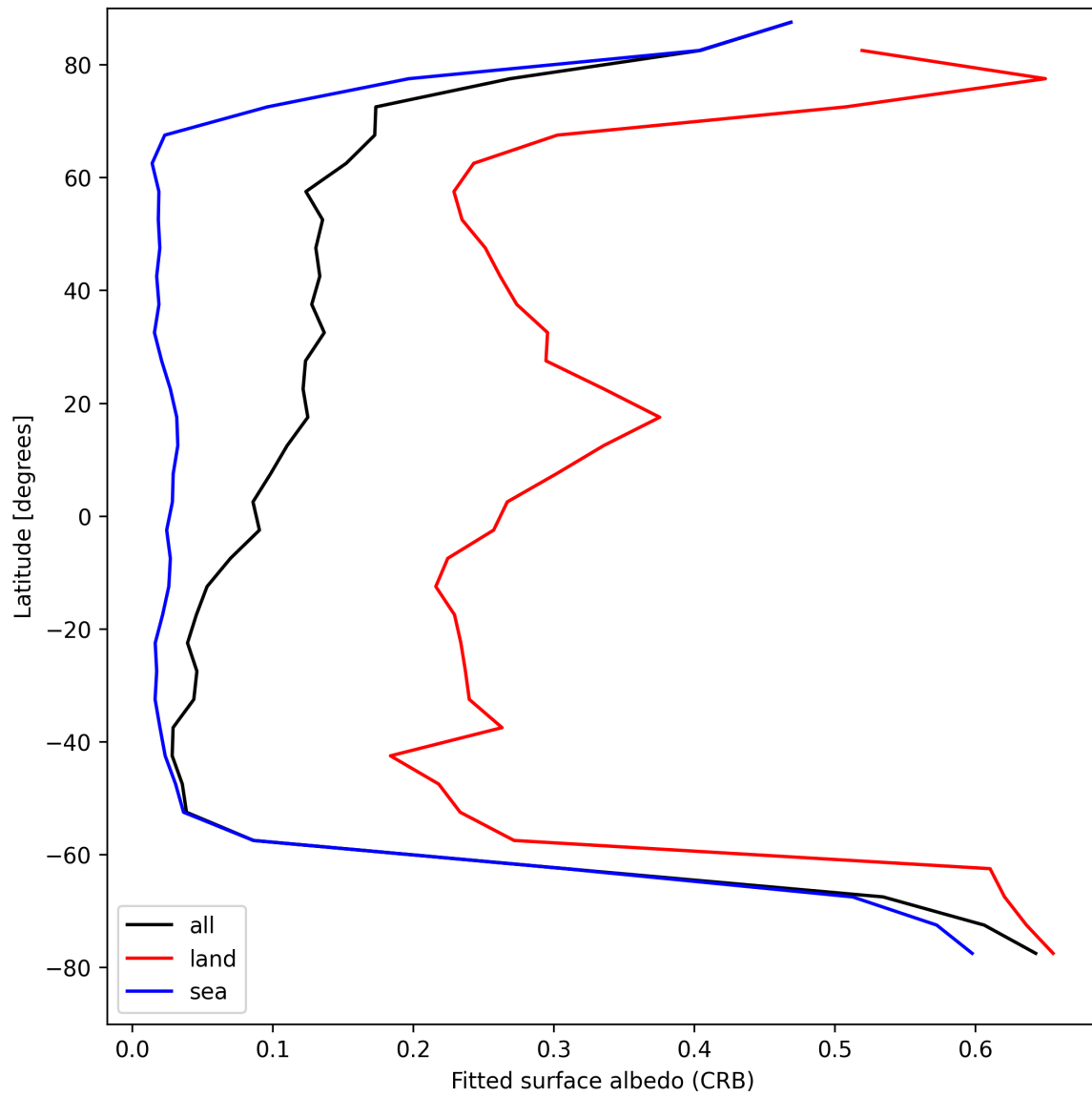
Figure 28: Zonal average of “Fitted surface albedo (CRB)” for 2025-08-27 to 2025-08-28.
