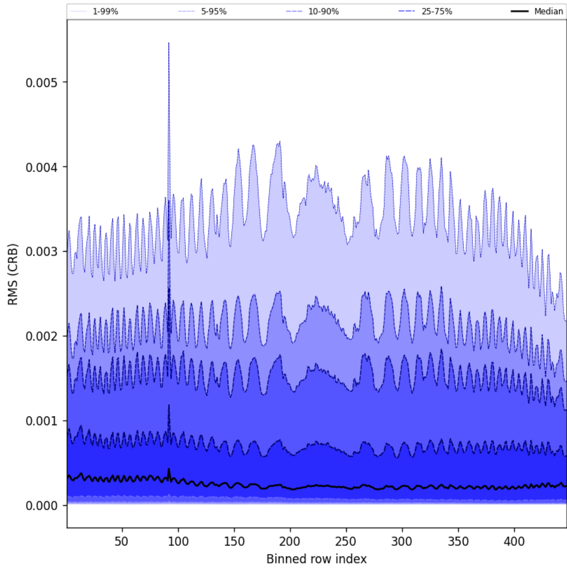
Figure 62: Along track statistics of “RMS (CRB)” for 2025-08-27 to 2025-08-28
