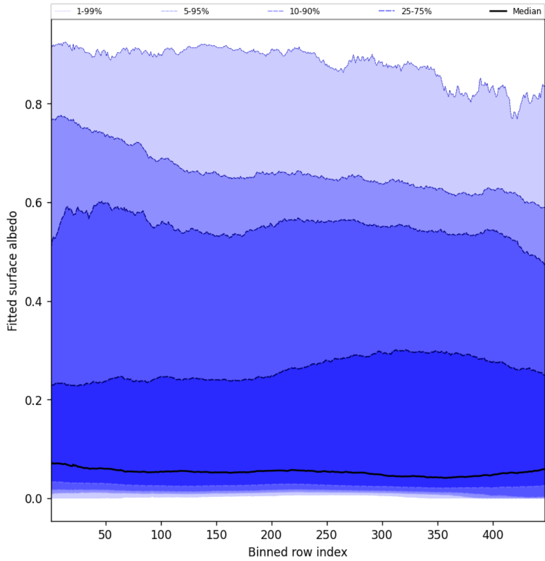
Figure 59: Along track statistics of “Fitted surface albedo” for 2025-08-27 to 2025-08-28
