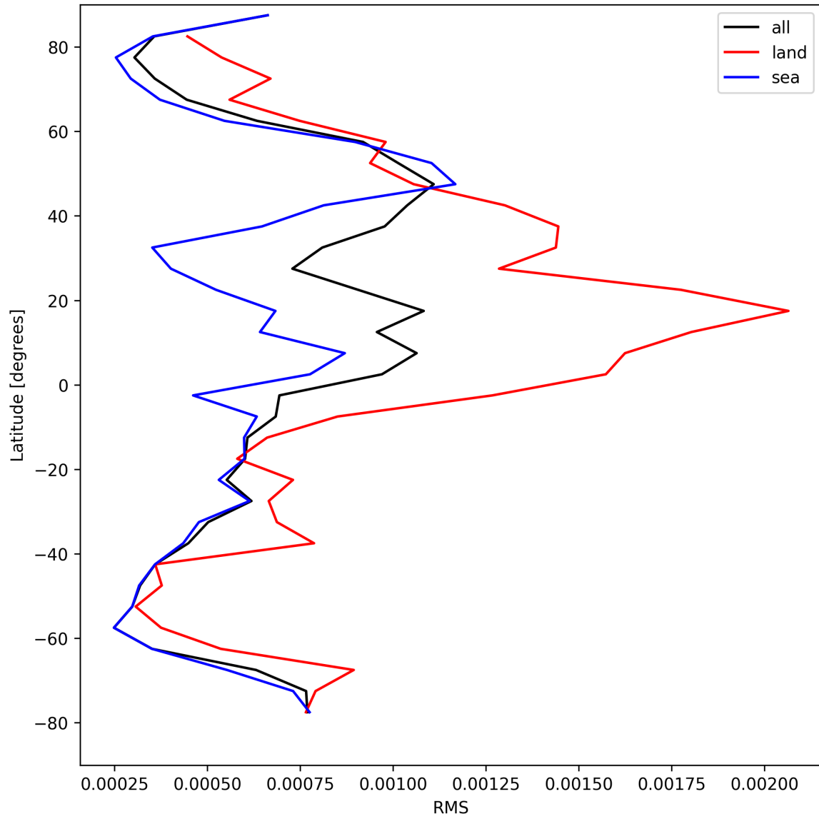
Figure 29: Zonal average of “RMS” for 2025-08-27 to 2025-08-28.
