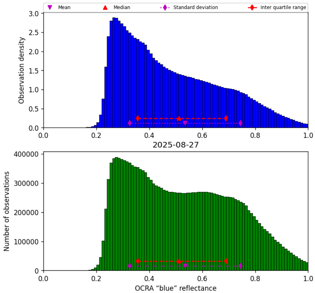
Figure 49: Histogram of “OCRA “blue” reflectance” for 2025-08-27 to 2025-08-28
