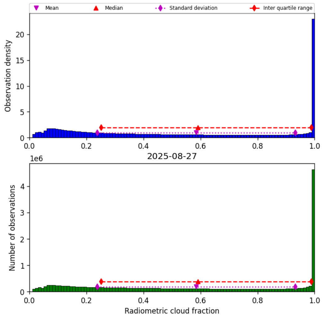
Figure 37: Histogram of “Radiometric cloud fraction” for 2025-08-27 to 2025-08-28
