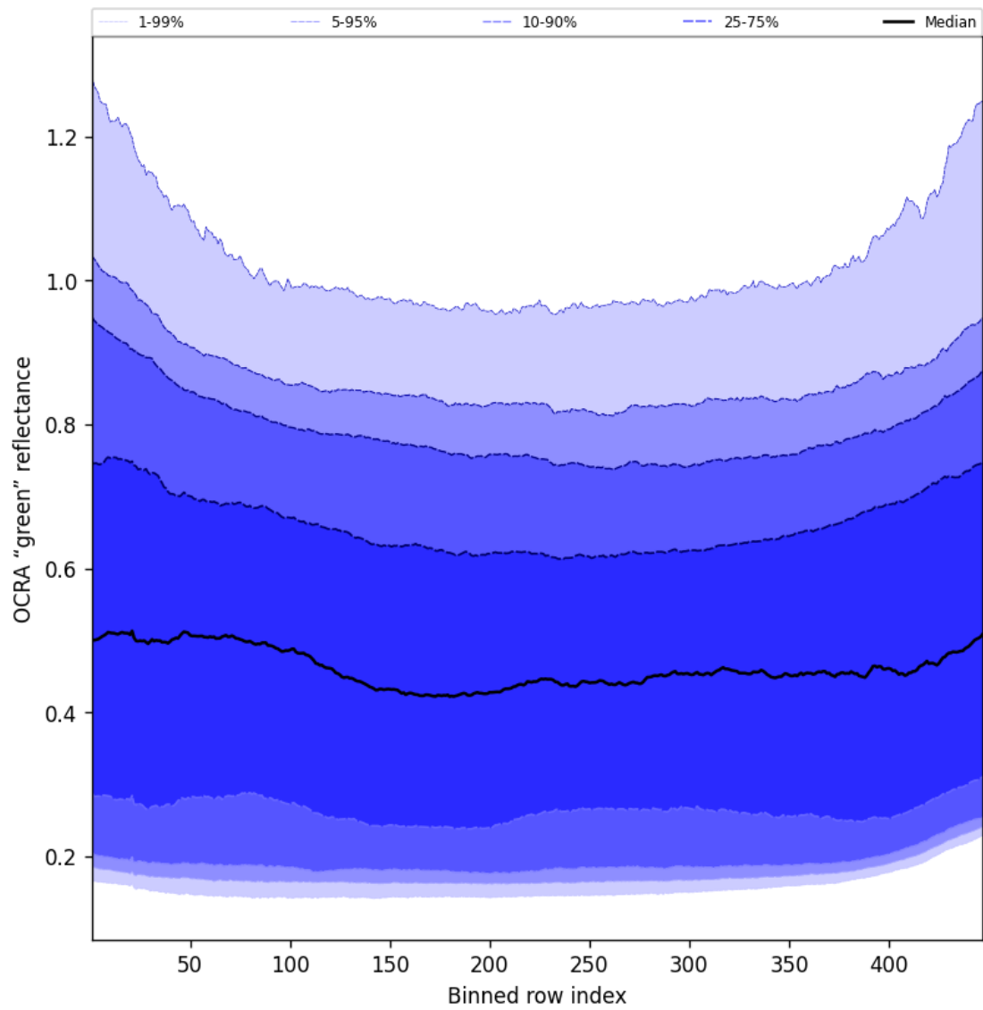
Figure 66: Along track statistics of “OCRA “green” reflectance” for 2025-08-27 to 2025-08-28
