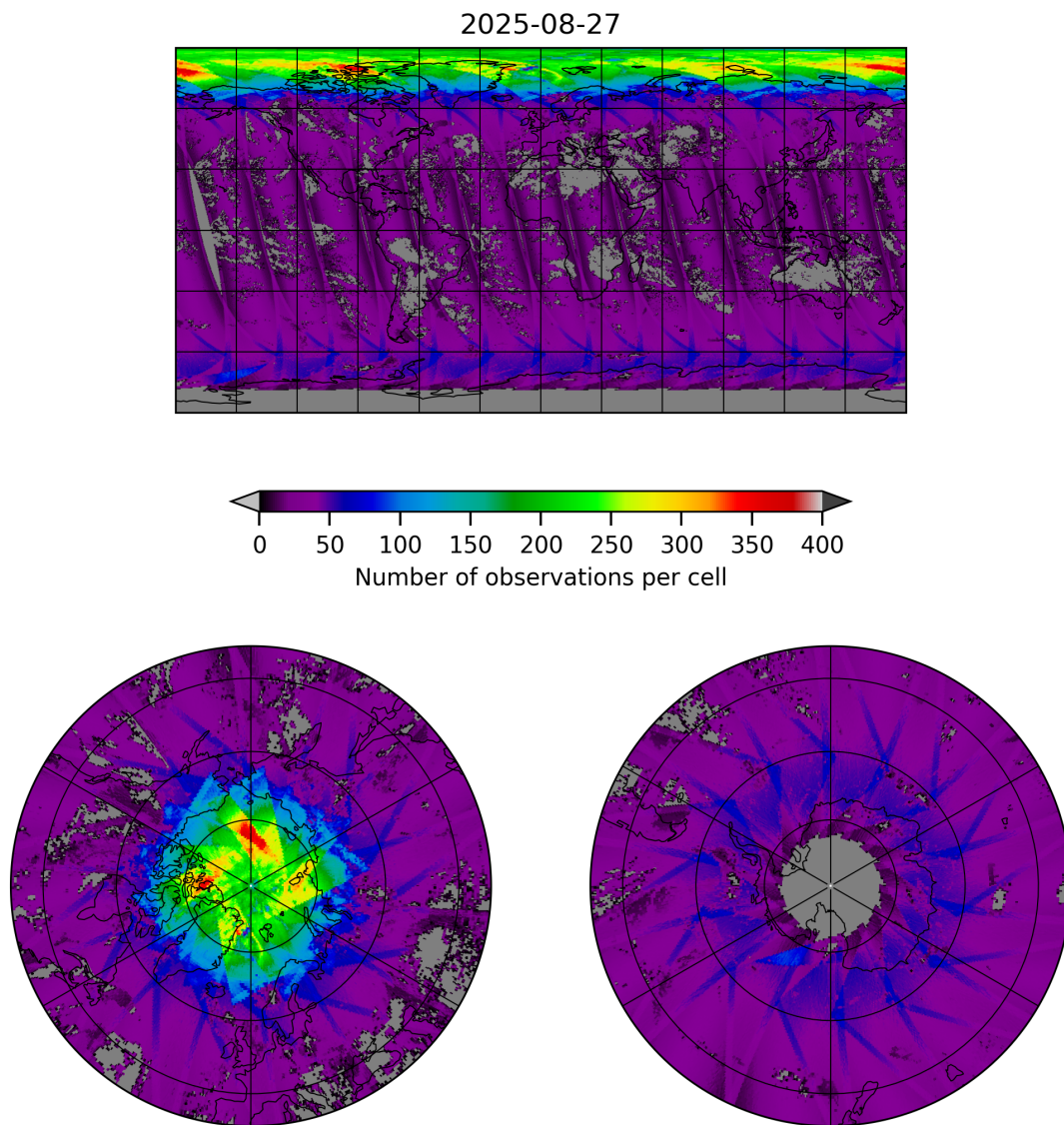
Figure 19: Map of the number of observations for 2025-08-27 to 2025-08-28
