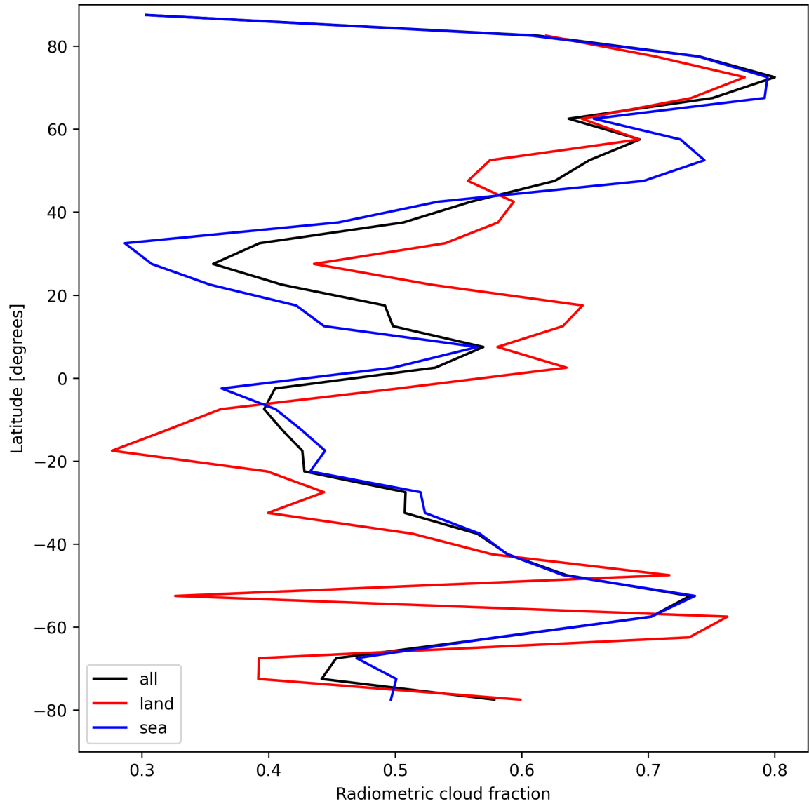
Figure 21: Zonal average of “Radiometric cloud fraction” for 2025-08-27 to 2025-08-28.
