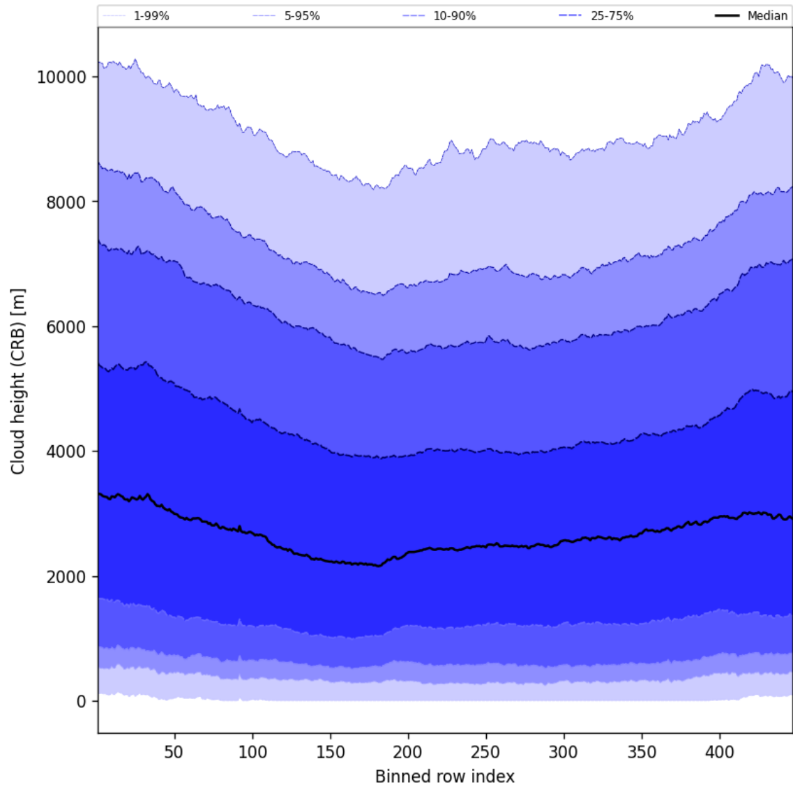
Figure 57: Along track statistics of “Cloud height (CRB)” for 2025-08-27 to 2025-08-28
