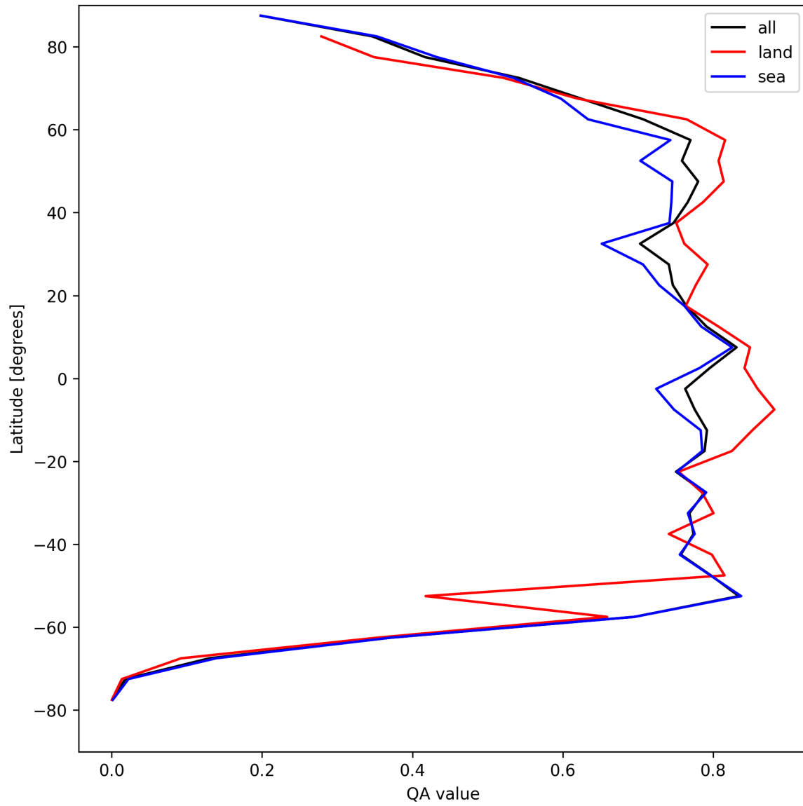
Figure 20: Zonal average of “QA value” for 2025-08-27 to 2025-08-28.
