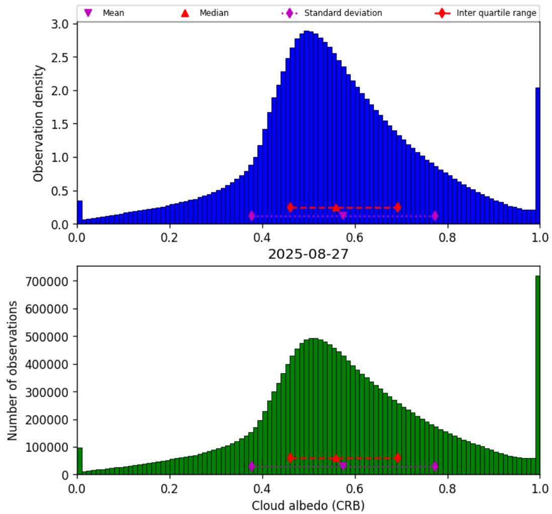
Figure 42: Histogram of “Cloud albedo (CRB)” for 2025-08-27 to 2025-08-28
