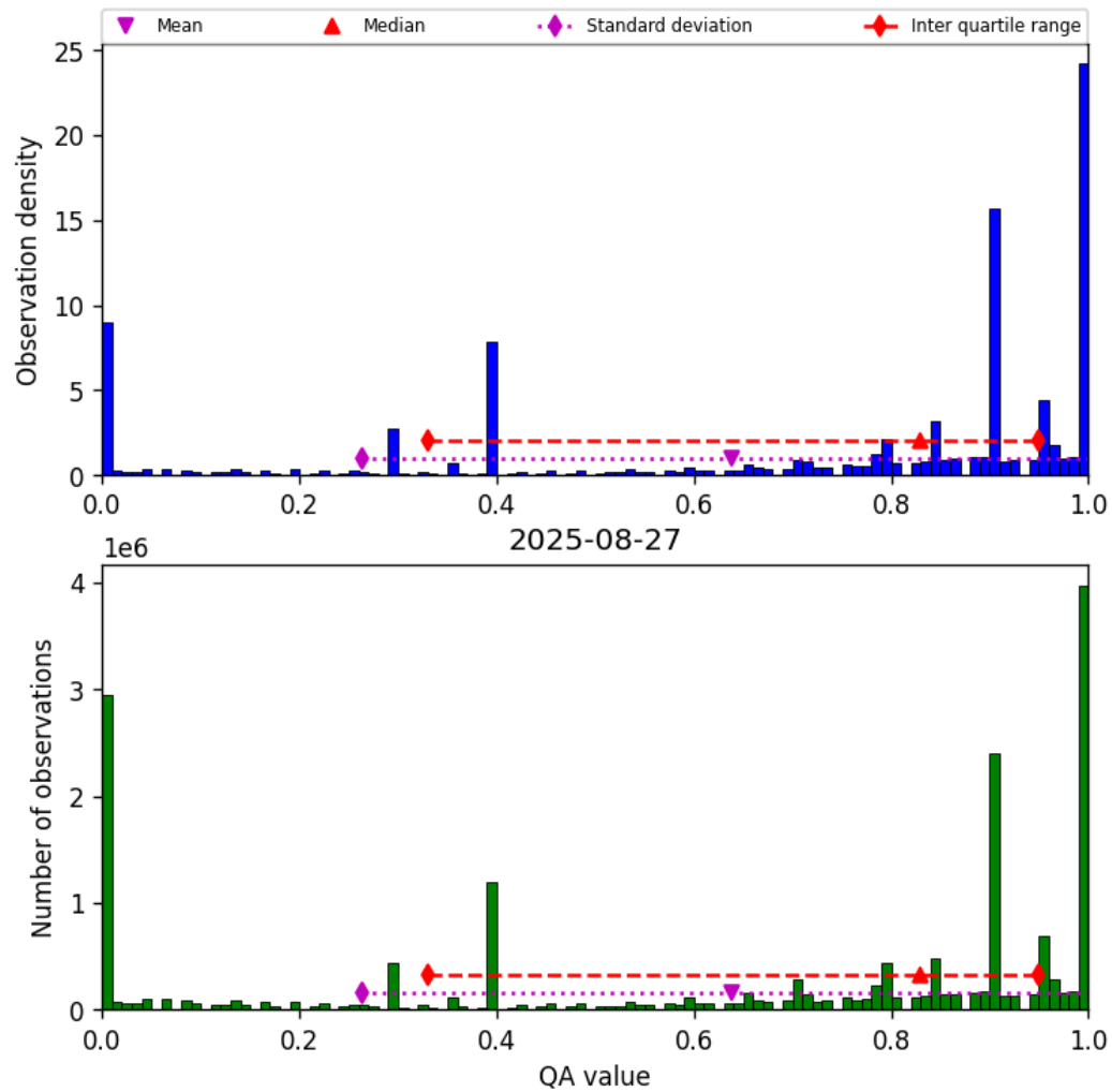
Figure 36: Histogram of “QA value” for 2025-08-27 to 2025-08-28
