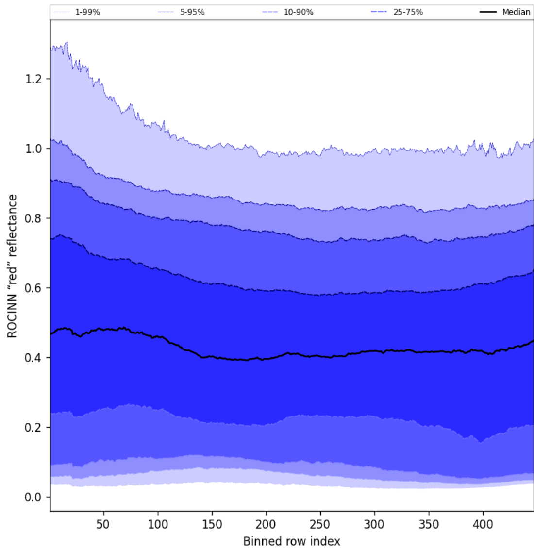
Figure 67: Along track statistics of "ROCINN "red" reflectance" for 2025-08-27 to 2025-08-28
