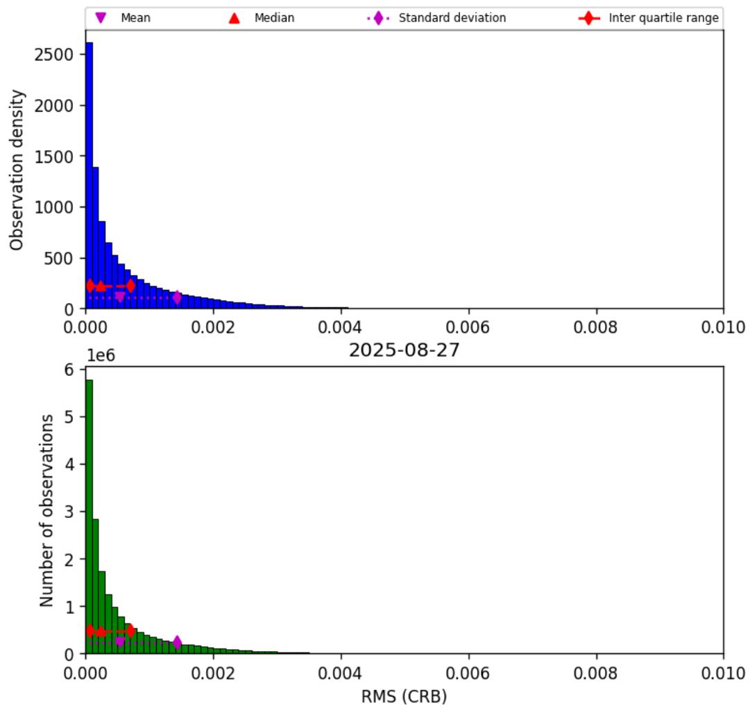
Figure 46: Histogram of “RMS (CRB)” for 2025-08-27 to 2025-08-28
