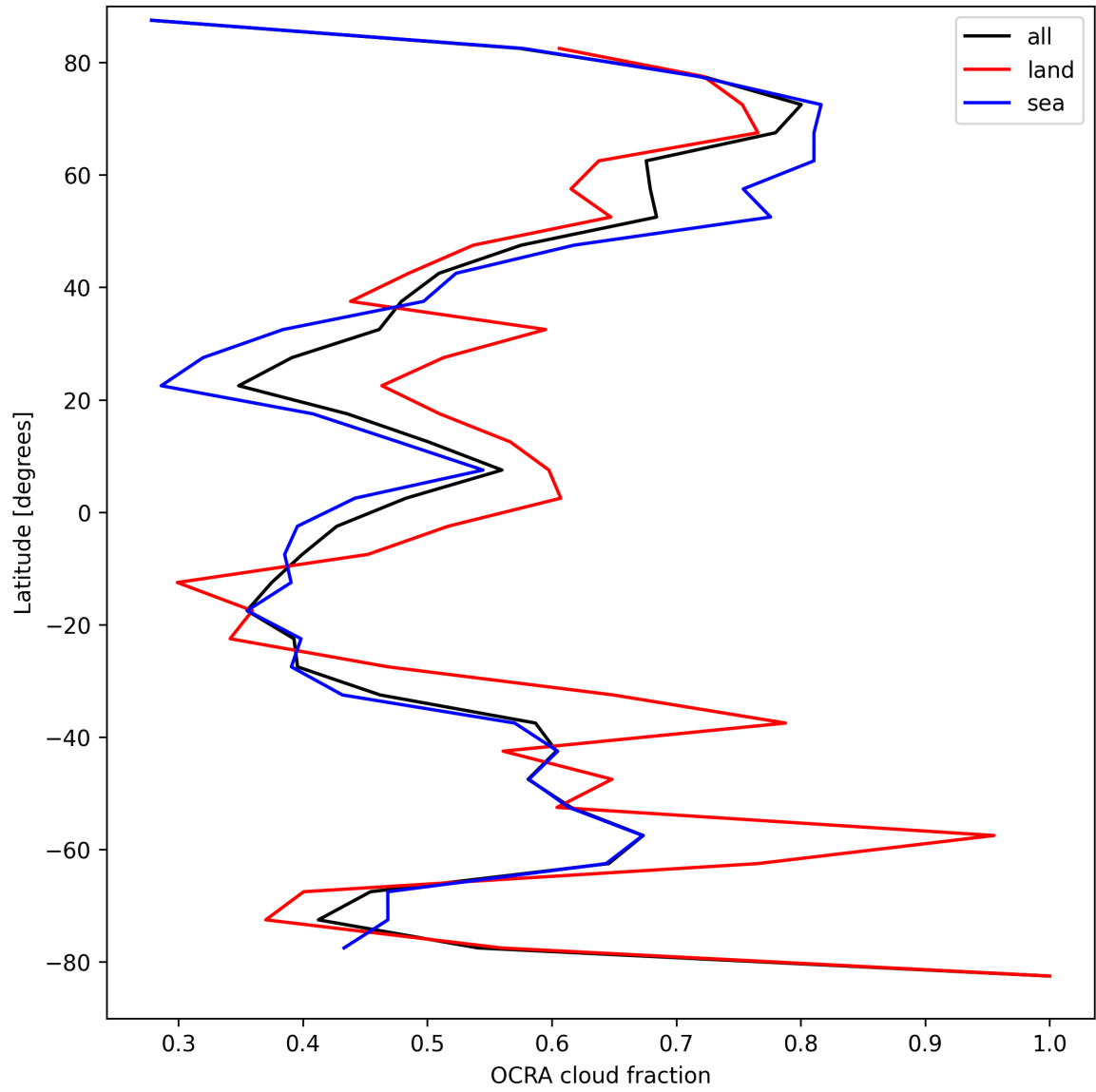
Figure 32: Zonal average of “OCRA cloud fraction” for 2025-08-30 to 2025-08-31.
