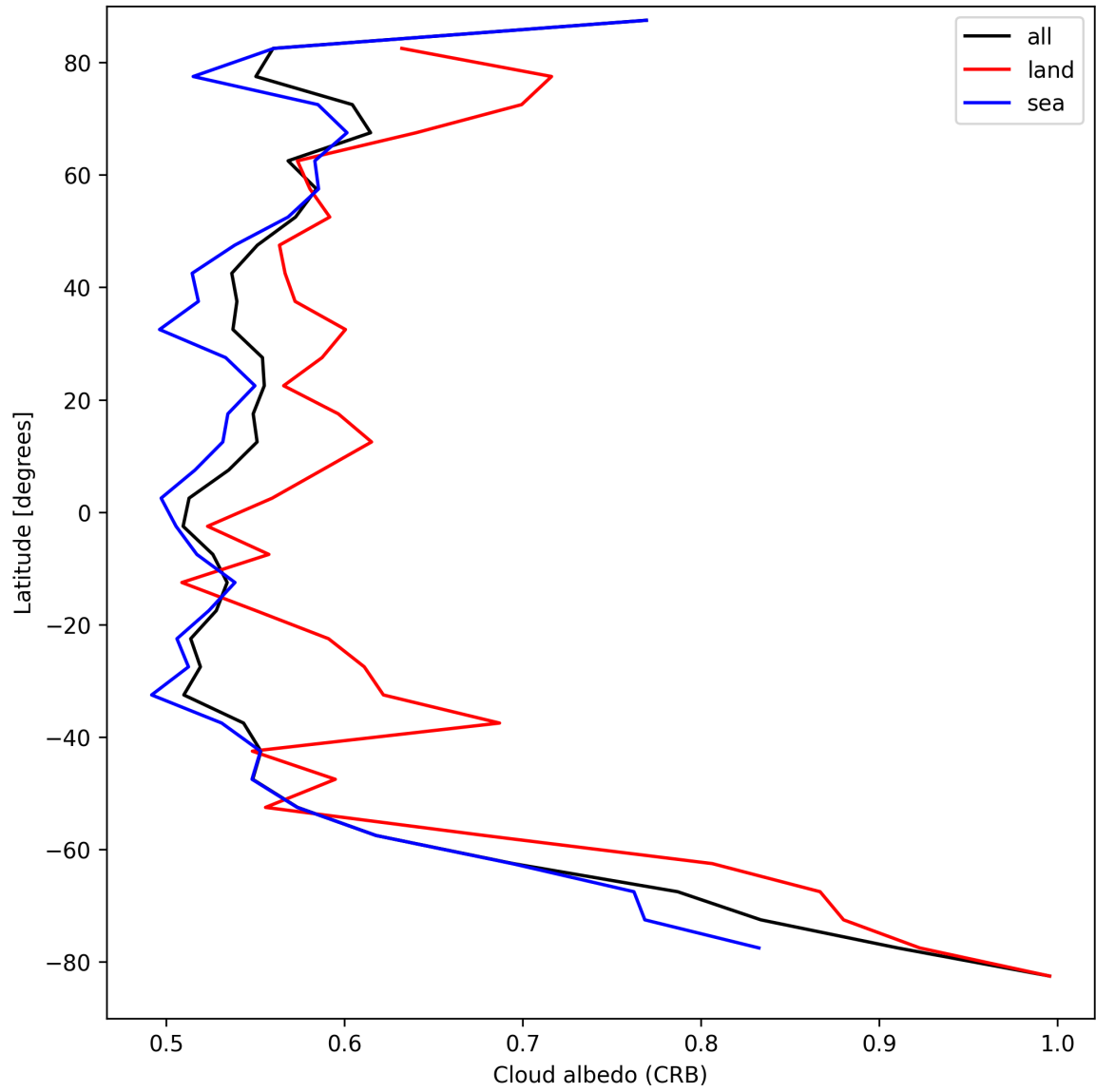
Figure 26: Zonal average of “Cloud albedo (CRB)” for 2025-08-30 to 2025-08-31.
