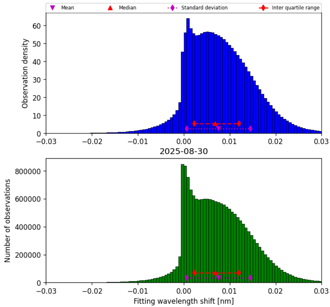
Figure 47: Histogram of “Fitting wavelength shift” for 2025-08-30 to 2025-08-31
