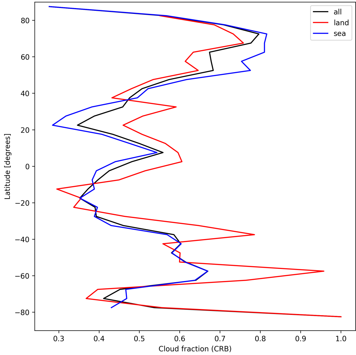
Figure 24: Zonal average of “Cloud fraction (CRB)” for 2025-08-30 to 2025-08-31.
