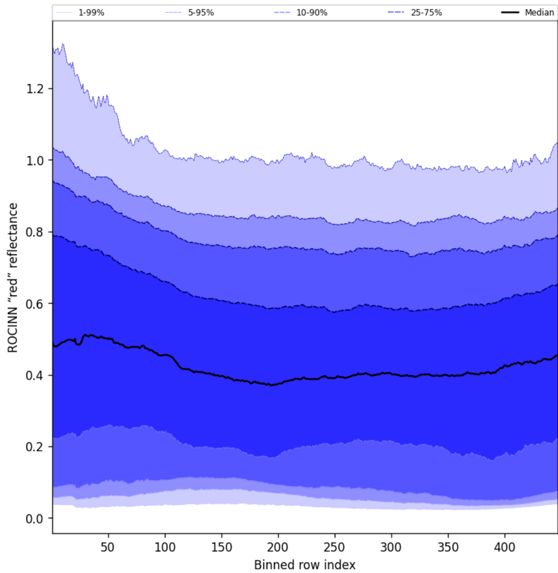
Figure 67: Along track statistics of “ROCINN “red” reflectance” for 2025-08-30 to 2025-08-31
