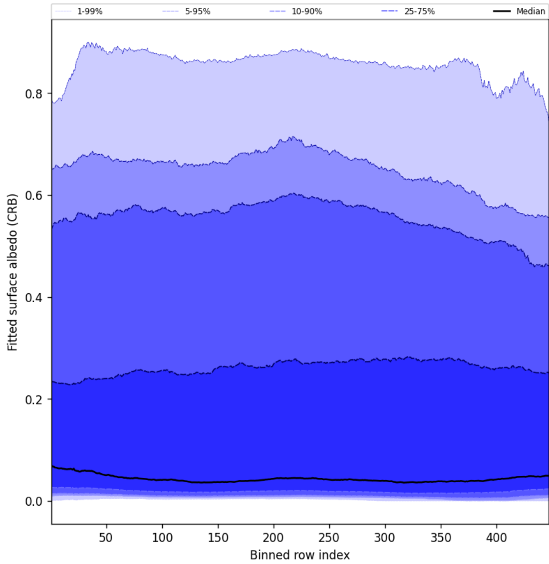
Figure 60: Along track statistics of “Fitted surface albedo (CRB)” for 2025-08-30 to 2025-08-31
