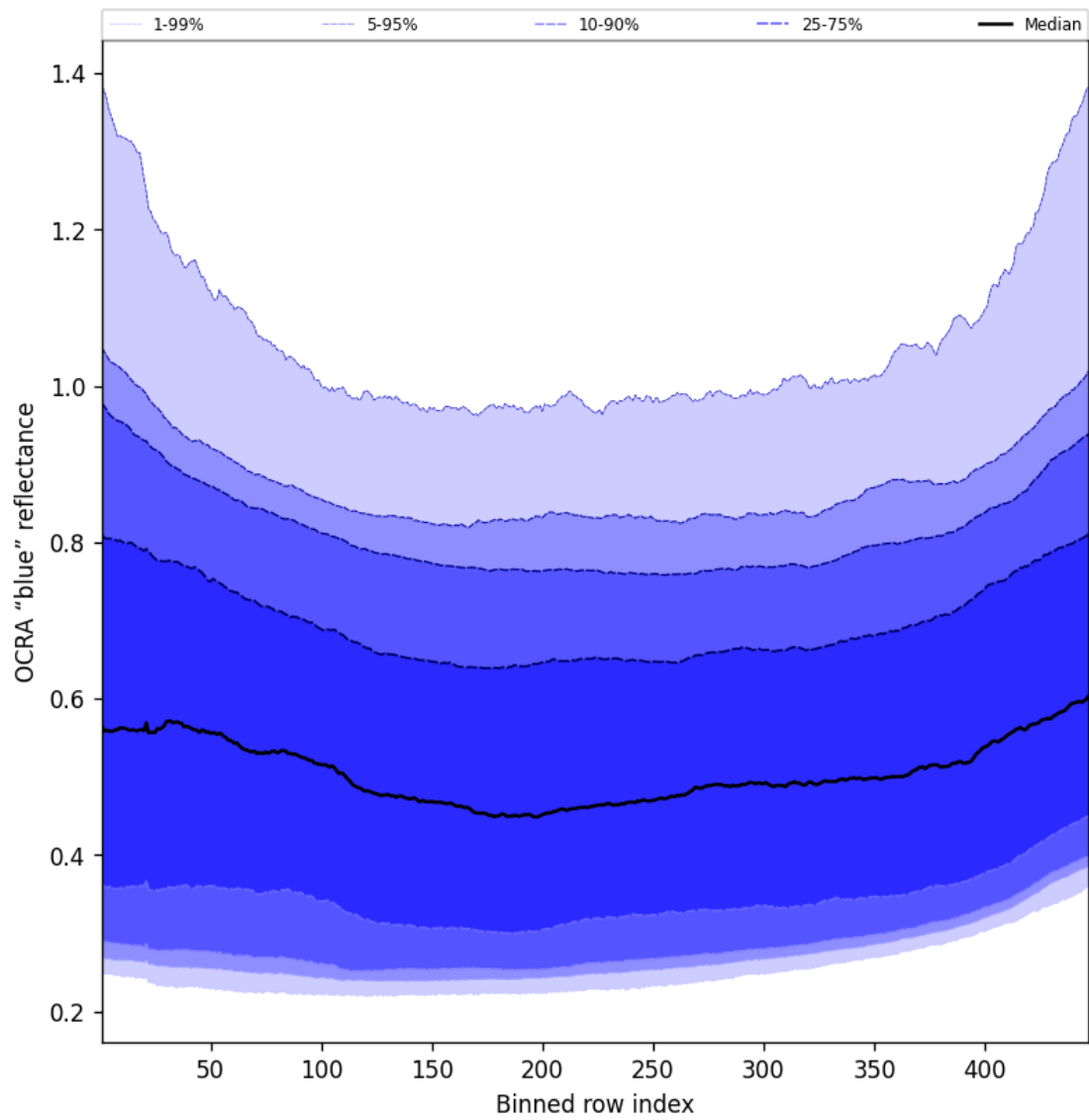
Figure 65: Along track statistics of “OCRA “blue” reflectance” for 2025-08-30 to 2025-08-31
