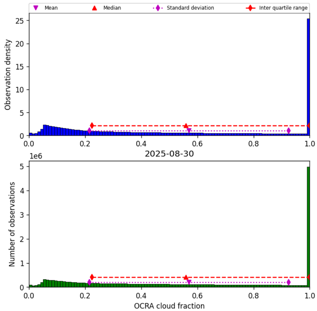
Figure 48: Histogram of “OCRA cloud fraction” for 2025-08-30 to 2025-08-31
