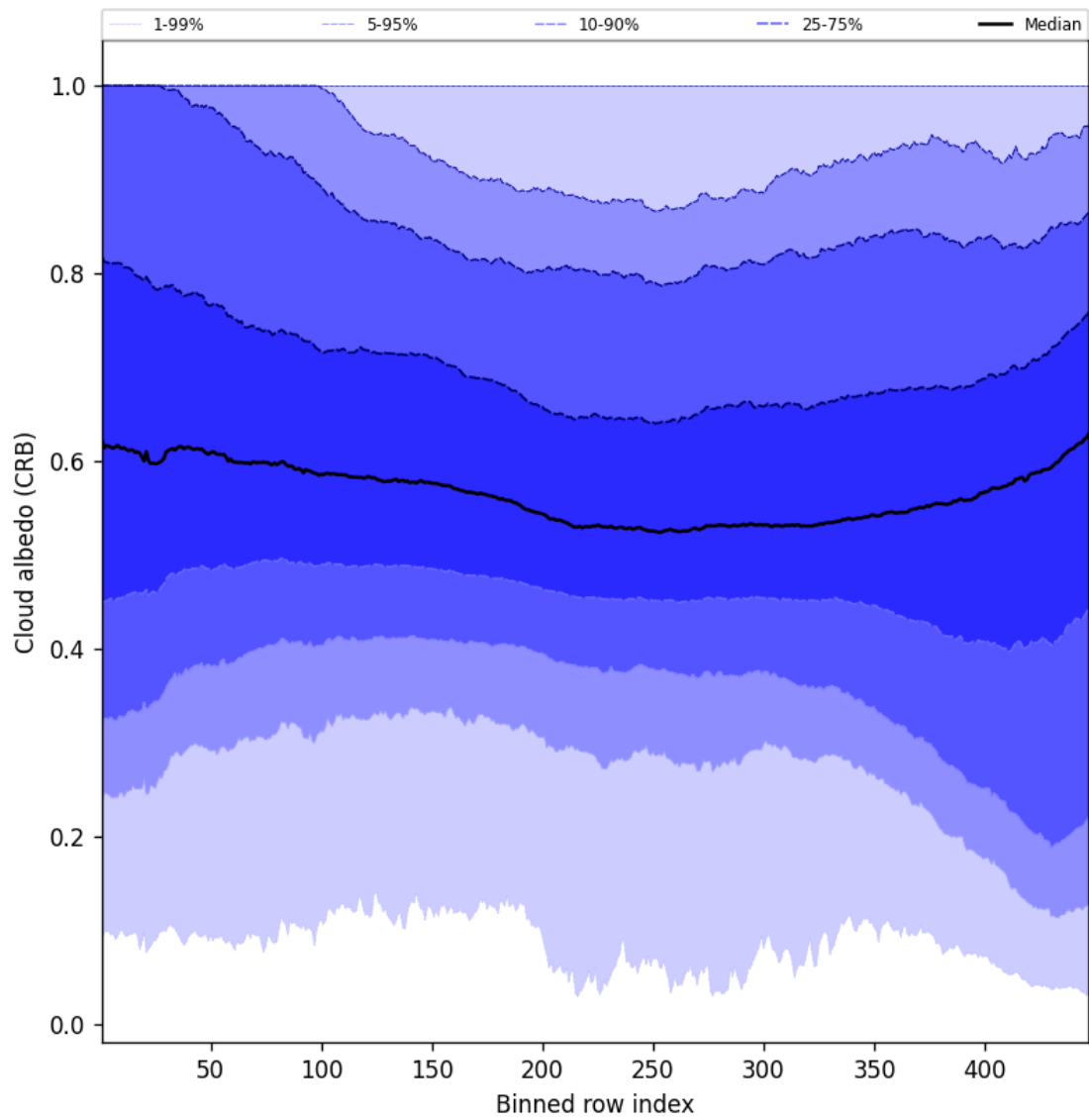
Figure 58: Along track statistics of “Cloud albedo (CRB)” for 2025-08-30 to 2025-08-31
