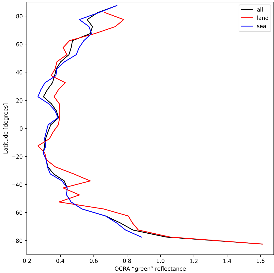
Figure 34: Zonal average of “OCRA “green” reflectance” for 2025-08-30 to 2025-08-31.
