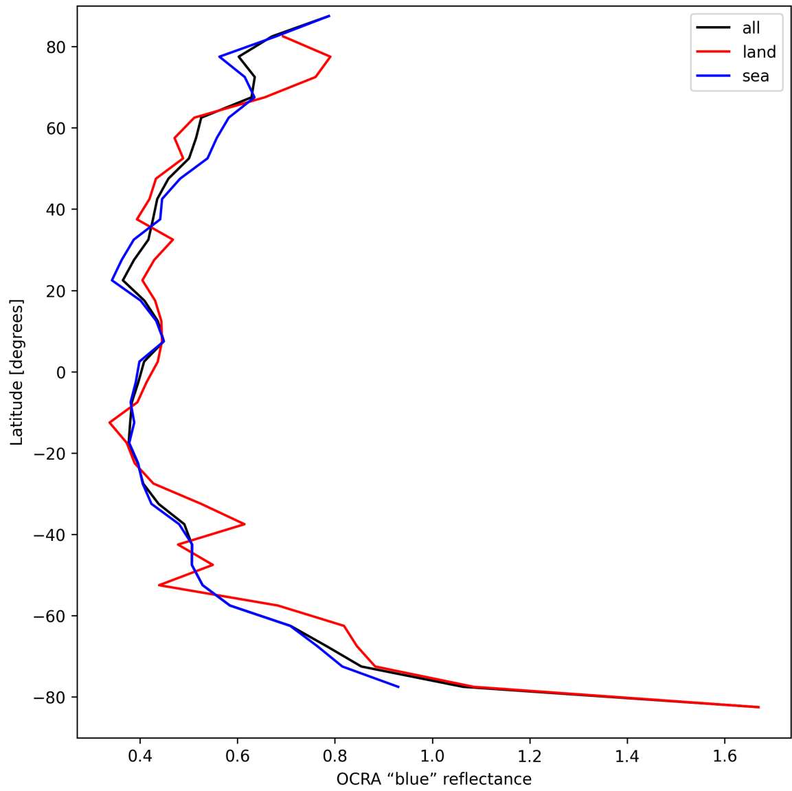
Figure 33: Zonal average of “OCRA “blue” reflectance” for 2025-08-30 to 2025-08-31.
