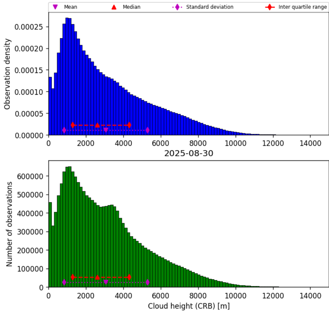
Figure 41: Histogram of “Cloud height (CRB)” for 2025-08-30 to 2025-08-31
