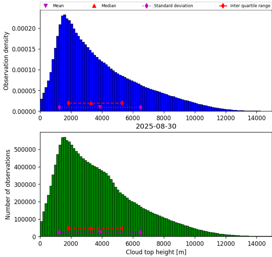
Figure 38: Histogram of “Cloud top height” for 2025-08-30 to 2025-08-31
