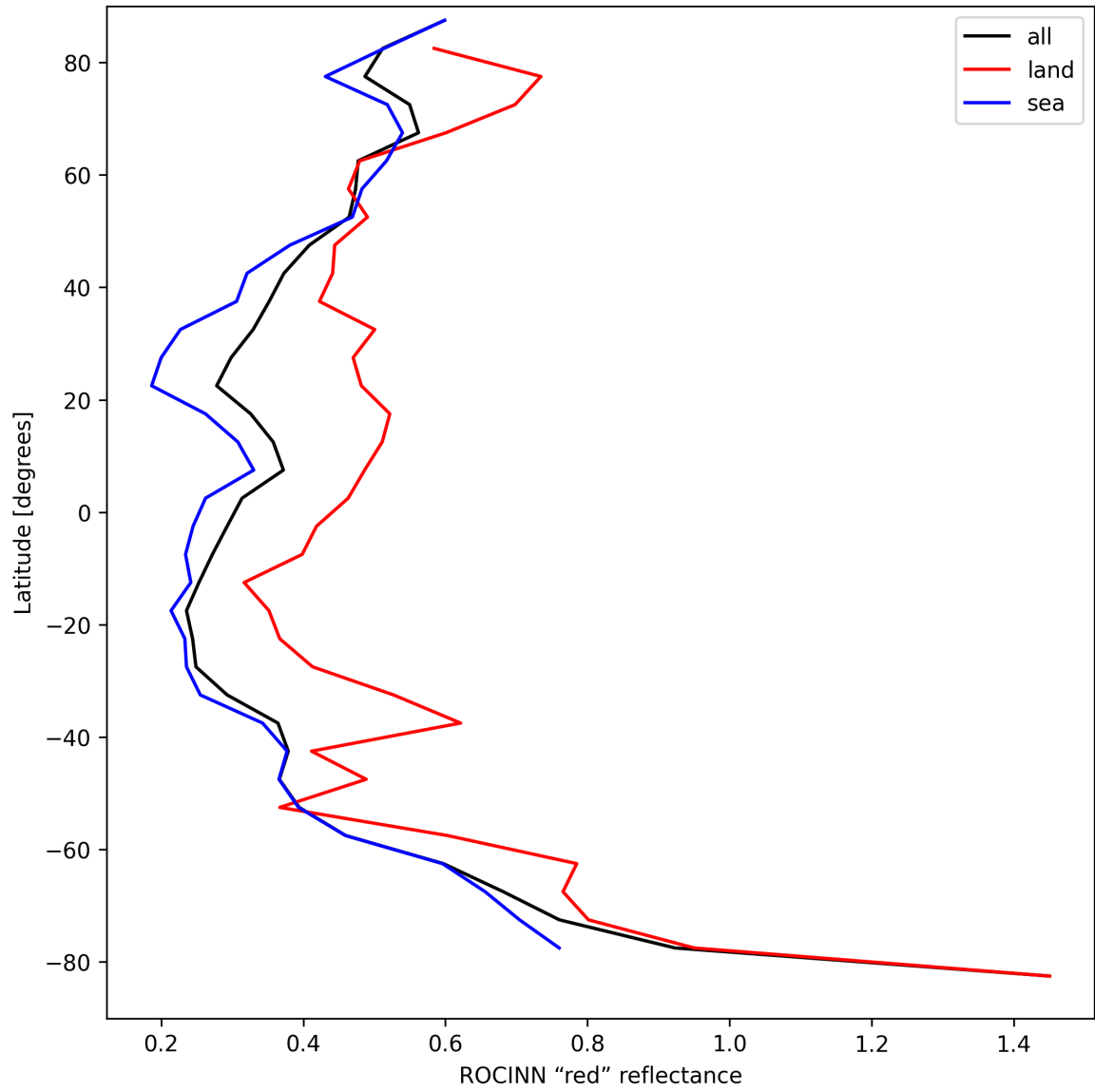
Figure 35: Zonal average of “ROCINN “red” reflectance” for 2025-08-30 to 2025-08-31.
