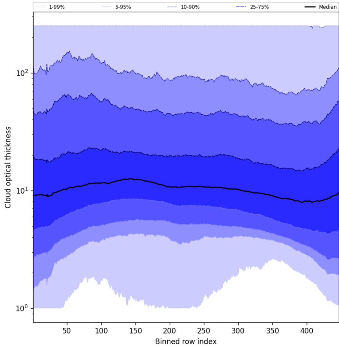
Figure 55: Along track statistics of “Cloud optical thickness” for 2025-08-30 to 2025-08-31
