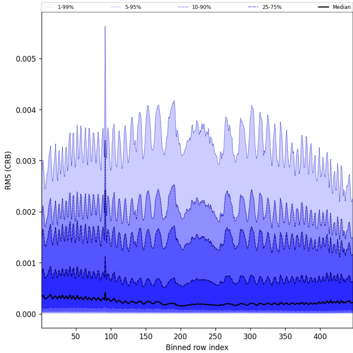
Figure 62: Along track statistics of “RMS (CRB)” for 2025-08-30 to 2025-08-31
