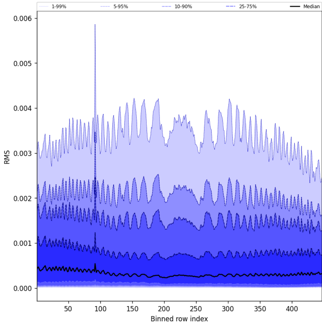
Figure 61: Along track statistics of “RMS” for 2025-08-30 to 2025-08-31
