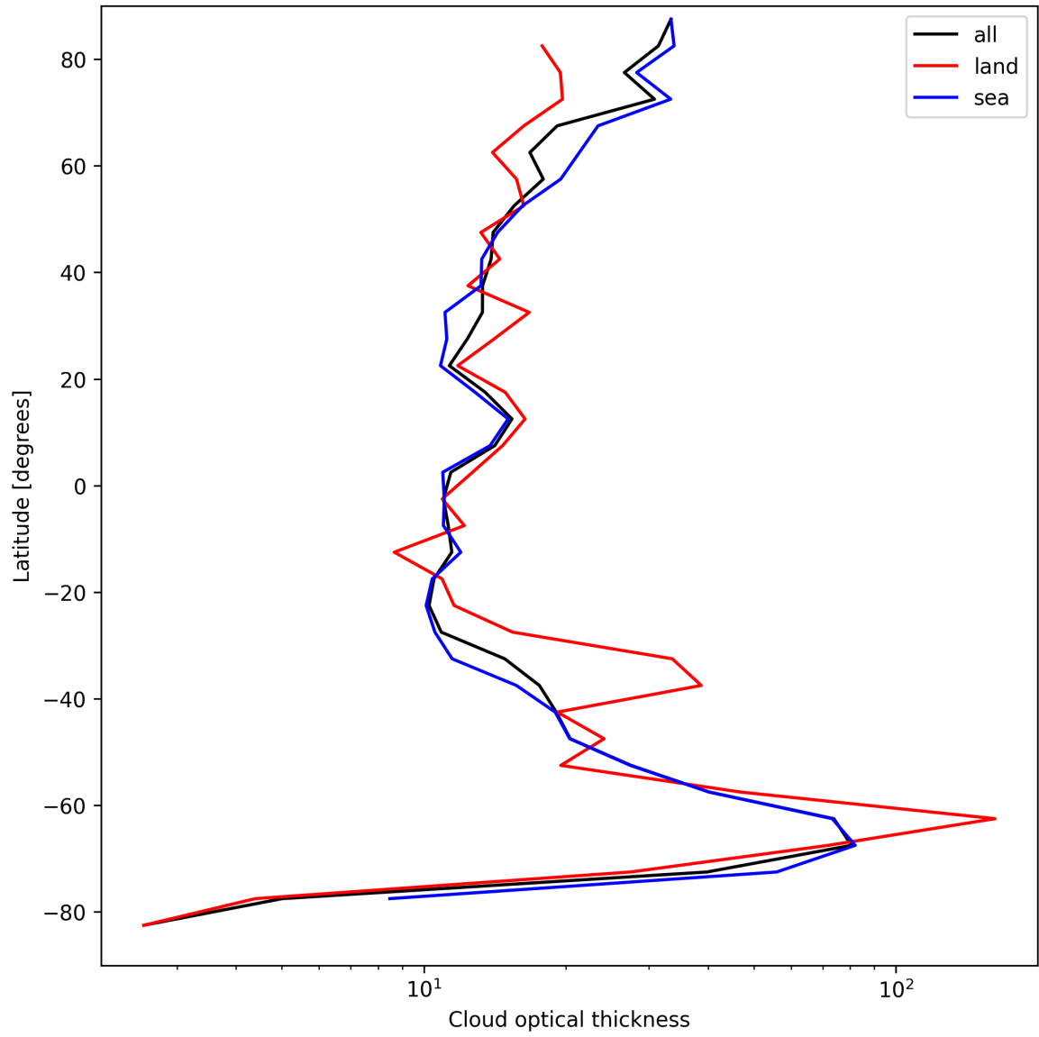
Figure 23: Zonal average of “Cloud optical thickness” for 2025-08-30 to 2025-08-31.
