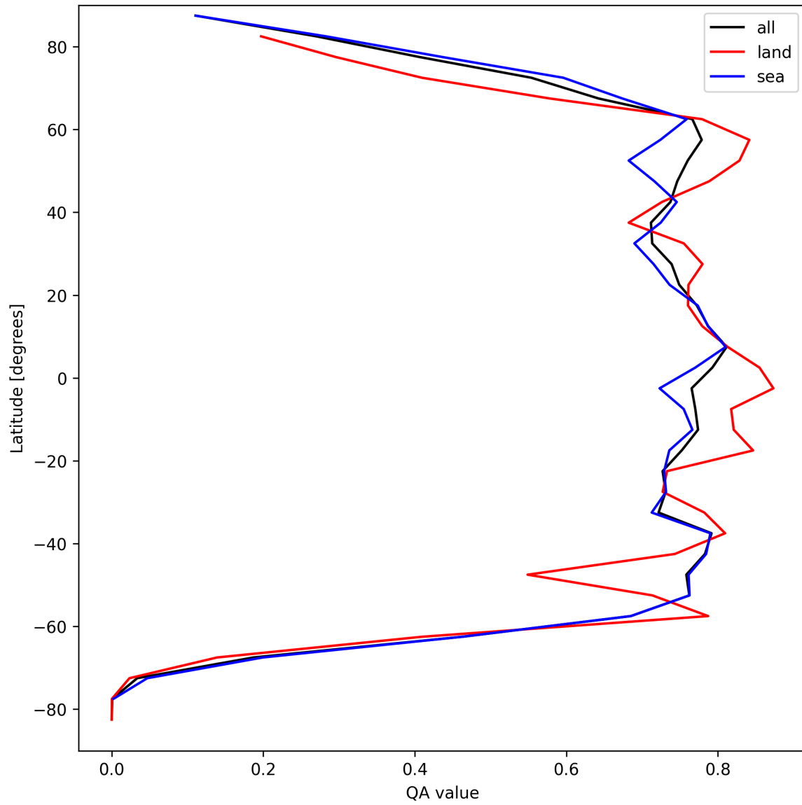
Figure 20: Zonal average of “QA value” for 2025-08-30 to 2025-08-31.
