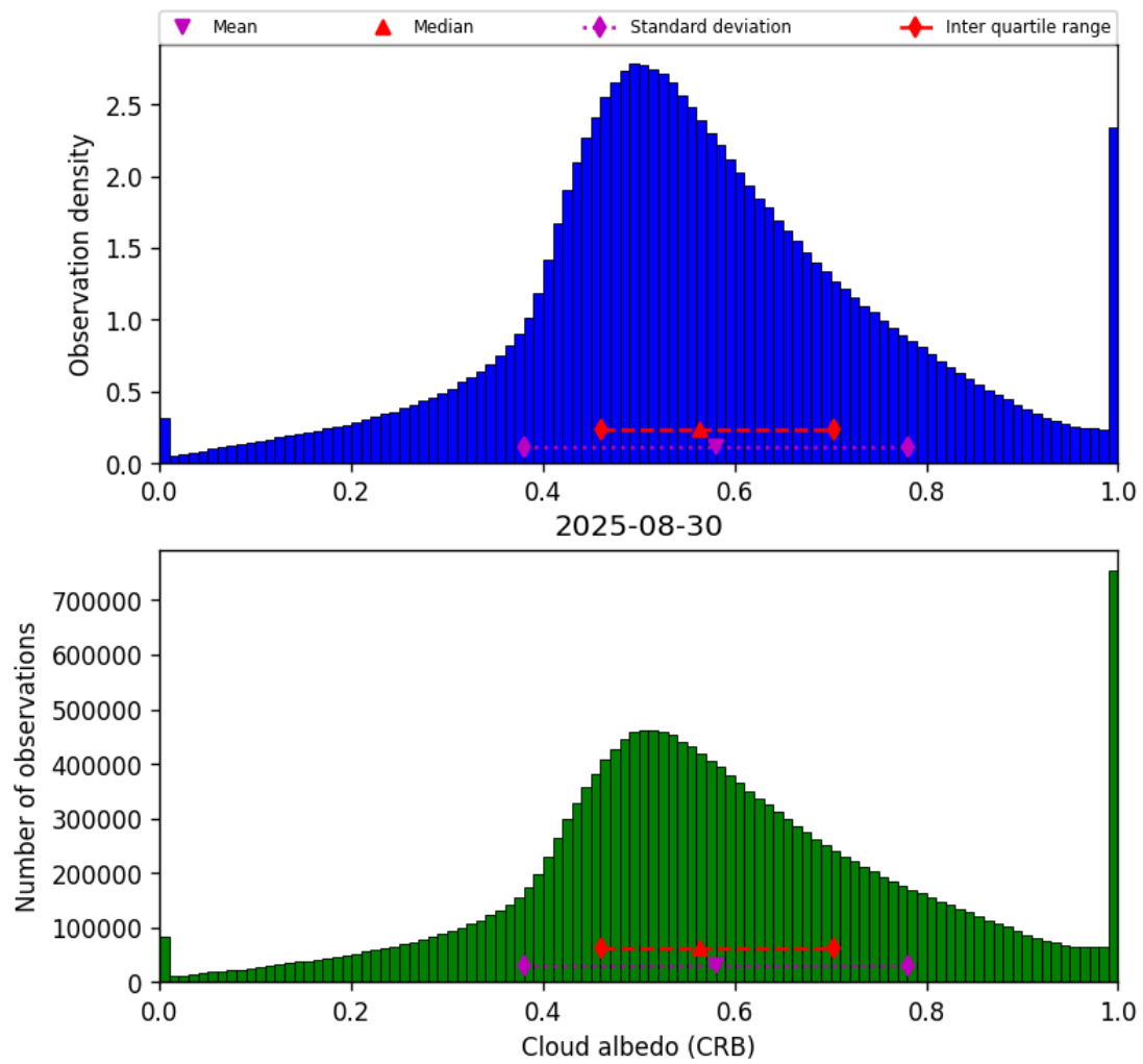
Figure 42: Histogram of “Cloud albedo (CRB)” for 2025-08-30 to 2025-08-31
