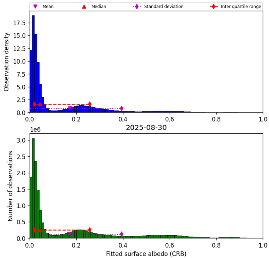
Figure 44: Histogram of “Fitted surface albedo (CRB)” for 2025-08-30 to 2025-08-31
