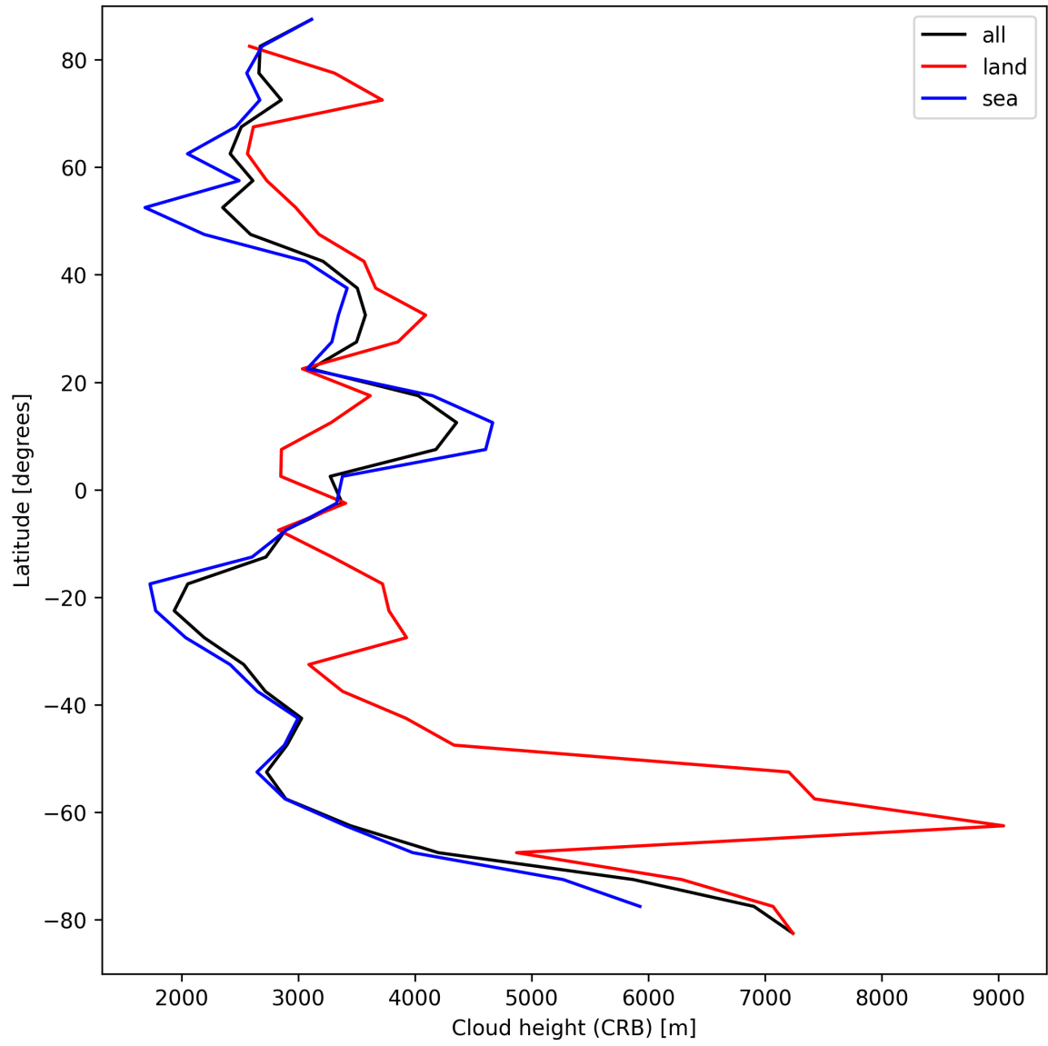
Figure 25: Zonal average of “Cloud height (CRB)” for 2025-08-30 to 2025-08-31.
