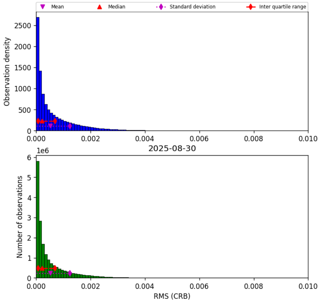
Figure 46: Histogram of “RMS (CRB)” for 2025-08-30 to 2025-08-31
