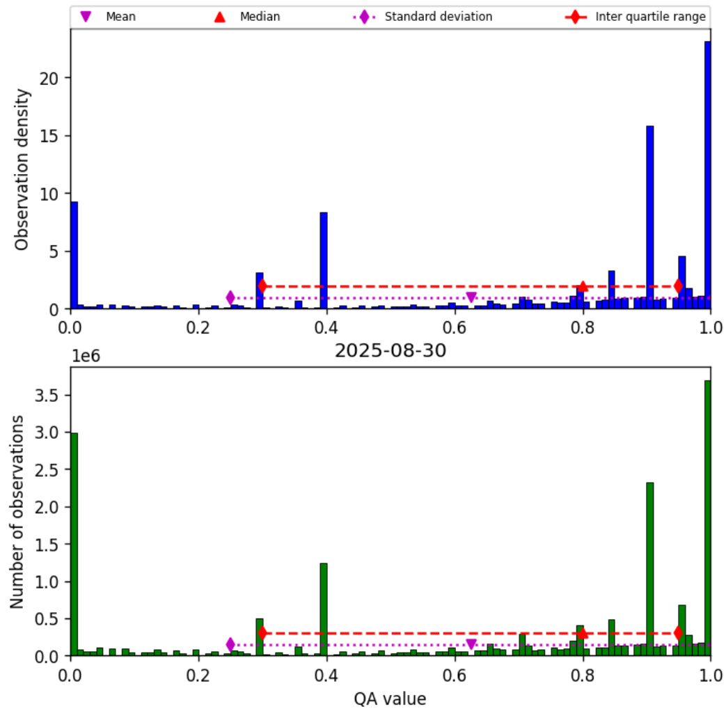
Figure 36: Histogram of “QA value” for 2025-08-30 to 2025-08-31
