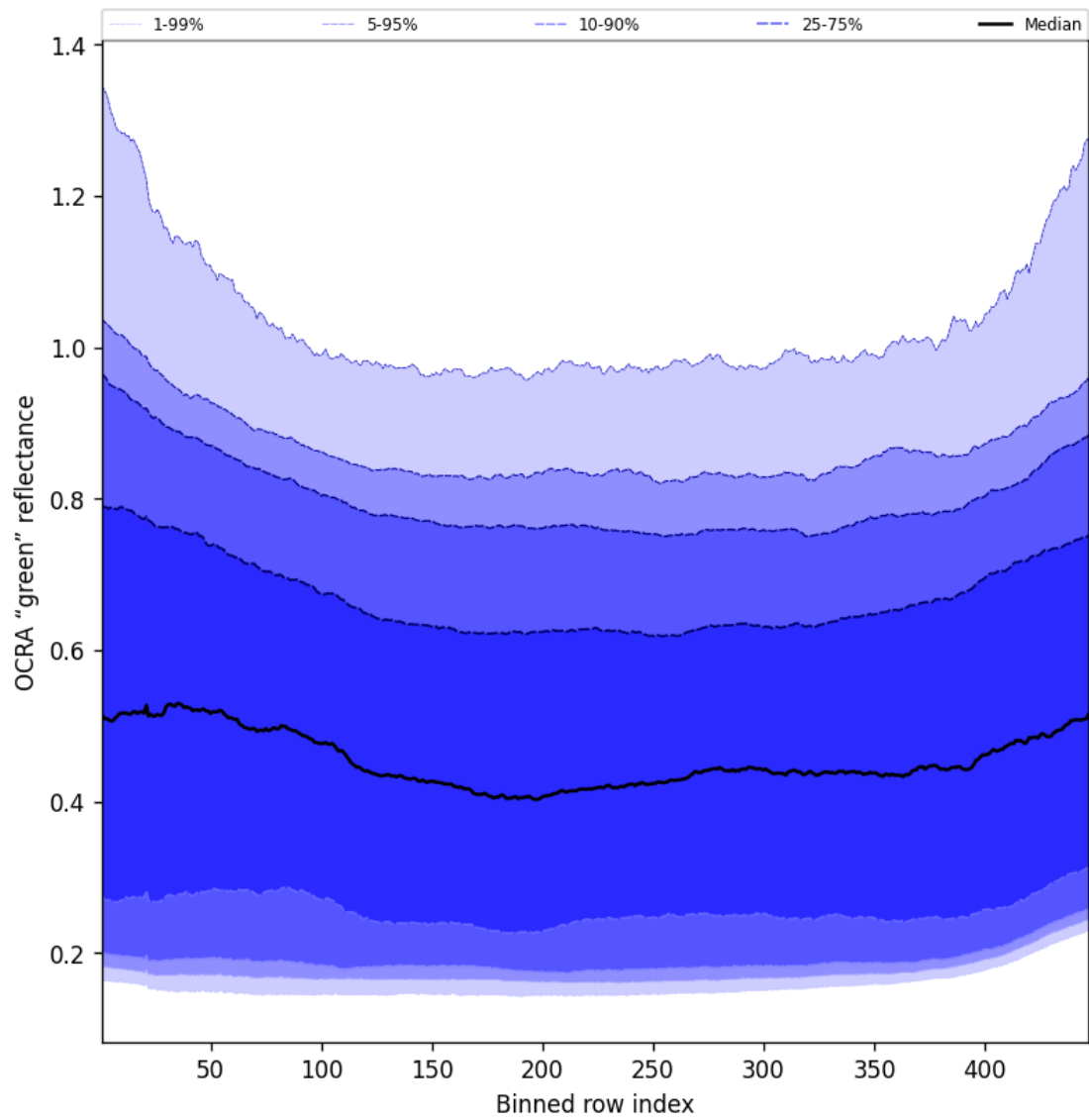
Figure 66: Along track statistics of “OCRA “green” reflectance” for 2025-08-30 to 2025-08-31
