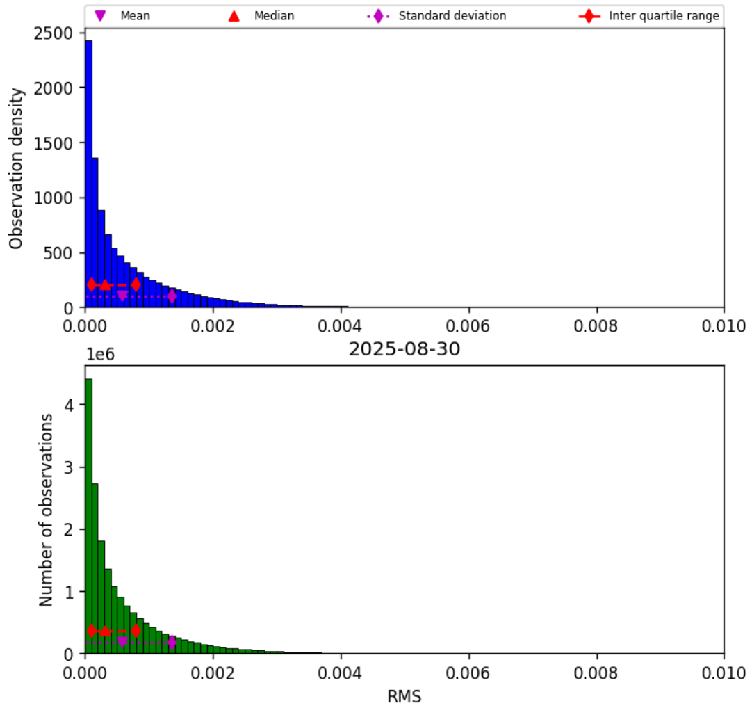
Figure 45: Histogram of “RMS” for 2025-08-30 to 2025-08-31
