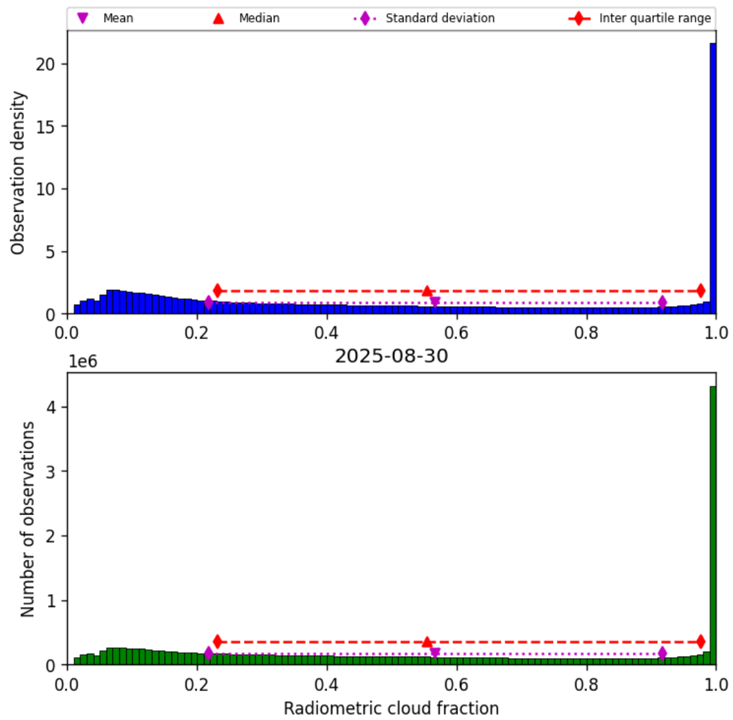
Figure 37: Histogram of “Radiometric cloud fraction” for 2025-08-30 to 2025-08-31
