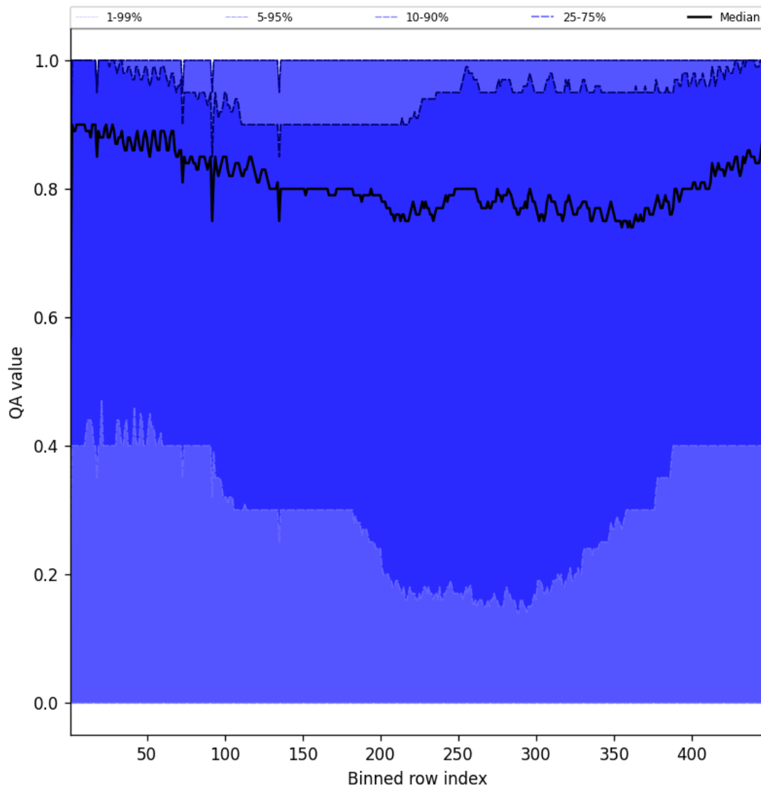
Figure 52: Along track statistics of “QA value” for 2025-08-30 to 2025-08-31
