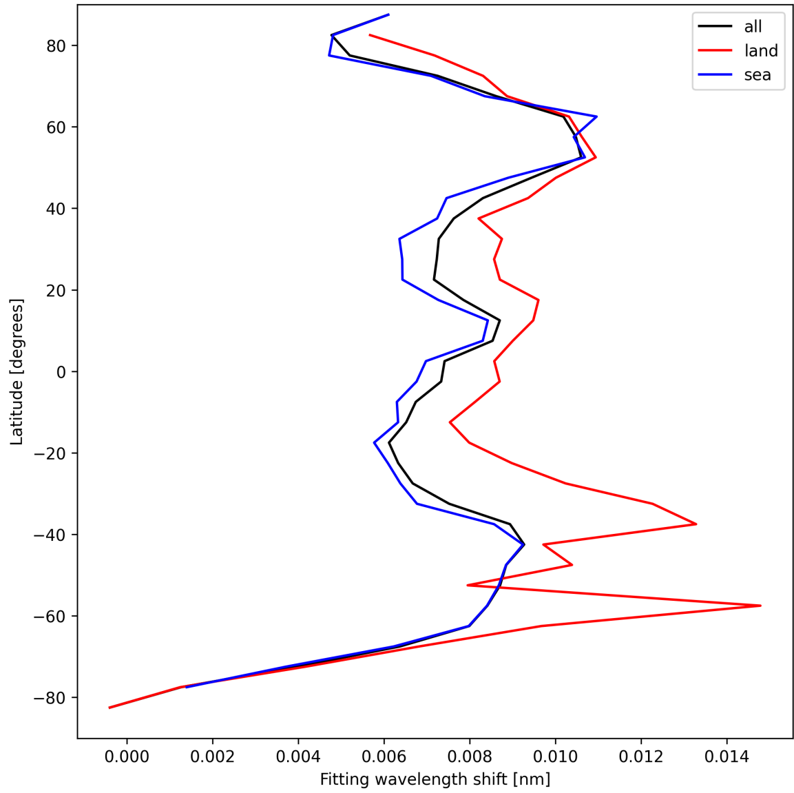
Figure 31: Zonal average of “Fitting wavelength shift” for 2025-08-30 to 2025-08-31.
