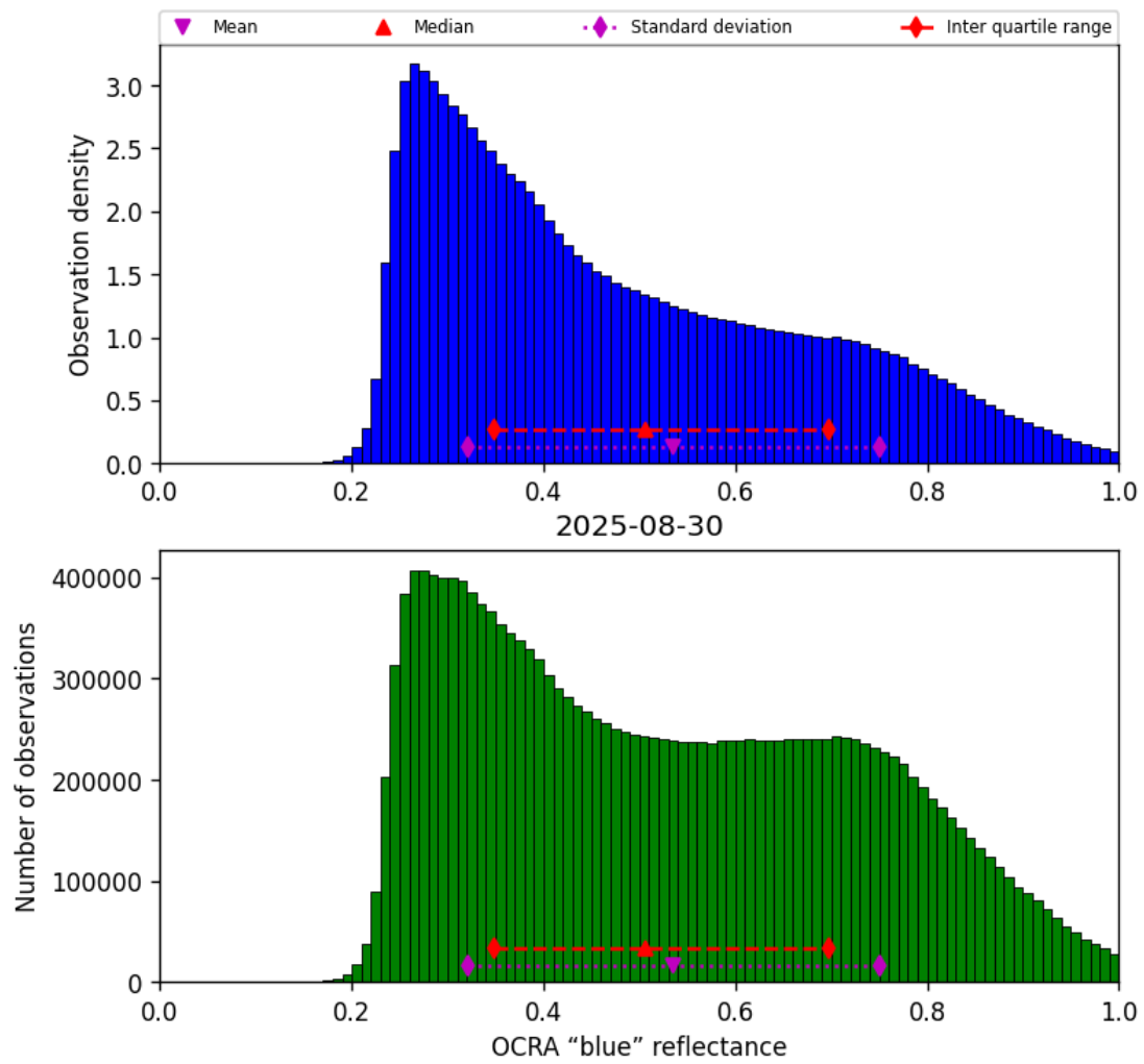
Figure 49: Histogram of “OCRA “blue” reflectance” for 2025-08-30 to 2025-08-31
