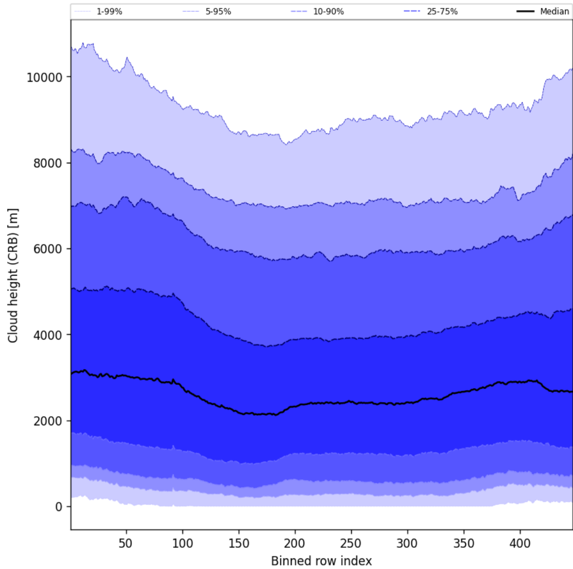
Figure 57: Along track statistics of “Cloud height (CRB)” for 2025-08-30 to 2025-08-31
