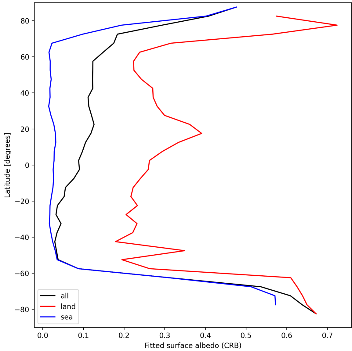
Figure 28: Zonal average of “Fitted surface albedo (CRB)” for 2025-08-30 to 2025-08-31.
