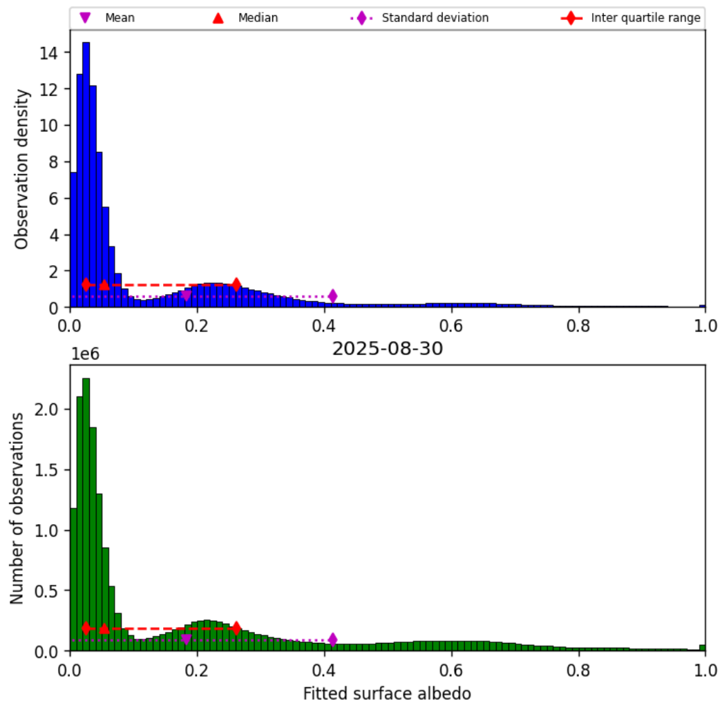
Figure 43: Histogram of “Fitted surface albedo” for 2025-08-30 to 2025-08-31
