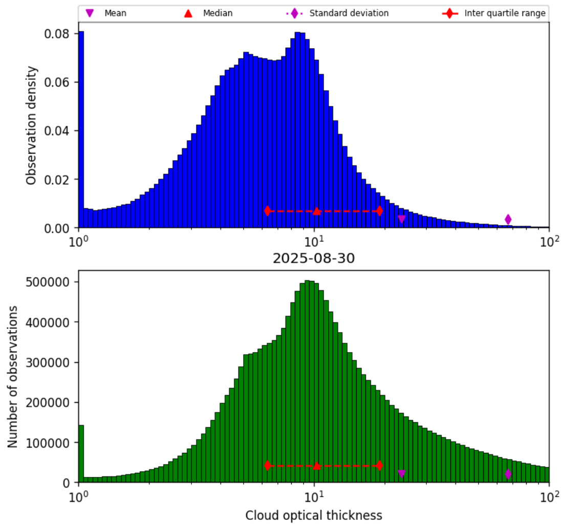
Figure 39: Histogram of “Cloud optical thickness” for 2025-08-30 to 2025-08-31
