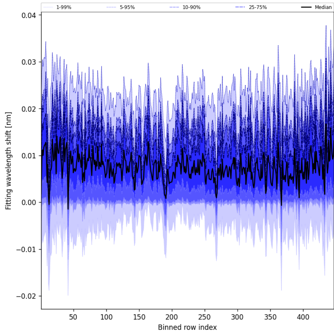
Figure 63: Along track statistics of “Fitting wavelength shift” for 2025-08-30 to 2025-08-31
