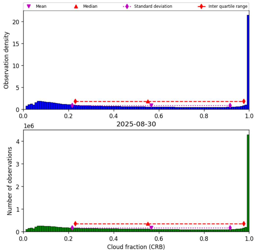
Figure 40: Histogram of “Cloud fraction (CRB)” for 2025-08-30 to 2025-08-31
