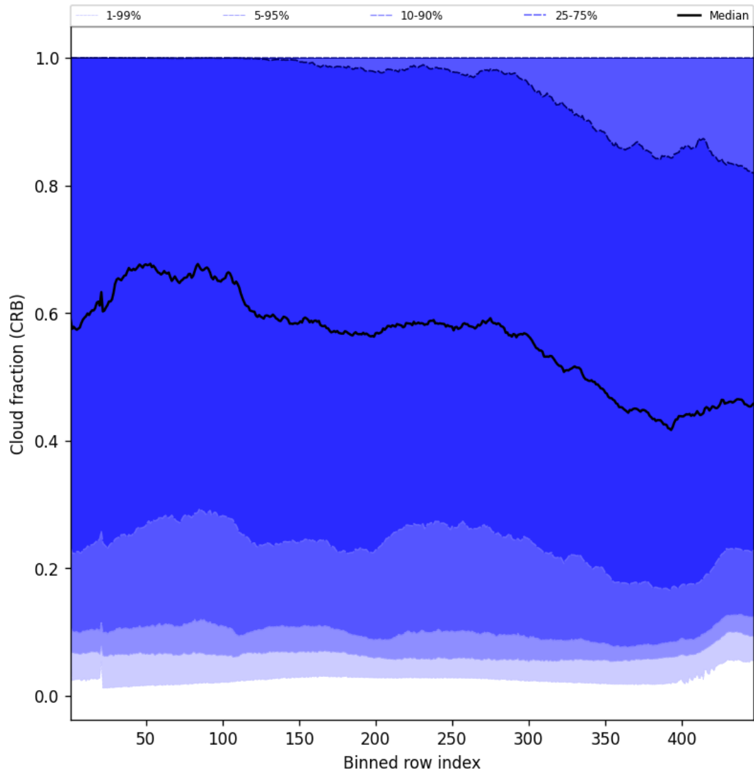
Figure 56: Along track statistics of “Cloud fraction (CRB)” for 2025-08-30 to 2025-08-31
