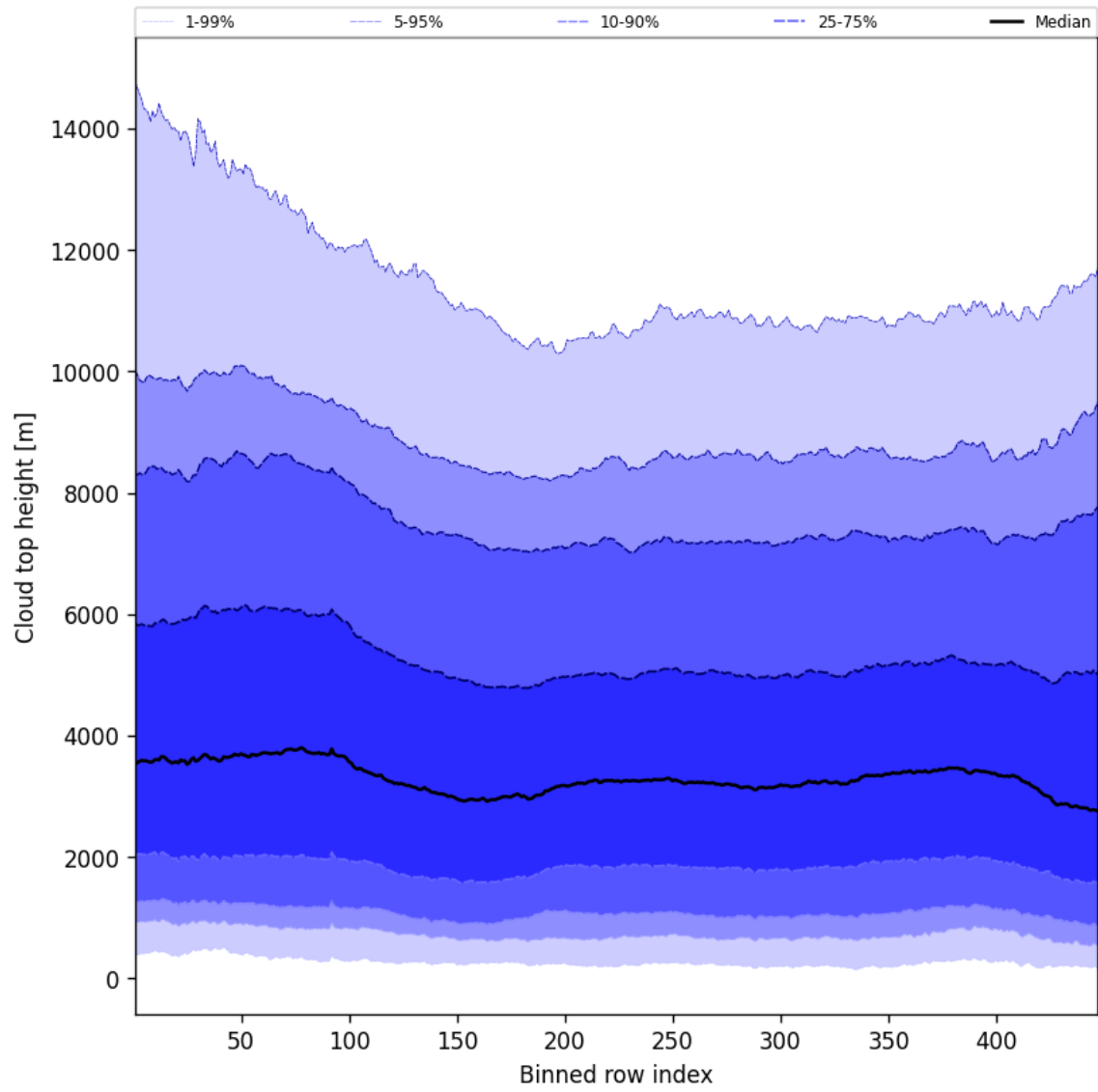
Figure 54: Along track statistics of “Cloud top height” for 2025-08-30 to 2025-08-31
