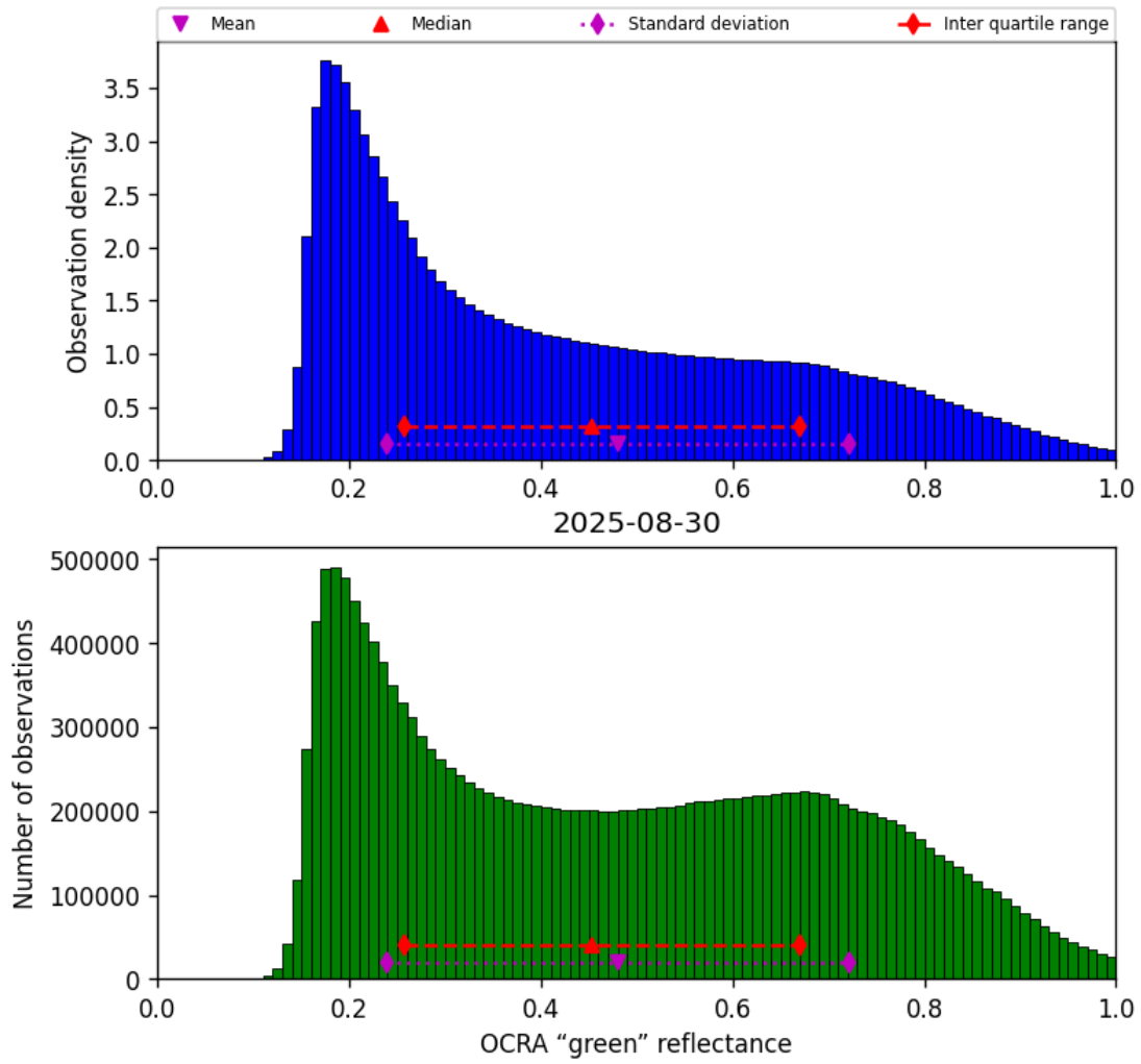
Figure 50: Histogram of “OCRA “green” reflectance” for 2025-08-30 to 2025-08-31
