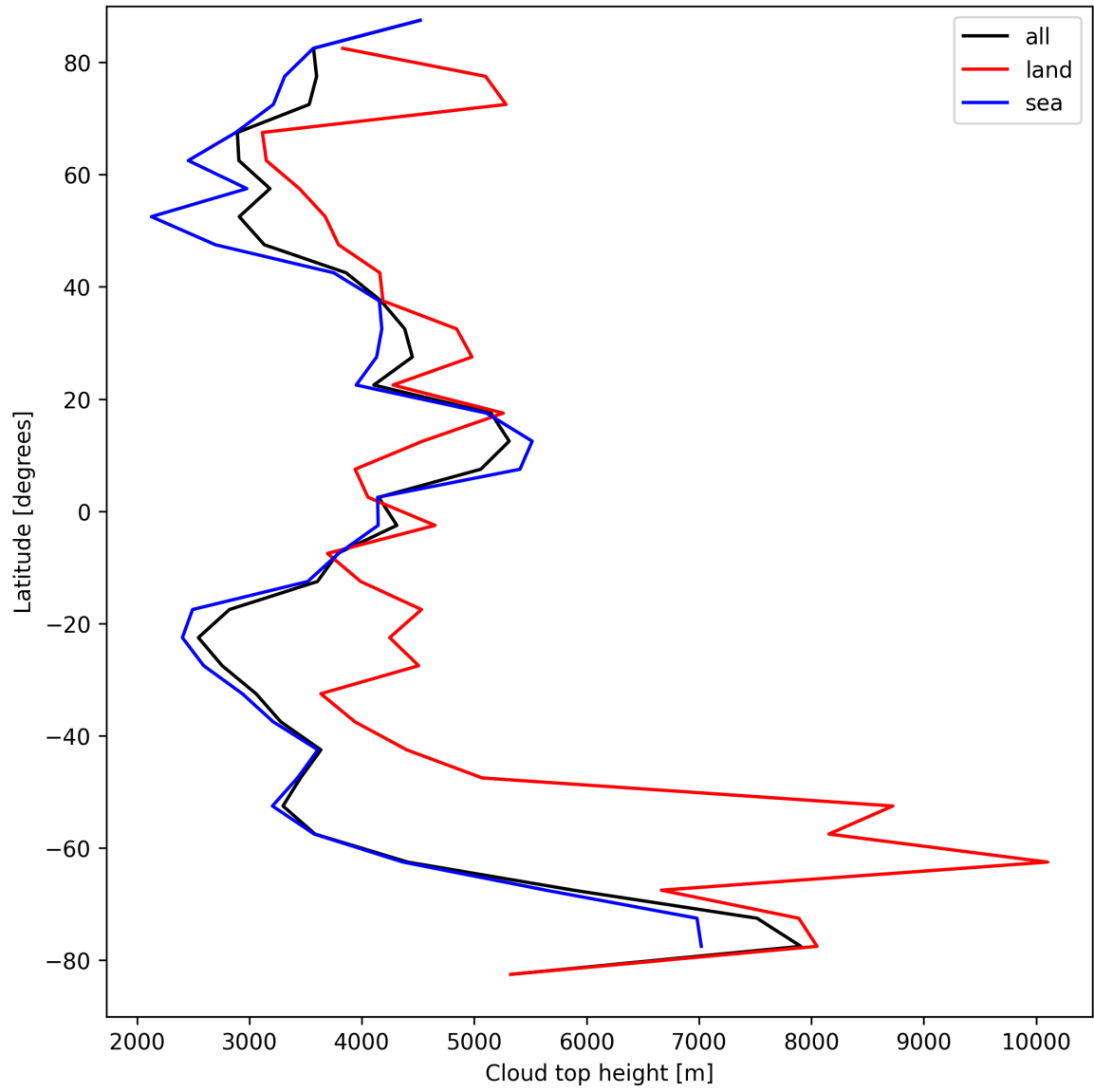
Figure 22: Zonal average of “Cloud top height” for 2025-08-30 to 2025-08-31.
