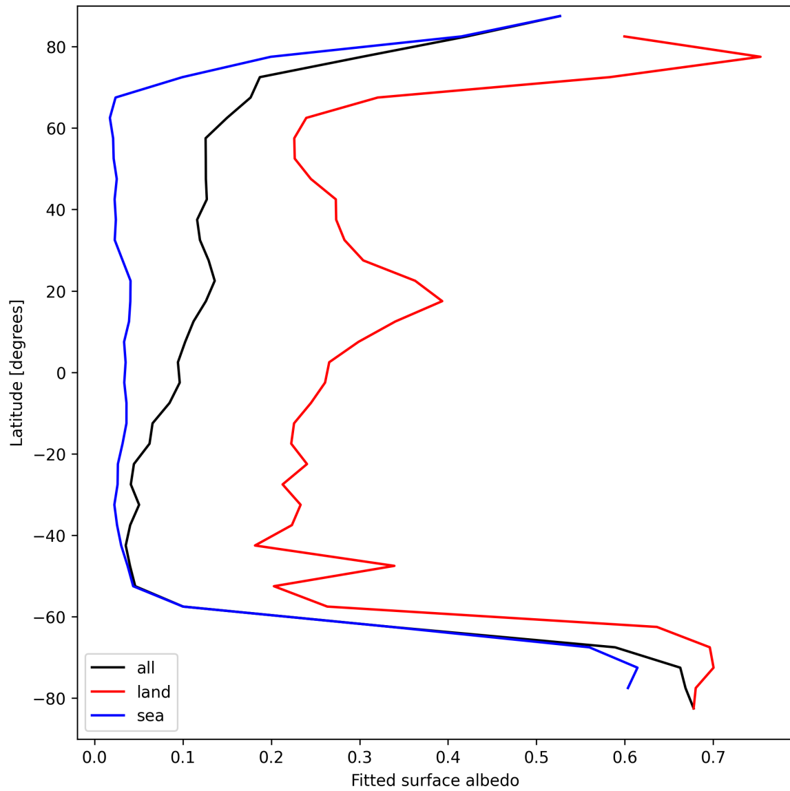
Figure 27: Zonal average of “Fitted surface albedo” for 2025-08-30 to 2025-08-31.
