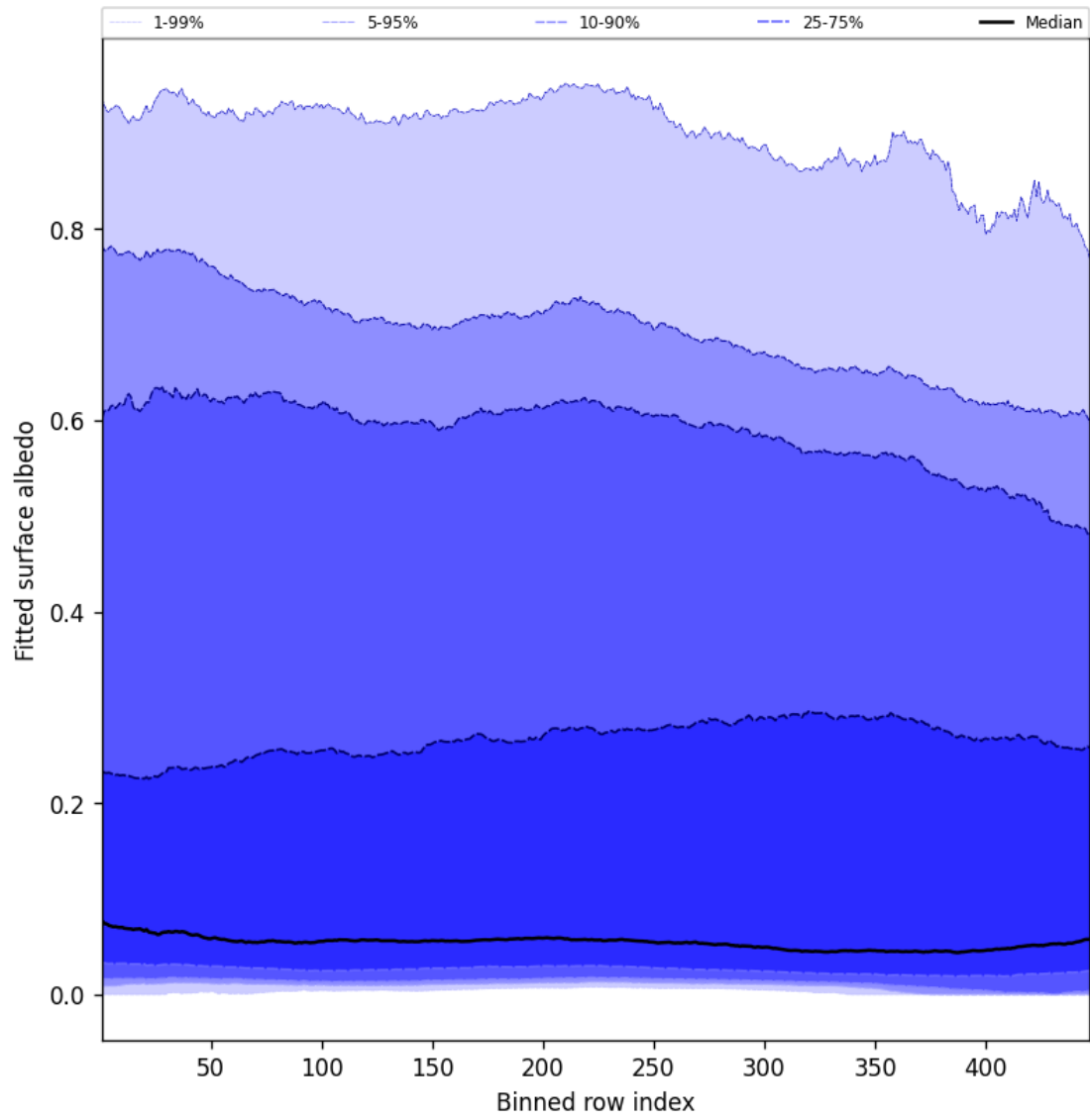
Figure 59: Along track statistics of “Fitted surface albedo” for 2025-08-30 to 2025-08-31
