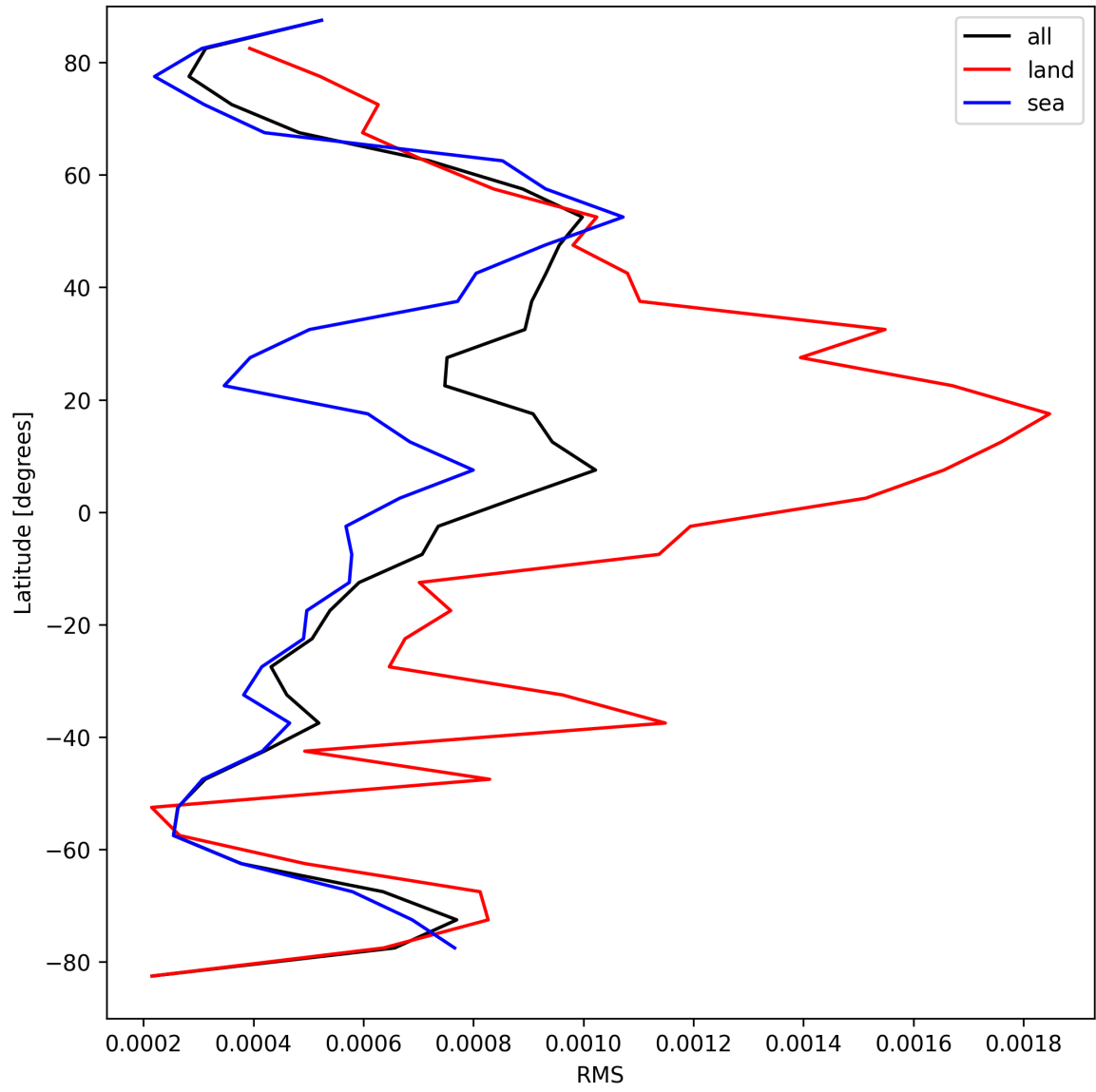
Figure 29: Zonal average of “RMS” for 2025-08-30 to 2025-08-31.
