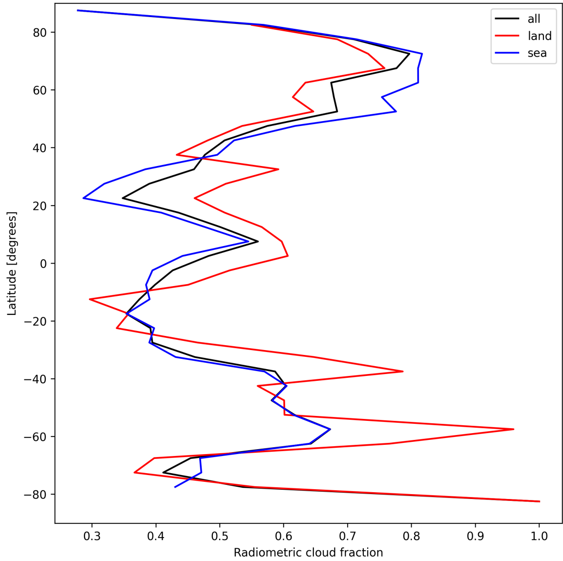
Figure 21: Zonal average of “Radiometric cloud fraction” for 2025-08-30 to 2025-08-31.
