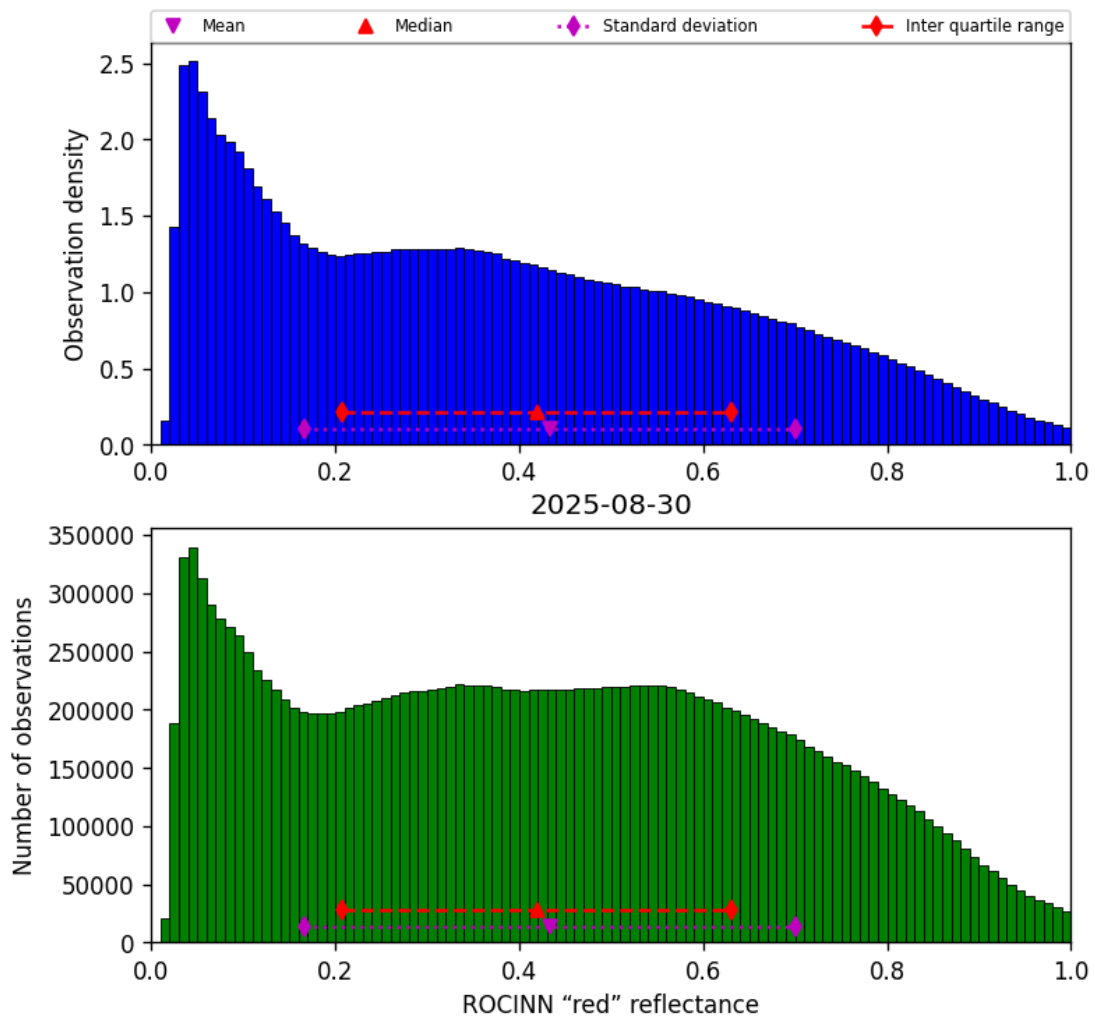
Figure 51: Histogram of “ROCINN “red” reflectance” for 2025-08-30 to 2025-08-31
