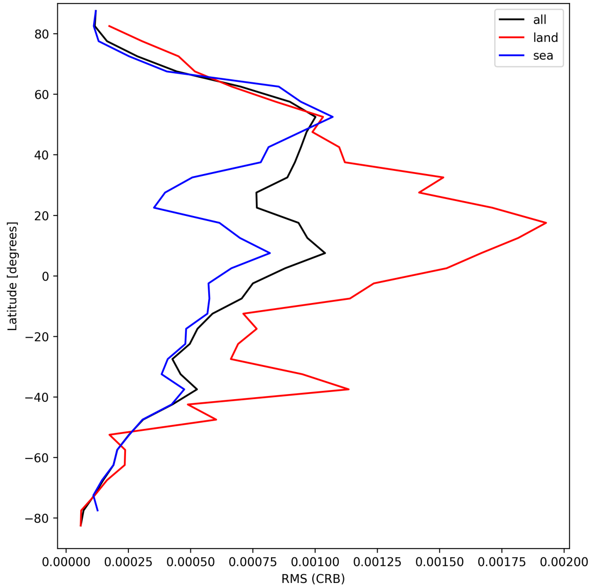
Figure 30: Zonal average of “RMS (CRB)” for 2025-08-30 to 2025-08-31.
