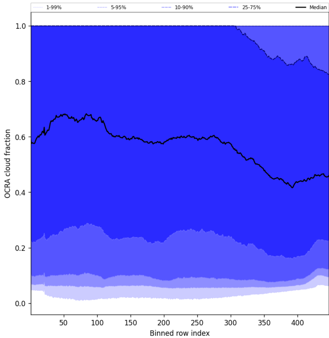
Figure 64: Along track statistics of “OCRA cloud fraction” for 2025-08-30 to 2025-08-31
