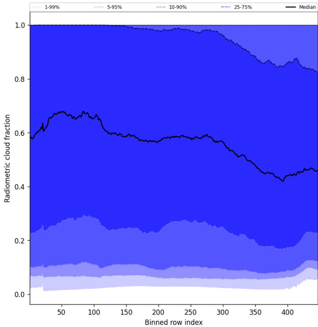
Figure 53: Along track statistics of “Radiometric cloud fraction” for 2025-08-30 to 2025-08-31
