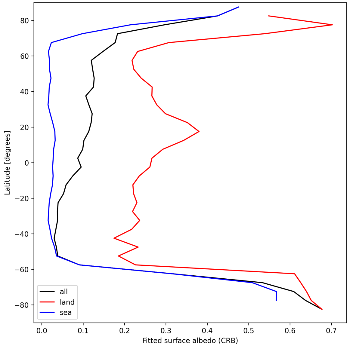
Figure 28: Zonal average of “Fitted surface albedo (CRB)” for 2025-08-31 to 2025-09-01.
