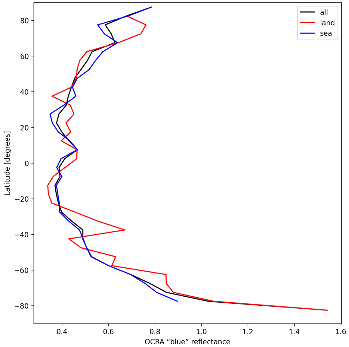
Figure 33: Zonal average of "OCRA "blue" reflectance" for 2025-08-31 to 2025-09-01.
