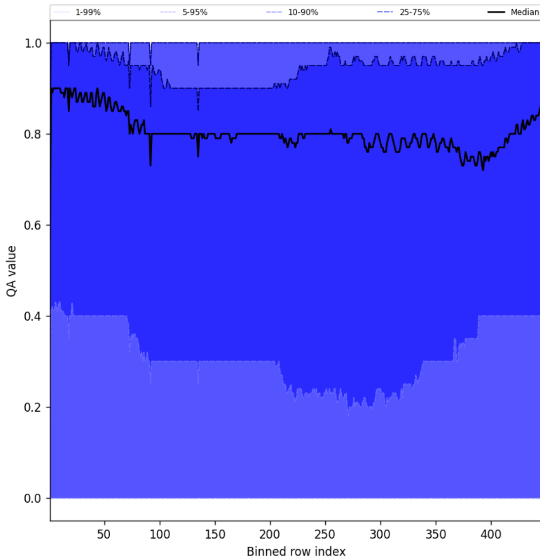
Figure 52: Along track statistics of “QA value” for 2025-08-31 to 2025-09-01
