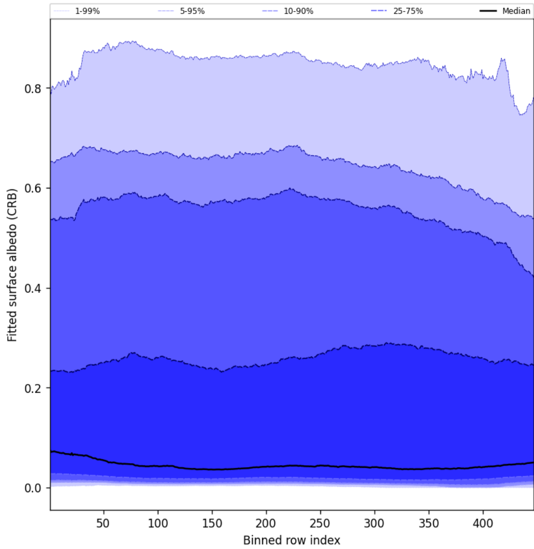
Figure 60: Along track statistics of “Fitted surface albedo (CRB)” for 2025-08-31 to 2025-09-01
