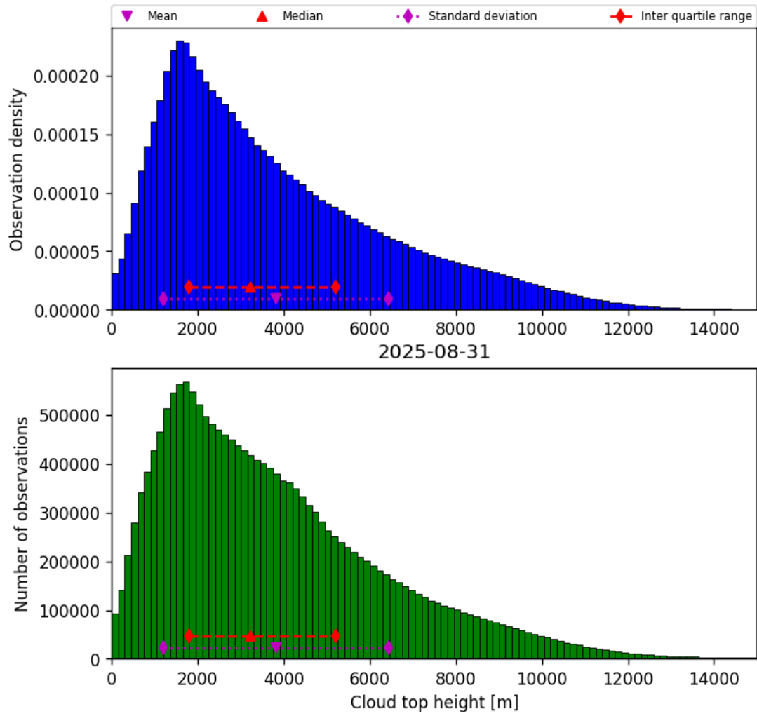
Figure 38: Histogram of “Cloud top height” for 2025-08-31 to 2025-09-01
