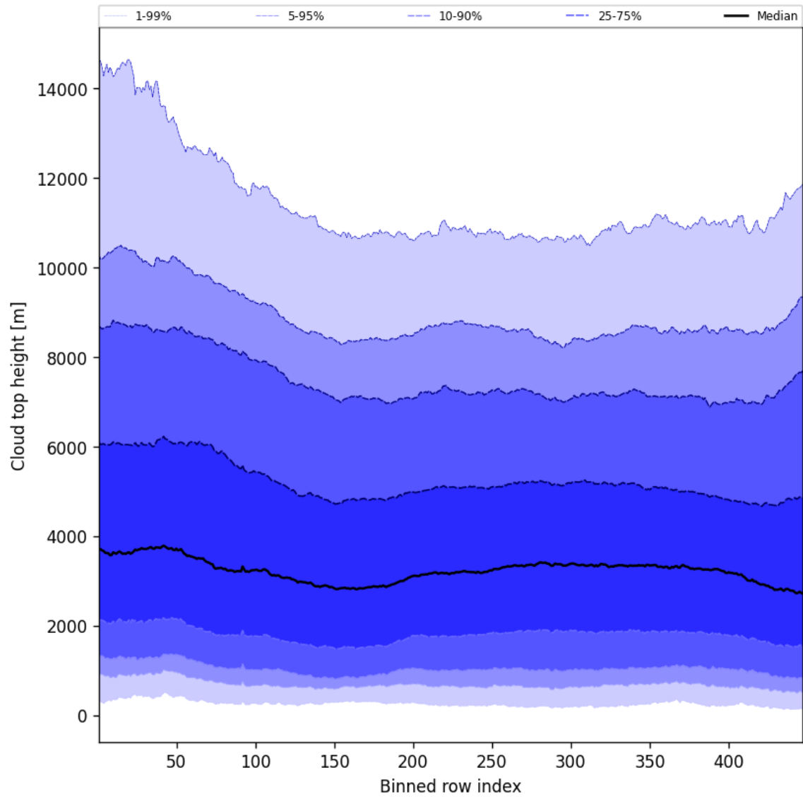
Figure 54: Along track statistics of “Cloud top height” for 2025-08-31 to 2025-09-01
