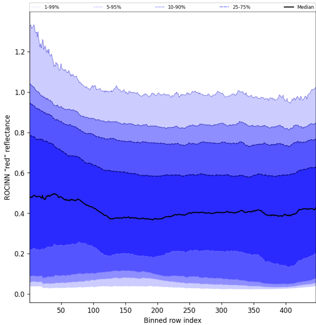
Figure 67: Along track statistics of "ROCINN "red" reflectance" for 2025-08-31 to 2025-09-01
