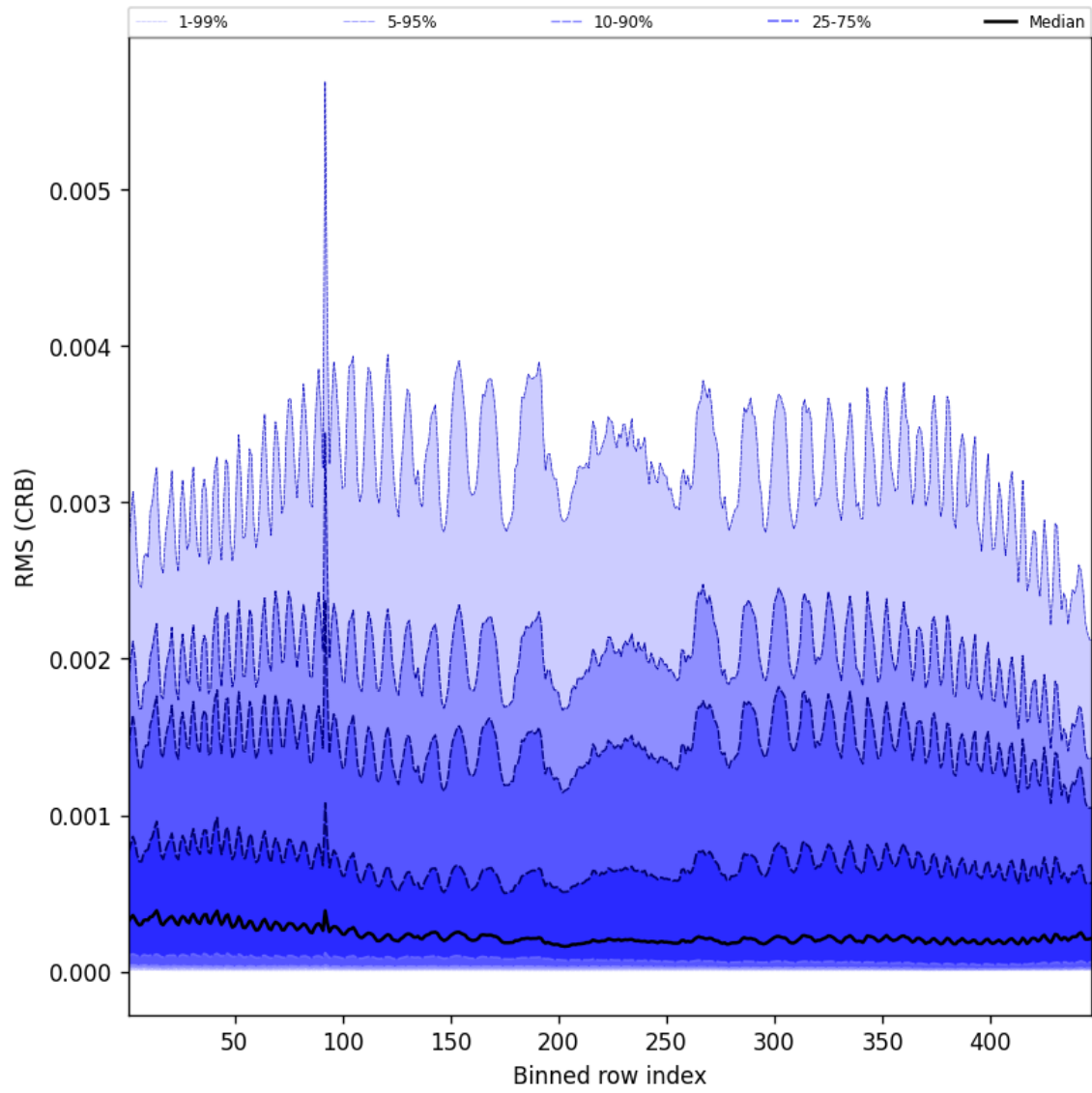
Figure 62: Along track statistics of “RMS (CRB)” for 2025-08-31 to 2025-09-01
