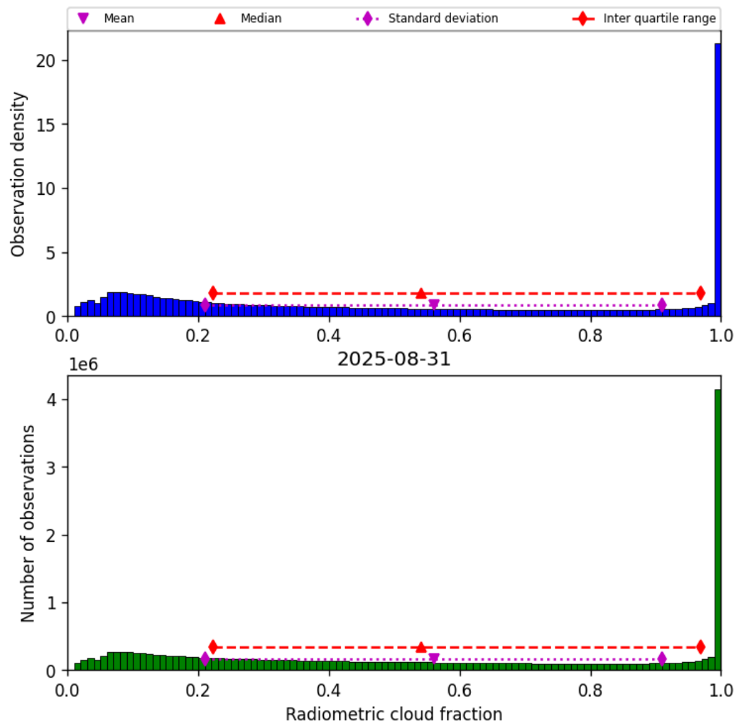
Figure 37: Histogram of “Radiometric cloud fraction” for 2025-08-31 to 2025-09-01
