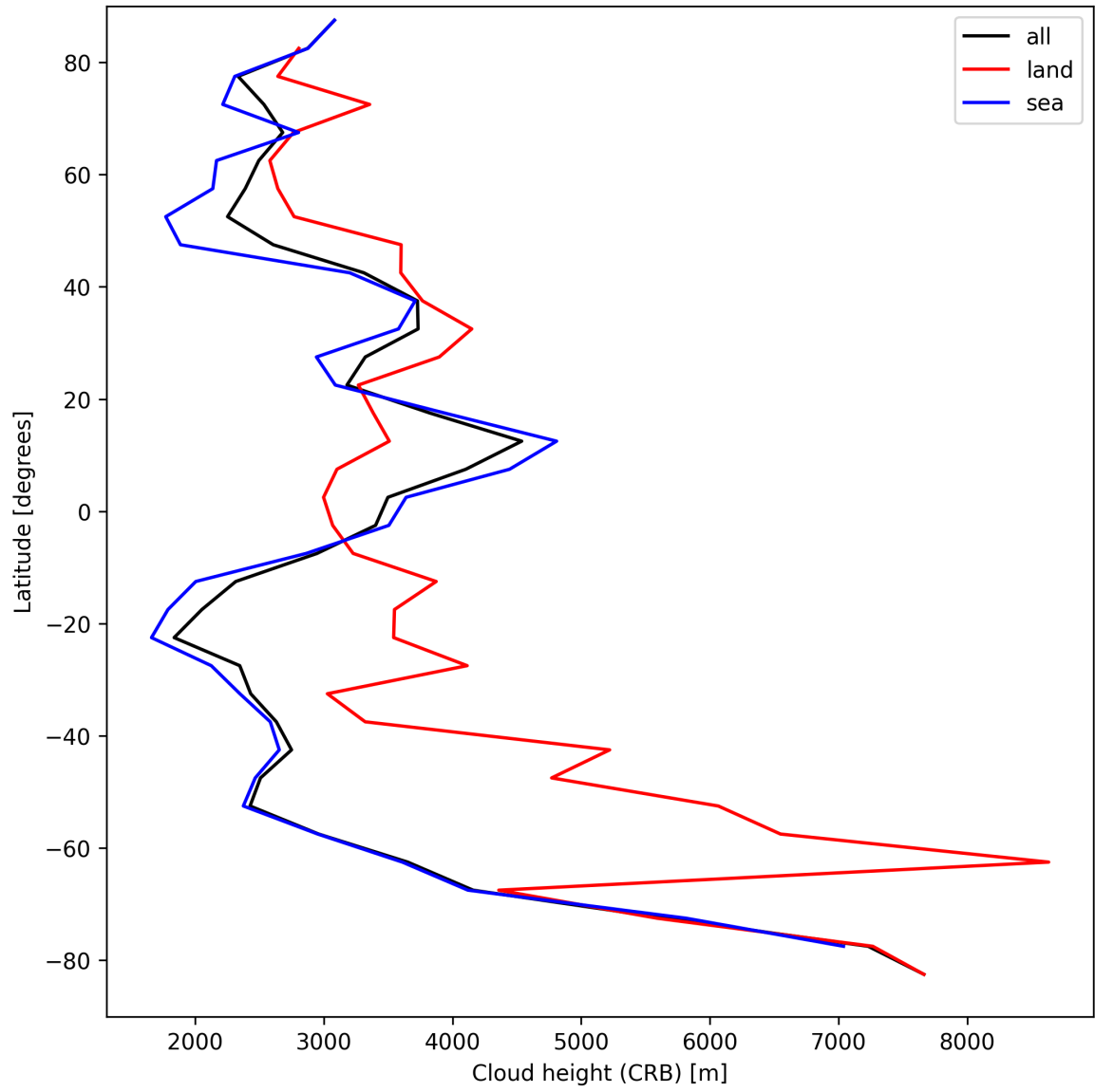
Figure 25: Zonal average of “Cloud height (CRB)” for 2025-08-31 to 2025-09-01.
