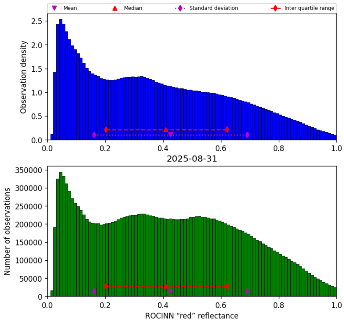
Figure 51: Histogram of “ROCINN “red” reflectance” for 2025-08-31 to 2025-09-01
