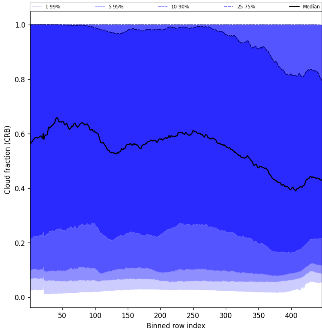
Figure 56: Along track statistics of “Cloud fraction (CRB)” for 2025-08-31 to 2025-09-01
