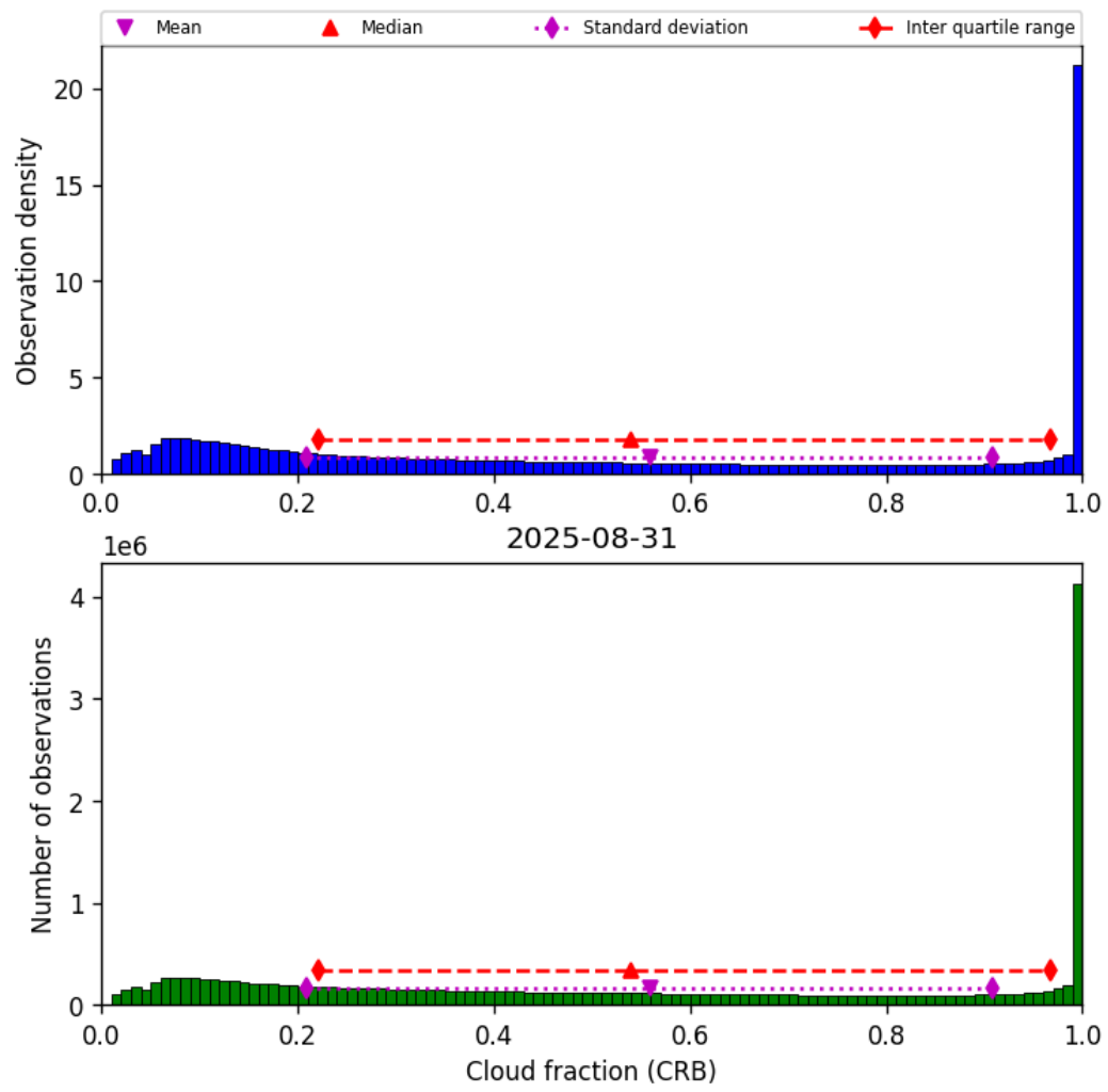
Figure 40: Histogram of “Cloud fraction (CRB)” for 2025-08-31 to 2025-09-01
