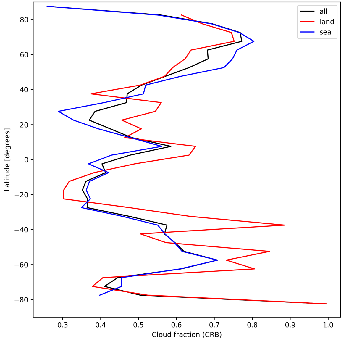
Figure 24: Zonal average of “Cloud fraction (CRB)” for 2025-08-31 to 2025-09-01.
