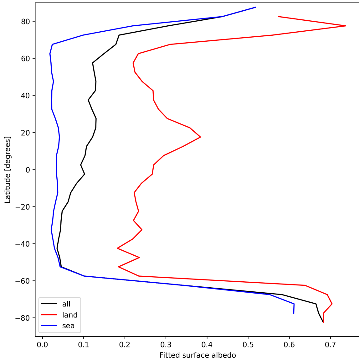
Figure 27: Zonal average of “Fitted surface albedo” for 2025-08-31 to 2025-09-01.
