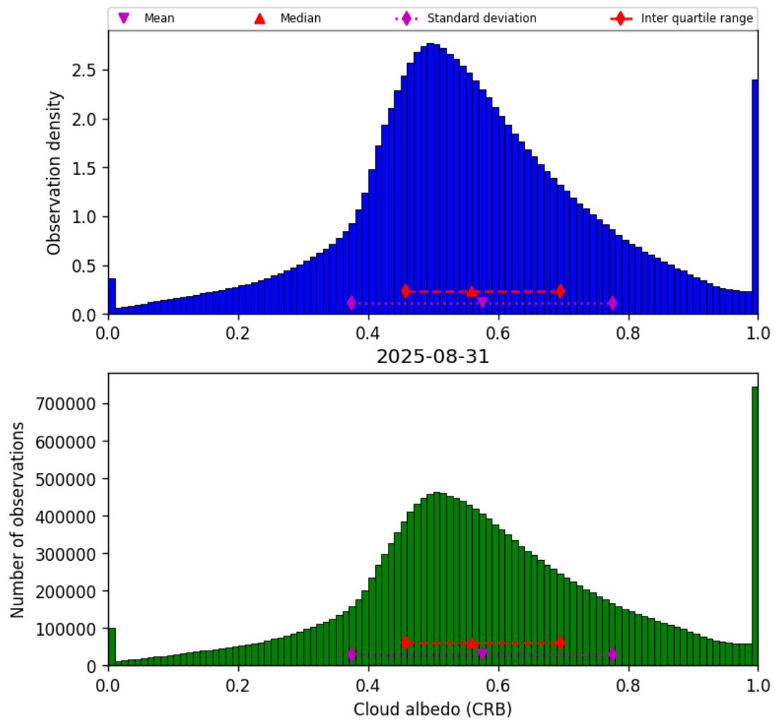
Figure 42: Histogram of “Cloud albedo (CRB)” for 2025-08-31 to 2025-09-01
