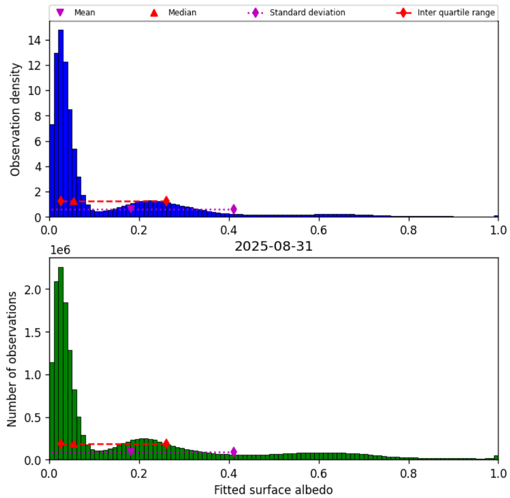
Figure 43: Histogram of “Fitted surface albedo” for 2025-08-31 to 2025-09-01
