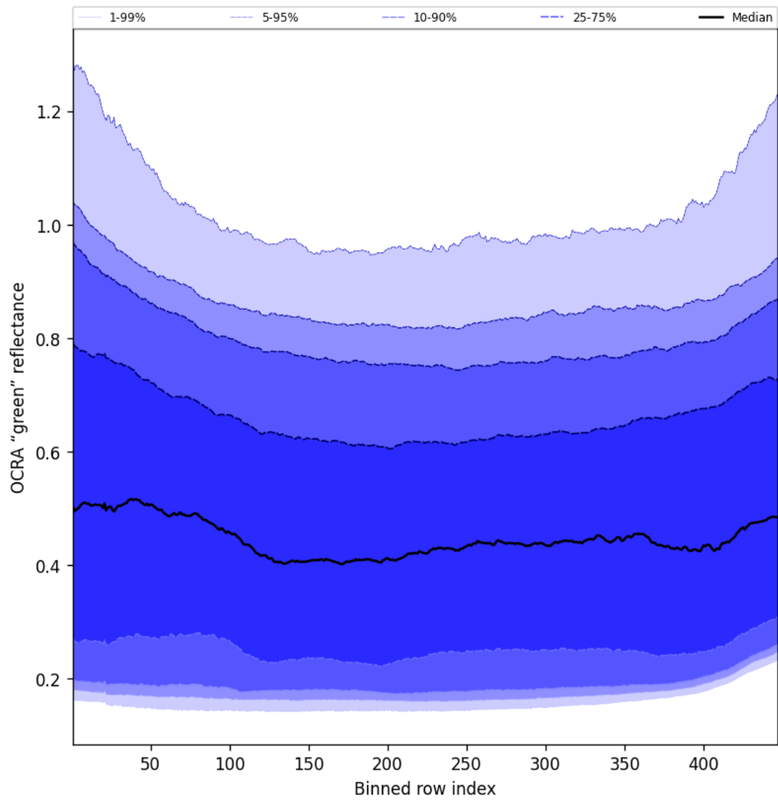
Figure 66: Along track statistics of “OCRA “green” reflectance” for 2025-08-31 to 2025-09-01
