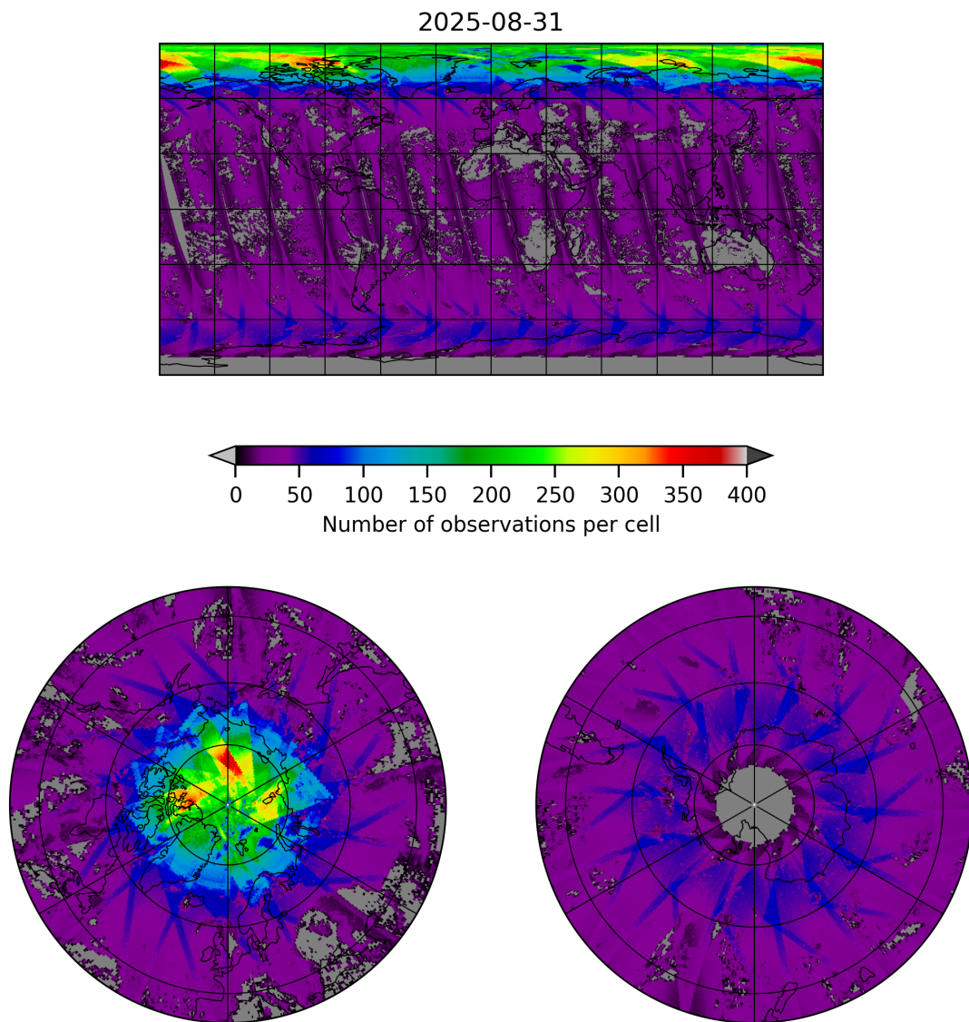
Figure 19: Map of the number of observations for 2025-08-31 to 2025-09-01
