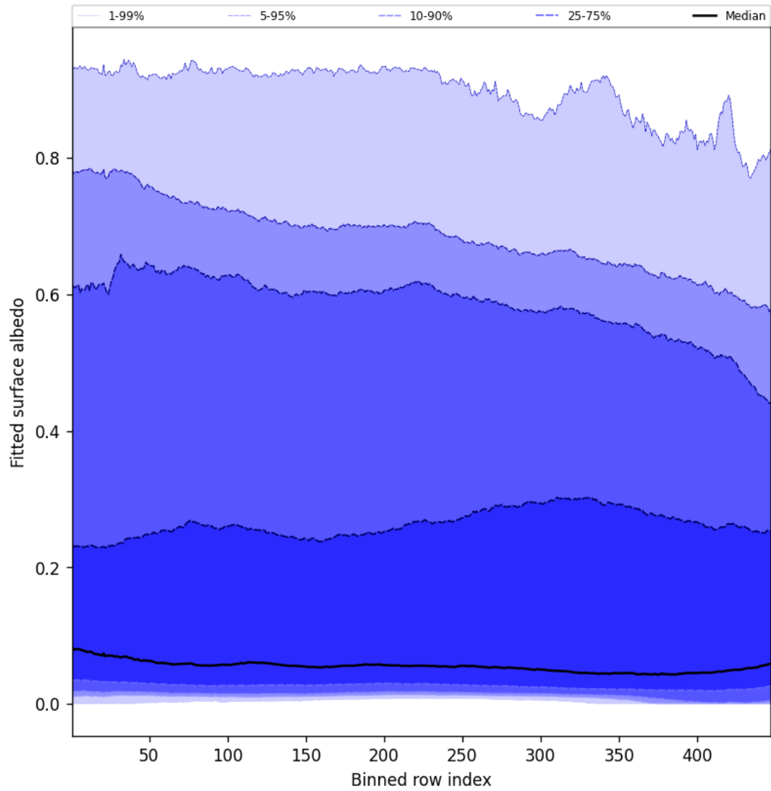
Figure 59: Along track statistics of “Fitted surface albedo” for 2025-08-31 to 2025-09-01
