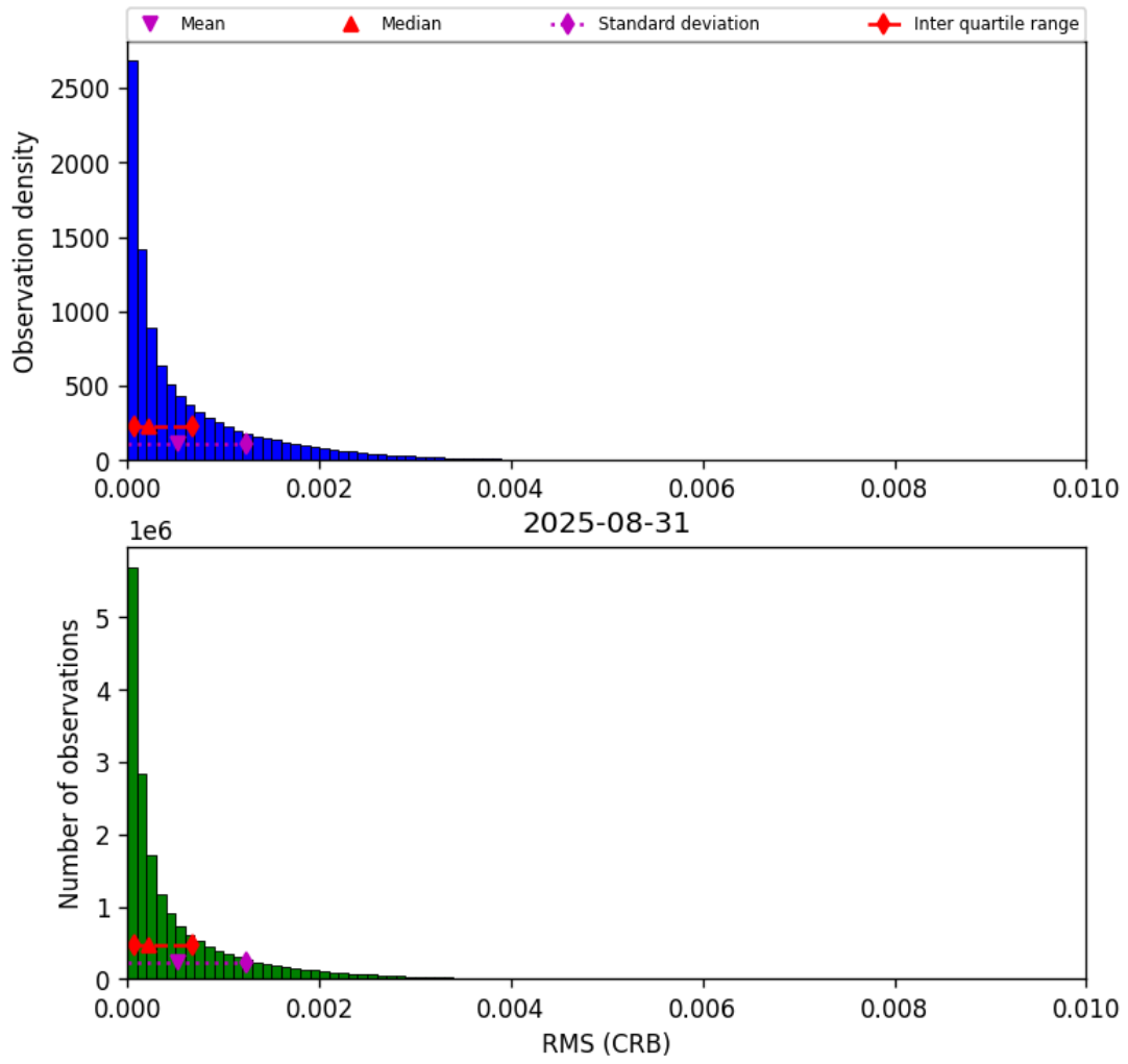
Figure 46: Histogram of “RMS (CRB)” for 2025-08-31 to 2025-09-01
