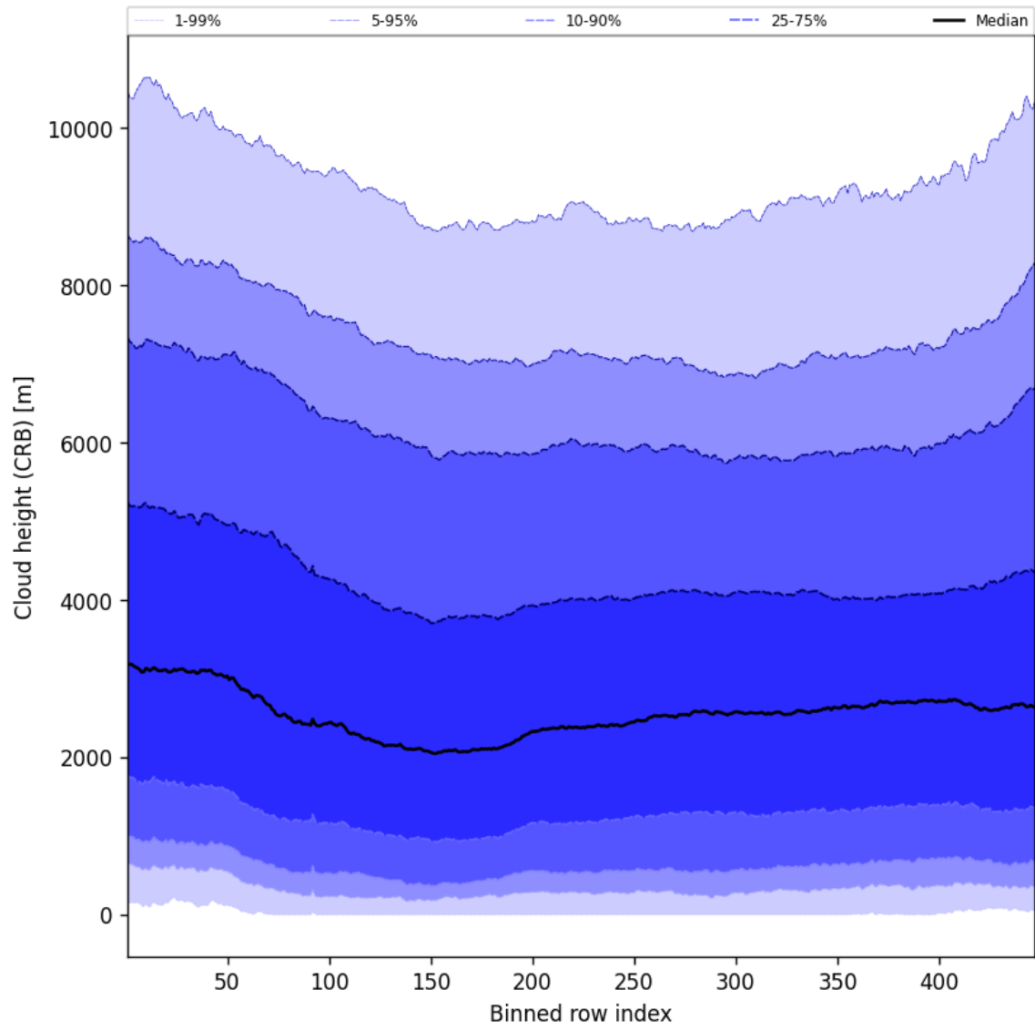
Figure 57: Along track statistics of “Cloud height (CRB)” for 2025-08-31 to 2025-09-01
