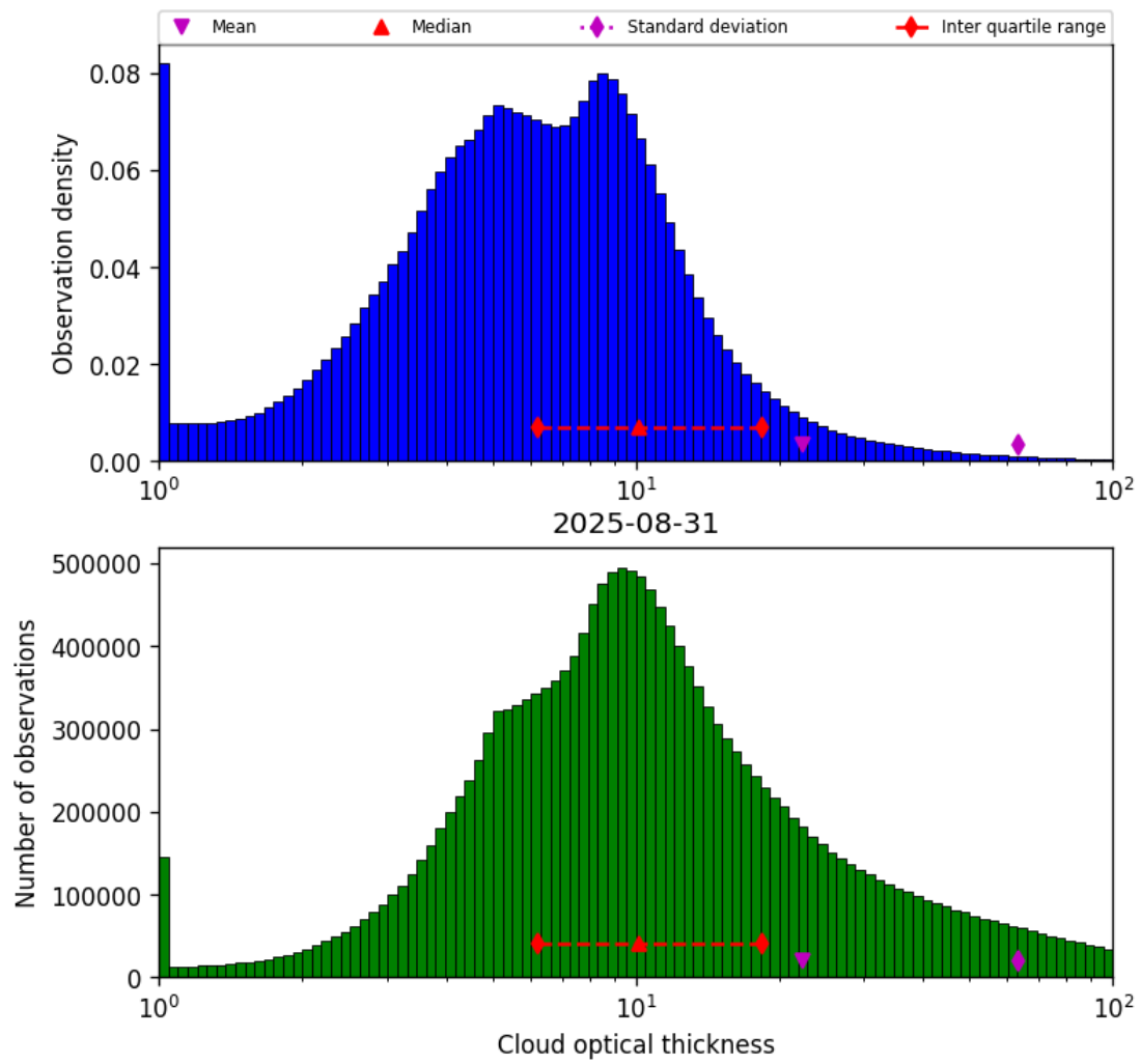
Figure 39: Histogram of “Cloud optical thickness” for 2025-08-31 to 2025-09-01
