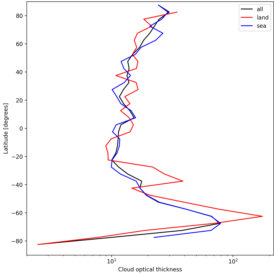
Figure 23: Zonal average of “Cloud optical thickness” for 2025-08-31 to 2025-09-01.
