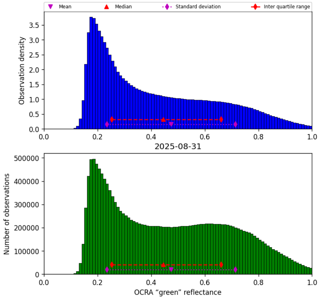
Figure 50: Histogram of “OCRA “green” reflectance” for 2025-08-31 to 2025-09-01
