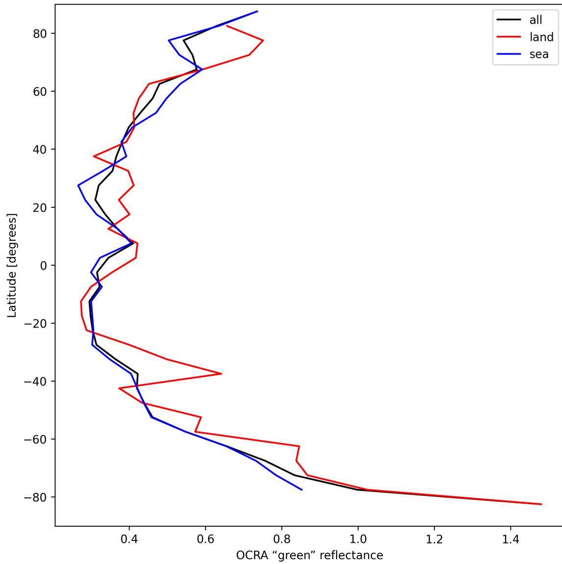
Figure 34: Zonal average of “OCRA “green” reflectance” for 2025-08-31 to 2025-09-01.
