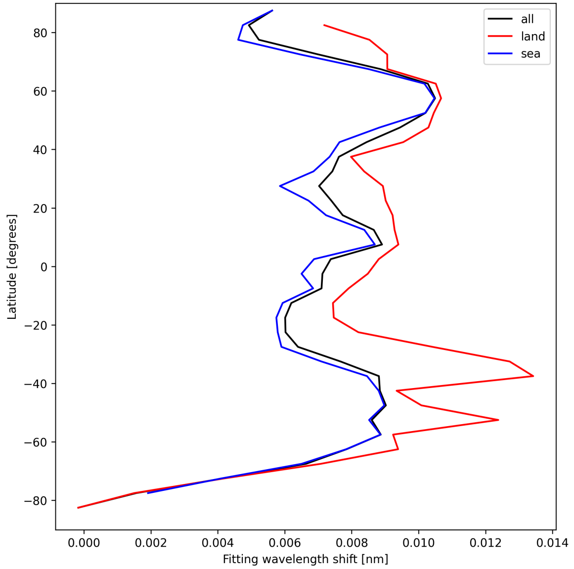
Figure 31: Zonal average of “Fitting wavelength shift” for 2025-08-31 to 2025-09-01.
