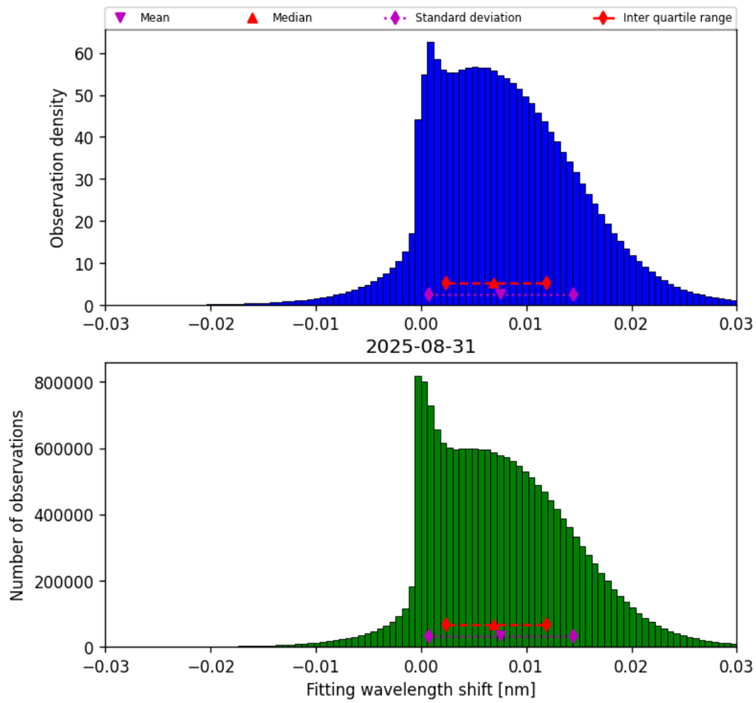
Figure 47: Histogram of “Fitting wavelength shift” for 2025-08-31 to 2025-09-01
