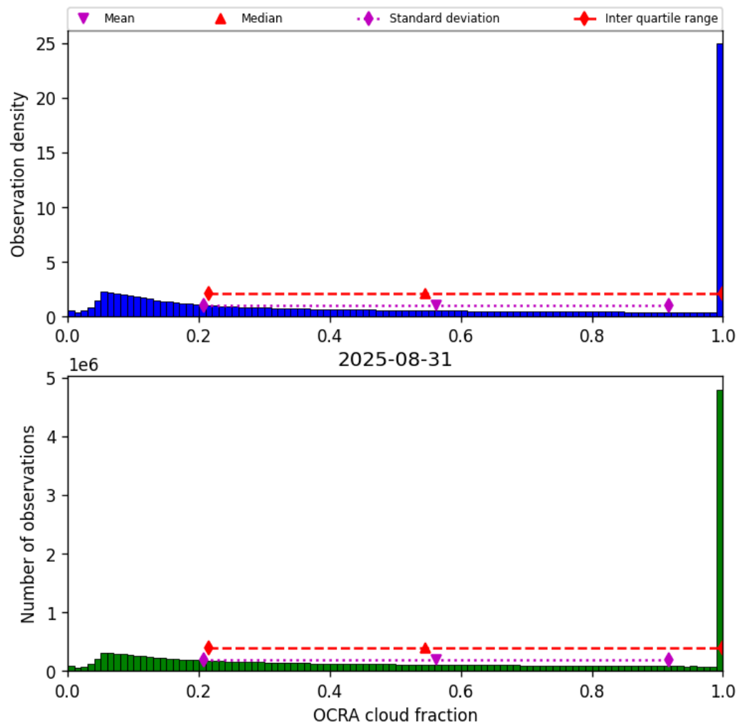
Figure 48: Histogram of “OCRA cloud fraction” for 2025-08-31 to 2025-09-01
