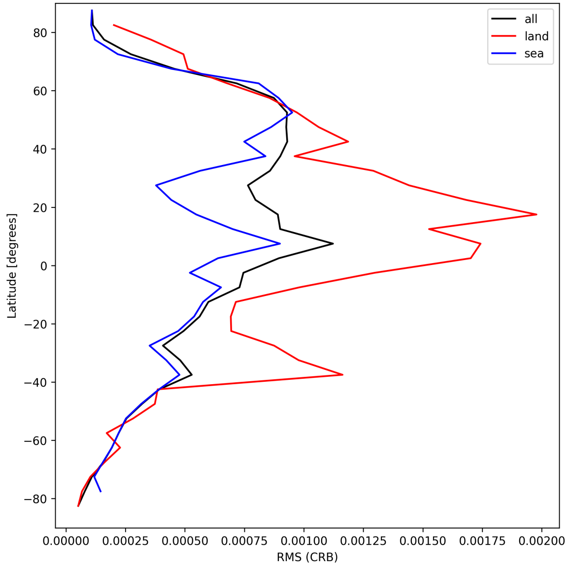
Figure 30: Zonal average of “RMS (CRB)” for 2025-08-31 to 2025-09-01.
