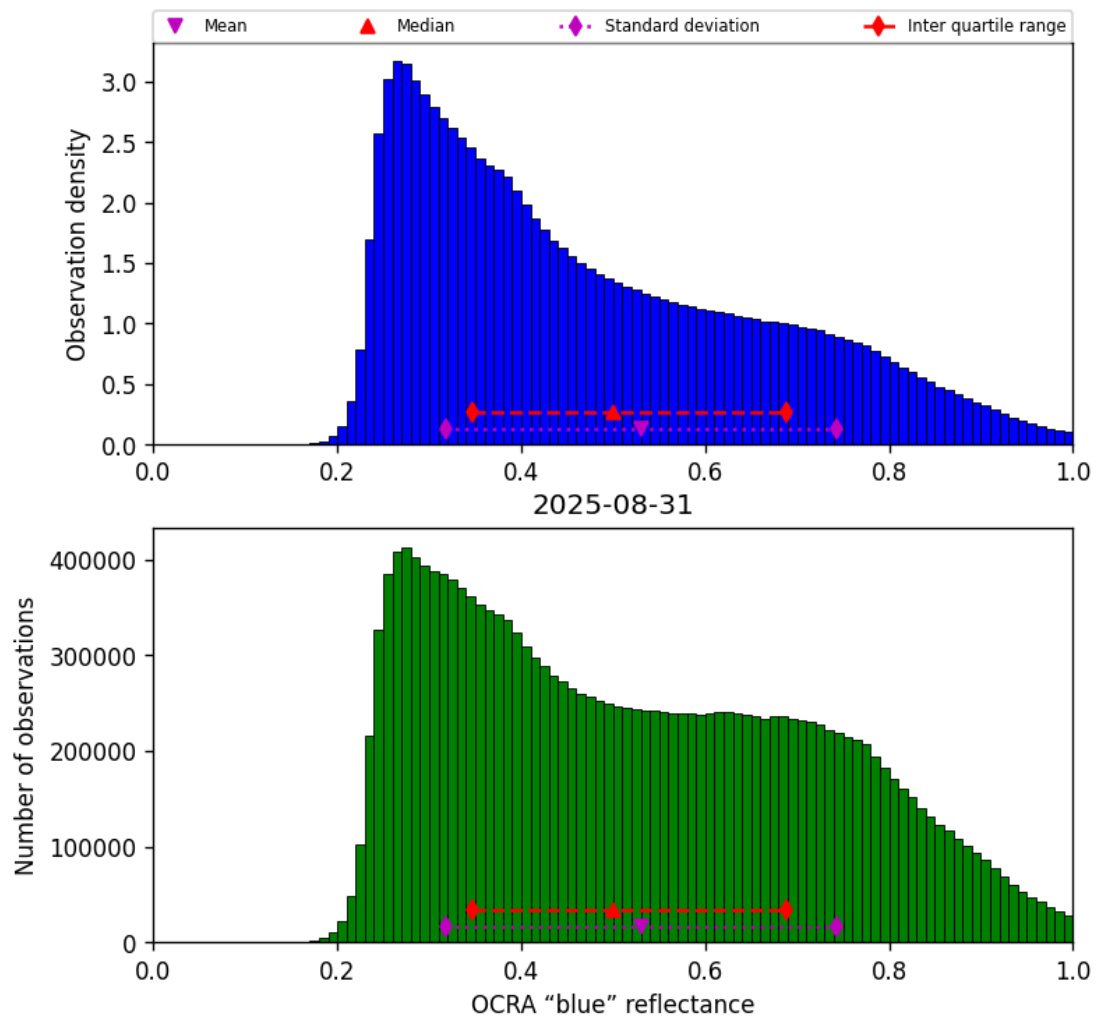
Figure 49: Histogram of “OCRA “blue” reflectance” for 2025-08-31 to 2025-09-01
