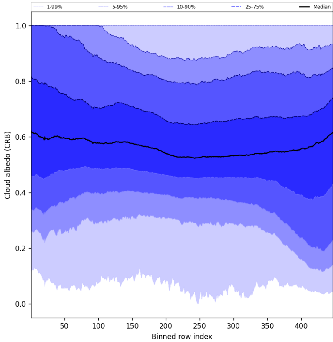
Figure 58: Along track statistics of “Cloud albedo (CRB)” for 2025-08-31 to 2025-09-01
