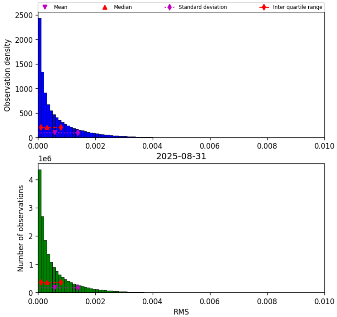
Figure 45: Histogram of “RMS” for 2025-08-31 to 2025-09-01
