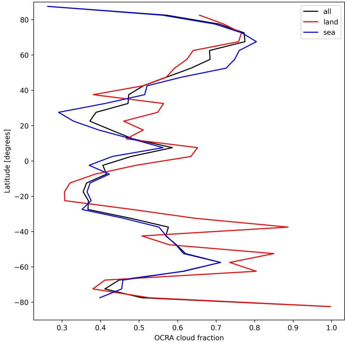
Figure 32: Zonal average of “OCRA cloud fraction” for 2025-08-31 to 2025-09-01.
