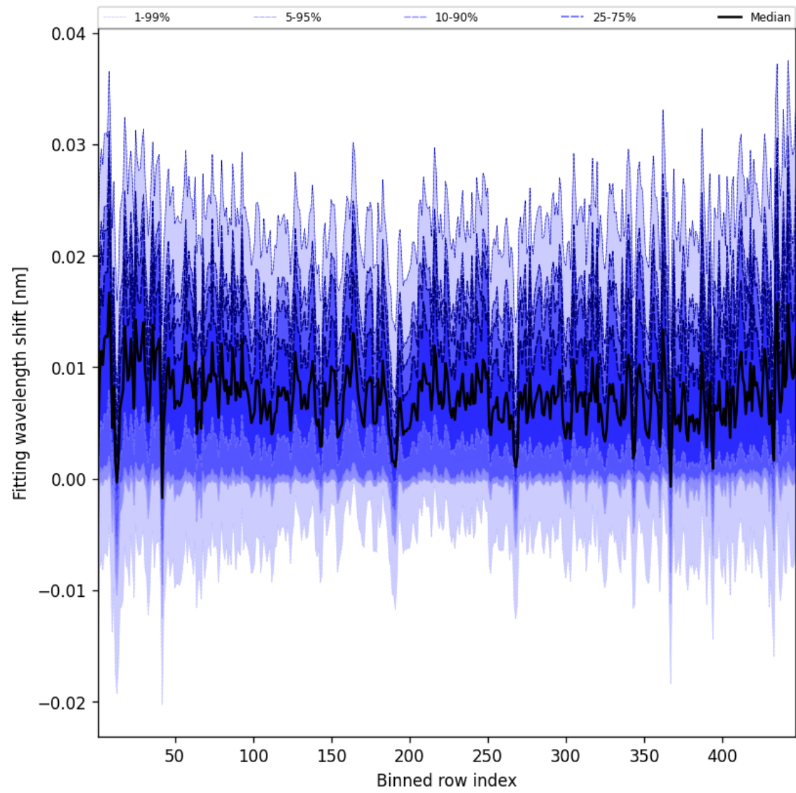
Figure 63: Along track statistics of “Fitting wavelength shift” for 2025-08-31 to 2025-09-01
