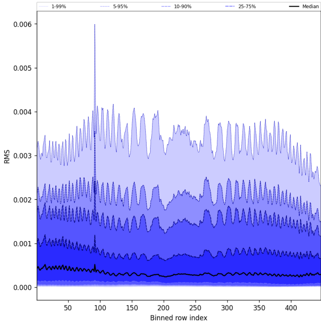
Figure 61: Along track statistics of “RMS” for 2025-08-31 to 2025-09-01
