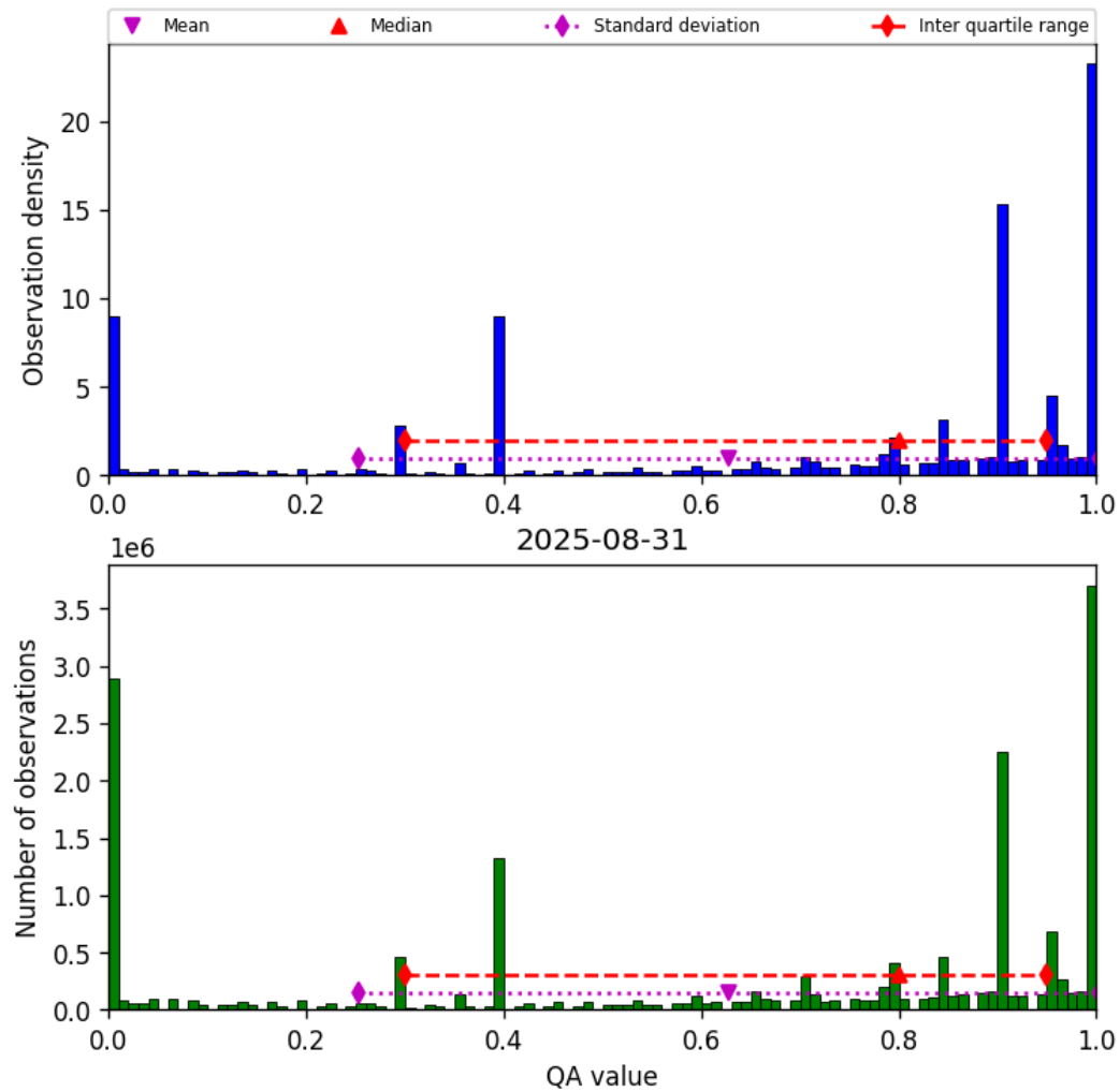
Figure 36: Histogram of “QA value” for 2025-08-31 to 2025-09-01
