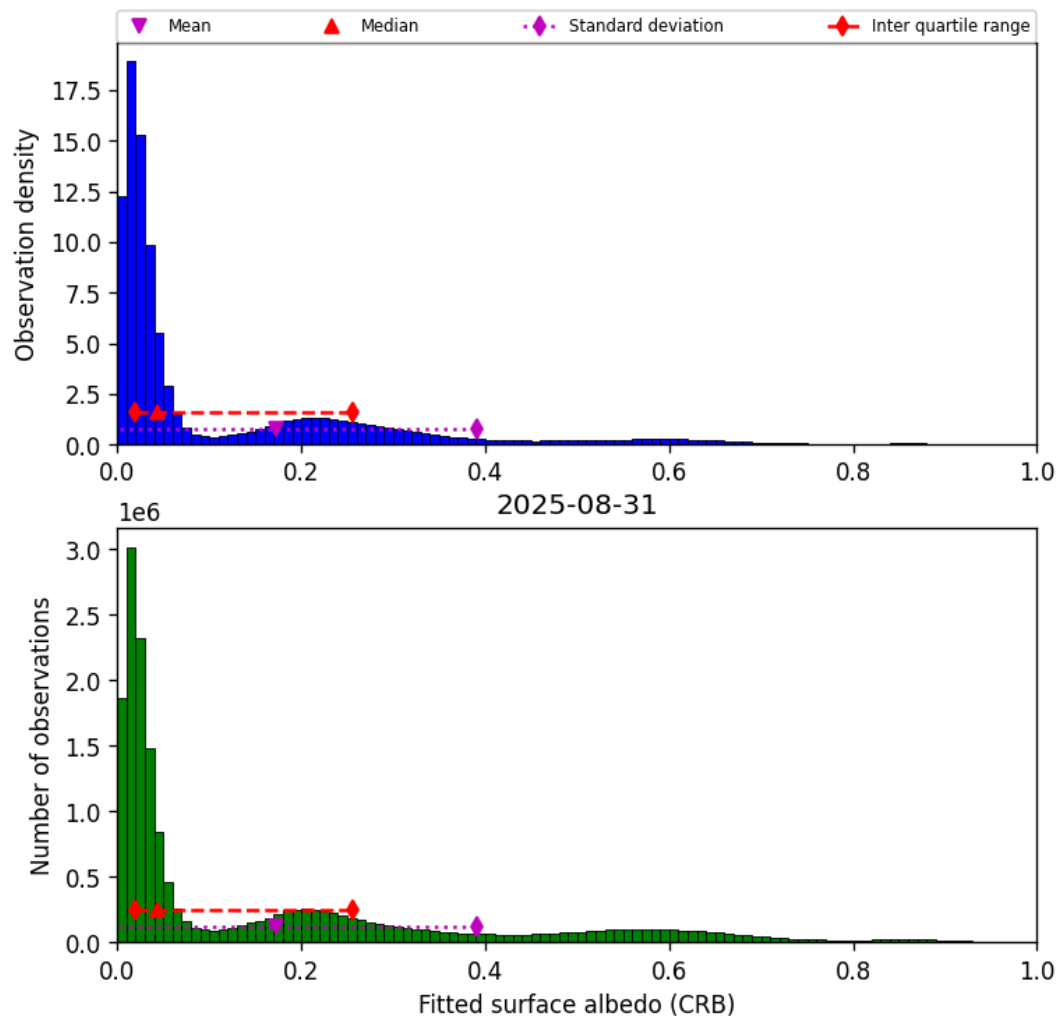
Figure 44: Histogram of “Fitted surface albedo (CRB)” for 2025-08-31 to 2025-09-01
