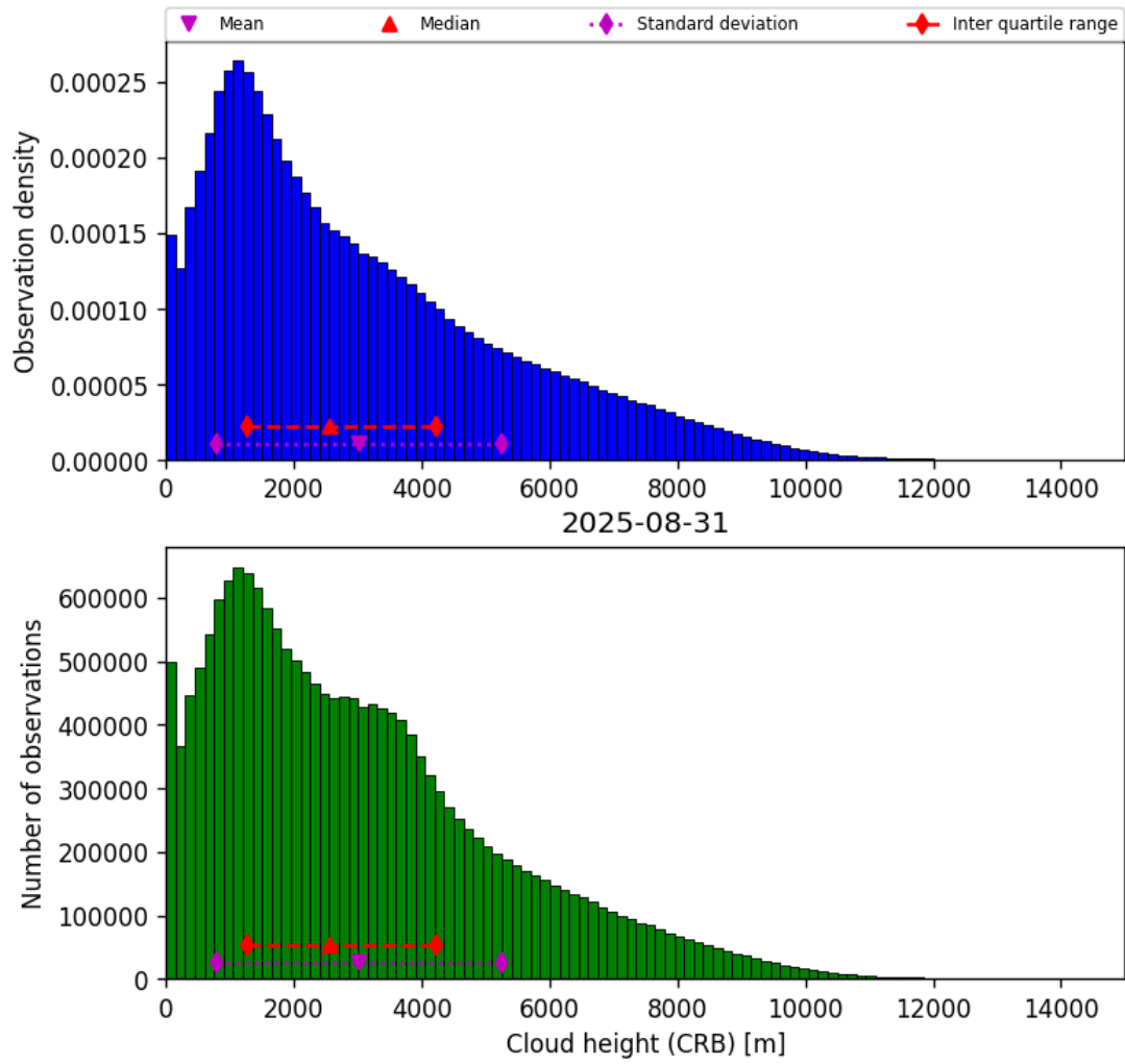
Figure 41: Histogram of “Cloud height (CRB)” for 2025-08-31 to 2025-09-01
