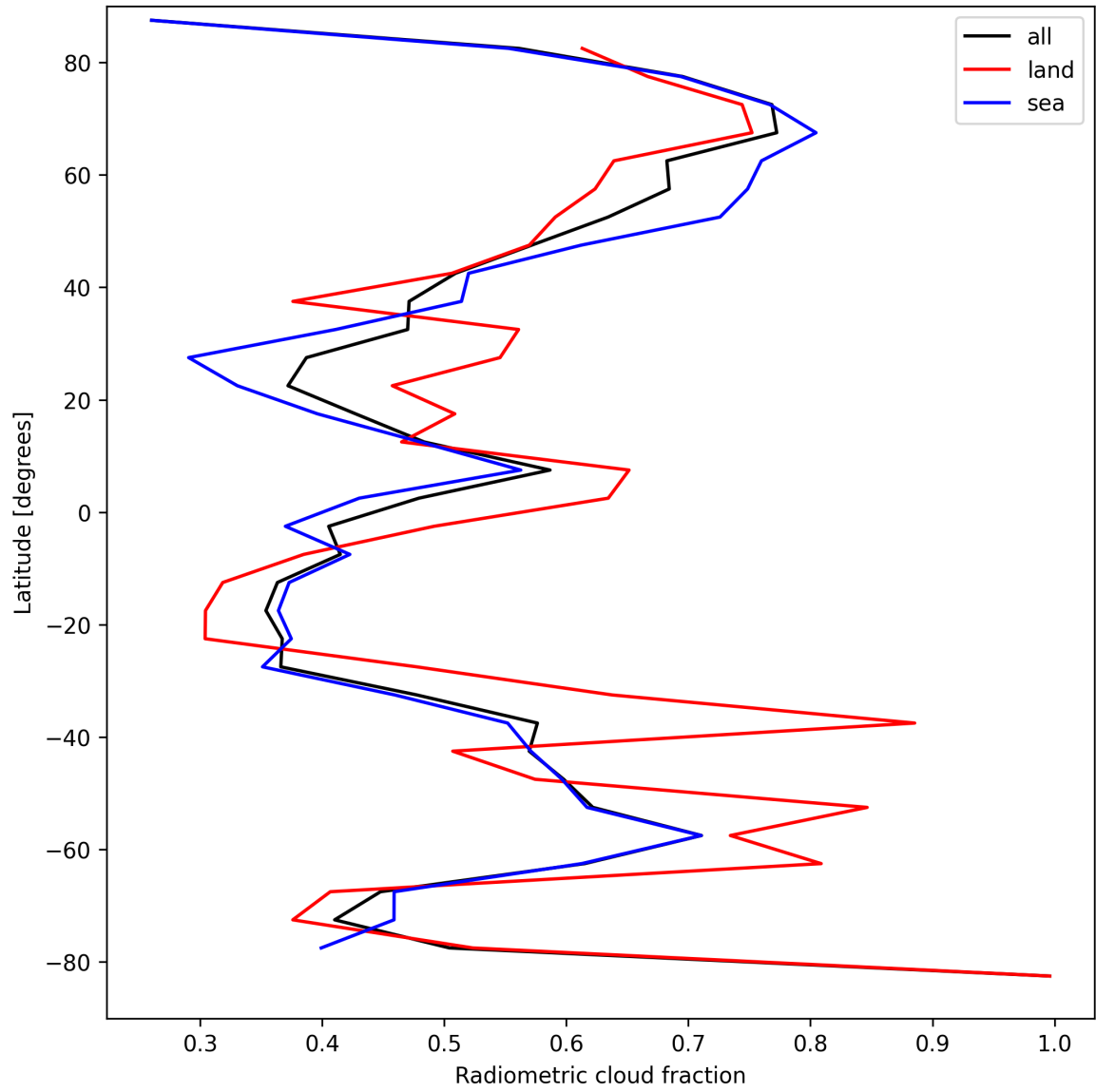
Figure 21: Zonal average of “Radiometric cloud fraction” for 2025-08-31 to 2025-09-01.
