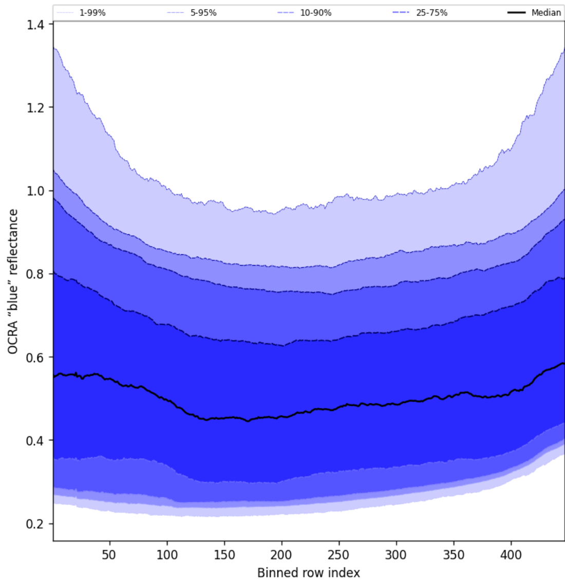
Figure 65: Along track statistics of “OCRA “blue” reflectance” for 2025-08-31 to 2025-09-01
