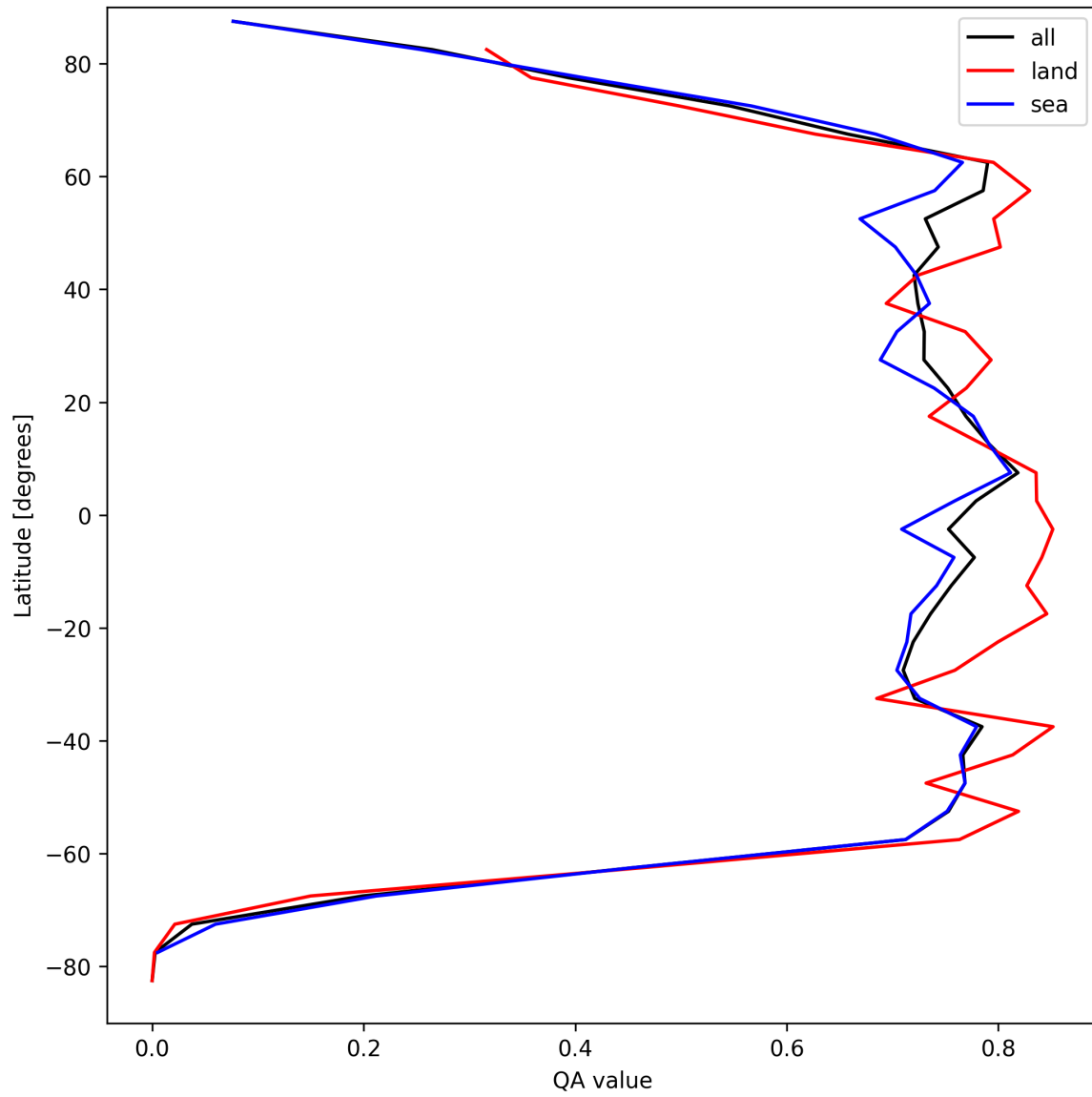
Figure 20: Zonal average of “QA value” for 2025-08-31 to 2025-09-01.
