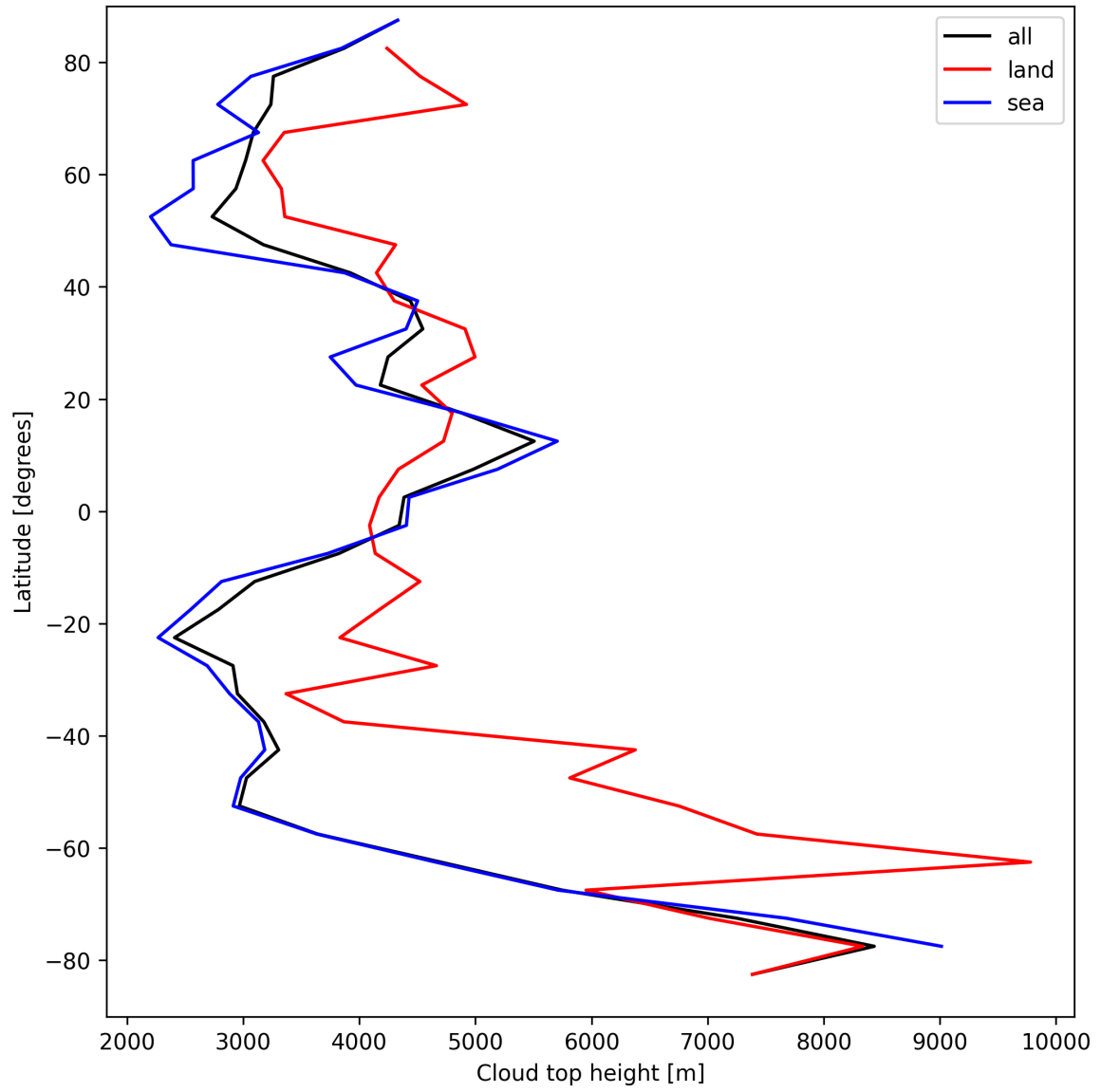
Figure 22: Zonal average of “Cloud top height” for 2025-08-31 to 2025-09-01.
