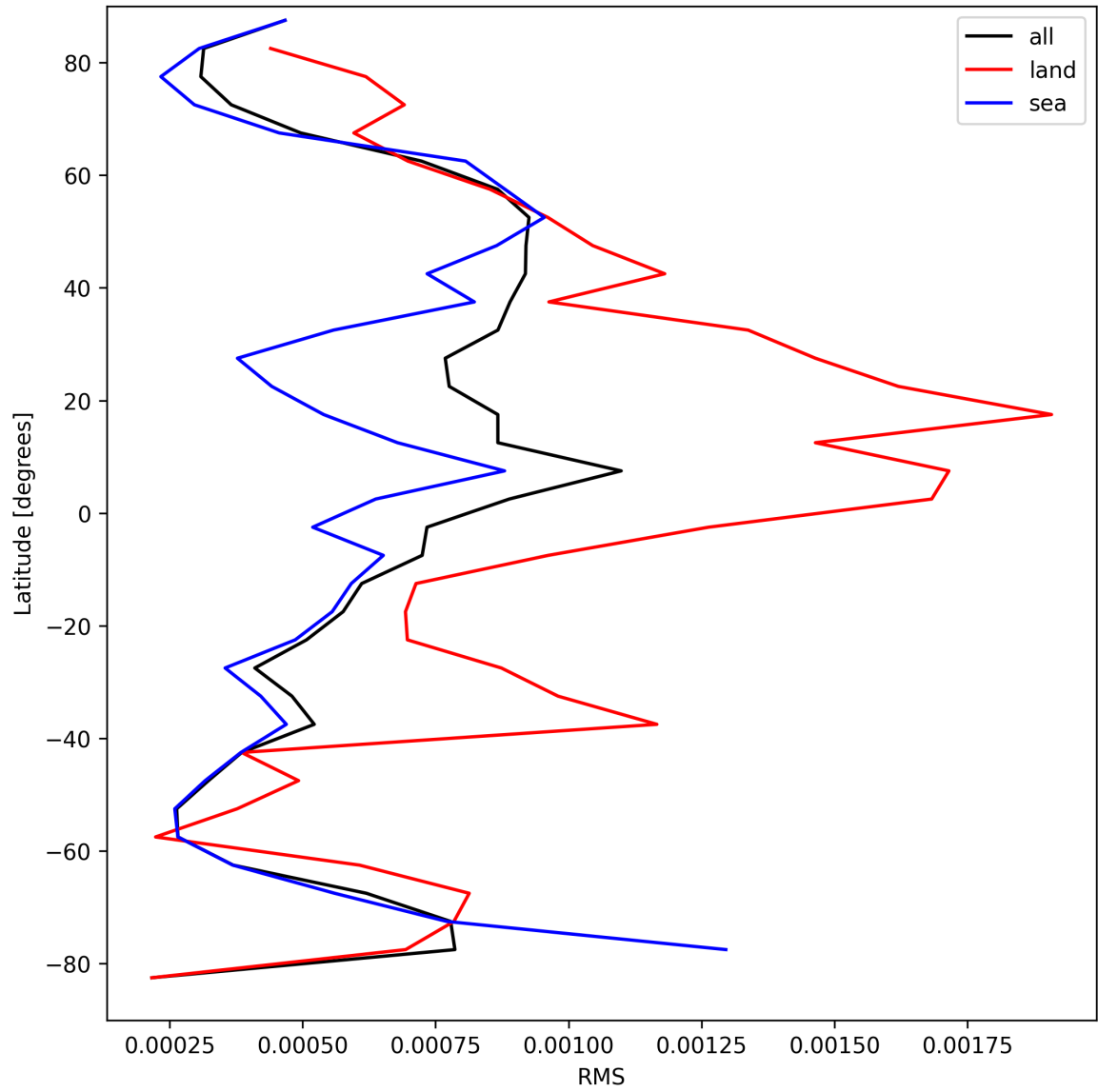
Figure 29: Zonal average of “RMS” for 2025-08-31 to 2025-09-01.
