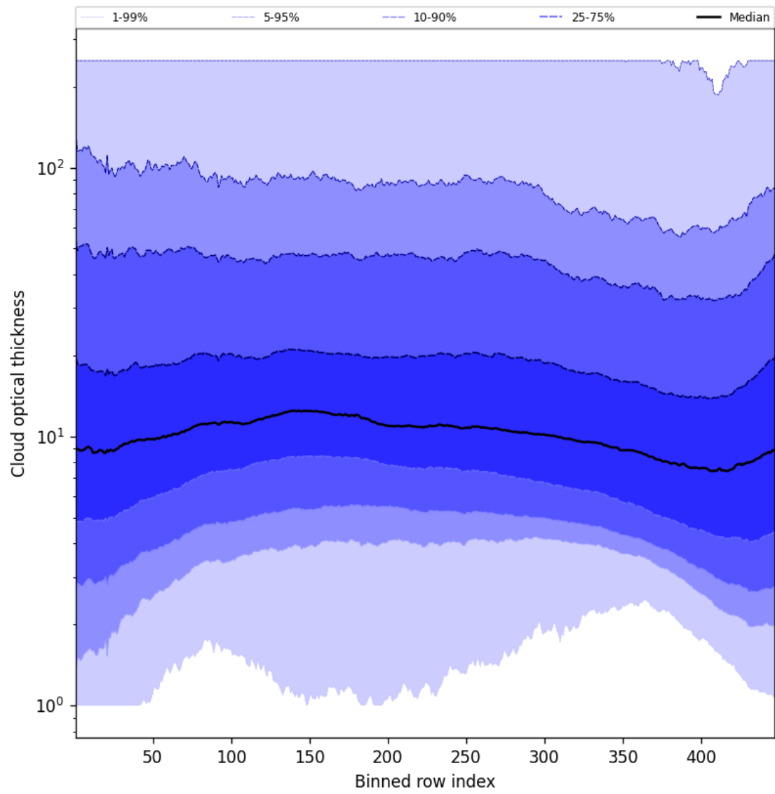
Figure 55: Along track statistics of “Cloud optical thickness” for 2025-08-31 to 2025-09-01
