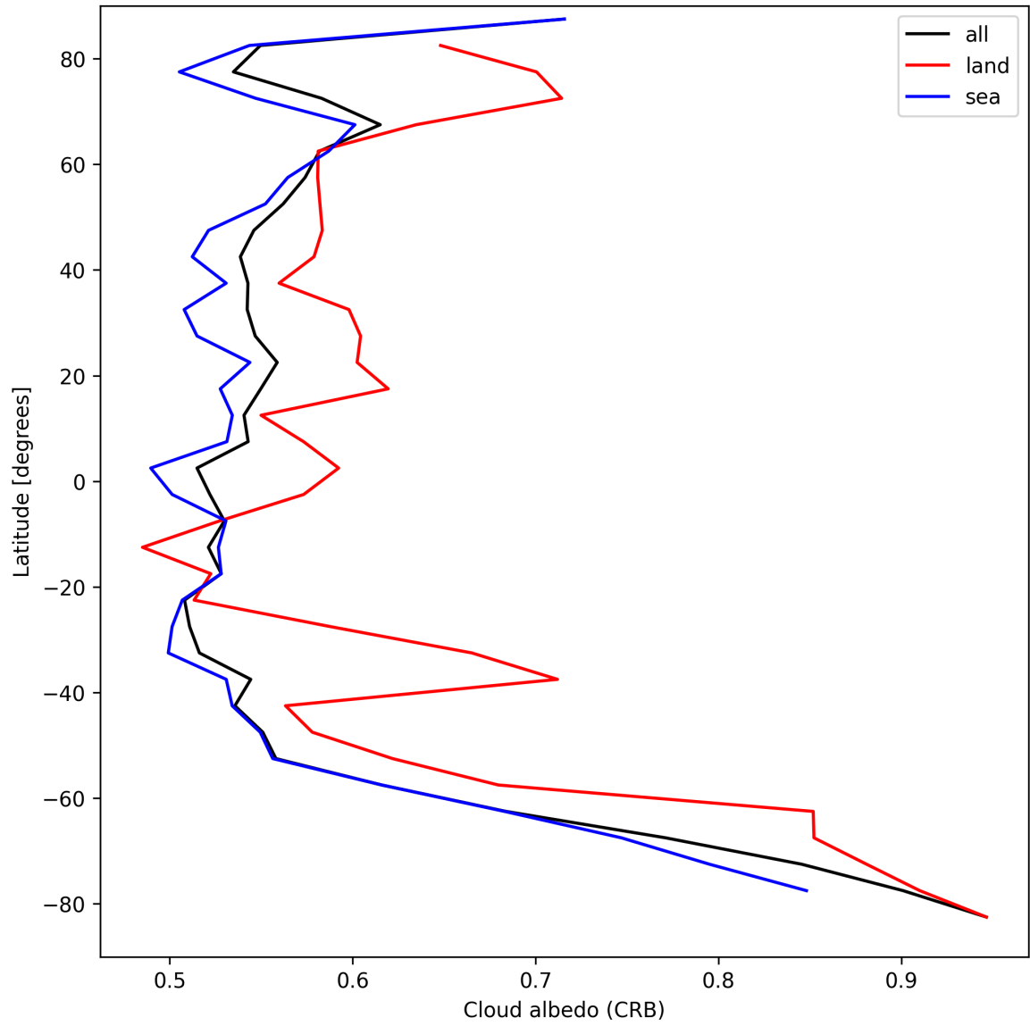
Figure 26: Zonal average of “Cloud albedo (CRB)” for 2025-08-31 to 2025-09-01.
