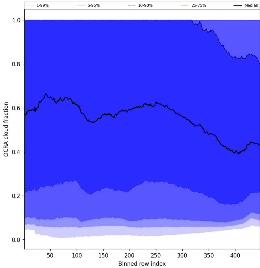
Figure 64: Along track statistics of “OCRA cloud fraction” for 2025-08-31 to 2025-09-01
