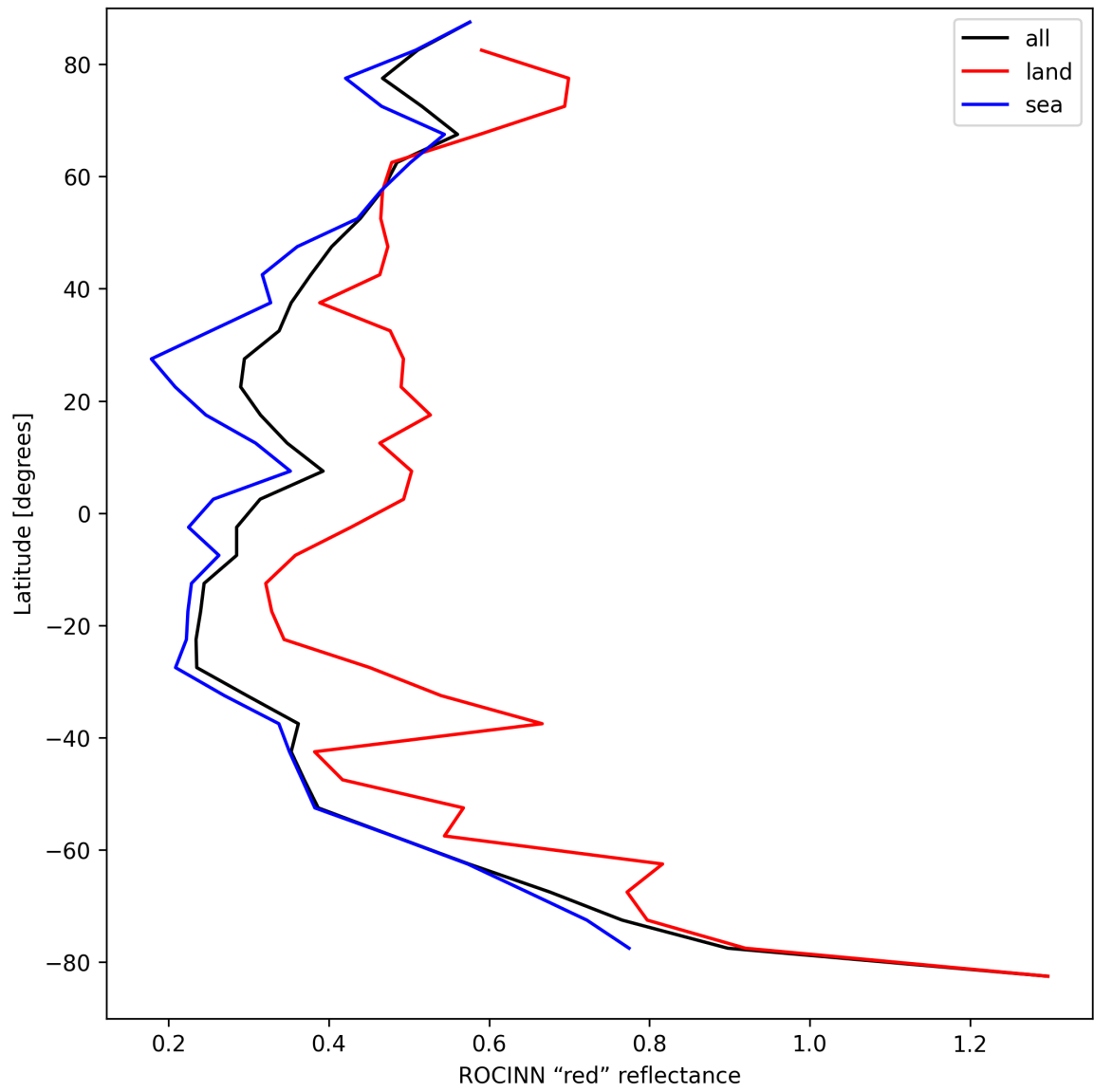
Figure 35: Zonal average of “ROCINN “red” reflectance” for 2025-08-31 to 2025-09-01.
