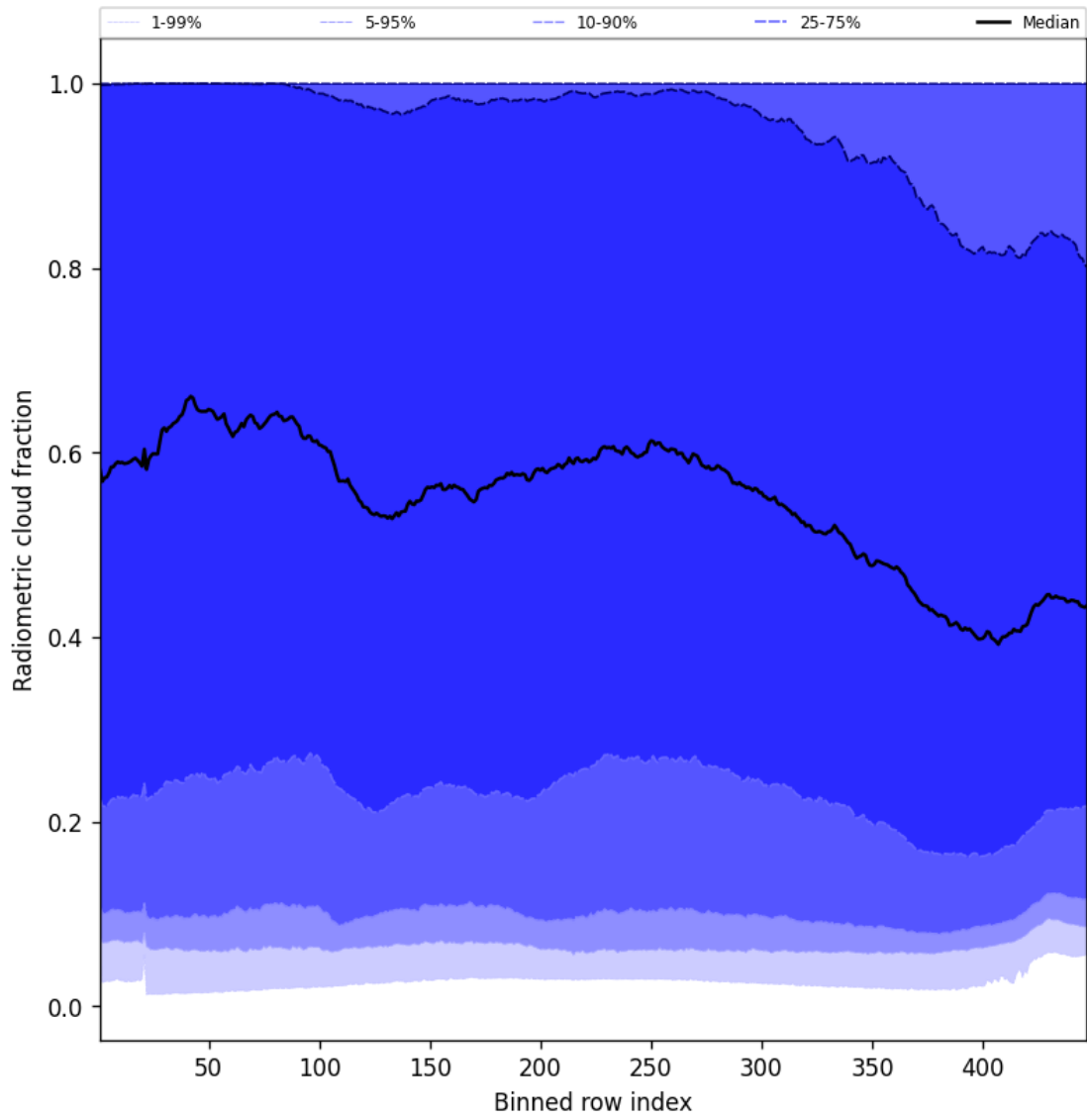
Figure 53: Along track statistics of “Radiometric cloud fraction” for 2025-08-31 to 2025-09-01
