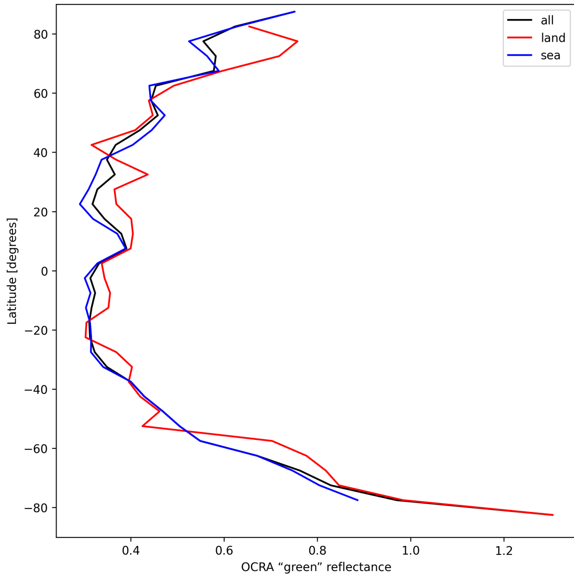
Figure 34: Zonal average of “OCRA “green” reflectance” for 2025-09-02 to 2025-09-02.
