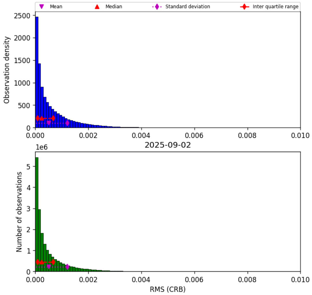
Figure 46: Histogram of “RMS (CRB)” for 2025-09-02 to 2025-09-02
