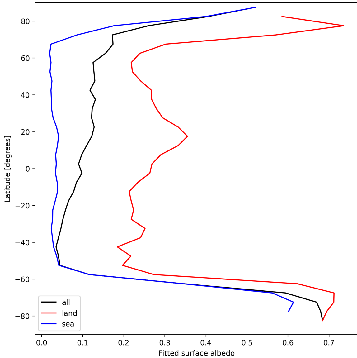
Figure 27: Zonal average of “Fitted surface albedo” for 2025-09-02 to 2025-09-02.
