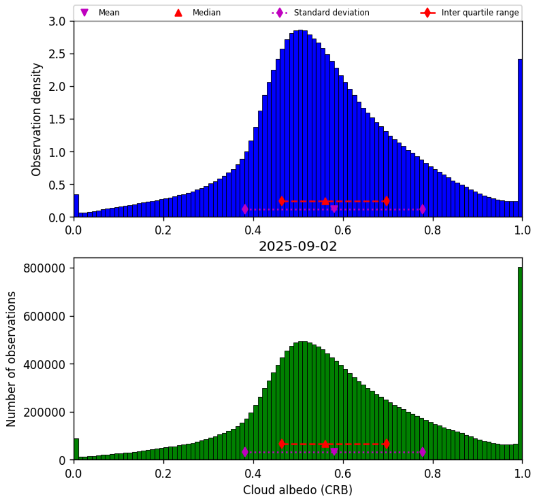
Figure 42: Histogram of “Cloud albedo (CRB)” for 2025-09-02 to 2025-09-02
