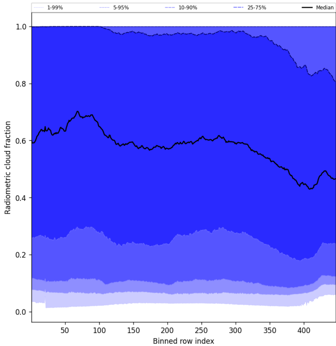
Figure 53: Along track statistics of “Radiometric cloud fraction” for 2025-09-02 to 2025-09-02
