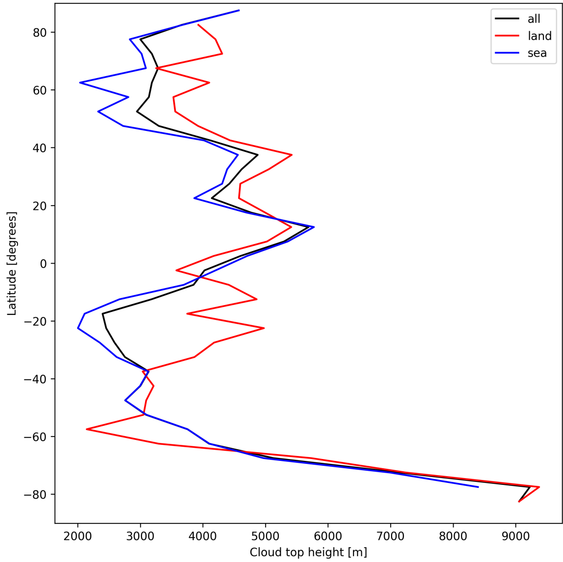
Figure 22: Zonal average of “Cloud top height” for 2025-09-02 to 2025-09-02.
