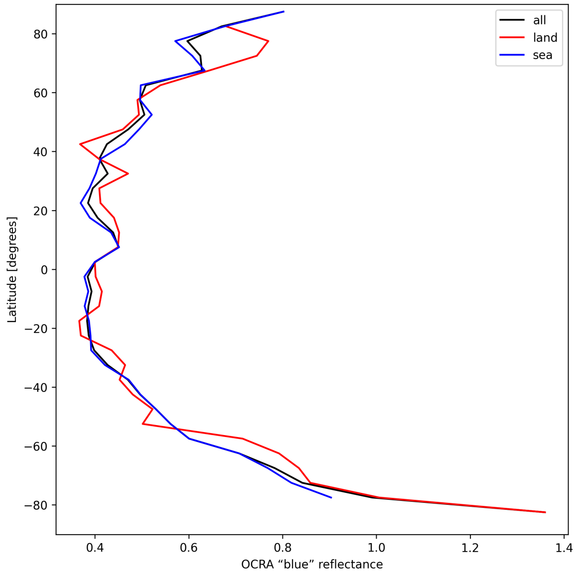
Figure 33: Zonal average of “OCRA “blue” reflectance” for 2025-09-02 to 2025-09-02.
