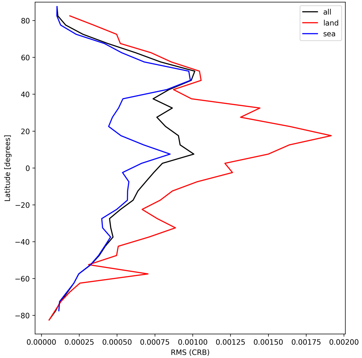
Figure 30: Zonal average of “RMS (CRB)” for 2025-09-02 to 2025-09-02.
