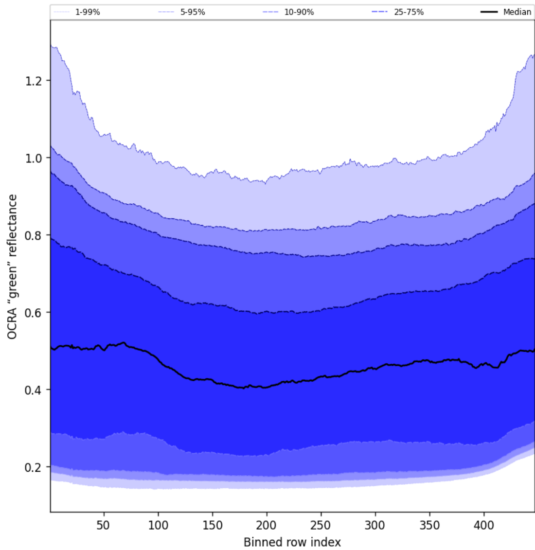
Figure 66: Along track statistics of “OCRA “green” reflectance” for 2025-09-02 to 2025-09-02
