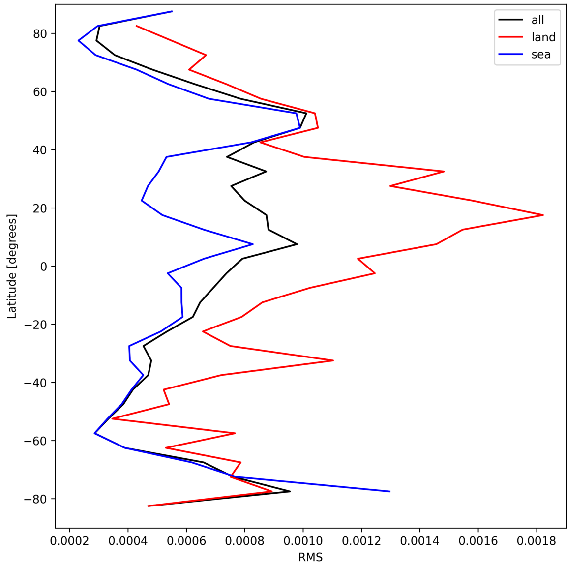
Figure 29: Zonal average of “RMS” for 2025-09-02 to 2025-09-02.
