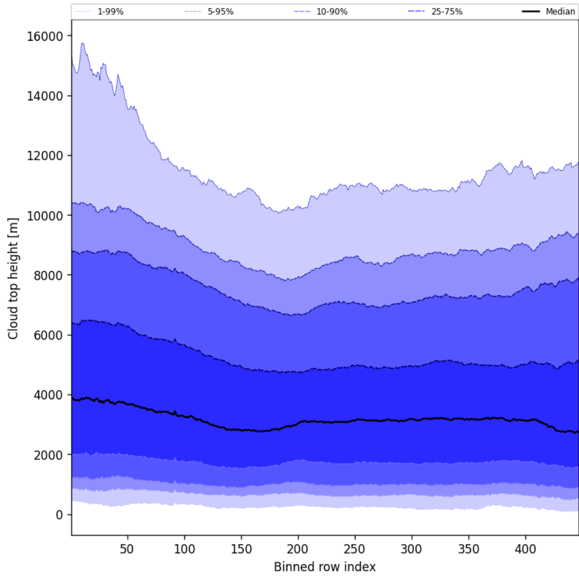
Figure 54: Along track statistics of “Cloud top height” for 2025-09-02 to 2025-09-02
