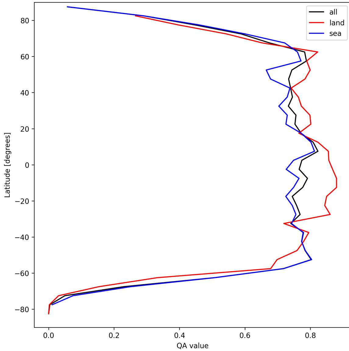
Figure 20: Zonal average of “QA value” for 2025-09-02 to 2025-09-02.
