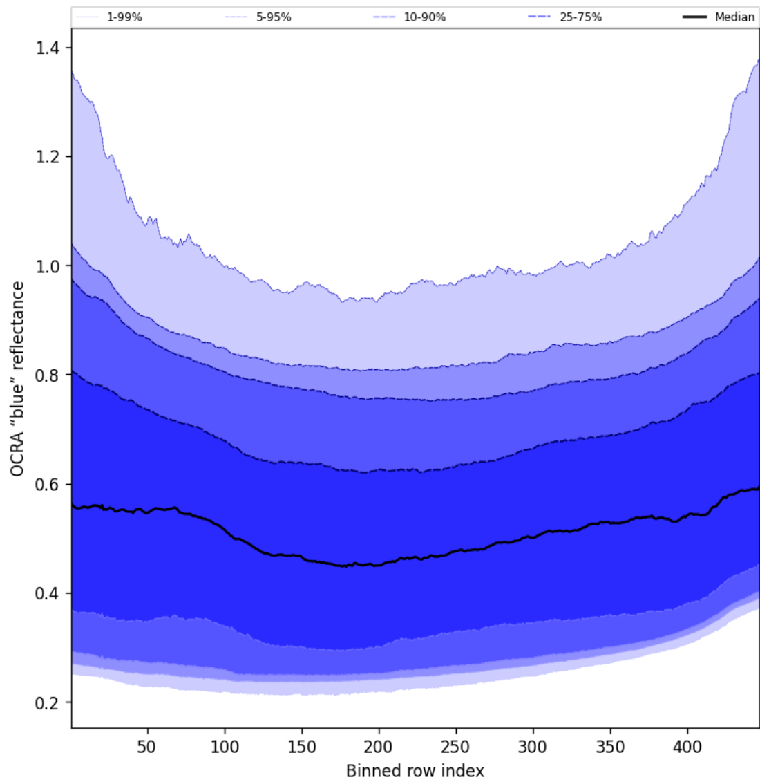
Figure 65: Along track statistics of “OCRA “blue” reflectance” for 2025-09-02 to 2025-09-02
