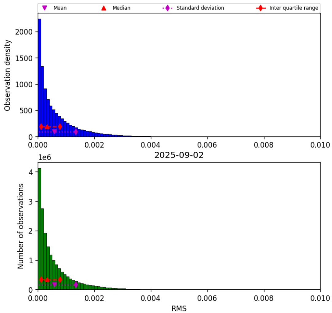
Figure 45: Histogram of “RMS” for 2025-09-02 to 2025-09-02
