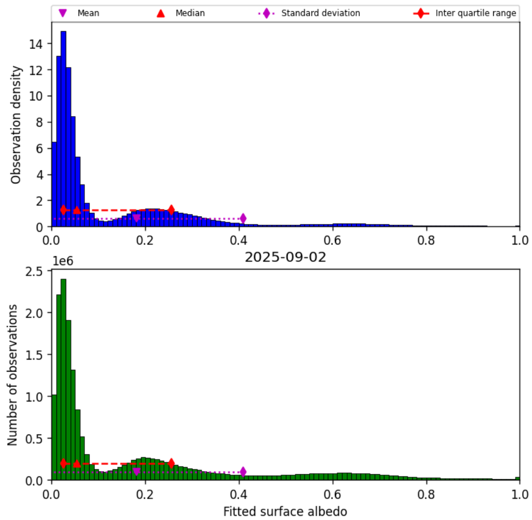
Figure 43: Histogram of “Fitted surface albedo” for 2025-09-02 to 2025-09-02
