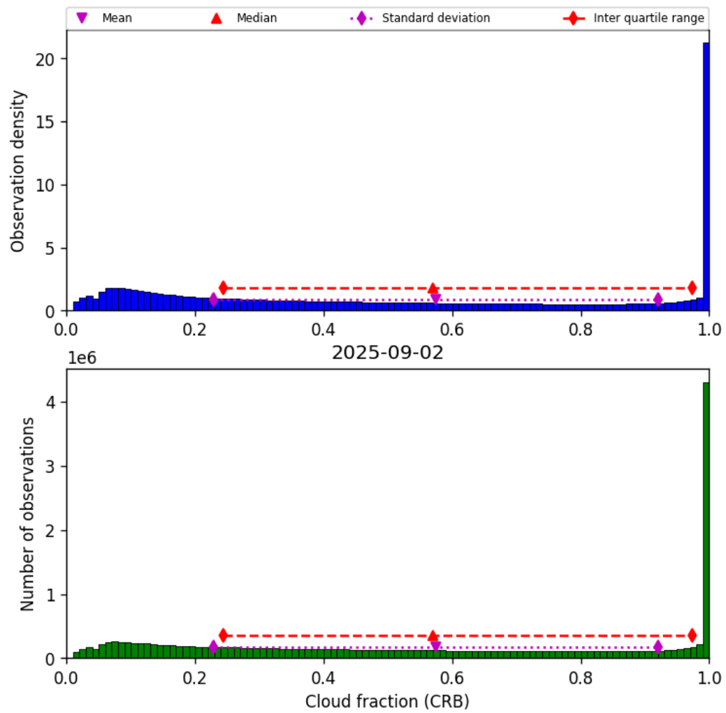
Figure 40: Histogram of “Cloud fraction (CRB)” for 2025-09-02 to 2025-09-02
