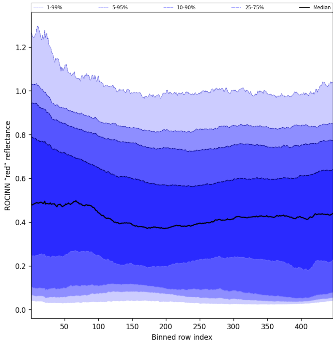
Figure 67: Along track statistics of “ROCINN “red” reflectance” for 2025-09-02 to 2025-09-02
