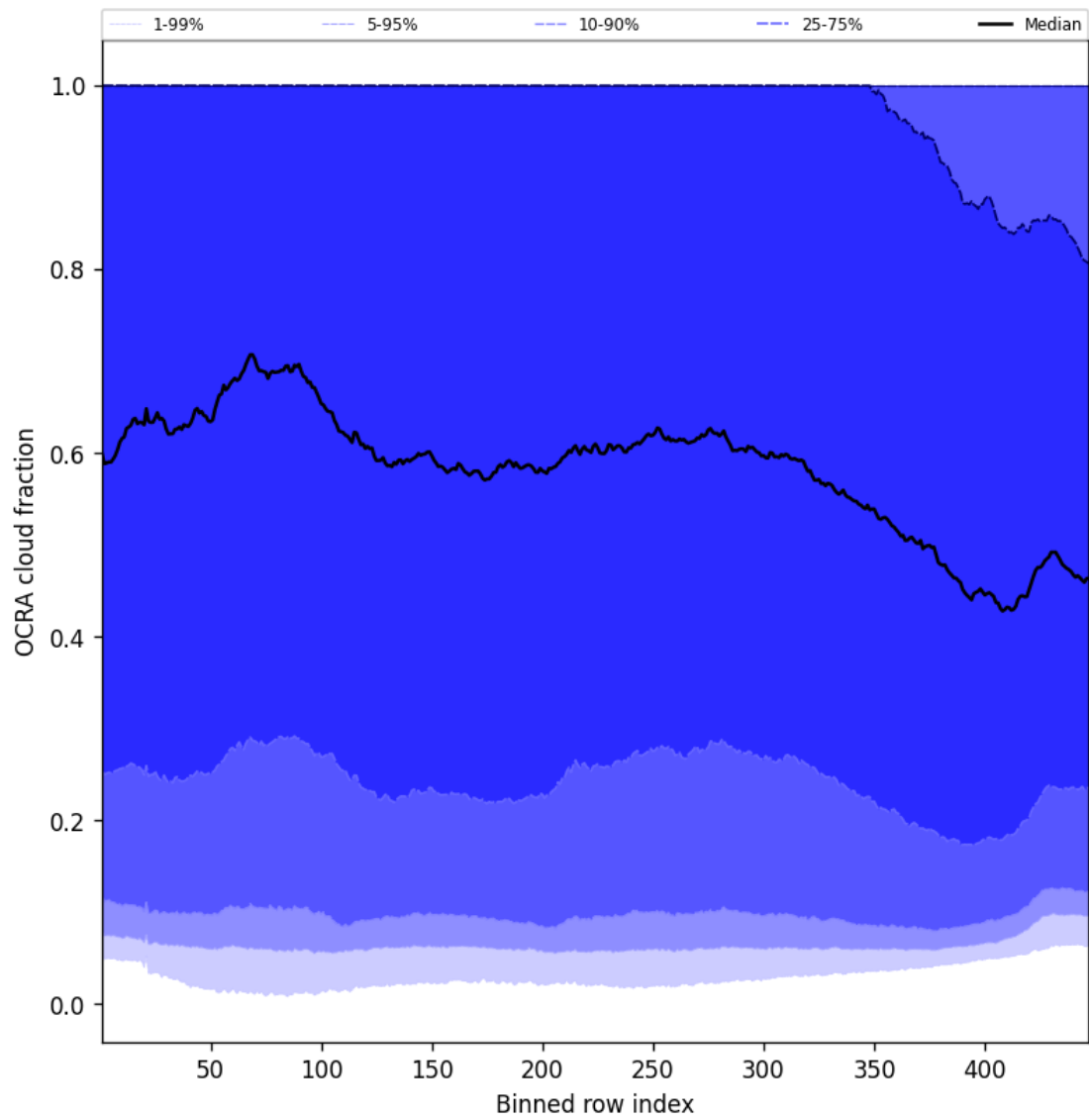
Figure 64: Along track statistics of “OCRA cloud fraction” for 2025-09-02 to 2025-09-02
