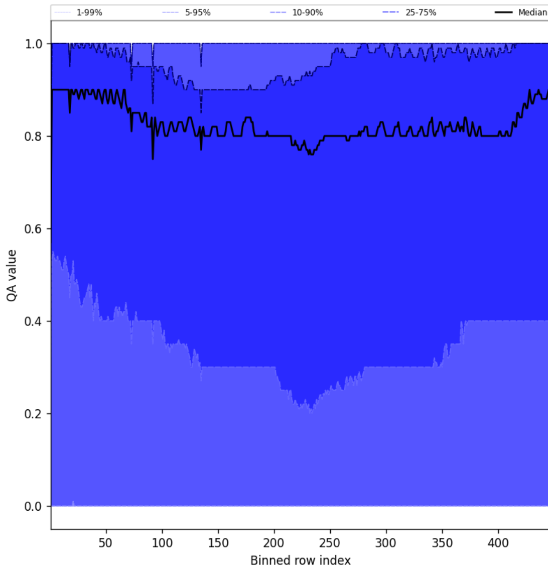
Figure 52: Along track statistics of “QA value” for 2025-09-02 to 2025-09-02
