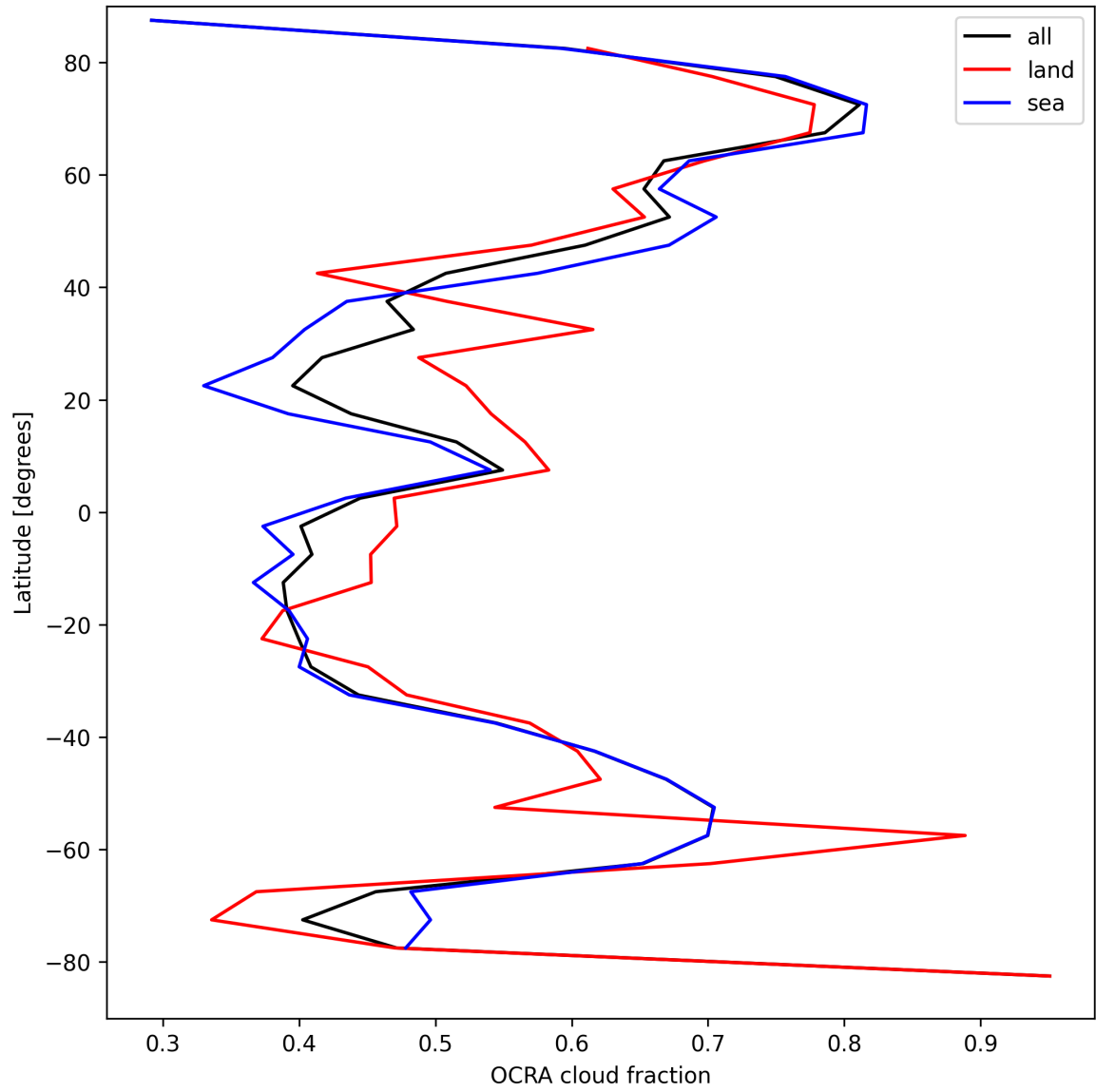
Figure 32: Zonal average of “OCRA cloud fraction” for 2025-09-02 to 2025-09-02.
