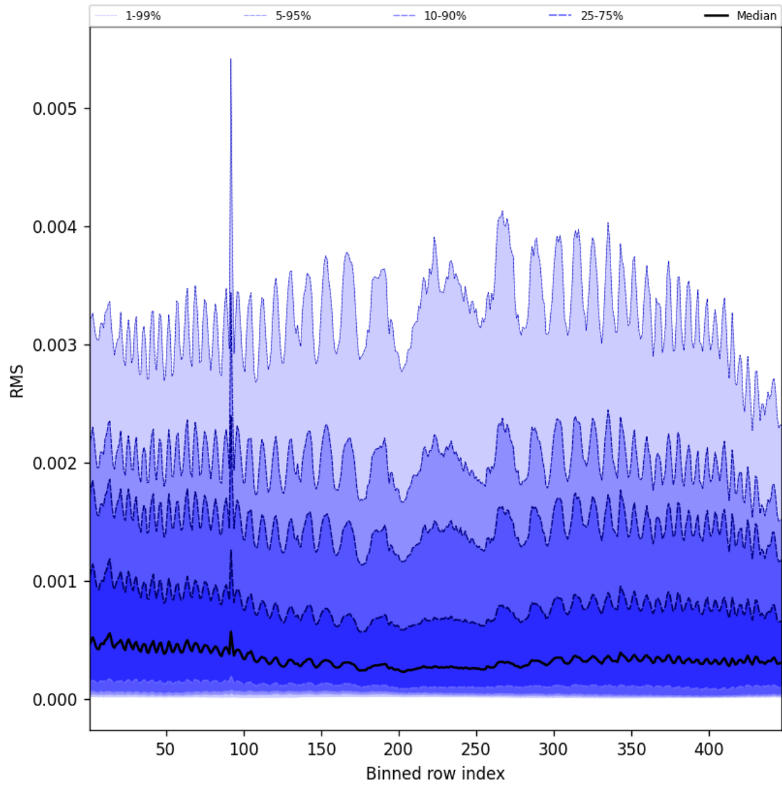
Figure 61: Along track statistics of “RMS” for 2025-09-02 to 2025-09-02
