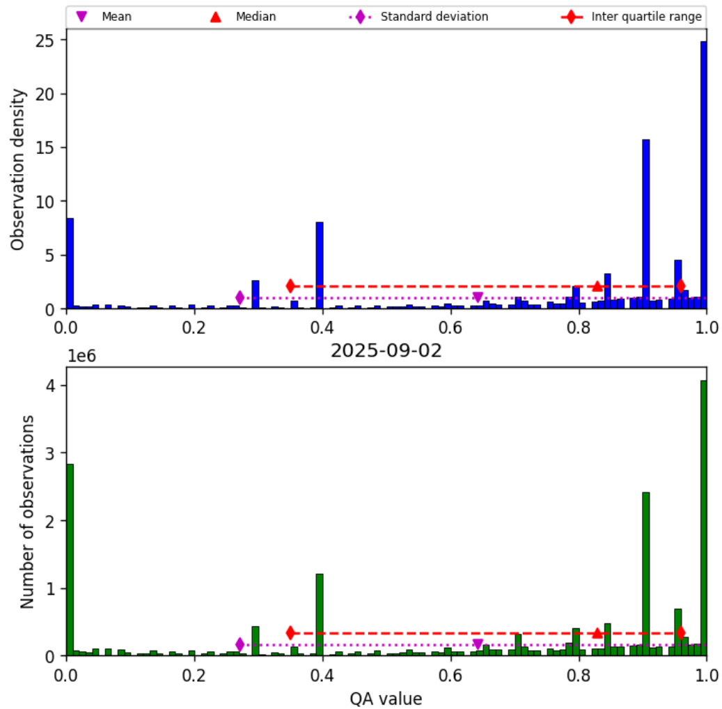
Figure 36: Histogram of “QA value” for 2025-09-02 to 2025-09-02
