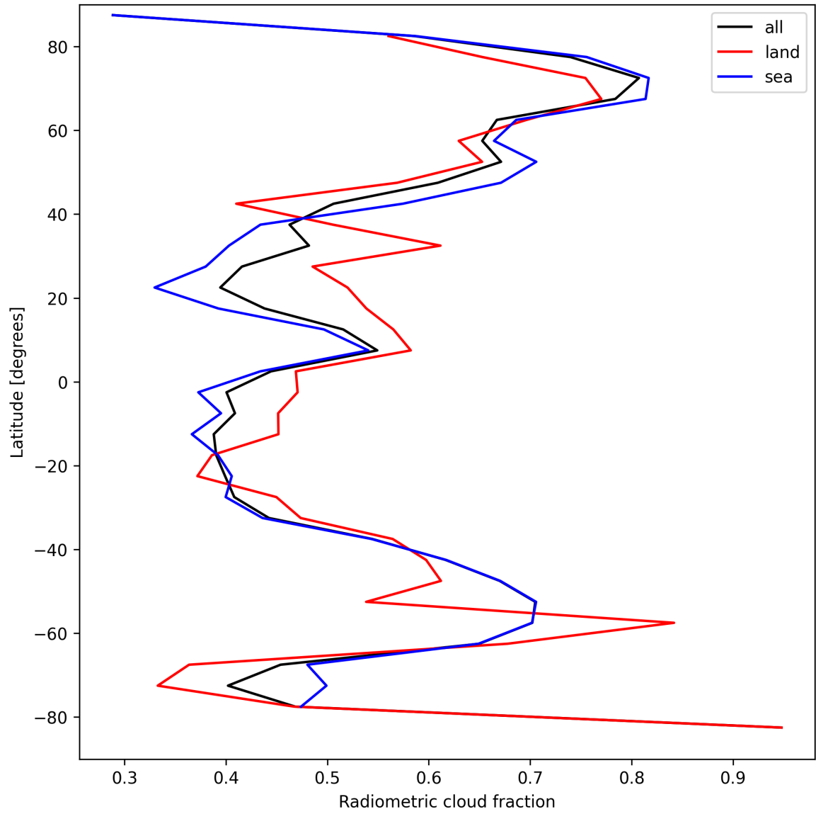
Figure 21: Zonal average of “Radiometric cloud fraction” for 2025-09-02 to 2025-09-02.
