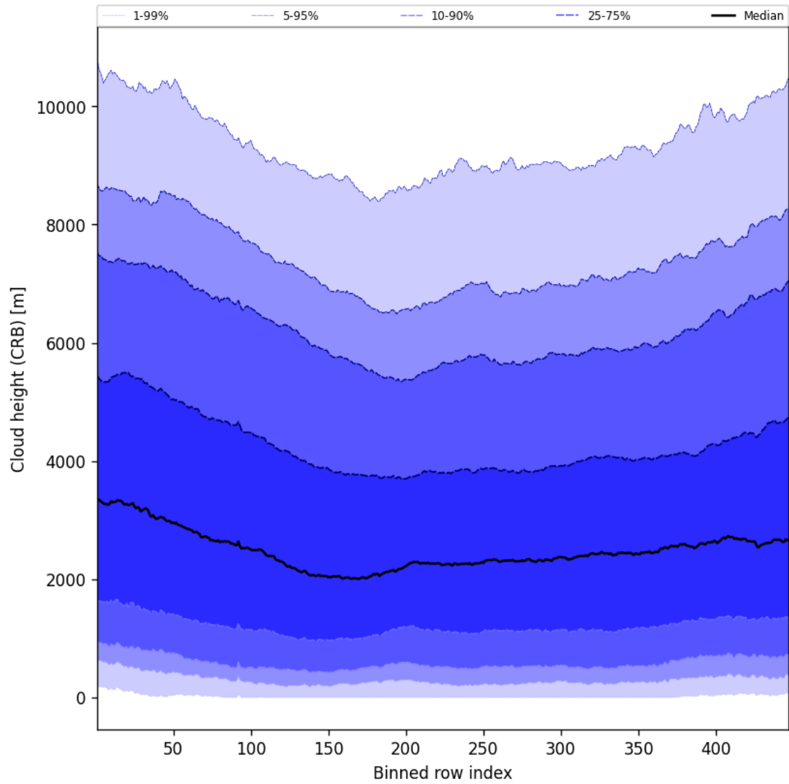
Figure 57: Along track statistics of “Cloud height (CRB)” for 2025-09-02 to 2025-09-02
