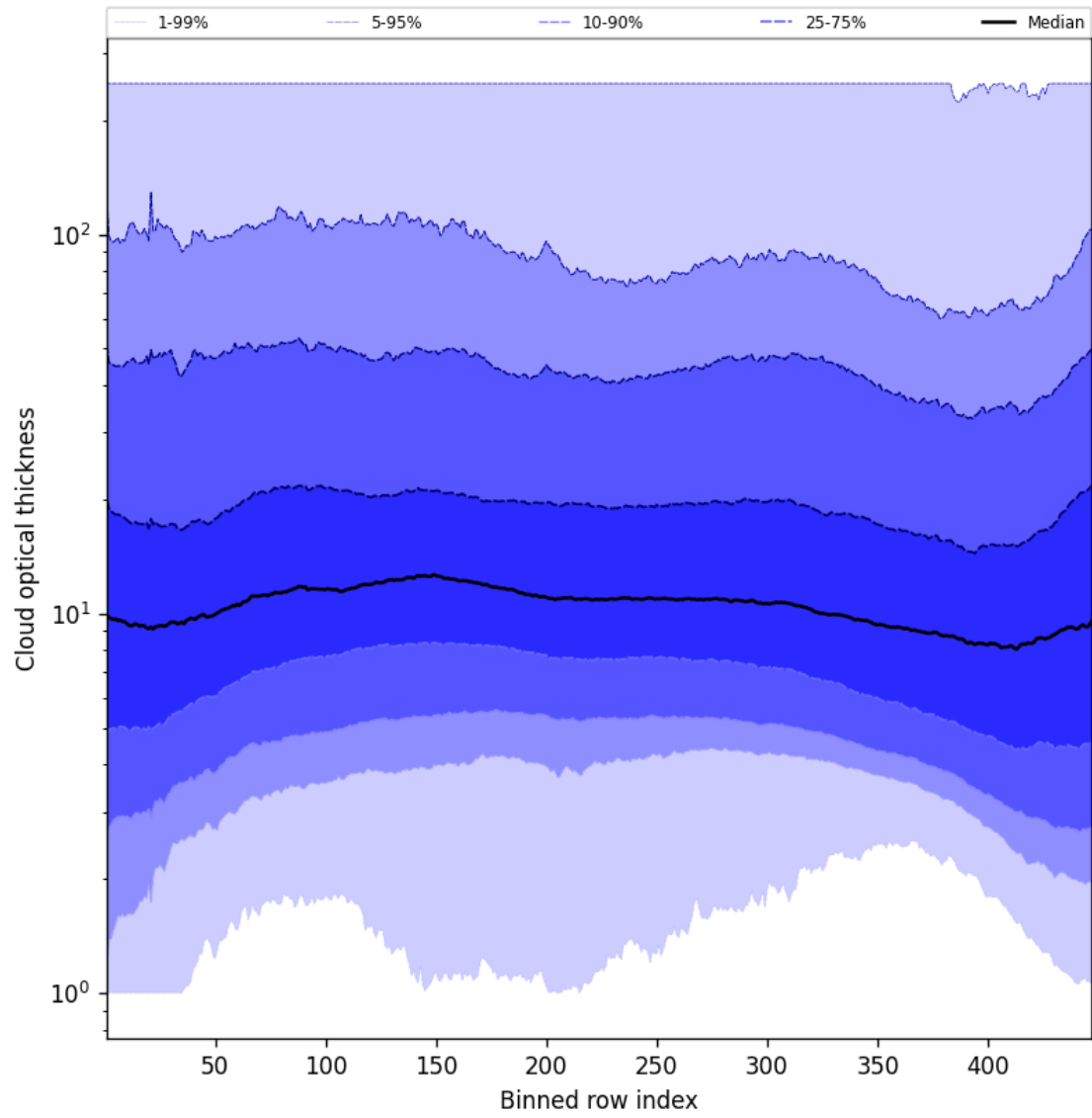
Figure 55: Along track statistics of “Cloud optical thickness” for 2025-09-02 to 2025-09-02
