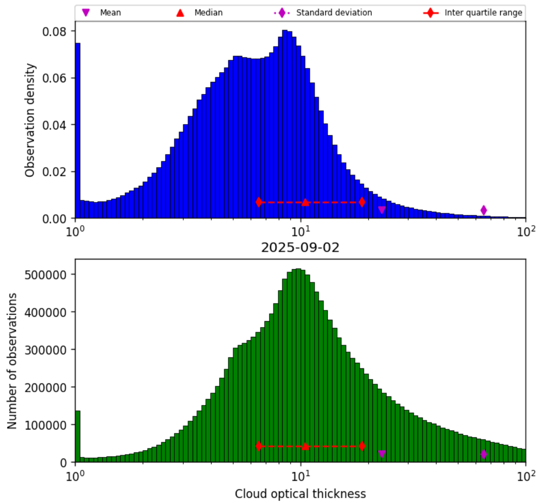
Figure 39: Histogram of “Cloud optical thickness” for 2025-09-02 to 2025-09-02
