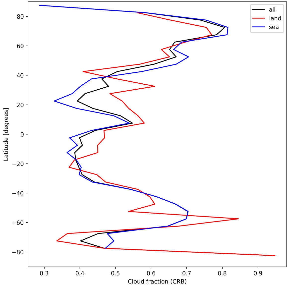
Figure 24: Zonal average of “Cloud fraction (CRB)” for 2025-09-02 to 2025-09-02.
