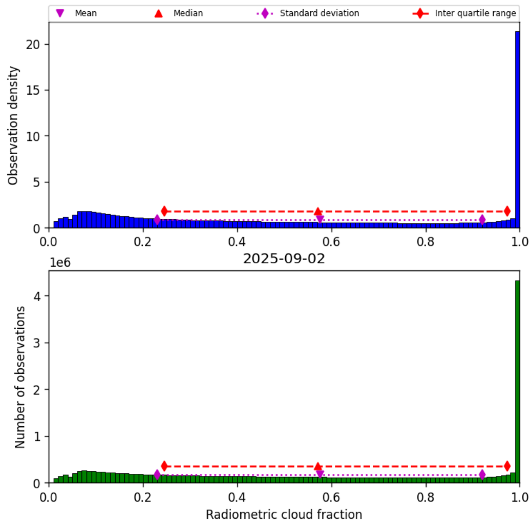
Figure 37: Histogram of “Radiometric cloud fraction” for 2025-09-02 to 2025-09-02
