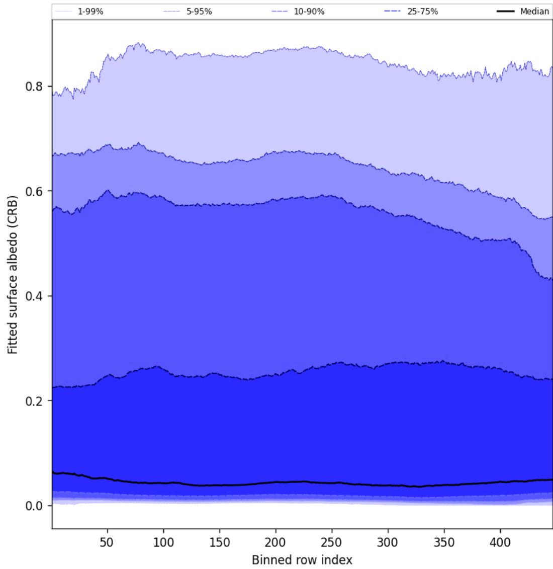
Figure 60: Along track statistics of “Fitted surface albedo (CRB)” for 2025-09-02 to 2025-09-02
