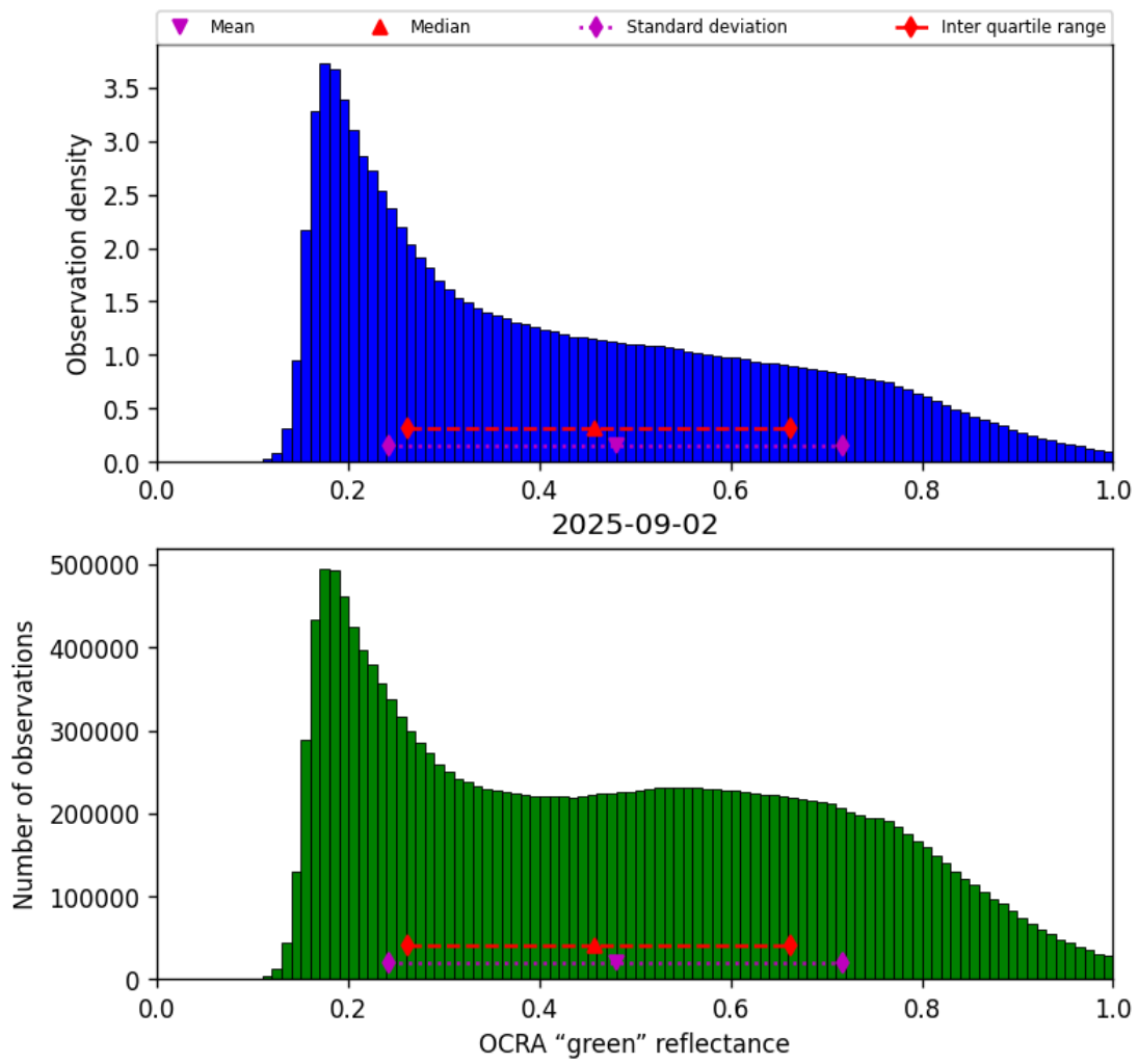
Figure 50: Histogram of “OCRA “green” reflectance” for 2025-09-02 to 2025-09-02
