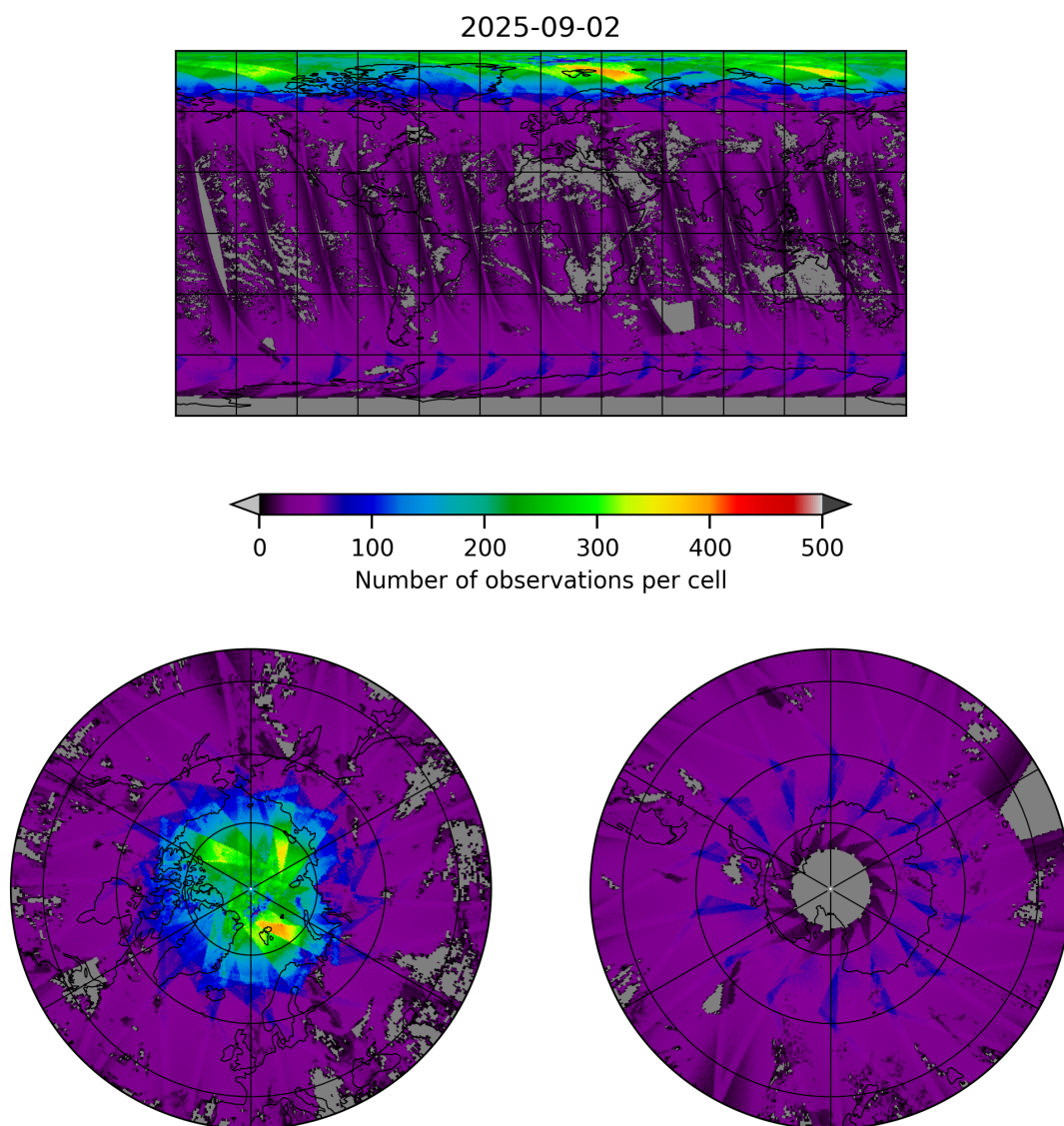
Figure 19: Map of the number of observations for 2025-09-02 to 2025-09-02
