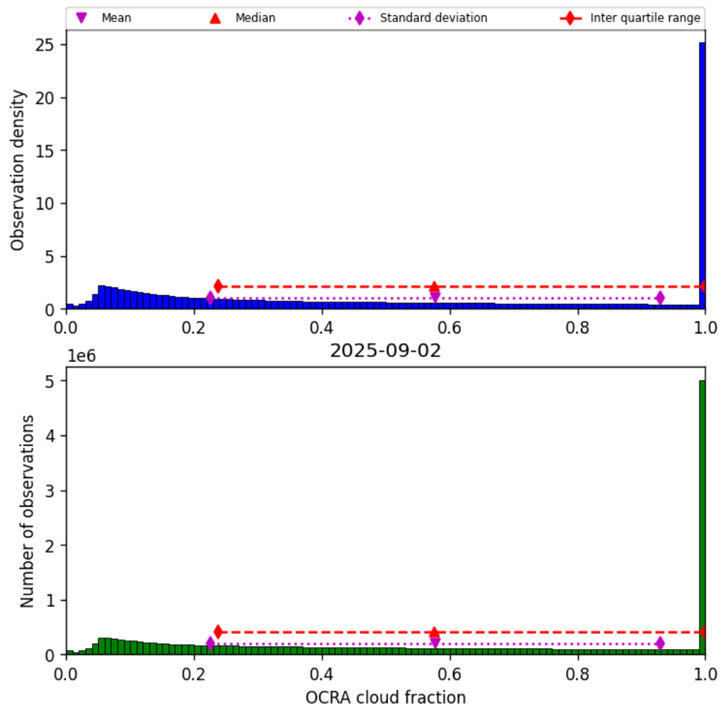
Figure 48: Histogram of “OCRA cloud fraction” for 2025-09-02 to 2025-09-02
