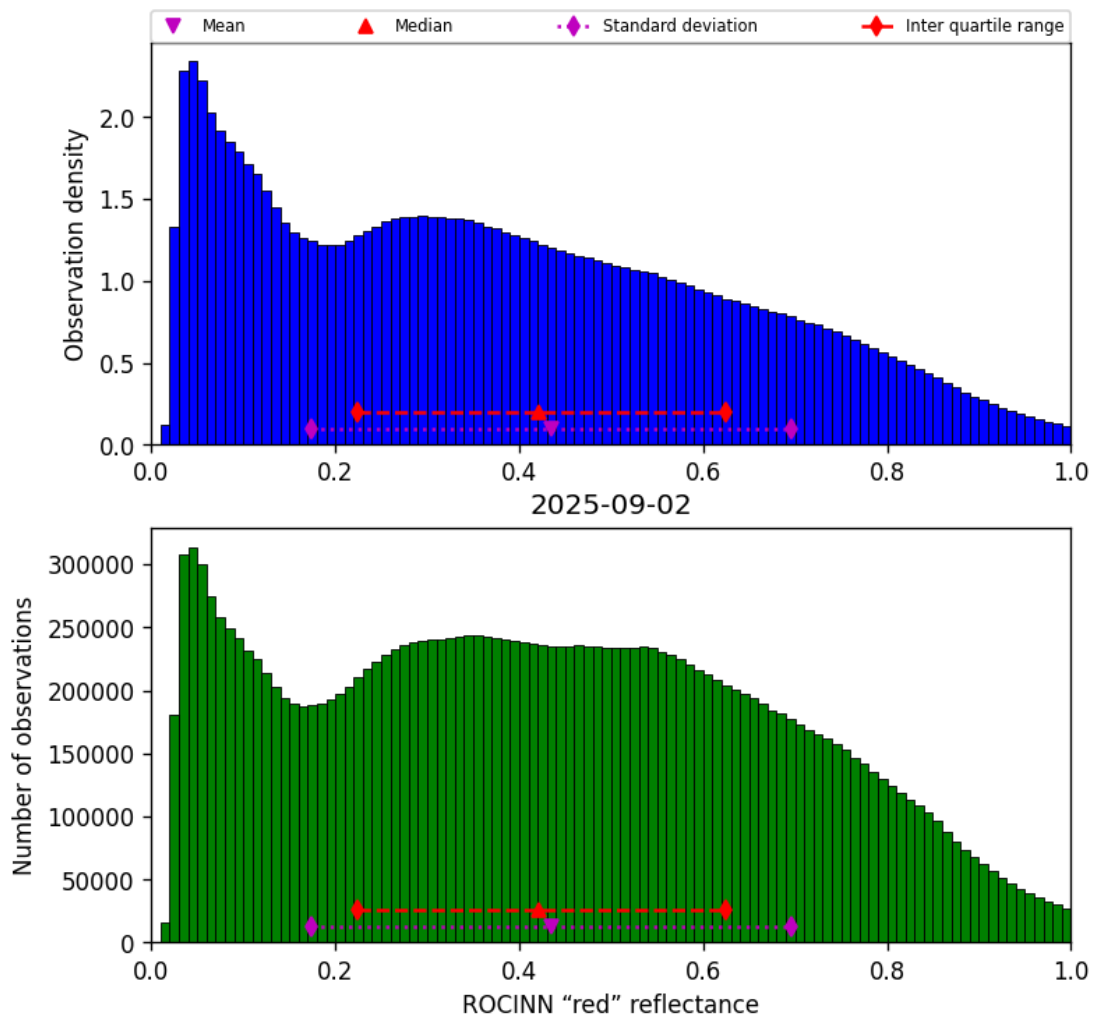
Figure 51: Histogram of “ROCINN “red” reflectance” for 2025-09-02 to 2025-09-02
