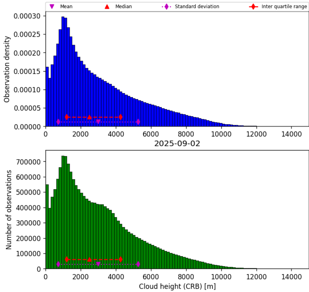
Figure 41: Histogram of “Cloud height (CRB)” for 2025-09-02 to 2025-09-02
