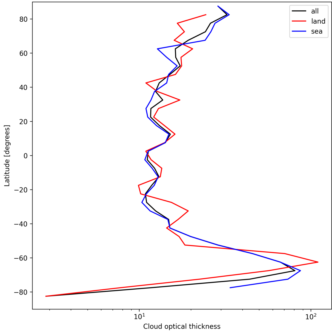
Figure 23: Zonal average of “Cloud optical thickness” for 2025-09-02 to 2025-09-02.
