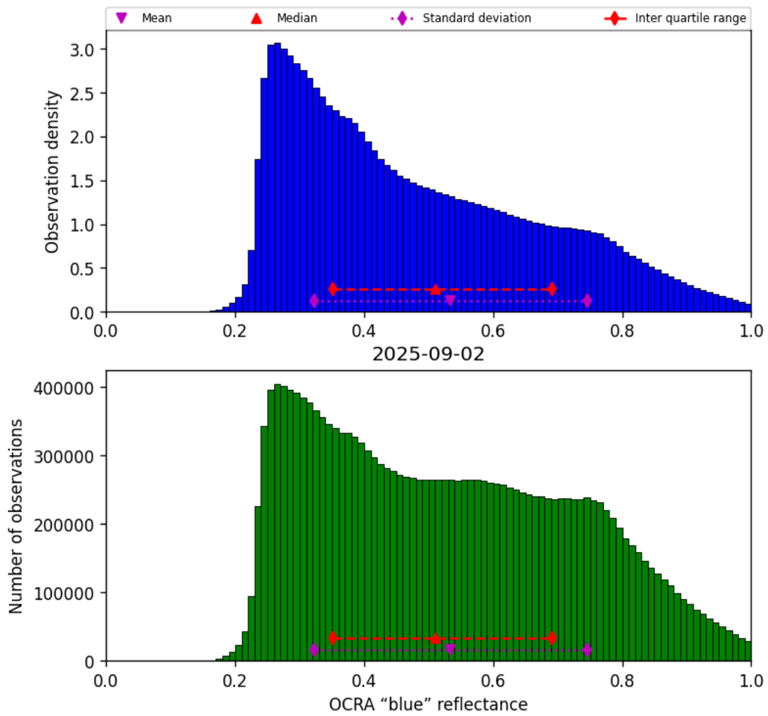
Figure 49: Histogram of “OCRA “blue” reflectance” for 2025-09-02 to 2025-09-02
