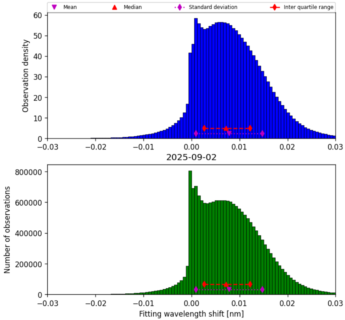
Figure 47: Histogram of “Fitting wavelength shift” for 2025-09-02 to 2025-09-02
