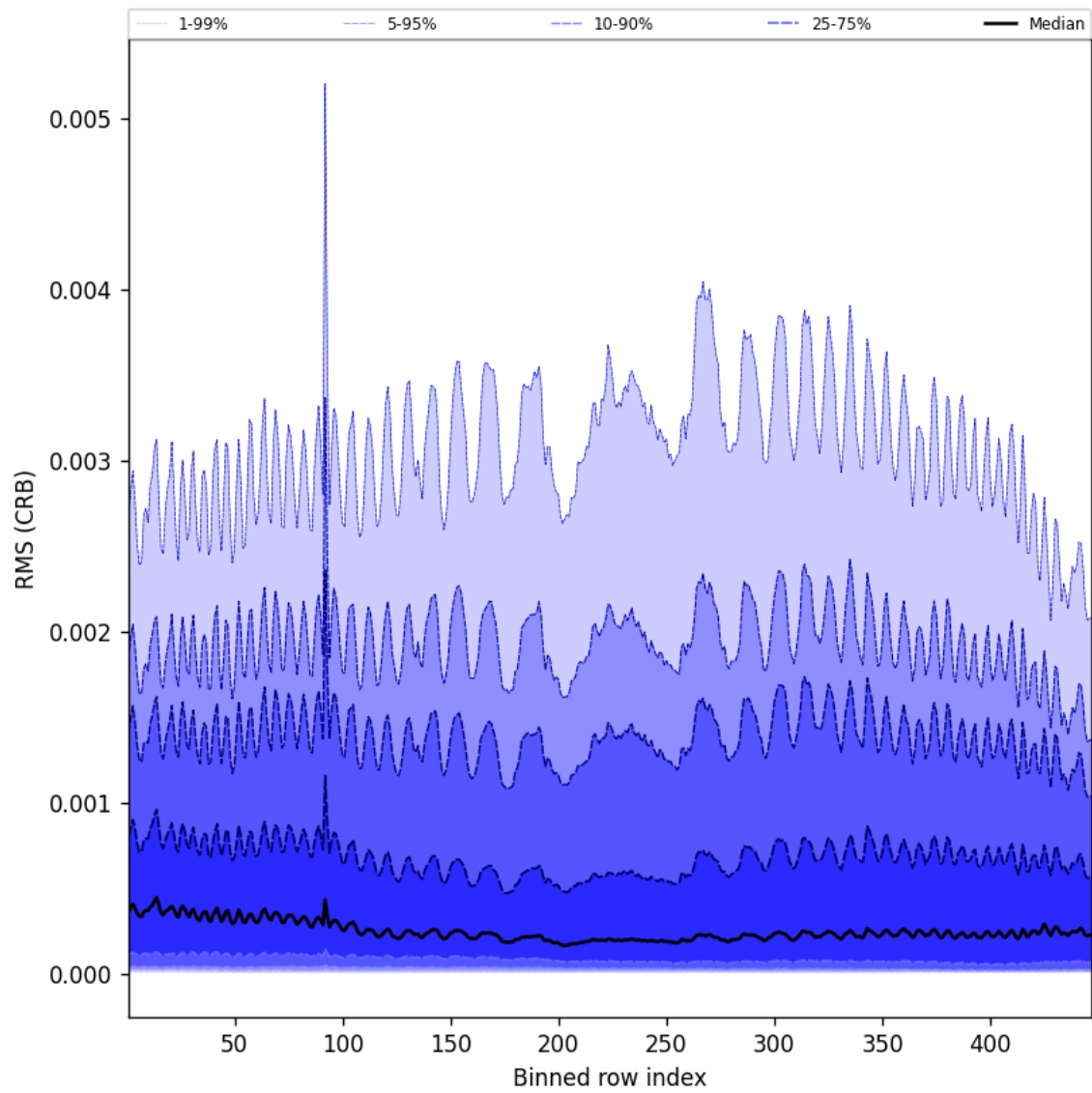
Figure 62: Along track statistics of “RMS (CRB)” for 2025-09-02 to 2025-09-02
