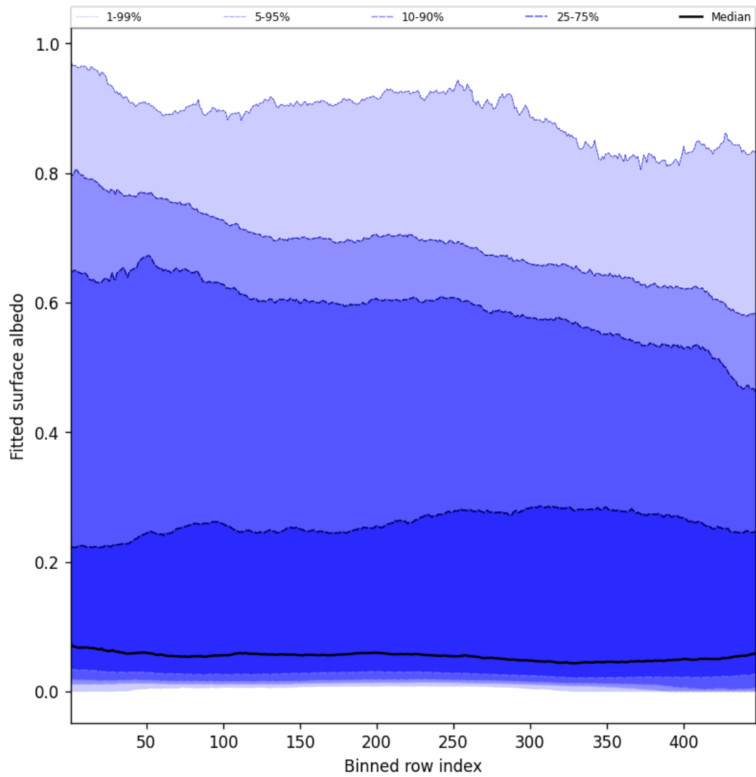
Figure 59: Along track statistics of “Fitted surface albedo” for 2025-09-02 to 2025-09-02
