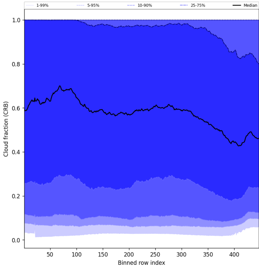
Figure 56: Along track statistics of “Cloud fraction (CRB)” for 2025-09-02 to 2025-09-02
