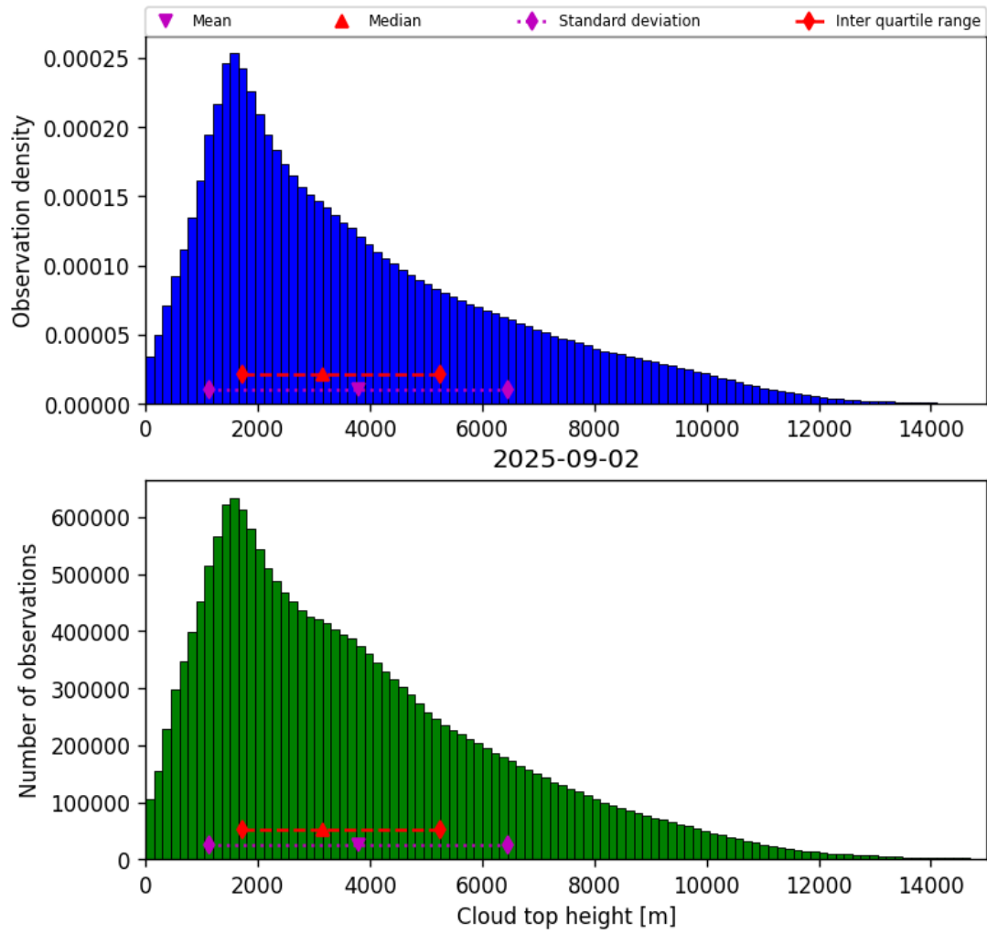
Figure 38: Histogram of “Cloud top height” for 2025-09-02 to 2025-09-02
