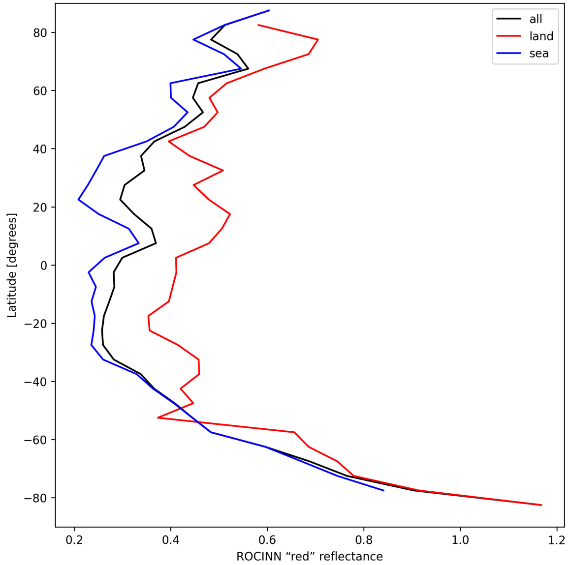
Figure 35: Zonal average of “ROCINN “red” reflectance” for 2025-09-02 to 2025-09-02.
