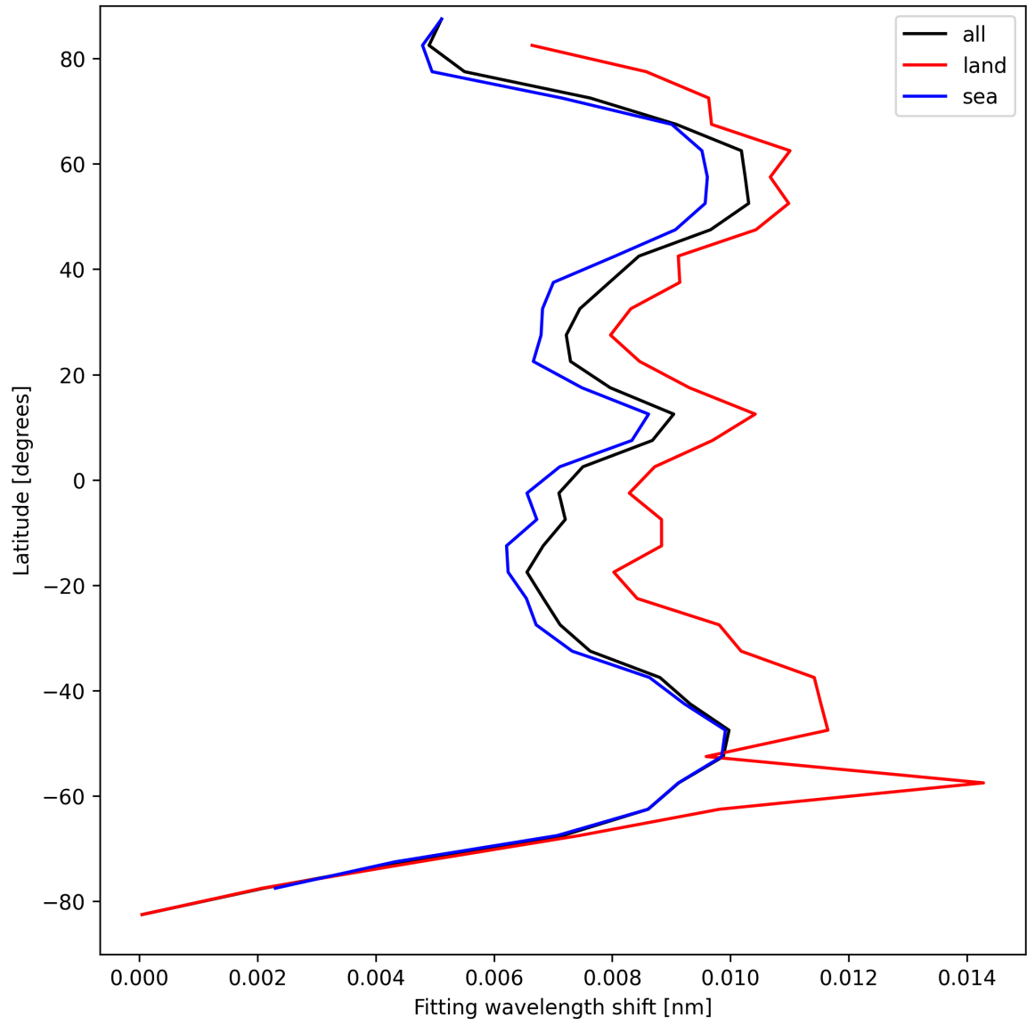
Figure 31: Zonal average of “Fitting wavelength shift” for 2025-09-02 to 2025-09-02.
