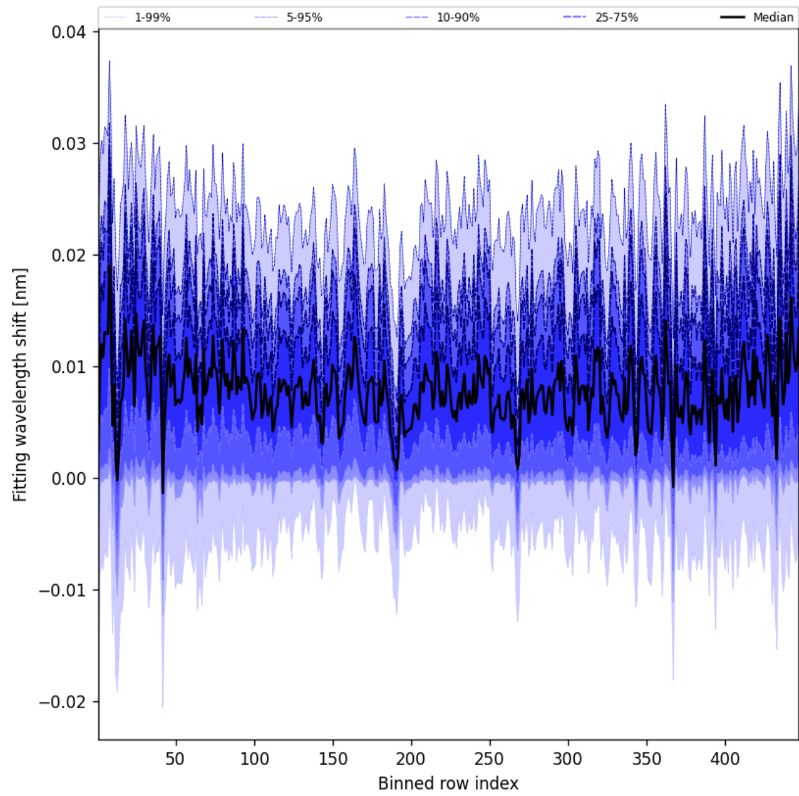
Figure 63: Along track statistics of “Fitting wavelength shift” for 2025-09-02 to 2025-09-02
