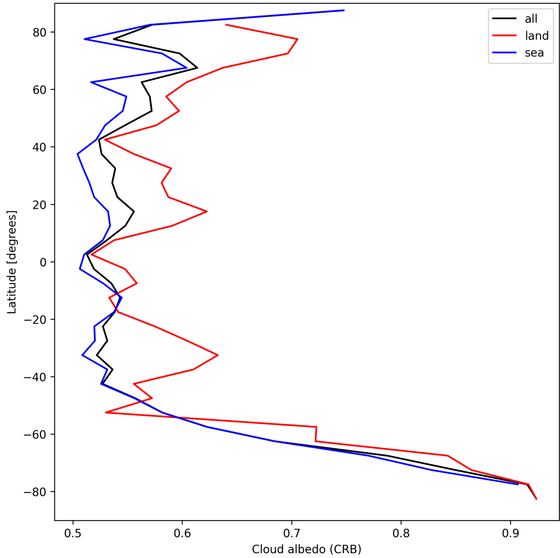
Figure 26: Zonal average of “Cloud albedo (CRB)” for 2025-09-02 to 2025-09-02.
