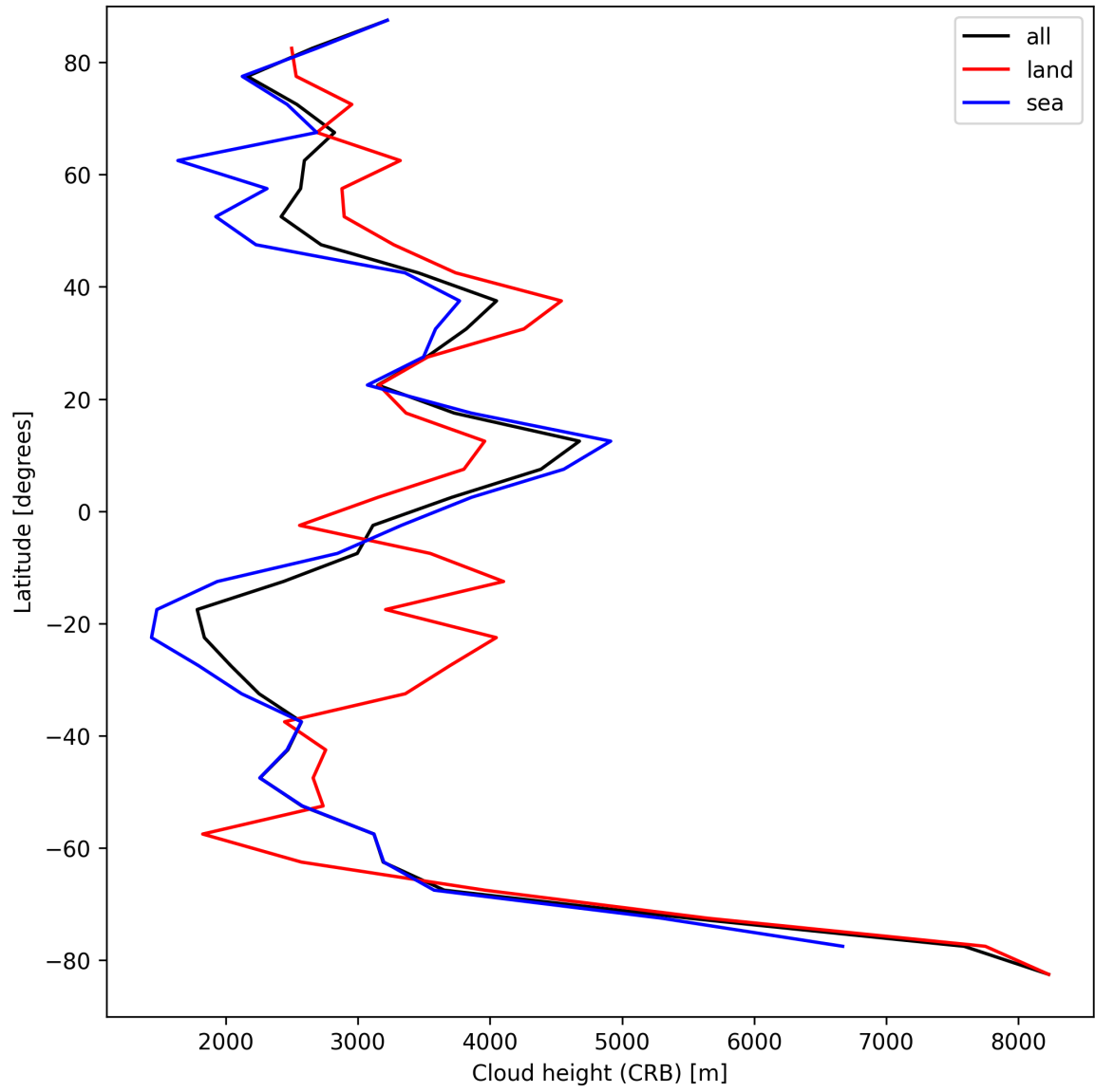
Figure 25: Zonal average of “Cloud height (CRB)” for 2025-09-02 to 2025-09-02.
