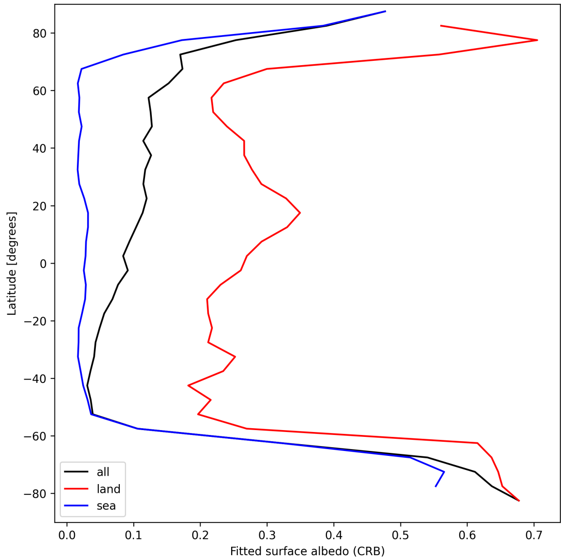
Figure 28: Zonal average of “Fitted surface albedo (CRB)” for 2025-09-02 to 2025-09-02.
