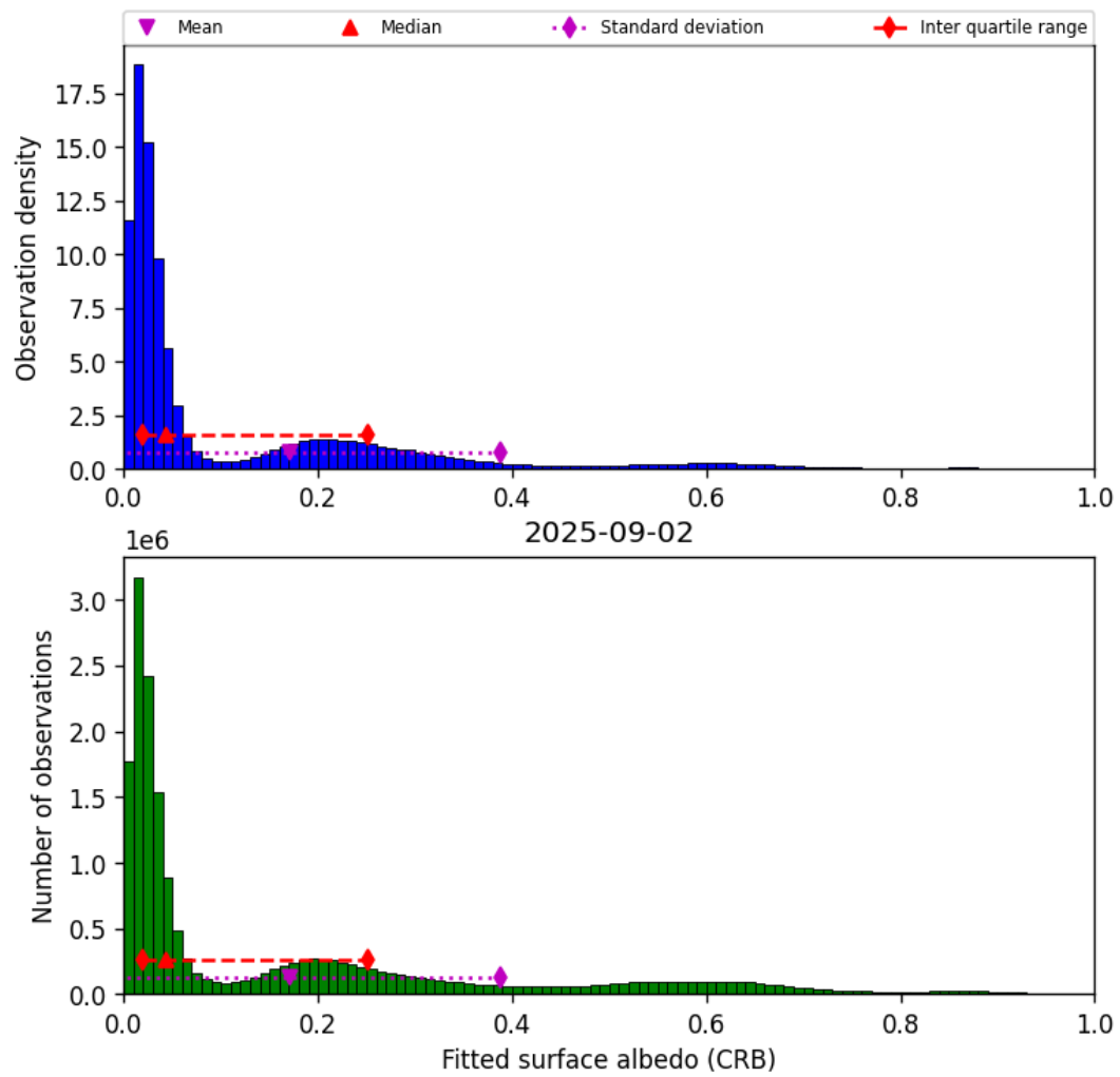
Figure 44: Histogram of “Fitted surface albedo (CRB)” for 2025-09-02 to 2025-09-02
