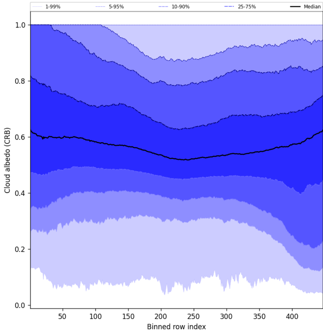
Figure 58: Along track statistics of “Cloud albedo (CRB)” for 2025-09-02 to 2025-09-02
