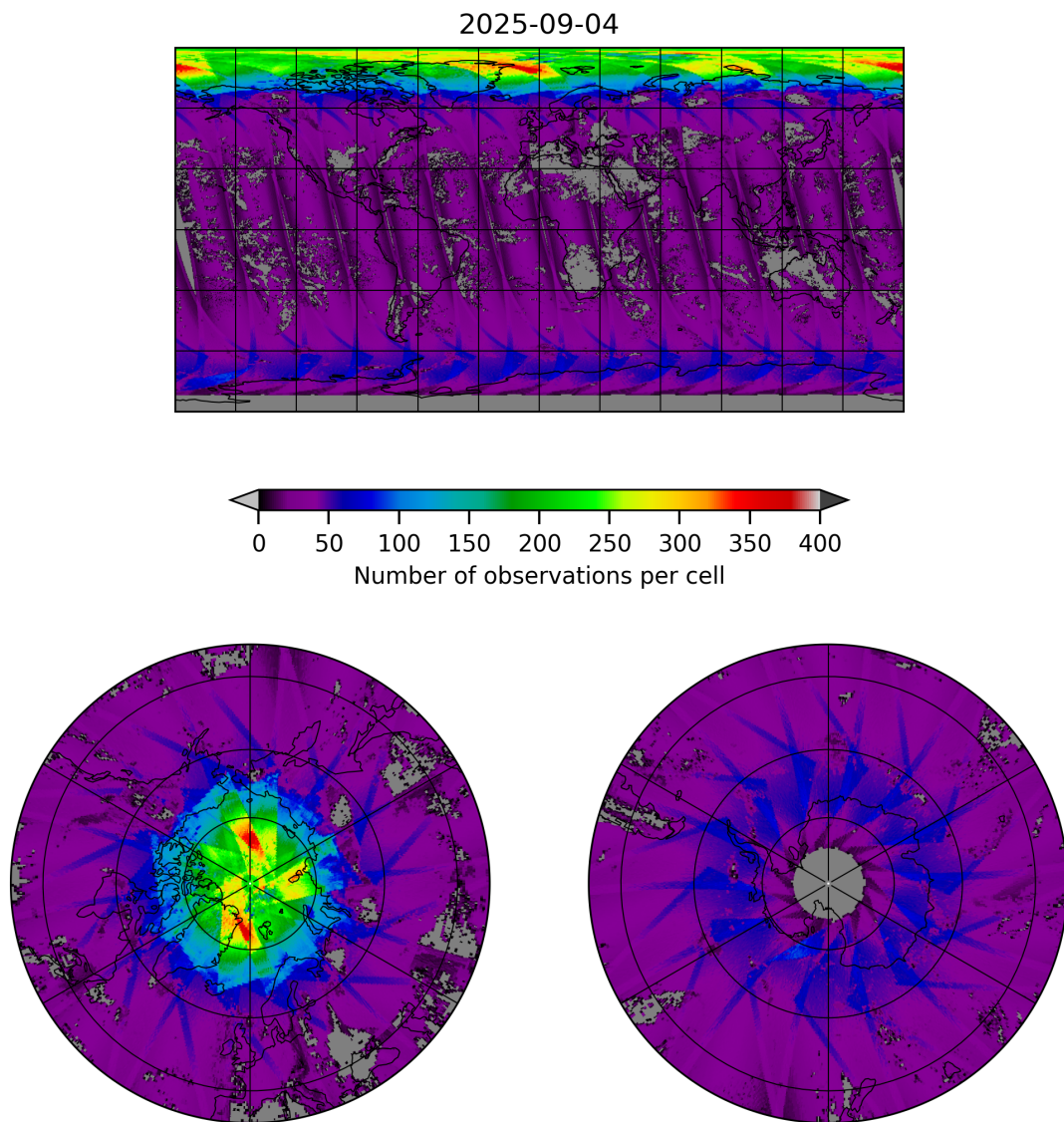
Figure 19: Map of the number of observations for 2025-09-04 to 2025-09-05
