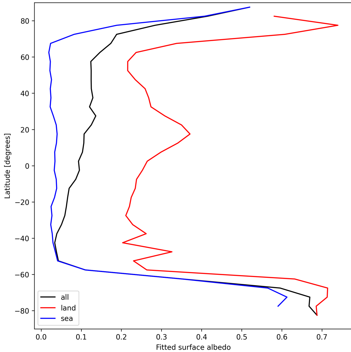
Figure 27: Zonal average of “Fitted surface albedo” for 2025-09-04 to 2025-09-05.
