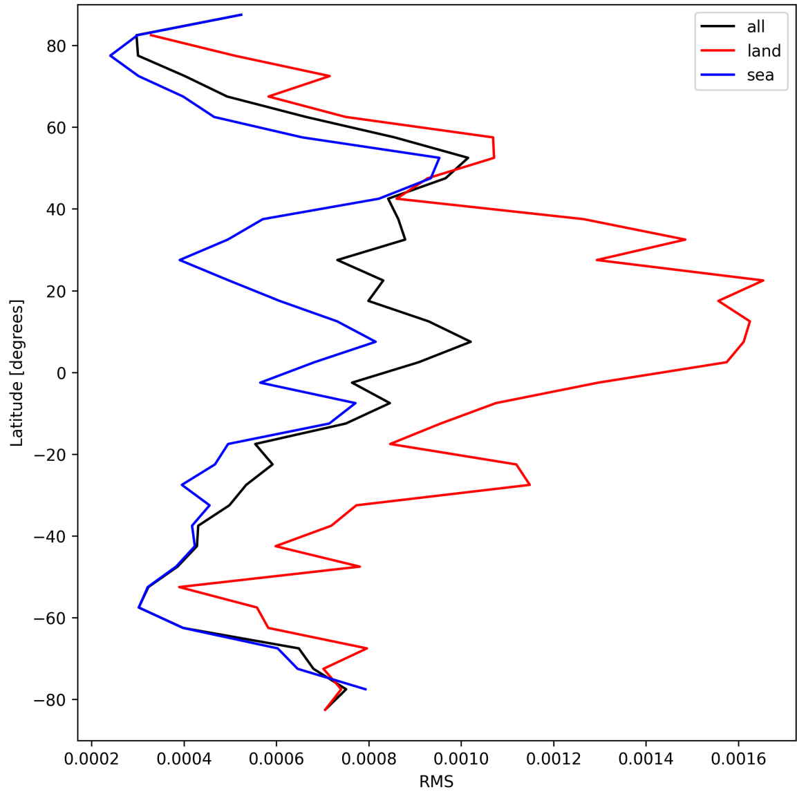
Figure 29: Zonal average of “RMS” for 2025-09-04 to 2025-09-05.
