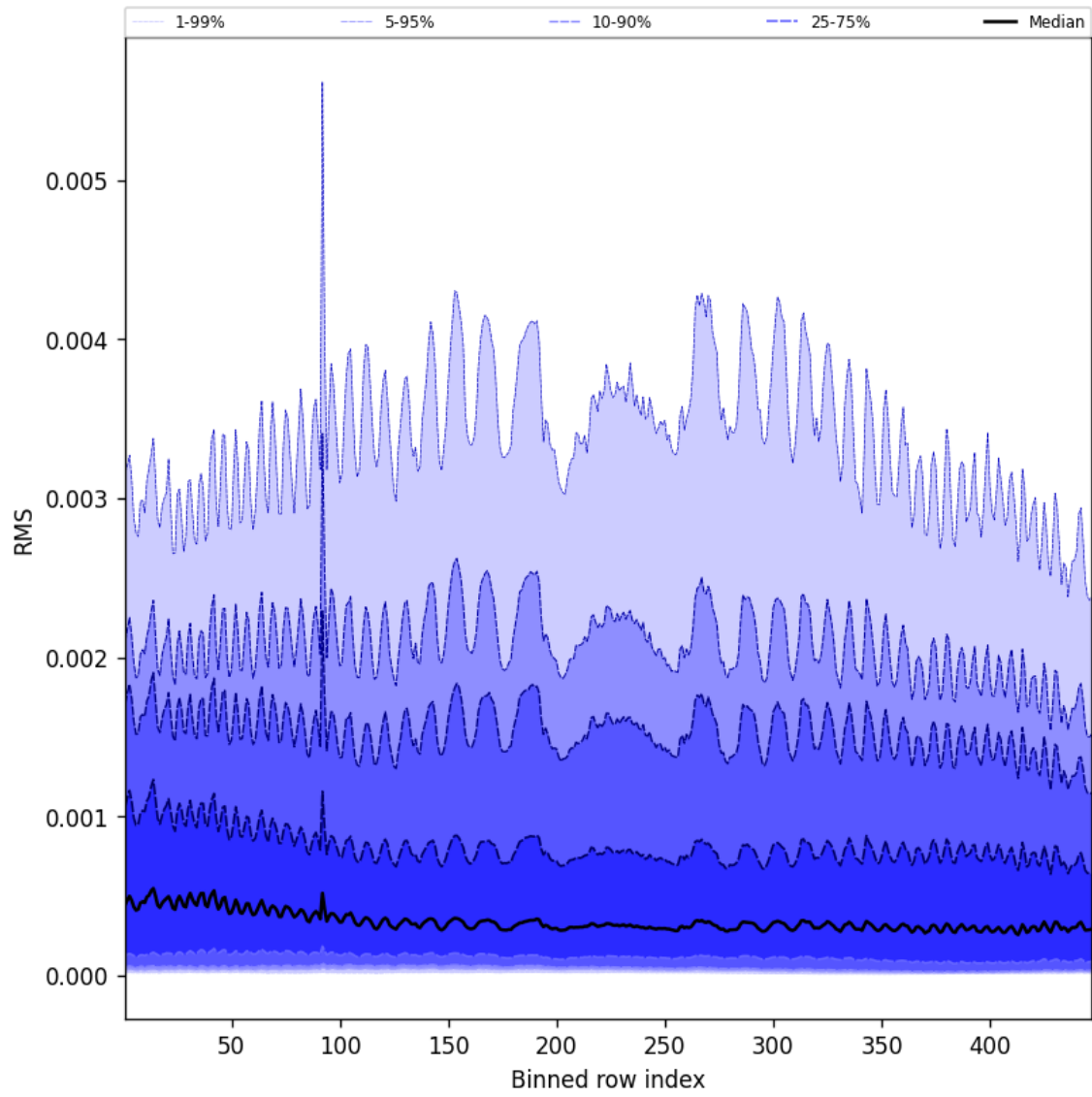
Figure 61: Along track statistics of “RMS” for 2025-09-04 to 2025-09-05
