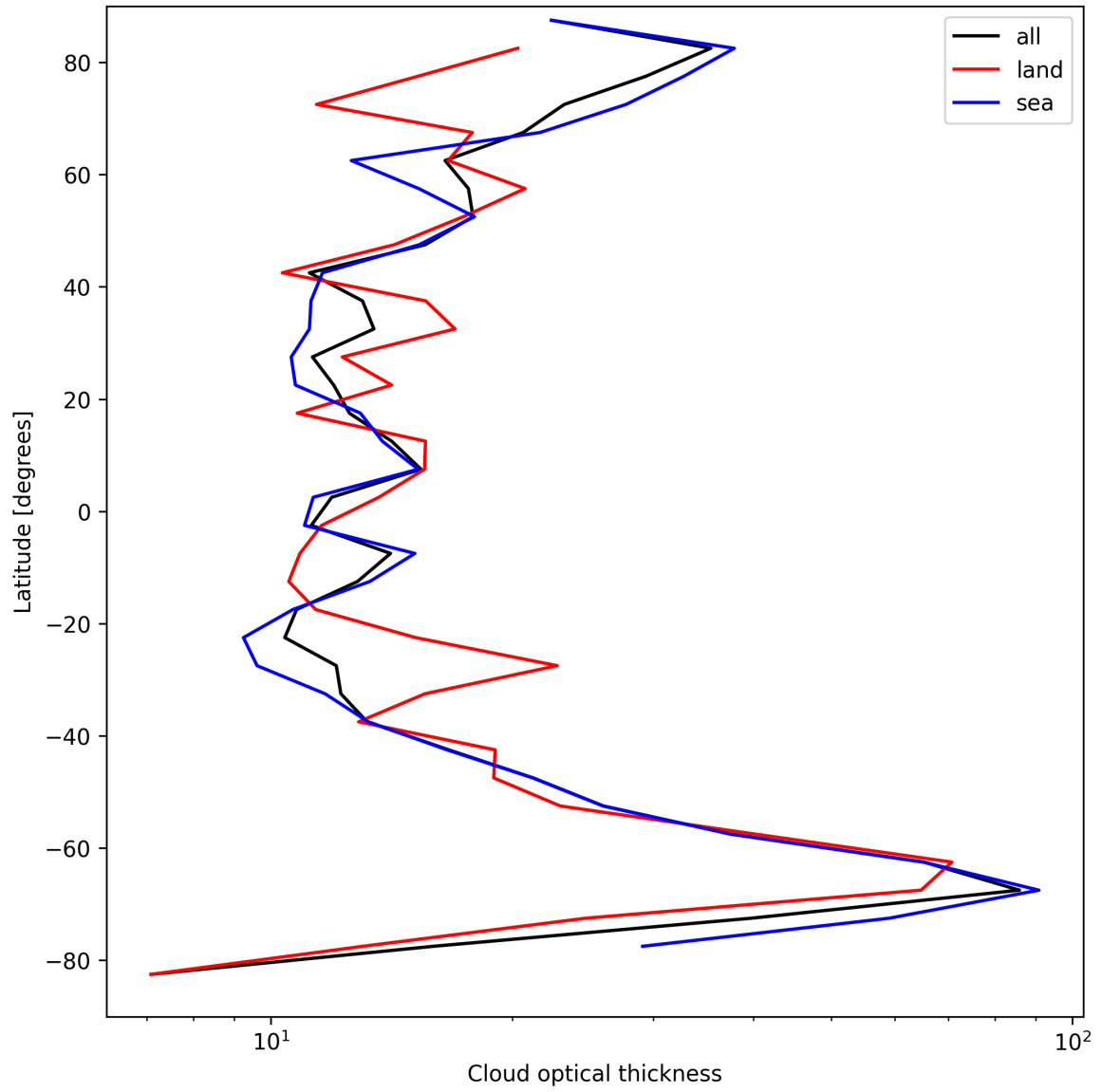
Figure 23: Zonal average of “Cloud optical thickness” for 2025-09-04 to 2025-09-05.
