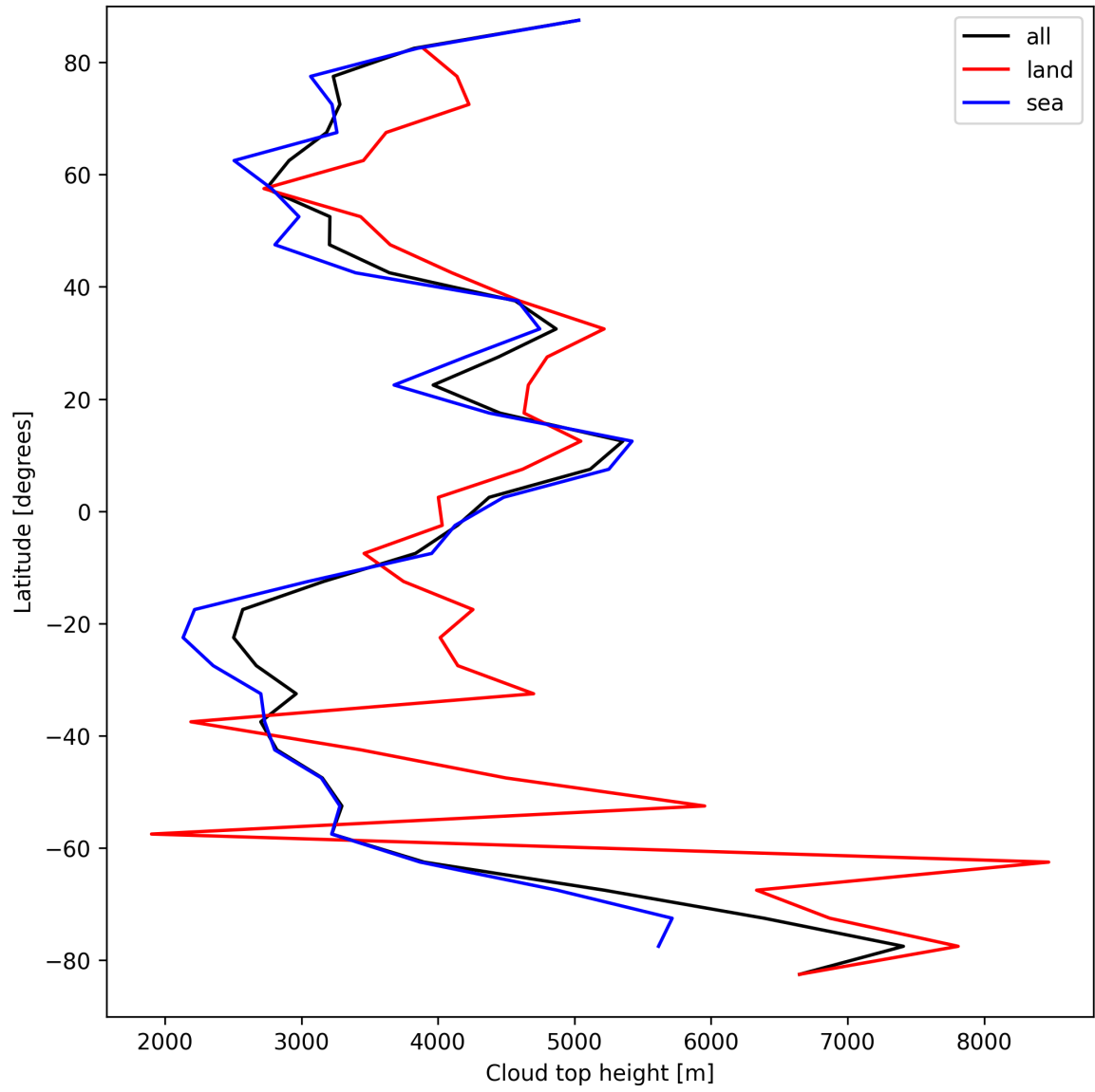
Figure 22: Zonal average of “Cloud top height” for 2025-09-04 to 2025-09-05.
