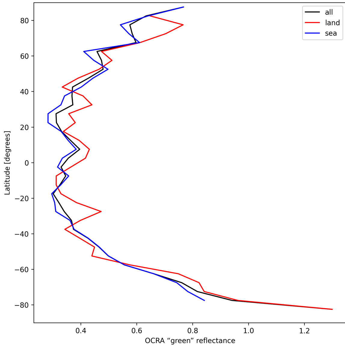
Figure 34: Zonal average of “OCRA “green” reflectance” for 2025-09-04 to 2025-09-05.
