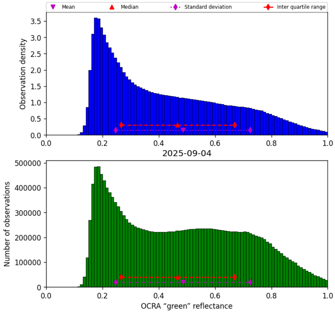
Figure 50: Histogram of “OCRA “green” reflectance” for 2025-09-04 to 2025-09-05
