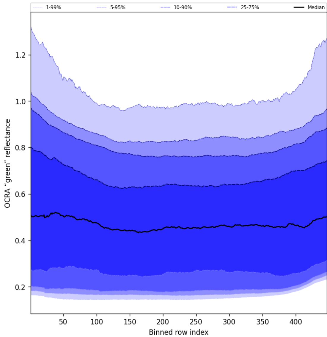
Figure 66: Along track statistics of “OCRA “green” reflectance” for 2025-09-04 to 2025-09-05
