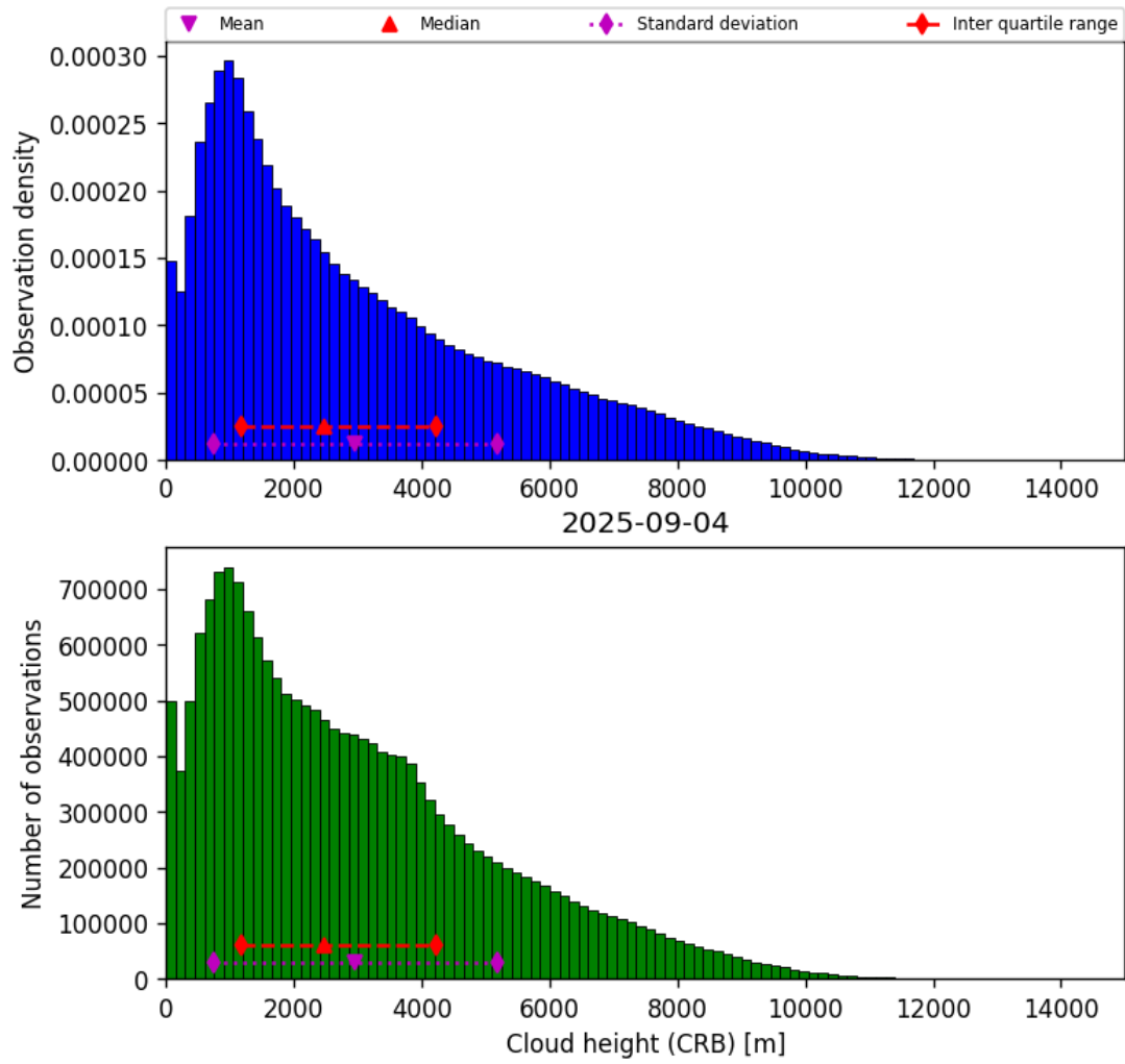
Figure 41: Histogram of “Cloud height (CRB)” for 2025-09-04 to 2025-09-05
