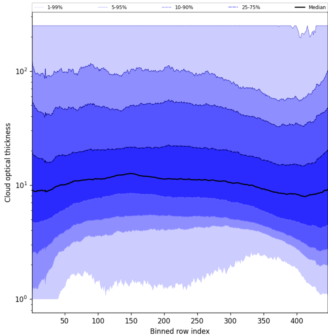
Figure 55: Along track statistics of “Cloud optical thickness” for 2025-09-04 to 2025-09-05
