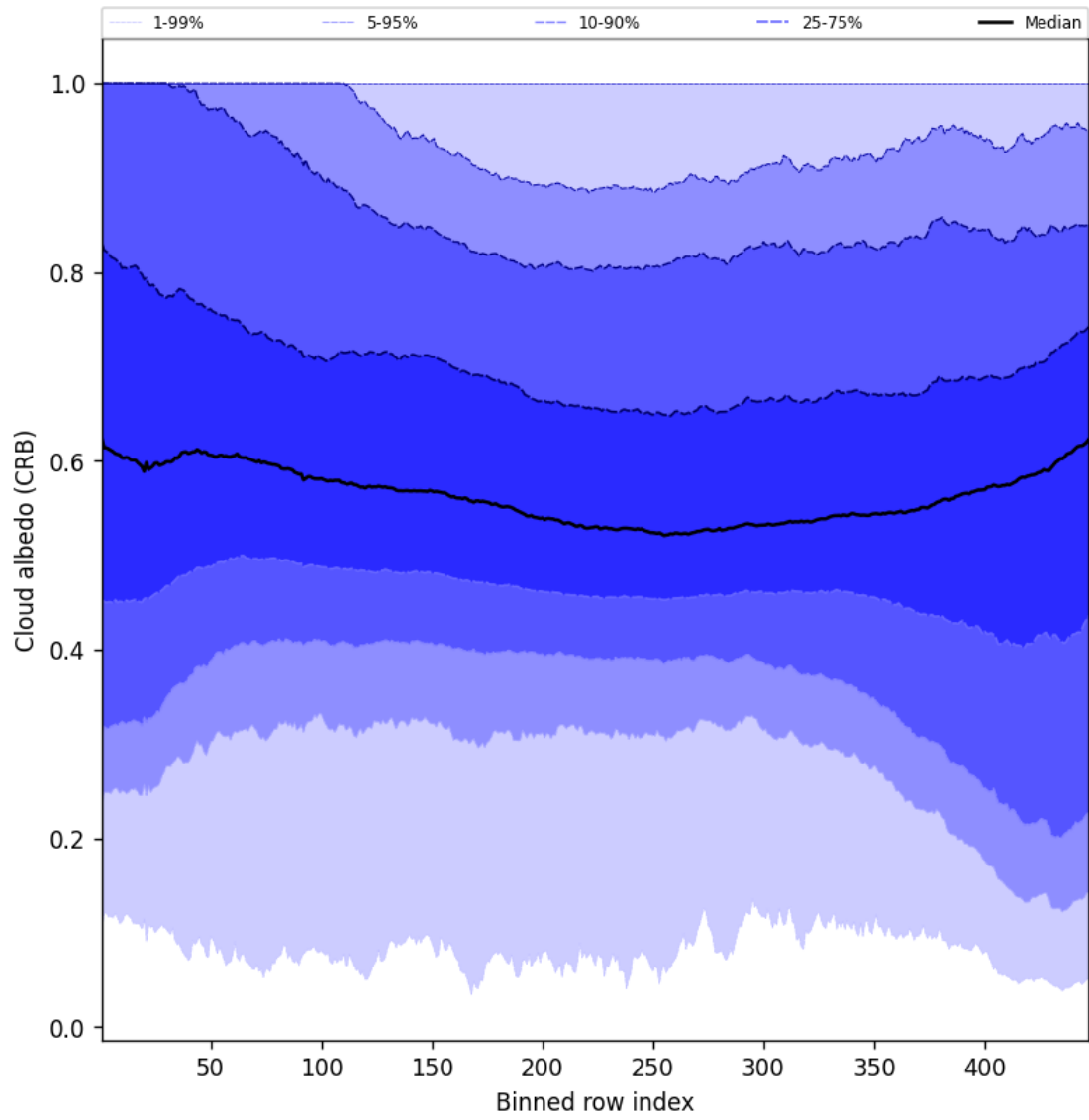
Figure 58: Along track statistics of “Cloud albedo (CRB)” for 2025-09-04 to 2025-09-05
