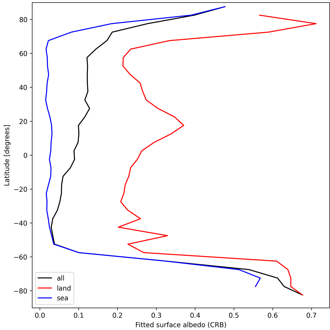
Figure 28: Zonal average of “Fitted surface albedo (CRB)” for 2025-09-04 to 2025-09-05.
