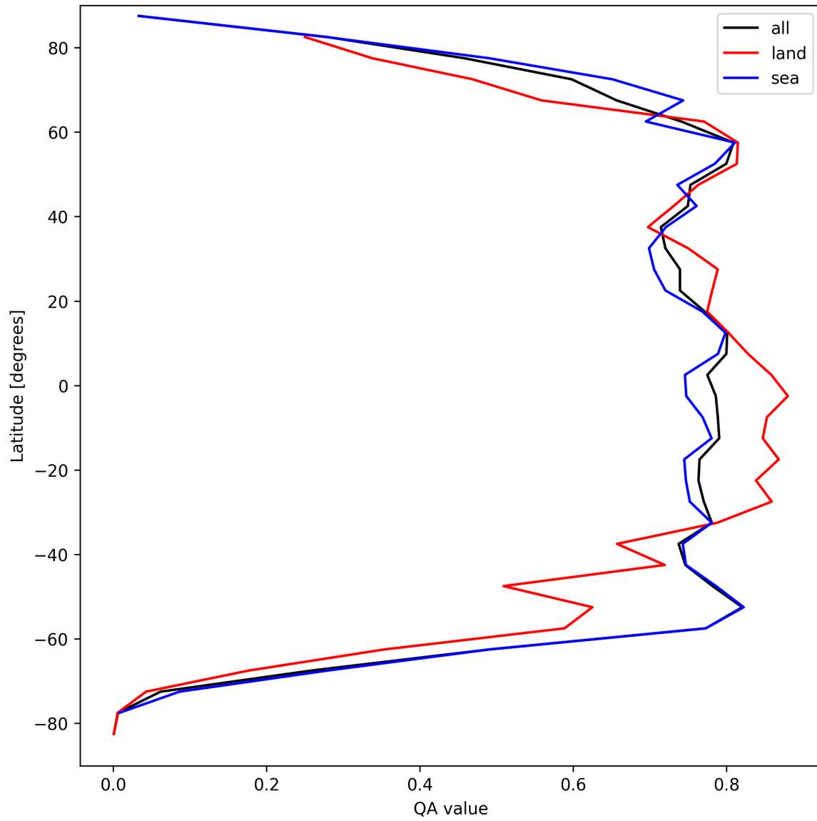
Figure 20: Zonal average of “QA value” for 2025-09-04 to 2025-09-05.
