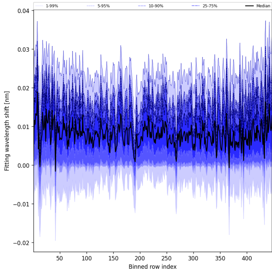
Figure 63: Along track statistics of “Fitting wavelength shift” for 2025-09-04 to 2025-09-05
