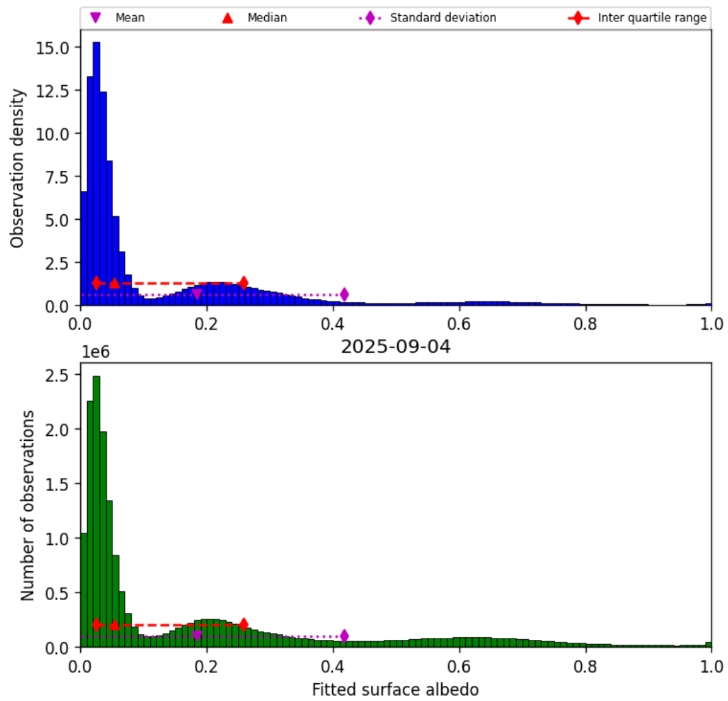
Figure 43: Histogram of “Fitted surface albedo” for 2025-09-04 to 2025-09-05
