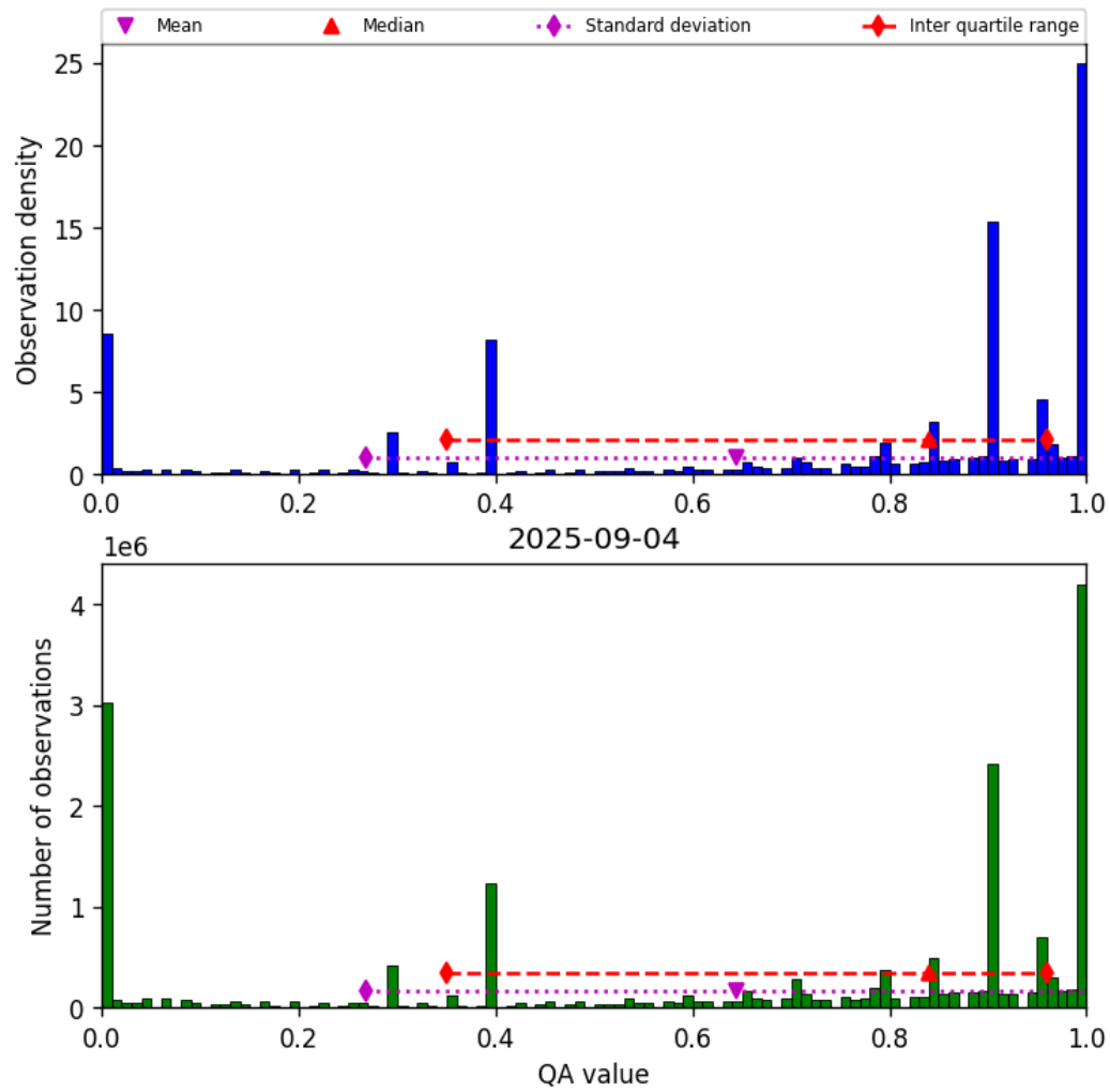
Figure 36: Histogram of “QA value” for 2025-09-04 to 2025-09-05
