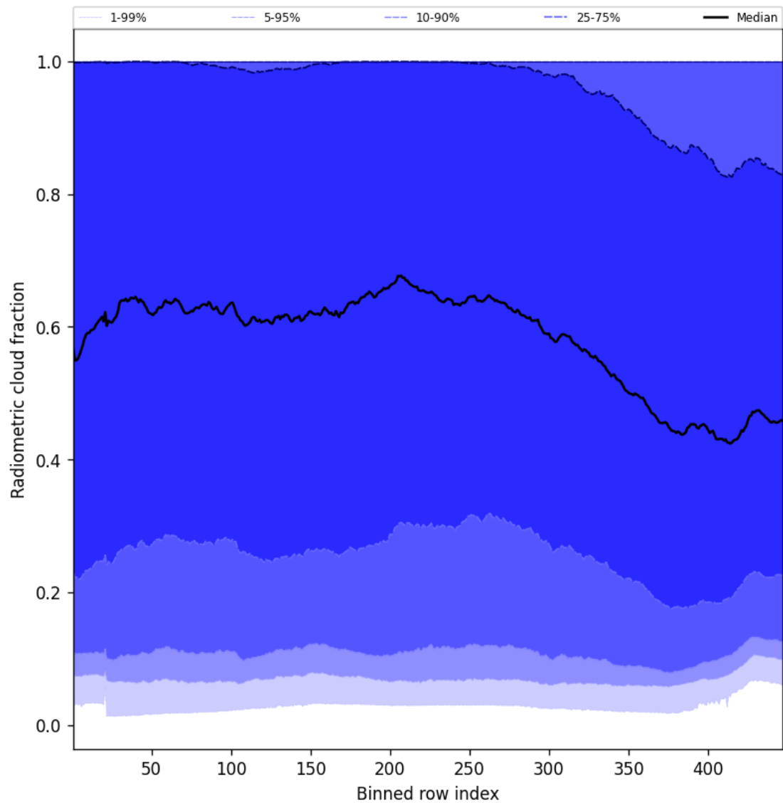
Figure 53: Along track statistics of “Radiometric cloud fraction” for 2025-09-04 to 2025-09-05
