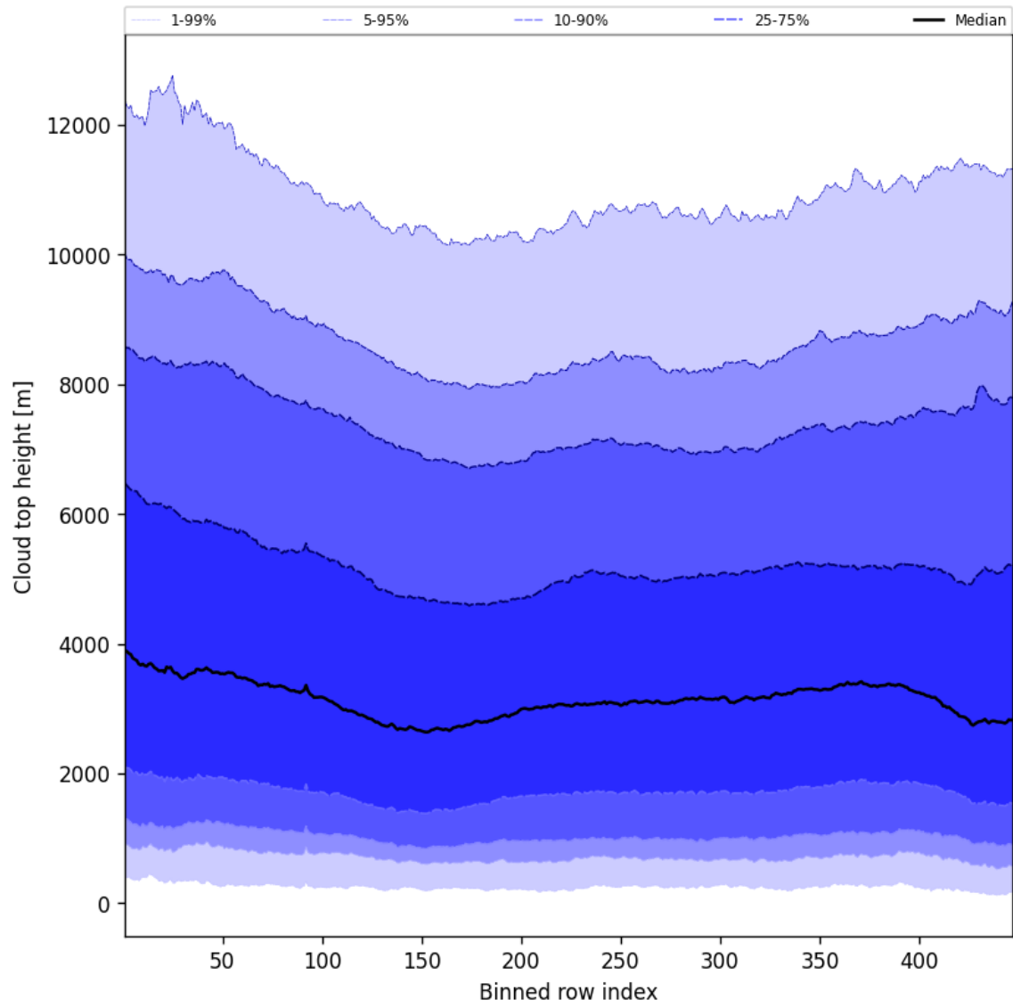
Figure 54: Along track statistics of “Cloud top height” for 2025-09-04 to 2025-09-05
