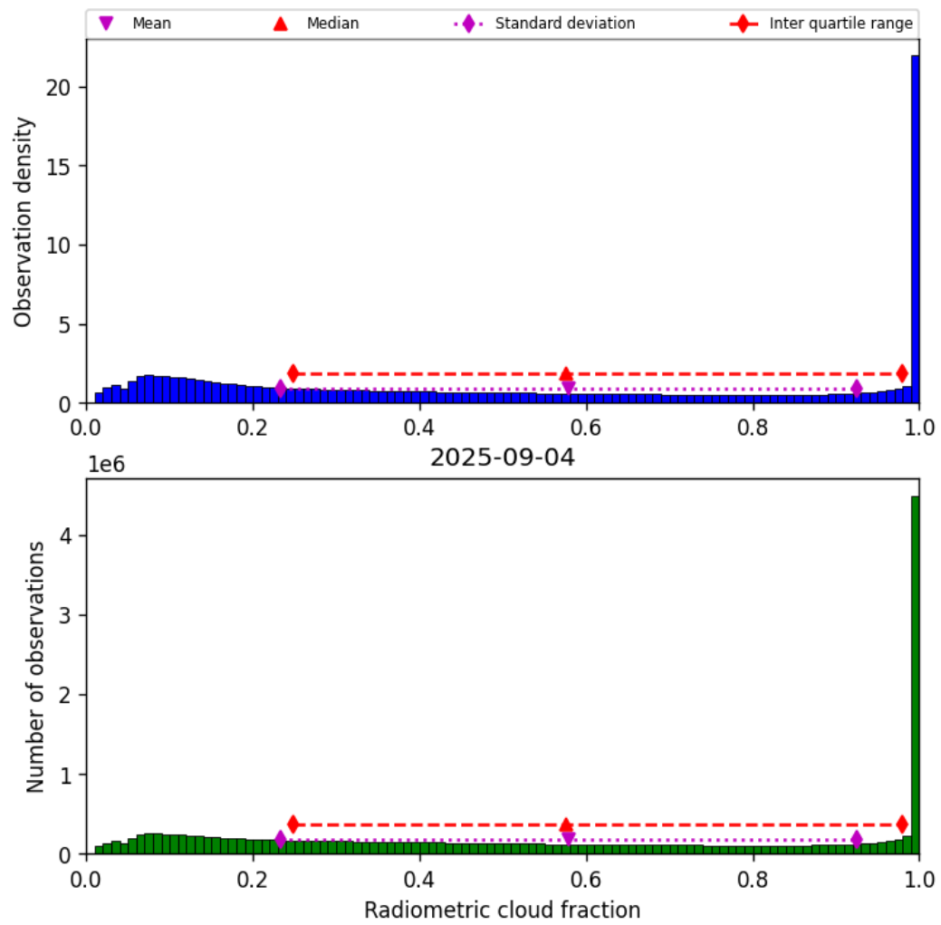
Figure 37: Histogram of “Radiometric cloud fraction” for 2025-09-04 to 2025-09-05
