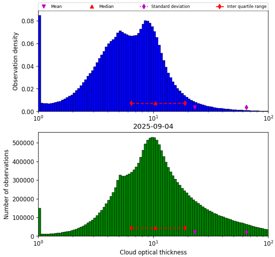
Figure 39: Histogram of “Cloud optical thickness” for 2025-09-04 to 2025-09-05
