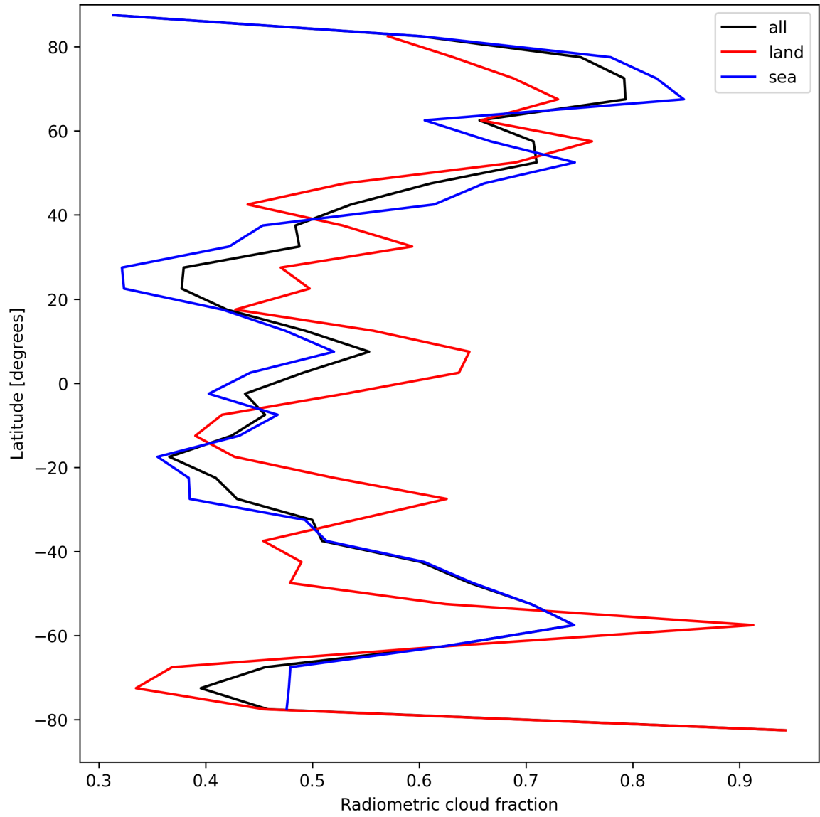
Figure 21: Zonal average of “Radiometric cloud fraction” for 2025-09-04 to 2025-09-05.
