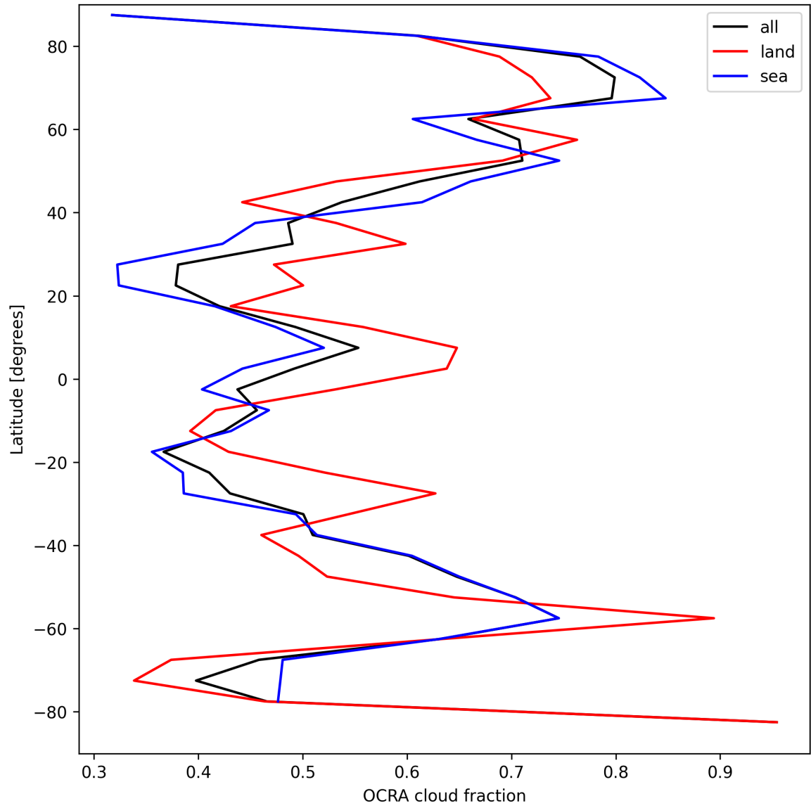
Figure 32: Zonal average of “OCRA cloud fraction” for 2025-09-04 to 2025-09-05.
