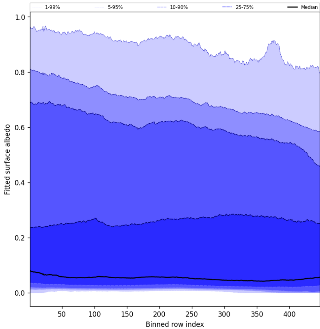
Figure 59: Along track statistics of “Fitted surface albedo” for 2025-09-04 to 2025-09-05
