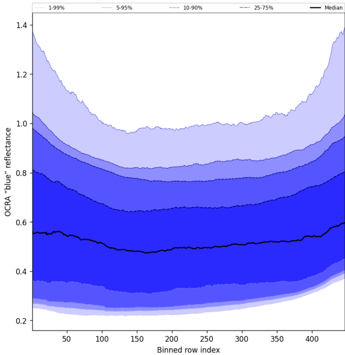
Figure 65: Along track statistics of “OCRA “blue” reflectance” for 2025-09-04 to 2025-09-05
