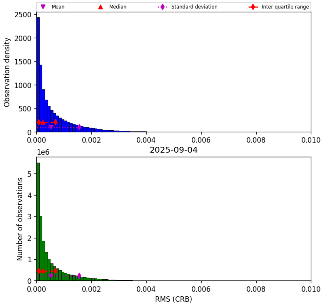
Figure 46: Histogram of "RMS (CRB)" for 2025-09-04 to 2025-09-05
