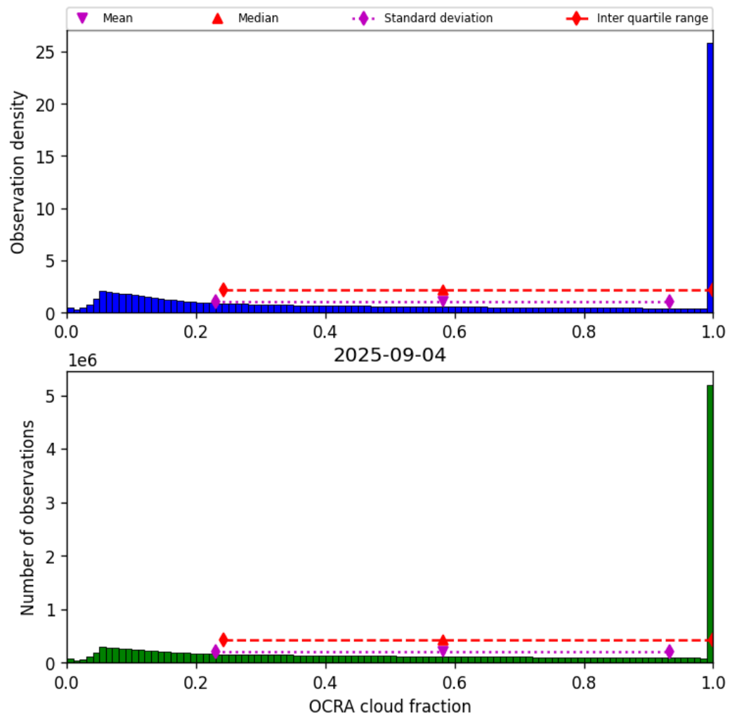
Figure 48: Histogram of “OCRA cloud fraction” for 2025-09-04 to 2025-09-05
