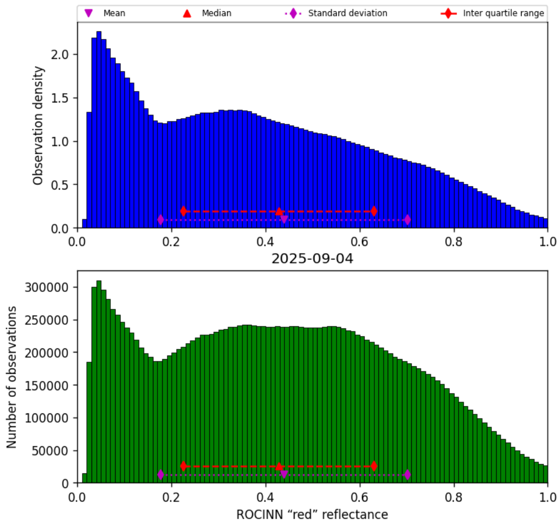
Figure 51: Histogram of “ROCINN “red” reflectance” for 2025-09-04 to 2025-09-05
