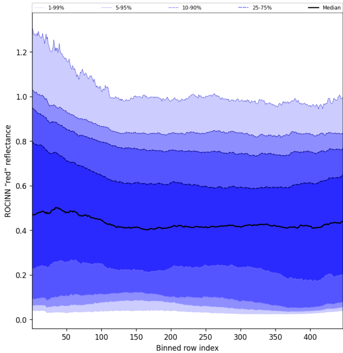
Figure 67: Along track statistics of "ROCINN "red" reflectance" for 2025-09-04 to 2025-09-05
