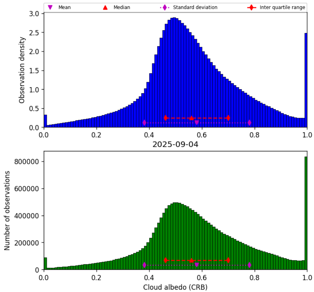
Figure 42: Histogram of “Cloud albedo (CRB)” for 2025-09-04 to 2025-09-05
