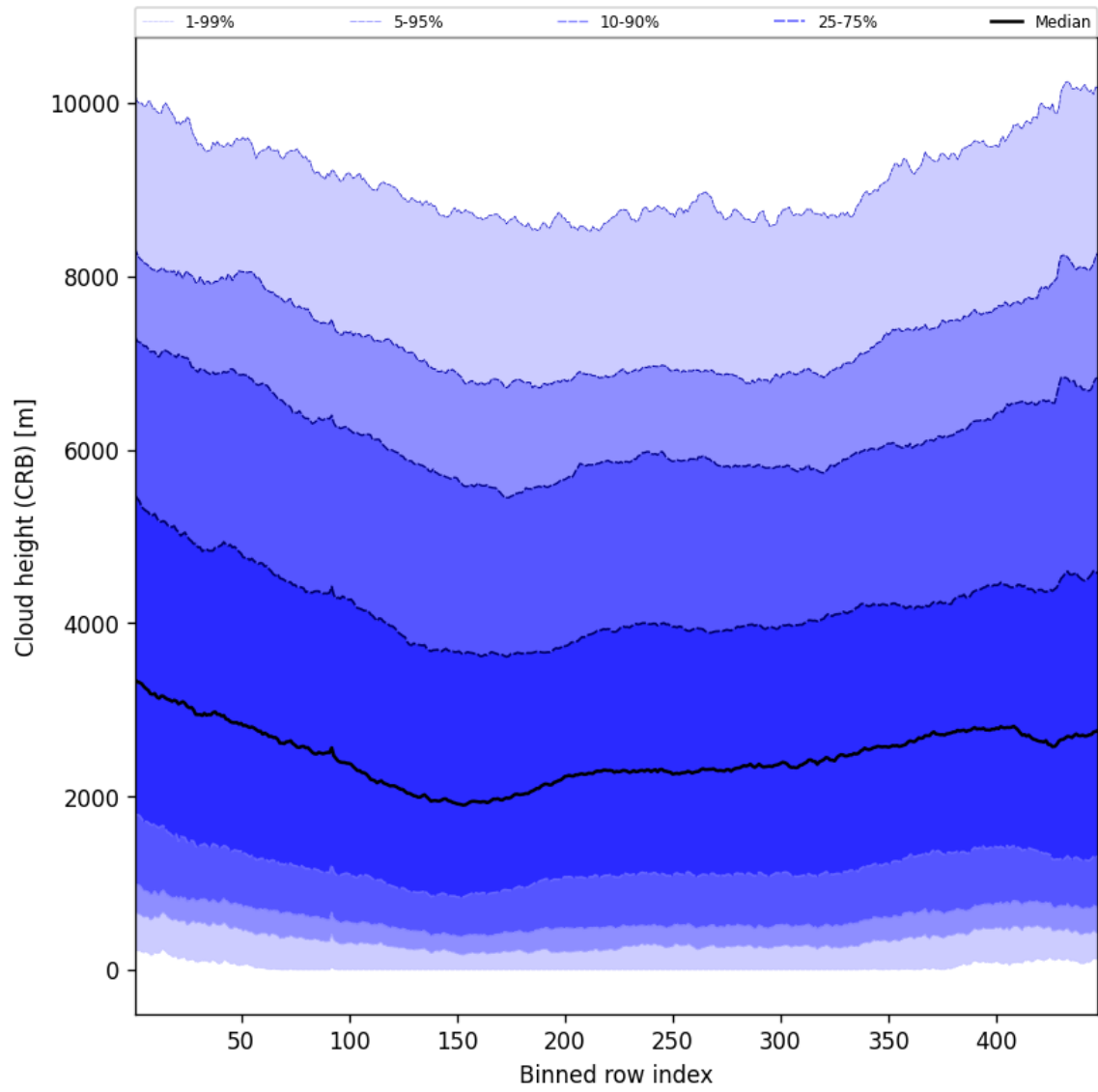
Figure 57: Along track statistics of “Cloud height (CRB)” for 2025-09-04 to 2025-09-05
