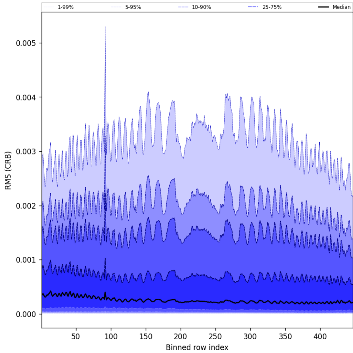
Figure 62: Along track statistics of “RMS (CRB)” for 2025-09-04 to 2025-09-05
