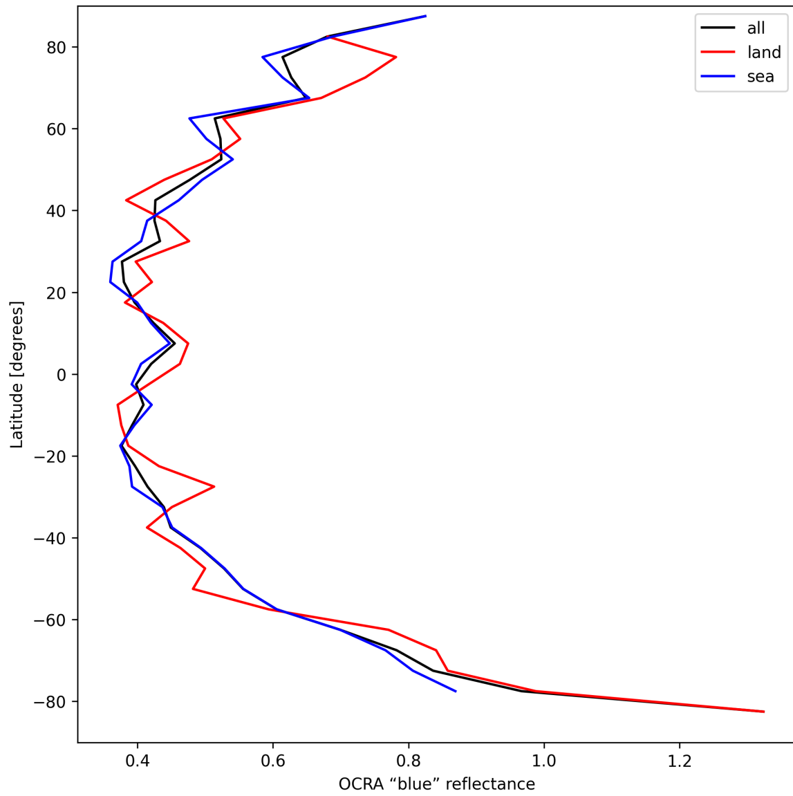
Figure 33: Zonal average of “OCRA “blue” reflectance” for 2025-09-04 to 2025-09-05.
