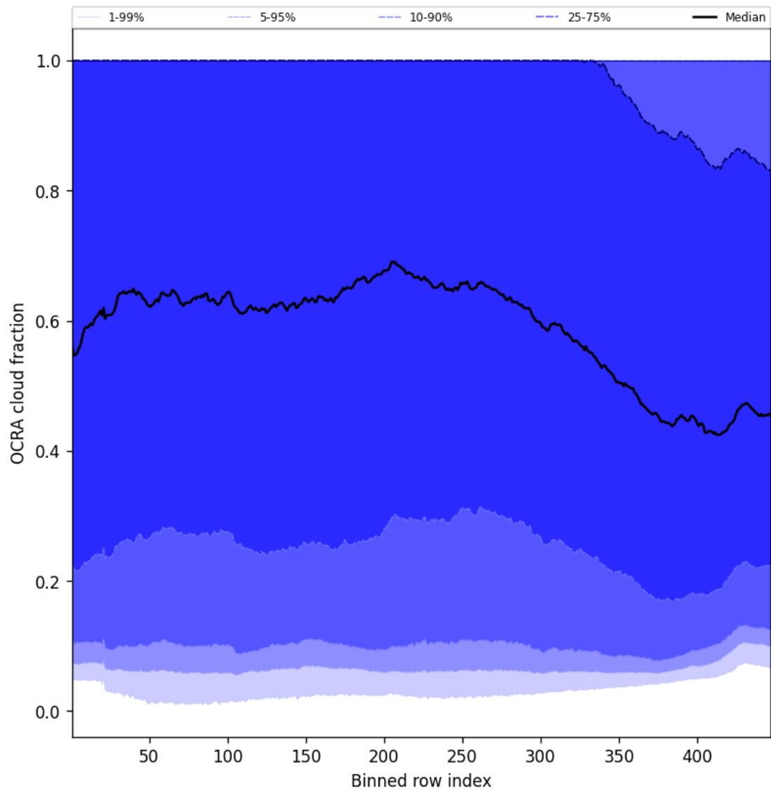
Figure 64: Along track statistics of “OCRA cloud fraction” for 2025-09-04 to 2025-09-05
