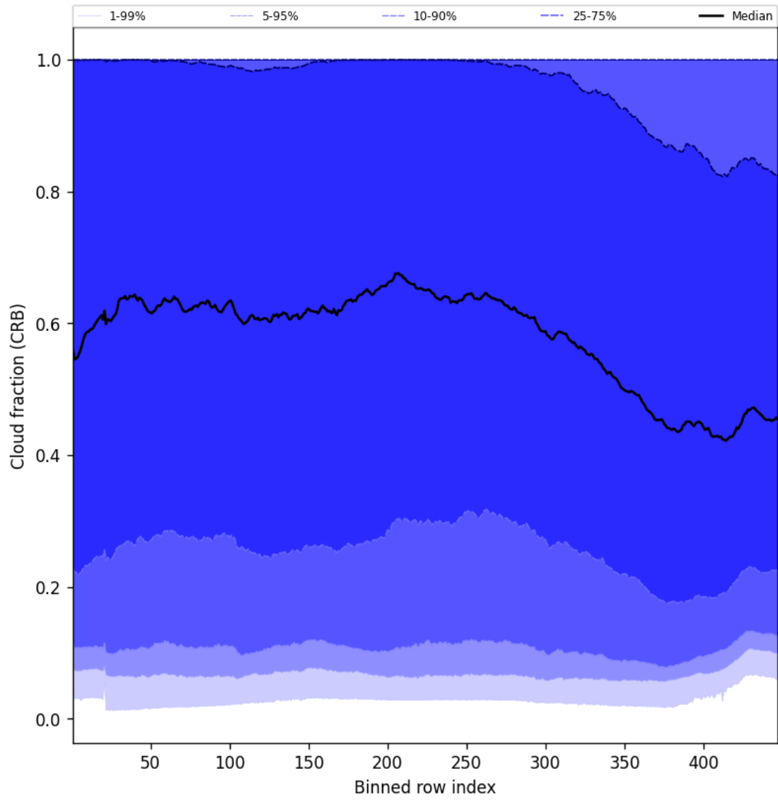
Figure 56: Along track statistics of “Cloud fraction (CRB)” for 2025-09-04 to 2025-09-05
