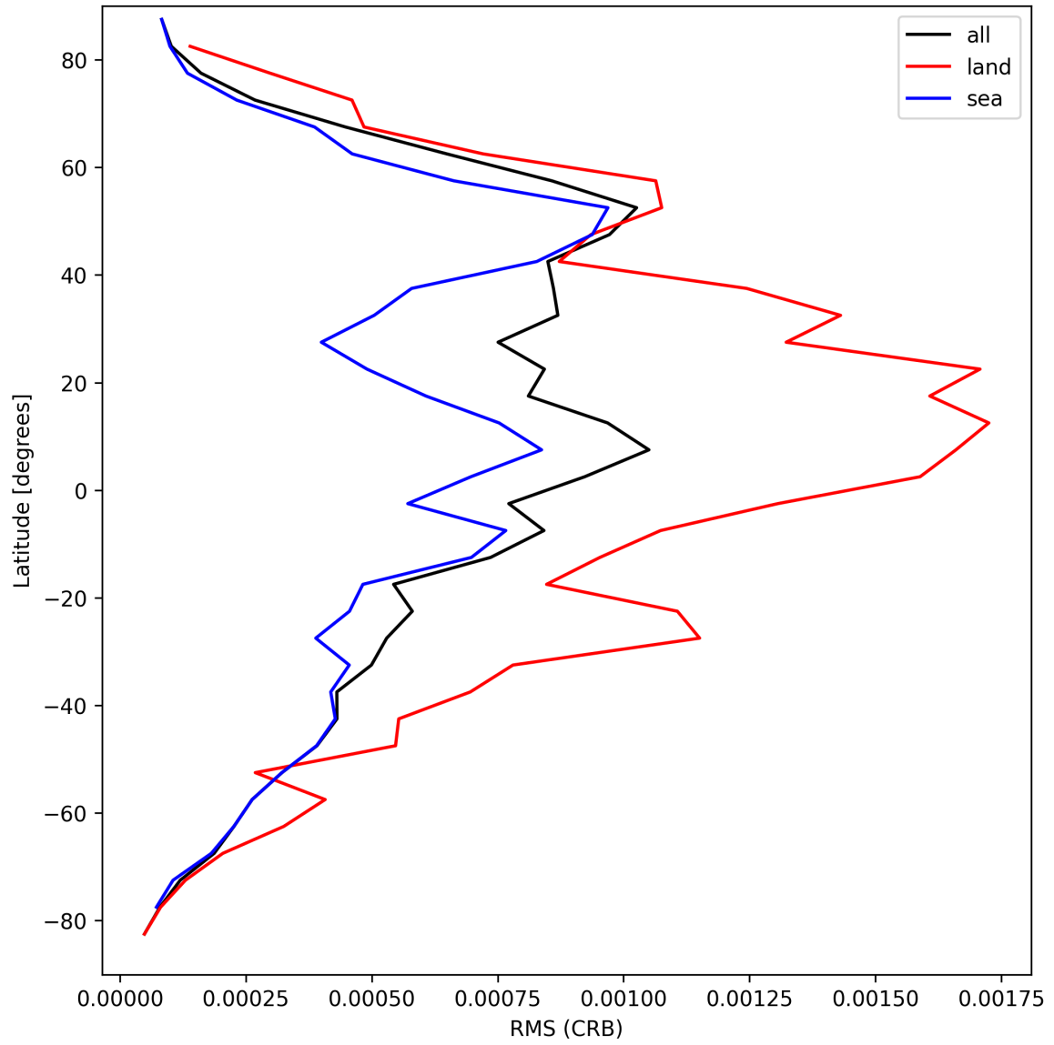
Figure 30: Zonal average of “RMS (CRB)” for 2025-09-04 to 2025-09-05.
