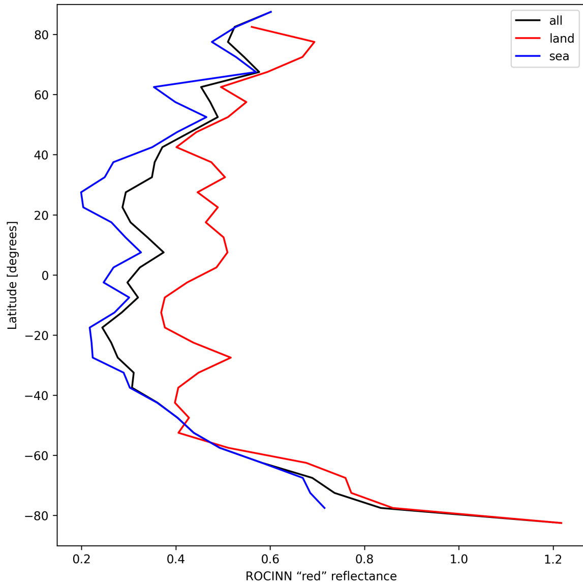
Figure 35: Zonal average of “ROCINN “red” reflectance” for 2025-09-04 to 2025-09-05.
