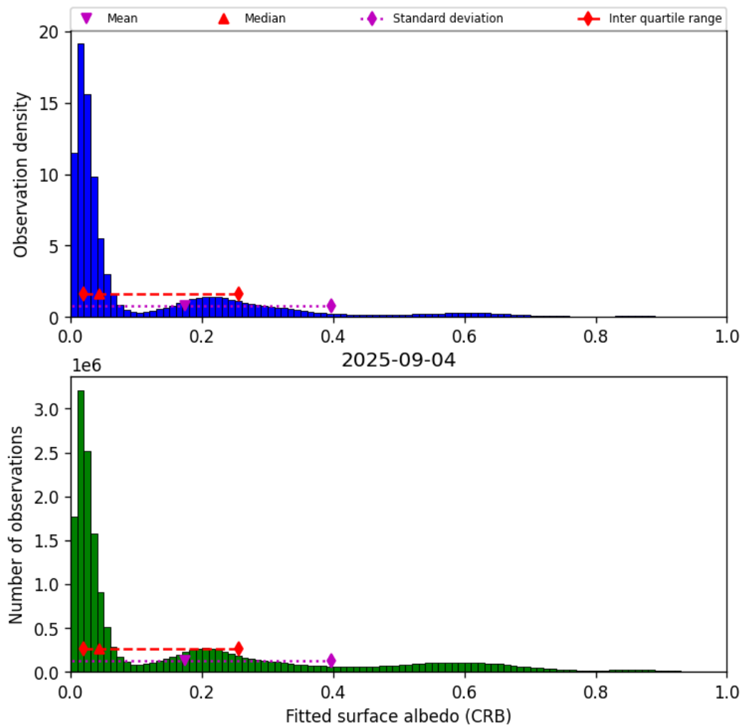
Figure 44: Histogram of “Fitted surface albedo (CRB)” for 2025-09-04 to 2025-09-05
