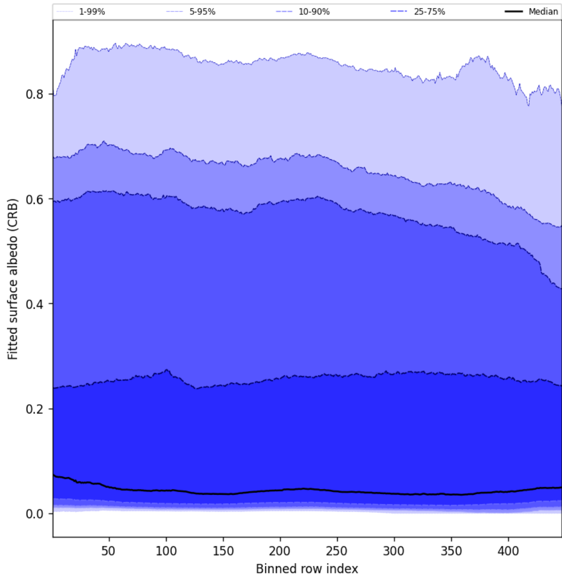
Figure 60: Along track statistics of “Fitted surface albedo (CRB)” for 2025-09-04 to 2025-09-05
