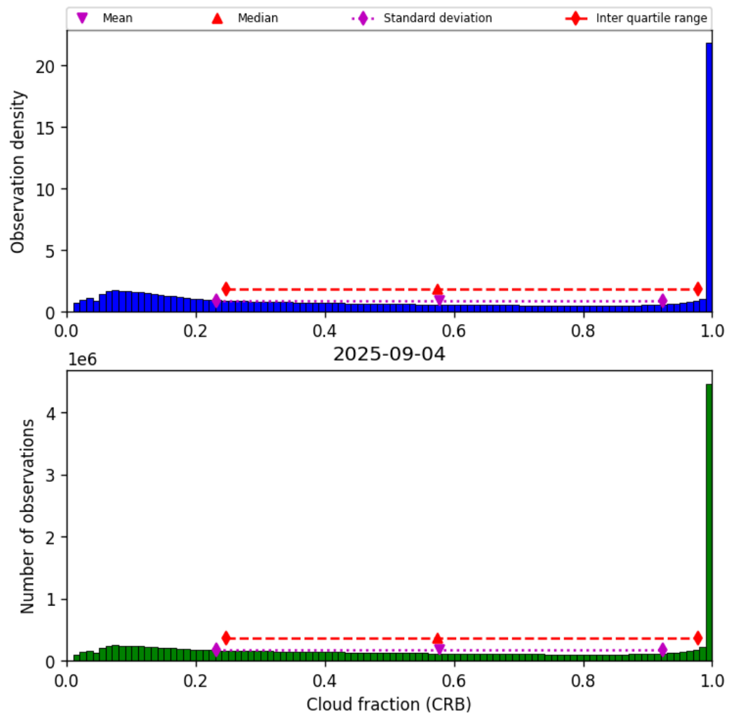
Figure 40: Histogram of “Cloud fraction (CRB)” for 2025-09-04 to 2025-09-05
