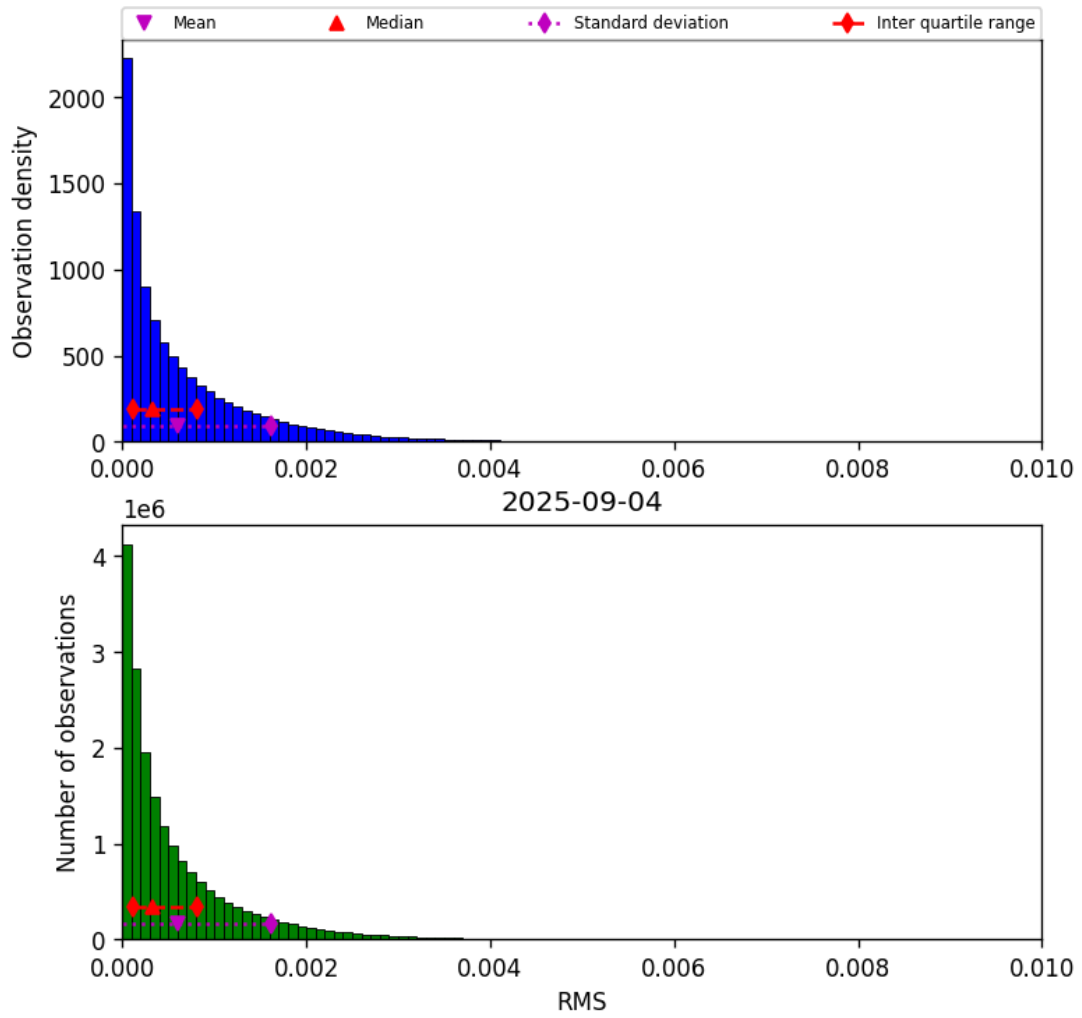
Figure 45: Histogram of “RMS” for 2025-09-04 to 2025-09-05
