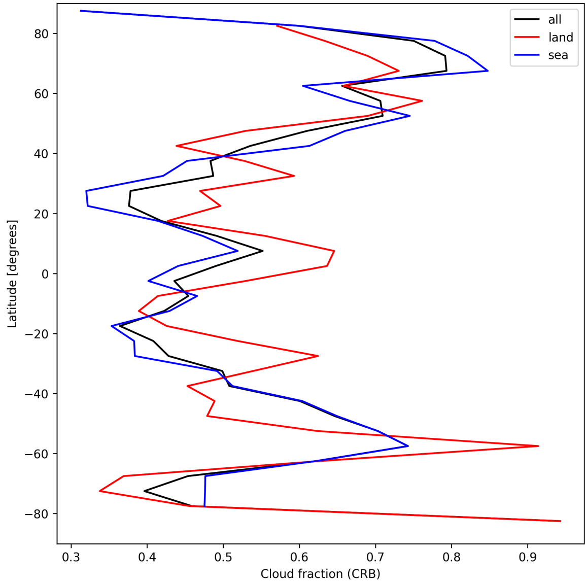
Figure 24: Zonal average of “Cloud fraction (CRB)” for 2025-09-04 to 2025-09-05.
