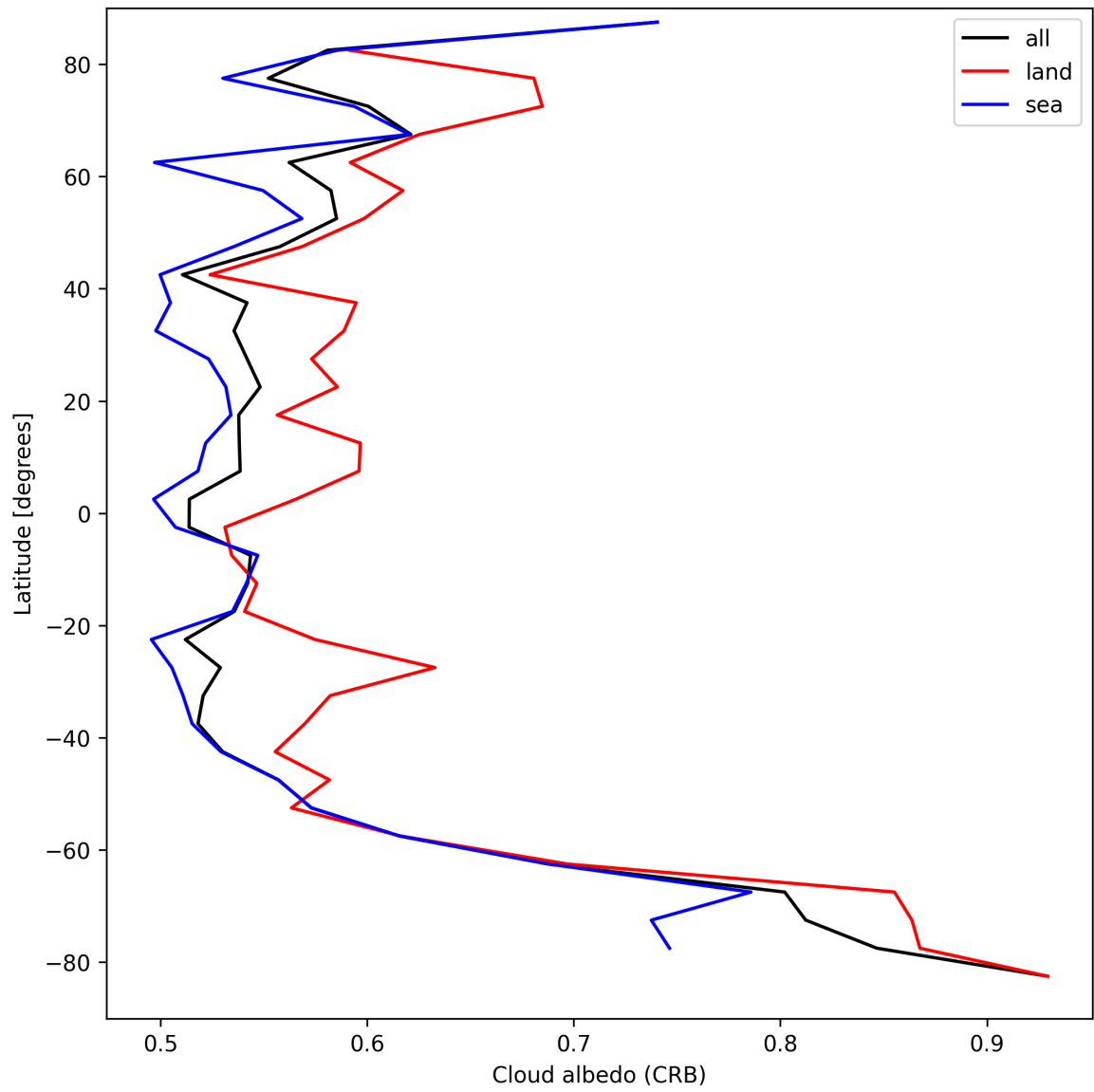
Figure 26: Zonal average of “Cloud albedo (CRB)” for 2025-09-04 to 2025-09-05.
