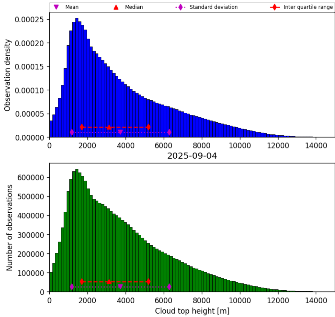
Figure 38: Histogram of “Cloud top height” for 2025-09-04 to 2025-09-05
