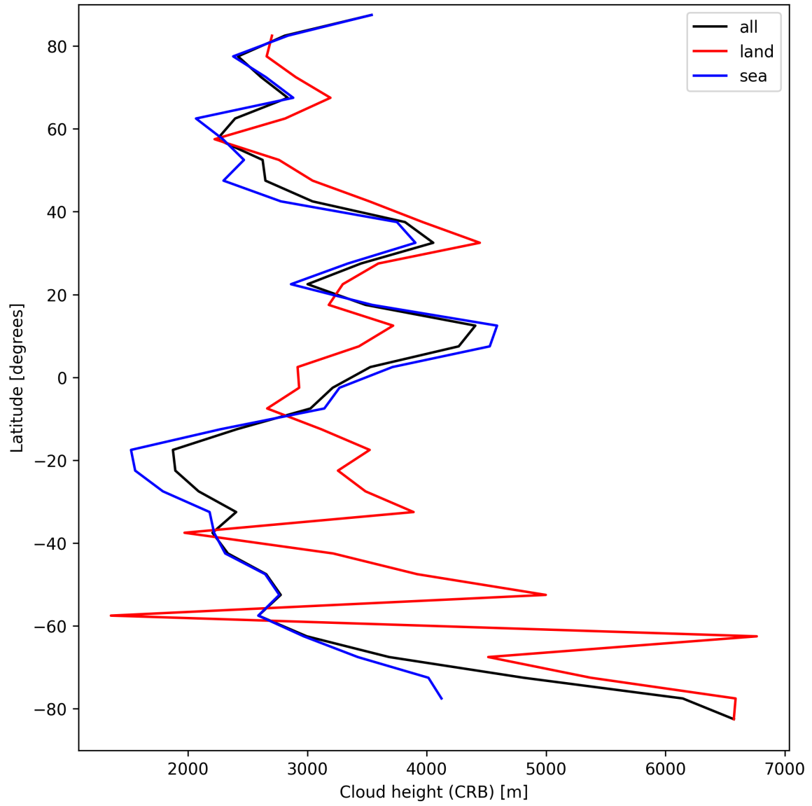
Figure 25: Zonal average of “Cloud height (CRB)” for 2025-09-04 to 2025-09-05.
