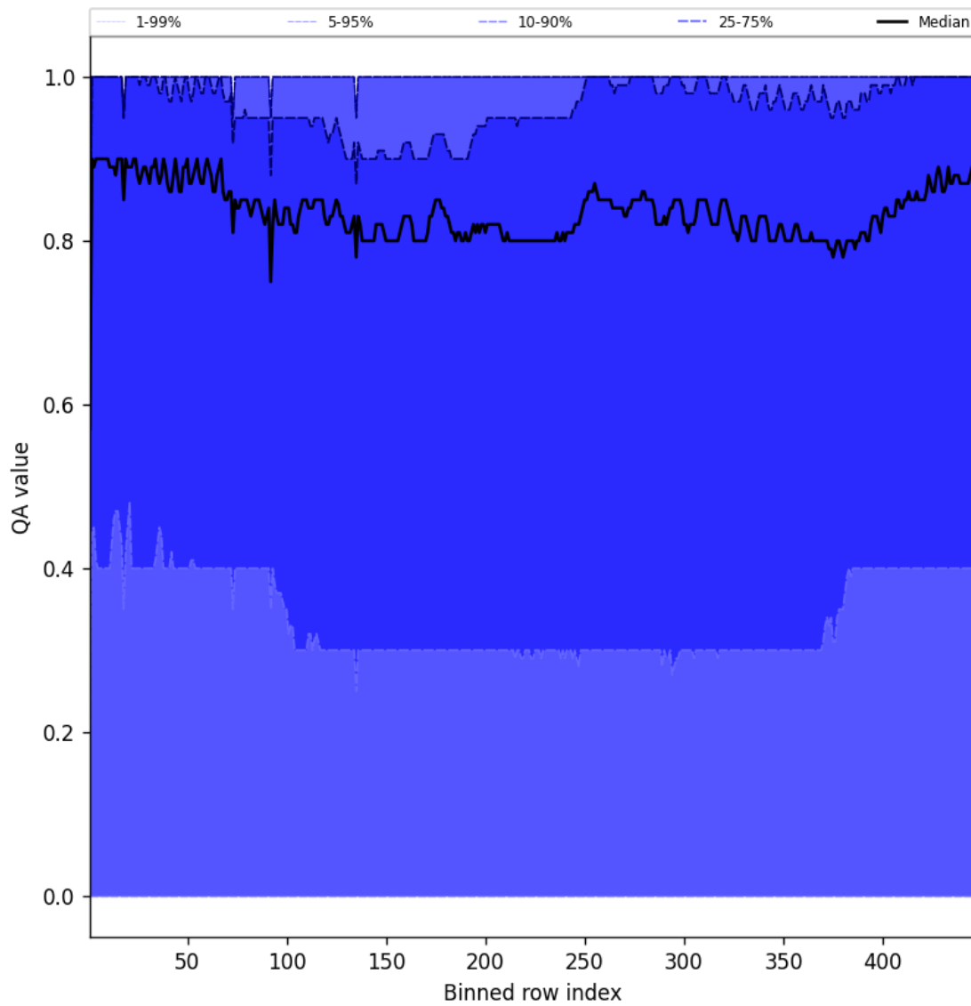
Figure 52: Along track statistics of “QA value” for 2025-09-04 to 2025-09-05
