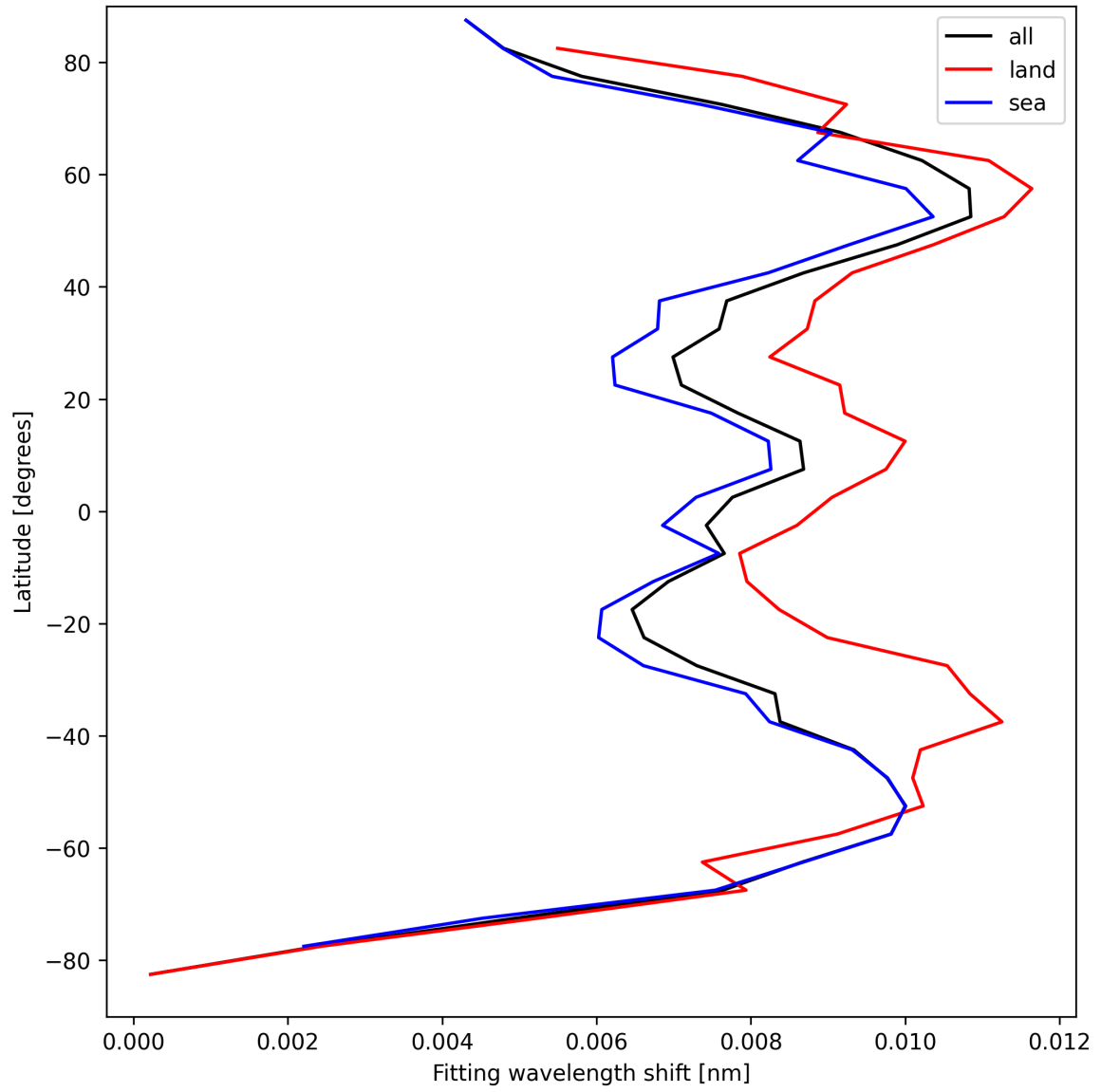
Figure 31: Zonal average of “Fitting wavelength shift” for 2025-09-04 to 2025-09-05.
