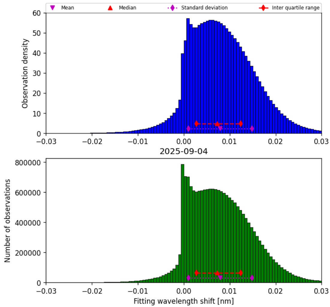
Figure 47: Histogram of “Fitting wavelength shift” for 2025-09-04 to 2025-09-05
