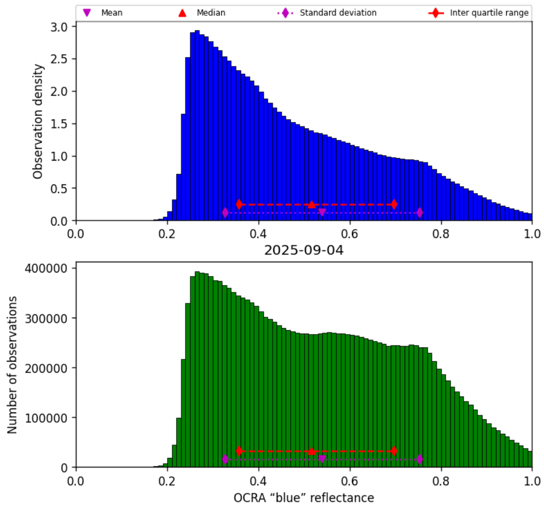
Figure 49: Histogram of “OCRA “blue” reflectance” for 2025-09-04 to 2025-09-05
