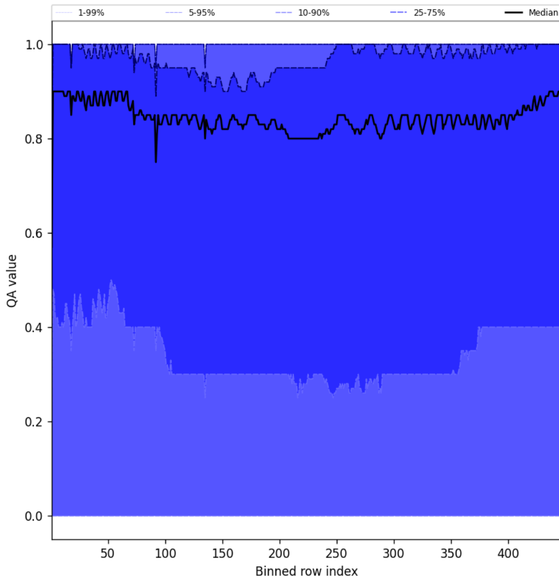
Figure 52: Along track statistics of “QA value” for 2025-09-05 to 2025-09-06
