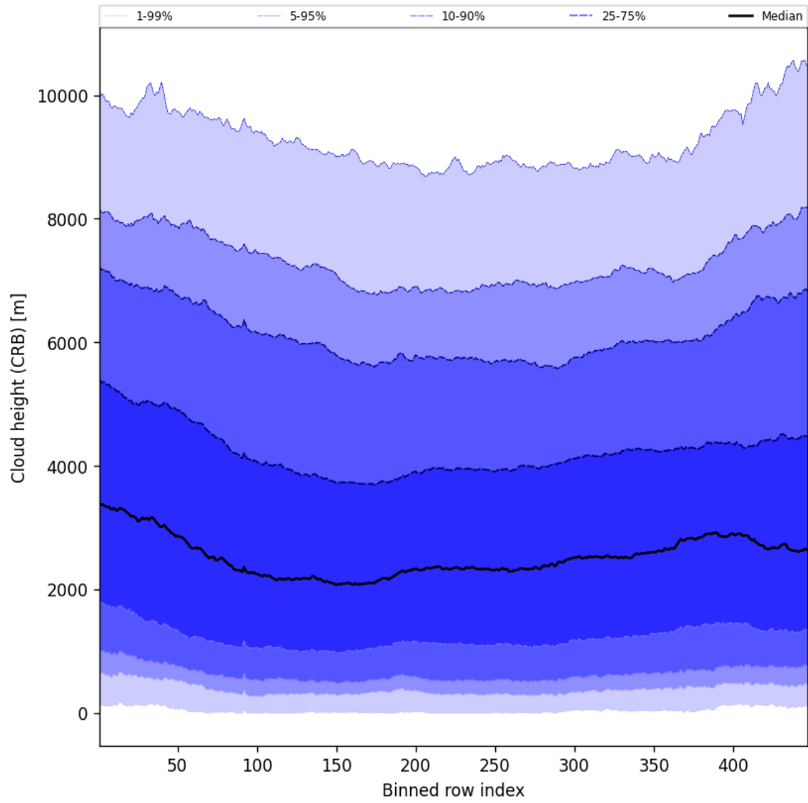
Figure 57: Along track statistics of “Cloud height (CRB)” for 2025-09-05 to 2025-09-06
