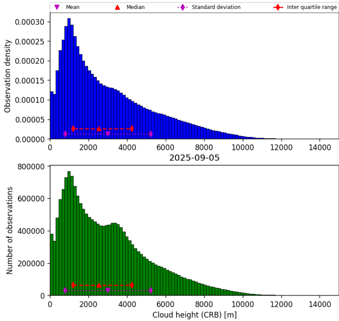
Figure 41: Histogram of “Cloud height (CRB)” for 2025-09-05 to 2025-09-06
