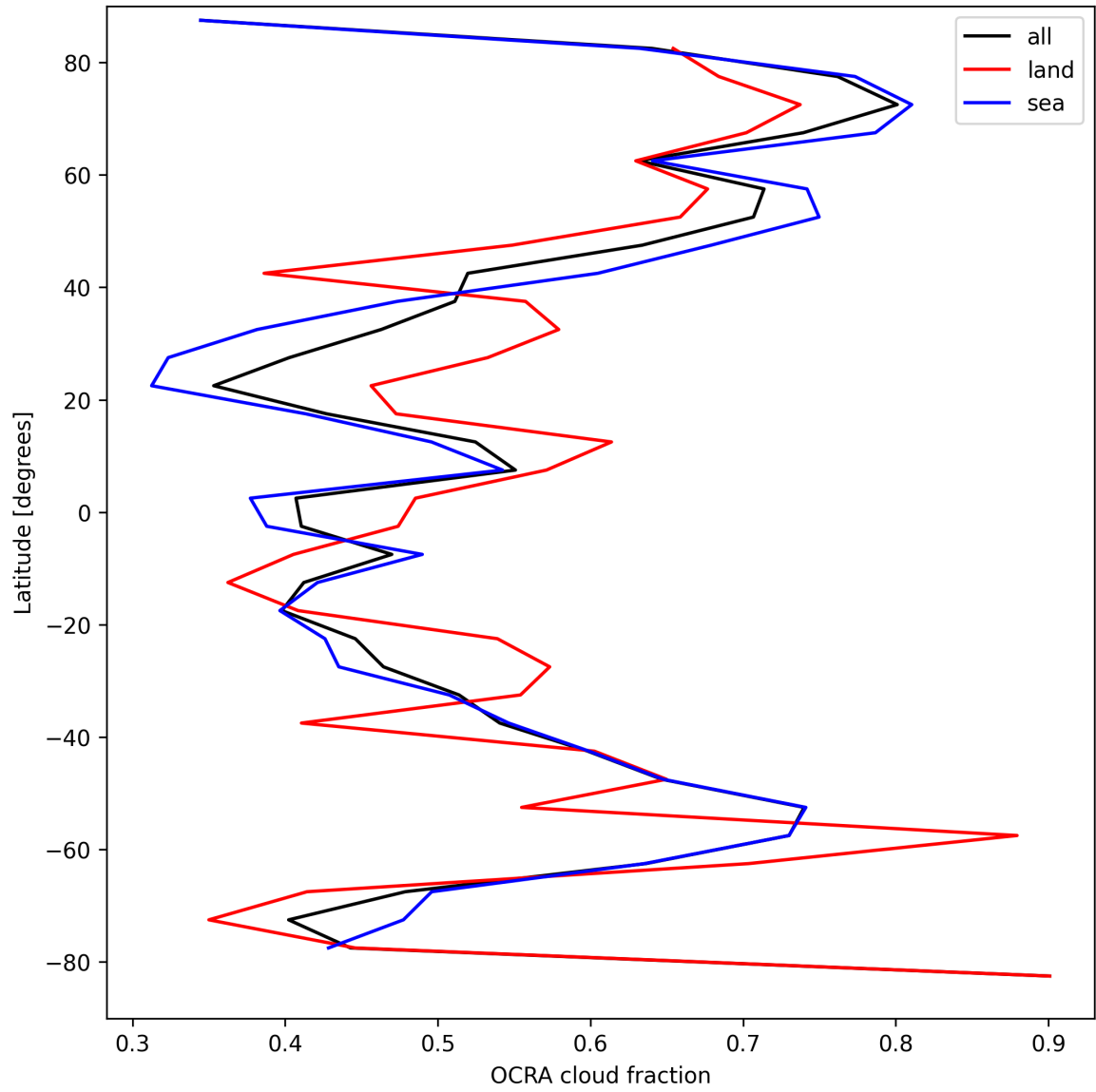
Figure 32: Zonal average of “OCRA cloud fraction” for 2025-09-05 to 2025-09-06.
