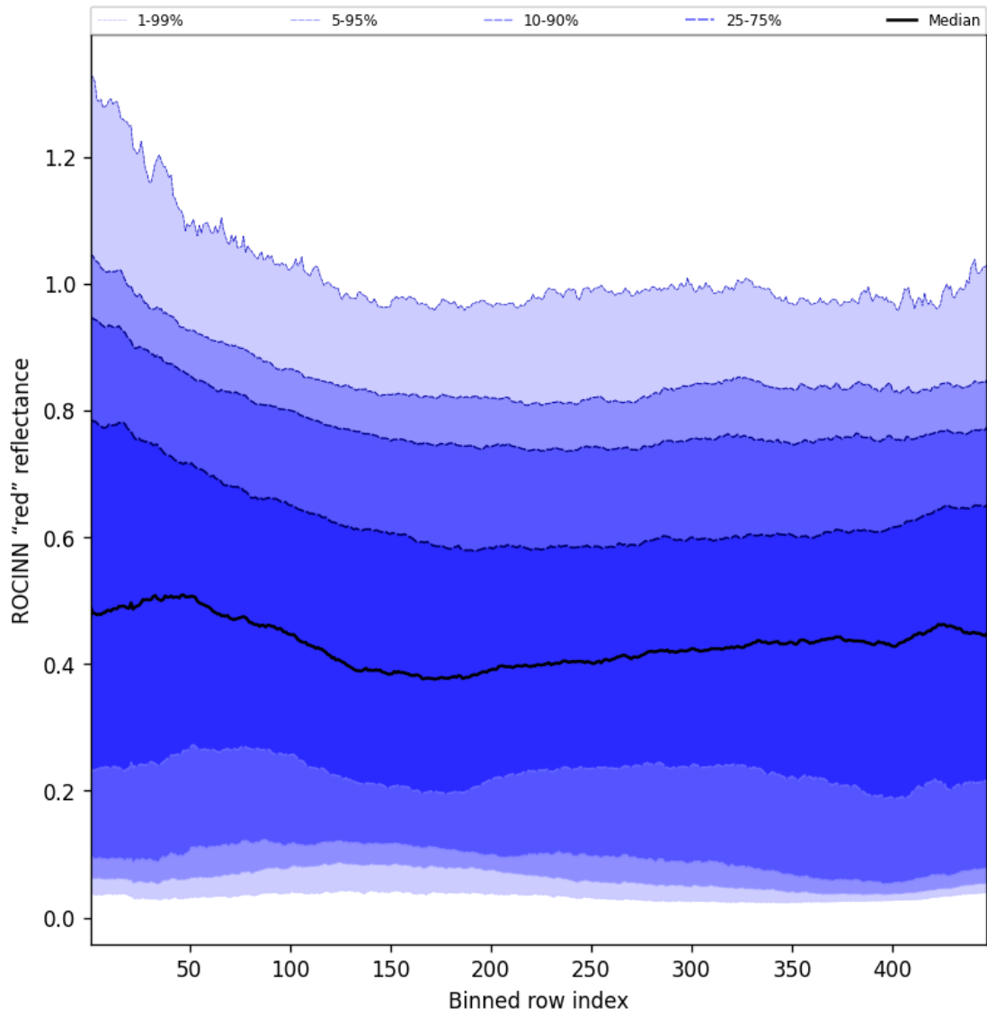
Figure 67: Along track statistics of "ROCINN "red" reflectance" for 2025-09-05 to 2025-09-06
