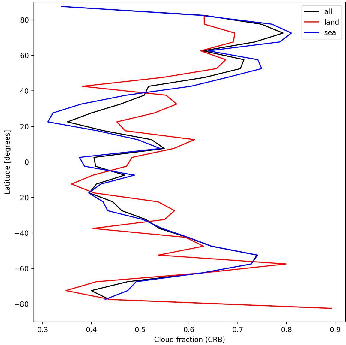
Figure 24: Zonal average of “Cloud fraction (CRB)” for 2025-09-05 to 2025-09-06.
