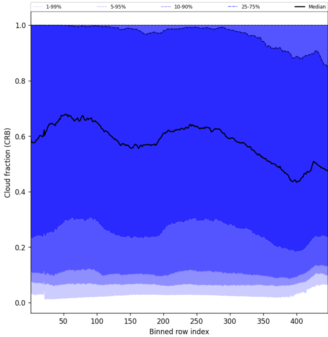
Figure 56: Along track statistics of “Cloud fraction (CRB)” for 2025-09-05 to 2025-09-06
