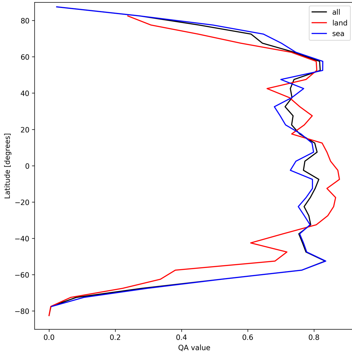
Figure 20: Zonal average of “QA value” for 2025-09-05 to 2025-09-06.
