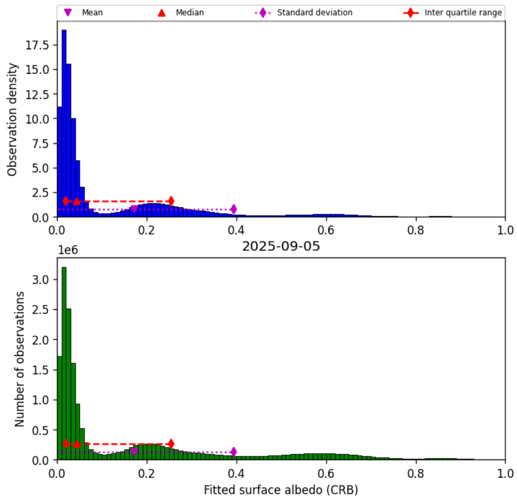
Figure 44: Histogram of “Fitted surface albedo (CRB)” for 2025-09-05 to 2025-09-06
