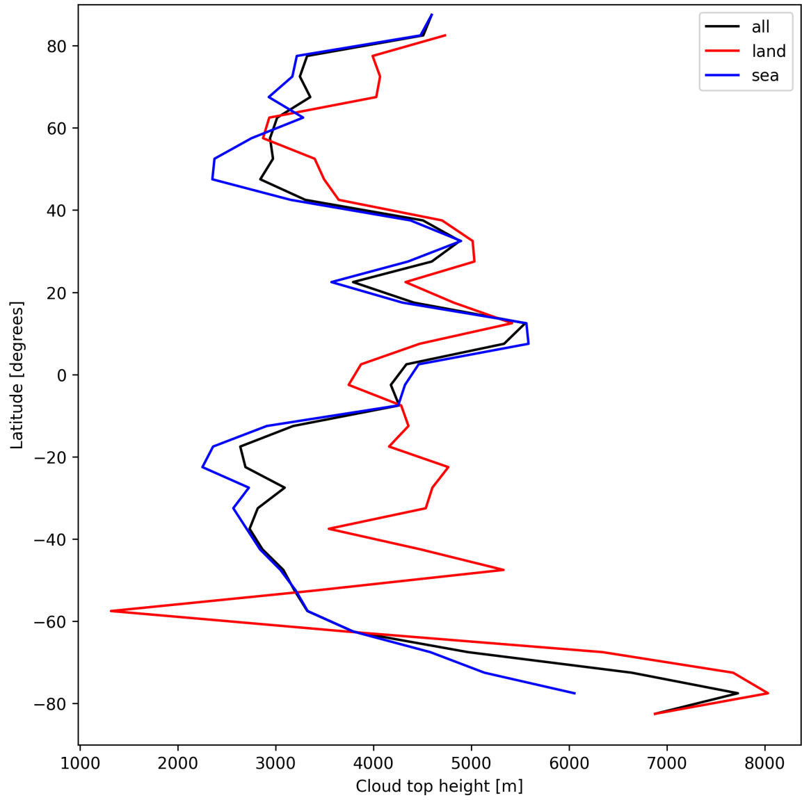
Figure 22: Zonal average of “Cloud top height” for 2025-09-05 to 2025-09-06.
