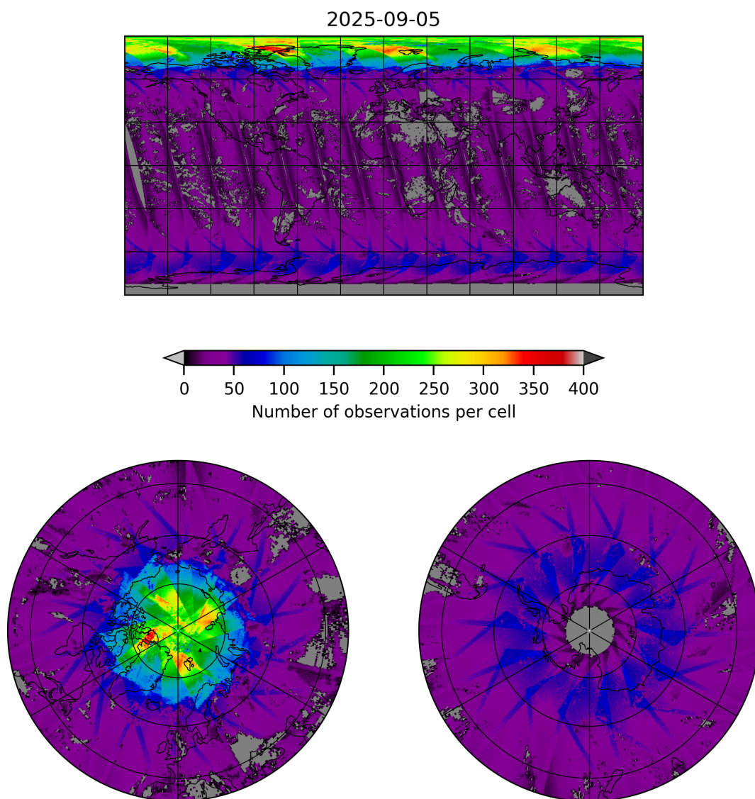
Figure 19: Map of the number of observations for 2025-09-05 to 2025-09-06
