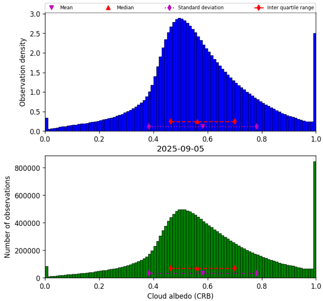
Figure 42: Histogram of “Cloud albedo (CRB)” for 2025-09-05 to 2025-09-06
