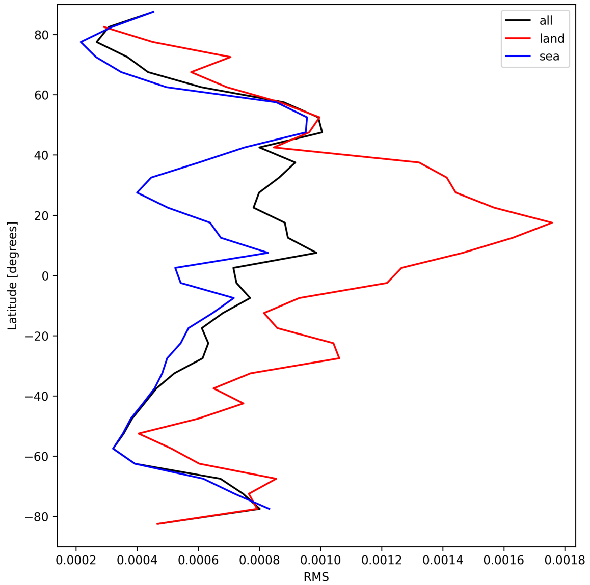
Figure 29: Zonal average of “RMS” for 2025-09-05 to 2025-09-06.
