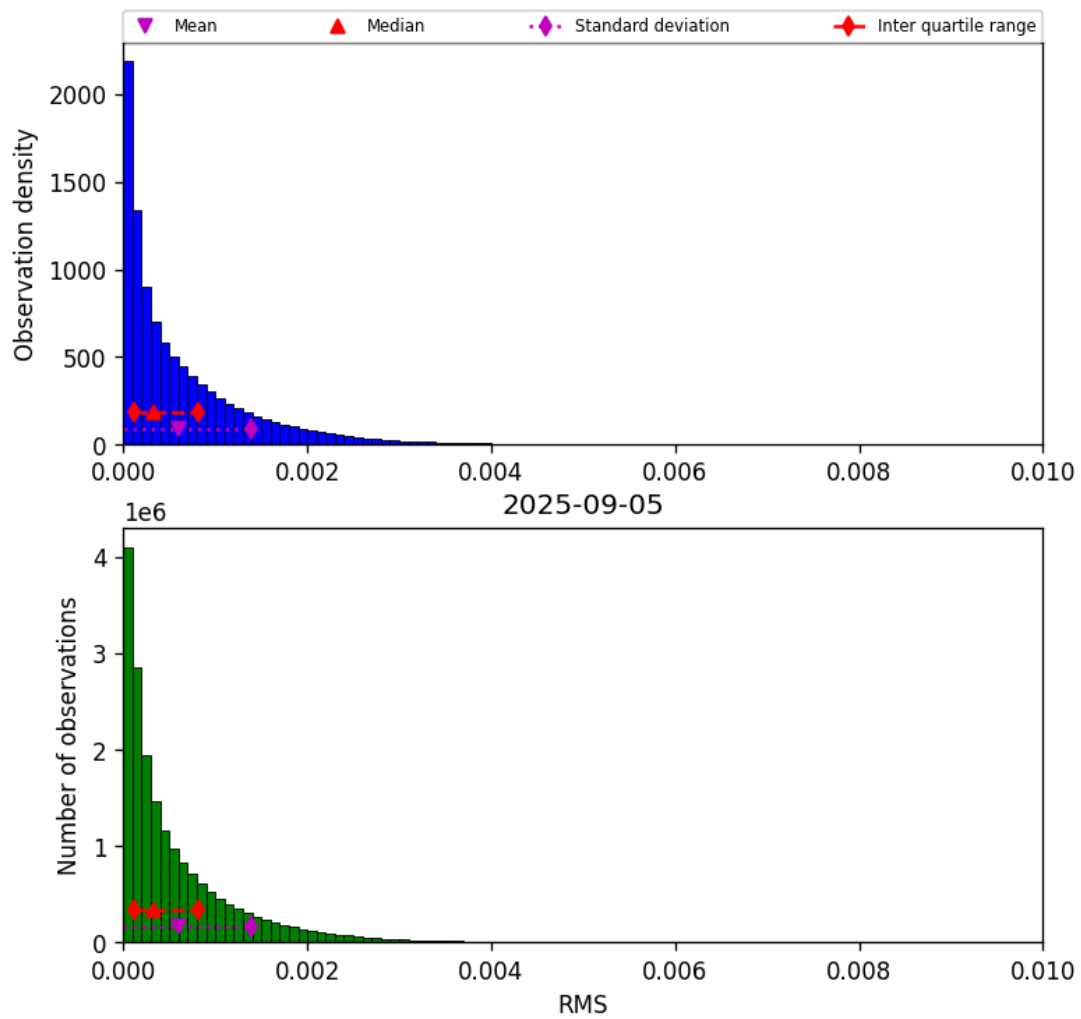
Figure 45: Histogram of “RMS” for 2025-09-05 to 2025-09-06
