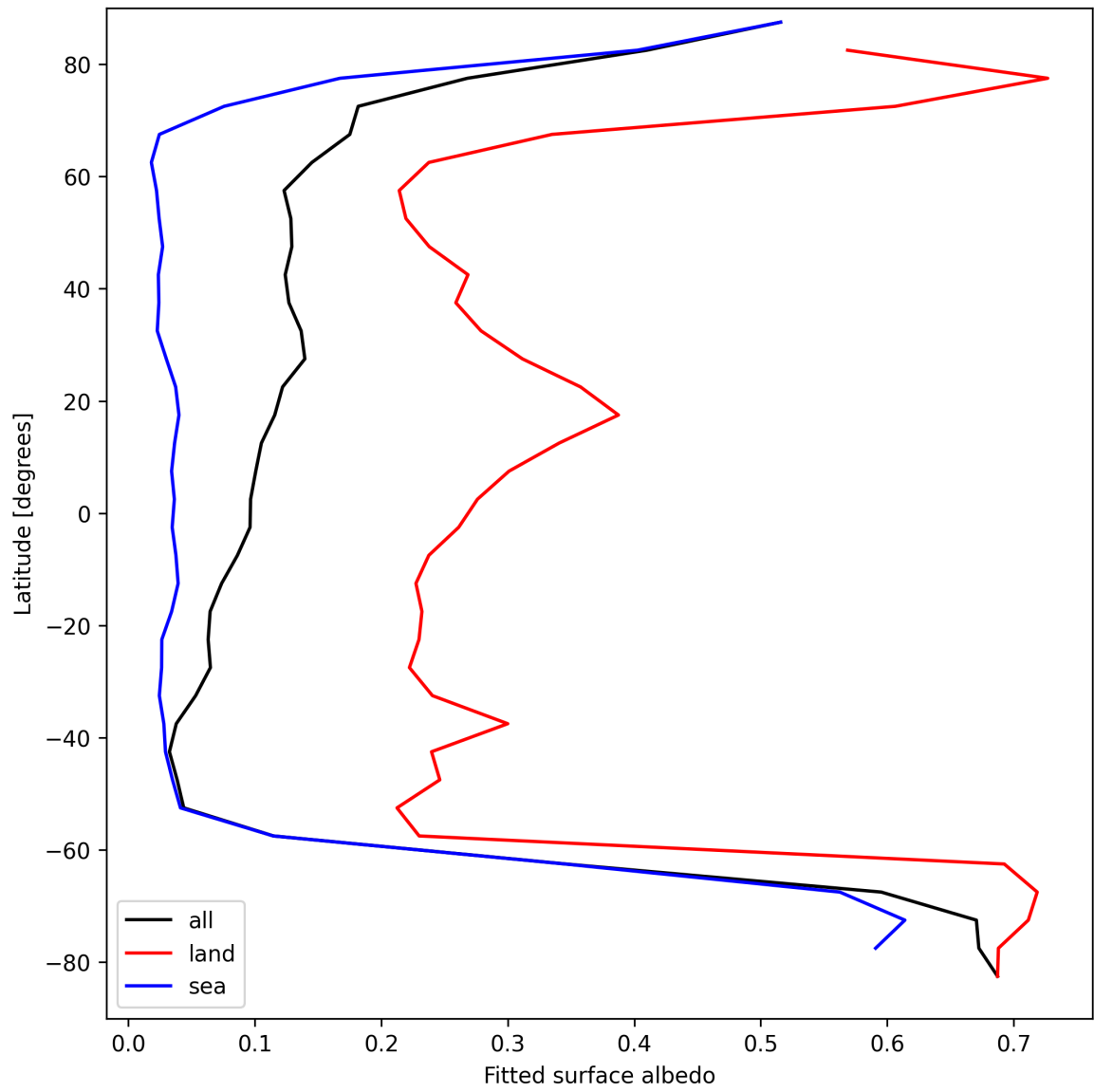
Figure 27: Zonal average of “Fitted surface albedo” for 2025-09-05 to 2025-09-06.
