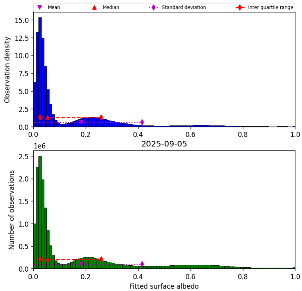
Figure 43: Histogram of “Fitted surface albedo” for 2025-09-05 to 2025-09-06
