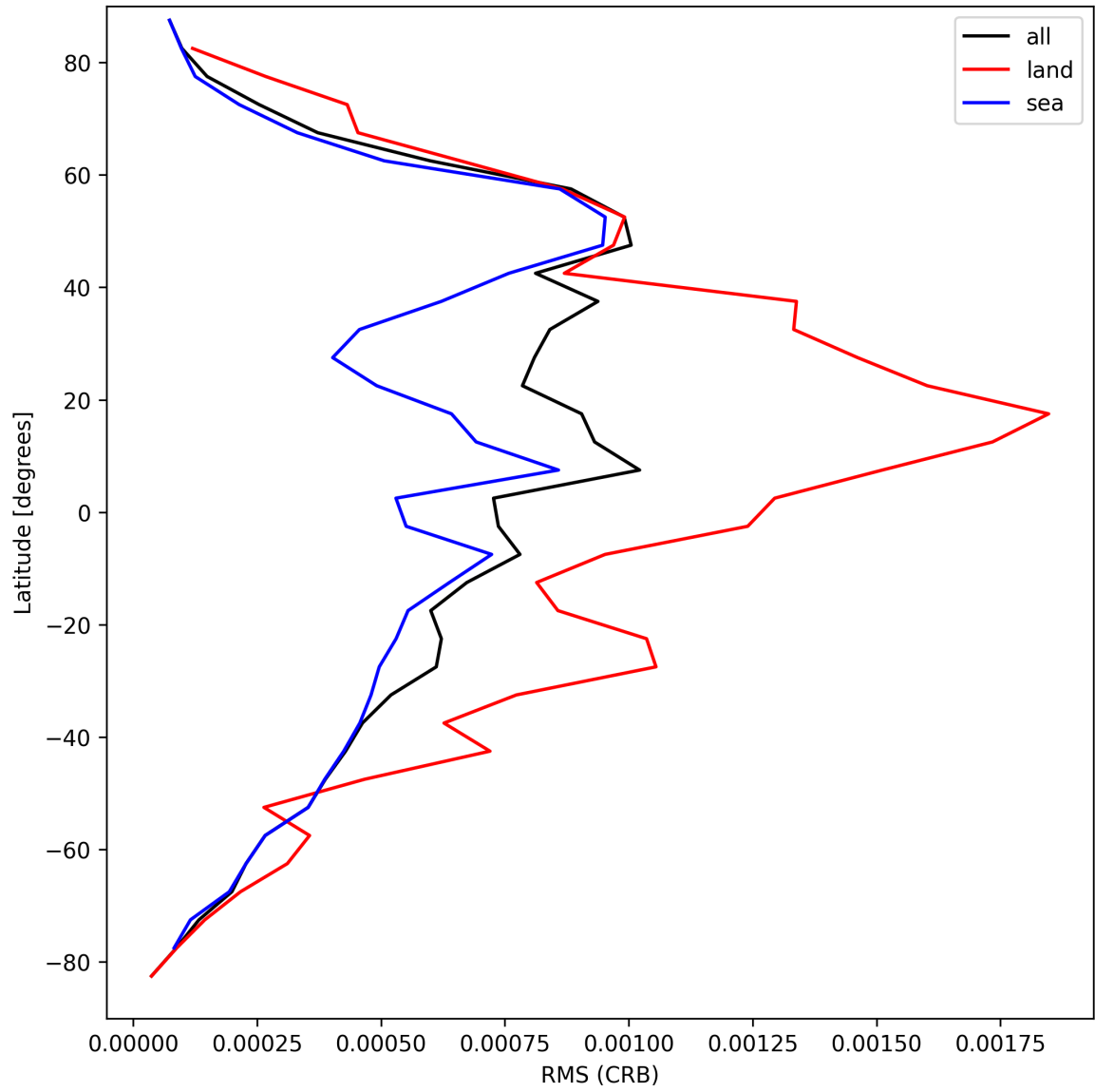
Figure 30: Zonal average of “RMS (CRB)” for 2025-09-05 to 2025-09-06.
