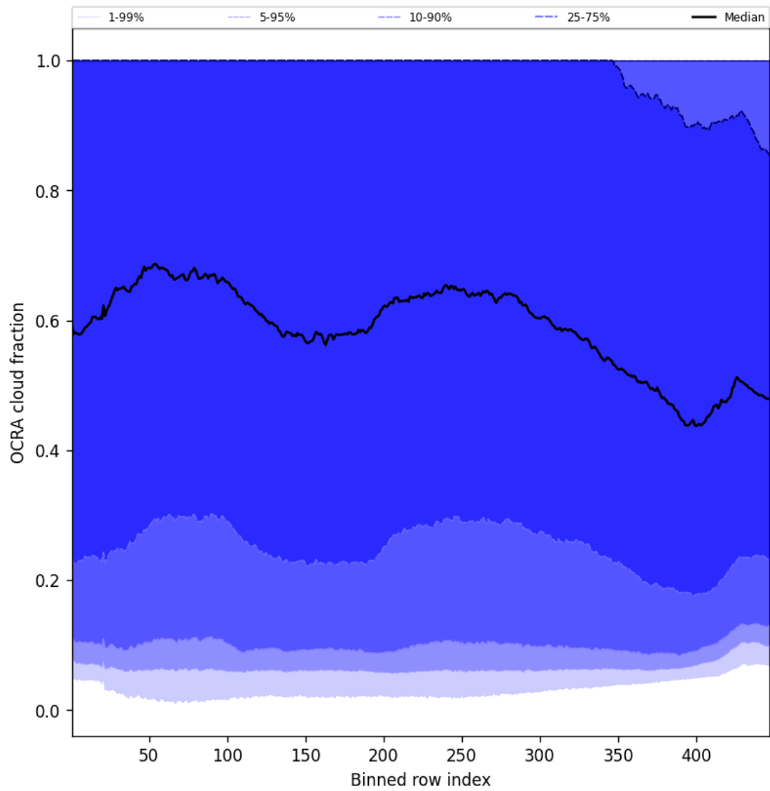
Figure 64: Along track statistics of “OCRA cloud fraction” for 2025-09-05 to 2025-09-06
