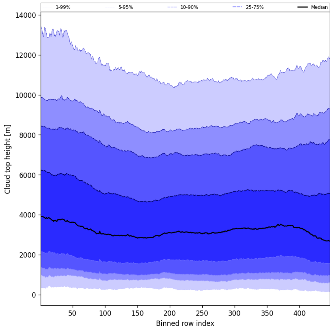
Figure 54: Along track statistics of “Cloud top height” for 2025-09-05 to 2025-09-06
