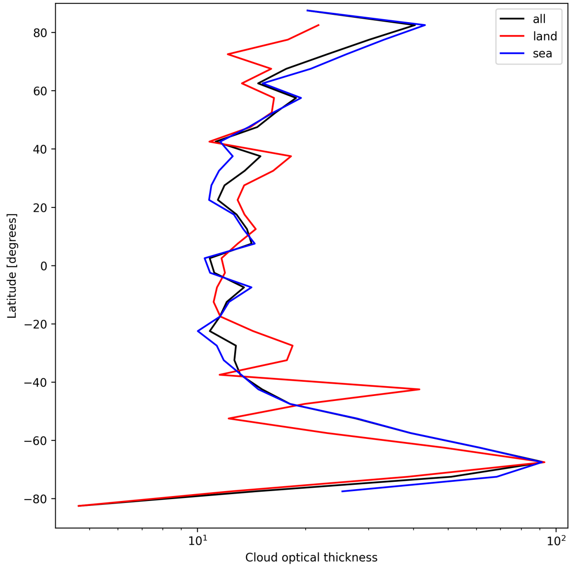
Figure 23: Zonal average of “Cloud optical thickness” for 2025-09-05 to 2025-09-06.
