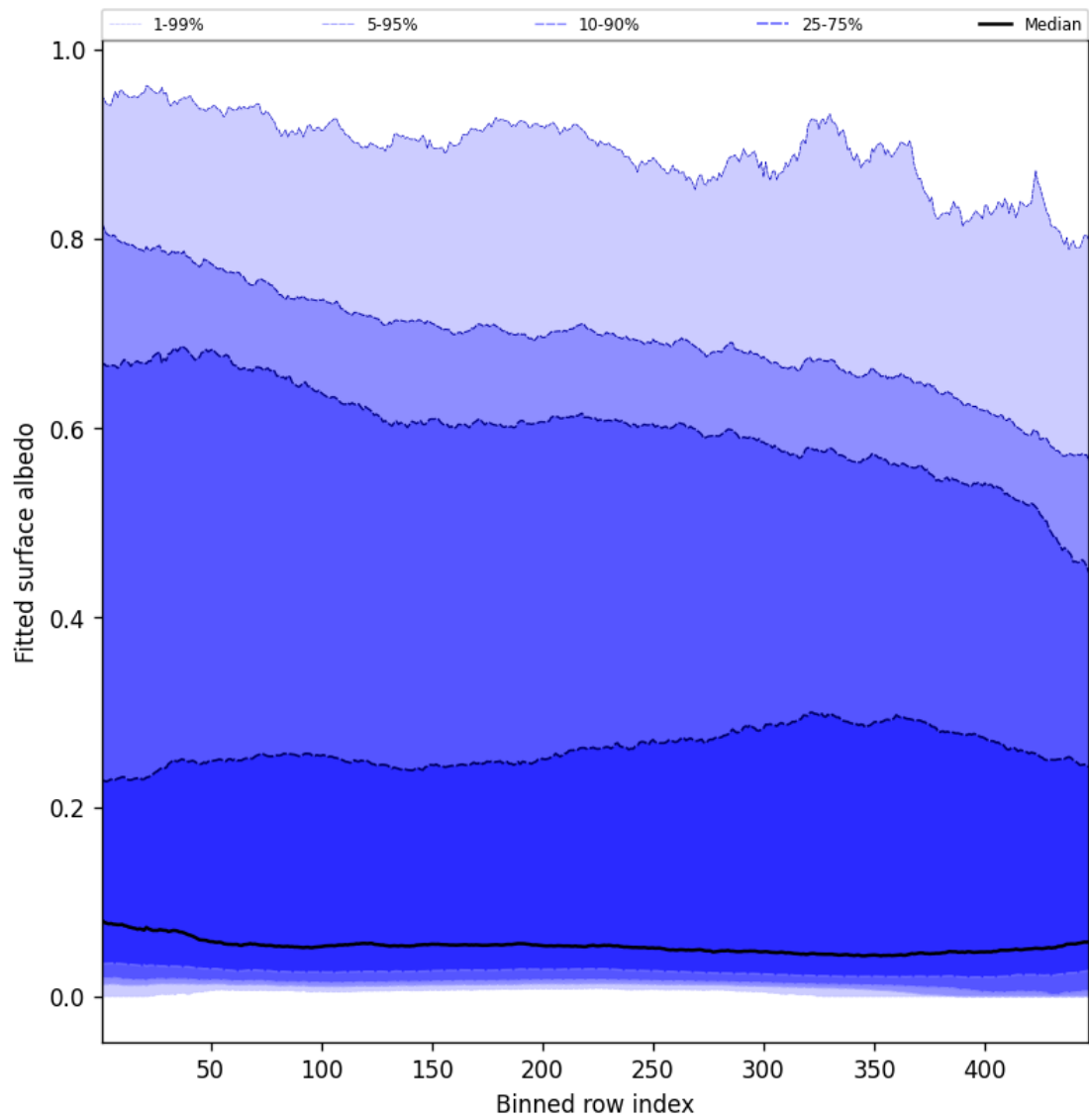
Figure 59: Along track statistics of “Fitted surface albedo” for 2025-09-05 to 2025-09-06
