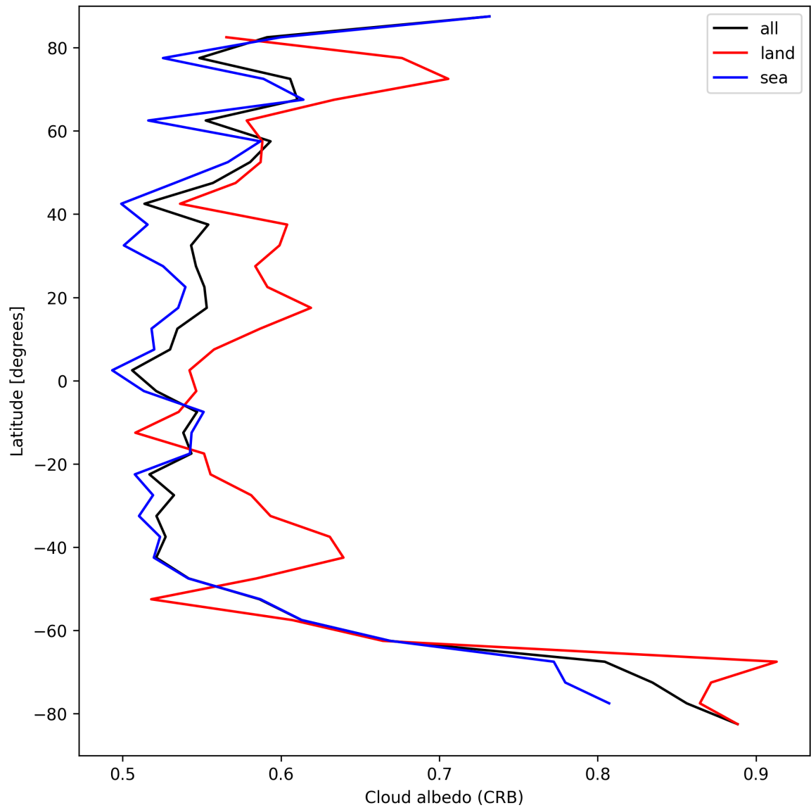
Figure 26: Zonal average of “Cloud albedo (CRB)” for 2025-09-05 to 2025-09-06.
