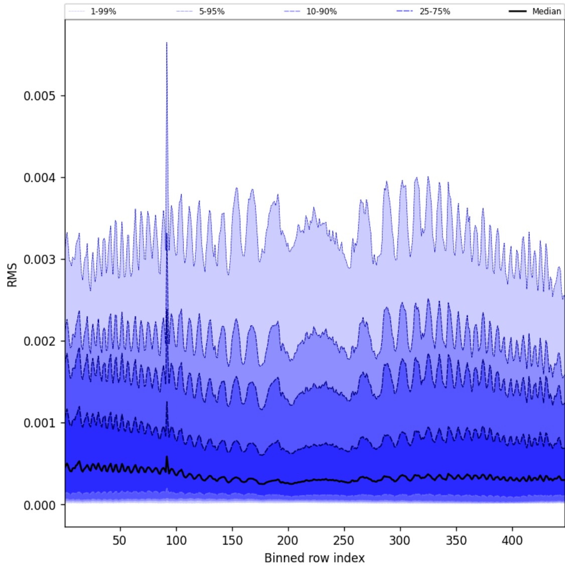
Figure 61: Along track statistics of “RMS” for 2025-09-05 to 2025-09-06
