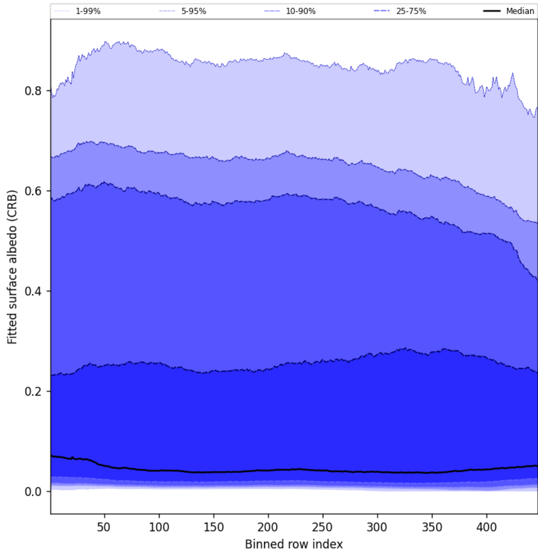
Figure 60: Along track statistics of “Fitted surface albedo (CRB)” for 2025-09-05 to 2025-09-06
