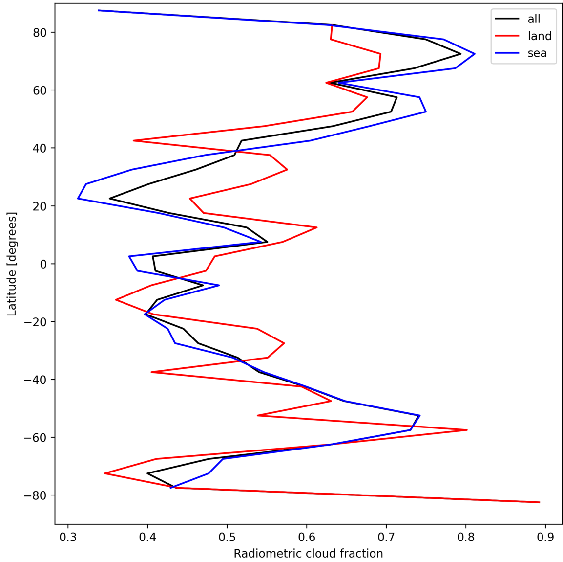
Figure 21: Zonal average of “Radiometric cloud fraction” for 2025-09-05 to 2025-09-06.
