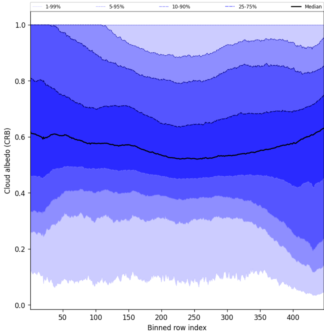
Figure 58: Along track statistics of “Cloud albedo (CRB)” for 2025-09-05 to 2025-09-06
