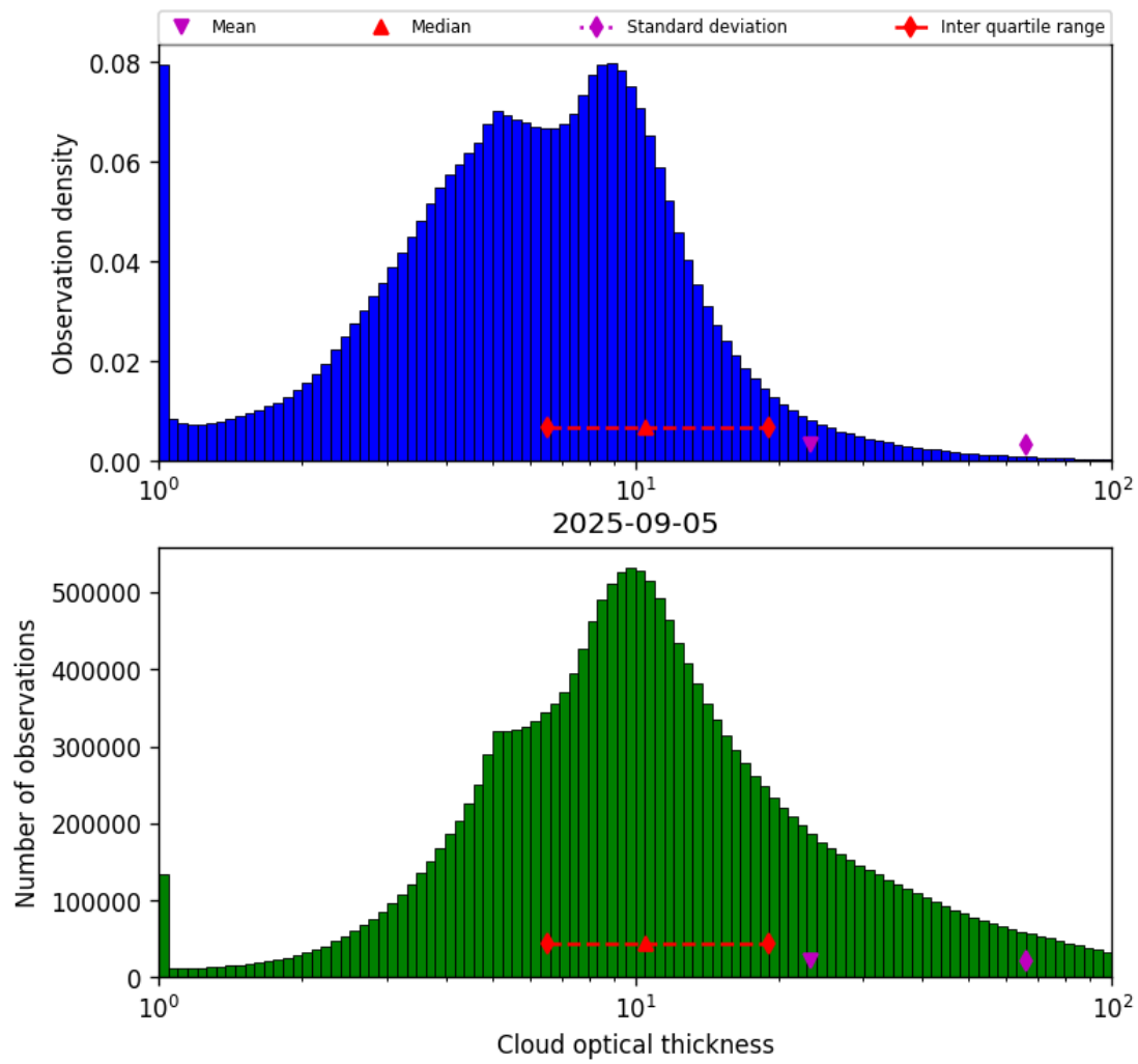
Figure 39: Histogram of “Cloud optical thickness” for 2025-09-05 to 2025-09-06
