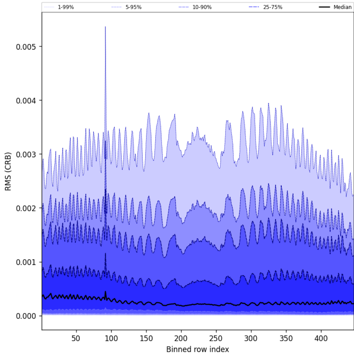
Figure 62: Along track statistics of “RMS (CRB)” for 2025-09-05 to 2025-09-06
