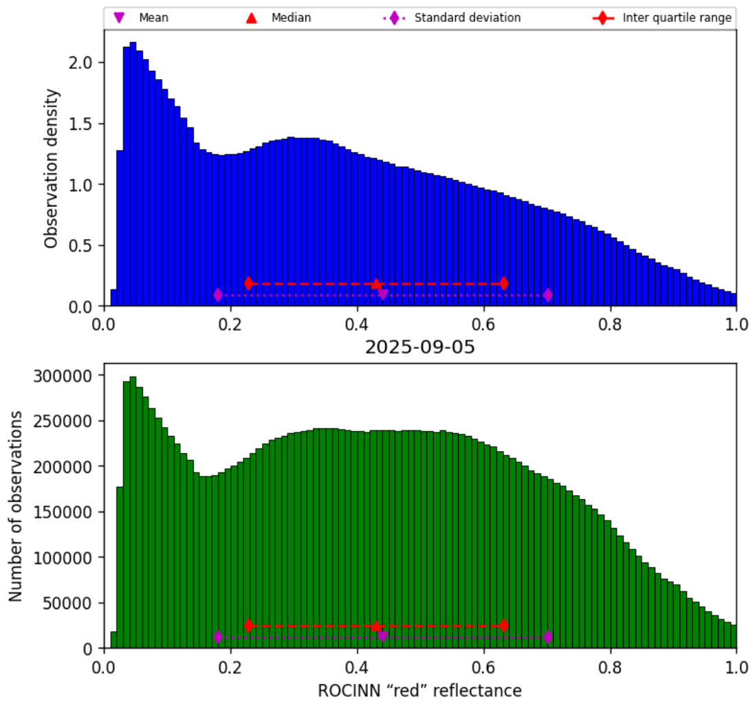
Figure 51: Histogram of "ROCINN "red" reflectance" for 2025-09-05 to 2025-09-06
