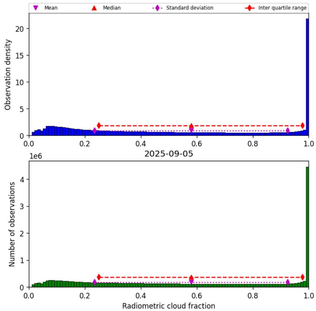
Figure 37: Histogram of “Radiometric cloud fraction” for 2025-09-05 to 2025-09-06
