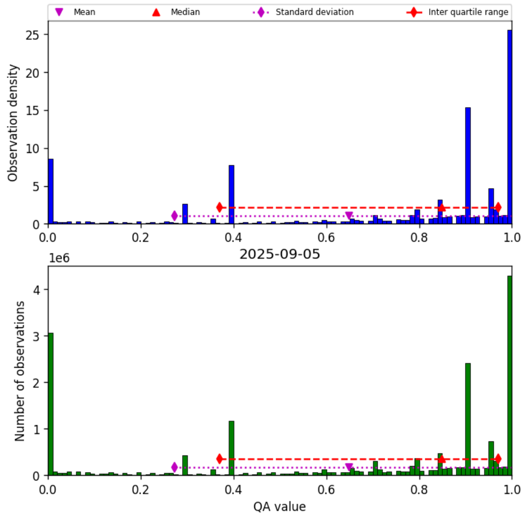
Figure 36: Histogram of “QA value” for 2025-09-05 to 2025-09-06
