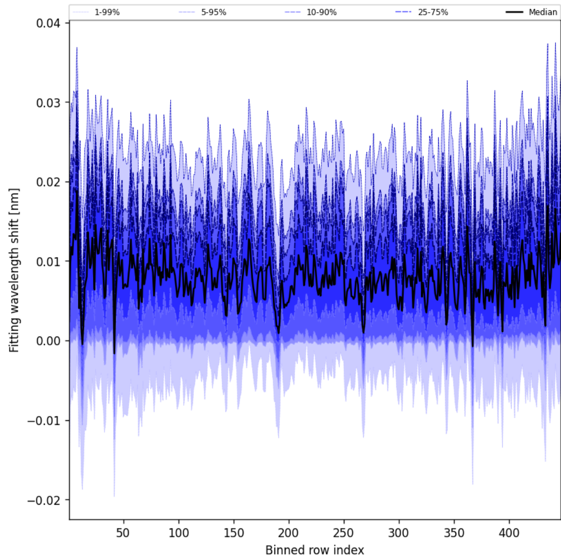
Figure 63: Along track statistics of “Fitting wavelength shift” for 2025-09-05 to 2025-09-06
