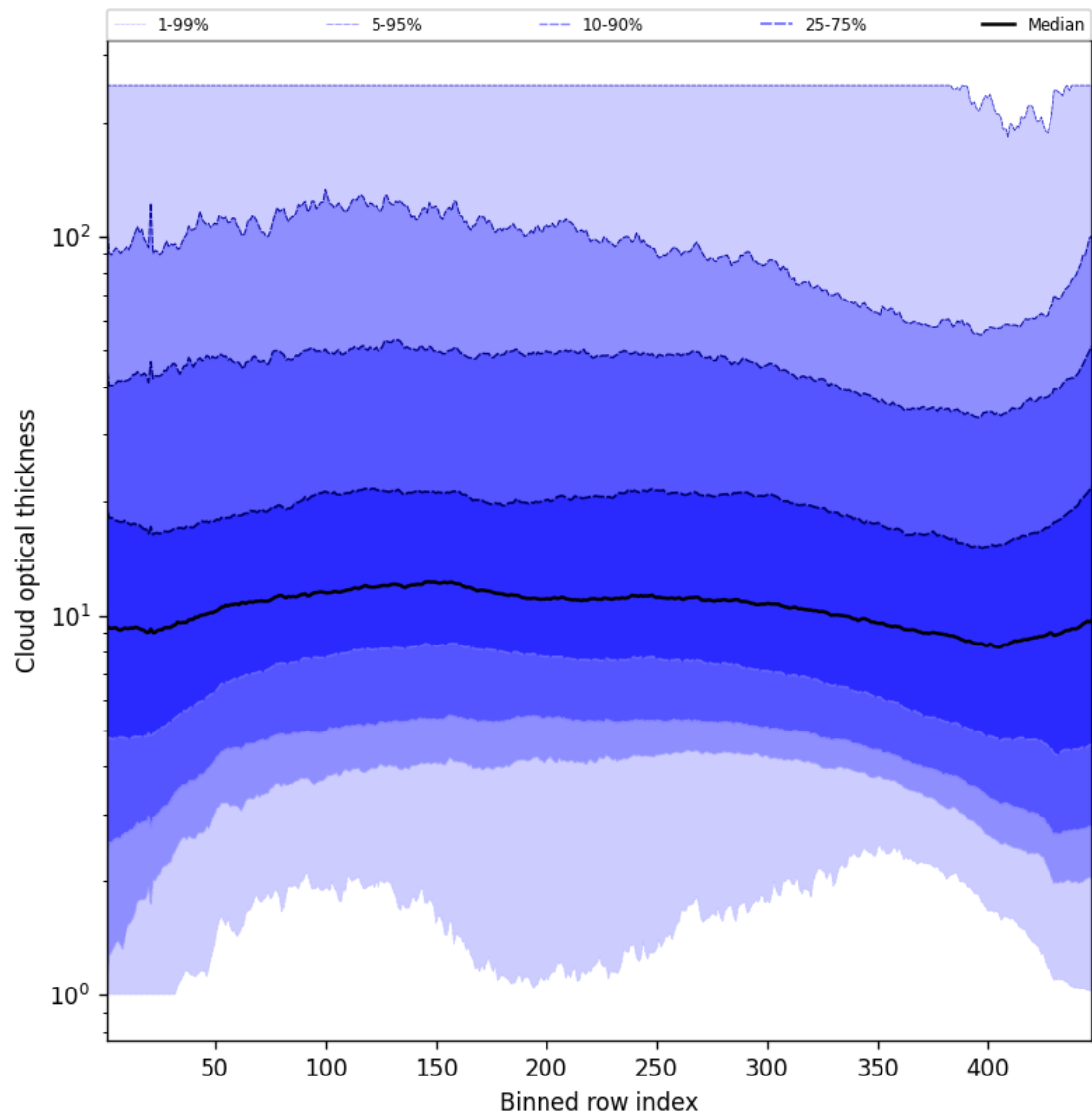
Figure 55: Along track statistics of “Cloud optical thickness” for 2025-09-05 to 2025-09-06
