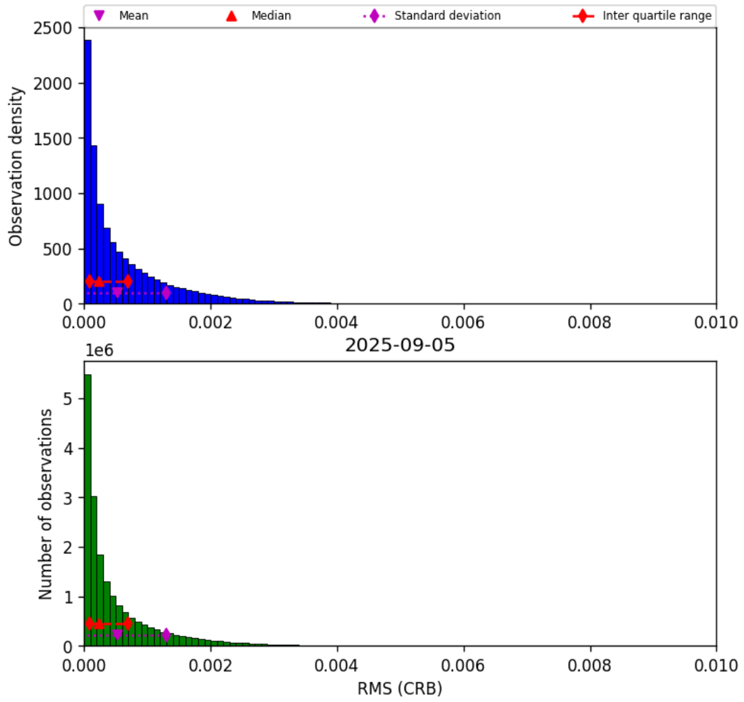
Figure 46: Histogram of “RMS (CRB)” for 2025-09-05 to 2025-09-06
