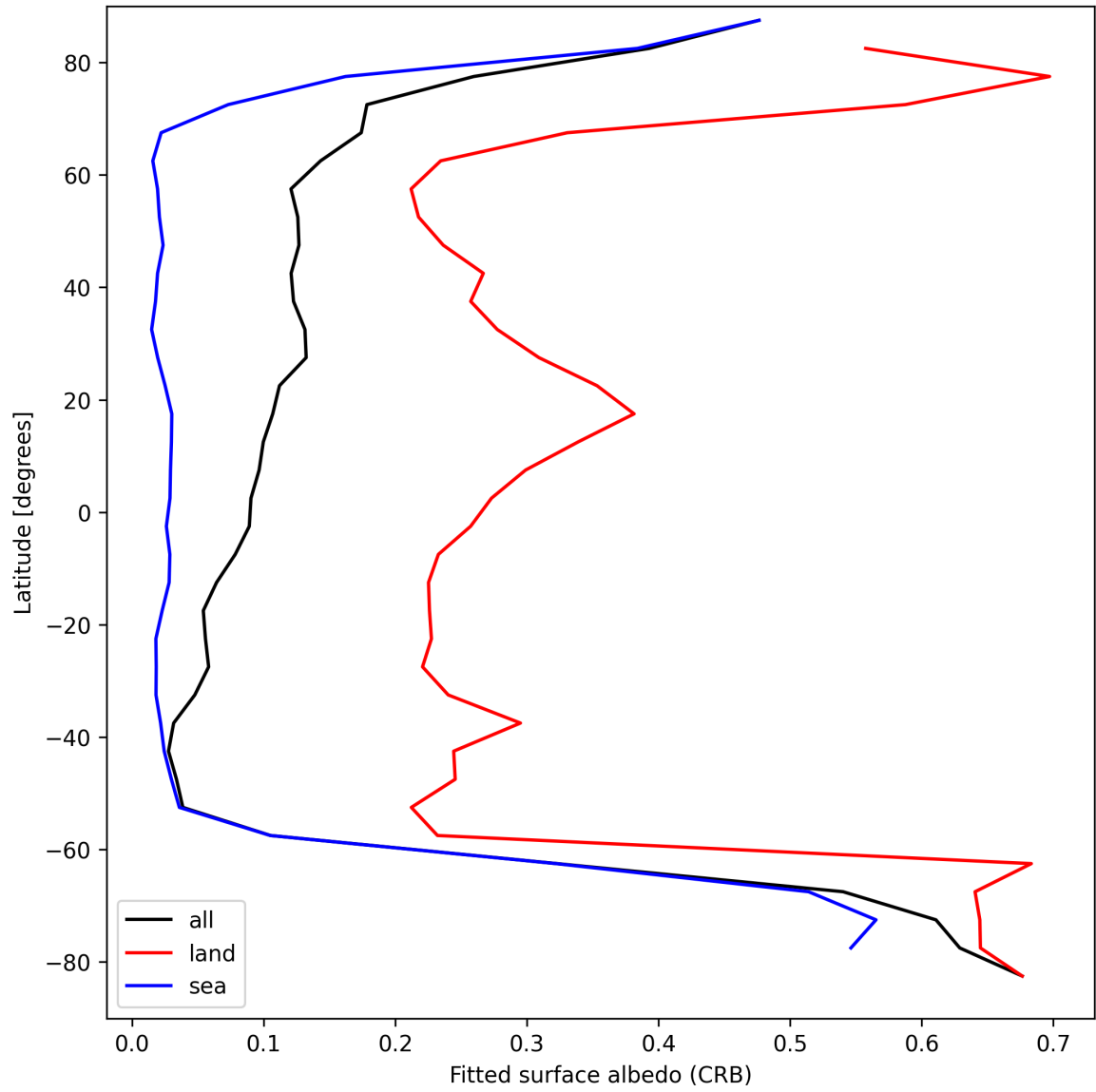
Figure 28: Zonal average of “Fitted surface albedo (CRB)” for 2025-09-05 to 2025-09-06.
