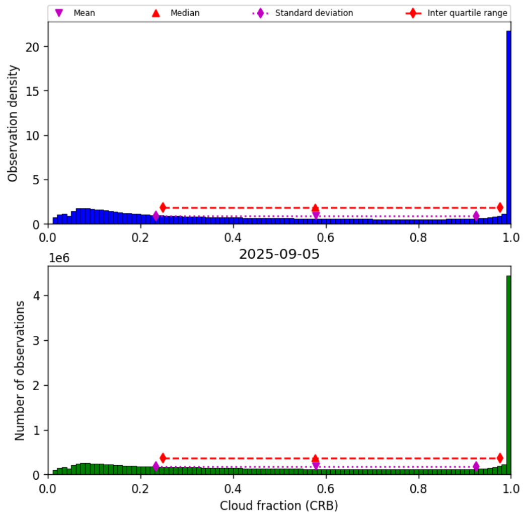
Figure 40: Histogram of "Cloud fraction (CRB)" for 2025-09-05 to 2025-09-06
