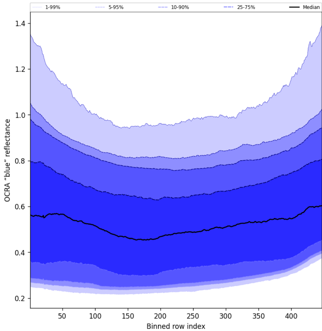
Figure 65: Along track statistics of “OCRA “blue” reflectance” for 2025-09-05 to 2025-09-06
