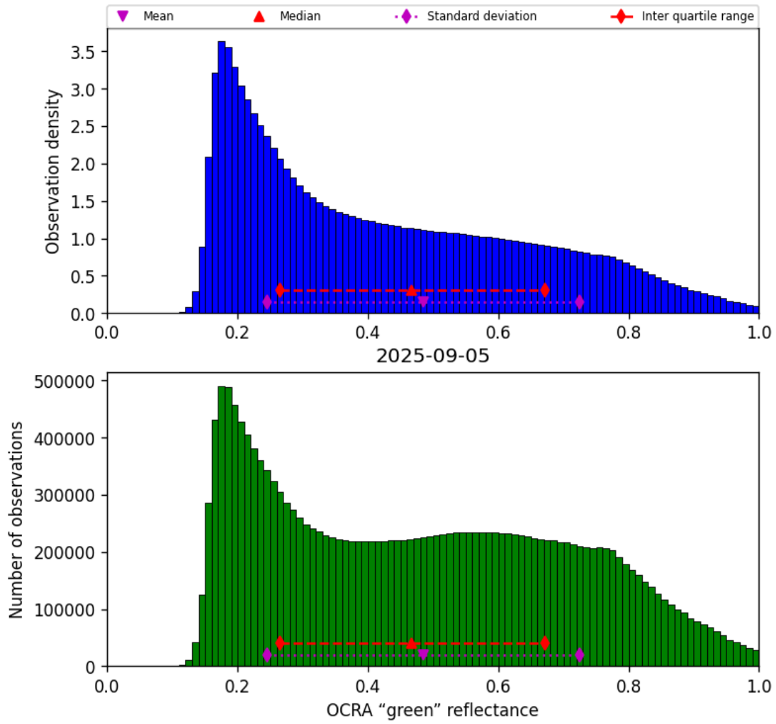
Figure 50: Histogram of “OCRA “green” reflectance” for 2025-09-05 to 2025-09-06
