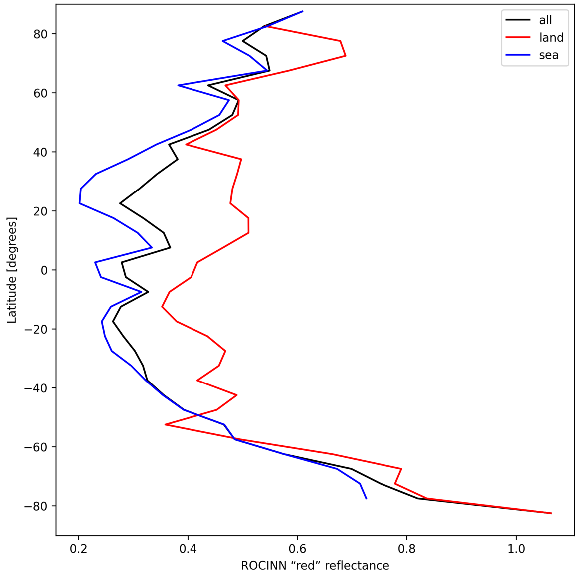
Figure 35: Zonal average of “ROCINN “red” reflectance” for 2025-09-05 to 2025-09-06.
