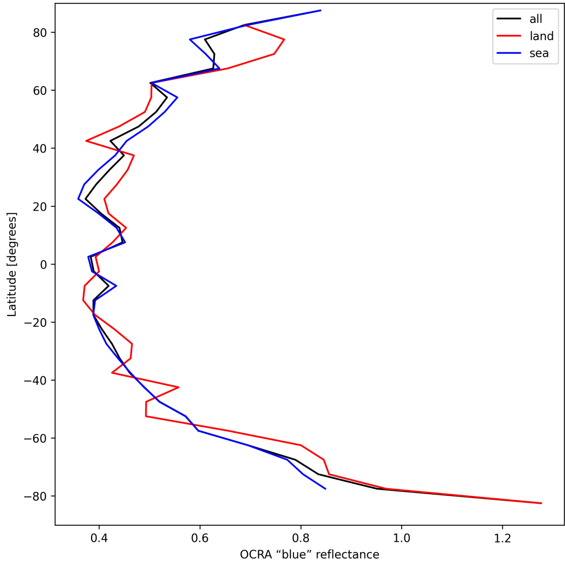
Figure 33: Zonal average of “OCRA “blue” reflectance” for 2025-09-05 to 2025-09-06.
