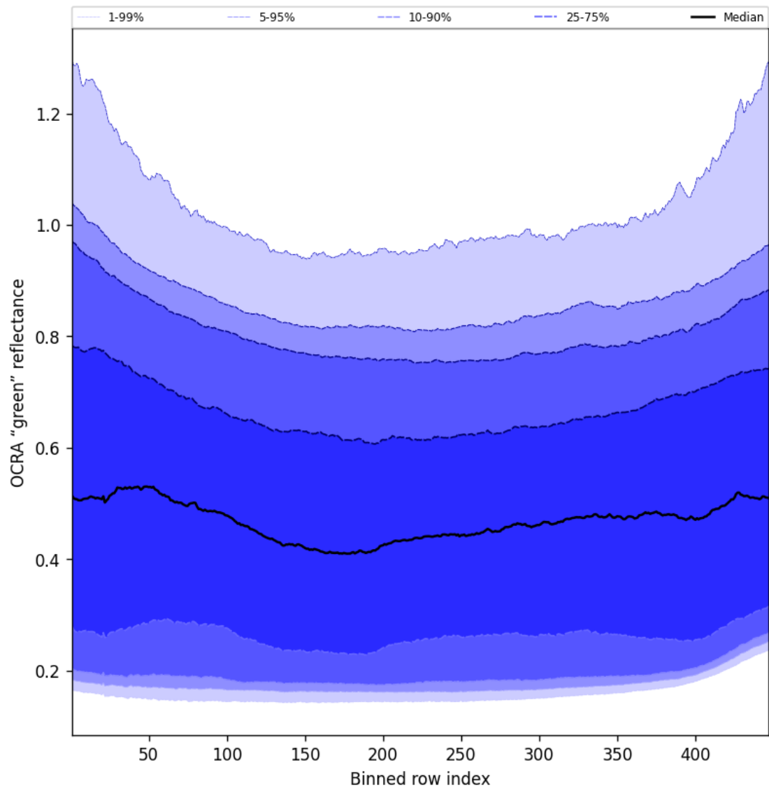
Figure 66: Along track statistics of “OCRA “green” reflectance” for 2025-09-05 to 2025-09-06
