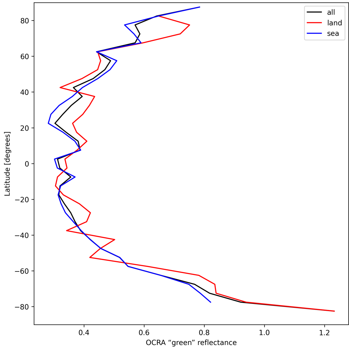
Figure 34: Zonal average of “OCRA “green” reflectance” for 2025-09-05 to 2025-09-06.
