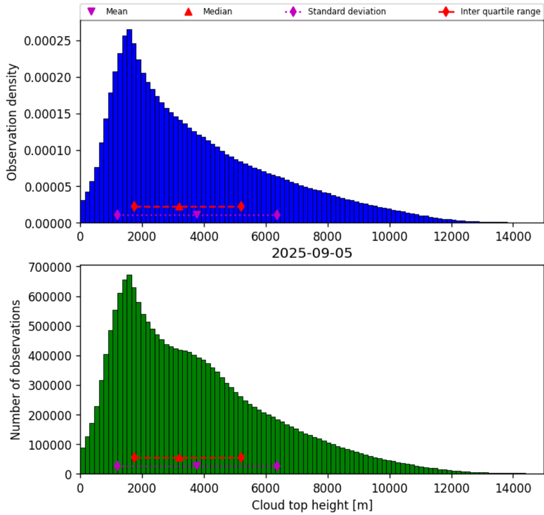
Figure 38: Histogram of “Cloud top height” for 2025-09-05 to 2025-09-06
