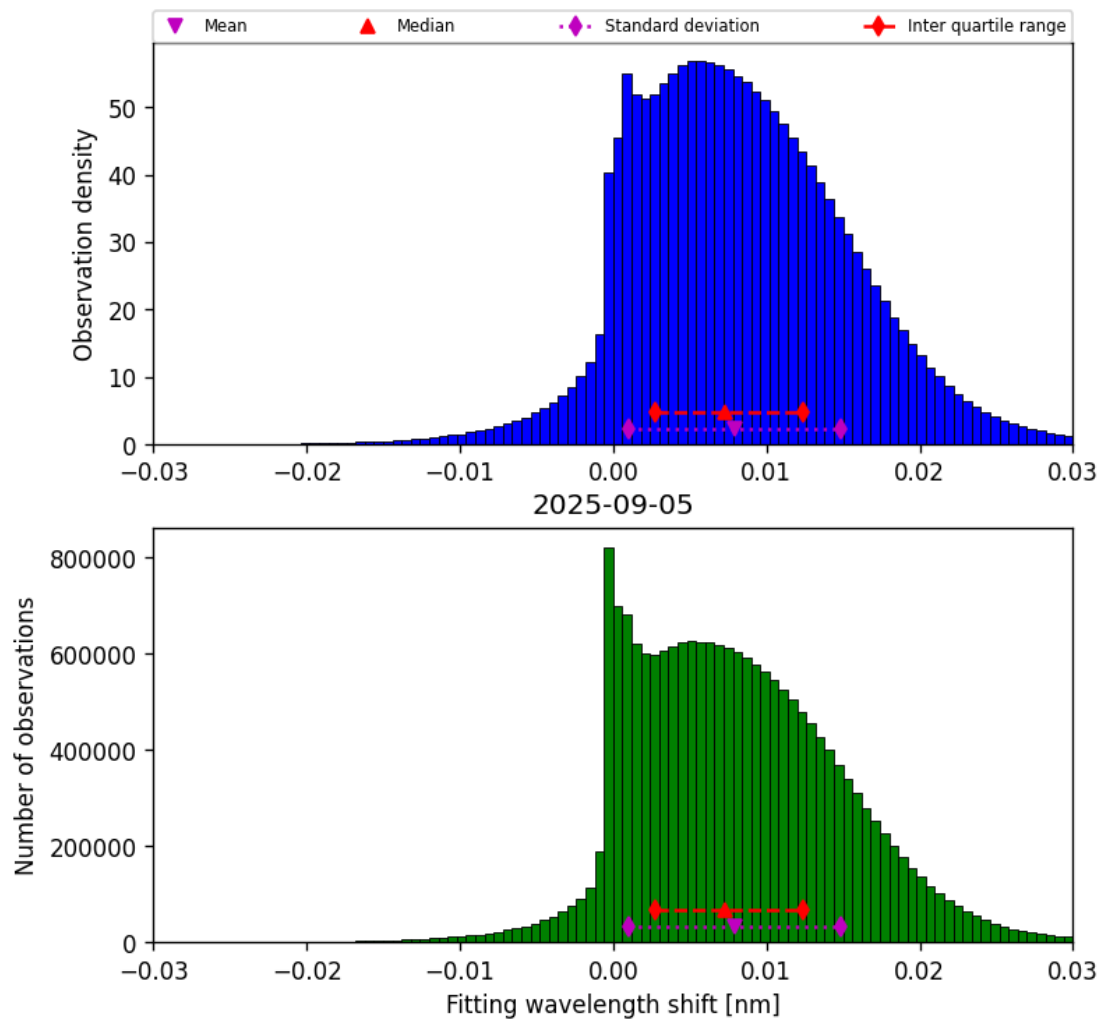
Figure 47: Histogram of “Fitting wavelength shift” for 2025-09-05 to 2025-09-06
