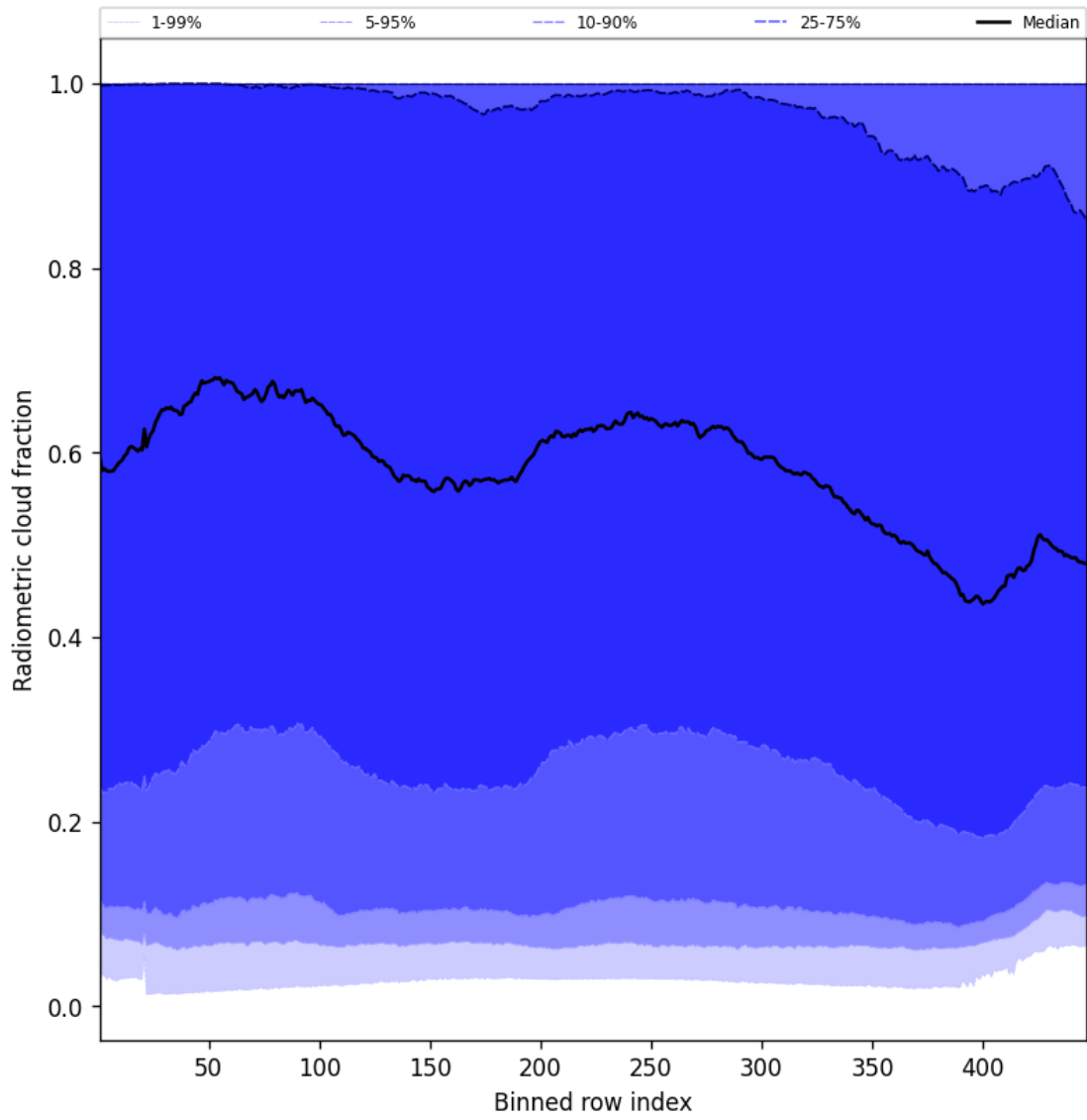
Figure 53: Along track statistics of “Radiometric cloud fraction” for 2025-09-05 to 2025-09-06
