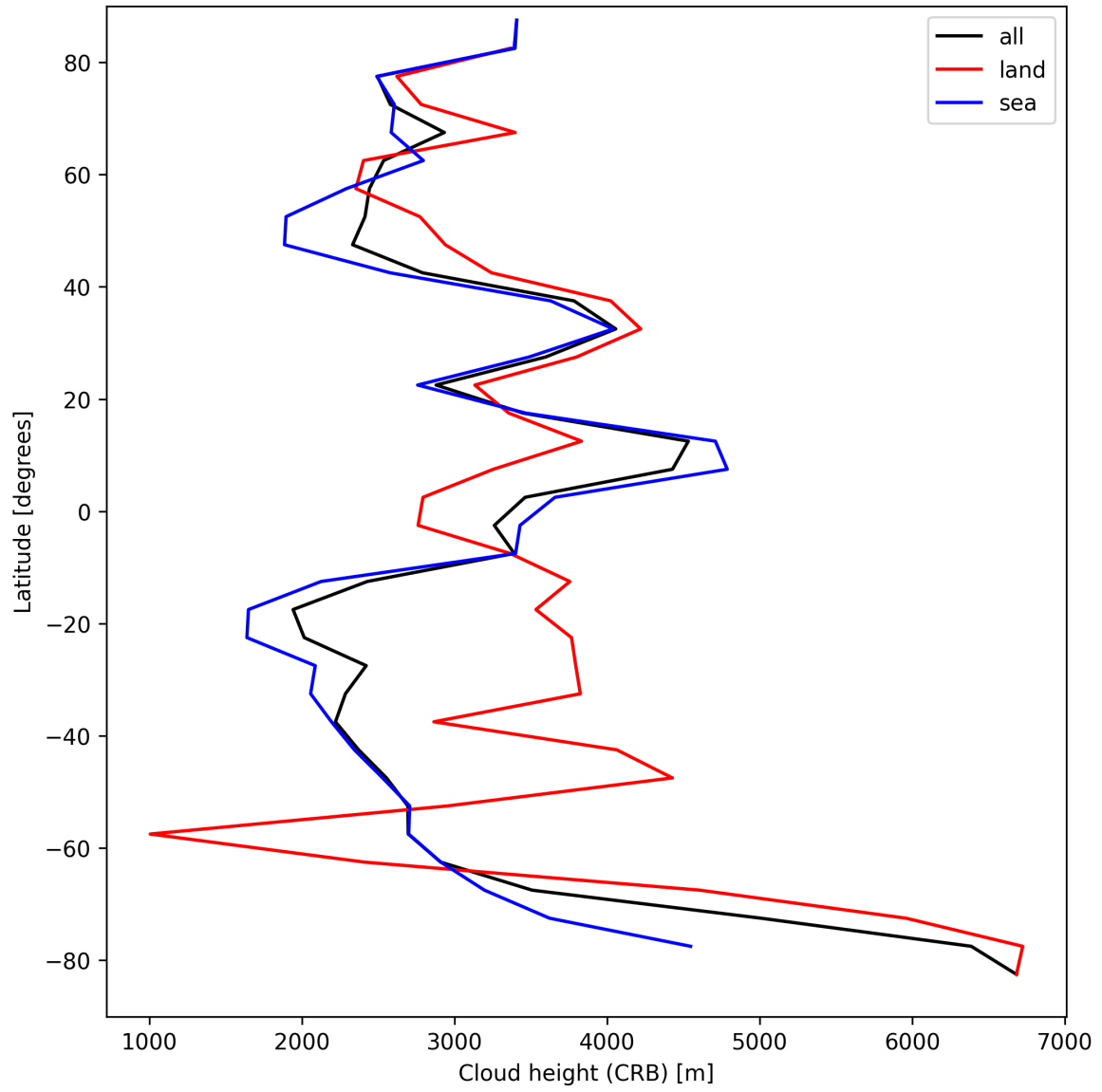
Figure 25: Zonal average of “Cloud height (CRB)” for 2025-09-05 to 2025-09-06.
