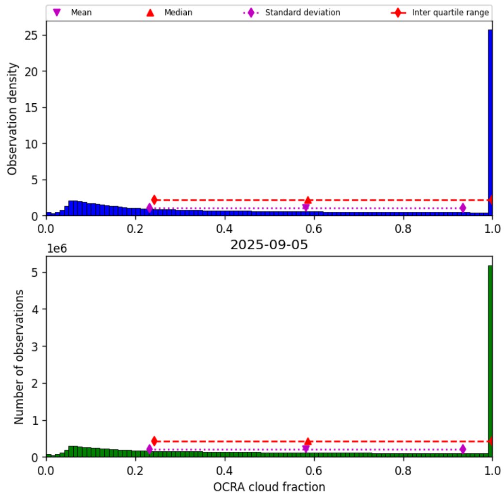
Figure 48: Histogram of “OCRA cloud fraction” for 2025-09-05 to 2025-09-06
