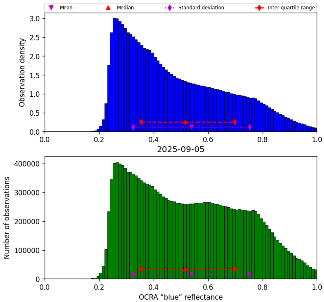
Figure 49: Histogram of “OCRA “blue” reflectance” for 2025-09-05 to 2025-09-06
