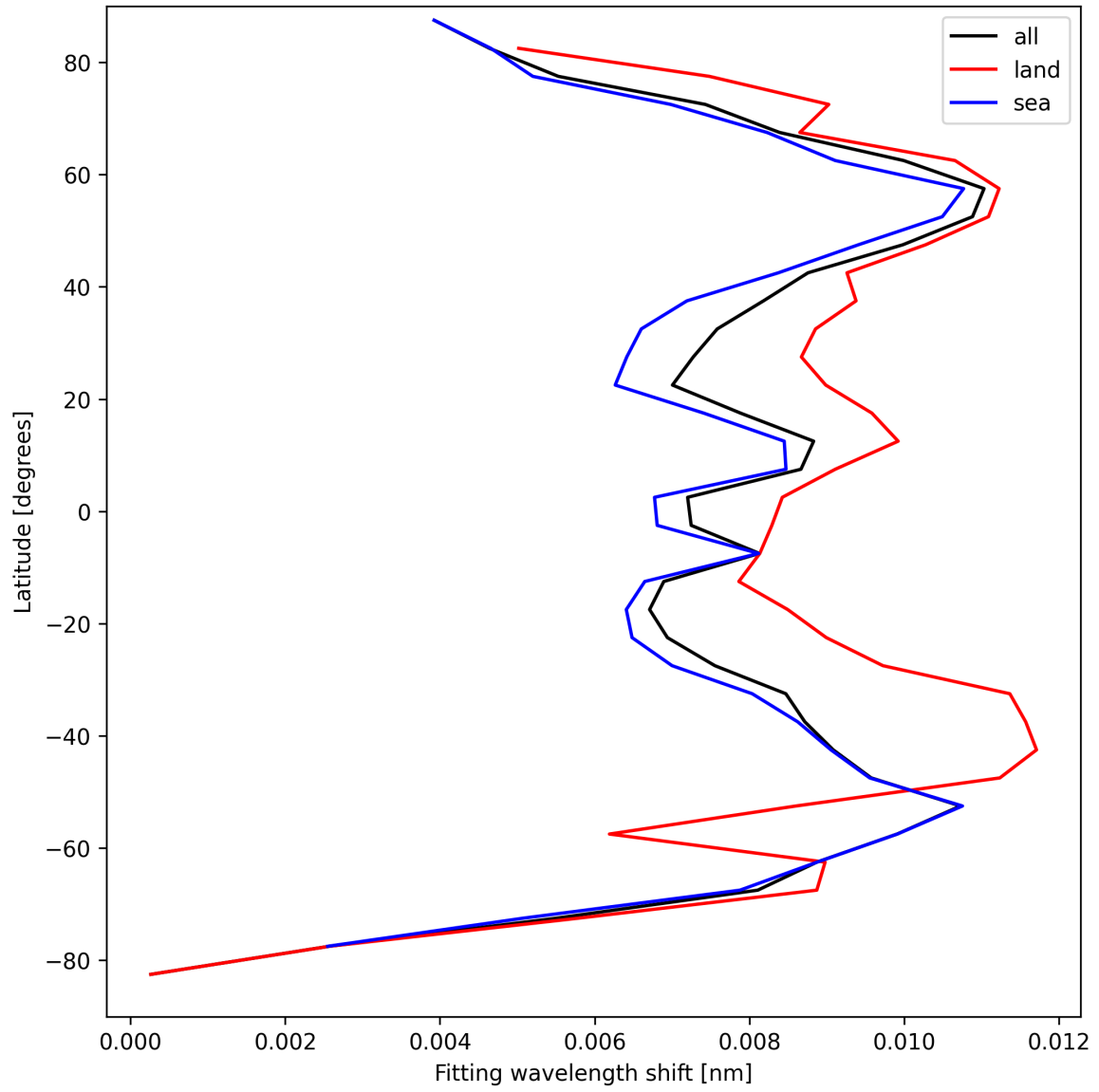
Figure 31: Zonal average of “Fitting wavelength shift” for 2025-09-05 to 2025-09-06.
