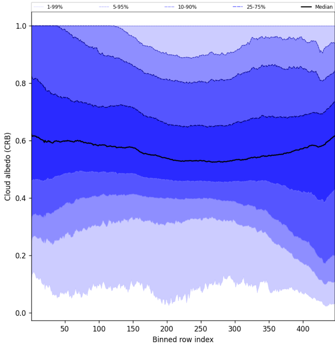
Figure 58: Along track statistics of “Cloud albedo (CRB)” for 2025-09-08 to 2025-09-08
