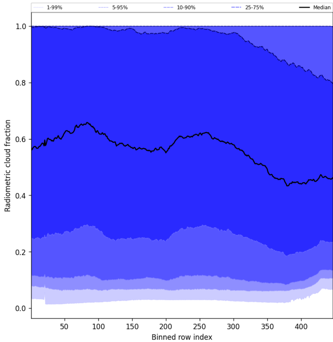
Figure 53: Along track statistics of “Radiometric cloud fraction” for 2025-09-08 to 2025-09-08
