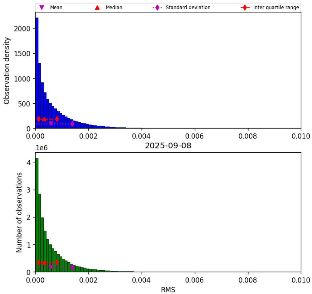
Figure 45: Histogram of “RMS” for 2025-09-08 to 2025-09-08
