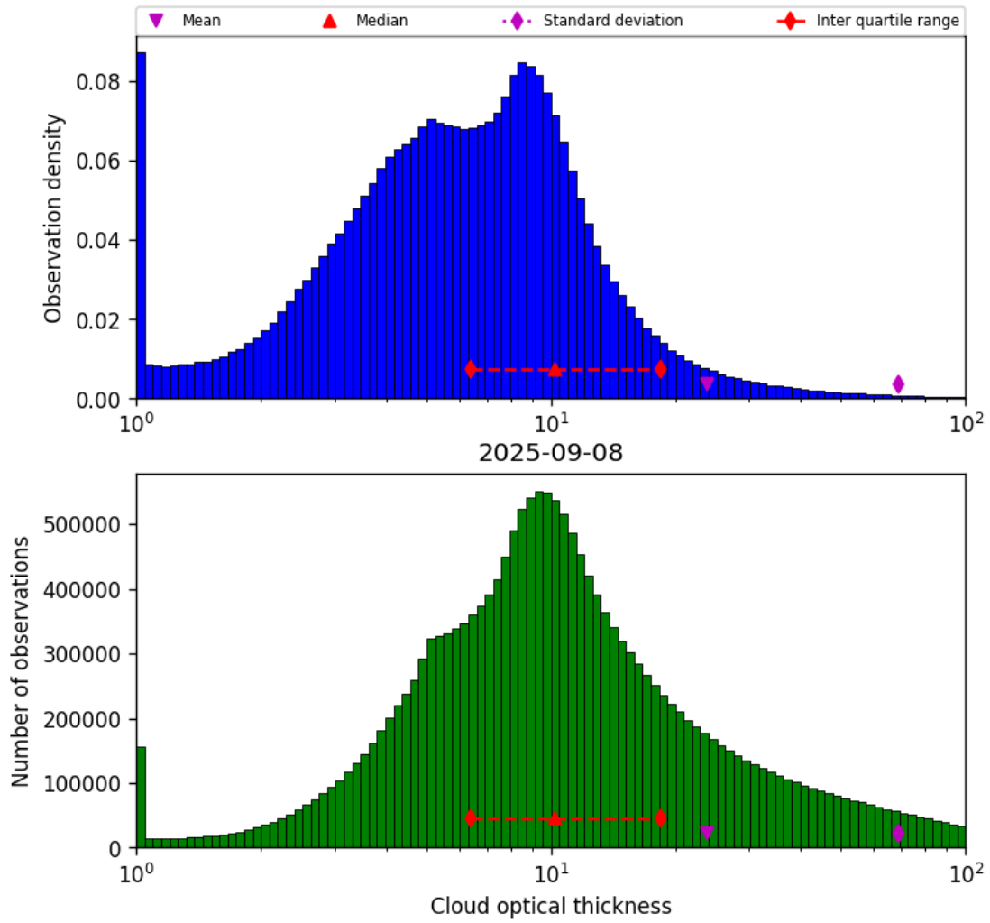
Figure 39: Histogram of “Cloud optical thickness” for 2025-09-08 to 2025-09-08
