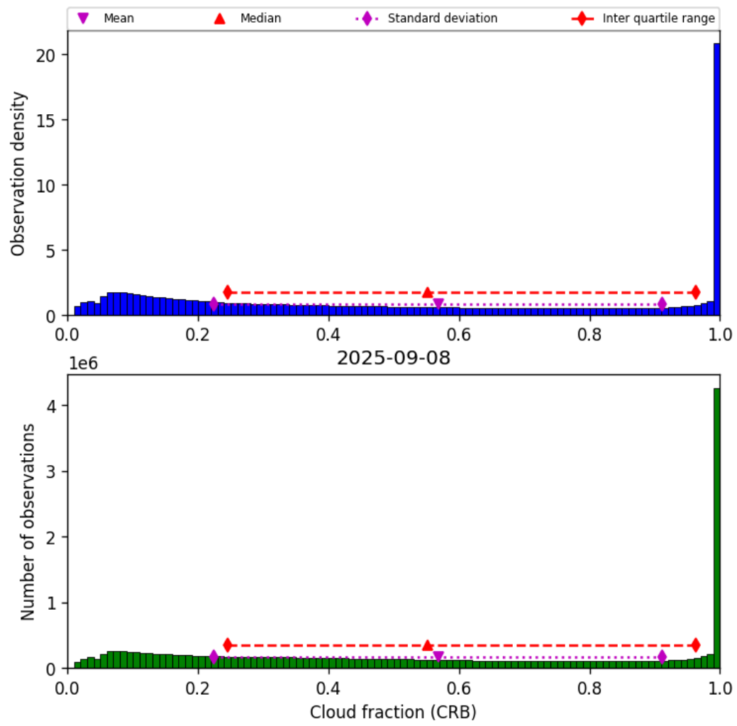
Figure 40: Histogram of “Cloud fraction (CRB)” for 2025-09-08 to 2025-09-08
