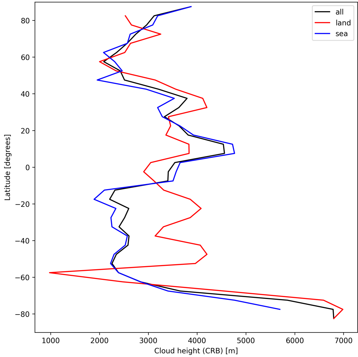
Figure 25: Zonal average of “Cloud height (CRB)” for 2025-09-08 to 2025-09-08.
