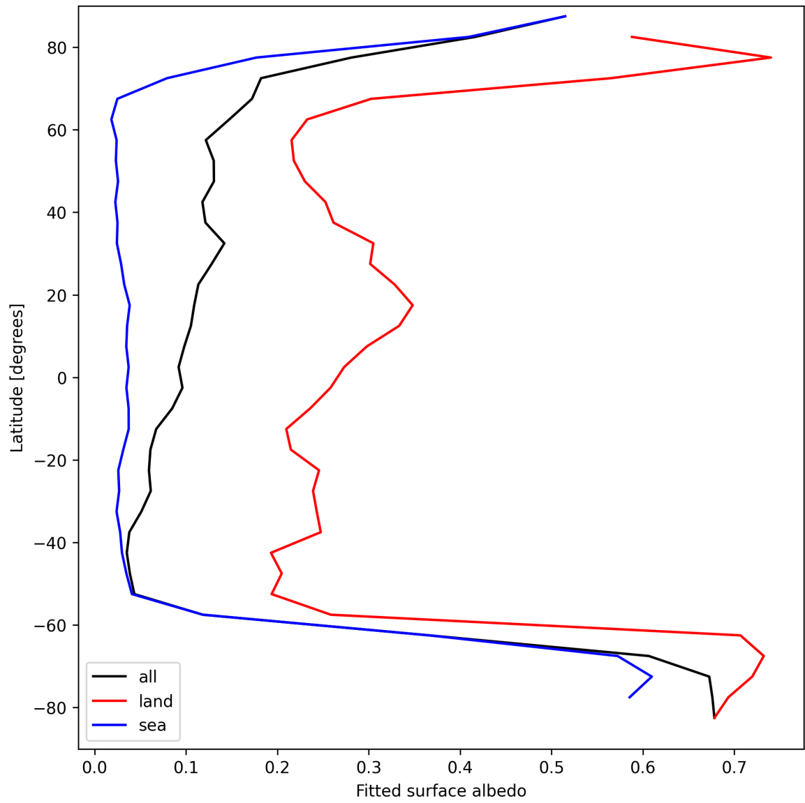
Figure 27: Zonal average of “Fitted surface albedo” for 2025-09-08 to 2025-09-08.
