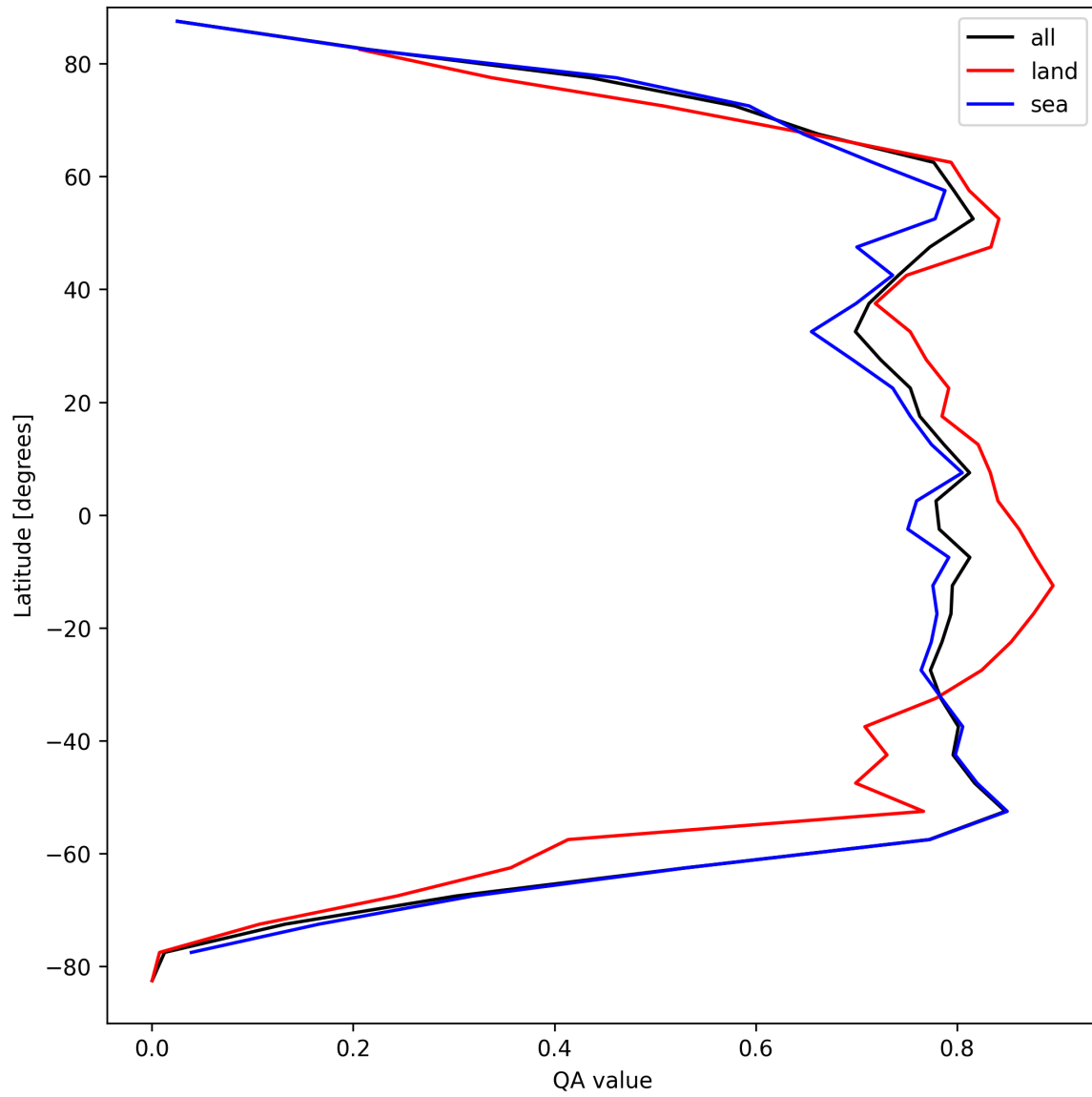
Figure 20: Zonal average of “QA value” for 2025-09-08 to 2025-09-08.
