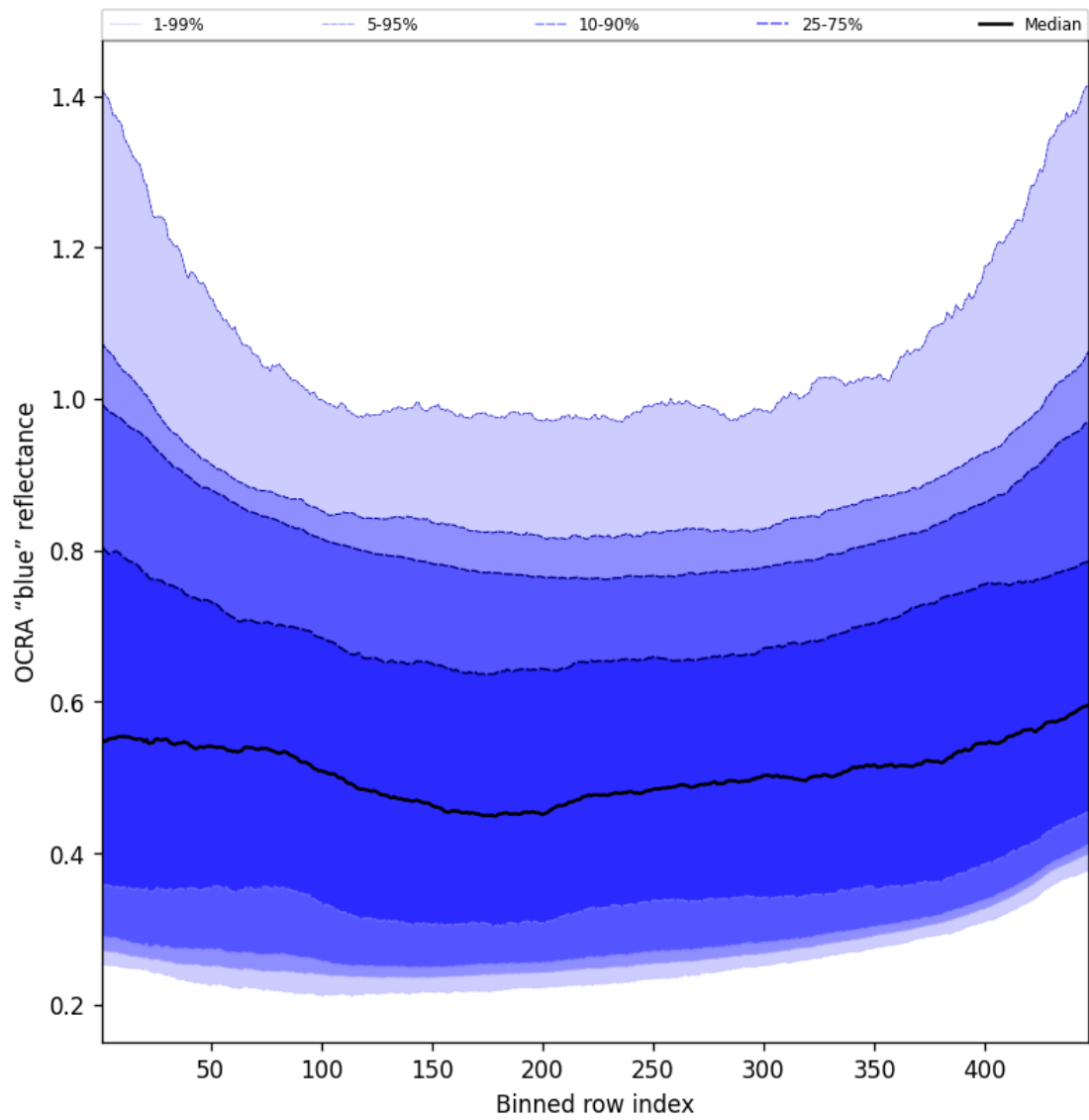
Figure 65: Along track statistics of “OCRA “blue” reflectance” for 2025-09-08 to 2025-09-08
