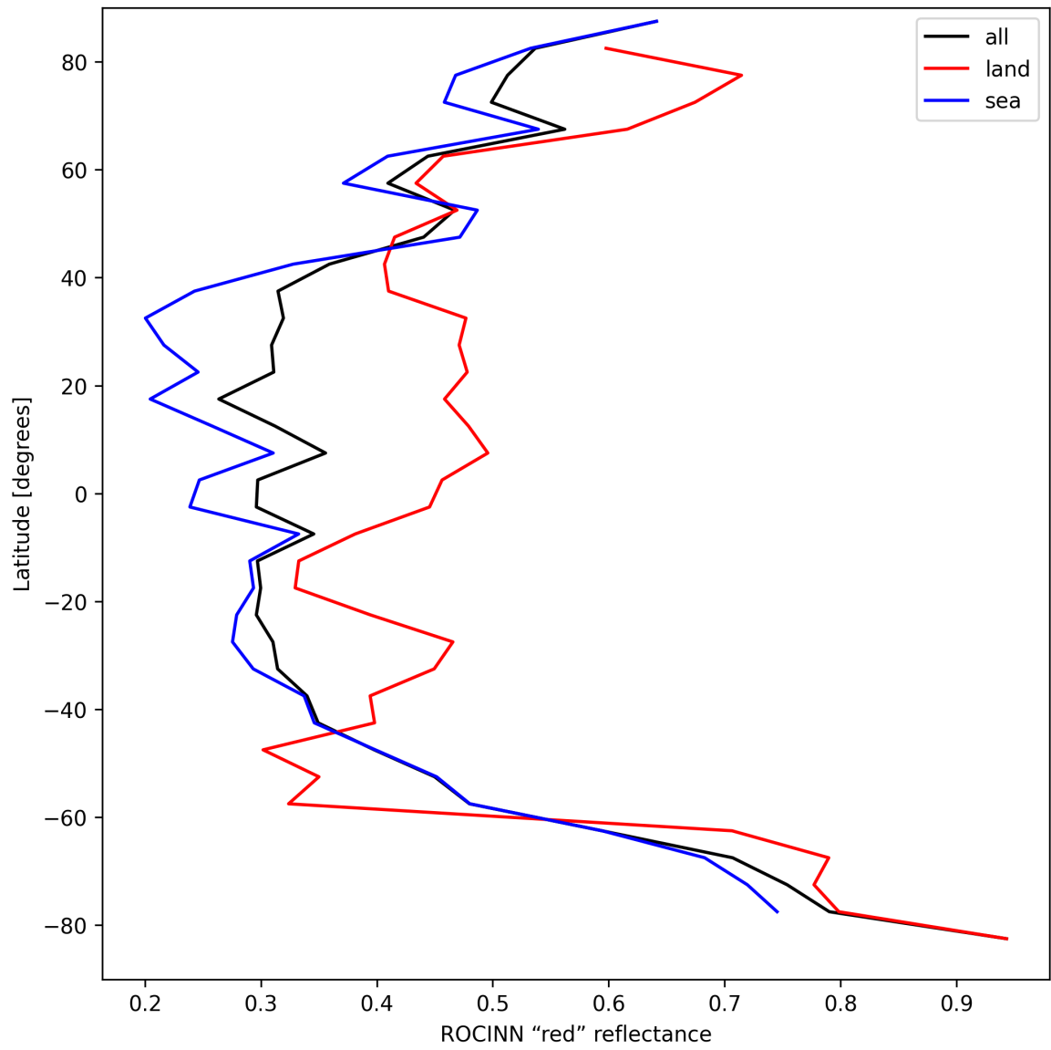
Figure 35: Zonal average of “ROCINN “red” reflectance” for 2025-09-08 to 2025-09-08.
