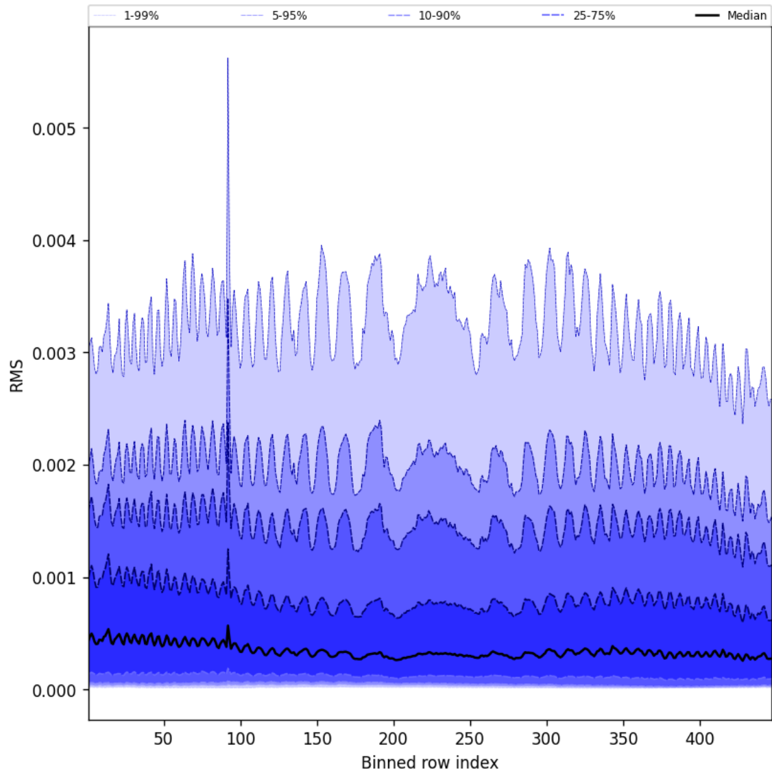
Figure 61: Along track statistics of “RMS” for 2025-09-08 to 2025-09-08
