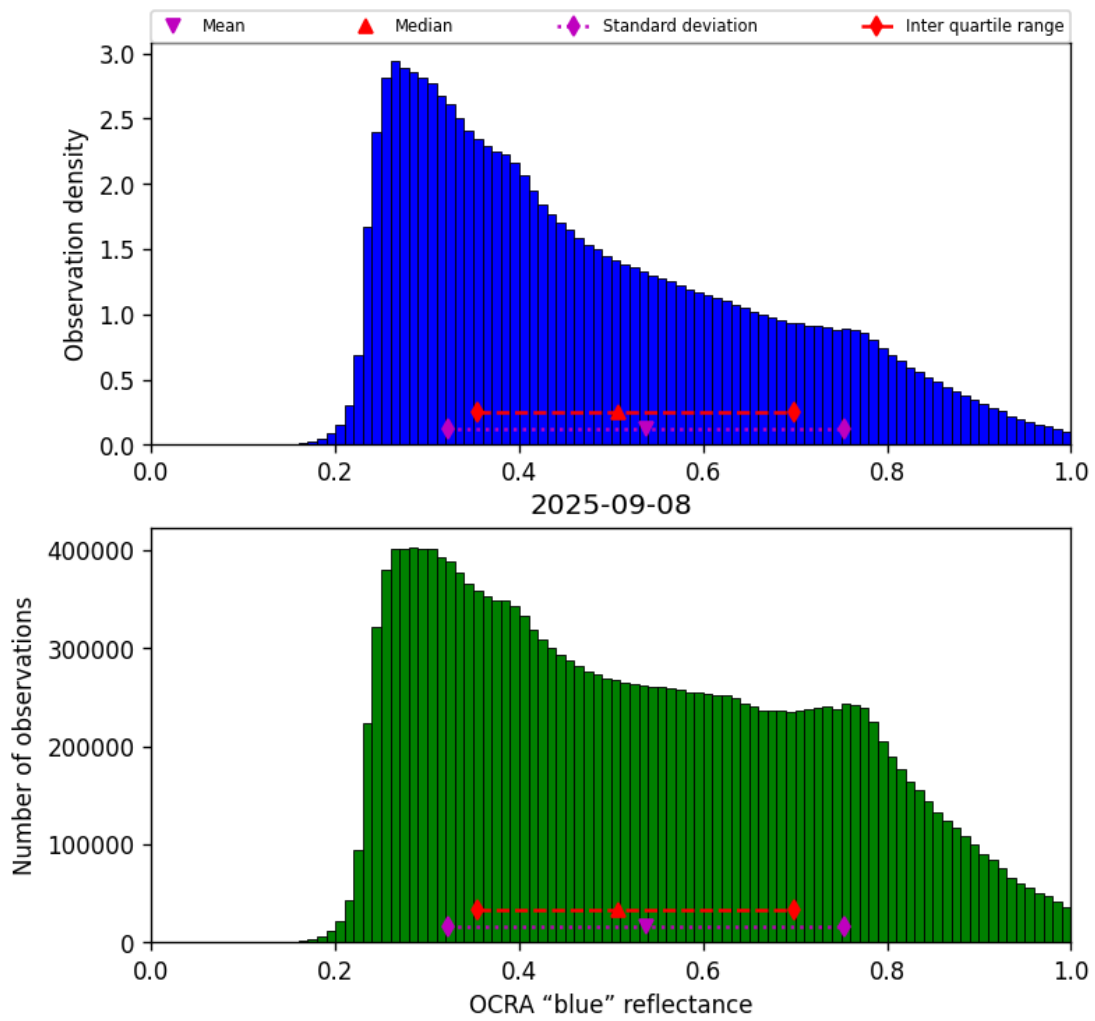
Figure 49: Histogram of “OCRA “blue” reflectance” for 2025-09-08 to 2025-09-08
