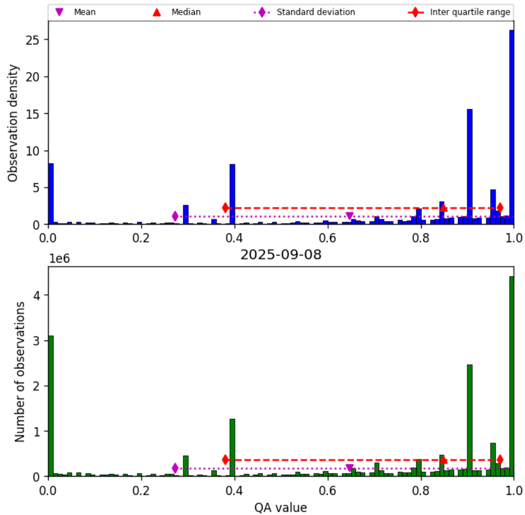
Figure 36: Histogram of “QA value” for 2025-09-08 to 2025-09-08
