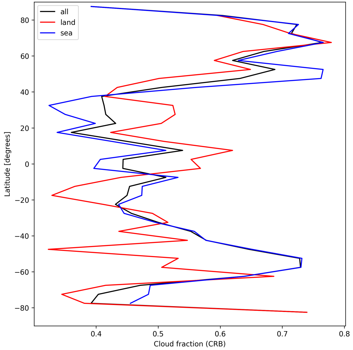
Figure 24: Zonal average of “Cloud fraction (CRB)” for 2025-09-08 to 2025-09-08.
