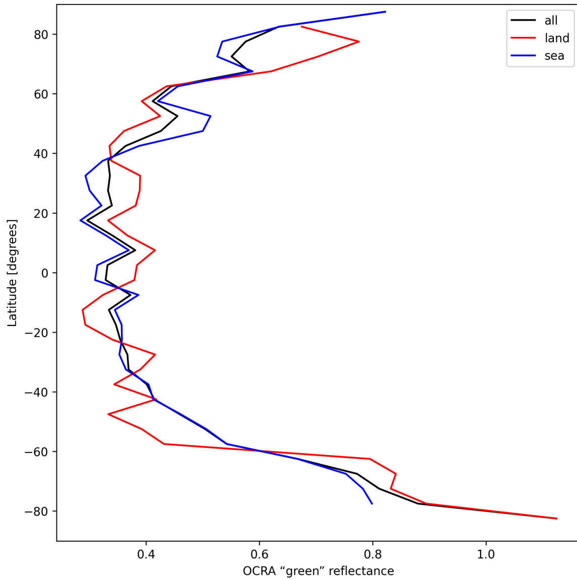
Figure 34: Zonal average of “OCRA “green” reflectance” for 2025-09-08 to 2025-09-08.
