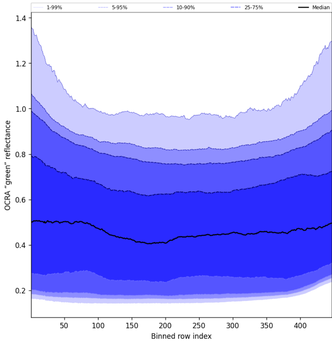
Figure 66: Along track statistics of “OCRA “green” reflectance” for 2025-09-08 to 2025-09-08
