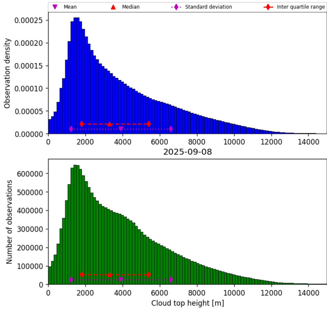
Figure 38: Histogram of “Cloud top height” for 2025-09-08 to 2025-09-08
