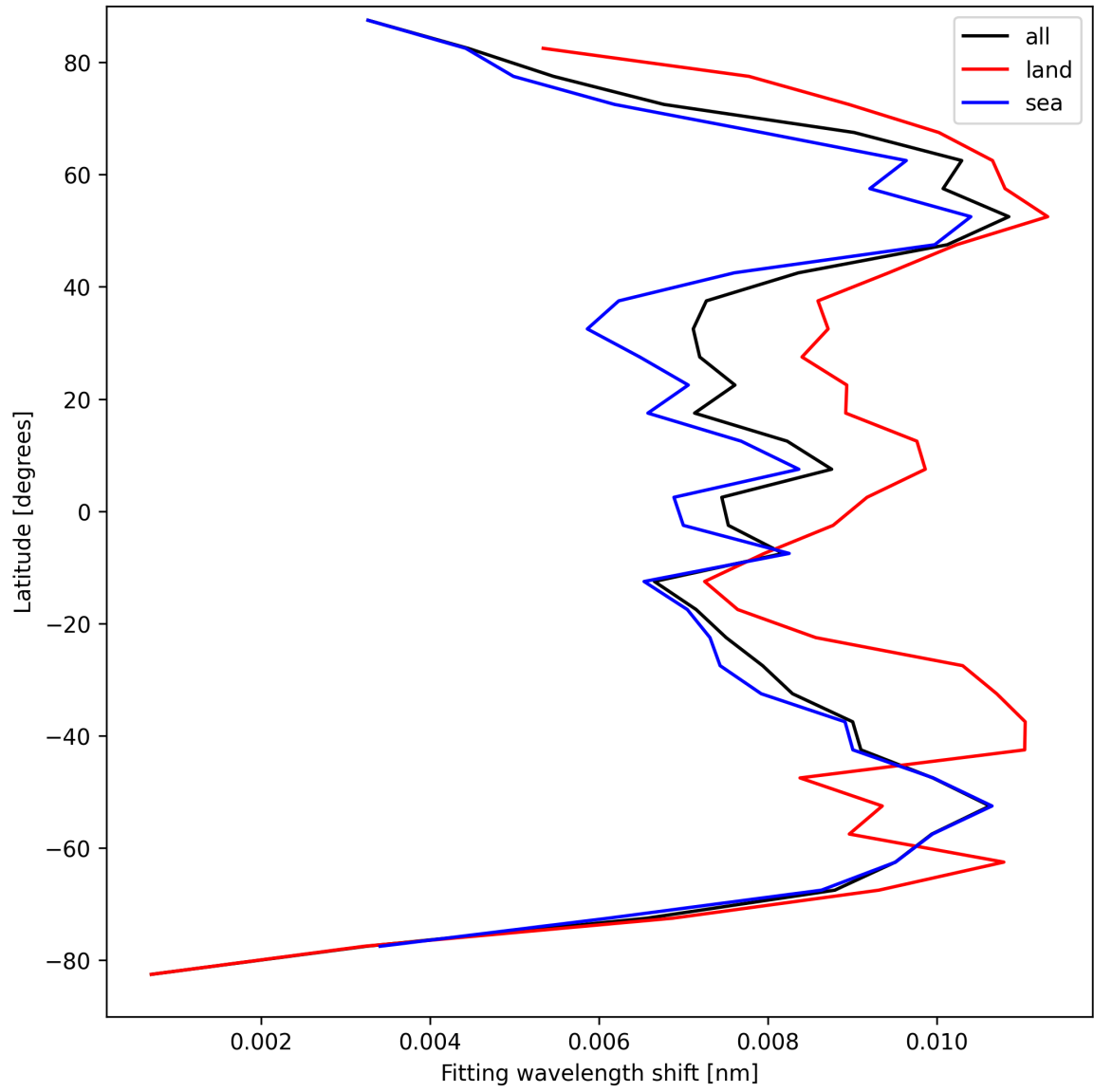
Figure 31: Zonal average of “Fitting wavelength shift” for 2025-09-08 to 2025-09-08.
