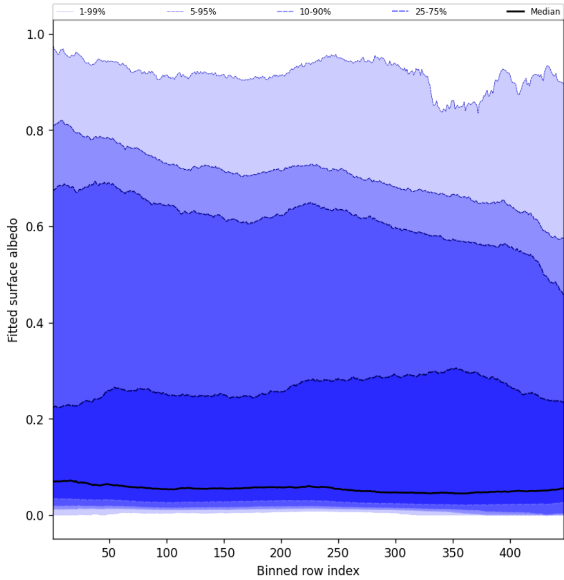
Figure 59: Along track statistics of “Fitted surface albedo” for 2025-09-08 to 2025-09-08
