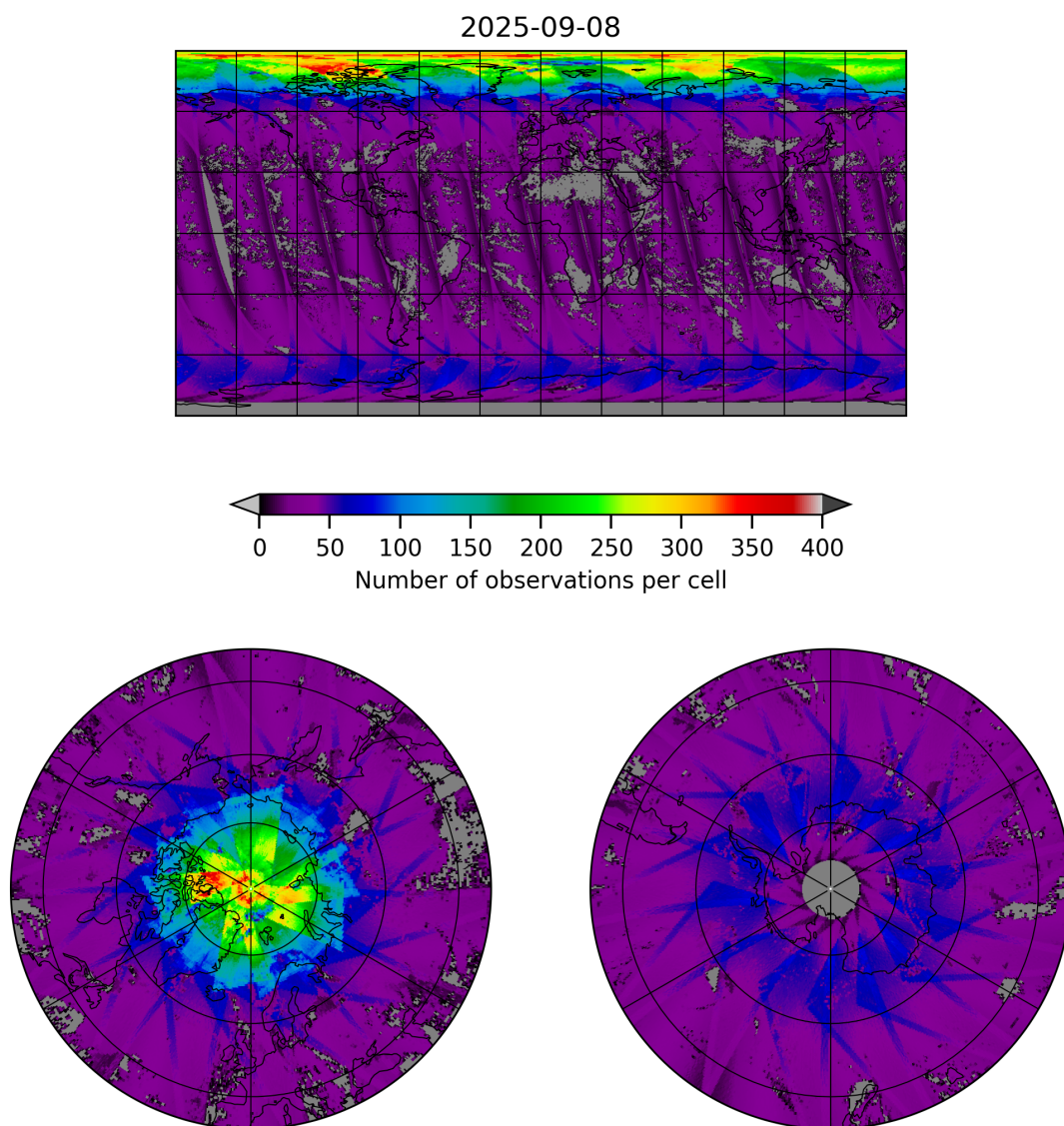
Figure 19: Map of the number of observations for 2025-09-08 to 2025-09-08
