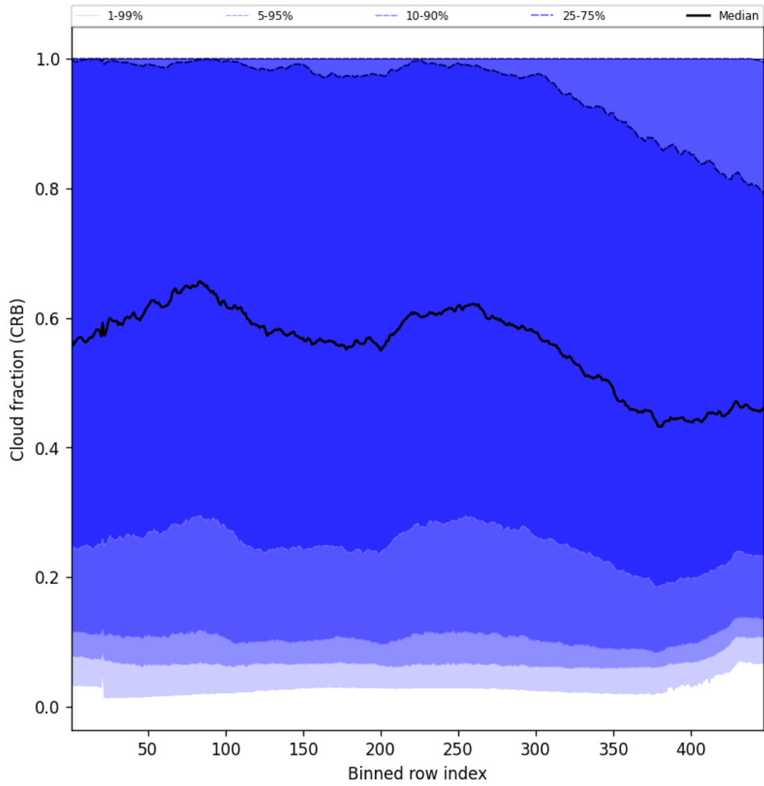
Figure 56: Along track statistics of “Cloud fraction (CRB)” for 2025-09-08 to 2025-09-08
