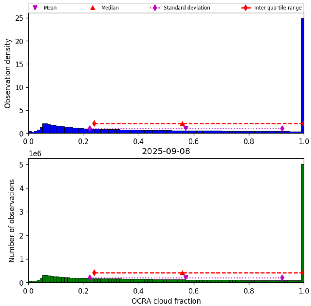
Figure 48: Histogram of “OCRA cloud fraction” for 2025-09-08 to 2025-09-08
