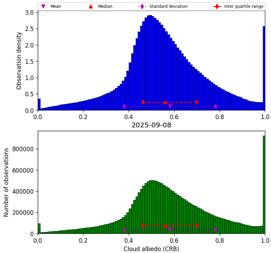
Figure 42: Histogram of “Cloud albedo (CRB)” for 2025-09-08 to 2025-09-08
