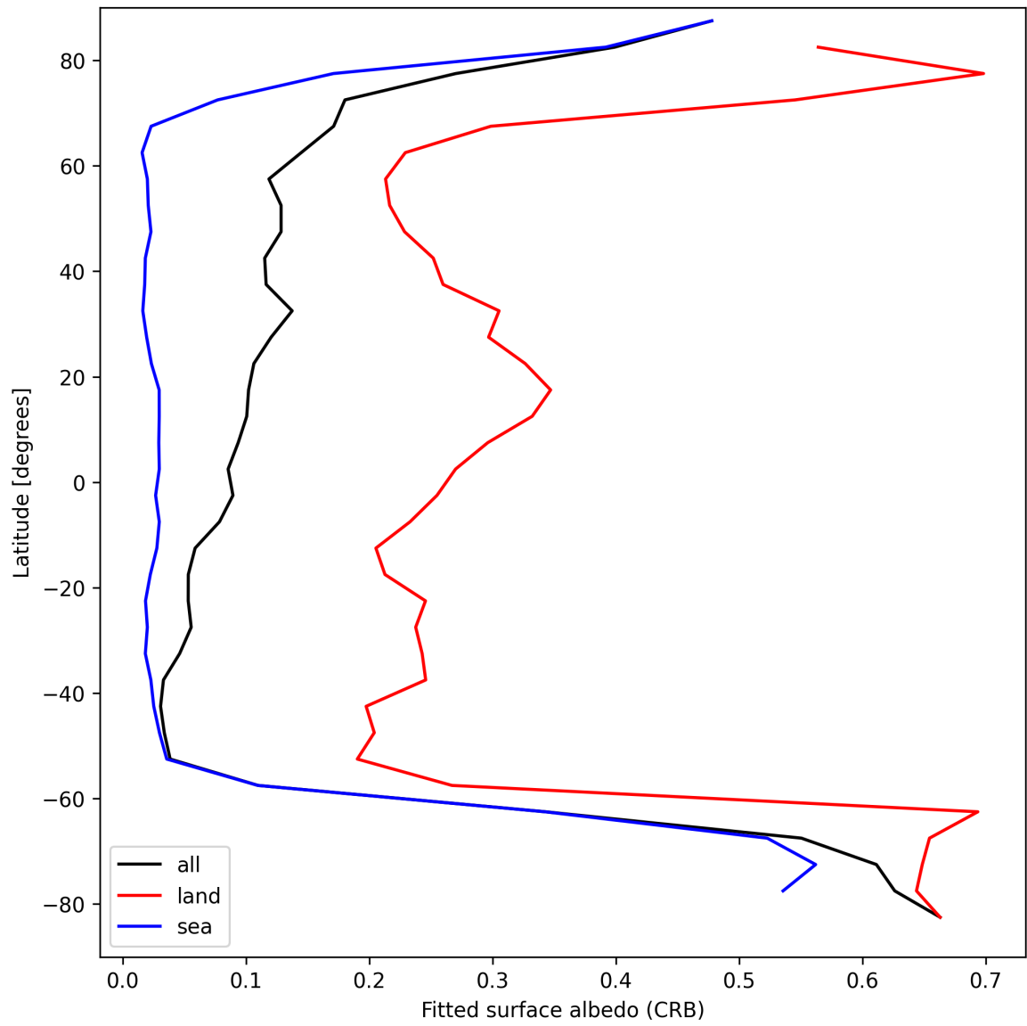
Figure 28: Zonal average of “Fitted surface albedo (CRB)” for 2025-09-08 to 2025-09-08.
