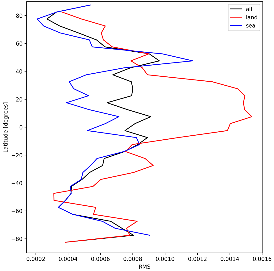
Figure 29: Zonal average of “RMS” for 2025-09-08 to 2025-09-08.
