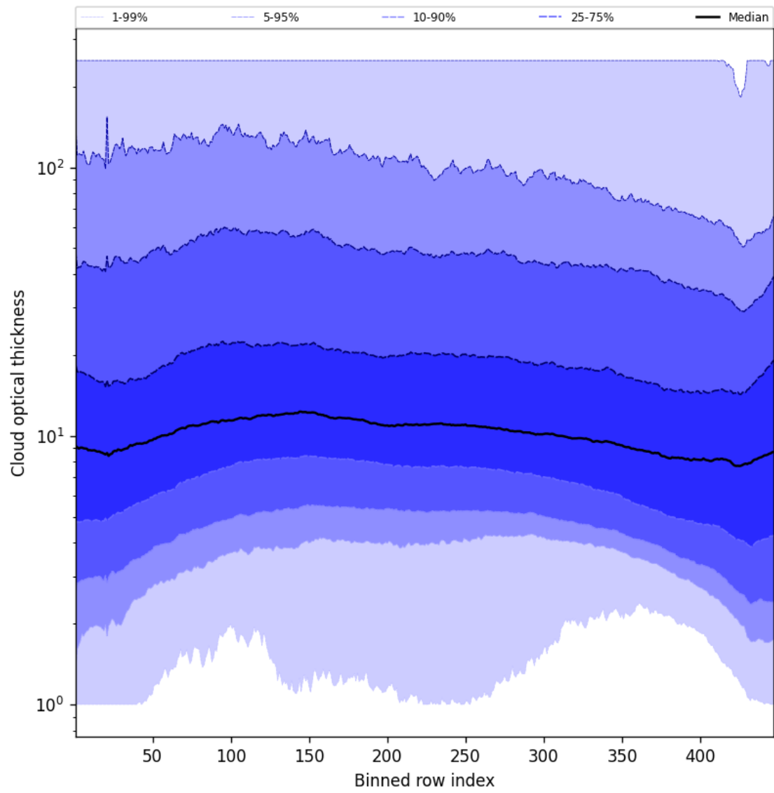
Figure 55: Along track statistics of “Cloud optical thickness” for 2025-09-08 to 2025-09-08
