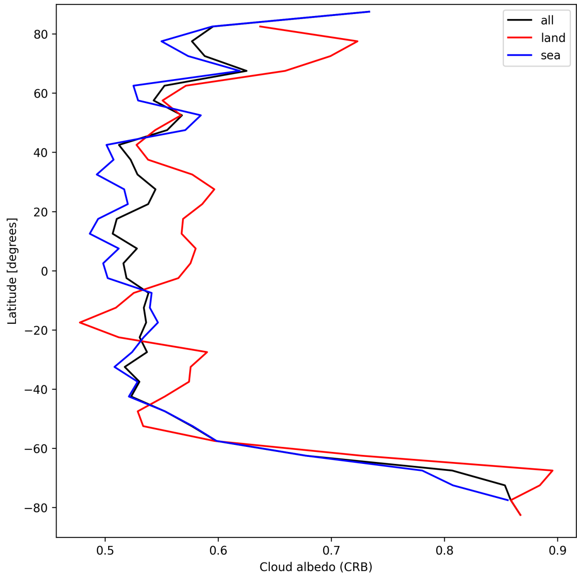
Figure 26: Zonal average of “Cloud albedo (CRB)” for 2025-09-08 to 2025-09-08.
