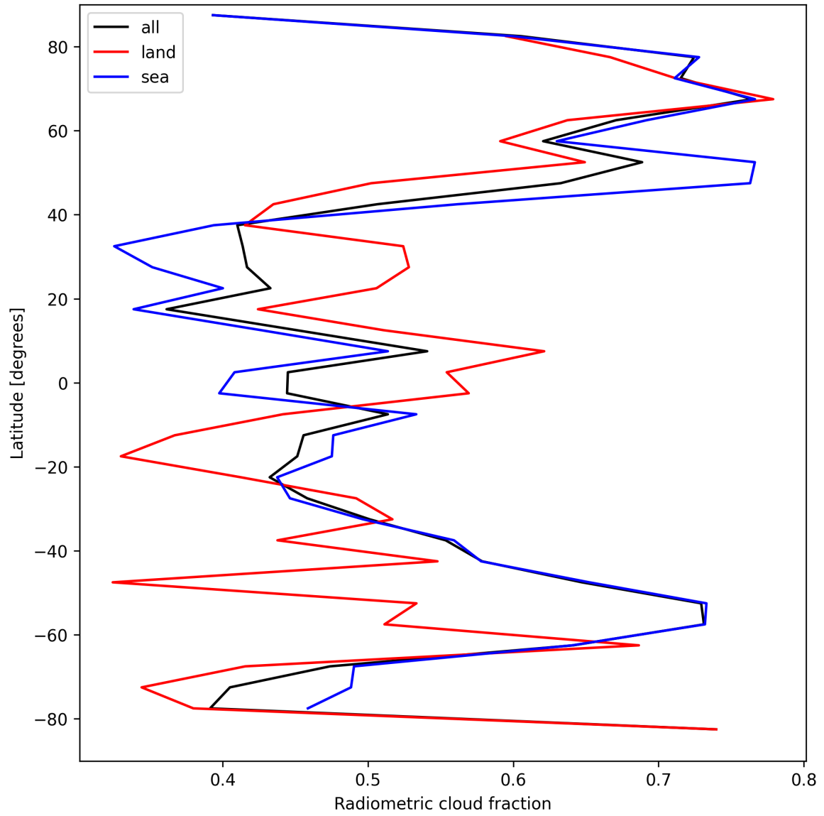
Figure 21: Zonal average of “Radiometric cloud fraction” for 2025-09-08 to 2025-09-08.
