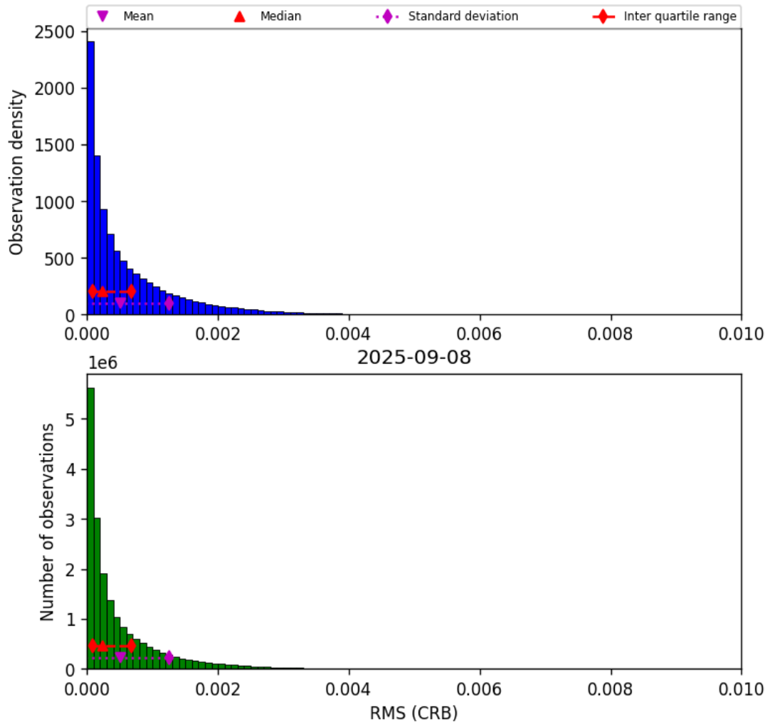
Figure 46: Histogram of “RMS (CRB)” for 2025-09-08 to 2025-09-08
