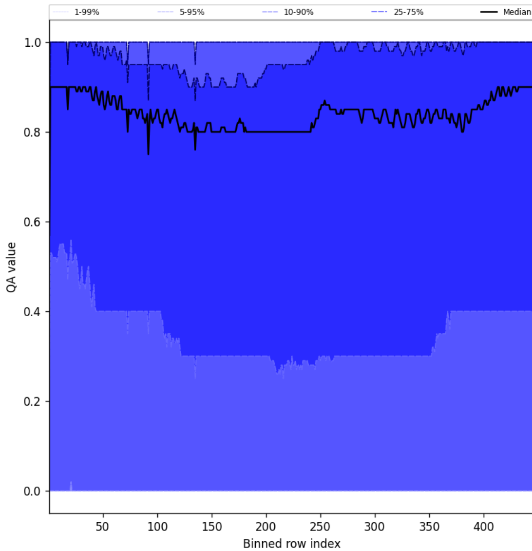
Figure 52: Along track statistics of “QA value” for 2025-09-08 to 2025-09-08
