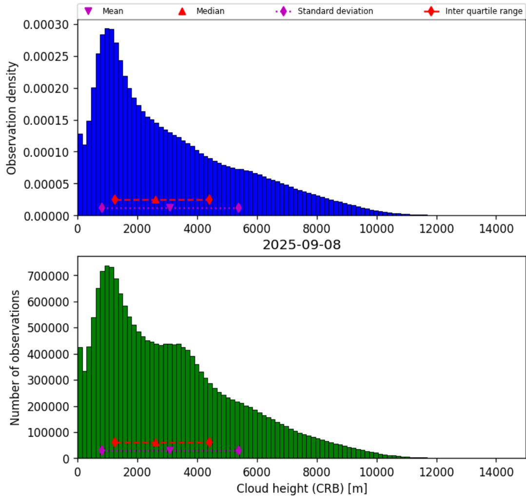
Figure 41: Histogram of “Cloud height (CRB)” for 2025-09-08 to 2025-09-08
