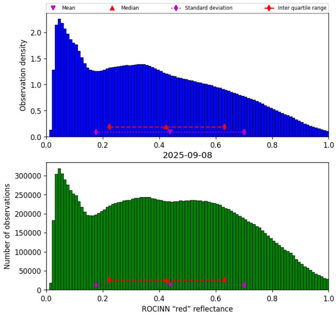
Figure 51: Histogram of “ROCINN “red” reflectance” for 2025-09-08 to 2025-09-08
