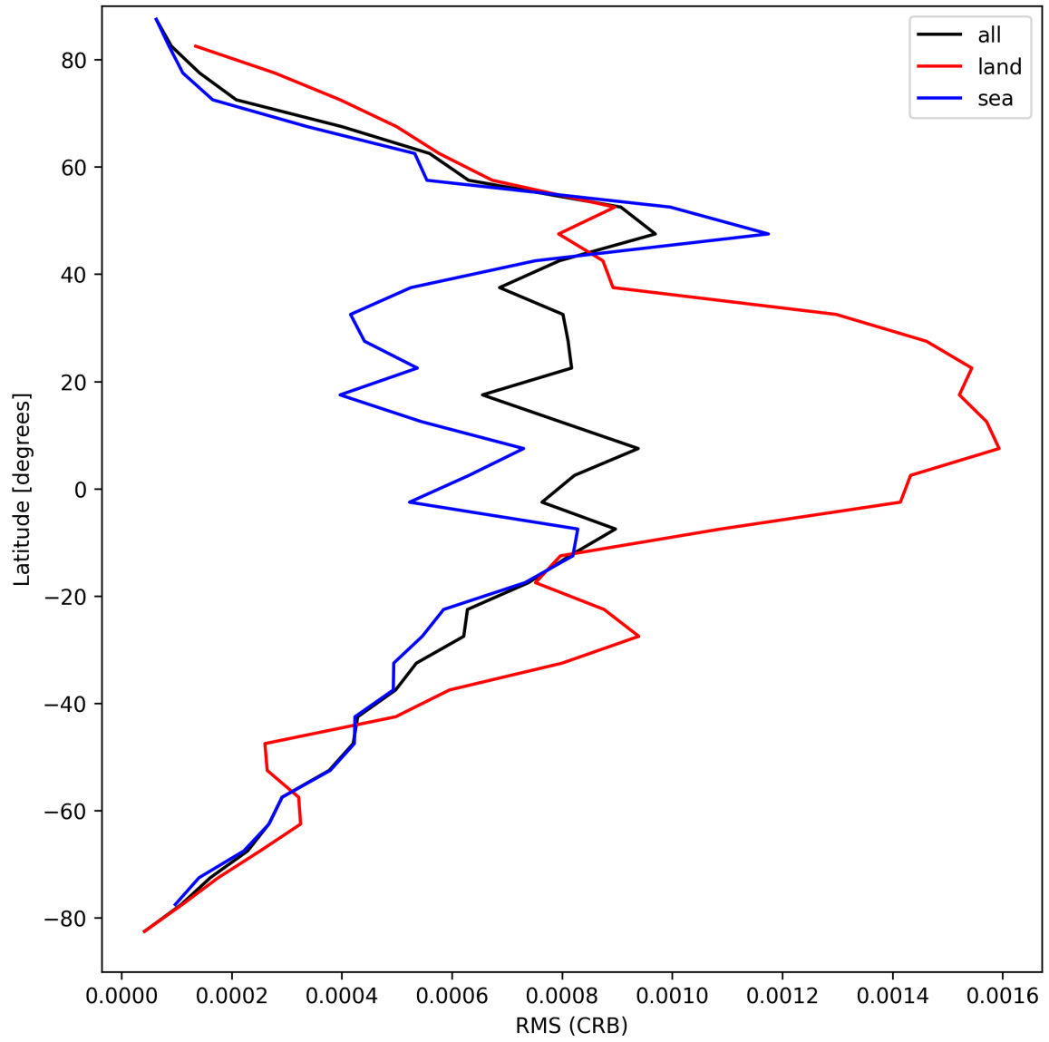
Figure 30: Zonal average of “RMS (CRB)” for 2025-09-08 to 2025-09-08.
