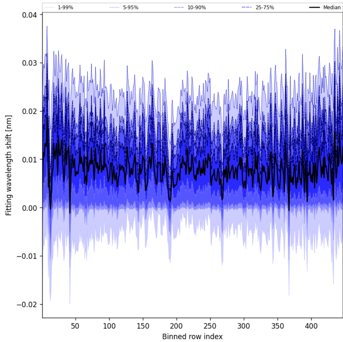
Figure 63: Along track statistics of “Fitting wavelength shift” for 2025-09-08 to 2025-09-08
