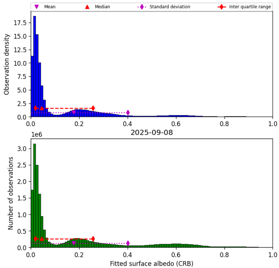
Figure 44: Histogram of “Fitted surface albedo (CRB)” for 2025-09-08 to 2025-09-08
