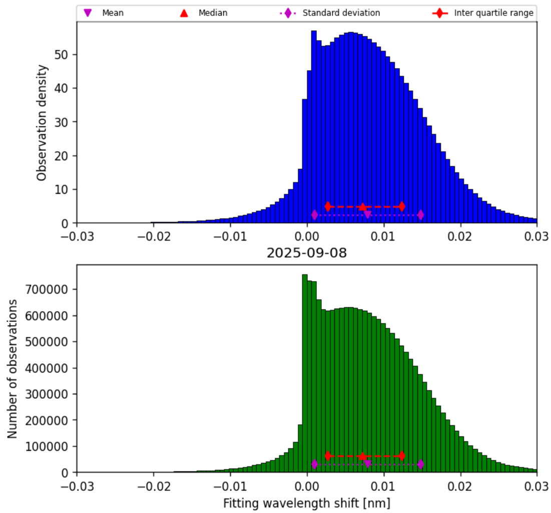
Figure 47: Histogram of “Fitting wavelength shift” for 2025-09-08 to 2025-09-08
