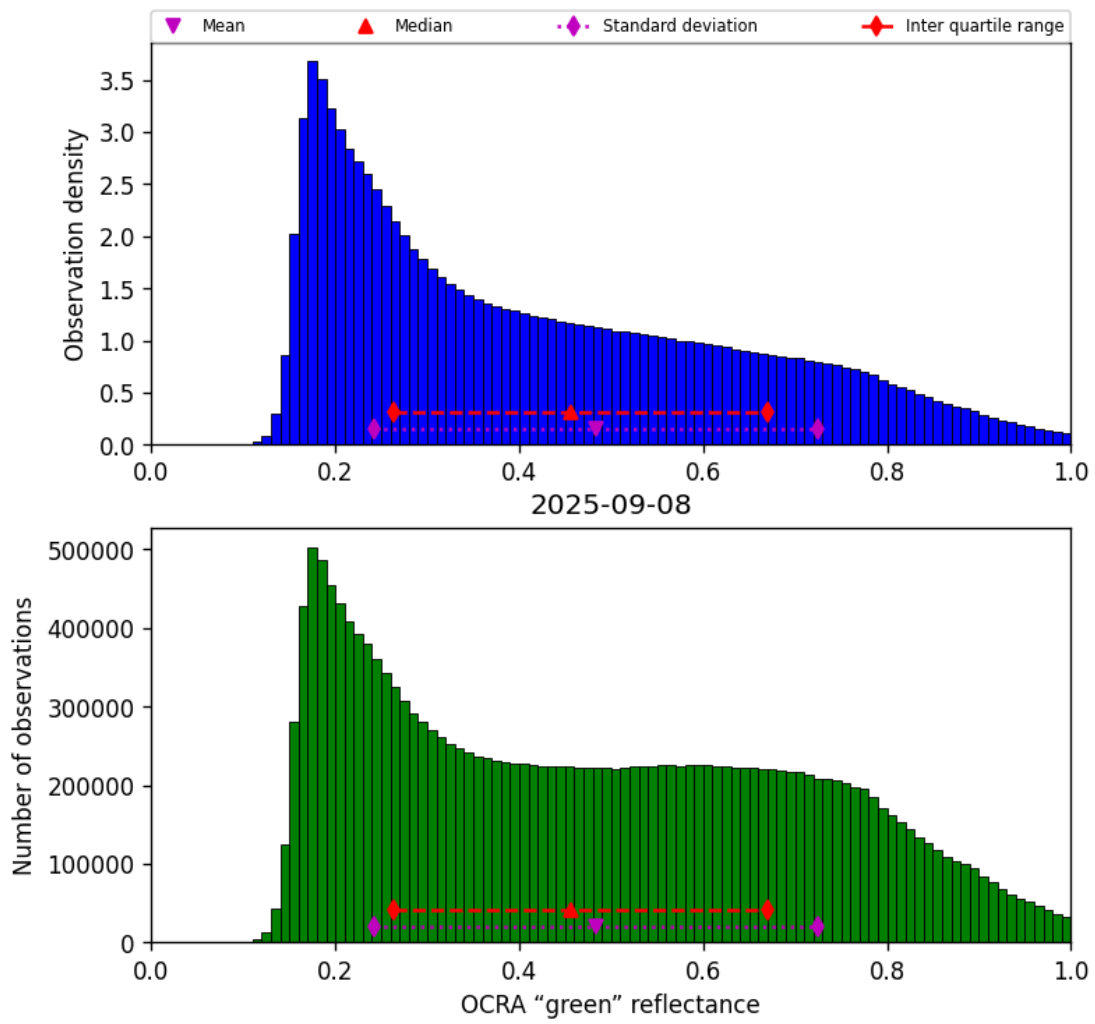
Figure 50: Histogram of “OCRA “green” reflectance” for 2025-09-08 to 2025-09-08
