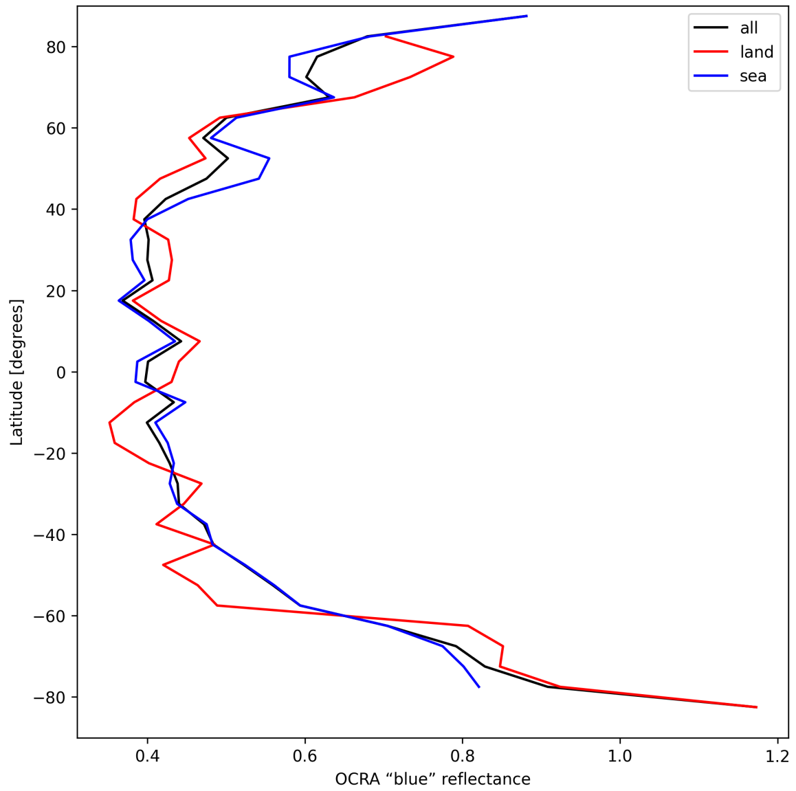
Figure 33: Zonal average of “OCRA “blue” reflectance” for 2025-09-08 to 2025-09-08.
