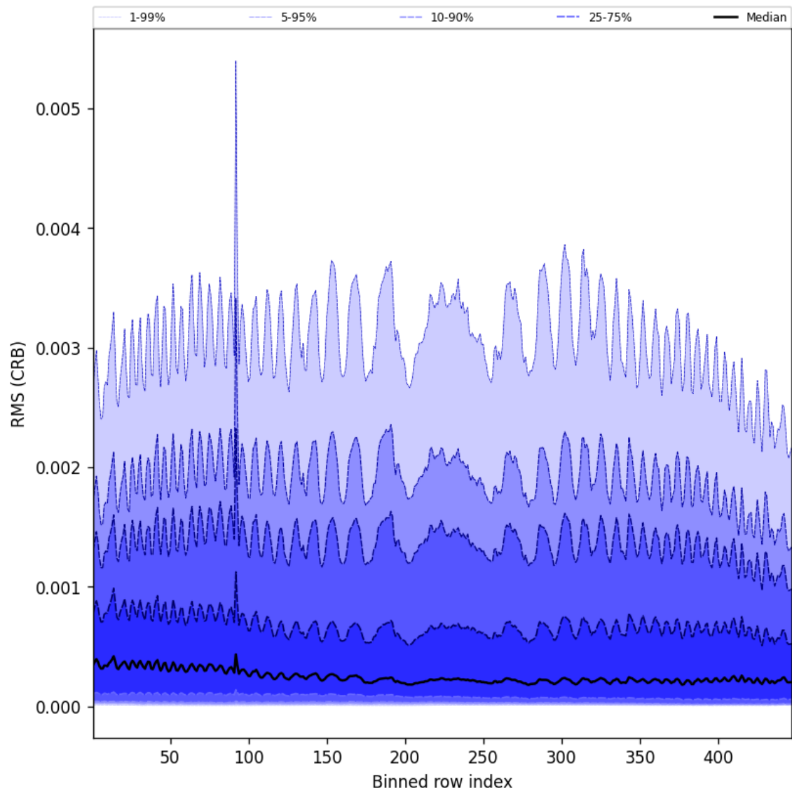
Figure 62: Along track statistics of “RMS (CRB)” for 2025-09-08 to 2025-09-08
