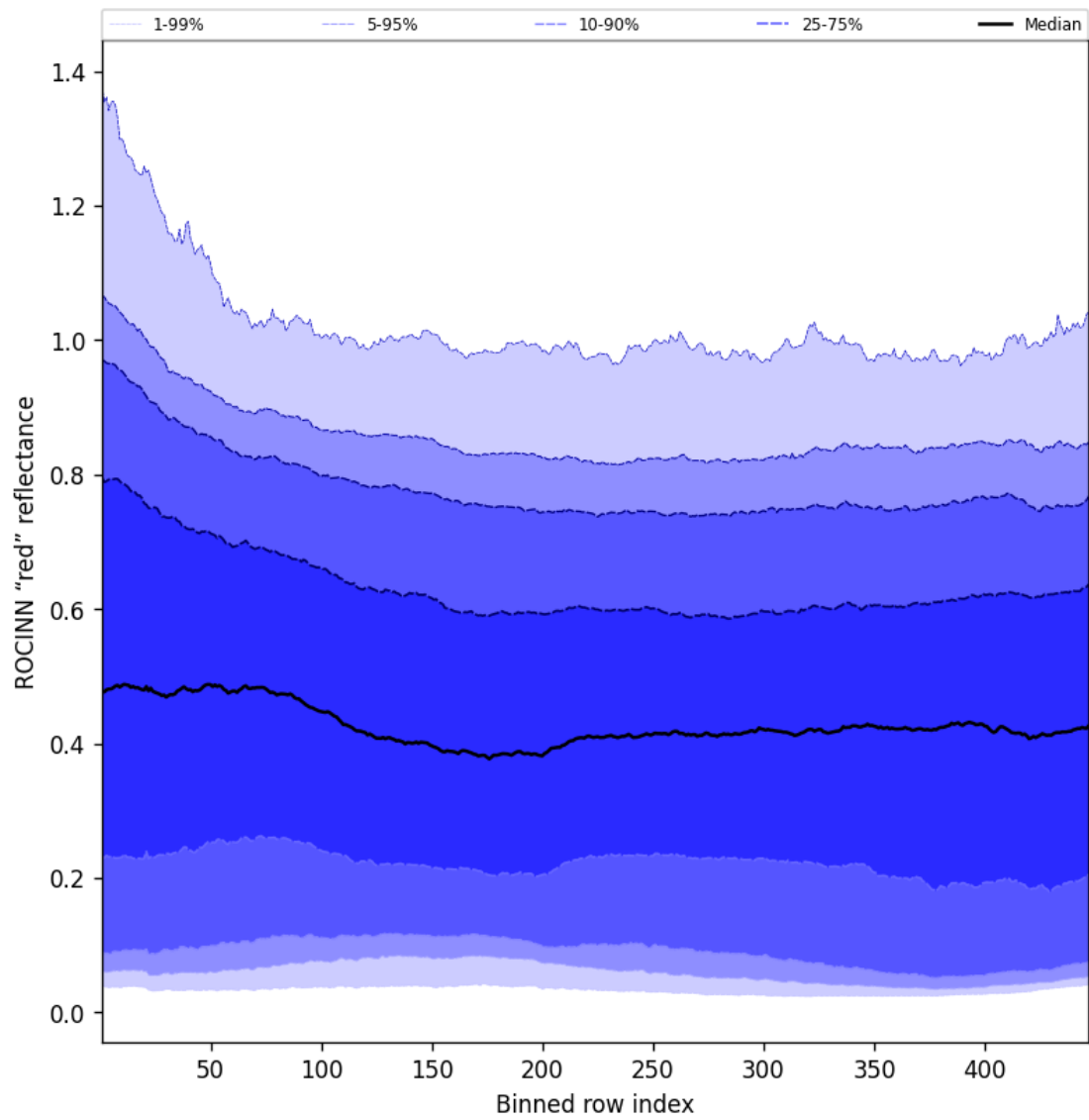
Figure 67: Along track statistics of “ROCINN “red” reflectance” for 2025-09-08 to 2025-09-08
