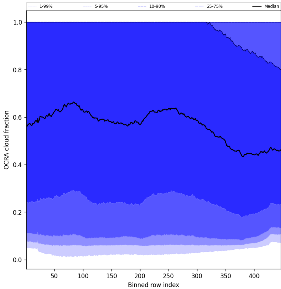
Figure 64: Along track statistics of “OCRA cloud fraction” for 2025-09-08 to 2025-09-08
