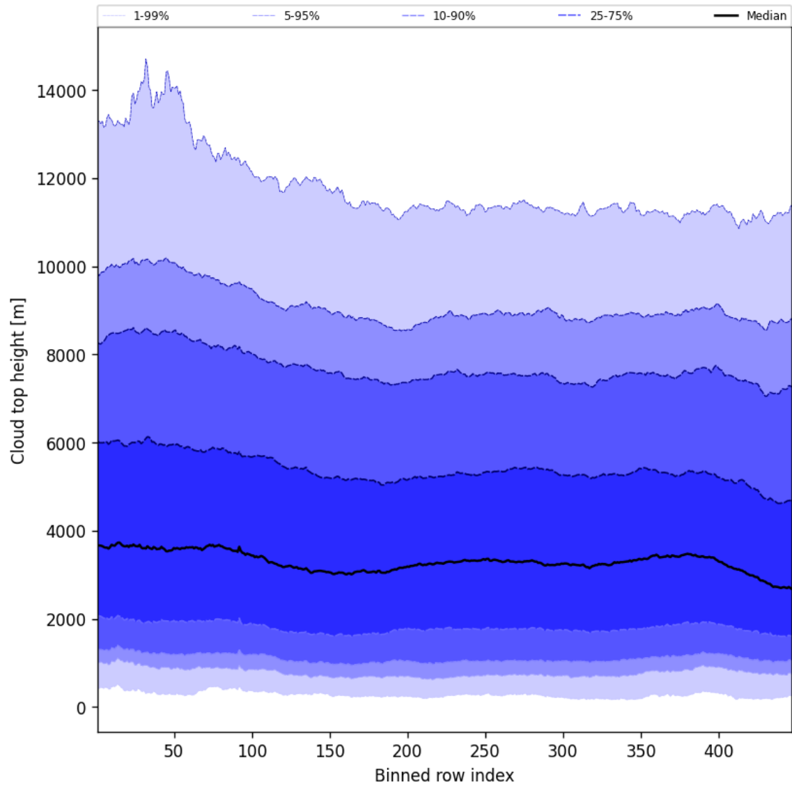
Figure 54: Along track statistics of “Cloud top height” for 2025-09-08 to 2025-09-08
