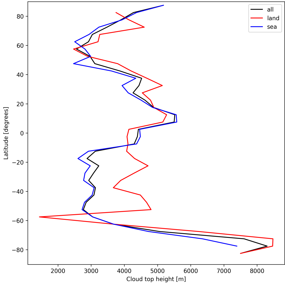
Figure 22: Zonal average of “Cloud top height” for 2025-09-08 to 2025-09-08.
