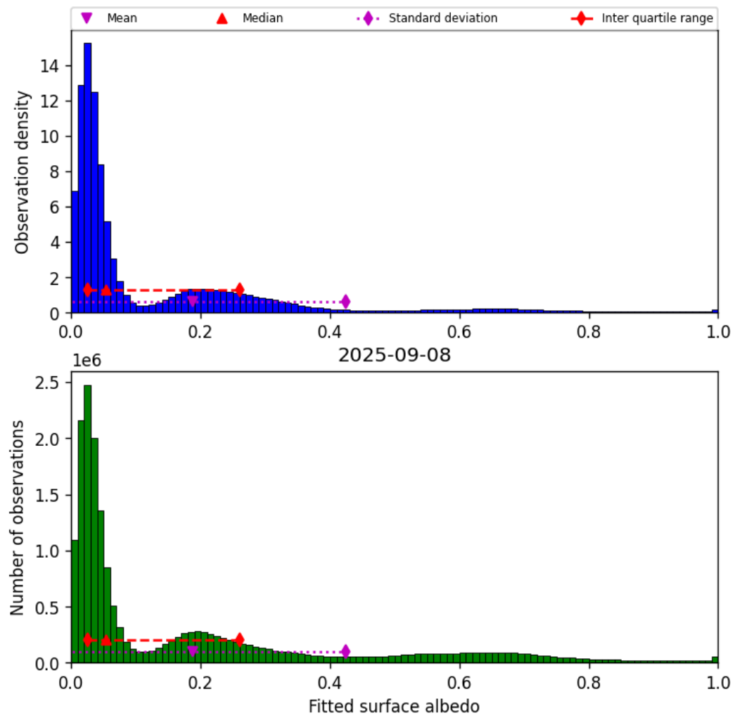
Figure 43: Histogram of “Fitted surface albedo” for 2025-09-08 to 2025-09-08
