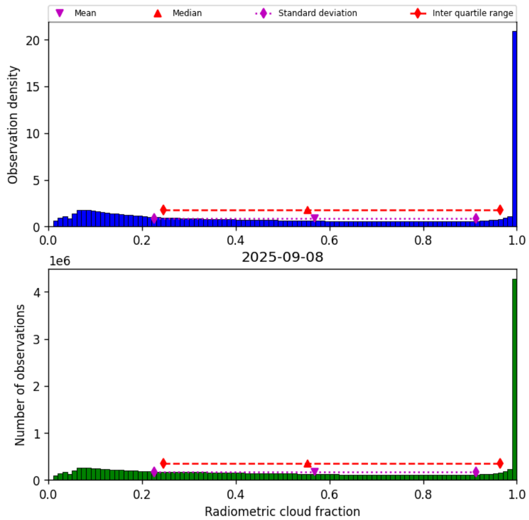
Figure 37: Histogram of “Radiometric cloud fraction” for 2025-09-08 to 2025-09-08
