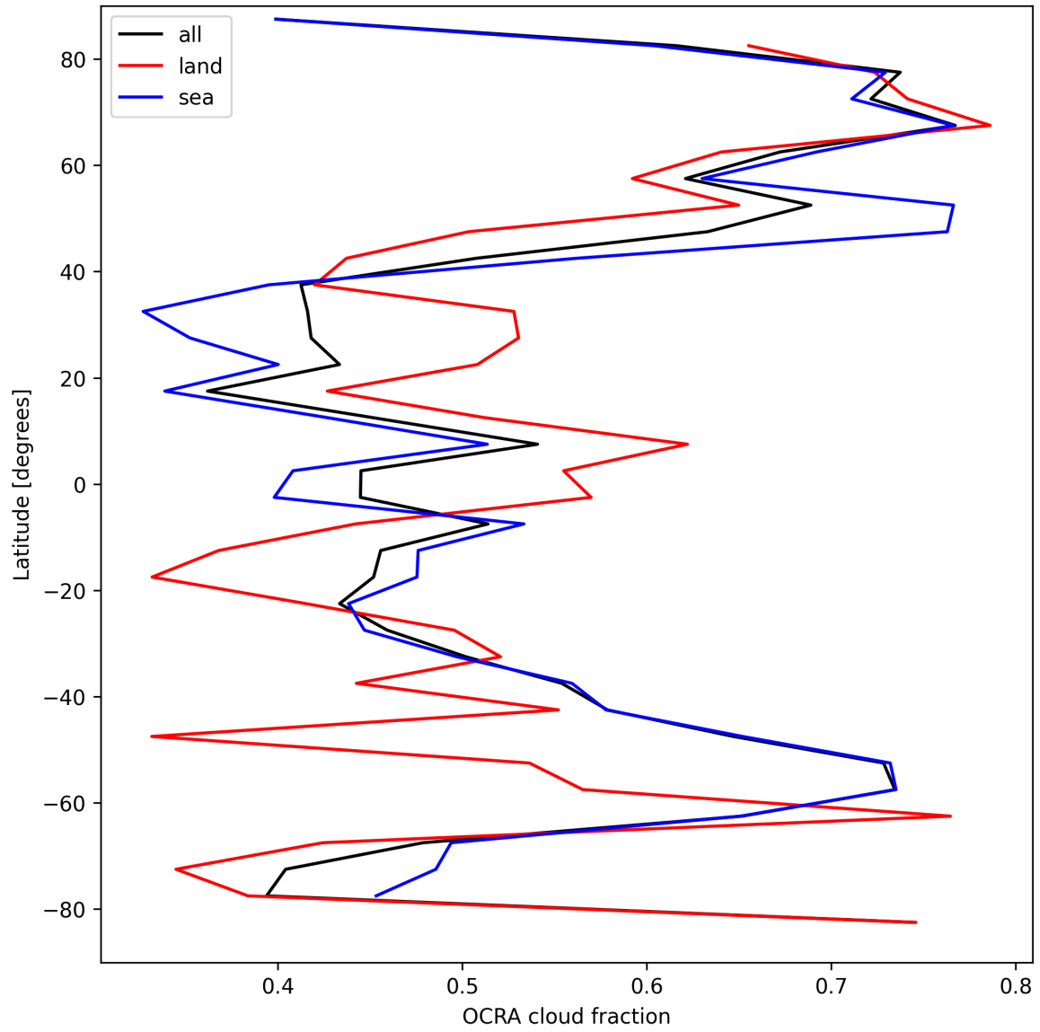
Figure 32: Zonal average of “OCRA cloud fraction” for 2025-09-08 to 2025-09-08.
