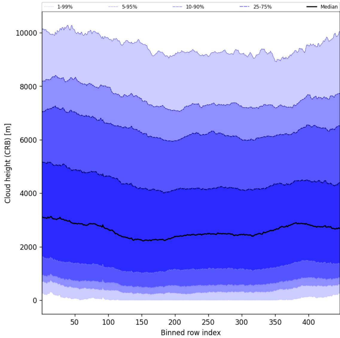
Figure 57: Along track statistics of “Cloud height (CRB)” for 2025-09-08 to 2025-09-08
