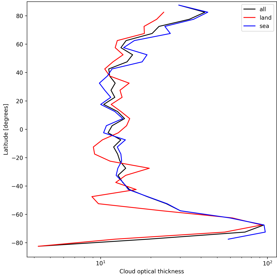
Figure 23: Zonal average of “Cloud optical thickness” for 2025-09-08 to 2025-09-08.
