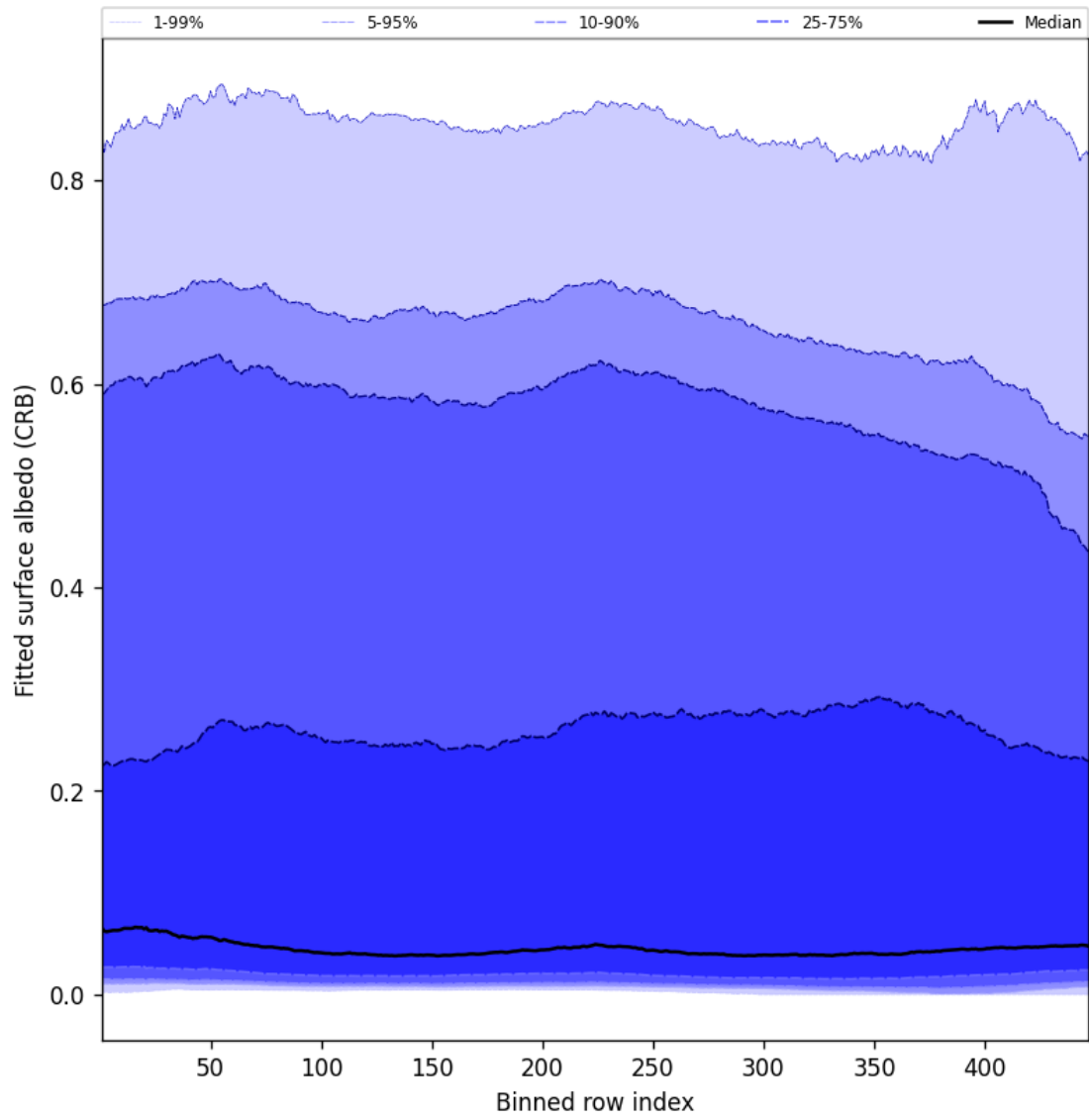
Figure 60: Along track statistics of “Fitted surface albedo (CRB)” for 2025-09-08 to 2025-09-08
