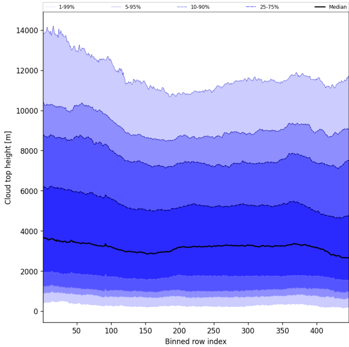
Figure 54: Along track statistics of “Cloud top height” for 2025-09-10 to 2025-09-11
