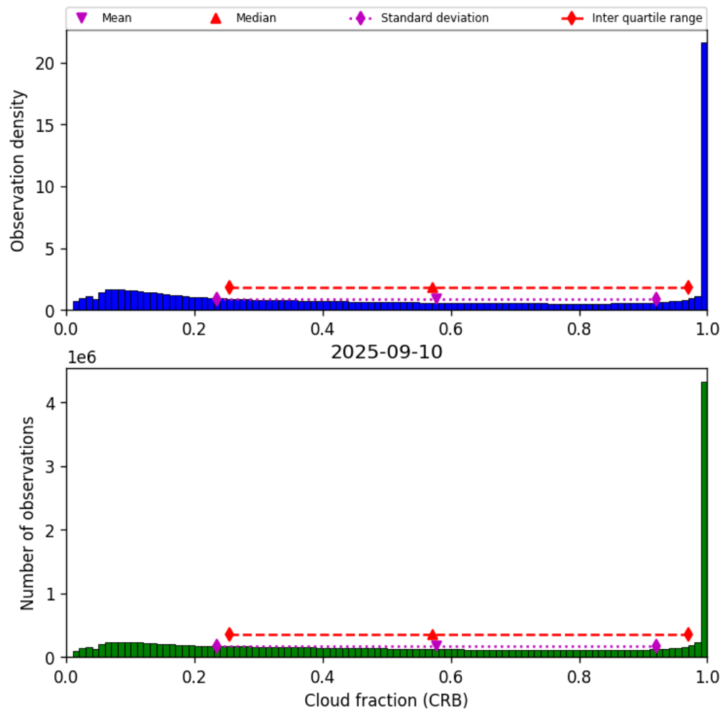
Figure 40: Histogram of “Cloud fraction (CRB)” for 2025-09-10 to 2025-09-11
