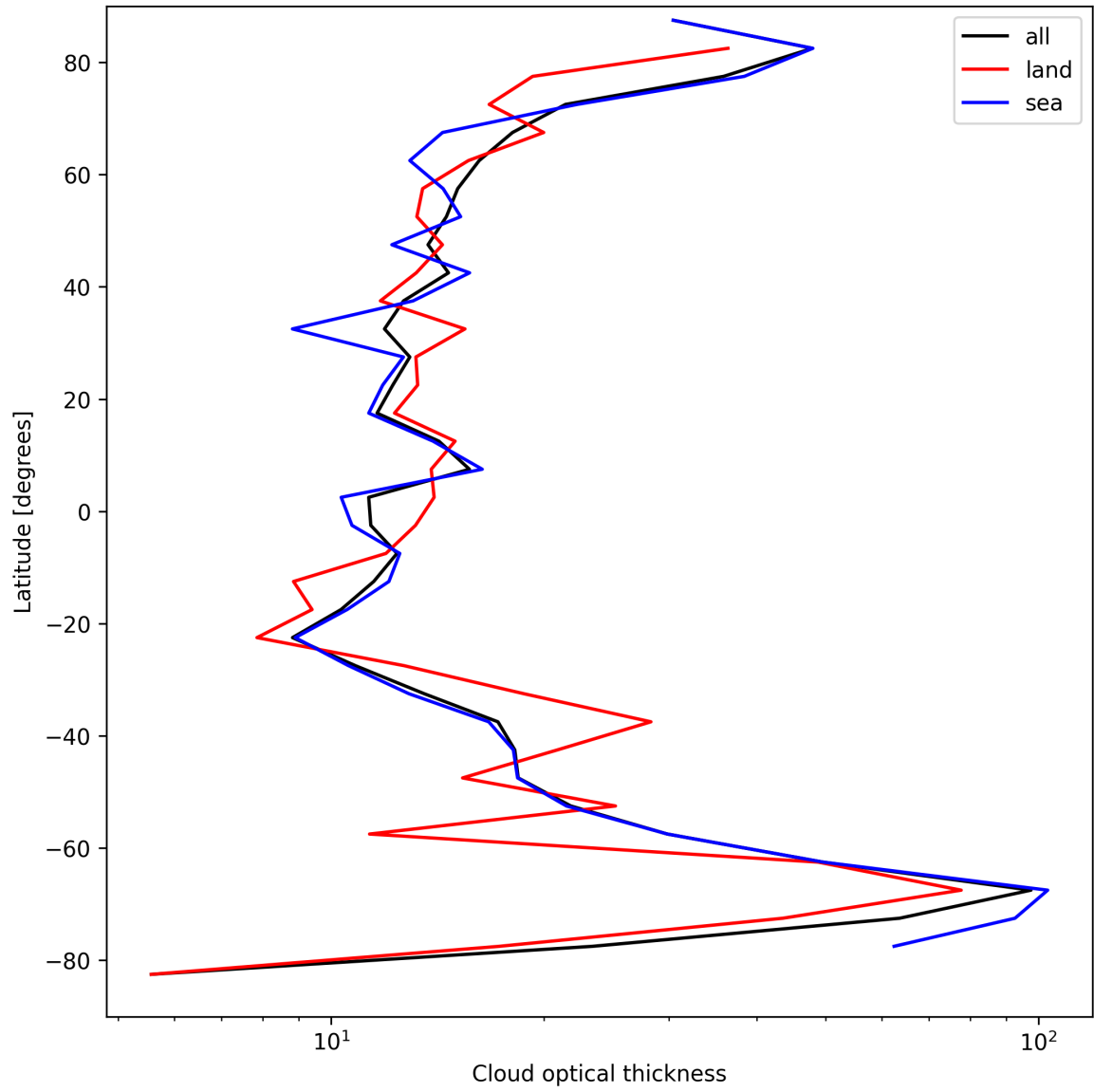
Figure 23: Zonal average of “Cloud optical thickness” for 2025-09-10 to 2025-09-11.
