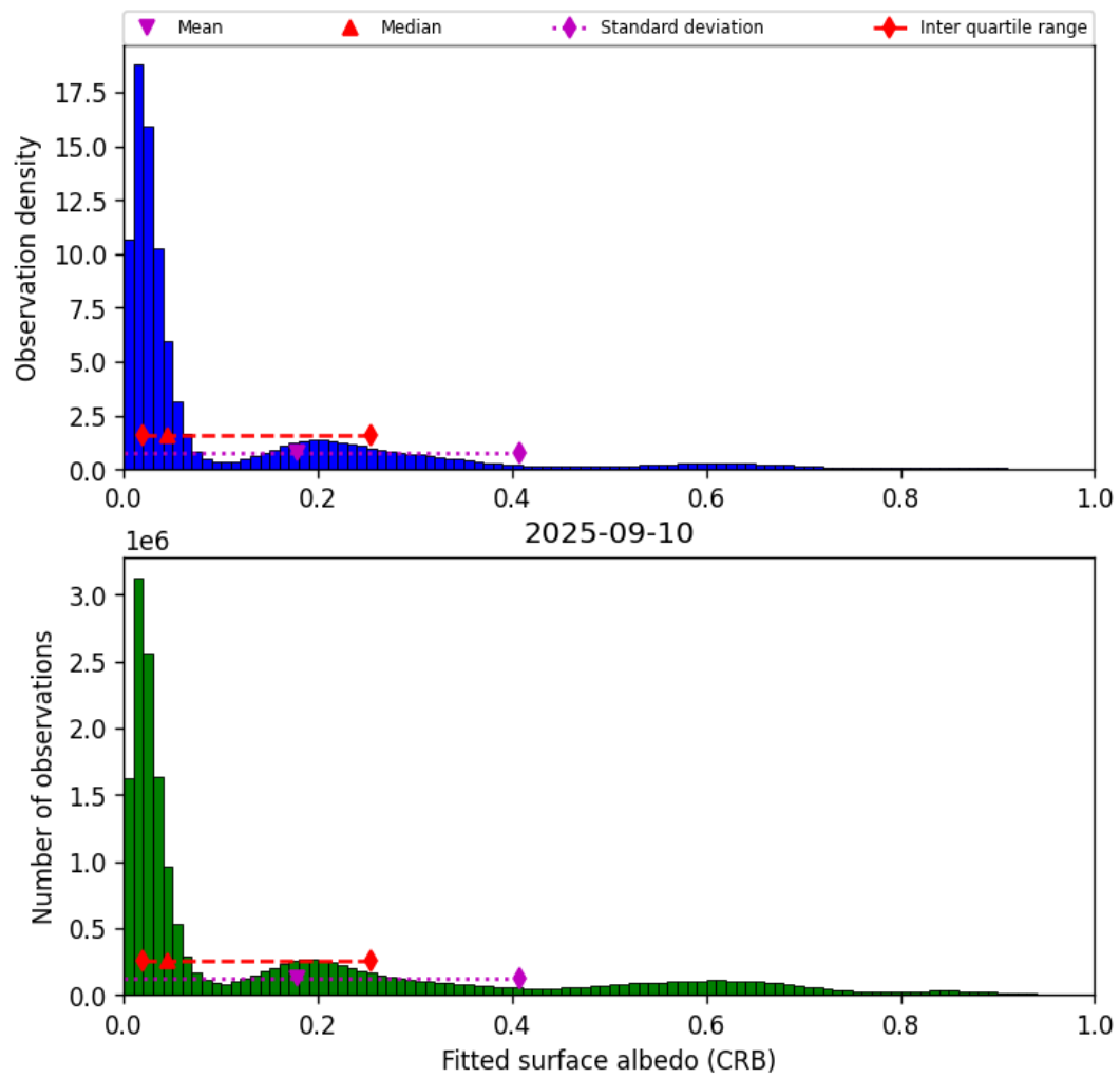
Figure 44: Histogram of “Fitted surface albedo (CRB)” for 2025-09-10 to 2025-09-11
