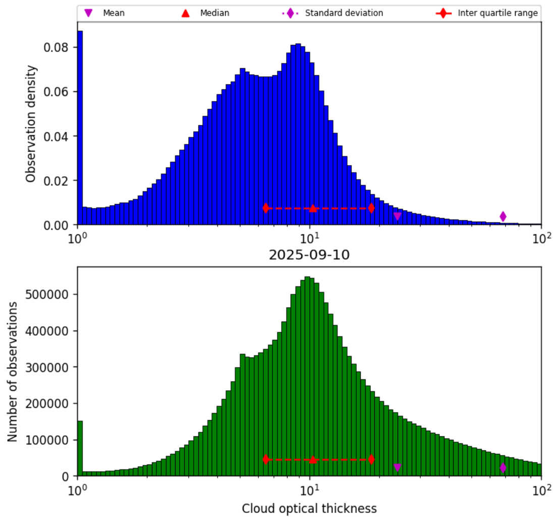
Figure 39: Histogram of “Cloud optical thickness” for 2025-09-10 to 2025-09-11
