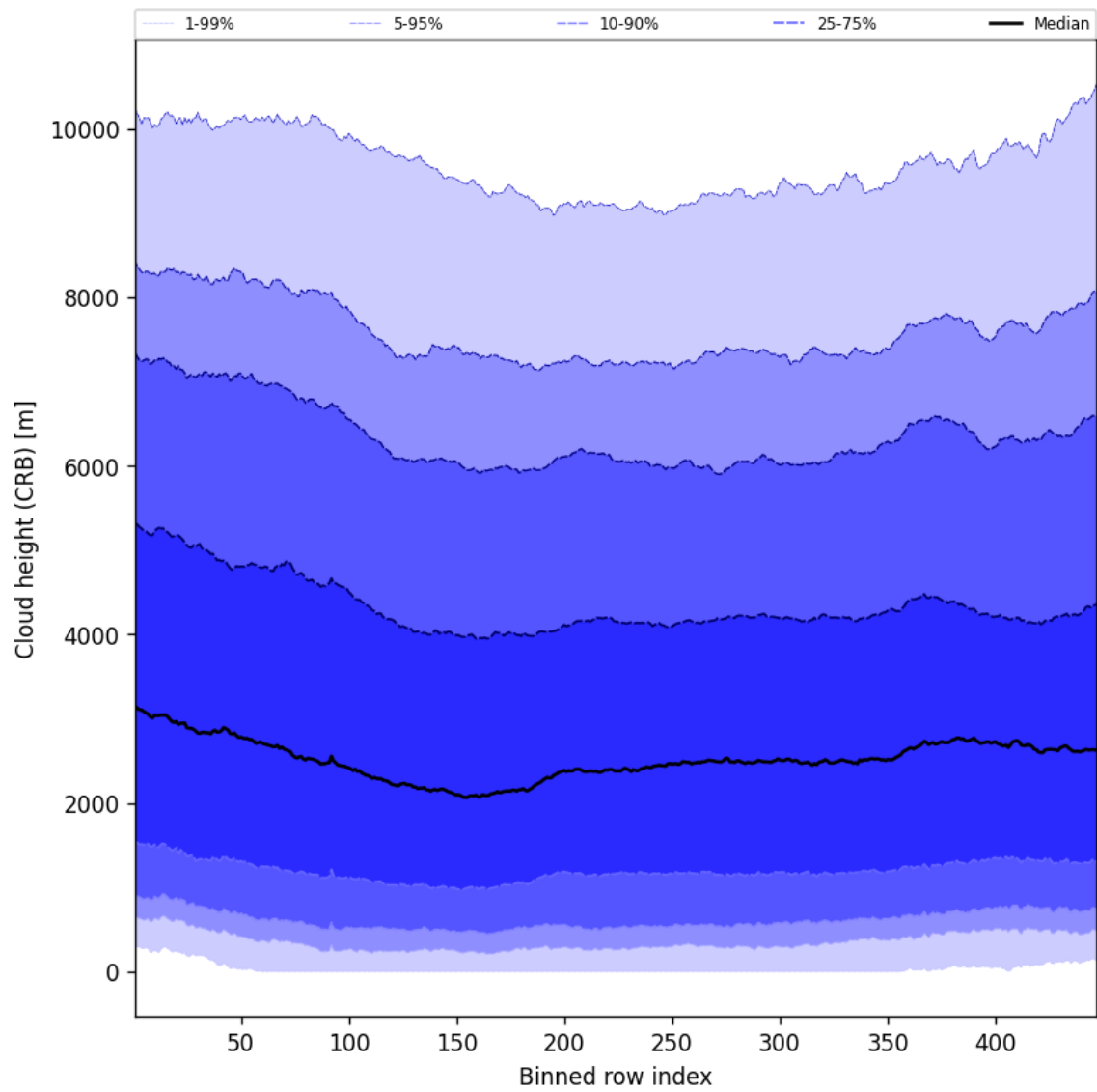
Figure 57: Along track statistics of “Cloud height (CRB)” for 2025-09-10 to 2025-09-11
