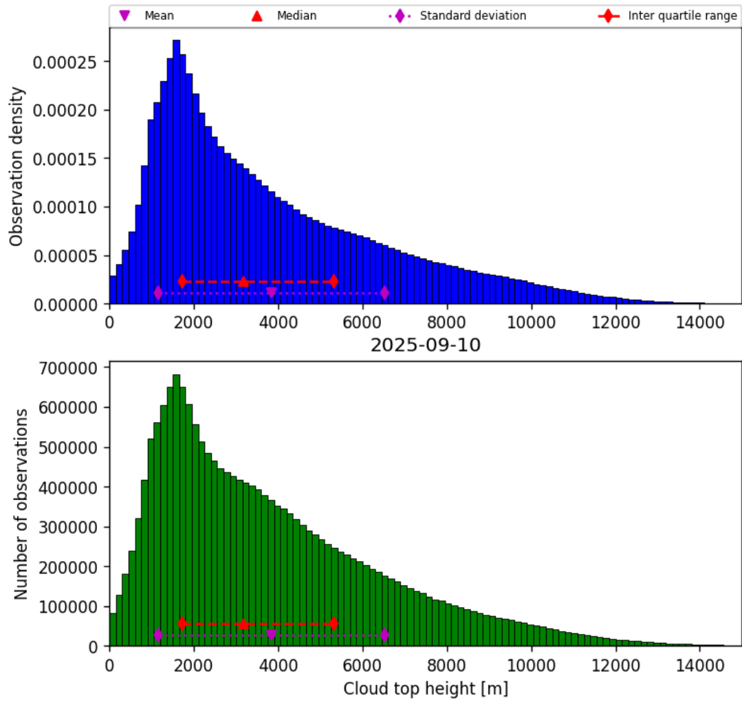
Figure 38: Histogram of “Cloud top height” for 2025-09-10 to 2025-09-11
