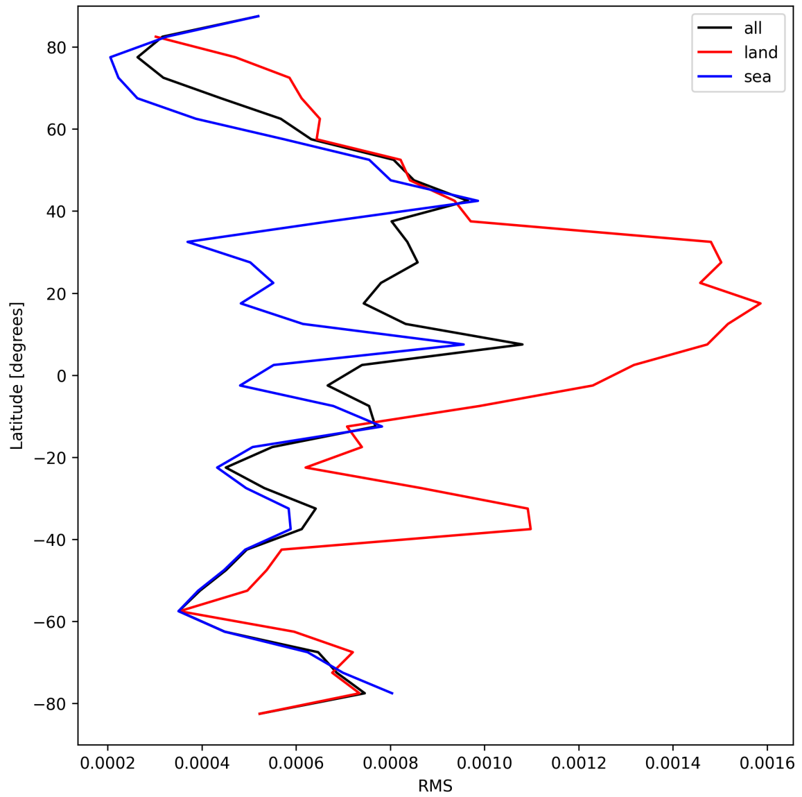
Figure 29: Zonal average of “RMS” for 2025-09-10 to 2025-09-11.
