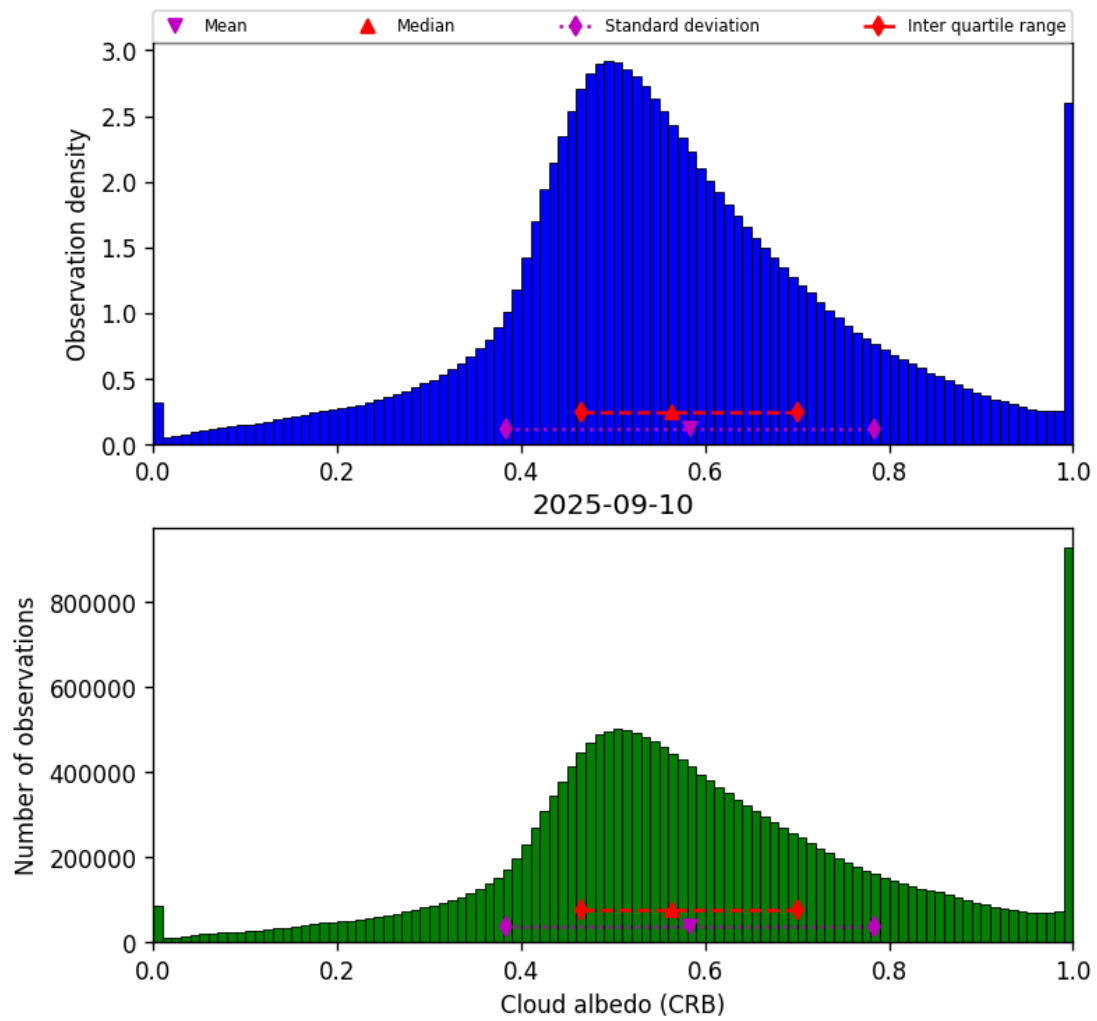
Figure 42: Histogram of “Cloud albedo (CRB)” for 2025-09-10 to 2025-09-11
