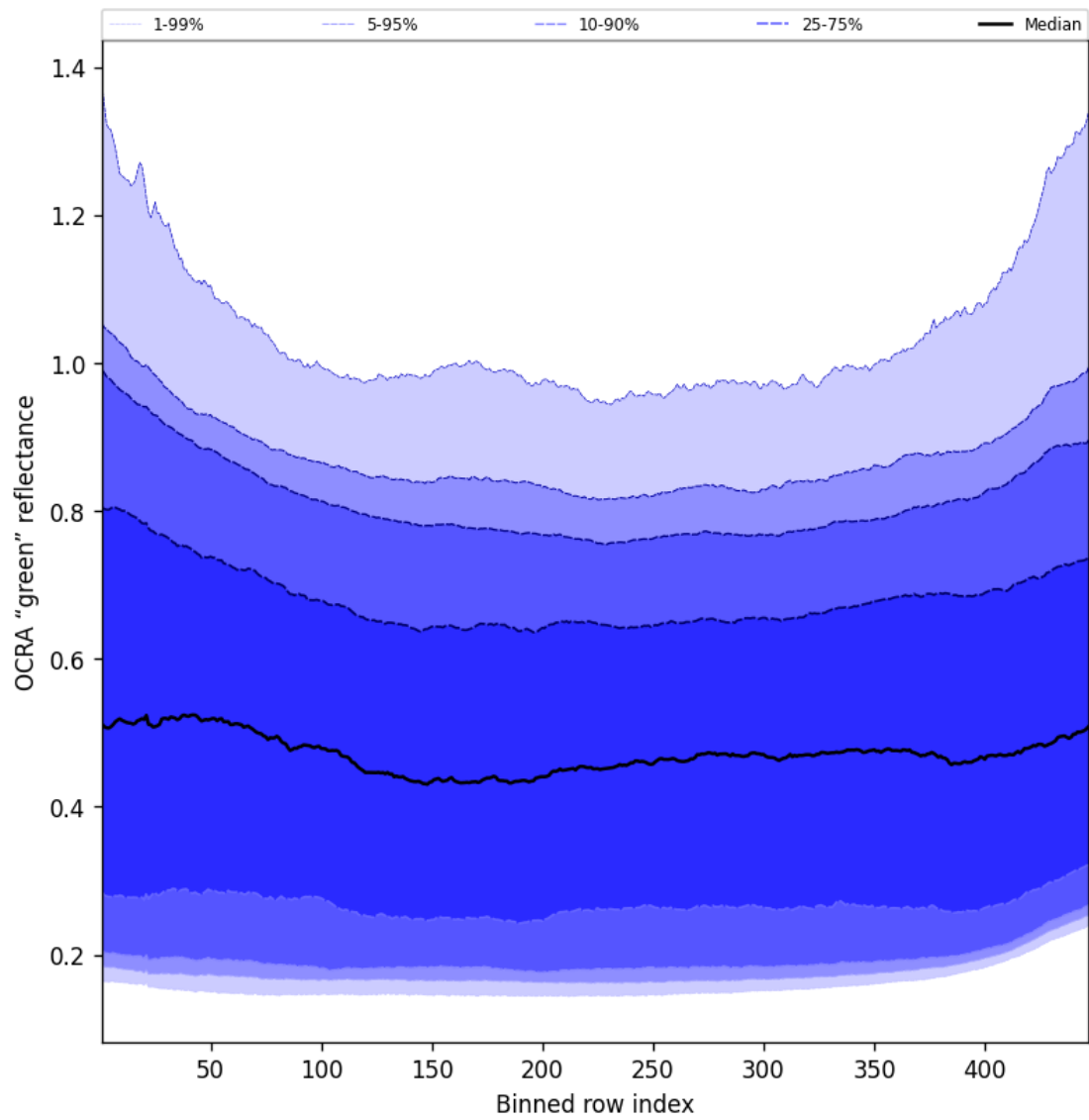
Figure 66: Along track statistics of “OCRA “green” reflectance” for 2025-09-10 to 2025-09-11
