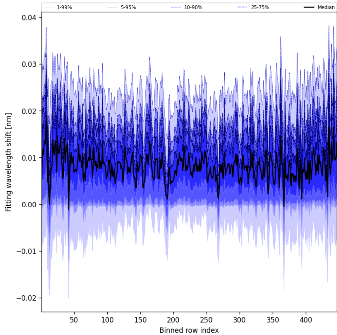
Figure 63: Along track statistics of “Fitting wavelength shift” for 2025-09-10 to 2025-09-11
