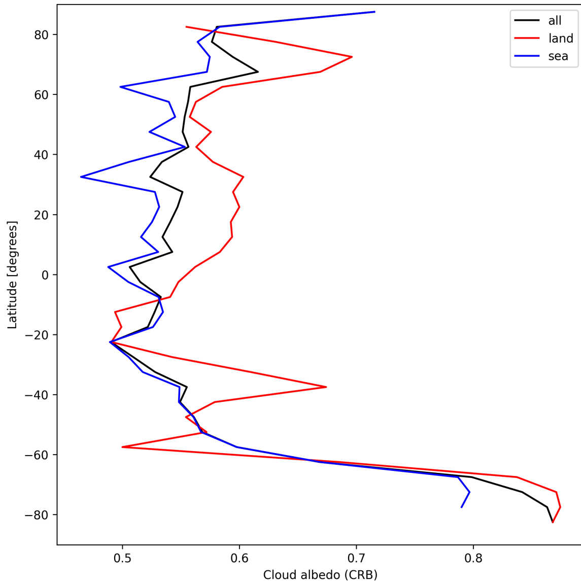
Figure 26: Zonal average of “Cloud albedo (CRB)” for 2025-09-10 to 2025-09-11.
