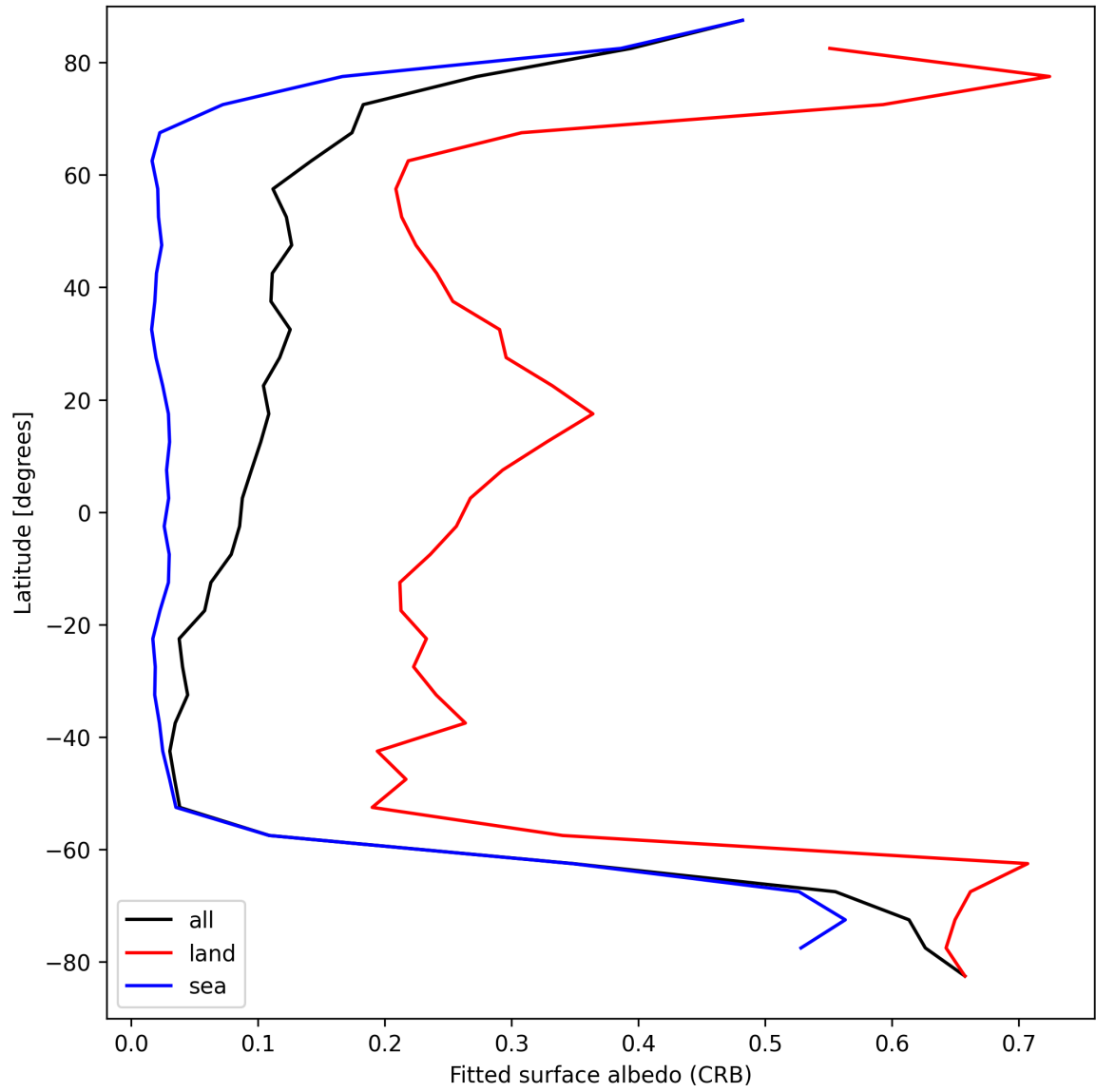
Figure 28: Zonal average of “Fitted surface albedo (CRB)” for 2025-09-10 to 2025-09-11.
