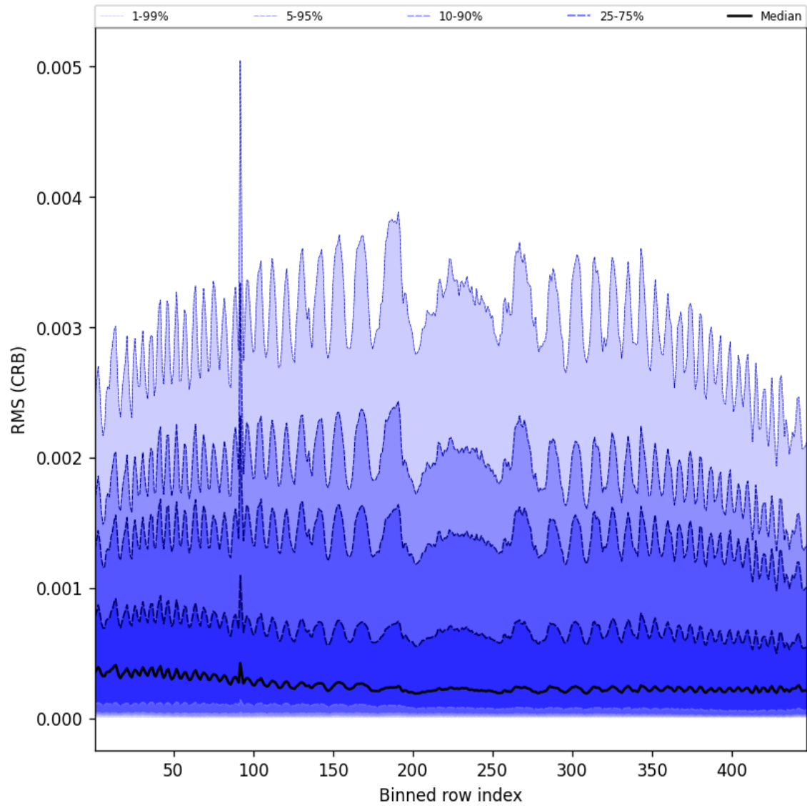
Figure 62: Along track statistics of “RMS (CRB)” for 2025-09-10 to 2025-09-11
