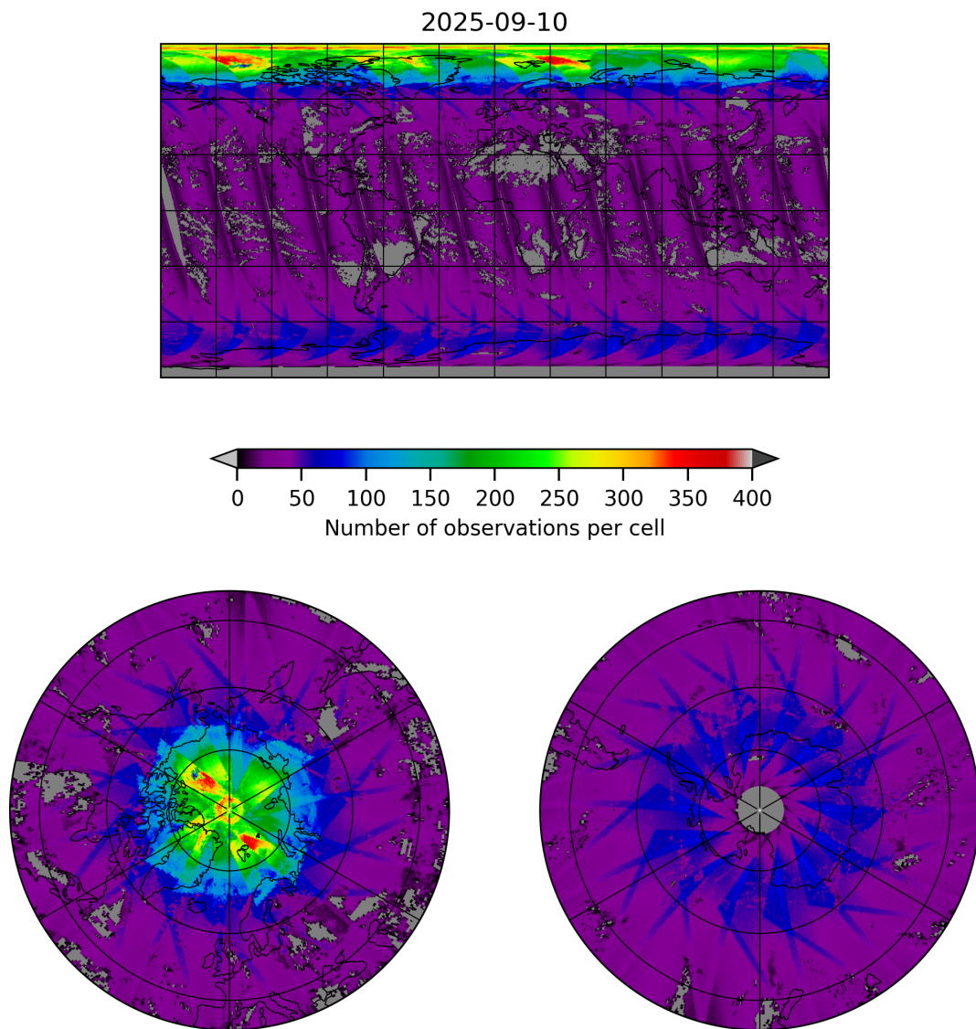
Figure 19: Map of the number of observations for 2025-09-10 to 2025-09-11
