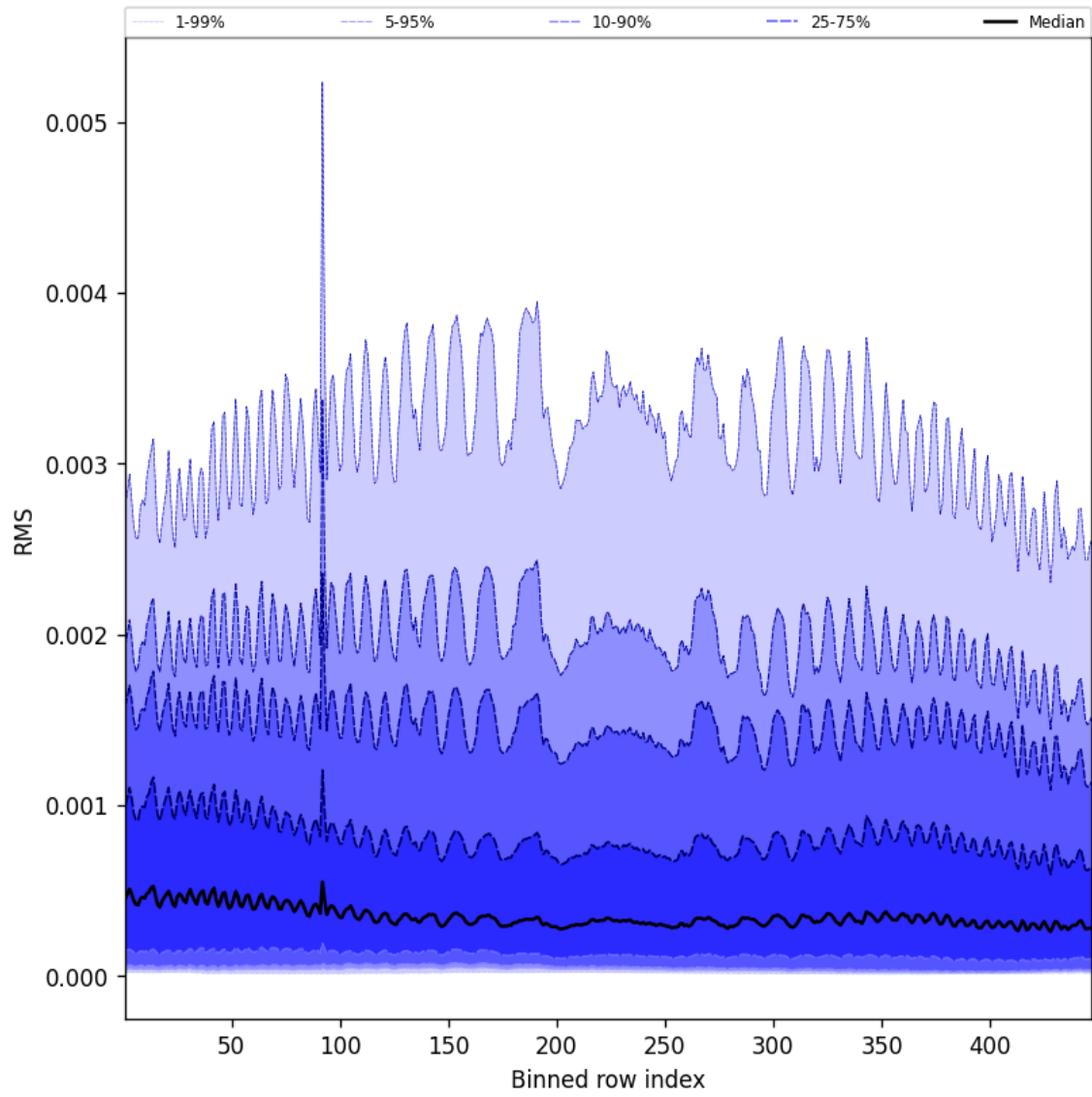
Figure 61: Along track statistics of “RMS” for 2025-09-10 to 2025-09-11
