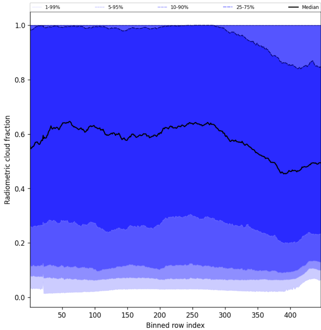
Figure 53: Along track statistics of “Radiometric cloud fraction” for 2025-09-10 to 2025-09-11
