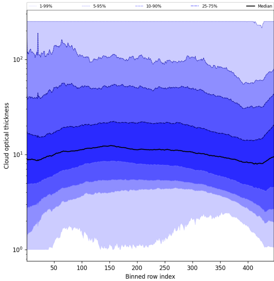
Figure 55: Along track statistics of “Cloud optical thickness” for 2025-09-10 to 2025-09-11
