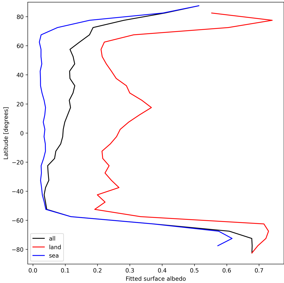
Figure 27: Zonal average of “Fitted surface albedo” for 2025-09-10 to 2025-09-11.
