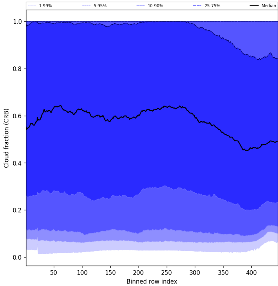
Figure 56: Along track statistics of “Cloud fraction (CRB)” for 2025-09-10 to 2025-09-11
