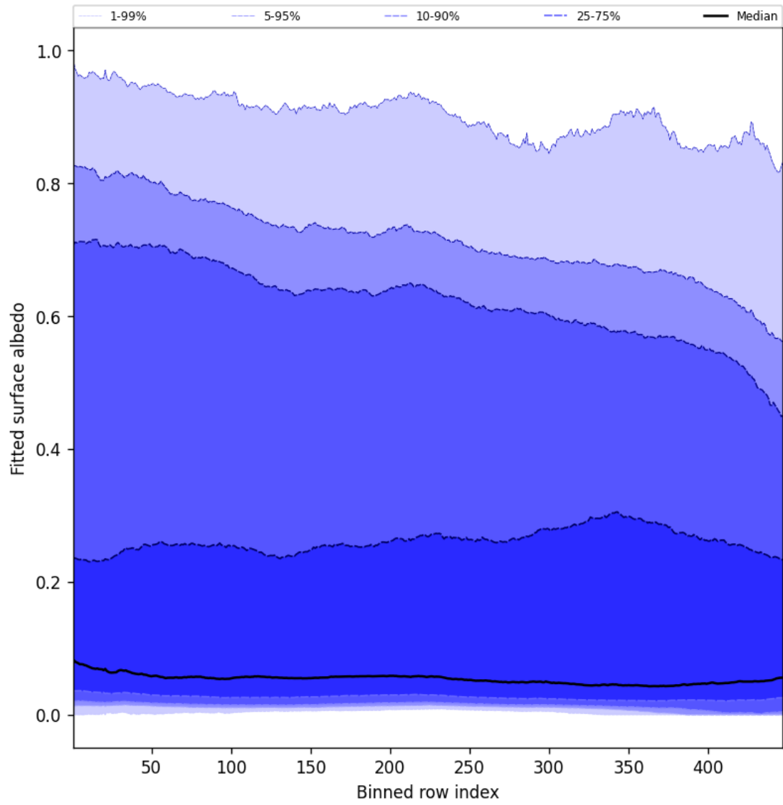
Figure 59: Along track statistics of “Fitted surface albedo” for 2025-09-10 to 2025-09-11
