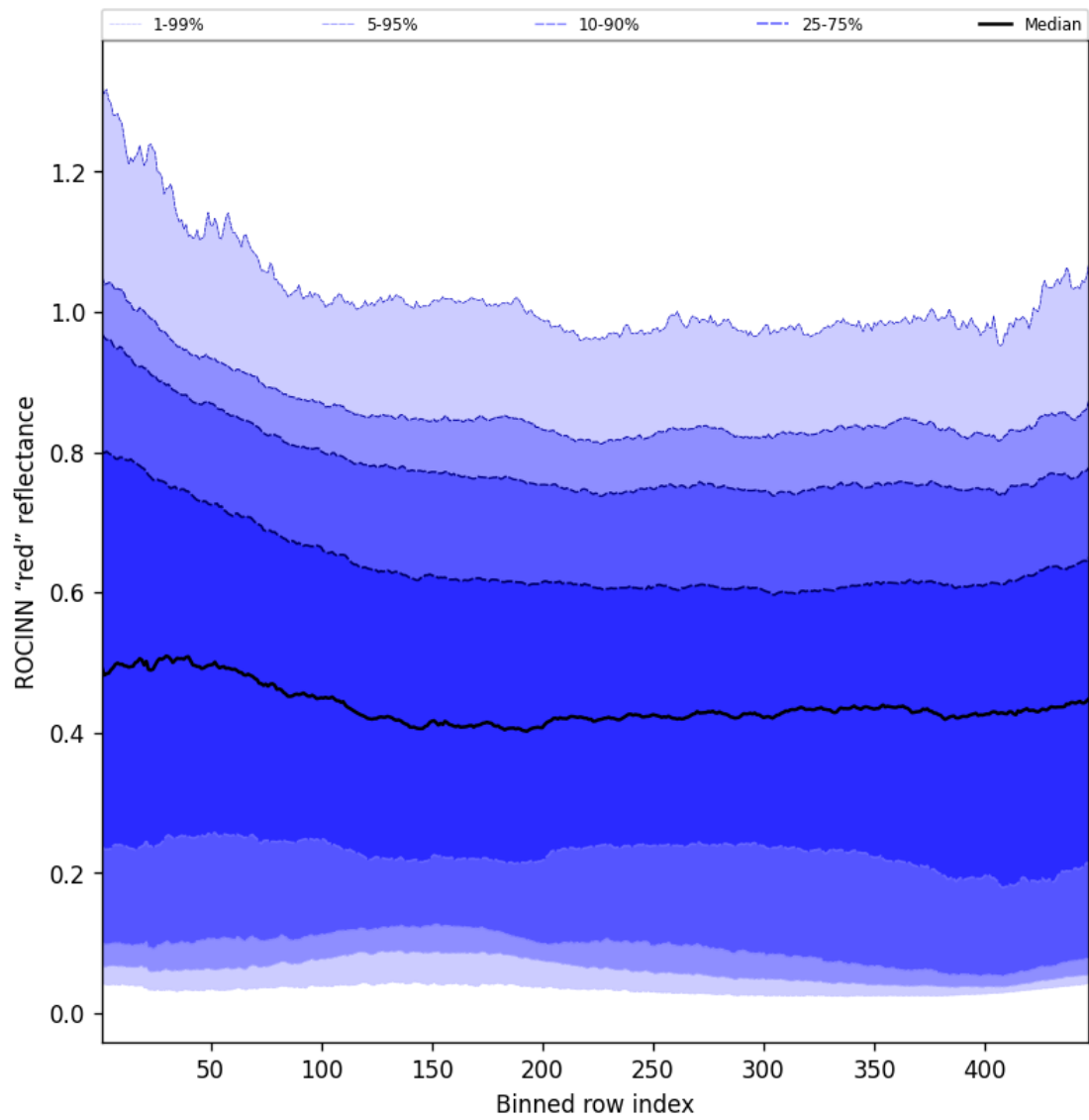
Figure 67: Along track statistics of “ROCINN “red” reflectance” for 2025-09-10 to 2025-09-11
