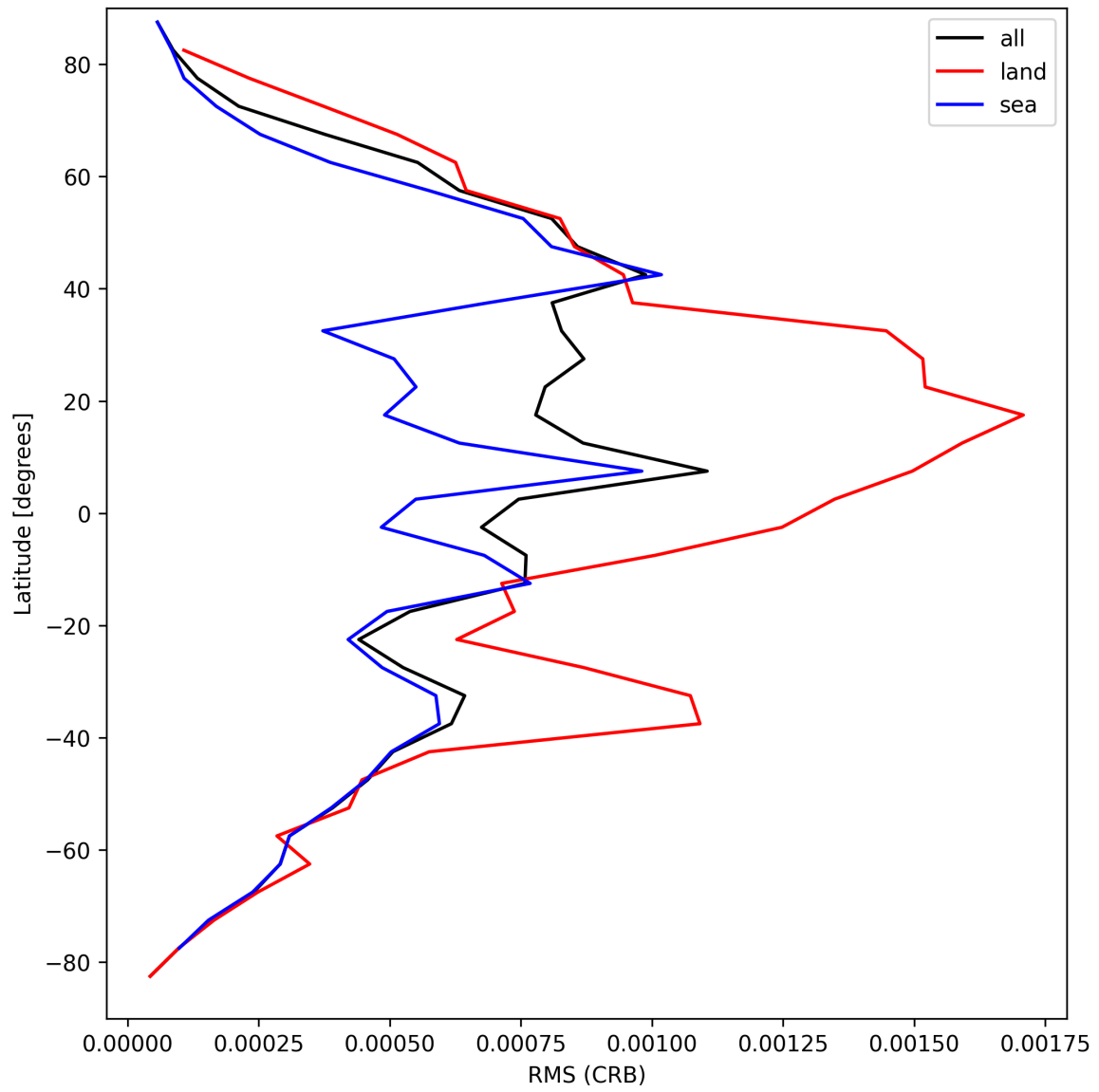
Figure 30: Zonal average of “RMS (CRB)” for 2025-09-10 to 2025-09-11.
