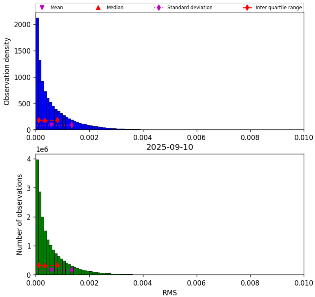
Figure 45: Histogram of “RMS” for 2025-09-10 to 2025-09-11
