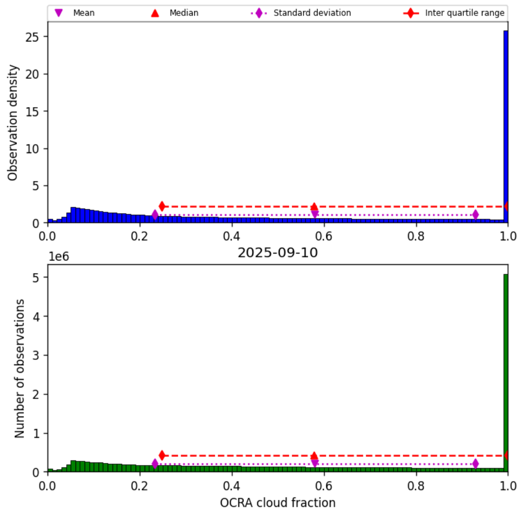
Figure 48: Histogram of “OCRA cloud fraction” for 2025-09-10 to 2025-09-11
