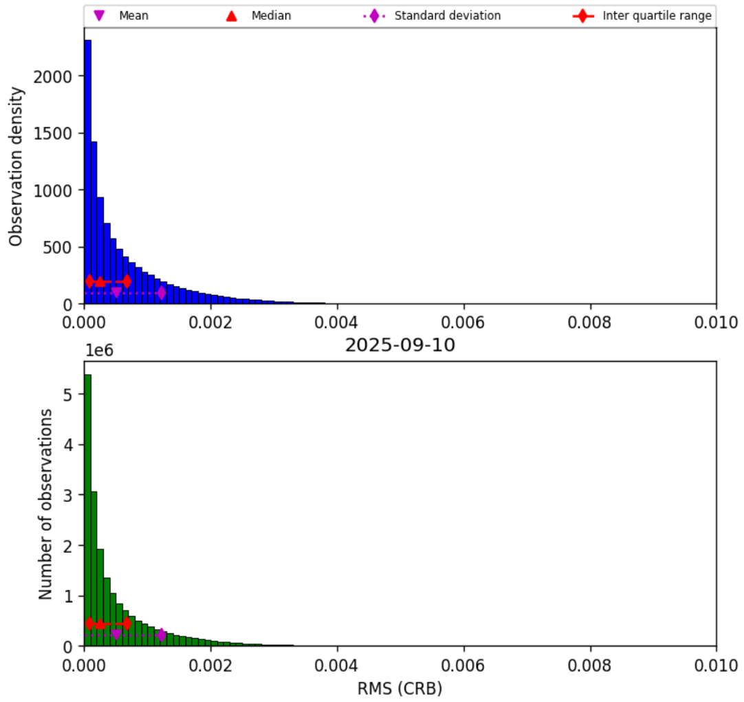
Figure 46: Histogram of “RMS (CRB)” for 2025-09-10 to 2025-09-11
