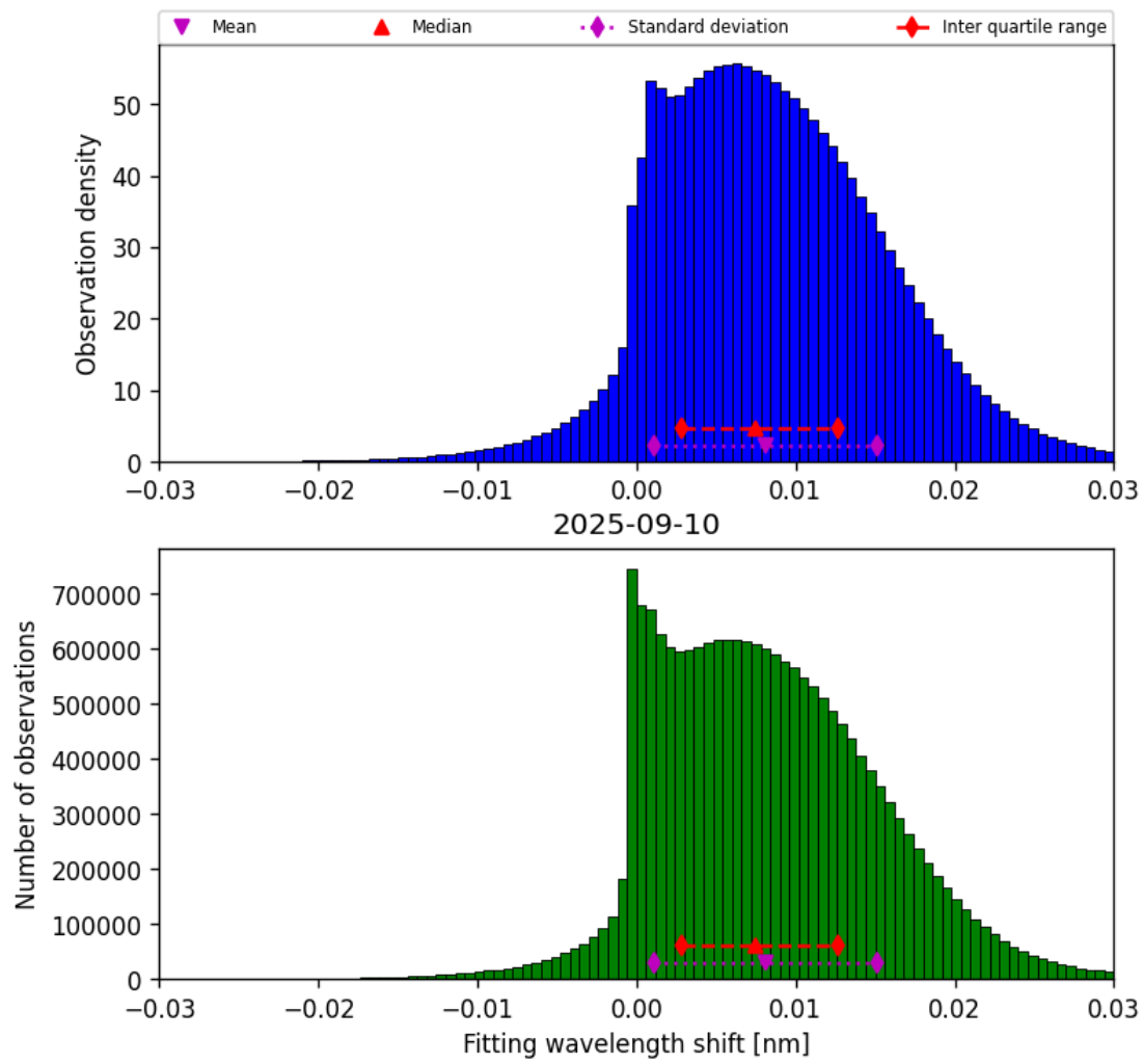
Figure 47: Histogram of “Fitting wavelength shift” for 2025-09-10 to 2025-09-11
