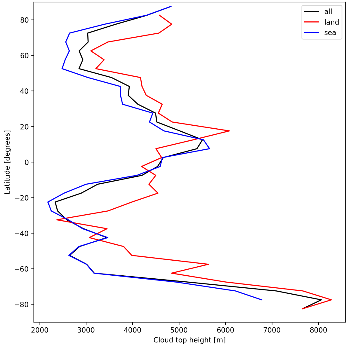
Figure 22: Zonal average of “Cloud top height” for 2025-09-10 to 2025-09-11.
