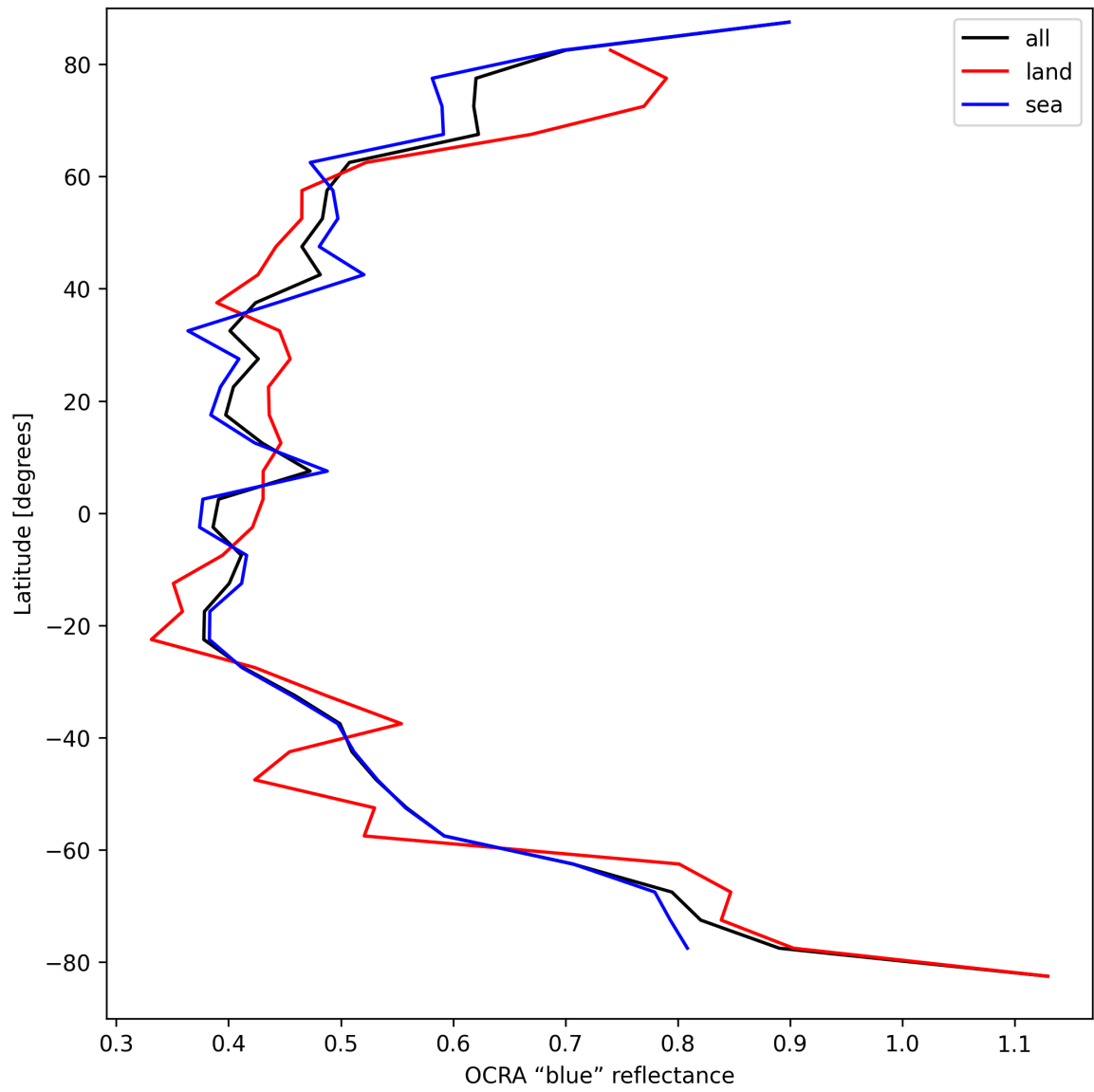
Figure 33: Zonal average of “OCRA “blue” reflectance” for 2025-09-10 to 2025-09-11.
