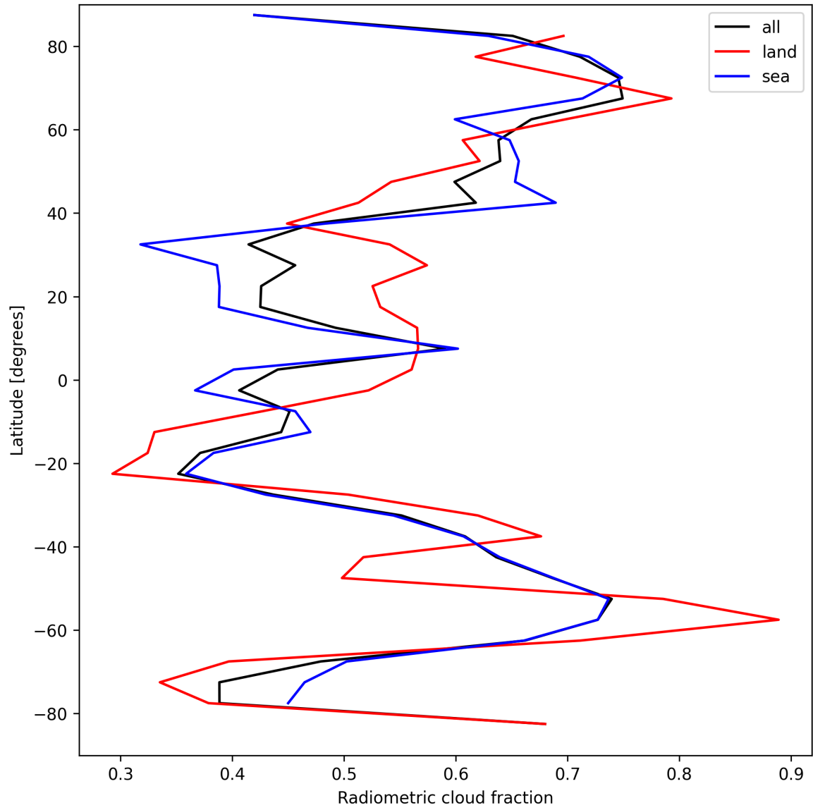
Figure 21: Zonal average of “Radiometric cloud fraction” for 2025-09-10 to 2025-09-11.
