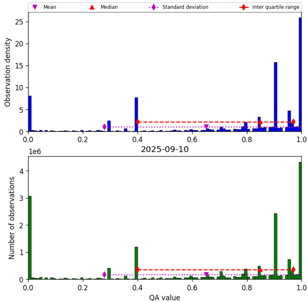
Figure 36: Histogram of “QA value” for 2025-09-10 to 2025-09-11
