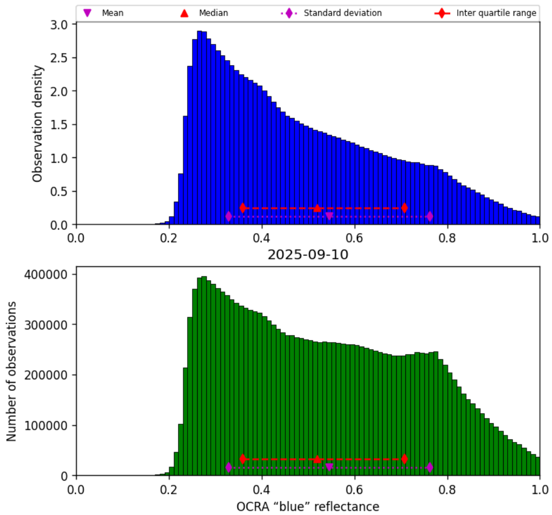
Figure 49: Histogram of “OCRA “blue” reflectance” for 2025-09-10 to 2025-09-11
