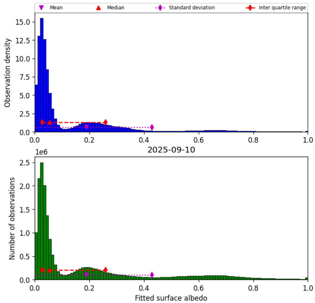
Figure 43: Histogram of “Fitted surface albedo” for 2025-09-10 to 2025-09-11
