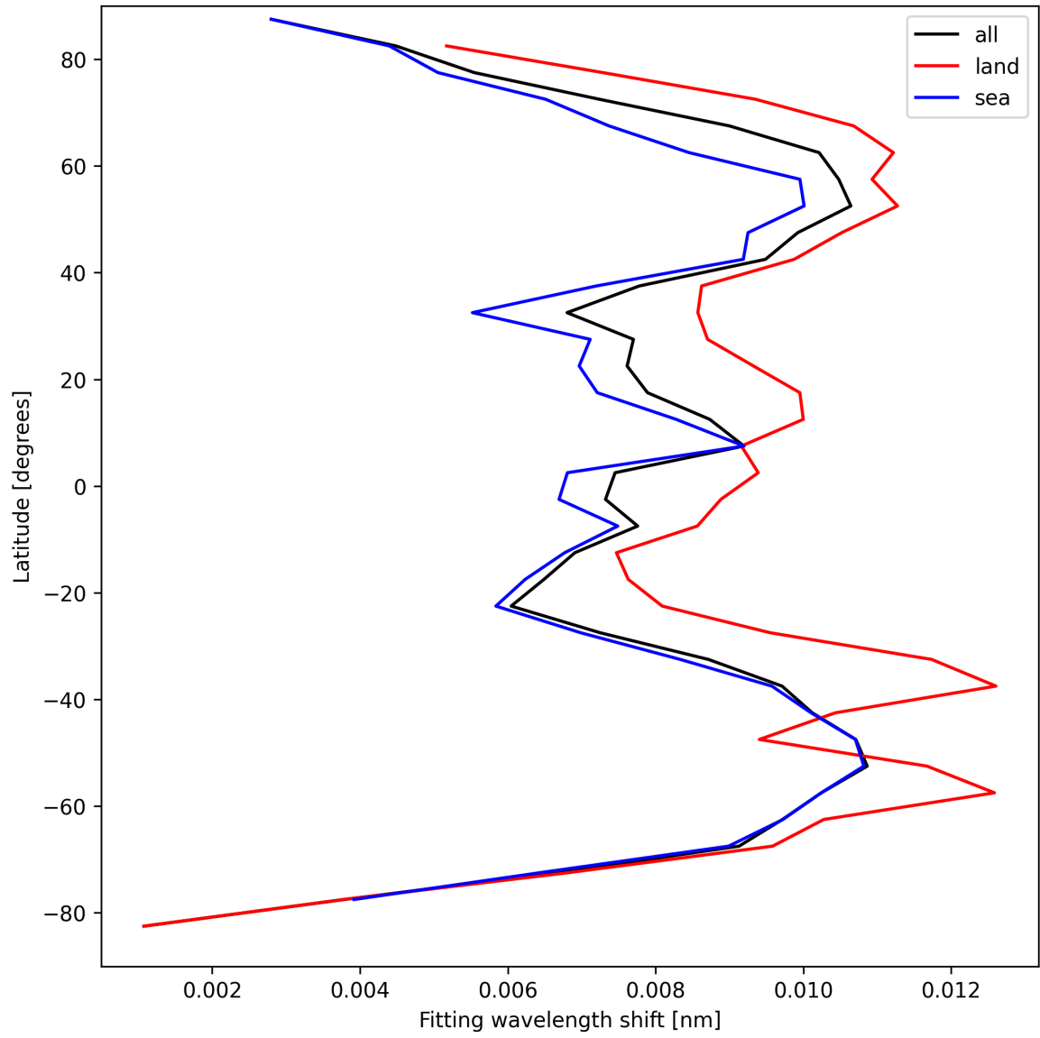
Figure 31: Zonal average of “Fitting wavelength shift” for 2025-09-10 to 2025-09-11.
