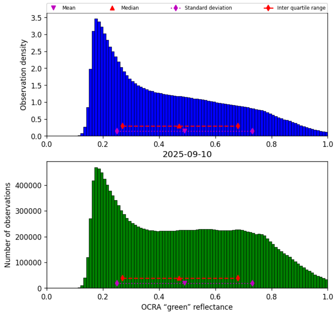
Figure 50: Histogram of “OCRA “green” reflectance” for 2025-09-10 to 2025-09-11
