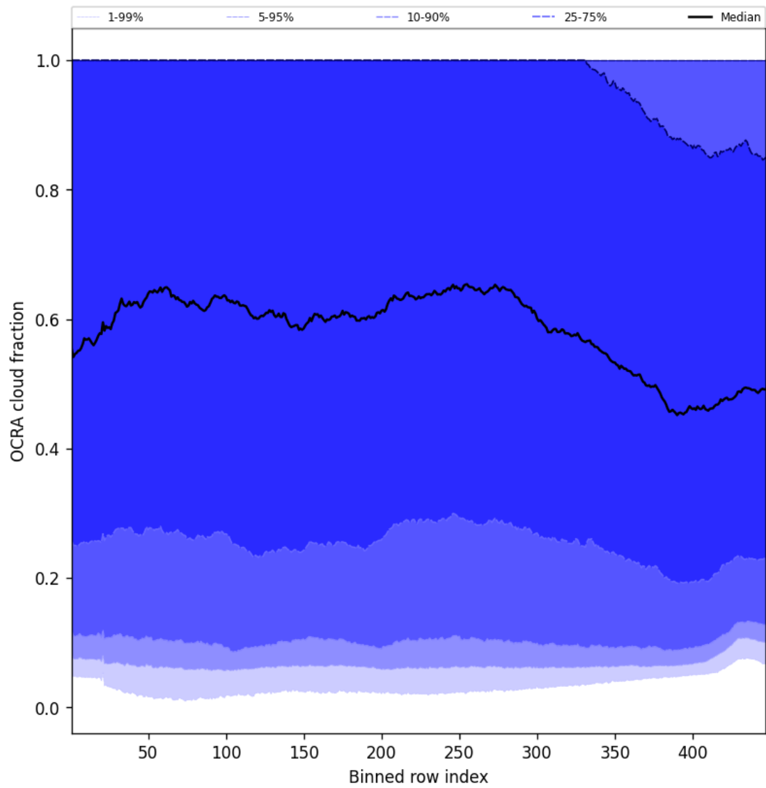
Figure 64: Along track statistics of “OCRA cloud fraction” for 2025-09-10 to 2025-09-11
