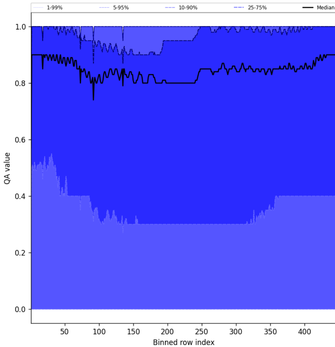
Figure 52: Along track statistics of “QA value” for 2025-09-10 to 2025-09-11
