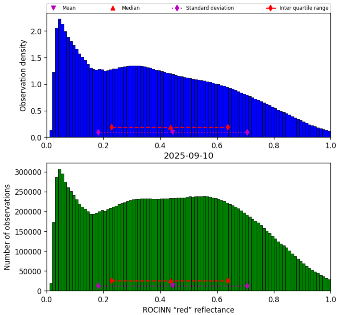
Figure 51: Histogram of “ROCINN “red” reflectance” for 2025-09-10 to 2025-09-11
