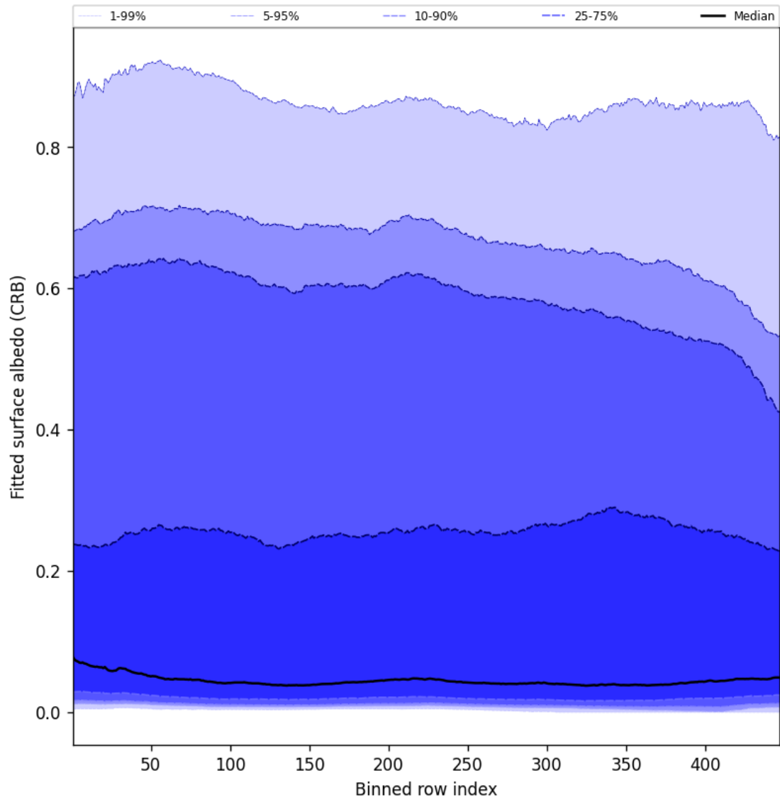
Figure 60: Along track statistics of “Fitted surface albedo (CRB)” for 2025-09-10 to 2025-09-11
