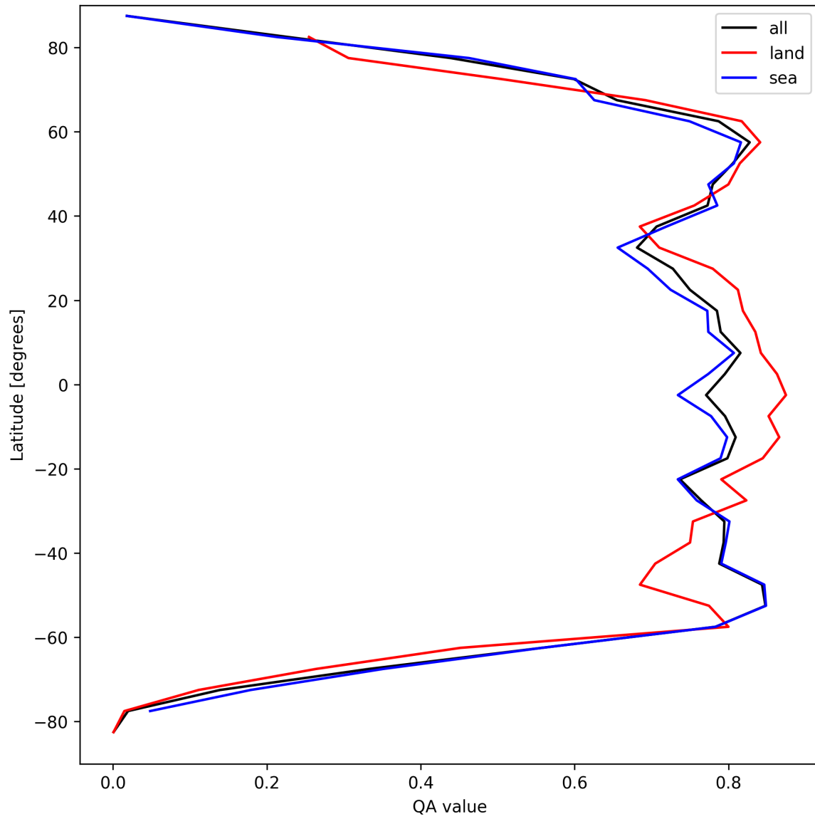
Figure 20: Zonal average of “QA value” for 2025-09-10 to 2025-09-11.
