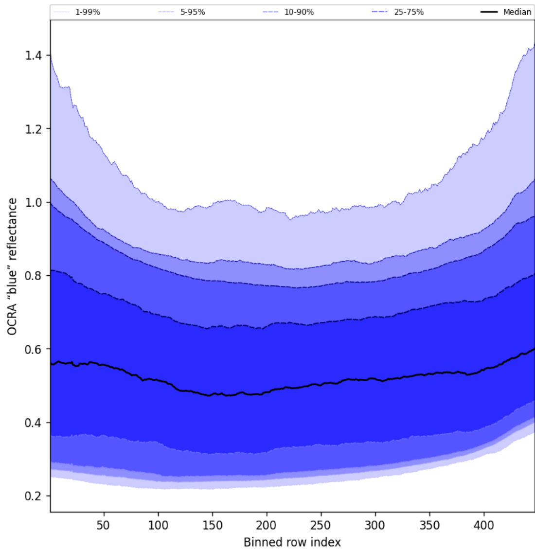
Figure 65: Along track statistics of “OCRA “blue” reflectance” for 2025-09-10 to 2025-09-11
