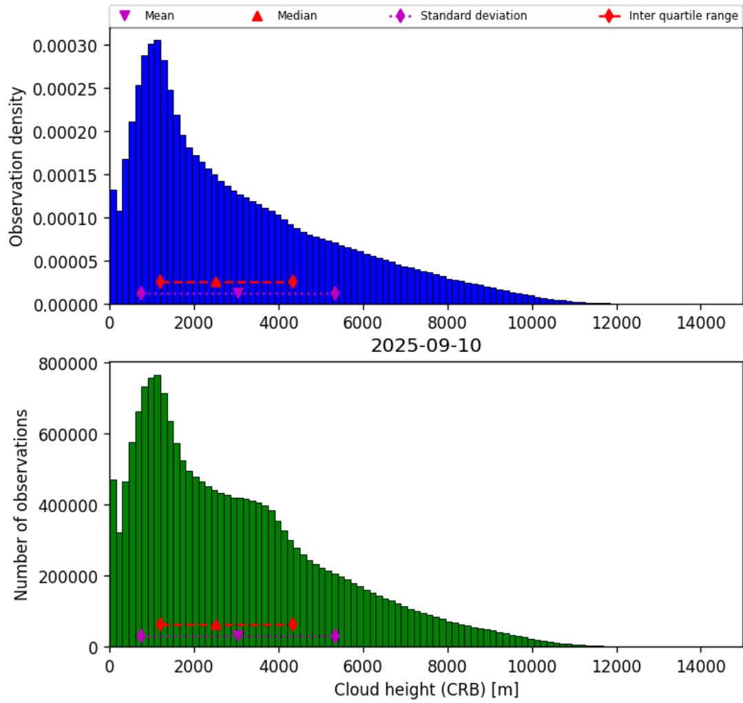
Figure 41: Histogram of “Cloud height (CRB)” for 2025-09-10 to 2025-09-11
