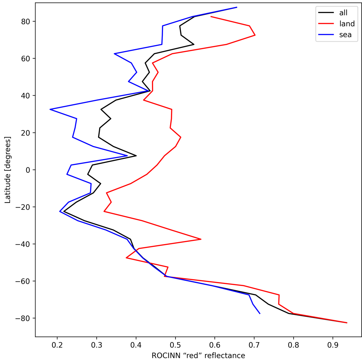
Figure 35: Zonal average of “ROCINN “red” reflectance” for 2025-09-10 to 2025-09-11.
