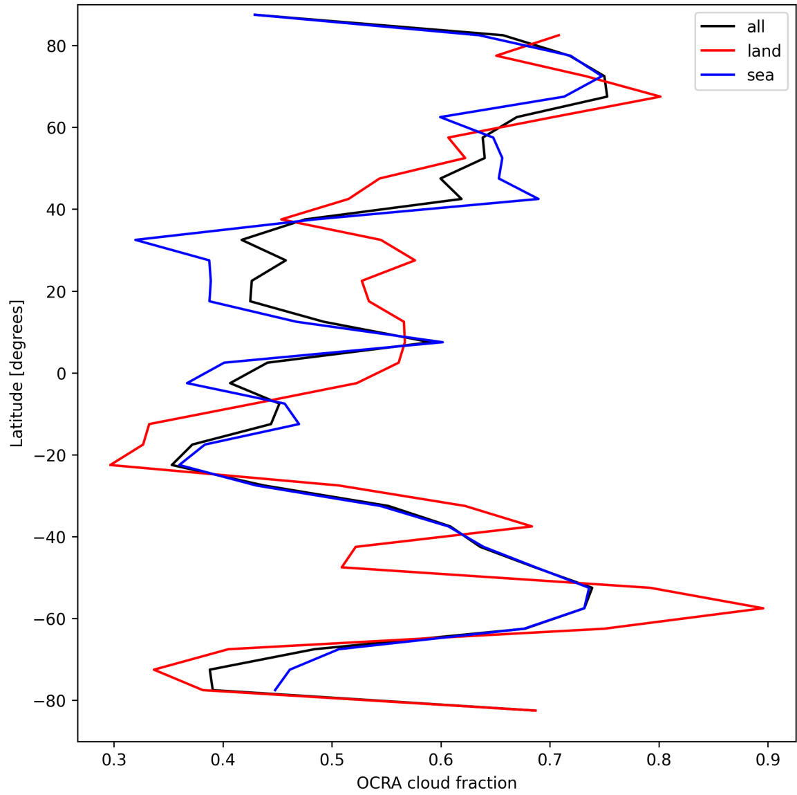
Figure 32: Zonal average of “OCRA cloud fraction” for 2025-09-10 to 2025-09-11.
