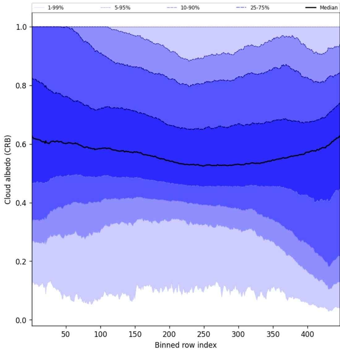
Figure 58: Along track statistics of “Cloud albedo (CRB)” for 2025-09-10 to 2025-09-11
