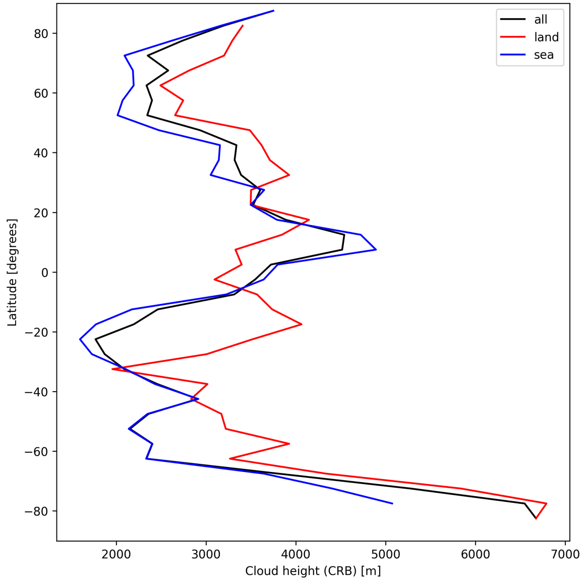
Figure 25: Zonal average of “Cloud height (CRB)” for 2025-09-10 to 2025-09-11.
