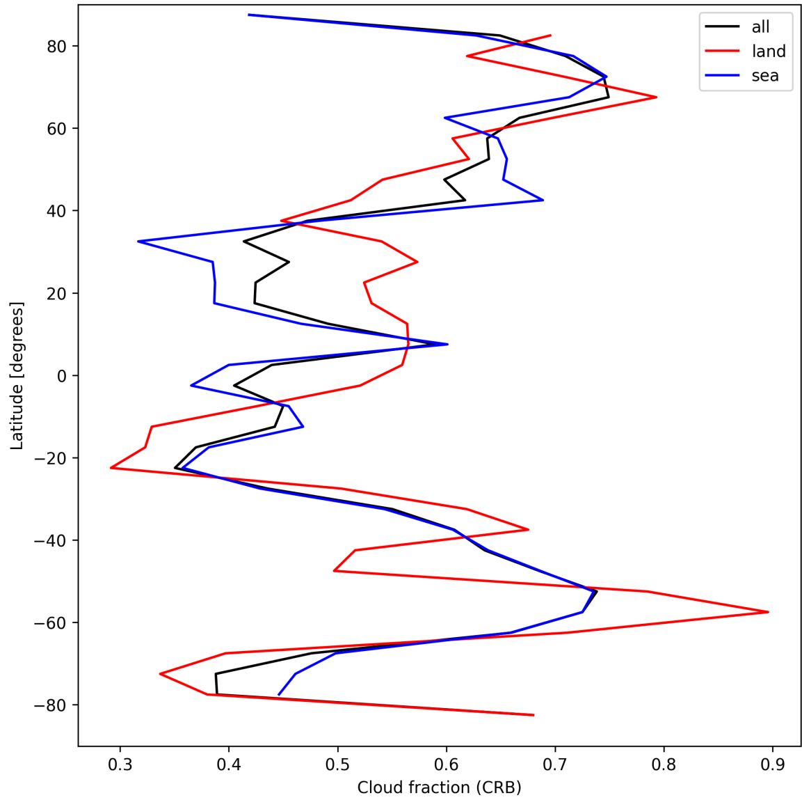
Figure 24: Zonal average of “Cloud fraction (CRB)” for 2025-09-10 to 2025-09-11.
