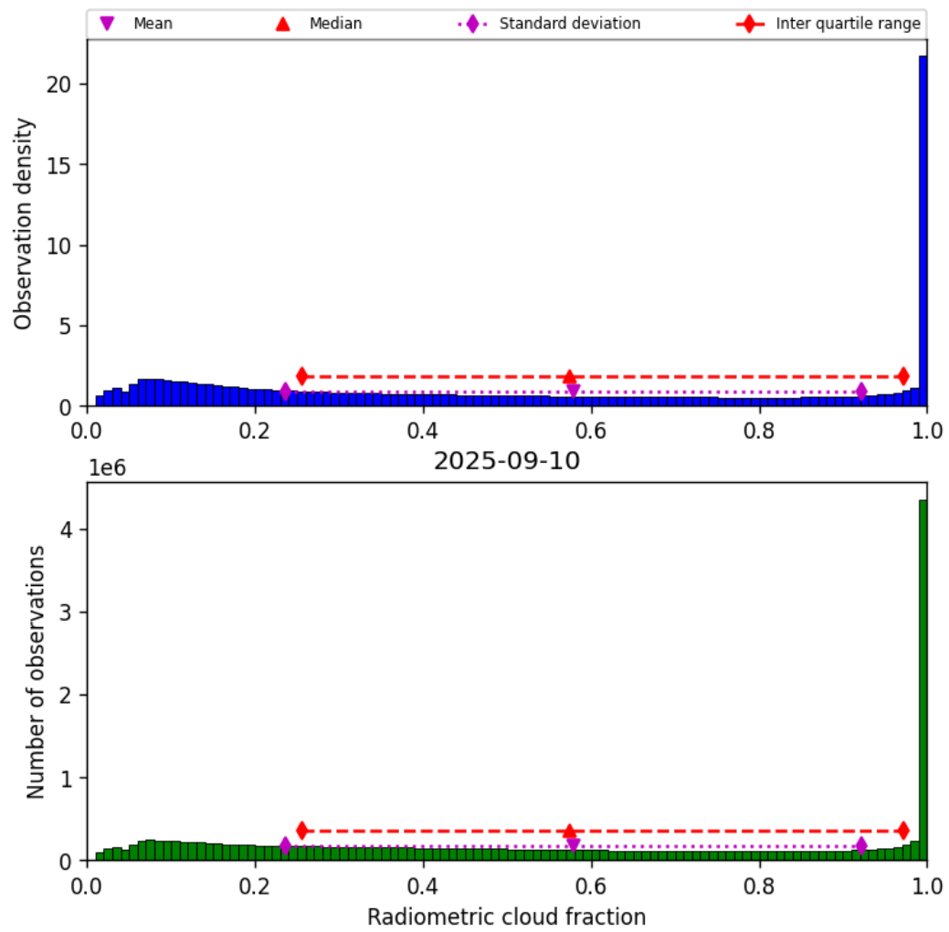
Figure 37: Histogram of “Radiometric cloud fraction” for 2025-09-10 to 2025-09-11
