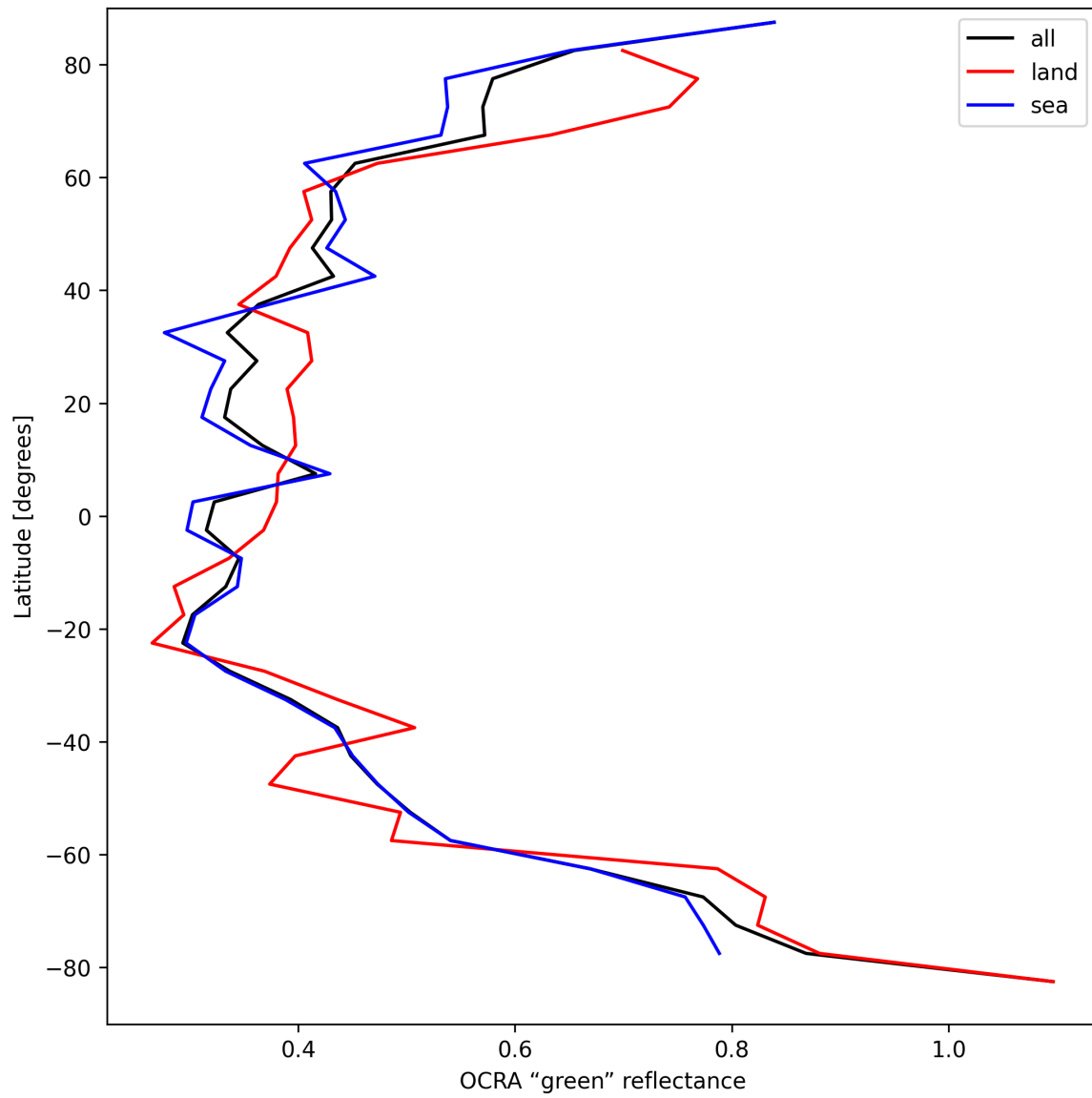
Figure 34: Zonal average of “OCRA “green” reflectance” for 2025-09-10 to 2025-09-11.
