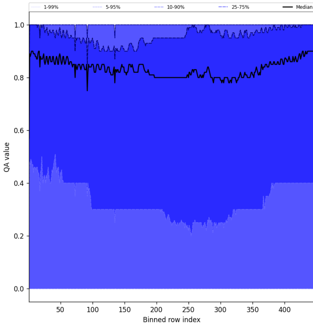
Figure 52: Along track statistics of “QA value” for 2025-09-11 to 2025-09-12
