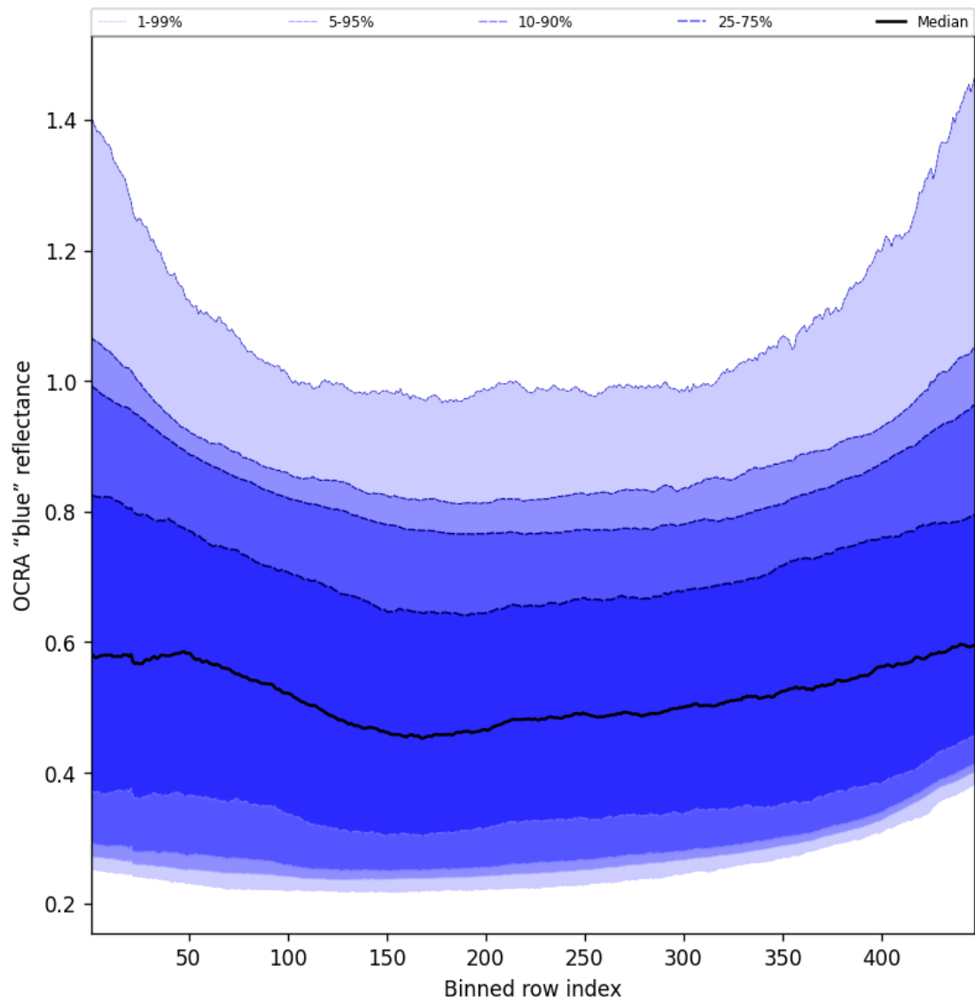
Figure 65: Along track statistics of “OCRA “blue” reflectance” for 2025-09-11 to 2025-09-12
