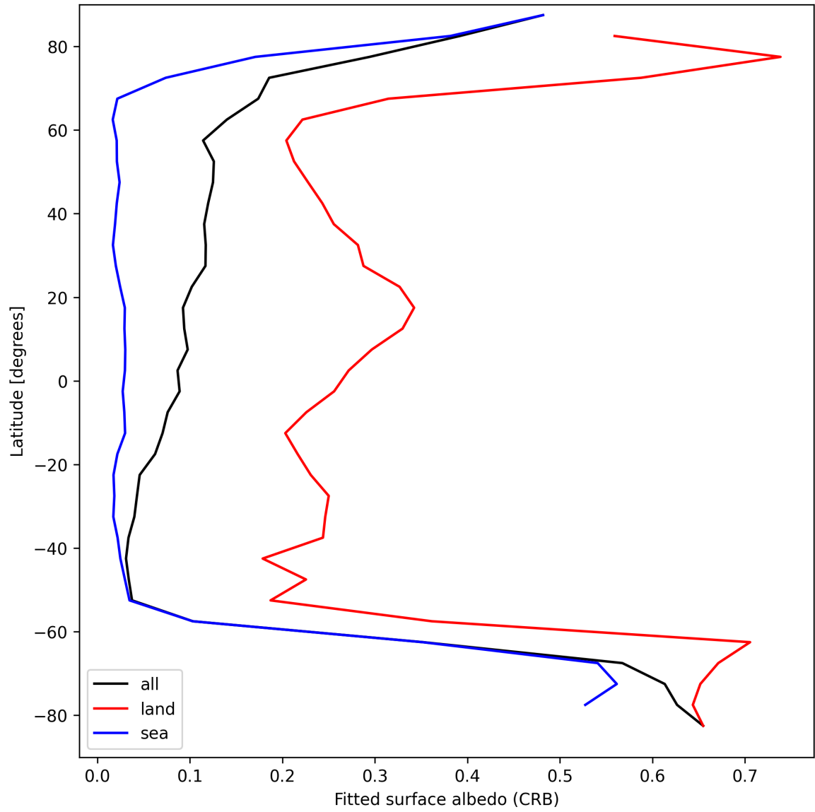
Figure 28: Zonal average of “Fitted surface albedo (CRB)” for 2025-09-11 to 2025-09-12.
