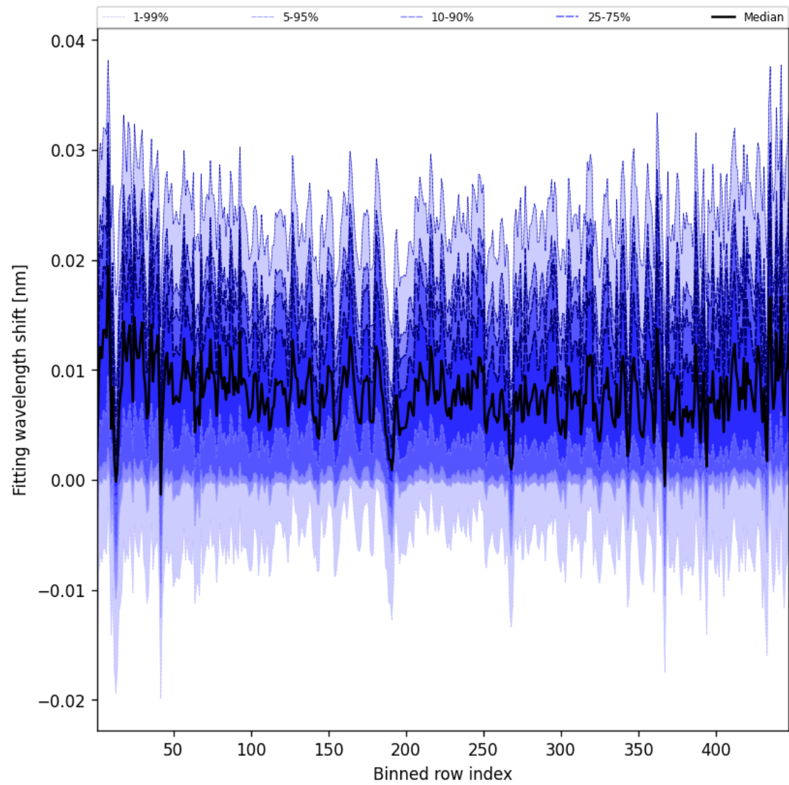
Figure 63: Along track statistics of “Fitting wavelength shift” for 2025-09-11 to 2025-09-12
