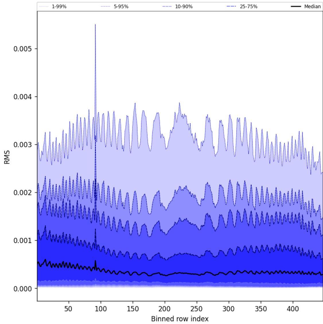
Figure 61: Along track statistics of “RMS” for 2025-09-11 to 2025-09-12
