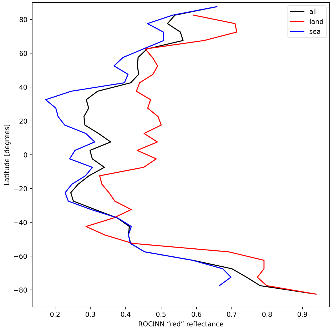
Figure 35: Zonal average of “ROCINN “red” reflectance” for 2025-09-11 to 2025-09-12.
