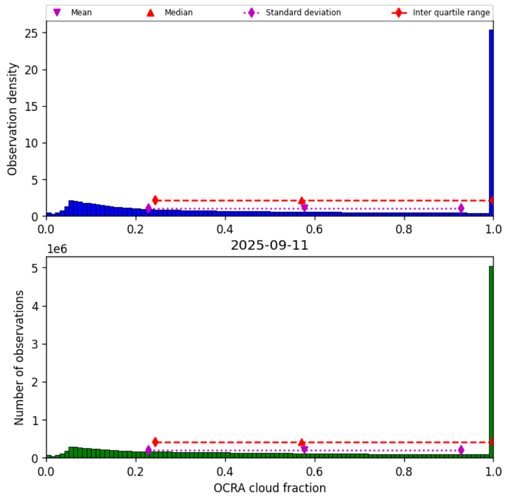
Figure 48: Histogram of “OCRA cloud fraction” for 2025-09-11 to 2025-09-12
