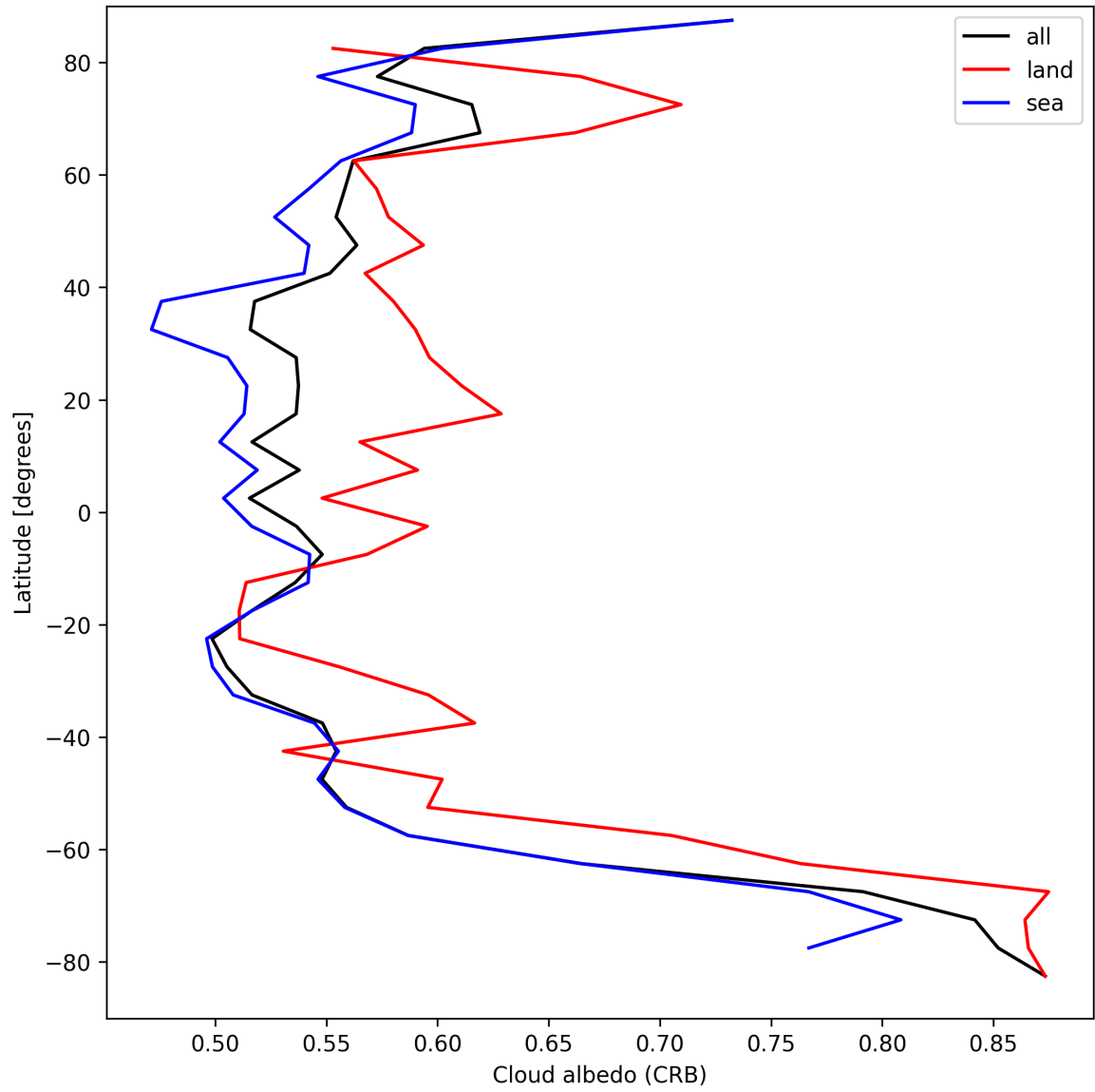
Figure 26: Zonal average of “Cloud albedo (CRB)” for 2025-09-11 to 2025-09-12.
