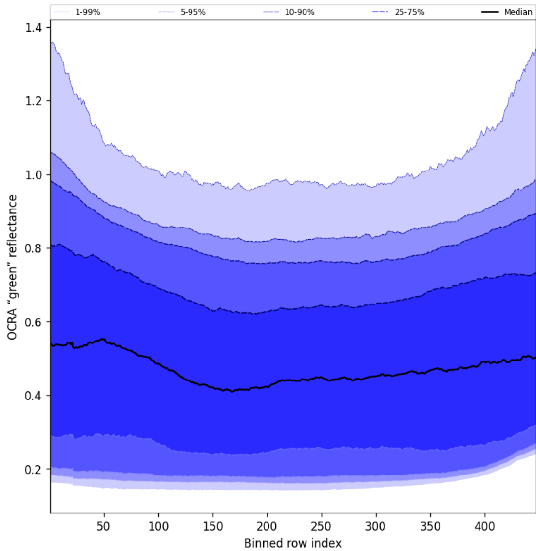
Figure 66: Along track statistics of “OCRA “green” reflectance” for 2025-09-11 to 2025-09-12
