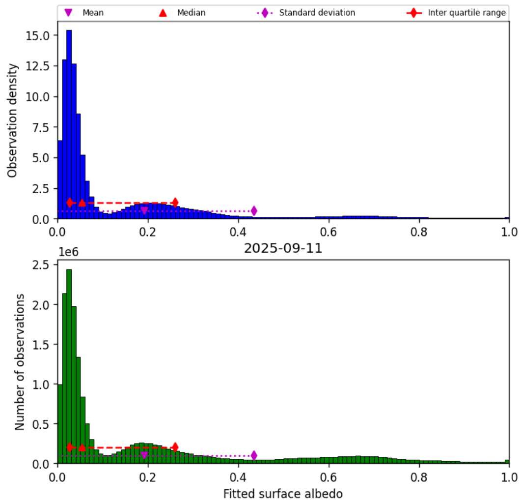
Figure 43: Histogram of “Fitted surface albedo” for 2025-09-11 to 2025-09-12
