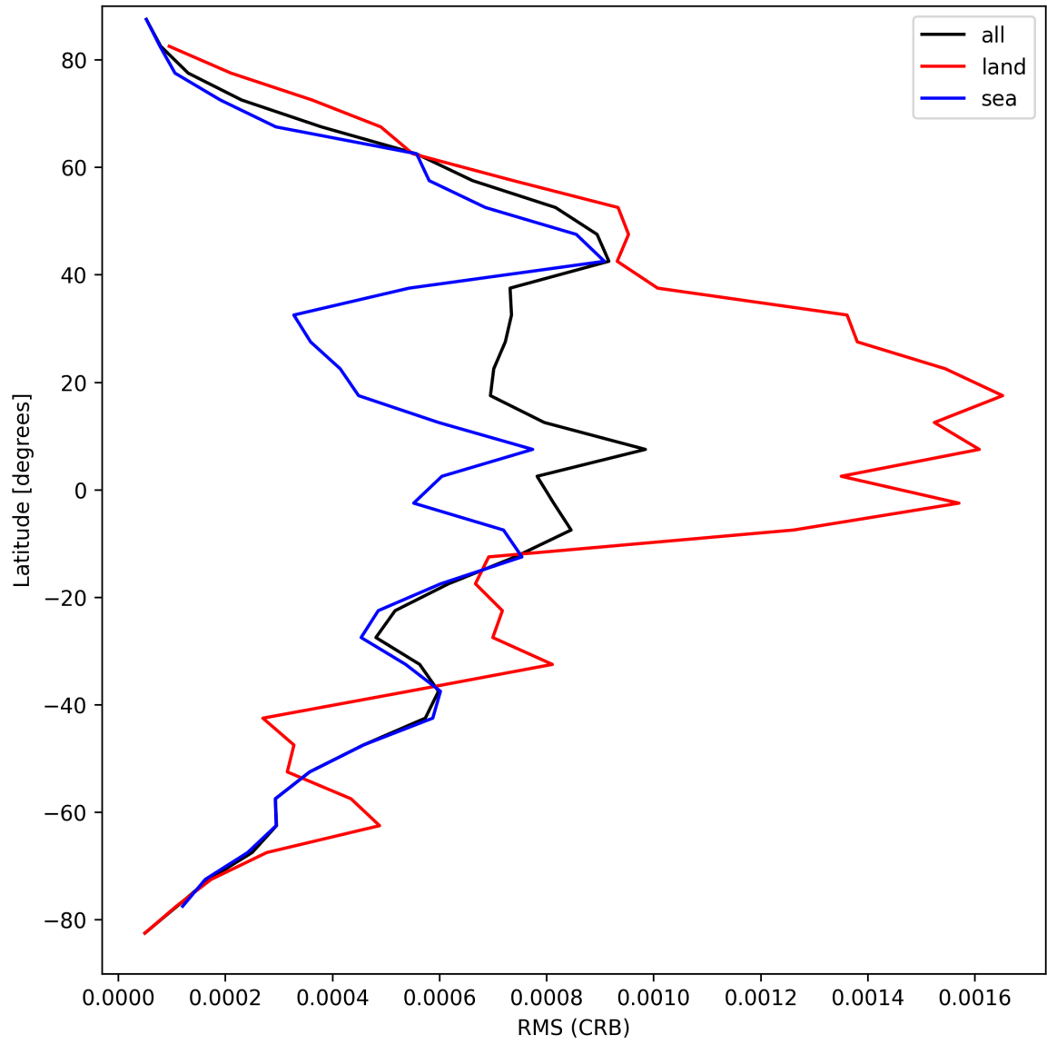
Figure 30: Zonal average of “RMS (CRB)” for 2025-09-11 to 2025-09-12.
