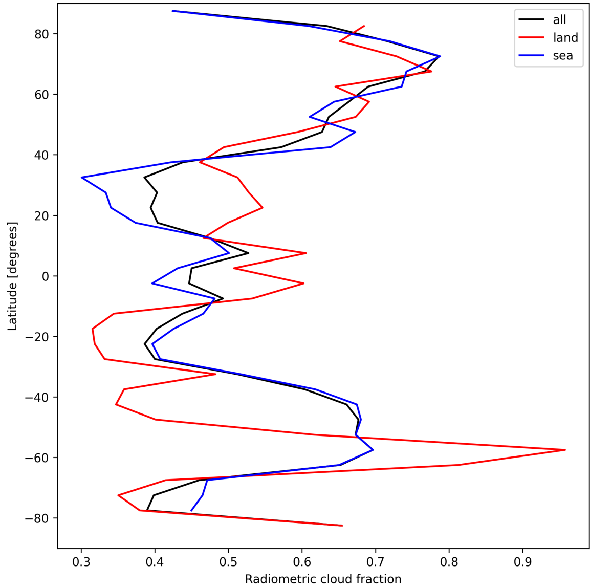
Figure 21: Zonal average of “Radiometric cloud fraction” for 2025-09-11 to 2025-09-12.
