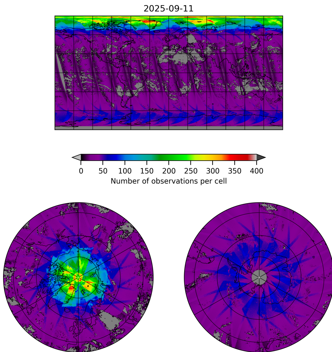
Figure 19: Map of the number of observations for 2025-09-11 to 2025-09-12
