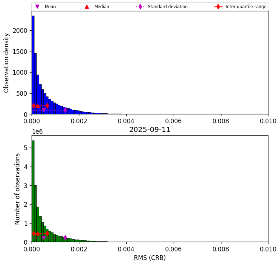
Figure 46: Histogram of “RMS (CRB)” for 2025-09-11 to 2025-09-12
