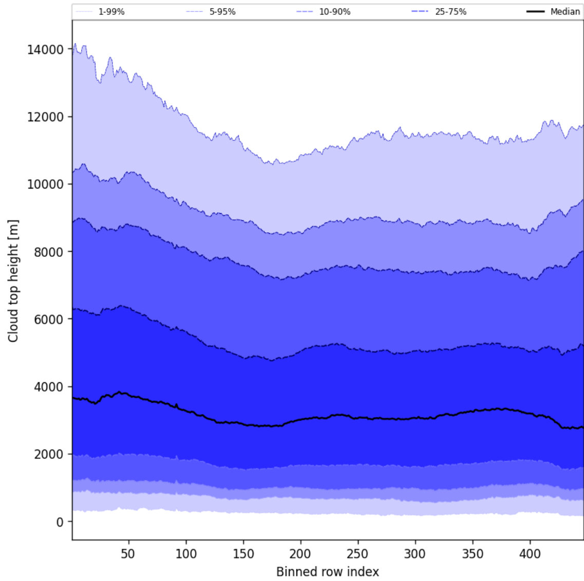
Figure 54: Along track statistics of “Cloud top height” for 2025-09-11 to 2025-09-12
