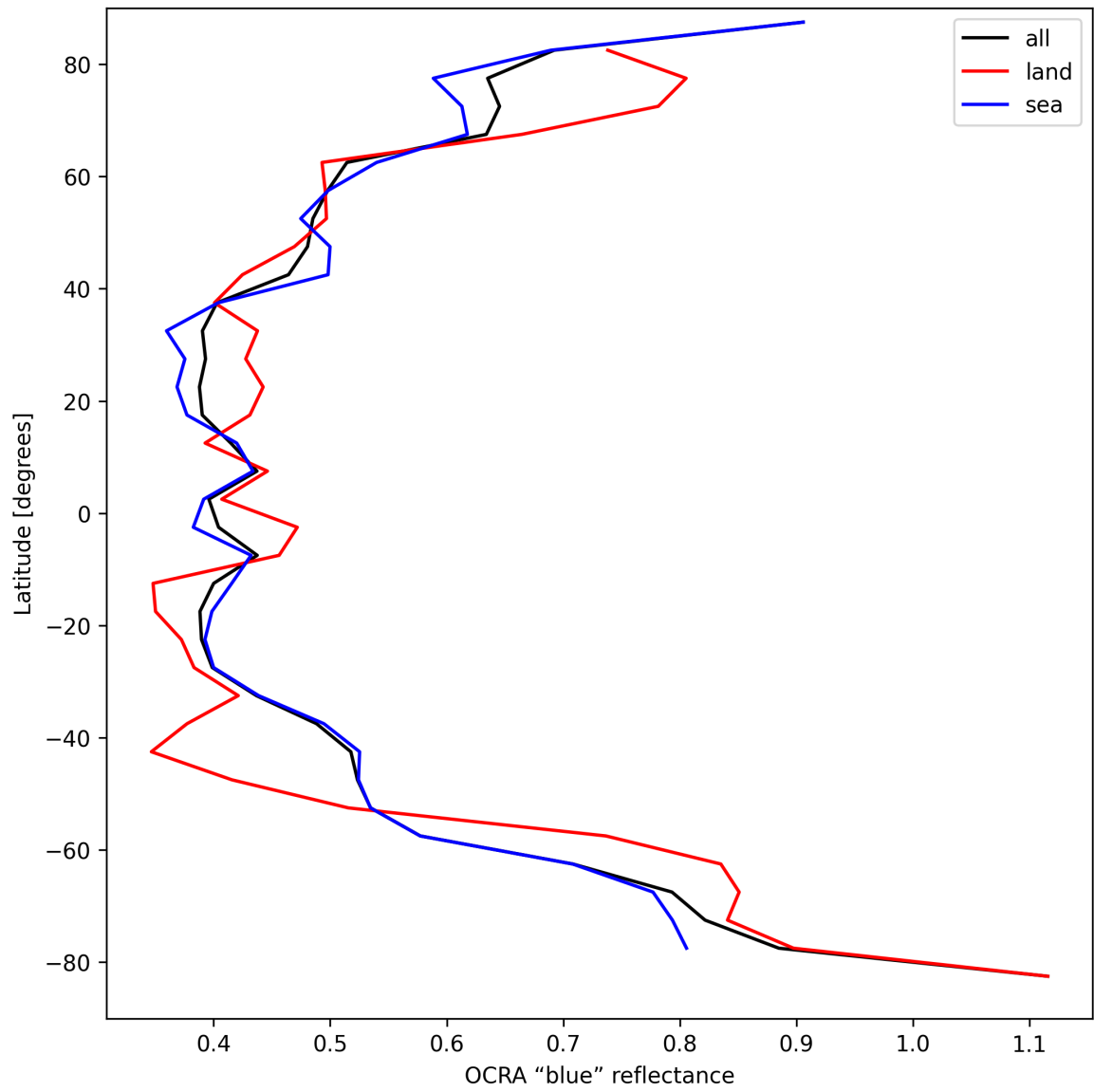
Figure 33: Zonal average of “OCRA “blue” reflectance” for 2025-09-11 to 2025-09-12.
