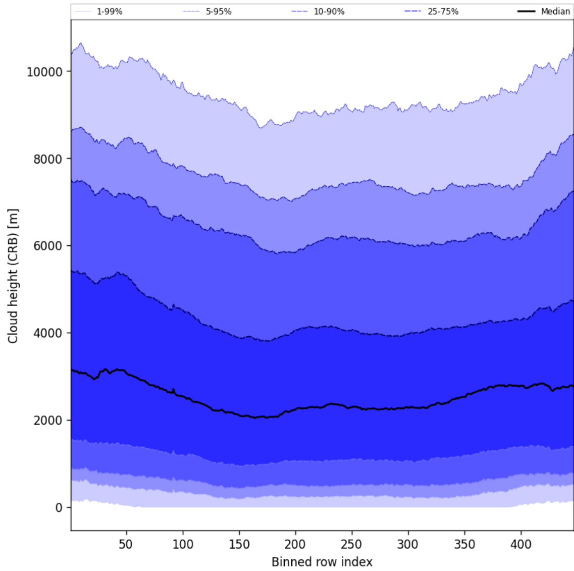
Figure 57: Along track statistics of “Cloud height (CRB)” for 2025-09-11 to 2025-09-12
