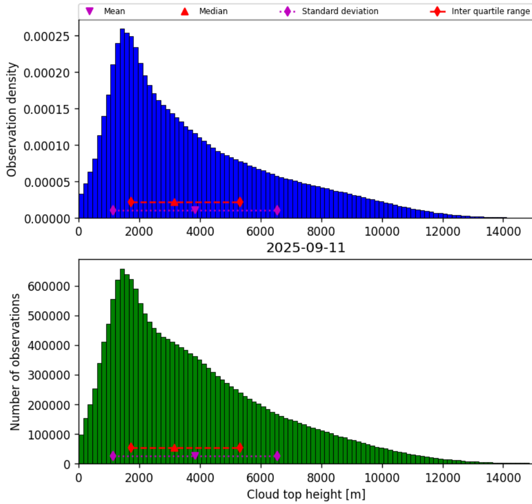
Figure 38: Histogram of “Cloud top height” for 2025-09-11 to 2025-09-12
