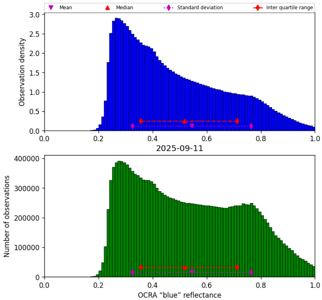
Figure 49: Histogram of “OCRA “blue” reflectance” for 2025-09-11 to 2025-09-12
