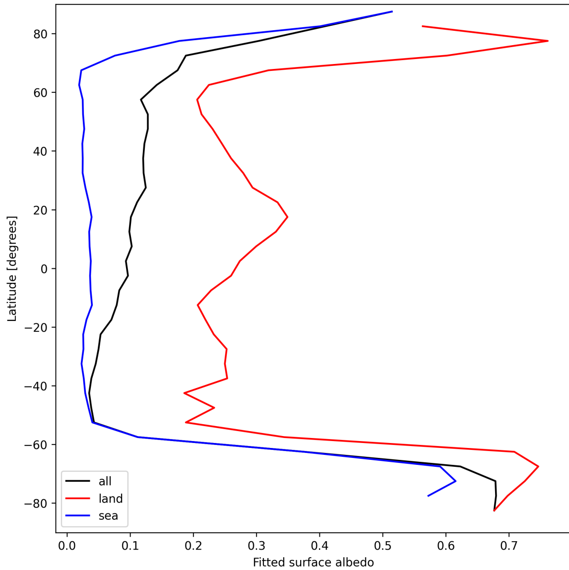
Figure 27: Zonal average of “Fitted surface albedo” for 2025-09-11 to 2025-09-12.
