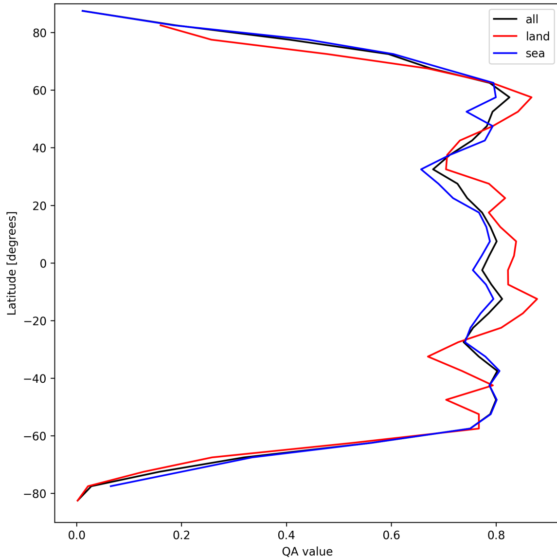
Figure 20: Zonal average of “QA value” for 2025-09-11 to 2025-09-12.
