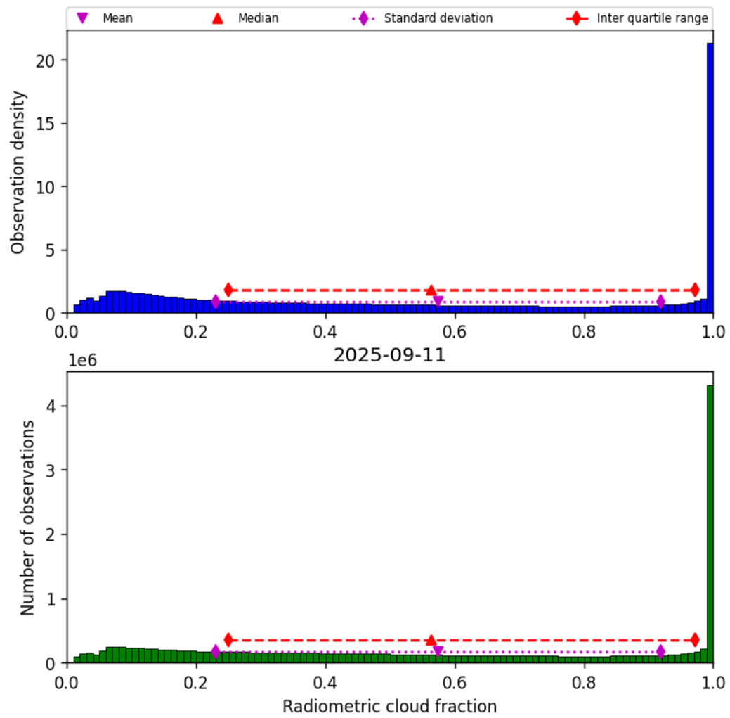
Figure 37: Histogram of “Radiometric cloud fraction” for 2025-09-11 to 2025-09-12
