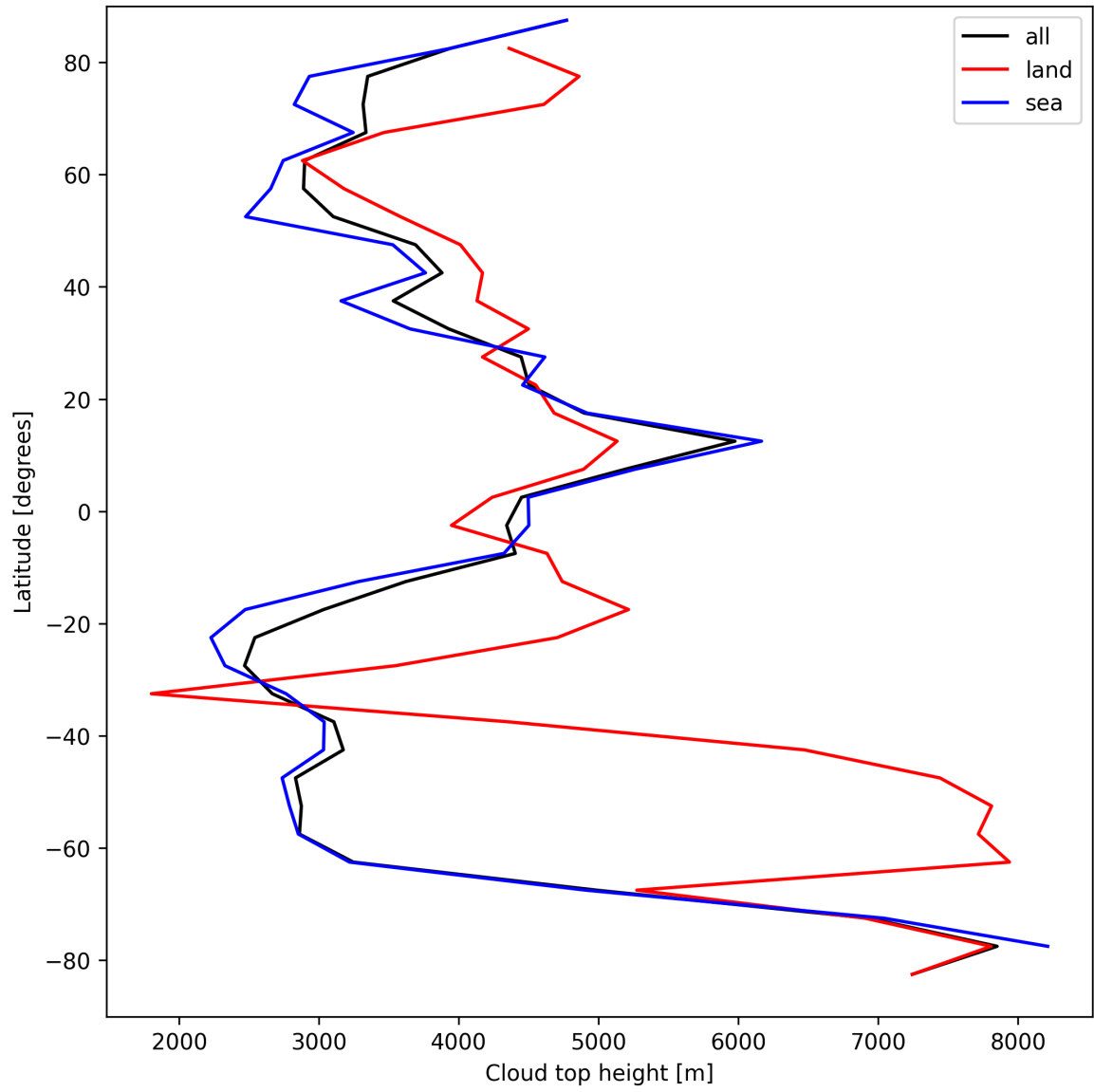
Figure 22: Zonal average of “Cloud top height” for 2025-09-11 to 2025-09-12.
