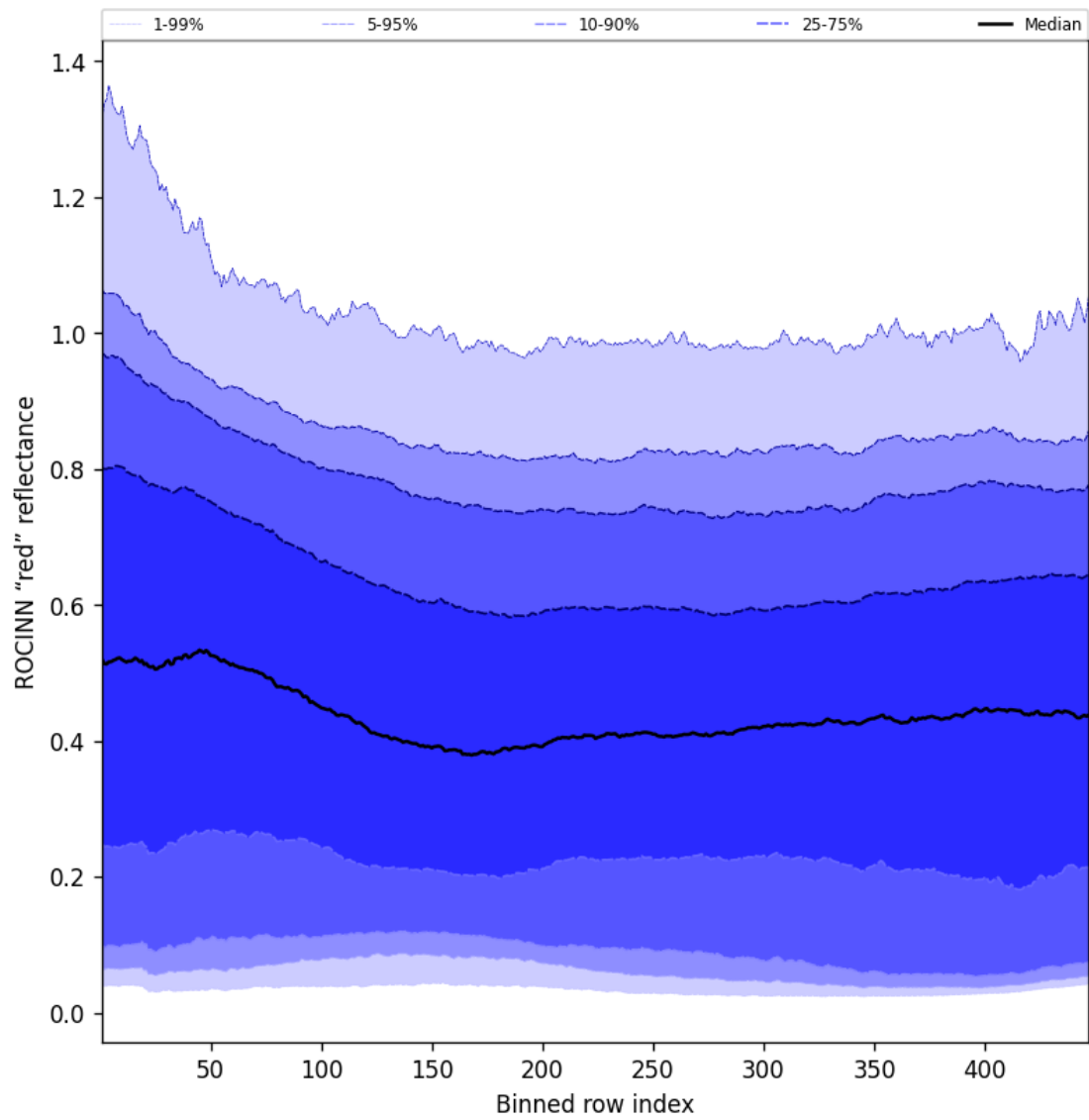
Figure 67: Along track statistics of “ROCINN “red” reflectance” for 2025-09-11 to 2025-09-12
