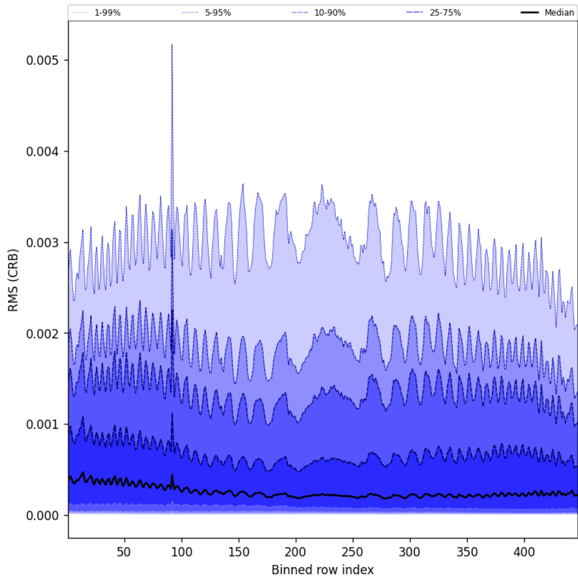
Figure 62: Along track statistics of “RMS (CRB)” for 2025-09-11 to 2025-09-12
