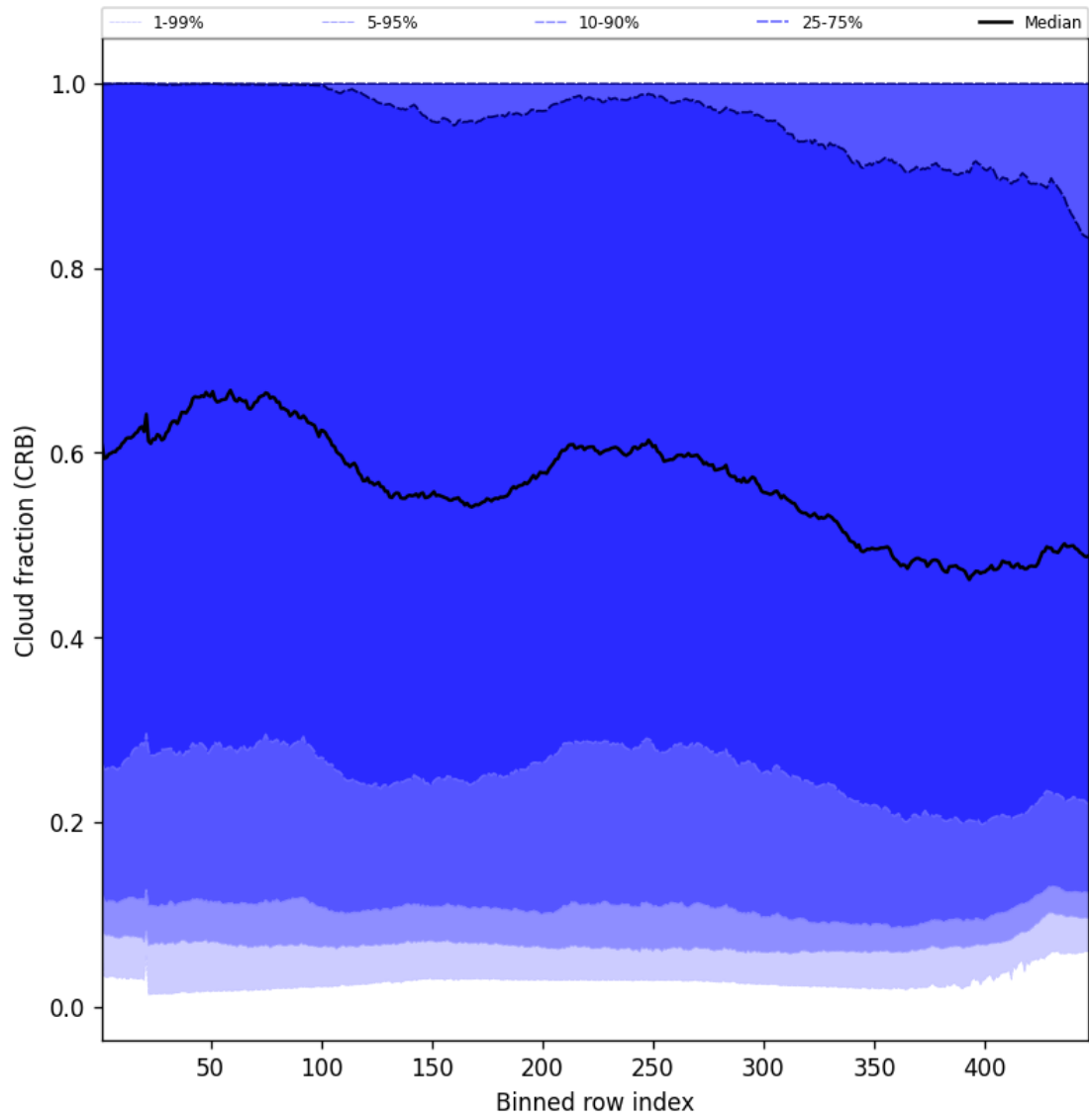
Figure 56: Along track statistics of “Cloud fraction (CRB)” for 2025-09-11 to 2025-09-12
