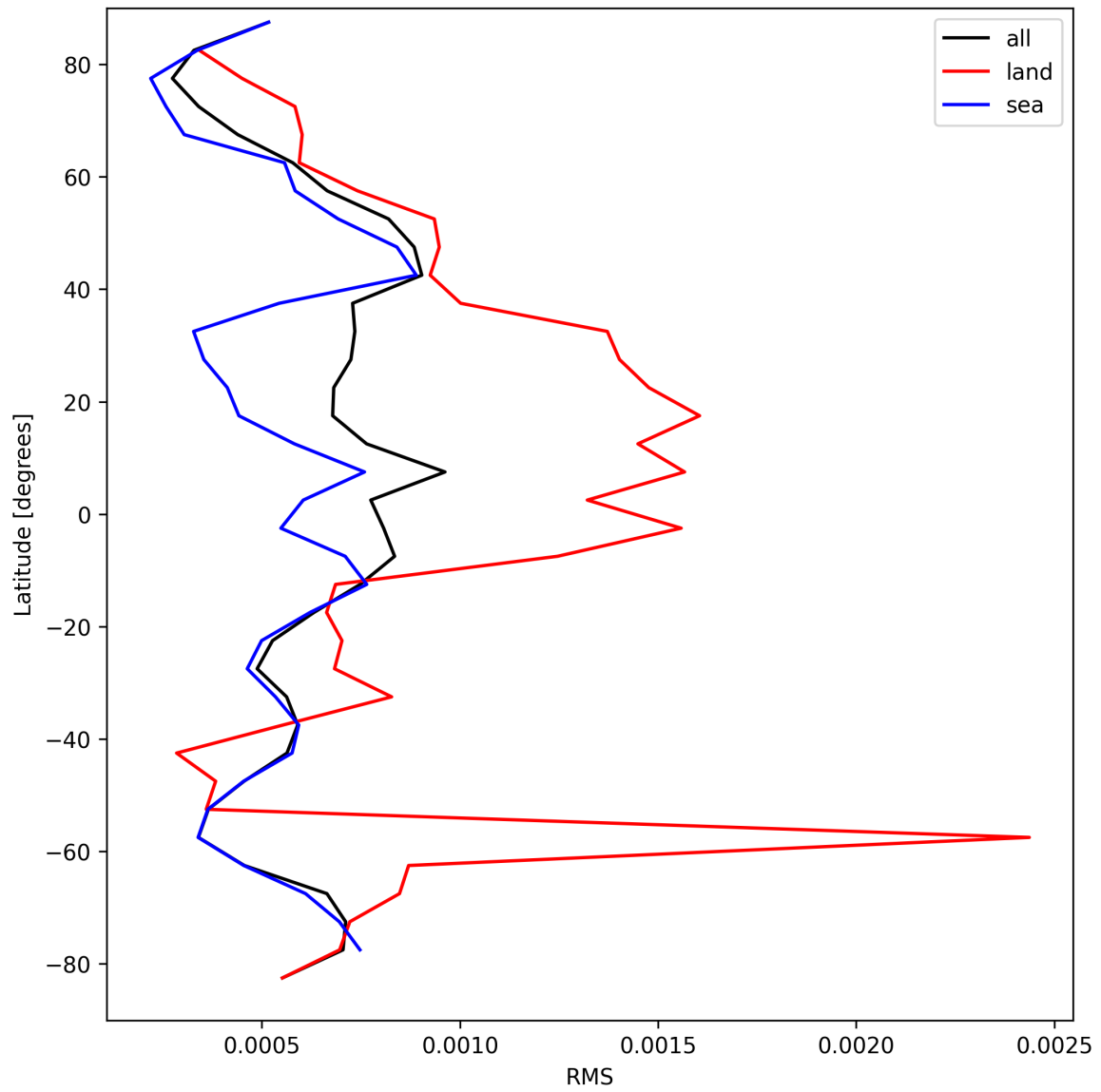
Figure 29: Zonal average of “RMS” for 2025-09-11 to 2025-09-12.
