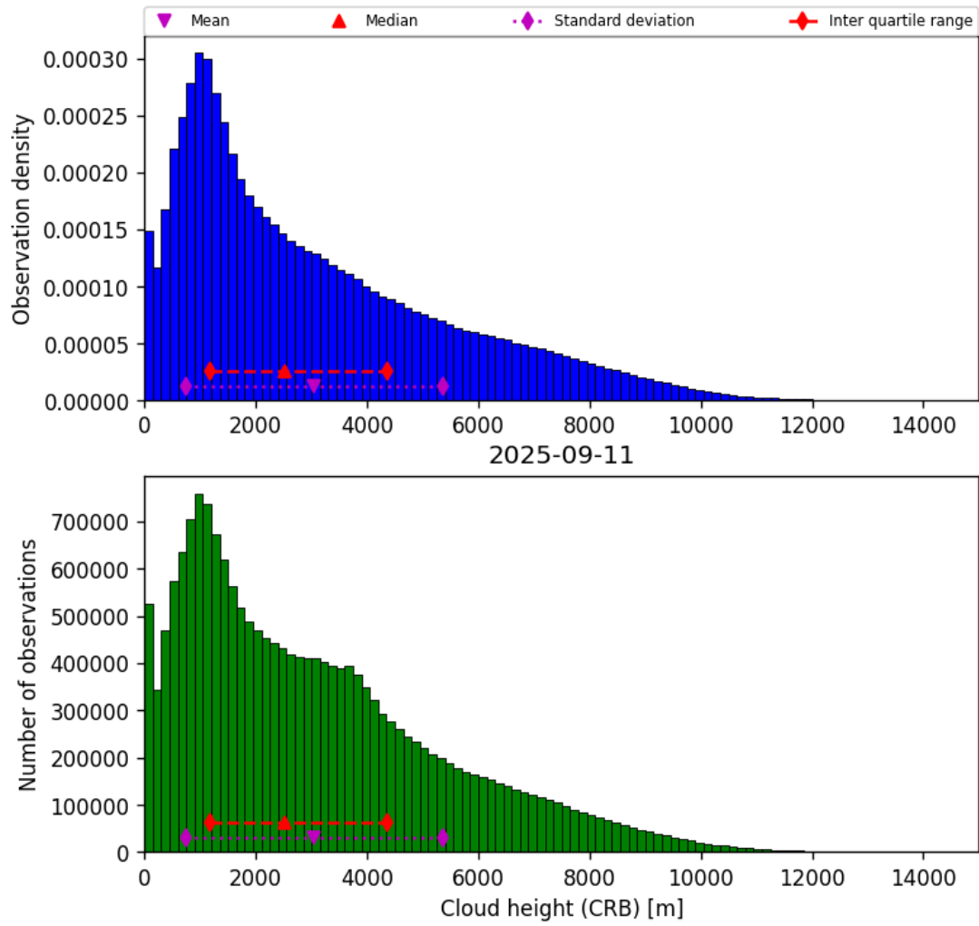
Figure 41: Histogram of “Cloud height (CRB)” for 2025-09-11 to 2025-09-12
