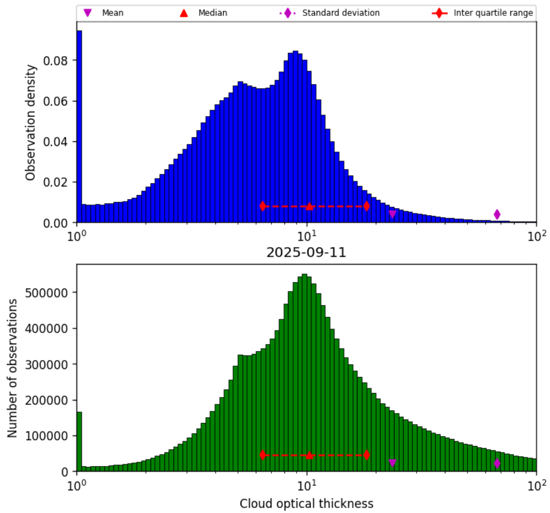
Figure 39: Histogram of “Cloud optical thickness” for 2025-09-11 to 2025-09-12
