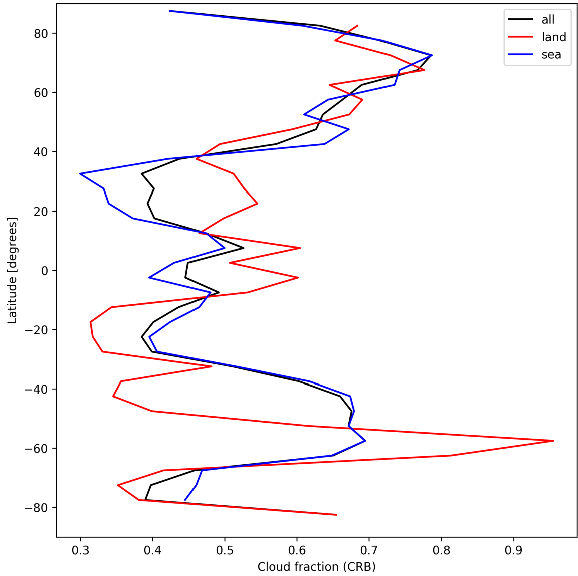
Figure 24: Zonal average of “Cloud fraction (CRB)” for 2025-09-11 to 2025-09-12.
