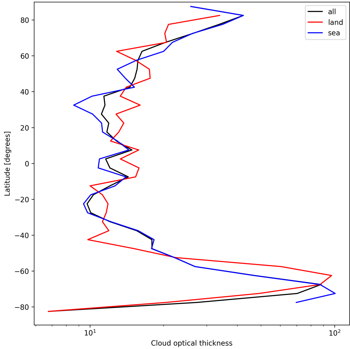
Figure 23: Zonal average of “Cloud optical thickness” for 2025-09-11 to 2025-09-12.
