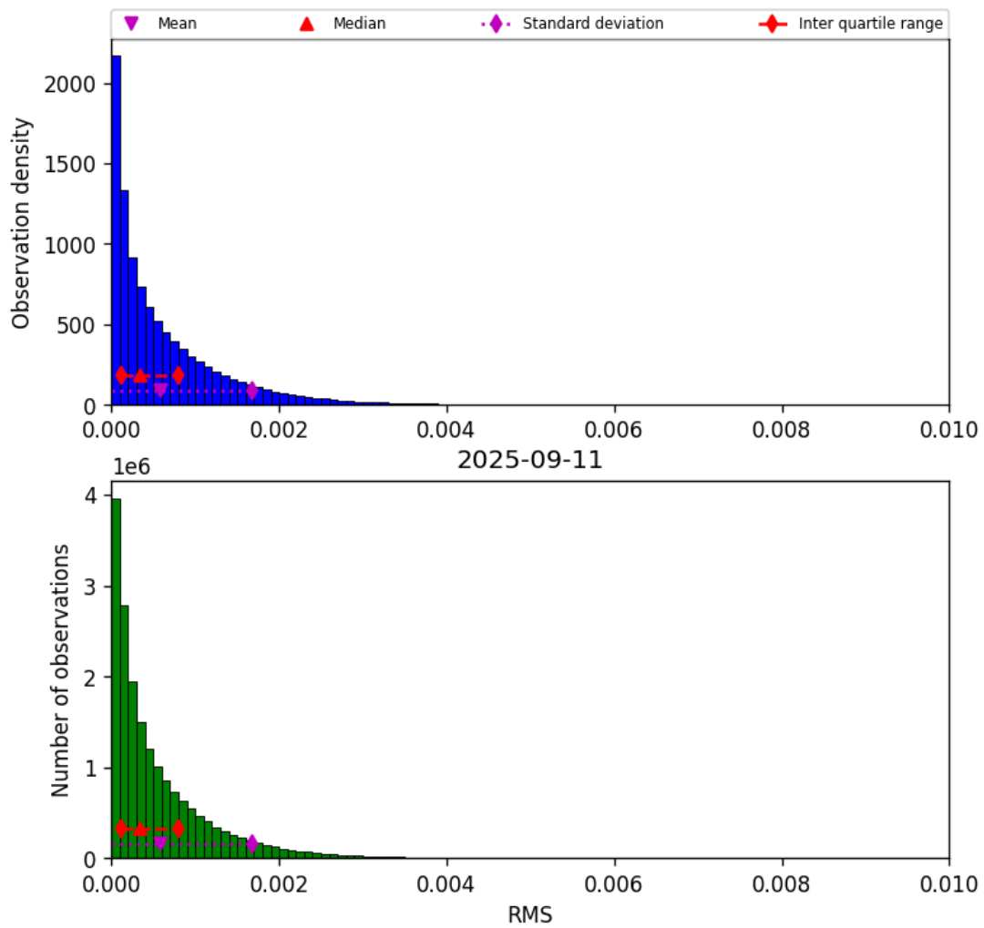
Figure 45: Histogram of “RMS” for 2025-09-11 to 2025-09-12
