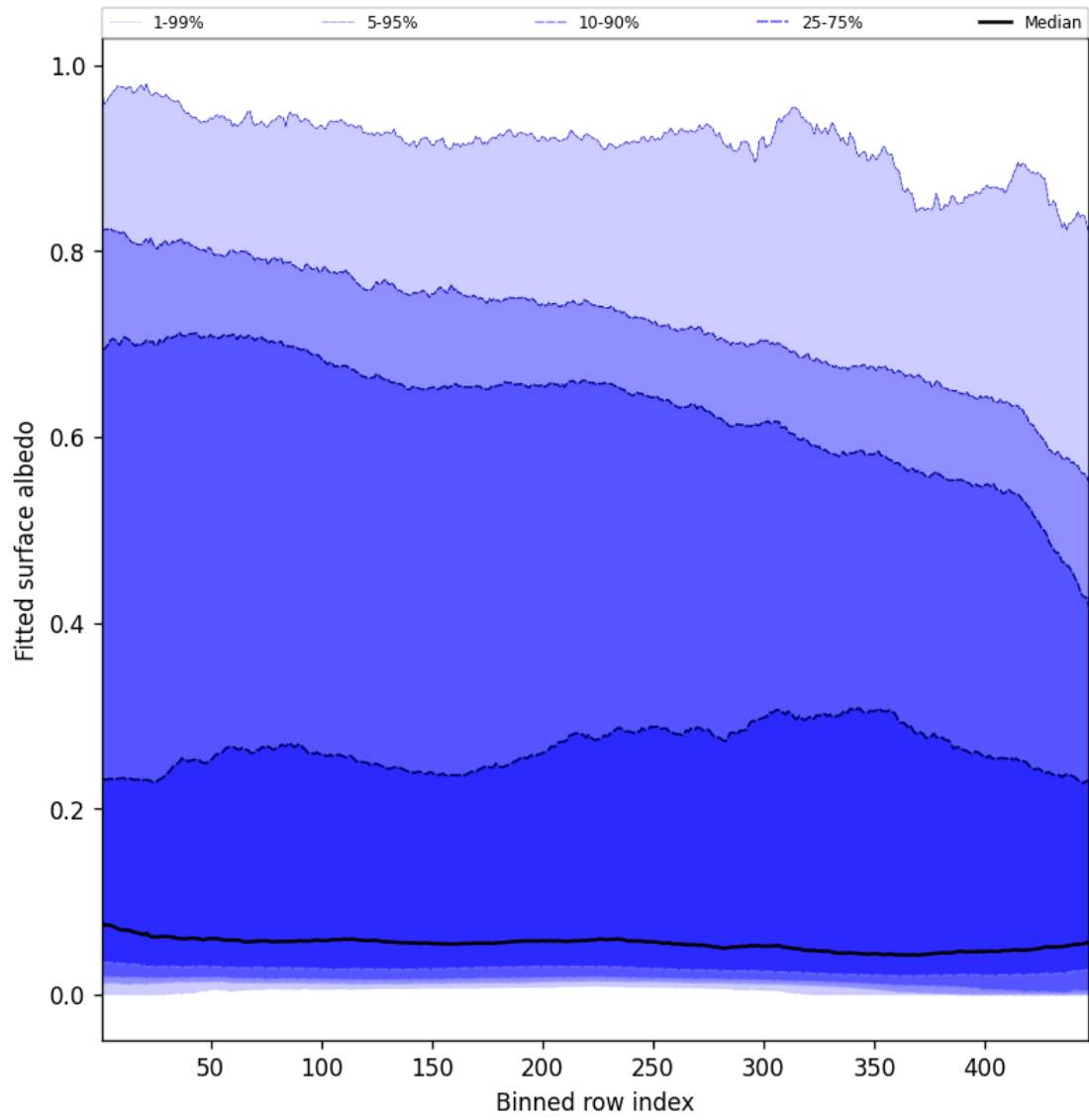
Figure 59: Along track statistics of “Fitted surface albedo” for 2025-09-11 to 2025-09-12
