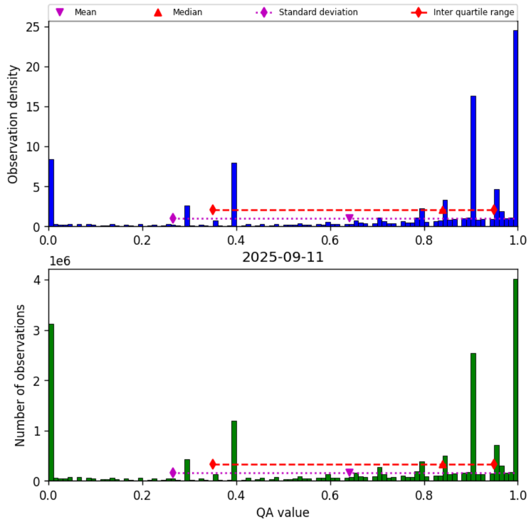
Figure 36: Histogram of “QA value” for 2025-09-11 to 2025-09-12
