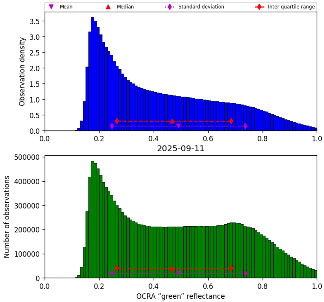
Figure 50: Histogram of “OCRA “green” reflectance” for 2025-09-11 to 2025-09-12
