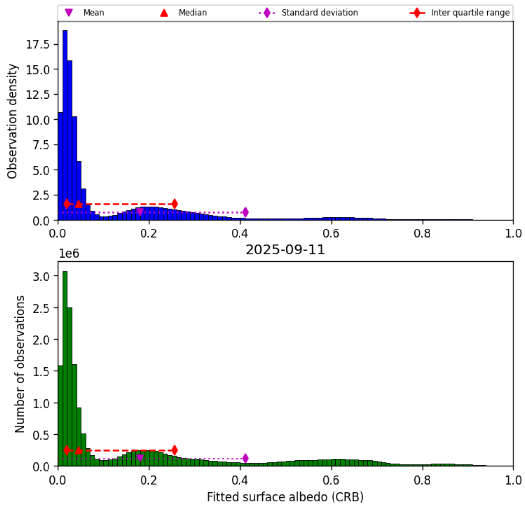
Figure 44: Histogram of “Fitted surface albedo (CRB)” for 2025-09-11 to 2025-09-12
