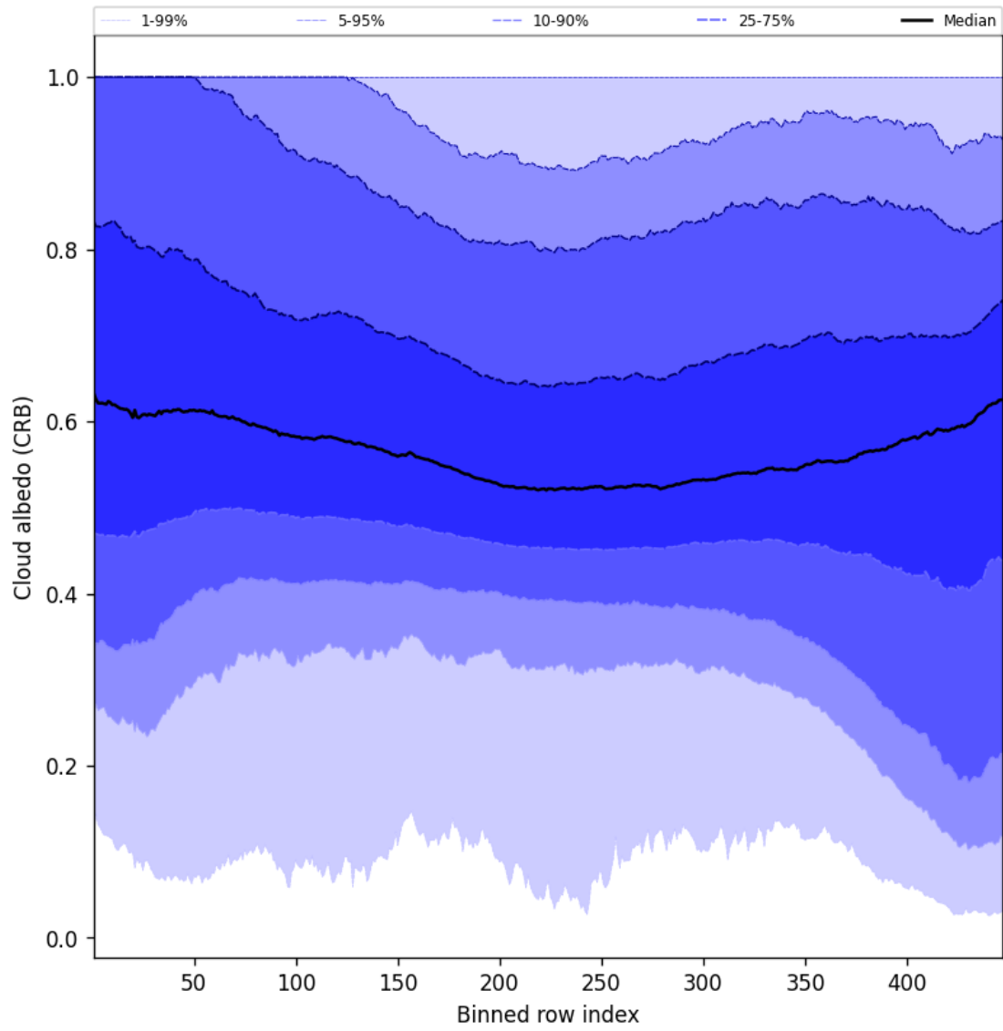
Figure 58: Along track statistics of “Cloud albedo (CRB)” for 2025-09-11 to 2025-09-12
