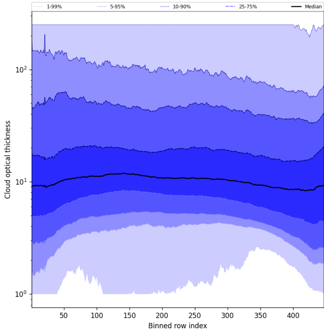
Figure 55: Along track statistics of “Cloud optical thickness” for 2025-09-11 to 2025-09-12
