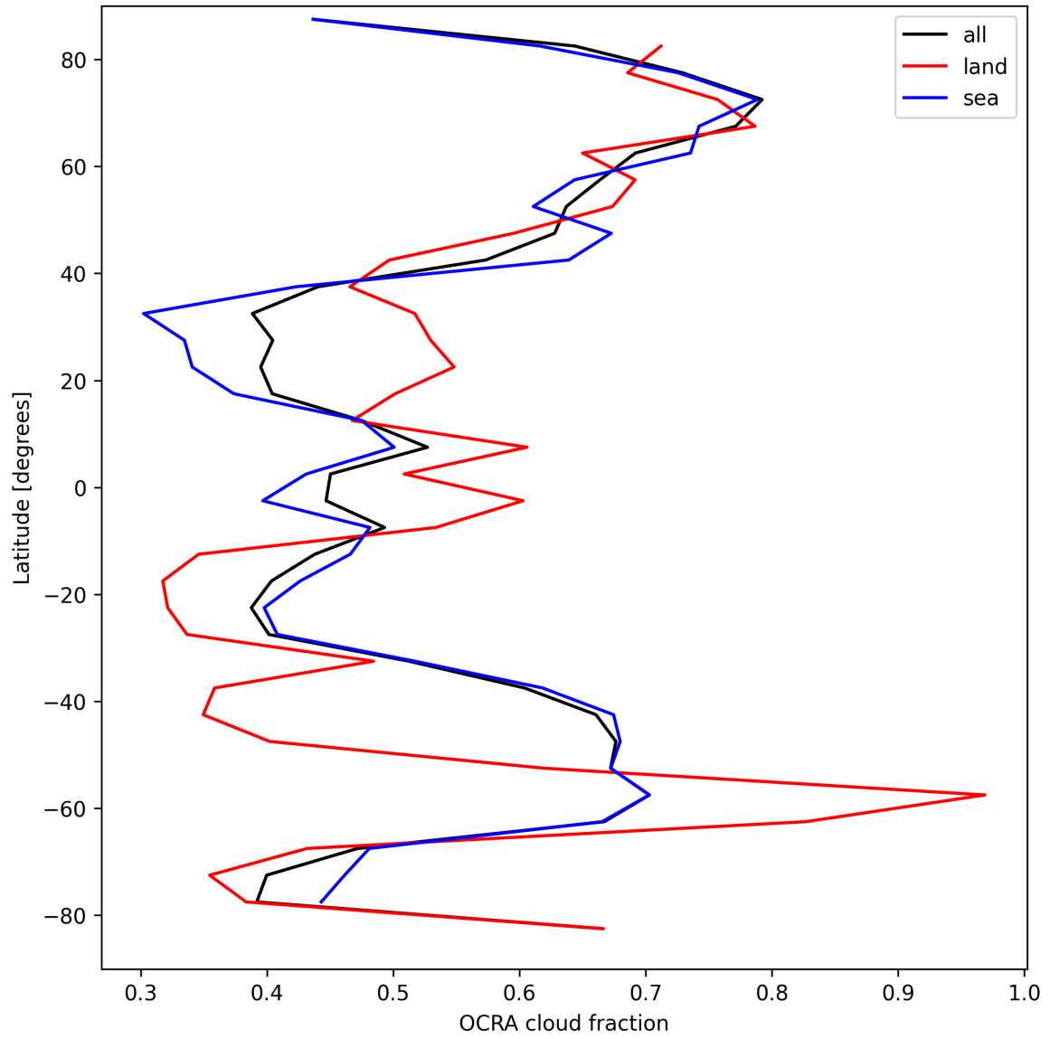
Figure 32: Zonal average of “OCRA cloud fraction” for 2025-09-11 to 2025-09-12.
