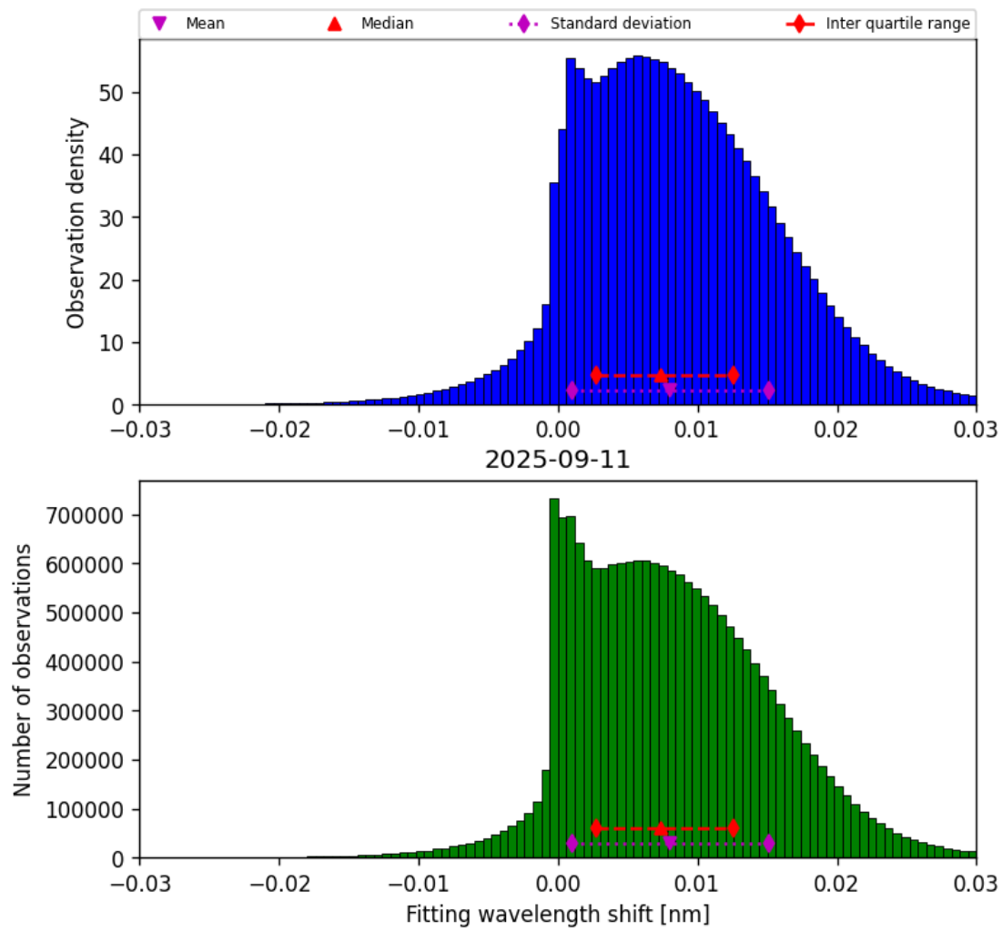
Figure 47: Histogram of “Fitting wavelength shift” for 2025-09-11 to 2025-09-12
