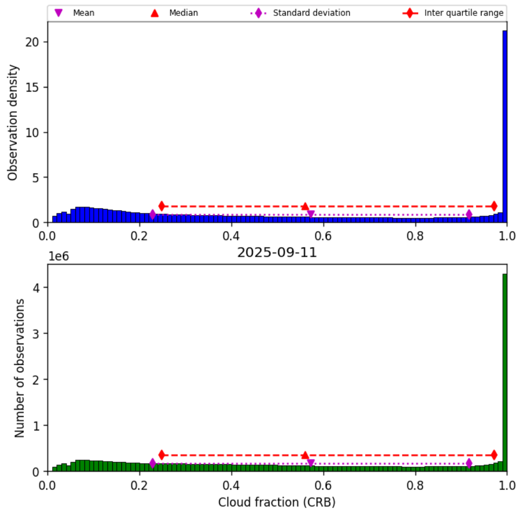
Figure 40: Histogram of “Cloud fraction (CRB)” for 2025-09-11 to 2025-09-12
