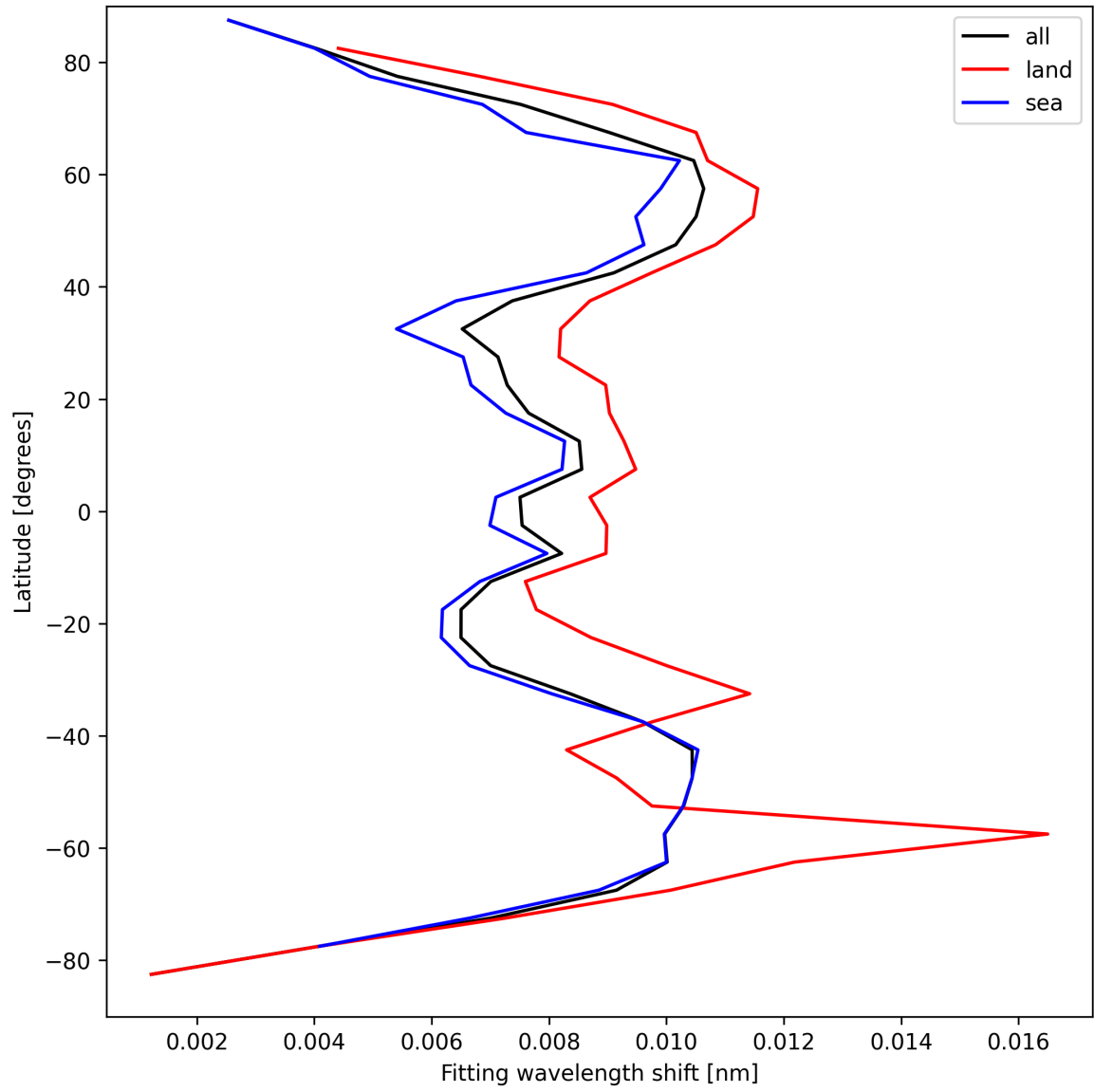
Figure 31: Zonal average of “Fitting wavelength shift” for 2025-09-11 to 2025-09-12.
