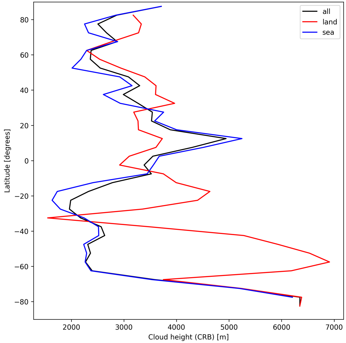
Figure 25: Zonal average of “Cloud height (CRB)” for 2025-09-11 to 2025-09-12.
