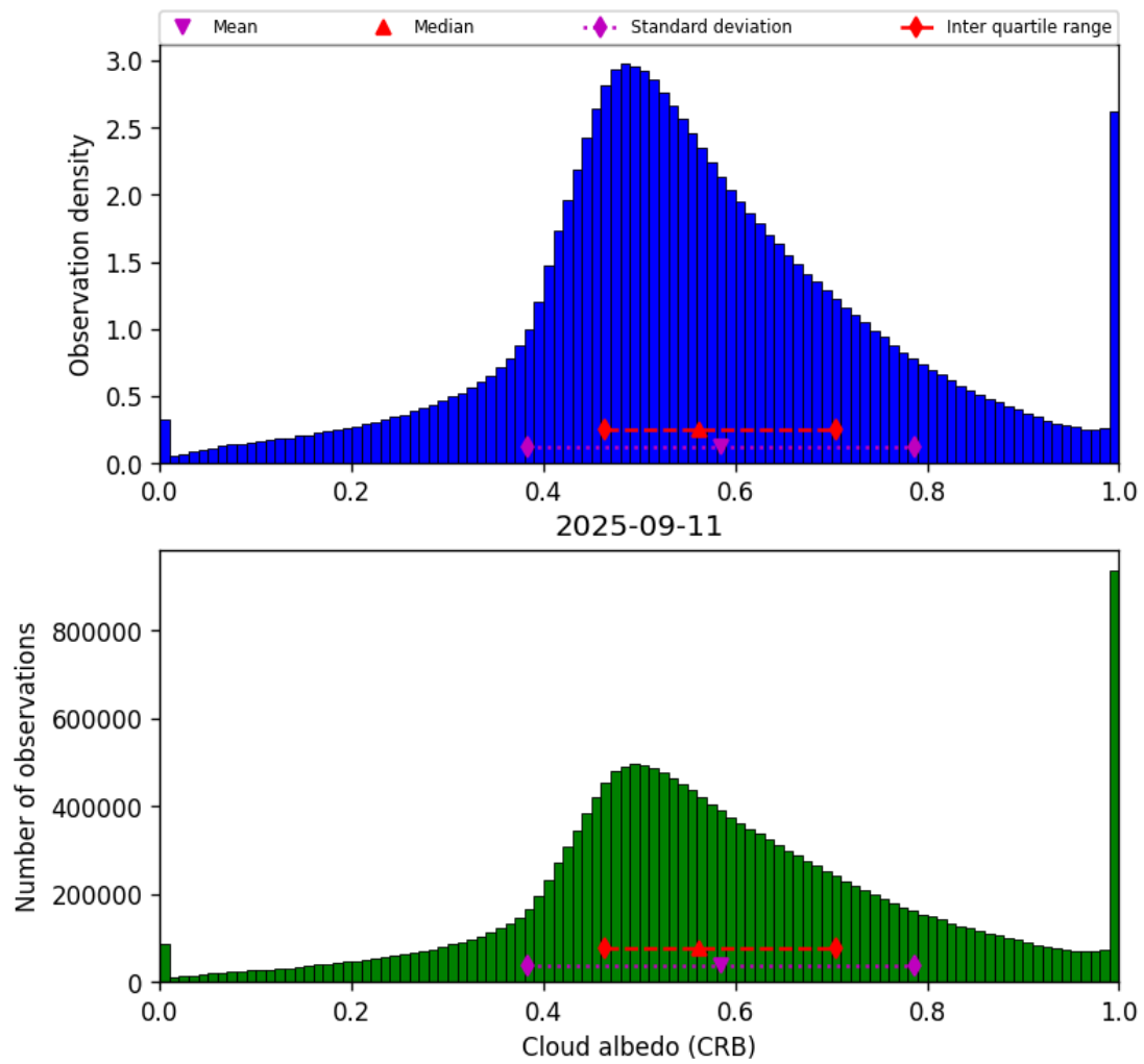
Figure 42: Histogram of “Cloud albedo (CRB)” for 2025-09-11 to 2025-09-12
