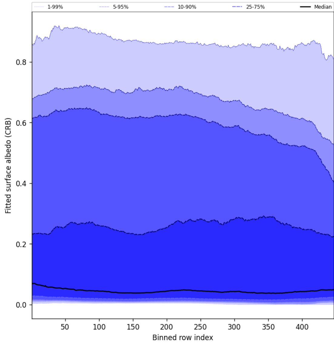
Figure 60: Along track statistics of “Fitted surface albedo (CRB)” for 2025-09-11 to 2025-09-12
