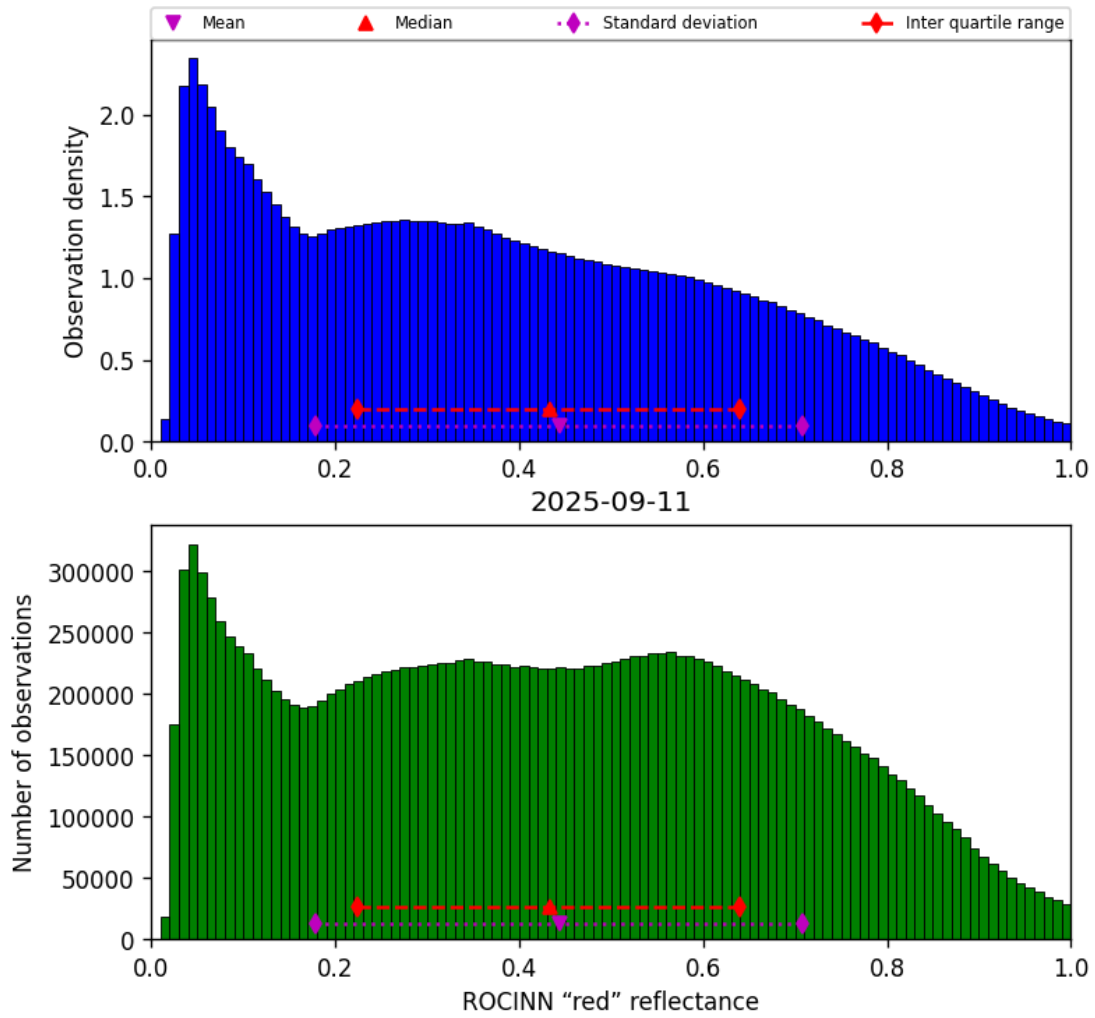
Figure 51: Histogram of “ROCINN “red” reflectance” for 2025-09-11 to 2025-09-12
