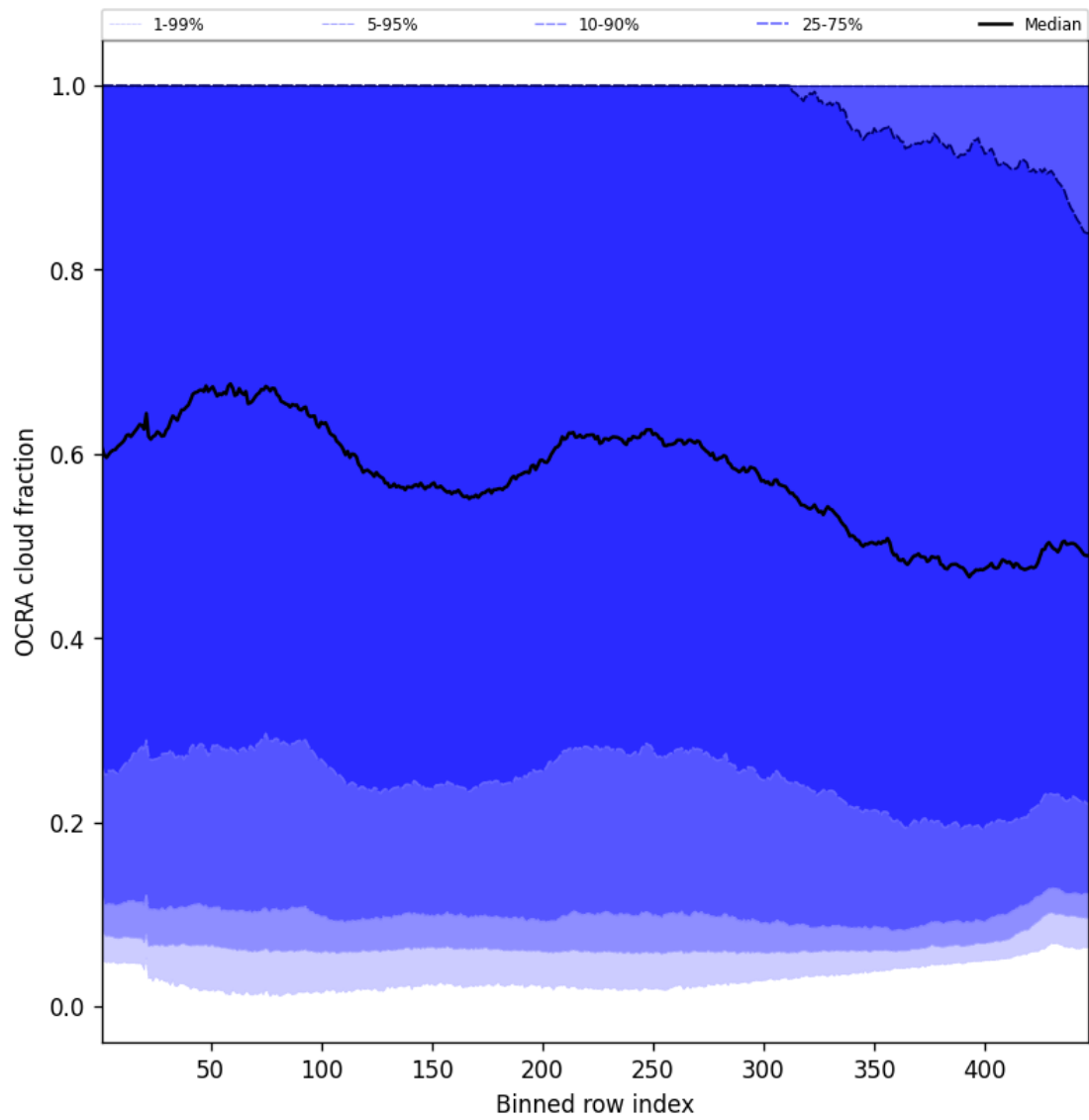
Figure 64: Along track statistics of “OCRA cloud fraction” for 2025-09-11 to 2025-09-12
