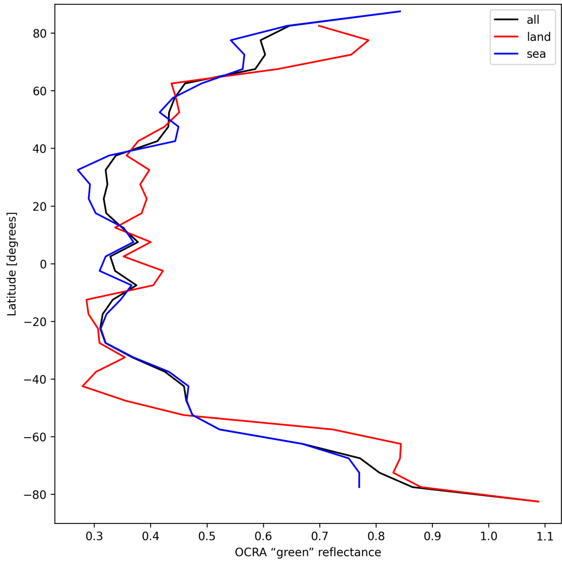
Figure 34: Zonal average of “OCRA “green” reflectance” for 2025-09-11 to 2025-09-12.
