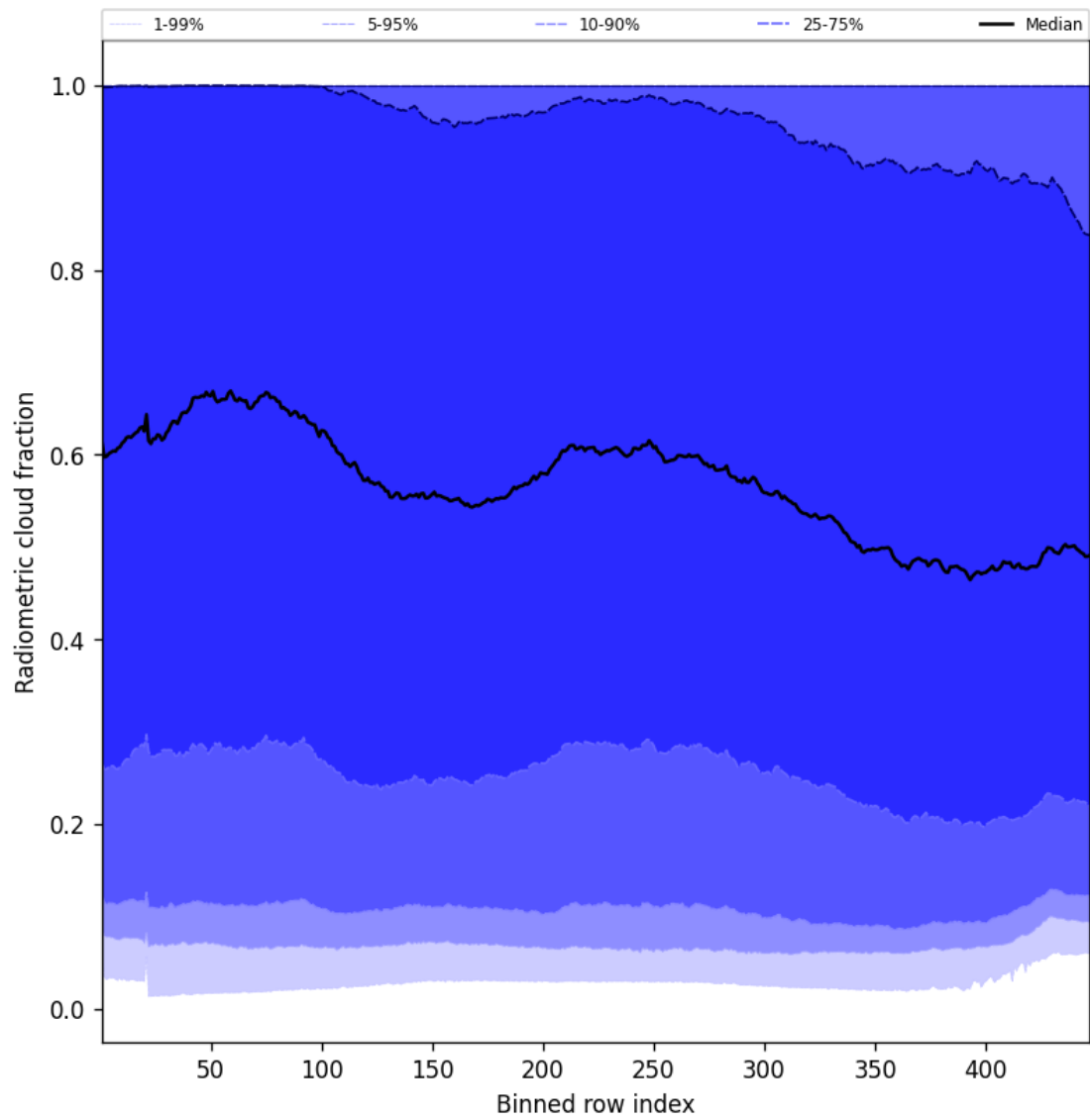
Figure 53: Along track statistics of “Radiometric cloud fraction” for 2025-09-11 to 2025-09-12
