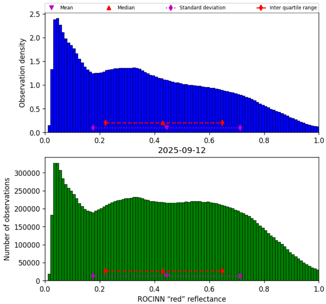
Figure 51: Histogram of "ROCINN "red" reflectance" for 2025-09-12 to 2025-09-13
