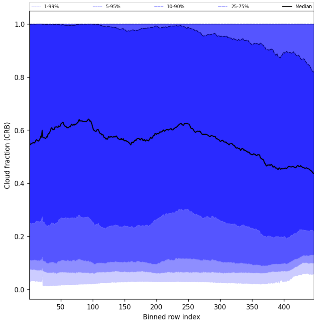
Figure 56: Along track statistics of “Cloud fraction (CRB)” for 2025-09-12 to 2025-09-13
