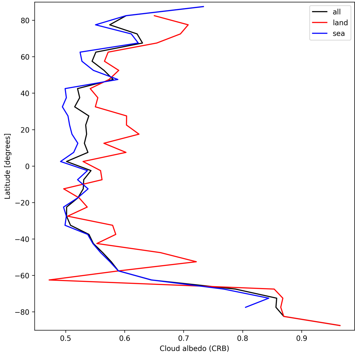
Figure 26: Zonal average of “Cloud albedo (CRB)” for 2025-09-12 to 2025-09-13.
