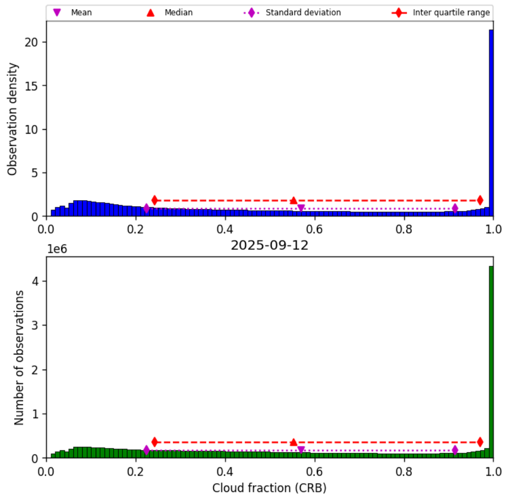
Figure 40: Histogram of “Cloud fraction (CRB)” for 2025-09-12 to 2025-09-13
