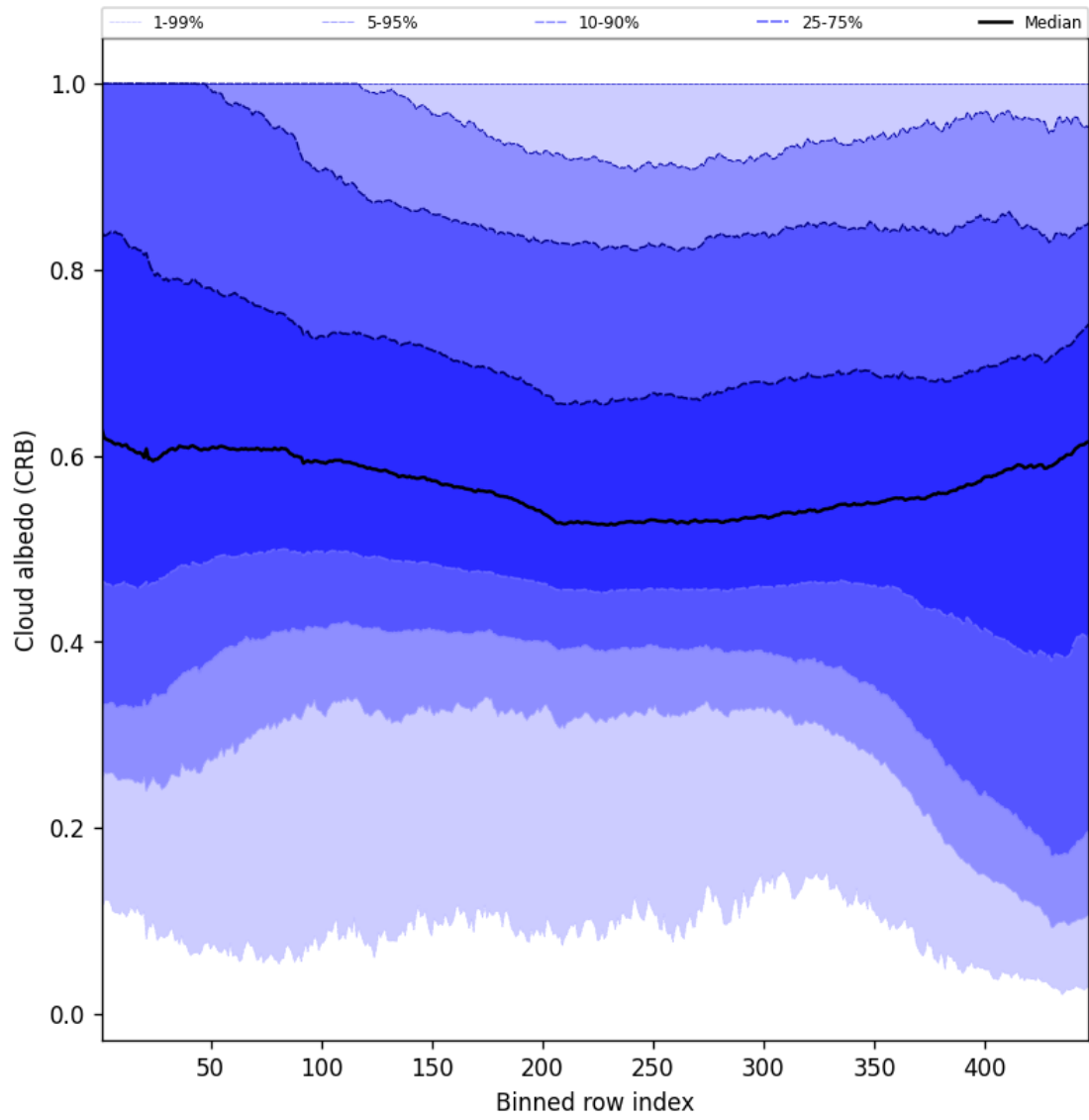
Figure 58: Along track statistics of “Cloud albedo (CRB)” for 2025-09-12 to 2025-09-13
