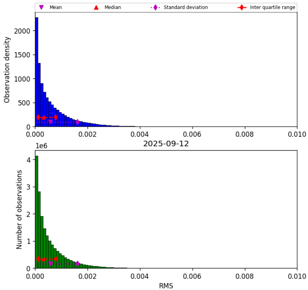
Figure 45: Histogram of “RMS” for 2025-09-12 to 2025-09-13
