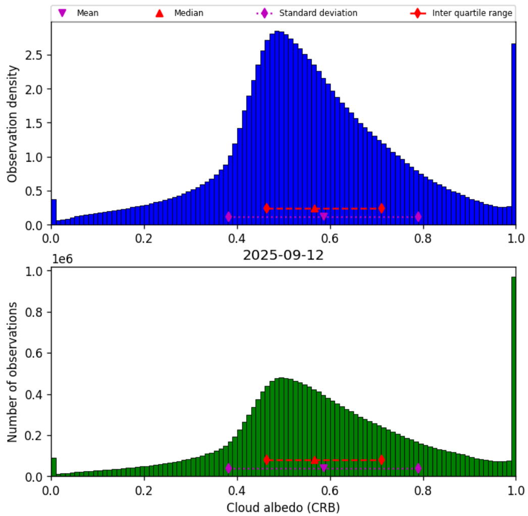
Figure 42: Histogram of “Cloud albedo (CRB)” for 2025-09-12 to 2025-09-13
