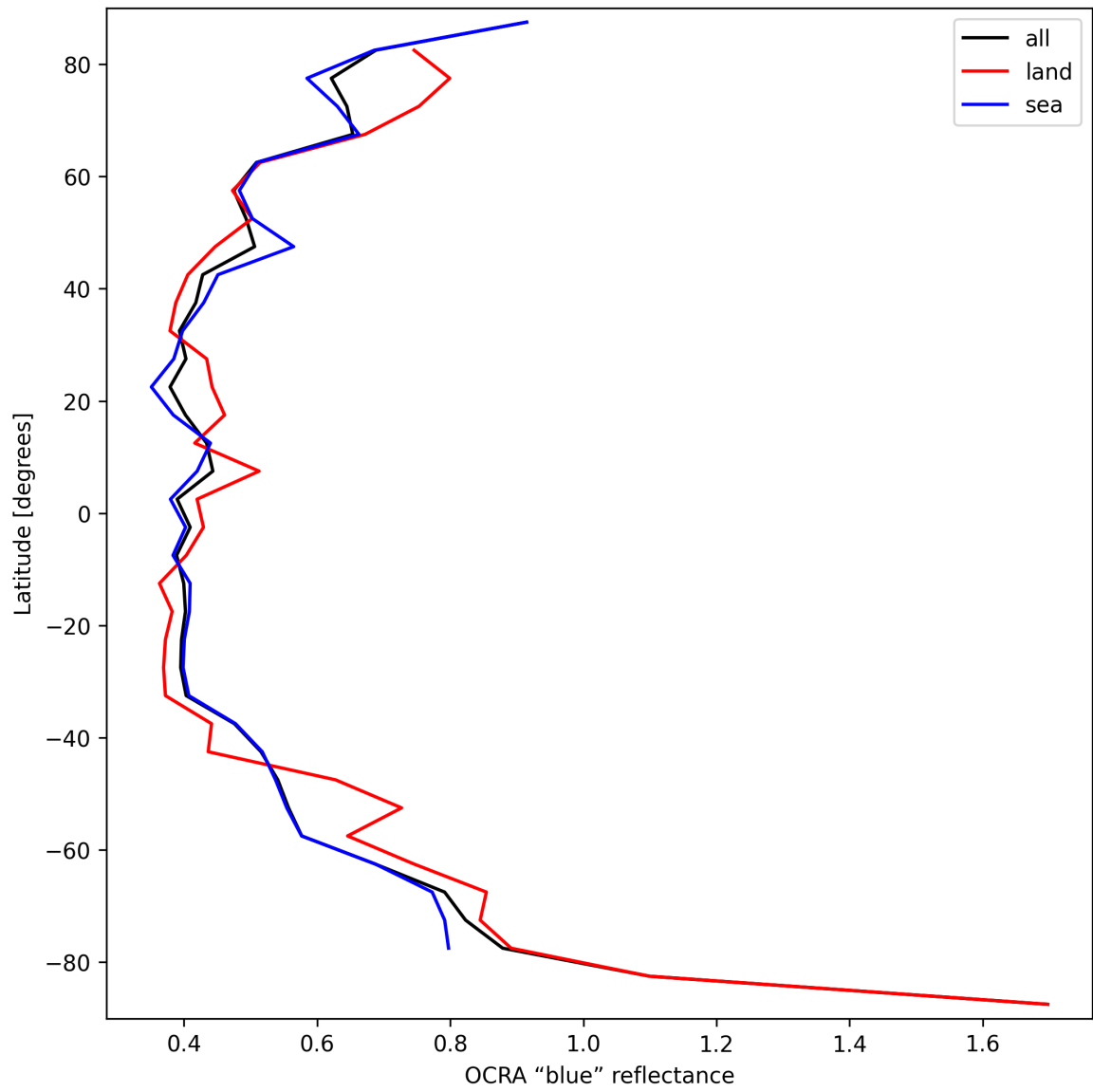
Figure 33: Zonal average of “OCRA “blue” reflectance” for 2025-09-12 to 2025-09-13.
