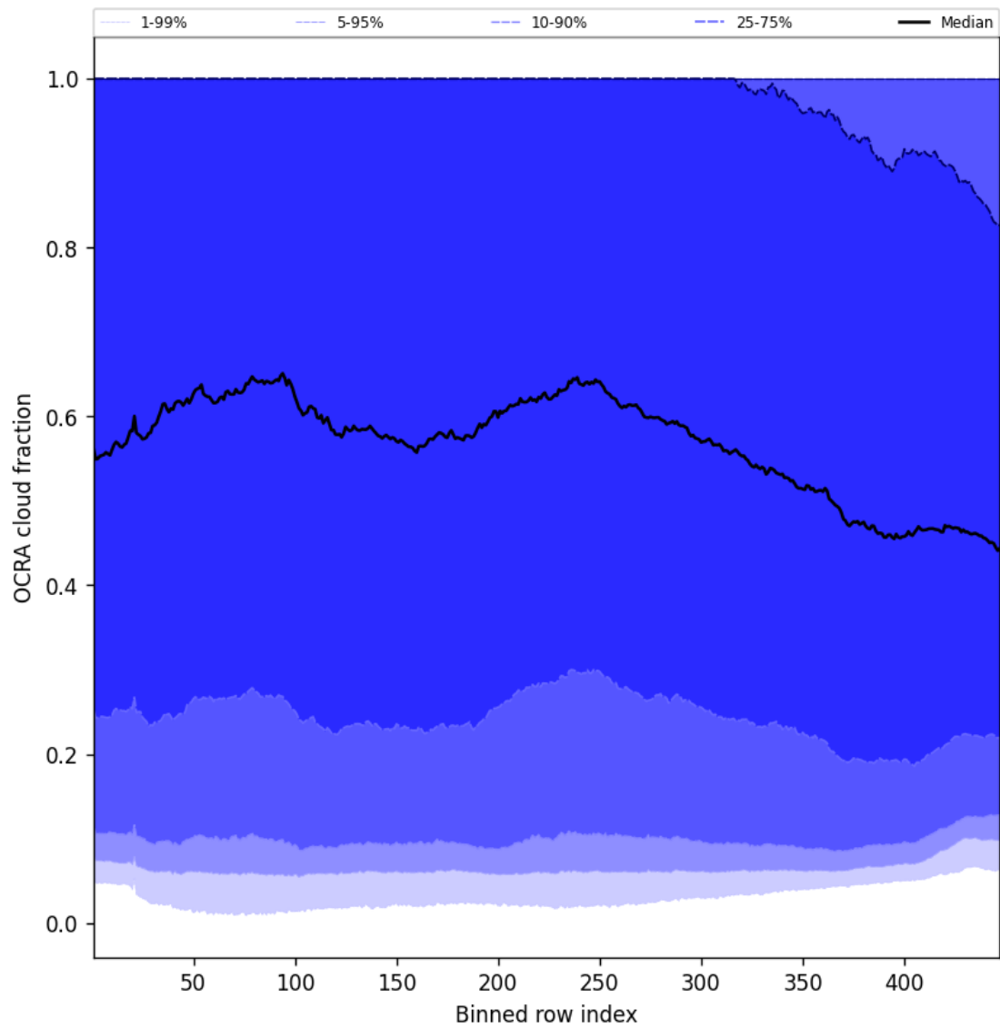
Figure 64: Along track statistics of “OCRA cloud fraction” for 2025-09-12 to 2025-09-13
