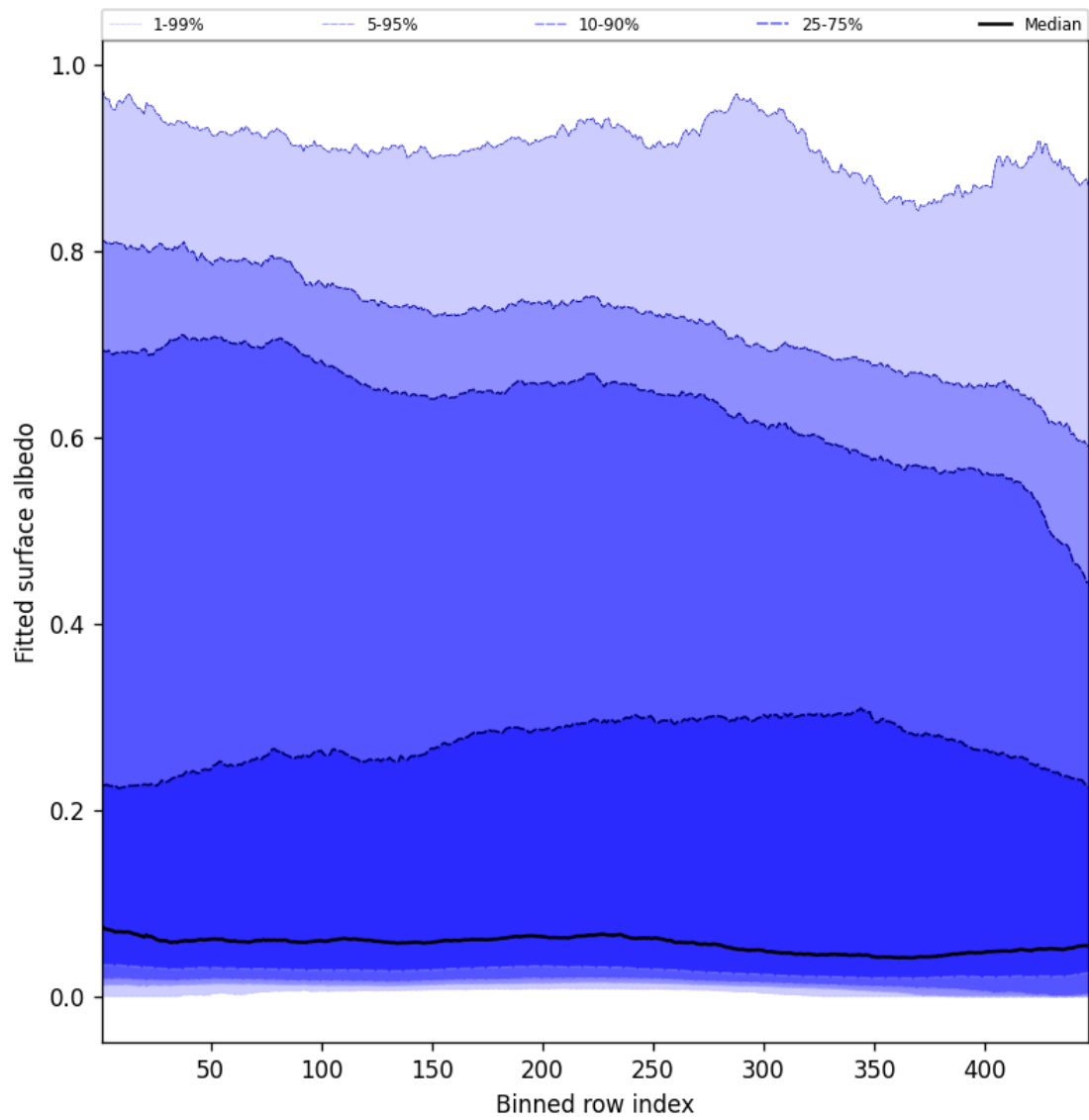
Figure 59: Along track statistics of “Fitted surface albedo” for 2025-09-12 to 2025-09-13
