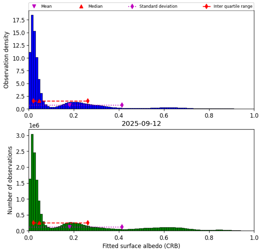
Figure 44: Histogram of “Fitted surface albedo (CRB)” for 2025-09-12 to 2025-09-13
