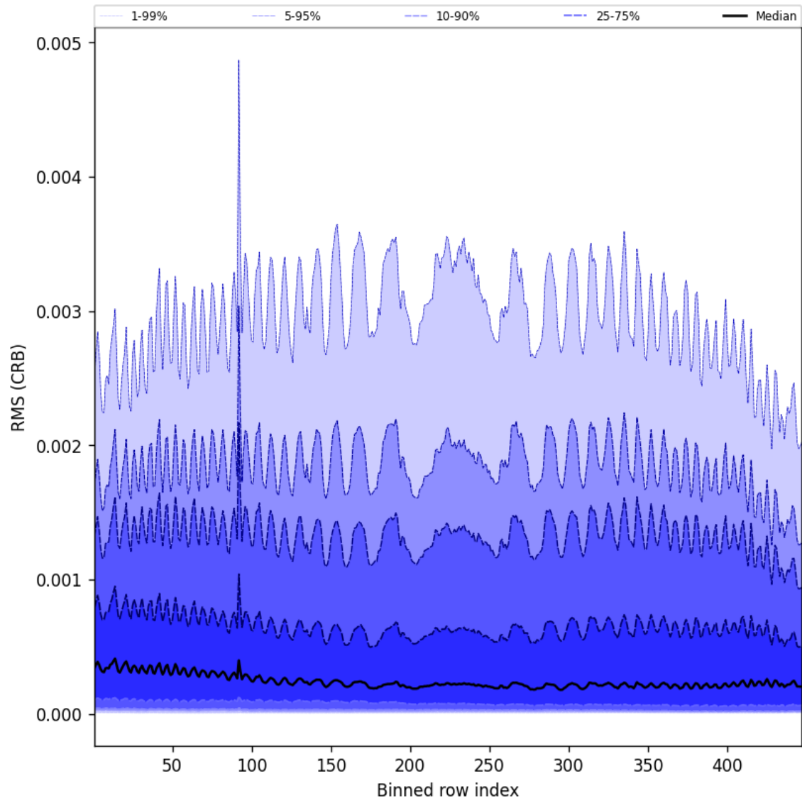
Figure 62: Along track statistics of “RMS (CRB)” for 2025-09-12 to 2025-09-13
