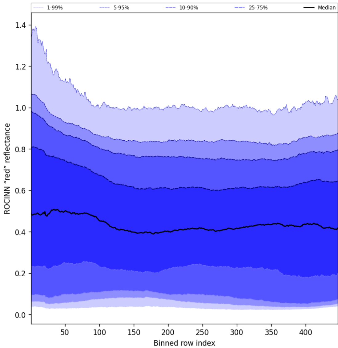
Figure 67: Along track statistics of "ROCINN "red" reflectance" for 2025-09-12 to 2025-09-13
