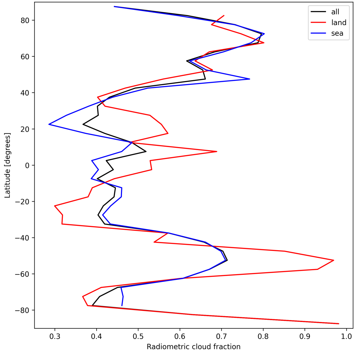
Figure 21: Zonal average of “Radiometric cloud fraction” for 2025-09-12 to 2025-09-13.
