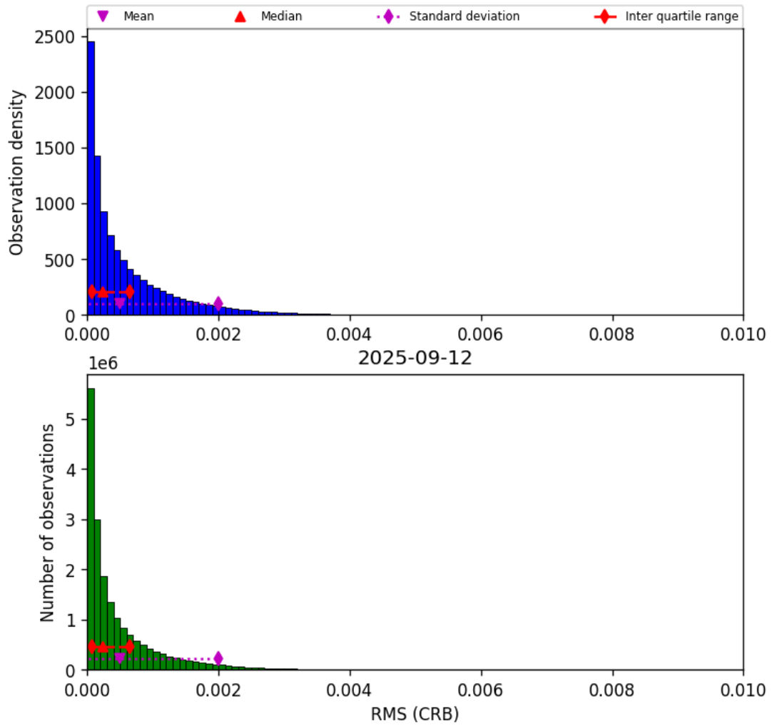
Figure 46: Histogram of “RMS (CRB)” for 2025-09-12 to 2025-09-13
