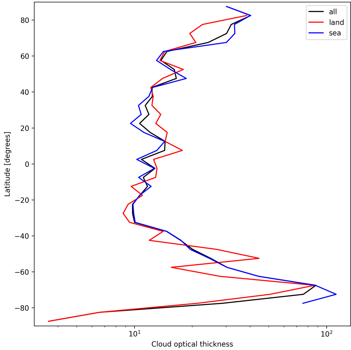
Figure 23: Zonal average of “Cloud optical thickness” for 2025-09-12 to 2025-09-13.
