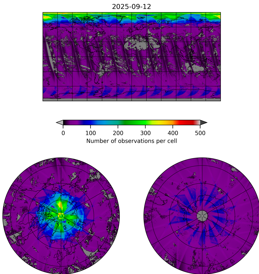
Figure 19: Map of the number of observations for 2025-09-12 to 2025-09-13
