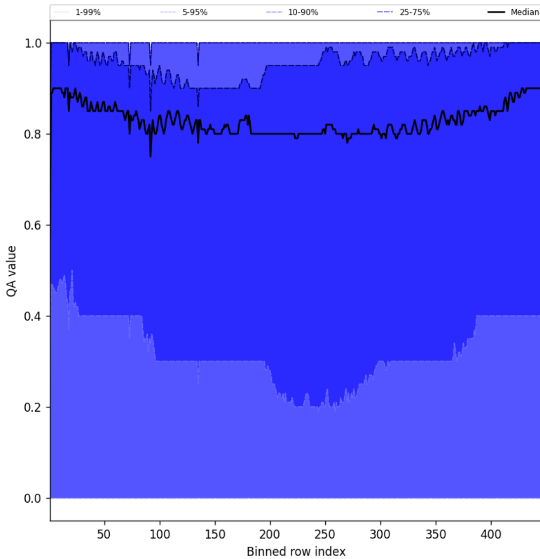
Figure 52: Along track statistics of “QA value” for 2025-09-12 to 2025-09-13
