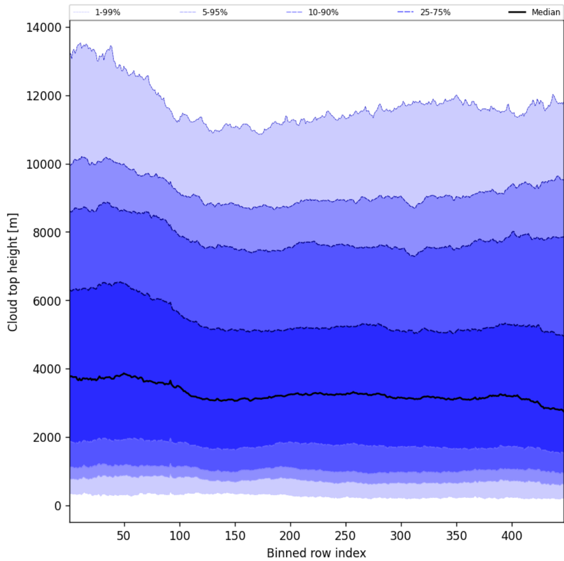
Figure 54: Along track statistics of “Cloud top height” for 2025-09-12 to 2025-09-13
