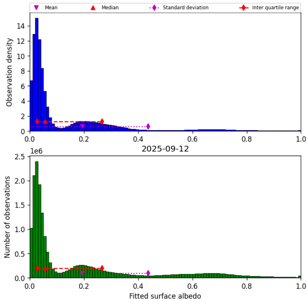
Figure 43: Histogram of “Fitted surface albedo” for 2025-09-12 to 2025-09-13
