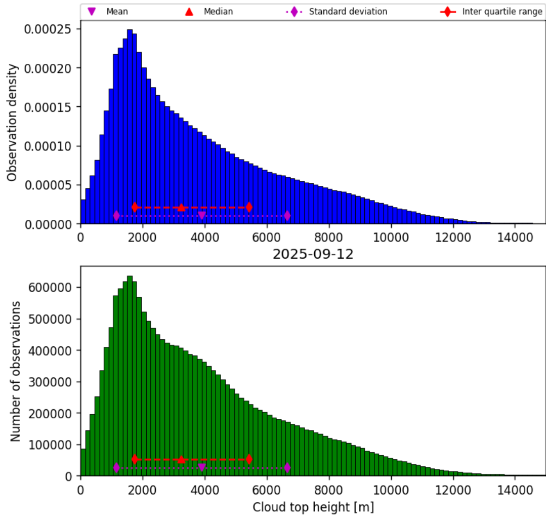
Figure 38: Histogram of “Cloud top height” for 2025-09-12 to 2025-09-13
