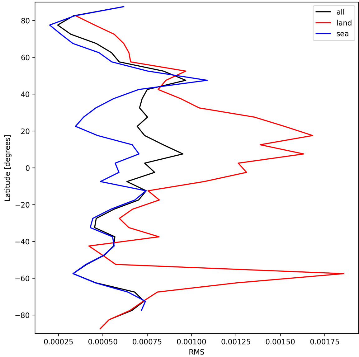
Figure 29: Zonal average of “RMS” for 2025-09-12 to 2025-09-13.
