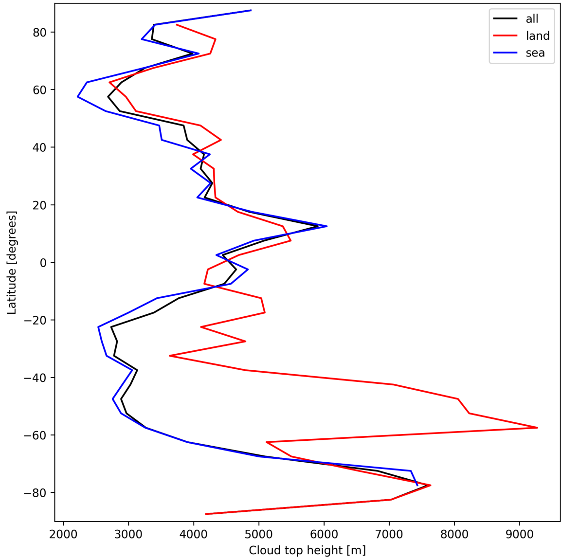
Figure 22: Zonal average of “Cloud top height” for 2025-09-12 to 2025-09-13.
