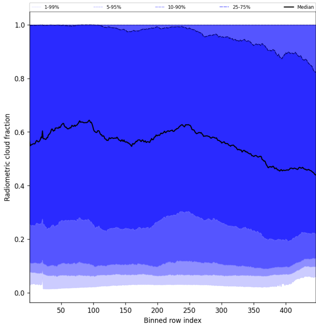
Figure 53: Along track statistics of “Radiometric cloud fraction” for 2025-09-12 to 2025-09-13
