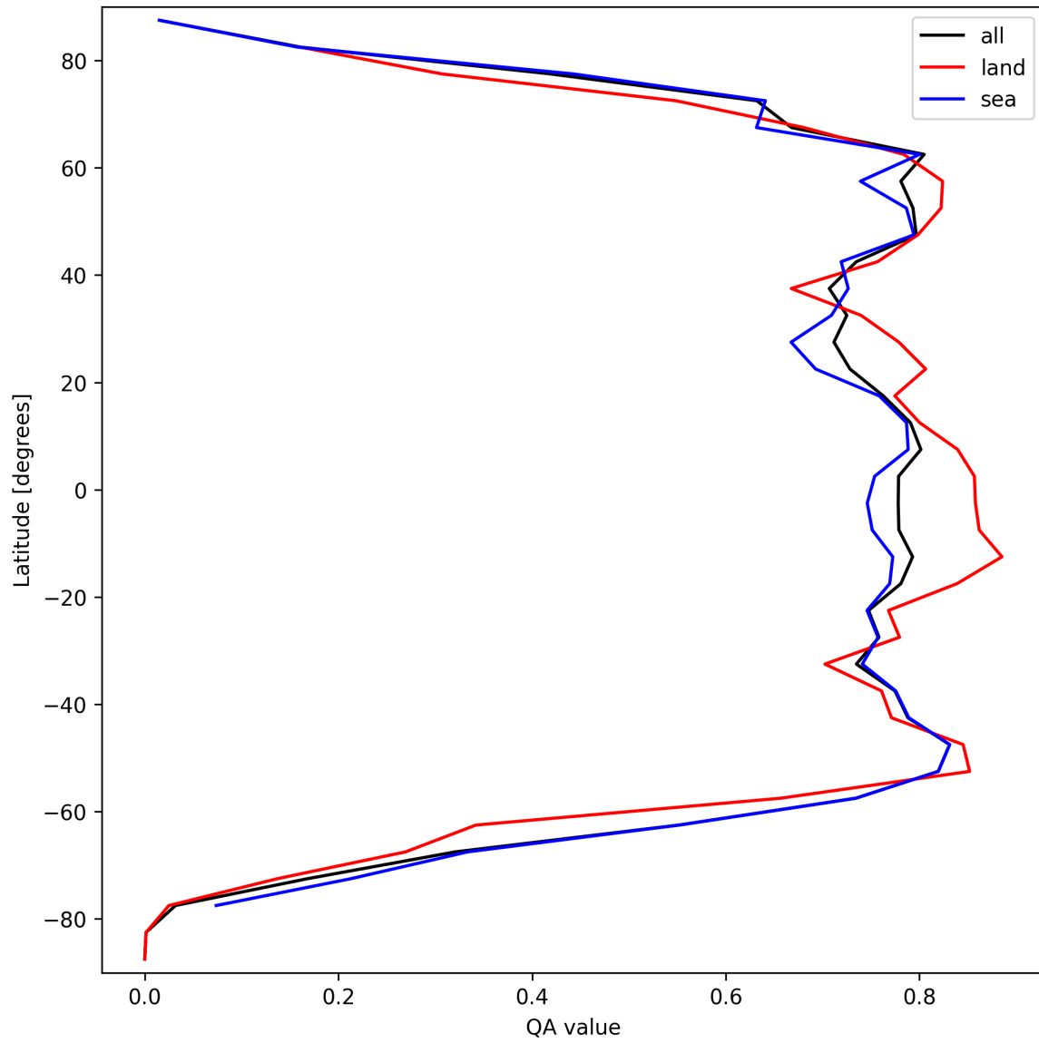
Figure 20: Zonal average of “QA value” for 2025-09-12 to 2025-09-13.
