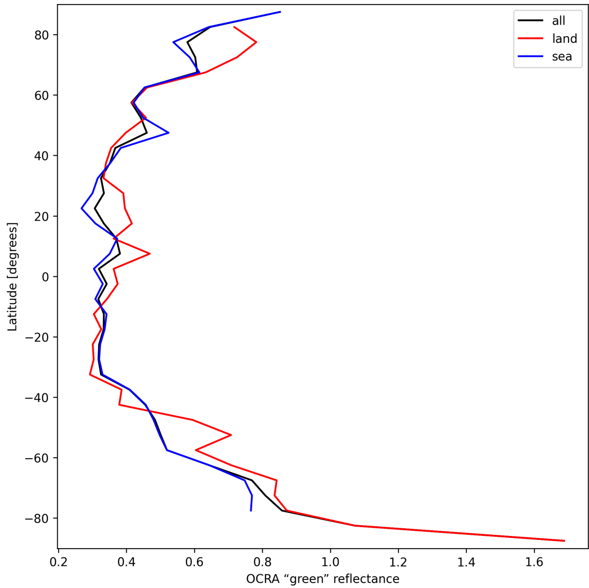
Figure 34: Zonal average of “OCRA “green” reflectance” for 2025-09-12 to 2025-09-13.
