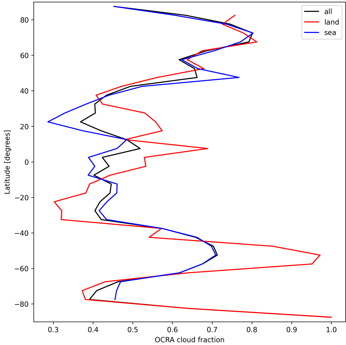
Figure 32: Zonal average of “OCRA cloud fraction” for 2025-09-12 to 2025-09-13.
