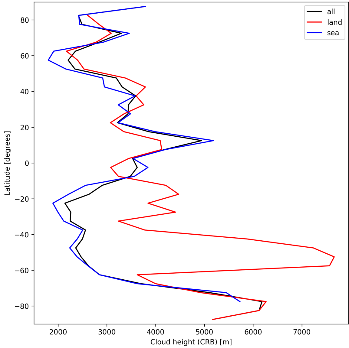
Figure 25: Zonal average of “Cloud height (CRB)” for 2025-09-12 to 2025-09-13.
