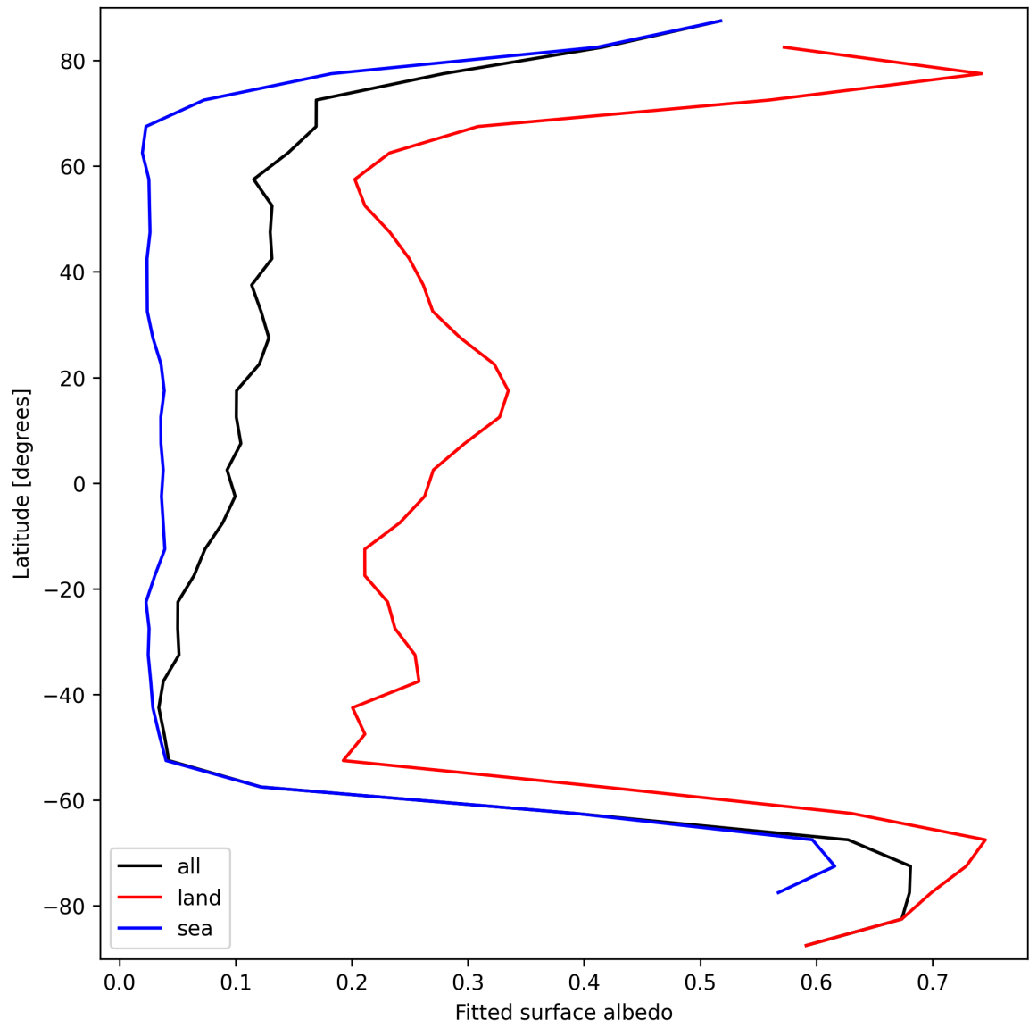
Figure 27: Zonal average of “Fitted surface albedo” for 2025-09-12 to 2025-09-13.
