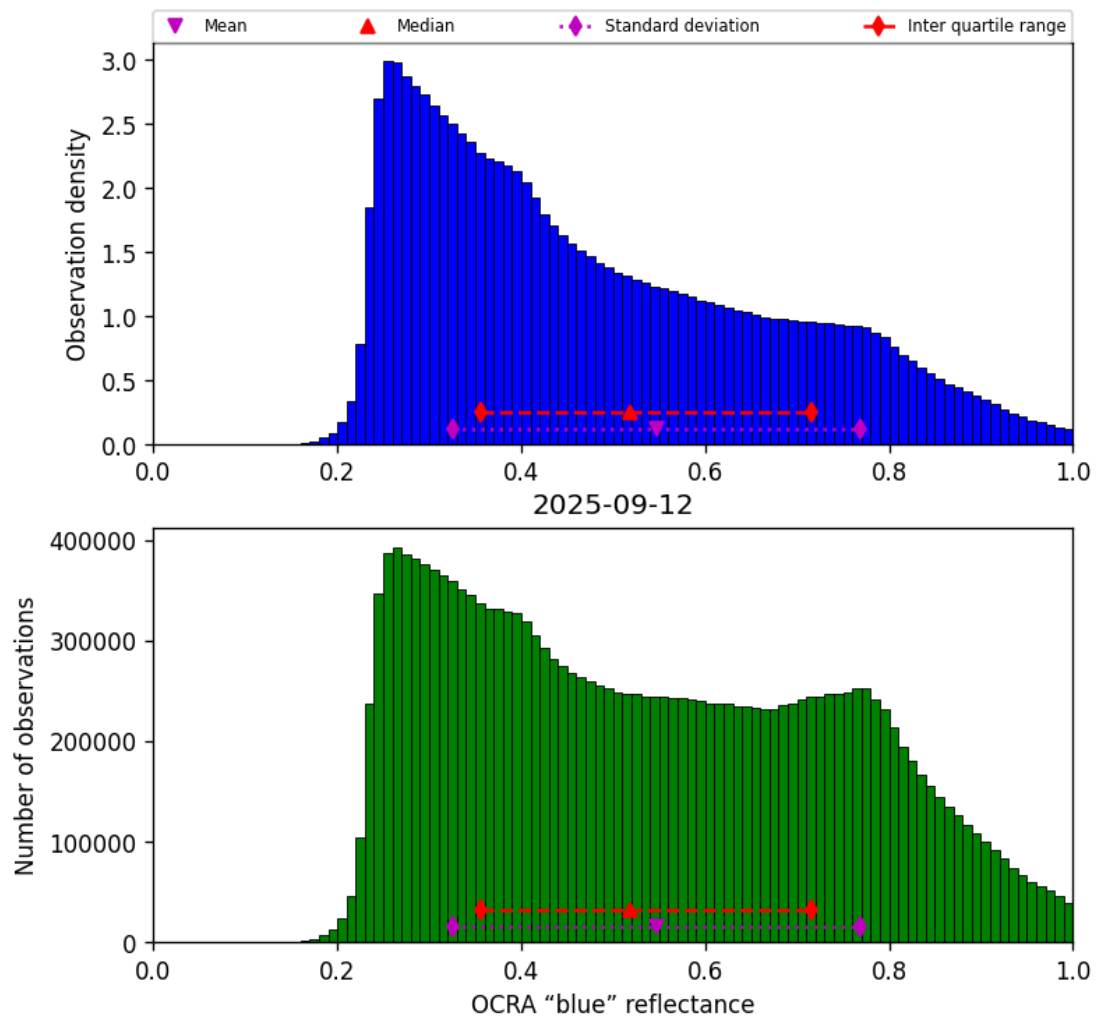
Figure 49: Histogram of “OCRA “blue” reflectance” for 2025-09-12 to 2025-09-13
