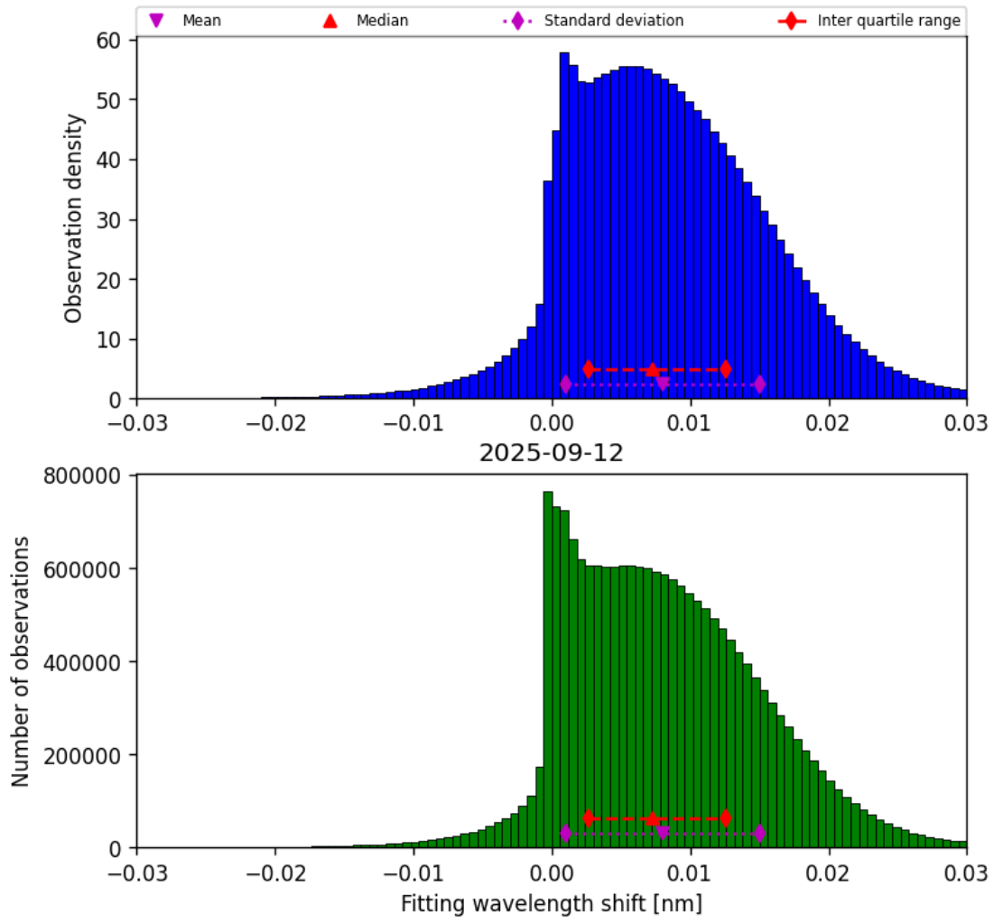
Figure 47: Histogram of “Fitting wavelength shift” for 2025-09-12 to 2025-09-13
