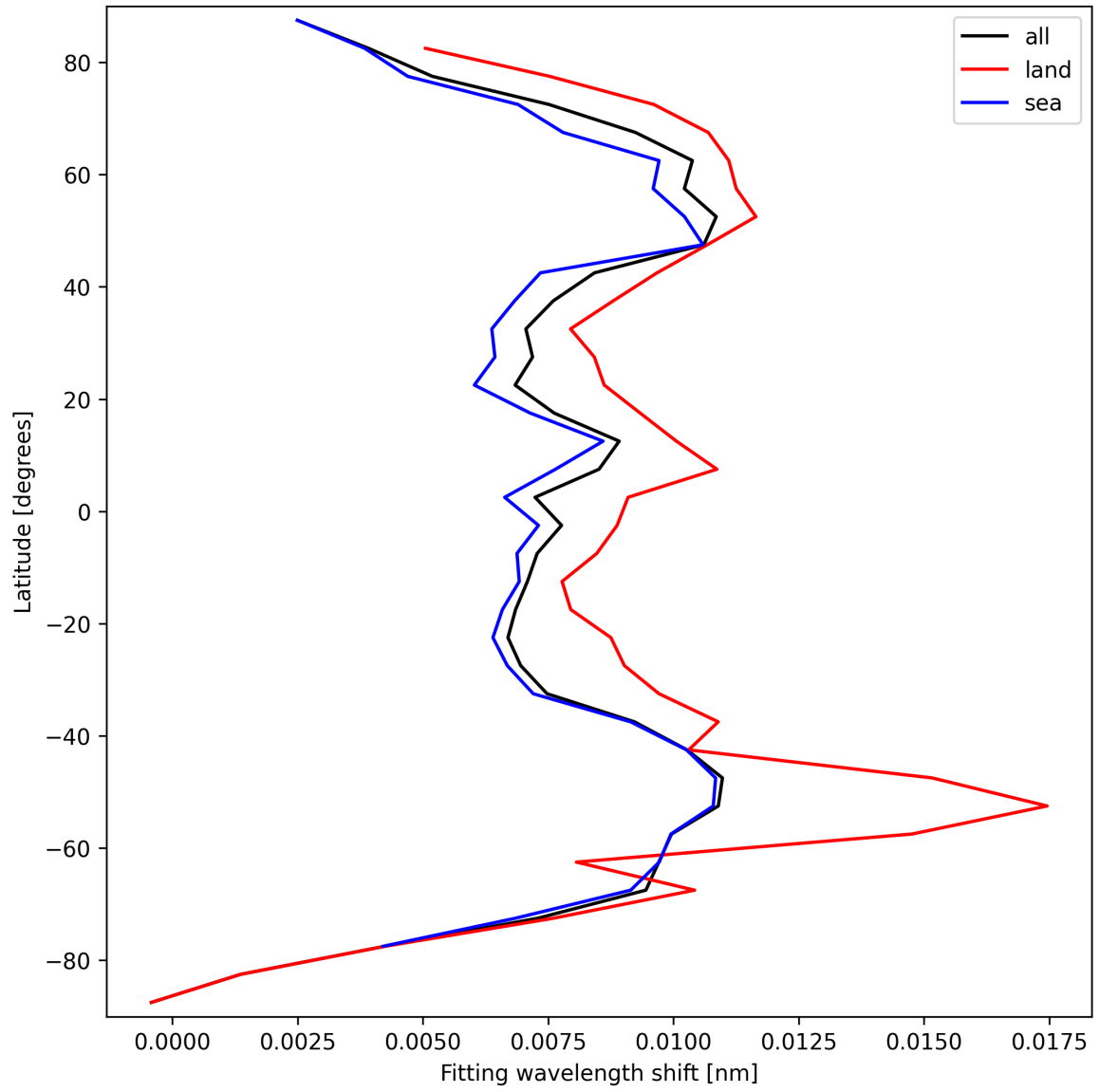
Figure 31: Zonal average of “Fitting wavelength shift” for 2025-09-12 to 2025-09-13.
