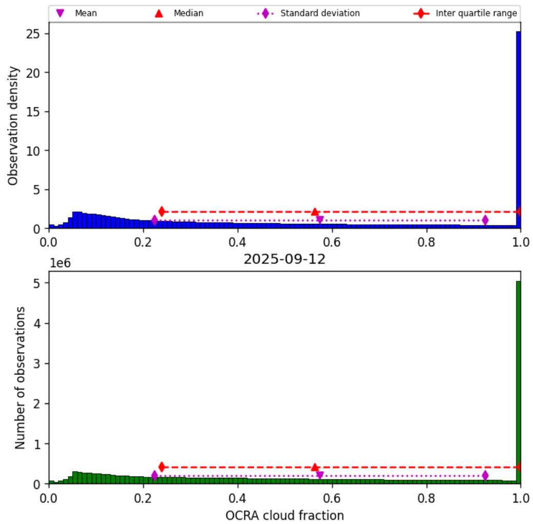
Figure 48: Histogram of “OCRA cloud fraction” for 2025-09-12 to 2025-09-13
