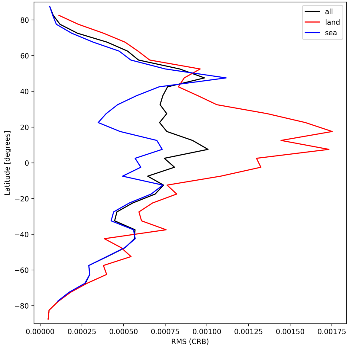
Figure 30: Zonal average of “RMS (CRB)” for 2025-09-12 to 2025-09-13.
