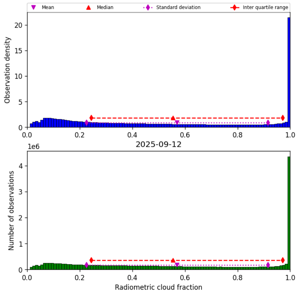
Figure 37: Histogram of “Radiometric cloud fraction” for 2025-09-12 to 2025-09-13
