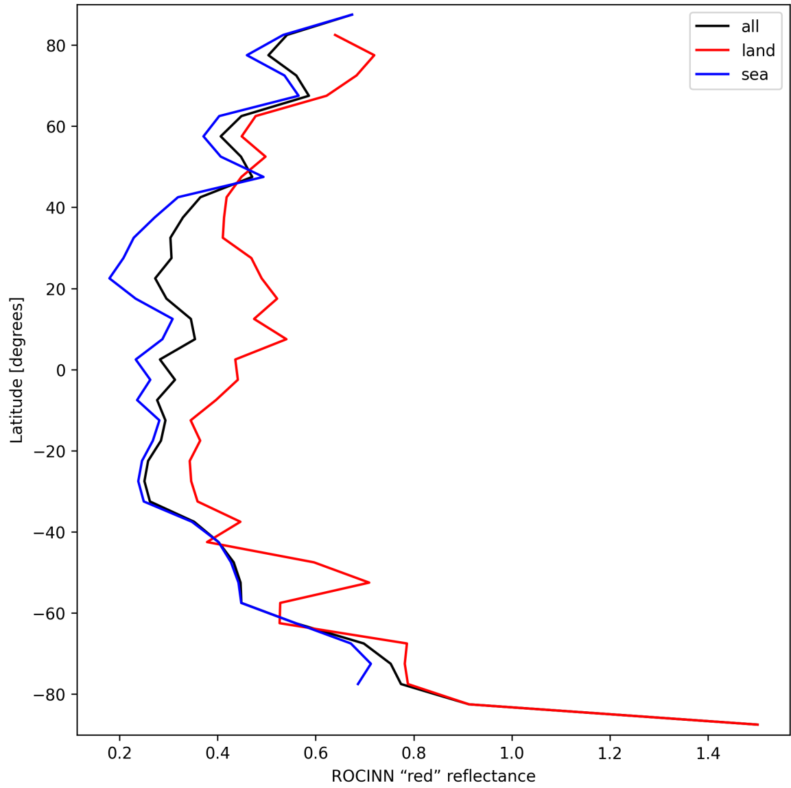
Figure 35: Zonal average of “ROCINN “red” reflectance” for 2025-09-12 to 2025-09-13.
