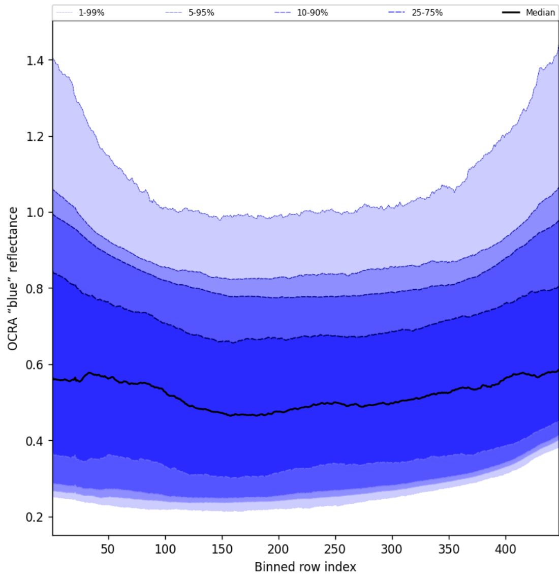
Figure 65: Along track statistics of "OCRA "blue" reflectance" for 2025-09-12 to 2025-09-13
