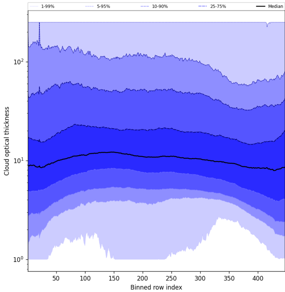
Figure 55: Along track statistics of “Cloud optical thickness” for 2025-09-12 to 2025-09-13
