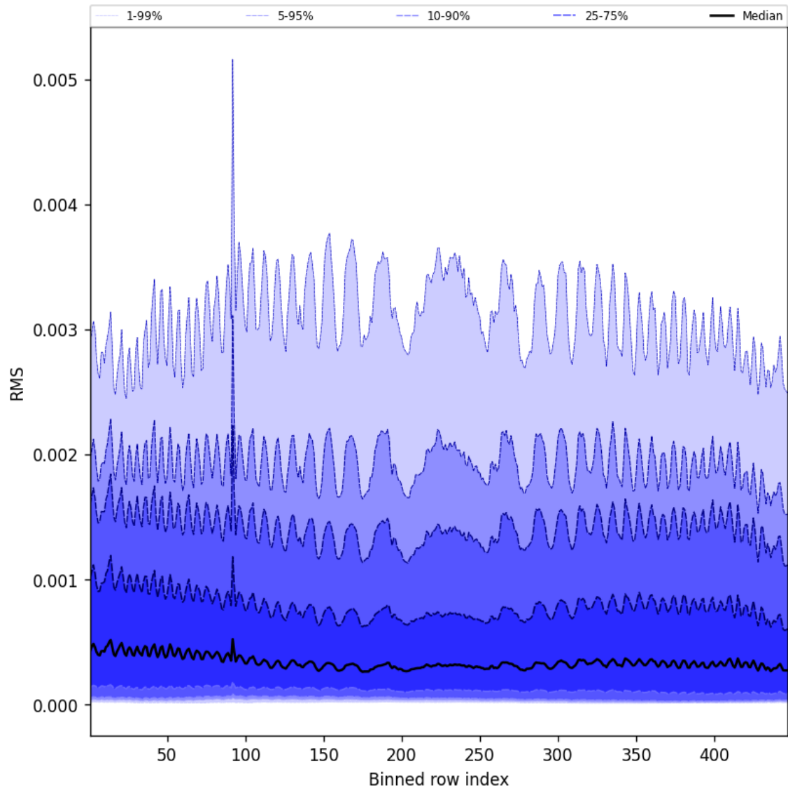
Figure 61: Along track statistics of “RMS” for 2025-09-12 to 2025-09-13
