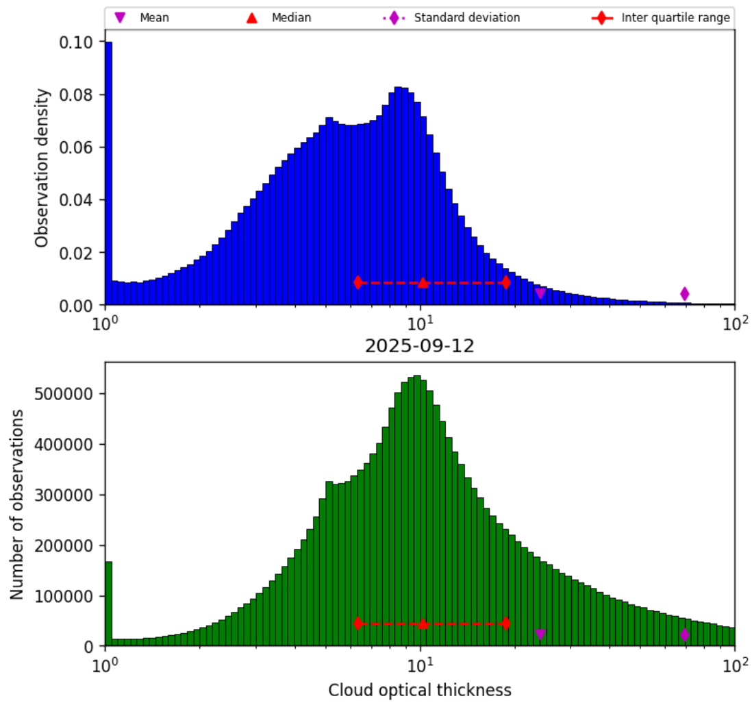
Figure 39: Histogram of “Cloud optical thickness” for 2025-09-12 to 2025-09-13
