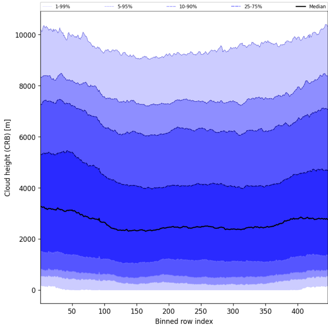
Figure 57: Along track statistics of “Cloud height (CRB)” for 2025-09-12 to 2025-09-13
