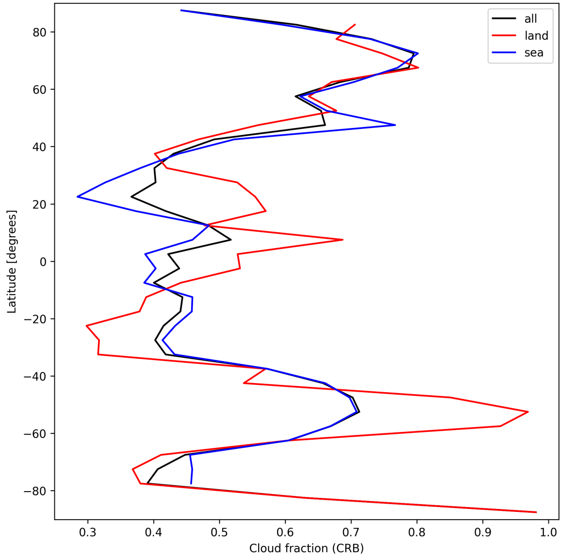
Figure 24: Zonal average of “Cloud fraction (CRB)” for 2025-09-12 to 2025-09-13.
