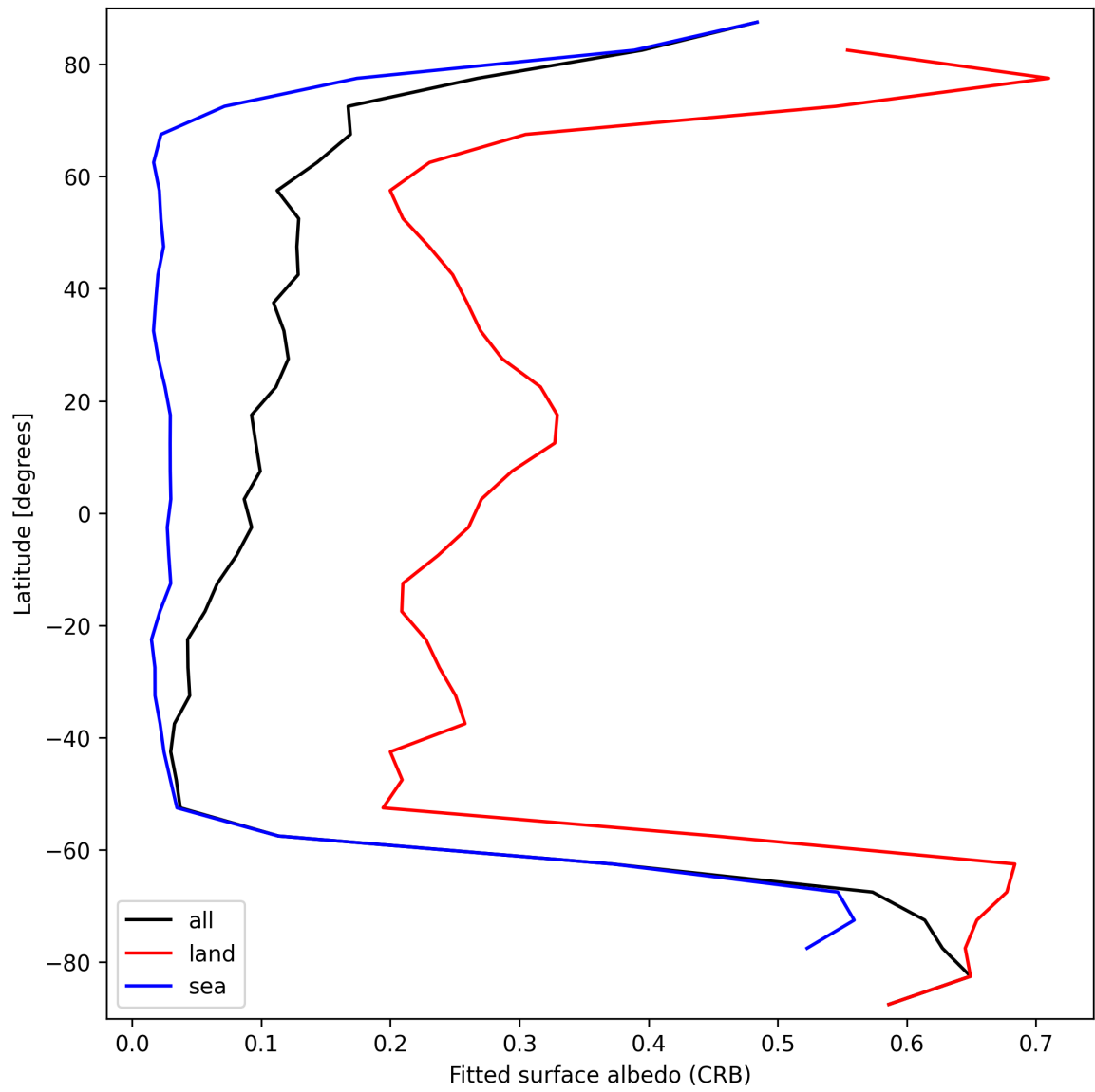
Figure 28: Zonal average of “Fitted surface albedo (CRB)” for 2025-09-12 to 2025-09-13.
