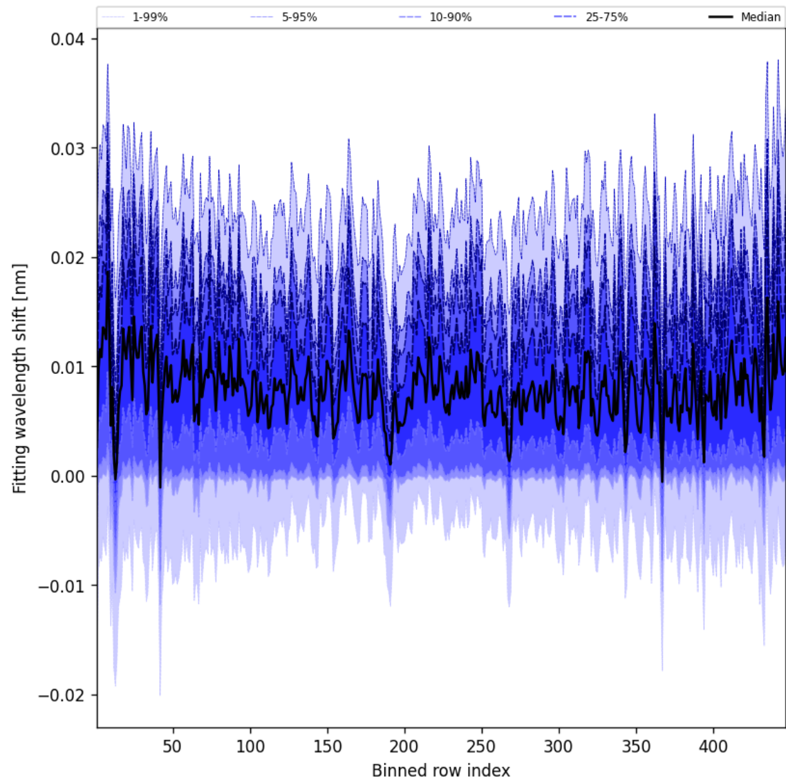
Figure 63: Along track statistics of “Fitting wavelength shift” for 2025-09-12 to 2025-09-13
