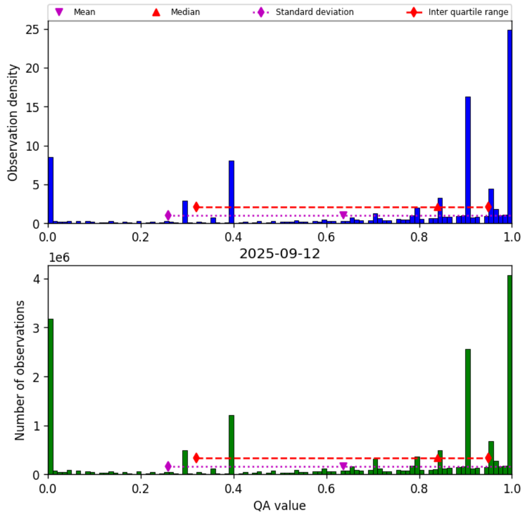
Figure 36: Histogram of “QA value” for 2025-09-12 to 2025-09-13
