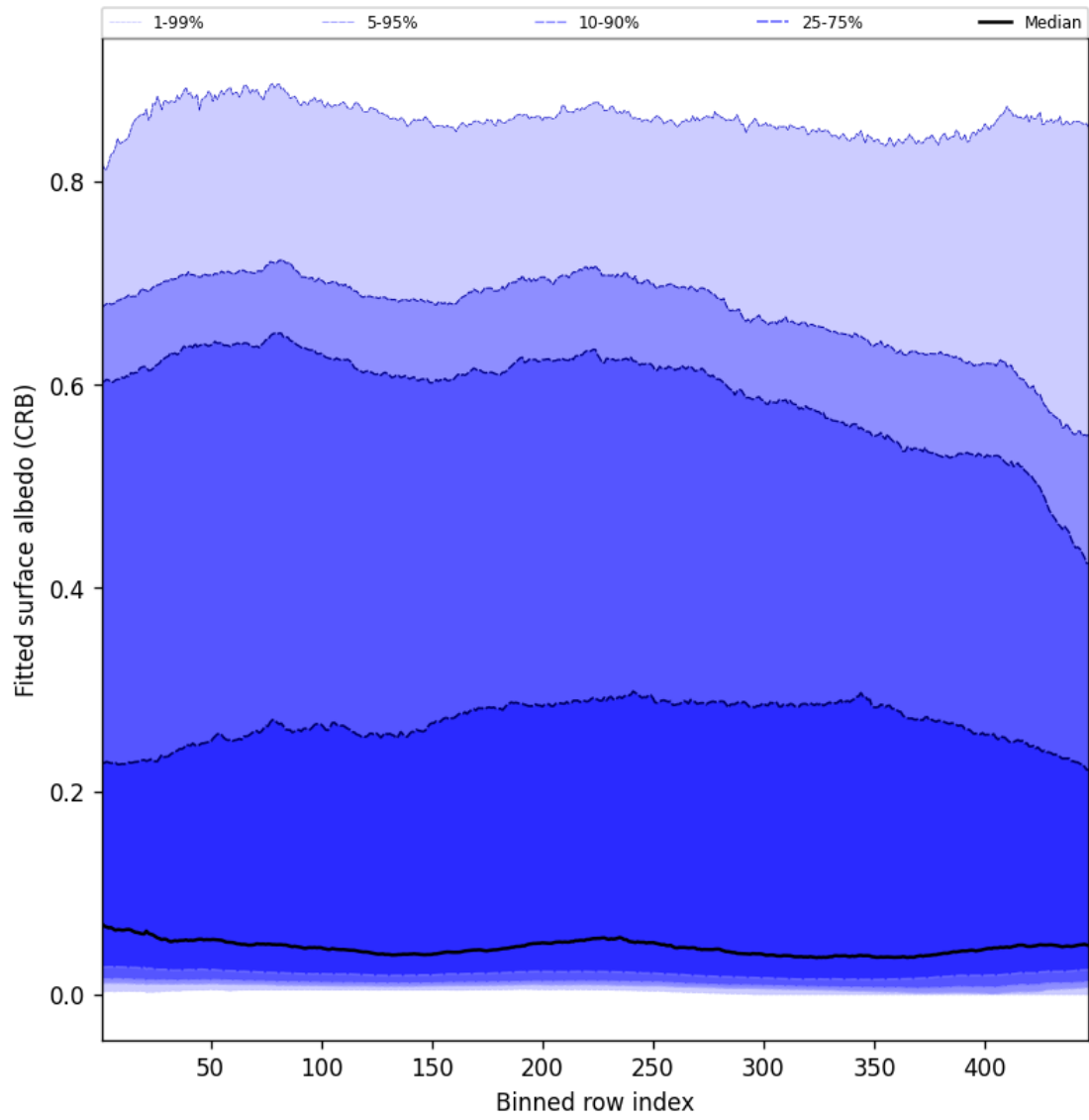
Figure 60: Along track statistics of “Fitted surface albedo (CRB)” for 2025-09-12 to 2025-09-13
