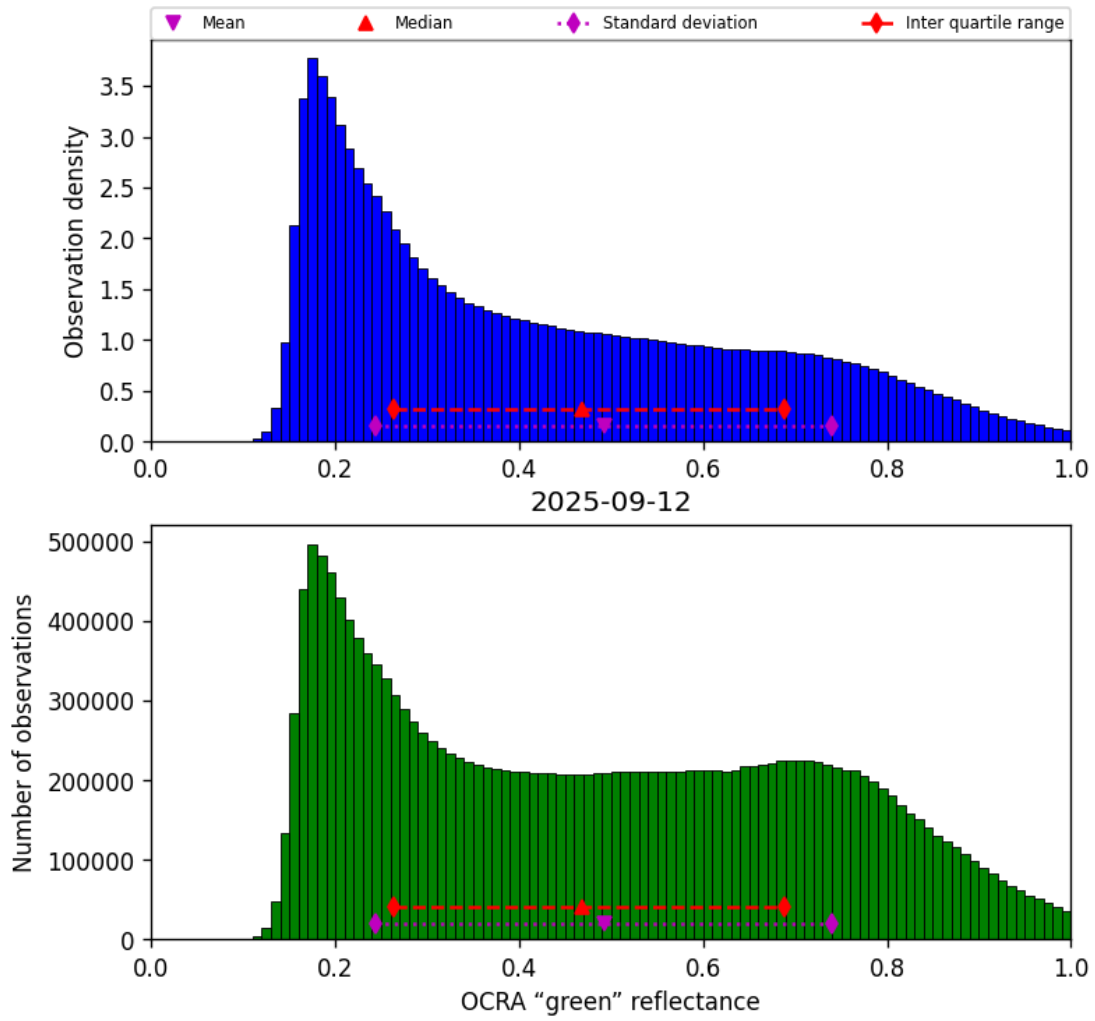
Figure 50: Histogram of “OCRA “green” reflectance” for 2025-09-12 to 2025-09-13
