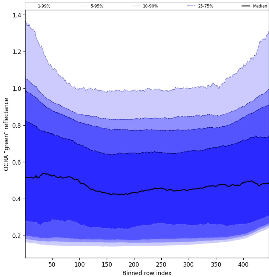
Figure 66: Along track statistics of “OCRA “green” reflectance” for 2025-09-12 to 2025-09-13
