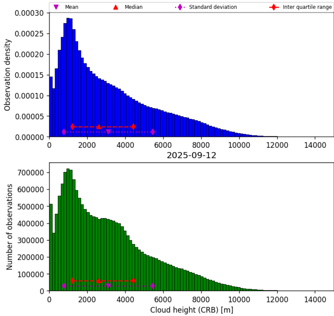
Figure 41: Histogram of “Cloud height (CRB)” for 2025-09-12 to 2025-09-13
