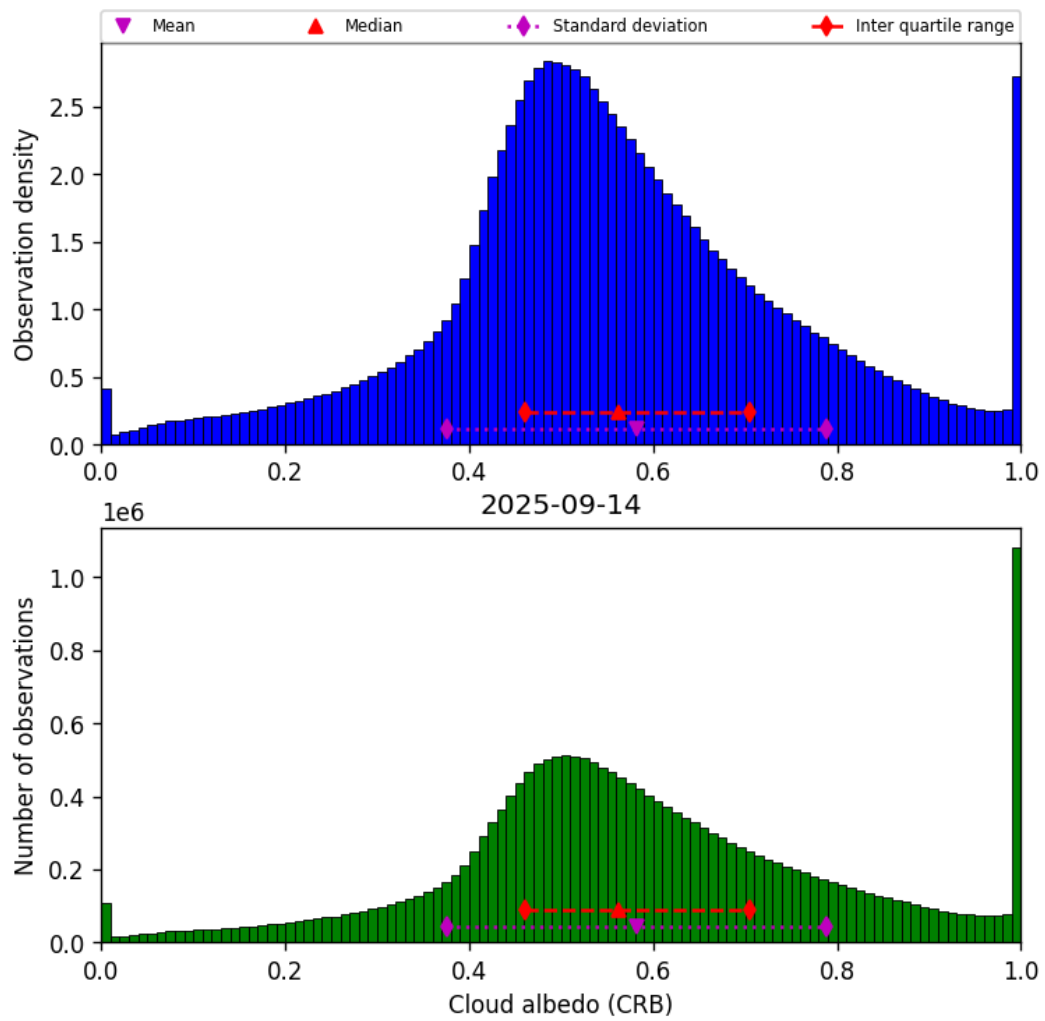
Figure 42: Histogram of “Cloud albedo (CRB)” for 2025-09-14 to 2025-09-15
