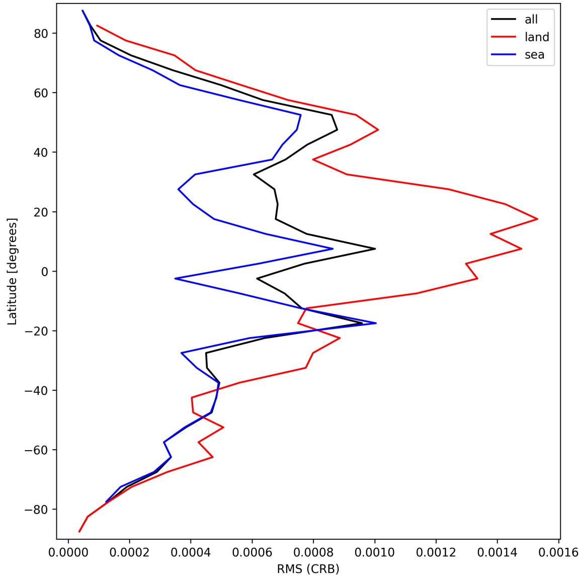
Figure 30: Zonal average of “RMS (CRB)” for 2025-09-14 to 2025-09-15.
