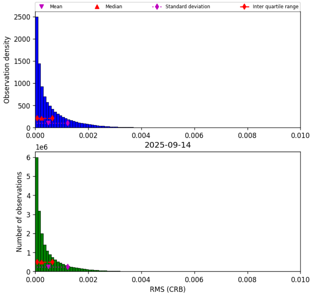
Figure 46: Histogram of “RMS (CRB)” for 2025-09-14 to 2025-09-15
