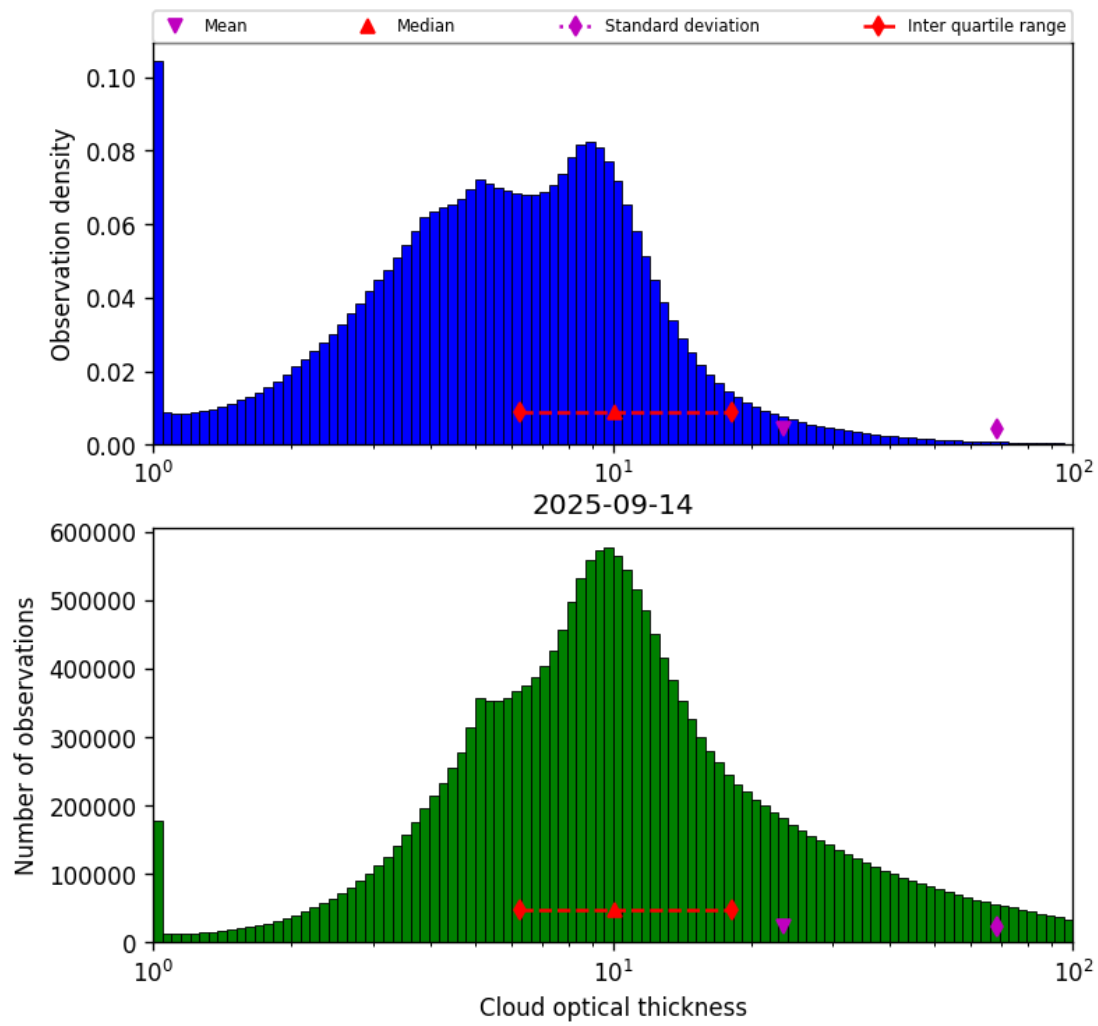
Figure 39: Histogram of “Cloud optical thickness” for 2025-09-14 to 2025-09-15
