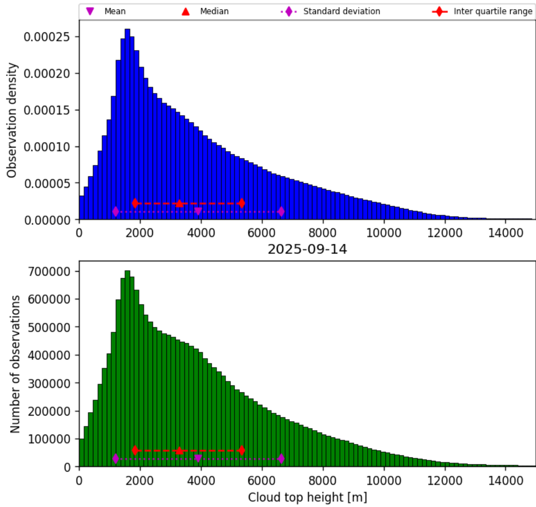
Figure 38: Histogram of “Cloud top height” for 2025-09-14 to 2025-09-15
