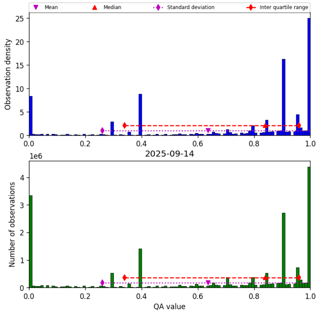
Figure 36: Histogram of “QA value” for 2025-09-14 to 2025-09-15
