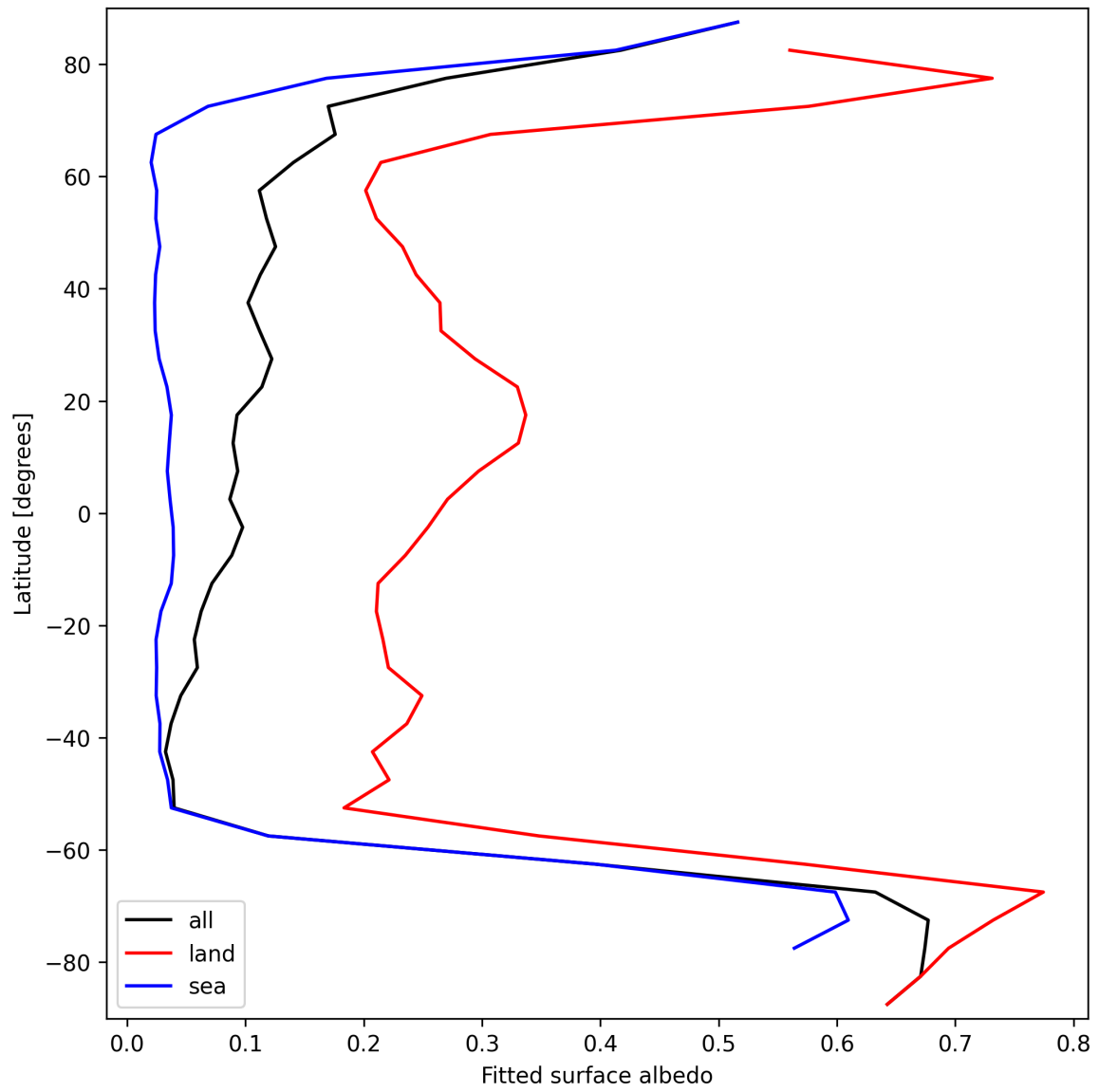
Figure 27: Zonal average of “Fitted surface albedo” for 2025-09-14 to 2025-09-15.
