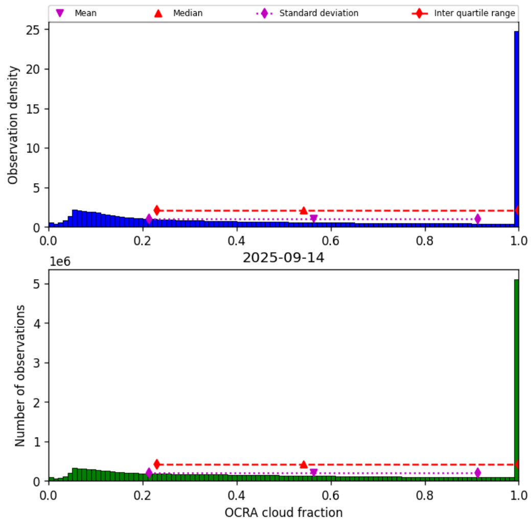
Figure 48: Histogram of “OCRA cloud fraction” for 2025-09-14 to 2025-09-15
