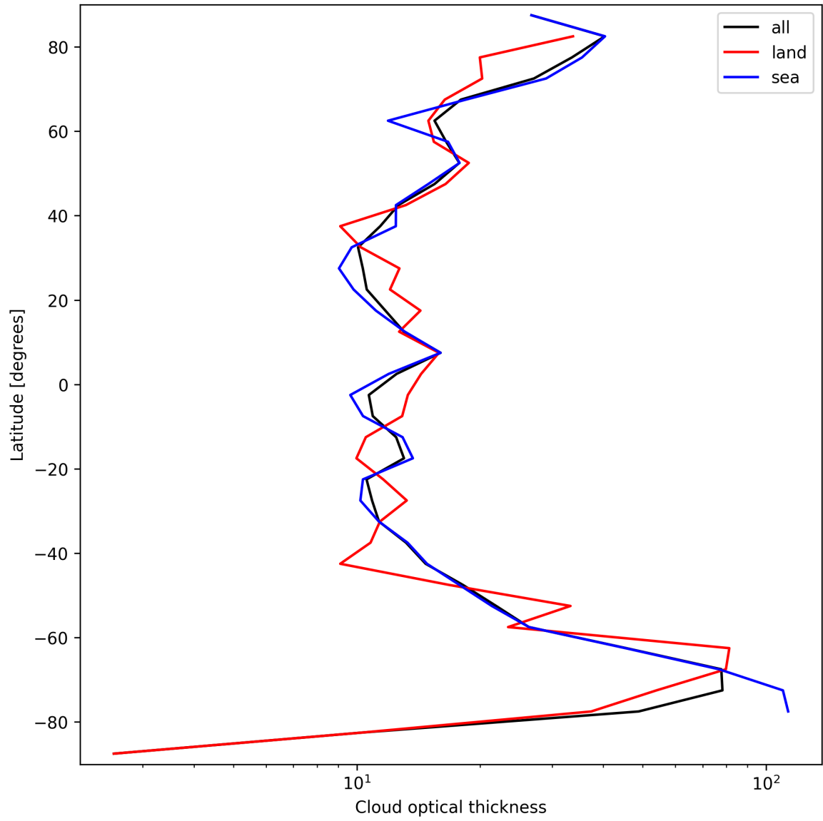
Figure 23: Zonal average of “Cloud optical thickness” for 2025-09-14 to 2025-09-15.
