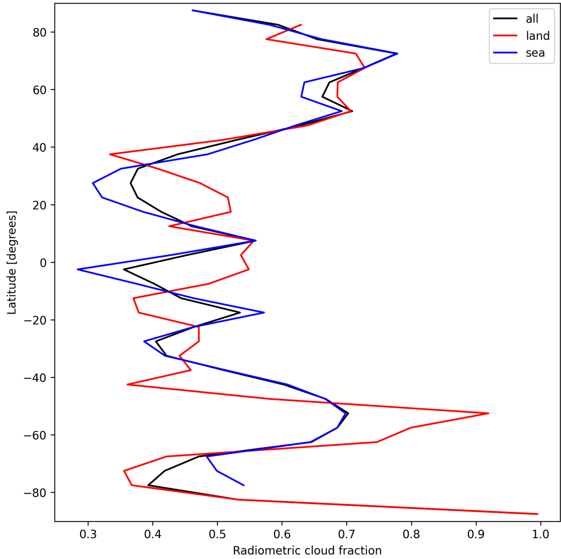
Figure 21: Zonal average of “Radiometric cloud fraction” for 2025-09-14 to 2025-09-15.
