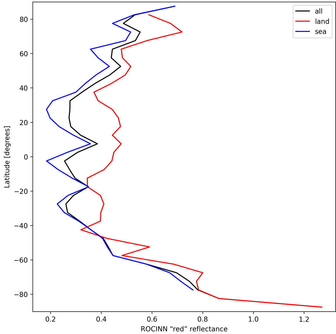
Figure 35: Zonal average of “ROCINN “red” reflectance” for 2025-09-14 to 2025-09-15.
