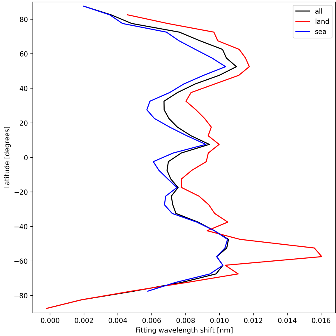
Figure 31: Zonal average of “Fitting wavelength shift” for 2025-09-14 to 2025-09-15.
