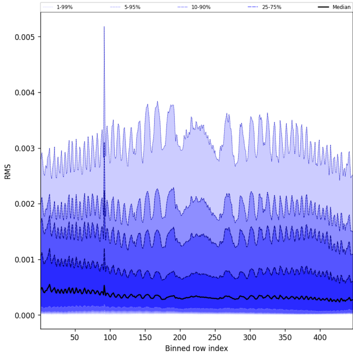
Figure 61: Along track statistics of “RMS” for 2025-09-14 to 2025-09-15
