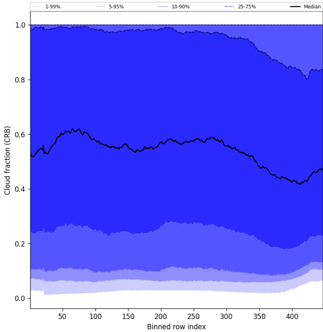
Figure 56: Along track statistics of “Cloud fraction (CRB)” for 2025-09-14 to 2025-09-15
