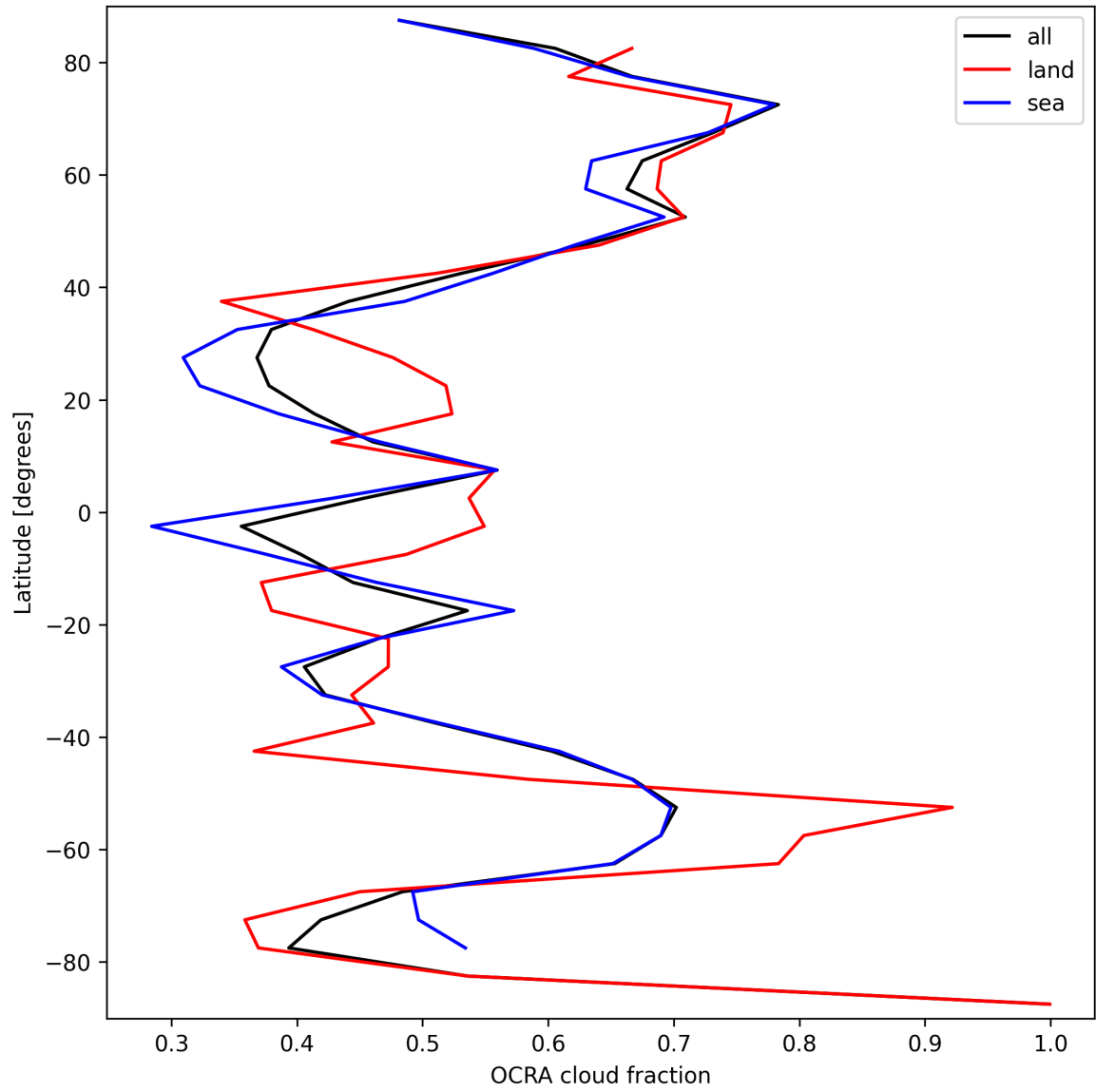
Figure 32: Zonal average of “OCRA cloud fraction” for 2025-09-14 to 2025-09-15.
