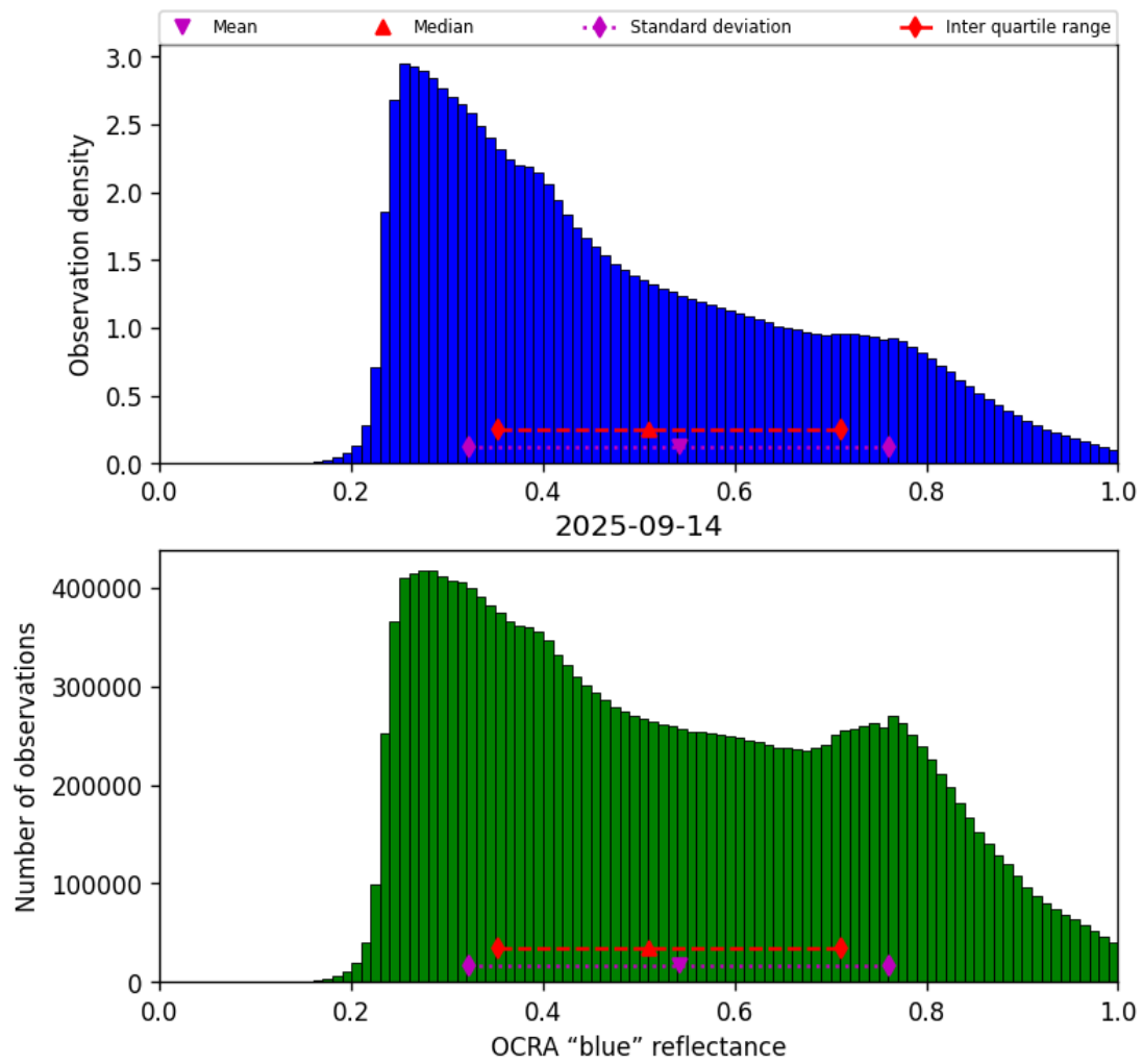
Figure 49: Histogram of “OCRA “blue” reflectance” for 2025-09-14 to 2025-09-15
