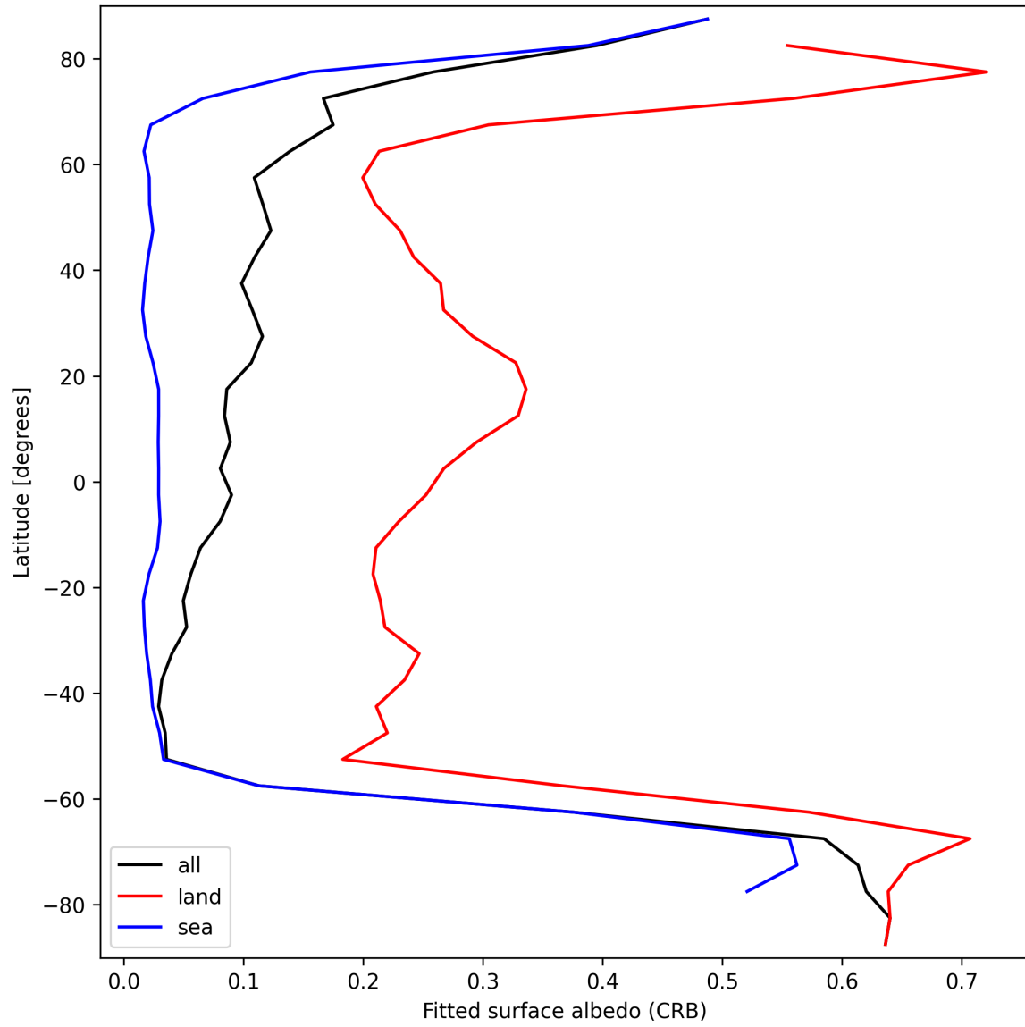
Figure 28: Zonal average of “Fitted surface albedo (CRB)” for 2025-09-14 to 2025-09-15.
