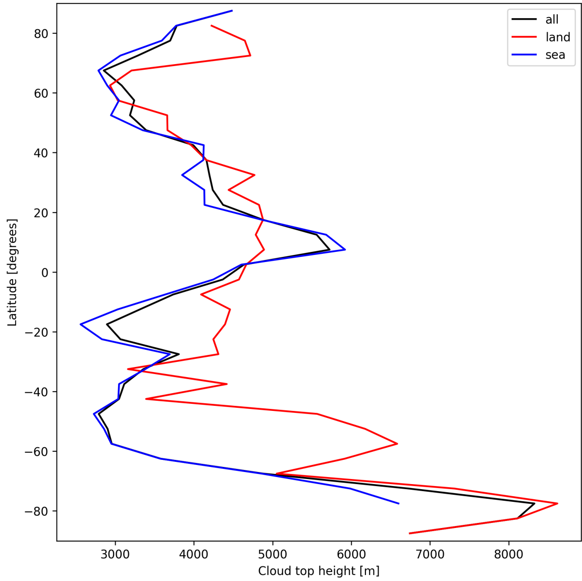
Figure 22: Zonal average of “Cloud top height” for 2025-09-14 to 2025-09-15.
