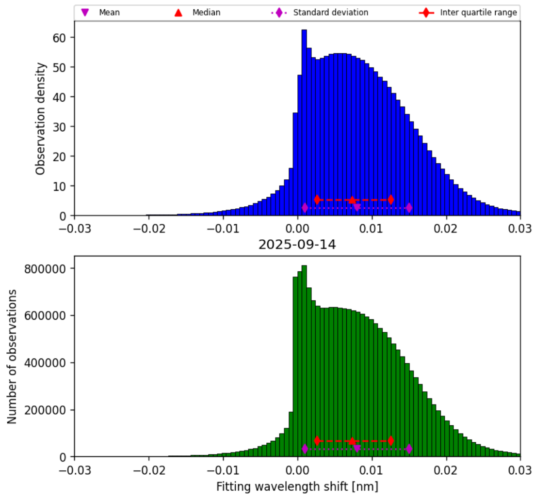
Figure 47: Histogram of “Fitting wavelength shift” for 2025-09-14 to 2025-09-15
