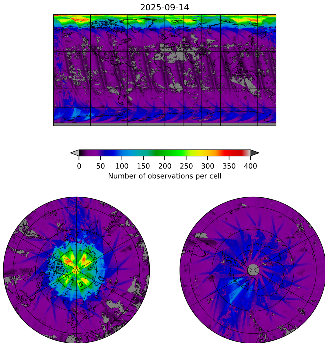
Figure 19: Map of the number of observations for 2025-09-14 to 2025-09-15
