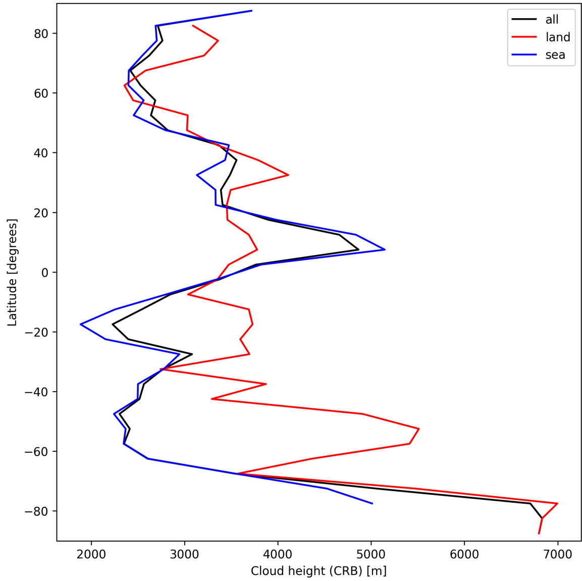
Figure 25: Zonal average of “Cloud height (CRB)” for 2025-09-14 to 2025-09-15.
