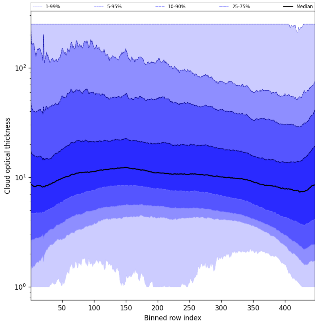
Figure 55: Along track statistics of “Cloud optical thickness” for 2025-09-14 to 2025-09-15
