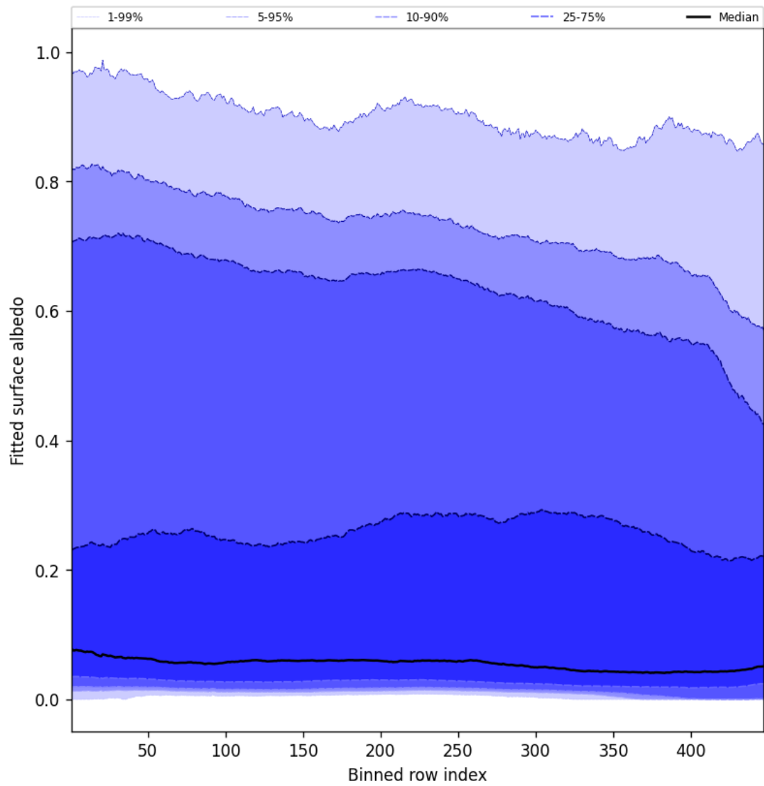
Figure 59: Along track statistics of “Fitted surface albedo” for 2025-09-14 to 2025-09-15
