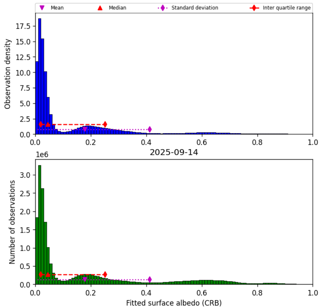
Figure 44: Histogram of “Fitted surface albedo (CRB)” for 2025-09-14 to 2025-09-15
