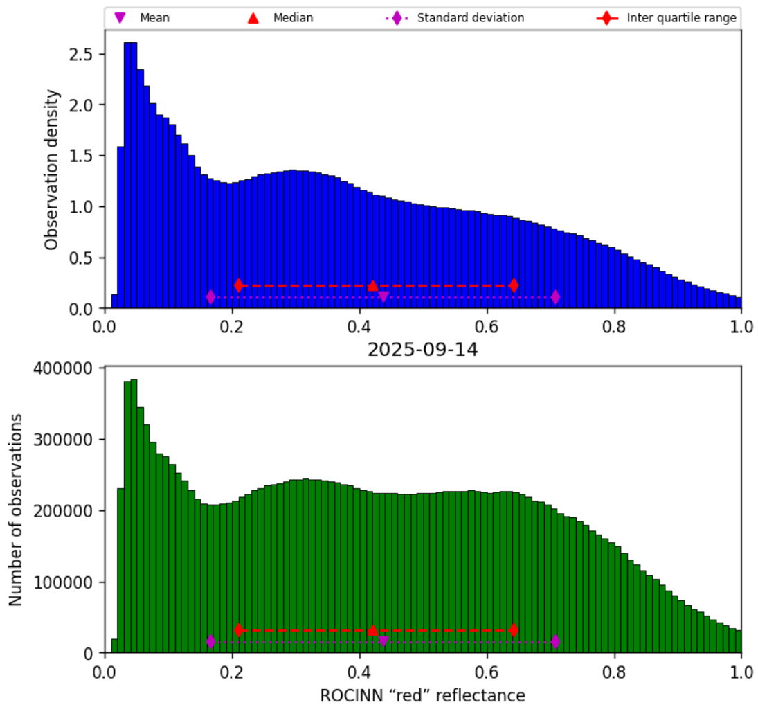
Figure 51: Histogram of “ROCINN “red” reflectance” for 2025-09-14 to 2025-09-15
