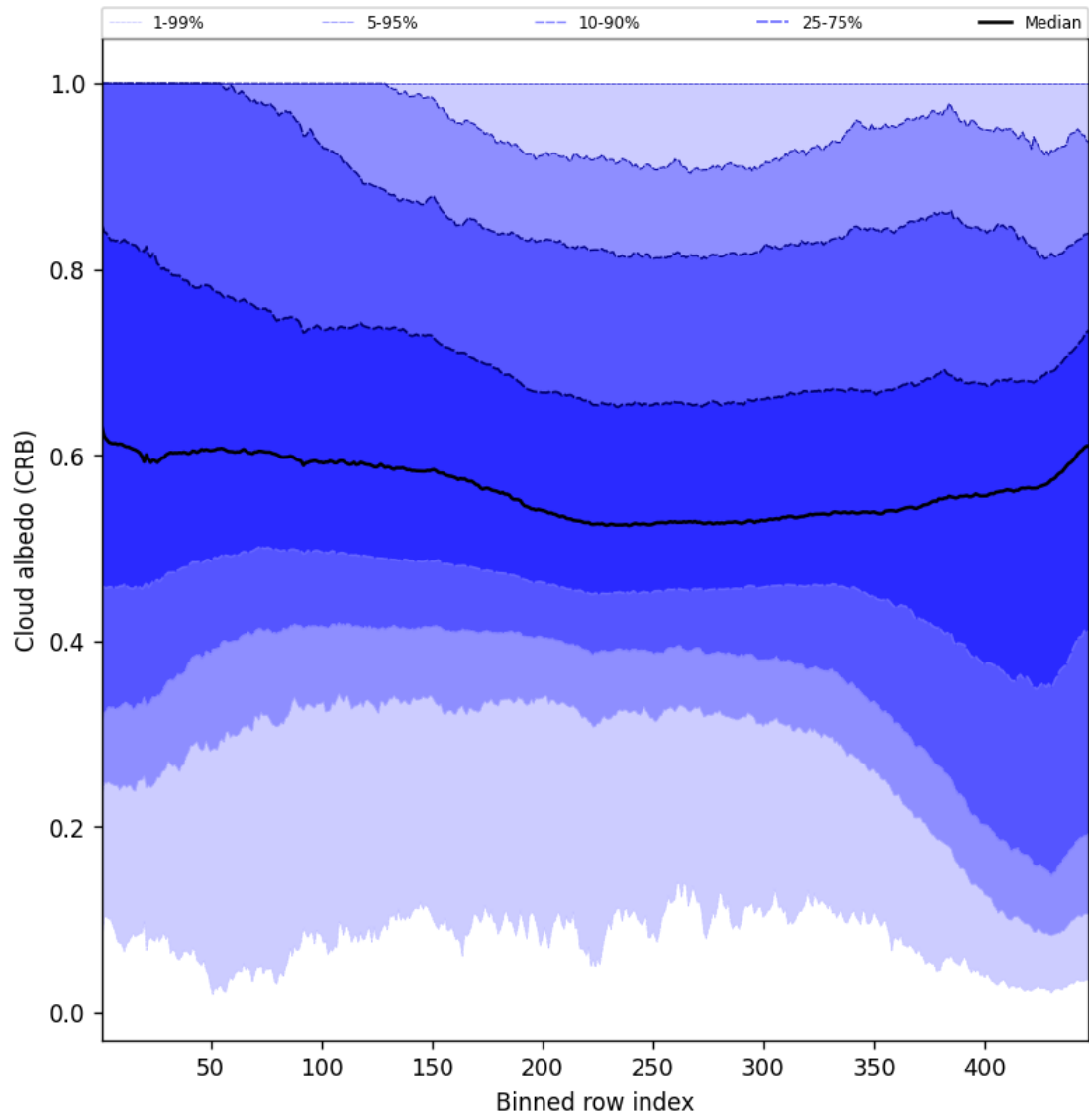
Figure 58: Along track statistics of “Cloud albedo (CRB)” for 2025-09-14 to 2025-09-15
