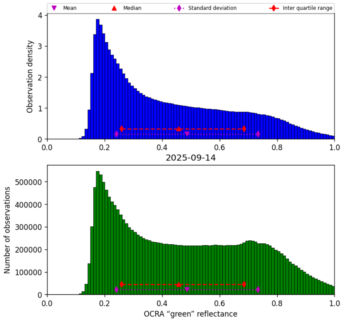
Figure 50: Histogram of “OCRA “green” reflectance” for 2025-09-14 to 2025-09-15
