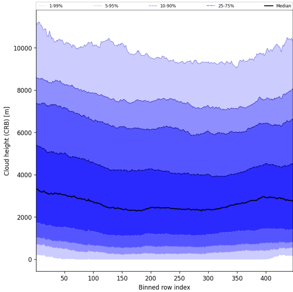
Figure 57: Along track statistics of “Cloud height (CRB)” for 2025-09-14 to 2025-09-15
