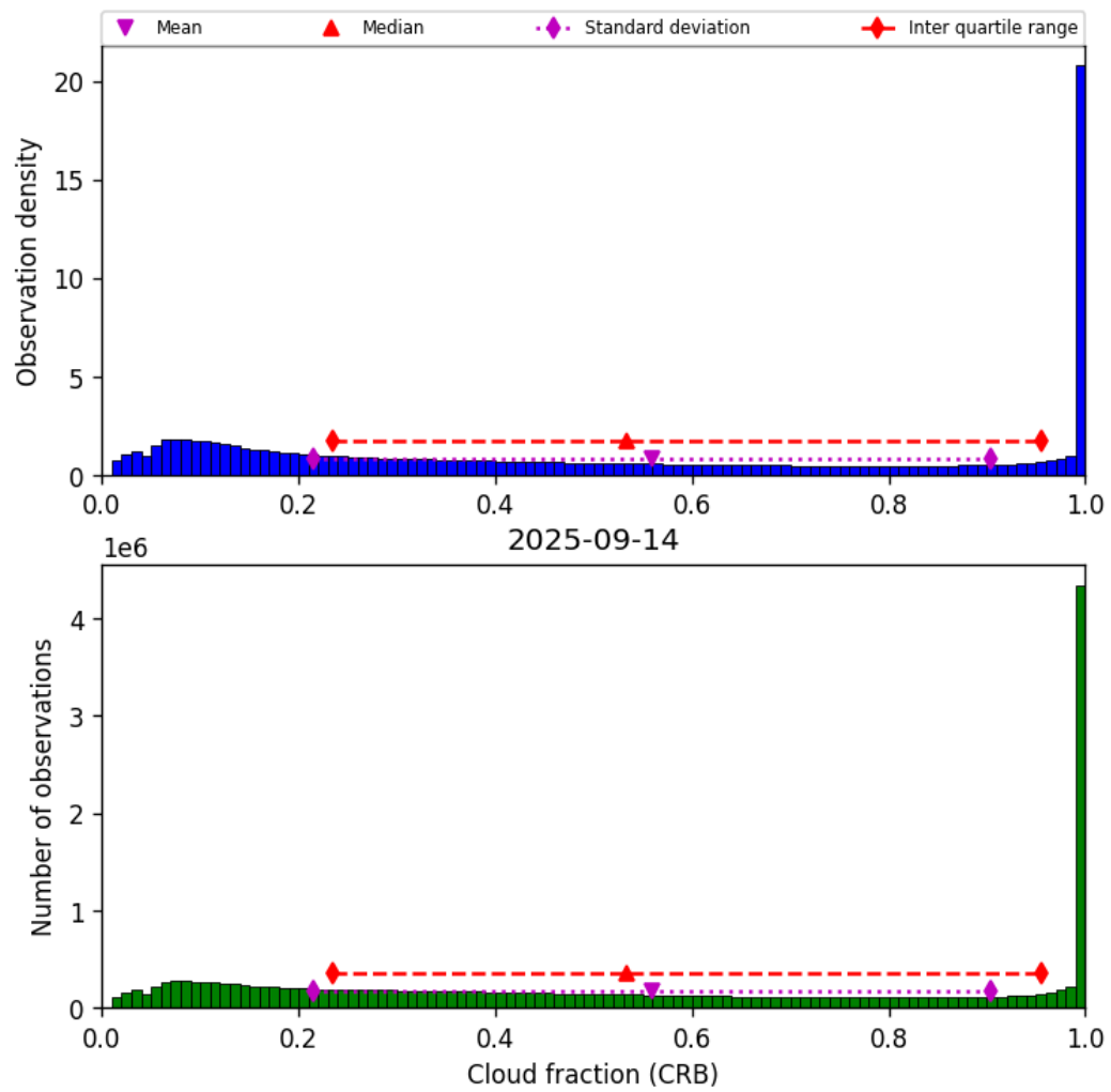
Figure 40: Histogram of “Cloud fraction (CRB)” for 2025-09-14 to 2025-09-15
