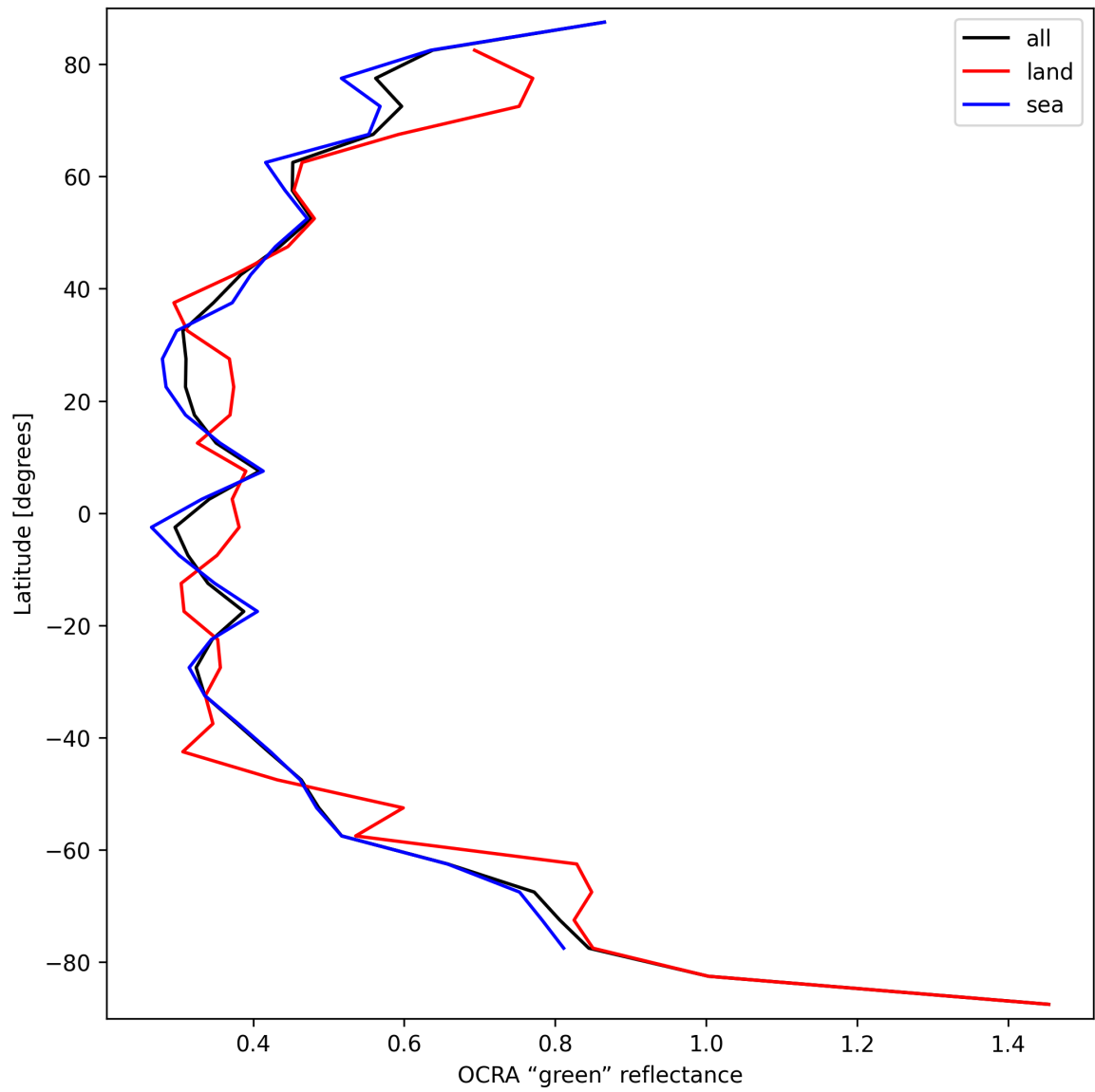
Figure 34: Zonal average of “OCRA “green” reflectance” for 2025-09-14 to 2025-09-15.
