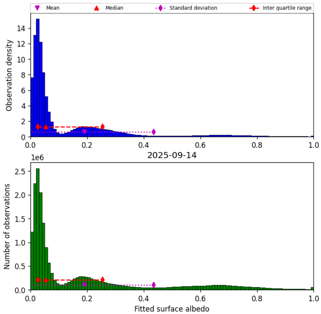
Figure 43: Histogram of “Fitted surface albedo” for 2025-09-14 to 2025-09-15
