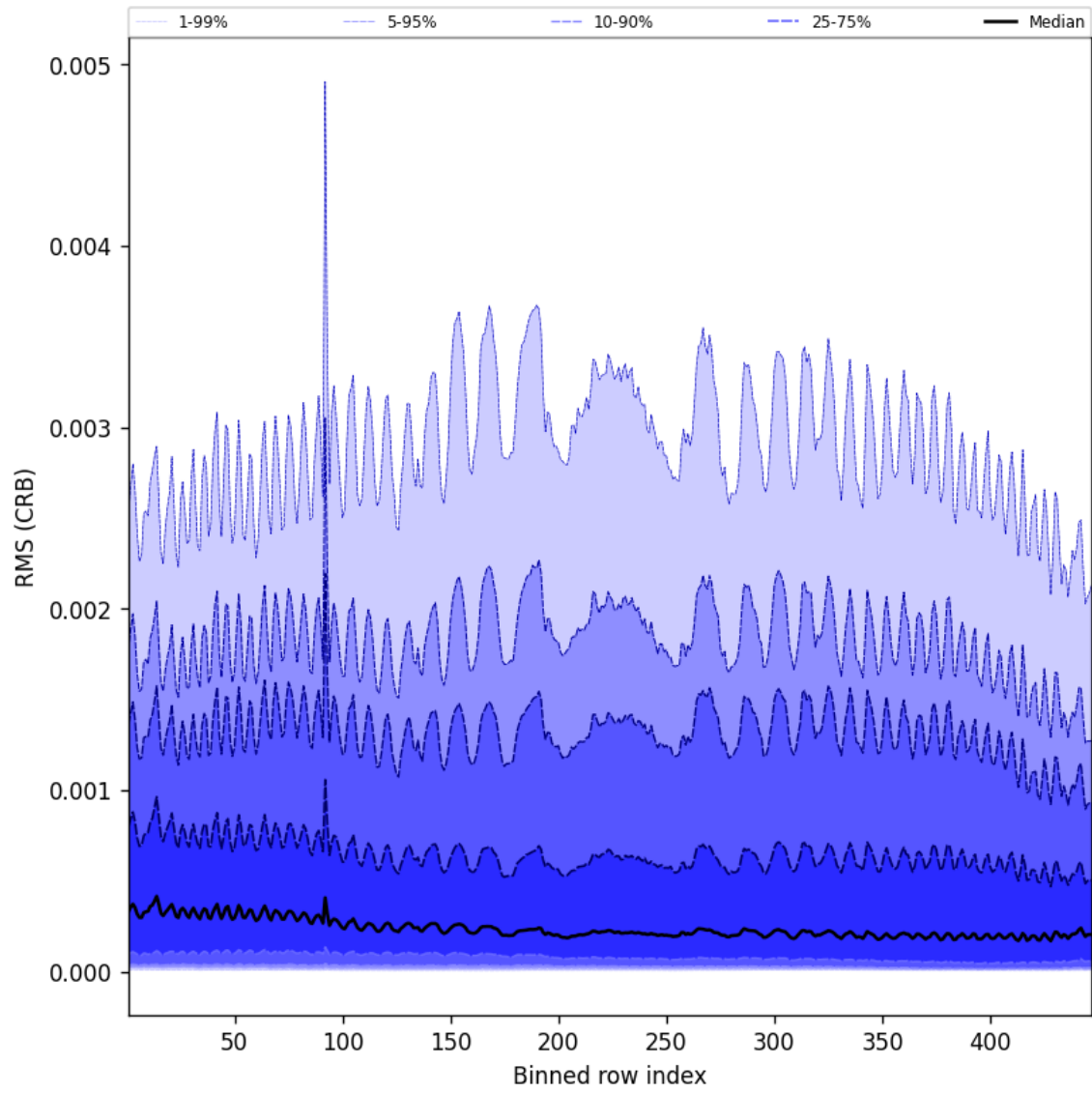
Figure 62: Along track statistics of “RMS (CRB)” for 2025-09-14 to 2025-09-15
