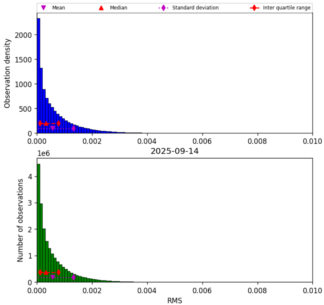
Figure 45: Histogram of “RMS” for 2025-09-14 to 2025-09-15
