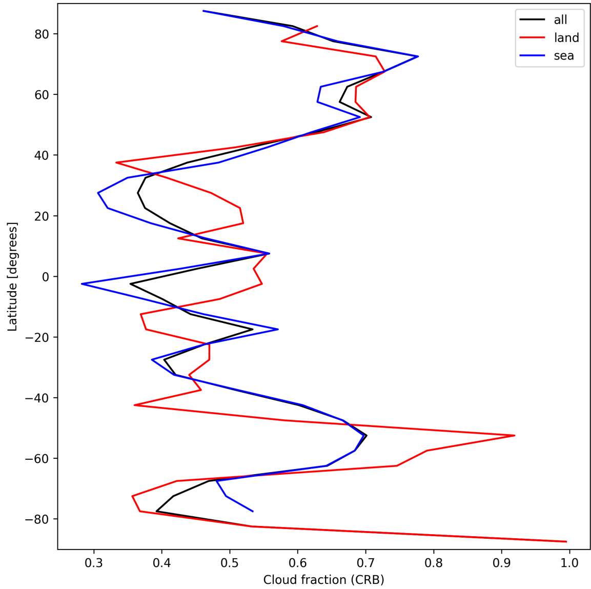
Figure 24: Zonal average of “Cloud fraction (CRB)” for 2025-09-14 to 2025-09-15.
