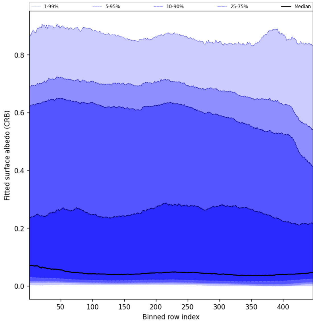
Figure 60: Along track statistics of “Fitted surface albedo (CRB)” for 2025-09-14 to 2025-09-15
