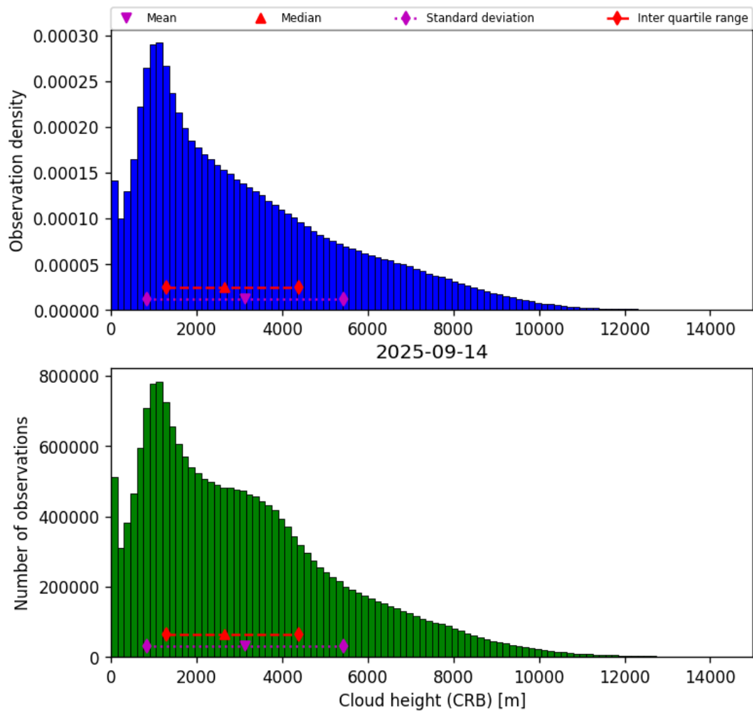
Figure 41: Histogram of “Cloud height (CRB)” for 2025-09-14 to 2025-09-15
