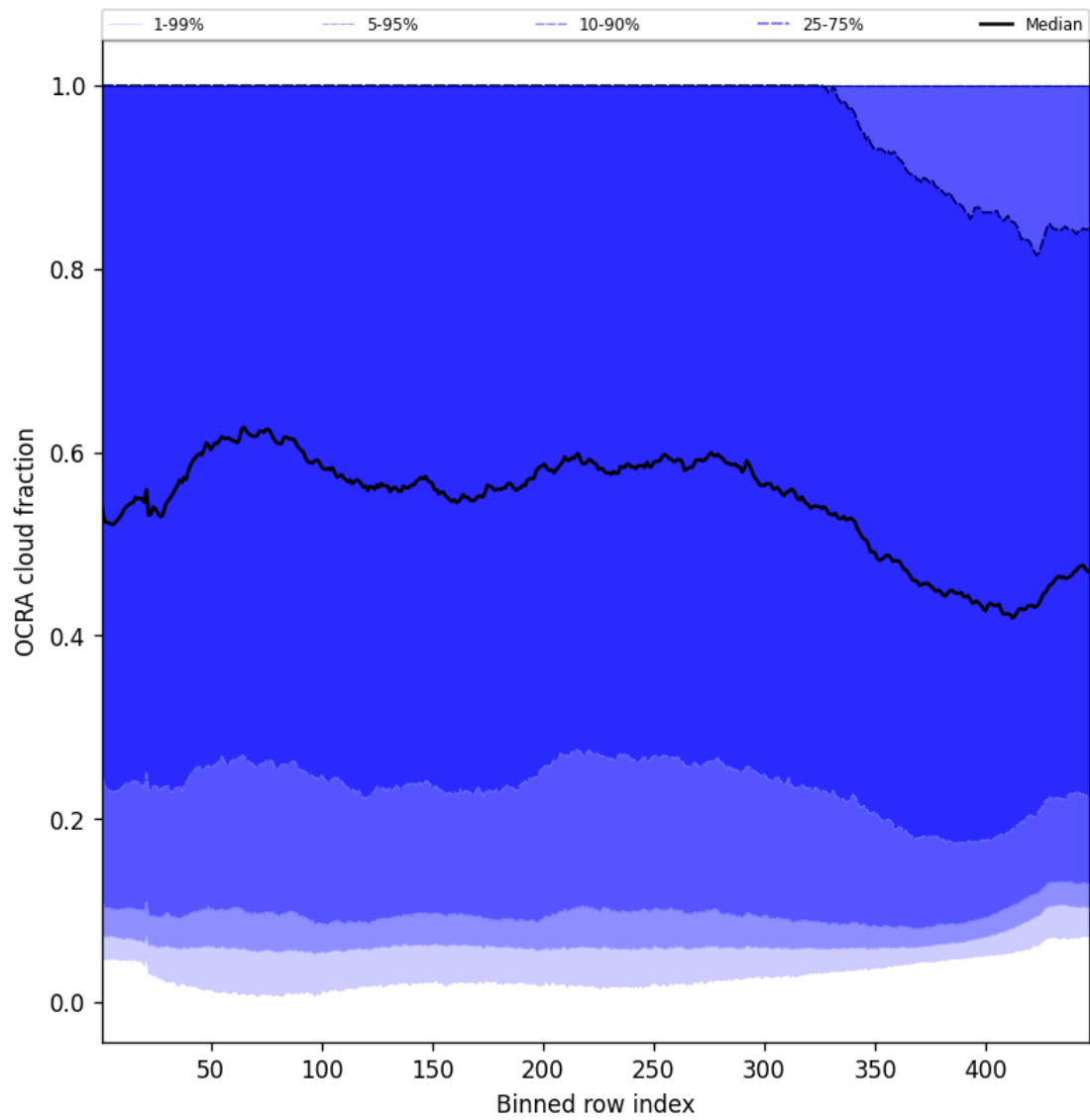
Figure 64: Along track statistics of “OCRA cloud fraction” for 2025-09-14 to 2025-09-15
