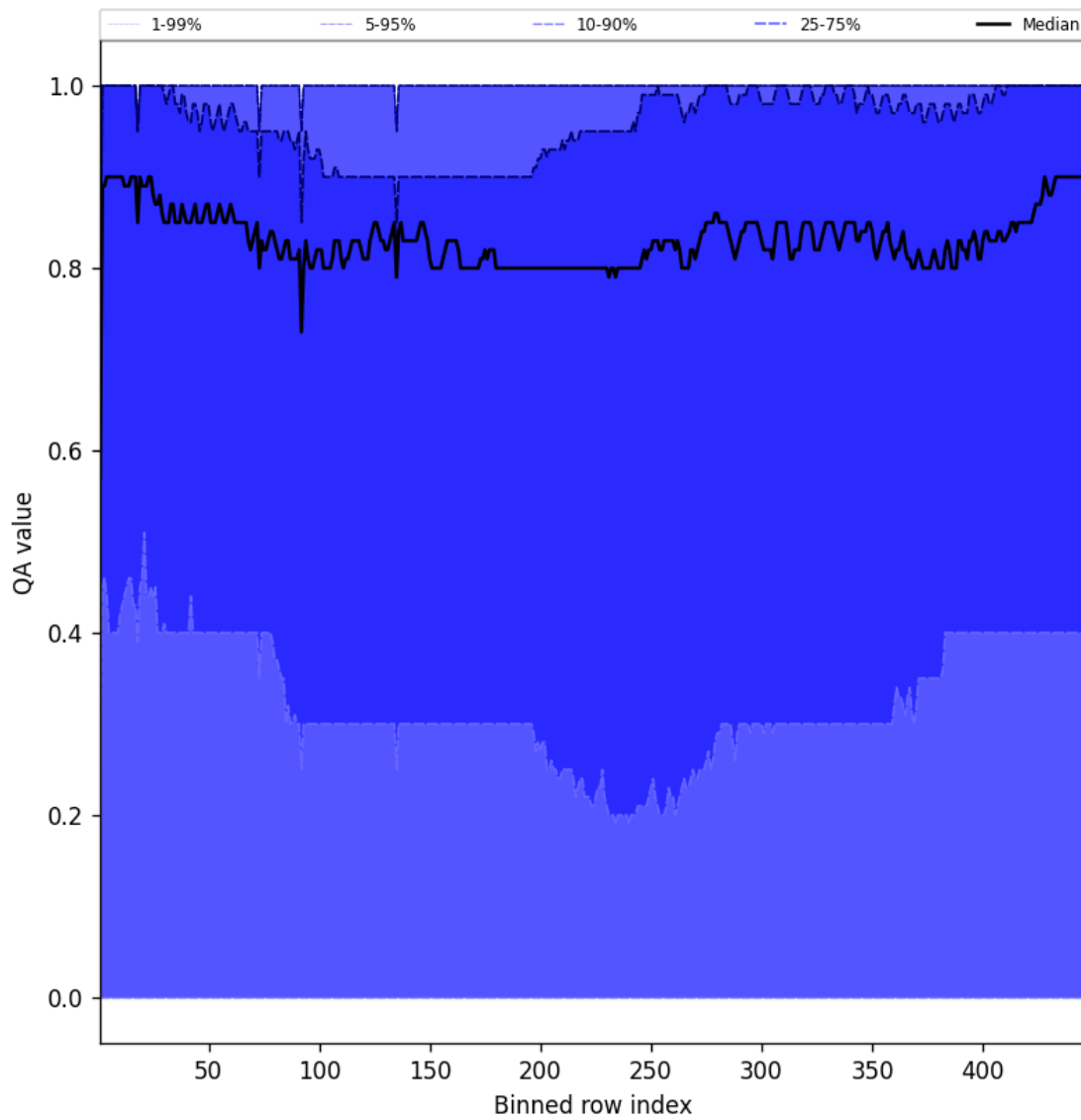
Figure 52: Along track statistics of “QA value” for 2025-09-14 to 2025-09-15
