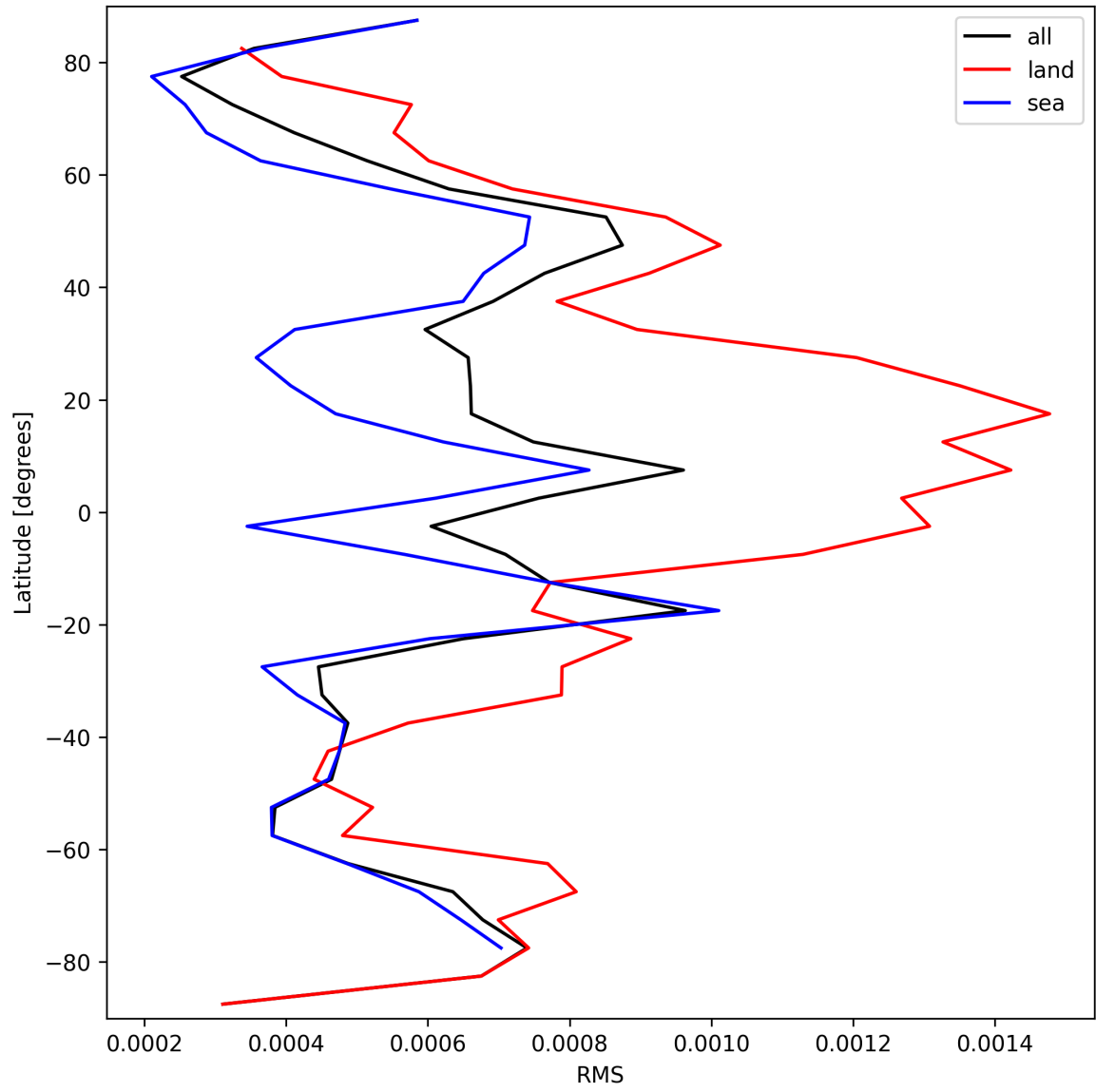
Figure 29: Zonal average of “RMS” for 2025-09-14 to 2025-09-15.
