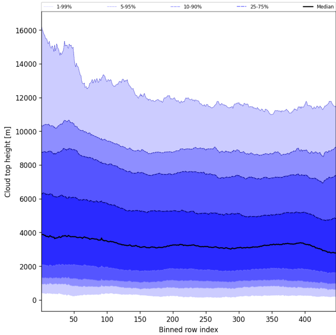
Figure 54: Along track statistics of “Cloud top height” for 2025-09-14 to 2025-09-15
