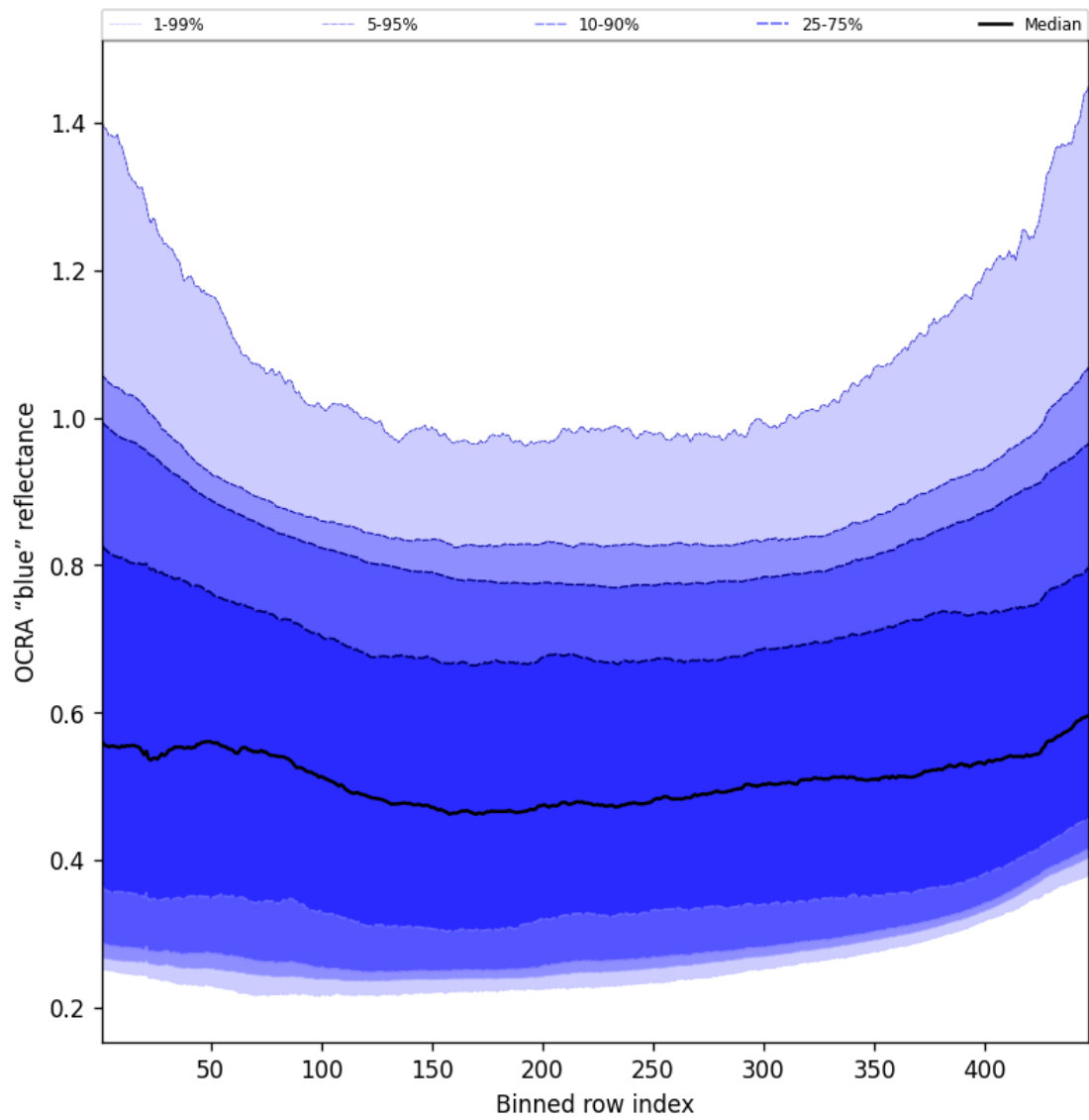
Figure 65: Along track statistics of “OCRA “blue” reflectance” for 2025-09-14 to 2025-09-15
