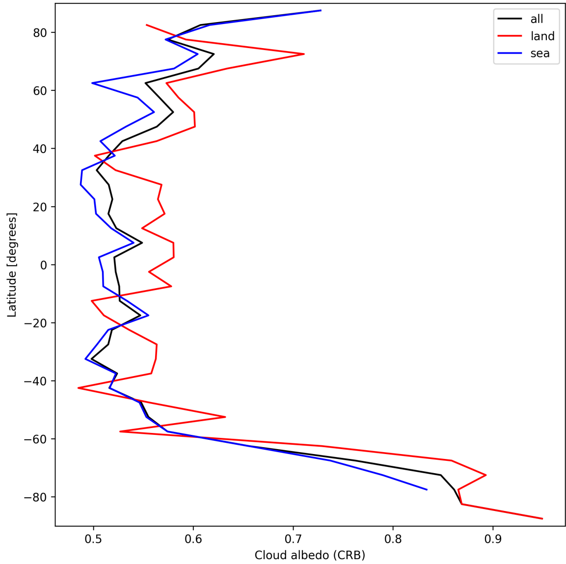
Figure 26: Zonal average of “Cloud albedo (CRB)” for 2025-09-14 to 2025-09-15.
