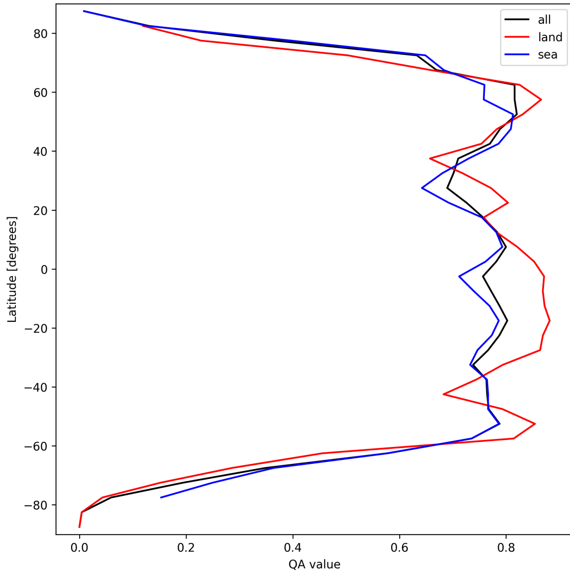
Figure 20: Zonal average of “QA value” for 2025-09-14 to 2025-09-15.
