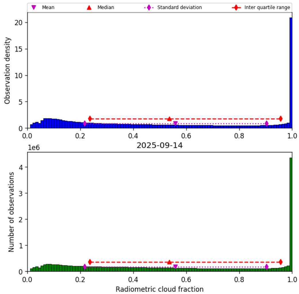
Figure 37: Histogram of “Radiometric cloud fraction” for 2025-09-14 to 2025-09-15
