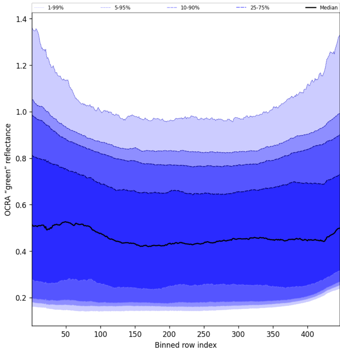
Figure 66: Along track statistics of “OCRA “green” reflectance” for 2025-09-14 to 2025-09-15
