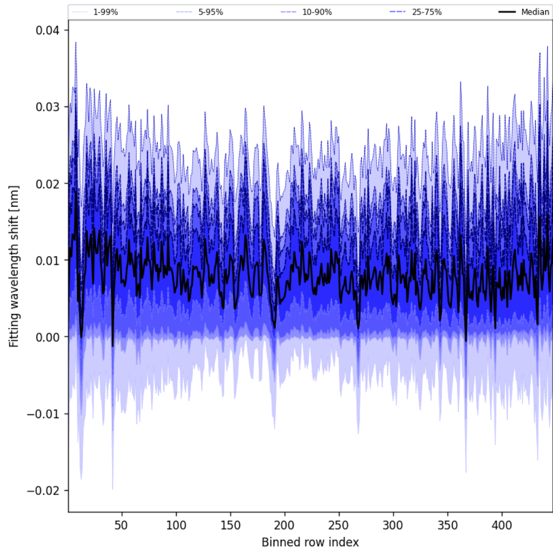
Figure 63: Along track statistics of “Fitting wavelength shift” for 2025-09-14 to 2025-09-15
