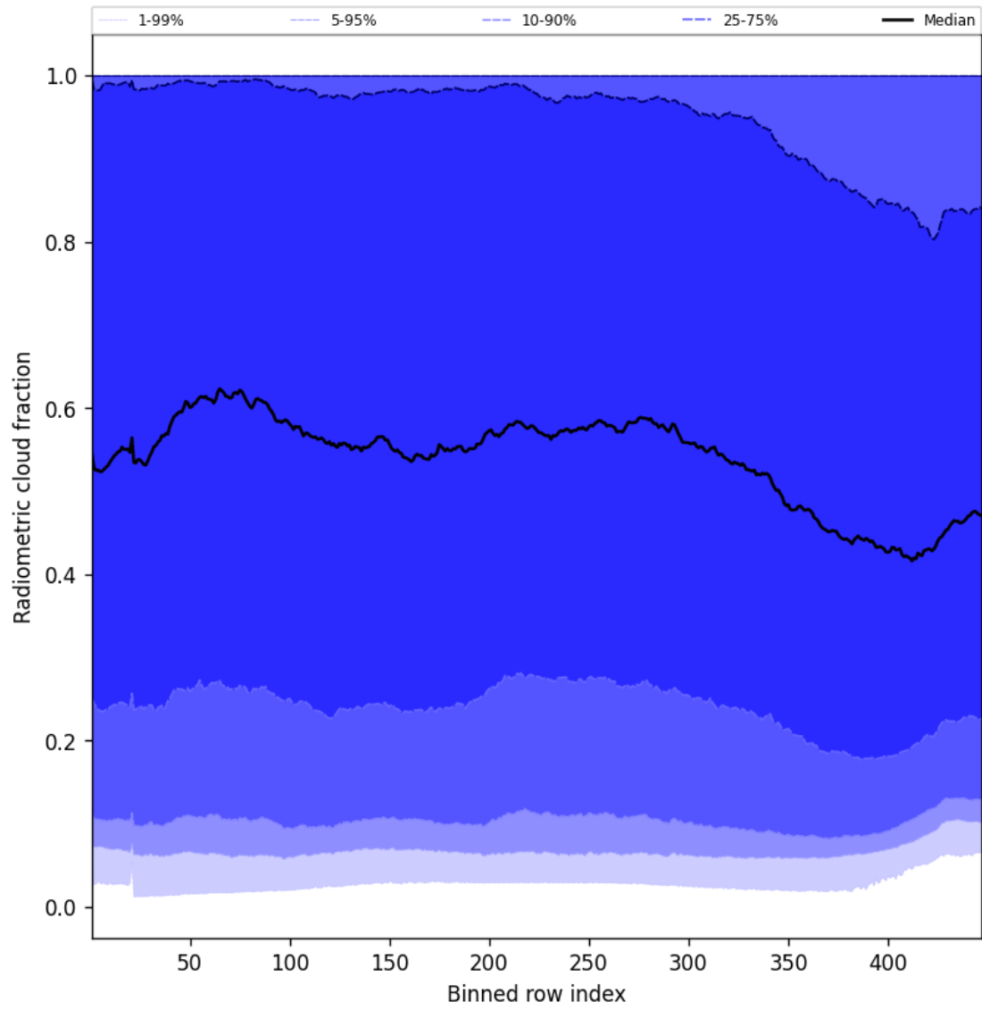
Figure 53: Along track statistics of “Radiometric cloud fraction” for 2025-09-14 to 2025-09-15
