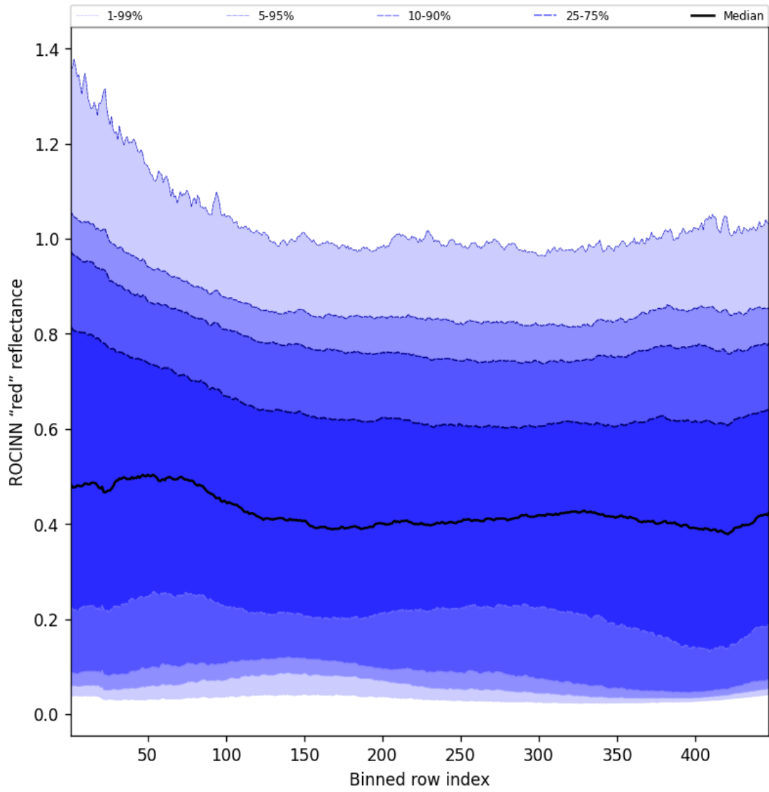
Figure 67: Along track statistics of “ROCINN “red” reflectance” for 2025-09-14 to 2025-09-15
