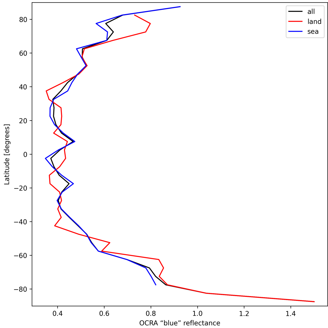
Figure 33: Zonal average of “OCRA “blue” reflectance” for 2025-09-14 to 2025-09-15.
