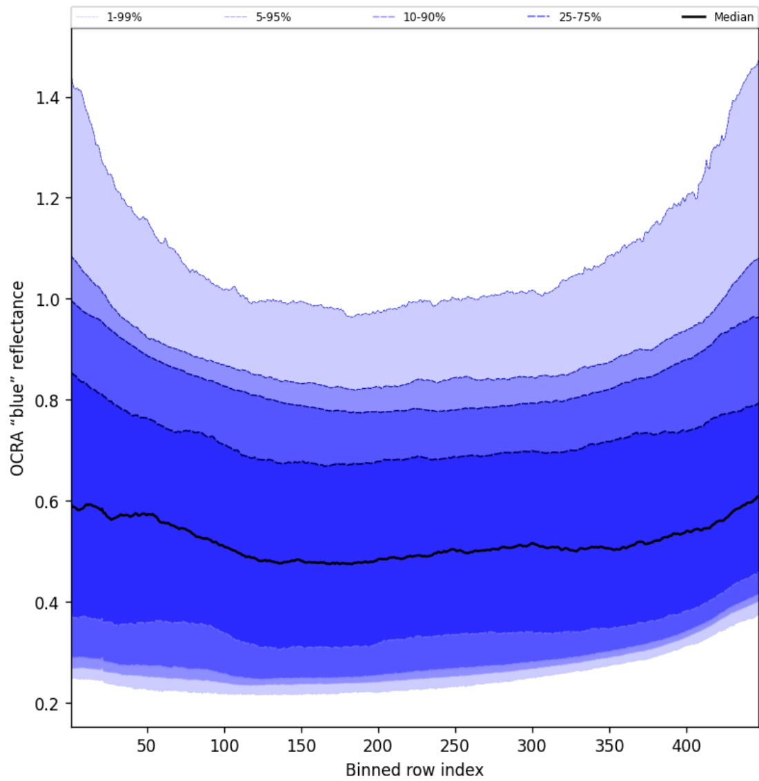
Figure 65: Along track statistics of "OCRA "blue" reflectance" for 2025-09-15 to 2025-09-16
