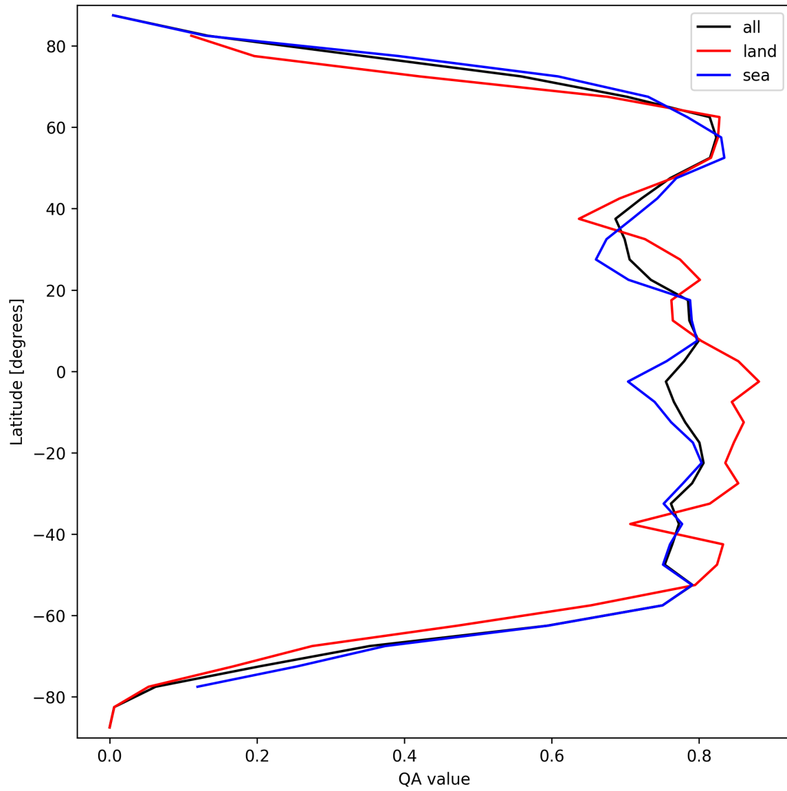
Figure 20: Zonal average of “QA value” for 2025-09-15 to 2025-09-16.
