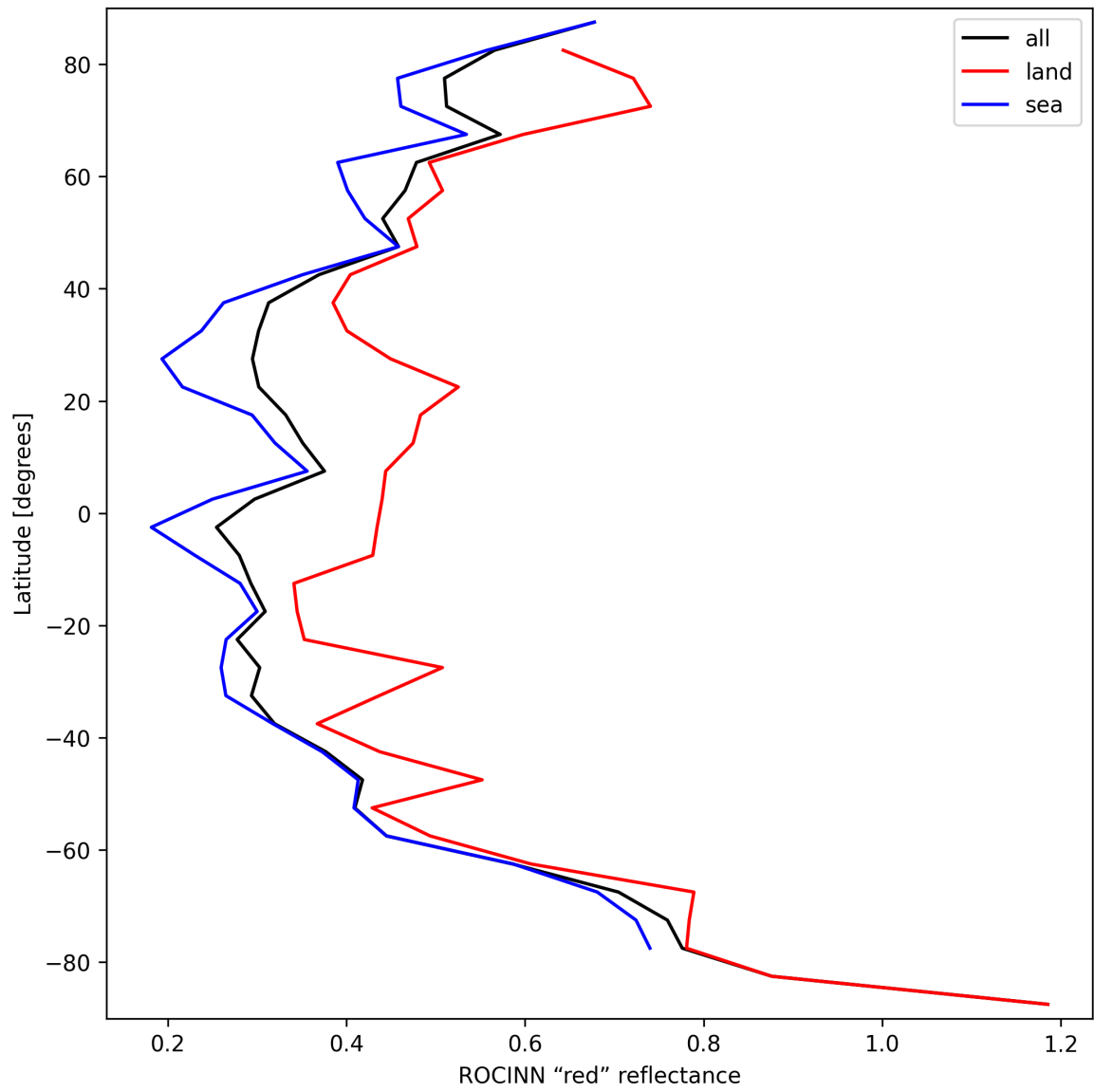
Figure 35: Zonal average of “ROCINN “red” reflectance” for 2025-09-15 to 2025-09-16.
