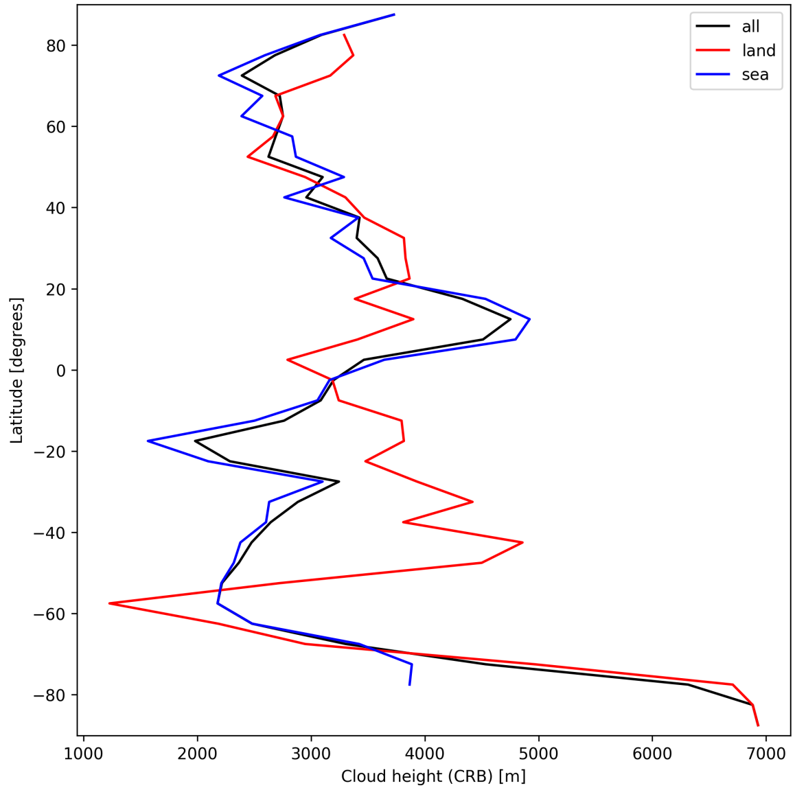
Figure 25: Zonal average of “Cloud height (CRB)” for 2025-09-15 to 2025-09-16.
