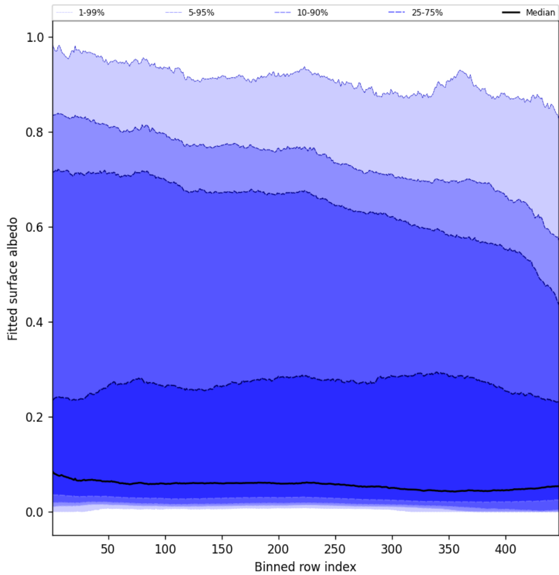
Figure 59: Along track statistics of “Fitted surface albedo” for 2025-09-15 to 2025-09-16
