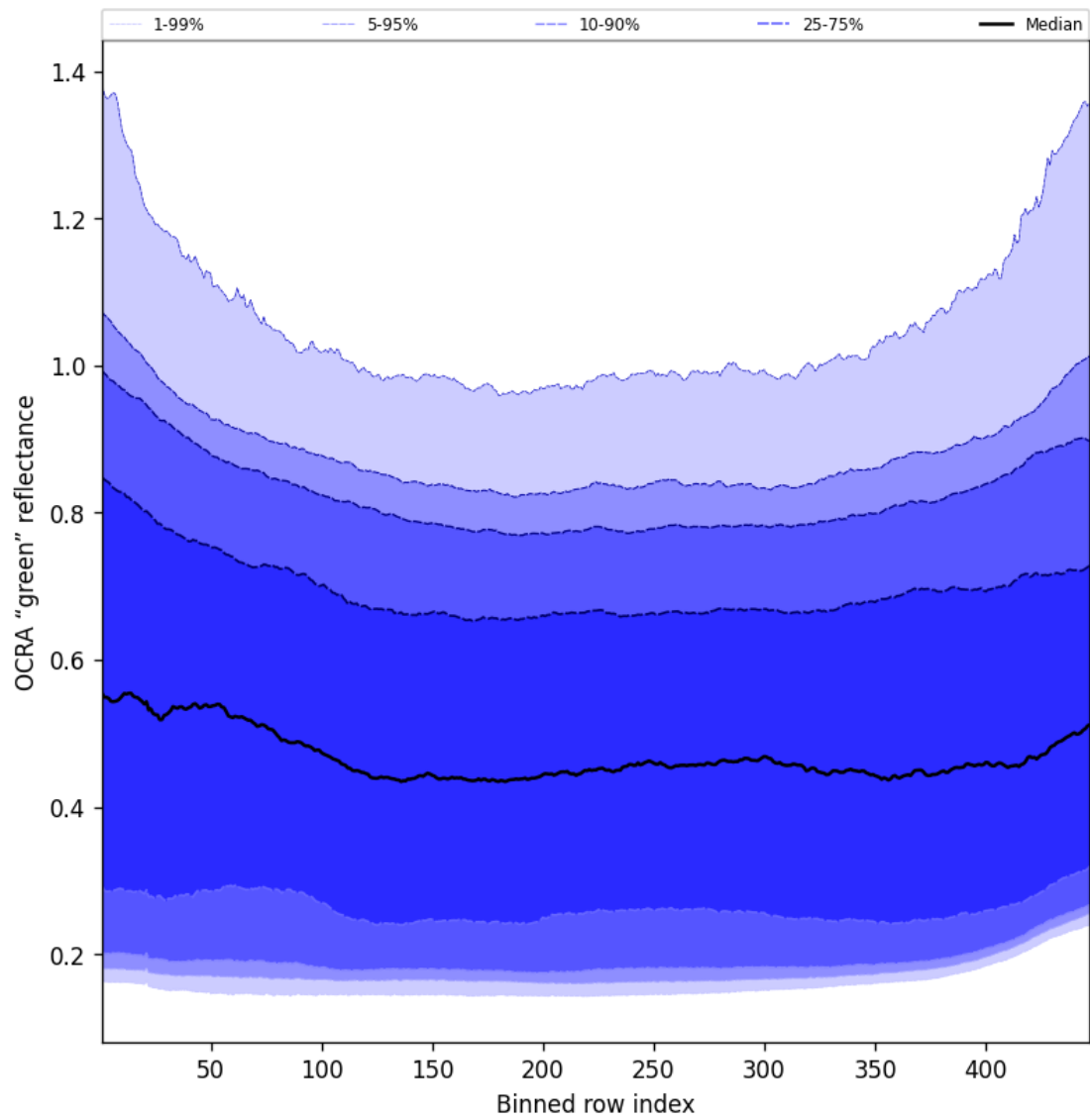
Figure 66: Along track statistics of “OCRA “green” reflectance” for 2025-09-15 to 2025-09-16
