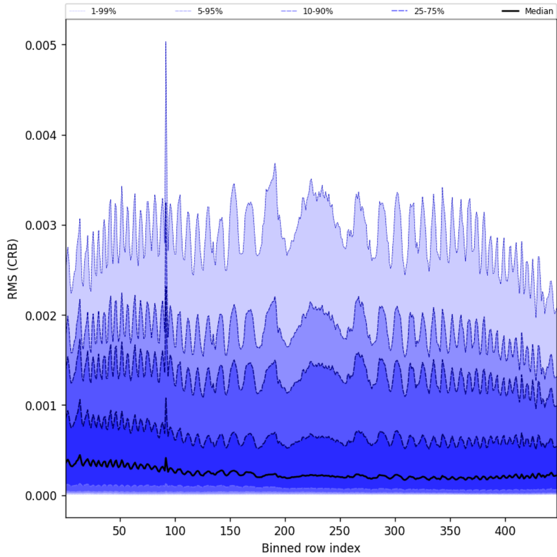
Figure 62: Along track statistics of “RMS (CRB)” for 2025-09-15 to 2025-09-16
