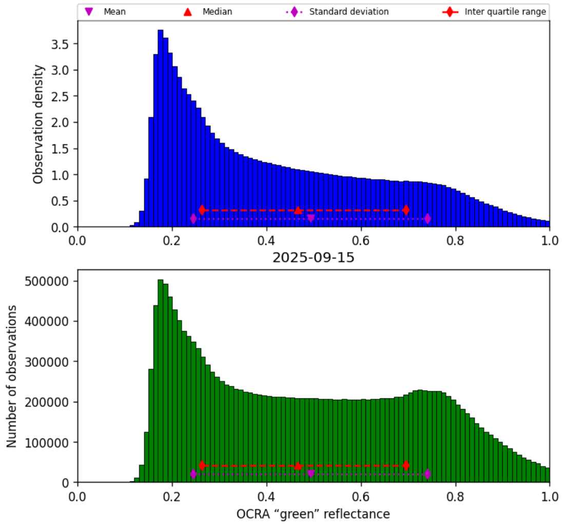
Figure 50: Histogram of “OCRA “green” reflectance” for 2025-09-15 to 2025-09-16
