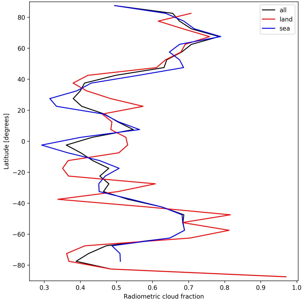
Figure 21: Zonal average of “Radiometric cloud fraction” for 2025-09-15 to 2025-09-16.
