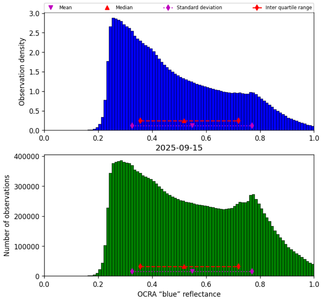
Figure 49: Histogram of “OCRA “blue” reflectance” for 2025-09-15 to 2025-09-16
