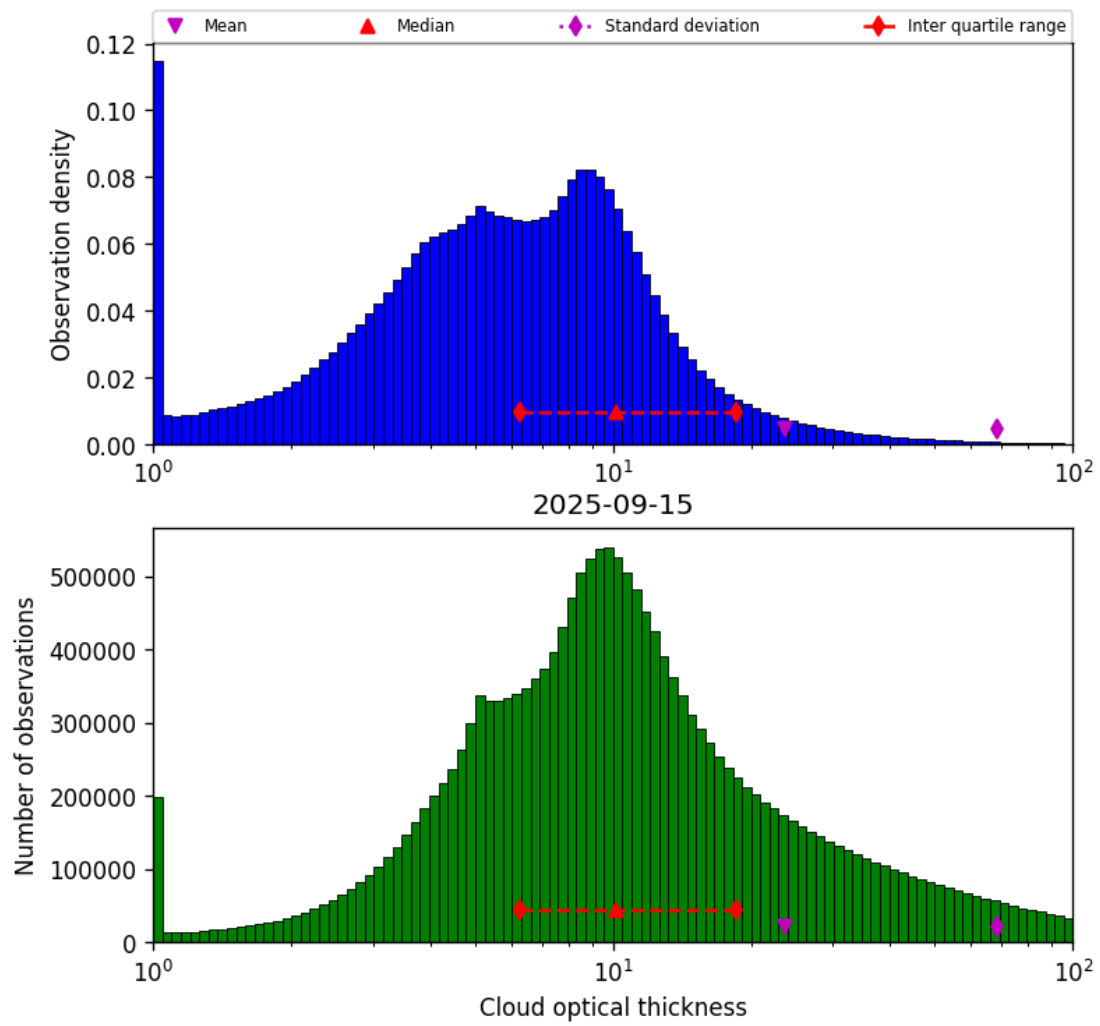
Figure 39: Histogram of “Cloud optical thickness” for 2025-09-15 to 2025-09-16
