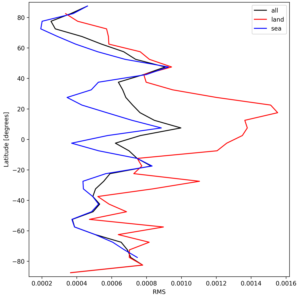
Figure 29: Zonal average of “RMS” for 2025-09-15 to 2025-09-16.
