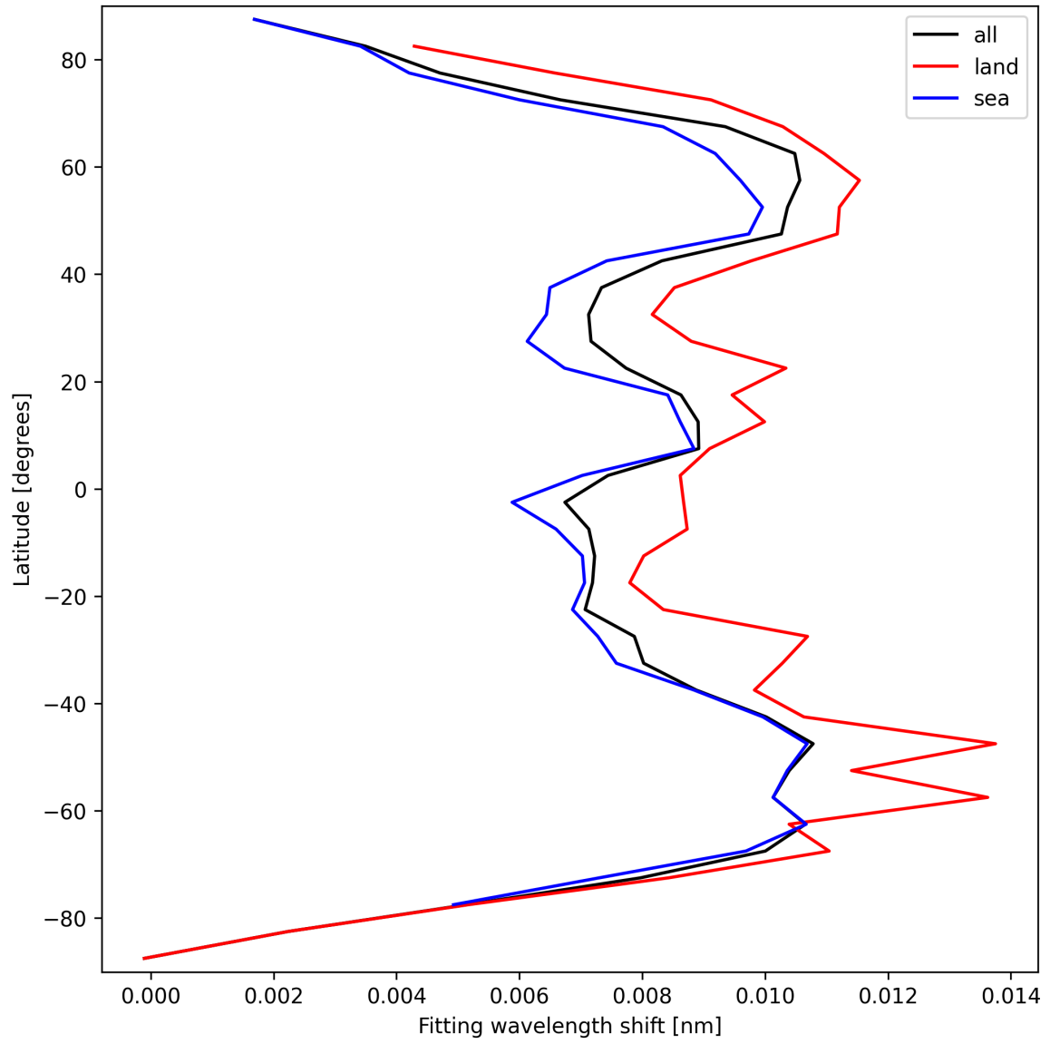
Figure 31: Zonal average of “Fitting wavelength shift” for 2025-09-15 to 2025-09-16.
