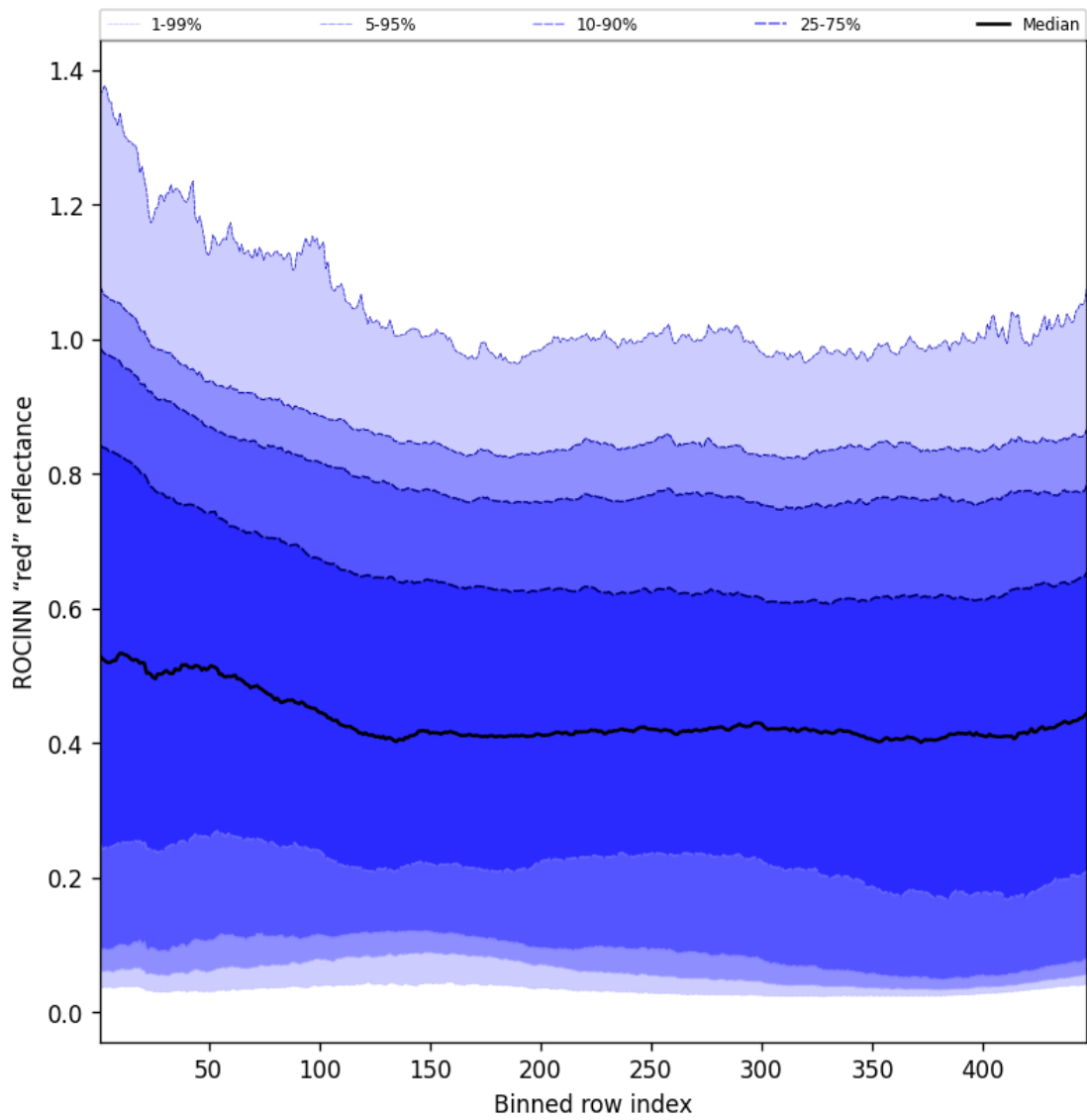
Figure 67: Along track statistics of “ROCINN “red” reflectance” for 2025-09-15 to 2025-09-16
