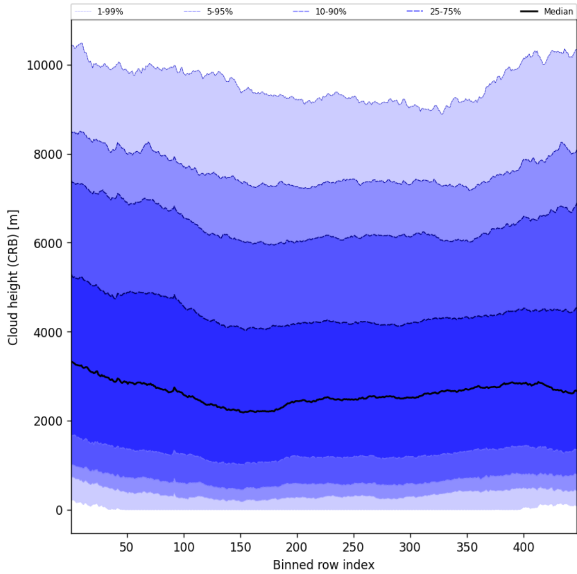
Figure 57: Along track statistics of “Cloud height (CRB)” for 2025-09-15 to 2025-09-16
