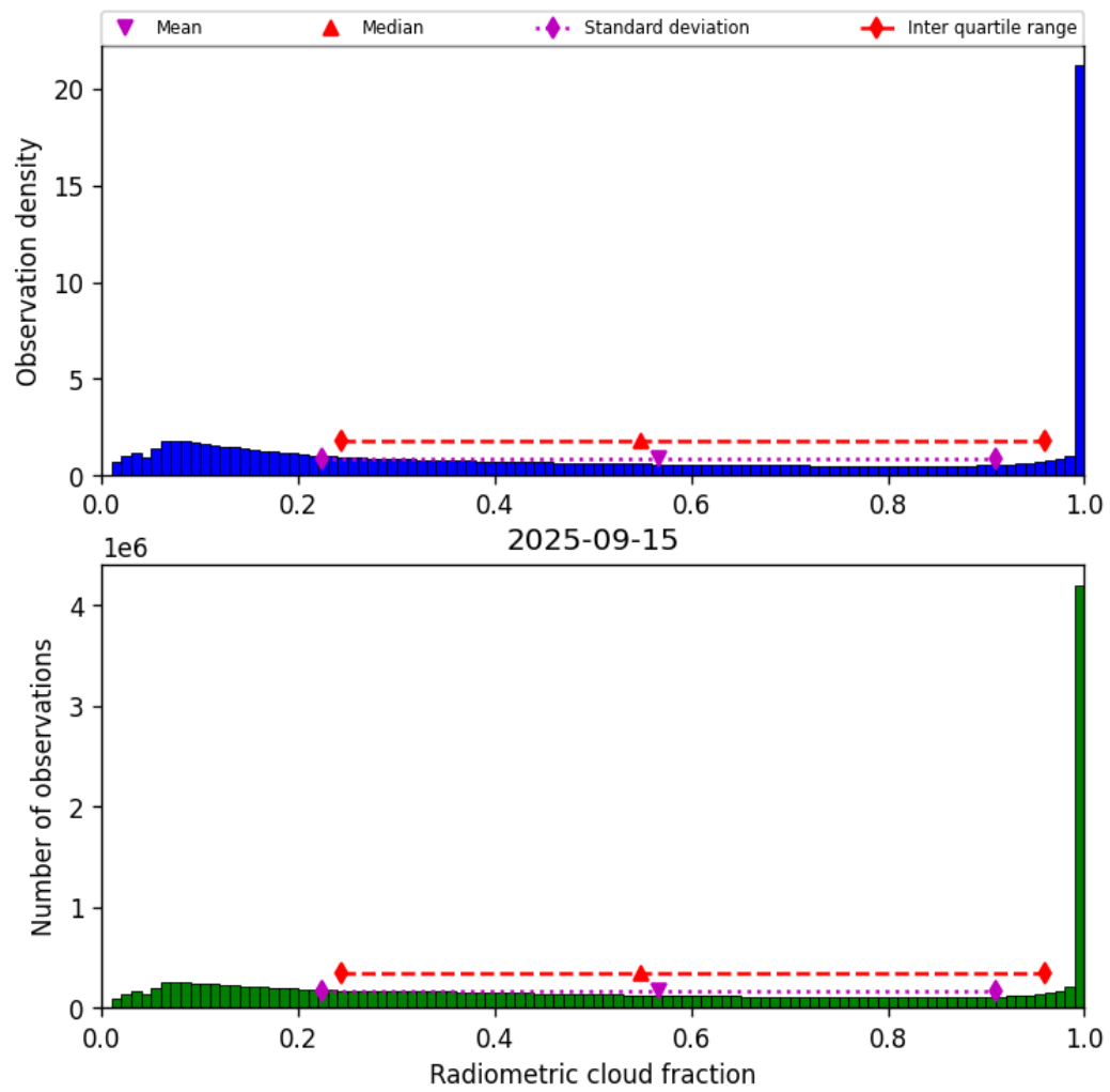
Figure 37: Histogram of “Radiometric cloud fraction” for 2025-09-15 to 2025-09-16
