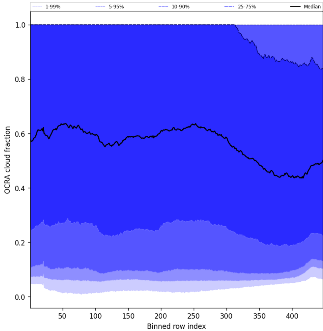
Figure 64: Along track statistics of “OCRA cloud fraction” for 2025-09-15 to 2025-09-16
