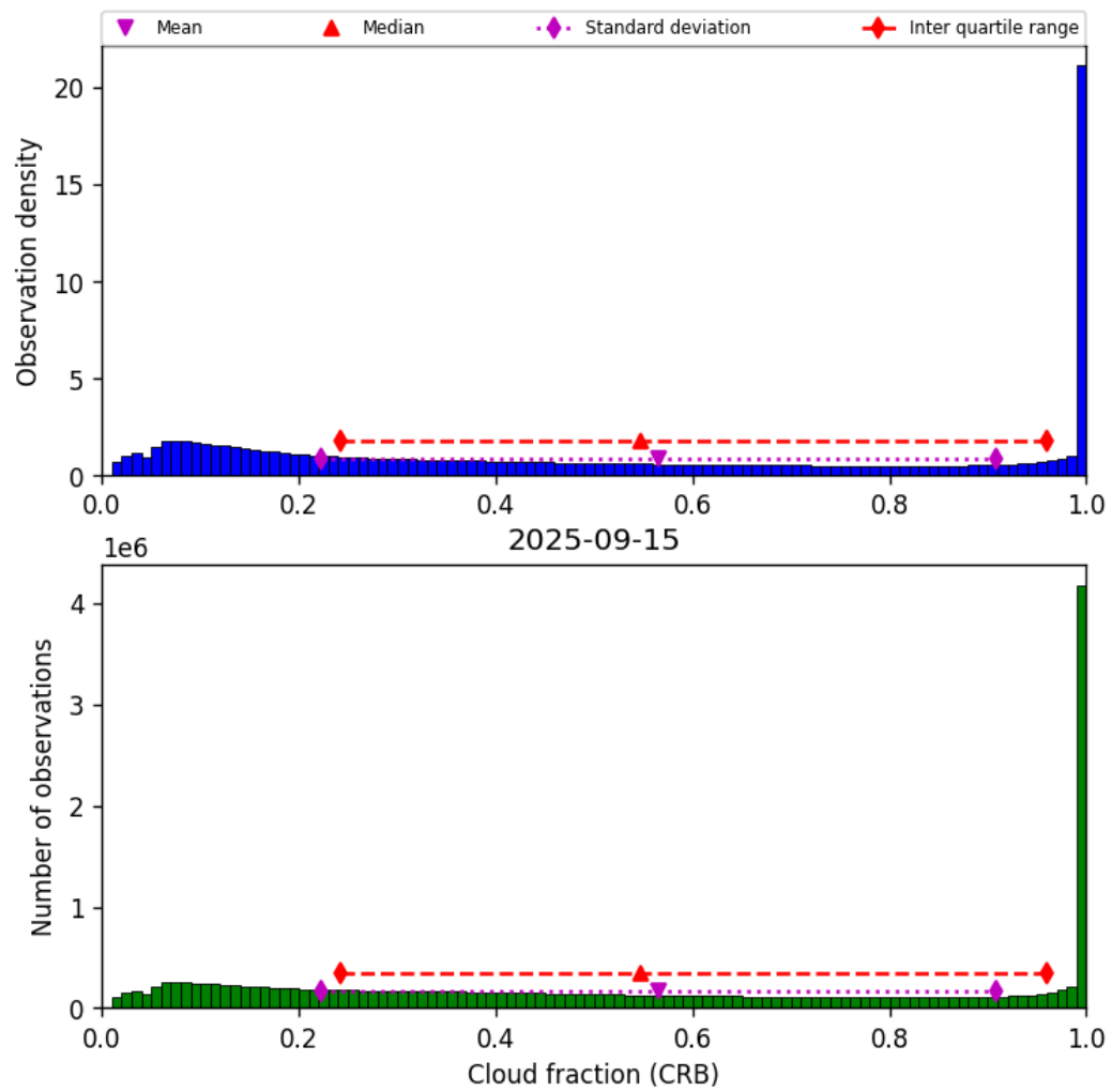
Figure 40: Histogram of “Cloud fraction (CRB)” for 2025-09-15 to 2025-09-16
