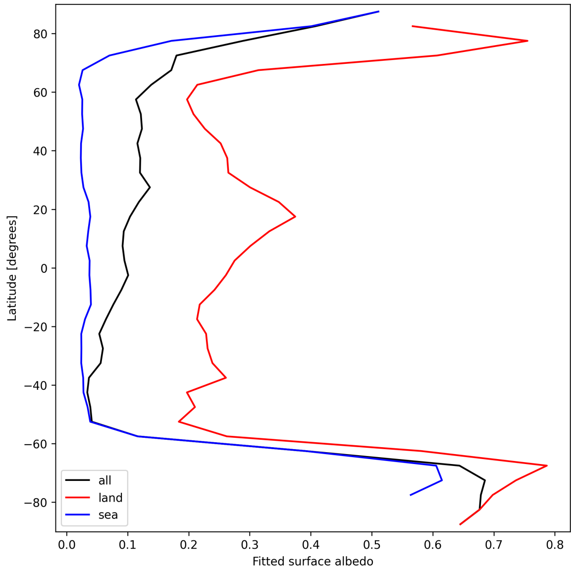
Figure 27: Zonal average of “Fitted surface albedo” for 2025-09-15 to 2025-09-16.
