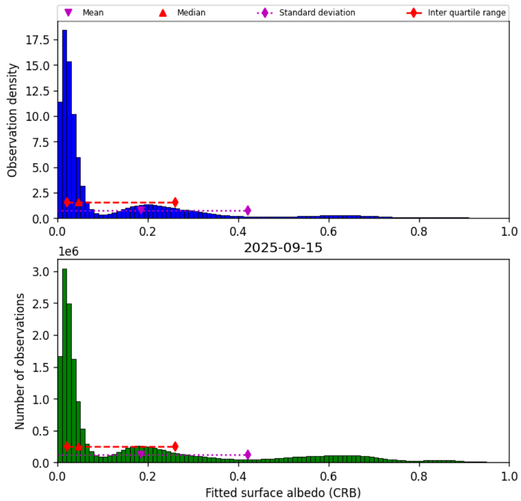
Figure 44: Histogram of “Fitted surface albedo (CRB)” for 2025-09-15 to 2025-09-16
