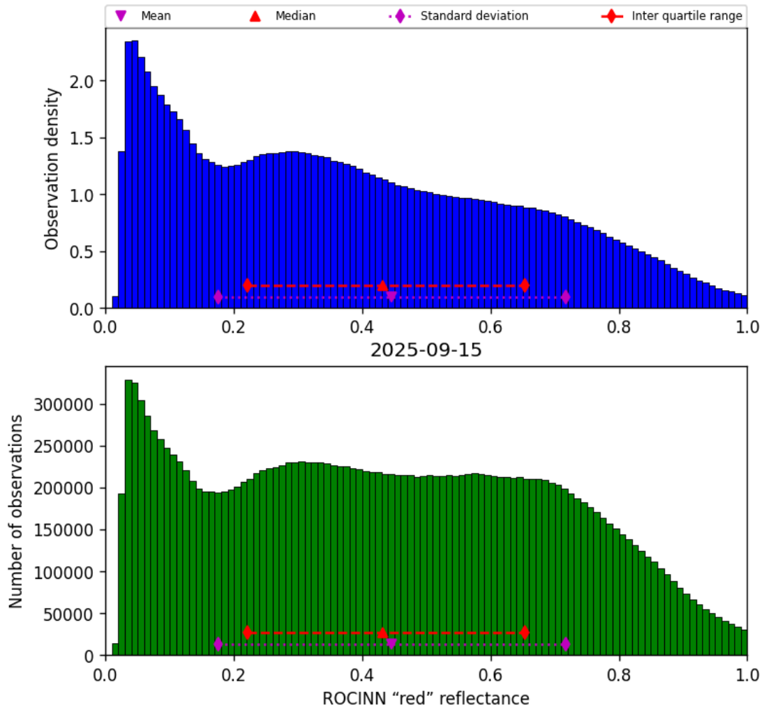
Figure 51: Histogram of “ROCINN “red” reflectance” for 2025-09-15 to 2025-09-16
