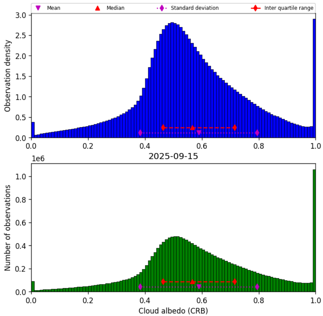
Figure 42: Histogram of “Cloud albedo (CRB)” for 2025-09-15 to 2025-09-16
