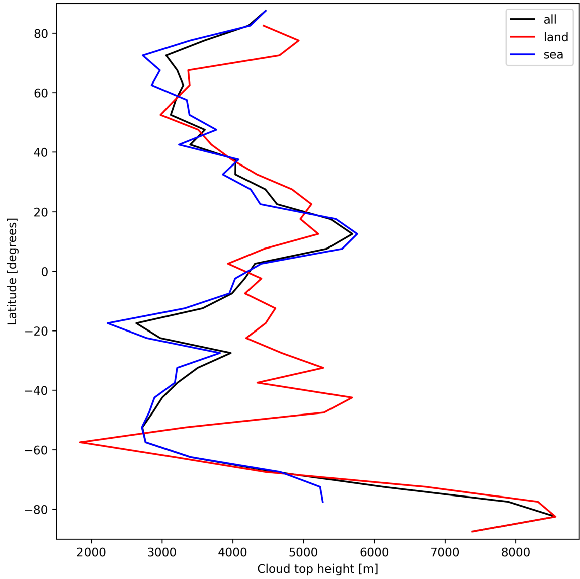
Figure 22: Zonal average of “Cloud top height” for 2025-09-15 to 2025-09-16.
