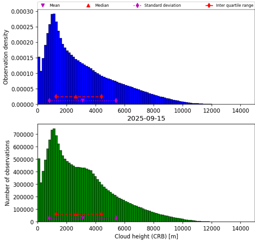
Figure 41: Histogram of “Cloud height (CRB)” for 2025-09-15 to 2025-09-16
