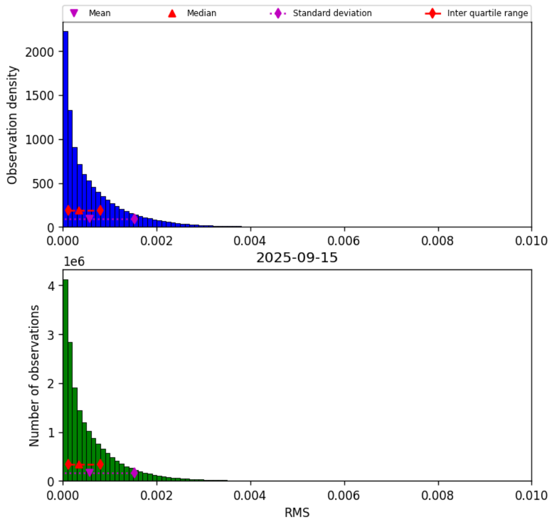
Figure 45: Histogram of “RMS” for 2025-09-15 to 2025-09-16
