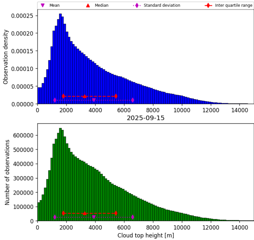
Figure 38: Histogram of “Cloud top height” for 2025-09-15 to 2025-09-16
