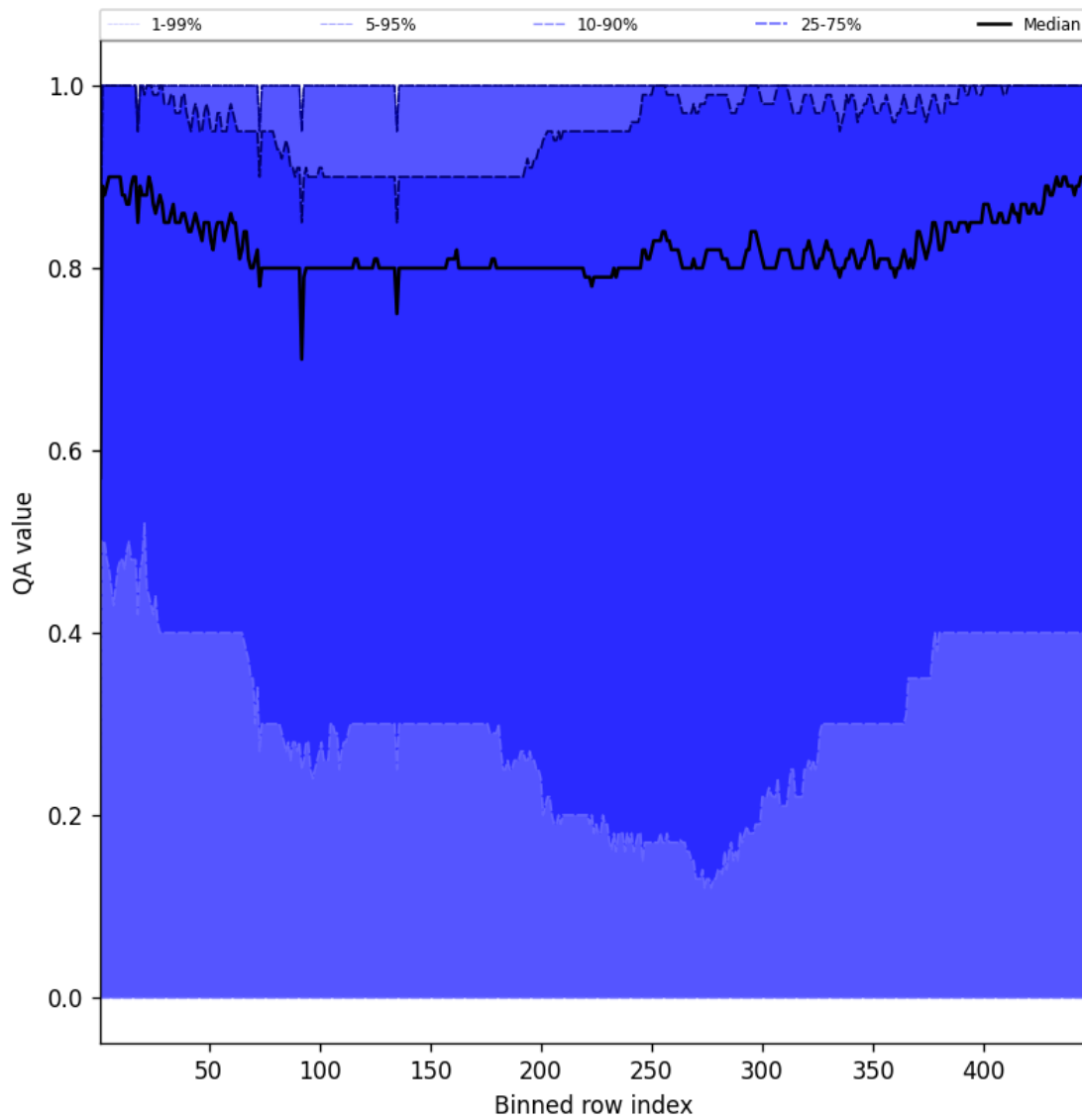
Figure 52: Along track statistics of “QA value” for 2025-09-15 to 2025-09-16
