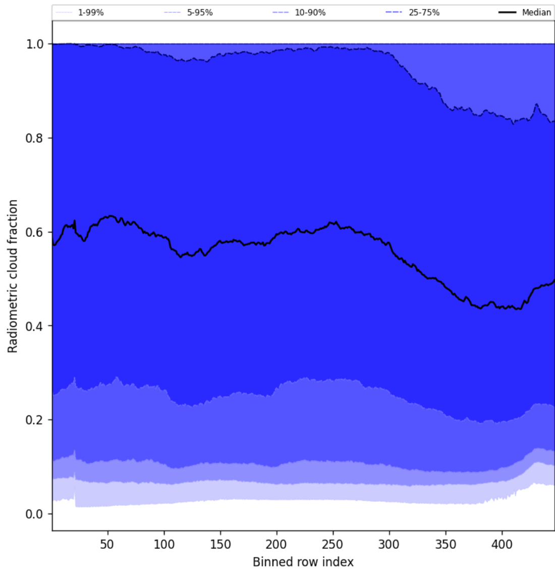
Figure 53: Along track statistics of “Radiometric cloud fraction” for 2025-09-15 to 2025-09-16
