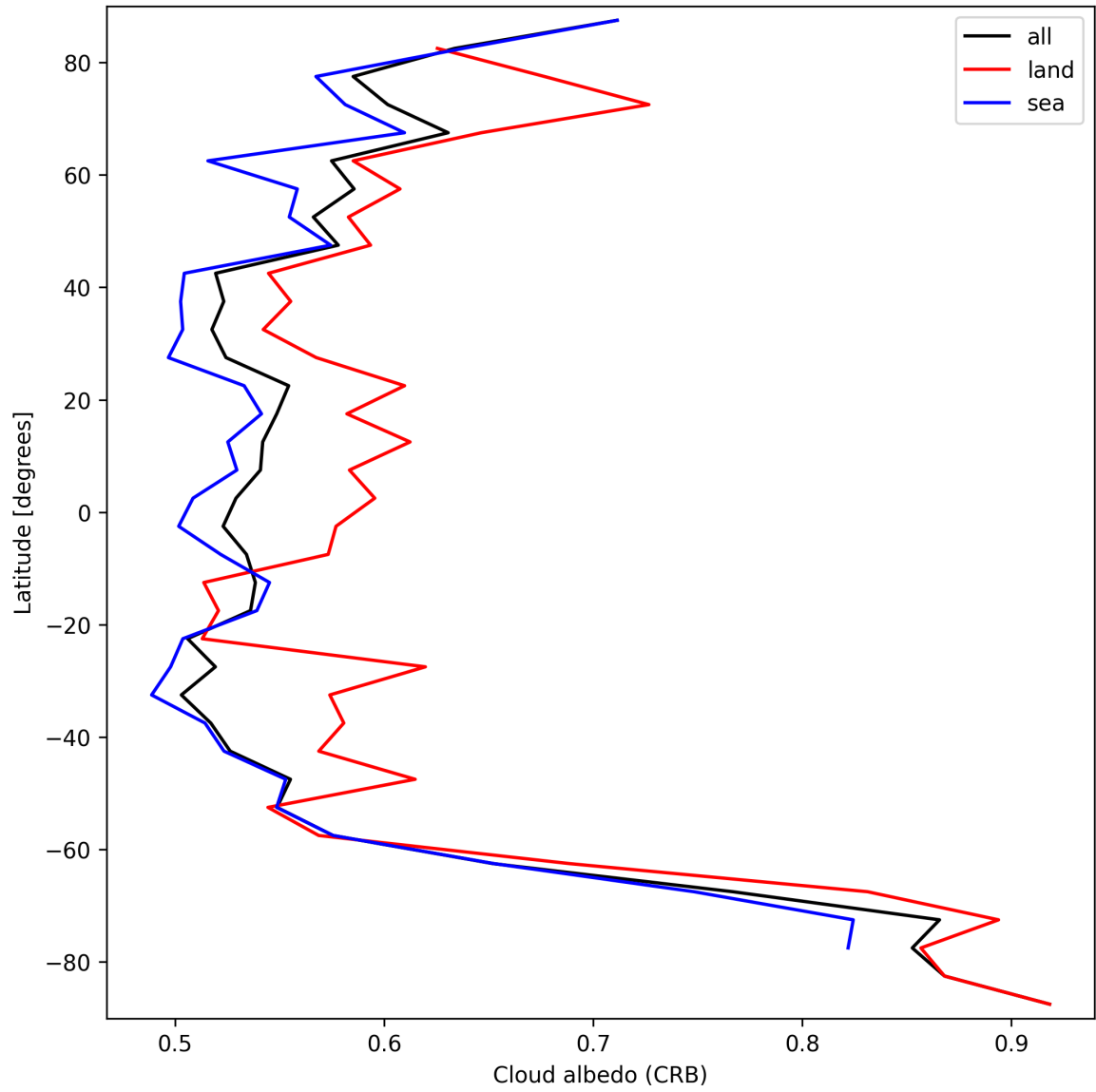
Figure 26: Zonal average of “Cloud albedo (CRB)” for 2025-09-15 to 2025-09-16.
