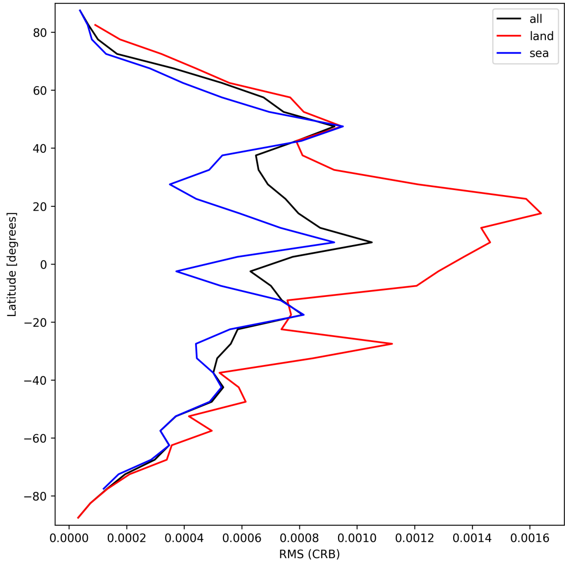
Figure 30: Zonal average of “RMS (CRB)” for 2025-09-15 to 2025-09-16.
