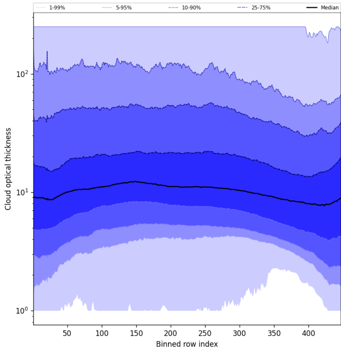
Figure 55: Along track statistics of “Cloud optical thickness” for 2025-09-15 to 2025-09-16
