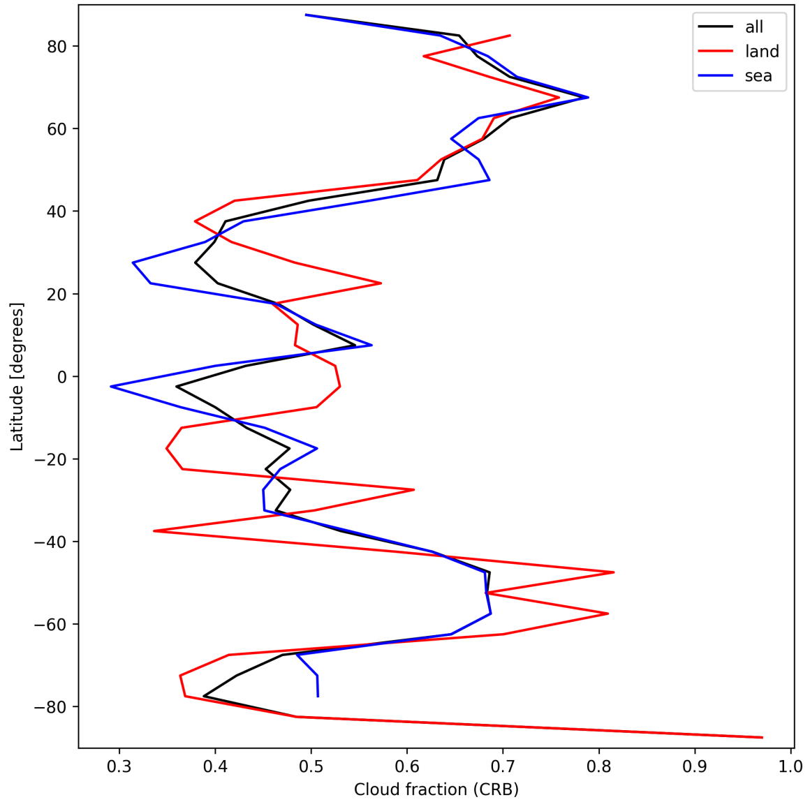
Figure 24: Zonal average of “Cloud fraction (CRB)” for 2025-09-15 to 2025-09-16.
