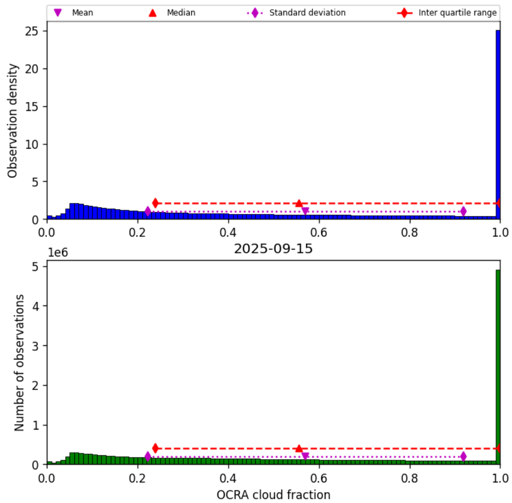
Figure 48: Histogram of “OCRA cloud fraction” for 2025-09-15 to 2025-09-16
