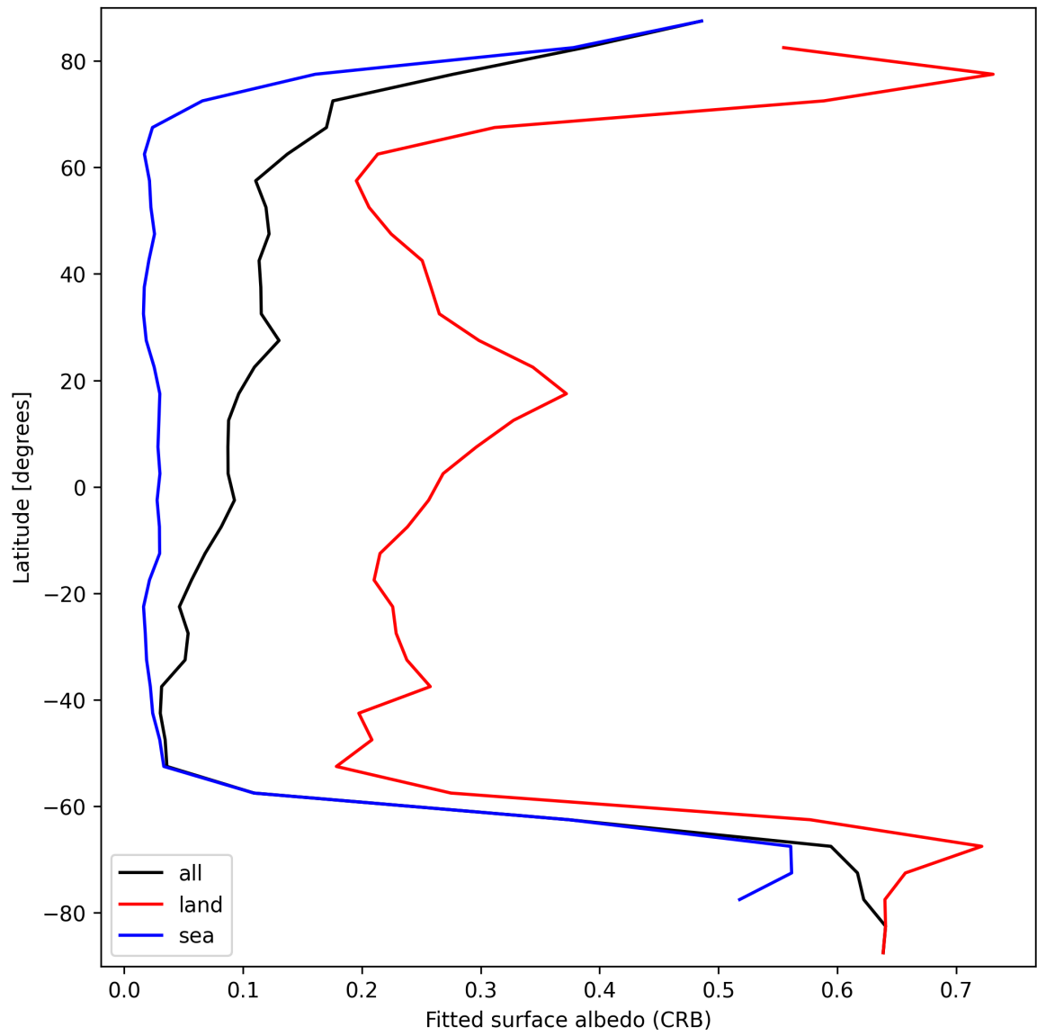
Figure 28: Zonal average of “Fitted surface albedo (CRB)” for 2025-09-15 to 2025-09-16.
