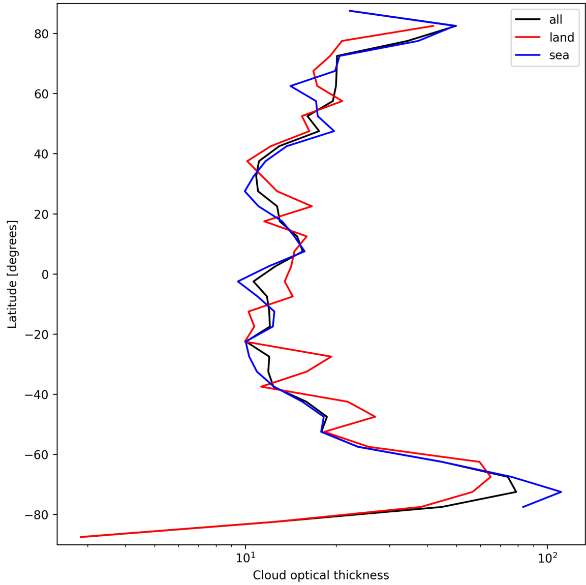
Figure 23: Zonal average of “Cloud optical thickness” for 2025-09-15 to 2025-09-16.
