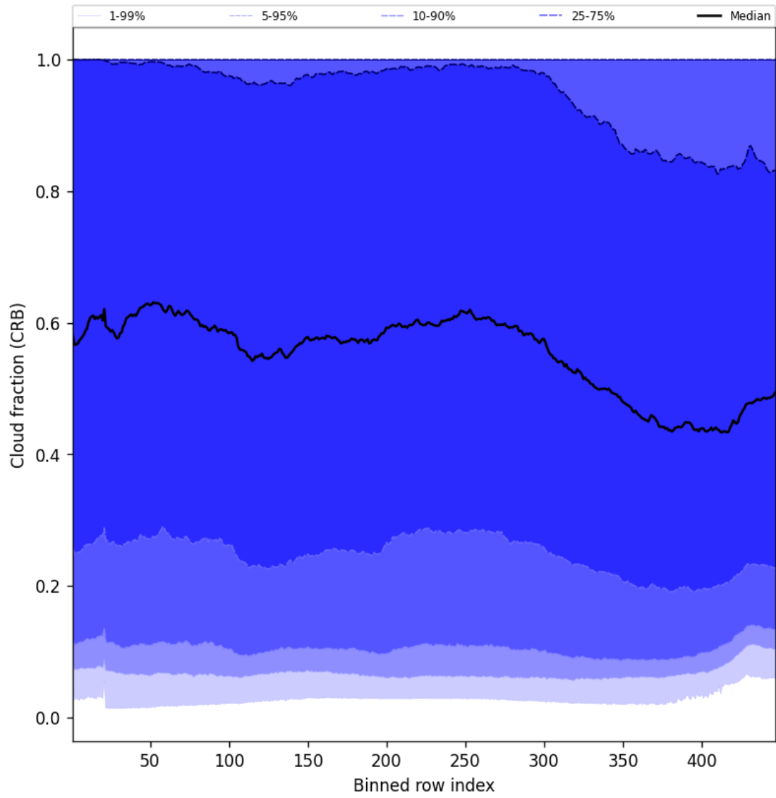
Figure 56: Along track statistics of “Cloud fraction (CRB)” for 2025-09-15 to 2025-09-16
