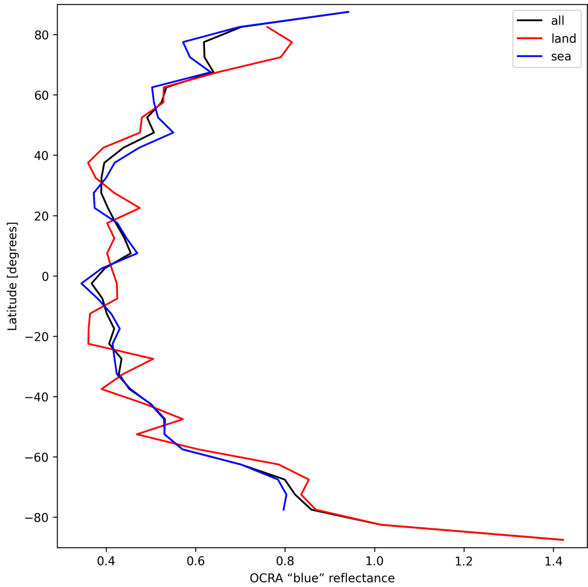
Figure 33: Zonal average of “OCRA “blue” reflectance” for 2025-09-15 to 2025-09-16.
