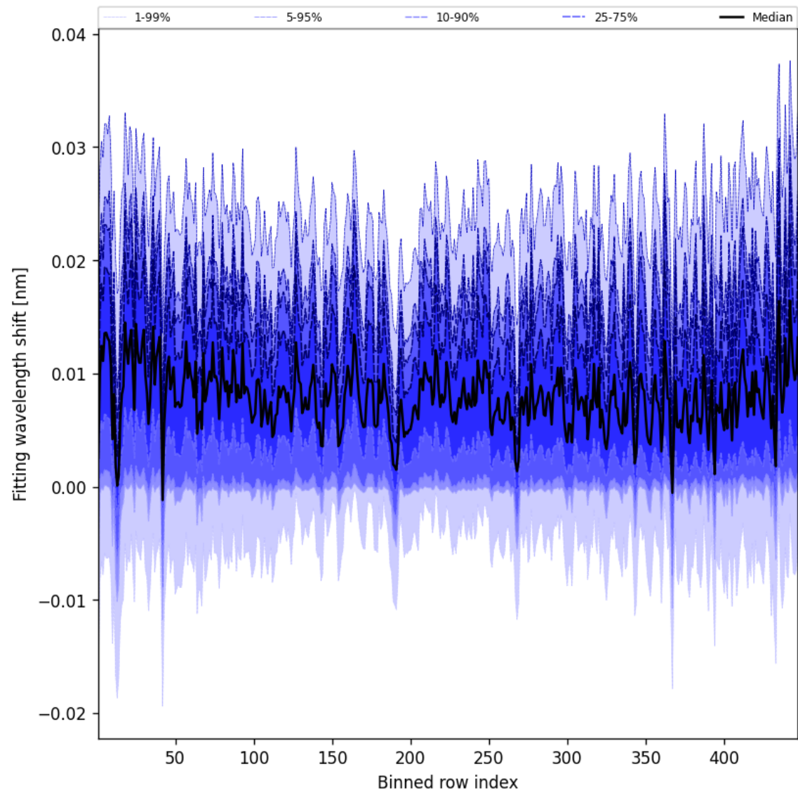
Figure 63: Along track statistics of “Fitting wavelength shift” for 2025-09-15 to 2025-09-16
