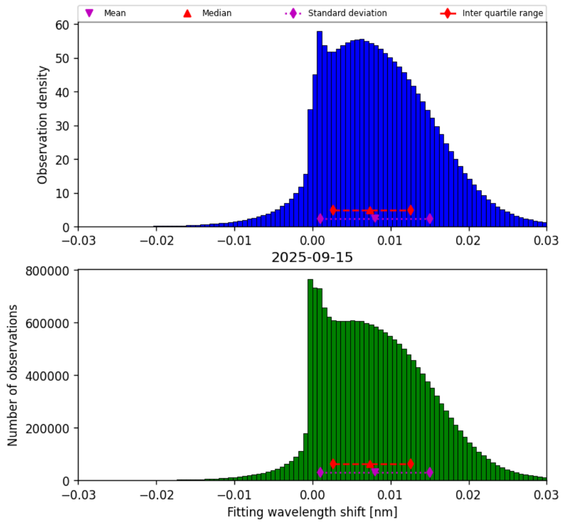
Figure 47: Histogram of “Fitting wavelength shift” for 2025-09-15 to 2025-09-16
