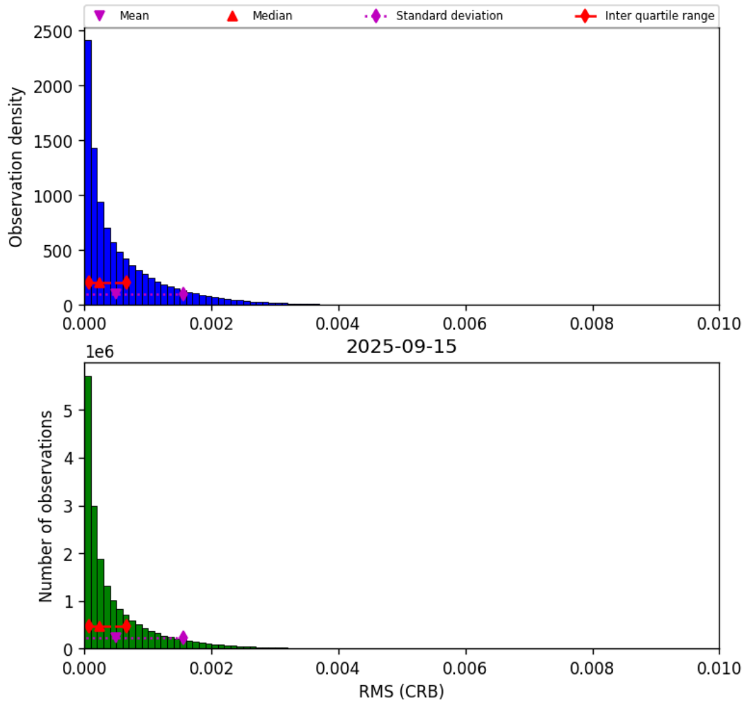
Figure 46: Histogram of “RMS (CRB)” for 2025-09-15 to 2025-09-16
