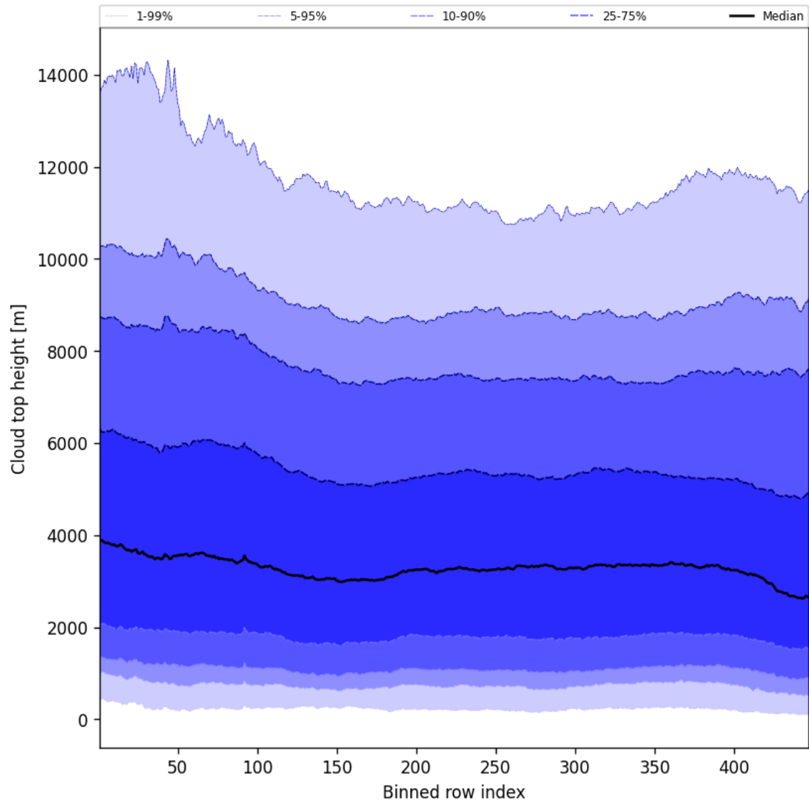
Figure 54: Along track statistics of “Cloud top height” for 2025-09-15 to 2025-09-16
