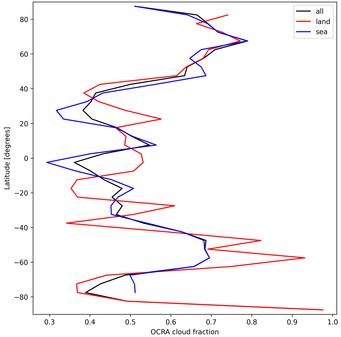
Figure 32: Zonal average of “OCRA cloud fraction” for 2025-09-15 to 2025-09-16.
