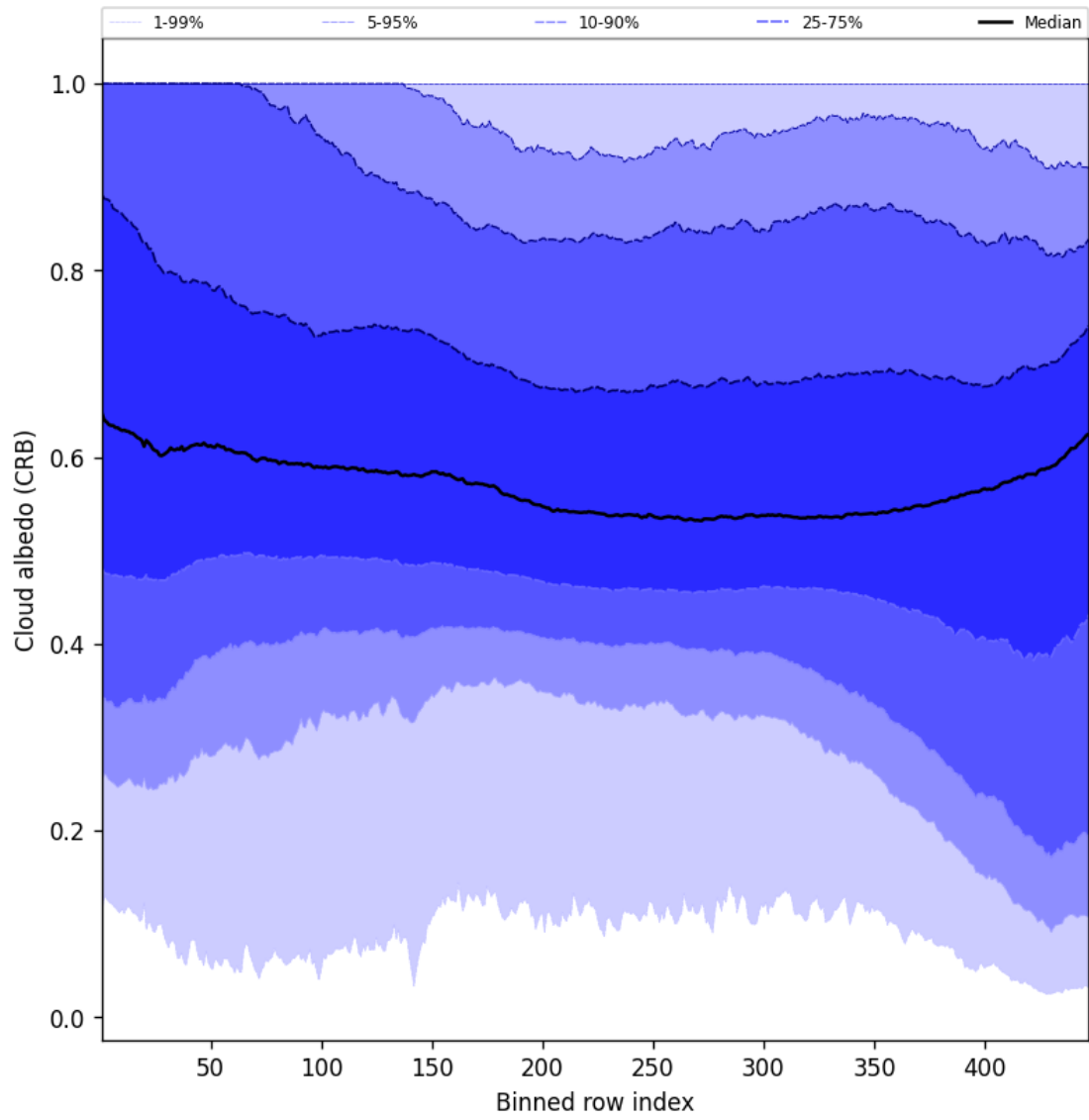
Figure 58: Along track statistics of “Cloud albedo (CRB)” for 2025-09-15 to 2025-09-16
