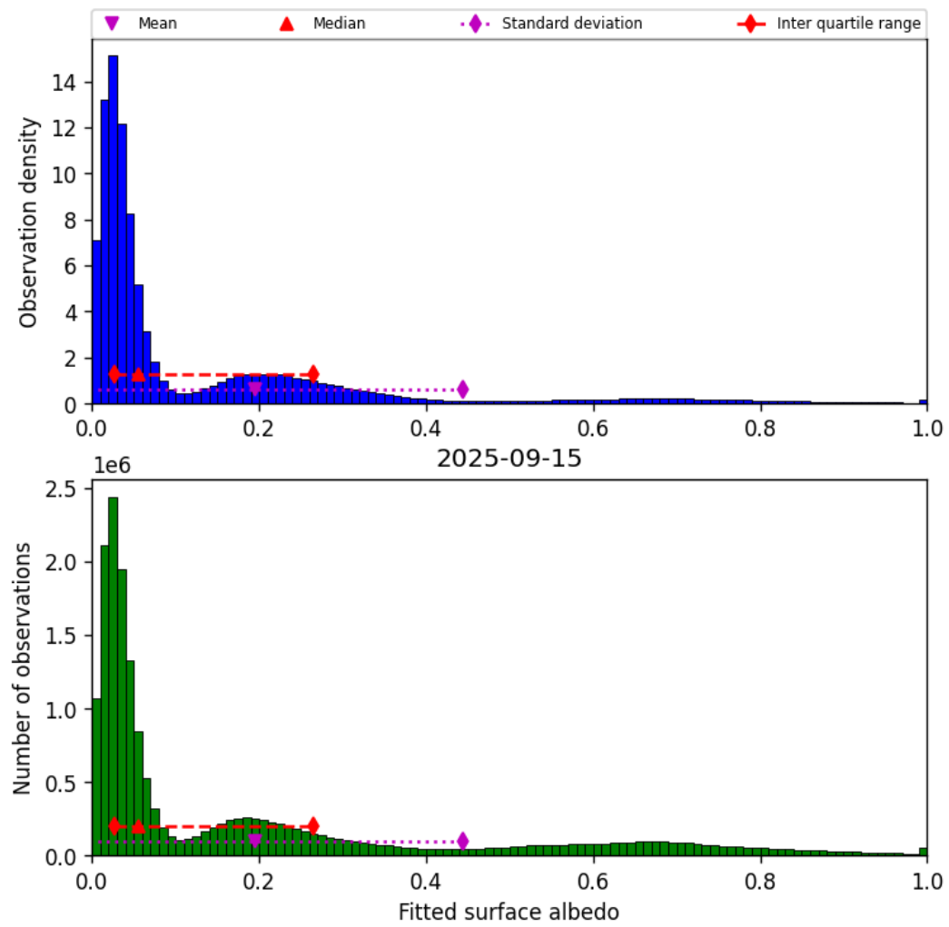
Figure 43: Histogram of “Fitted surface albedo” for 2025-09-15 to 2025-09-16
