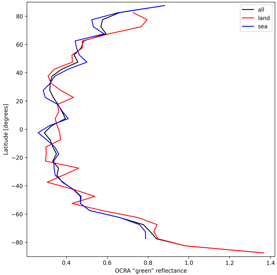
Figure 34: Zonal average of “OCRA “green” reflectance” for 2025-09-15 to 2025-09-16.
