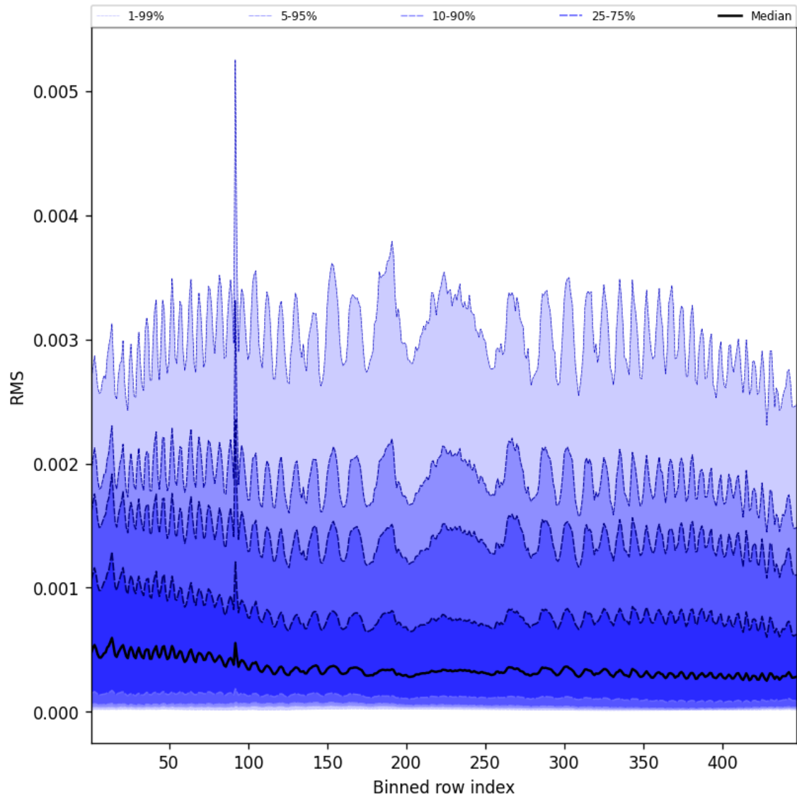
Figure 61: Along track statistics of “RMS” for 2025-09-15 to 2025-09-16
