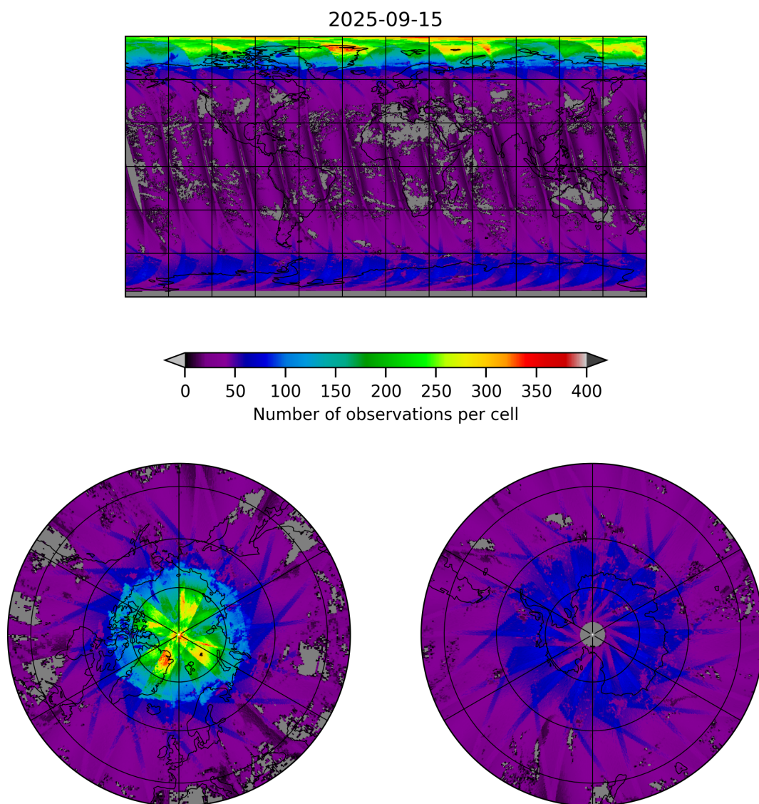
Figure 19: Map of the number of observations for 2025-09-15 to 2025-09-16
