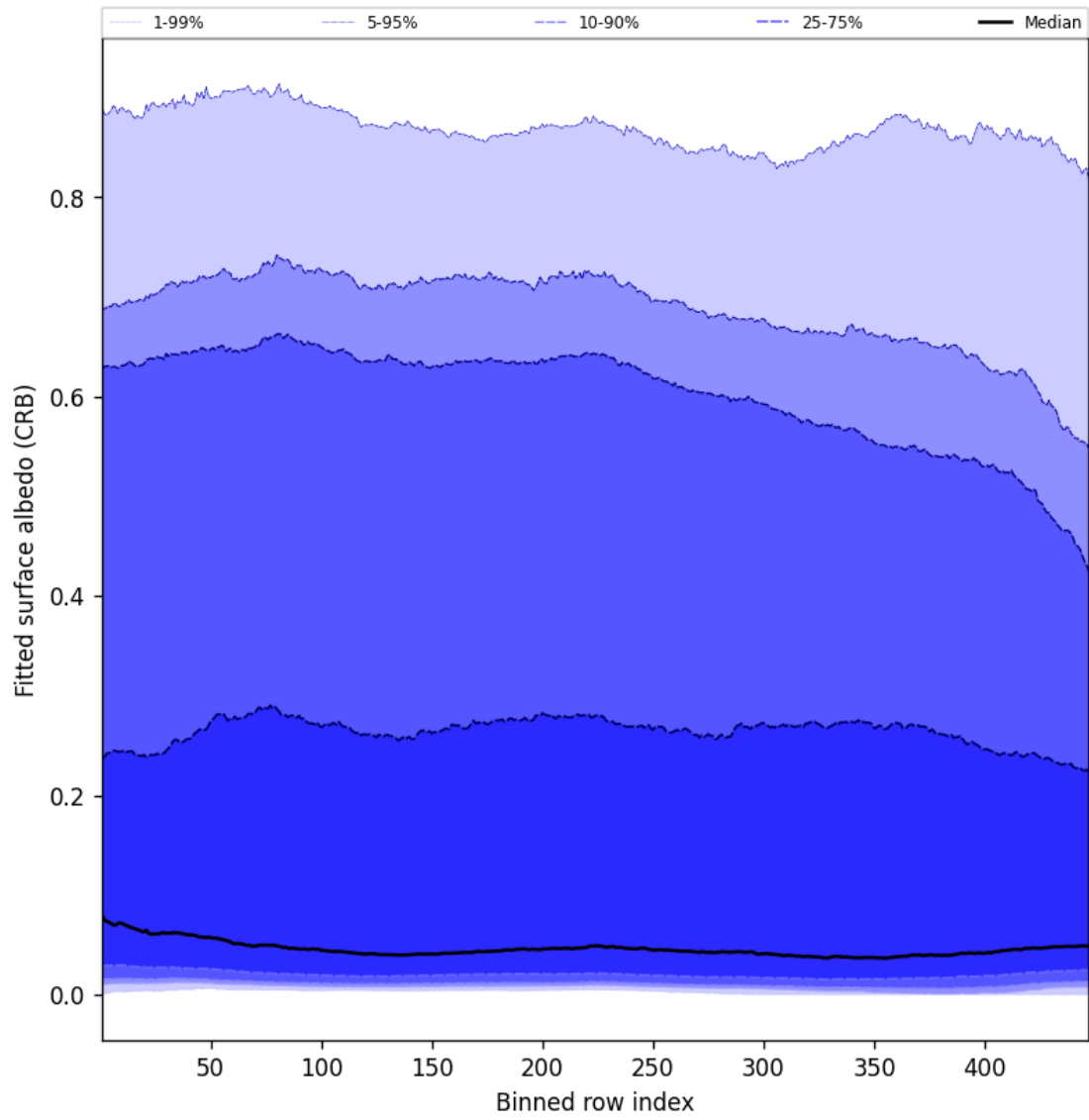
Figure 60: Along track statistics of “Fitted surface albedo (CRB)” for 2025-09-15 to 2025-09-16
