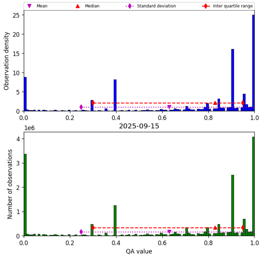
Figure 36: Histogram of “QA value” for 2025-09-15 to 2025-09-16
