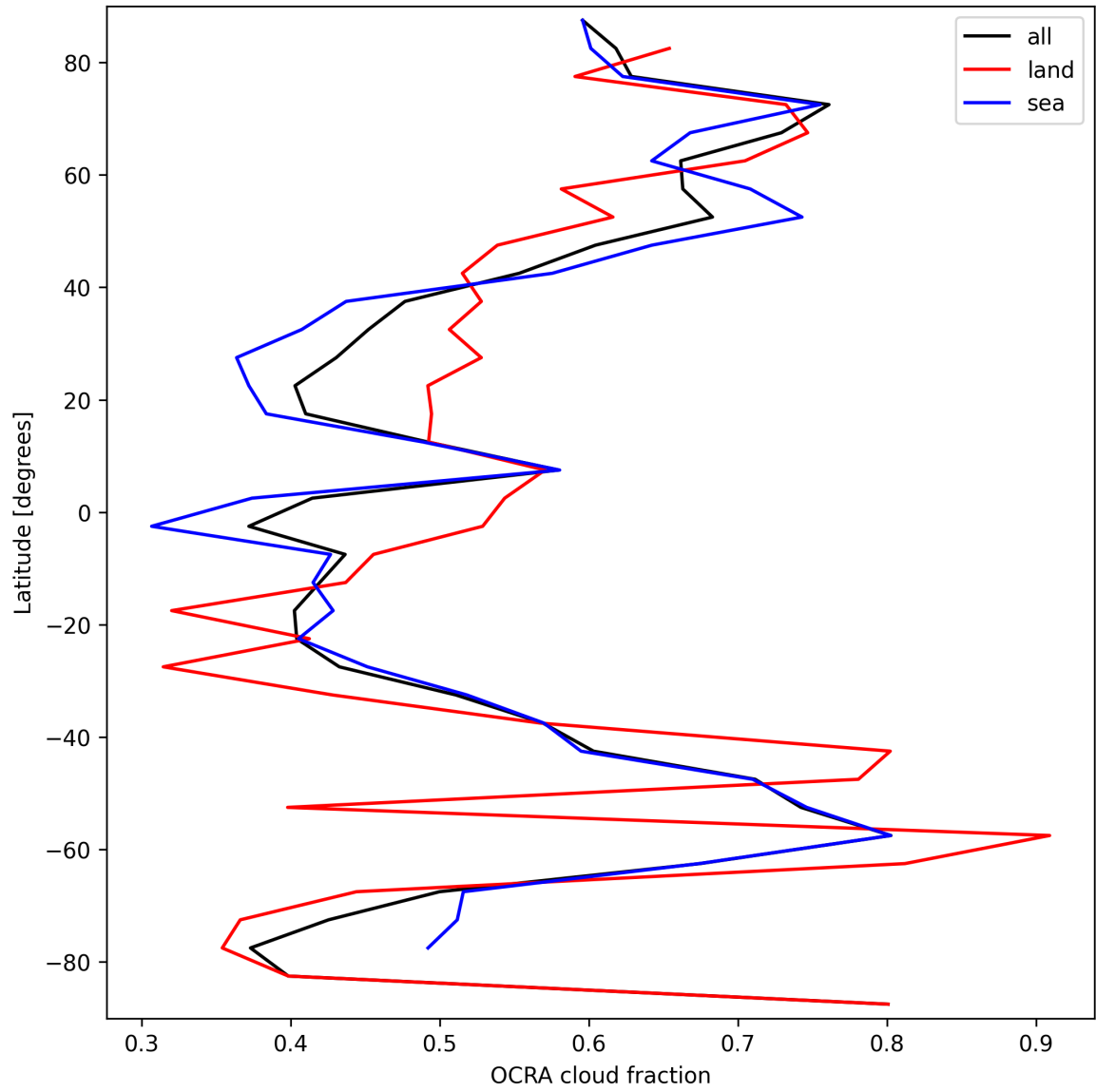
Figure 32: Zonal average of “OCRA cloud fraction” for 2025-09-18 to 2025-09-18.
