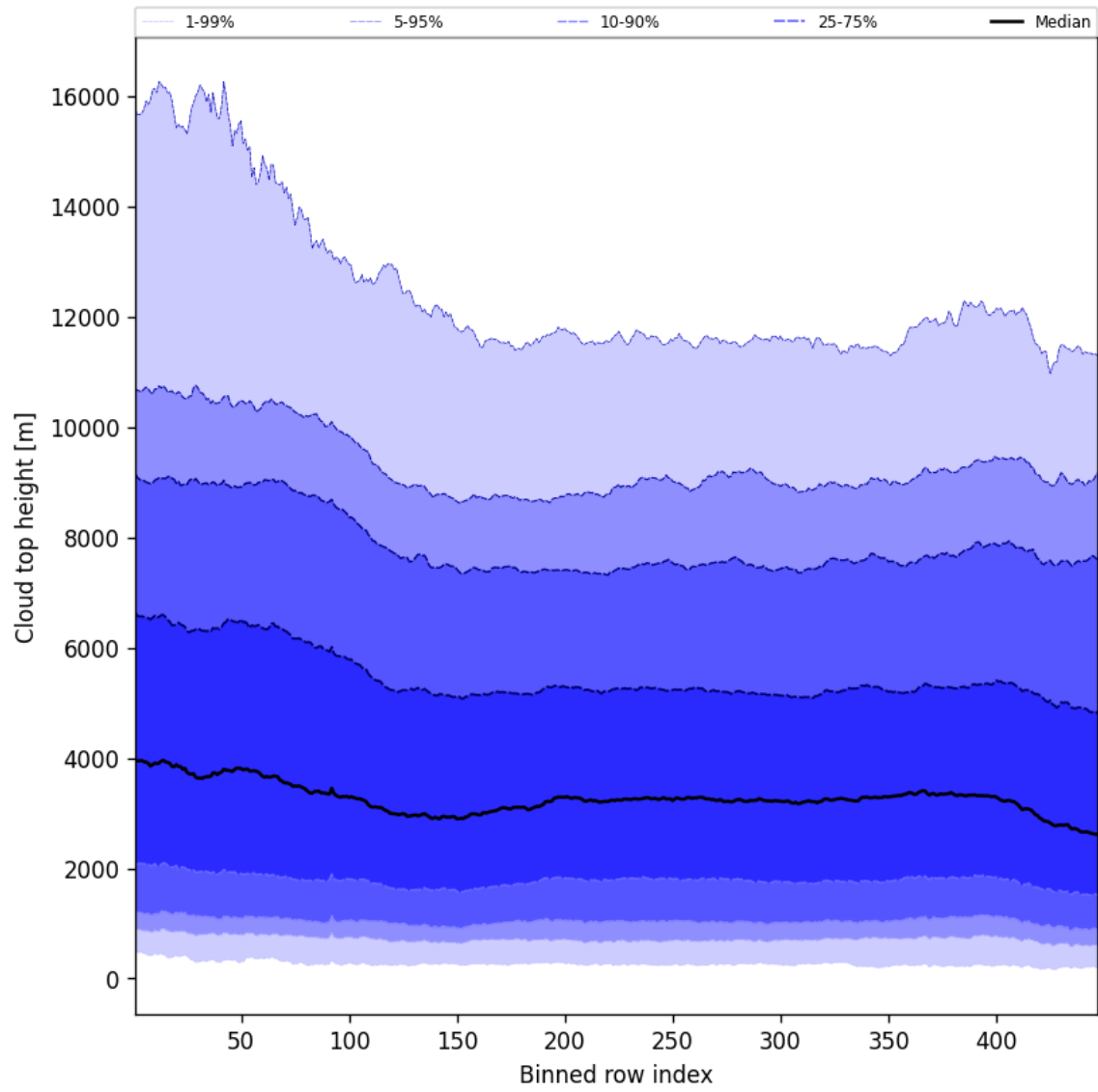
Figure 54: Along track statistics of “Cloud top height” for 2025-09-18 to 2025-09-18
