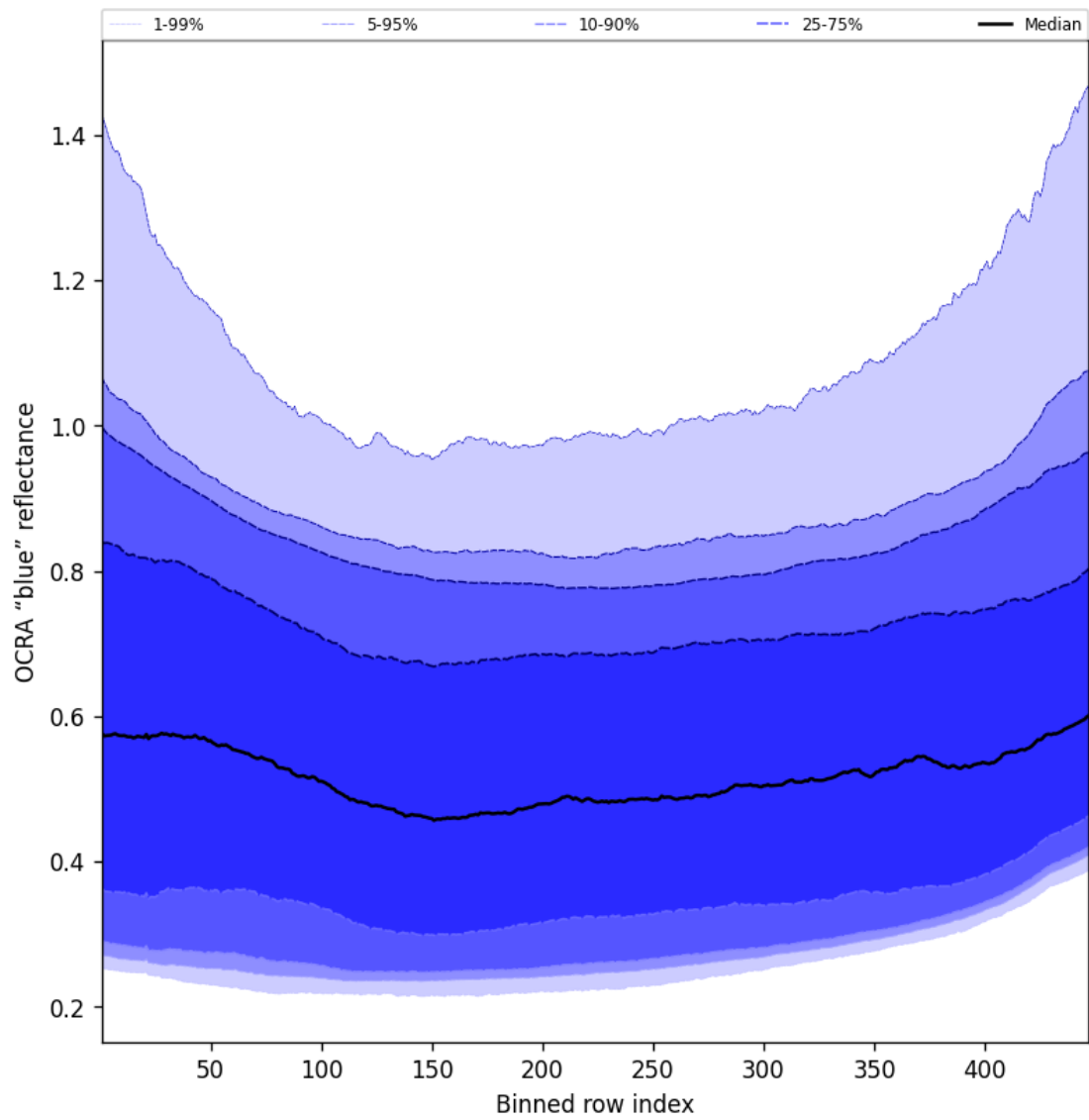
Figure 65: Along track statistics of “OCRA “blue” reflectance” for 2025-09-18 to 2025-09-18
