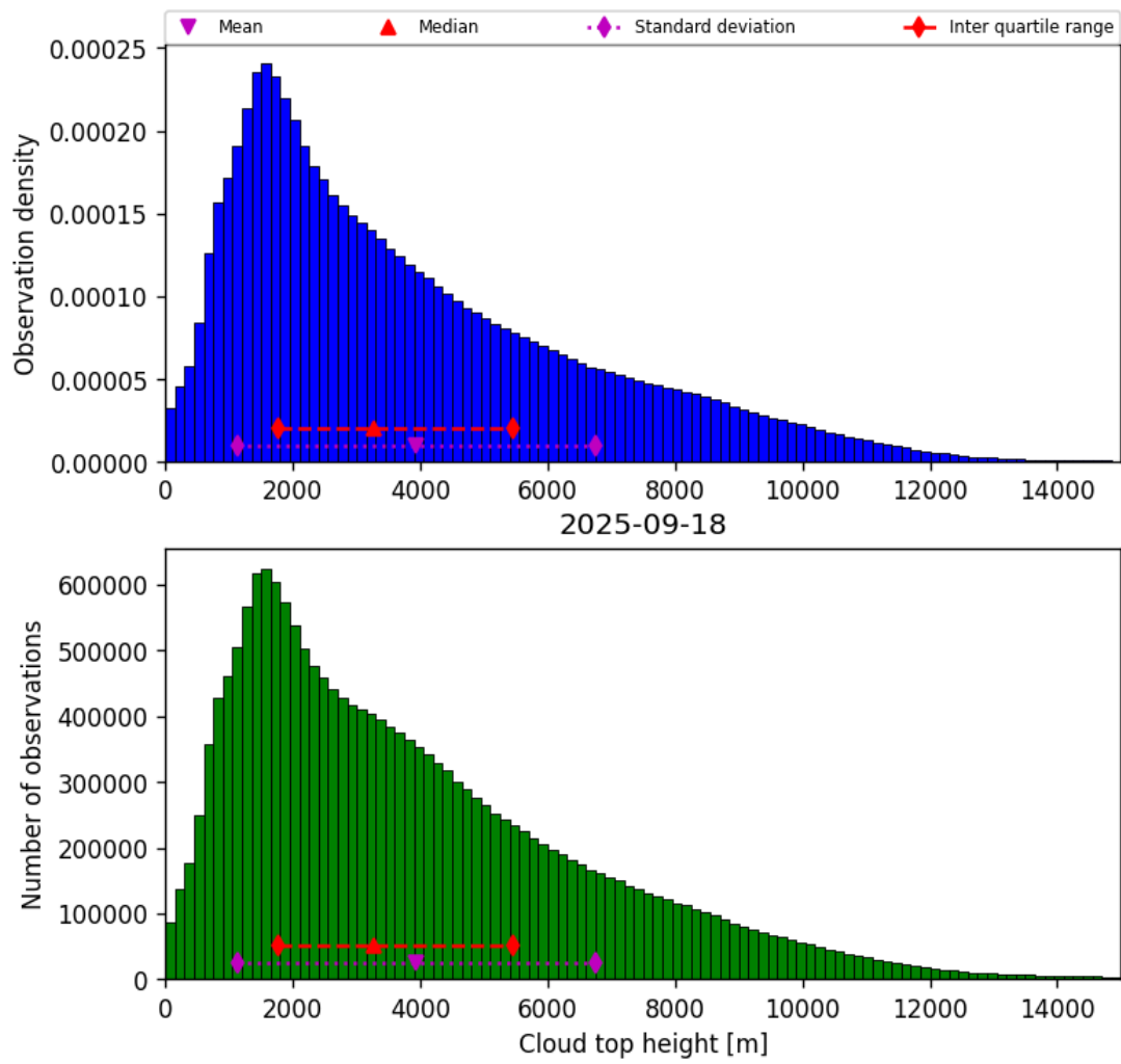
Figure 38: Histogram of “Cloud top height” for 2025-09-18 to 2025-09-18
