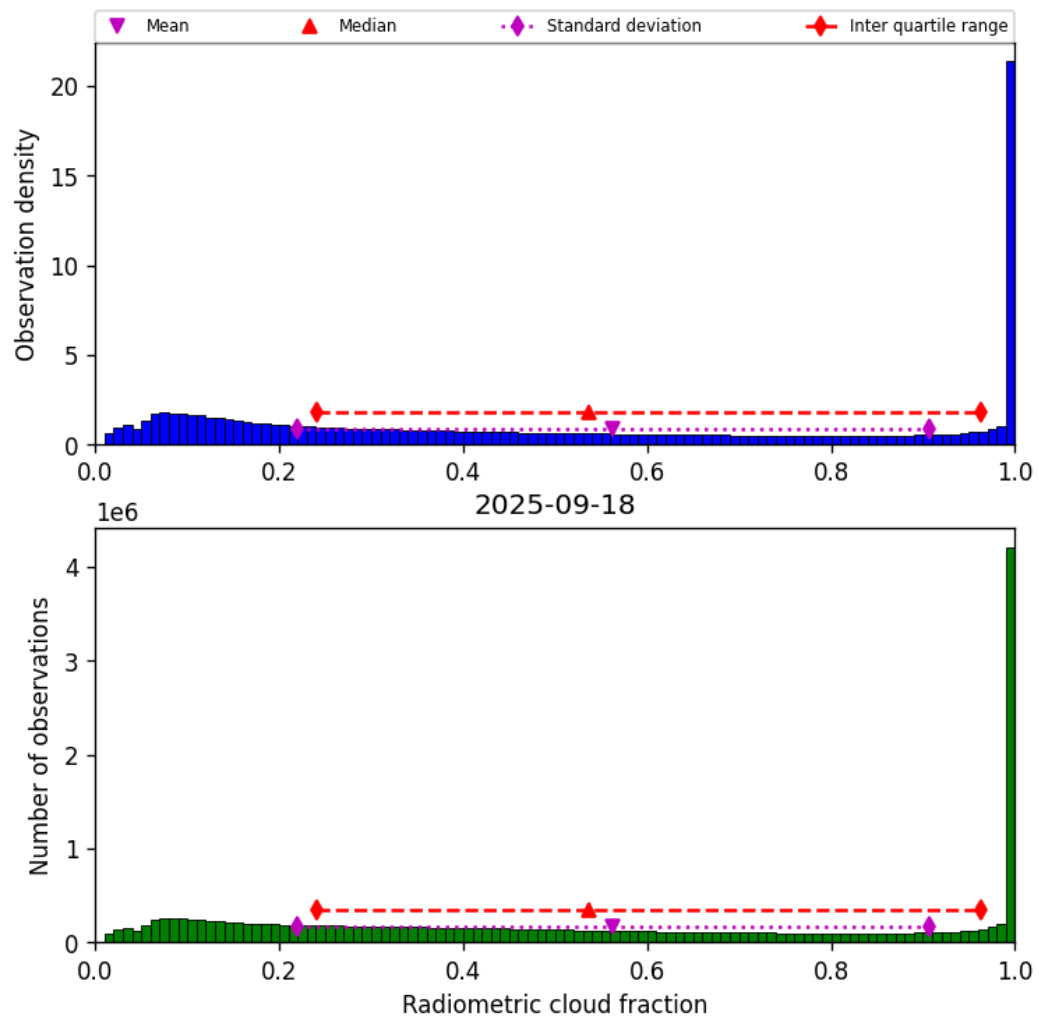
Figure 37: Histogram of “Radiometric cloud fraction” for 2025-09-18 to 2025-09-18
