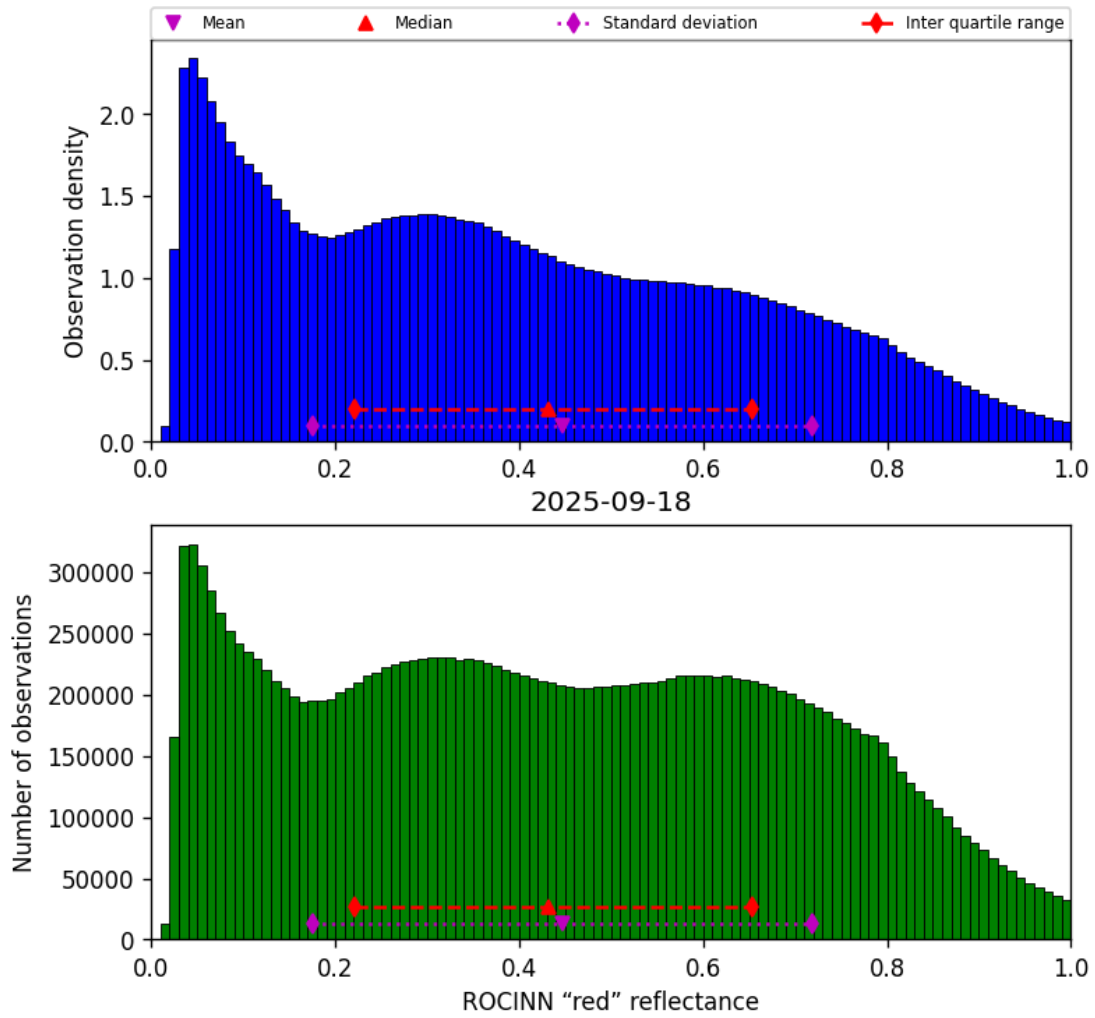
Figure 51: Histogram of “ROCINN “red” reflectance” for 2025-09-18 to 2025-09-18
