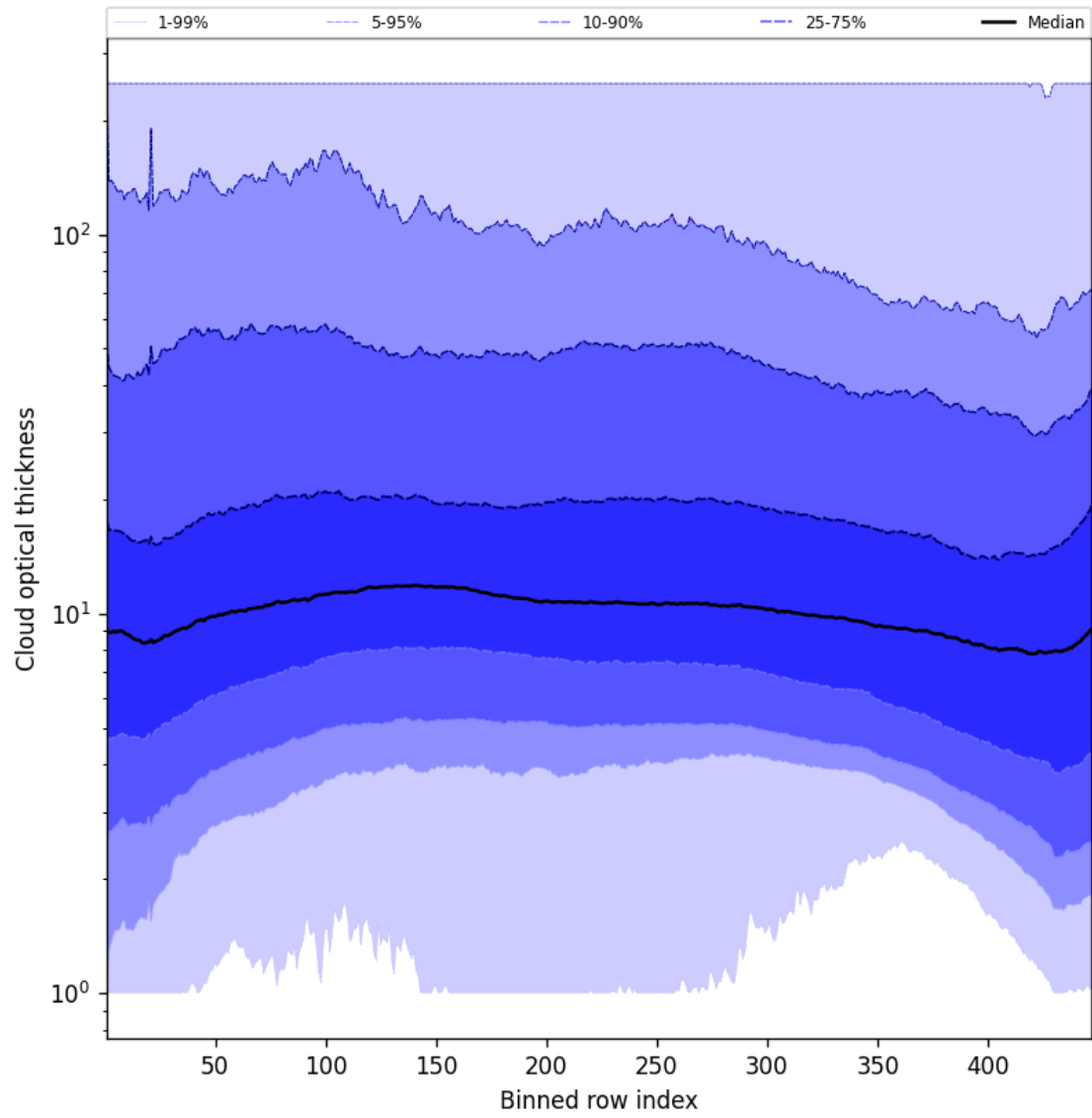
Figure 55: Along track statistics of “Cloud optical thickness” for 2025-09-18 to 2025-09-18
