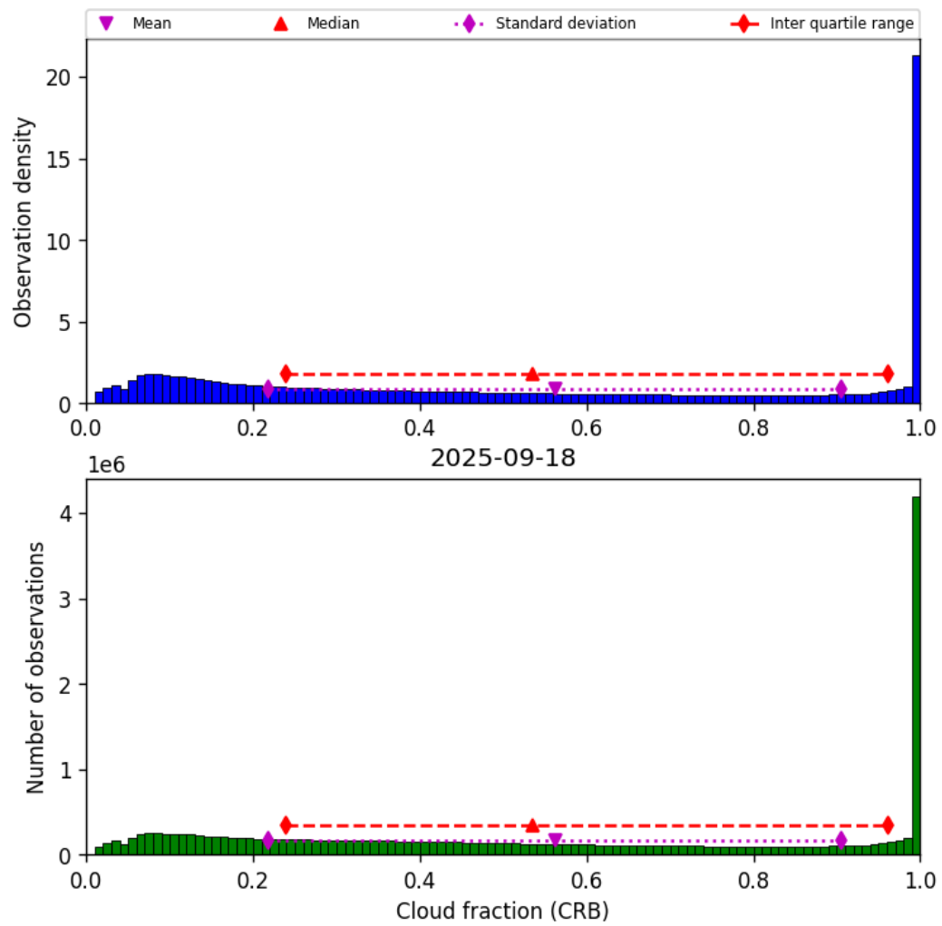
Figure 40: Histogram of “Cloud fraction (CRB)” for 2025-09-18 to 2025-09-18
