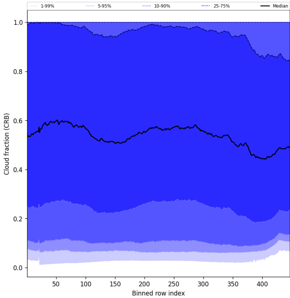
Figure 56: Along track statistics of “Cloud fraction (CRB)” for 2025-09-18 to 2025-09-18
