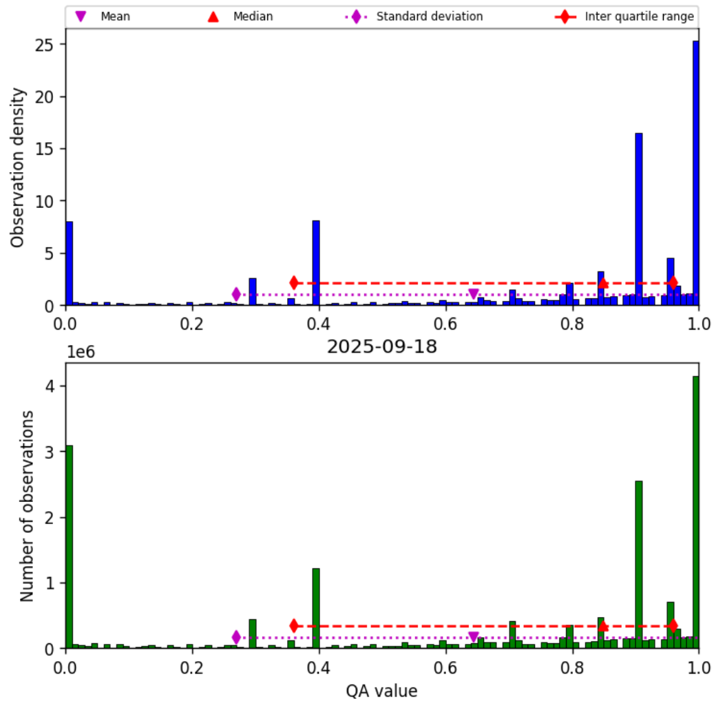
Figure 36: Histogram of “QA value” for 2025-09-18 to 2025-09-18
