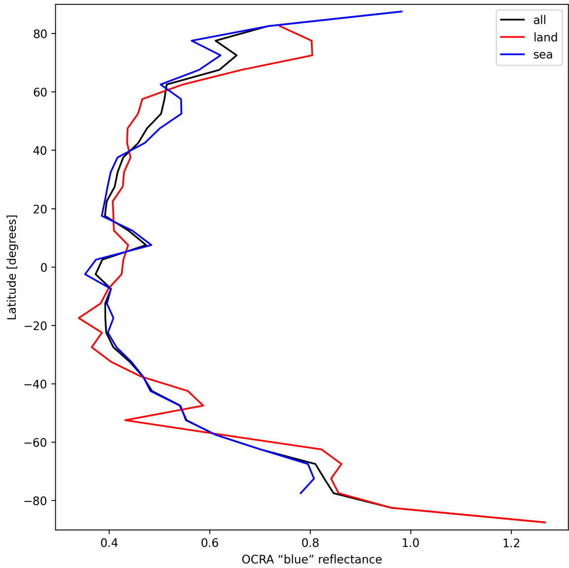
Figure 33: Zonal average of “OCRA “blue” reflectance” for 2025-09-18 to 2025-09-18.
