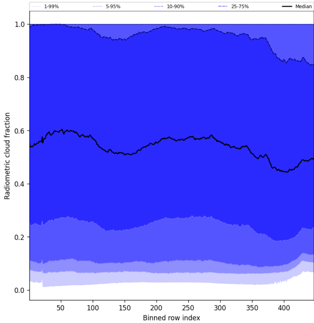
Figure 53: Along track statistics of “Radiometric cloud fraction” for 2025-09-18 to 2025-09-18
