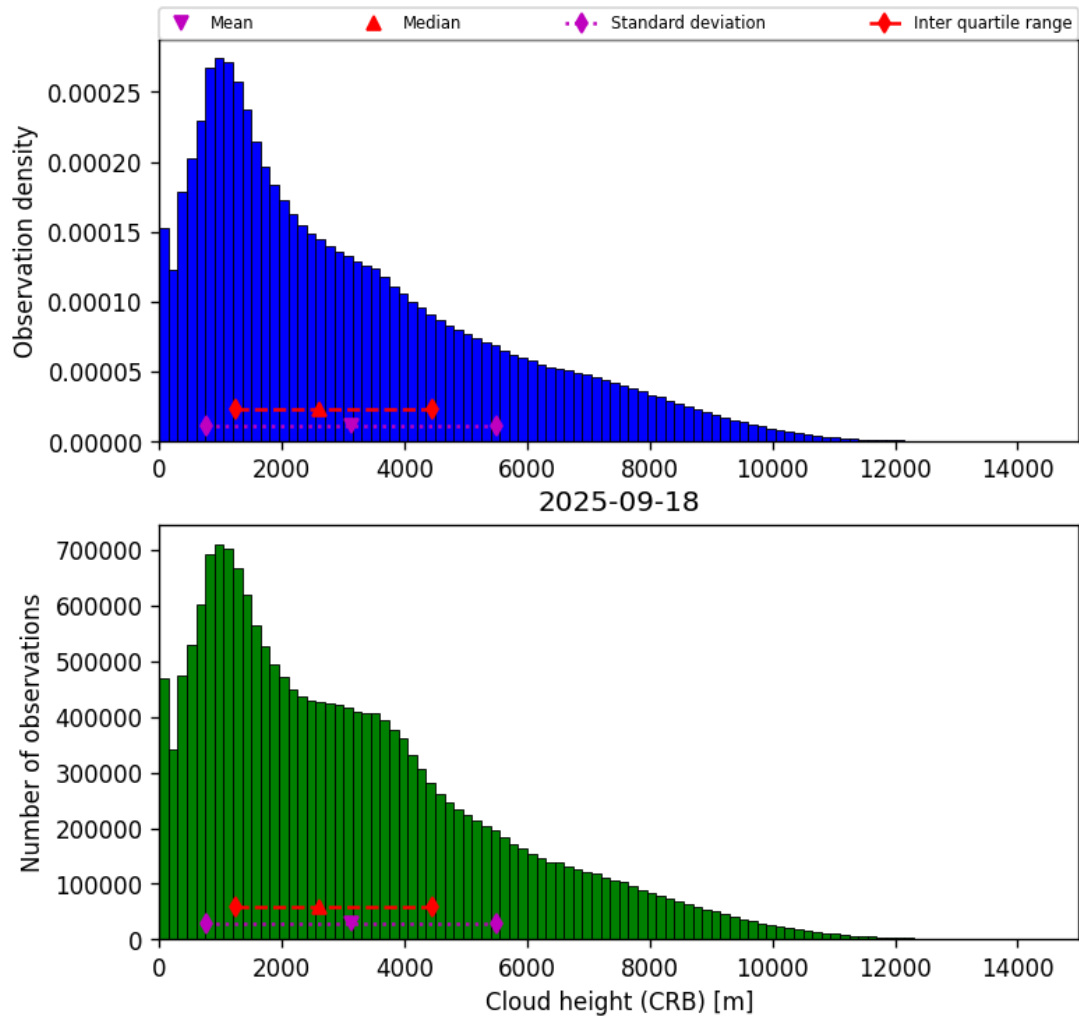
Figure 41: Histogram of “Cloud height (CRB)” for 2025-09-18 to 2025-09-18
