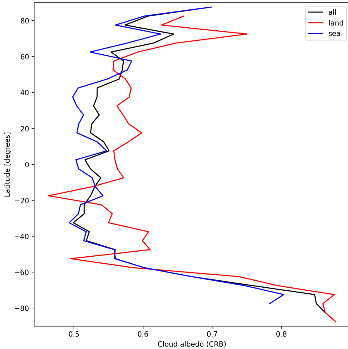
Figure 26: Zonal average of “Cloud albedo (CRB)” for 2025-09-18 to 2025-09-18.
