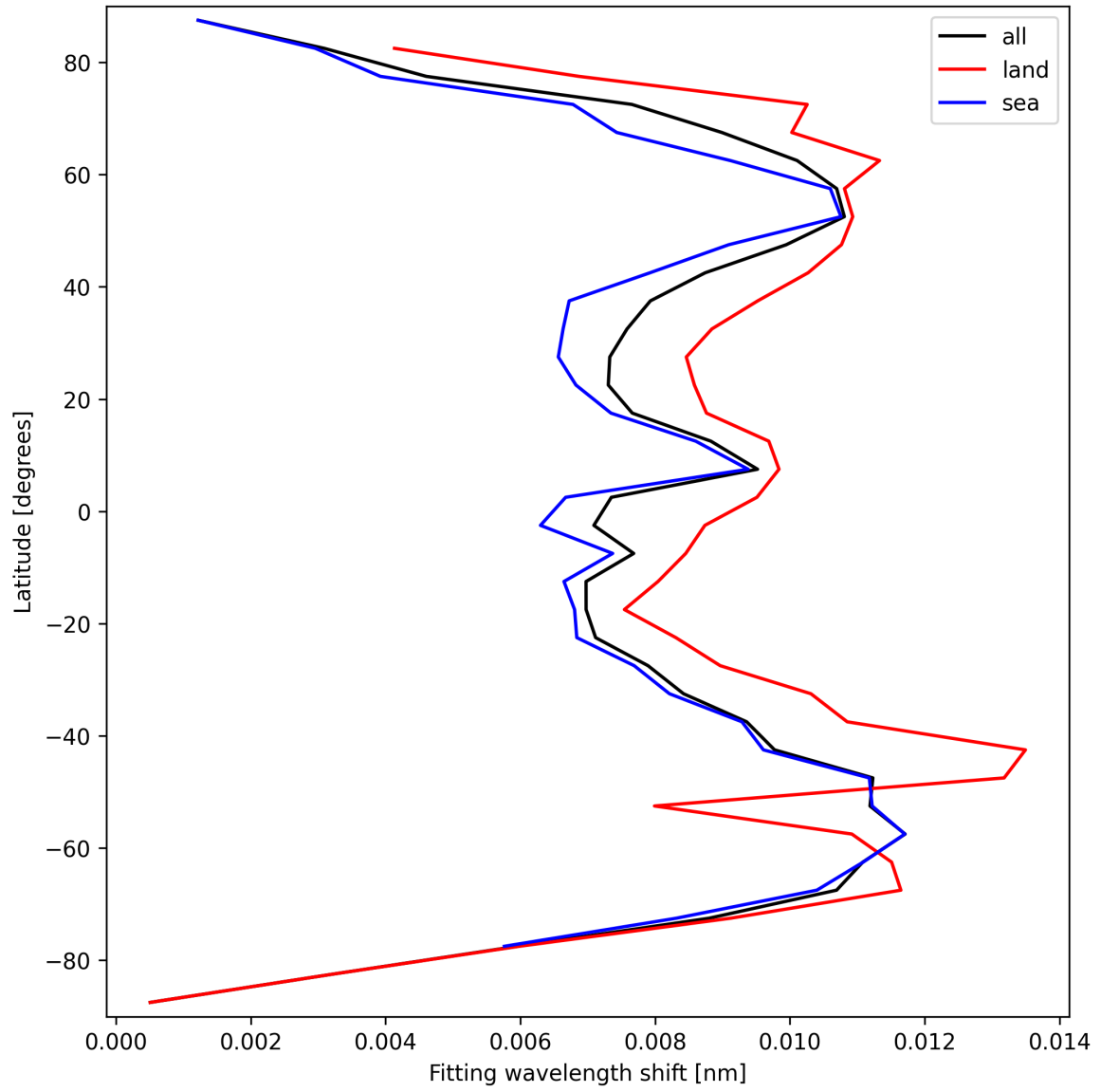
Figure 31: Zonal average of “Fitting wavelength shift” for 2025-09-18 to 2025-09-18.
