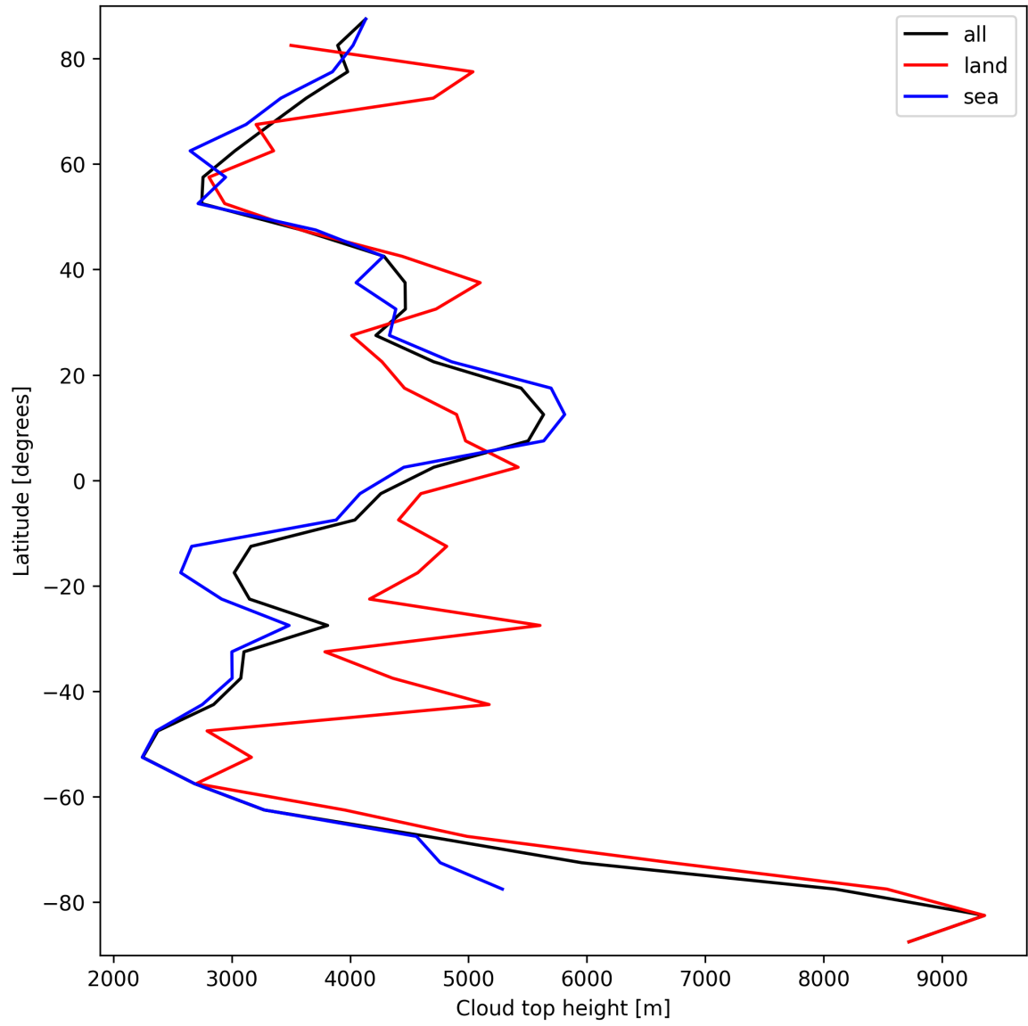
Figure 22: Zonal average of “Cloud top height” for 2025-09-18 to 2025-09-18.
