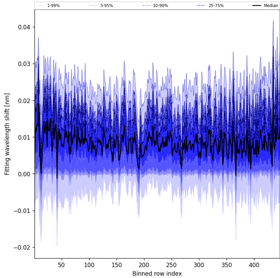
Figure 63: Along track statistics of “Fitting wavelength shift” for 2025-09-18 to 2025-09-18
