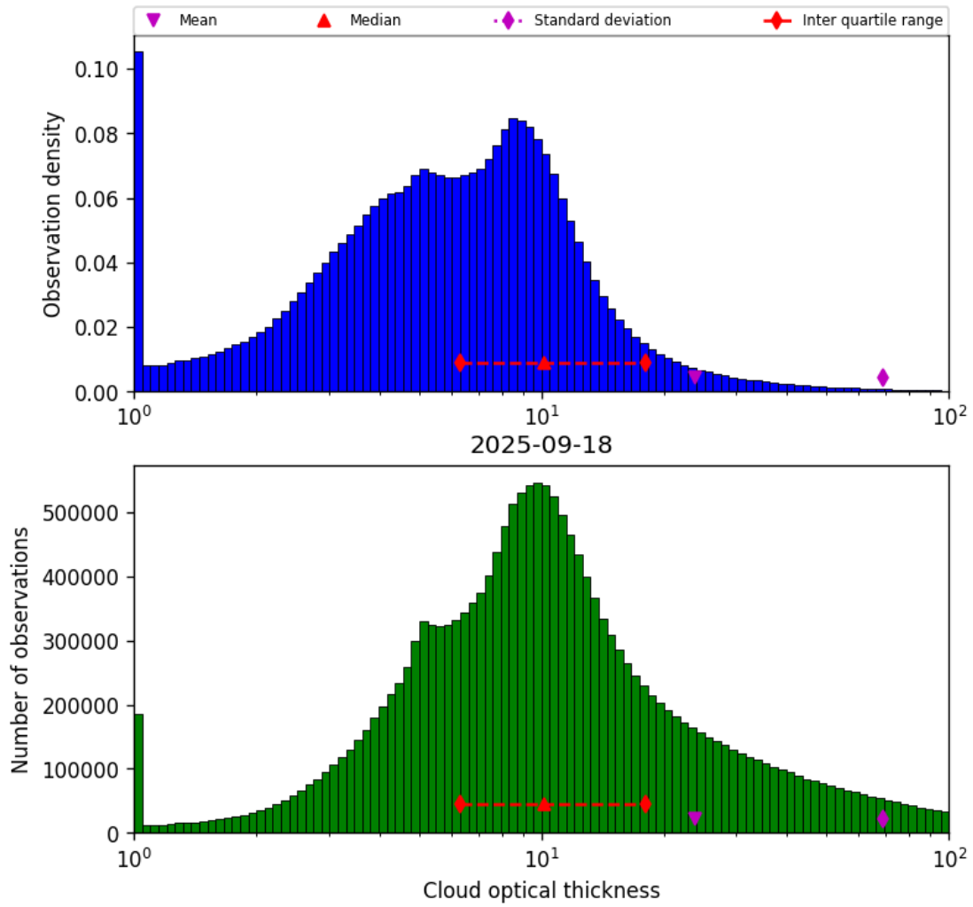
Figure 39: Histogram of “Cloud optical thickness” for 2025-09-18 to 2025-09-18
