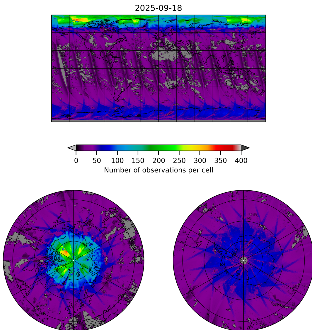
Figure 19: Map of the number of observations for 2025-09-18 to 2025-09-18
