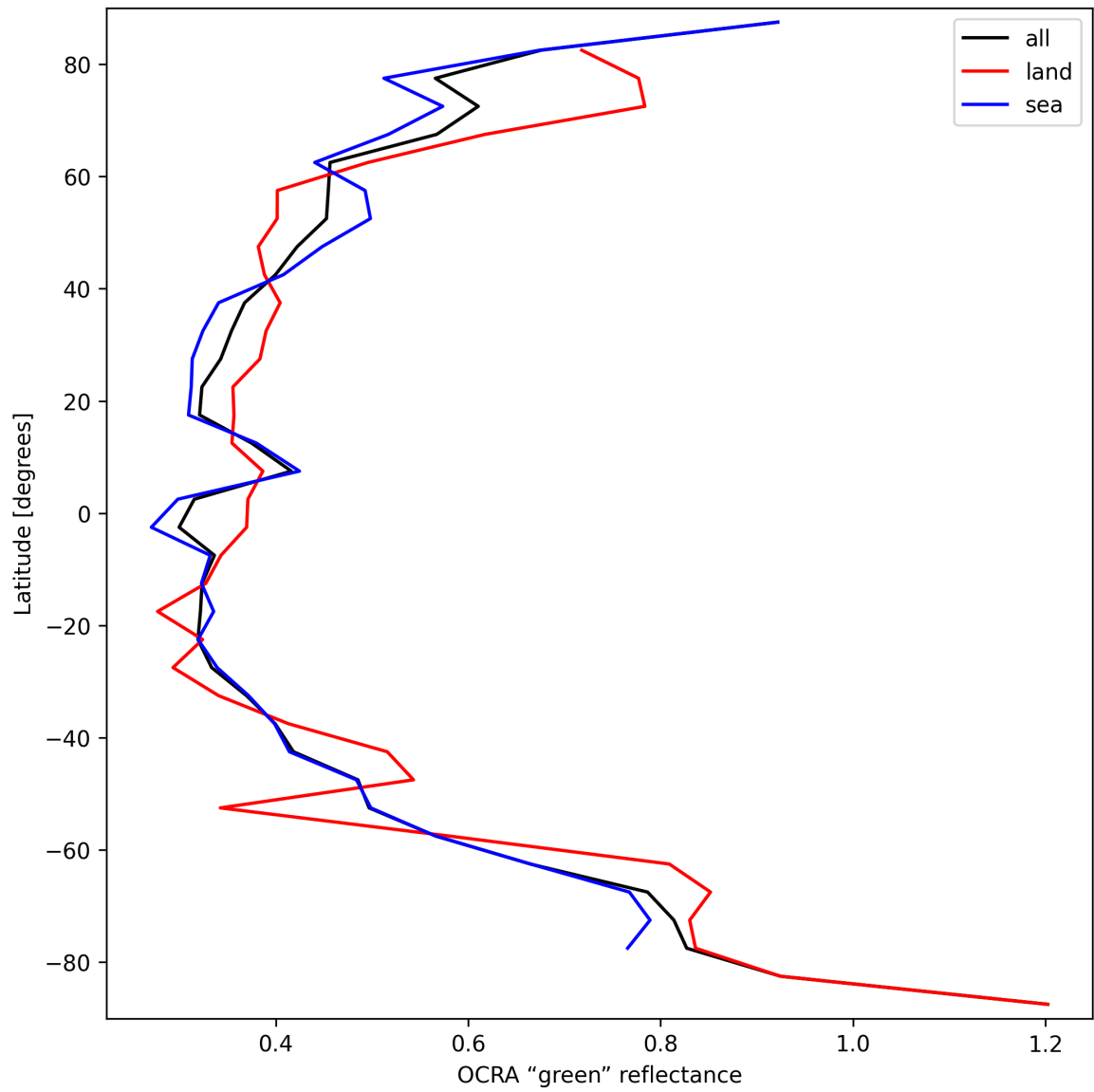
Figure 34: Zonal average of “OCRA “green” reflectance” for 2025-09-18 to 2025-09-18.
