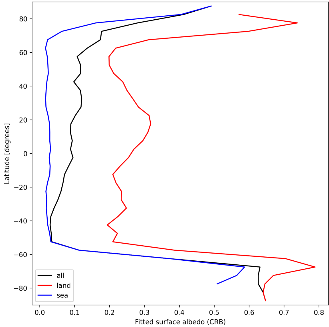
Figure 28: Zonal average of “Fitted surface albedo (CRB)” for 2025-09-18 to 2025-09-18.
