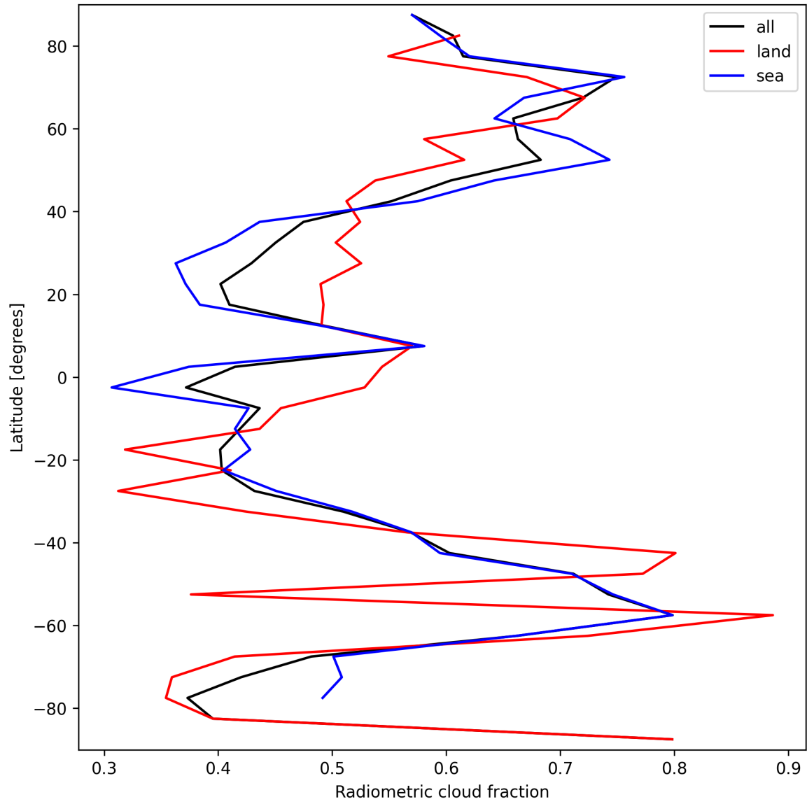
Figure 21: Zonal average of “Radiometric cloud fraction” for 2025-09-18 to 2025-09-18.
