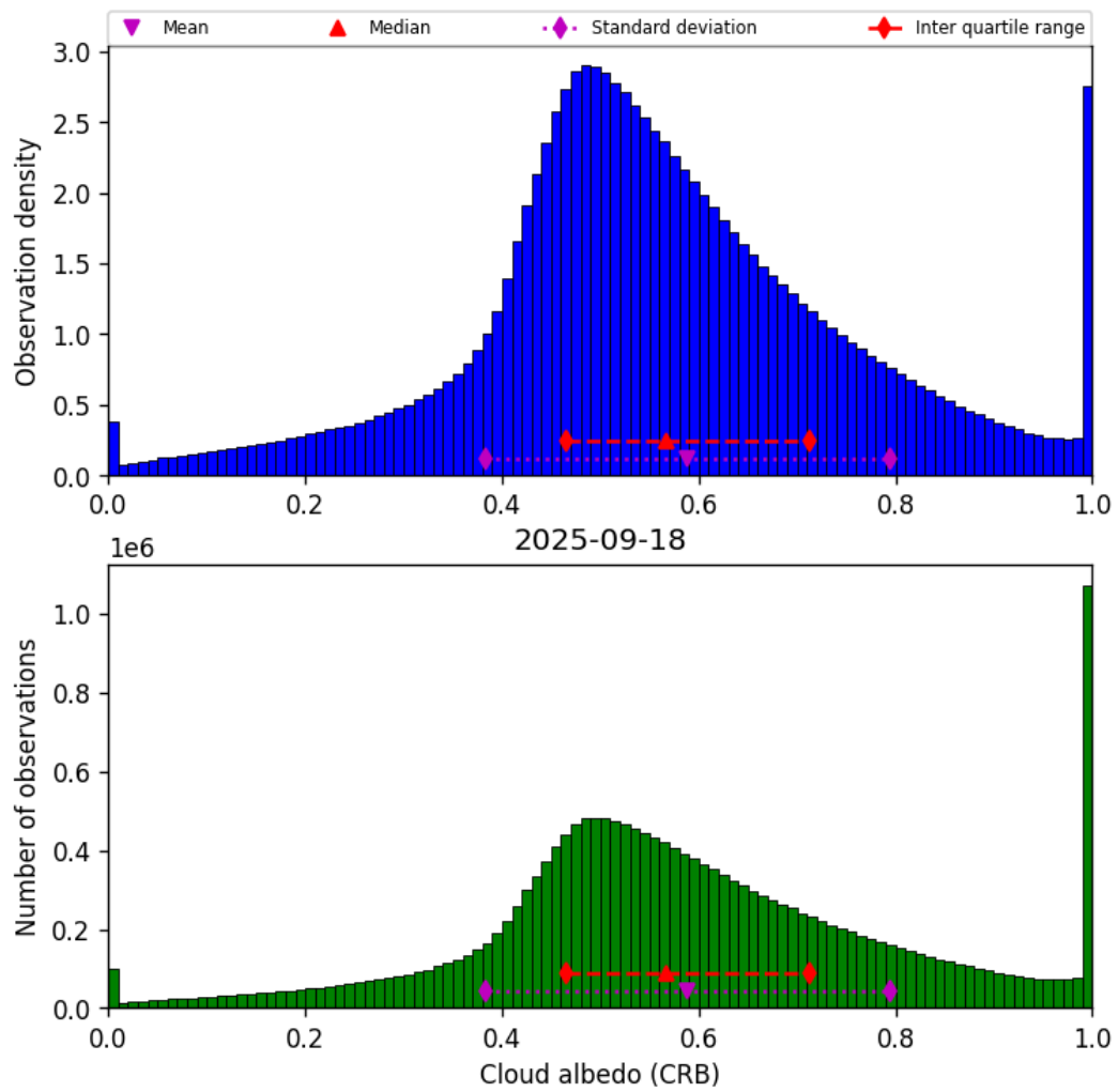
Figure 42: Histogram of “Cloud albedo (CRB)” for 2025-09-18 to 2025-09-18
