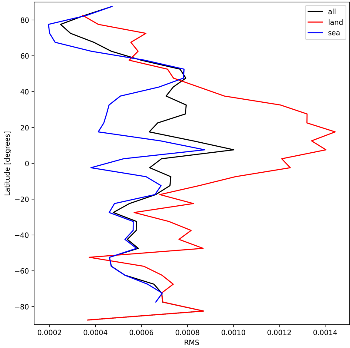
Figure 29: Zonal average of “RMS” for 2025-09-18 to 2025-09-18.
