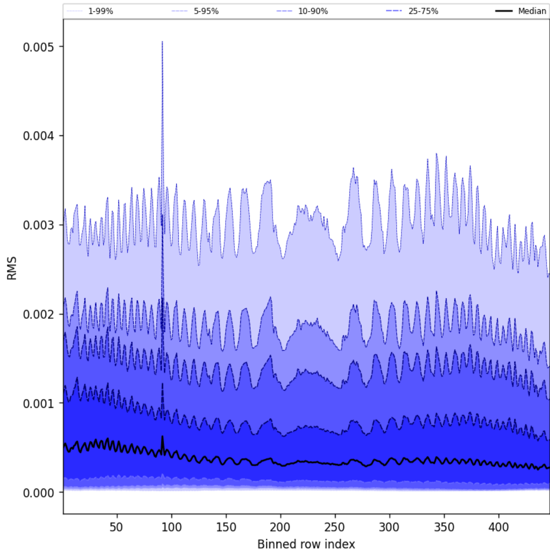
Figure 61: Along track statistics of “RMS” for 2025-09-18 to 2025-09-18
