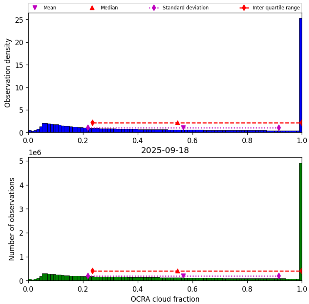
Figure 48: Histogram of “OCRA cloud fraction” for 2025-09-18 to 2025-09-18
