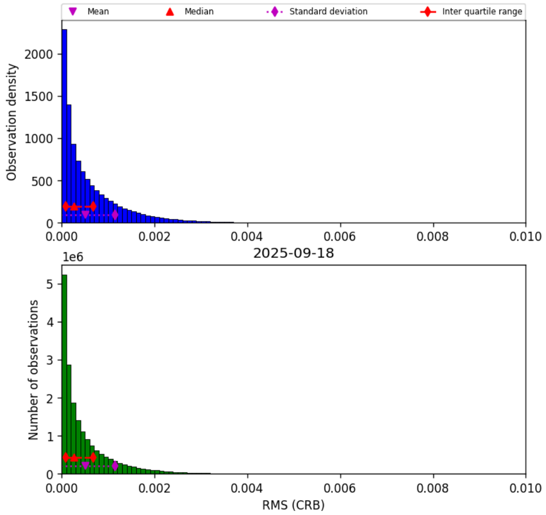
Figure 46: Histogram of “RMS (CRB)” for 2025-09-18 to 2025-09-18
