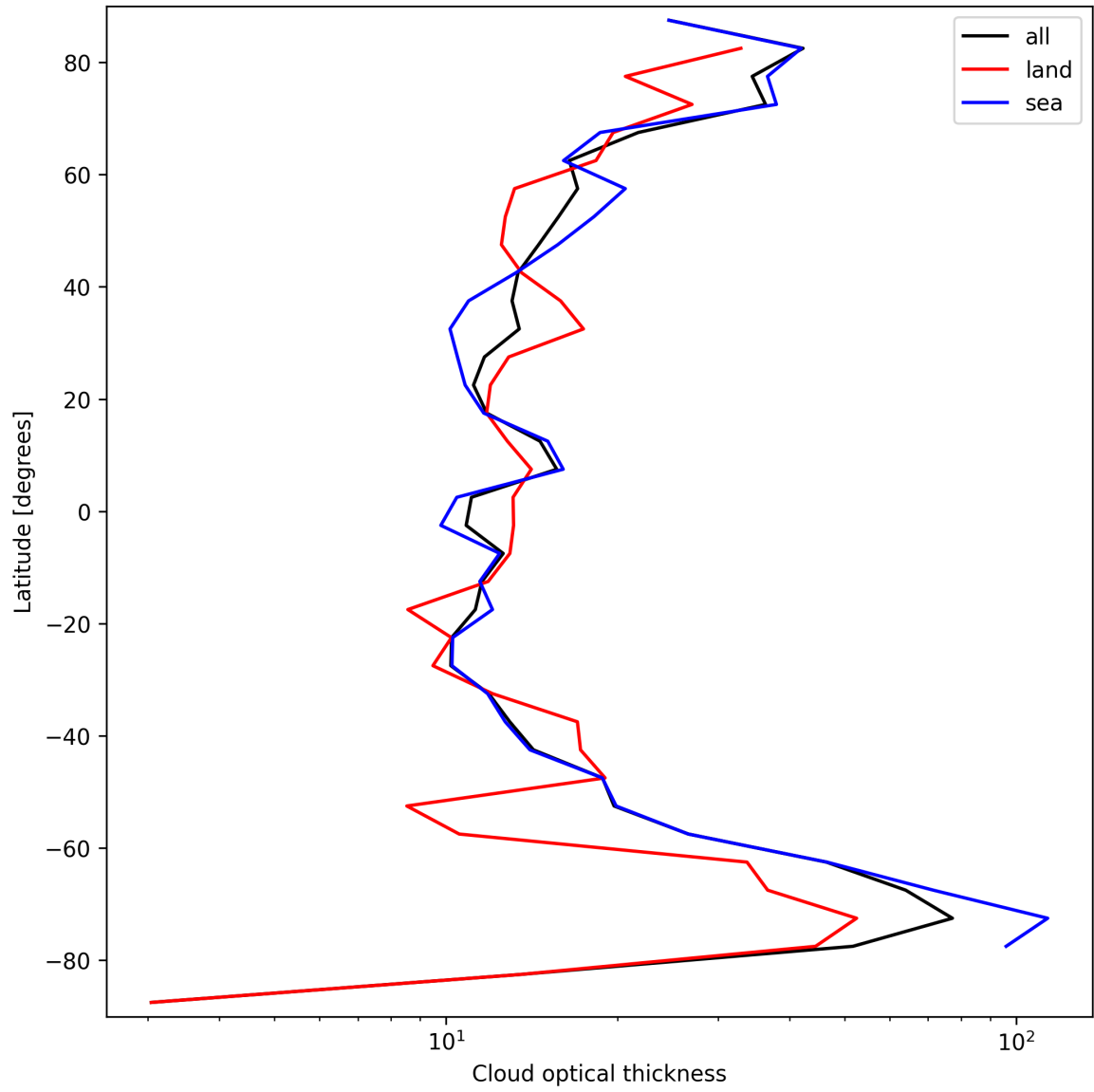
Figure 23: Zonal average of “Cloud optical thickness” for 2025-09-18 to 2025-09-18.
