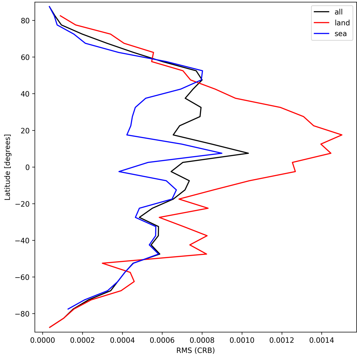
Figure 30: Zonal average of “RMS (CRB)” for 2025-09-18 to 2025-09-18.
