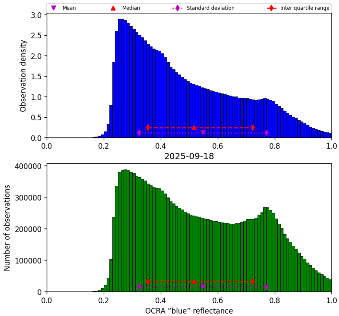
Figure 49: Histogram of “OCRA “blue” reflectance” for 2025-09-18 to 2025-09-18
