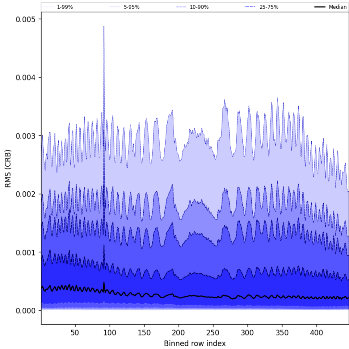
Figure 62: Along track statistics of “RMS (CRB)” for 2025-09-18 to 2025-09-18
