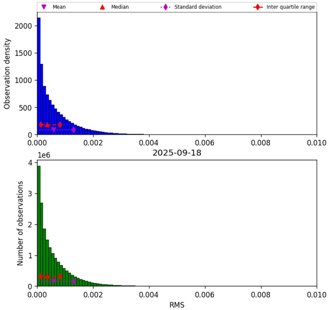
Figure 45: Histogram of “RMS” for 2025-09-18 to 2025-09-18
