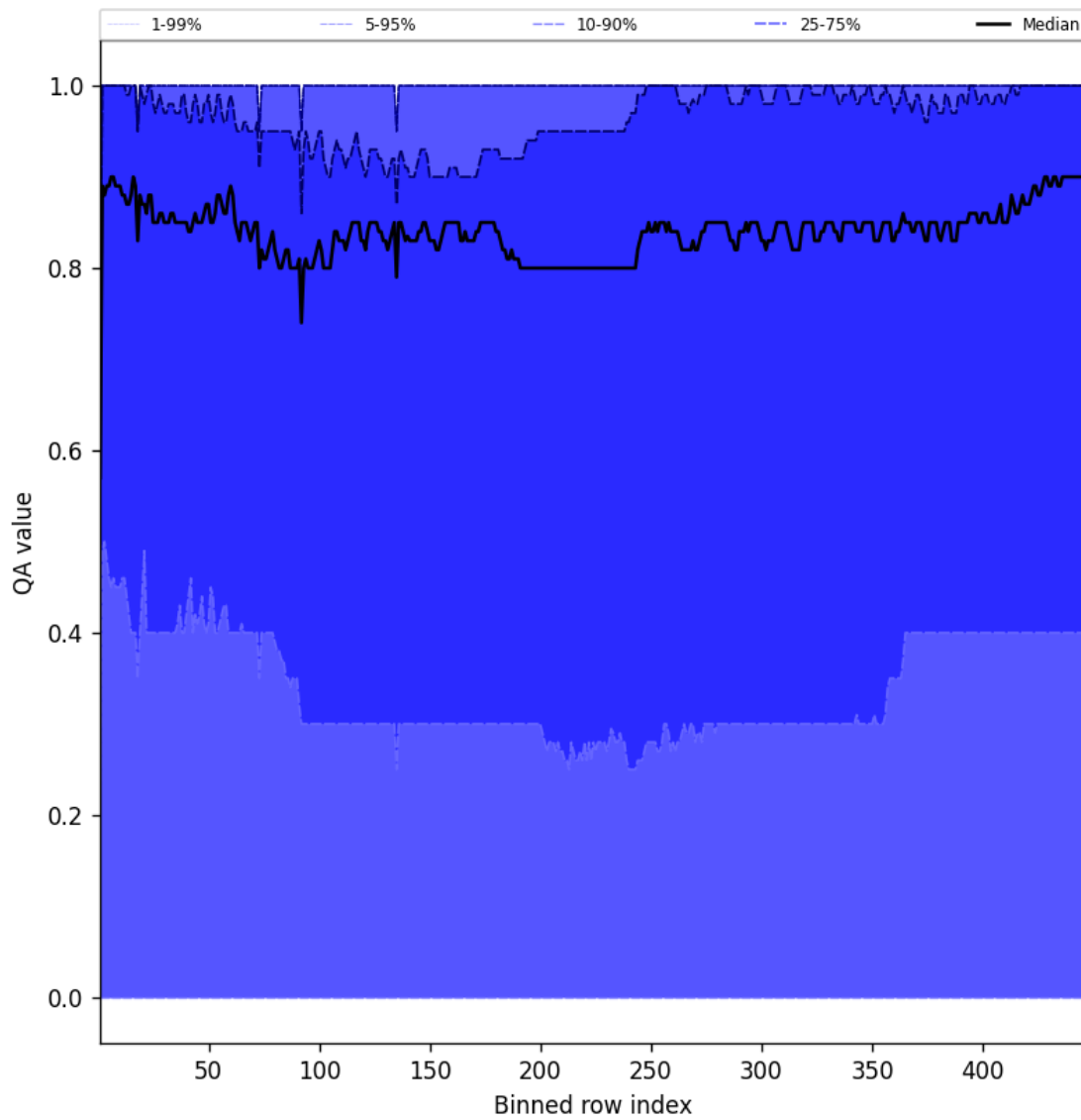
Figure 52: Along track statistics of “QA value” for 2025-09-18 to 2025-09-18
