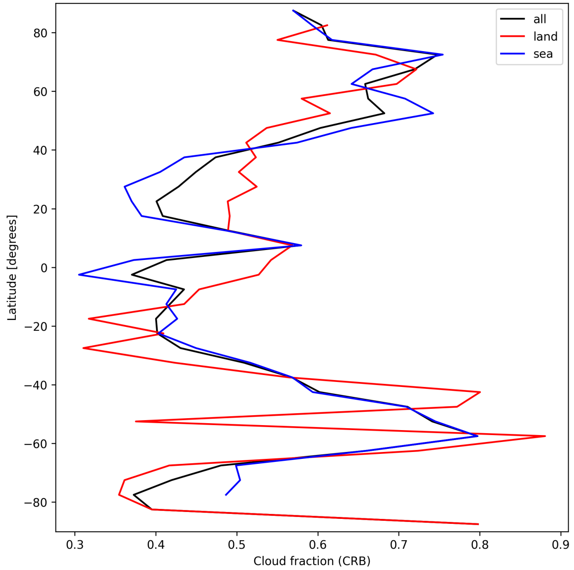
Figure 24: Zonal average of “Cloud fraction (CRB)” for 2025-09-18 to 2025-09-18.
