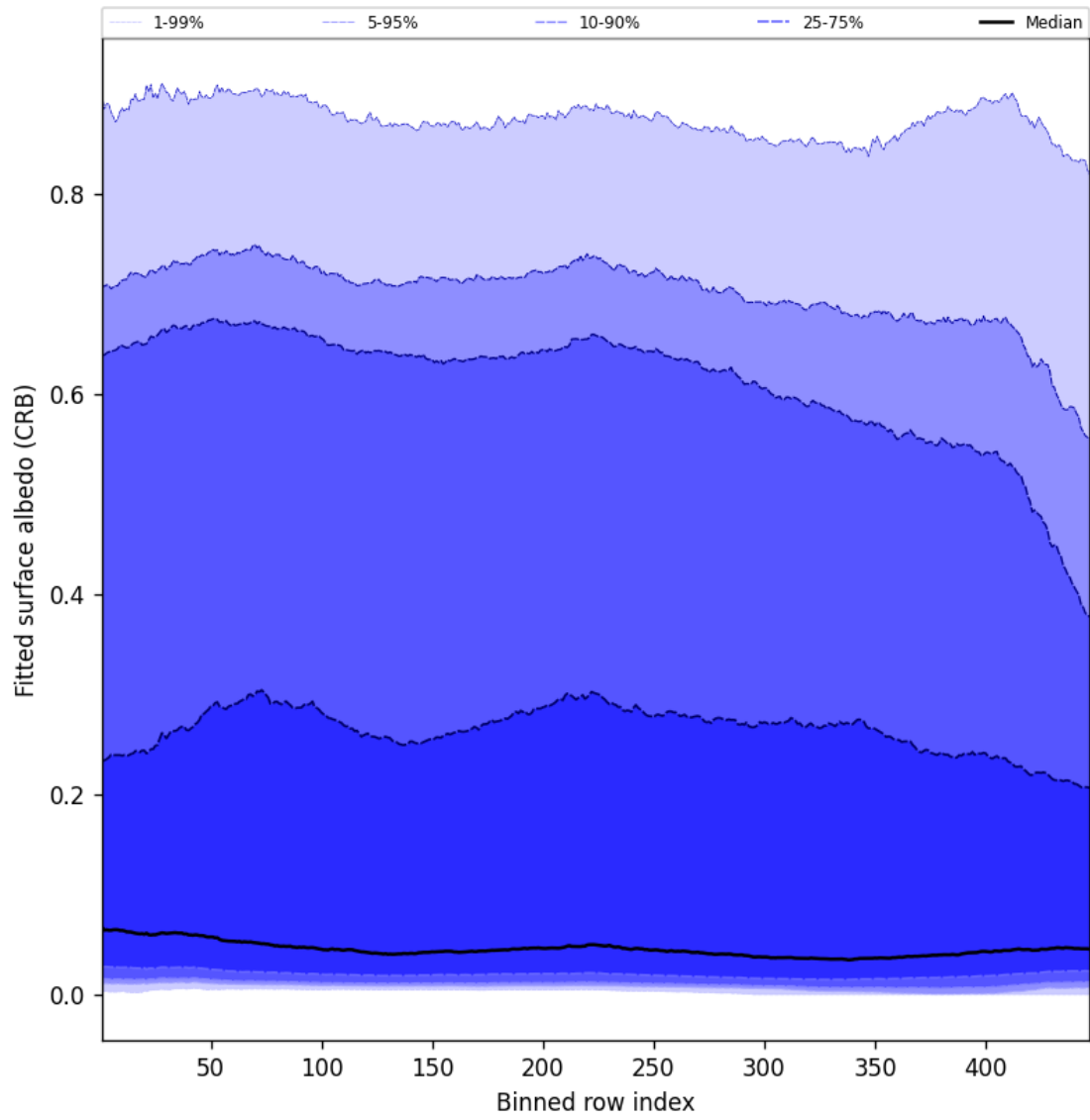
Figure 60: Along track statistics of “Fitted surface albedo (CRB)” for 2025-09-18 to 2025-09-18
