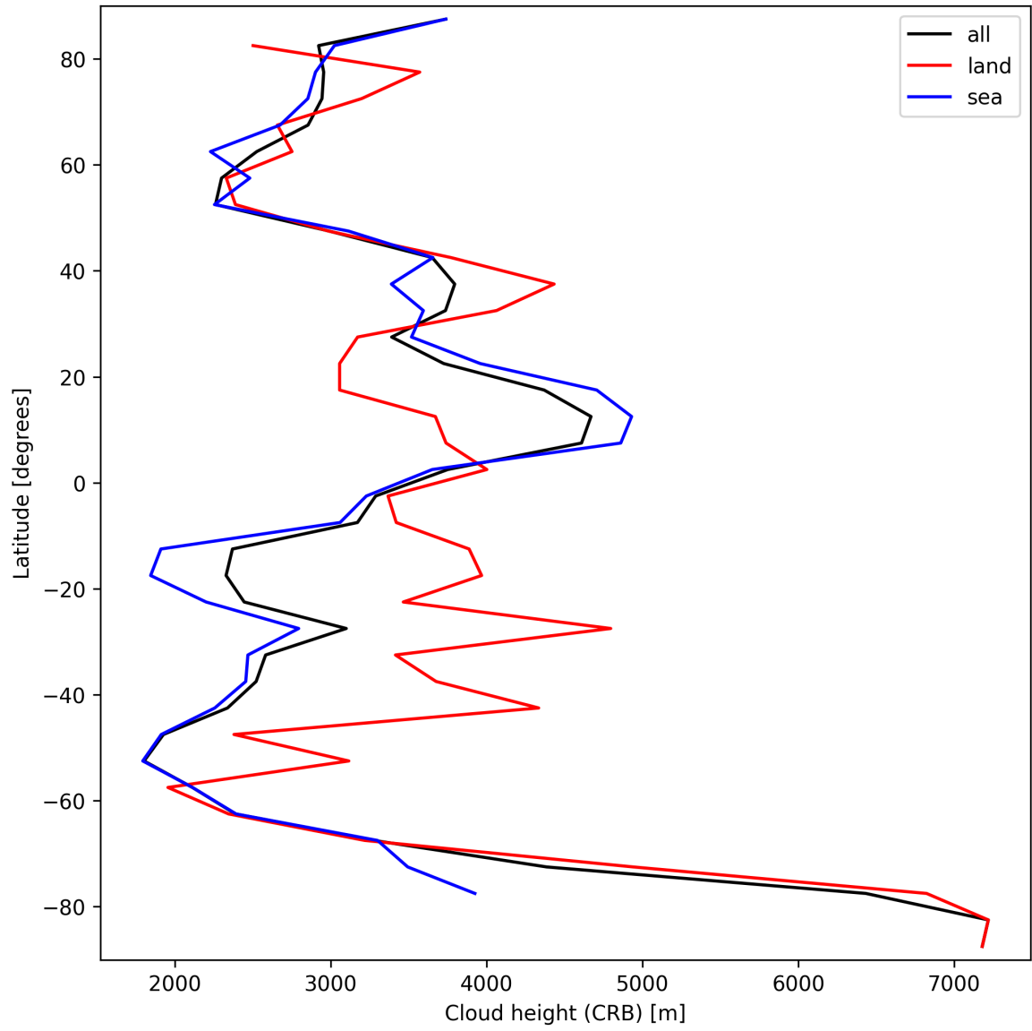
Figure 25: Zonal average of “Cloud height (CRB)” for 2025-09-18 to 2025-09-18.
