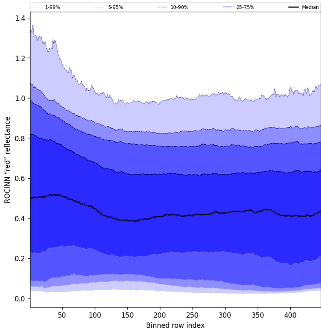
Figure 67: Along track statistics of "ROCINN "red" reflectance" for 2025-09-18 to 2025-09-18
