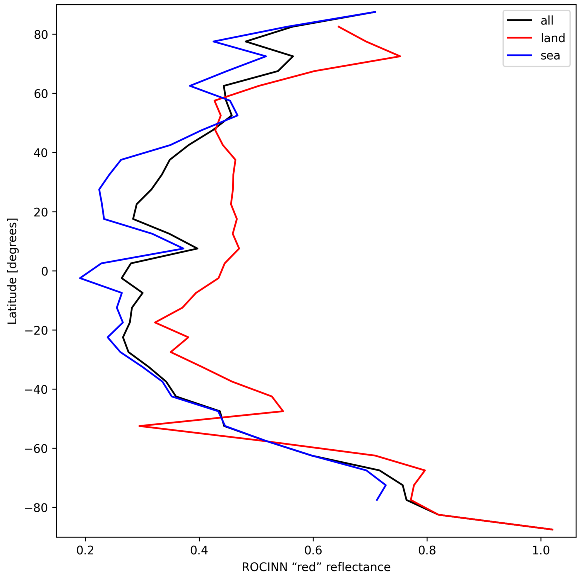
Figure 35: Zonal average of “ROCINN “red” reflectance” for 2025-09-18 to 2025-09-18.
