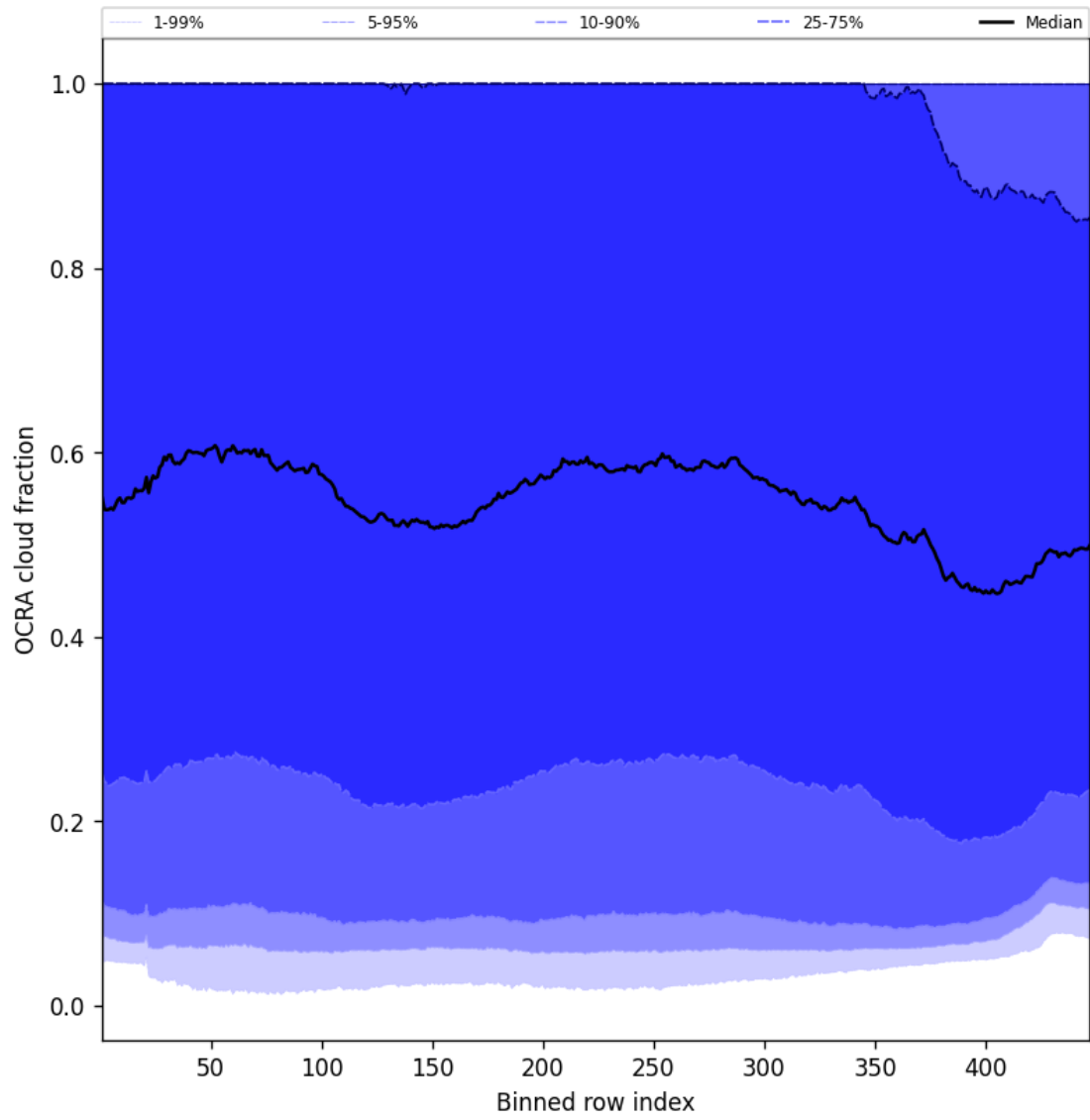
Figure 64: Along track statistics of “OCRA cloud fraction” for 2025-09-18 to 2025-09-18
