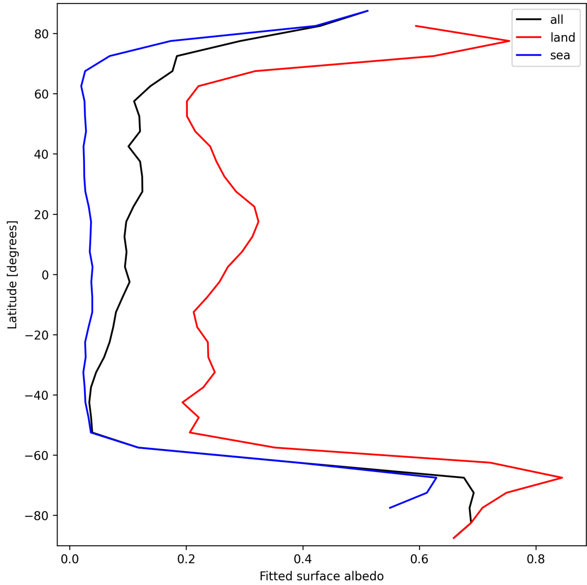
Figure 27: Zonal average of “Fitted surface albedo” for 2025-09-18 to 2025-09-18.
