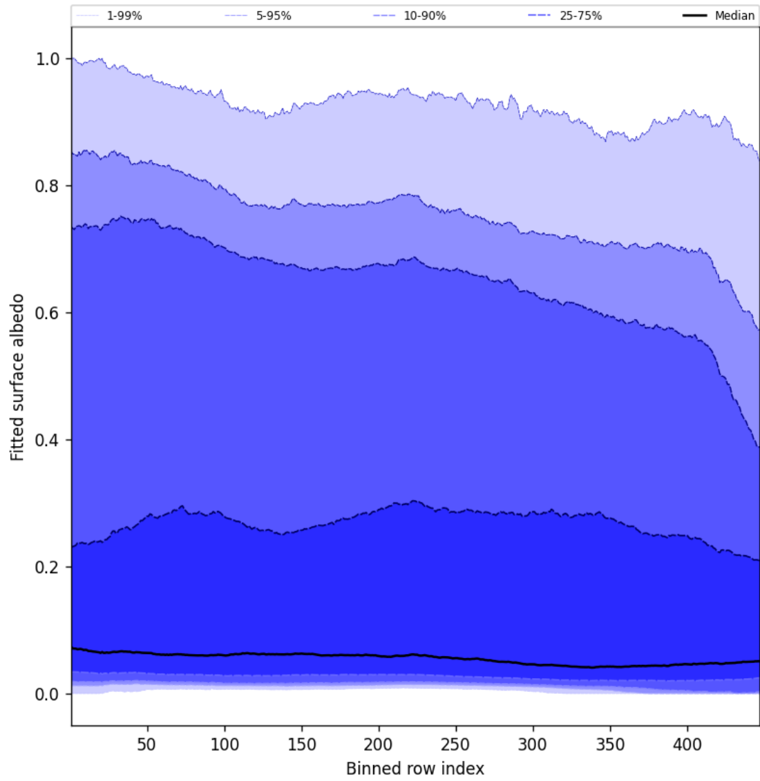
Figure 59: Along track statistics of “Fitted surface albedo” for 2025-09-18 to 2025-09-18
