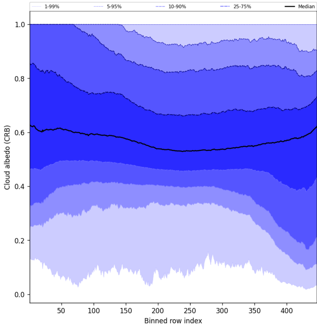
Figure 58: Along track statistics of “Cloud albedo (CRB)” for 2025-09-18 to 2025-09-18
