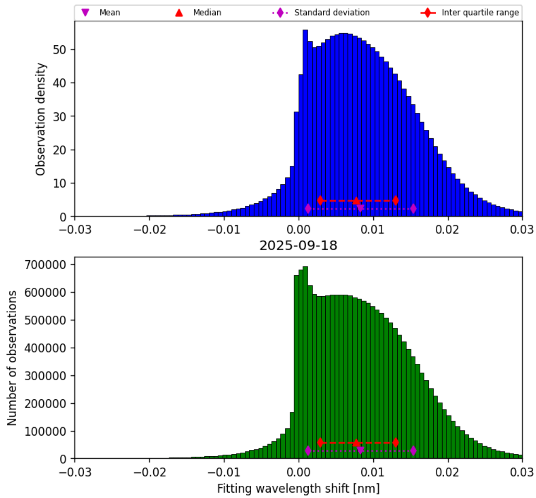
Figure 47: Histogram of “Fitting wavelength shift” for 2025-09-18 to 2025-09-18
