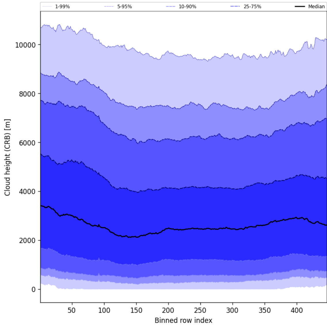
Figure 57: Along track statistics of “Cloud height (CRB)” for 2025-09-18 to 2025-09-18
