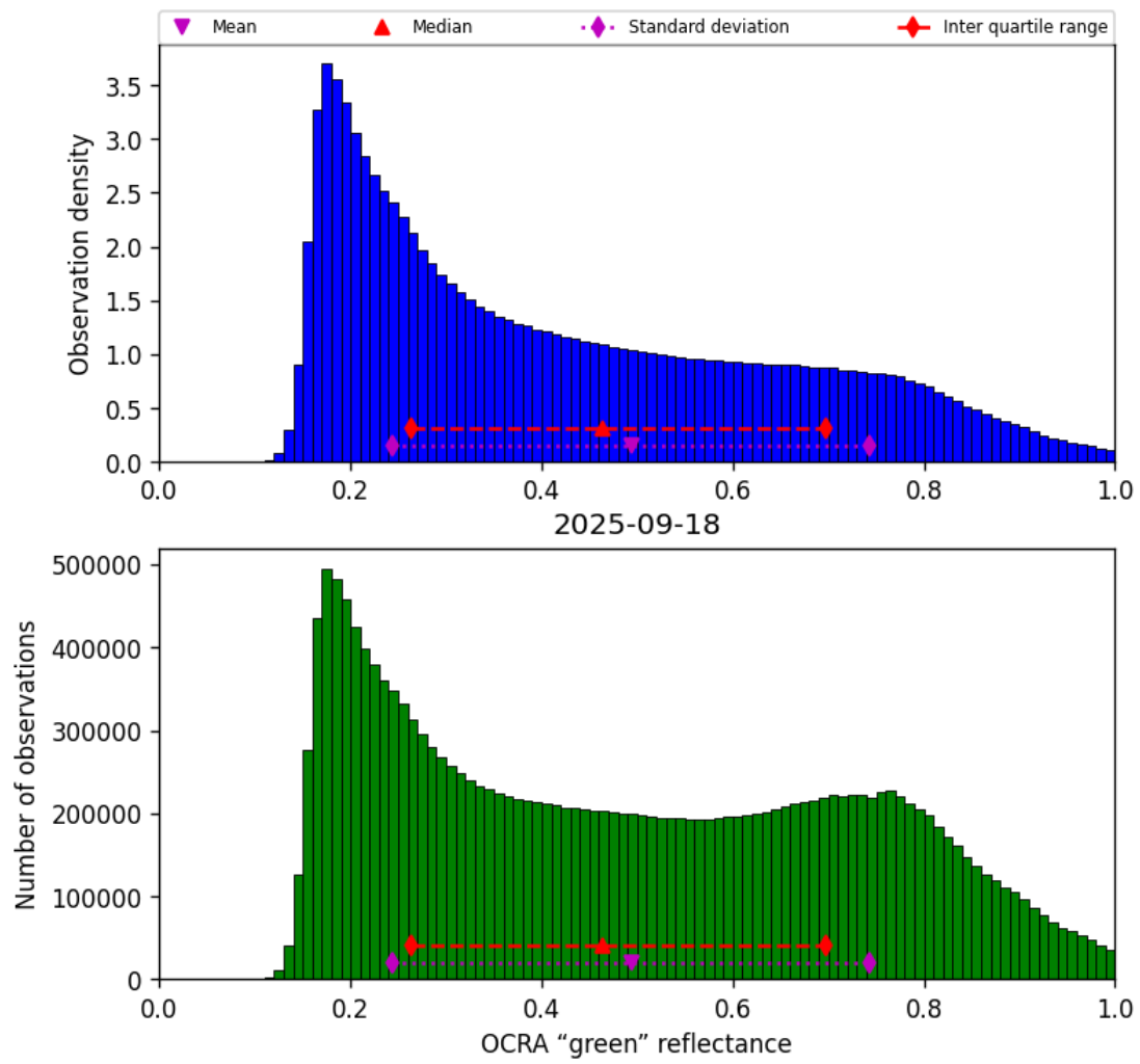
Figure 50: Histogram of “OCRA “green” reflectance” for 2025-09-18 to 2025-09-18
