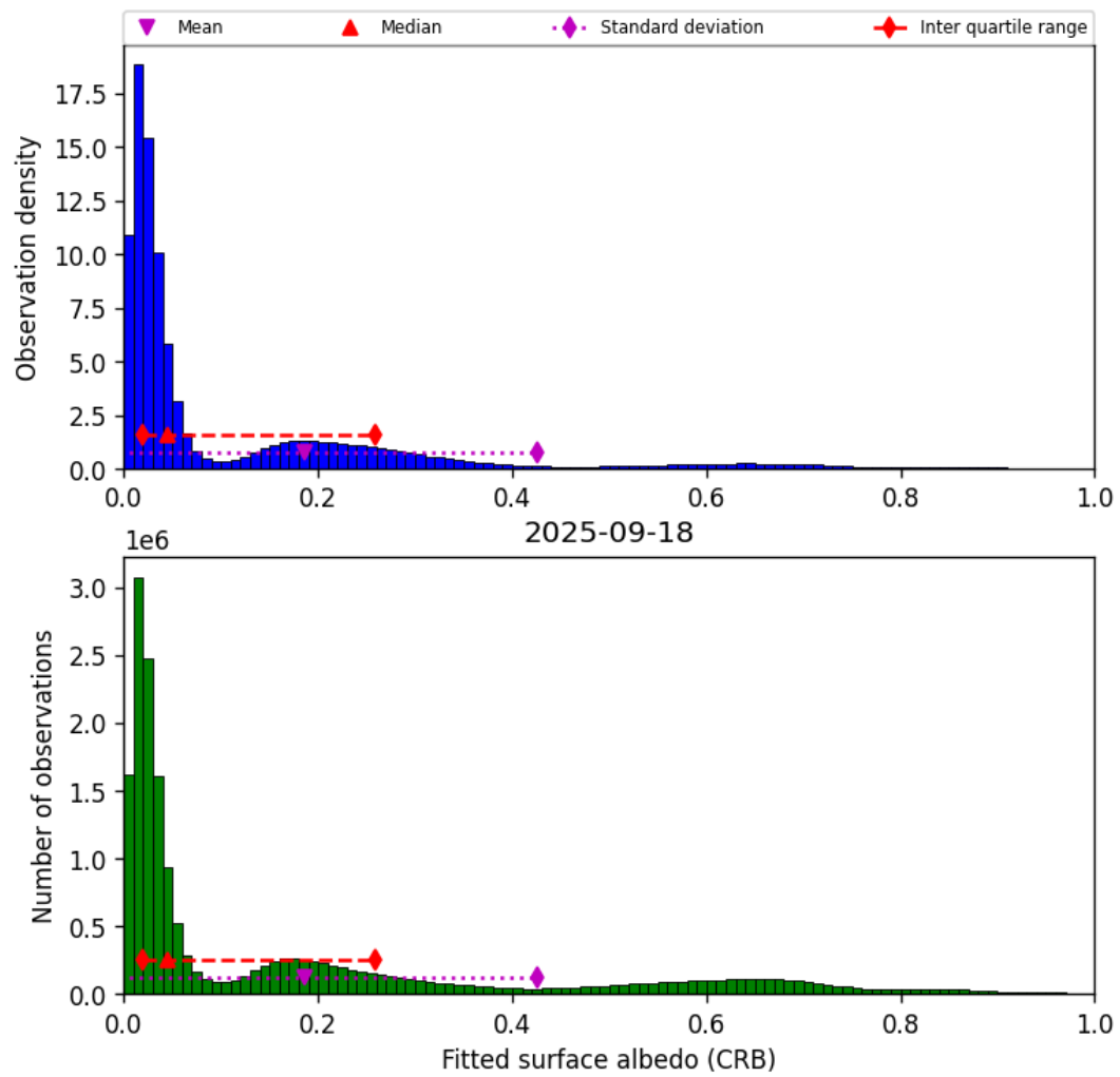
Figure 44: Histogram of “Fitted surface albedo (CRB)” for 2025-09-18 to 2025-09-18
