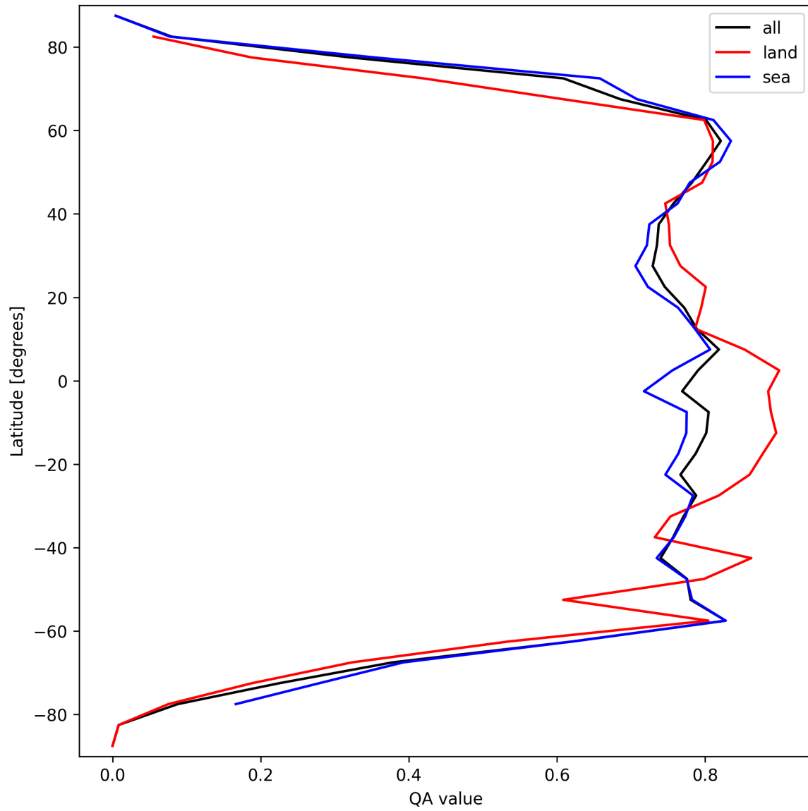
Figure 20: Zonal average of “QA value” for 2025-09-18 to 2025-09-18.
