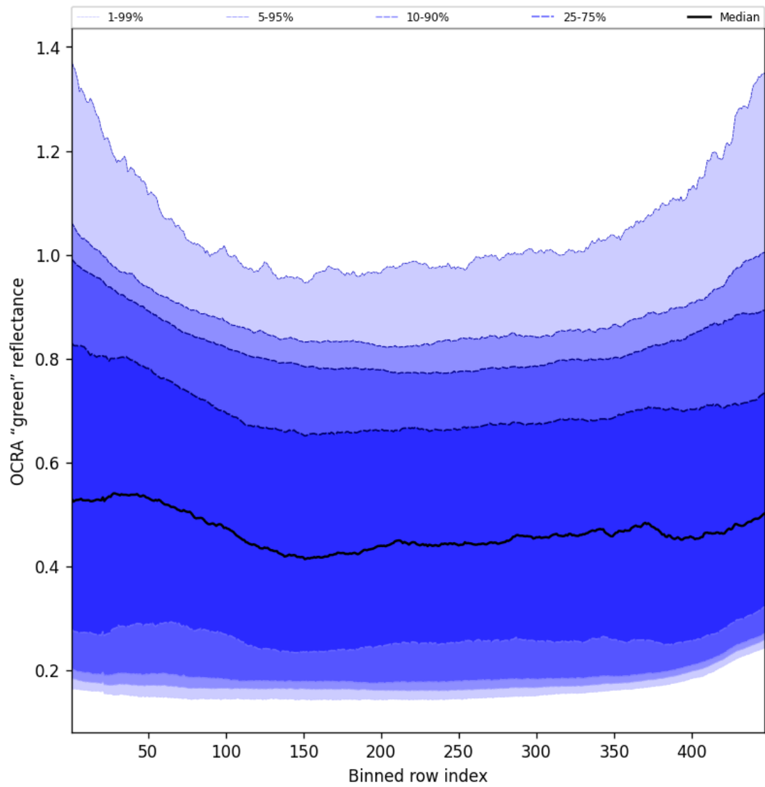
Figure 66: Along track statistics of “OCRA “green” reflectance” for 2025-09-18 to 2025-09-18
