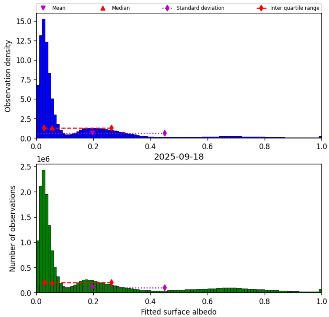
Figure 43: Histogram of “Fitted surface albedo” for 2025-09-18 to 2025-09-18
