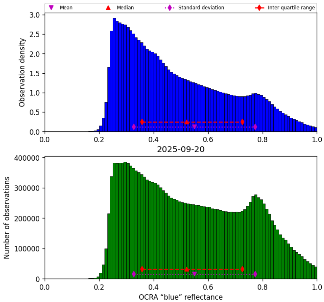
Figure 49: Histogram of “OCRA “blue” reflectance” for 2025-09-20 to 2025-09-21
