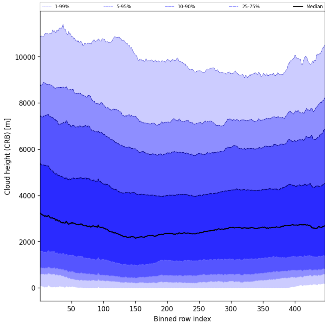
Figure 57: Along track statistics of “Cloud height (CRB)” for 2025-09-20 to 2025-09-21
