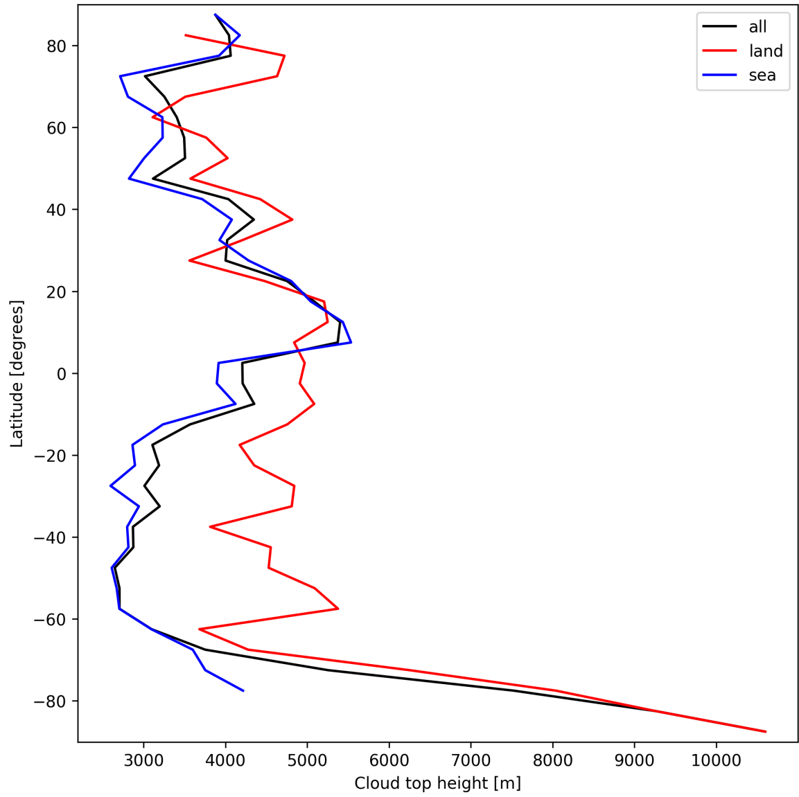
Figure 22: Zonal average of “Cloud top height” for 2025-09-20 to 2025-09-21.
