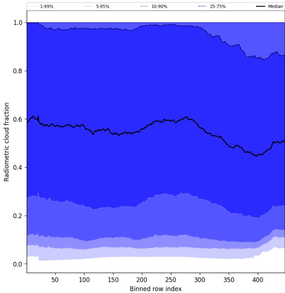
Figure 53: Along track statistics of “Radiometric cloud fraction” for 2025-09-20 to 2025-09-21
