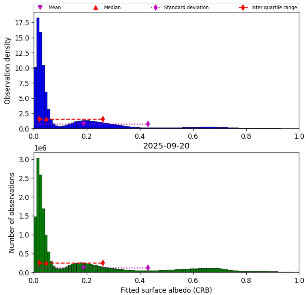
Figure 44: Histogram of “Fitted surface albedo (CRB)” for 2025-09-20 to 2025-09-21
