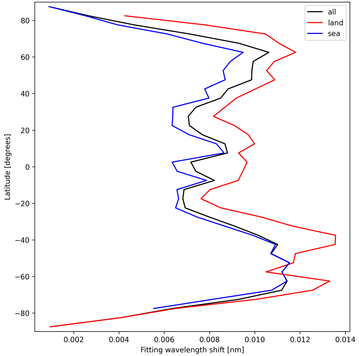
Figure 31: Zonal average of “Fitting wavelength shift” for 2025-09-20 to 2025-09-21.
