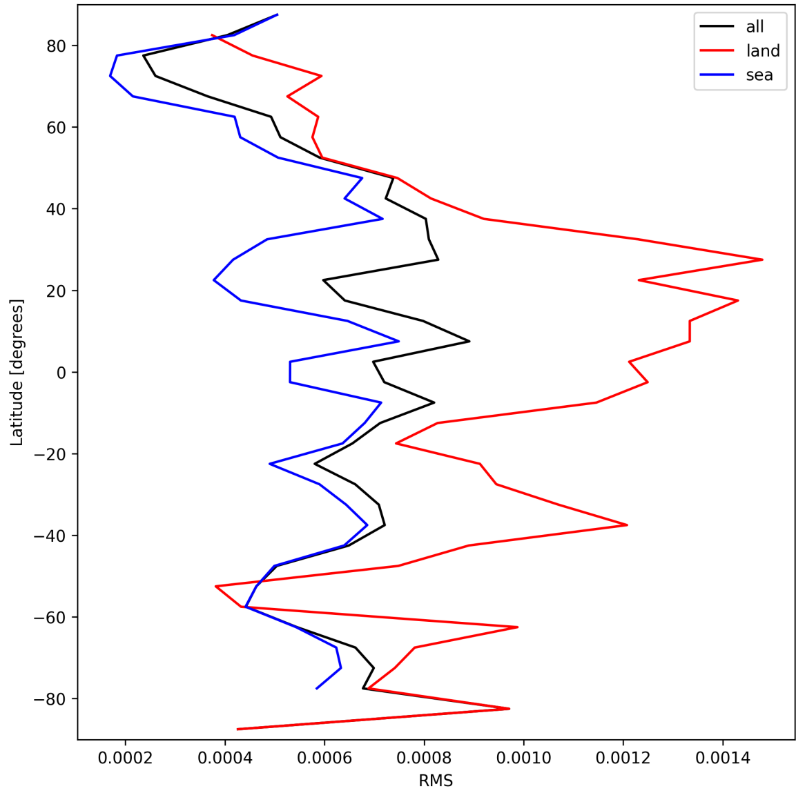
Figure 29: Zonal average of “RMS” for 2025-09-20 to 2025-09-21.
