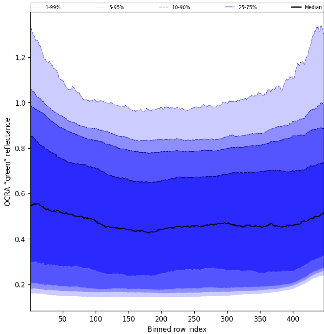
Figure 66: Along track statistics of “OCRA “green” reflectance” for 2025-09-20 to 2025-09-21
