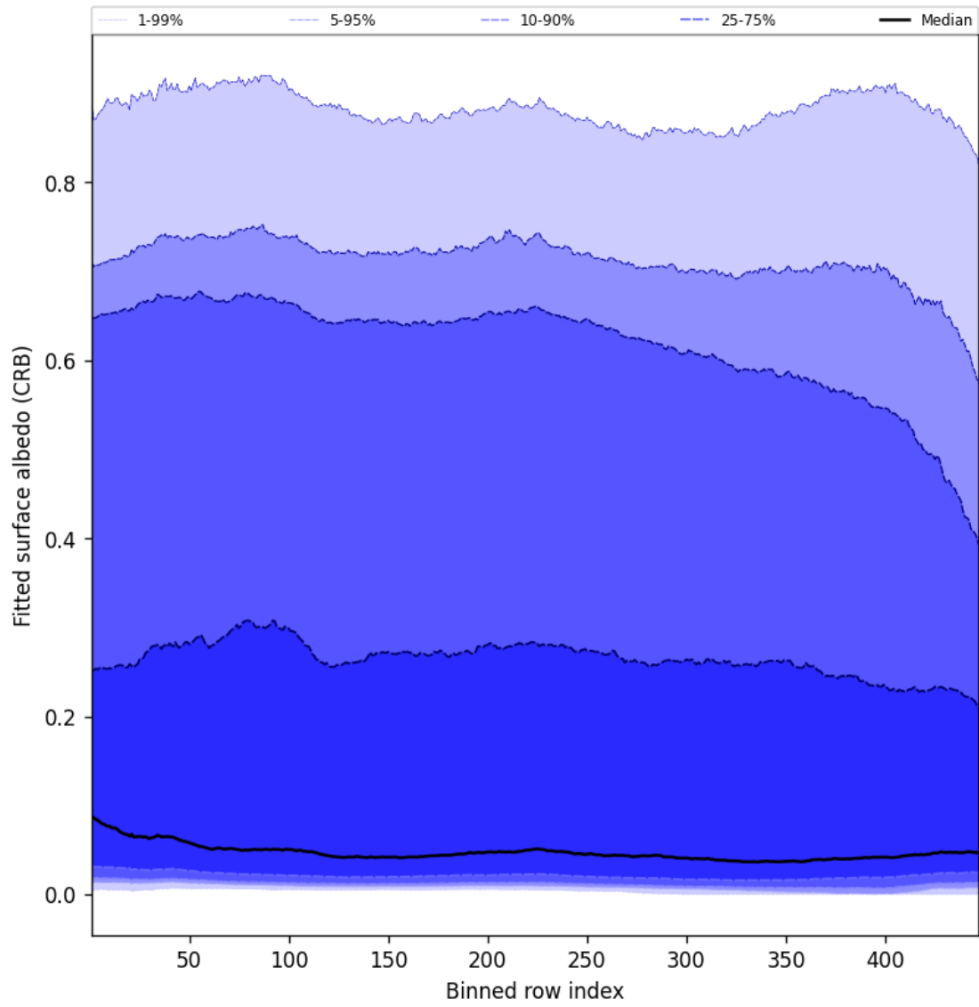
Figure 60: Along track statistics of “Fitted surface albedo (CRB)” for 2025-09-20 to 2025-09-21
