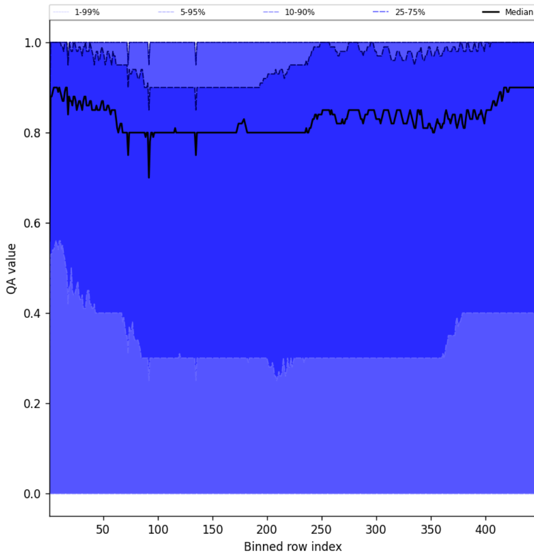
Figure 52: Along track statistics of “QA value” for 2025-09-20 to 2025-09-21
