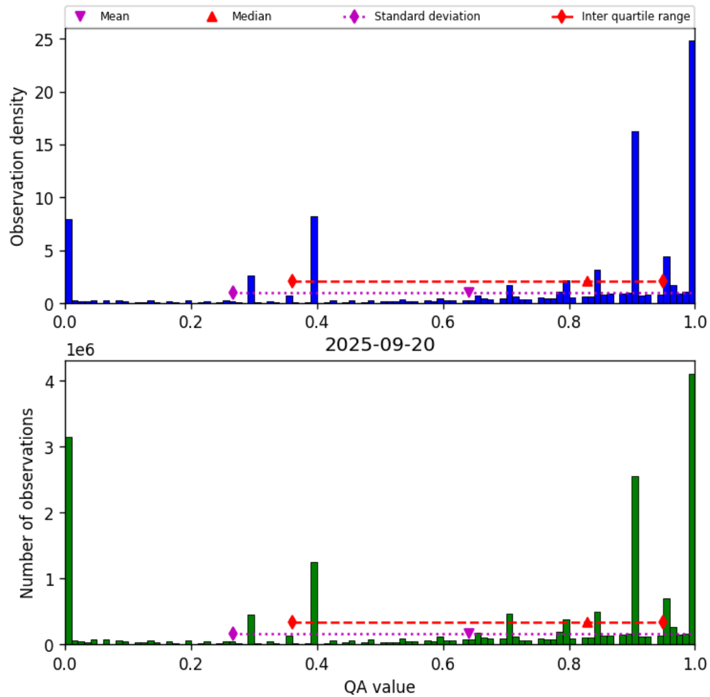
Figure 36: Histogram of “QA value” for 2025-09-20 to 2025-09-21
