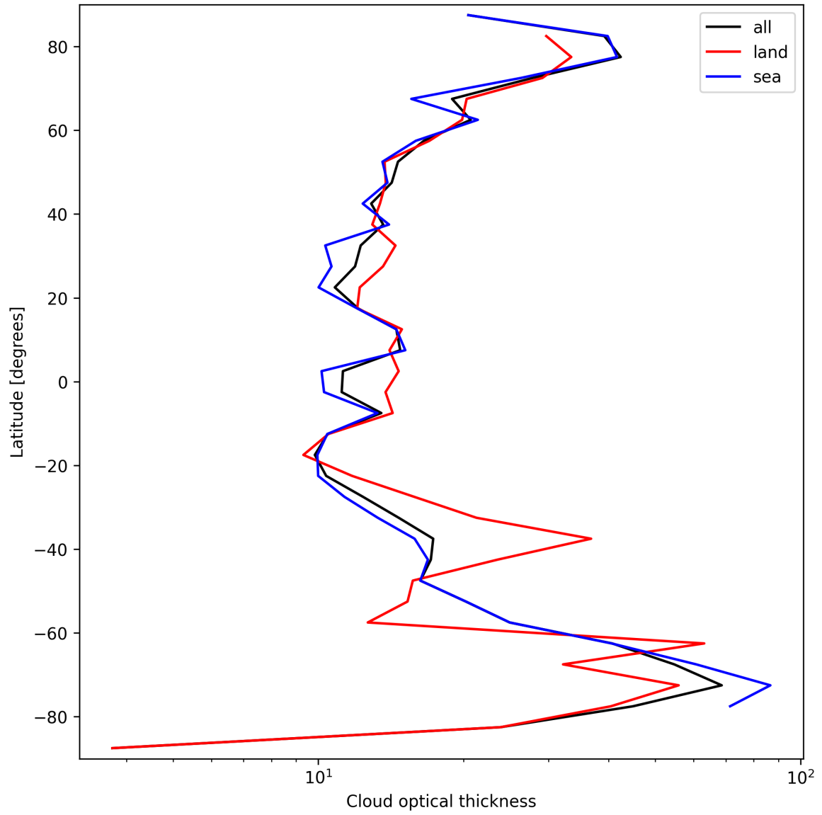
Figure 23: Zonal average of “Cloud optical thickness” for 2025-09-20 to 2025-09-21.
