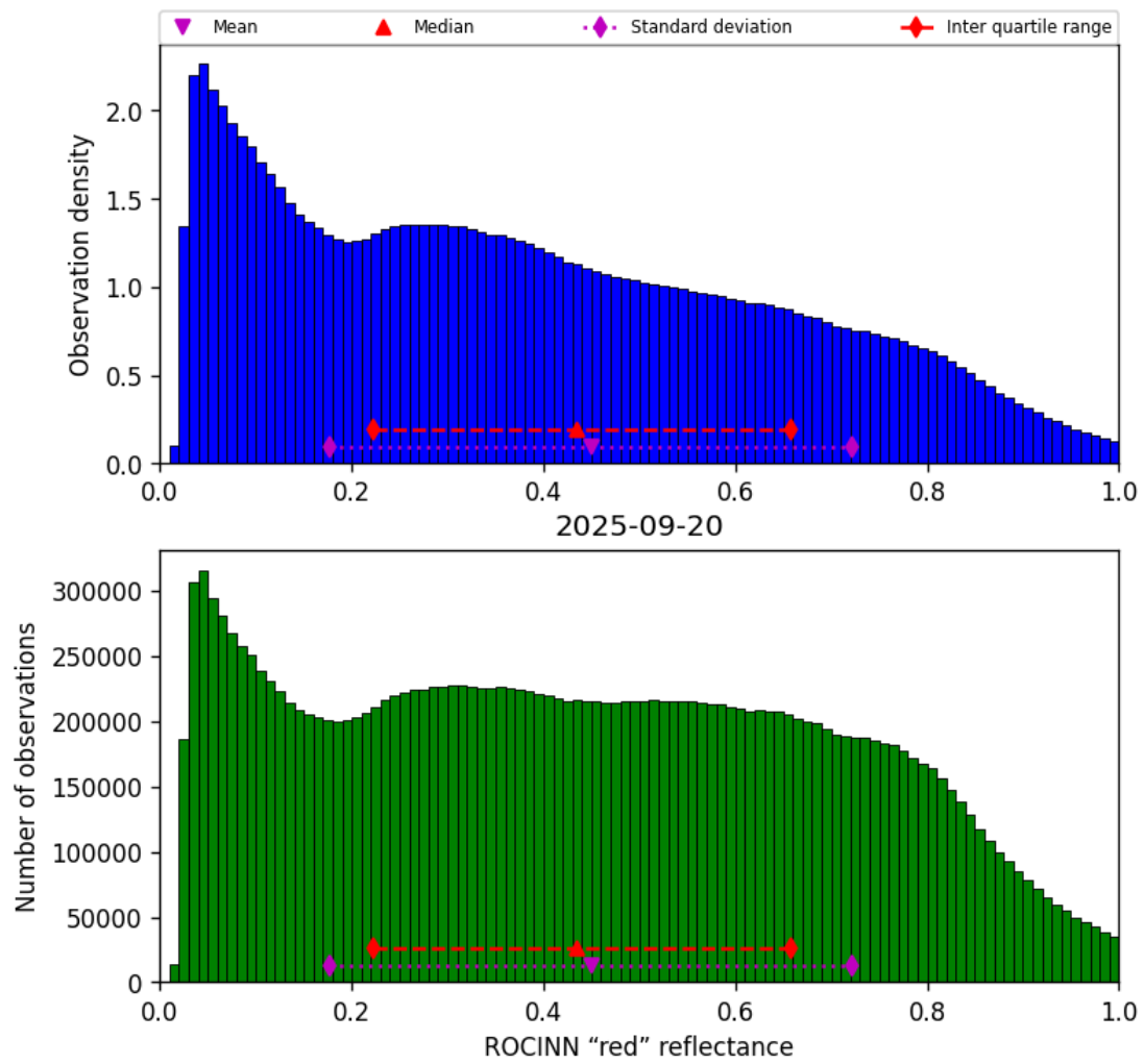
Figure 51: Histogram of “ROCINN “red” reflectance” for 2025-09-20 to 2025-09-21
