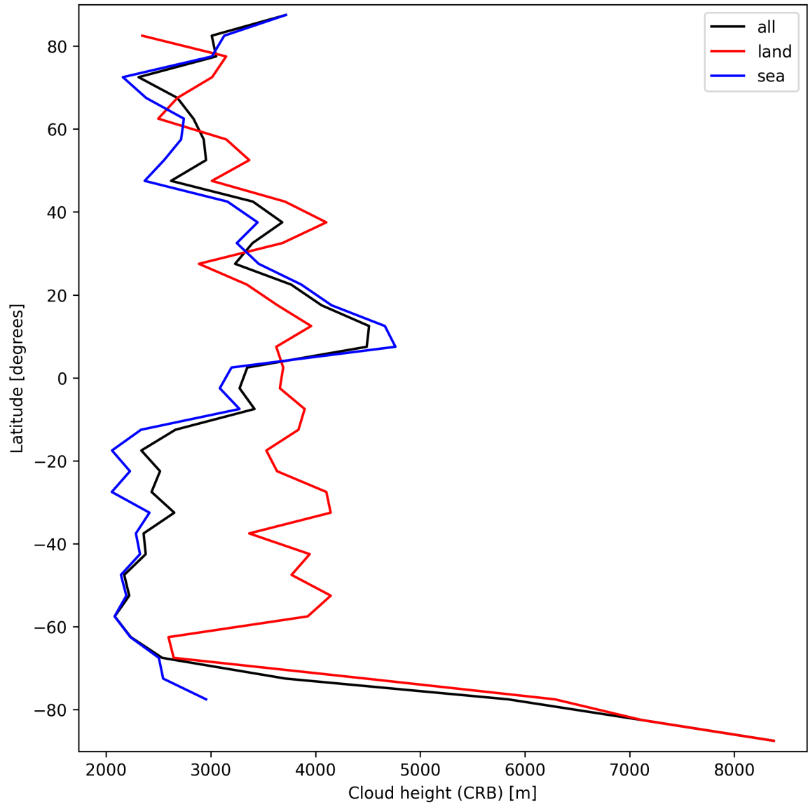
Figure 25: Zonal average of “Cloud height (CRB)” for 2025-09-20 to 2025-09-21.
