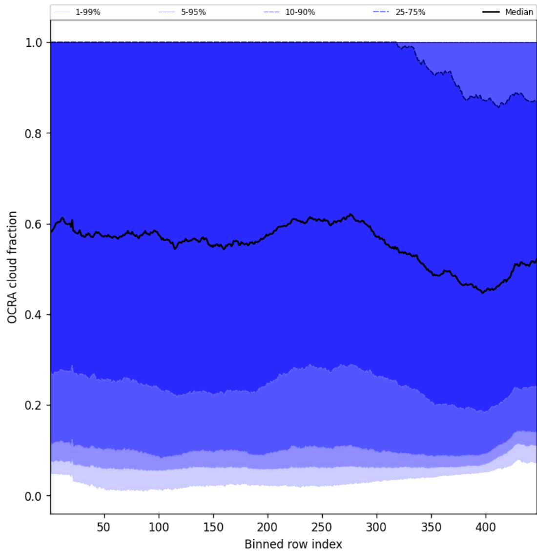
Figure 64: Along track statistics of “OCRA cloud fraction” for 2025-09-20 to 2025-09-21
