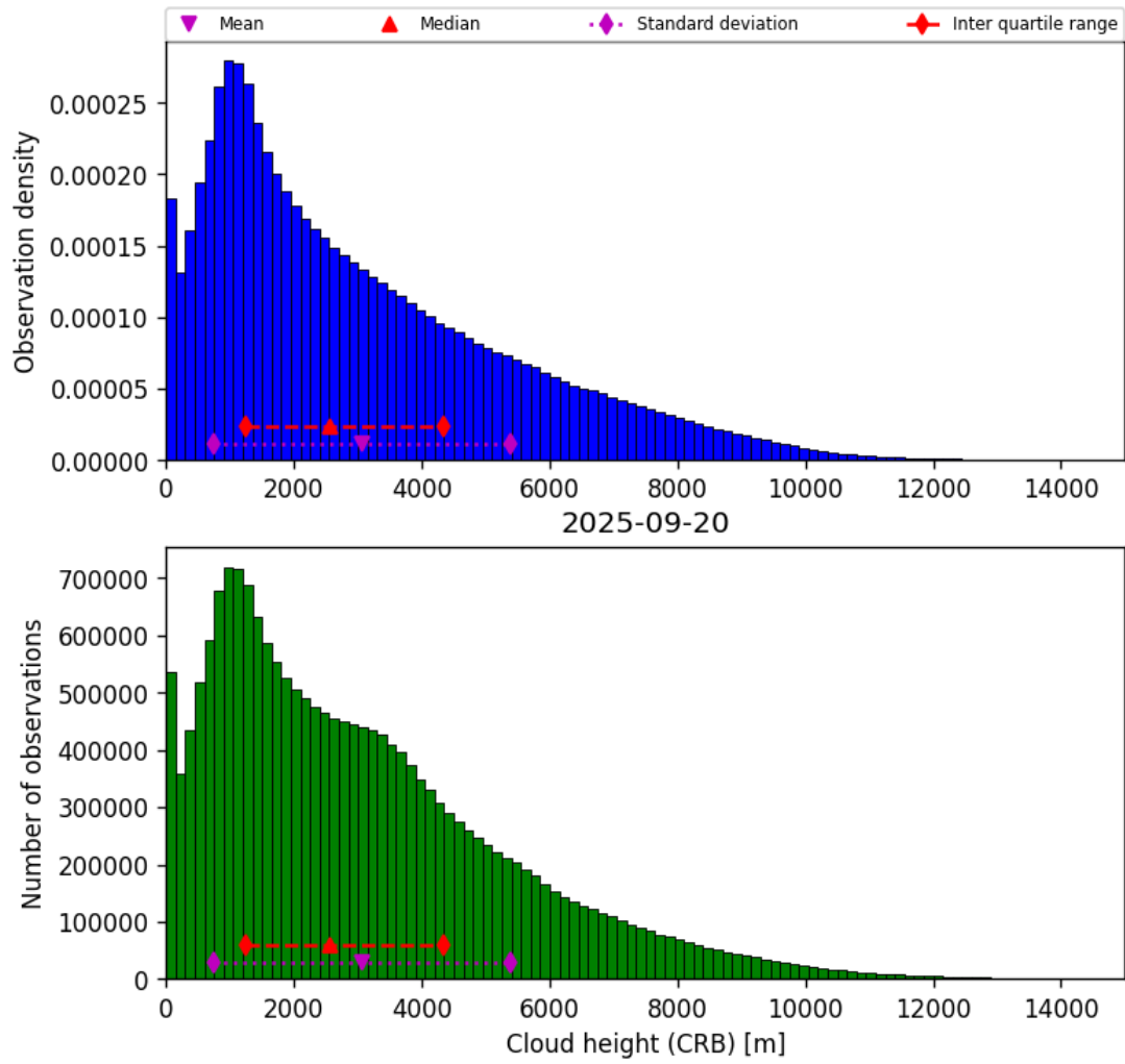
Figure 41: Histogram of “Cloud height (CRB)” for 2025-09-20 to 2025-09-21
