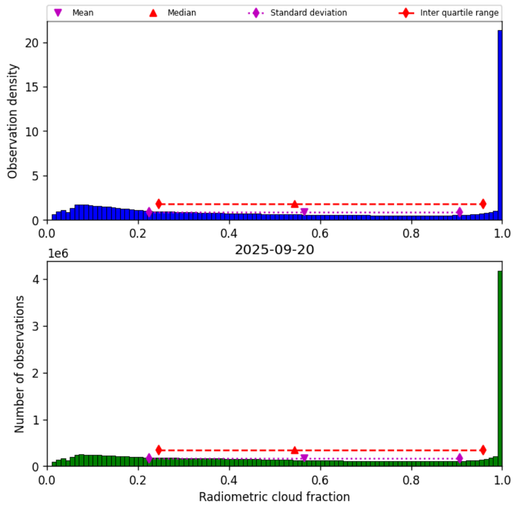
Figure 37: Histogram of “Radiometric cloud fraction” for 2025-09-20 to 2025-09-21
