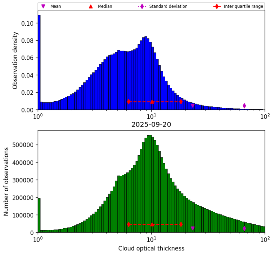
Figure 39: Histogram of “Cloud optical thickness” for 2025-09-20 to 2025-09-21
