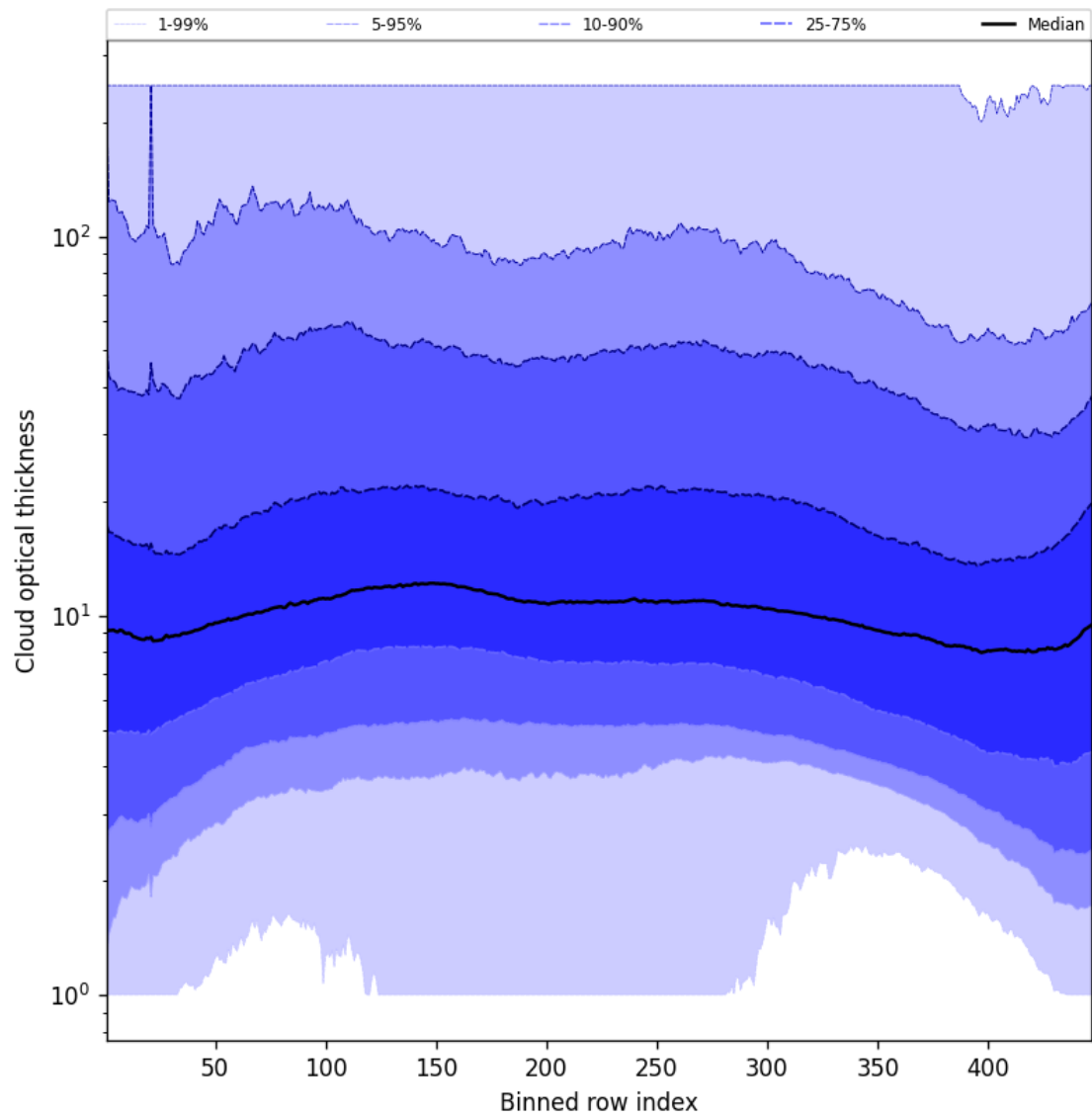
Figure 55: Along track statistics of “Cloud optical thickness” for 2025-09-20 to 2025-09-21
