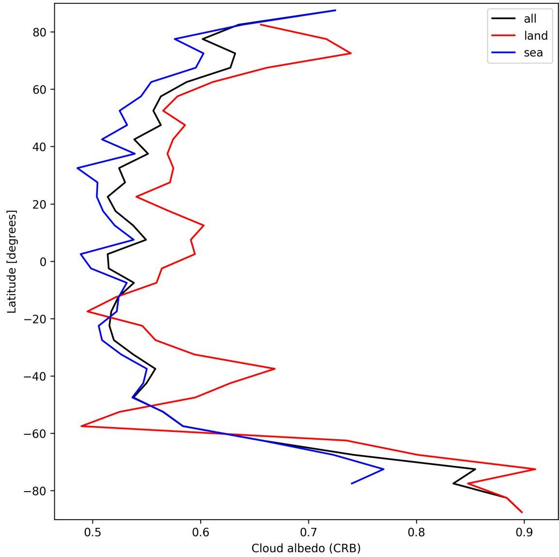
Figure 26: Zonal average of “Cloud albedo (CRB)” for 2025-09-20 to 2025-09-21.
