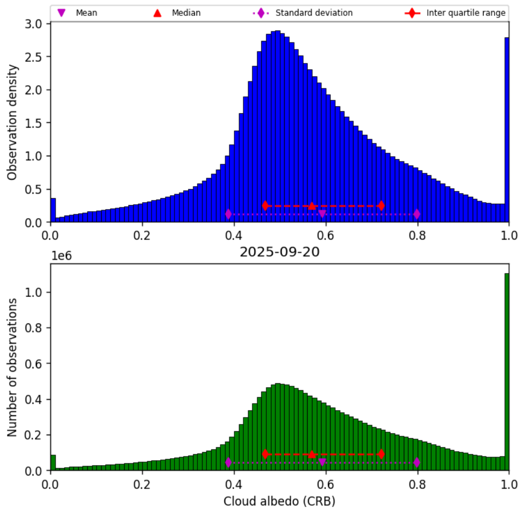
Figure 42: Histogram of “Cloud albedo (CRB)” for 2025-09-20 to 2025-09-21
