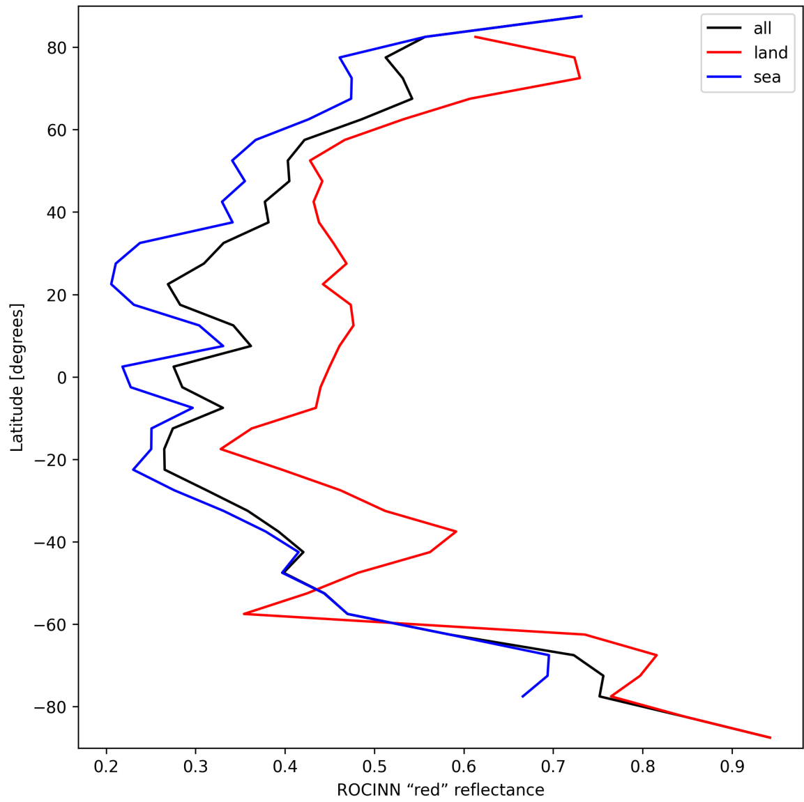
Figure 35: Zonal average of “ROCINN “red” reflectance” for 2025-09-20 to 2025-09-21.
