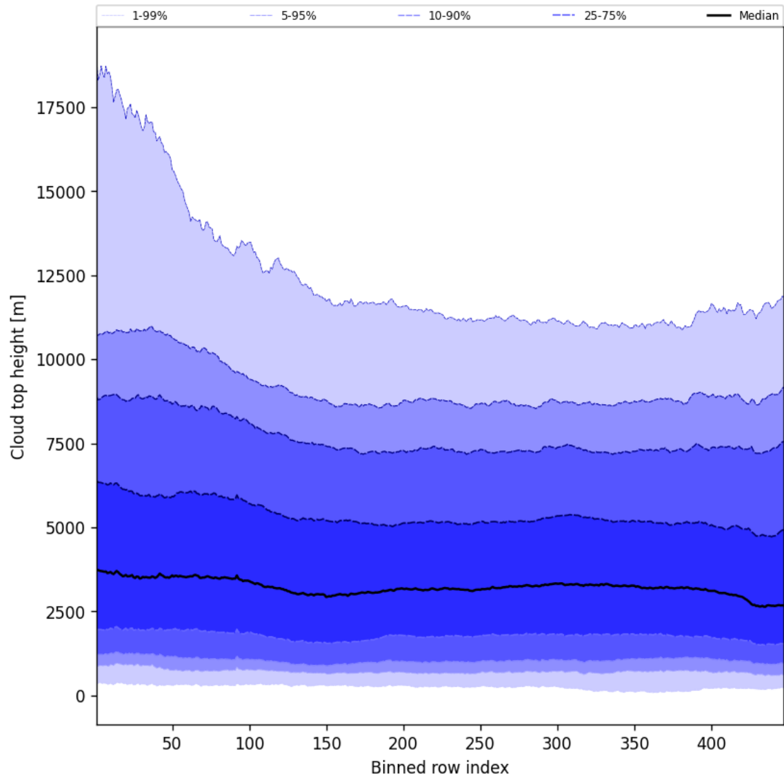
Figure 54: Along track statistics of “Cloud top height” for 2025-09-20 to 2025-09-21
