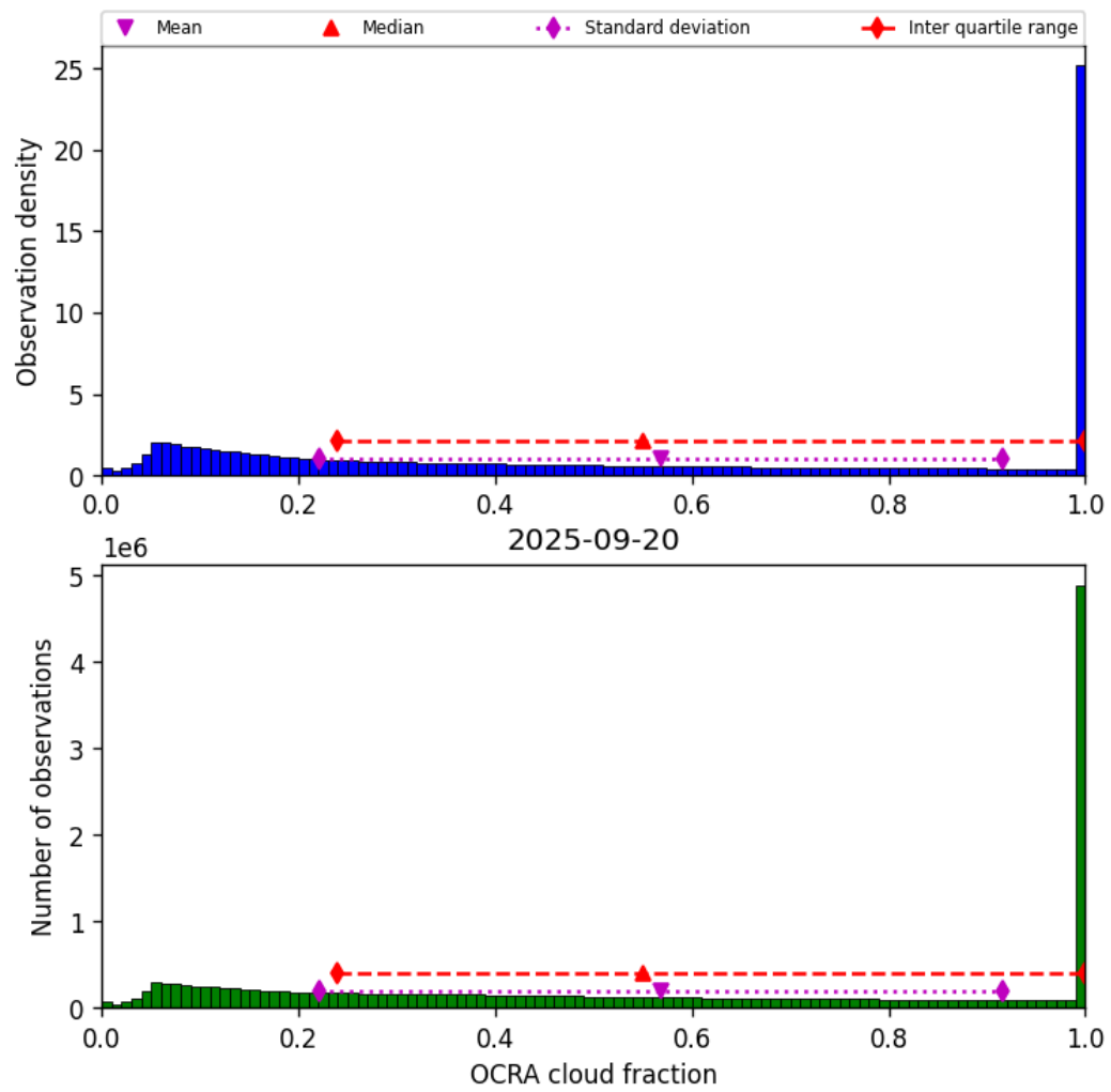
Figure 48: Histogram of “OCRA cloud fraction” for 2025-09-20 to 2025-09-21
