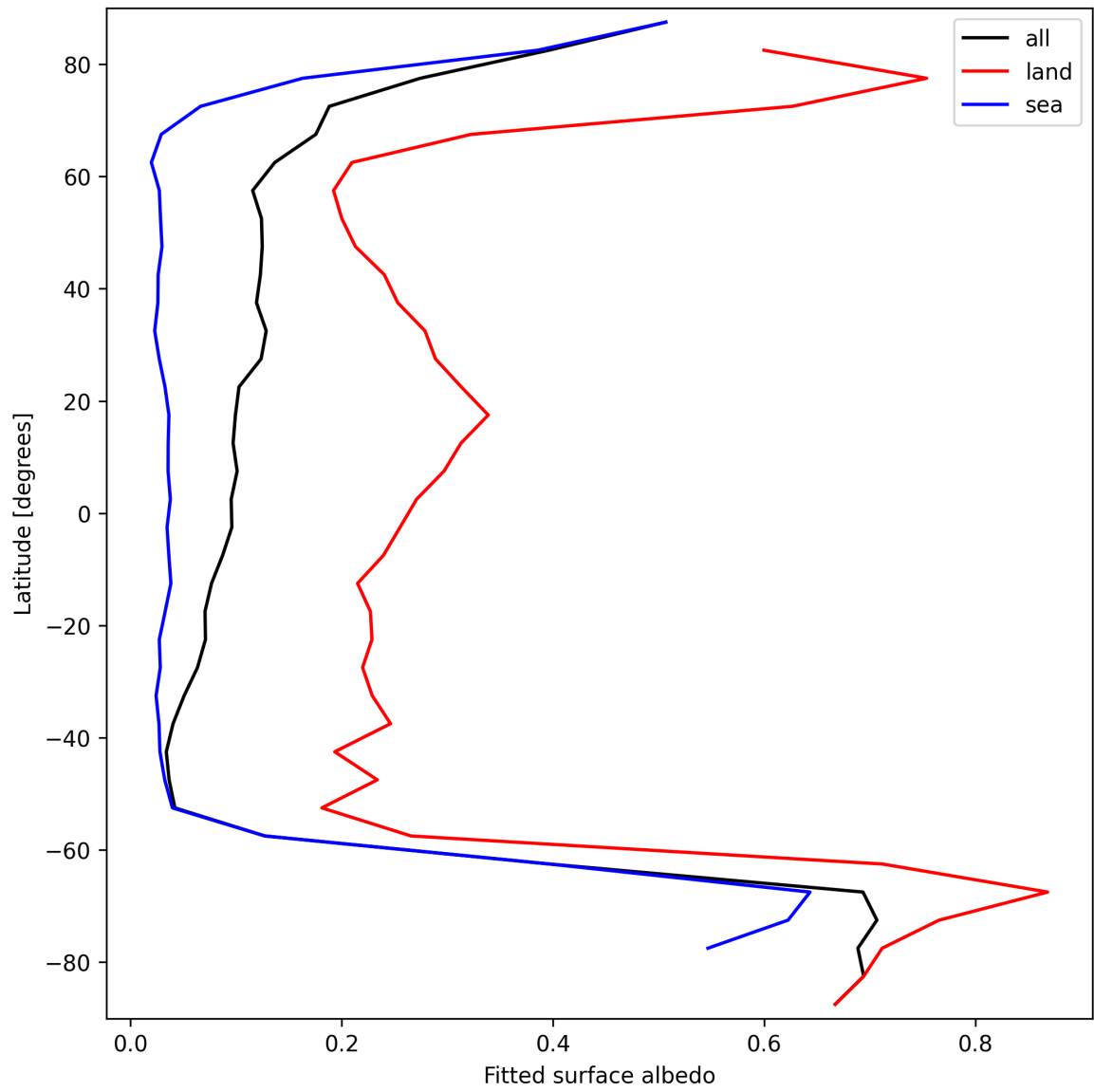
Figure 27: Zonal average of “Fitted surface albedo” for 2025-09-20 to 2025-09-21.
