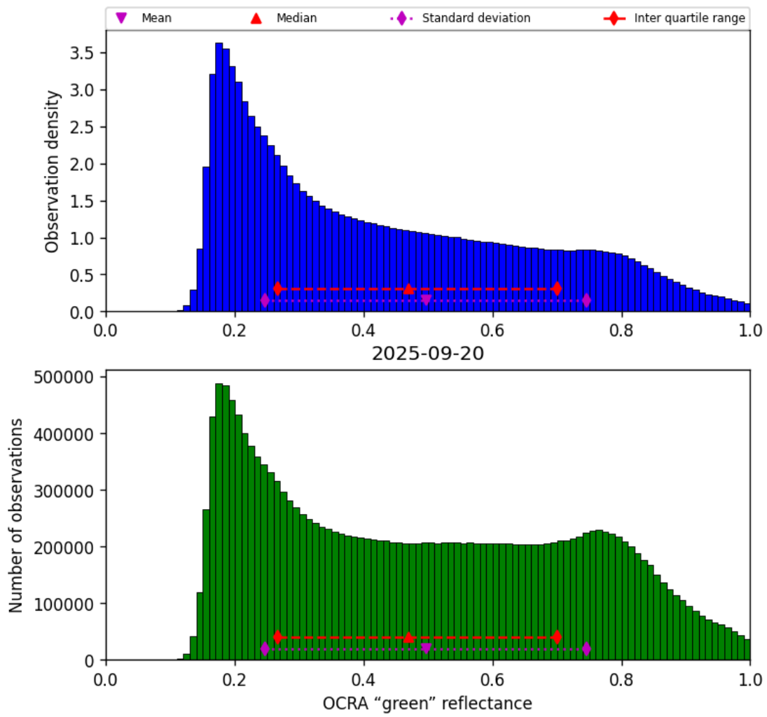
Figure 50: Histogram of “OCRA “green” reflectance” for 2025-09-20 to 2025-09-21
