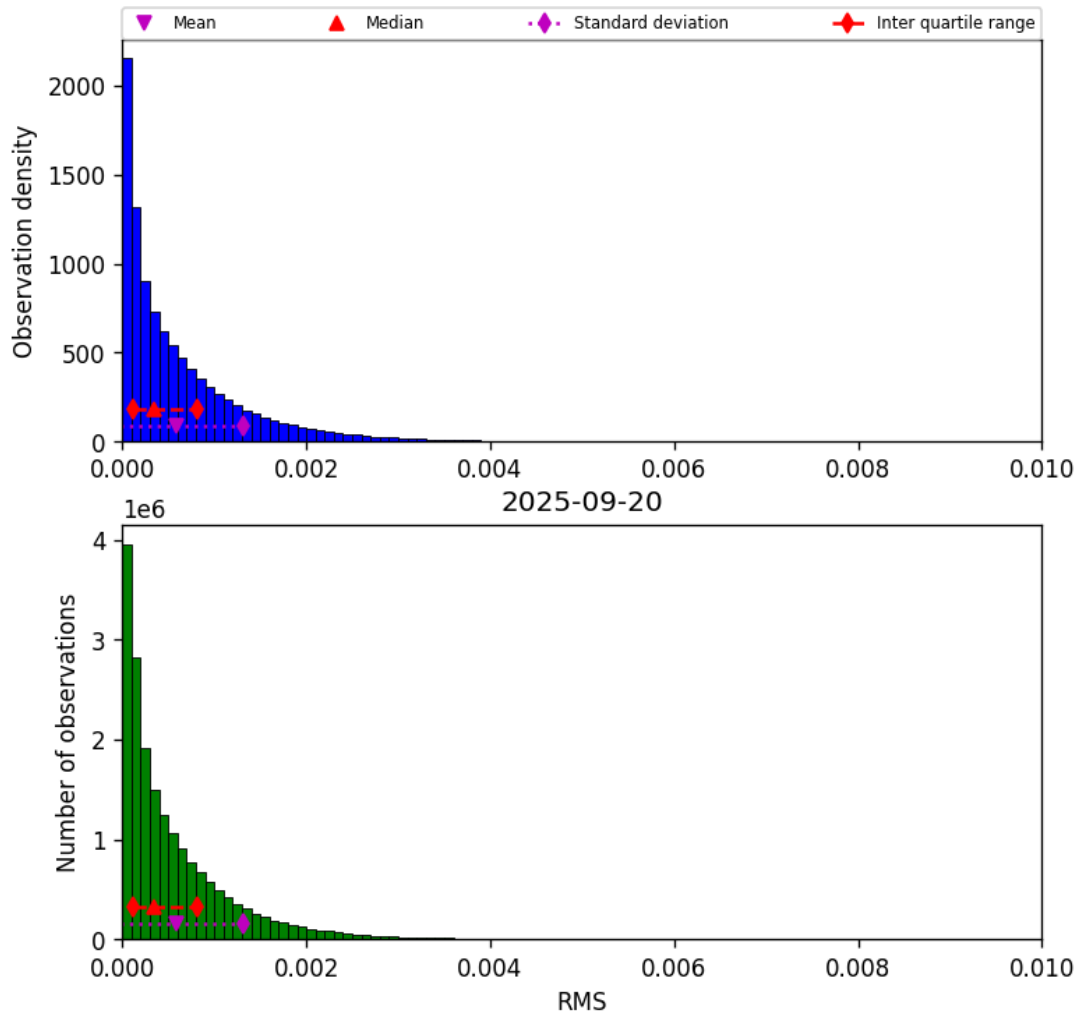
Figure 45: Histogram of “RMS” for 2025-09-20 to 2025-09-21
