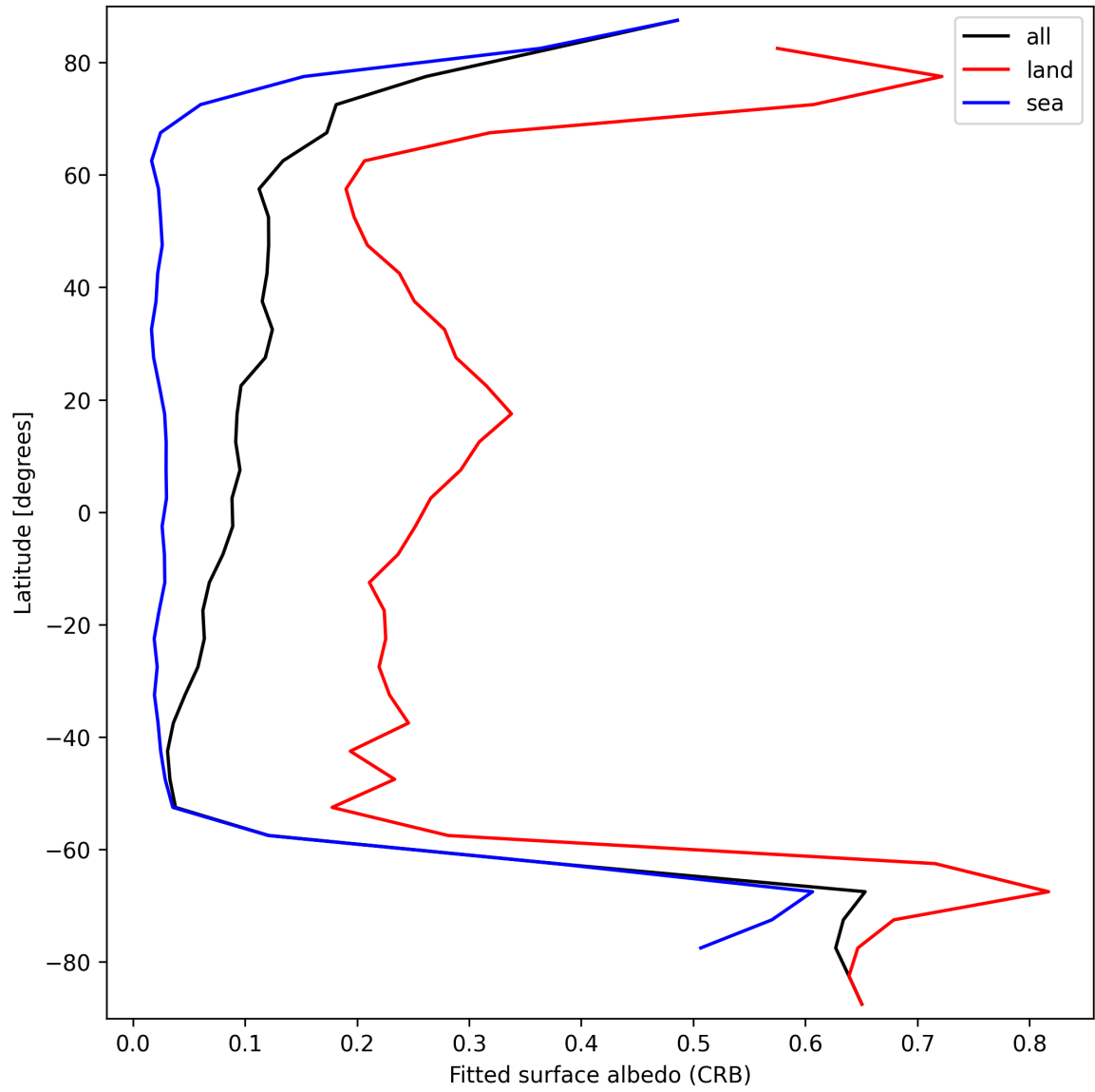
Figure 28: Zonal average of “Fitted surface albedo (CRB)” for 2025-09-20 to 2025-09-21.
