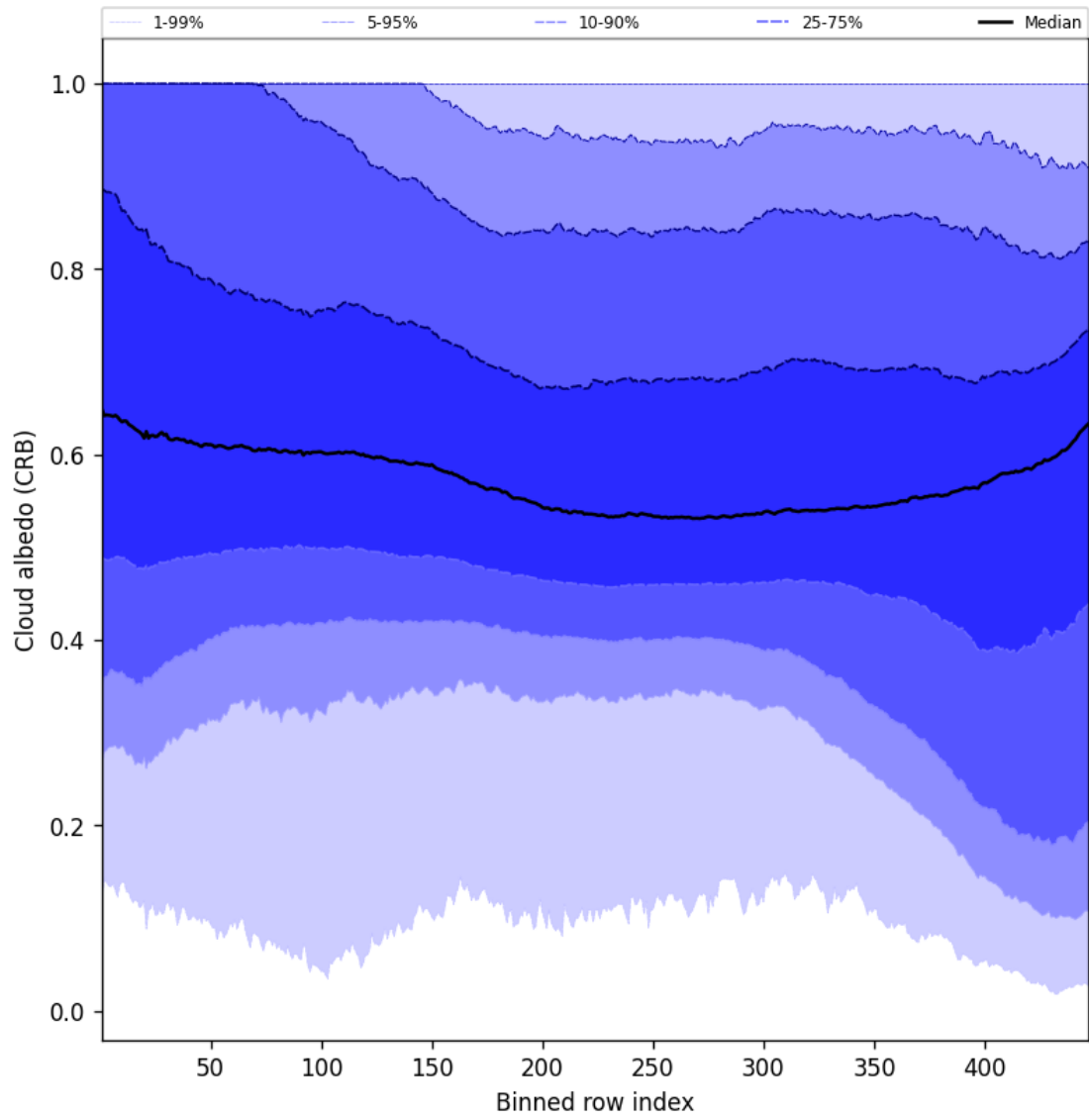
Figure 58: Along track statistics of “Cloud albedo (CRB)” for 2025-09-20 to 2025-09-21
