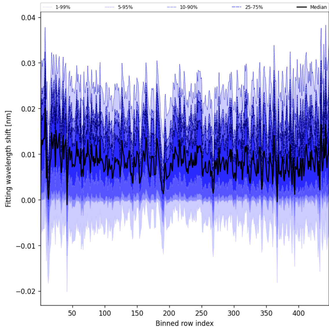
Figure 63: Along track statistics of “Fitting wavelength shift” for 2025-09-20 to 2025-09-21
