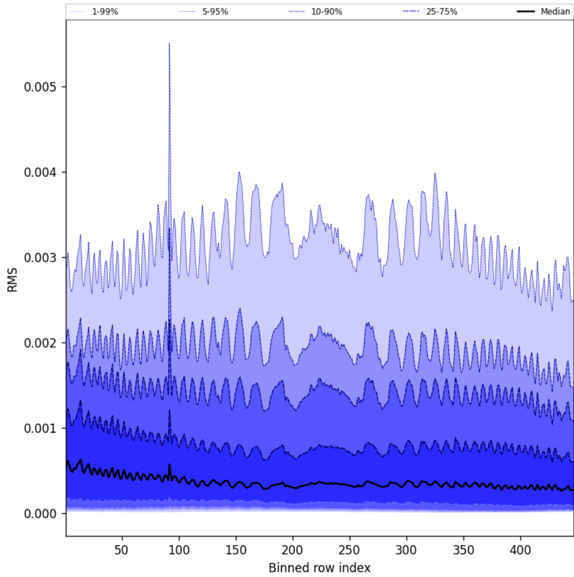
Figure 61: Along track statistics of “RMS” for 2025-09-20 to 2025-09-21
