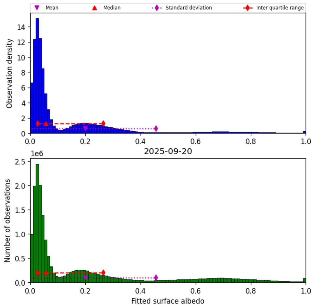
Figure 43: Histogram of “Fitted surface albedo” for 2025-09-20 to 2025-09-21
