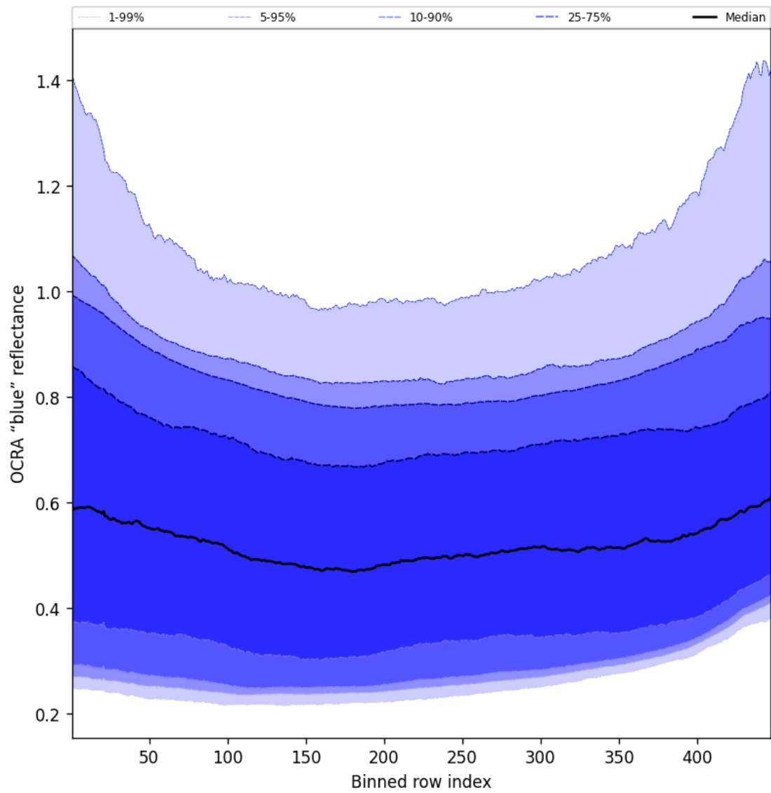
Figure 65: Along track statistics of “OCRA “blue” reflectance” for 2025-09-20 to 2025-09-21
