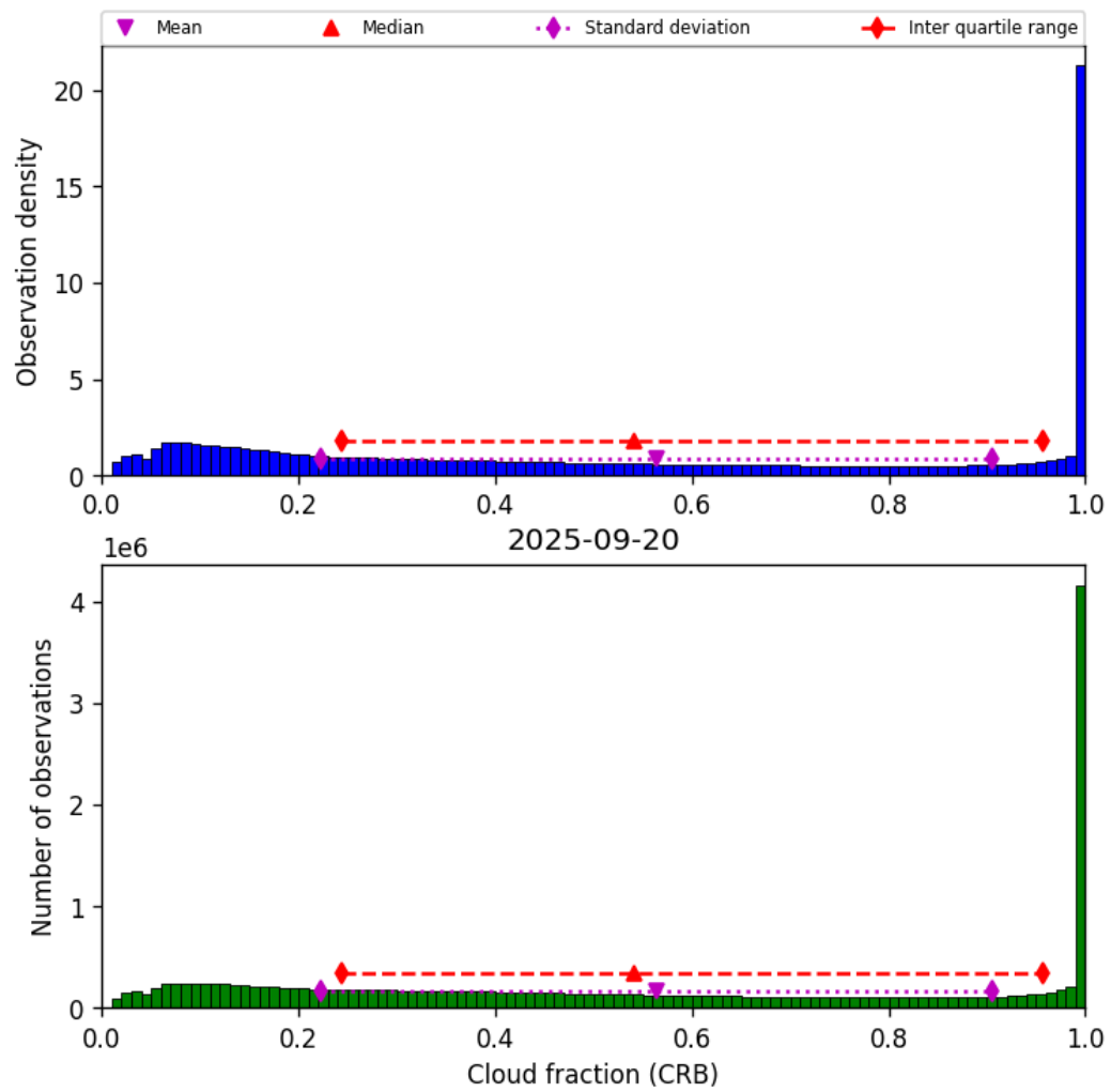
Figure 40: Histogram of “Cloud fraction (CRB)” for 2025-09-20 to 2025-09-21
