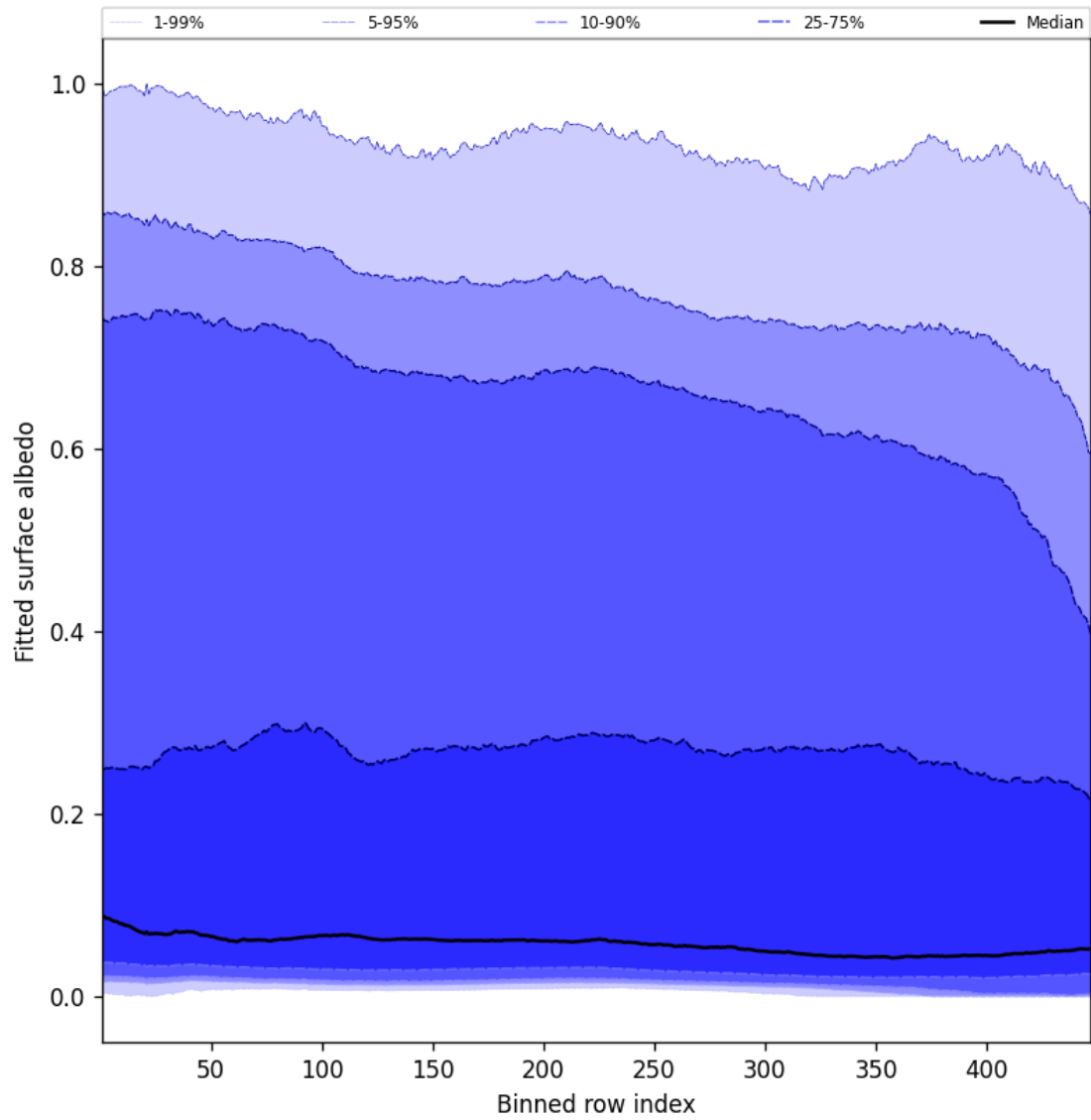
Figure 59: Along track statistics of “Fitted surface albedo” for 2025-09-20 to 2025-09-21
