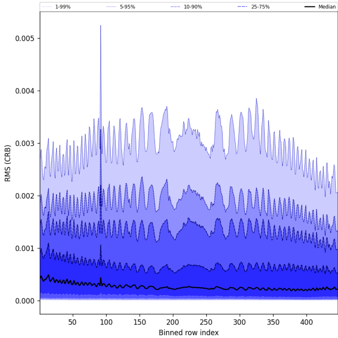
Figure 62: Along track statistics of “RMS (CRB)” for 2025-09-20 to 2025-09-21
