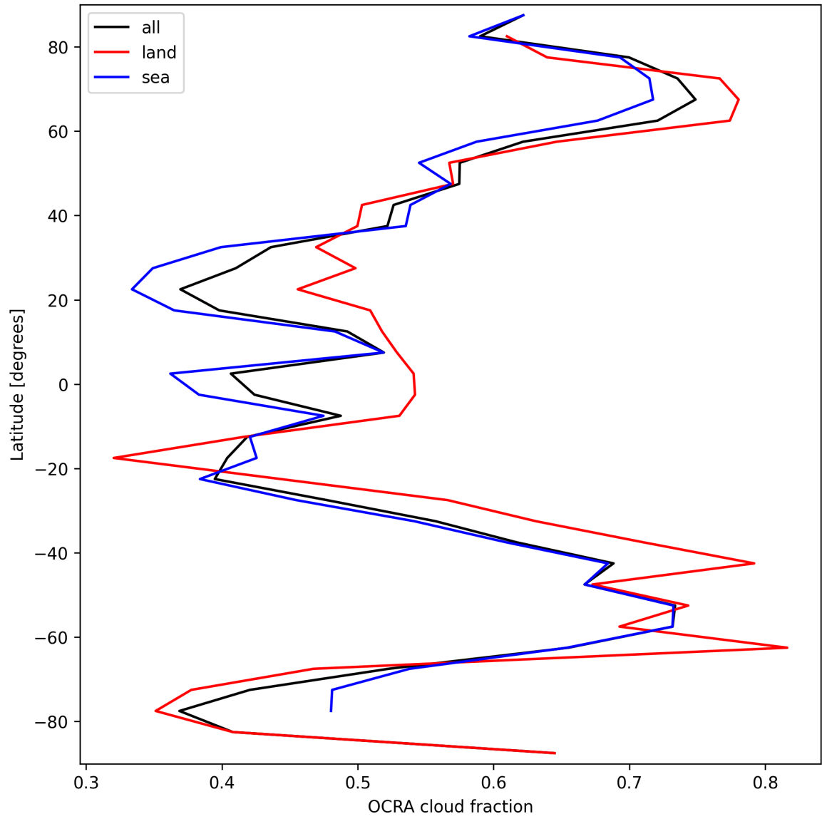
Figure 32: Zonal average of “OCRA cloud fraction” for 2025-09-20 to 2025-09-21.
