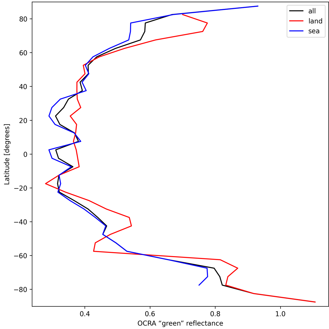
Figure 34: Zonal average of “OCRA “green” reflectance” for 2025-09-20 to 2025-09-21.
