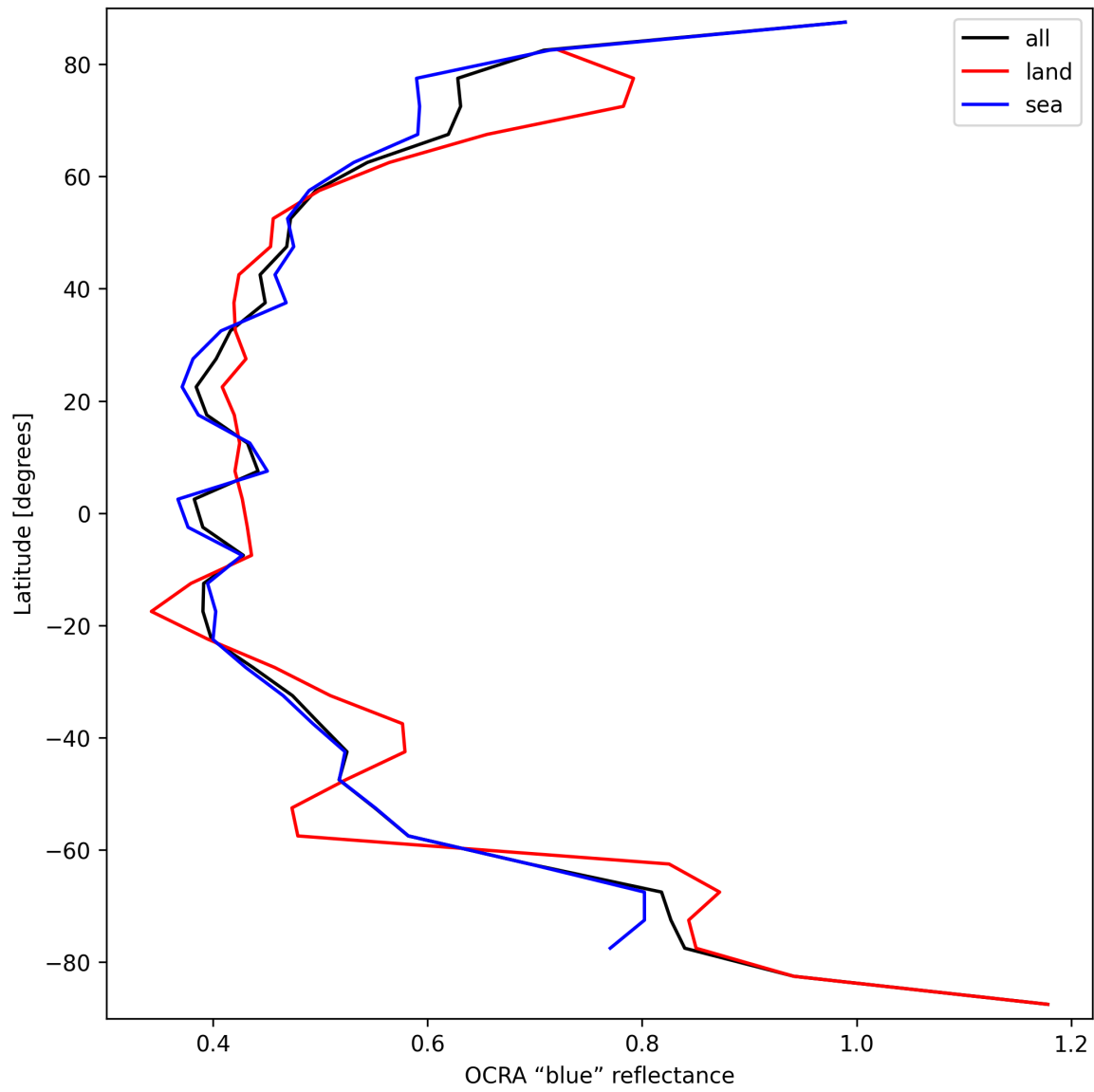
Figure 33: Zonal average of “OCRA “blue” reflectance” for 2025-09-20 to 2025-09-21.
