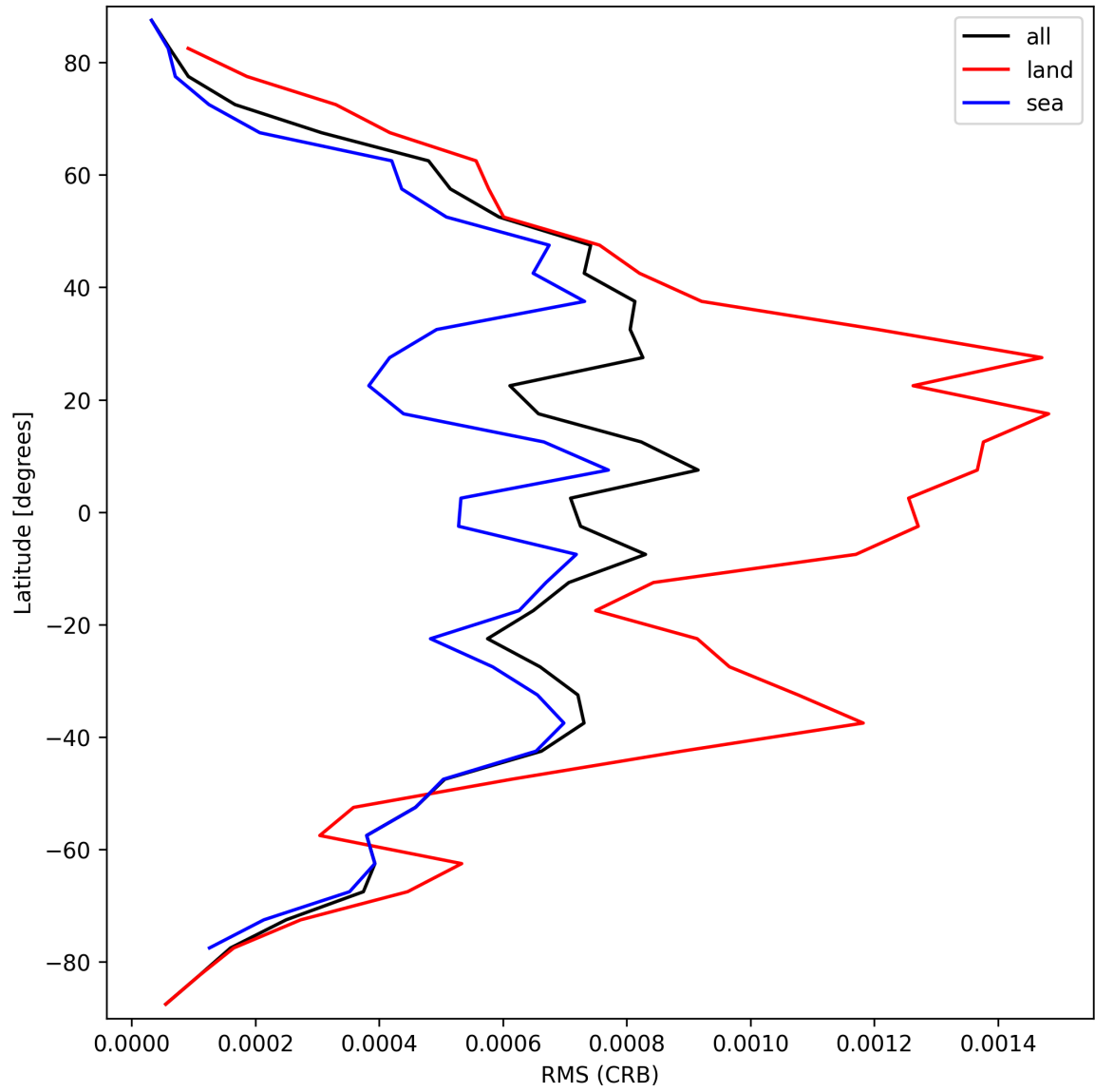
Figure 30: Zonal average of “RMS (CRB)” for 2025-09-20 to 2025-09-21.
