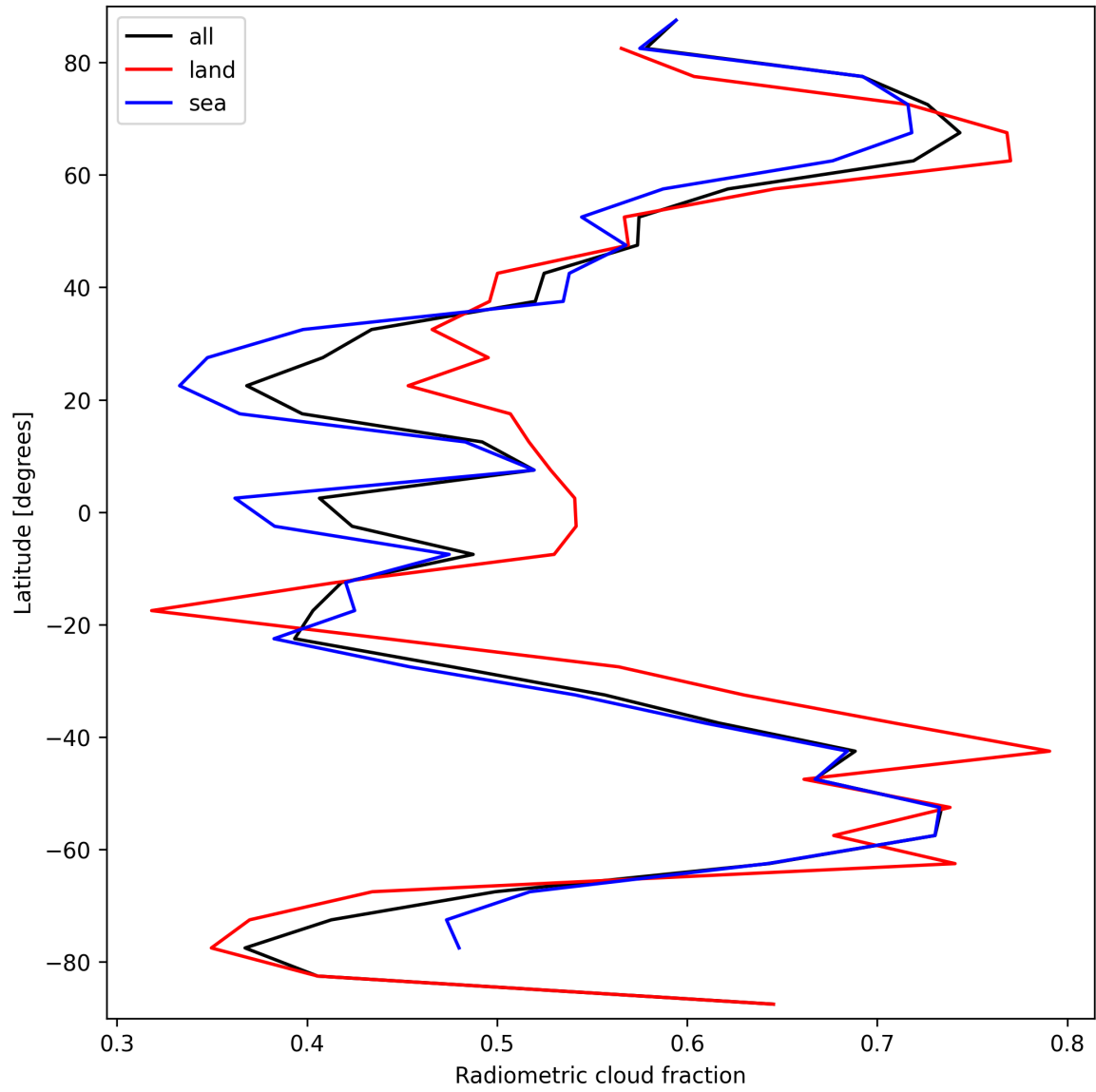
Figure 21: Zonal average of “Radiometric cloud fraction” for 2025-09-20 to 2025-09-21.
