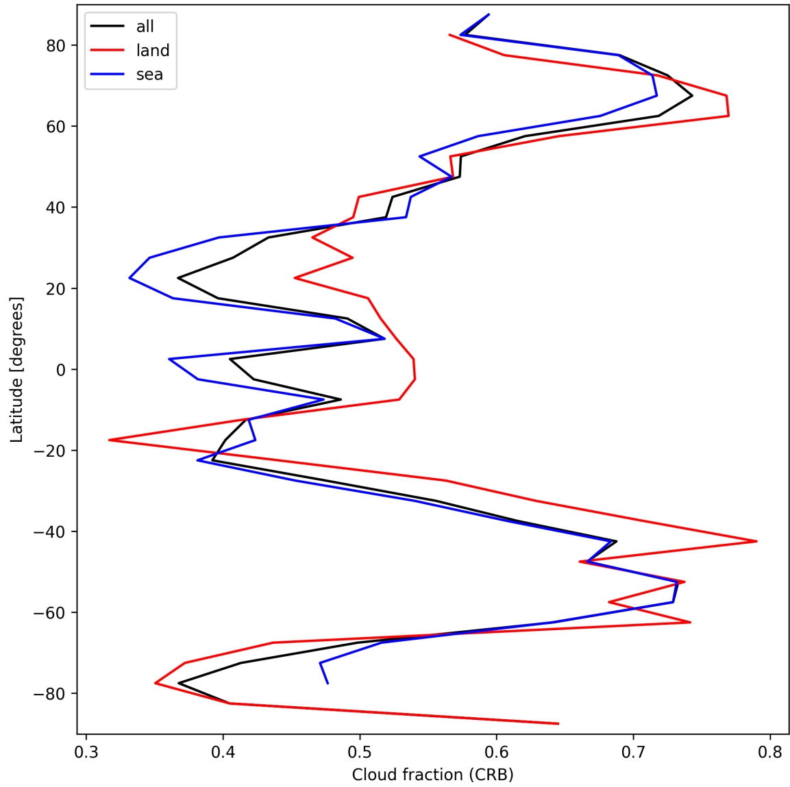
Figure 24: Zonal average of “Cloud fraction (CRB)” for 2025-09-20 to 2025-09-21.
