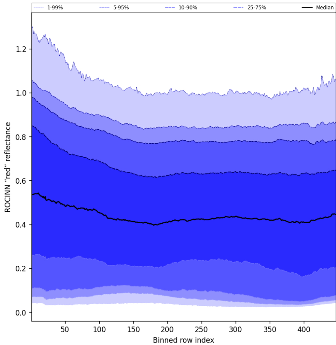
Figure 67: Along track statistics of “ROCINN “red” reflectance” for 2025-09-20 to 2025-09-21
