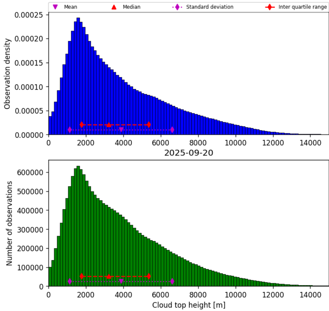
Figure 38: Histogram of “Cloud top height” for 2025-09-20 to 2025-09-21
