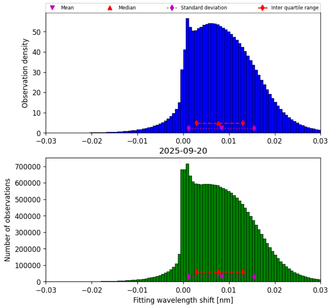
Figure 47: Histogram of “Fitting wavelength shift” for 2025-09-20 to 2025-09-21
