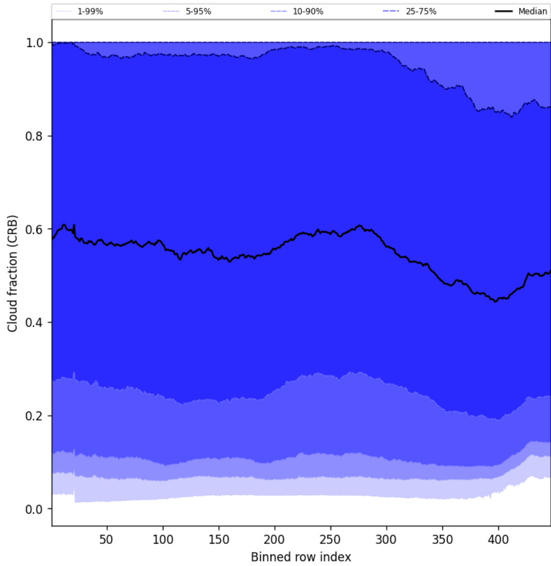
Figure 56: Along track statistics of “Cloud fraction (CRB)” for 2025-09-20 to 2025-09-21
