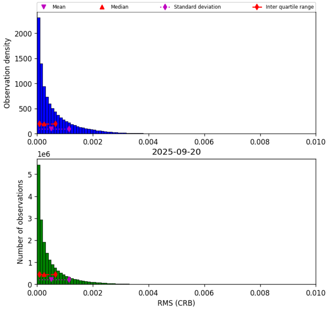
Figure 46: Histogram of “RMS (CRB)” for 2025-09-20 to 2025-09-21
