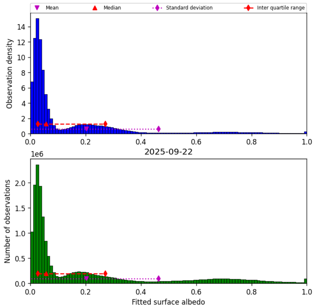
Figure 43: Histogram of “Fitted surface albedo” for 2025-09-22 to 2025-09-23
