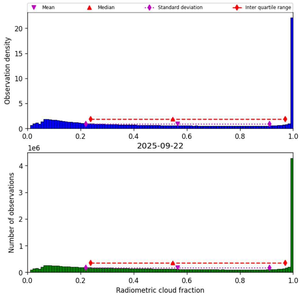
Figure 37: Histogram of “Radiometric cloud fraction” for 2025-09-22 to 2025-09-23
