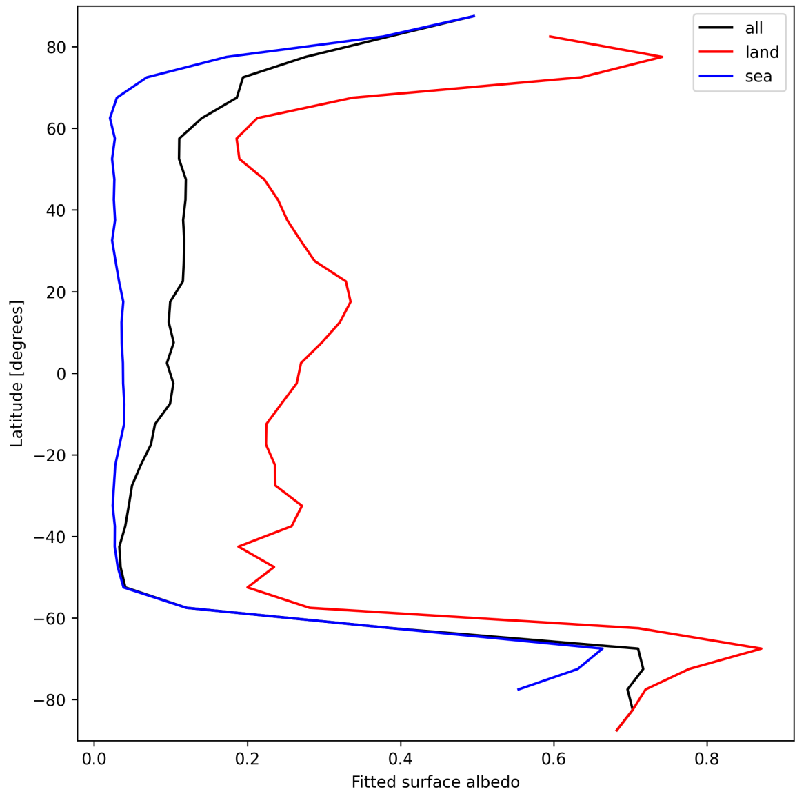
Figure 27: Zonal average of “Fitted surface albedo” for 2025-09-22 to 2025-09-23.
