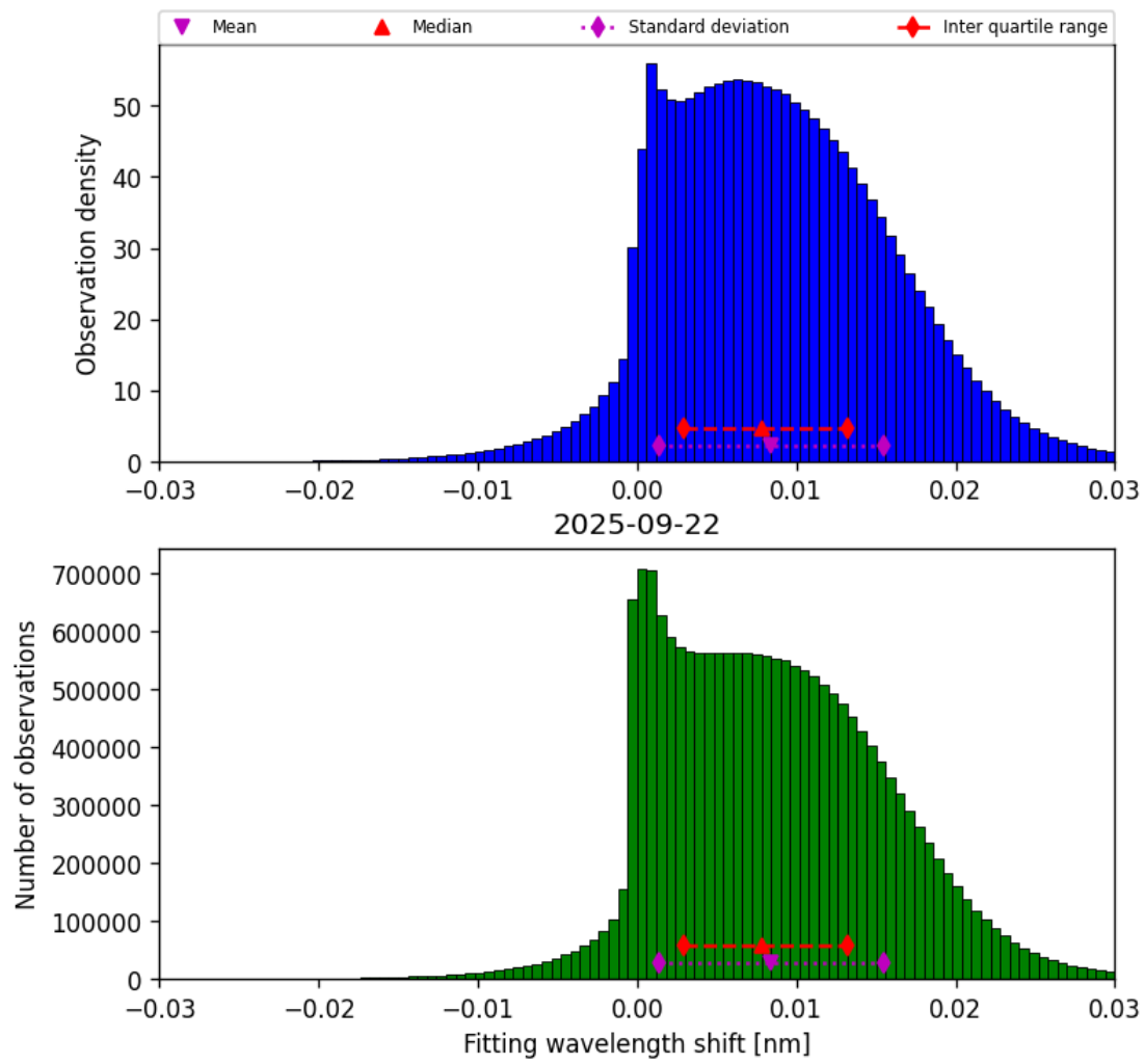
Figure 47: Histogram of “Fitting wavelength shift” for 2025-09-22 to 2025-09-23
