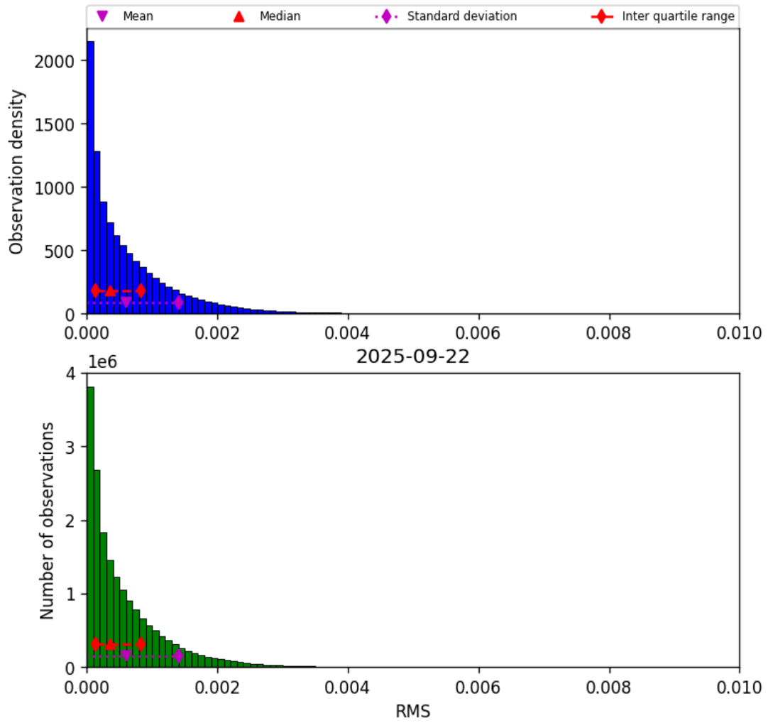
Figure 45: Histogram of “RMS” for 2025-09-22 to 2025-09-23
