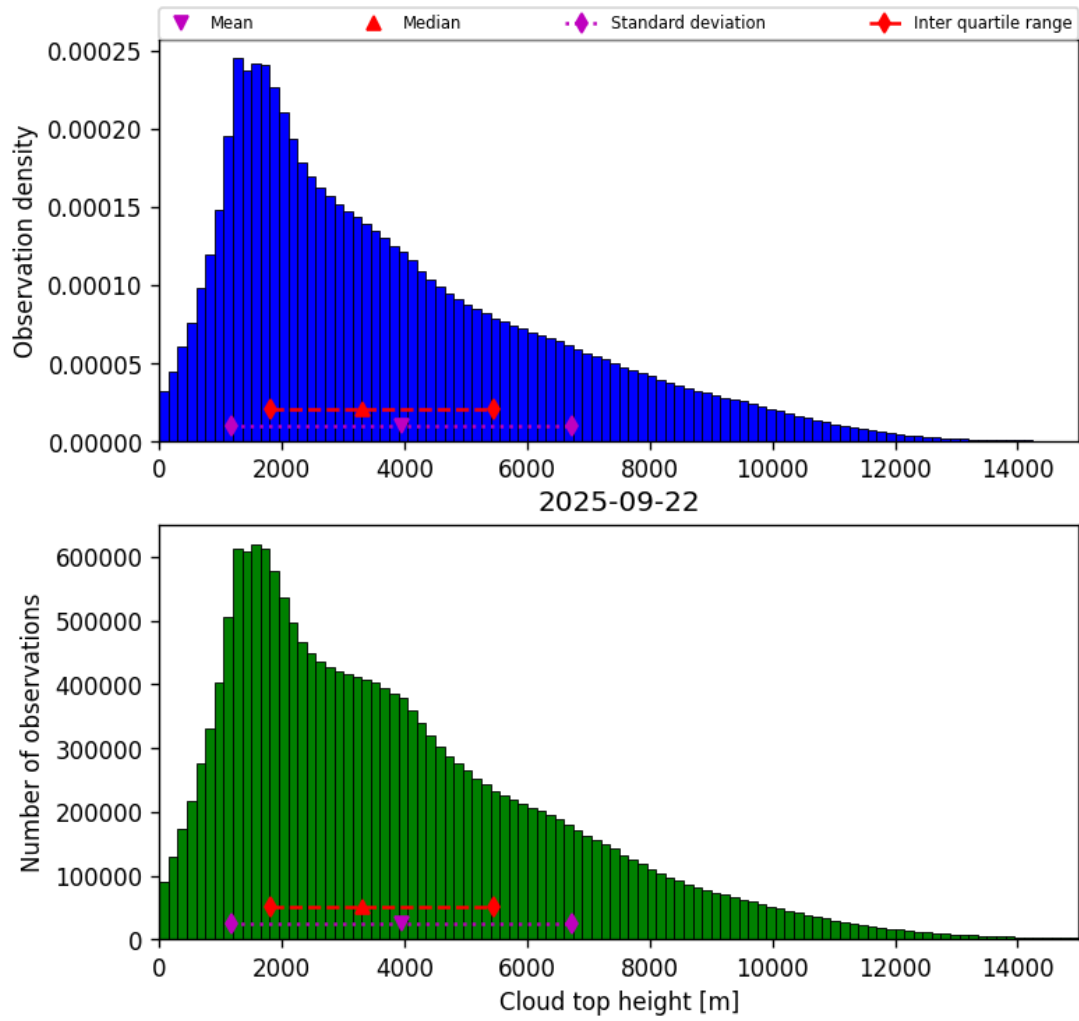
Figure 38: Histogram of “Cloud top height” for 2025-09-22 to 2025-09-23
