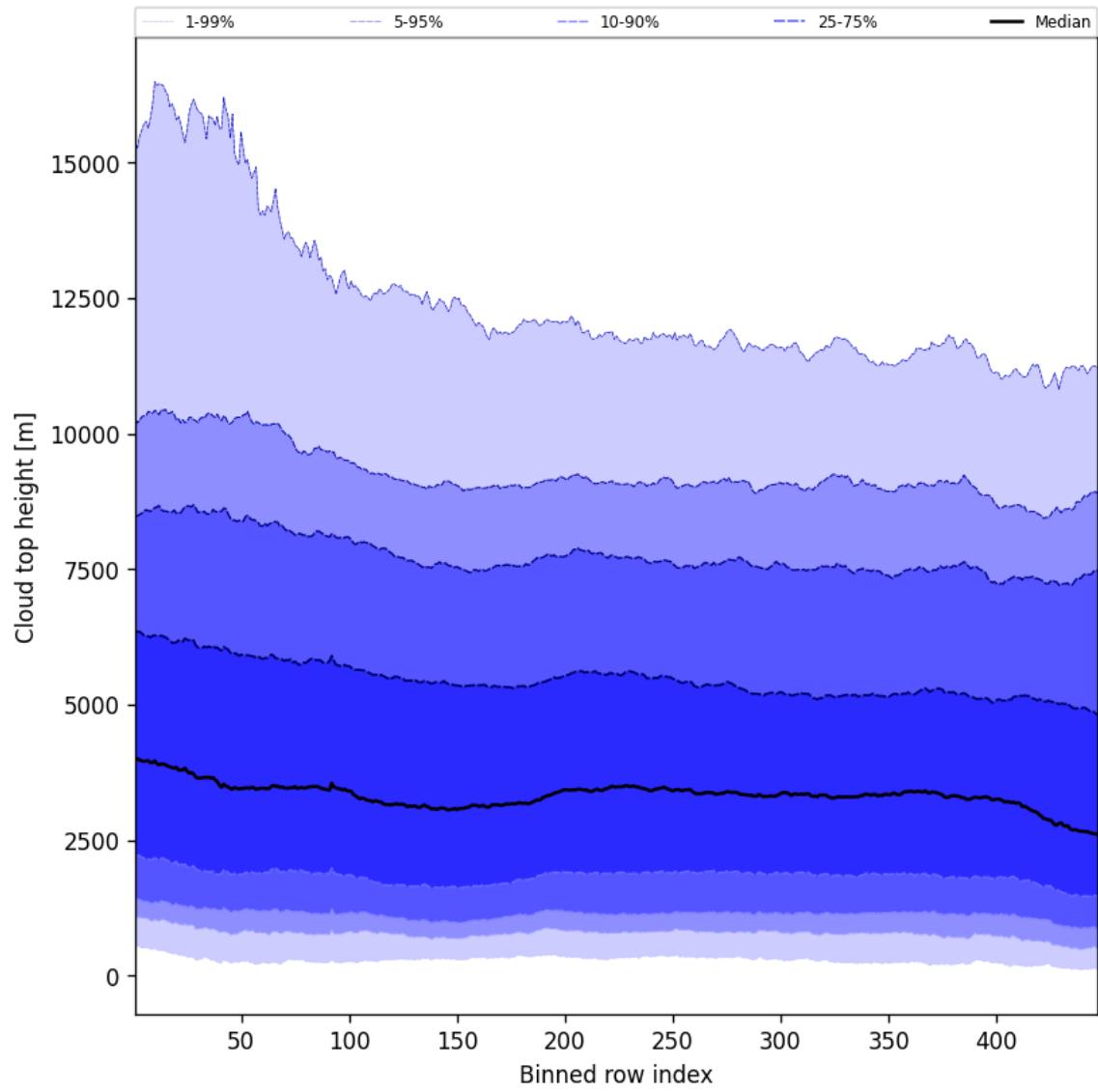
Figure 54: Along track statistics of “Cloud top height” for 2025-09-22 to 2025-09-23
