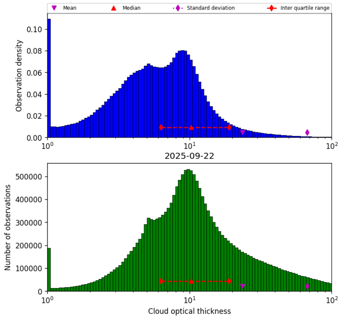
Figure 39: Histogram of “Cloud optical thickness” for 2025-09-22 to 2025-09-23
