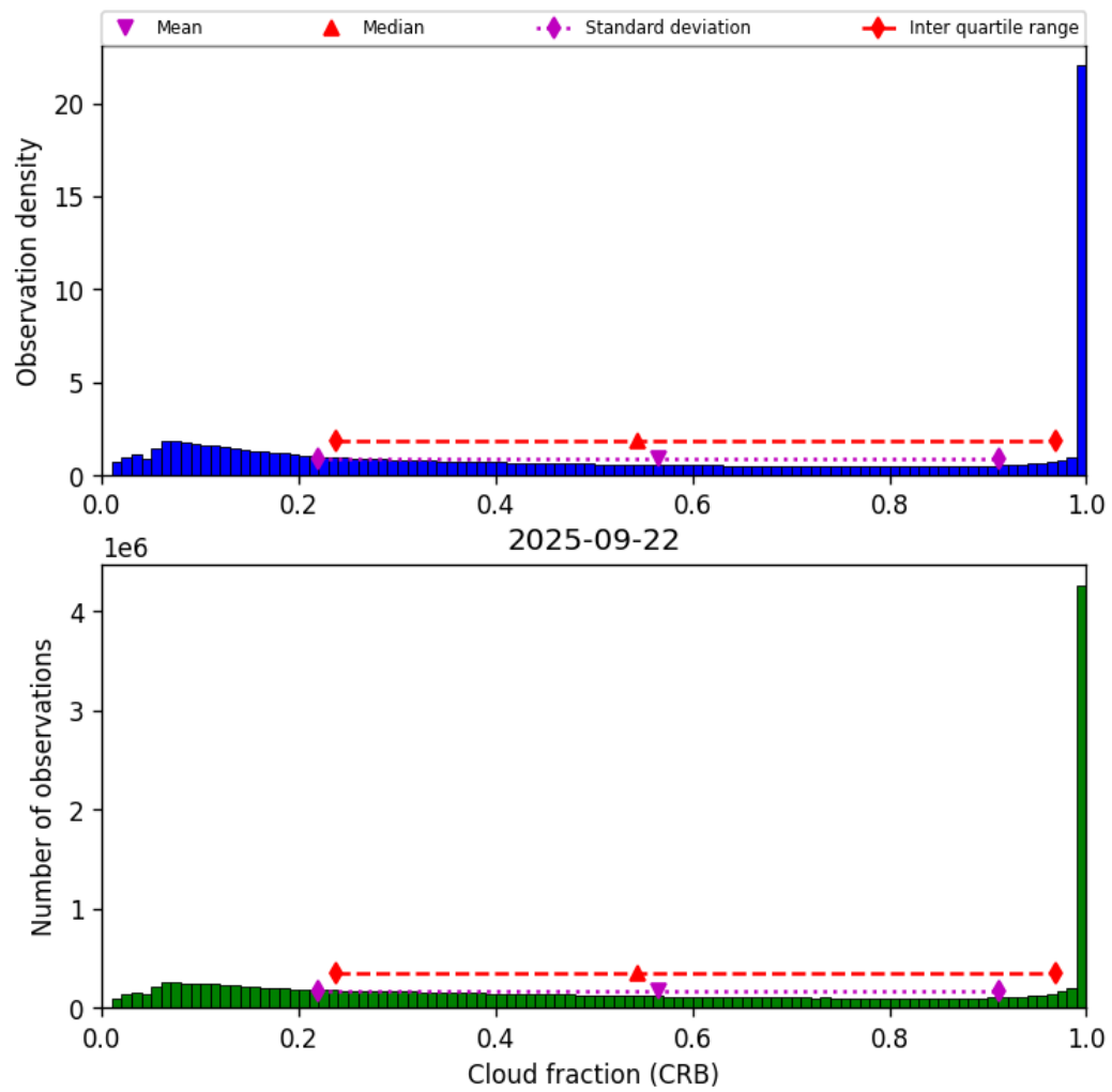
Figure 40: Histogram of “Cloud fraction (CRB)” for 2025-09-22 to 2025-09-23
