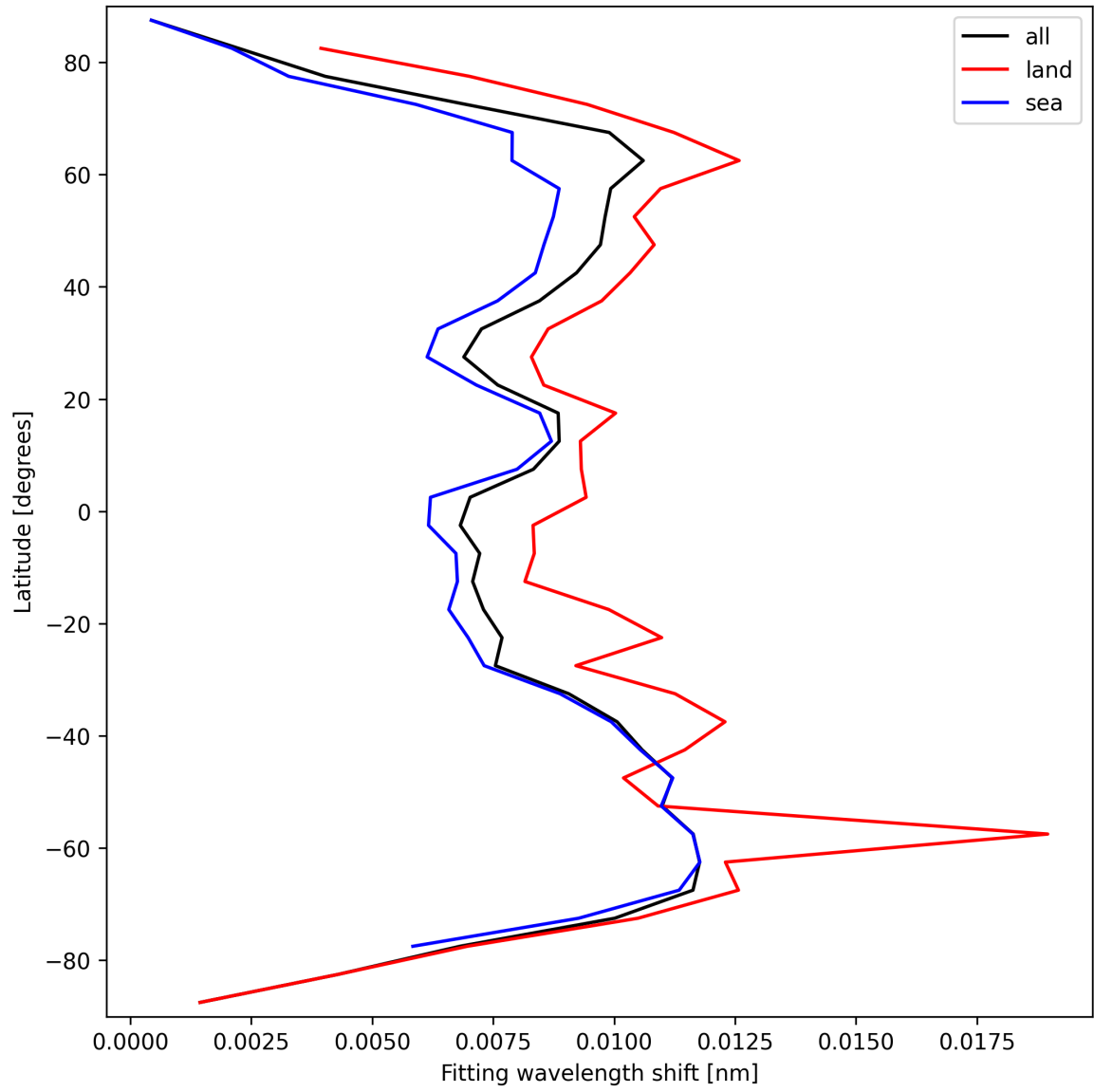
Figure 31: Zonal average of “Fitting wavelength shift” for 2025-09-22 to 2025-09-23.
