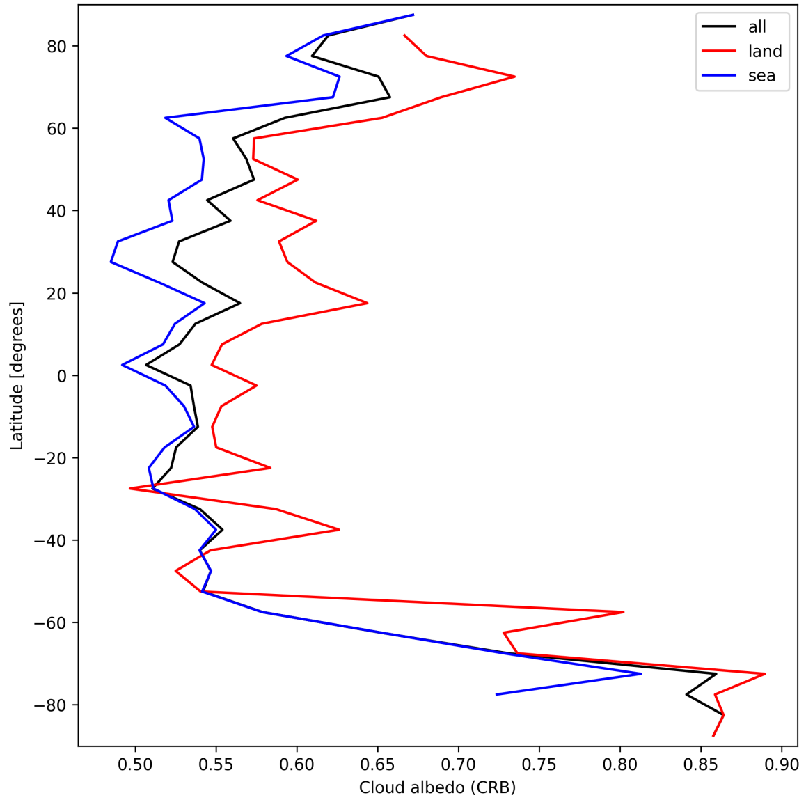
Figure 26: Zonal average of “Cloud albedo (CRB)” for 2025-09-22 to 2025-09-23.
