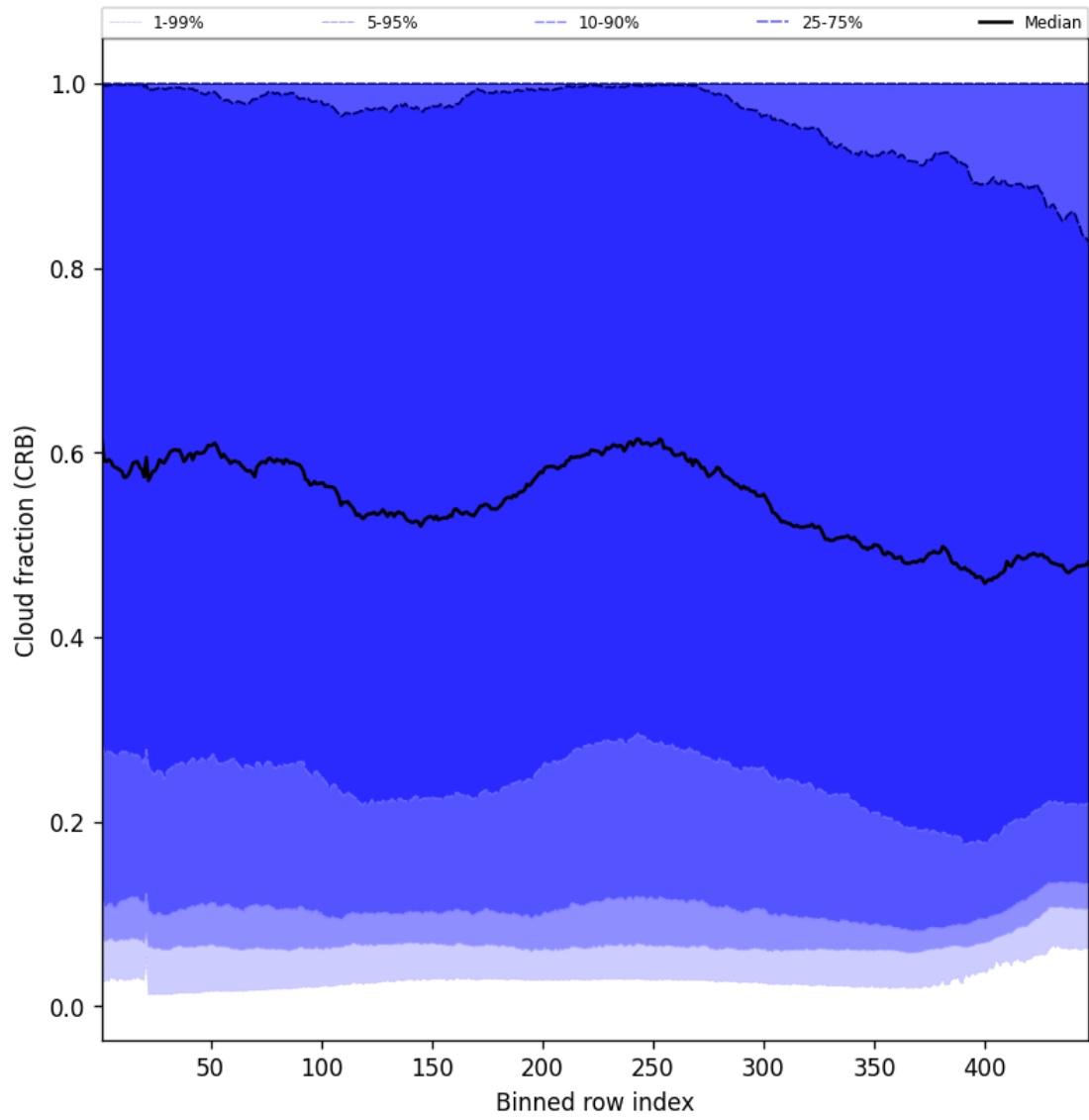
Figure 56: Along track statistics of “Cloud fraction (CRB)” for 2025-09-22 to 2025-09-23
