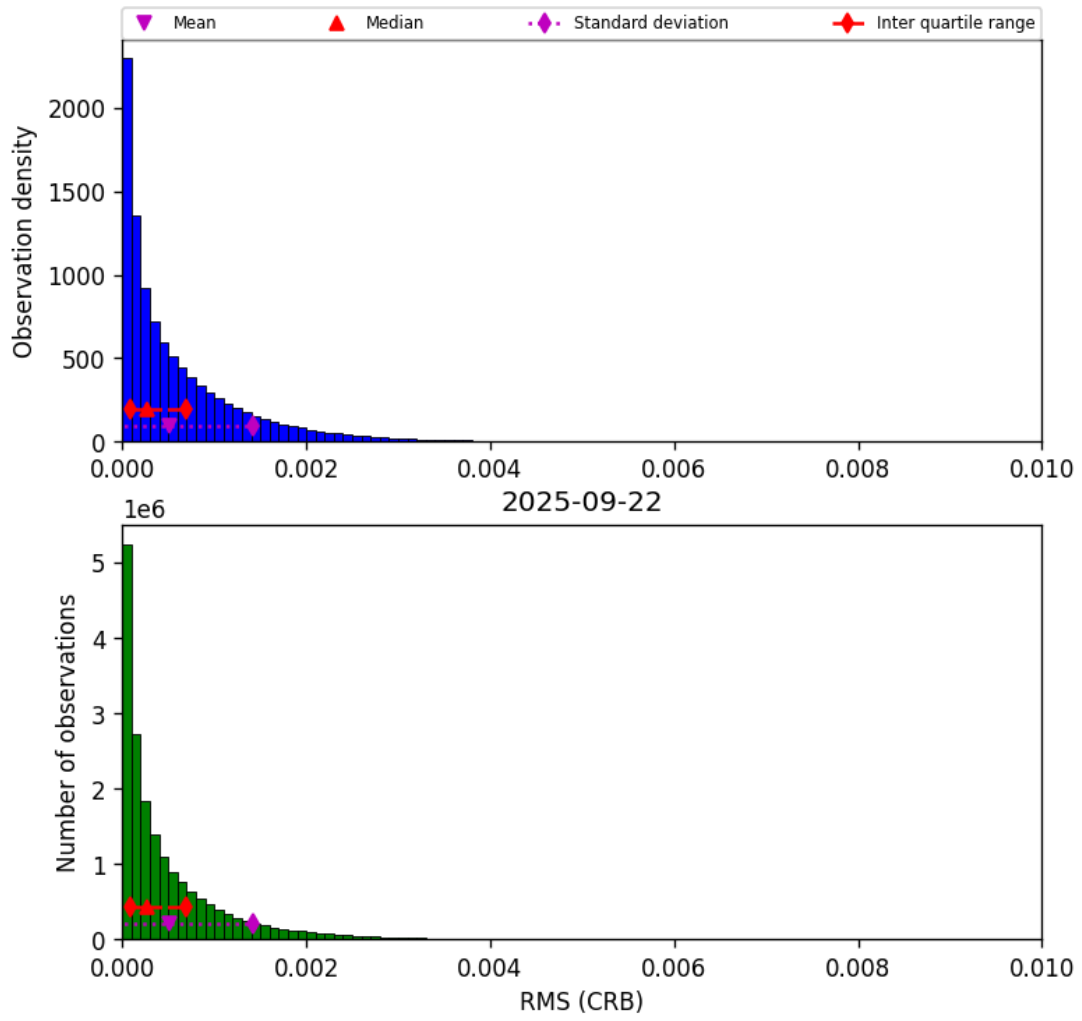
Figure 46: Histogram of “RMS (CRB)” for 2025-09-22 to 2025-09-23
