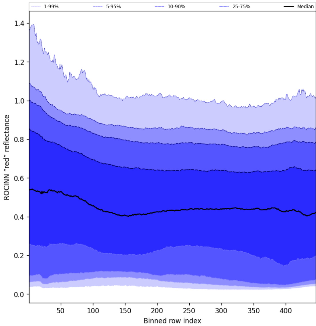
Figure 67: Along track statistics of "ROCINN "red" reflectance" for 2025-09-22 to 2025-09-23
