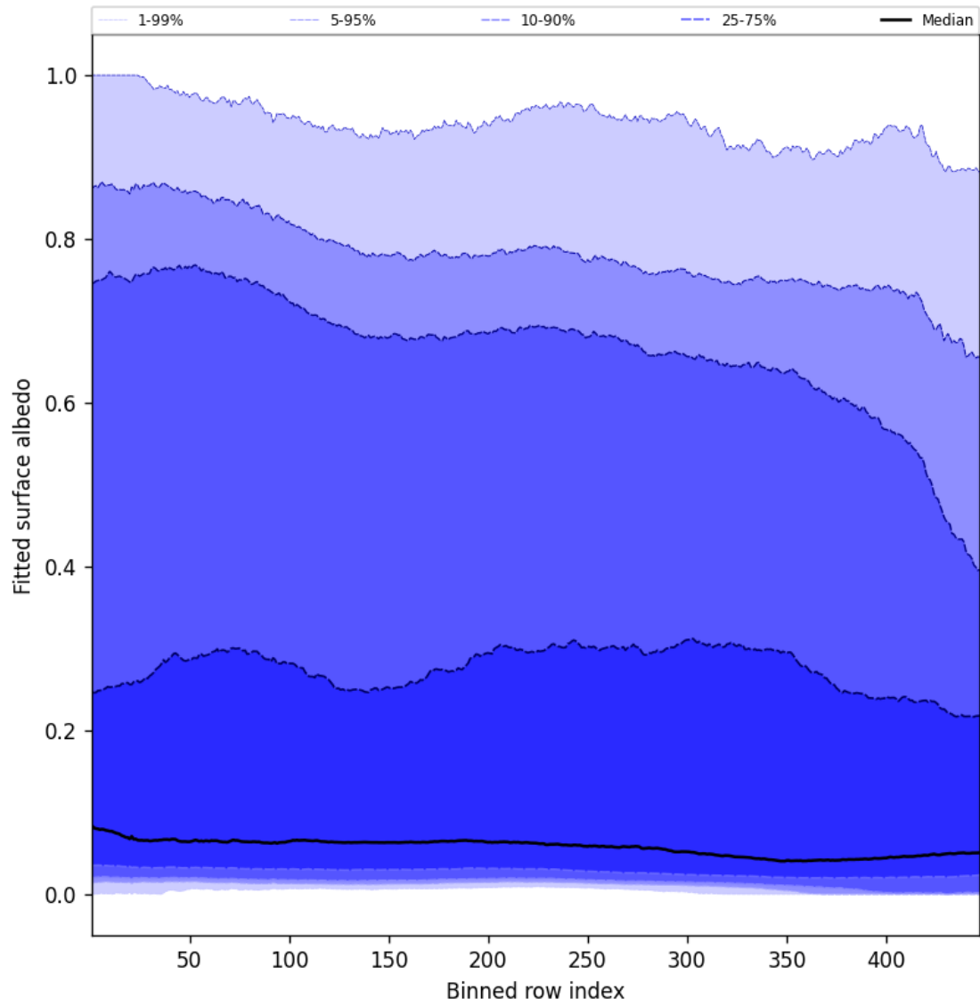
Figure 59: Along track statistics of “Fitted surface albedo” for 2025-09-22 to 2025-09-23
