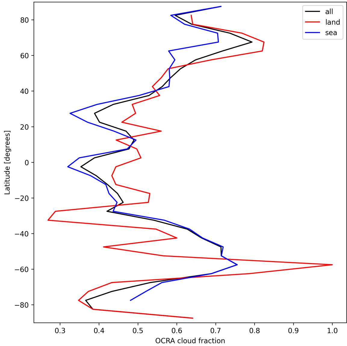
Figure 32: Zonal average of “OCRA cloud fraction” for 2025-09-22 to 2025-09-23.
