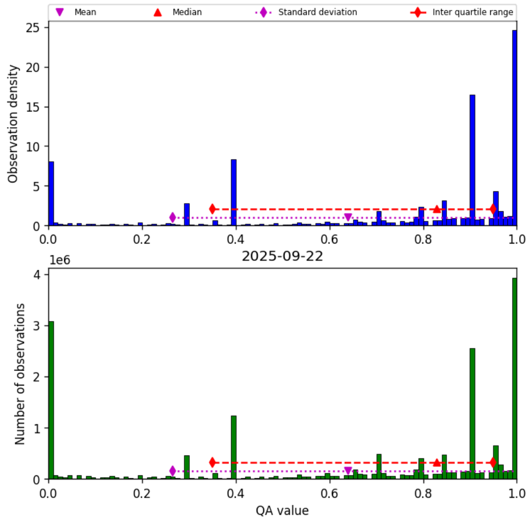
Figure 36: Histogram of “QA value” for 2025-09-22 to 2025-09-23
