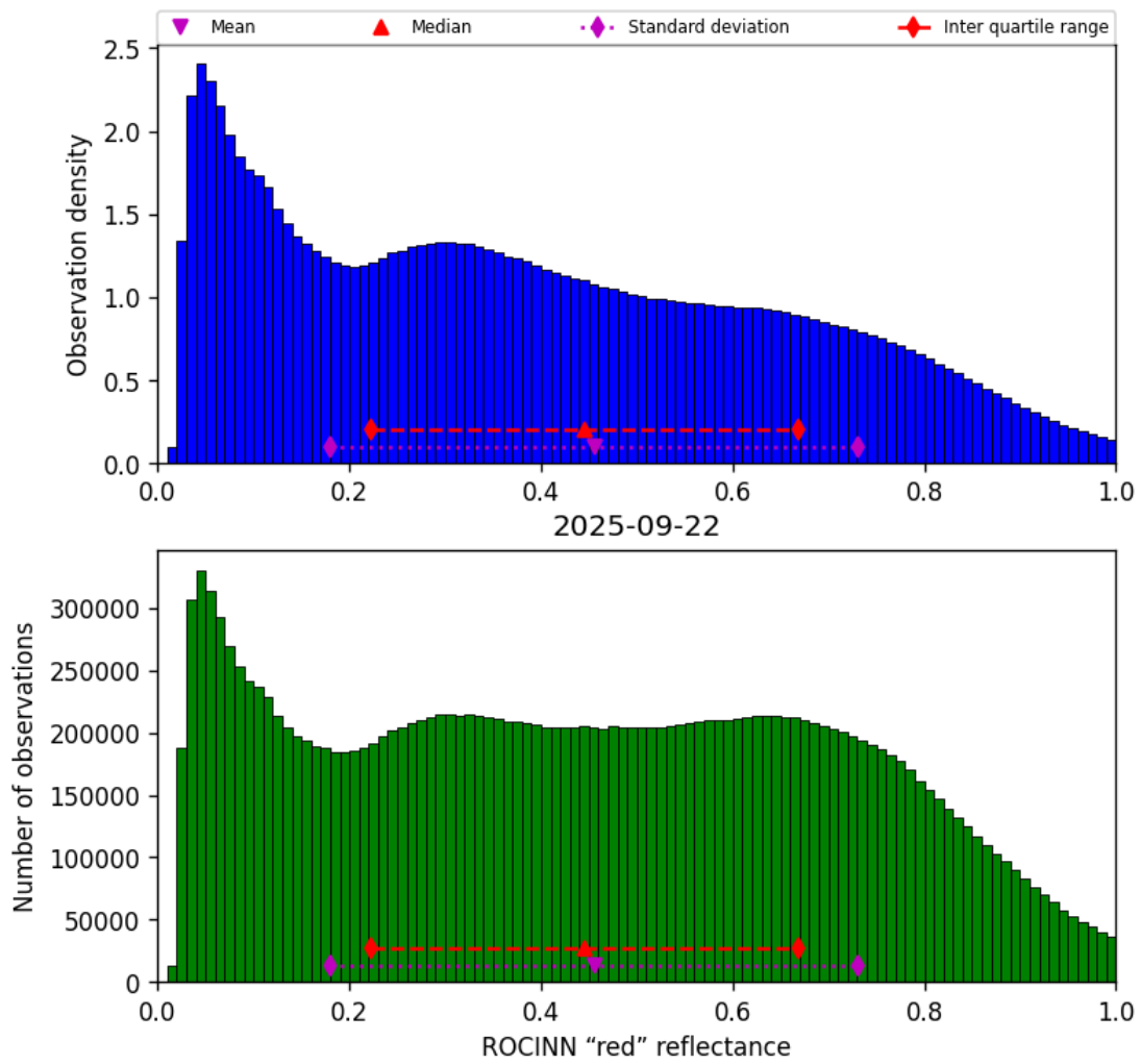
Figure 51: Histogram of “ROCINN “red” reflectance” for 2025-09-22 to 2025-09-23
