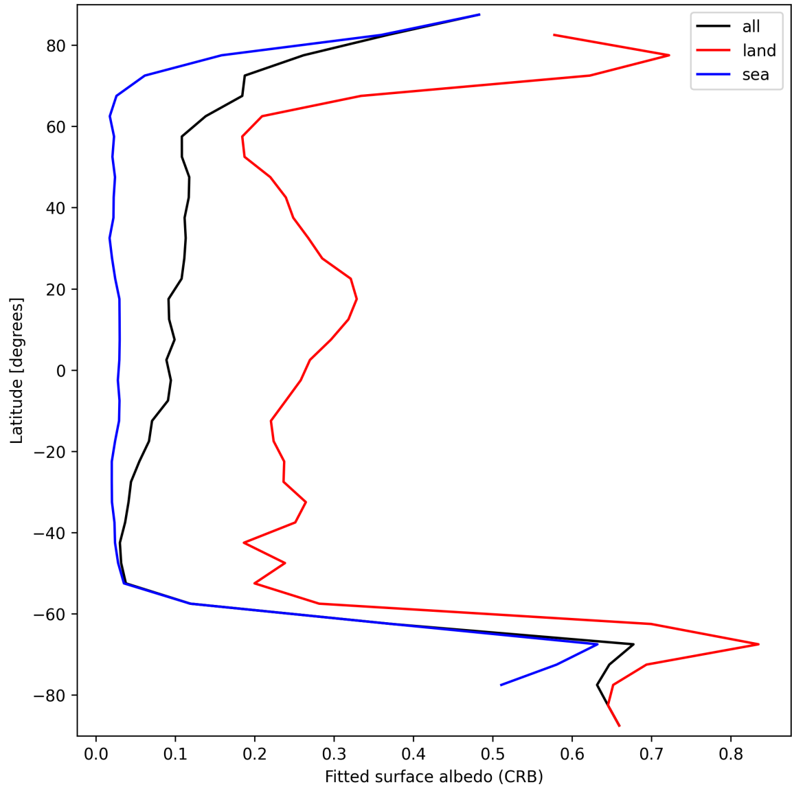
Figure 28: Zonal average of “Fitted surface albedo (CRB)” for 2025-09-22 to 2025-09-23.
