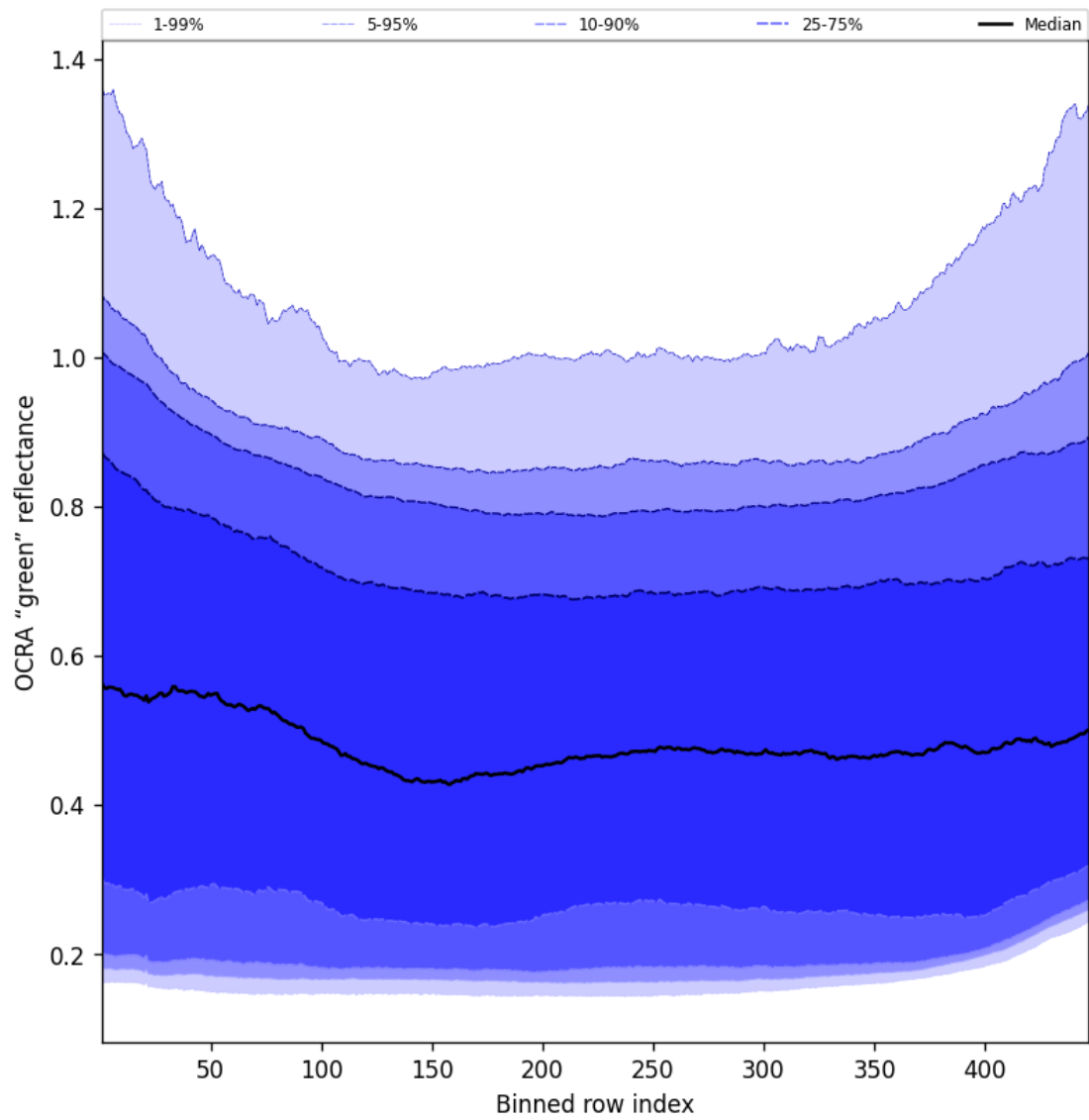
Figure 66: Along track statistics of “OCRA “green” reflectance” for 2025-09-22 to 2025-09-23
