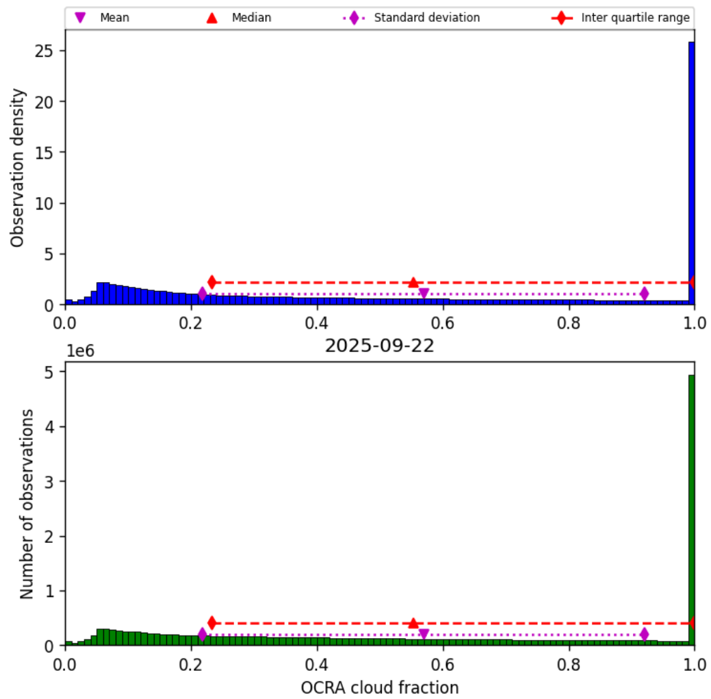
Figure 48: Histogram of “OCRA cloud fraction” for 2025-09-22 to 2025-09-23
