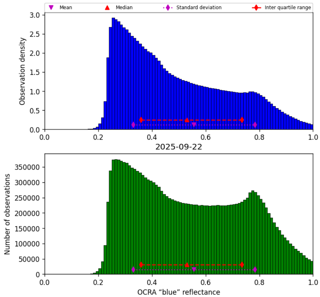
Figure 49: Histogram of “OCRA “blue” reflectance” for 2025-09-22 to 2025-09-23
