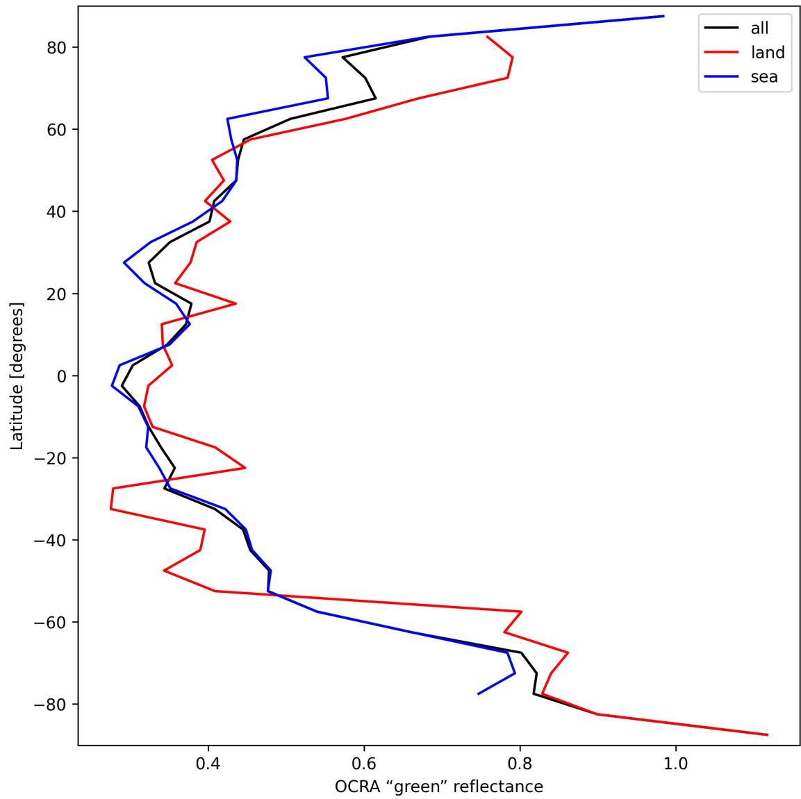
Figure 34: Zonal average of “OCRA “green” reflectance” for 2025-09-22 to 2025-09-23.
