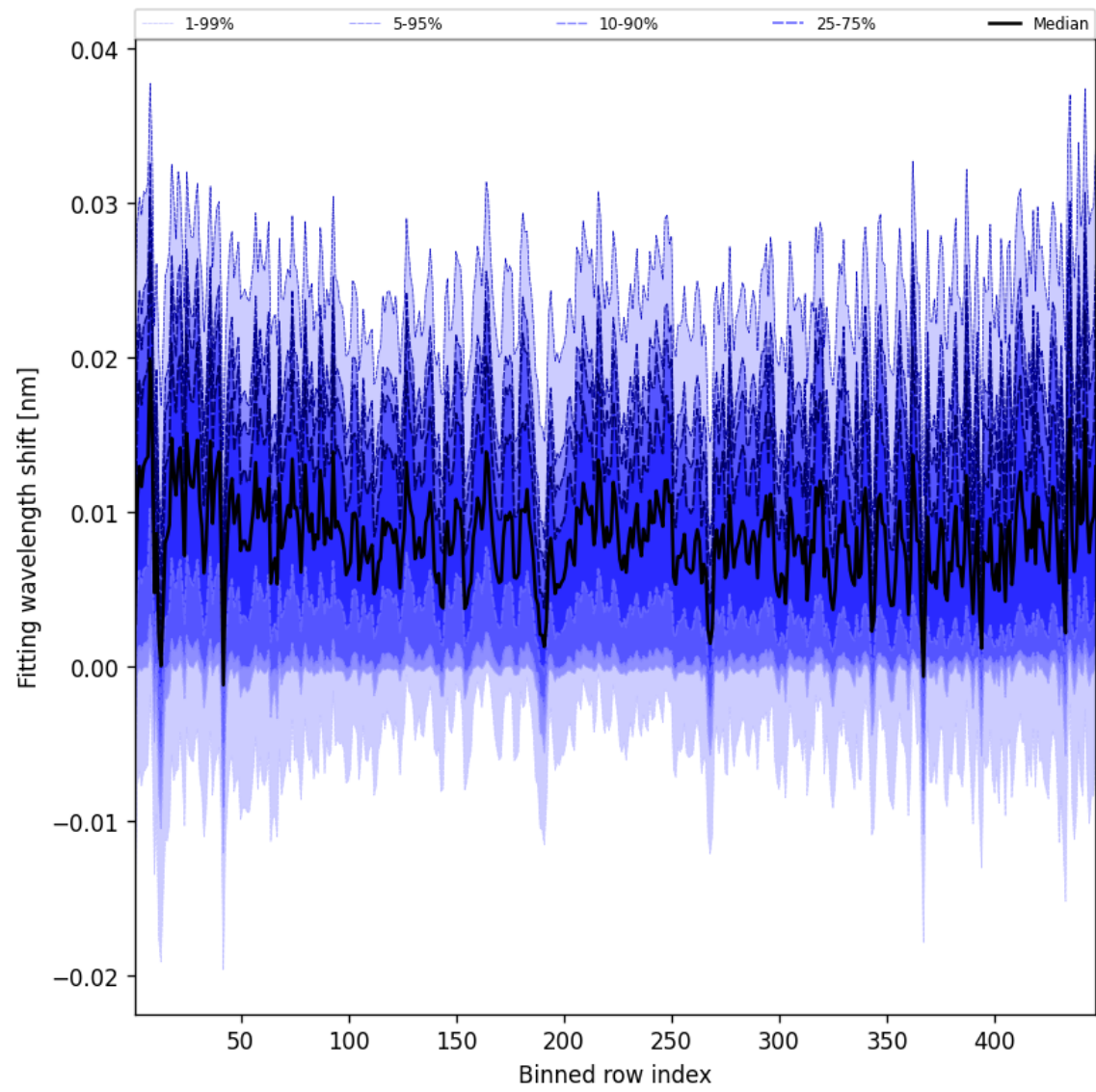
Figure 63: Along track statistics of “Fitting wavelength shift” for 2025-09-22 to 2025-09-23
