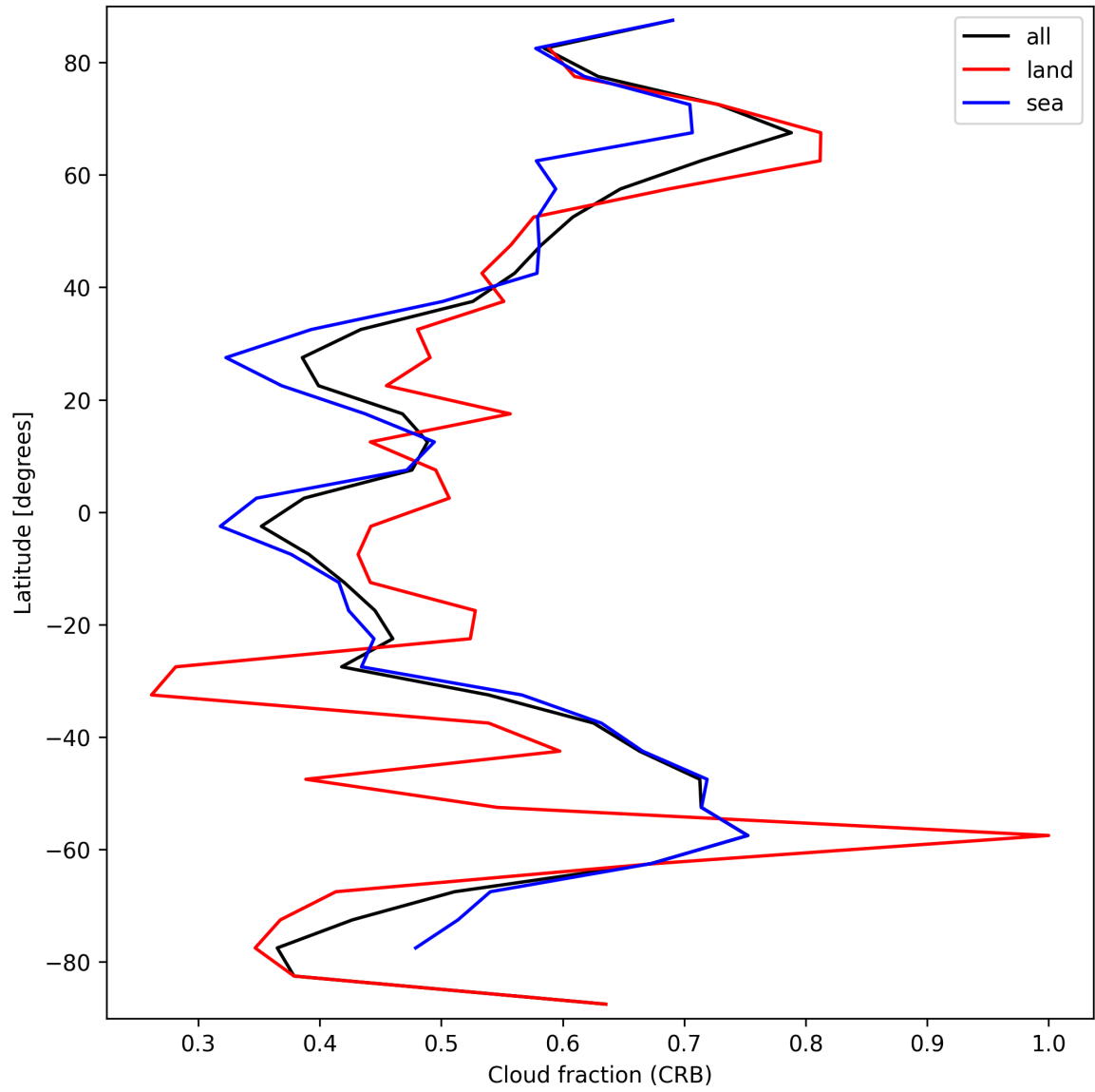
Figure 24: Zonal average of “Cloud fraction (CRB)” for 2025-09-22 to 2025-09-23.
