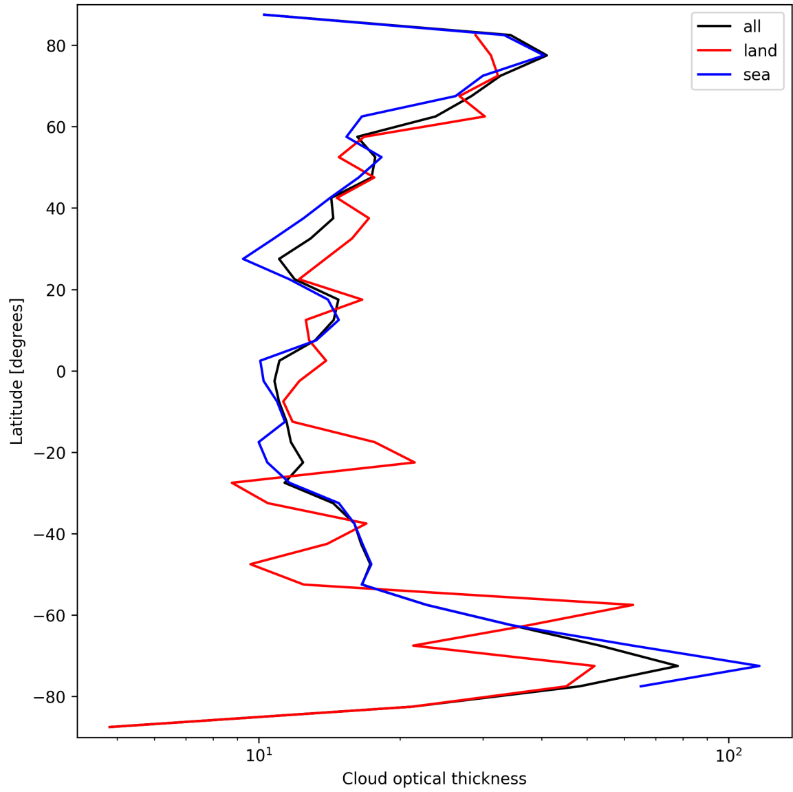
Figure 23: Zonal average of “Cloud optical thickness” for 2025-09-22 to 2025-09-23.
