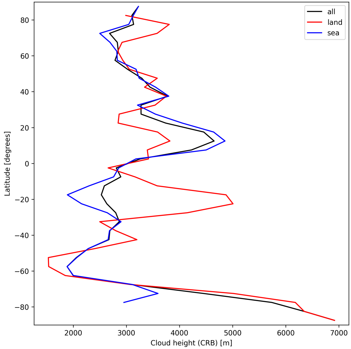
Figure 25: Zonal average of “Cloud height (CRB)” for 2025-09-22 to 2025-09-23.
