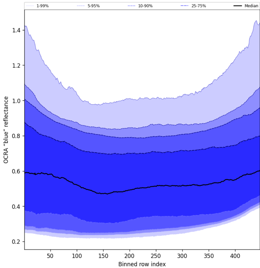
Figure 65: Along track statistics of “OCRA “blue” reflectance” for 2025-09-22 to 2025-09-23
