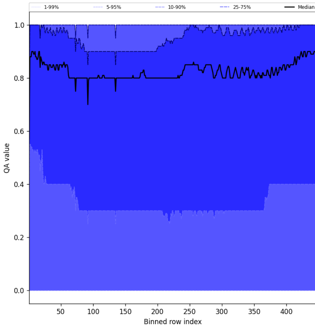
Figure 52: Along track statistics of “QA value” for 2025-09-22 to 2025-09-23
