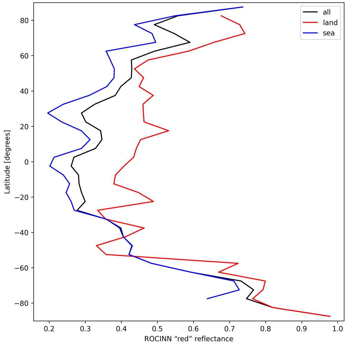
Figure 35: Zonal average of "ROCINN "red" reflectance" for 2025-09-22 to 2025-09-23.
