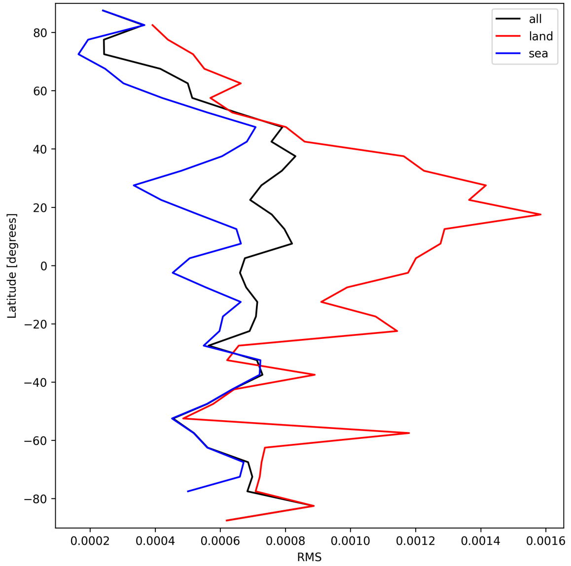
Figure 29: Zonal average of “RMS” for 2025-09-22 to 2025-09-23.
