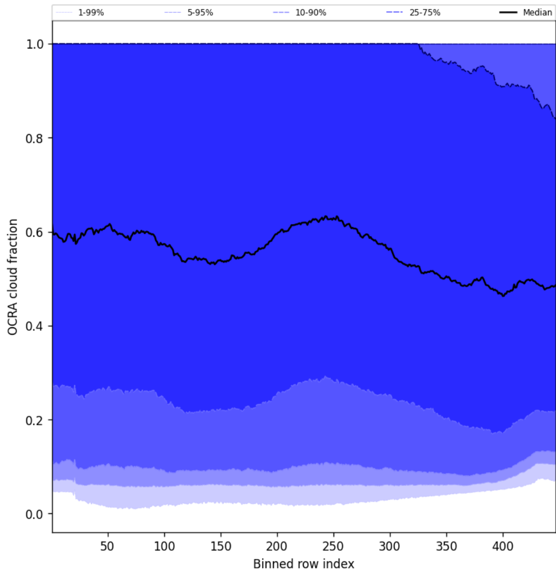
Figure 64: Along track statistics of “OCRA cloud fraction” for 2025-09-22 to 2025-09-23
