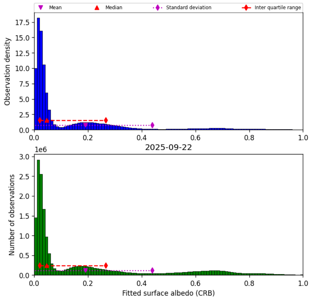
Figure 44: Histogram of “Fitted surface albedo (CRB)” for 2025-09-22 to 2025-09-23
