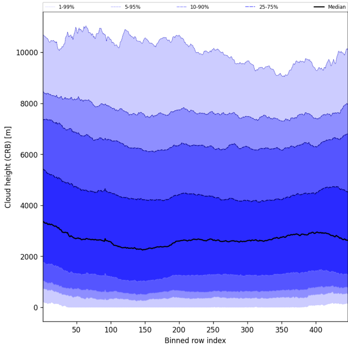
Figure 57: Along track statistics of “Cloud height (CRB)” for 2025-09-22 to 2025-09-23
