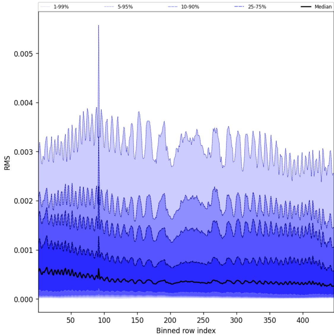
Figure 61: Along track statistics of “RMS” for 2025-09-22 to 2025-09-23
