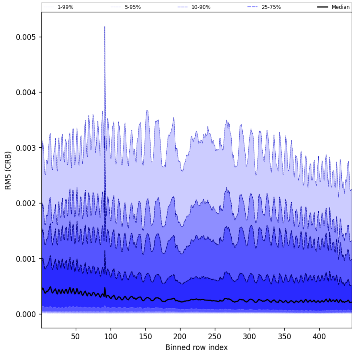
Figure 62: Along track statistics of “RMS (CRB)” for 2025-09-22 to 2025-09-23
