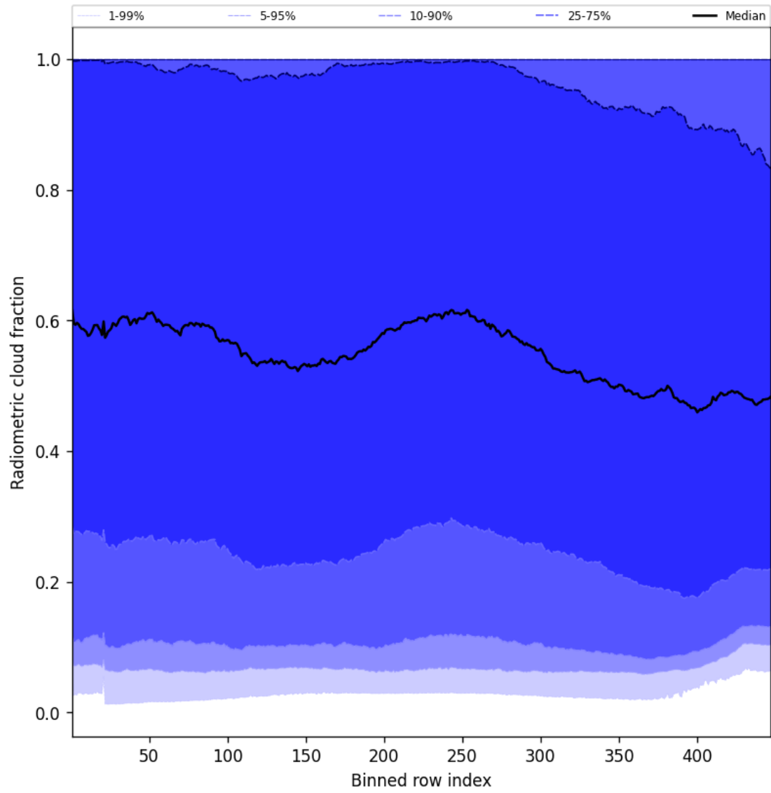
Figure 53: Along track statistics of “Radiometric cloud fraction” for 2025-09-22 to 2025-09-23
