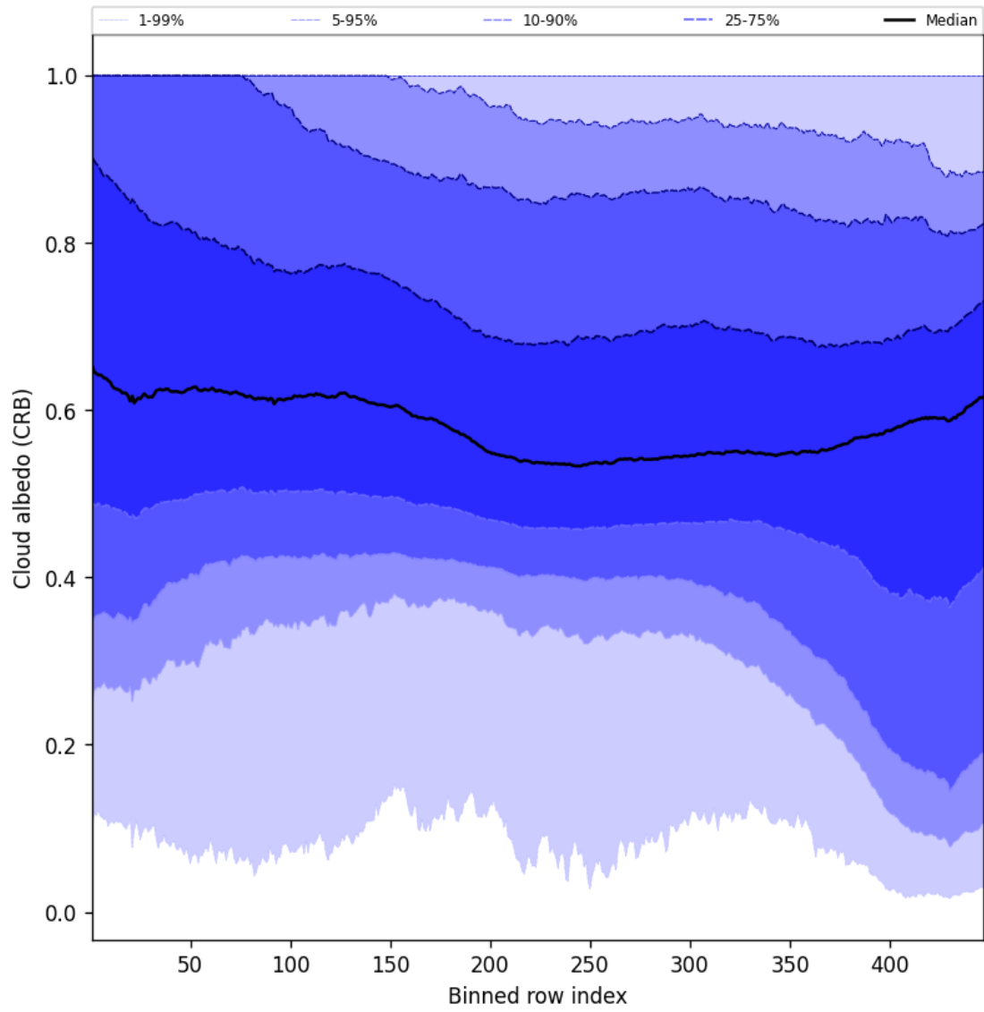
Figure 58: Along track statistics of “Cloud albedo (CRB)” for 2025-09-22 to 2025-09-23
