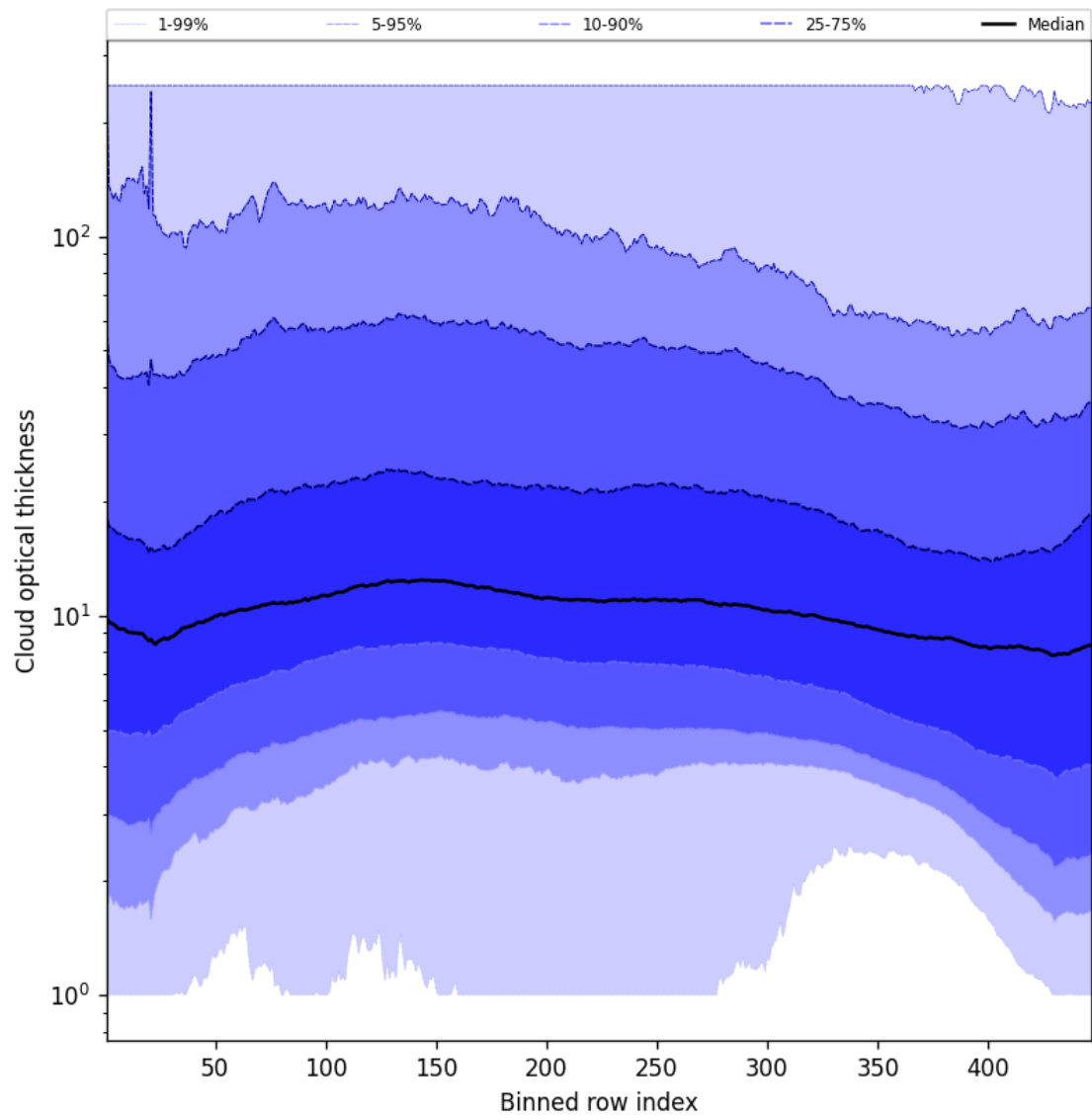
Figure 55: Along track statistics of “Cloud optical thickness” for 2025-09-22 to 2025-09-23
