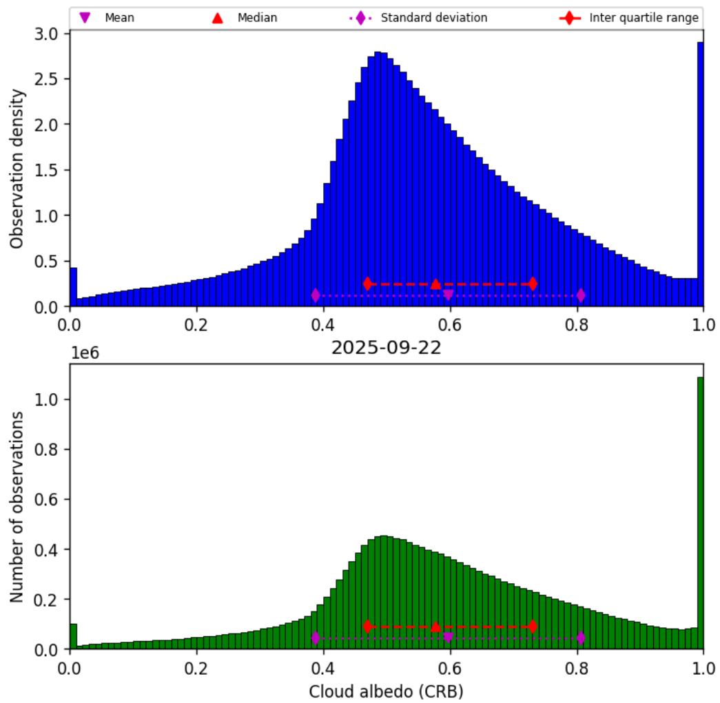
Figure 42: Histogram of “Cloud albedo (CRB)” for 2025-09-22 to 2025-09-23
