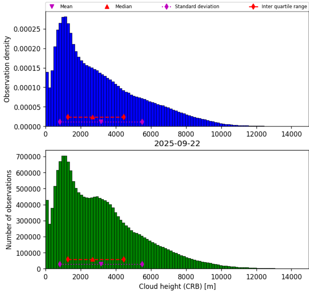
Figure 41: Histogram of “Cloud height (CRB)” for 2025-09-22 to 2025-09-23
