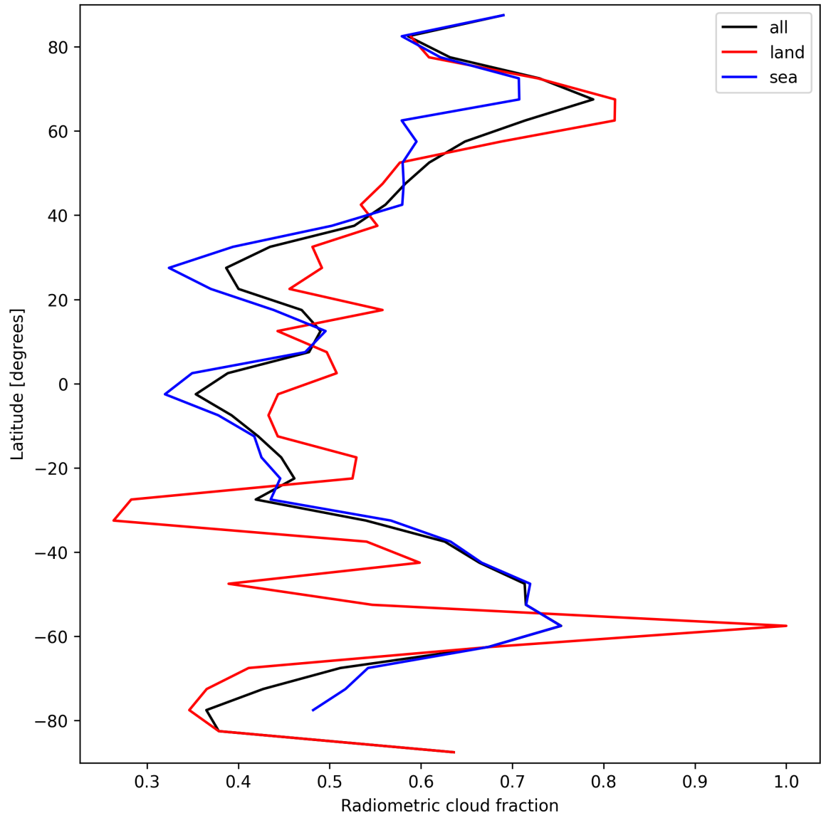
Figure 21: Zonal average of “Radiometric cloud fraction” for 2025-09-22 to 2025-09-23.
