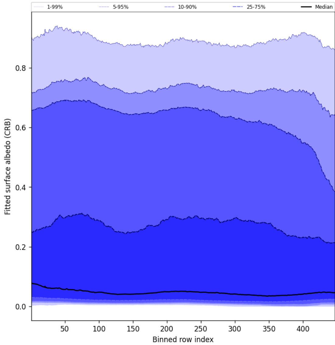
Figure 60: Along track statistics of “Fitted surface albedo (CRB)” for 2025-09-22 to 2025-09-23
