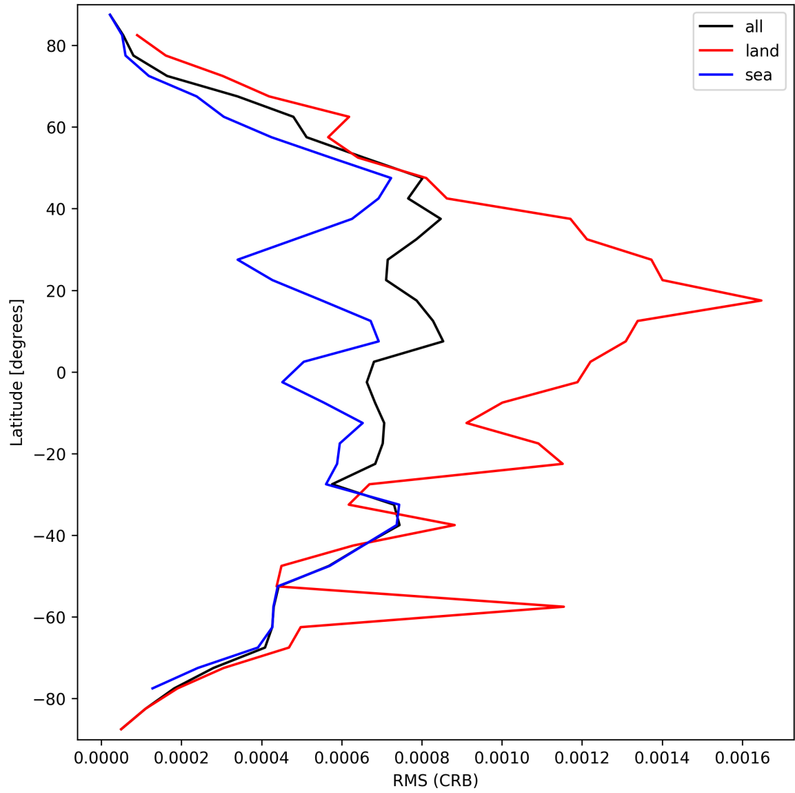
Figure 30: Zonal average of “RMS (CRB)” for 2025-09-22 to 2025-09-23.
