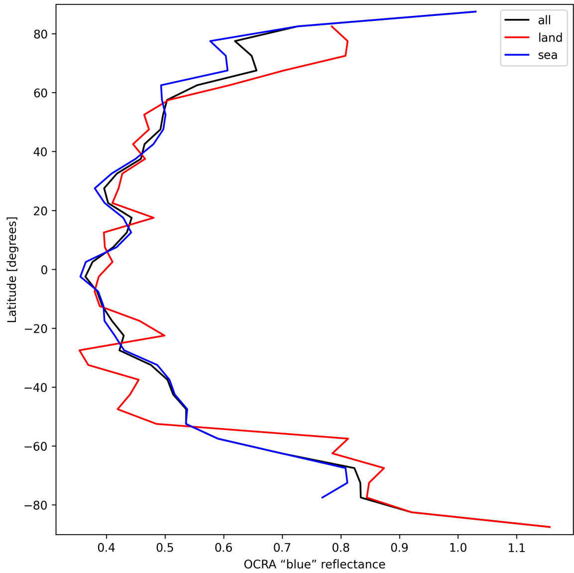
Figure 33: Zonal average of “OCRA “blue” reflectance” for 2025-09-22 to 2025-09-23.
