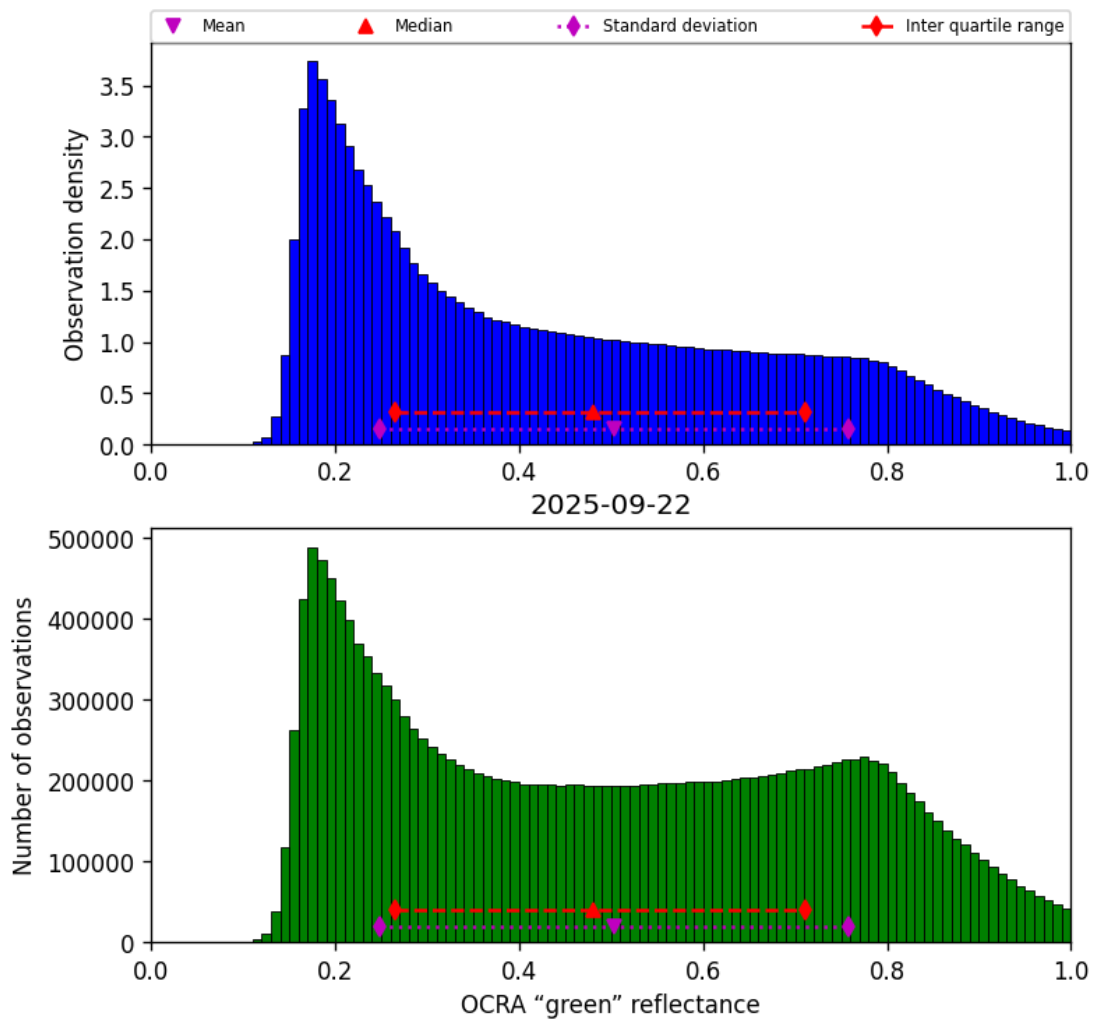
Figure 50: Histogram of “OCRA “green” reflectance” for 2025-09-22 to 2025-09-23
