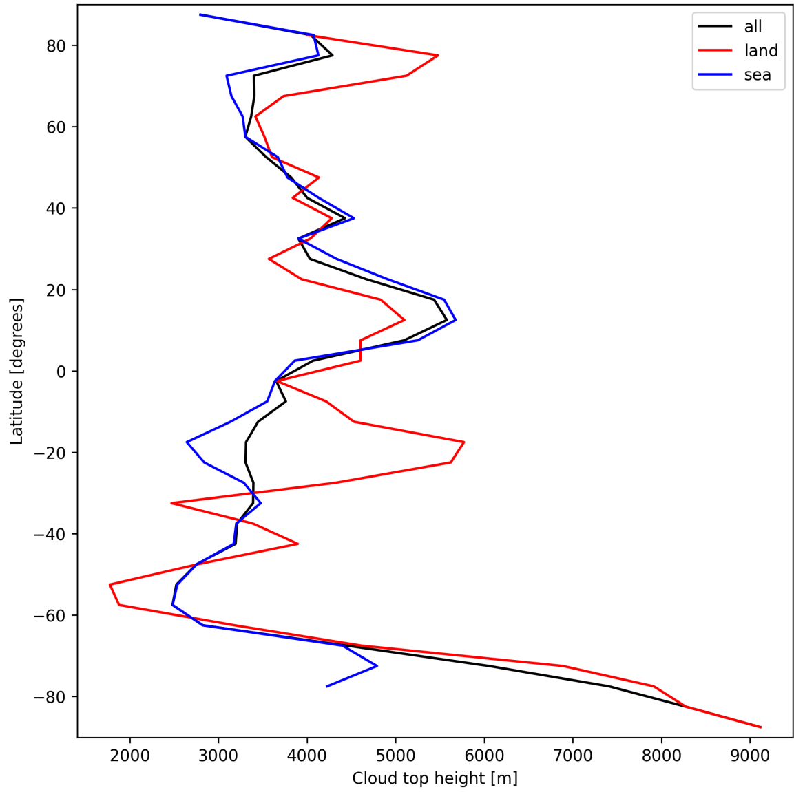
Figure 22: Zonal average of “Cloud top height” for 2025-09-22 to 2025-09-23.
