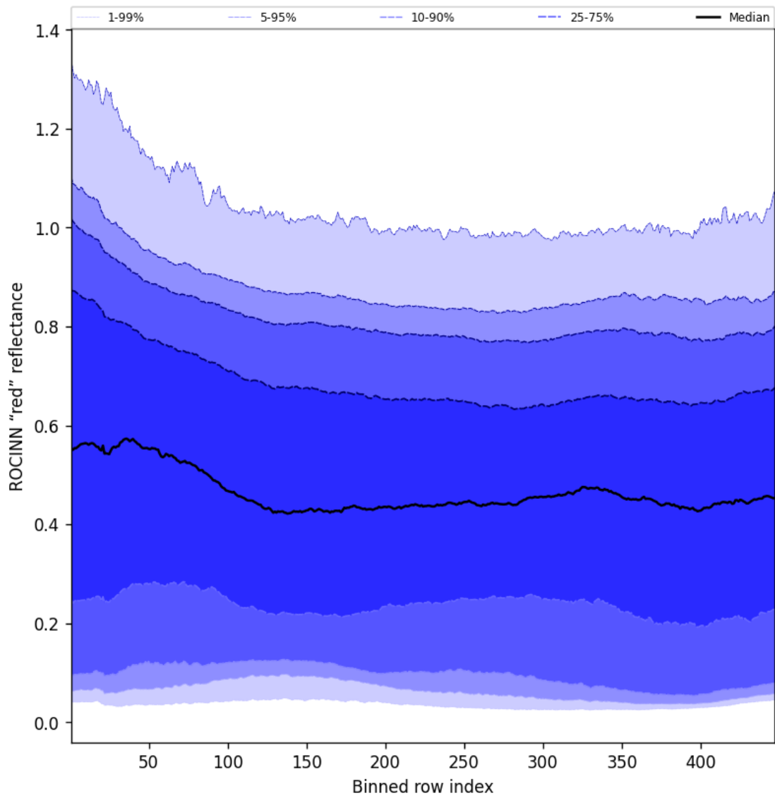
Figure 67: Along track statistics of “ROCINN “red” reflectance” for 2025-09-26 to 2025-09-27
