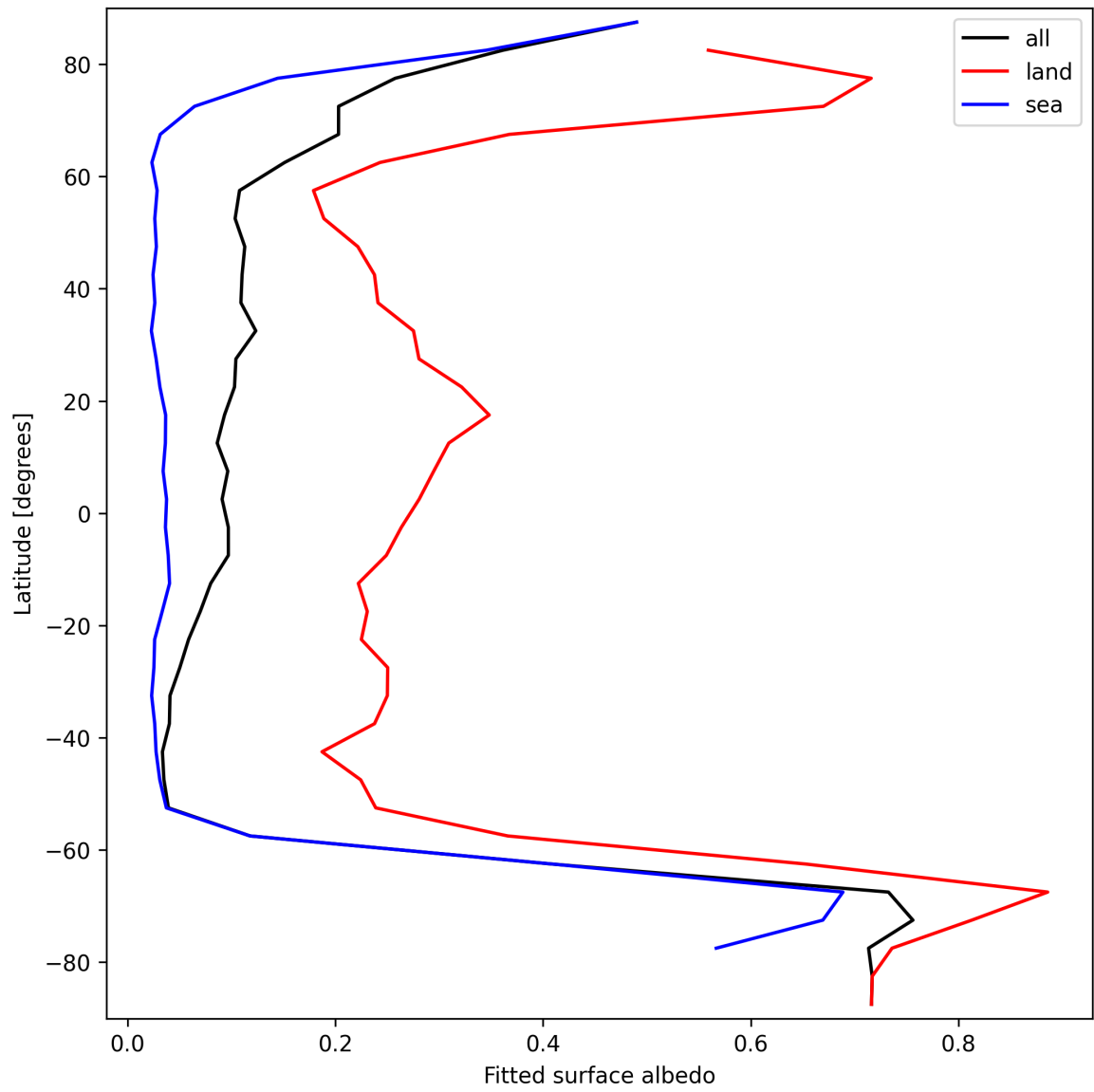
Figure 27: Zonal average of “Fitted surface albedo” for 2025-09-26 to 2025-09-27.
