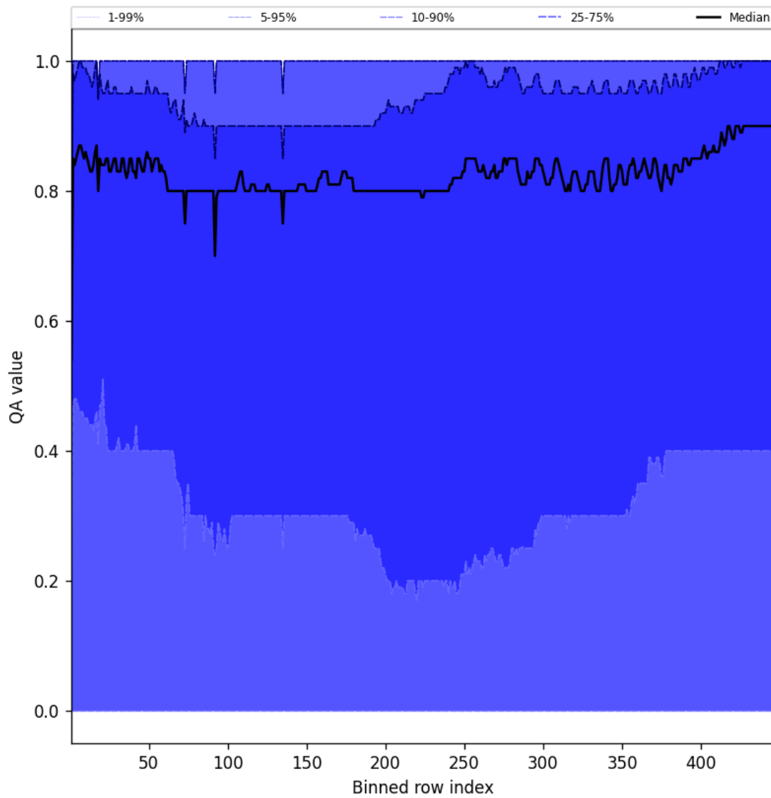
Figure 52: Along track statistics of “QA value” for 2025-09-26 to 2025-09-27
