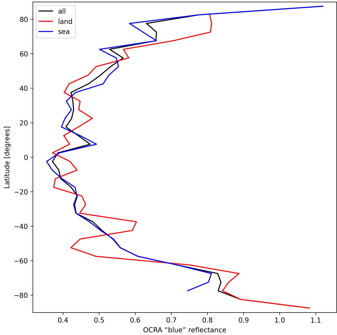
Figure 33: Zonal average of “OCRA “blue” reflectance” for 2025-09-26 to 2025-09-27.
