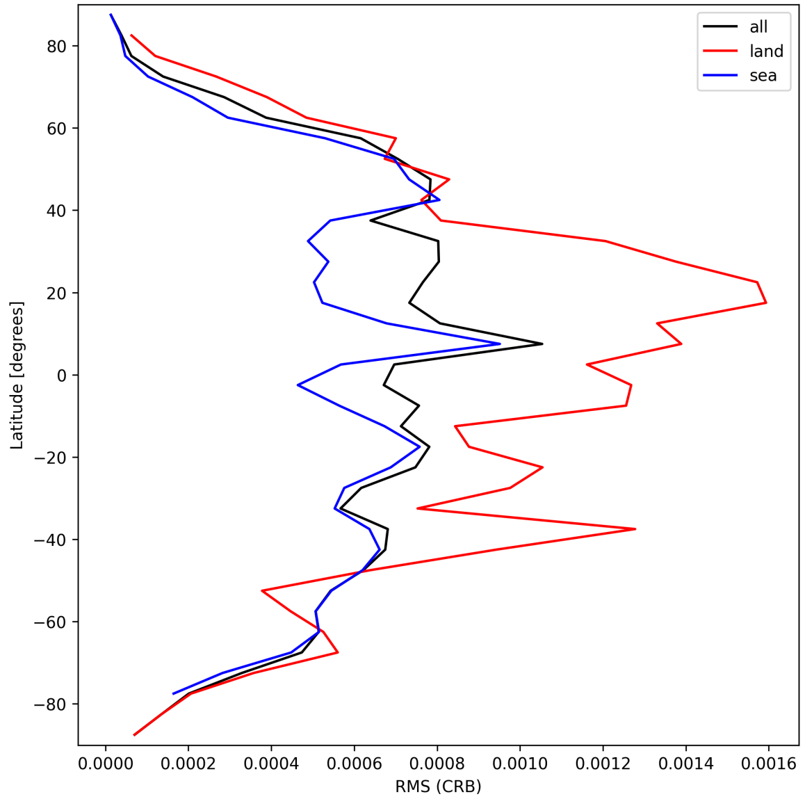
Figure 30: Zonal average of “RMS (CRB)” for 2025-09-26 to 2025-09-27.
