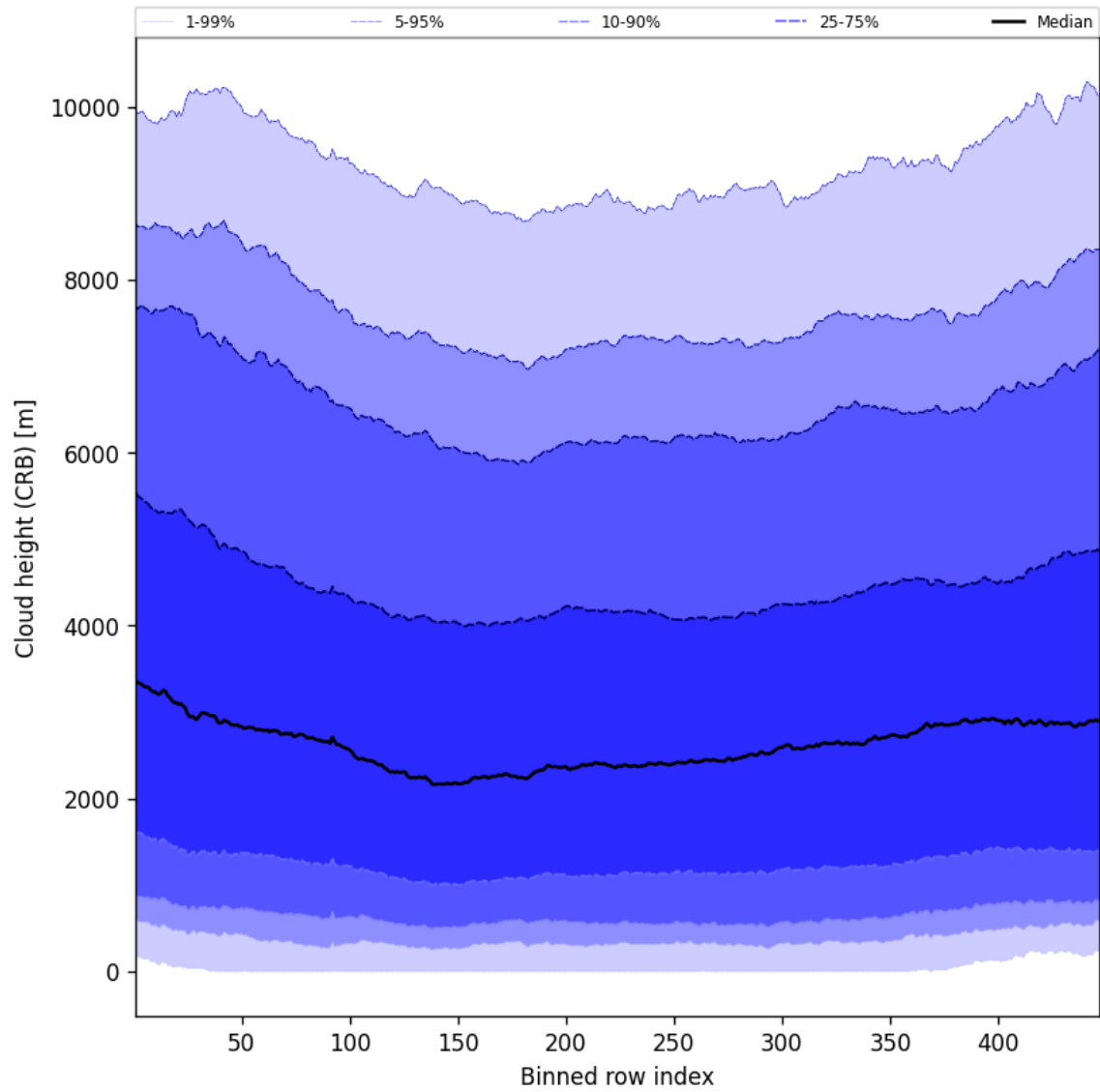
Figure 57: Along track statistics of “Cloud height (CRB)” for 2025-09-26 to 2025-09-27
