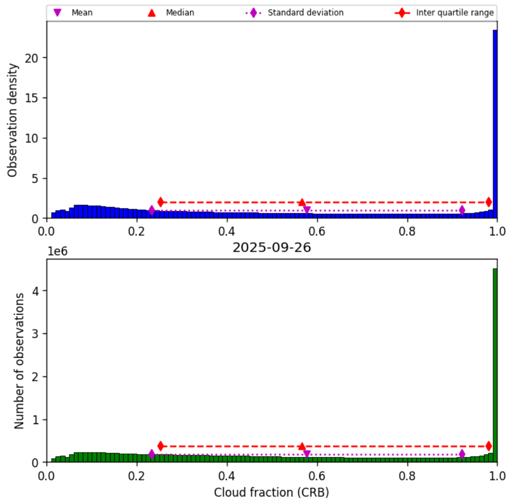
Figure 40: Histogram of “Cloud fraction (CRB)” for 2025-09-26 to 2025-09-27
