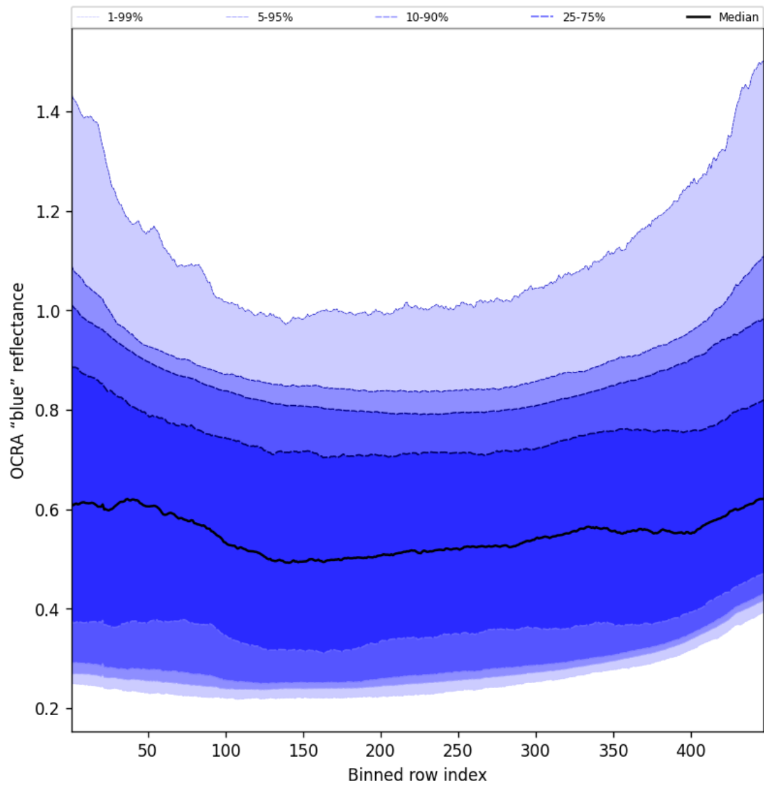
Figure 65: Along track statistics of “OCRA “blue” reflectance” for 2025-09-26 to 2025-09-27
