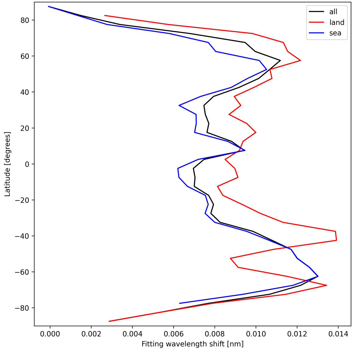
Figure 31: Zonal average of “Fitting wavelength shift” for 2025-09-26 to 2025-09-27.
