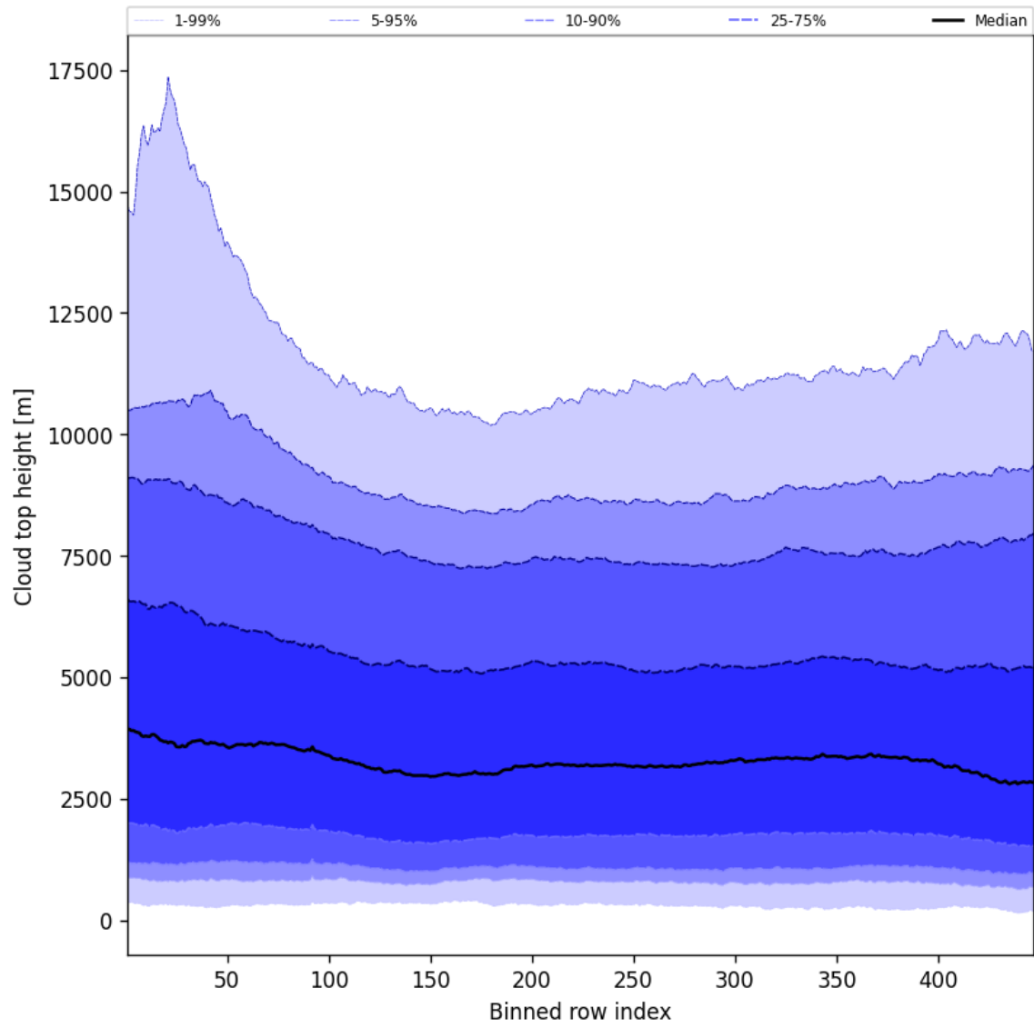
Figure 54: Along track statistics of “Cloud top height” for 2025-09-26 to 2025-09-27
