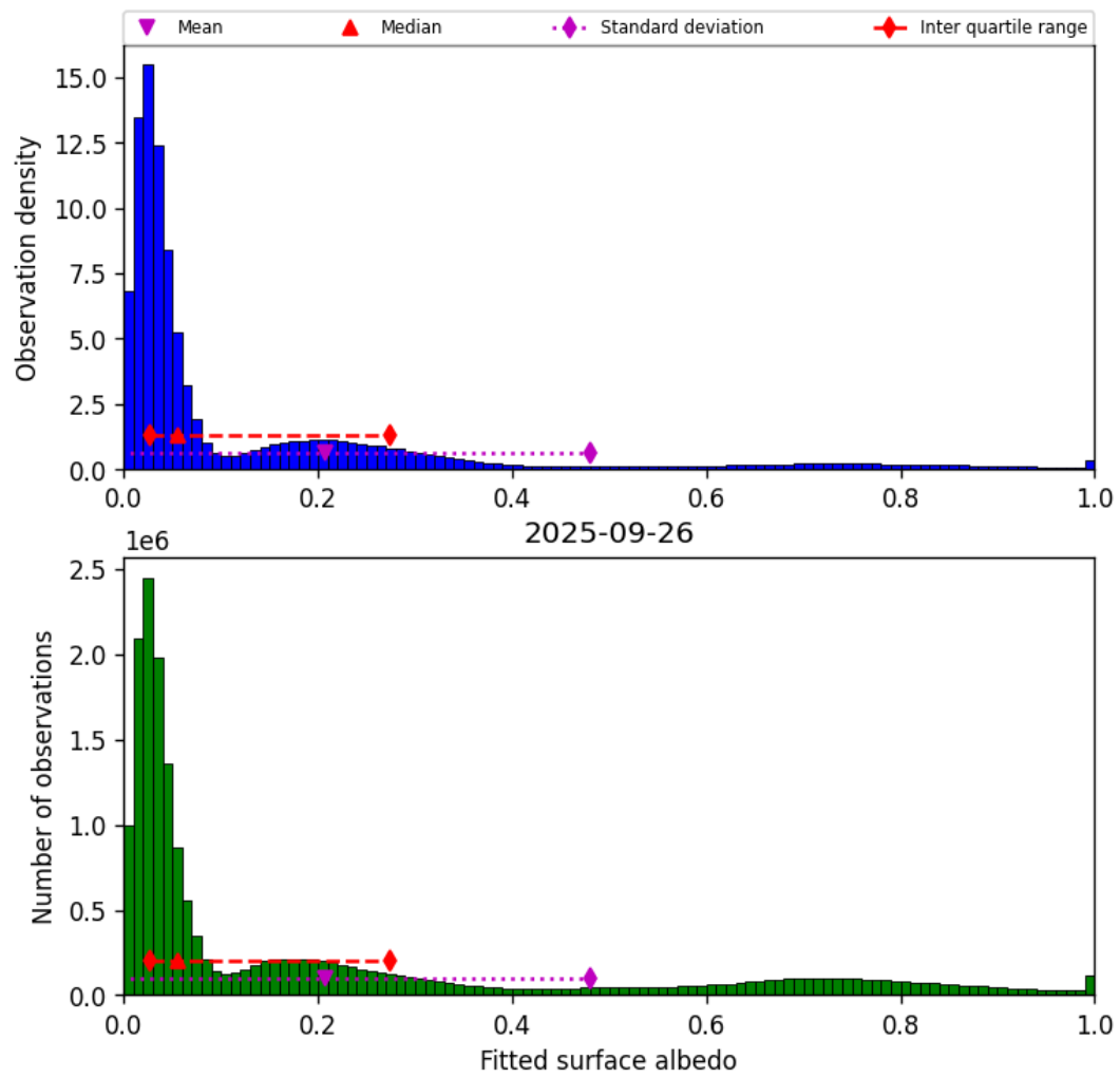
Figure 43: Histogram of “Fitted surface albedo” for 2025-09-26 to 2025-09-27
