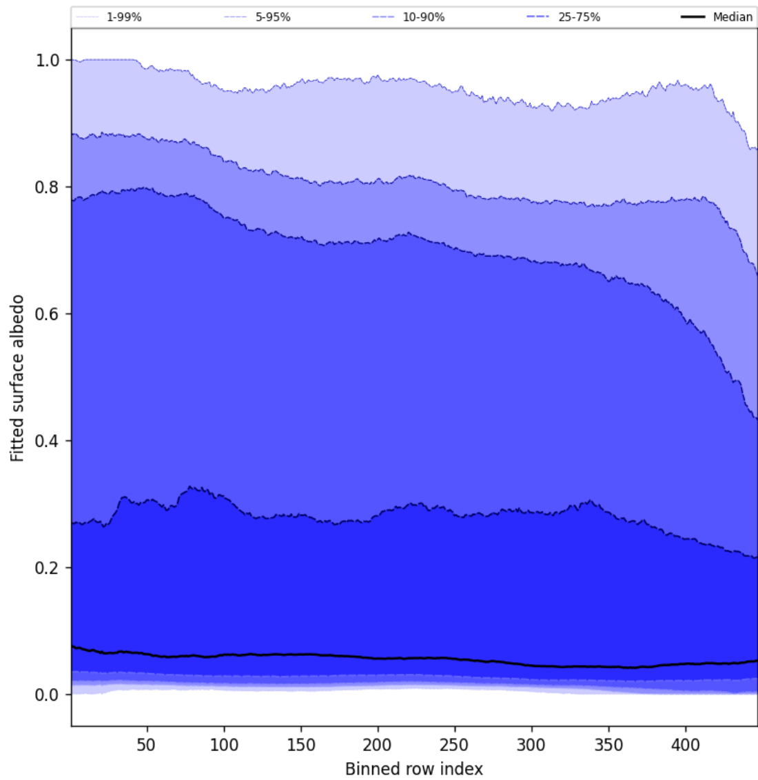
Figure 59: Along track statistics of “Fitted surface albedo” for 2025-09-26 to 2025-09-27
