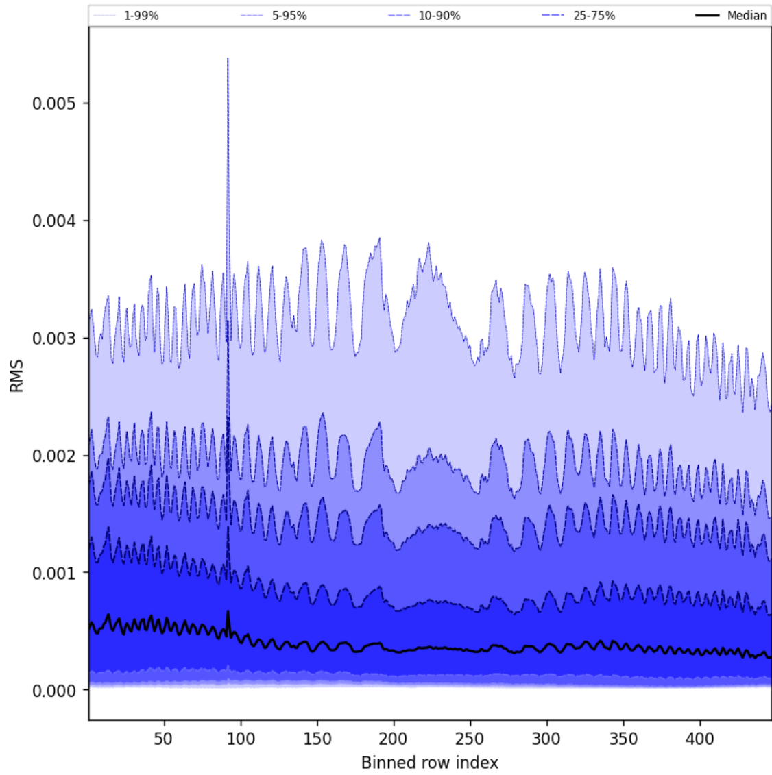
Figure 61: Along track statistics of “RMS” for 2025-09-26 to 2025-09-27
