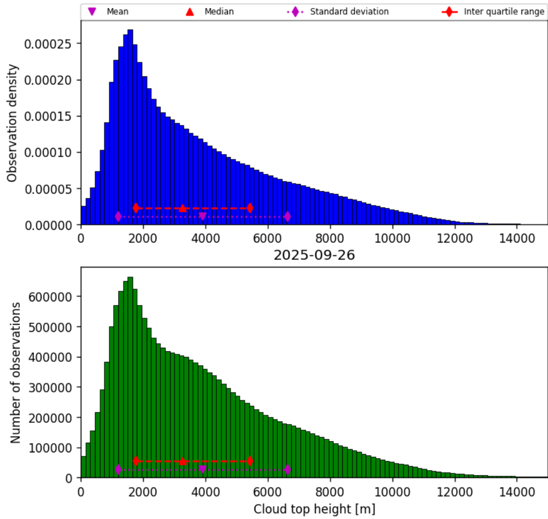
Figure 38: Histogram of “Cloud top height” for 2025-09-26 to 2025-09-27
