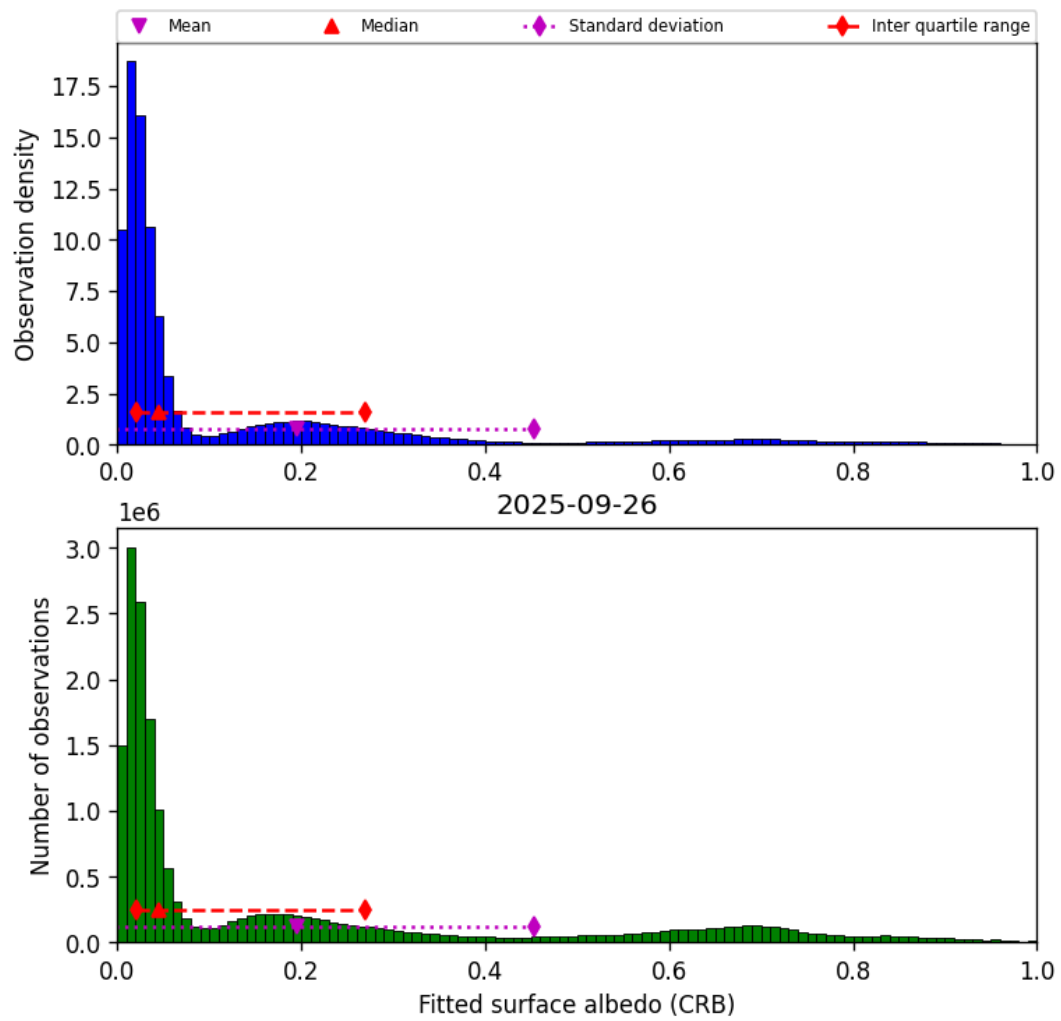
Figure 44: Histogram of “Fitted surface albedo (CRB)” for 2025-09-26 to 2025-09-27
