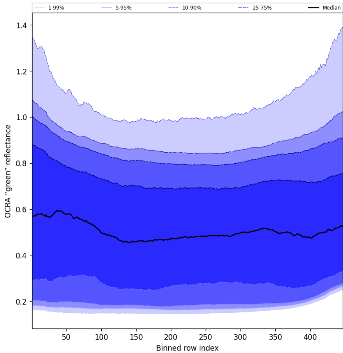
Figure 66: Along track statistics of “OCRA “green” reflectance” for 2025-09-26 to 2025-09-27
