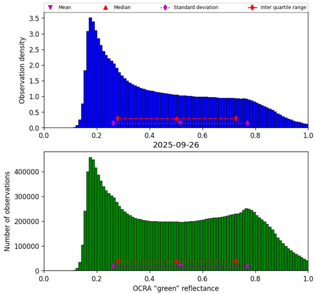
Figure 50: Histogram of “OCRA “green” reflectance” for 2025-09-26 to 2025-09-27
