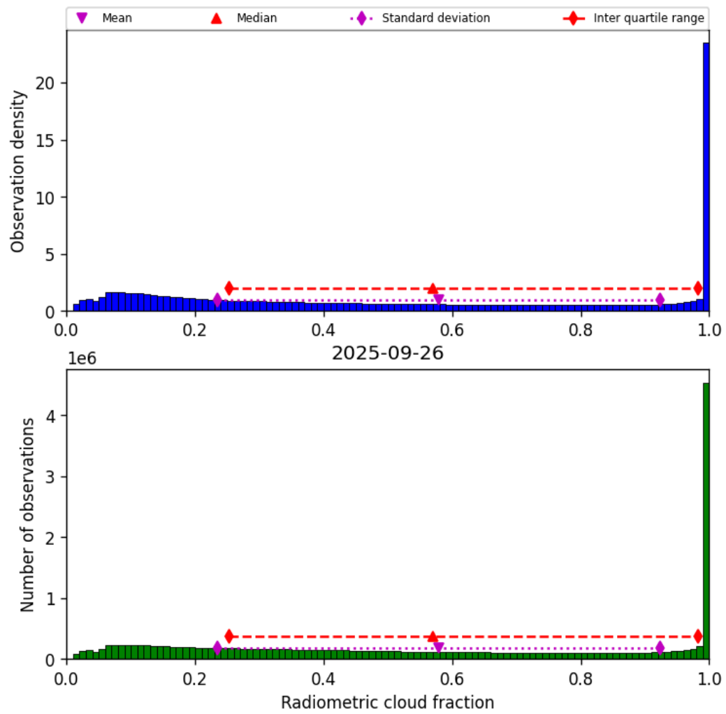
Figure 37: Histogram of “Radiometric cloud fraction” for 2025-09-26 to 2025-09-27
