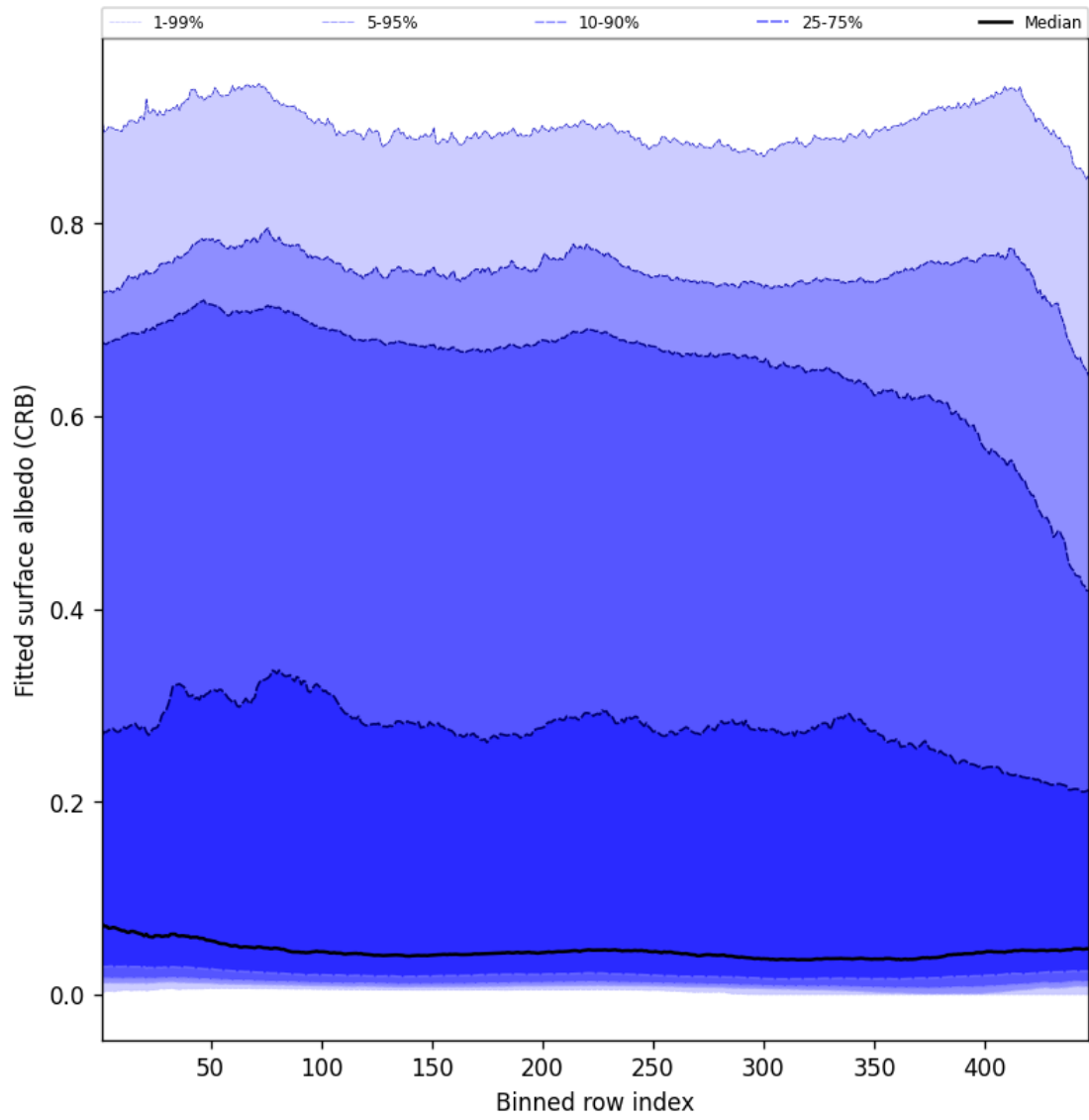
Figure 60: Along track statistics of “Fitted surface albedo (CRB)” for 2025-09-26 to 2025-09-27
