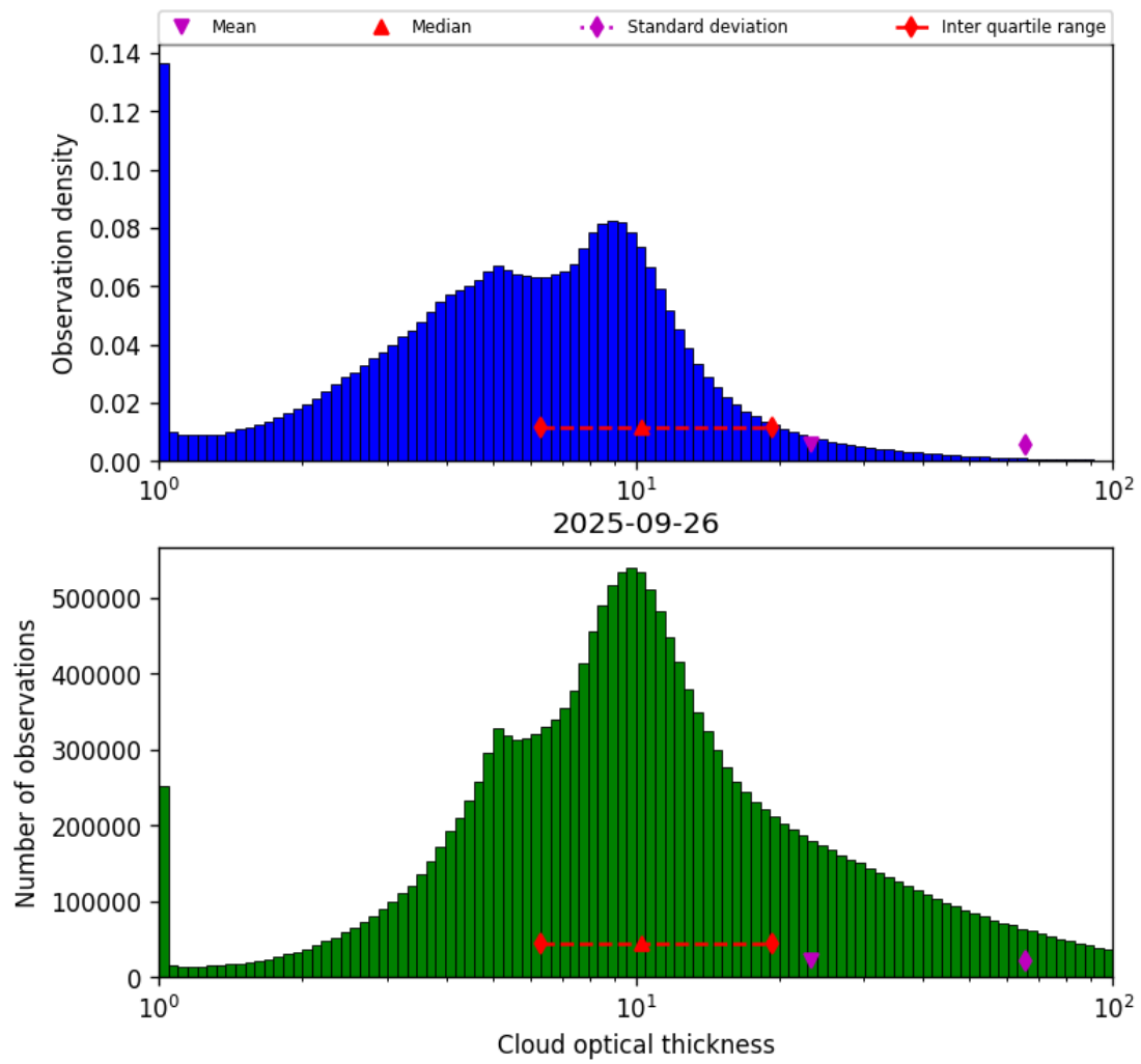
Figure 39: Histogram of “Cloud optical thickness” for 2025-09-26 to 2025-09-27
