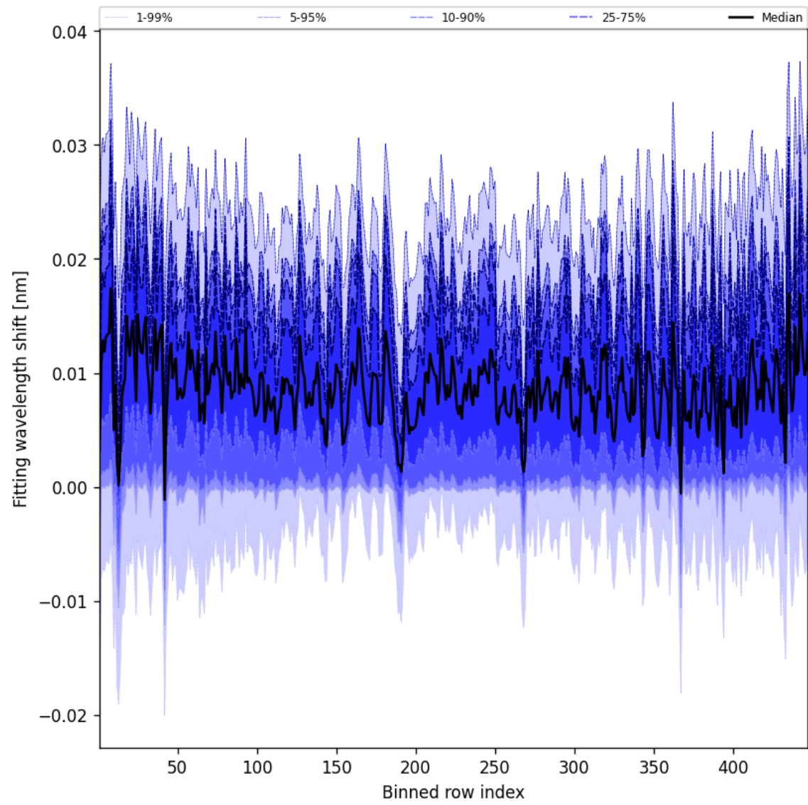
Figure 63: Along track statistics of “Fitting wavelength shift” for 2025-09-26 to 2025-09-27
