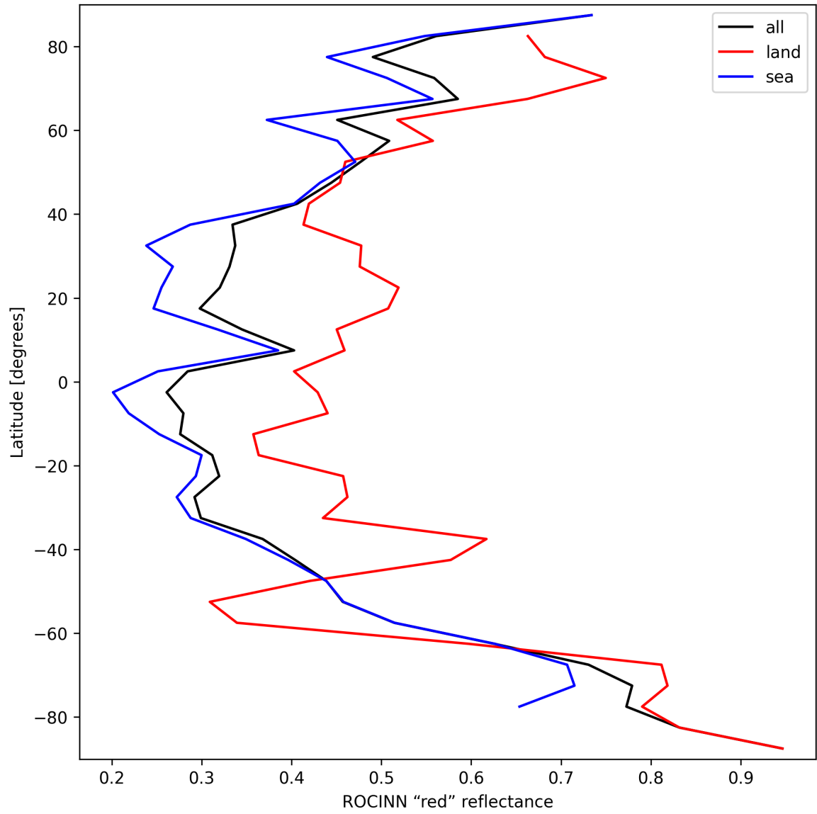
Figure 35: Zonal average of "ROCINN "red" reflectance" for 2025-09-26 to 2025-09-27.
