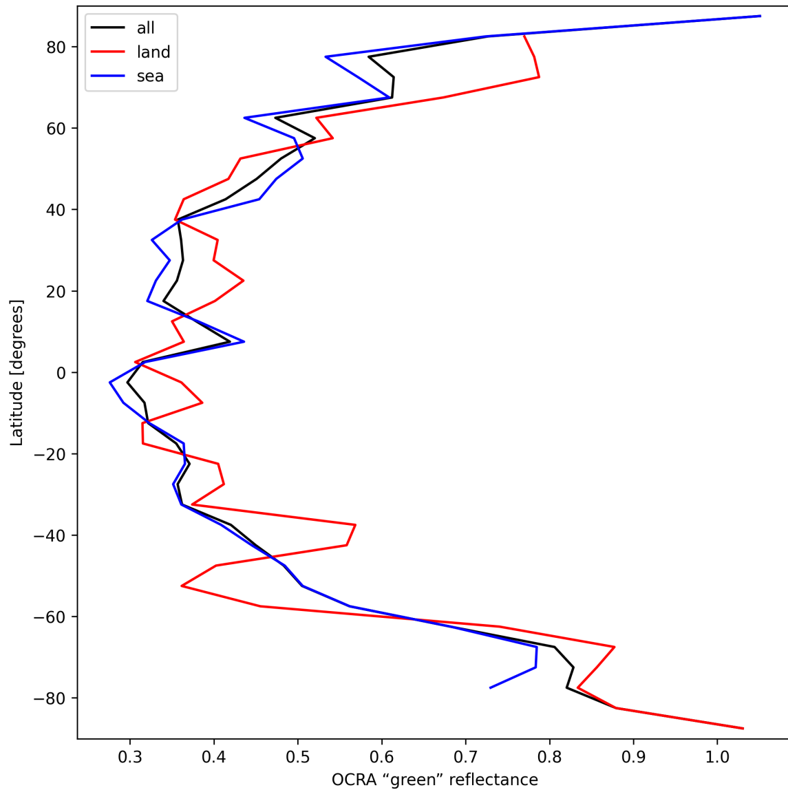
Figure 34: Zonal average of “OCRA “green” reflectance” for 2025-09-26 to 2025-09-27.
