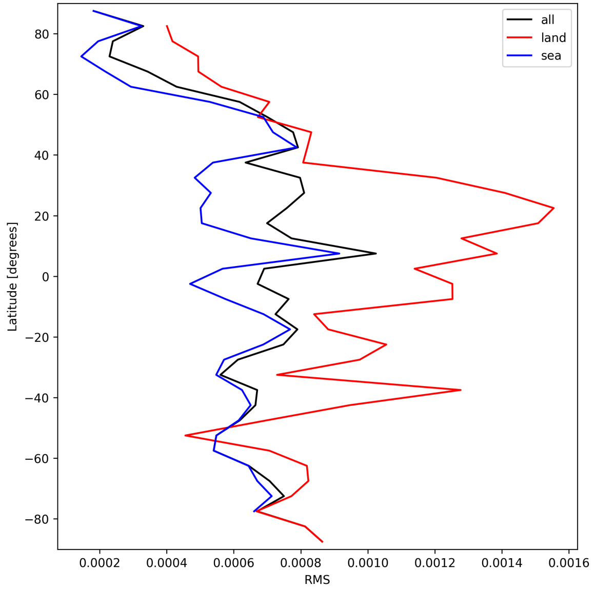
Figure 29: Zonal average of “RMS” for 2025-09-26 to 2025-09-27.
