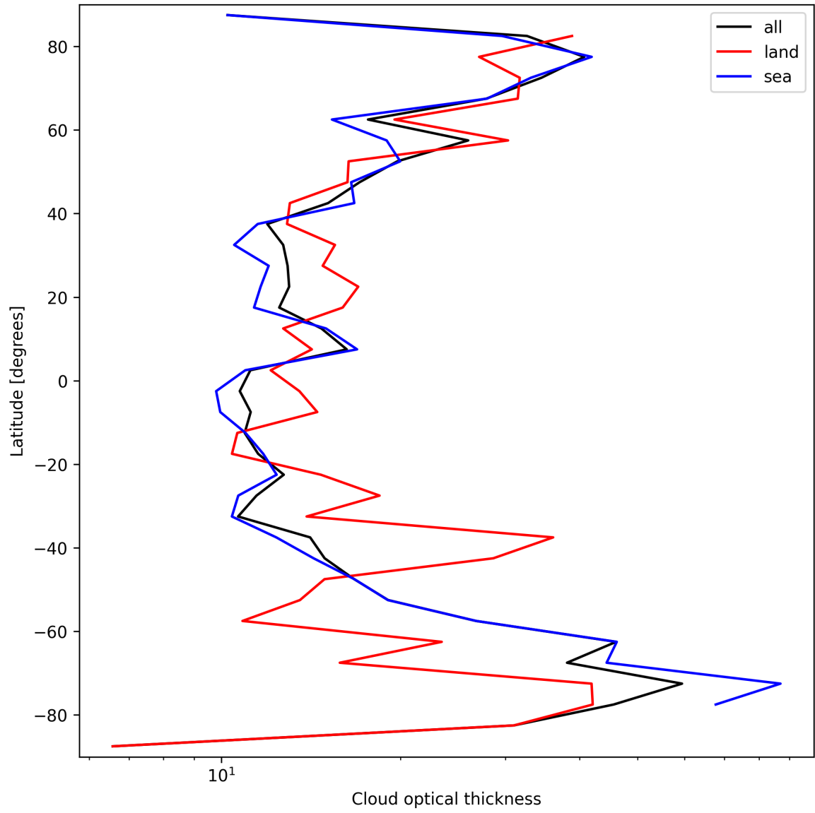
Figure 23: Zonal average of “Cloud optical thickness” for 2025-09-26 to 2025-09-27.
