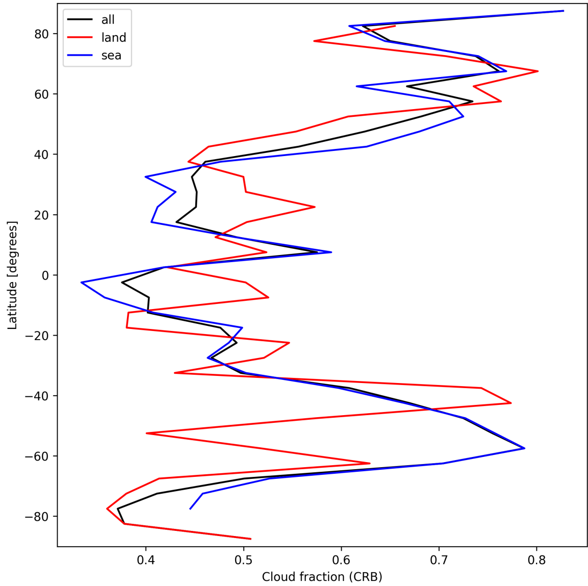
Figure 24: Zonal average of “Cloud fraction (CRB)” for 2025-09-26 to 2025-09-27.
