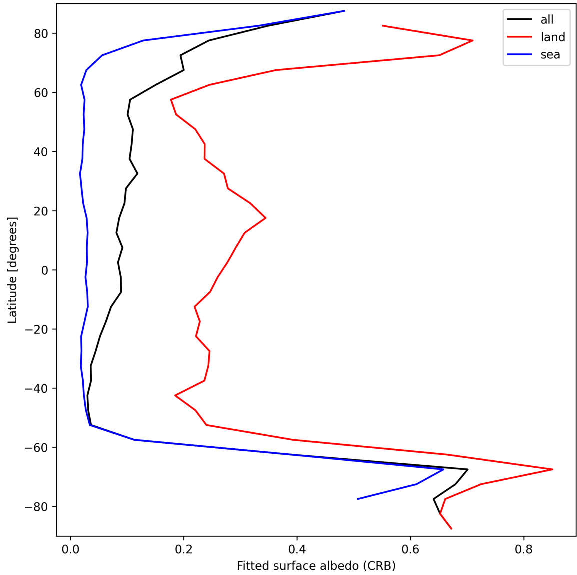
Figure 28: Zonal average of “Fitted surface albedo (CRB)” for 2025-09-26 to 2025-09-27.
