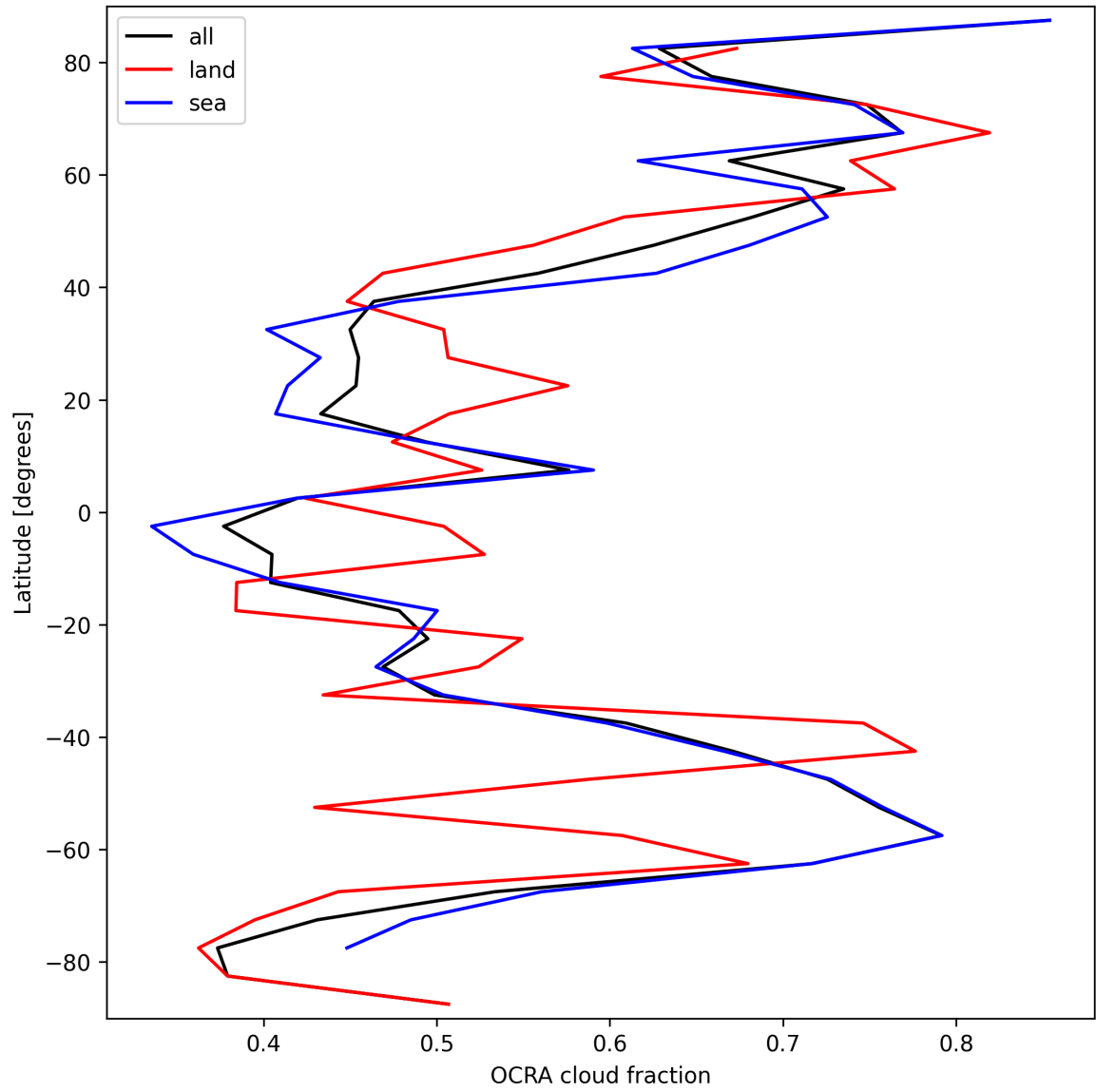
Figure 32: Zonal average of “OCRA cloud fraction” for 2025-09-26 to 2025-09-27.
