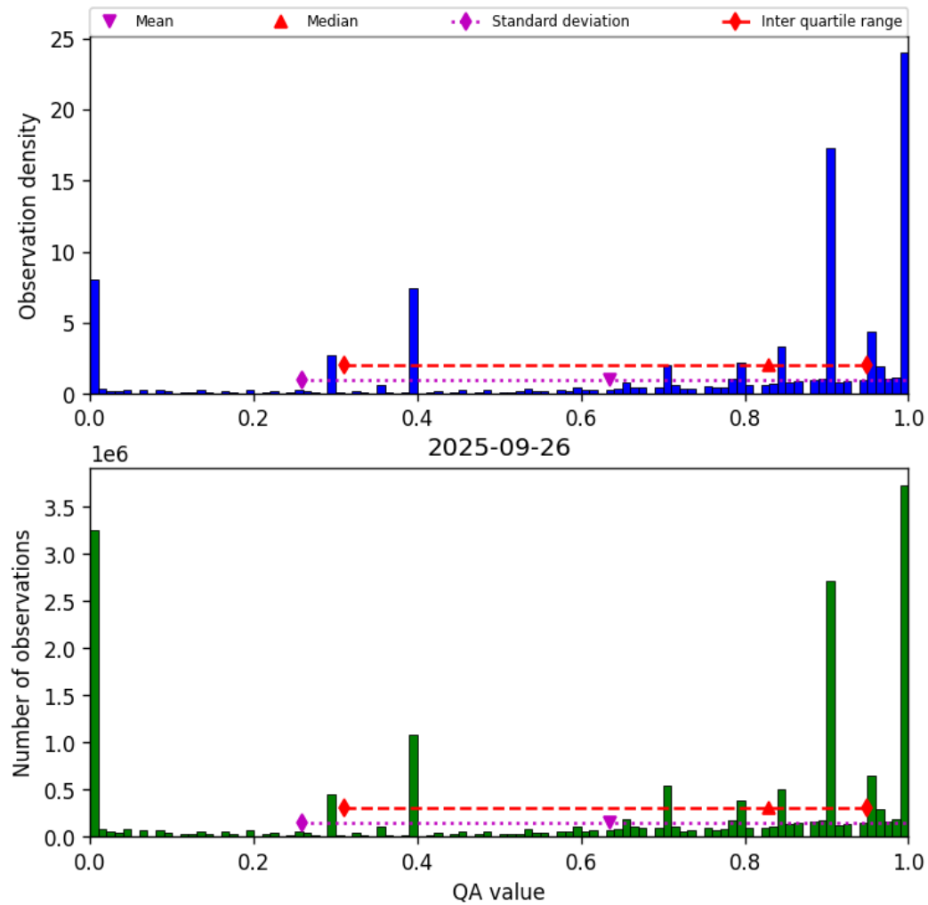
Figure 36: Histogram of “QA value” for 2025-09-26 to 2025-09-27
