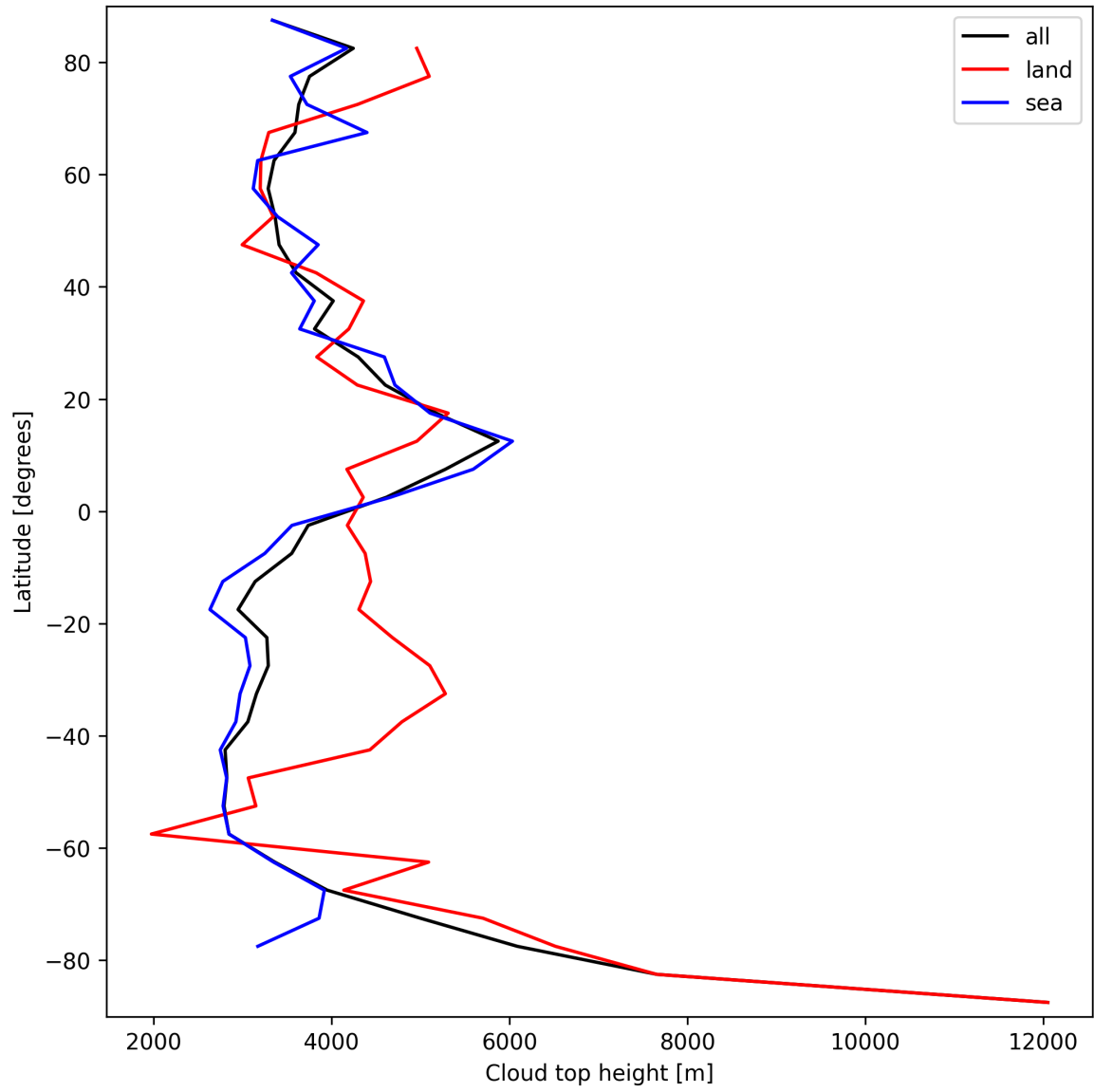
Figure 22: Zonal average of “Cloud top height” for 2025-09-26 to 2025-09-27.
