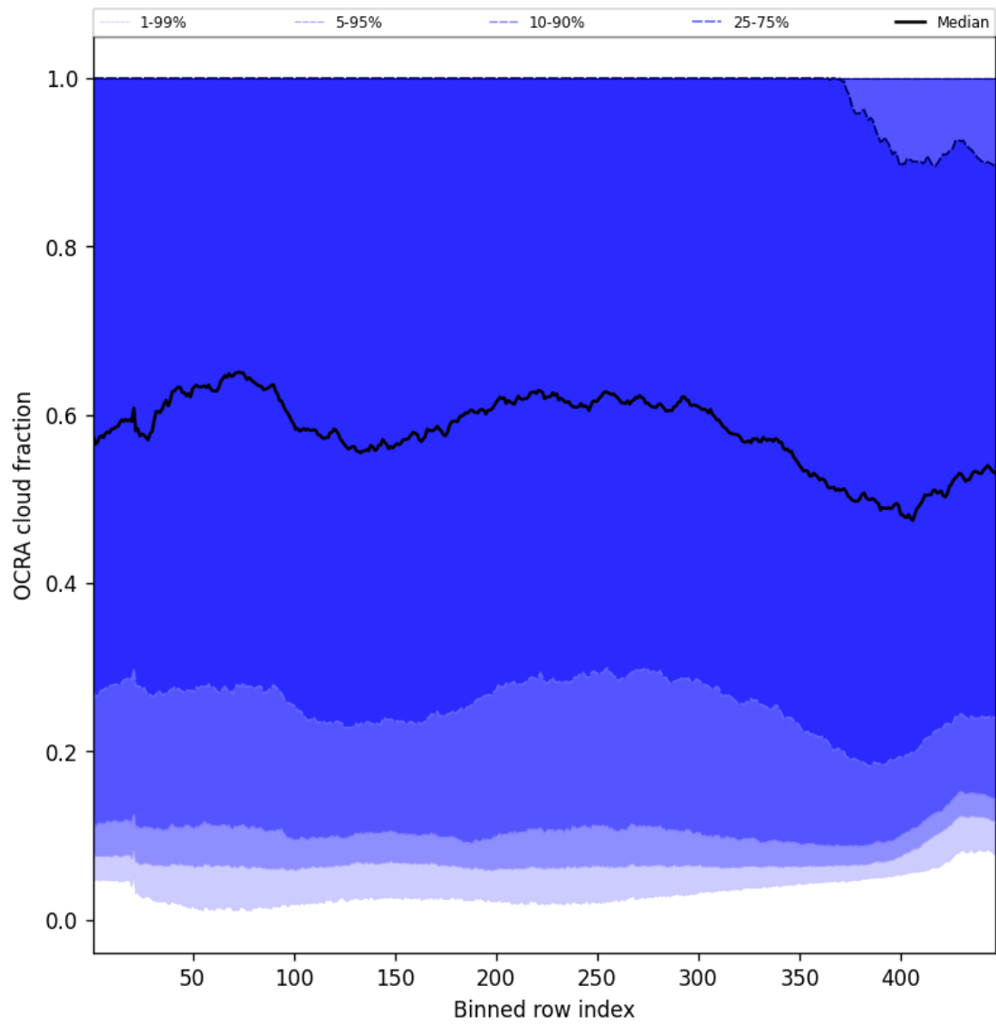
Figure 64: Along track statistics of “OCRA cloud fraction” for 2025-09-26 to 2025-09-27
