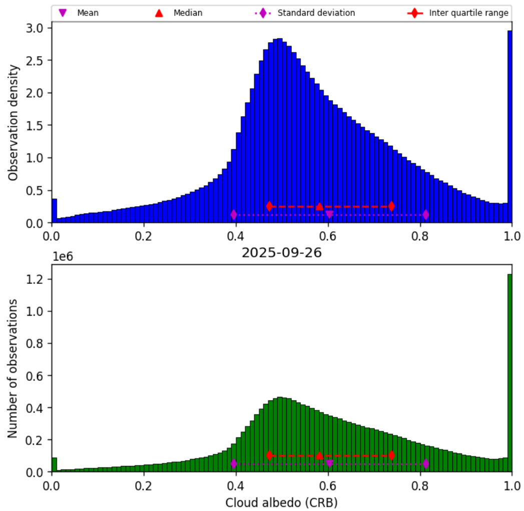
Figure 42: Histogram of “Cloud albedo (CRB)” for 2025-09-26 to 2025-09-27
