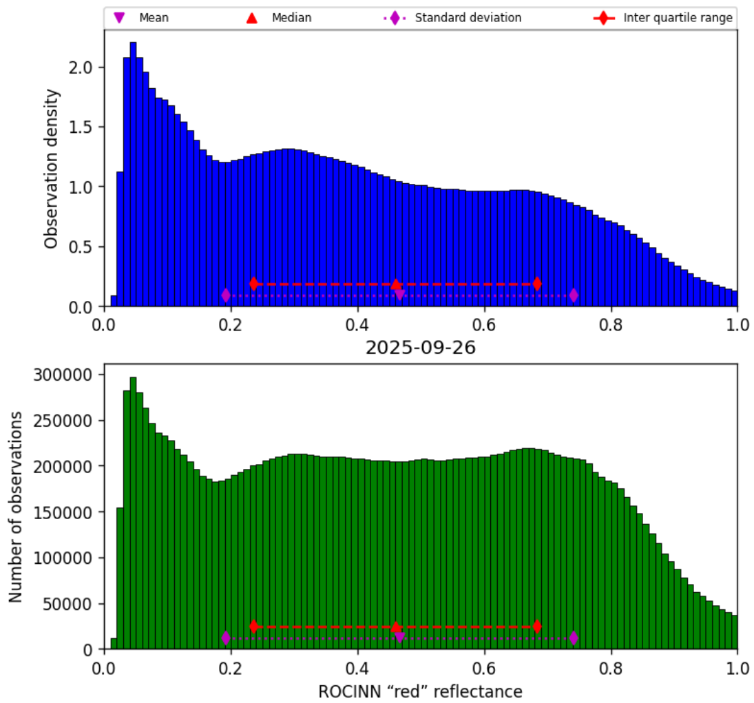
Figure 51: Histogram of “ROCINN “red” reflectance” for 2025-09-26 to 2025-09-27
