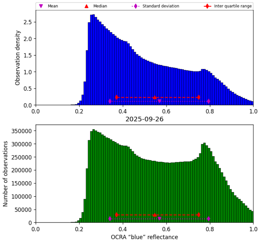
Figure 49: Histogram of “OCRA “blue” reflectance” for 2025-09-26 to 2025-09-27
