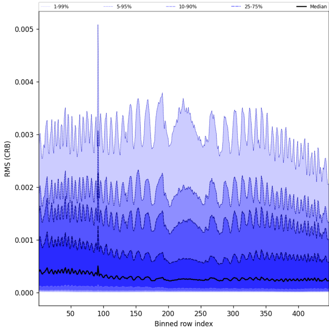
Figure 62: Along track statistics of “RMS (CRB)” for 2025-09-26 to 2025-09-27
