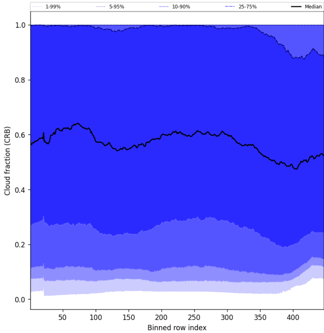
Figure 56: Along track statistics of “Cloud fraction (CRB)” for 2025-09-26 to 2025-09-27
