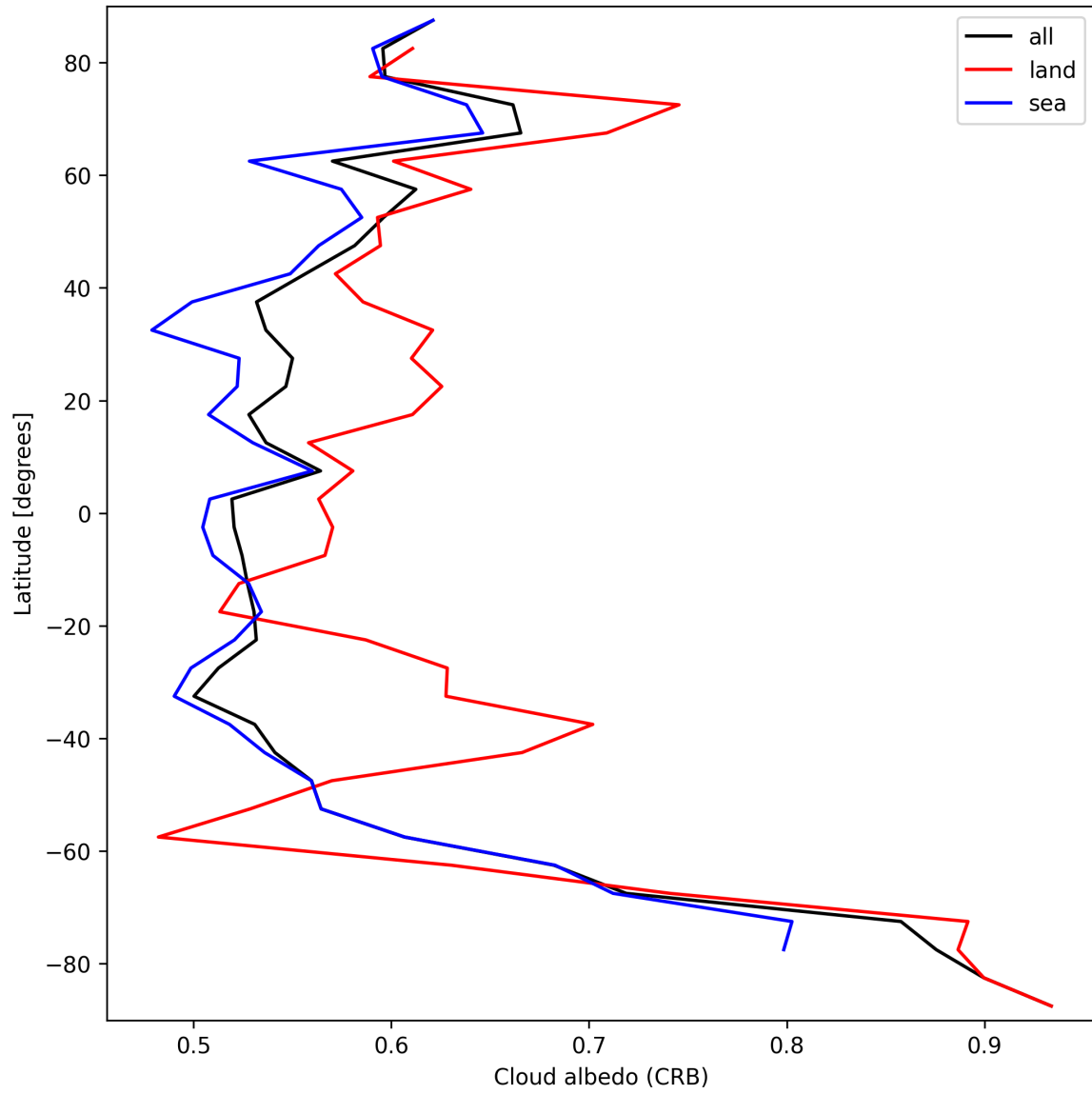
Figure 26: Zonal average of “Cloud albedo (CRB)” for 2025-09-26 to 2025-09-27.
