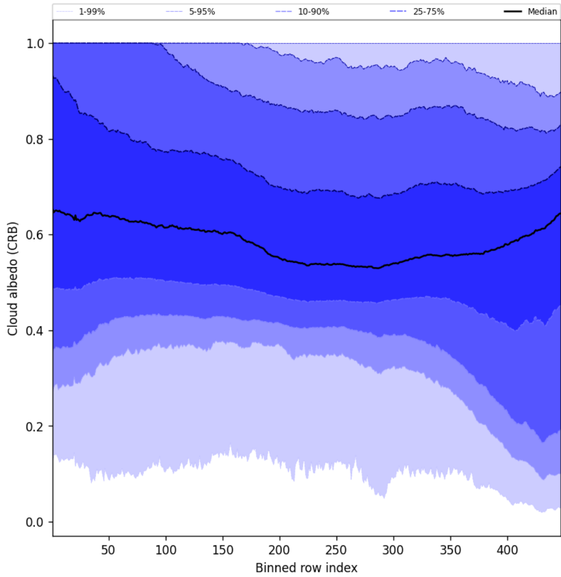
Figure 58: Along track statistics of “Cloud albedo (CRB)” for 2025-09-26 to 2025-09-27
