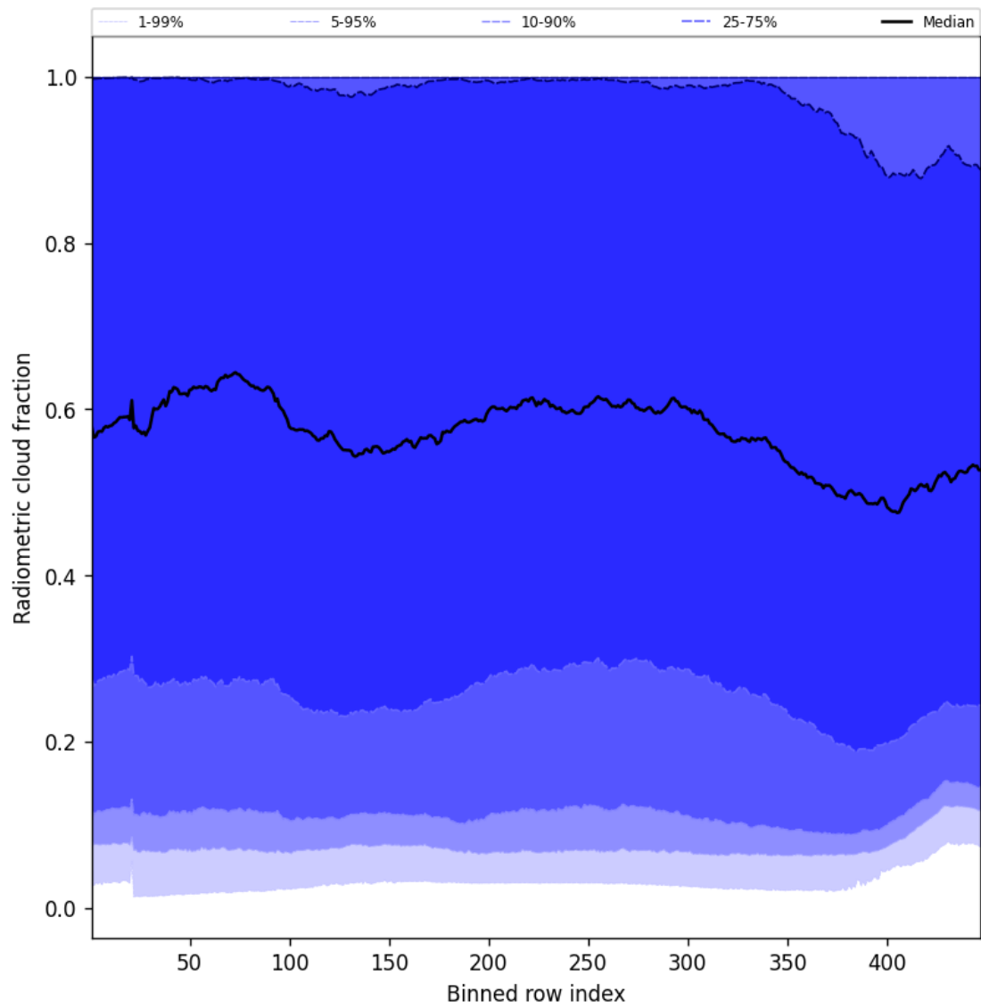
Figure 53: Along track statistics of “Radiometric cloud fraction” for 2025-09-26 to 2025-09-27
