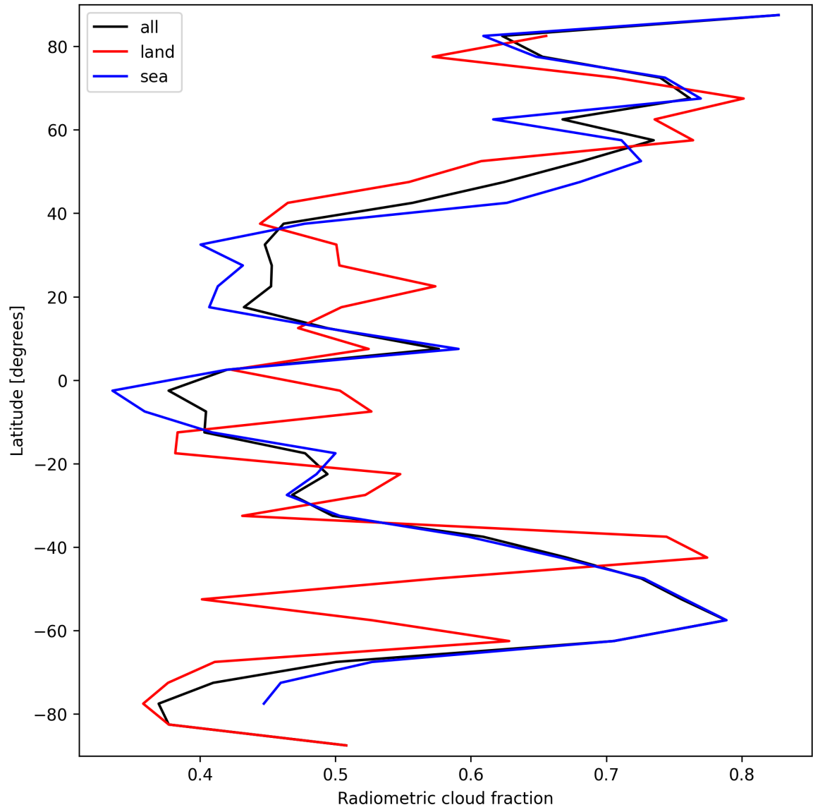
Figure 21: Zonal average of “Radiometric cloud fraction” for 2025-09-26 to 2025-09-27.
