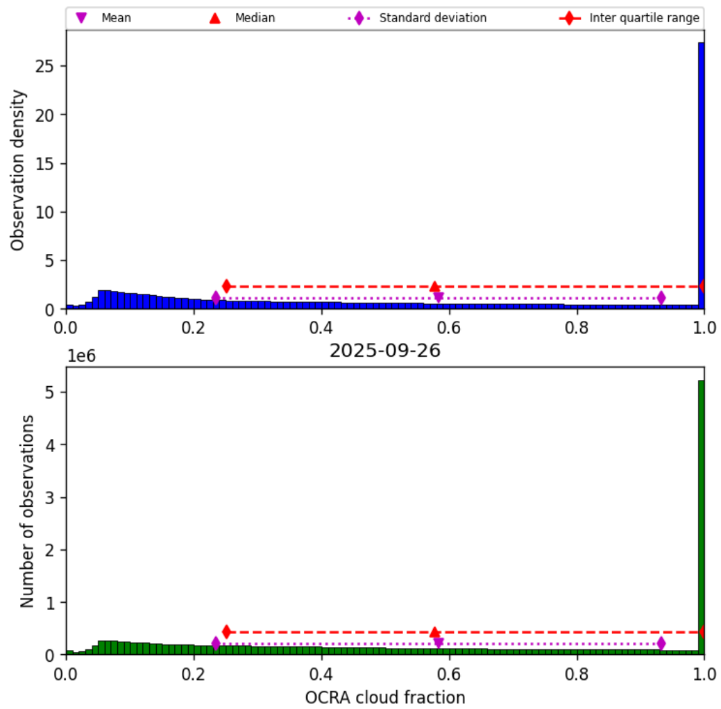
Figure 48: Histogram of “OCRA cloud fraction” for 2025-09-26 to 2025-09-27
