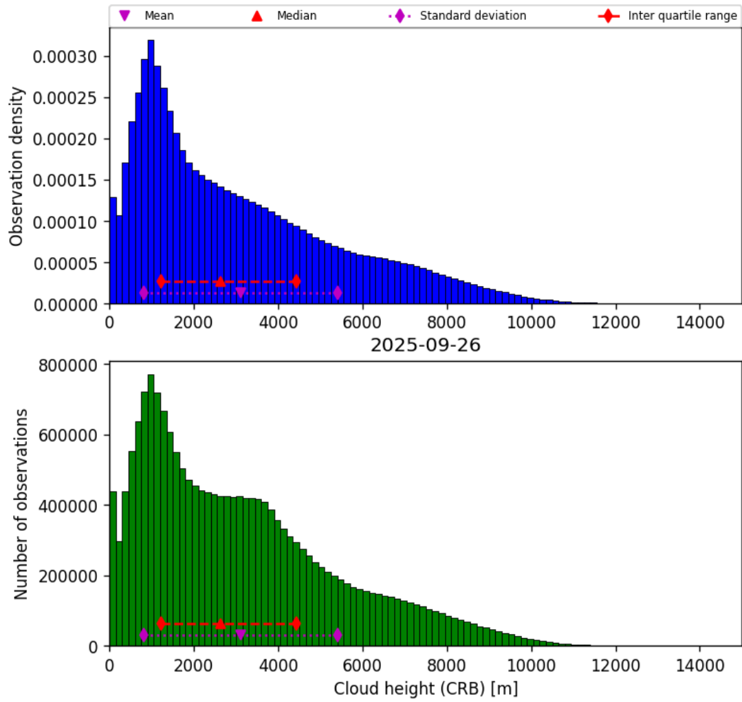
Figure 41: Histogram of “Cloud height (CRB)” for 2025-09-26 to 2025-09-27
