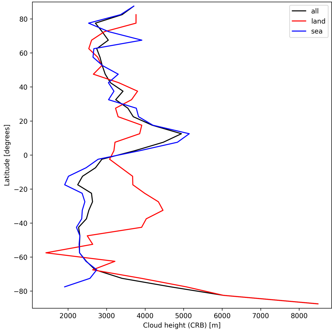
Figure 25: Zonal average of “Cloud height (CRB)” for 2025-09-26 to 2025-09-27.
