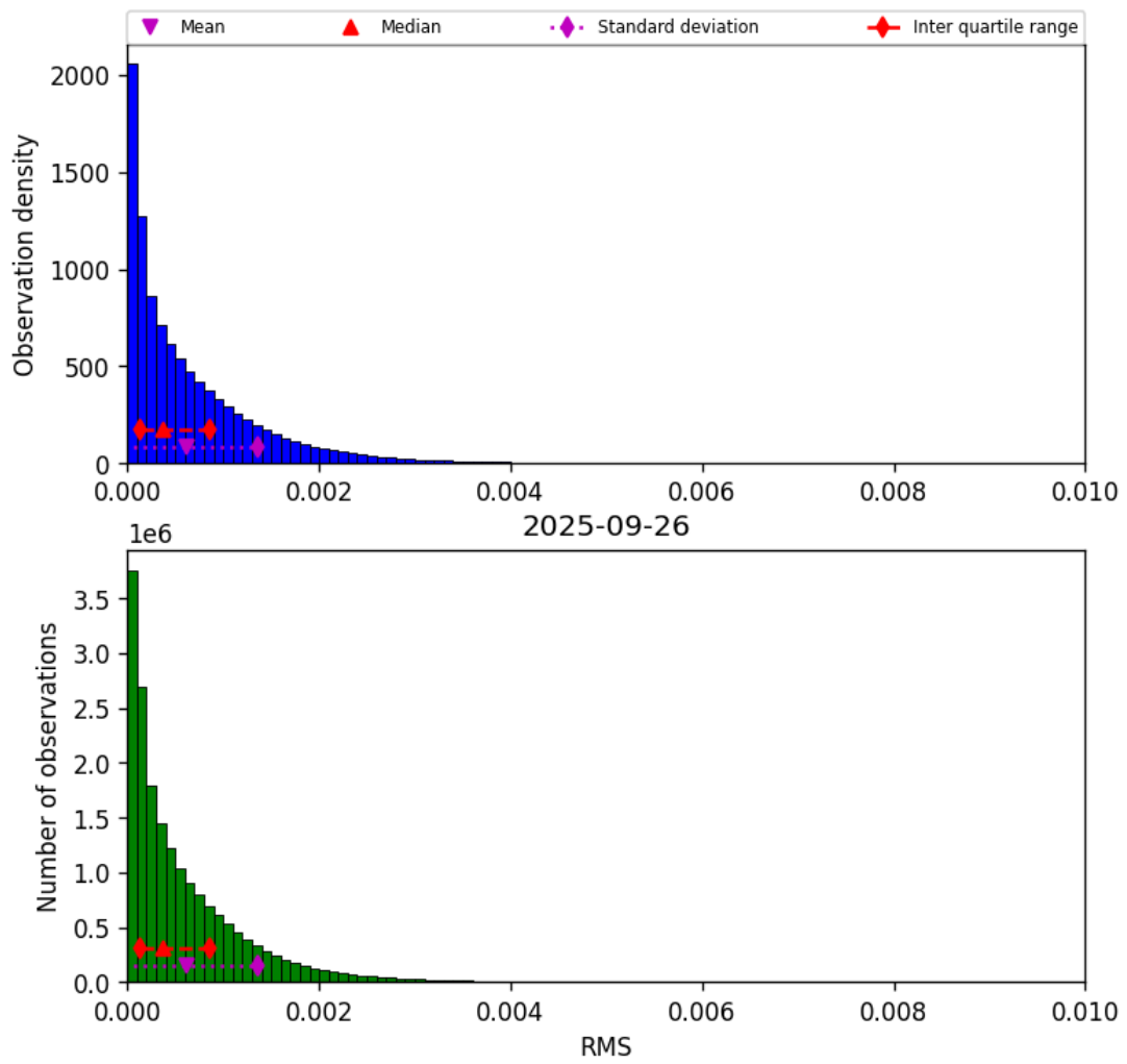
Figure 45: Histogram of “RMS” for 2025-09-26 to 2025-09-27
