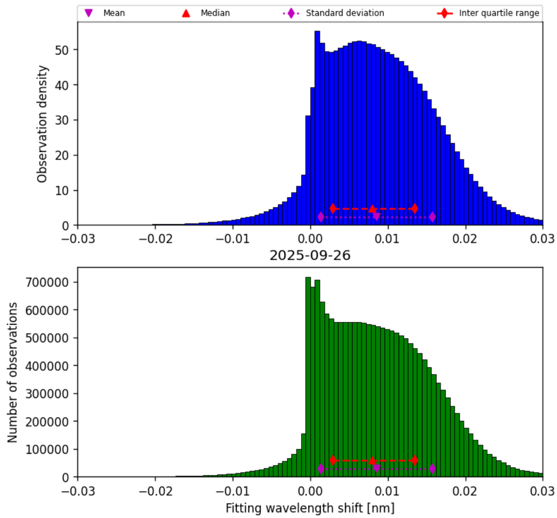
Figure 47: Histogram of “Fitting wavelength shift” for 2025-09-26 to 2025-09-27
