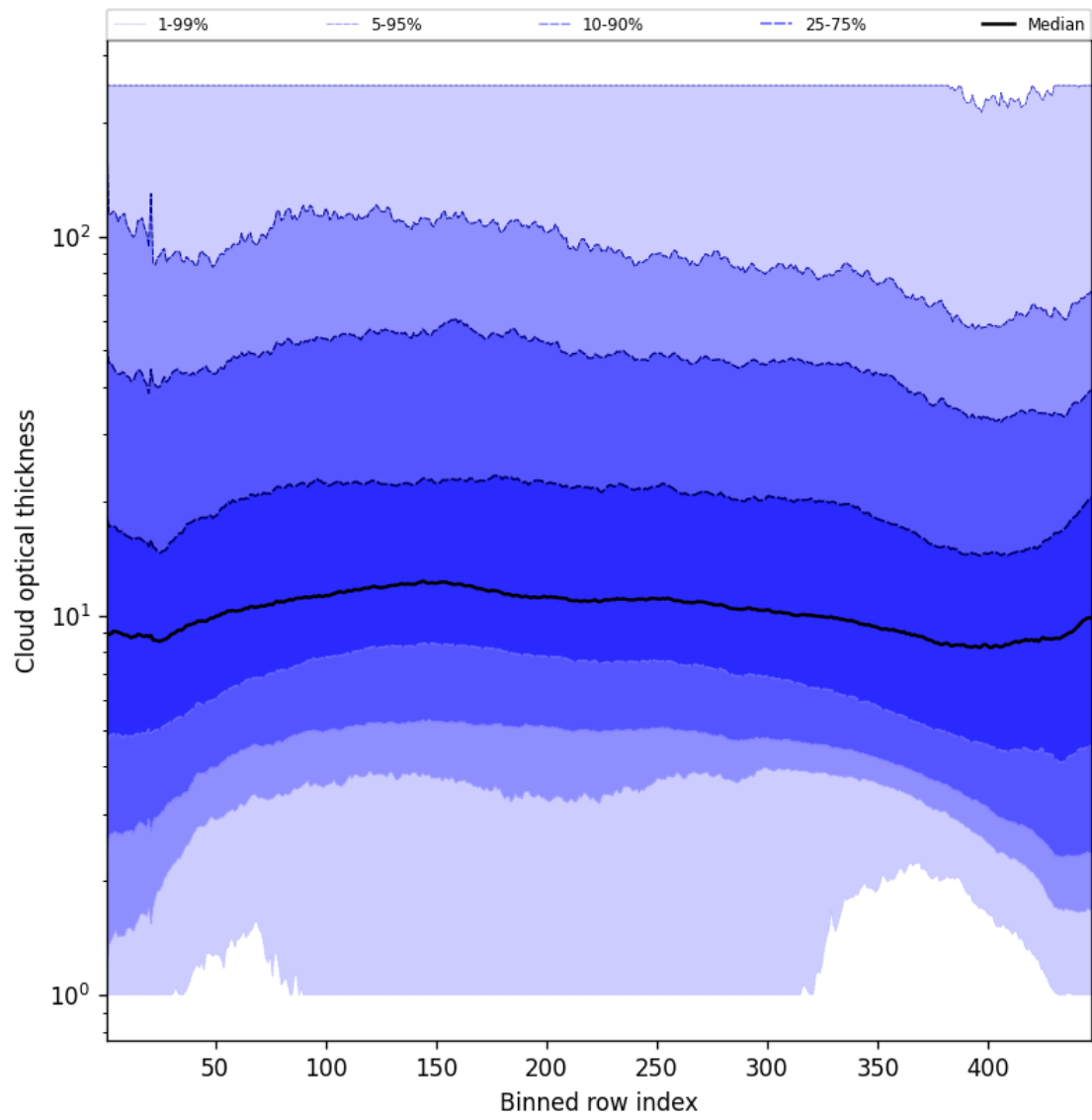
Figure 55: Along track statistics of “Cloud optical thickness” for 2025-09-26 to 2025-09-27
