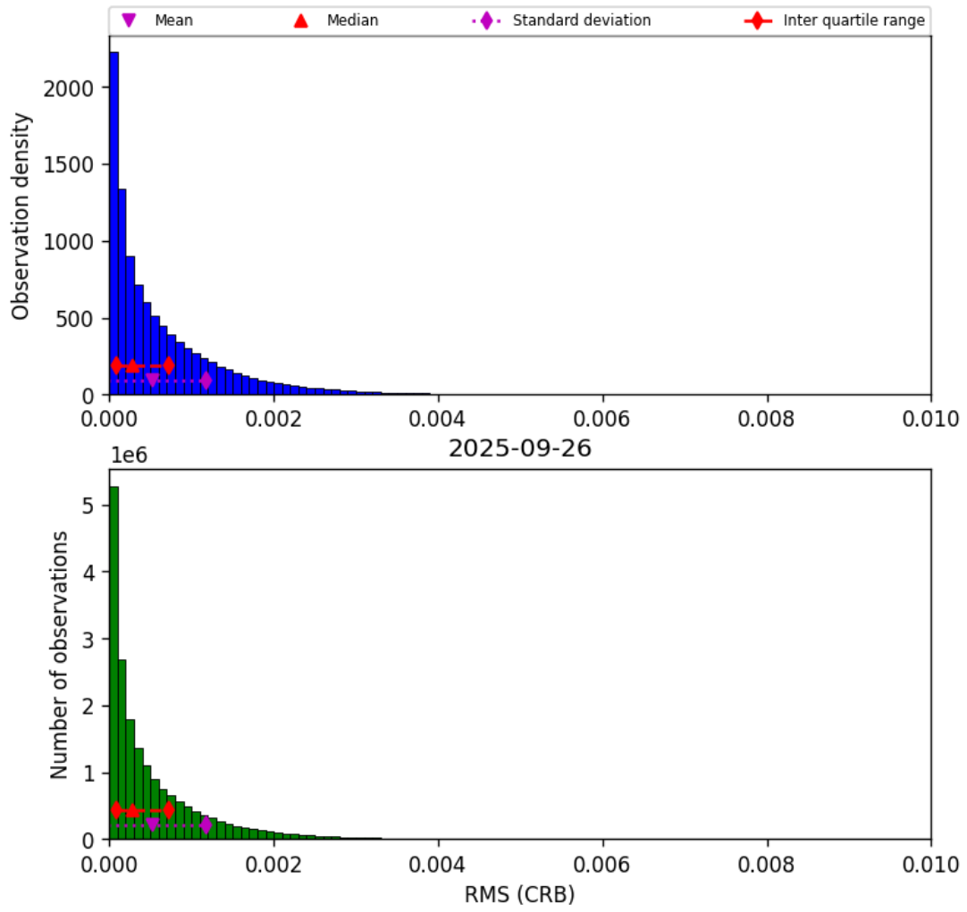
Figure 46: Histogram of “RMS (CRB)” for 2025-09-26 to 2025-09-27
