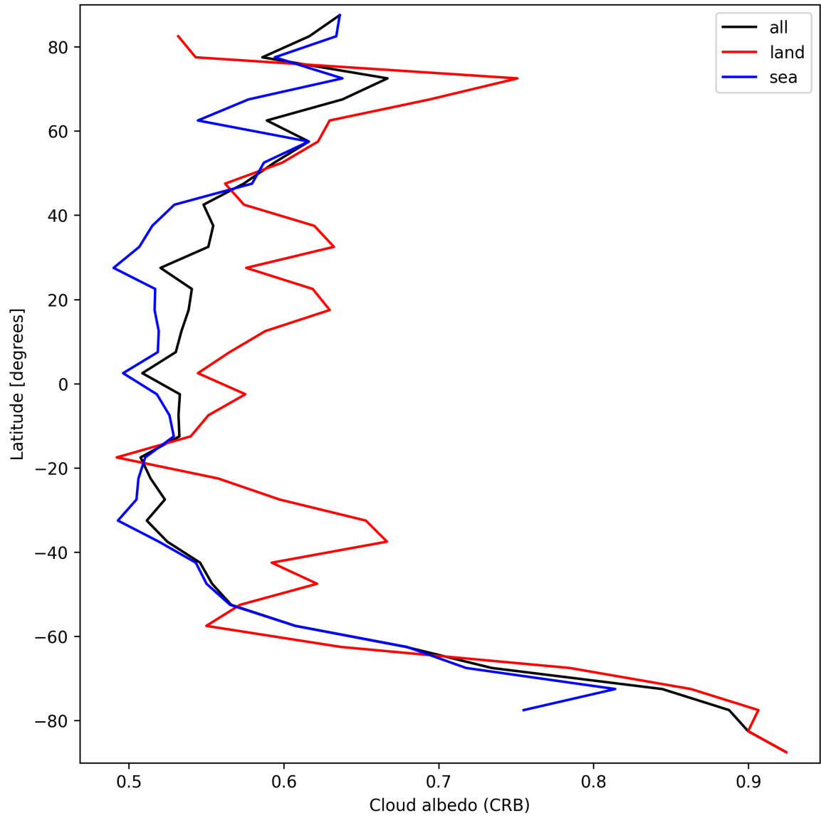
Figure 26: Zonal average of “Cloud albedo (CRB)” for 2025-09-27 to 2025-09-28.
