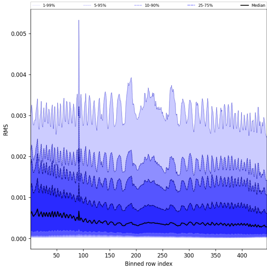
Figure 61: Along track statistics of “RMS” for 2025-09-27 to 2025-09-28
