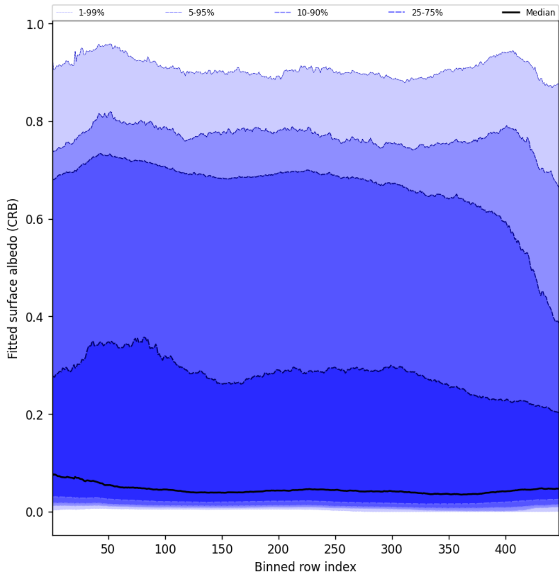
Figure 60: Along track statistics of “Fitted surface albedo (CRB)” for 2025-09-27 to 2025-09-28
