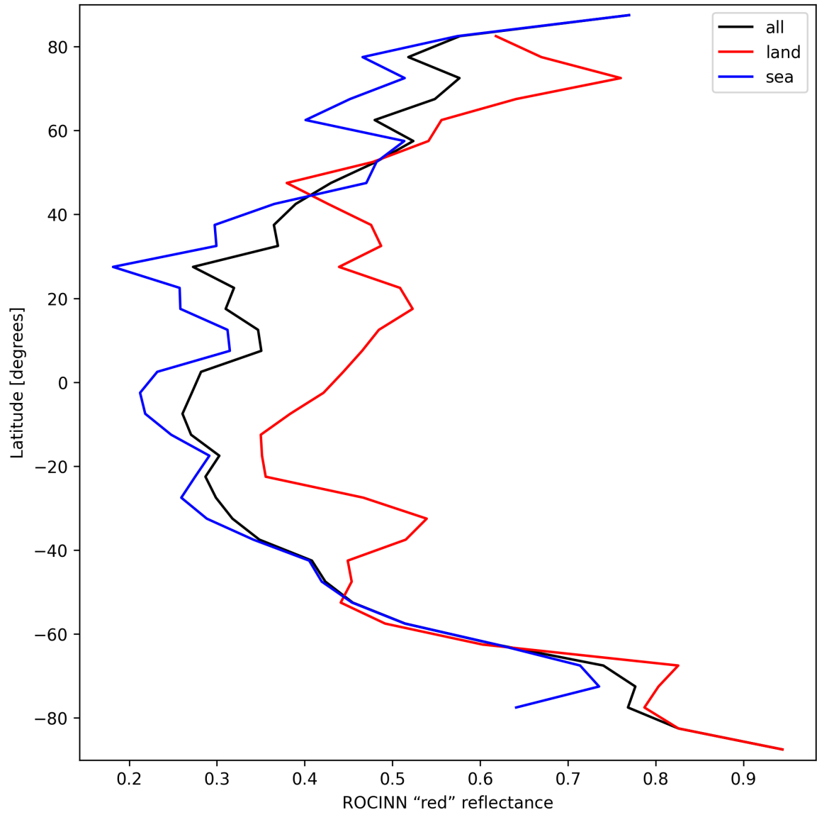
Figure 35: Zonal average of “ROCINN “red” reflectance” for 2025-09-27 to 2025-09-28.
