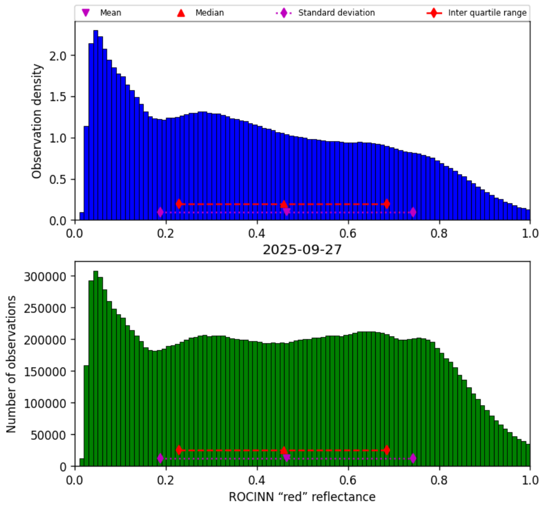
Figure 51: Histogram of “ROCINN “red” reflectance” for 2025-09-27 to 2025-09-28
