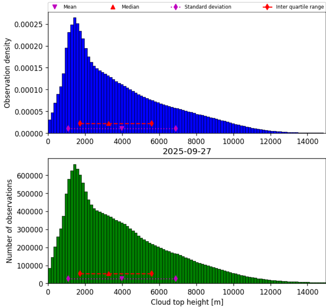
Figure 38: Histogram of “Cloud top height” for 2025-09-27 to 2025-09-28
