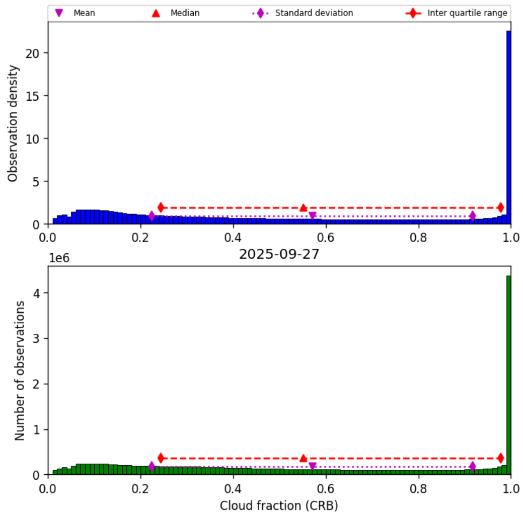
Figure 40: Histogram of “Cloud fraction (CRB)” for 2025-09-27 to 2025-09-28
