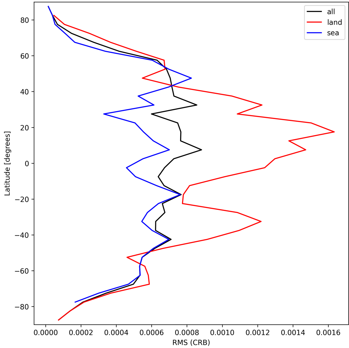
Figure 30: Zonal average of “RMS (CRB)” for 2025-09-27 to 2025-09-28.
