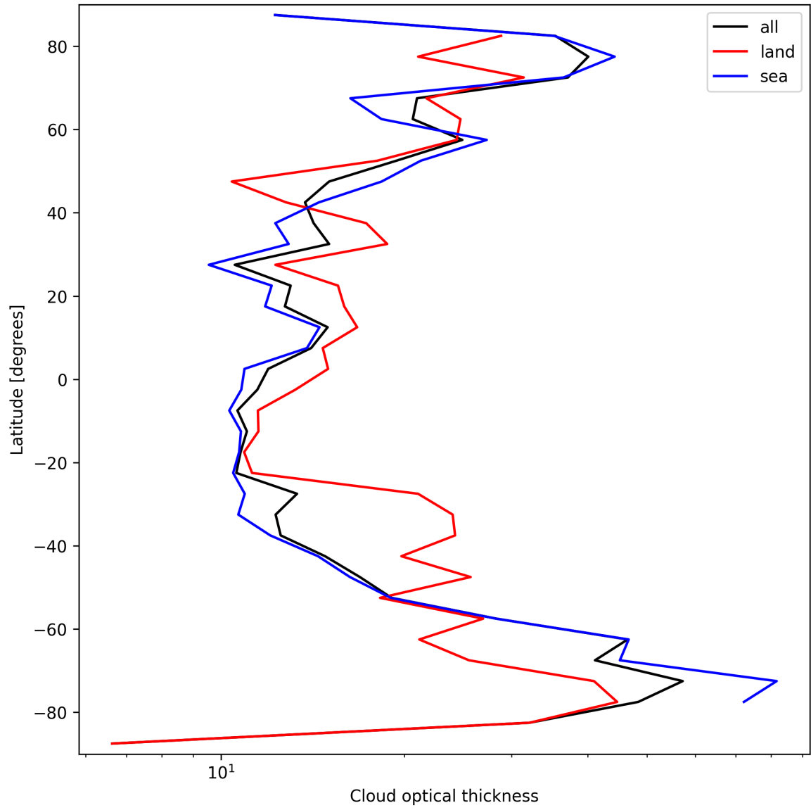
Figure 23: Zonal average of “Cloud optical thickness” for 2025-09-27 to 2025-09-28.
