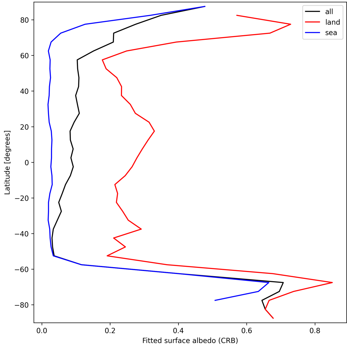
Figure 28: Zonal average of “Fitted surface albedo (CRB)” for 2025-09-27 to 2025-09-28.
