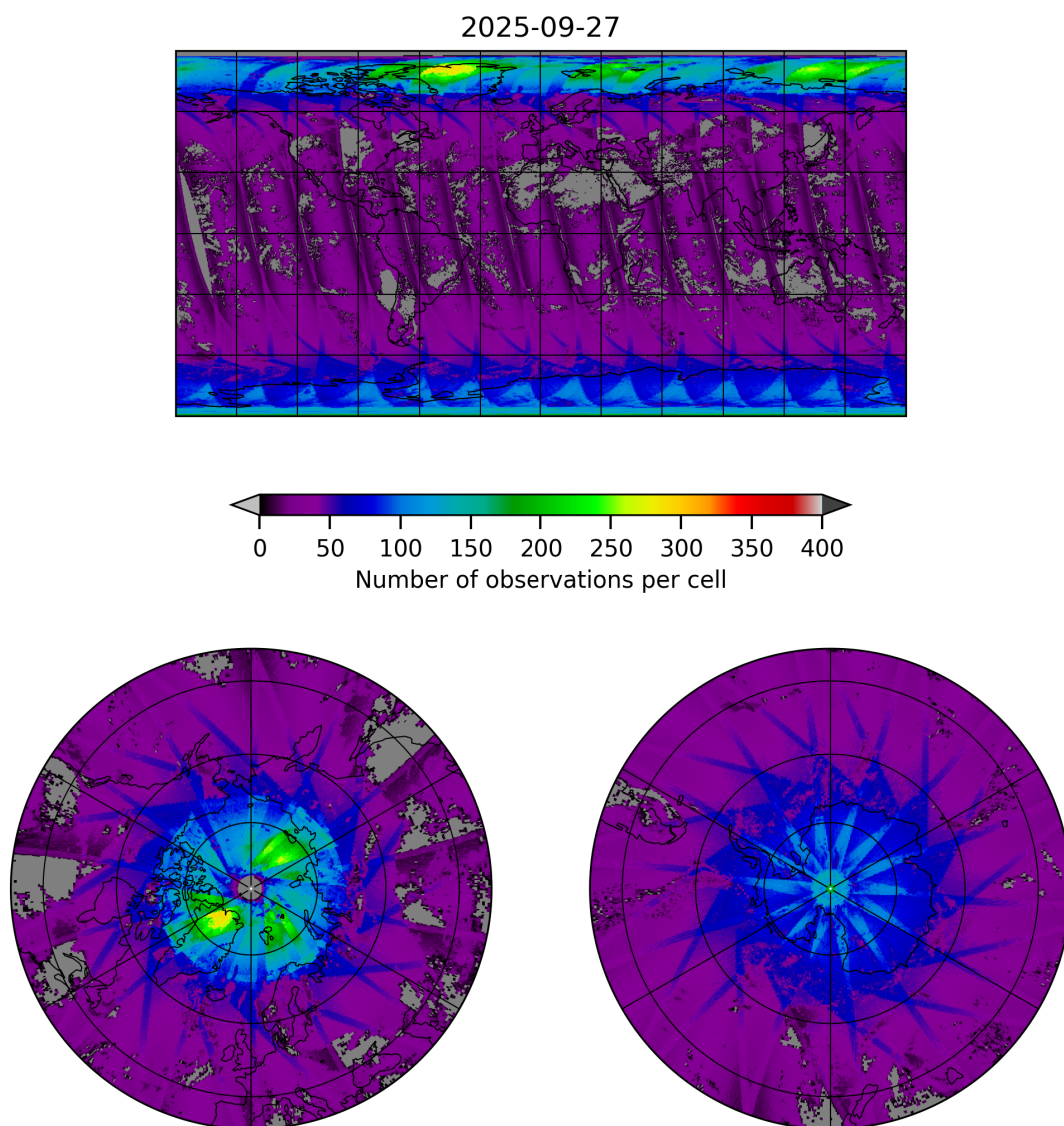
Figure 19: Map of the number of observations for 2025-09-27 to 2025-09-28
