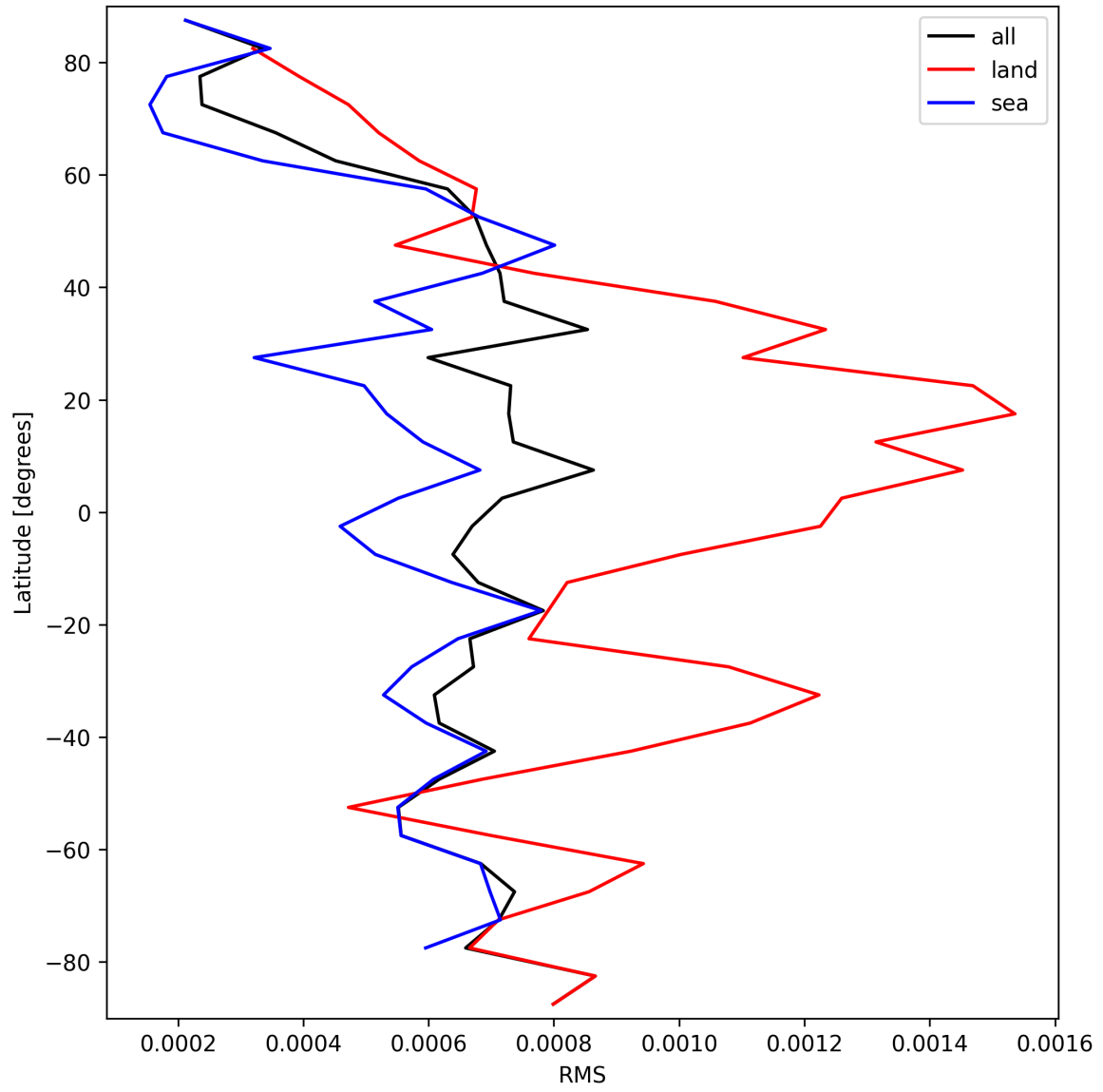
Figure 29: Zonal average of “RMS” for 2025-09-27 to 2025-09-28.
