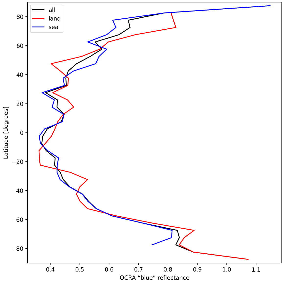
Figure 33: Zonal average of “OCRA “blue” reflectance” for 2025-09-27 to 2025-09-28.
