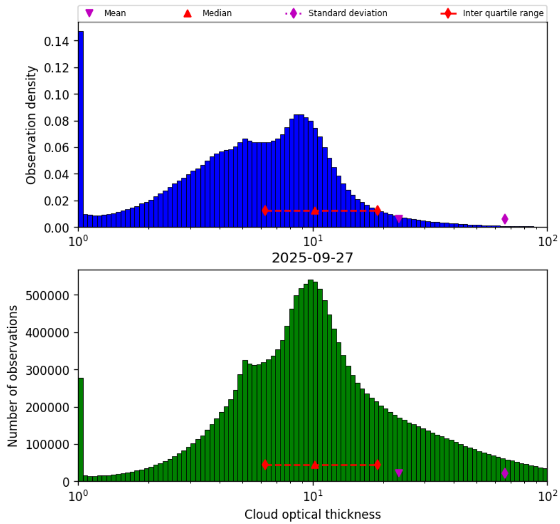
Figure 39: Histogram of “Cloud optical thickness” for 2025-09-27 to 2025-09-28
