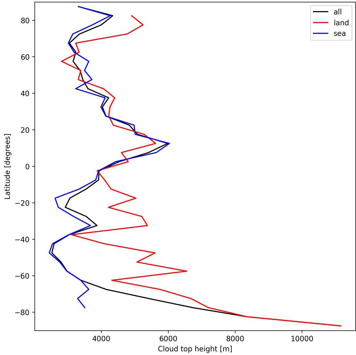
Figure 22: Zonal average of “Cloud top height” for 2025-09-27 to 2025-09-28.
