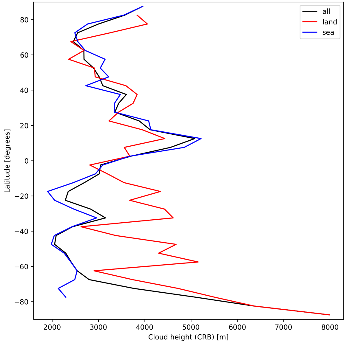
Figure 25: Zonal average of “Cloud height (CRB)” for 2025-09-27 to 2025-09-28.
