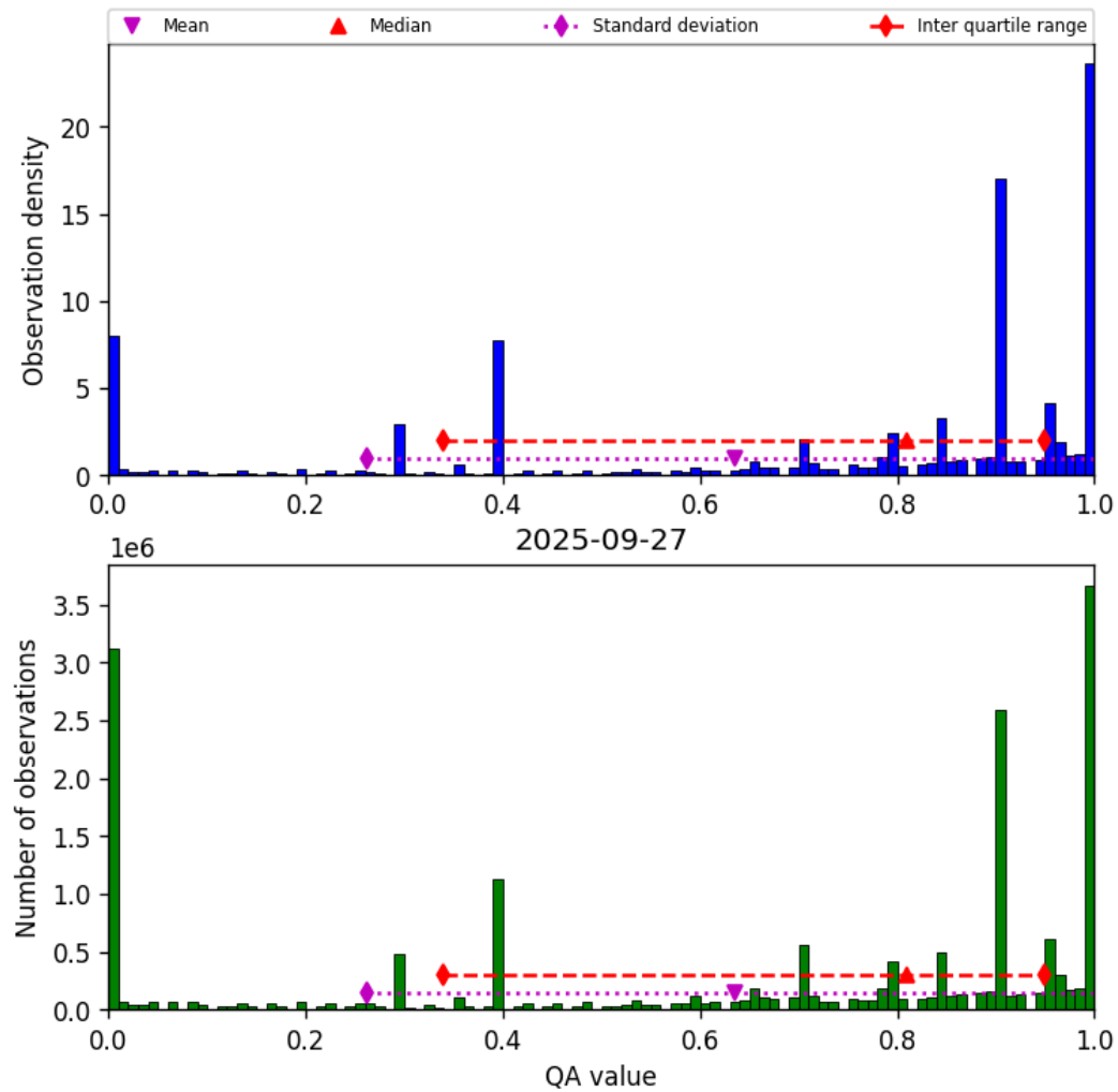
Figure 36: Histogram of “QA value” for 2025-09-27 to 2025-09-28
