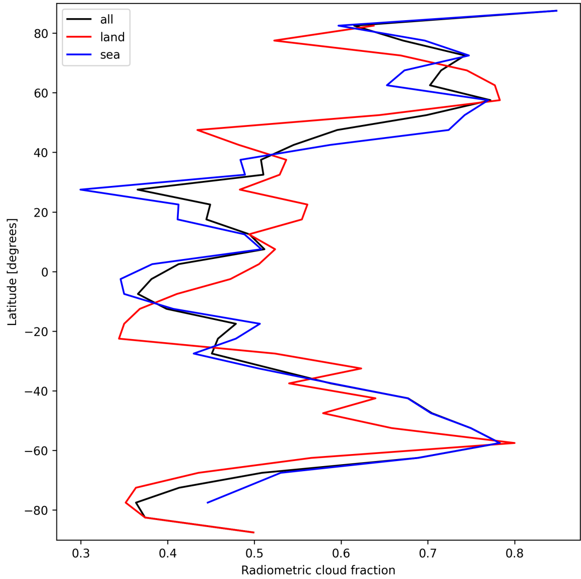
Figure 21: Zonal average of “Radiometric cloud fraction” for 2025-09-27 to 2025-09-28.
