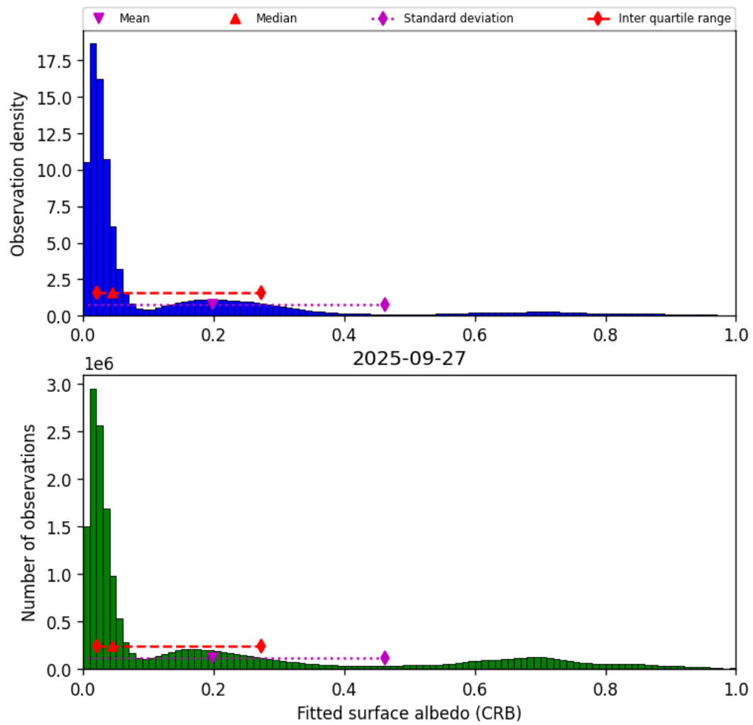
Figure 44: Histogram of “Fitted surface albedo (CRB)” for 2025-09-27 to 2025-09-28
