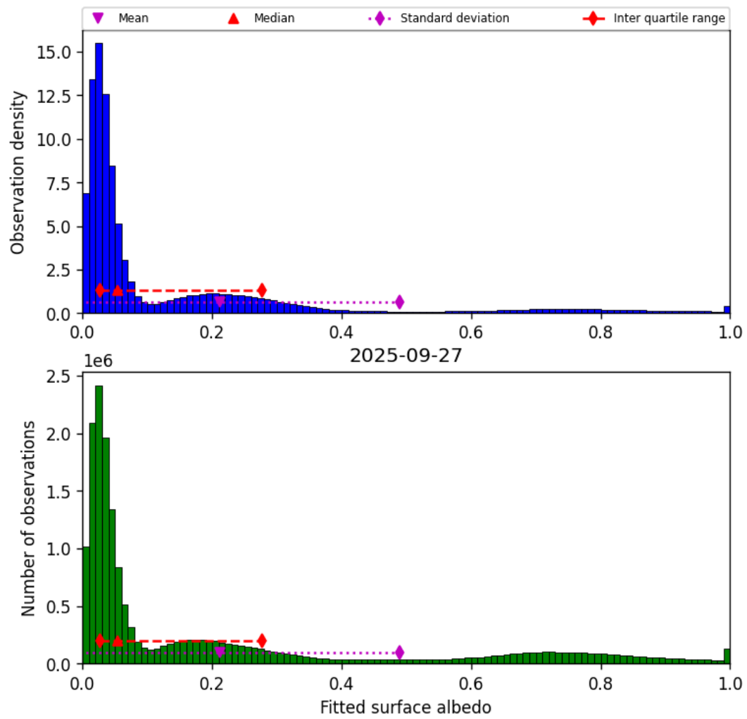
Figure 43: Histogram of “Fitted surface albedo” for 2025-09-27 to 2025-09-28
