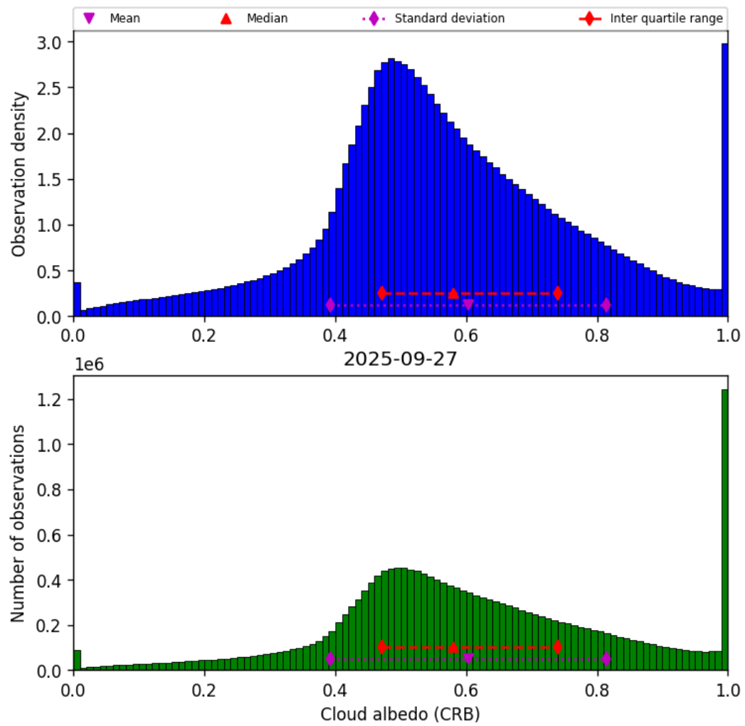
Figure 42: Histogram of “Cloud albedo (CRB)” for 2025-09-27 to 2025-09-28
