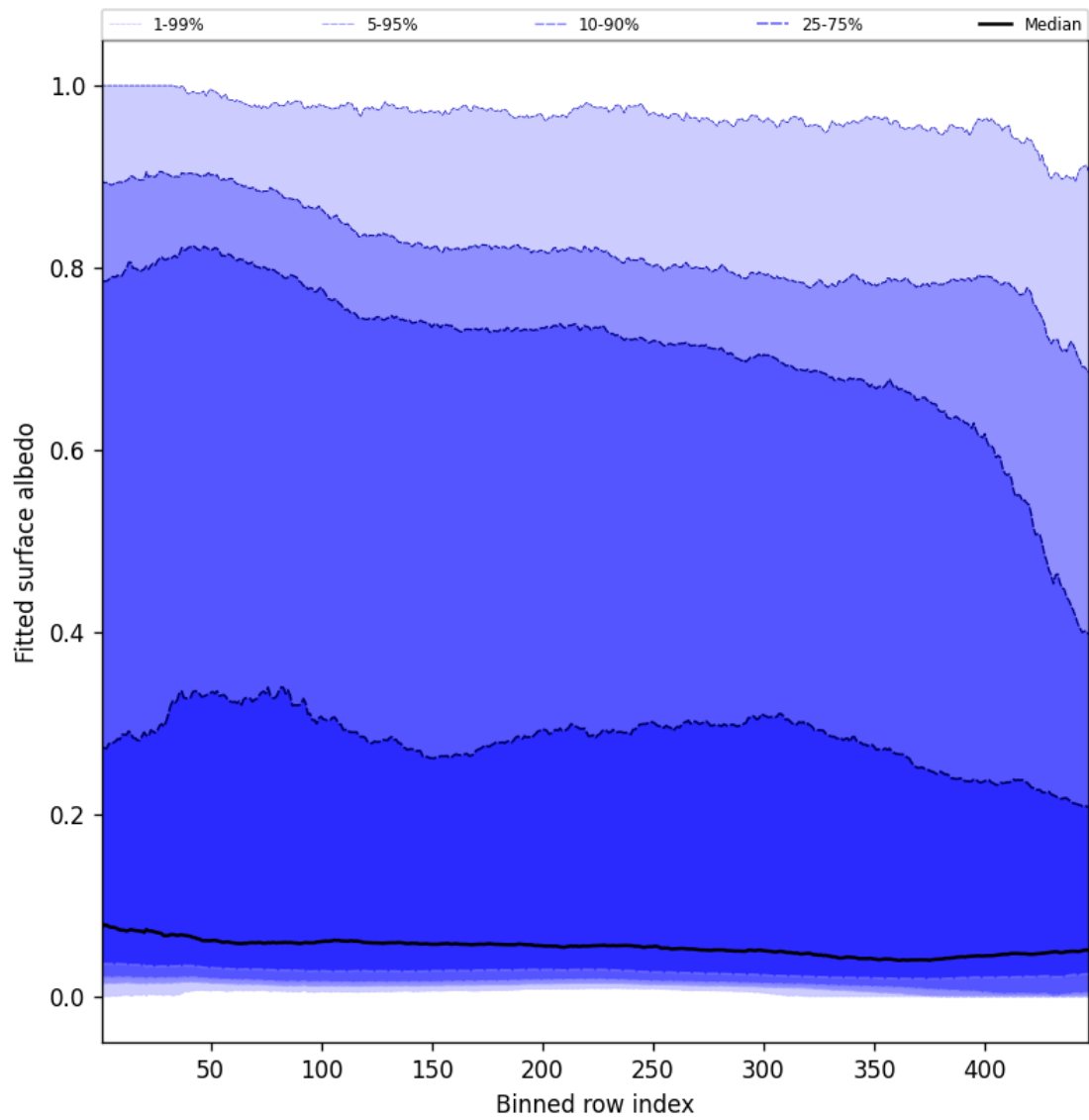
Figure 59: Along track statistics of “Fitted surface albedo” for 2025-09-27 to 2025-09-28
