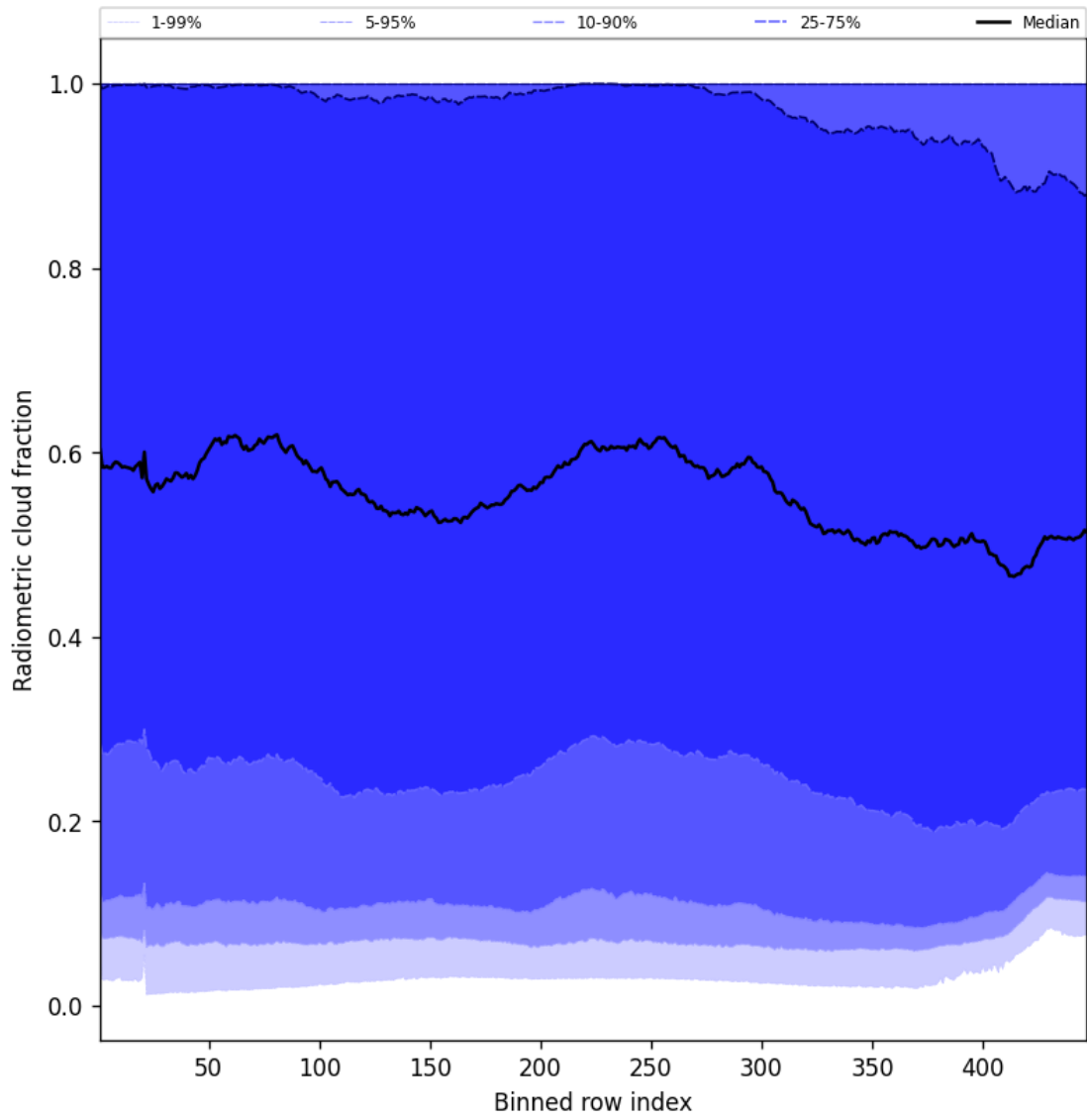
Figure 53: Along track statistics of “Radiometric cloud fraction” for 2025-09-27 to 2025-09-28
