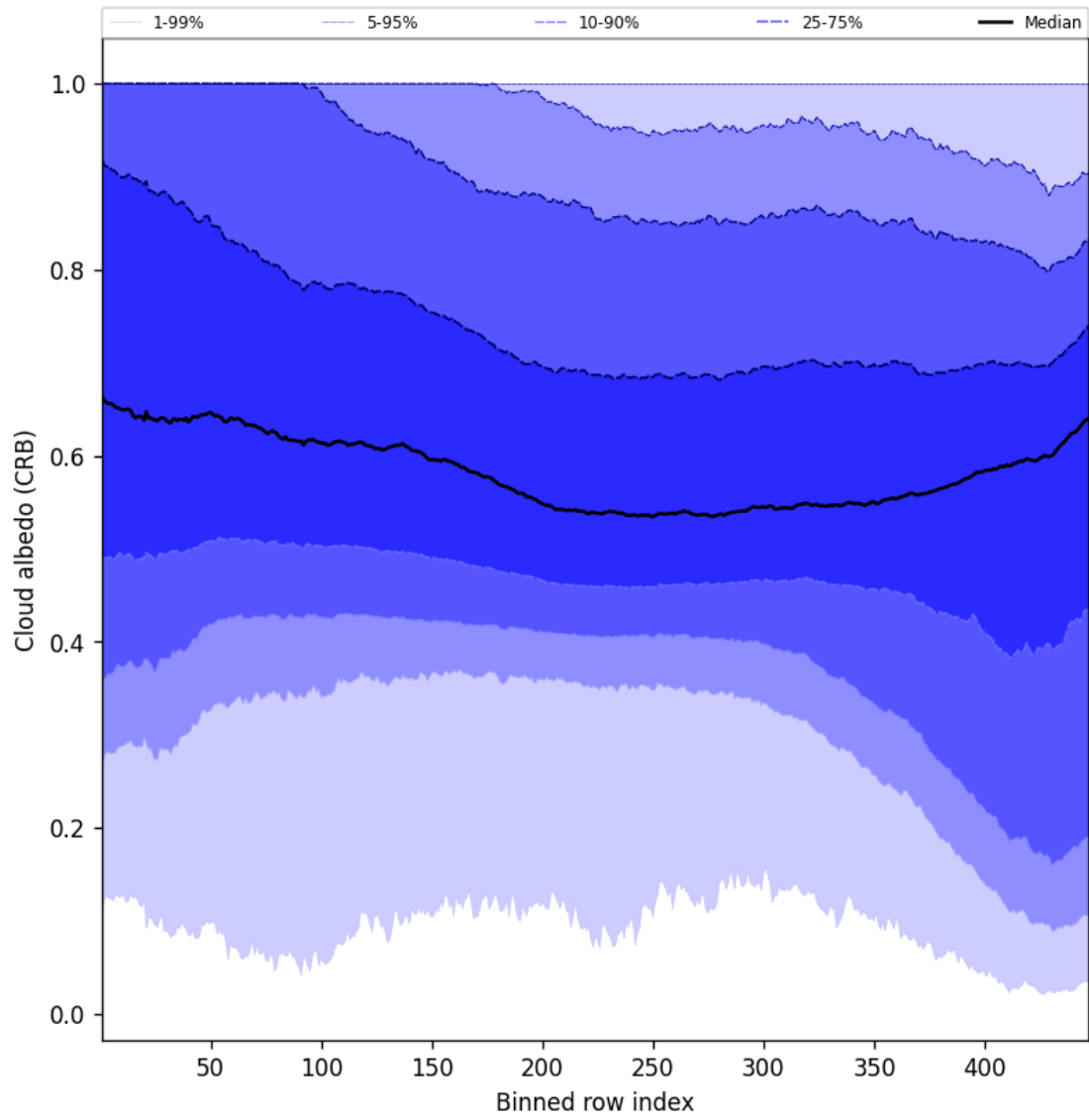
Figure 58: Along track statistics of “Cloud albedo (CRB)” for 2025-09-27 to 2025-09-28
