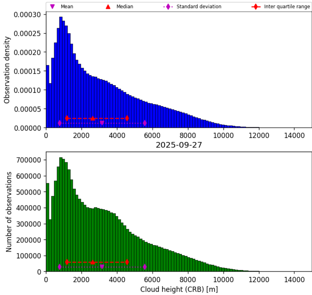
Figure 41: Histogram of “Cloud height (CRB)” for 2025-09-27 to 2025-09-28
