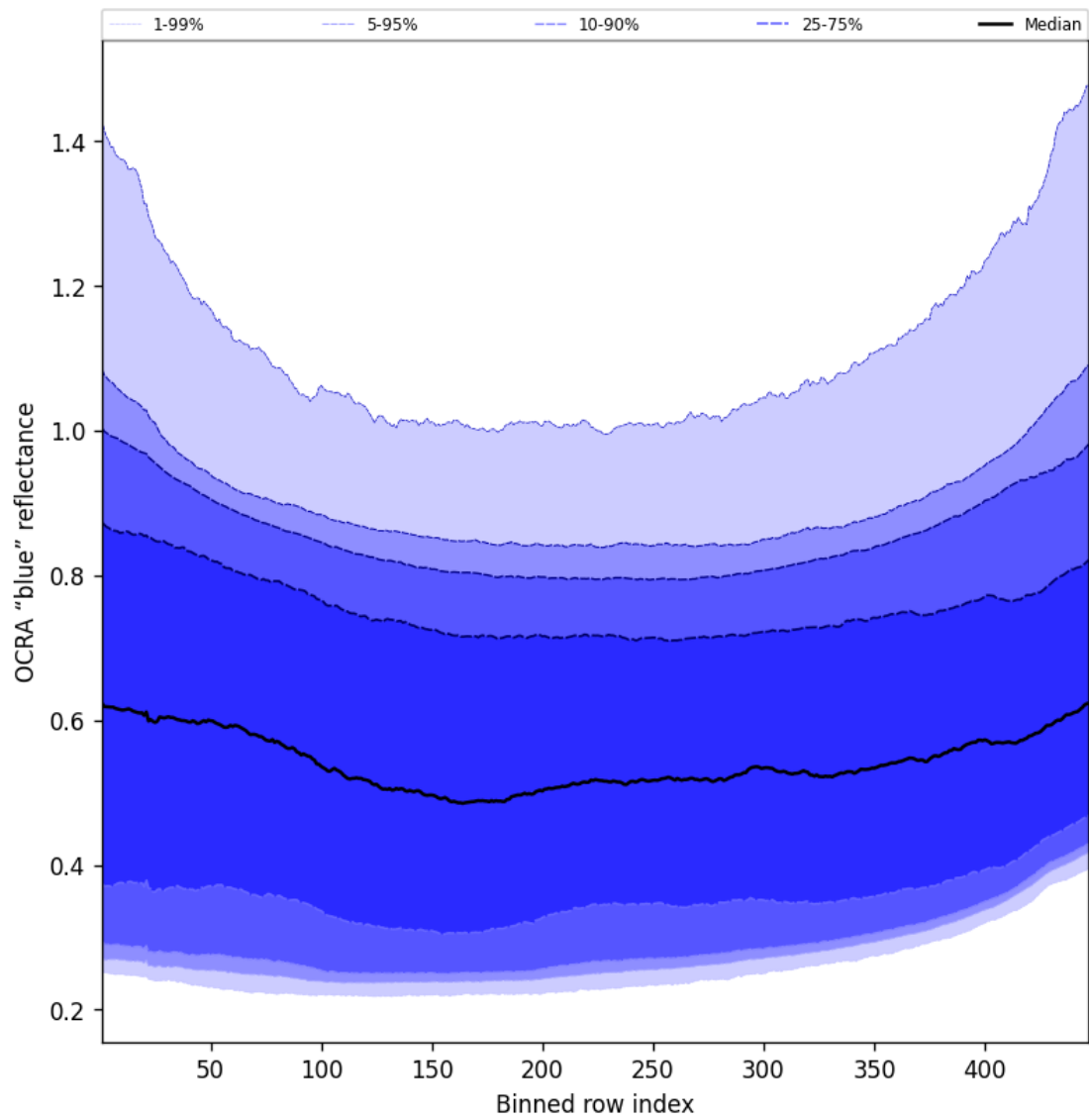
Figure 65: Along track statistics of “OCRA “blue” reflectance” for 2025-09-27 to 2025-09-28
