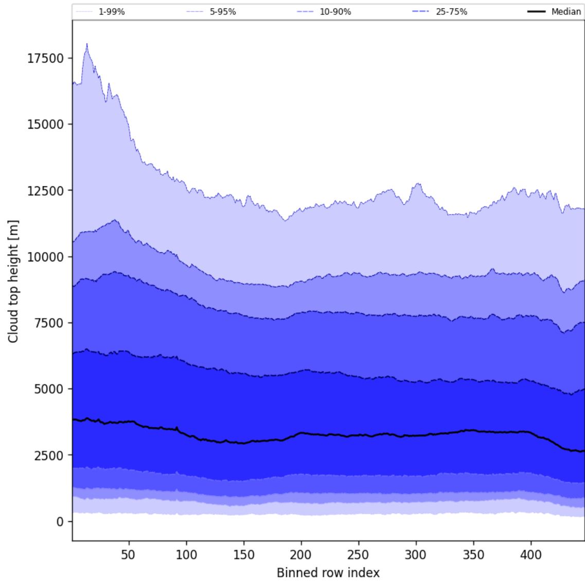
Figure 54: Along track statistics of “Cloud top height” for 2025-09-27 to 2025-09-28
