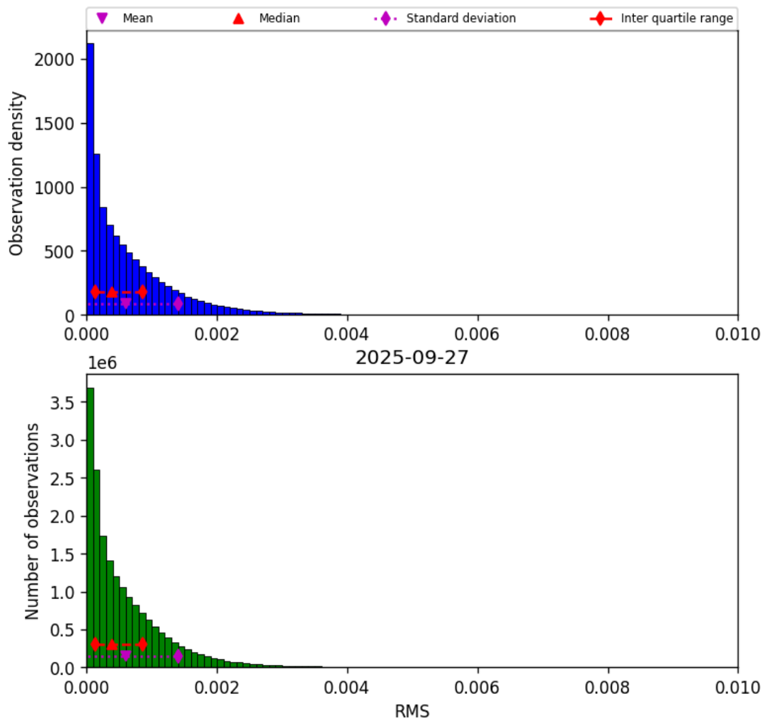
Figure 45: Histogram of “RMS” for 2025-09-27 to 2025-09-28
