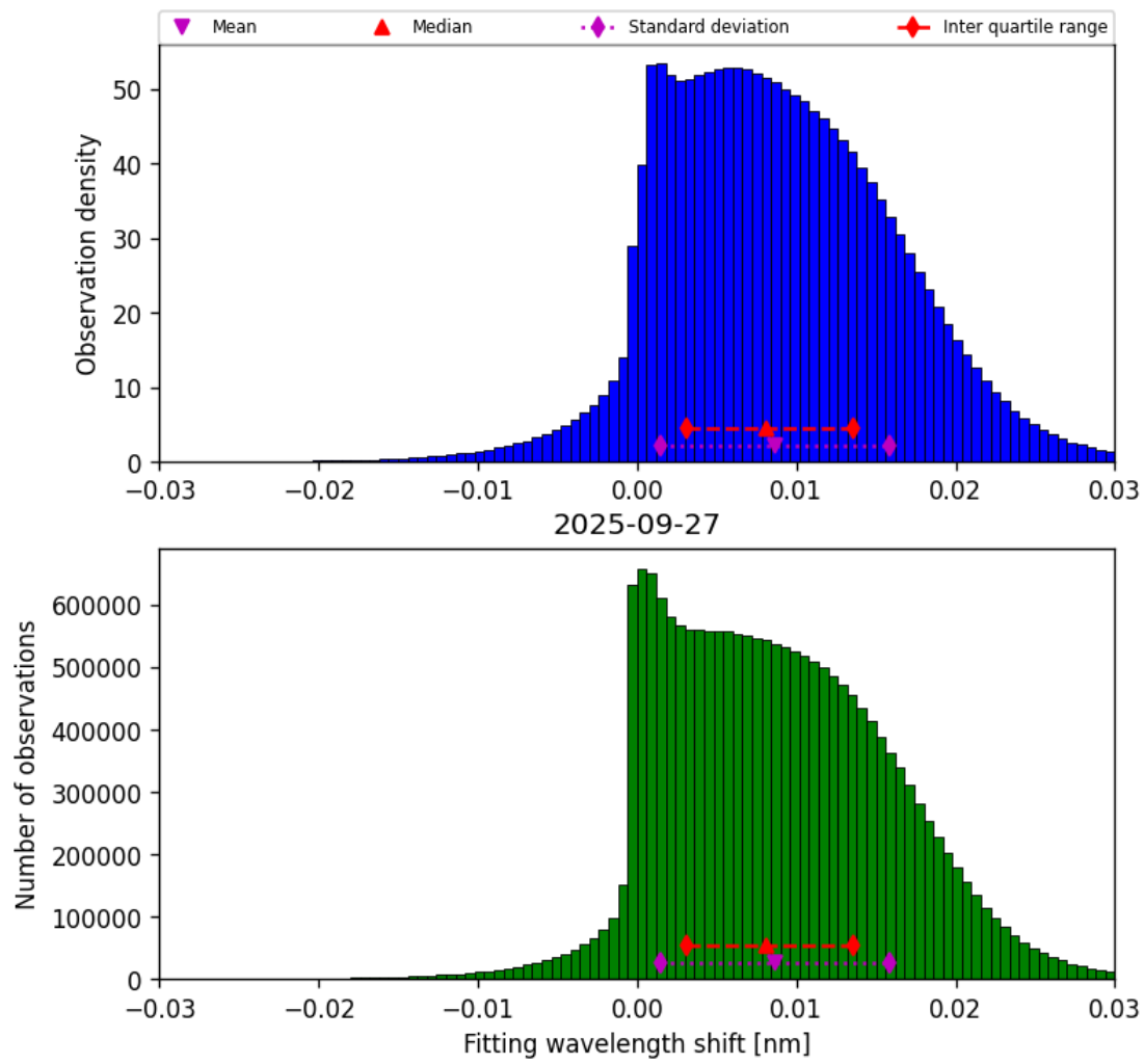
Figure 47: Histogram of “Fitting wavelength shift” for 2025-09-27 to 2025-09-28
