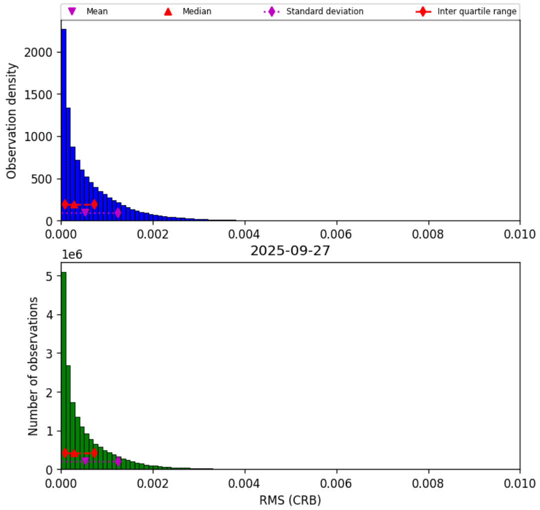
Figure 46: Histogram of "RMS (CRB)" for 2025-09-27 to 2025-09-28
