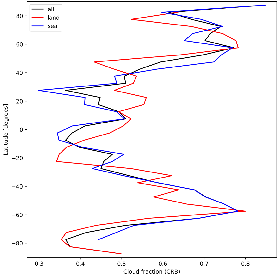
Figure 24: Zonal average of “Cloud fraction (CRB)” for 2025-09-27 to 2025-09-28.
