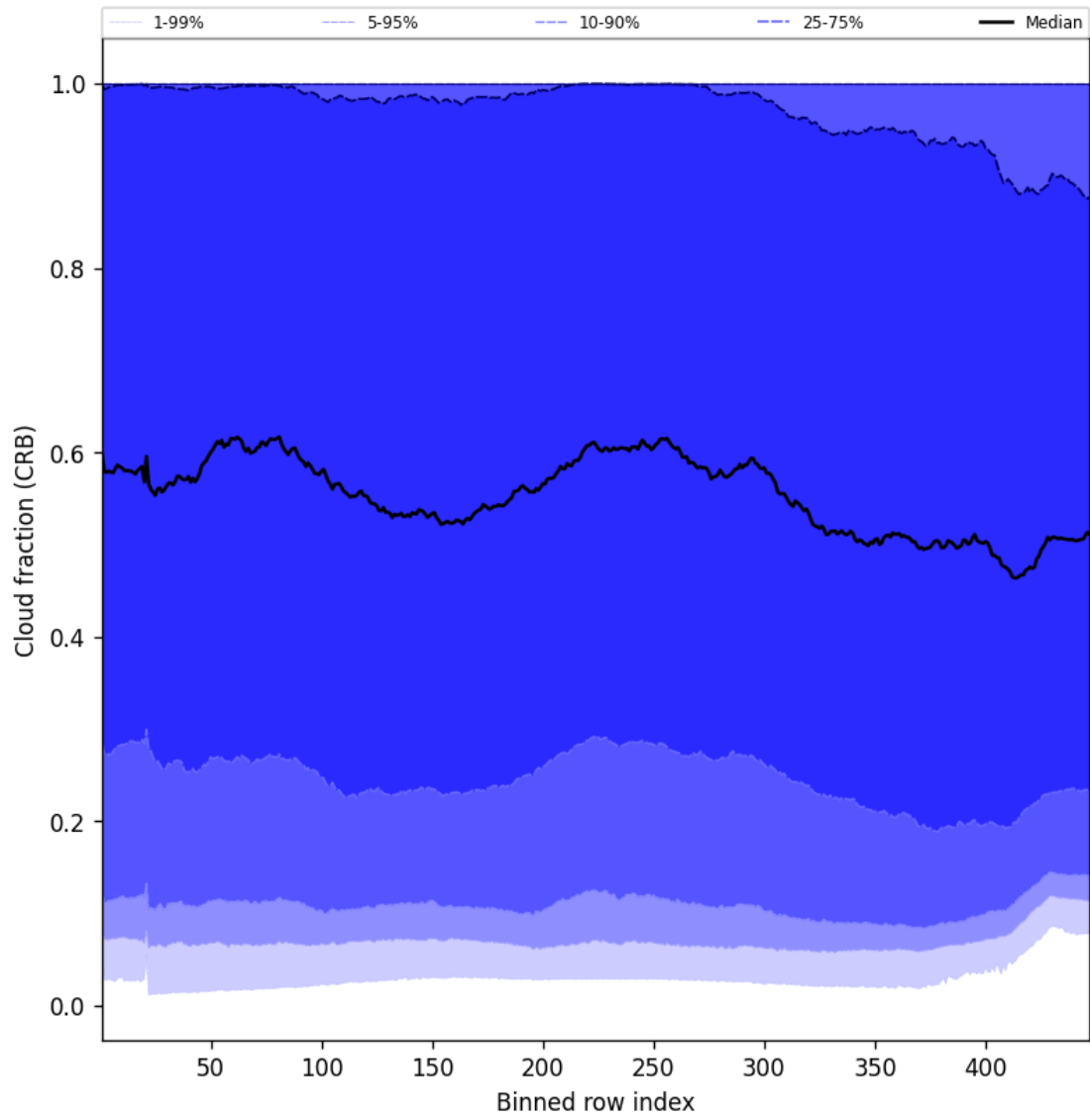
Figure 56: Along track statistics of “Cloud fraction (CRB)” for 2025-09-27 to 2025-09-28
