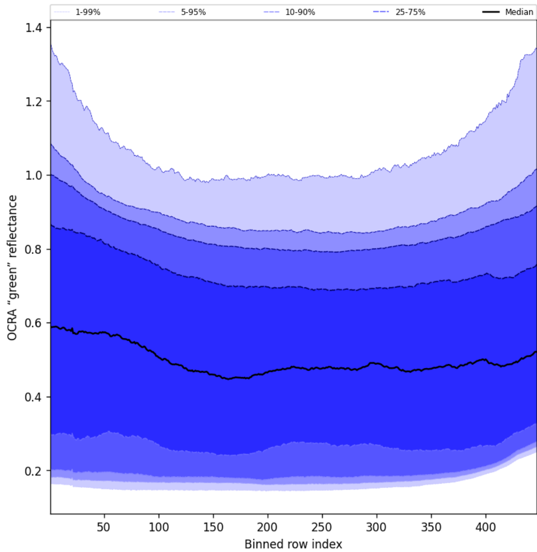
Figure 66: Along track statistics of “OCRA “green” reflectance” for 2025-09-27 to 2025-09-28
