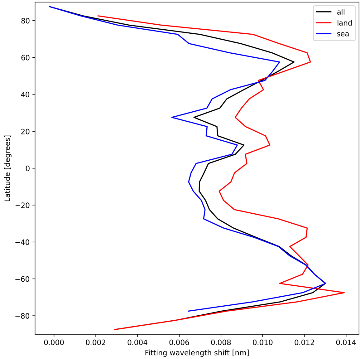
Figure 31: Zonal average of “Fitting wavelength shift” for 2025-09-27 to 2025-09-28.
