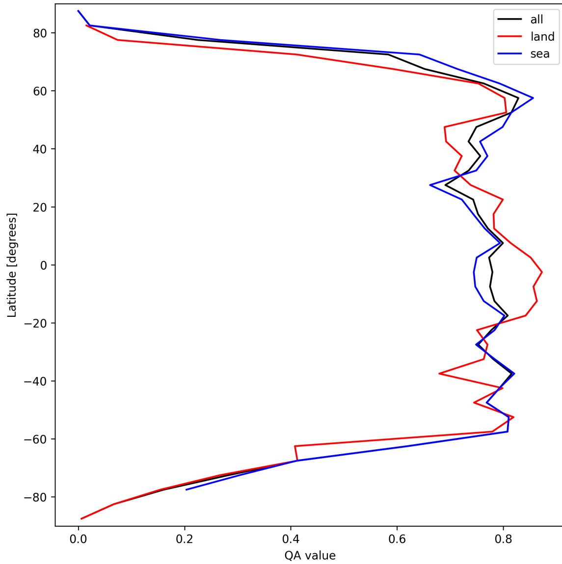
Figure 20: Zonal average of “QA value” for 2025-09-27 to 2025-09-28.
