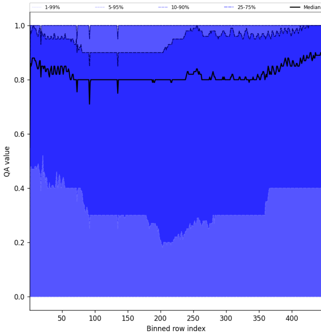
Figure 52: Along track statistics of “QA value” for 2025-09-27 to 2025-09-28
