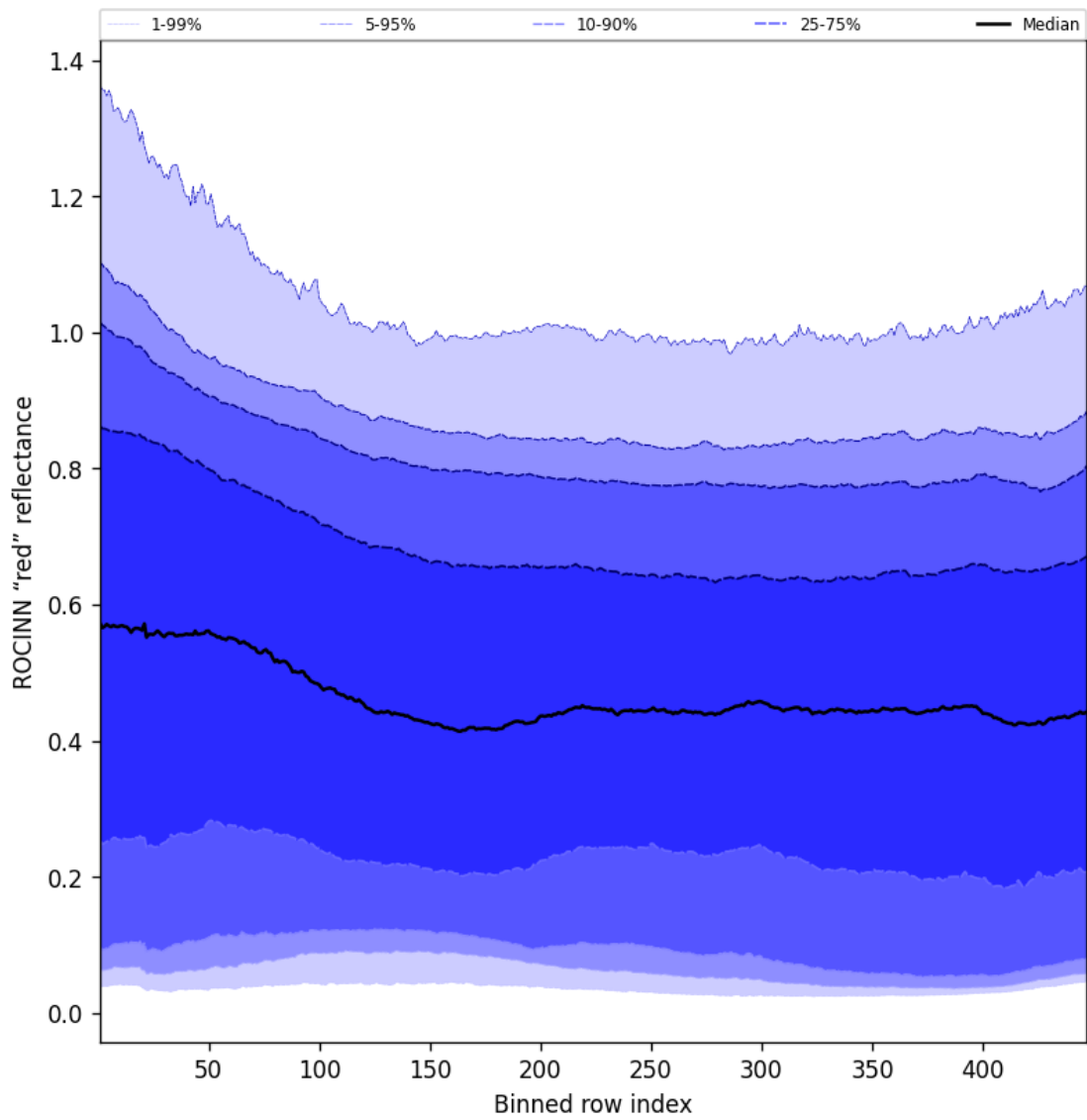
Figure 67: Along track statistics of "ROCINN "red" reflectance" for 2025-09-27 to 2025-09-28
