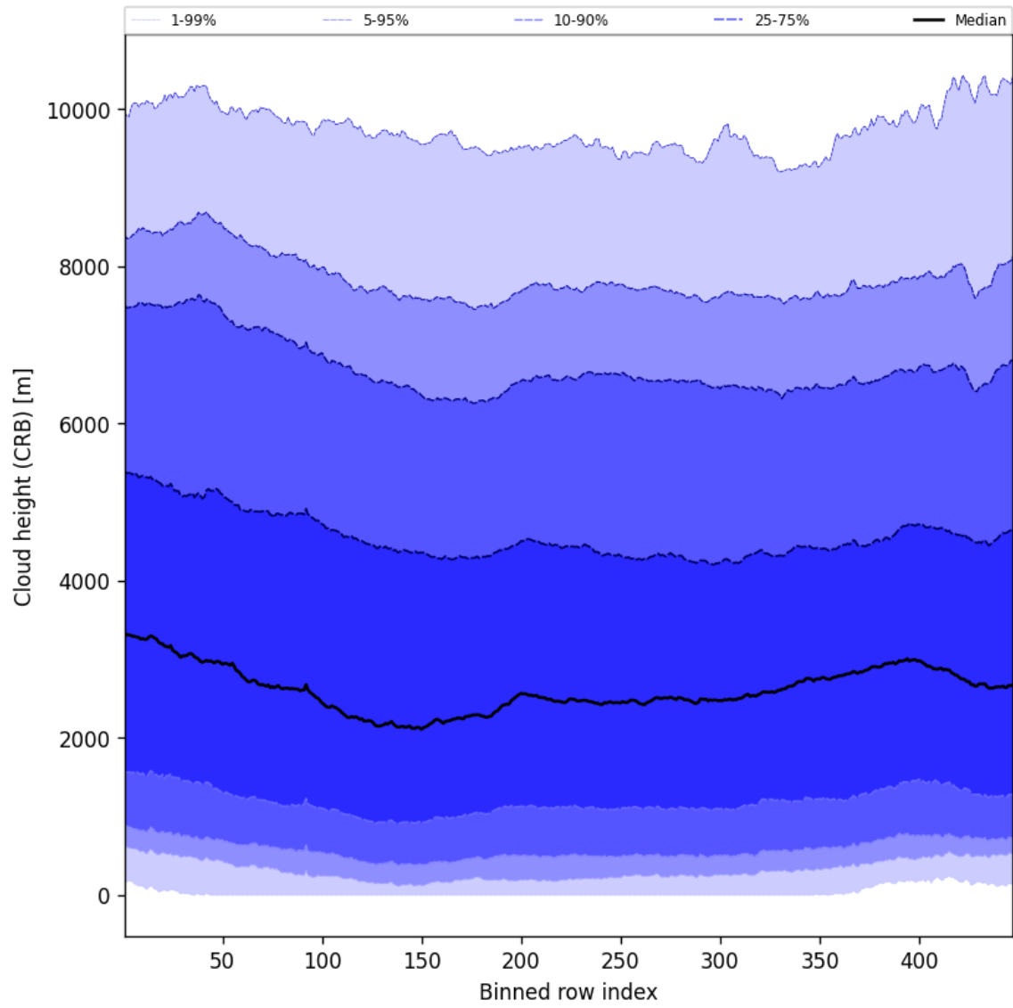
Figure 57: Along track statistics of “Cloud height (CRB)” for 2025-09-27 to 2025-09-28
