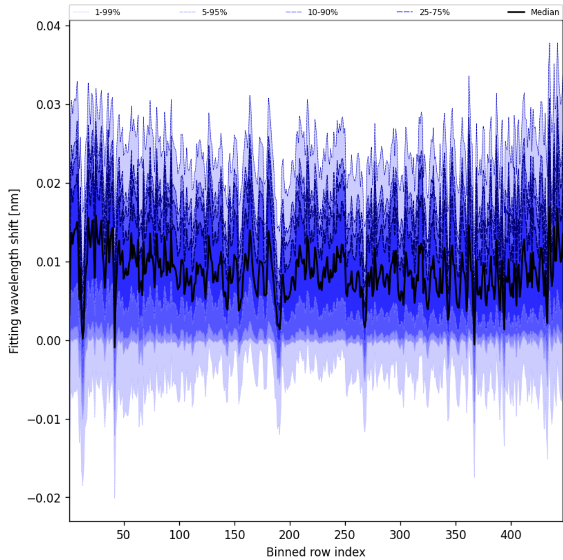
Figure 63: Along track statistics of “Fitting wavelength shift” for 2025-09-27 to 2025-09-28
