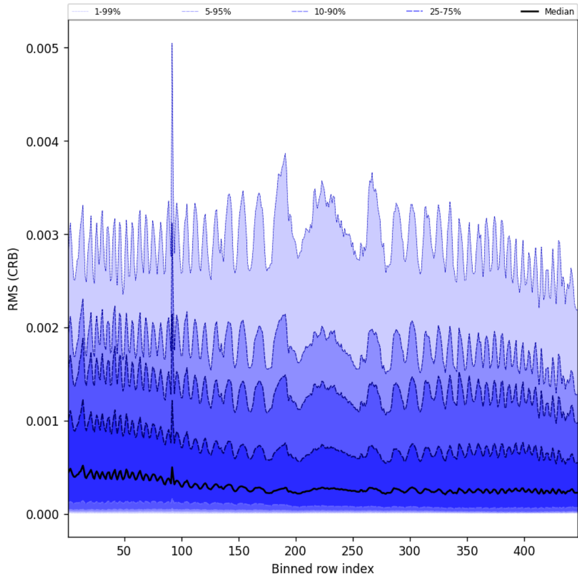
Figure 62: Along track statistics of “RMS (CRB)” for 2025-09-27 to 2025-09-28
