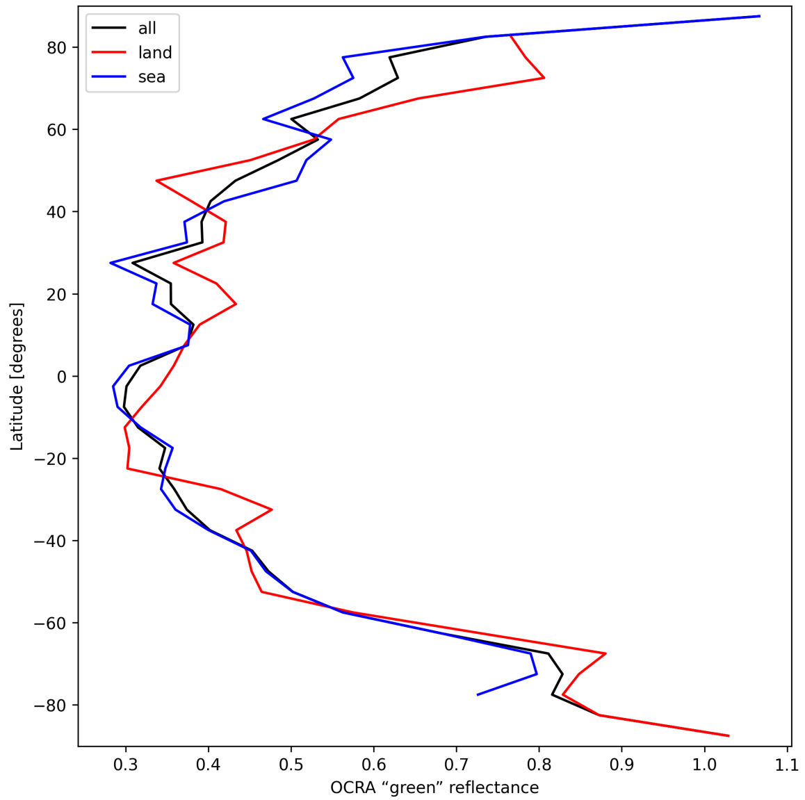
Figure 34: Zonal average of “OCRA “green” reflectance” for 2025-09-27 to 2025-09-28.
