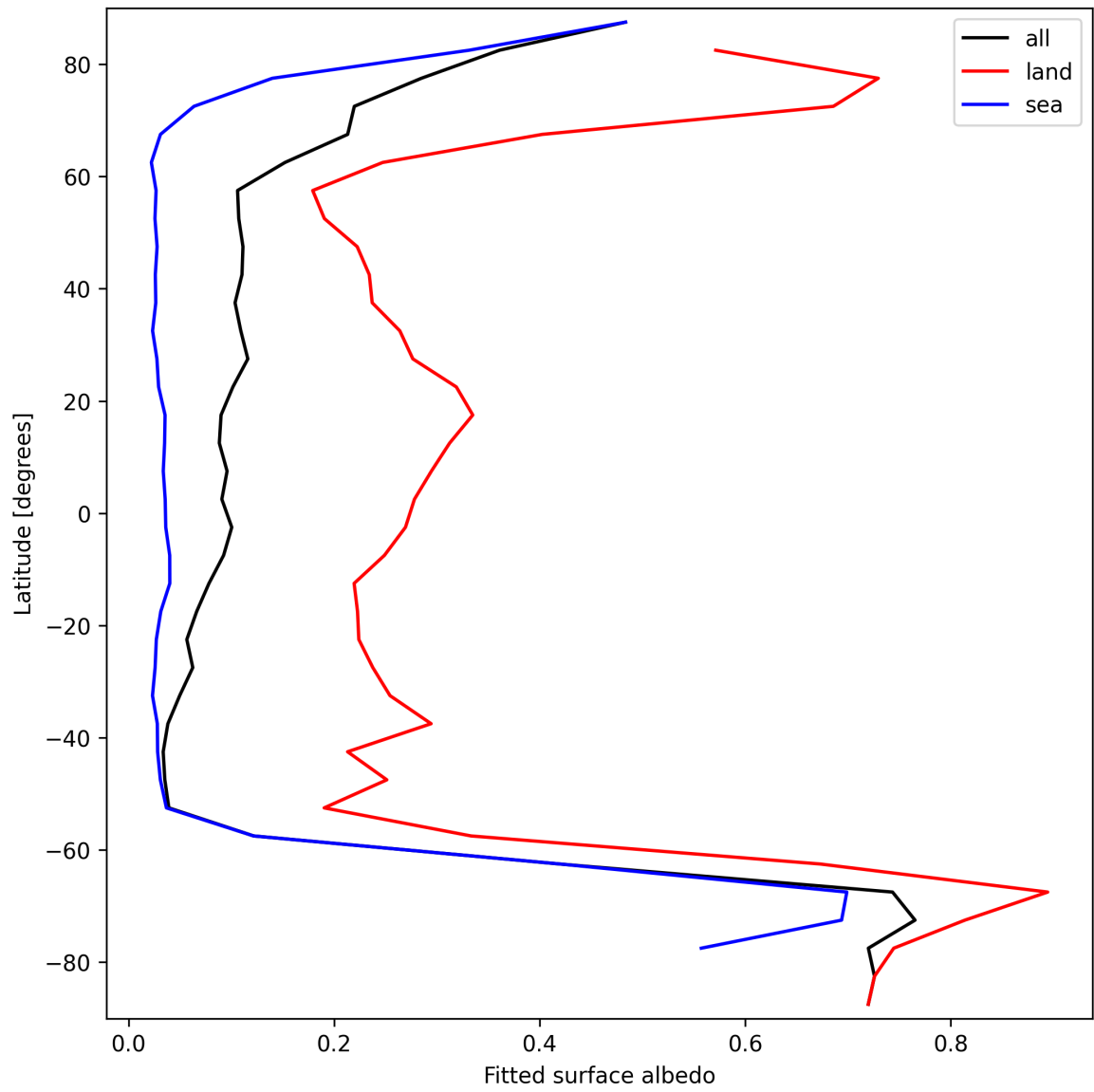
Figure 27: Zonal average of “Fitted surface albedo” for 2025-09-27 to 2025-09-28.
