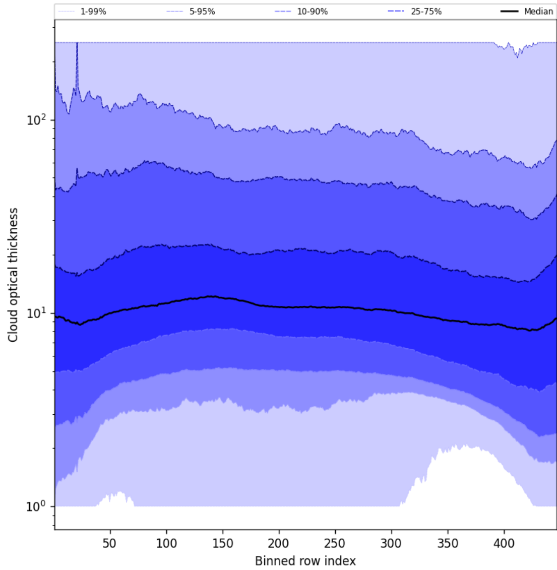
Figure 55: Along track statistics of “Cloud optical thickness” for 2025-09-27 to 2025-09-28
