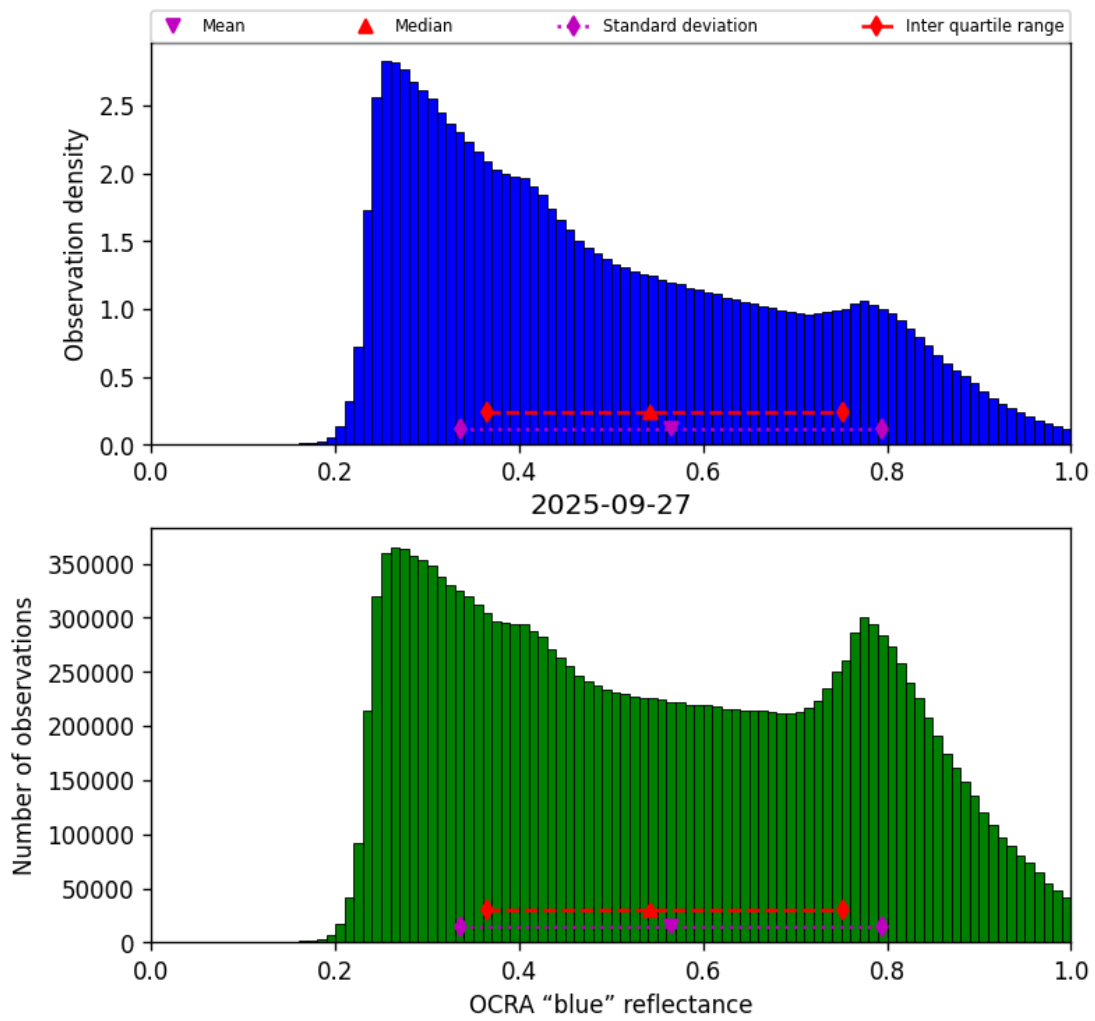
Figure 49: Histogram of “OCRA “blue” reflectance” for 2025-09-27 to 2025-09-28
