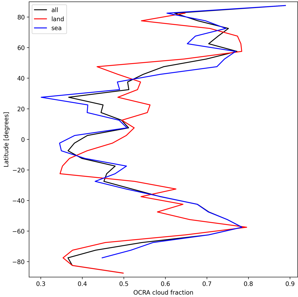
Figure 32: Zonal average of “OCRA cloud fraction” for 2025-09-27 to 2025-09-28.
