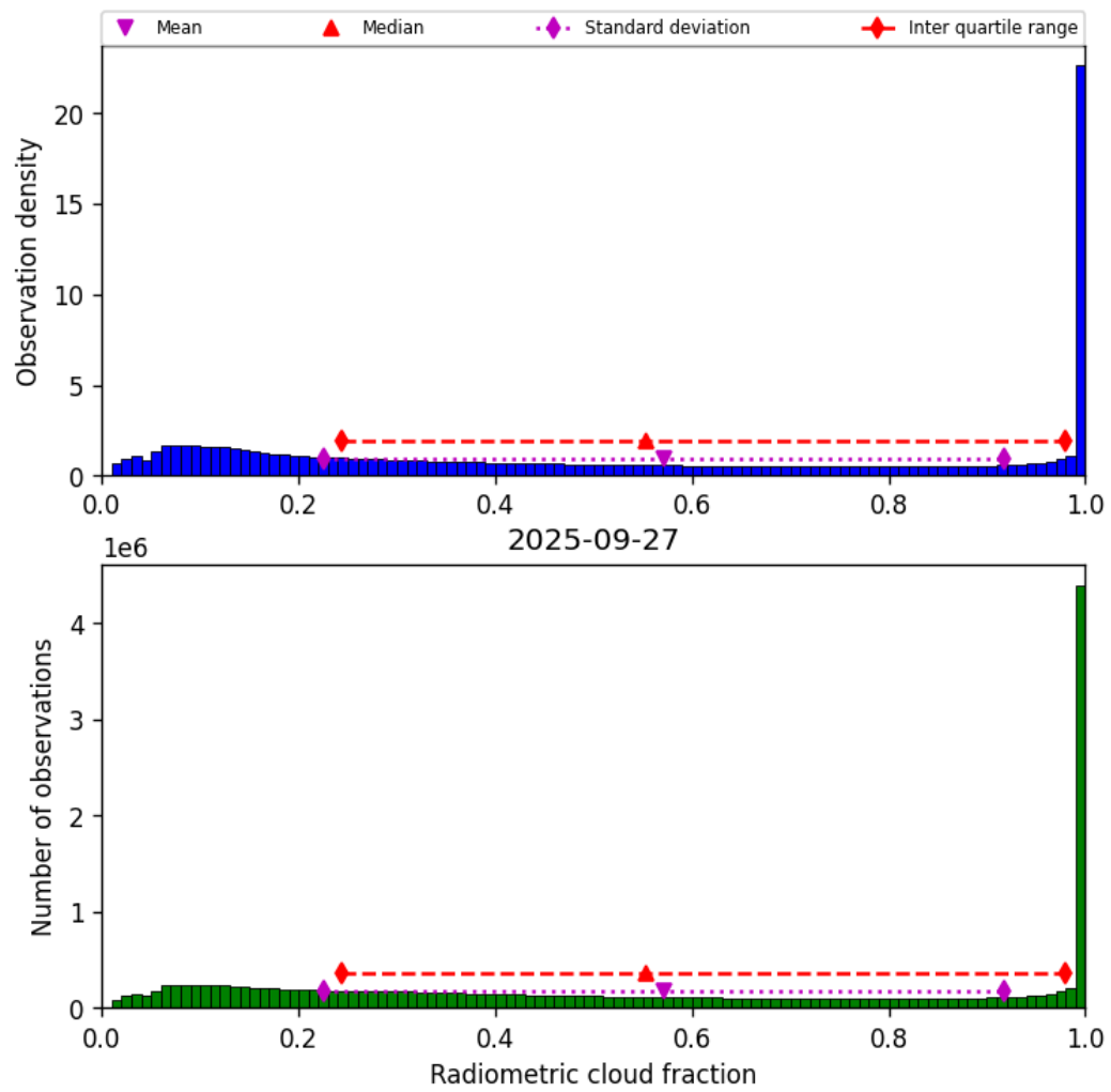
Figure 37: Histogram of “Radiometric cloud fraction” for 2025-09-27 to 2025-09-28
