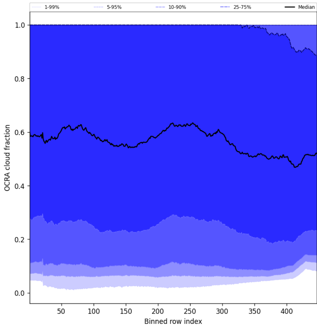
Figure 64: Along track statistics of “OCRA cloud fraction” for 2025-09-27 to 2025-09-28
