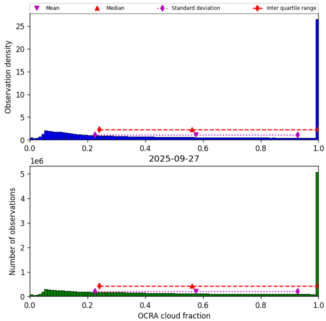
Figure 48: Histogram of “OCRA cloud fraction” for 2025-09-27 to 2025-09-28
