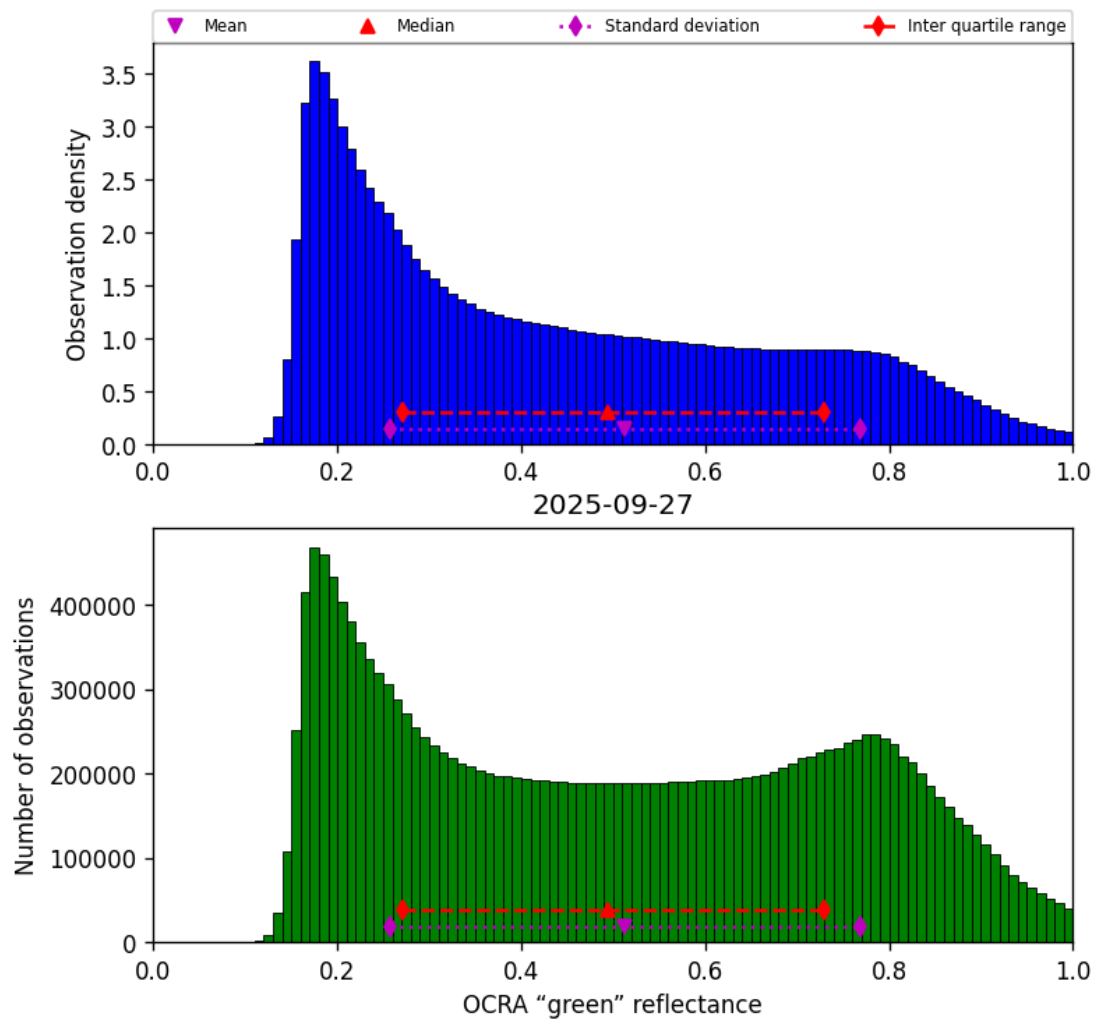
Figure 50: Histogram of “OCRA “green” reflectance” for 2025-09-27 to 2025-09-28
