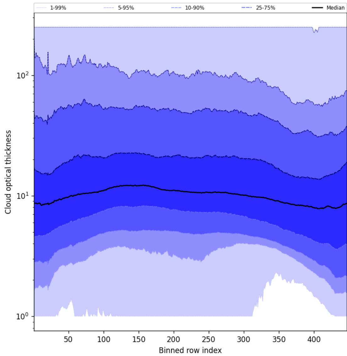
Figure 55: Along track statistics of “Cloud optical thickness” for 2025-09-29 to 2025-09-29
