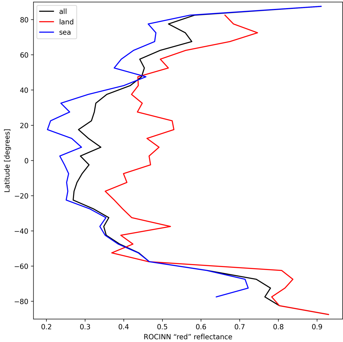
Figure 35: Zonal average of "ROCINN "red" reflectance" for 2025-09-29 to 2025-09-29.
