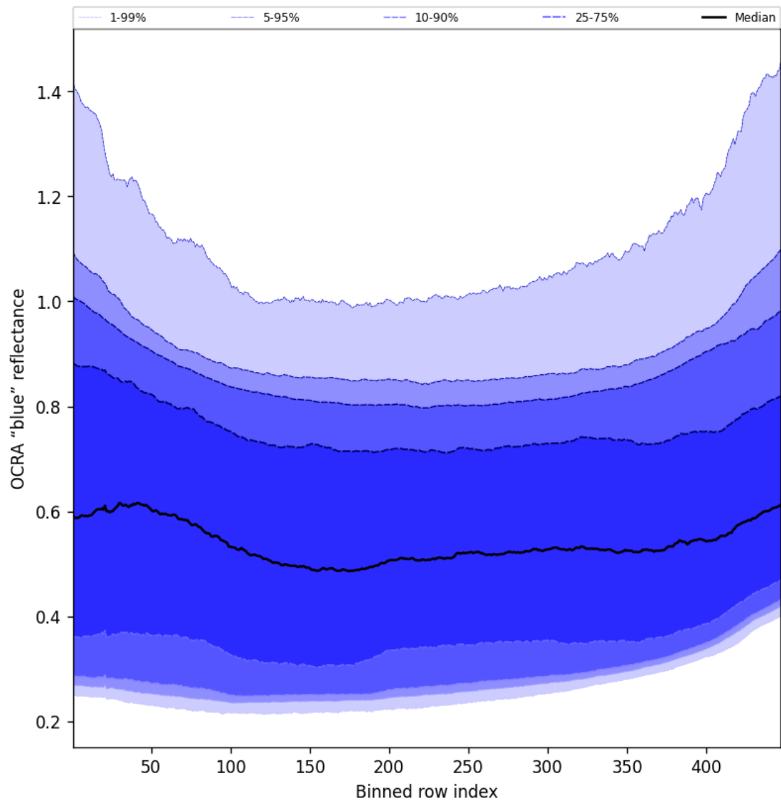
Figure 65: Along track statistics of "OCRA "blue" reflectance" for 2025-09-29 to 2025-09-29
