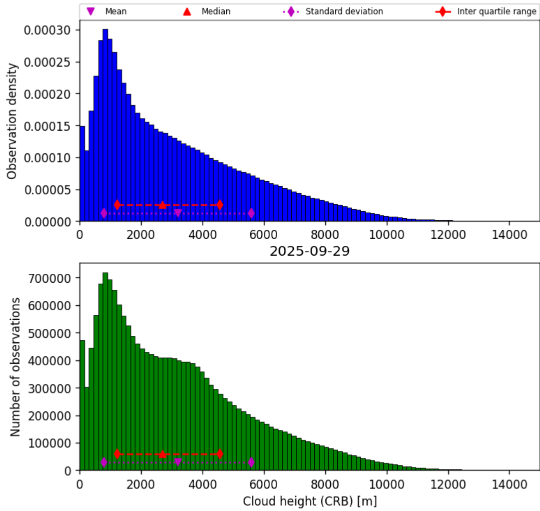
Figure 41: Histogram of “Cloud height (CRB)” for 2025-09-29 to 2025-09-29
