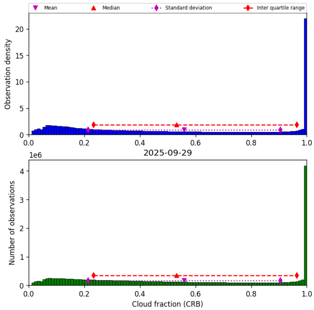
Figure 40: Histogram of "Cloud fraction (CRB)" for 2025-09-29 to 2025-09-29
