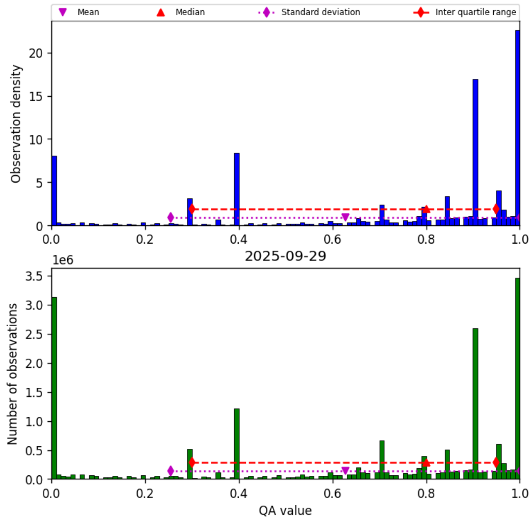
Figure 36: Histogram of “QA value” for 2025-09-29 to 2025-09-29
