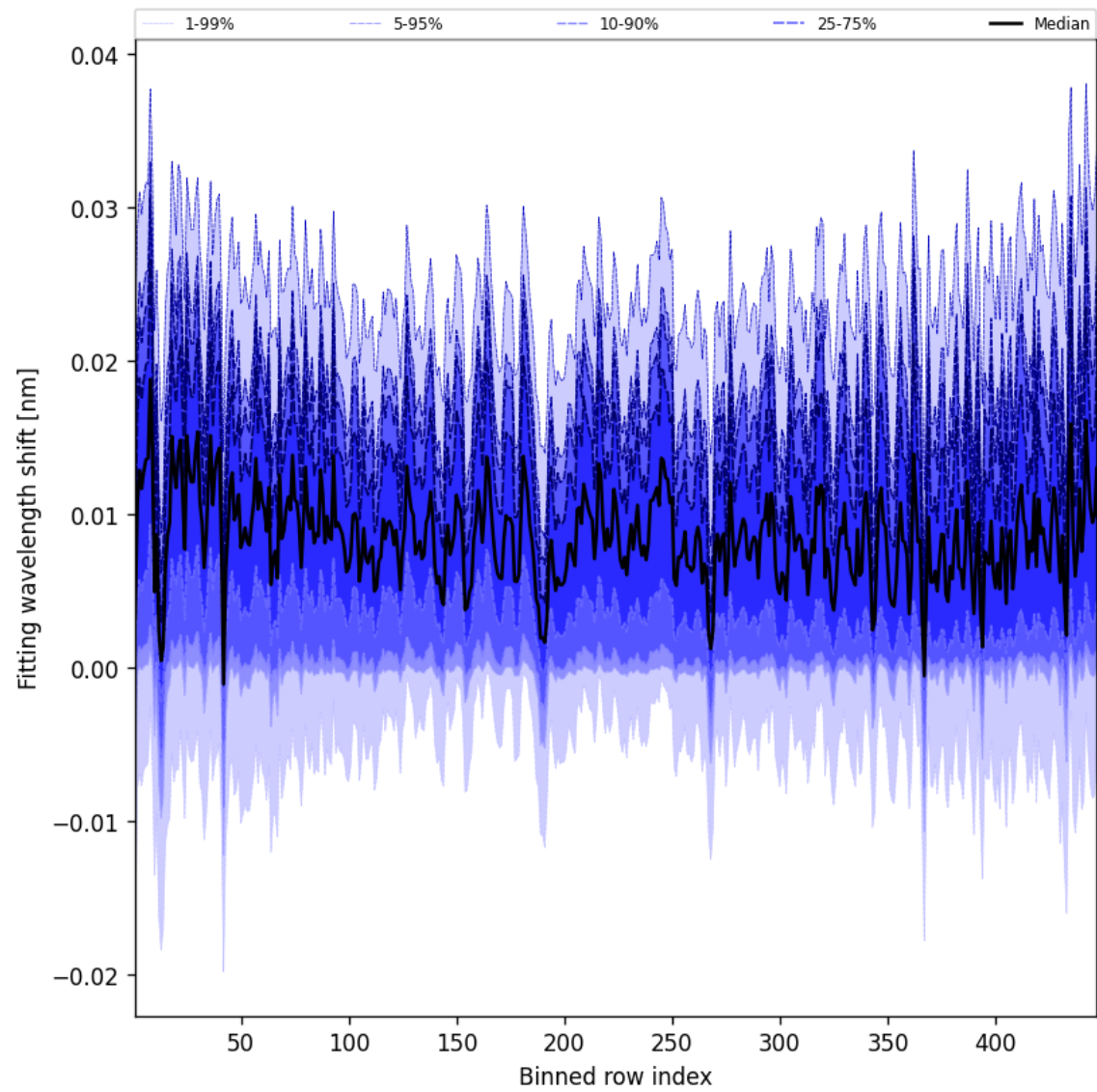
Figure 63: Along track statistics of “Fitting wavelength shift” for 2025-09-29 to 2025-09-29
