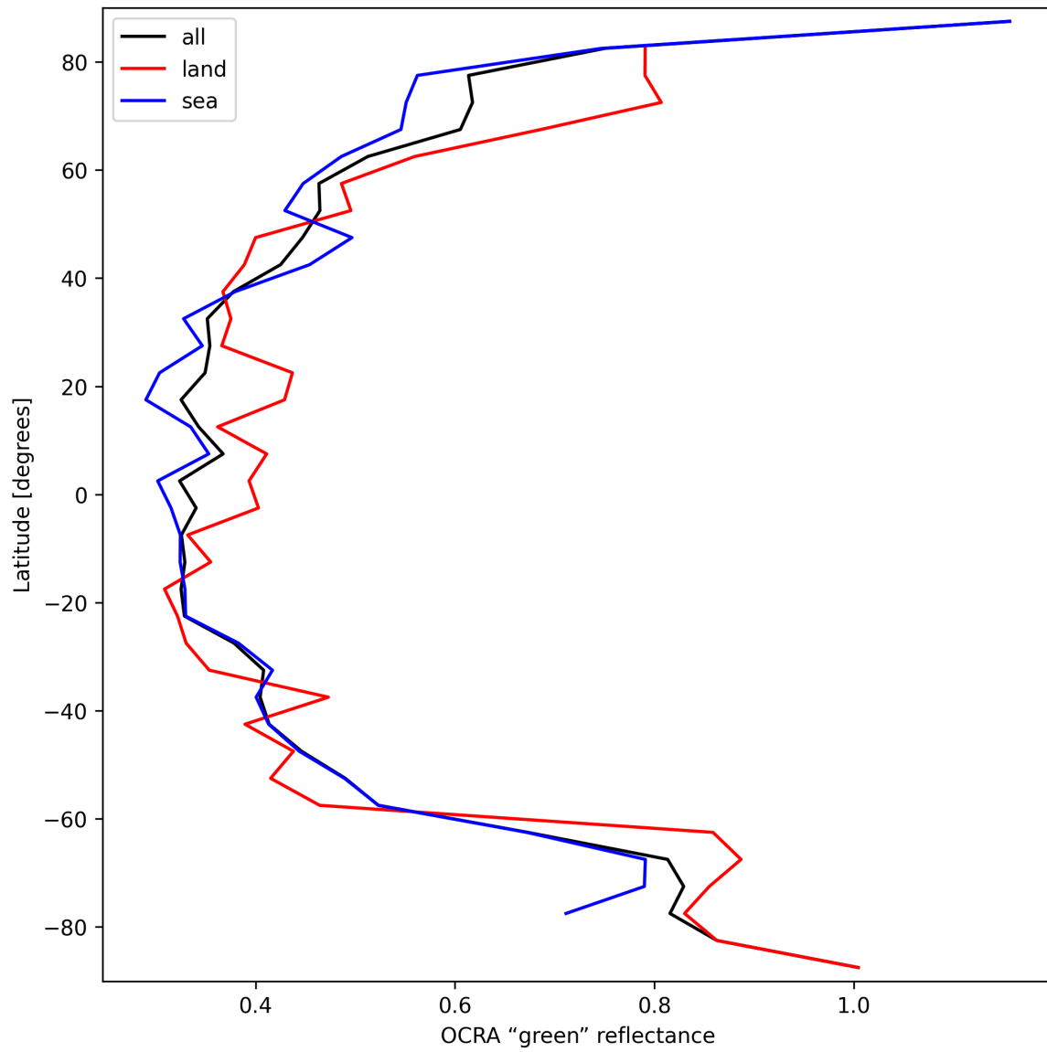
Figure 34: Zonal average of “OCRA “green” reflectance” for 2025-09-29 to 2025-09-29.
