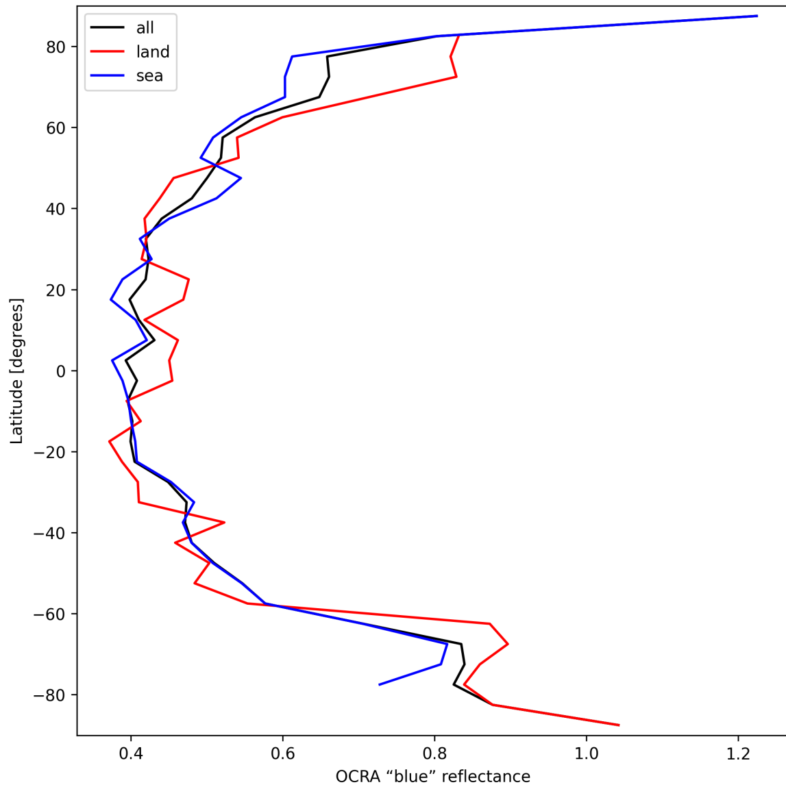
Figure 33: Zonal average of "OCRA "blue" reflectance" for 2025-09-29 to 2025-09-29.
