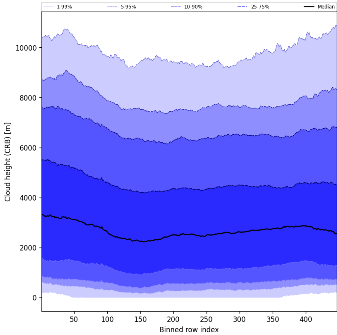
Figure 57: Along track statistics of “Cloud height (CRB)” for 2025-09-29 to 2025-09-29
