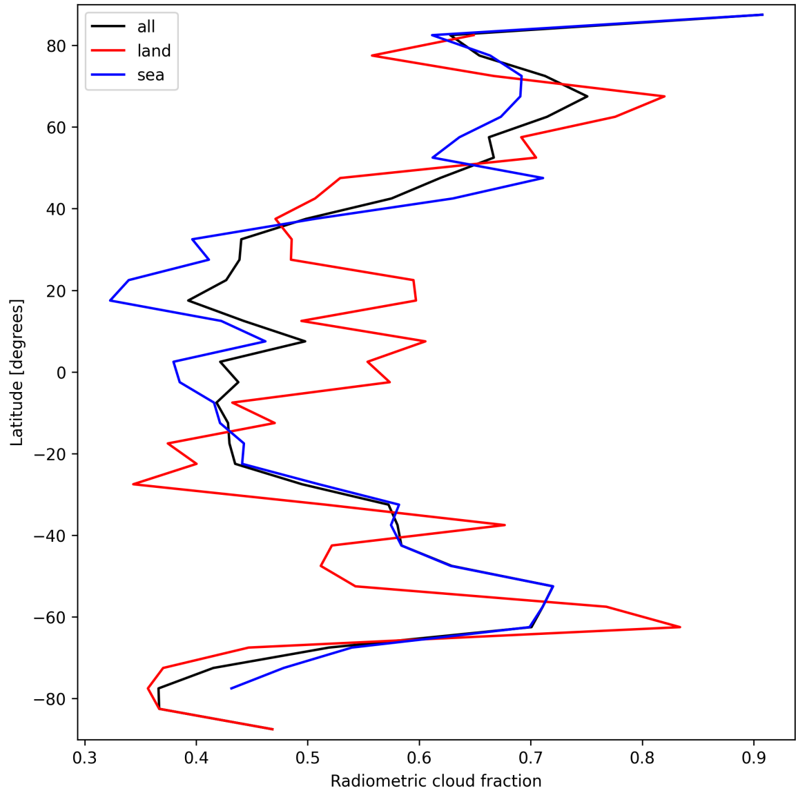
Figure 21: Zonal average of “Radiometric cloud fraction” for 2025-09-29 to 2025-09-29.
