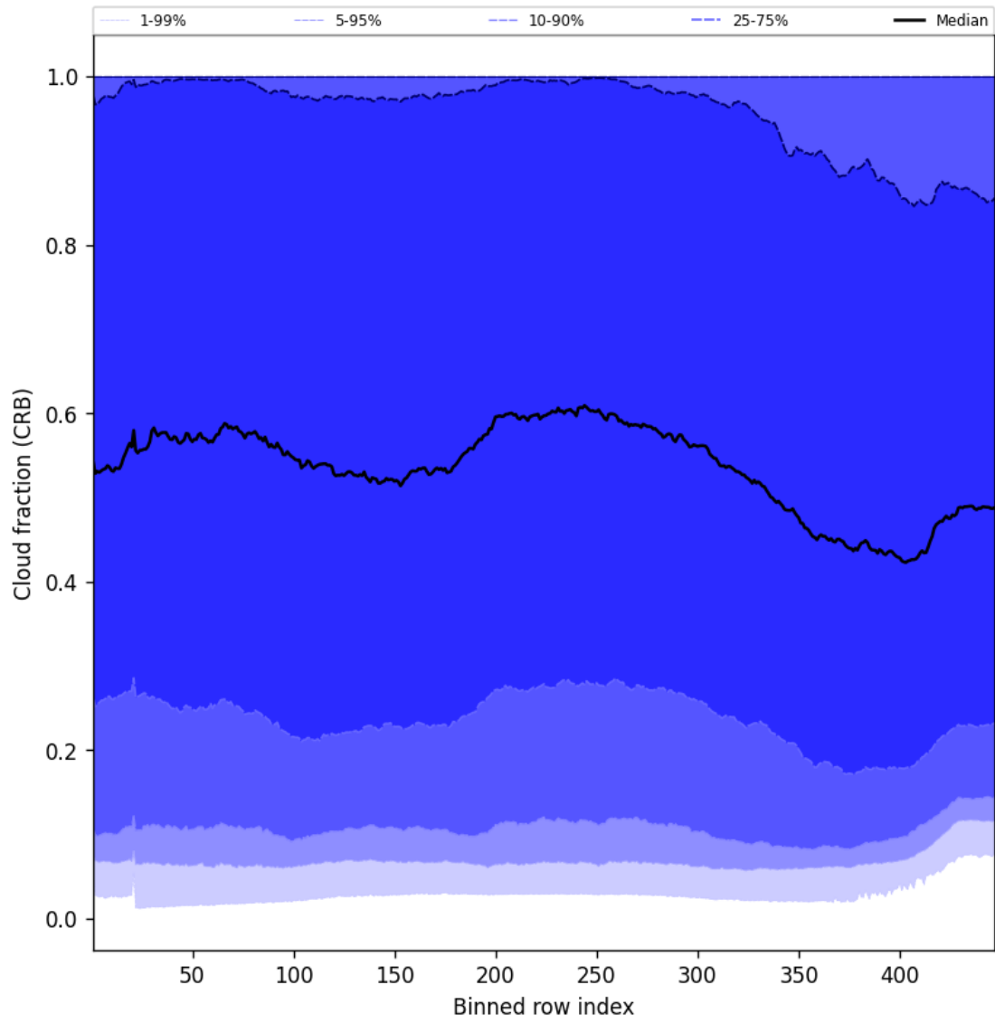
Figure 56: Along track statistics of “Cloud fraction (CRB)” for 2025-09-29 to 2025-09-29
