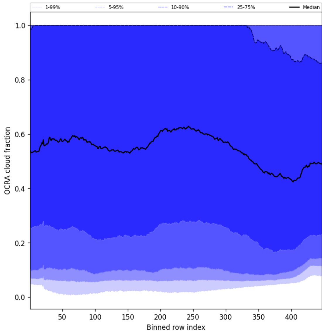
Figure 64: Along track statistics of “OCRA cloud fraction” for 2025-09-29 to 2025-09-29
