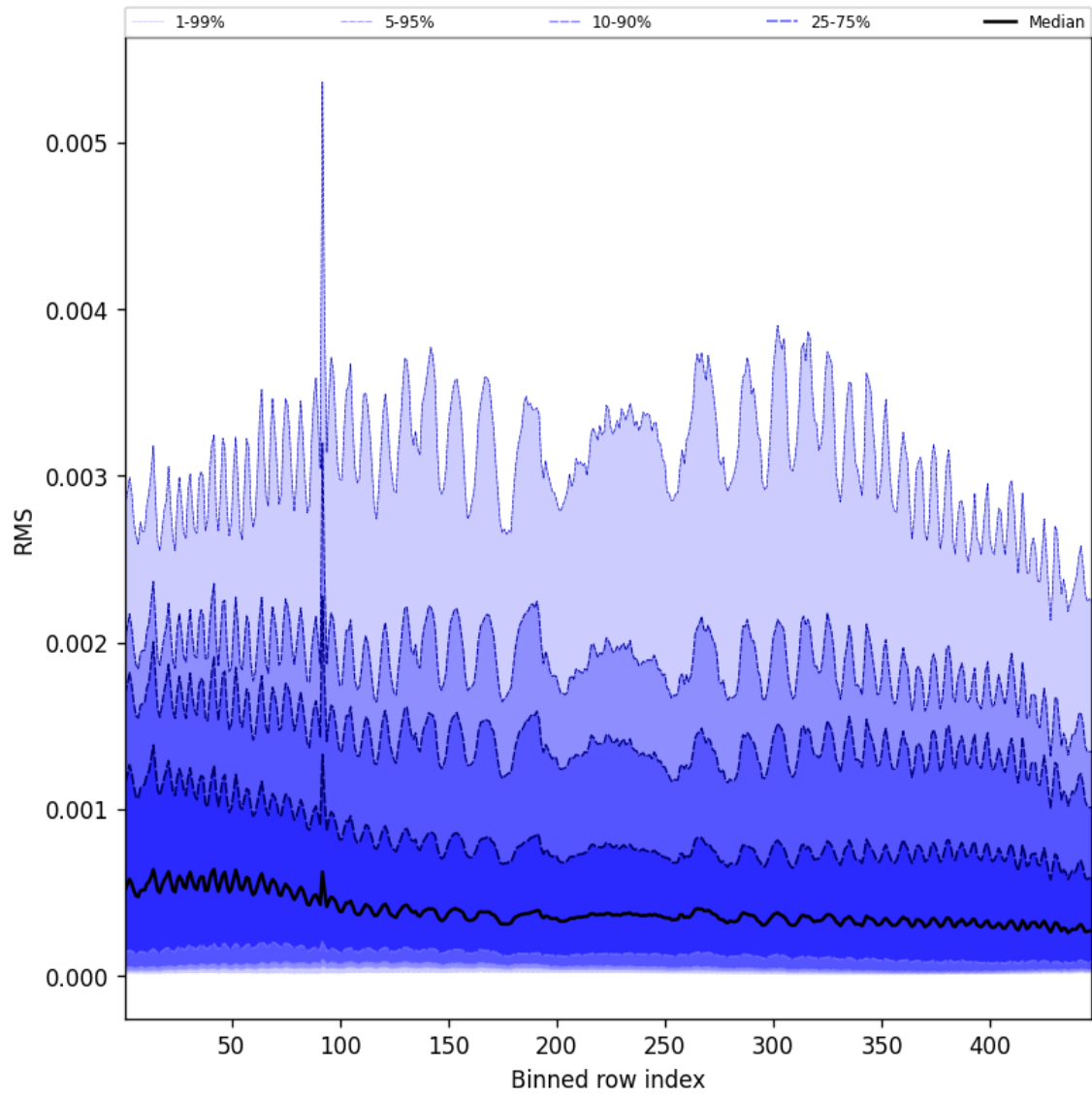
Figure 61: Along track statistics of “RMS” for 2025-09-29 to 2025-09-29
