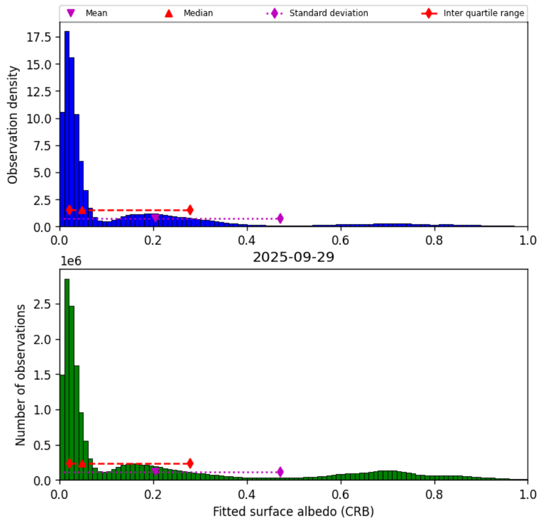
Figure 44: Histogram of “Fitted surface albedo (CRB)” for 2025-09-29 to 2025-09-29
