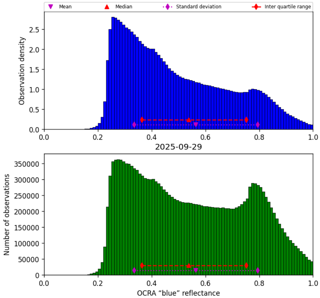
Figure 49: Histogram of “OCRA “blue” reflectance” for 2025-09-29 to 2025-09-29
