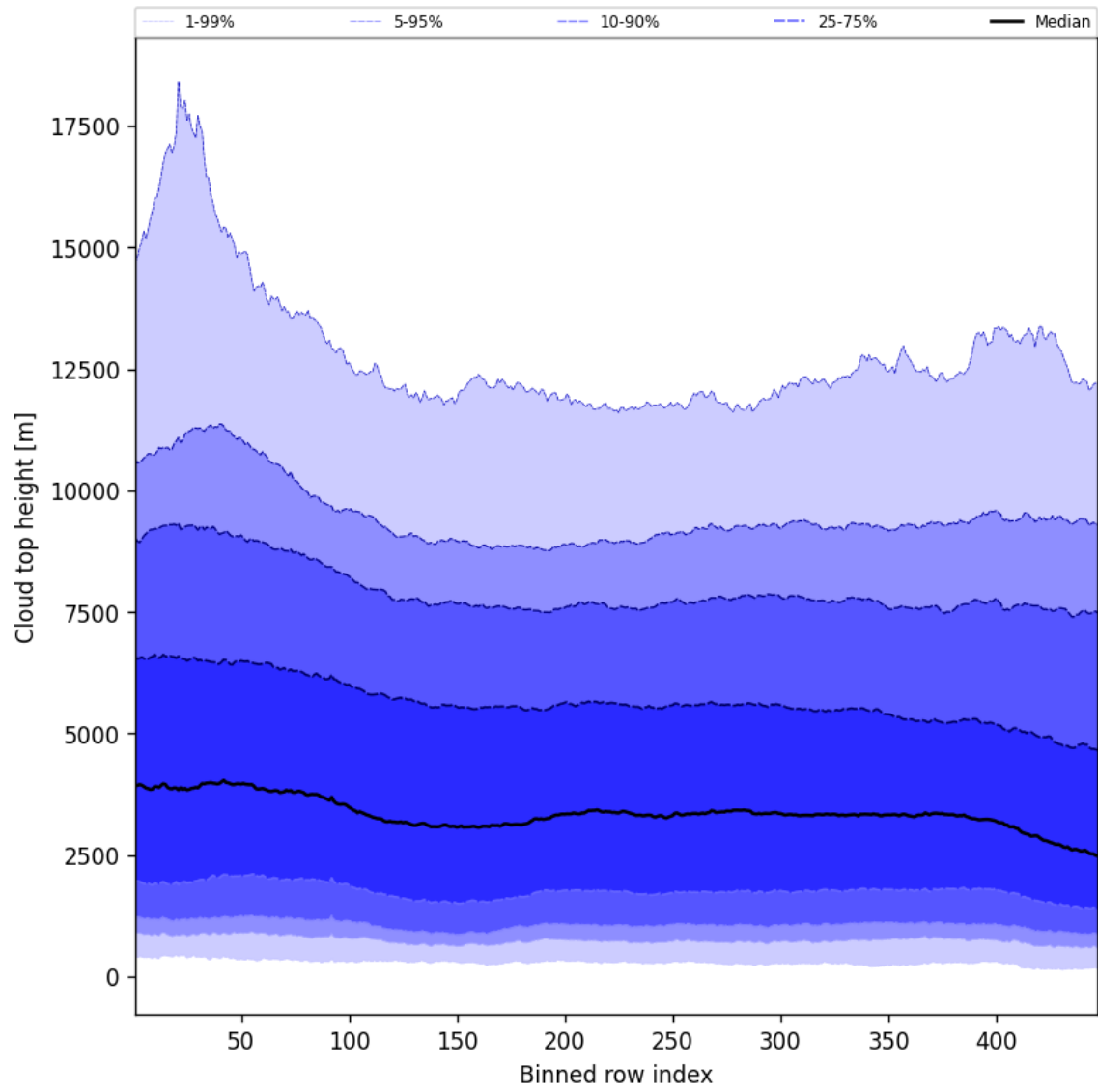
Figure 54: Along track statistics of “Cloud top height” for 2025-09-29 to 2025-09-29
