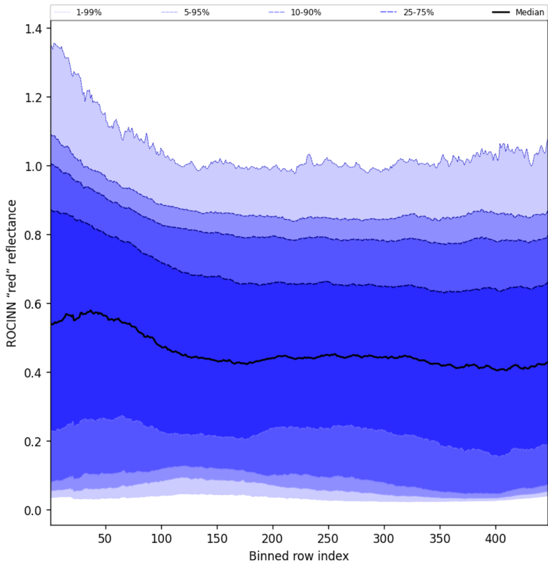
Figure 67: Along track statistics of "ROCINN "red" reflectance" for 2025-09-29 to 2025-09-29
