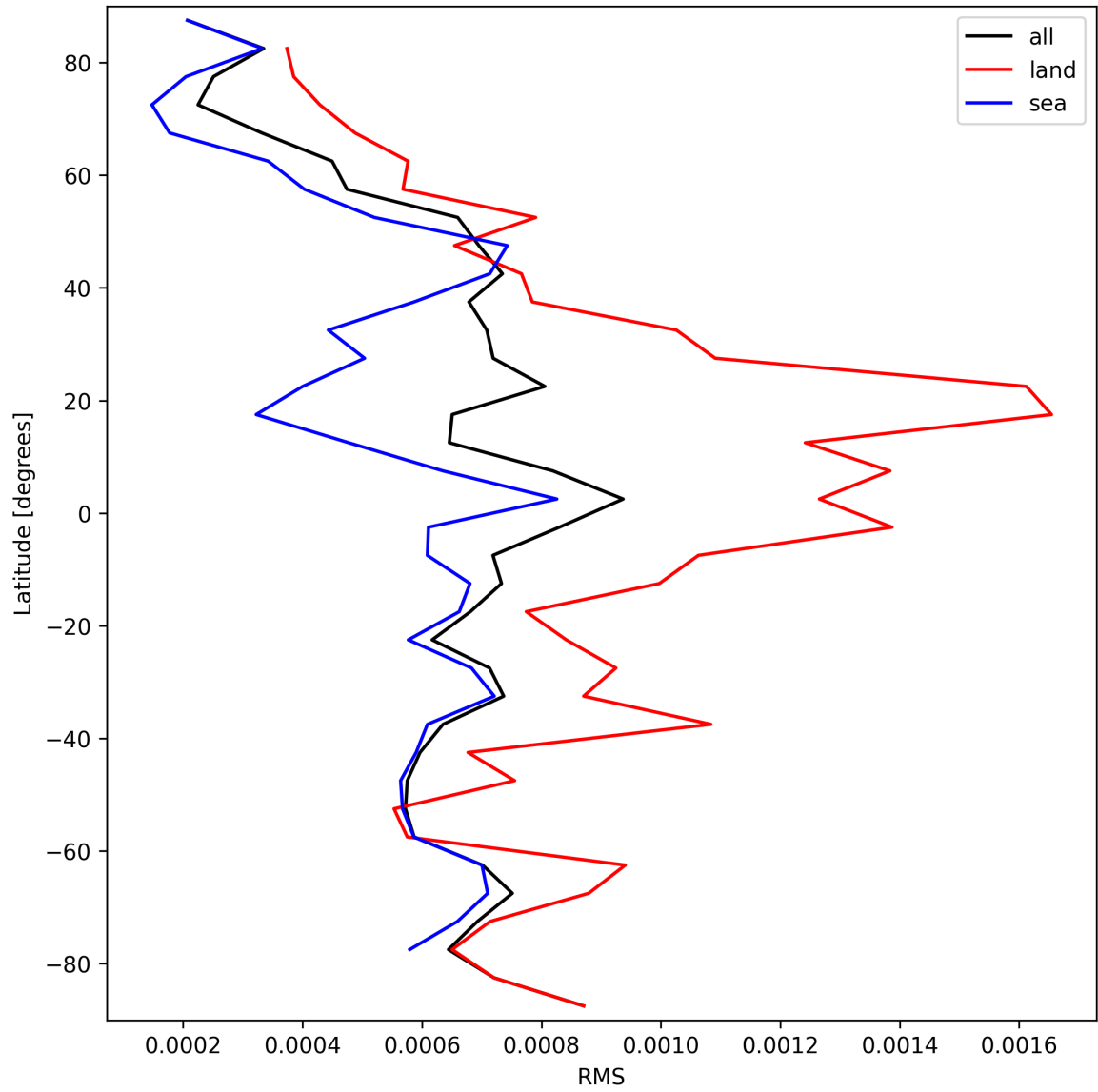
Figure 29: Zonal average of “RMS” for 2025-09-29 to 2025-09-29.
