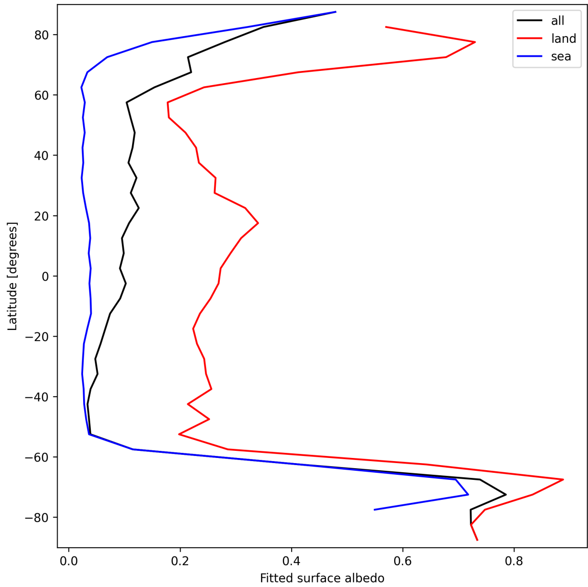
Figure 27: Zonal average of “Fitted surface albedo” for 2025-09-29 to 2025-09-29.
