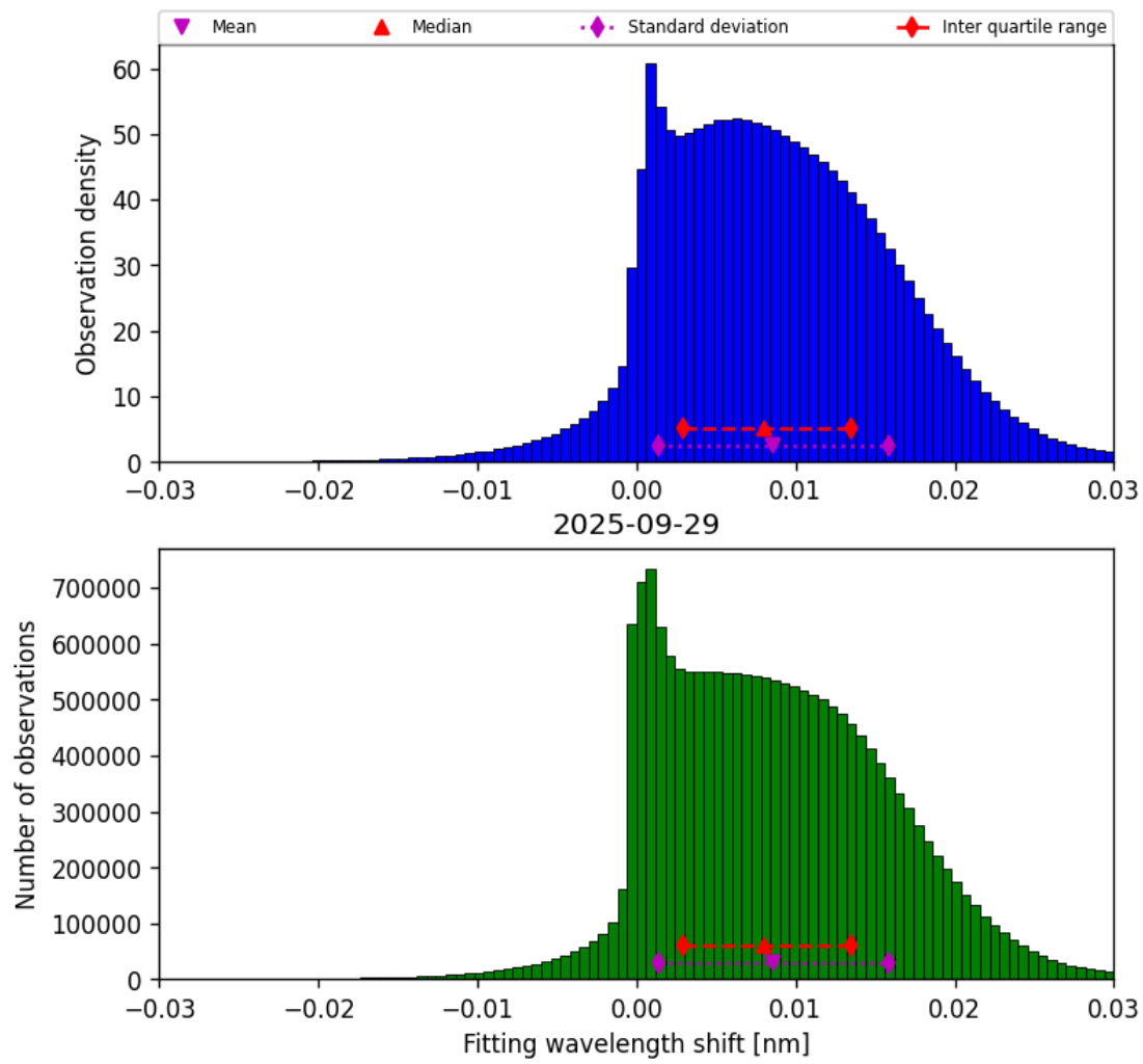
Figure 47: Histogram of “Fitting wavelength shift” for 2025-09-29 to 2025-09-29
