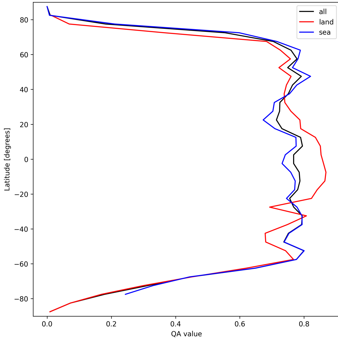
Figure 20: Zonal average of “QA value” for 2025-09-29 to 2025-09-29.
