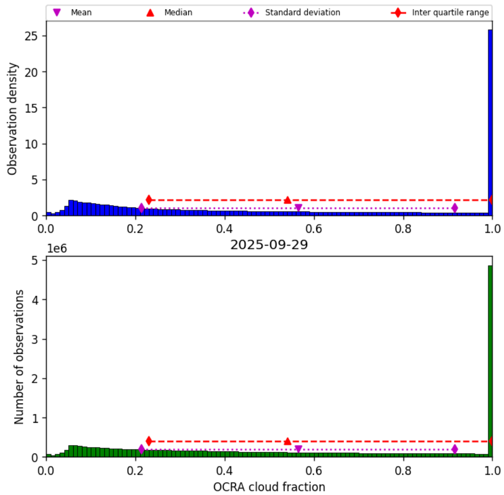
Figure 48: Histogram of “OCRA cloud fraction” for 2025-09-29 to 2025-09-29
