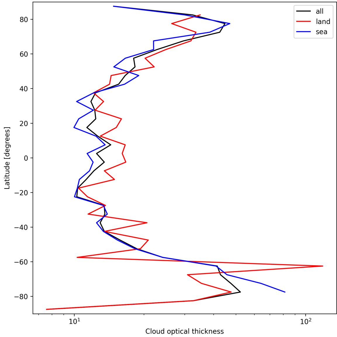
Figure 23: Zonal average of “Cloud optical thickness” for 2025-09-29 to 2025-09-29.
