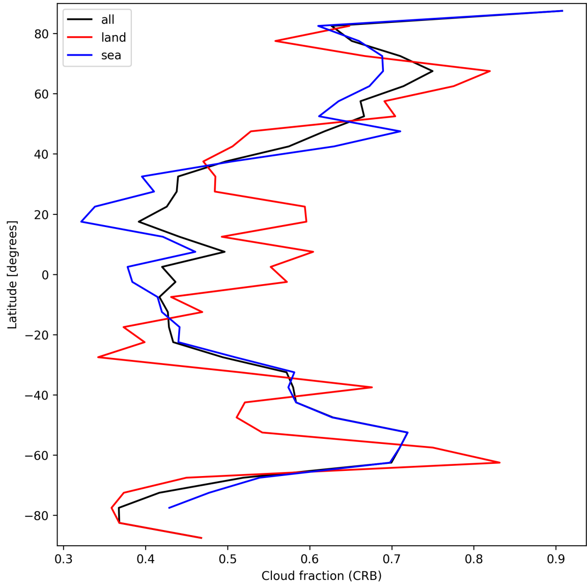
Figure 24: Zonal average of “Cloud fraction (CRB)” for 2025-09-29 to 2025-09-29.
