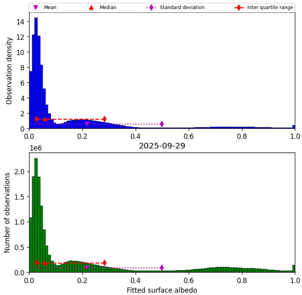
Figure 43: Histogram of “Fitted surface albedo” for 2025-09-29 to 2025-09-29
