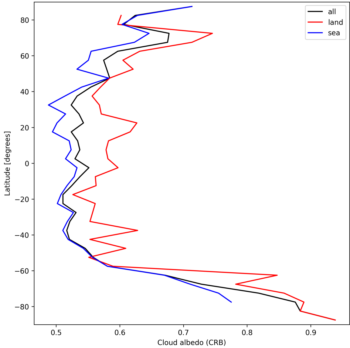
Figure 26: Zonal average of “Cloud albedo (CRB)” for 2025-09-29 to 2025-09-29.
