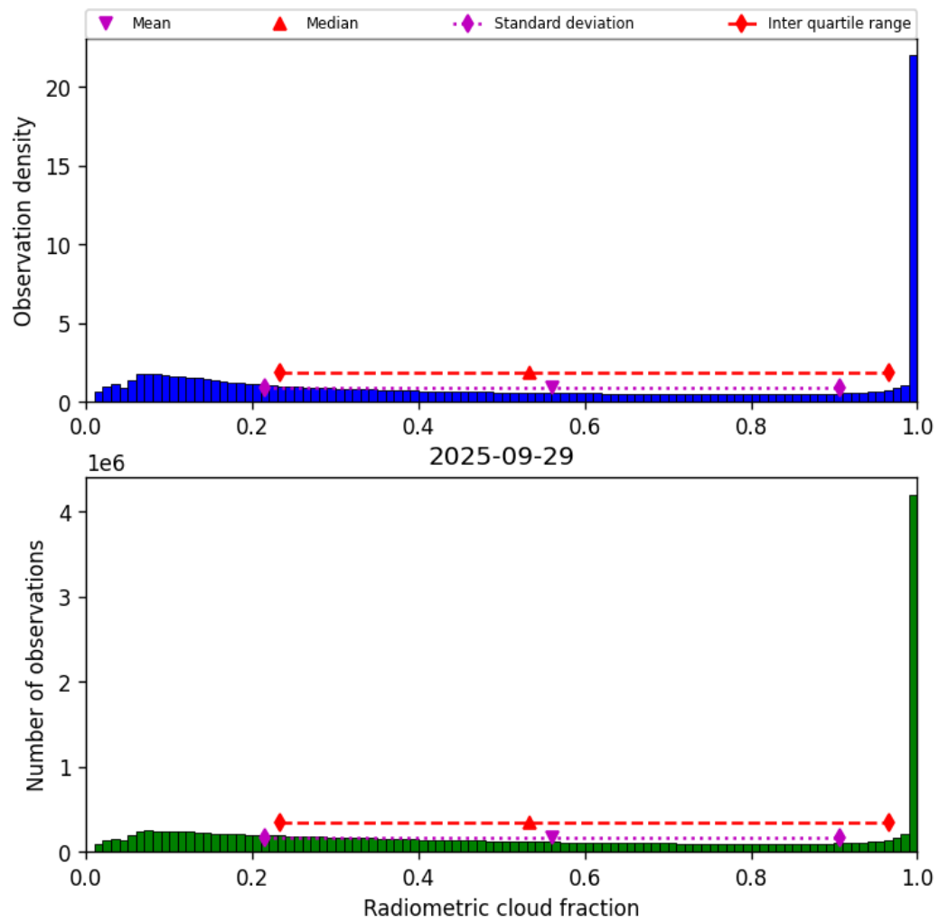
Figure 37: Histogram of “Radiometric cloud fraction” for 2025-09-29 to 2025-09-29
