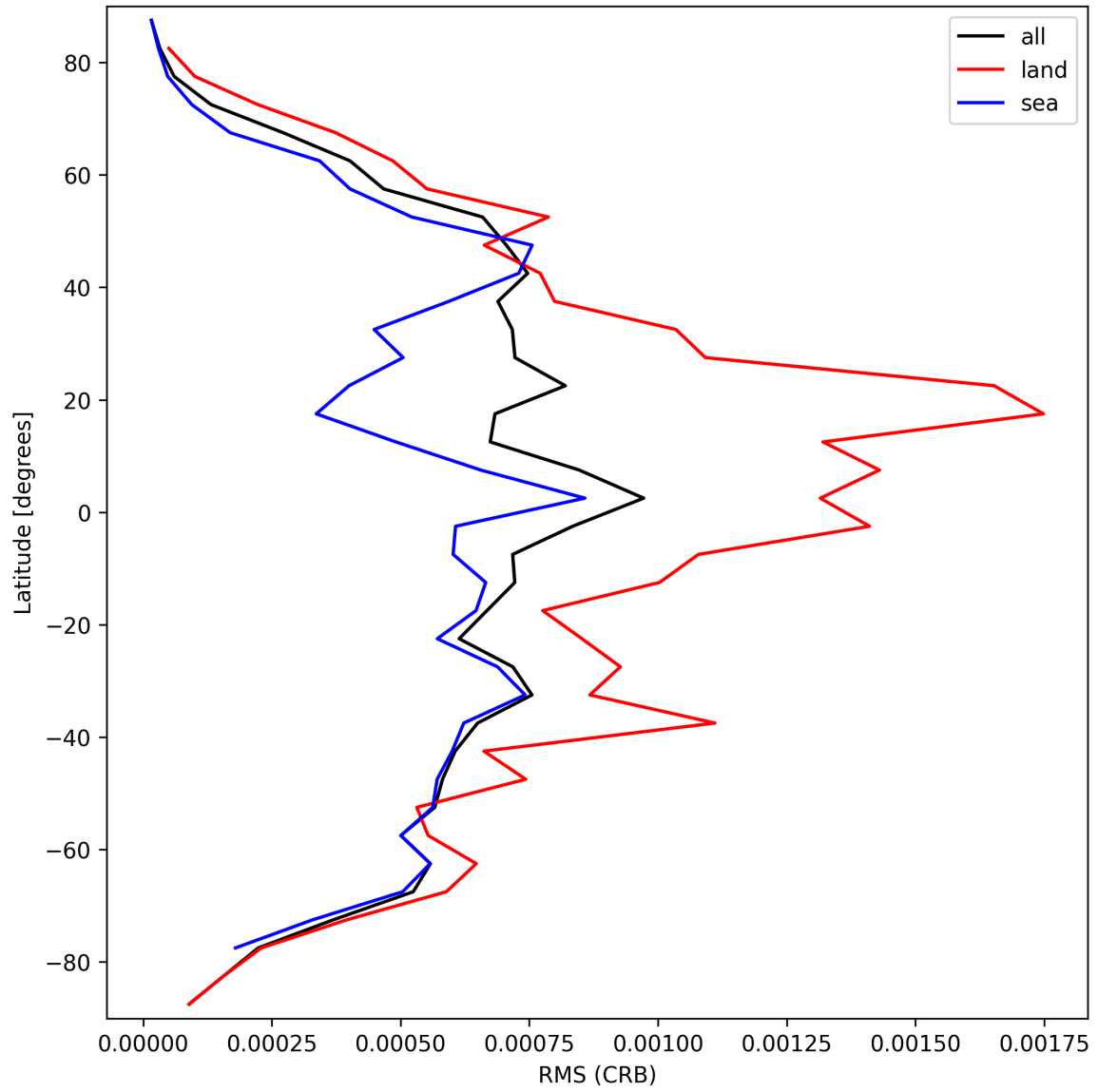
Figure 30: Zonal average of “RMS (CRB)” for 2025-09-29 to 2025-09-29.
