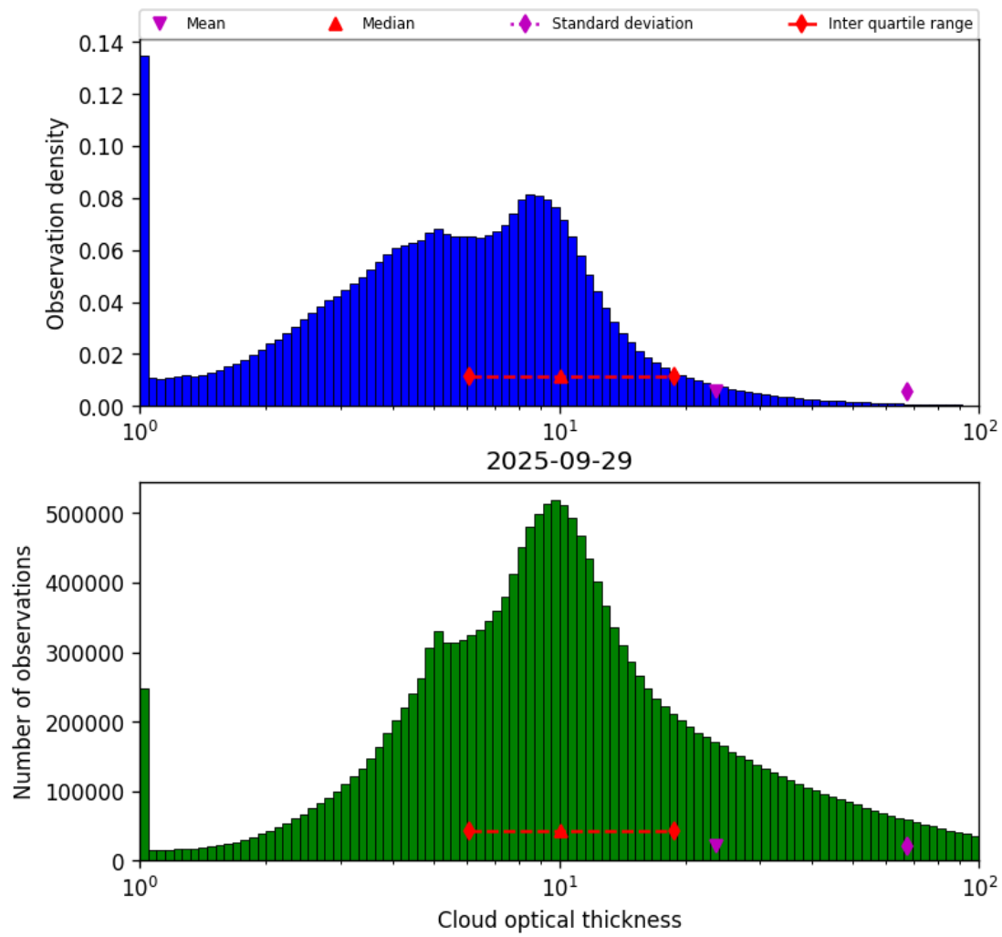
Figure 39: Histogram of “Cloud optical thickness” for 2025-09-29 to 2025-09-29
