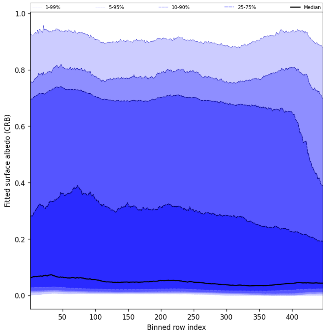
Figure 60: Along track statistics of “Fitted surface albedo (CRB)” for 2025-09-29 to 2025-09-29
