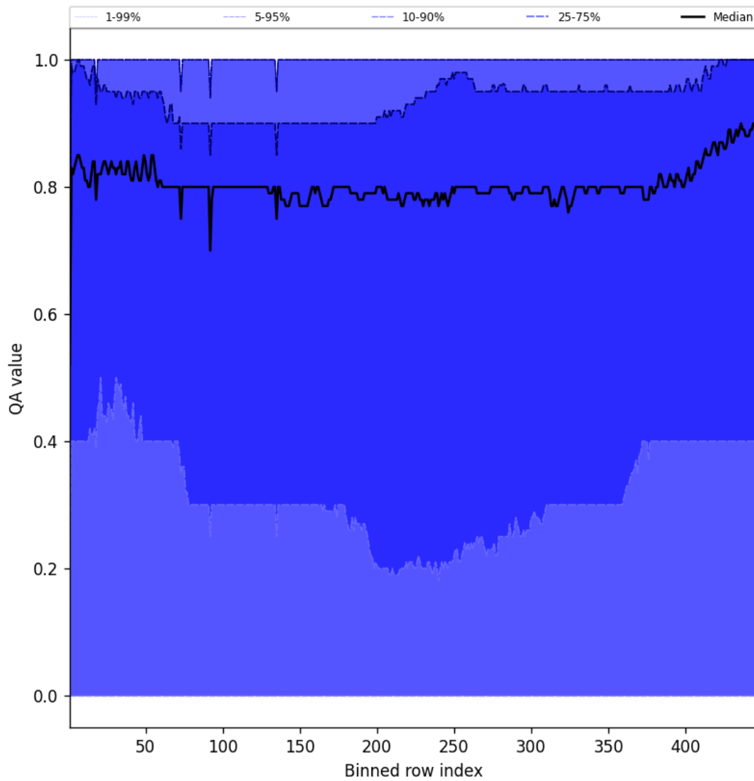
Figure 52: Along track statistics of “QA value” for 2025-09-29 to 2025-09-29
