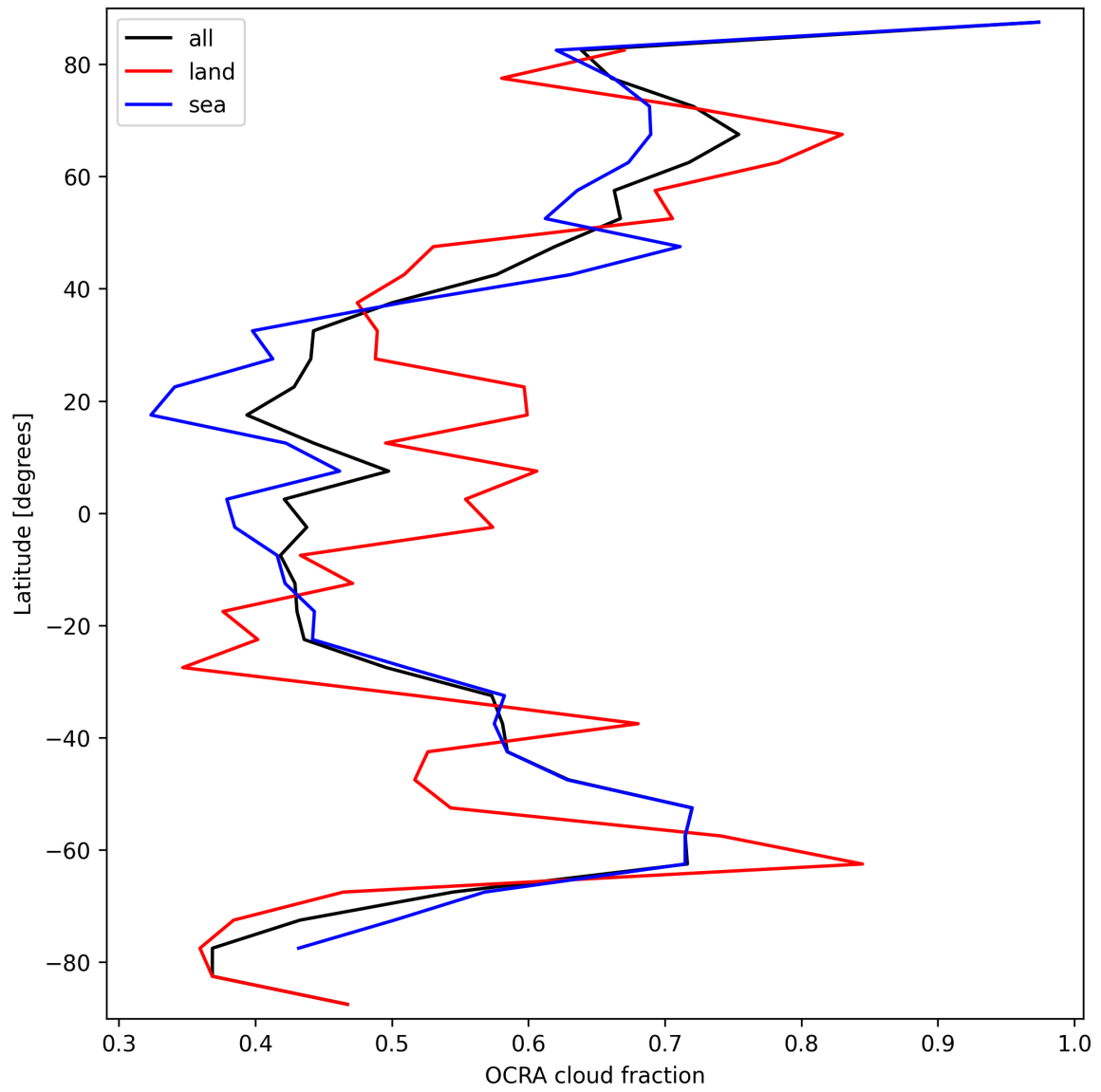
Figure 32: Zonal average of “OCRA cloud fraction” for 2025-09-29 to 2025-09-29.
