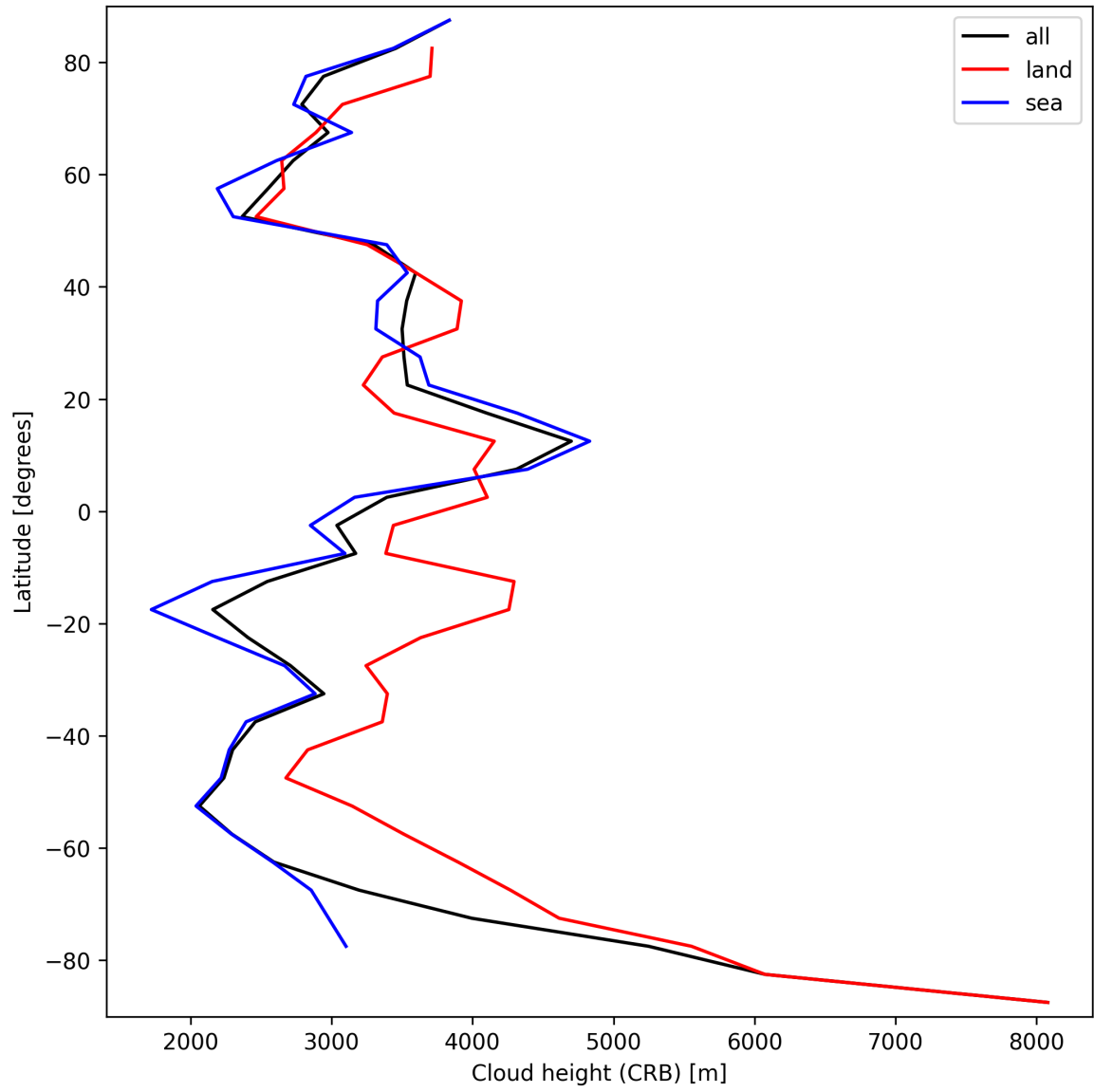
Figure 25: Zonal average of “Cloud height (CRB)” for 2025-09-29 to 2025-09-29.
