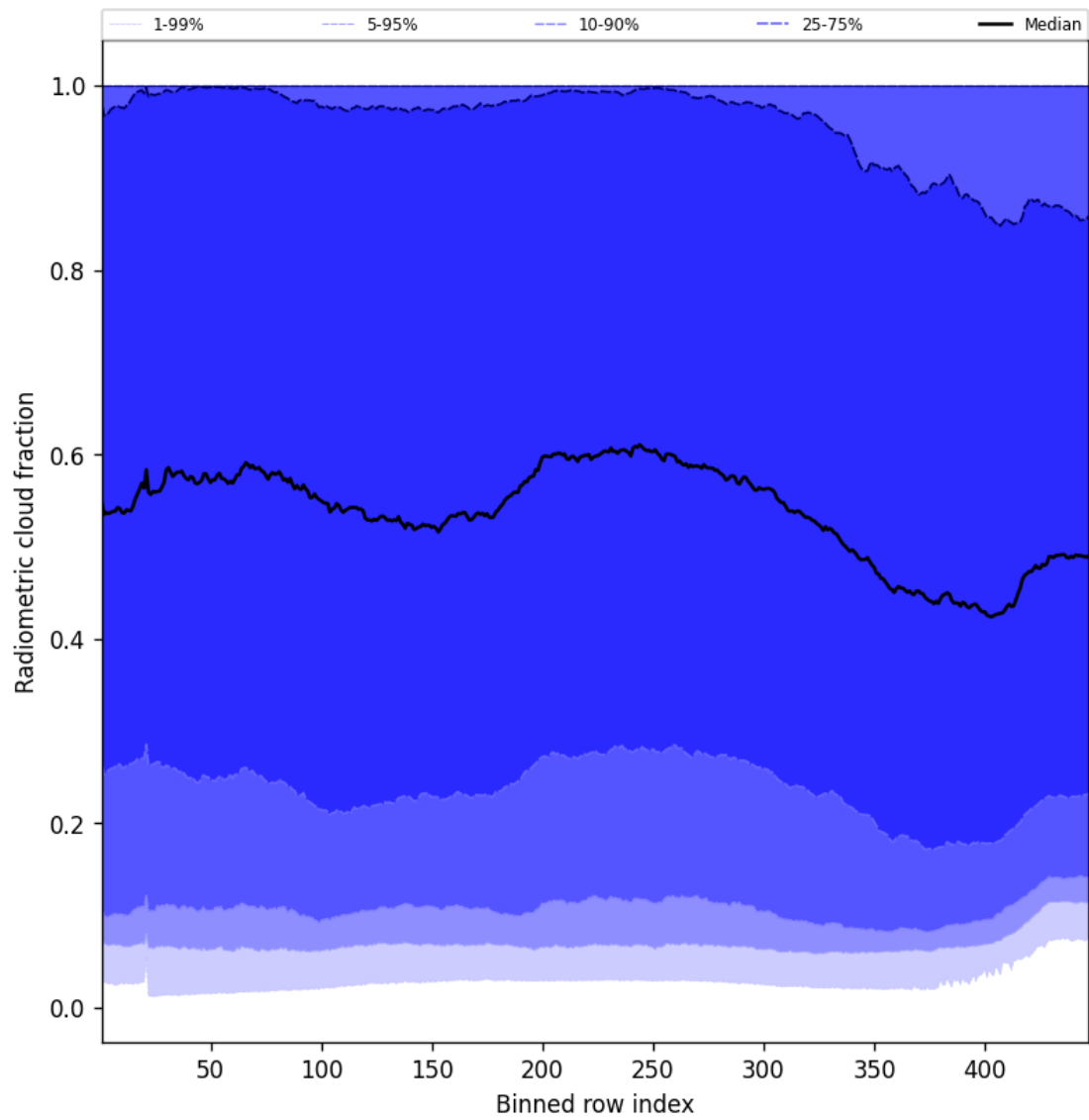
Figure 53: Along track statistics of “Radiometric cloud fraction” for 2025-09-29 to 2025-09-29
