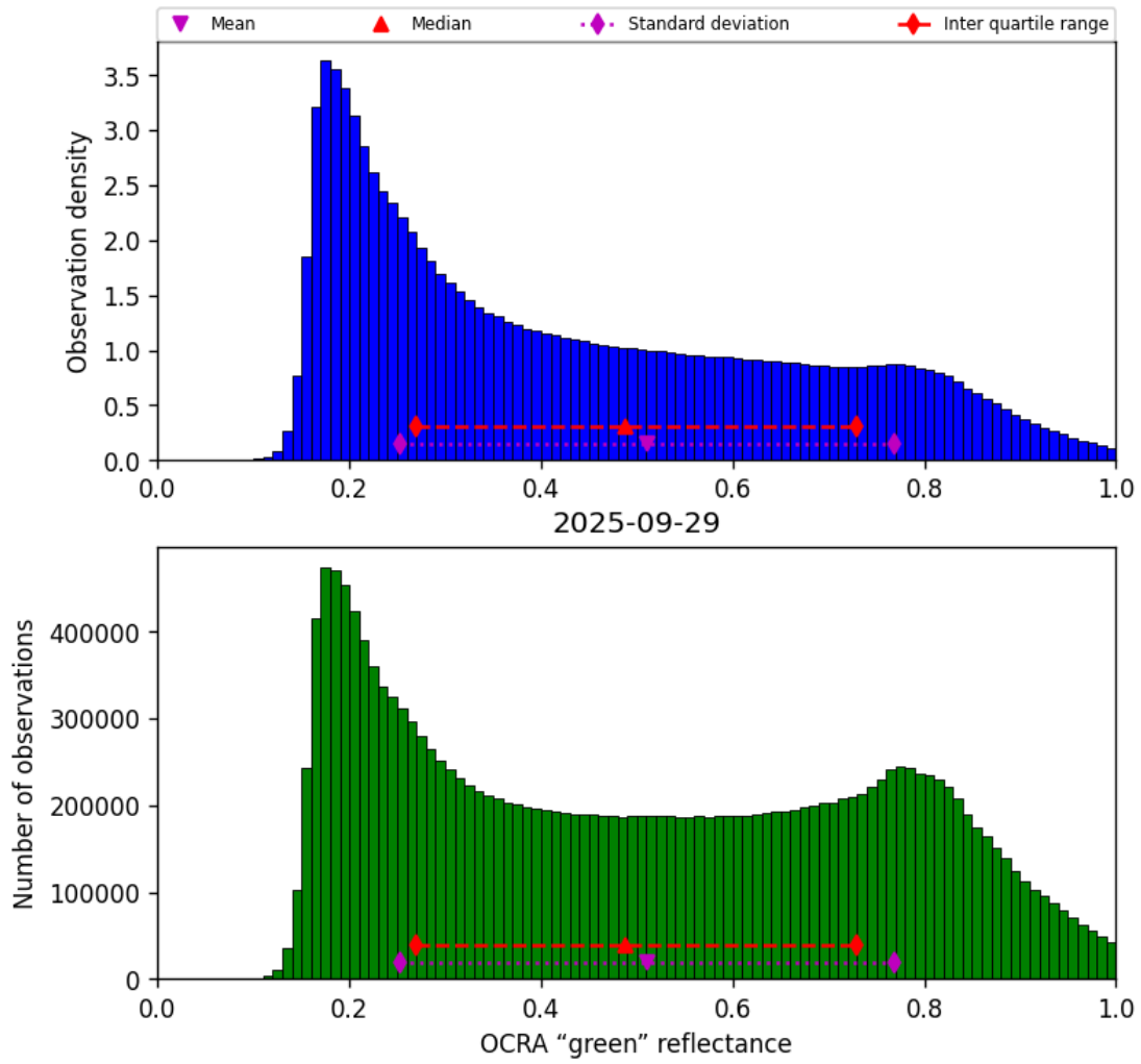
Figure 50: Histogram of “OCRA “green” reflectance” for 2025-09-29 to 2025-09-29
