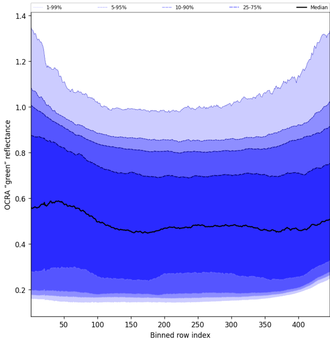
Figure 66: Along track statistics of “OCRA “green” reflectance” for 2025-09-29 to 2025-09-29
