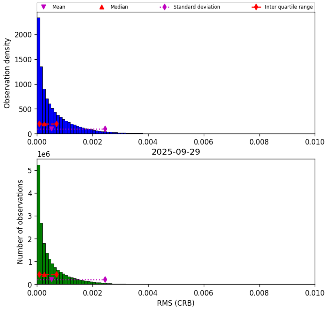
Figure 46: Histogram of “RMS (CRB)” for 2025-09-29 to 2025-09-29
