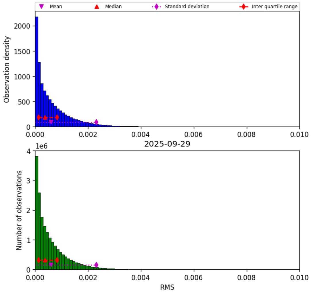
Figure 45: Histogram of “RMS” for 2025-09-29 to 2025-09-29
