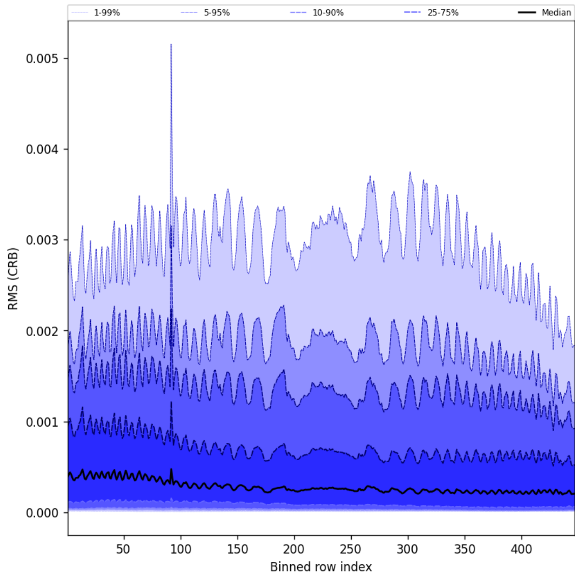
Figure 62: Along track statistics of “RMS (CRB)” for 2025-09-29 to 2025-09-29
