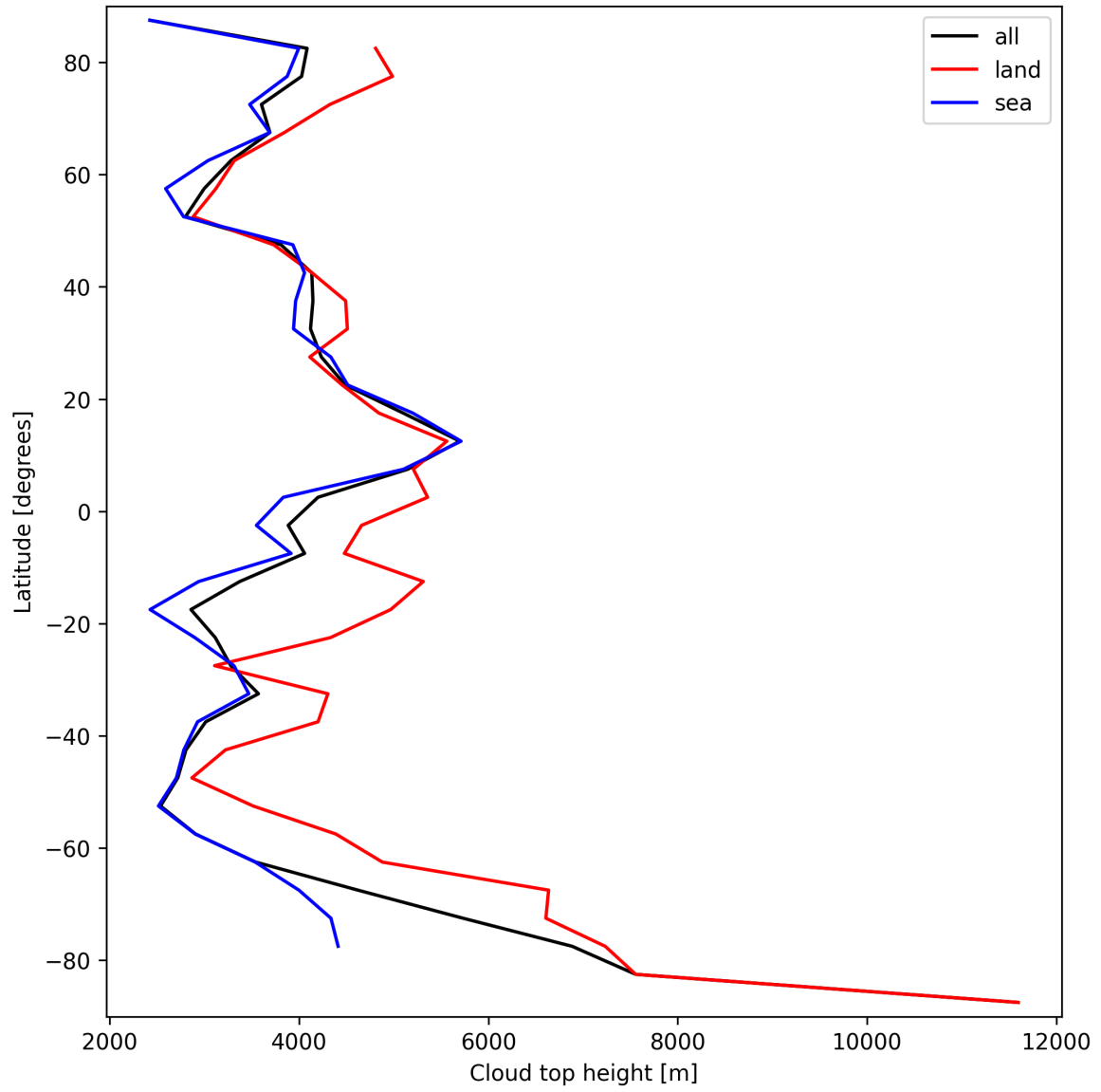
Figure 22: Zonal average of “Cloud top height” for 2025-09-29 to 2025-09-29.
