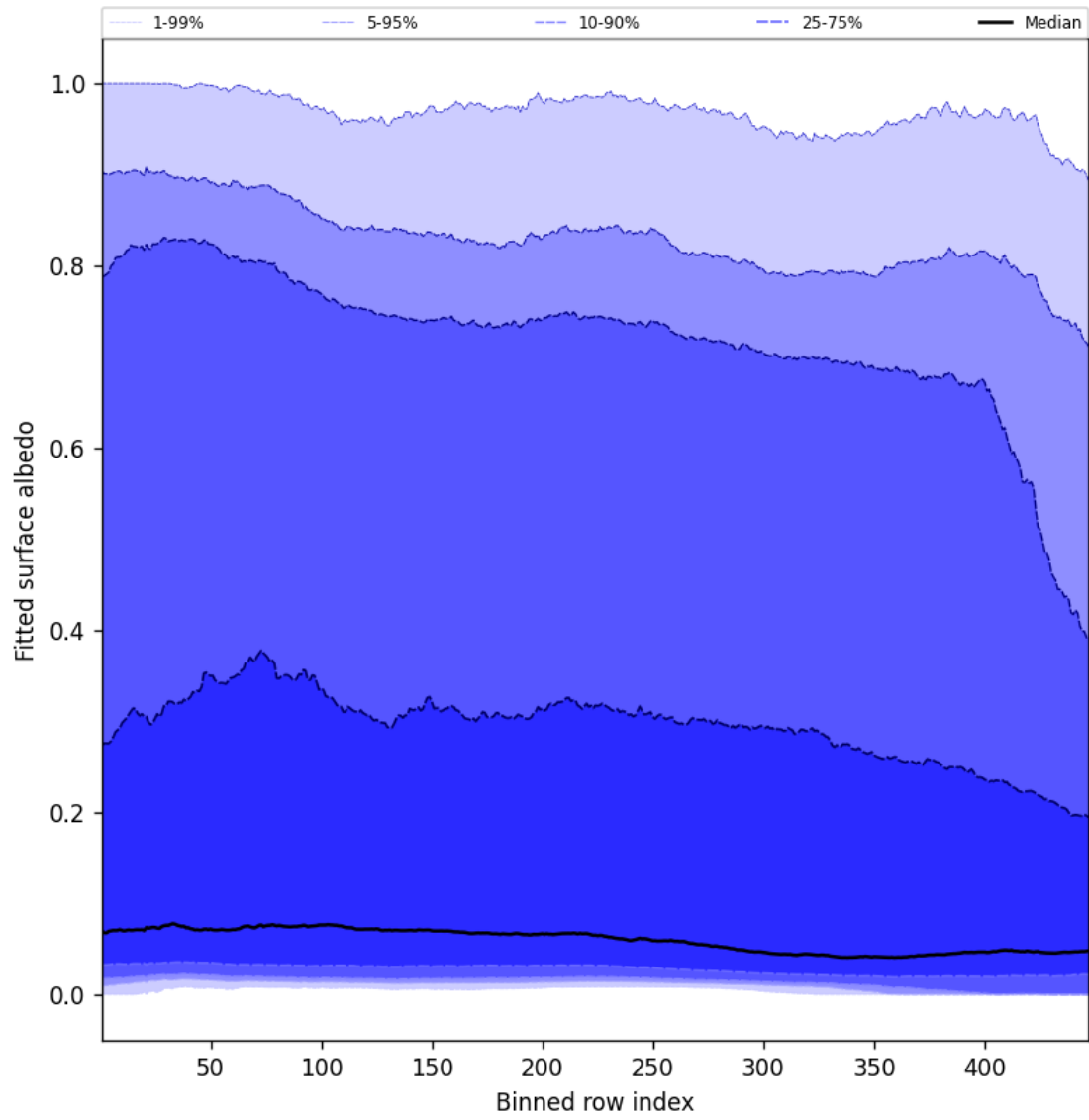
Figure 59: Along track statistics of “Fitted surface albedo” for 2025-09-29 to 2025-09-29
