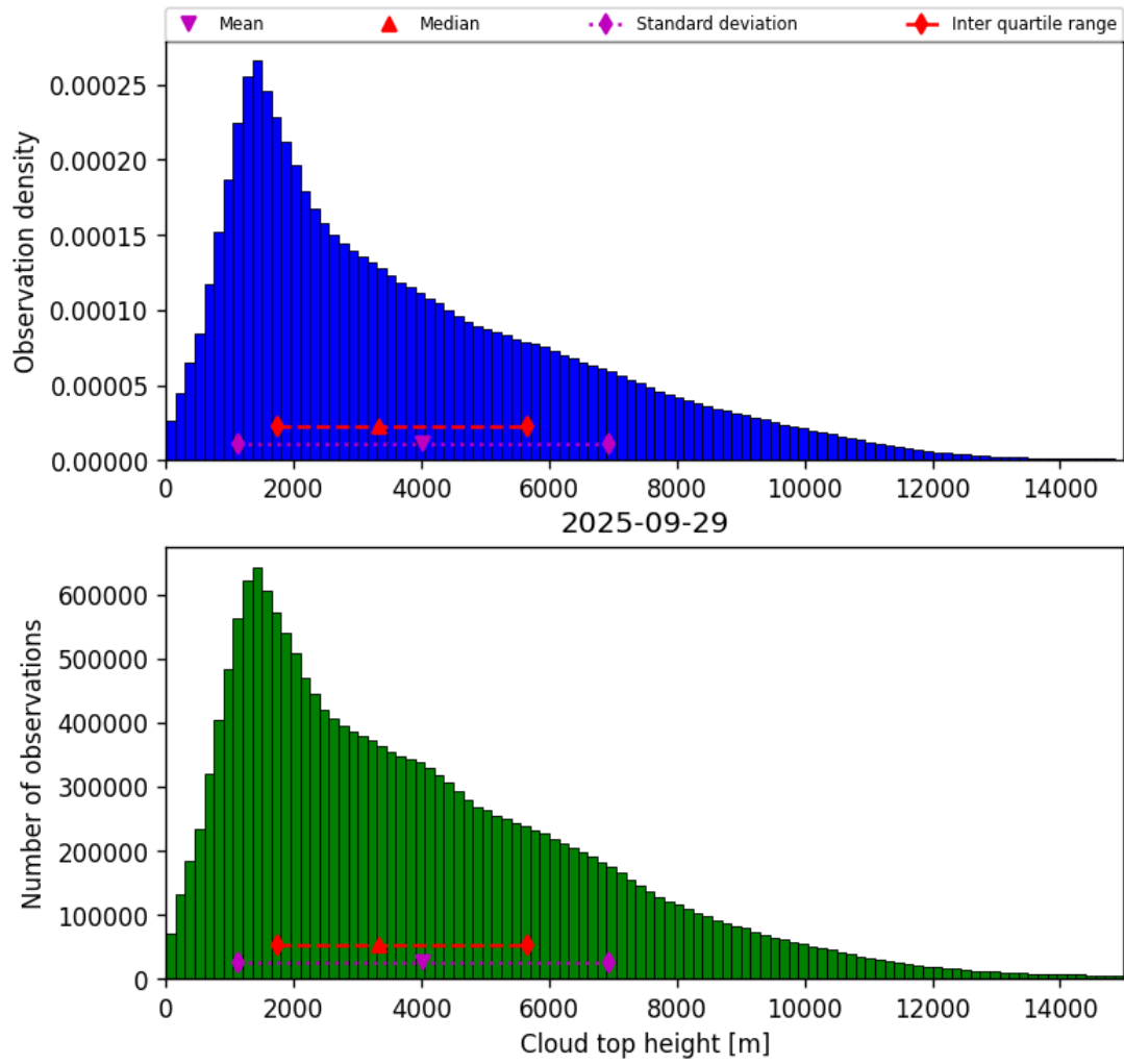
Figure 38: Histogram of “Cloud top height” for 2025-09-29 to 2025-09-29
