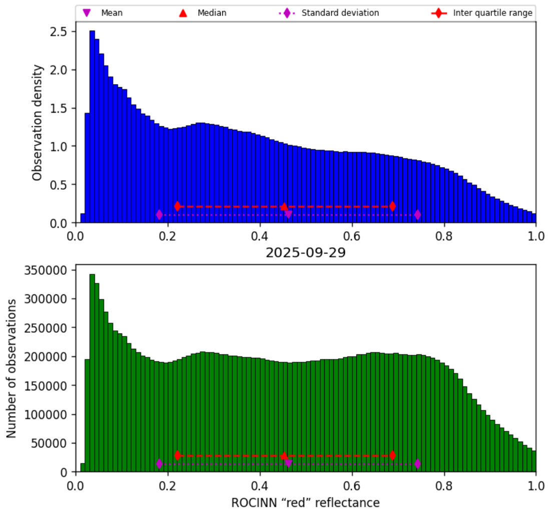
Figure 51: Histogram of “ROCINN “red” reflectance” for 2025-09-29 to 2025-09-29
