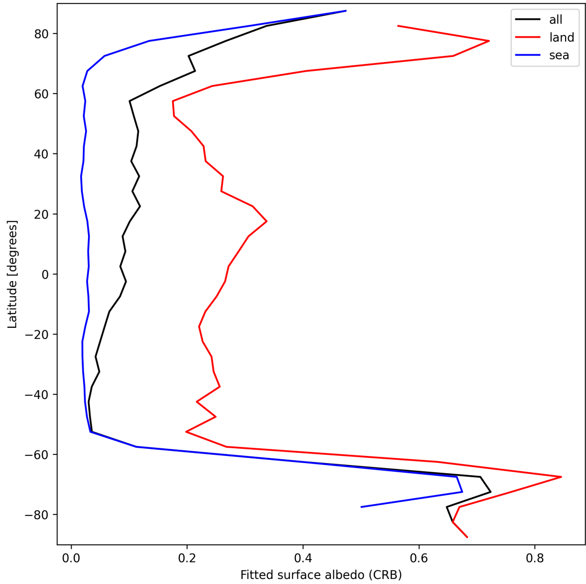
Figure 28: Zonal average of “Fitted surface albedo (CRB)” for 2025-09-29 to 2025-09-29.
