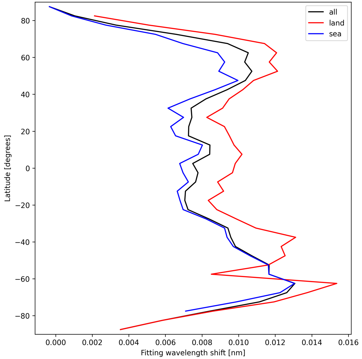
Figure 31: Zonal average of “Fitting wavelength shift” for 2025-09-29 to 2025-09-29.
