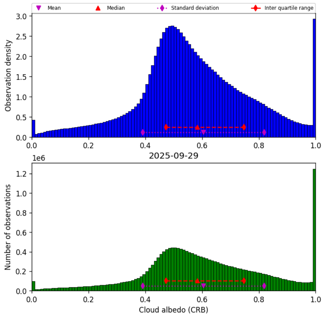
Figure 42: Histogram of “Cloud albedo (CRB)” for 2025-09-29 to 2025-09-29
