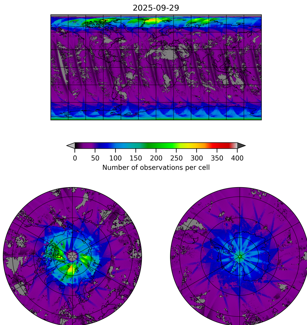
Figure 19: Map of the number of observations for 2025-09-29 to 2025-09-29
