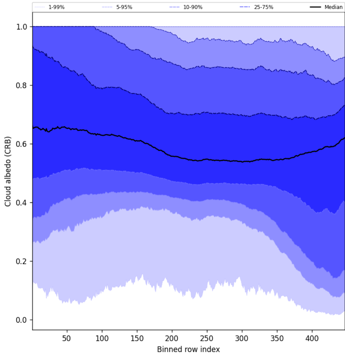
Figure 58: Along track statistics of “Cloud albedo (CRB)” for 2025-09-29 to 2025-09-29
