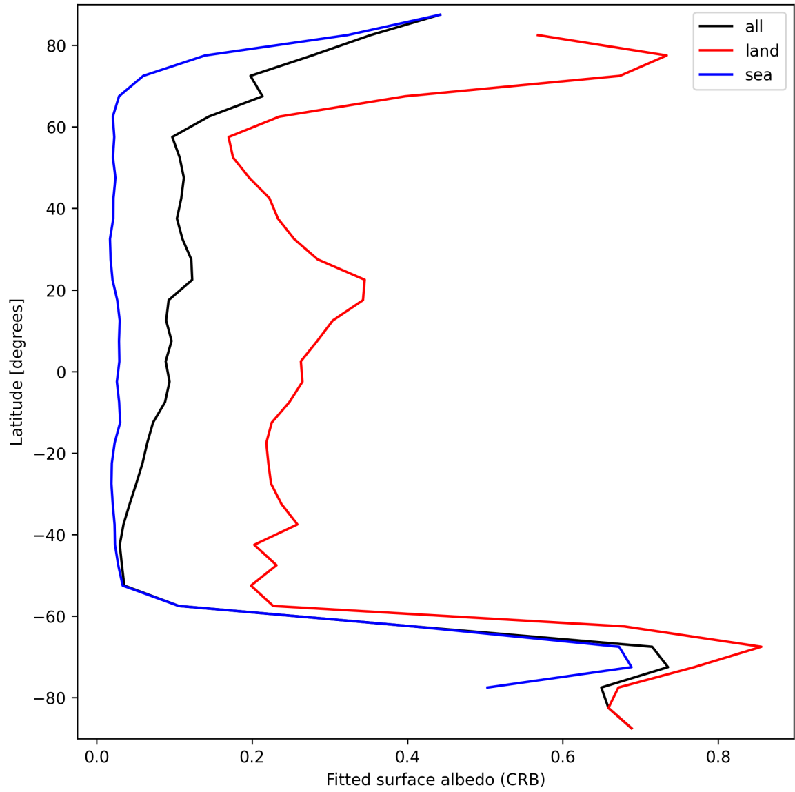
Figure 28: Zonal average of “Fitted surface albedo (CRB)” for 2025-10-01 to 2025-10-02.
