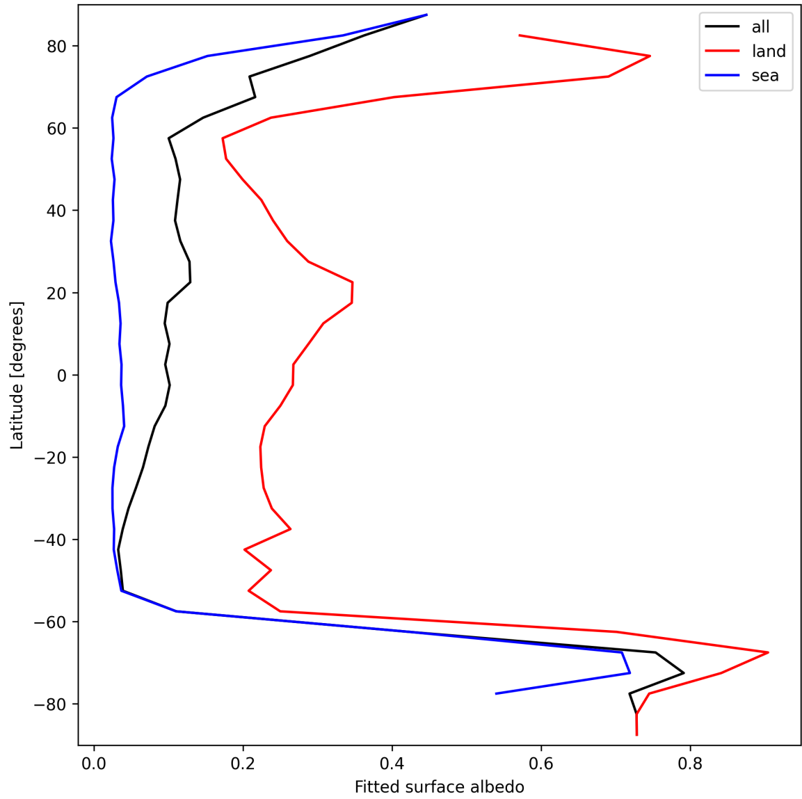
Figure 27: Zonal average of “Fitted surface albedo” for 2025-10-01 to 2025-10-02.
