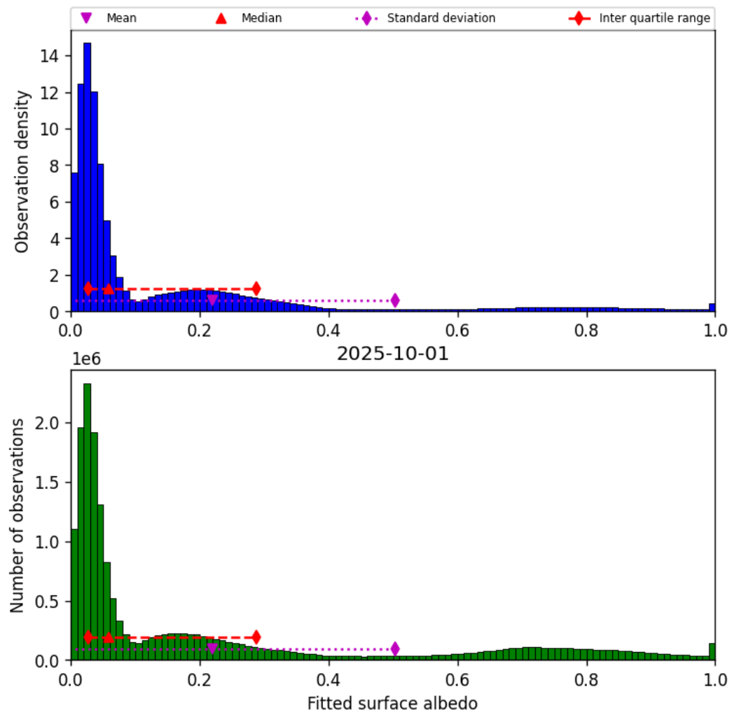
Figure 43: Histogram of “Fitted surface albedo” for 2025-10-01 to 2025-10-02
