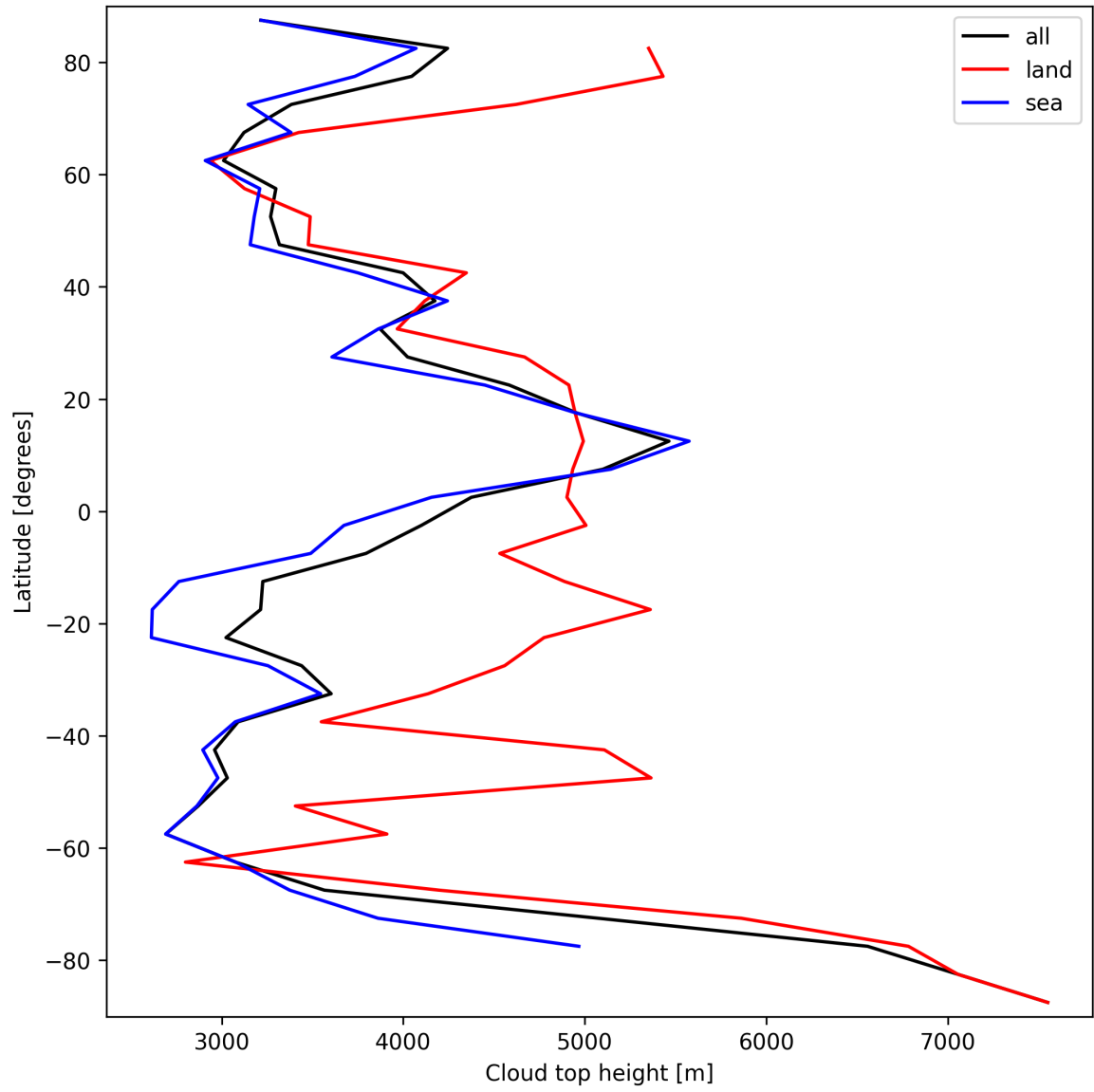
Figure 22: Zonal average of “Cloud top height” for 2025-10-01 to 2025-10-02.
