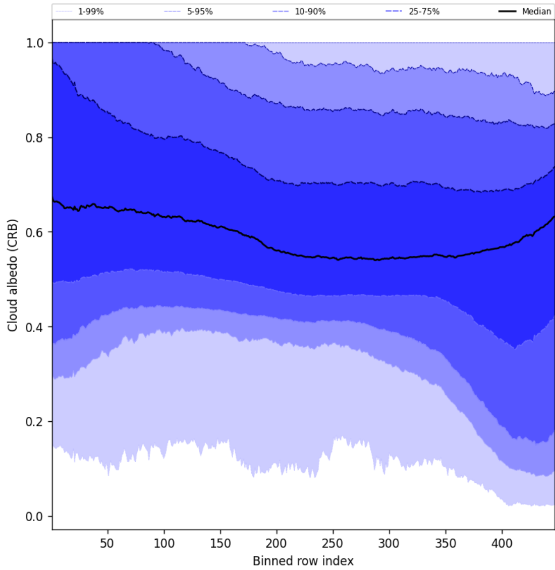
Figure 58: Along track statistics of “Cloud albedo (CRB)” for 2025-10-01 to 2025-10-02
