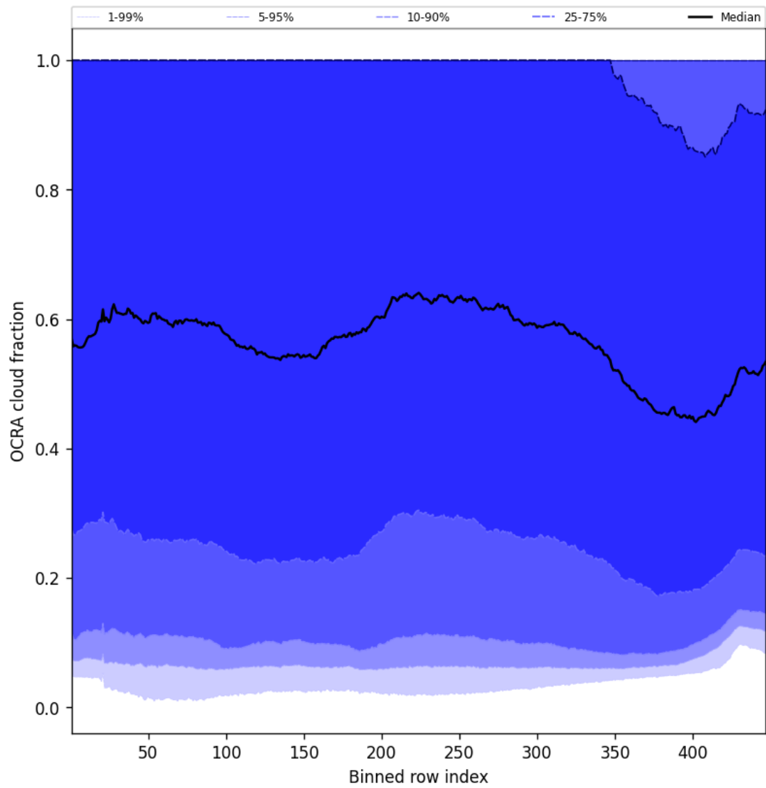
Figure 64: Along track statistics of “OCRA cloud fraction” for 2025-10-01 to 2025-10-02
