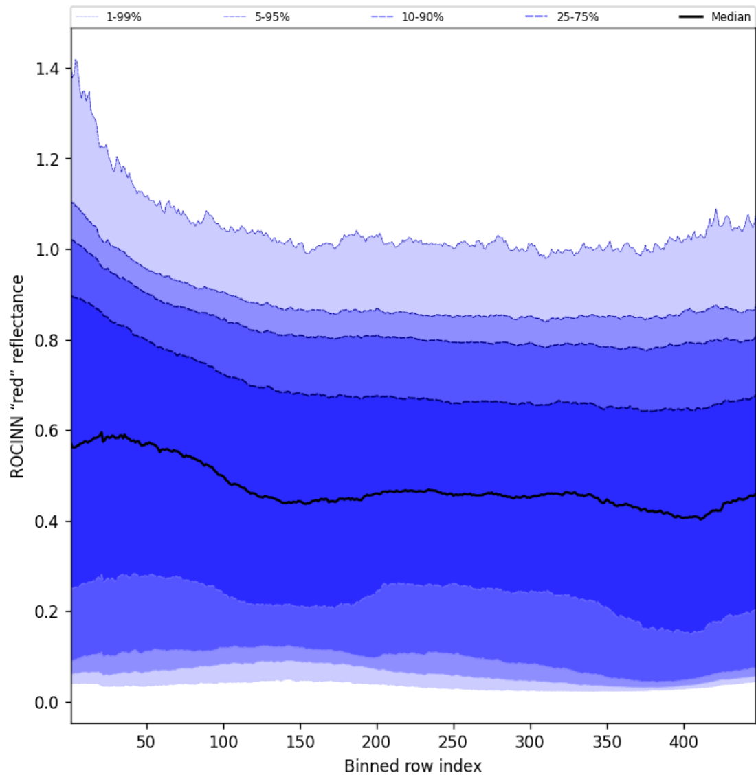
Figure 67: Along track statistics of "ROCINN "red" reflectance" for 2025-10-01 to 2025-10-02
