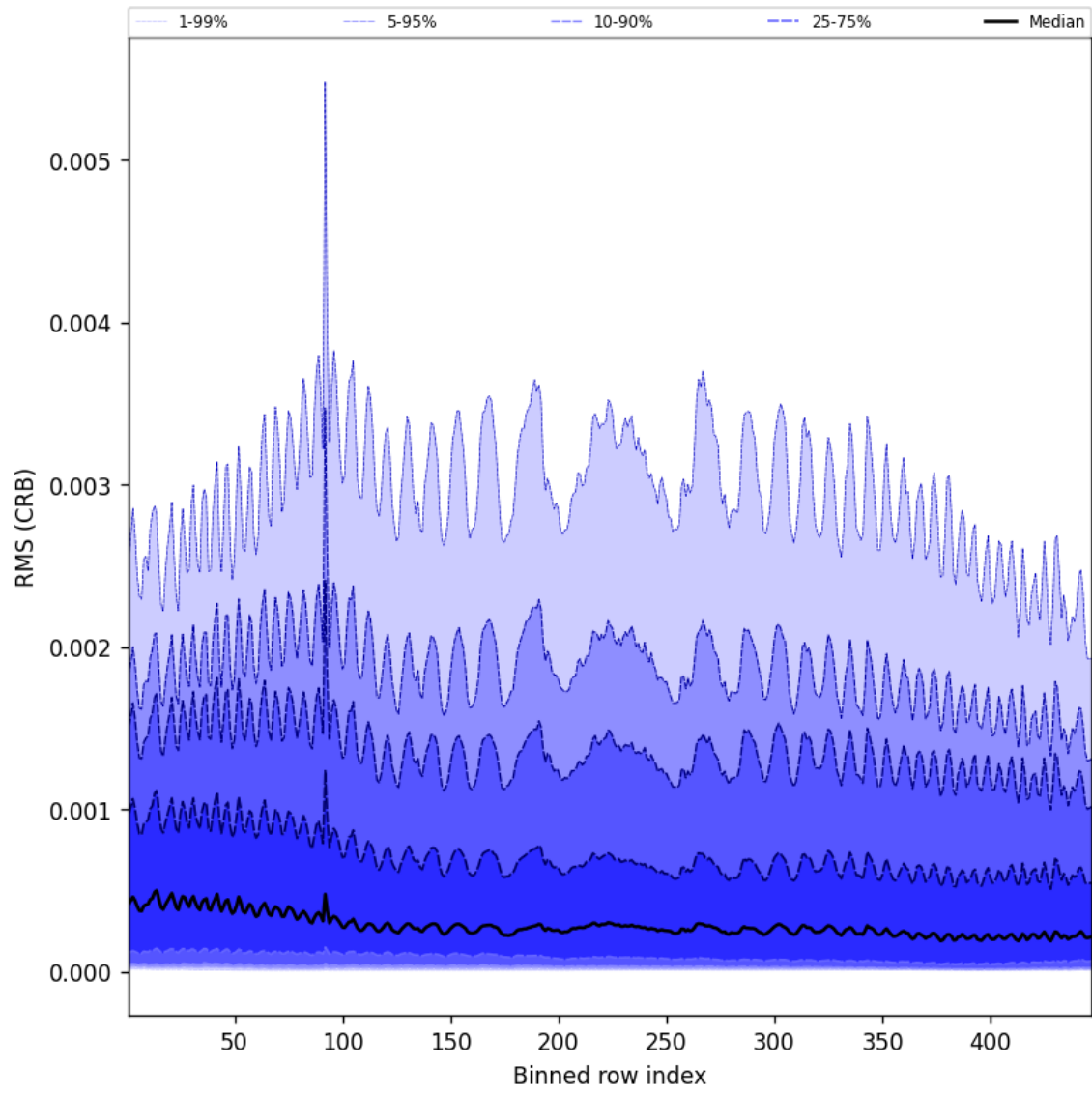
Figure 62: Along track statistics of “RMS (CRB)” for 2025-10-01 to 2025-10-02
