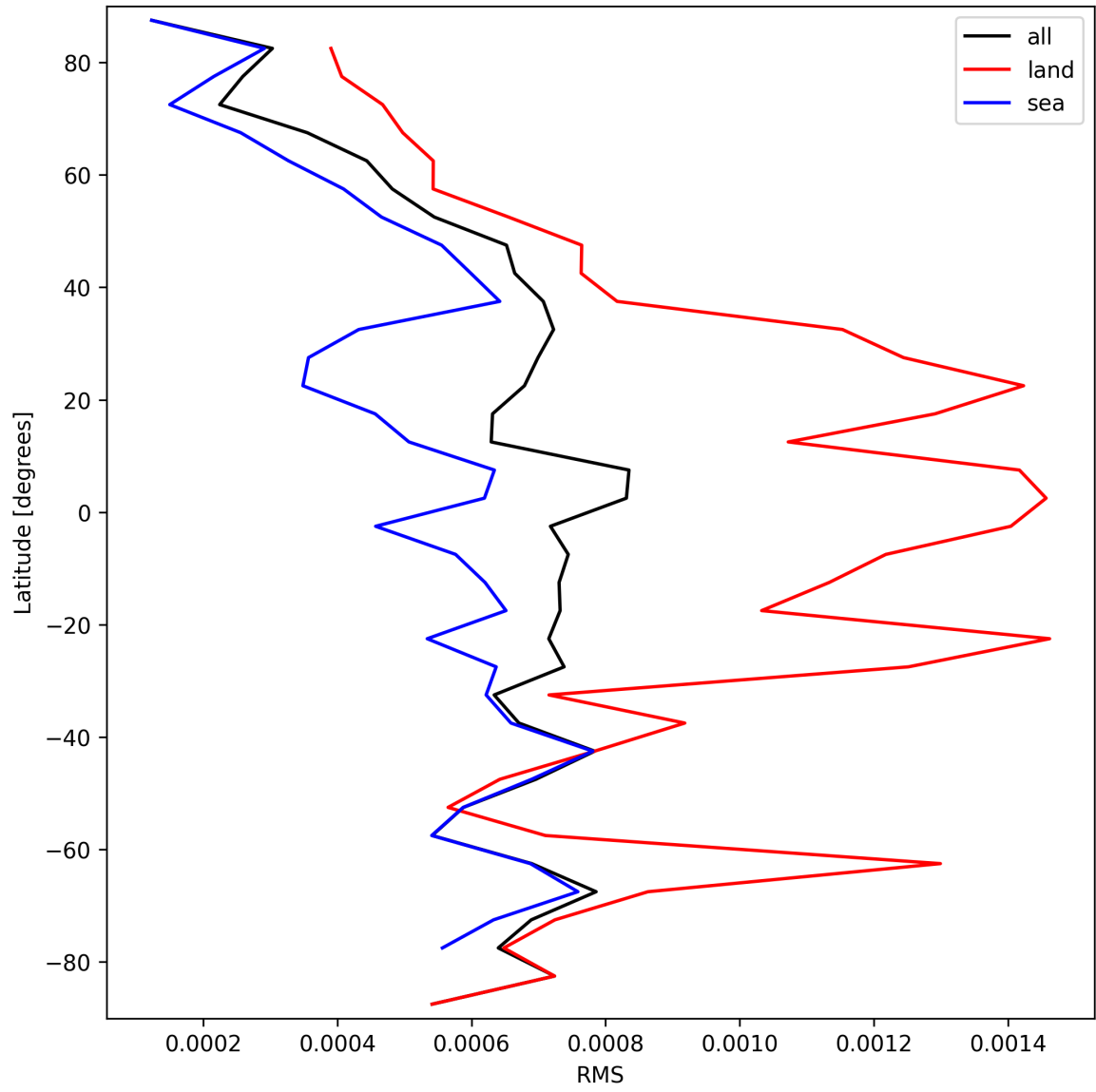
Figure 29: Zonal average of “RMS” for 2025-10-01 to 2025-10-02.
