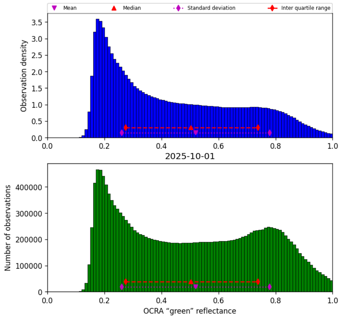
Figure 50: Histogram of “OCRA “green” reflectance” for 2025-10-01 to 2025-10-02
