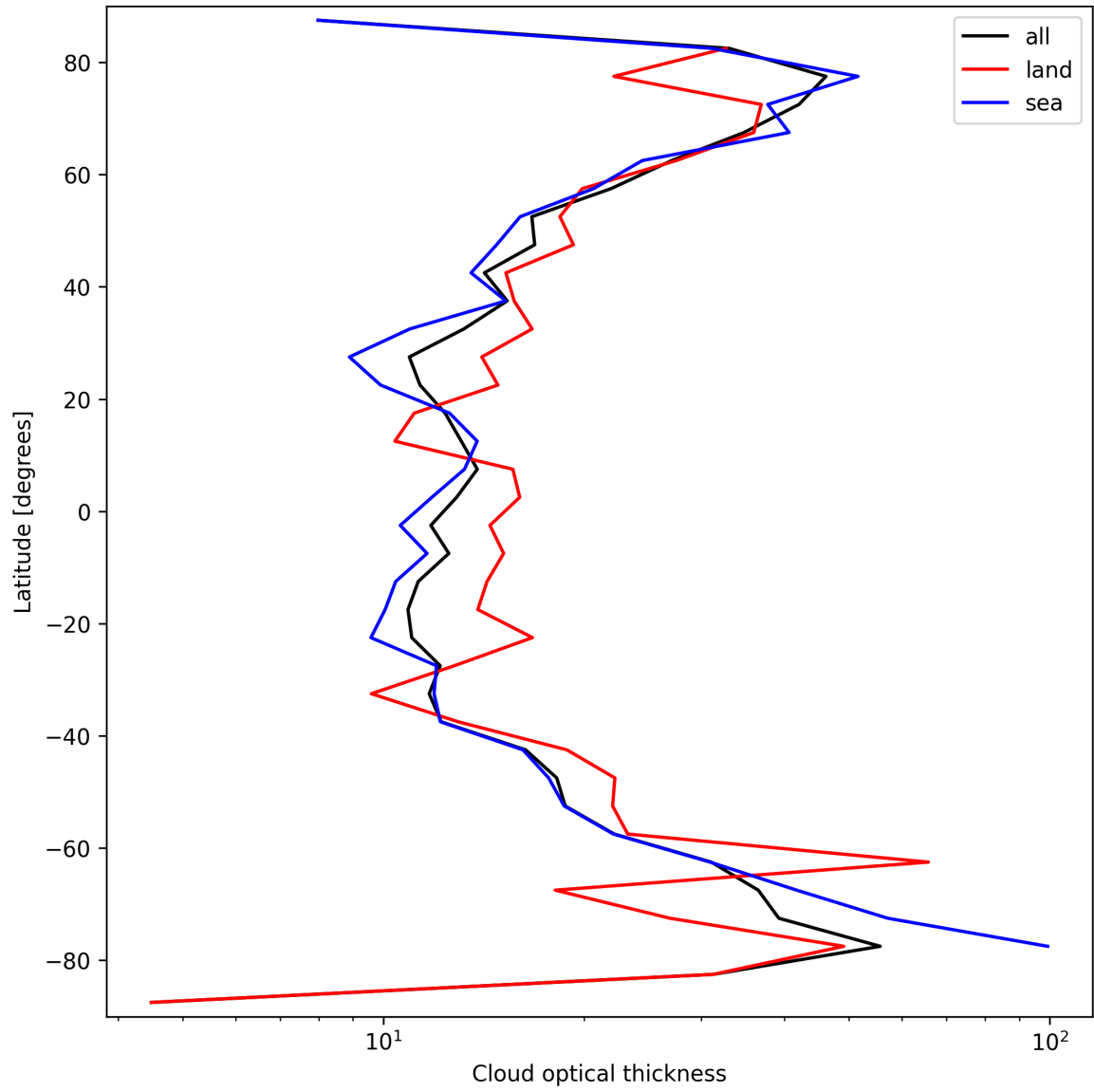
Figure 23: Zonal average of “Cloud optical thickness” for 2025-10-01 to 2025-10-02.
