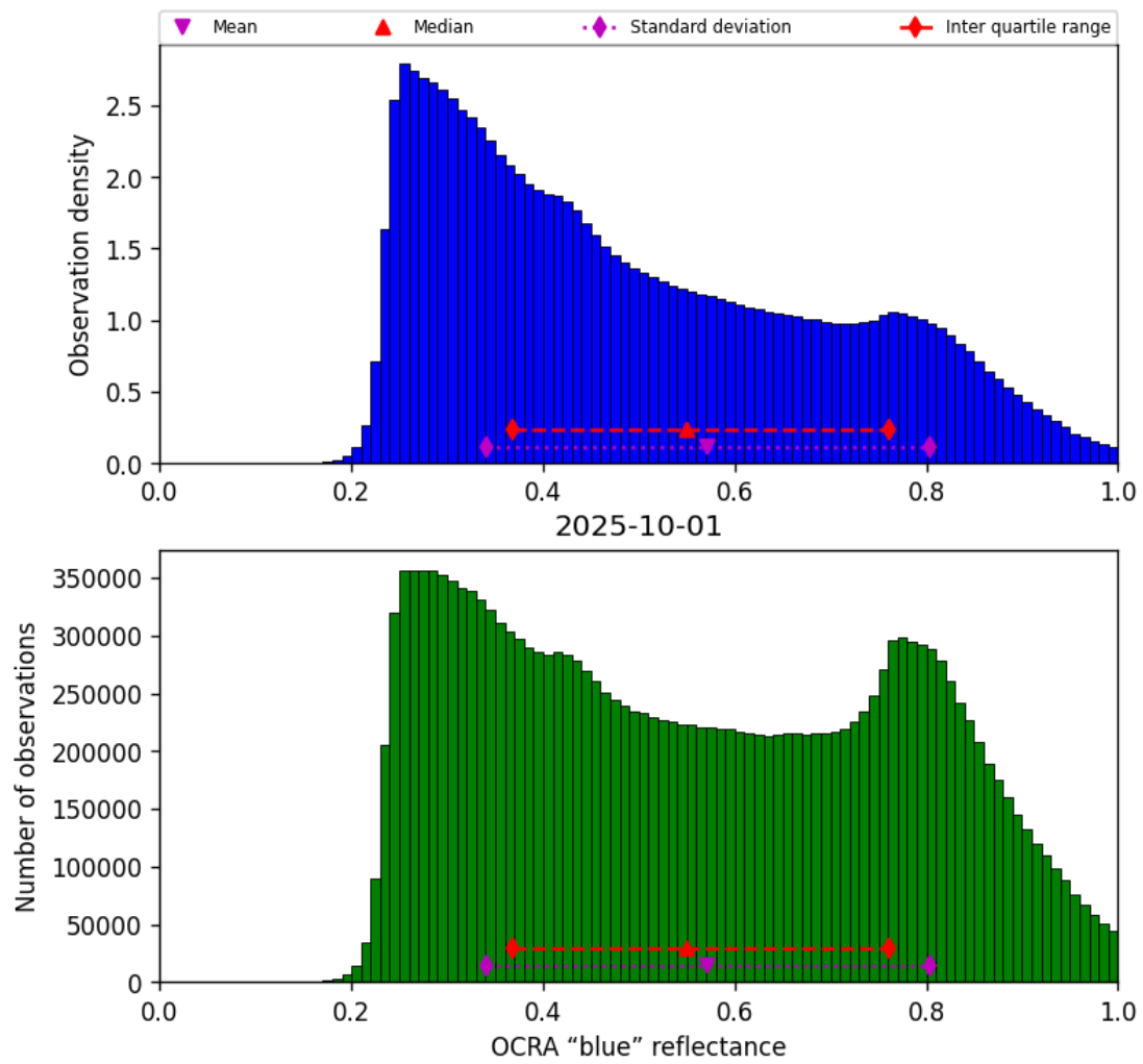
Figure 49: Histogram of “OCRA “blue” reflectance” for 2025-10-01 to 2025-10-02
