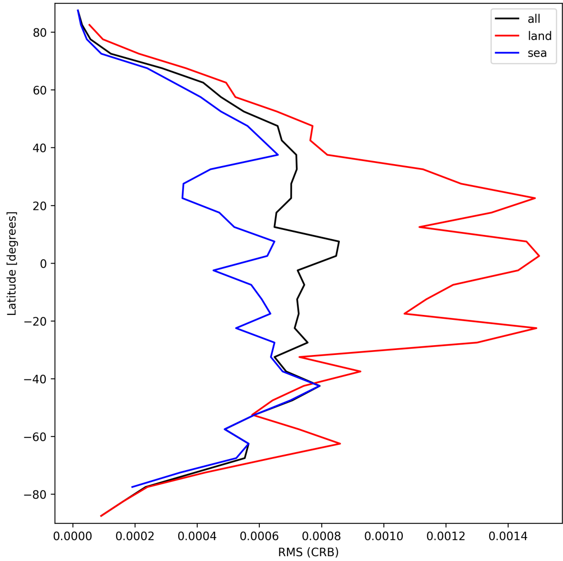
Figure 30: Zonal average of "RMS (CRB)" for 2025-10-01 to 2025-10-02.
