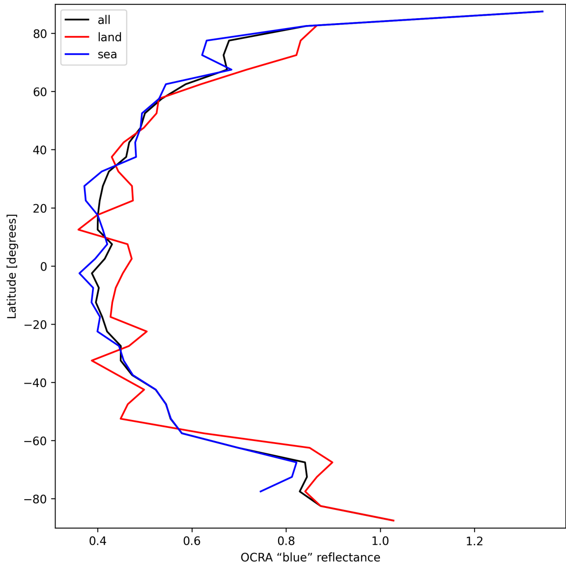
Figure 33: Zonal average of “OCRA “blue” reflectance” for 2025-10-01 to 2025-10-02.
