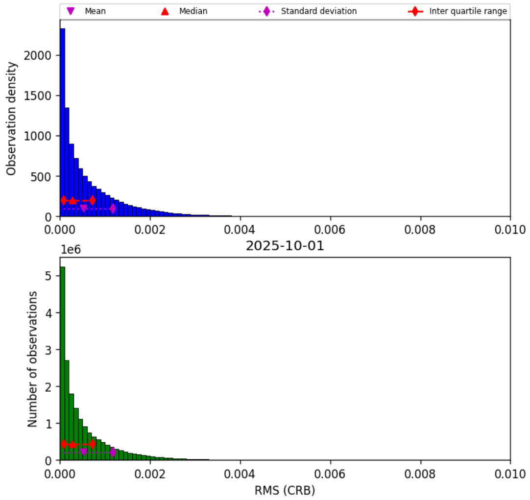
Figure 46: Histogram of “RMS (CRB)” for 2025-10-01 to 2025-10-02
