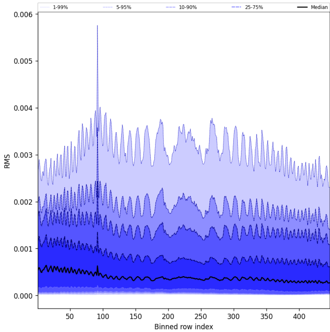
Figure 61: Along track statistics of “RMS” for 2025-10-01 to 2025-10-02
