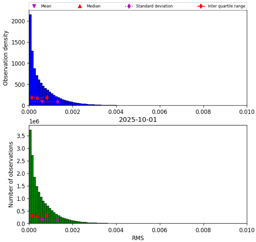
Figure 45: Histogram of “RMS” for 2025-10-01 to 2025-10-02
