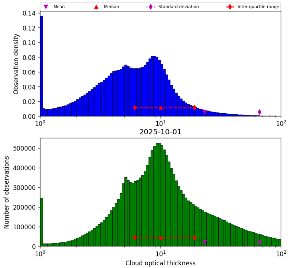
Figure 39: Histogram of “Cloud optical thickness” for 2025-10-01 to 2025-10-02
