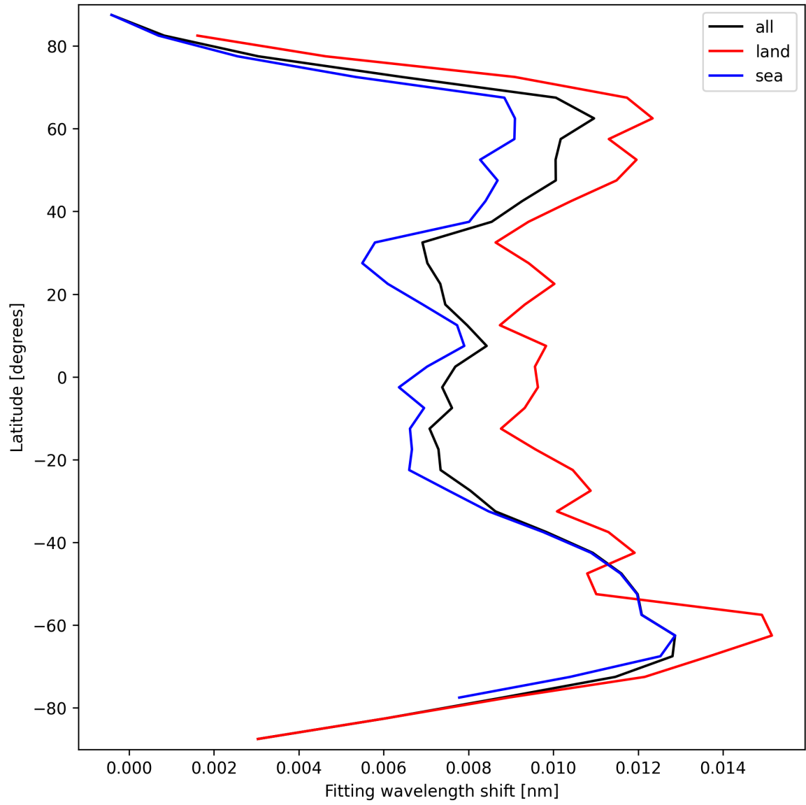
Figure 31: Zonal average of “Fitting wavelength shift” for 2025-10-01 to 2025-10-02.
