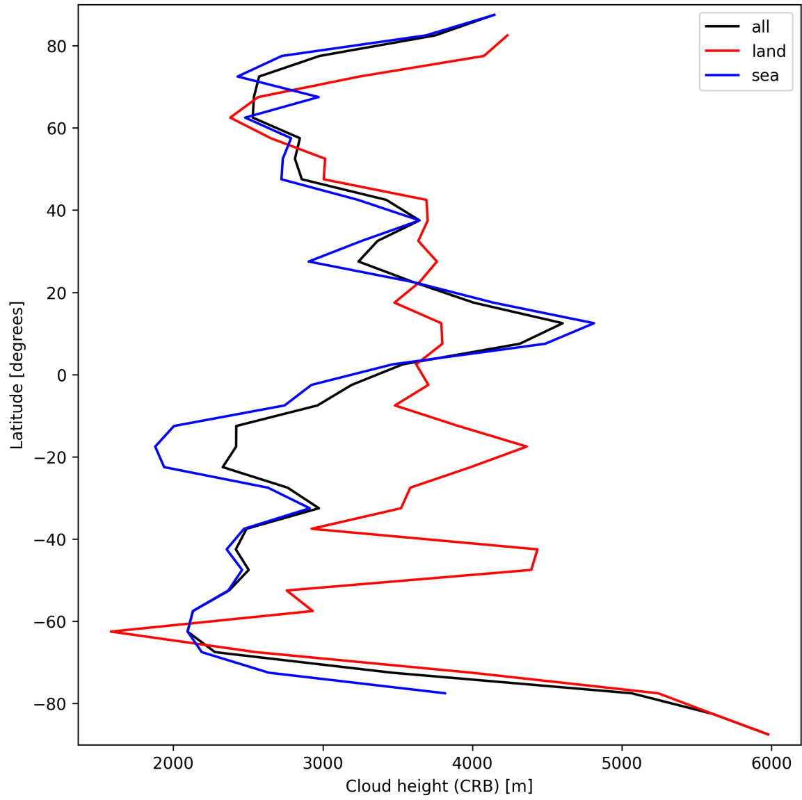
Figure 25: Zonal average of “Cloud height (CRB)” for 2025-10-01 to 2025-10-02.
