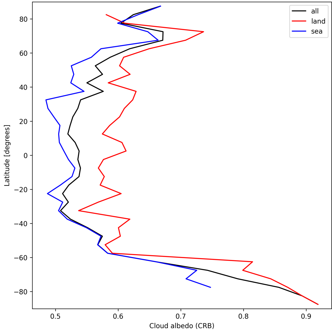
Figure 26: Zonal average of “Cloud albedo (CRB)” for 2025-10-01 to 2025-10-02.
