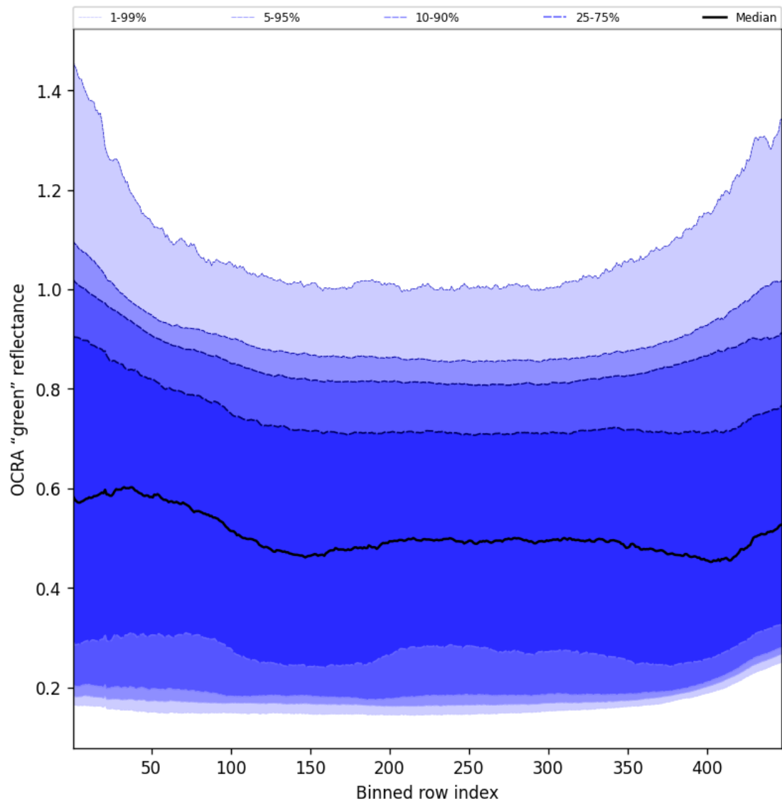
Figure 66: Along track statistics of “OCRA “green” reflectance” for 2025-10-01 to 2025-10-02
