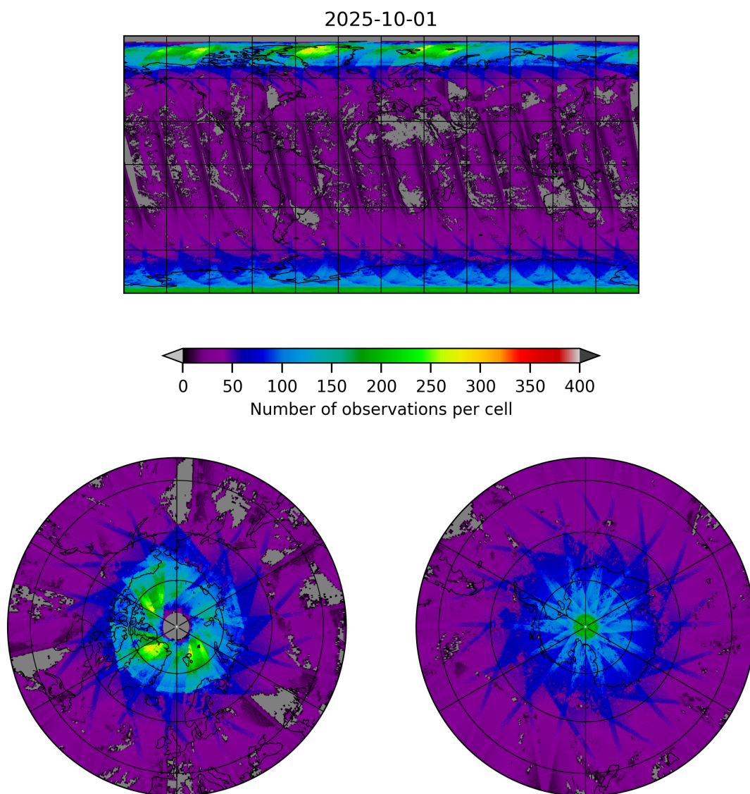
Figure 19: Map of the number of observations for 2025-10-01 to 2025-10-02
