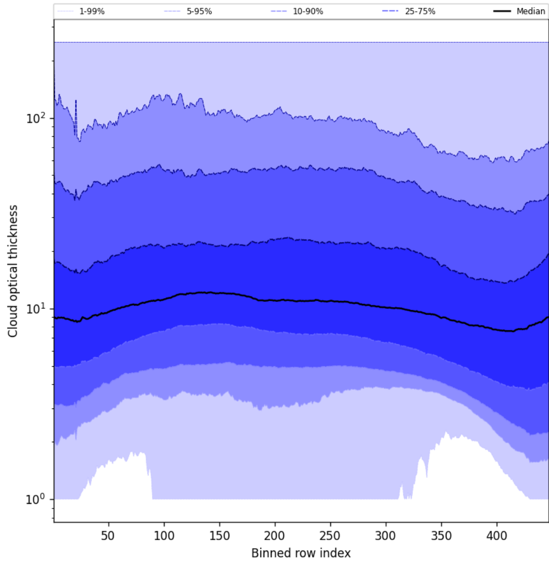
Figure 55: Along track statistics of “Cloud optical thickness” for 2025-10-01 to 2025-10-02
