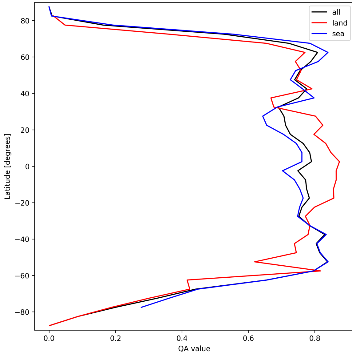
Figure 20: Zonal average of “QA value” for 2025-10-01 to 2025-10-02.
