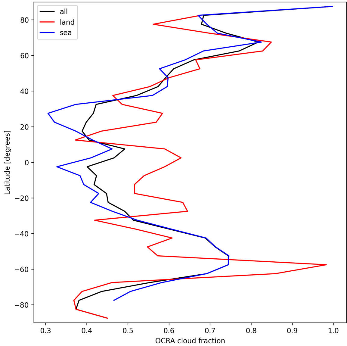
Figure 32: Zonal average of “OCRA cloud fraction” for 2025-10-01 to 2025-10-02.
