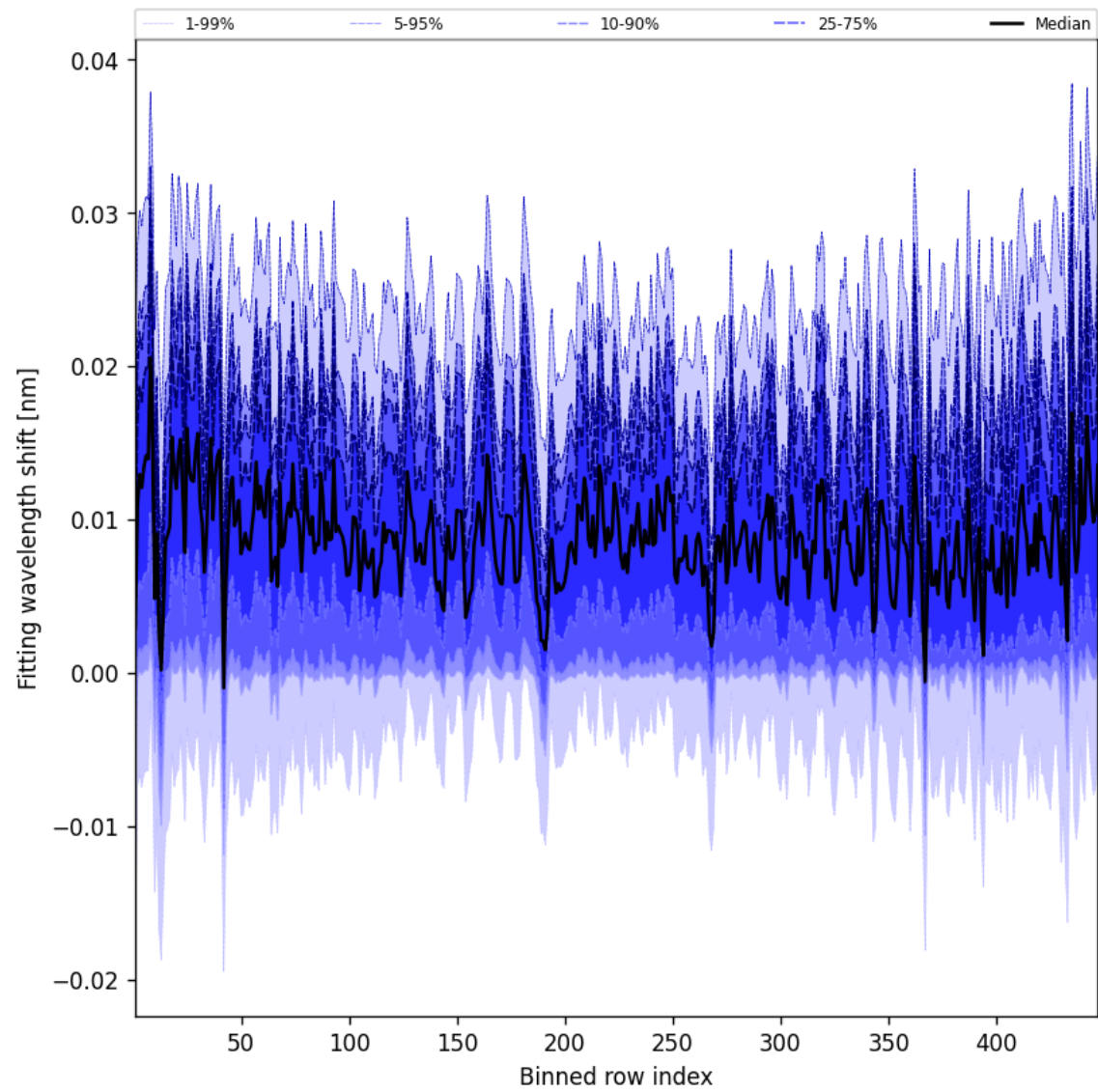
Figure 63: Along track statistics of “Fitting wavelength shift” for 2025-10-01 to 2025-10-02
