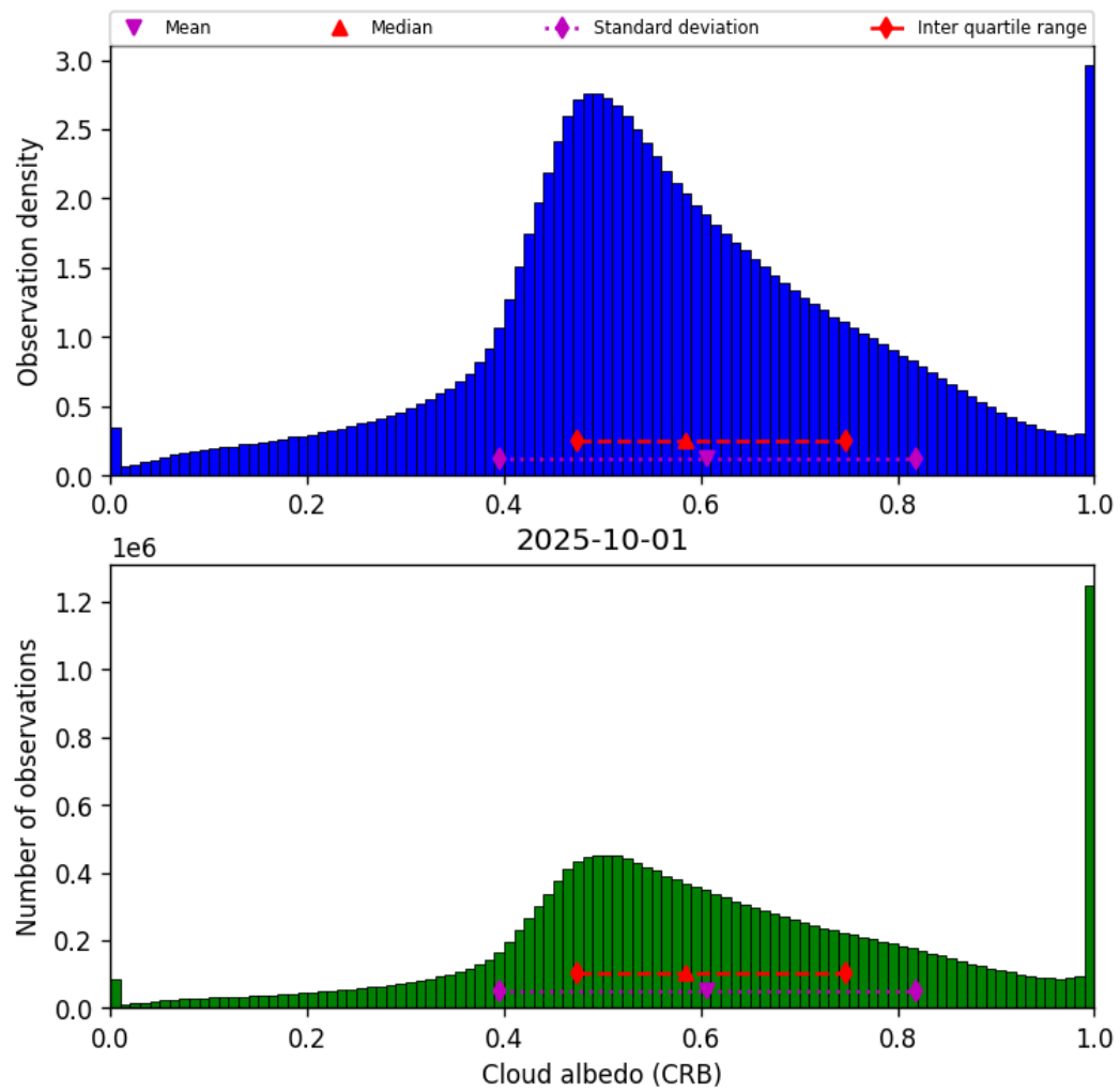
Figure 42: Histogram of “Cloud albedo (CRB)” for 2025-10-01 to 2025-10-02
