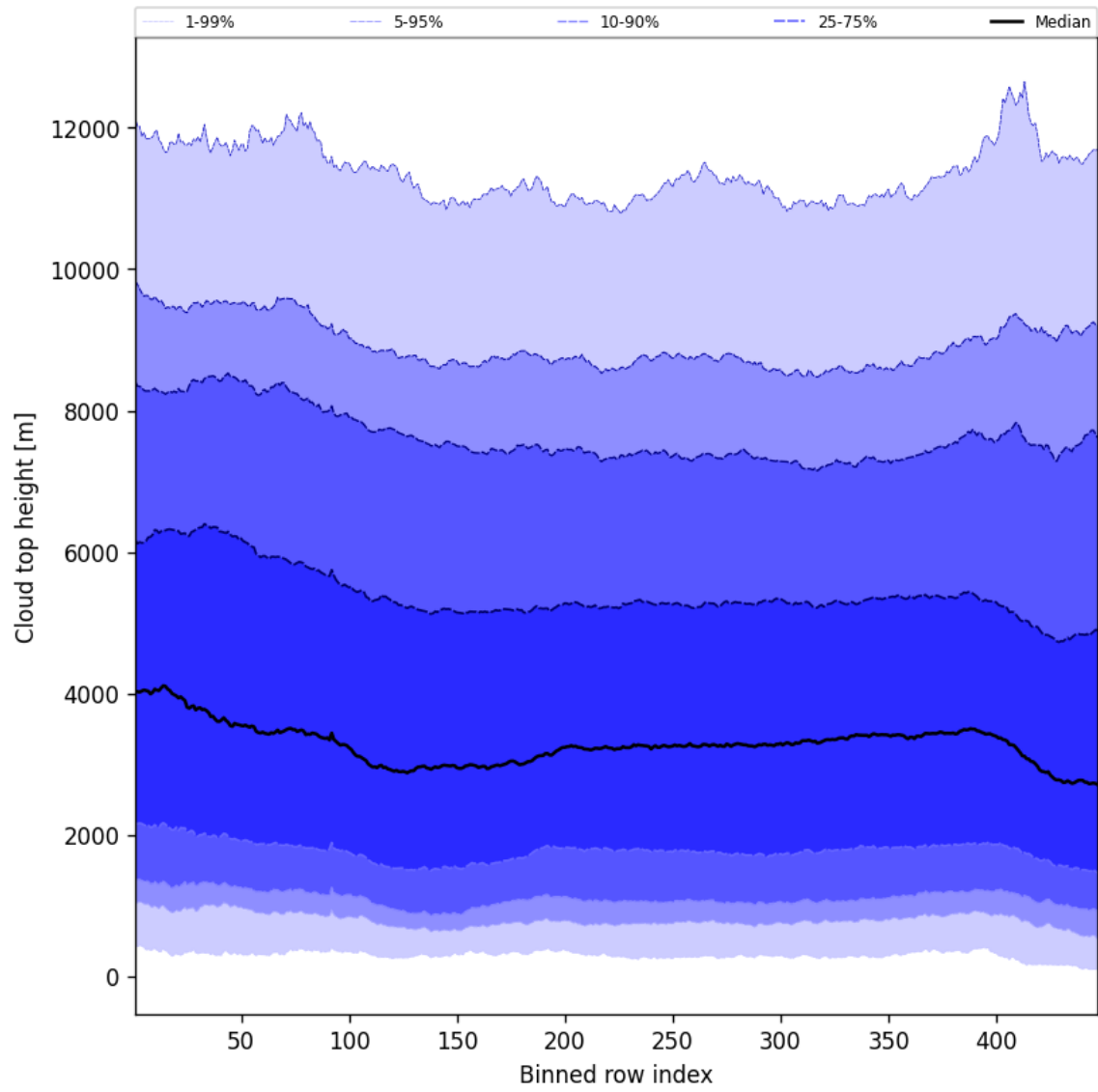
Figure 54: Along track statistics of “Cloud top height” for 2025-10-01 to 2025-10-02
