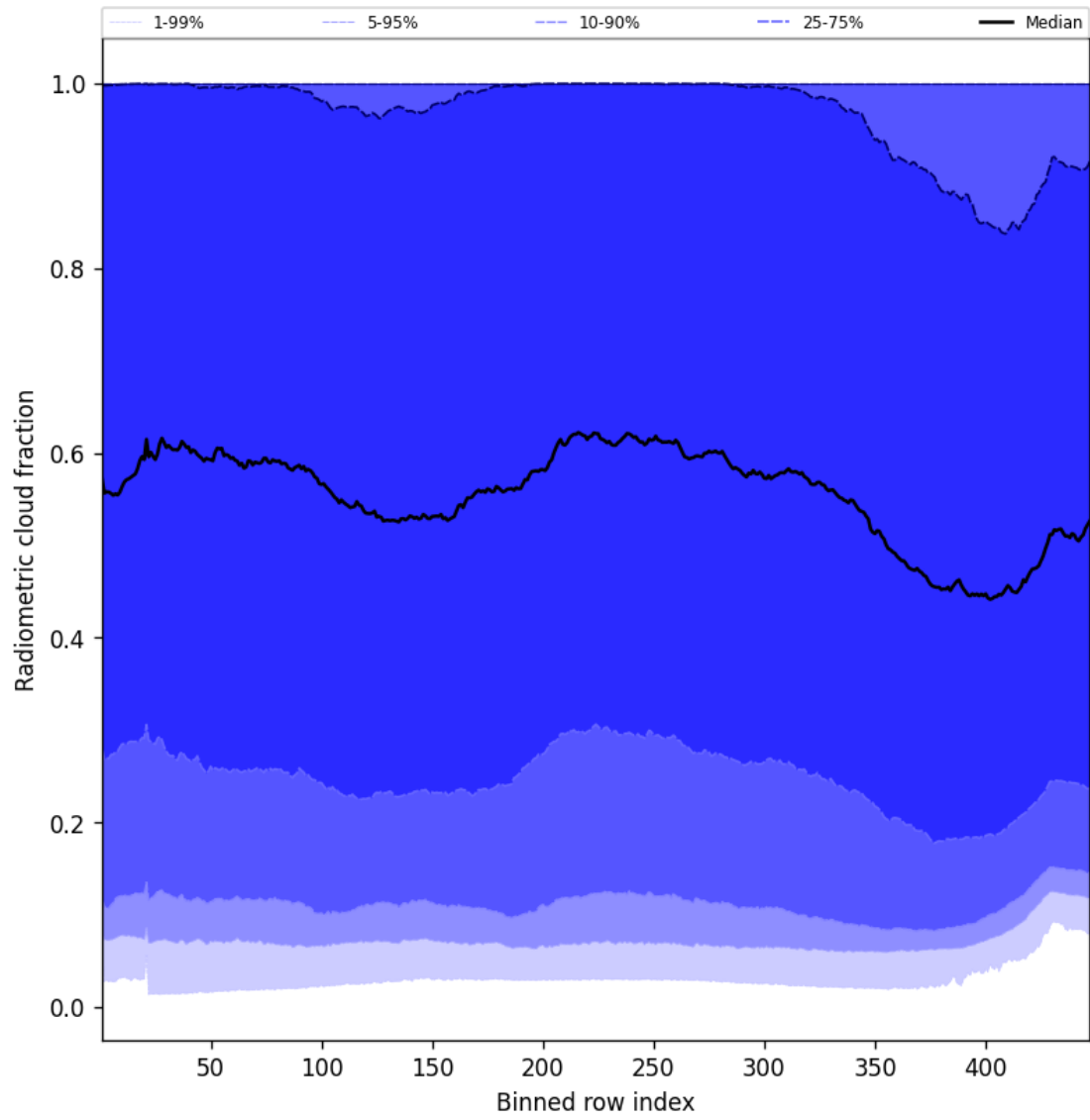
Figure 53: Along track statistics of “Radiometric cloud fraction” for 2025-10-01 to 2025-10-02
