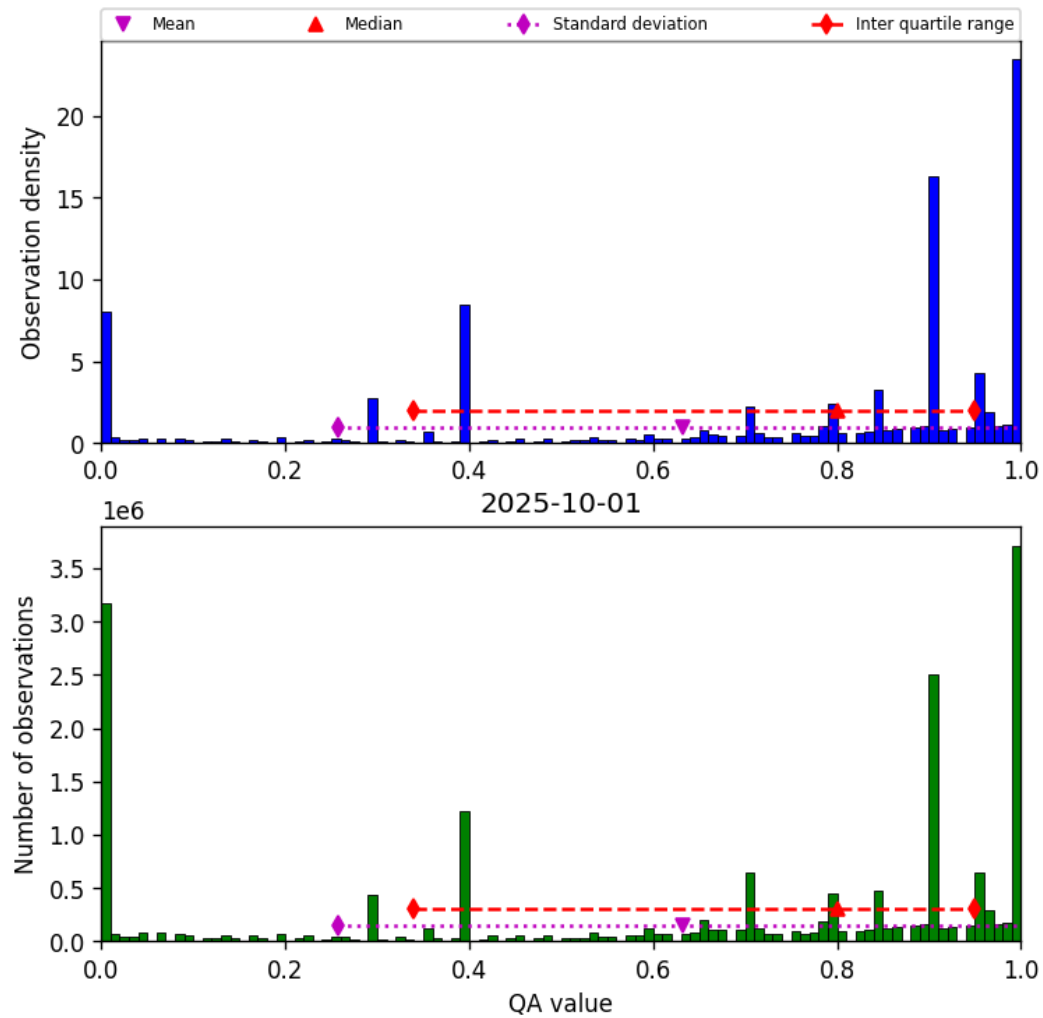
Figure 36: Histogram of “QA value” for 2025-10-01 to 2025-10-02
