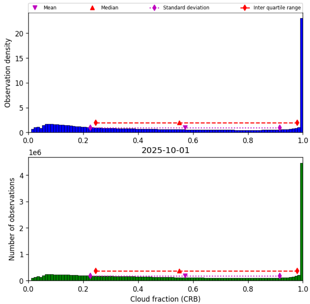
Figure 40: Histogram of “Cloud fraction (CRB)” for 2025-10-01 to 2025-10-02
