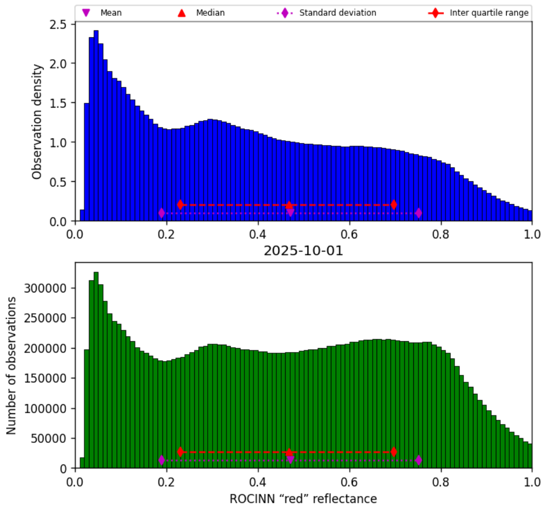
Figure 51: Histogram of “ROCINN “red” reflectance” for 2025-10-01 to 2025-10-02
