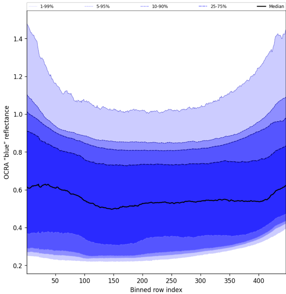
Figure 65: Along track statistics of “OCRA “blue” reflectance” for 2025-10-01 to 2025-10-02
