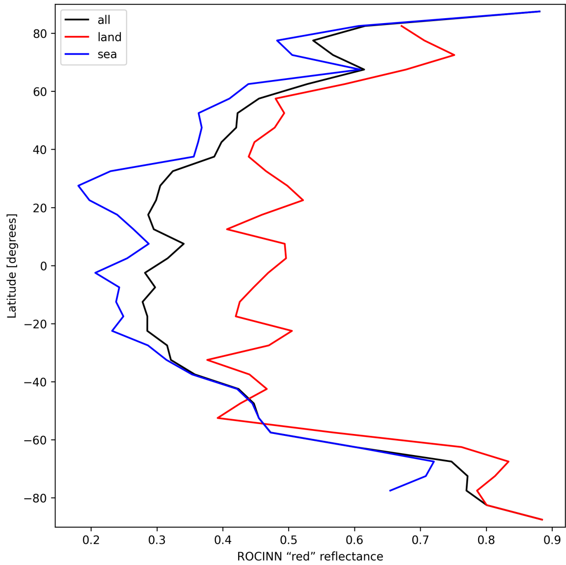
Figure 35: Zonal average of “ROCINN “red” reflectance” for 2025-10-01 to 2025-10-02.
