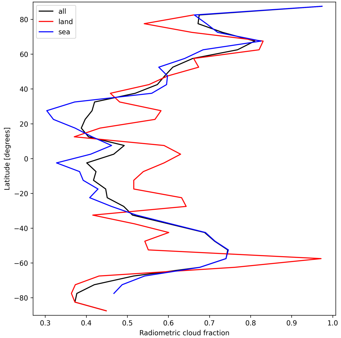
Figure 21: Zonal average of “Radiometric cloud fraction” for 2025-10-01 to 2025-10-02.
