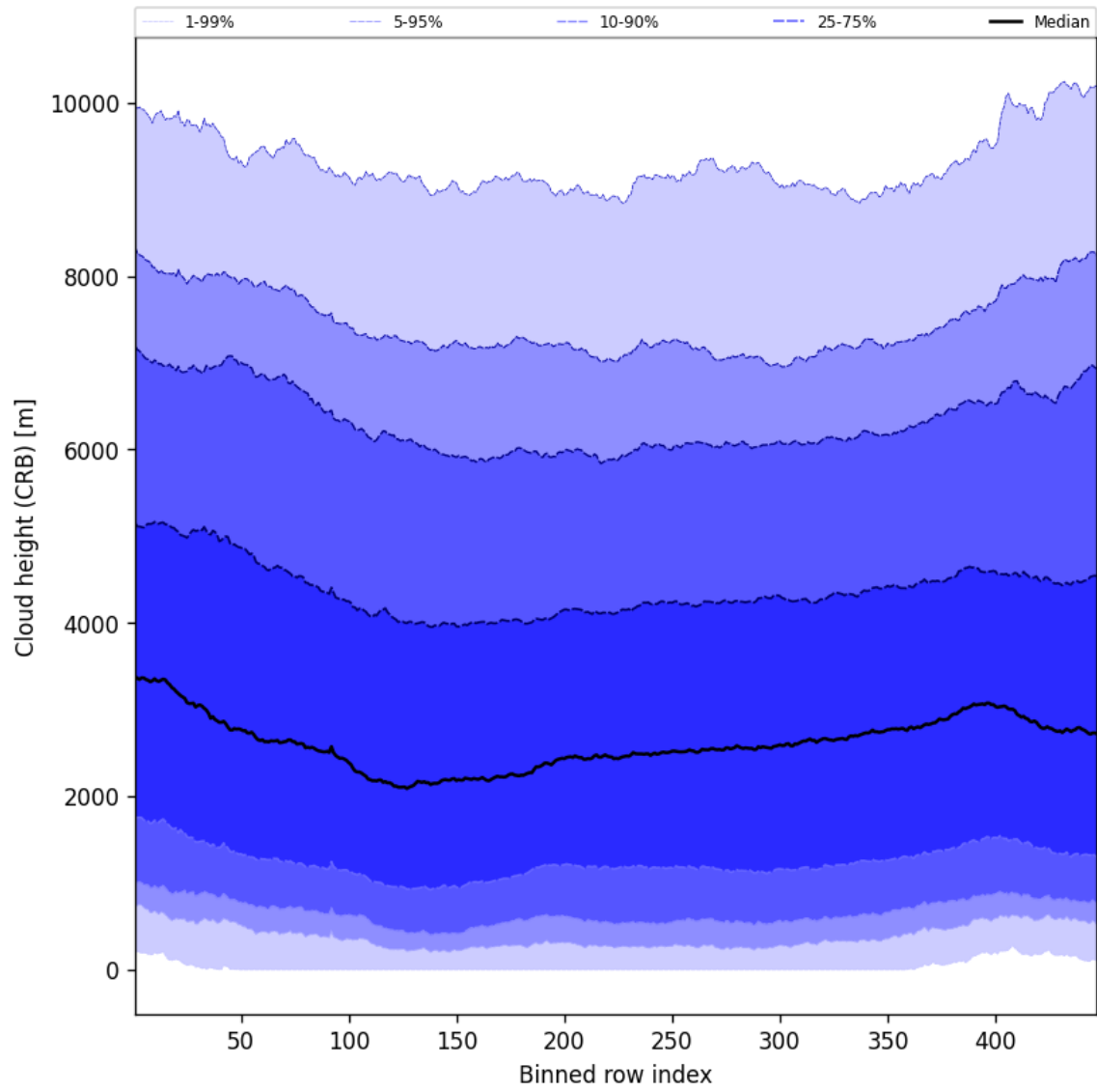
Figure 57: Along track statistics of “Cloud height (CRB)” for 2025-10-01 to 2025-10-02
