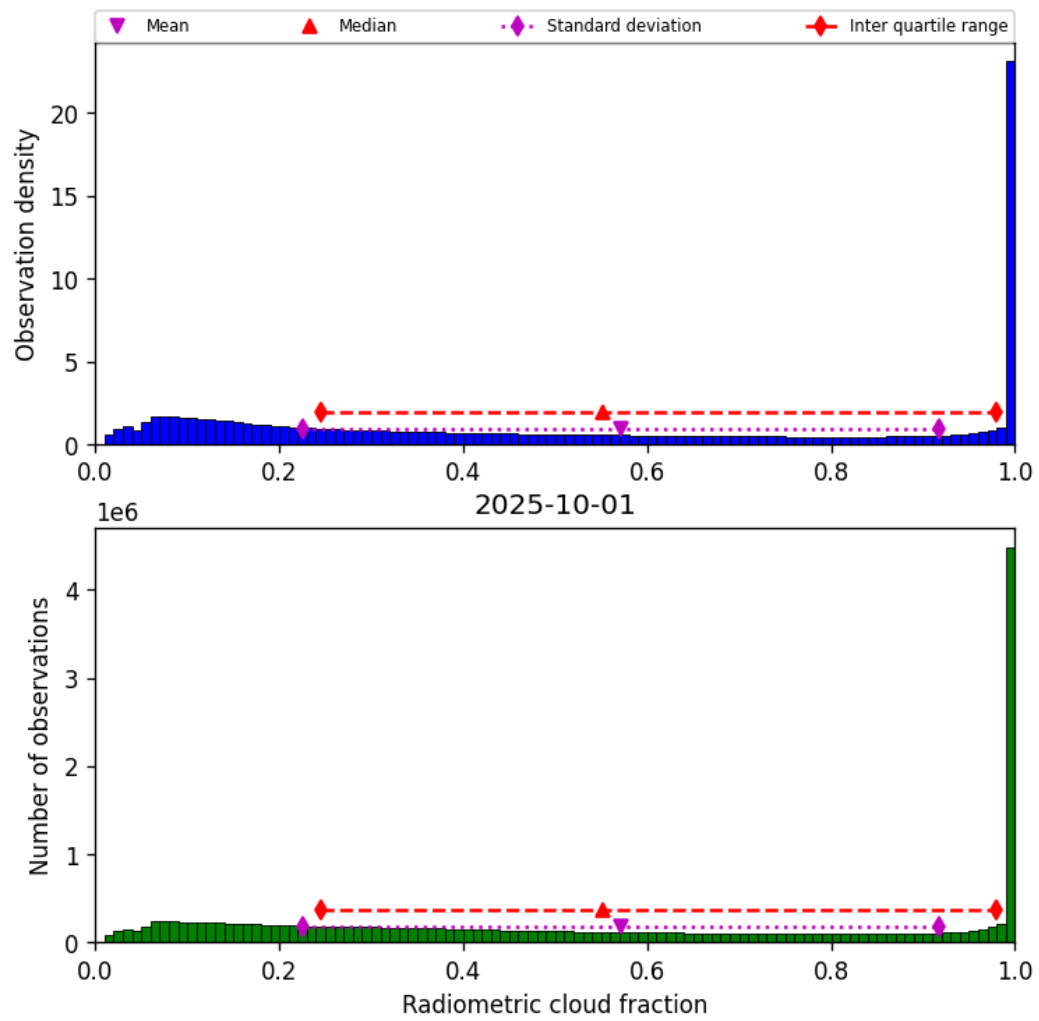
Figure 37: Histogram of “Radiometric cloud fraction” for 2025-10-01 to 2025-10-02
