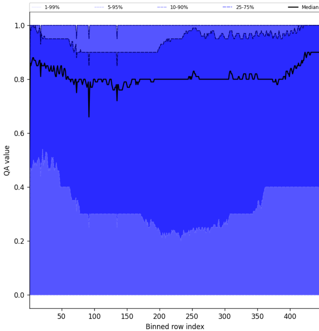
Figure 52: Along track statistics of “QA value” for 2025-10-01 to 2025-10-02
