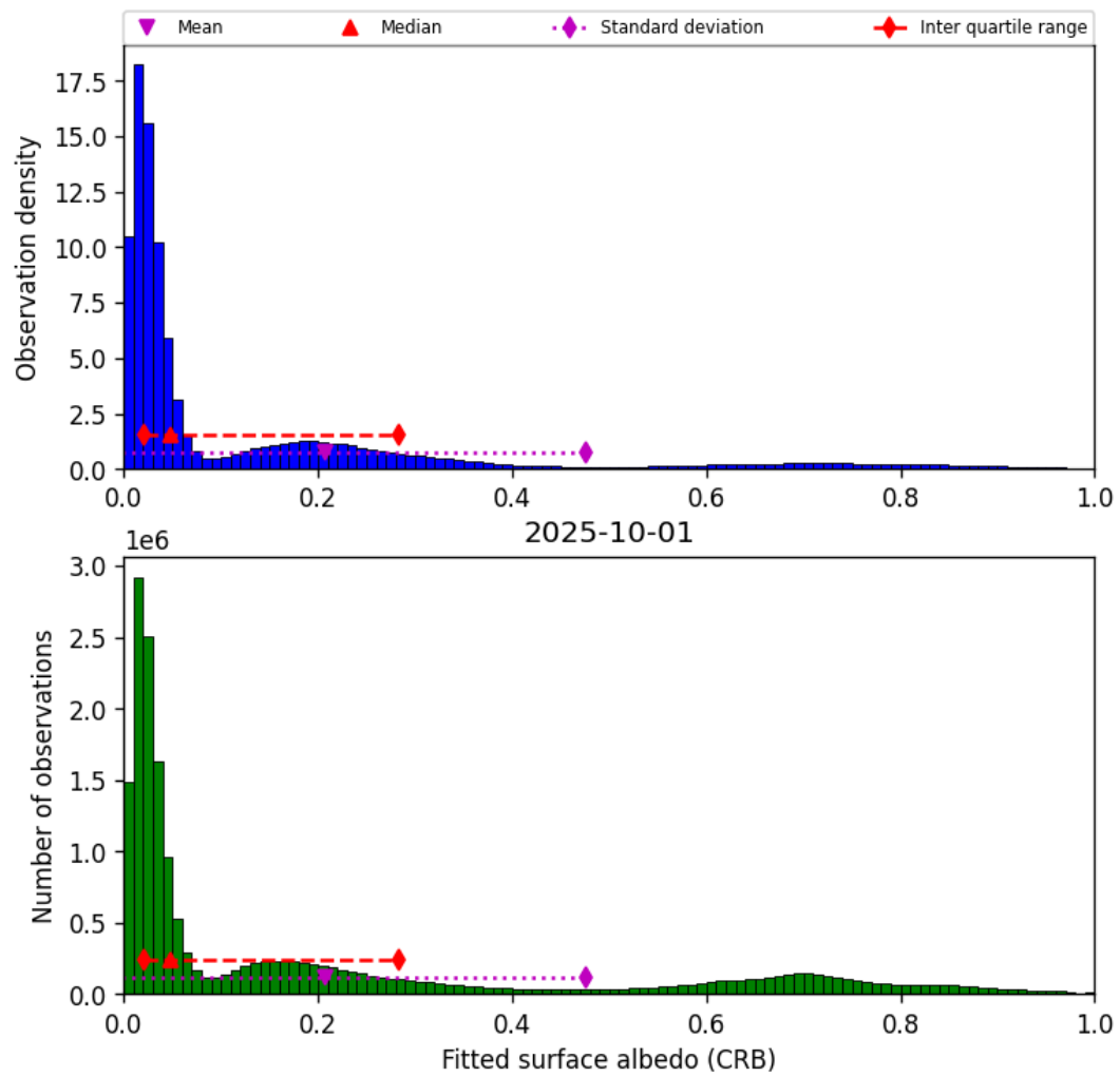
Figure 44: Histogram of “Fitted surface albedo (CRB)” for 2025-10-01 to 2025-10-02
