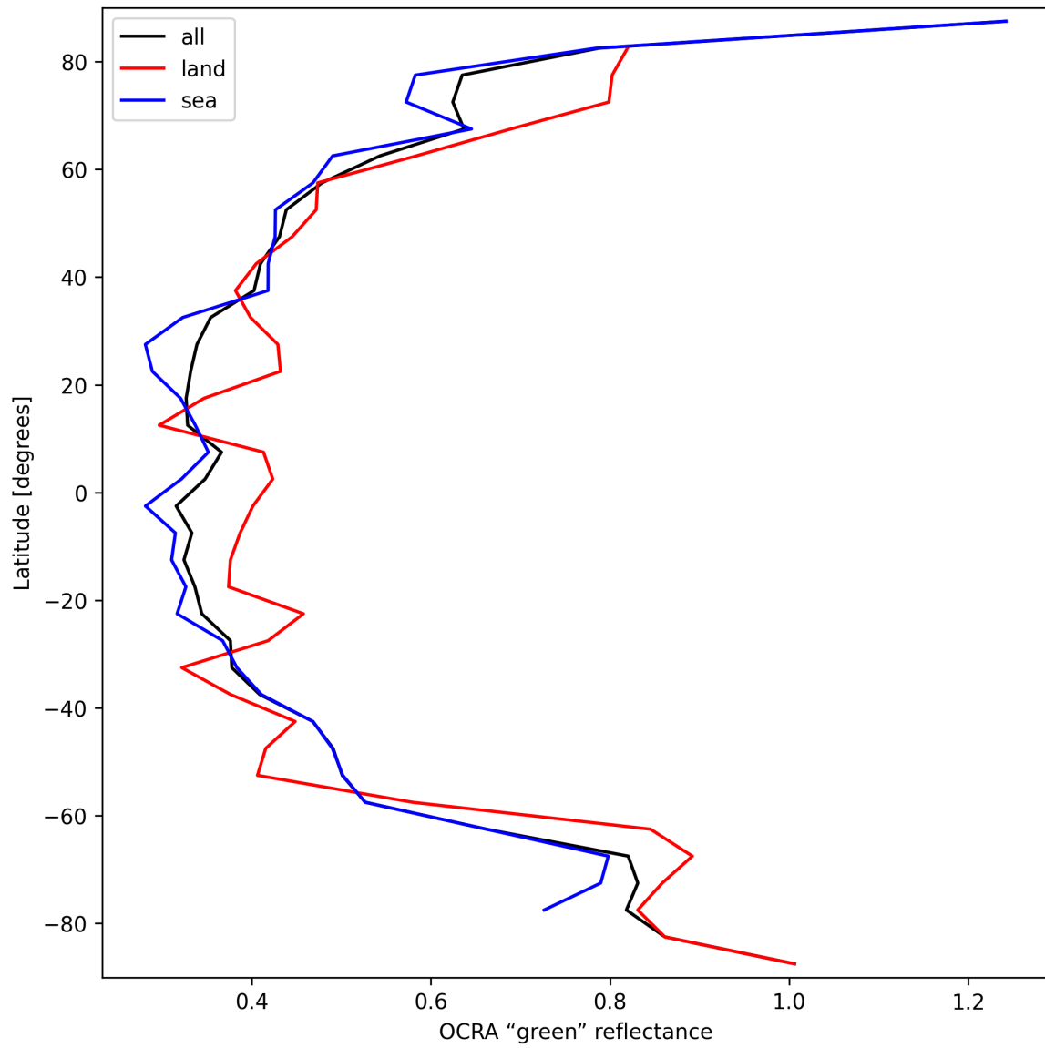
Figure 34: Zonal average of “OCRA “green” reflectance” for 2025-10-01 to 2025-10-02.
