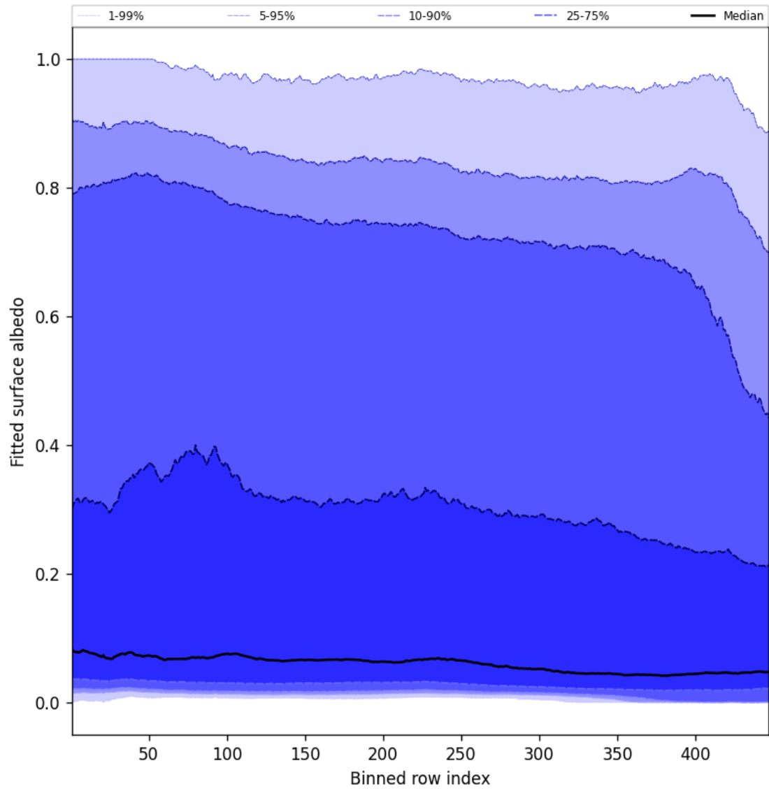
Figure 59: Along track statistics of “Fitted surface albedo” for 2025-10-01 to 2025-10-02
