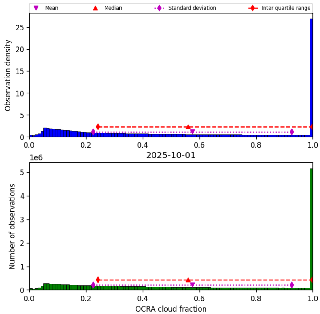
Figure 48: Histogram of “OCRA cloud fraction” for 2025-10-01 to 2025-10-02
