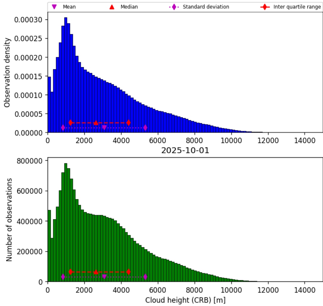
Figure 41: Histogram of “Cloud height (CRB)” for 2025-10-01 to 2025-10-02
