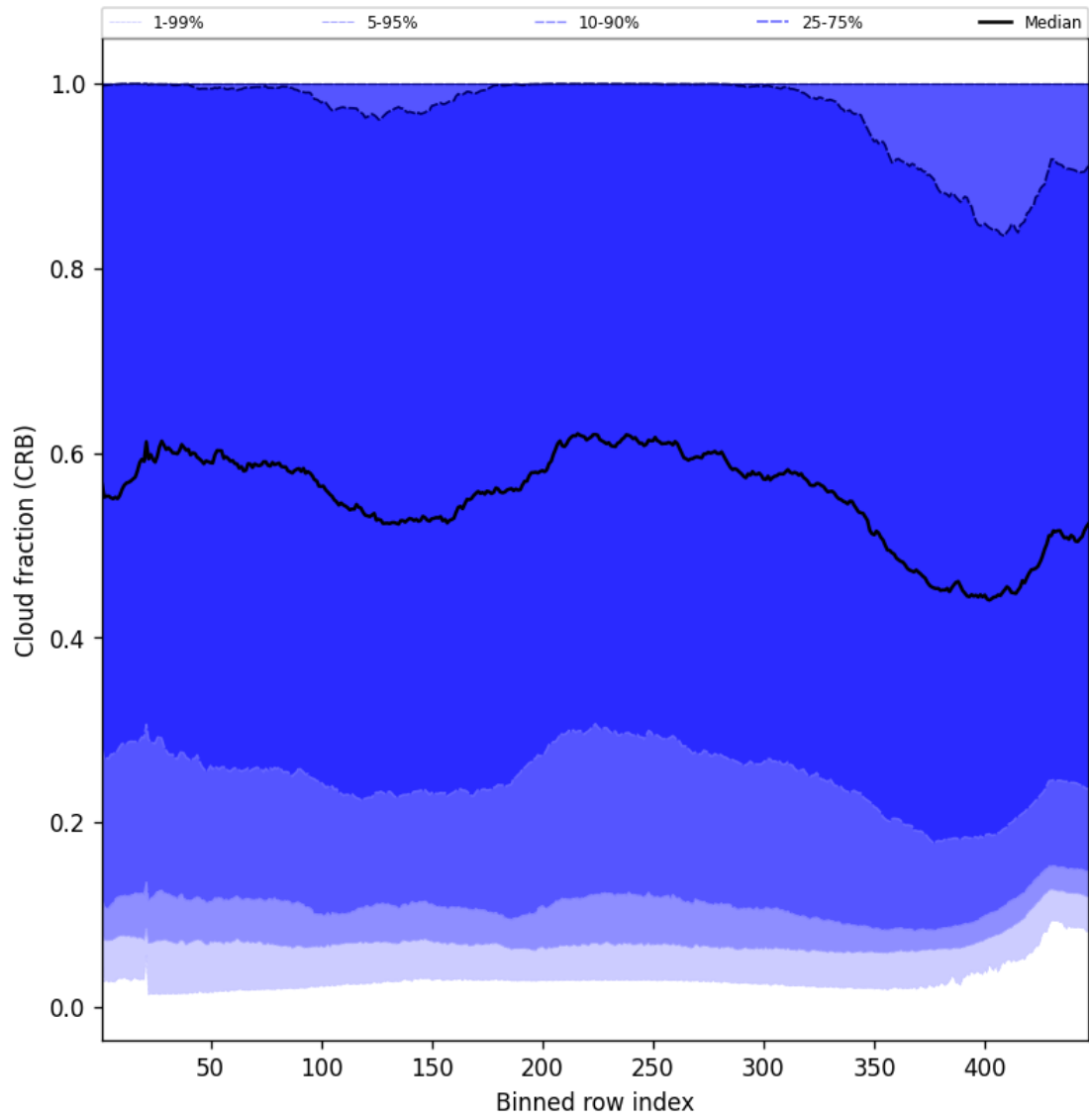
Figure 56: Along track statistics of “Cloud fraction (CRB)” for 2025-10-01 to 2025-10-02
