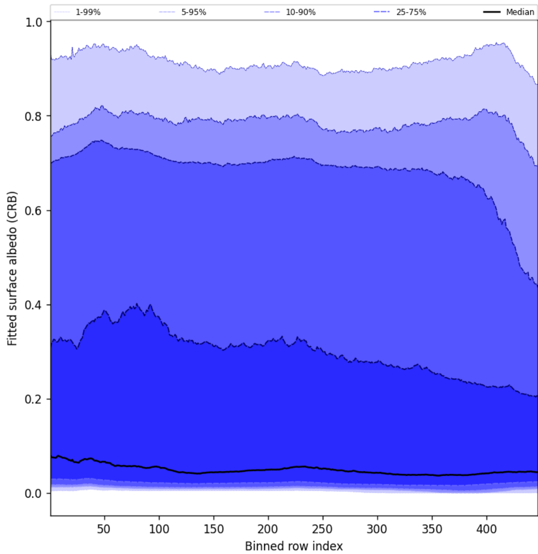
Figure 60: Along track statistics of “Fitted surface albedo (CRB)” for 2025-10-01 to 2025-10-02
