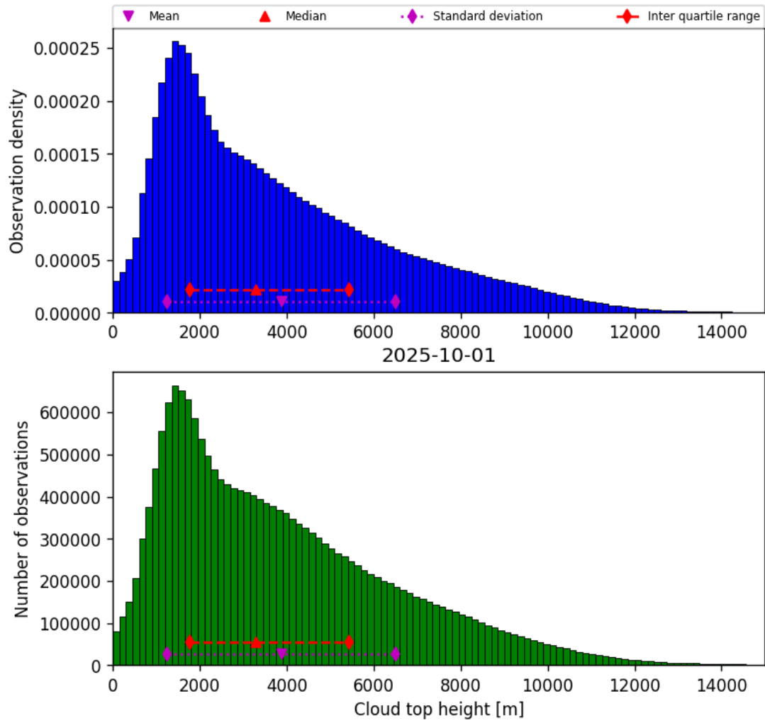
Figure 38: Histogram of “Cloud top height” for 2025-10-01 to 2025-10-02
