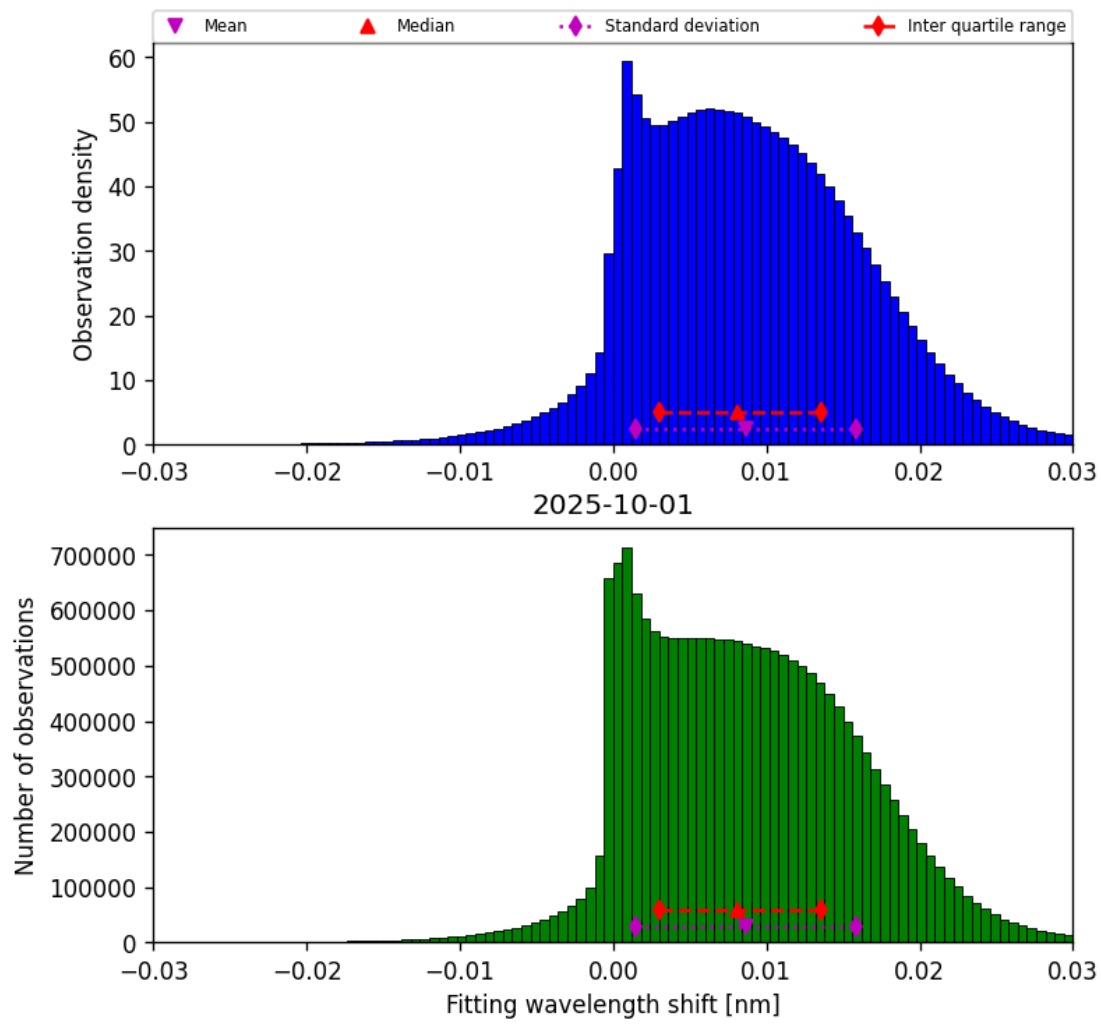
Figure 47: Histogram of “Fitting wavelength shift” for 2025-10-01 to 2025-10-02
