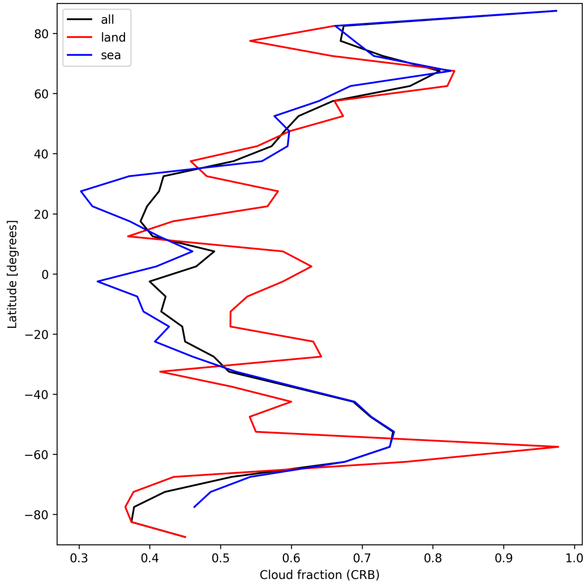
Figure 24: Zonal average of “Cloud fraction (CRB)” for 2025-10-01 to 2025-10-02.
