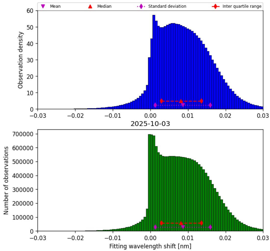
Figure 47: Histogram of “Fitting wavelength shift” for 2025-10-03 to 2025-10-04
