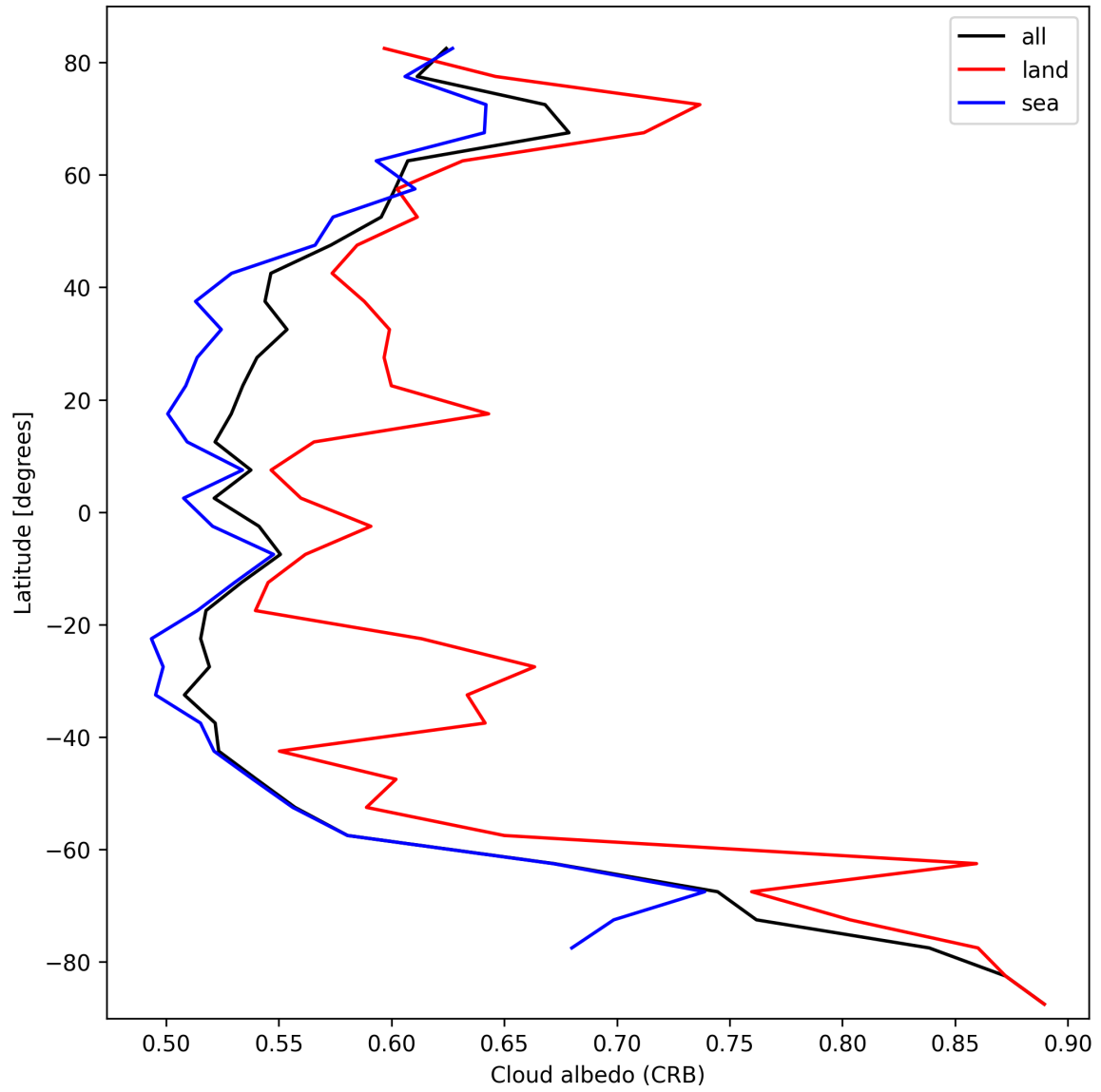
Figure 26: Zonal average of “Cloud albedo (CRB)” for 2025-10-03 to 2025-10-04.
