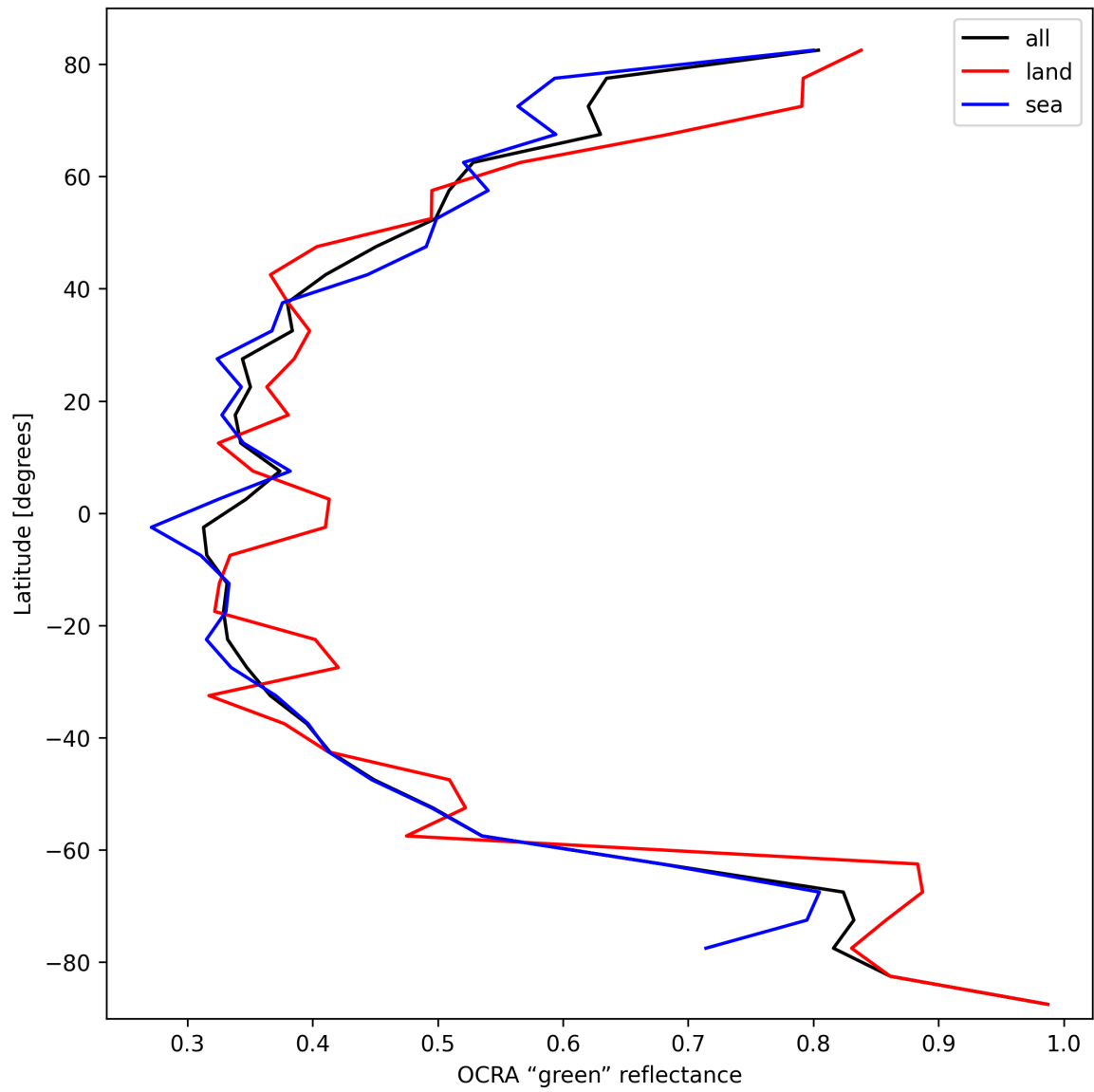
Figure 34: Zonal average of “OCRA “green” reflectance” for 2025-10-03 to 2025-10-04.
