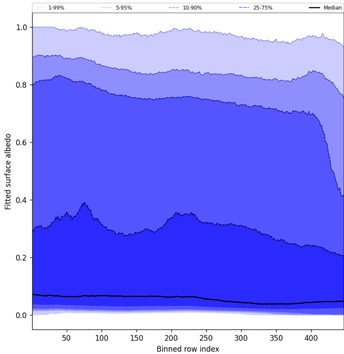
Figure 59: Along track statistics of “Fitted surface albedo” for 2025-10-03 to 2025-10-04
