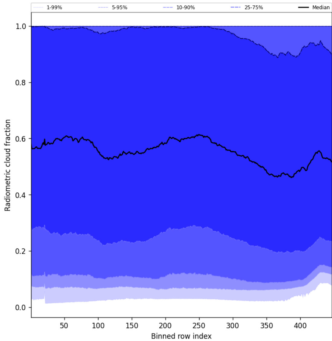
Figure 53: Along track statistics of “Radiometric cloud fraction” for 2025-10-03 to 2025-10-04
