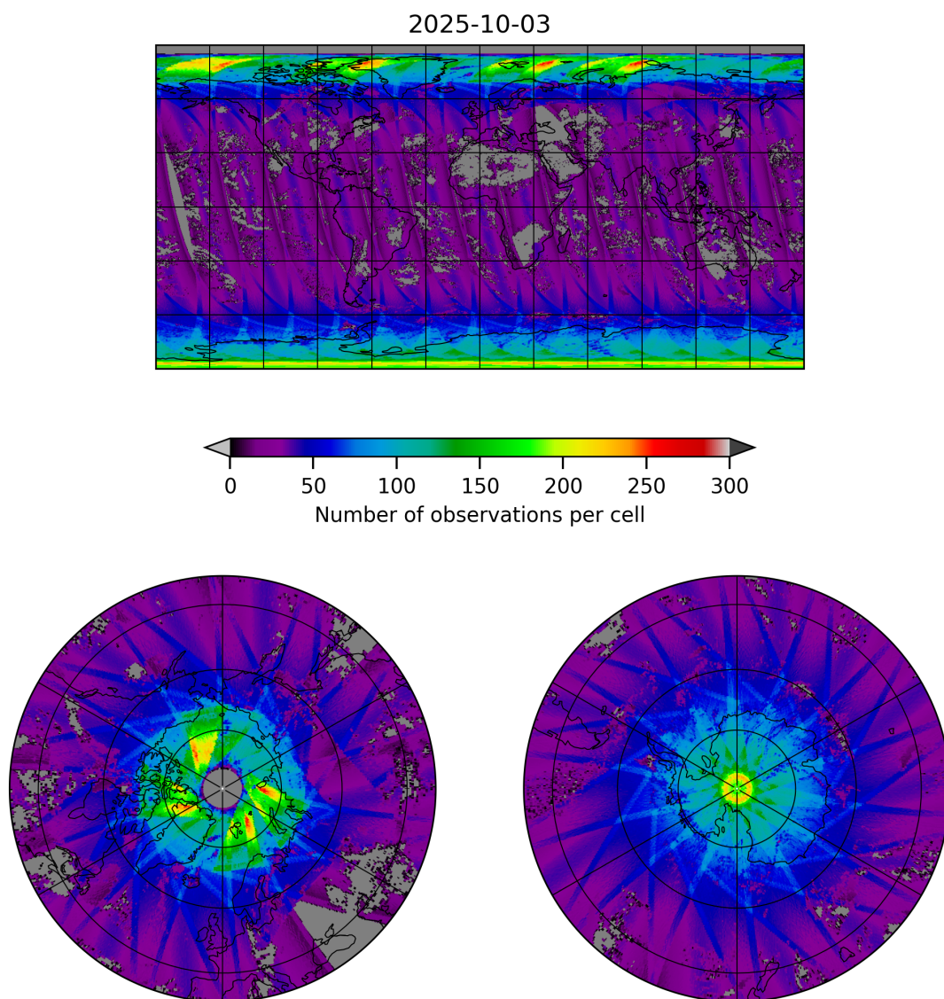
Figure 19: Map of the number of observations for 2025-10-03 to 2025-10-04
