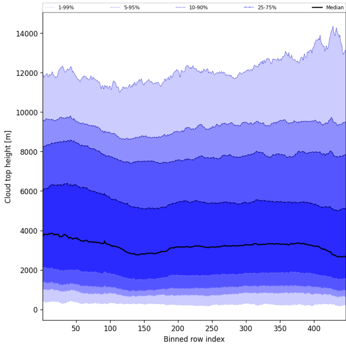
Figure 54: Along track statistics of “Cloud top height” for 2025-10-03 to 2025-10-04
