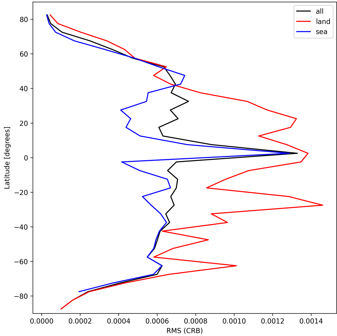
Figure 30: Zonal average of “RMS (CRB)” for 2025-10-03 to 2025-10-04.
