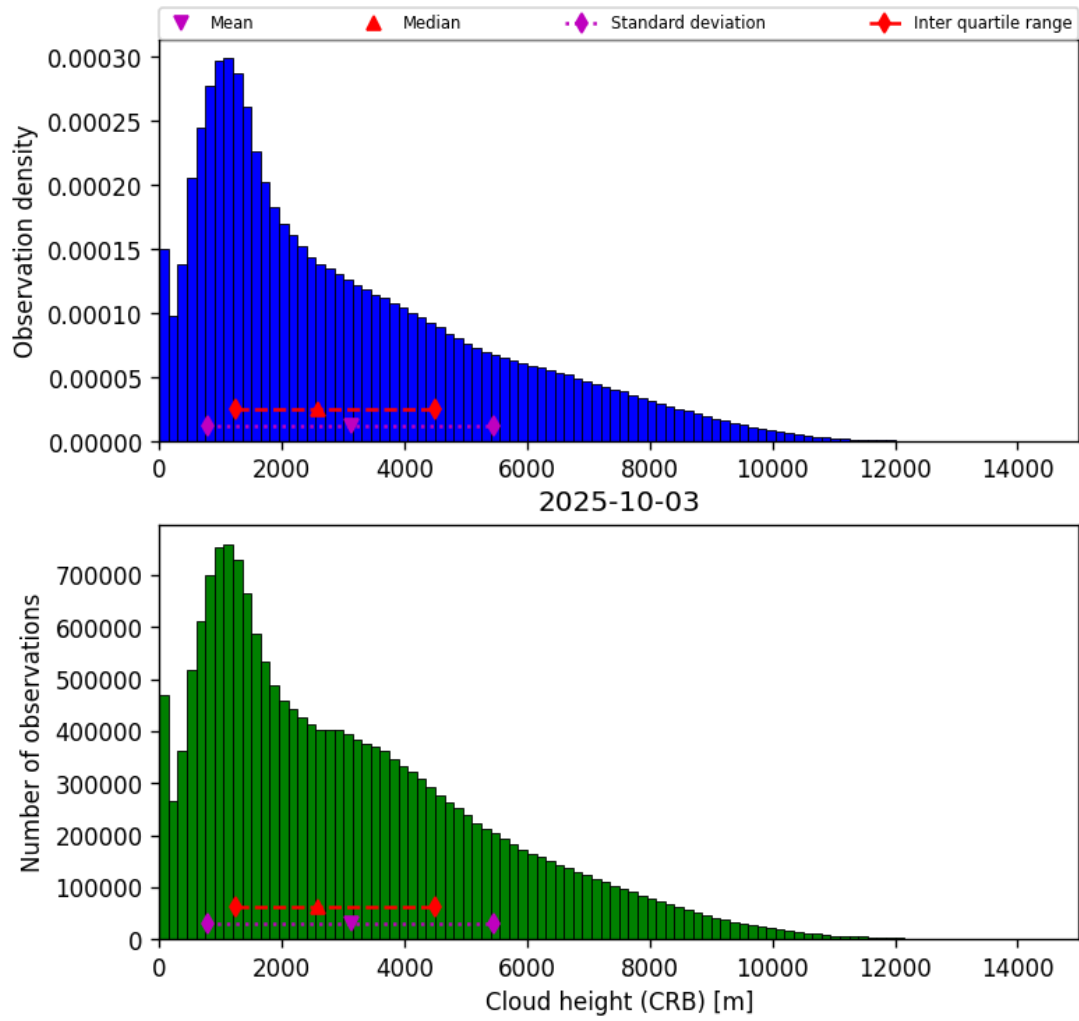
Figure 41: Histogram of “Cloud height (CRB)” for 2025-10-03 to 2025-10-04
