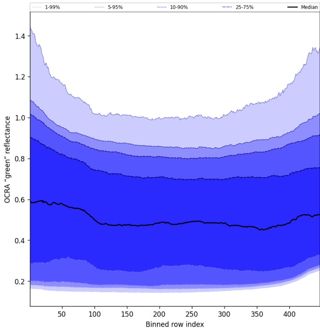
Figure 66: Along track statistics of “OCRA “green” reflectance” for 2025-10-03 to 2025-10-04
