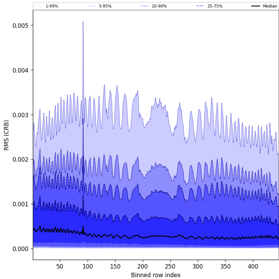
Figure 62: Along track statistics of “RMS (CRB)” for 2025-10-03 to 2025-10-04
