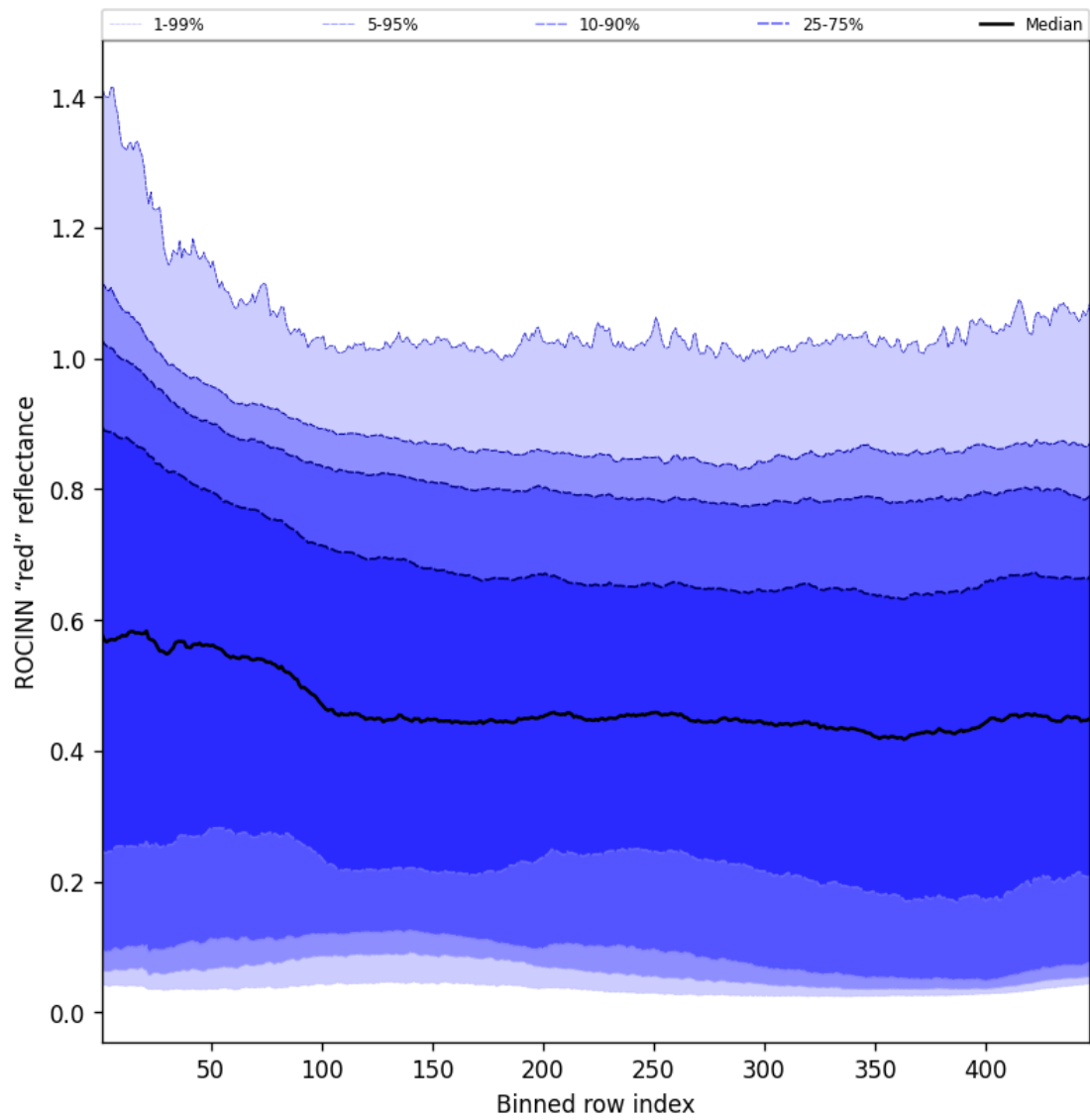
Figure 67: Along track statistics of “ROCINN “red” reflectance” for 2025-10-03 to 2025-10-04
