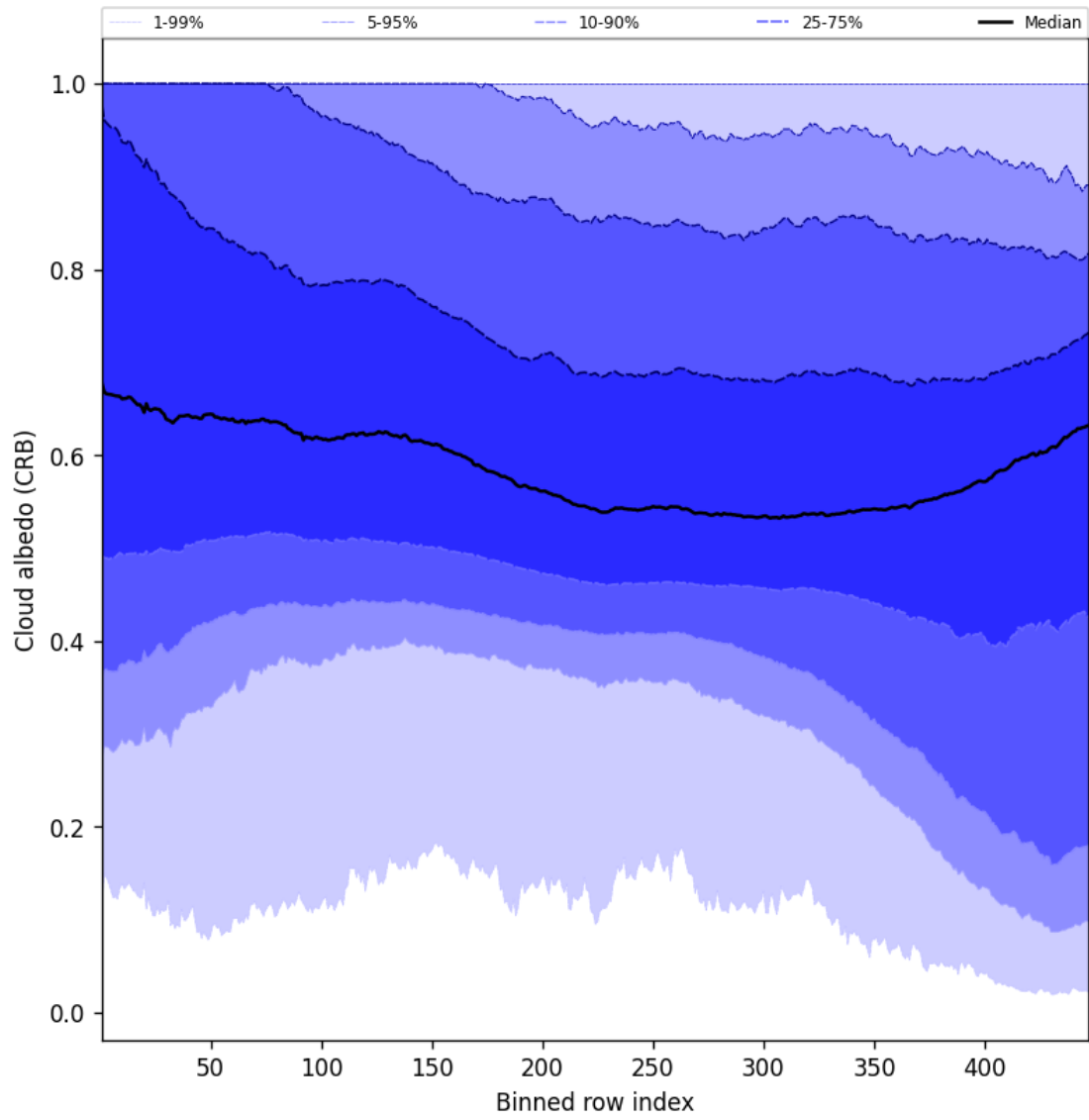
Figure 58: Along track statistics of “Cloud albedo (CRB)” for 2025-10-03 to 2025-10-04
