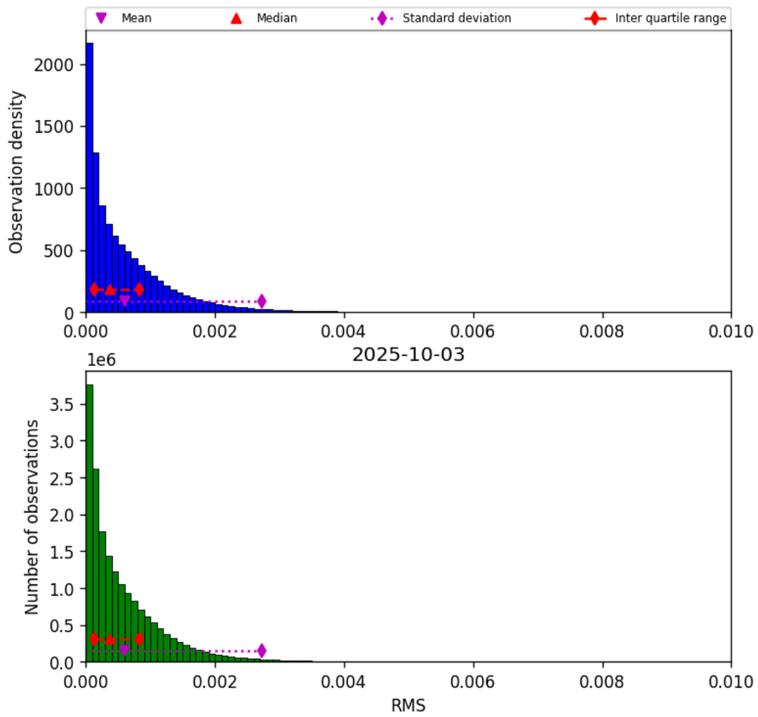
Figure 45: Histogram of “RMS” for 2025-10-03 to 2025-10-04
