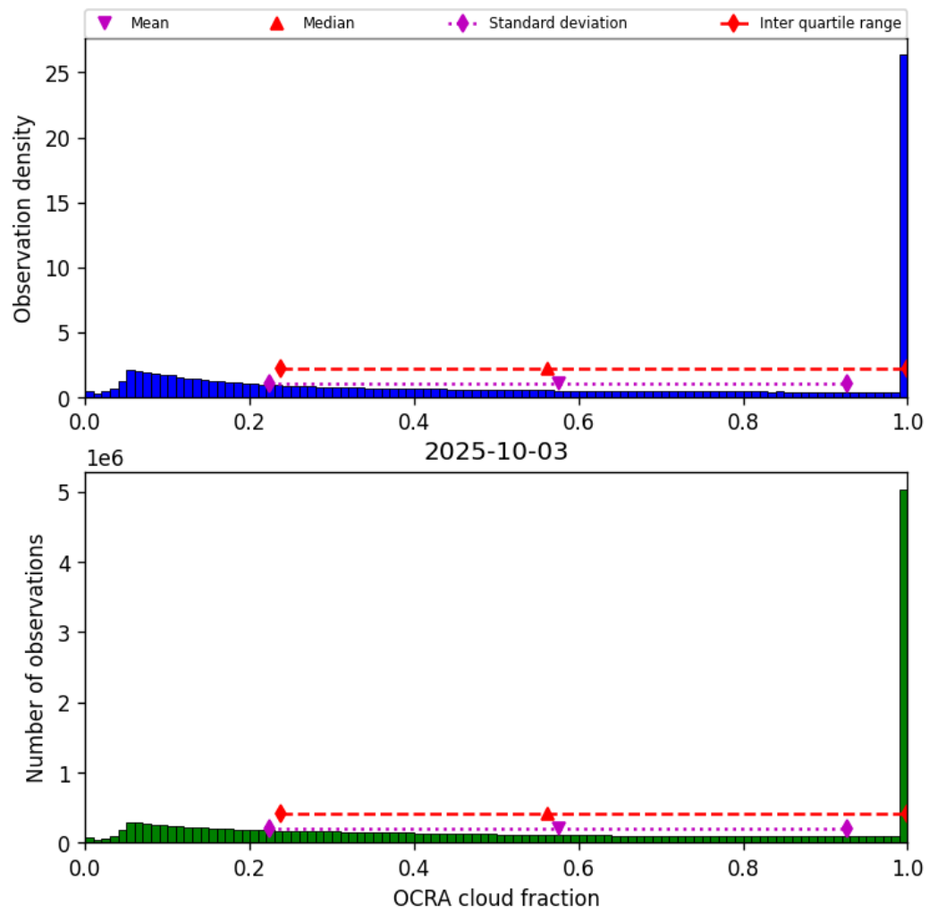
Figure 48: Histogram of “OCRA cloud fraction” for 2025-10-03 to 2025-10-04
