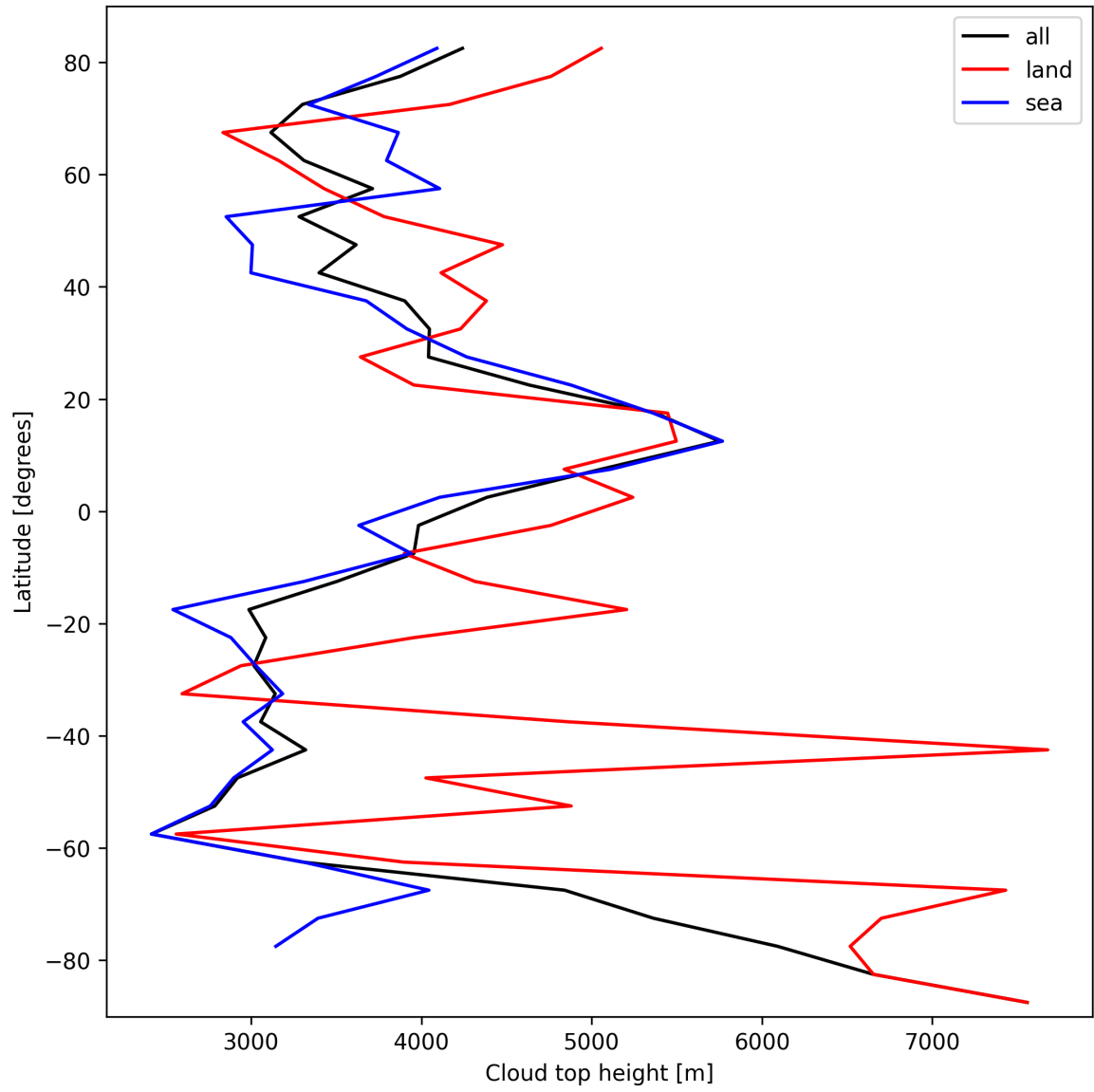
Figure 22: Zonal average of “Cloud top height” for 2025-10-03 to 2025-10-04.
