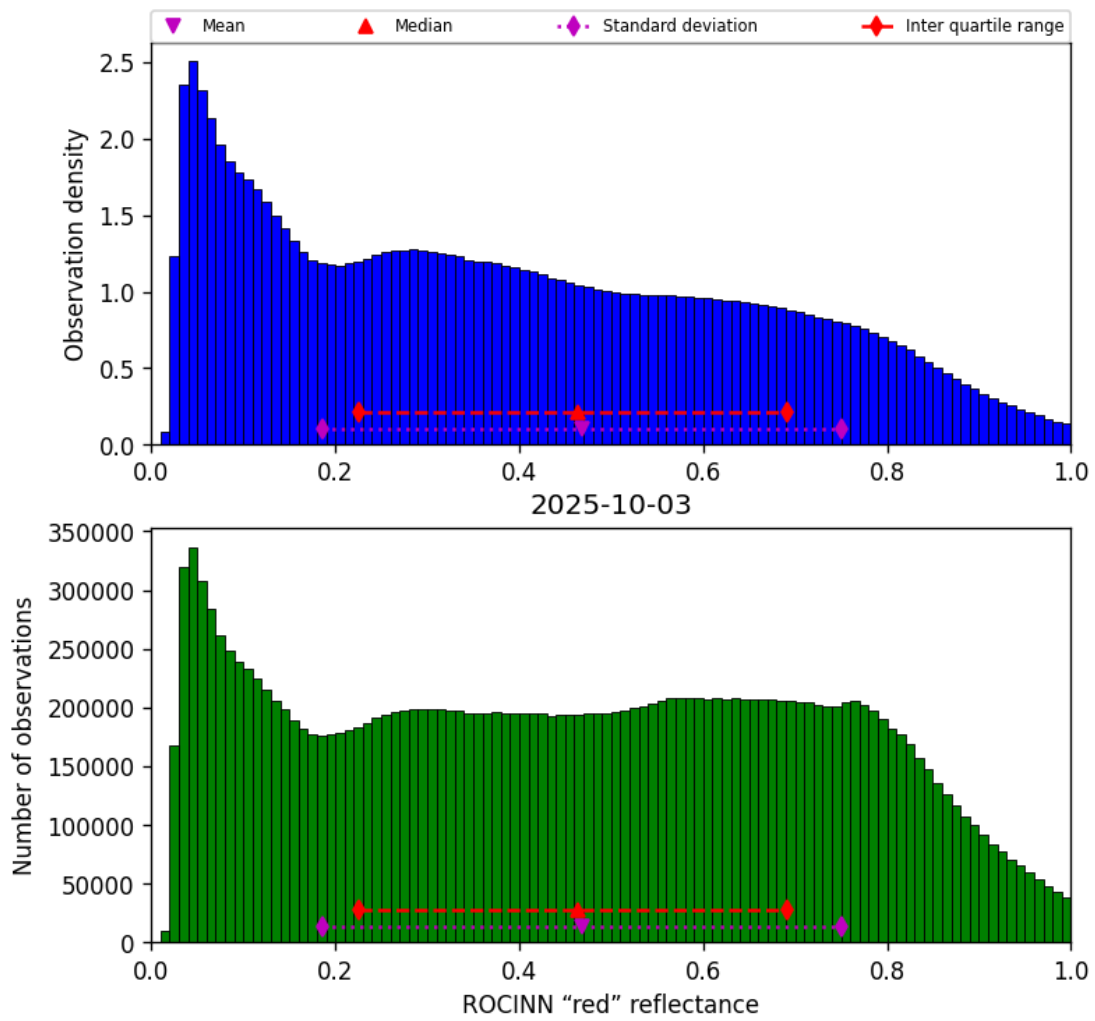
Figure 51: Histogram of “ROCINN “red” reflectance” for 2025-10-03 to 2025-10-04
