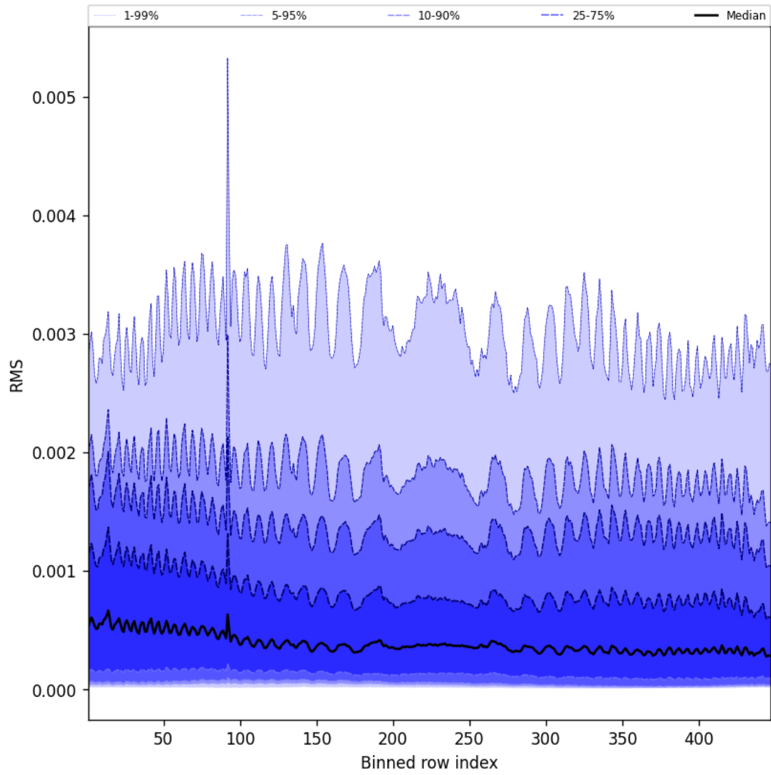
Figure 61: Along track statistics of “RMS” for 2025-10-03 to 2025-10-04
