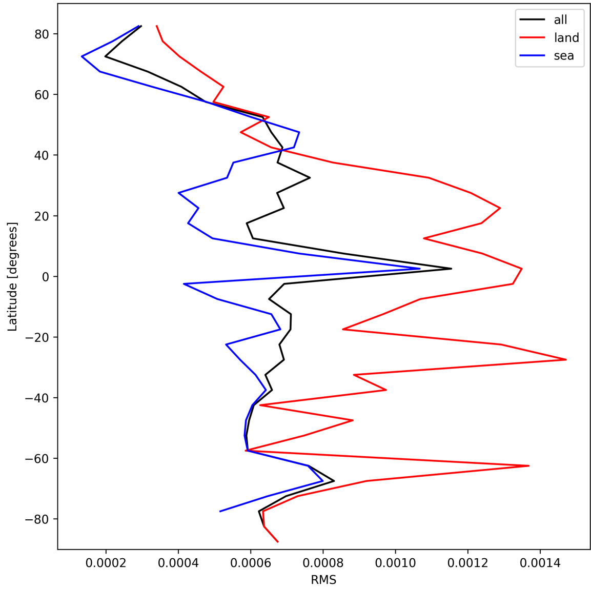
Figure 29: Zonal average of “RMS” for 2025-10-03 to 2025-10-04.
