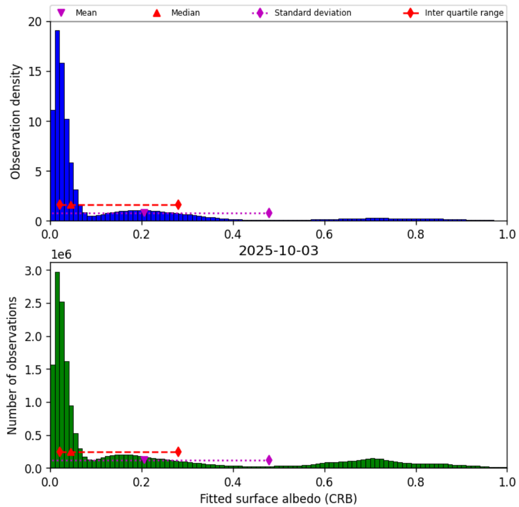
Figure 44: Histogram of “Fitted surface albedo (CRB)” for 2025-10-03 to 2025-10-04
