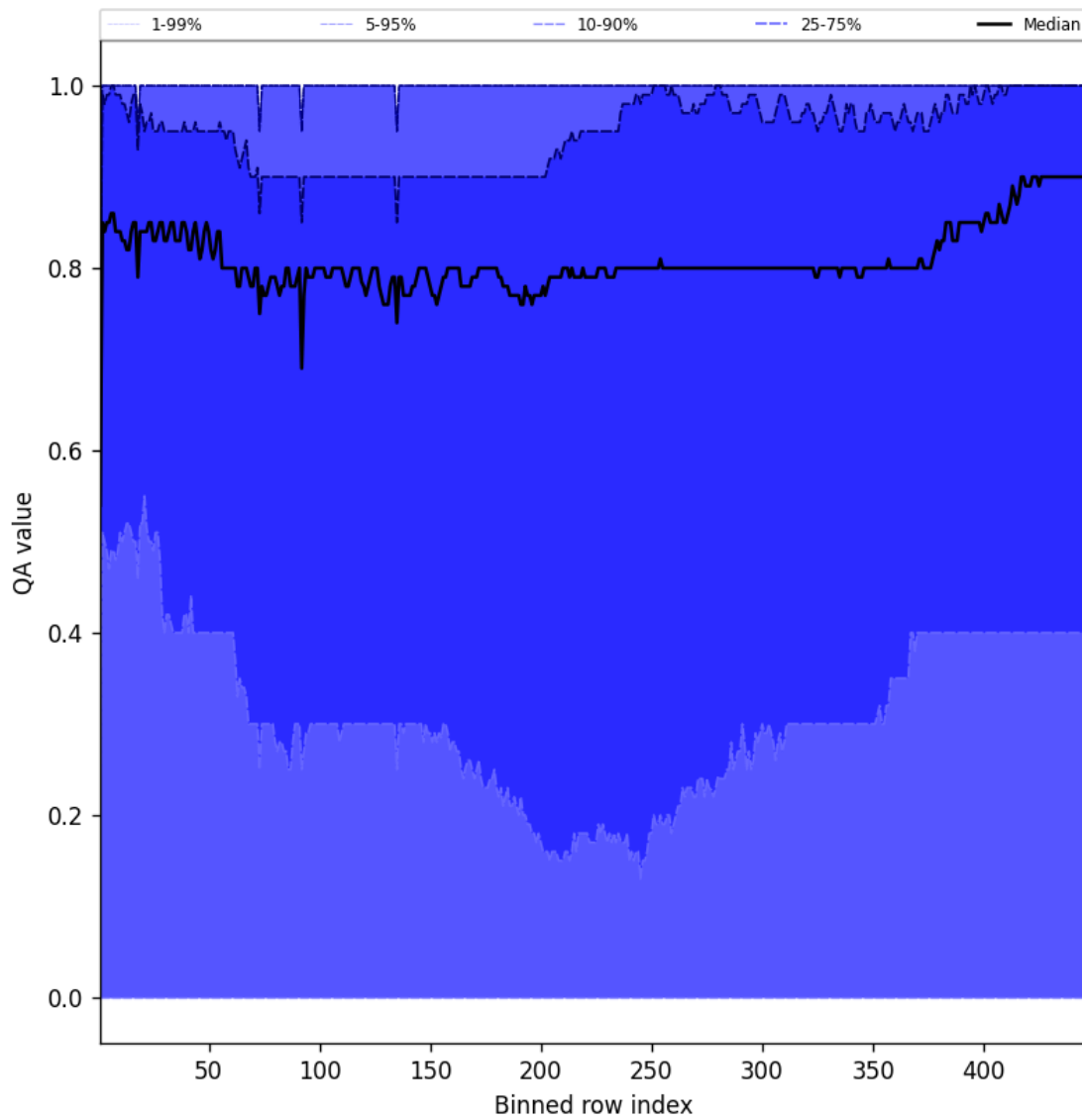
Figure 52: Along track statistics of “QA value” for 2025-10-03 to 2025-10-04
