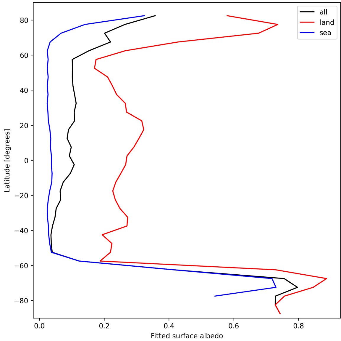
Figure 27: Zonal average of “Fitted surface albedo” for 2025-10-03 to 2025-10-04.
