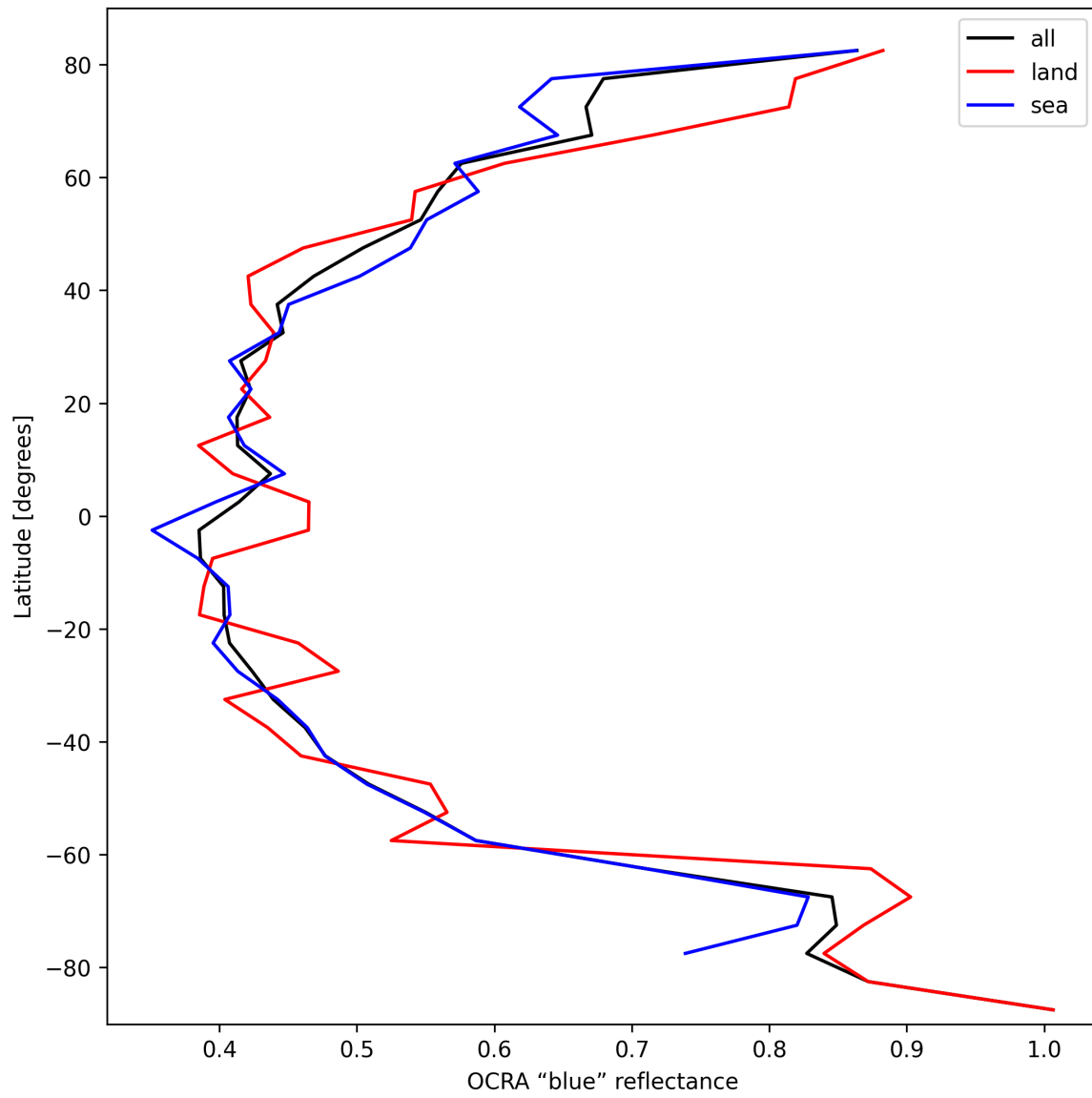
Figure 33: Zonal average of “OCRA “blue” reflectance” for 2025-10-03 to 2025-10-04.
