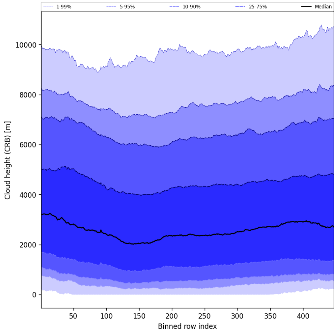
Figure 57: Along track statistics of “Cloud height (CRB)” for 2025-10-03 to 2025-10-04
