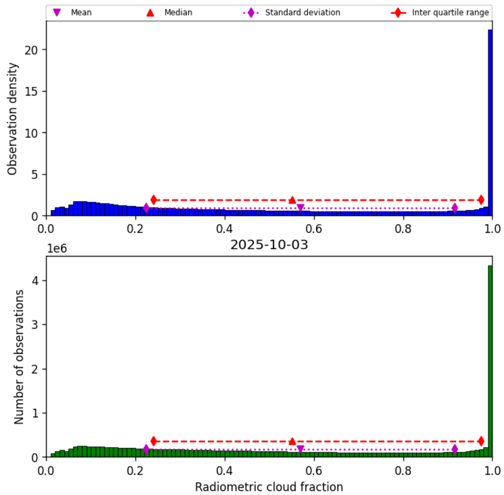
Figure 37: Histogram of "Radiometric cloud fraction" for 2025-10-03 to 2025-10-04
