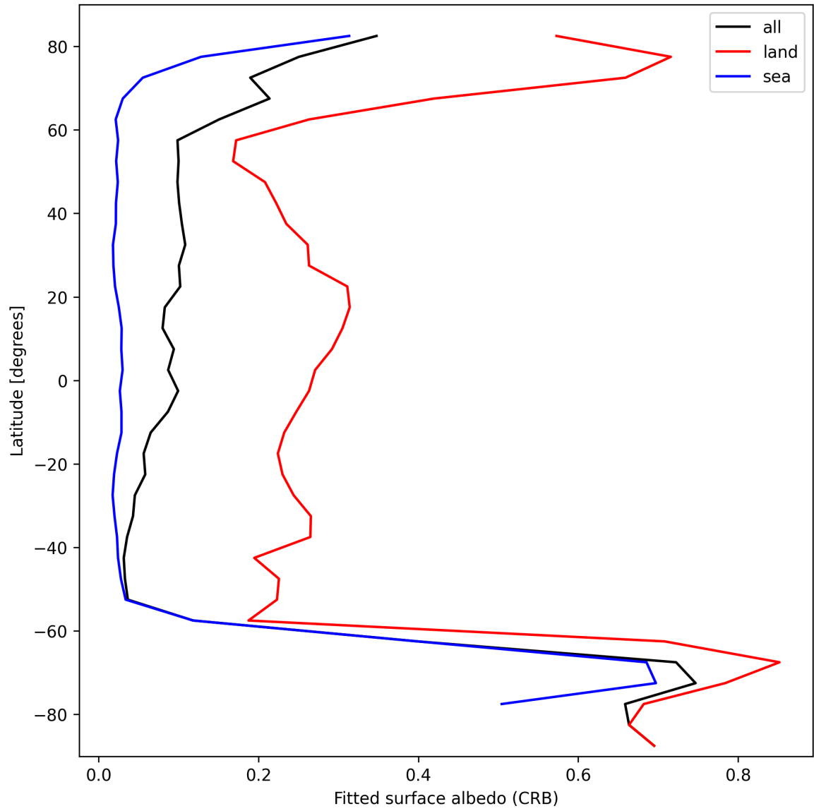
Figure 28: Zonal average of “Fitted surface albedo (CRB)” for 2025-10-03 to 2025-10-04.
