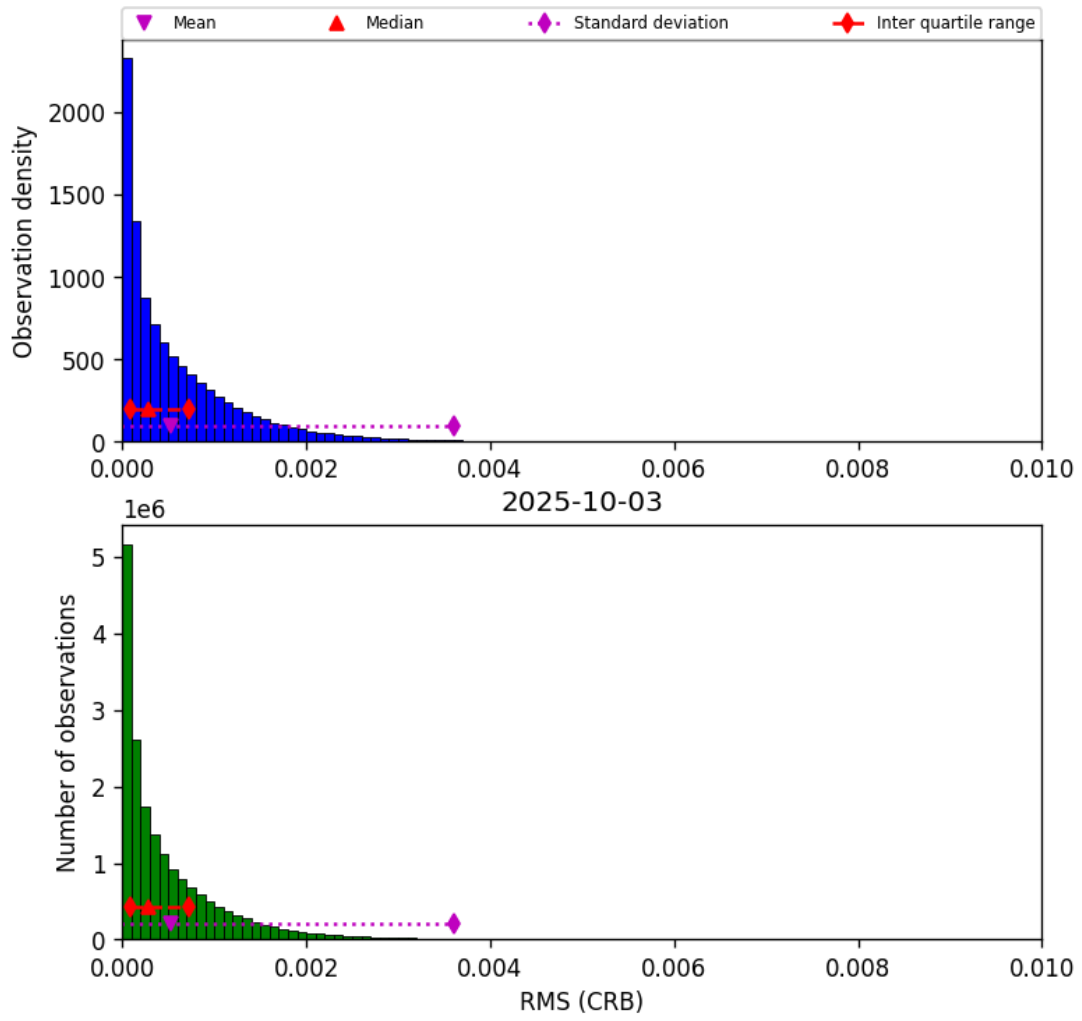
Figure 46: Histogram of "RMS (CRB)" for 2025-10-03 to 2025-10-04
