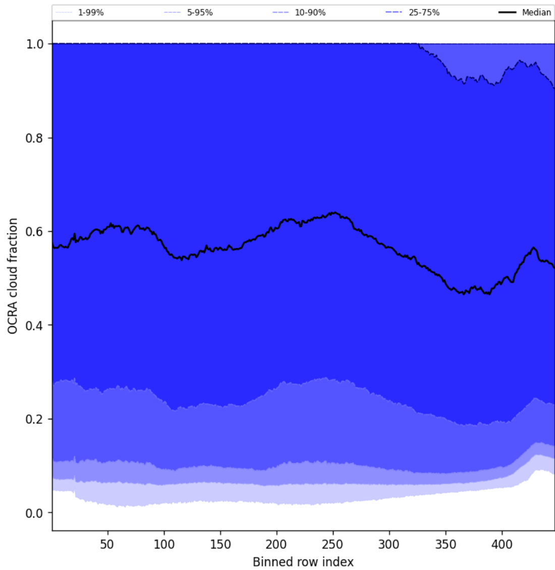
Figure 64: Along track statistics of “OCRA cloud fraction” for 2025-10-03 to 2025-10-04
