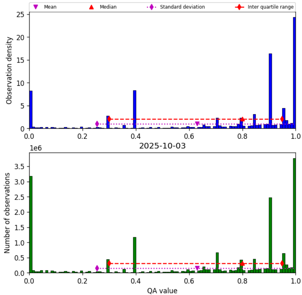
Figure 36: Histogram of “QA value” for 2025-10-03 to 2025-10-04
