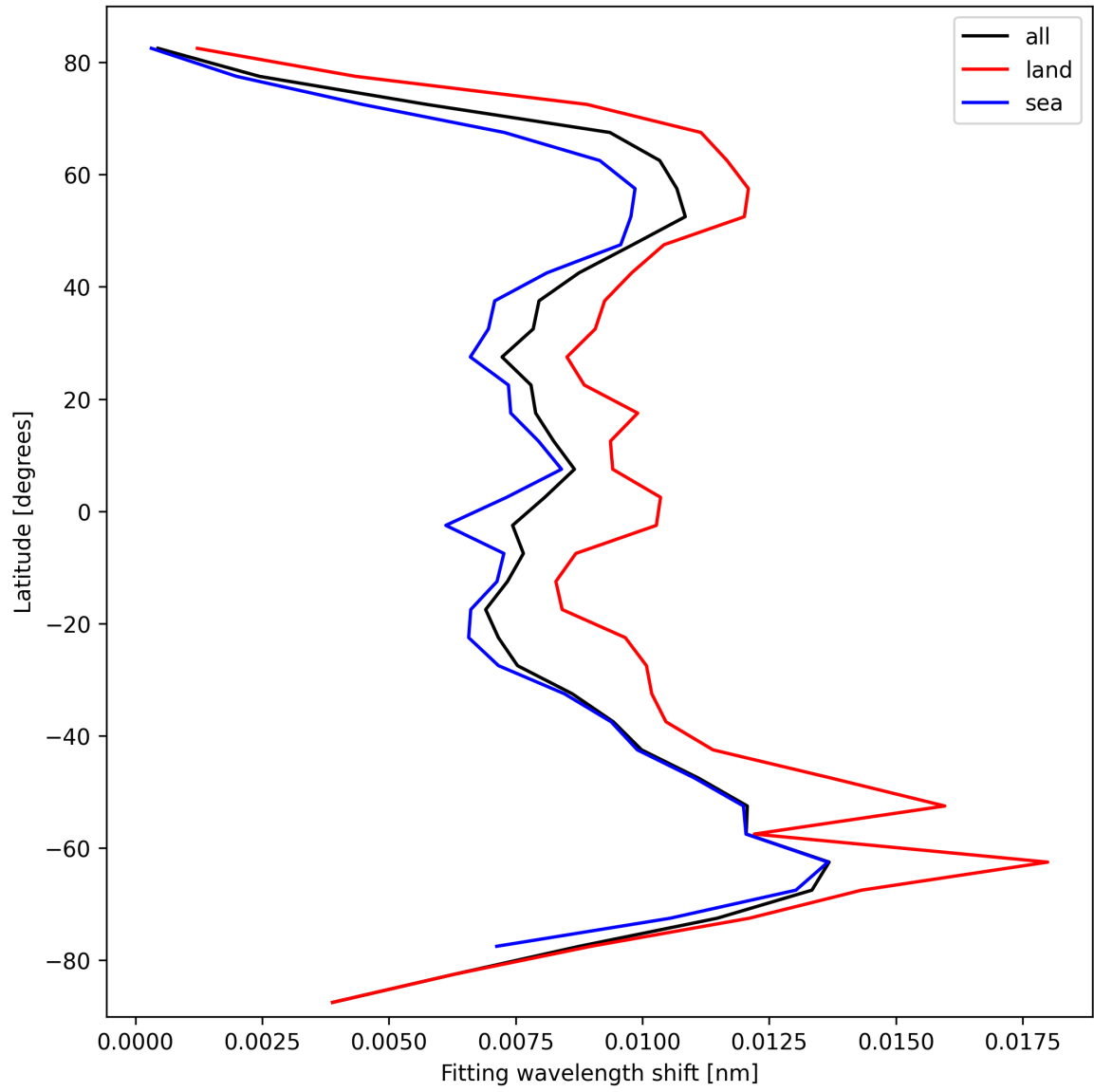
Figure 31: Zonal average of “Fitting wavelength shift” for 2025-10-03 to 2025-10-04.
