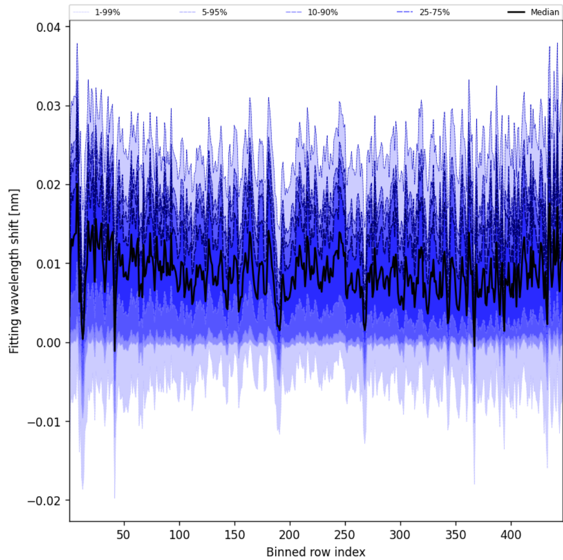
Figure 63: Along track statistics of “Fitting wavelength shift” for 2025-10-03 to 2025-10-04
