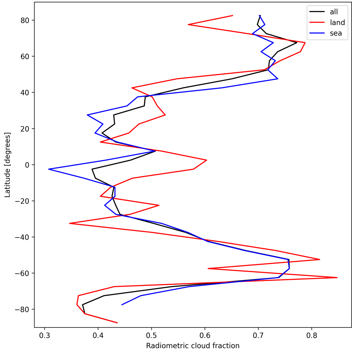
Figure 21: Zonal average of “Radiometric cloud fraction” for 2025-10-03 to 2025-10-04.
