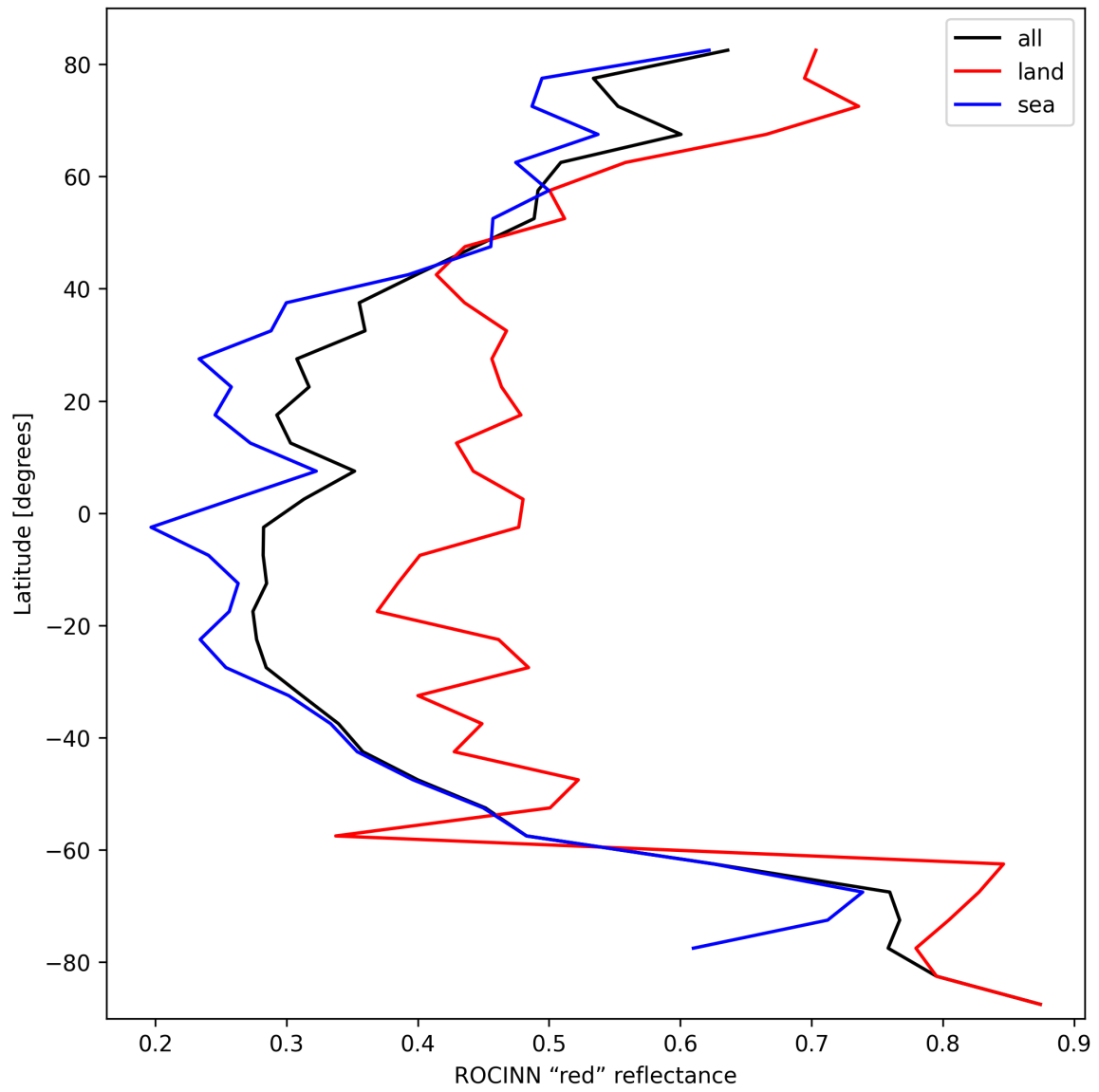
Figure 35: Zonal average of “ROCINN “red” reflectance” for 2025-10-03 to 2025-10-04.
