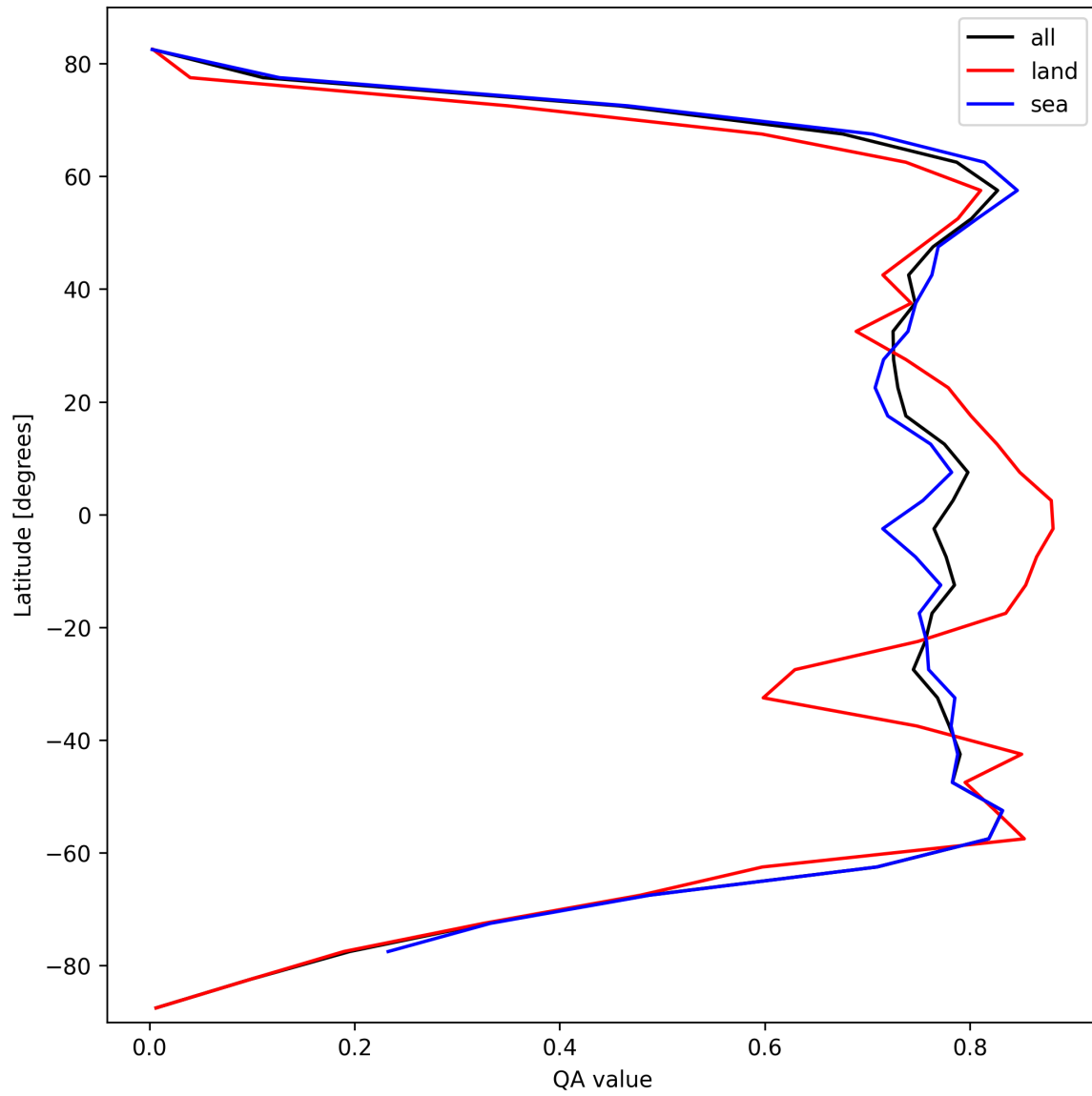
Figure 20: Zonal average of “QA value” for 2025-10-03 to 2025-10-04.
