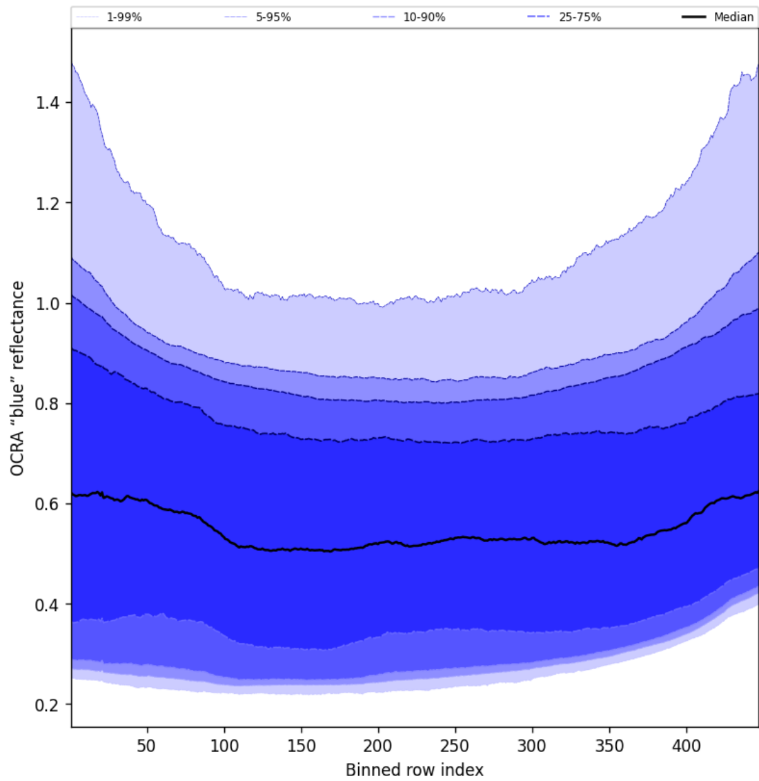
Figure 65: Along track statistics of “OCRA “blue” reflectance” for 2025-10-03 to 2025-10-04
