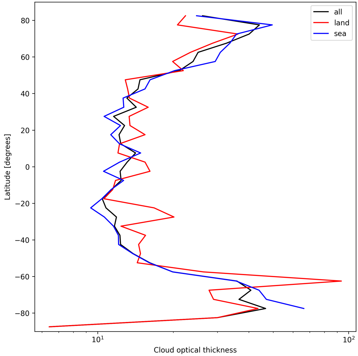
Figure 23: Zonal average of “Cloud optical thickness” for 2025-10-03 to 2025-10-04.
