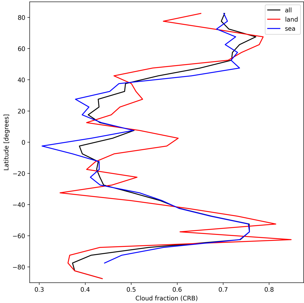
Figure 24: Zonal average of “Cloud fraction (CRB)” for 2025-10-03 to 2025-10-04.
