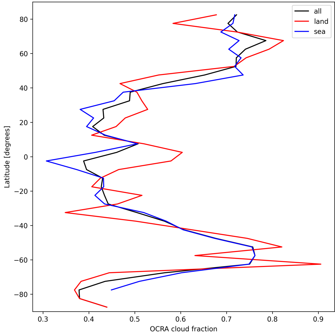
Figure 32: Zonal average of “OCRA cloud fraction” for 2025-10-03 to 2025-10-04.
