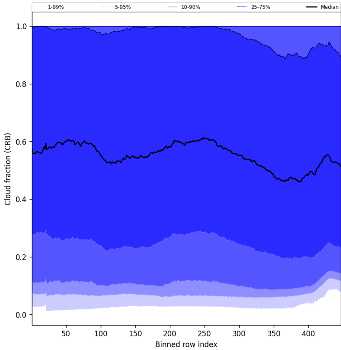
Figure 56: Along track statistics of “Cloud fraction (CRB)” for 2025-10-03 to 2025-10-04
