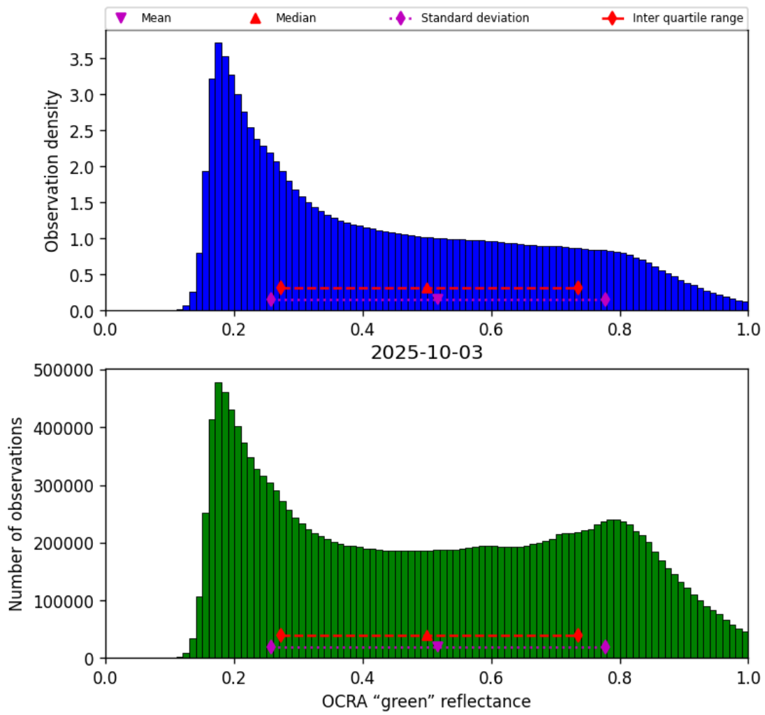
Figure 50: Histogram of “OCRA “green” reflectance” for 2025-10-03 to 2025-10-04
