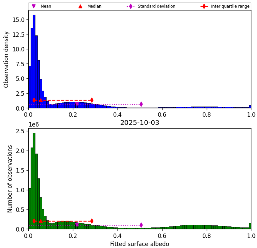
Figure 43: Histogram of “Fitted surface albedo” for 2025-10-03 to 2025-10-04
