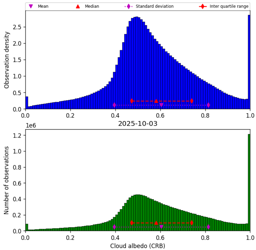
Figure 42: Histogram of “Cloud albedo (CRB)” for 2025-10-03 to 2025-10-04
