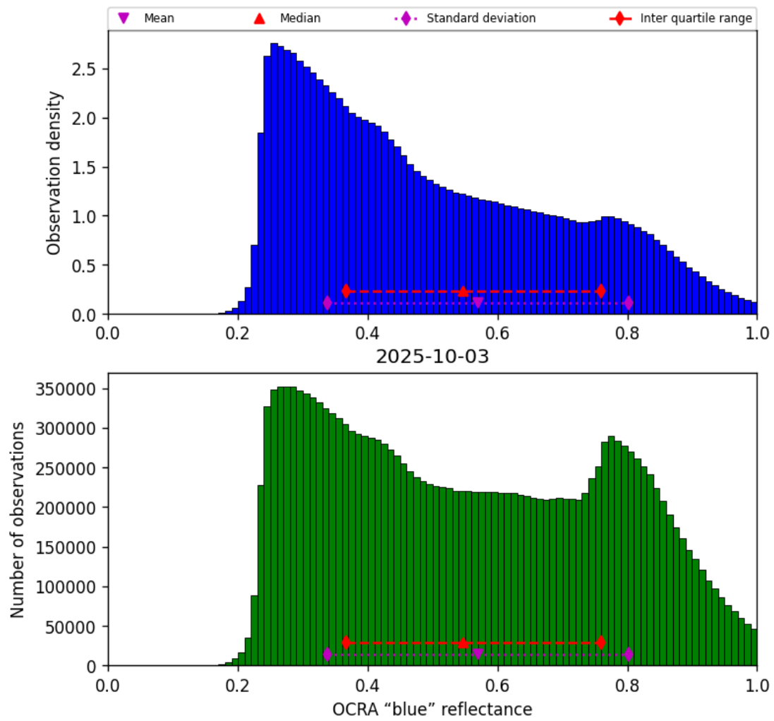
Figure 49: Histogram of “OCRA “blue” reflectance” for 2025-10-03 to 2025-10-04
