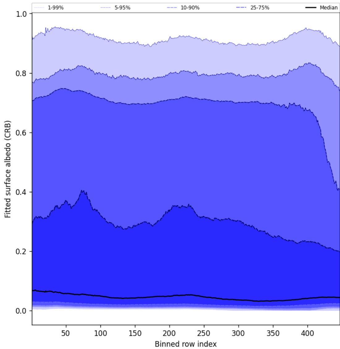
Figure 60: Along track statistics of “Fitted surface albedo (CRB)” for 2025-10-03 to 2025-10-04
