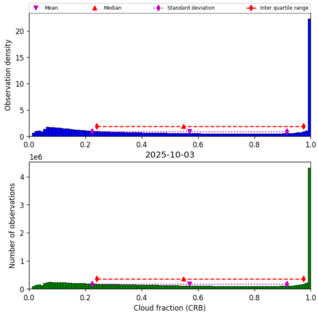
Figure 40: Histogram of “Cloud fraction (CRB)” for 2025-10-03 to 2025-10-04
