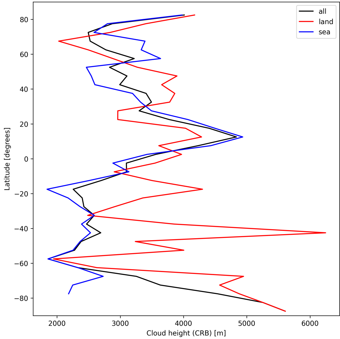
Figure 25: Zonal average of “Cloud height (CRB)” for 2025-10-03 to 2025-10-04.
