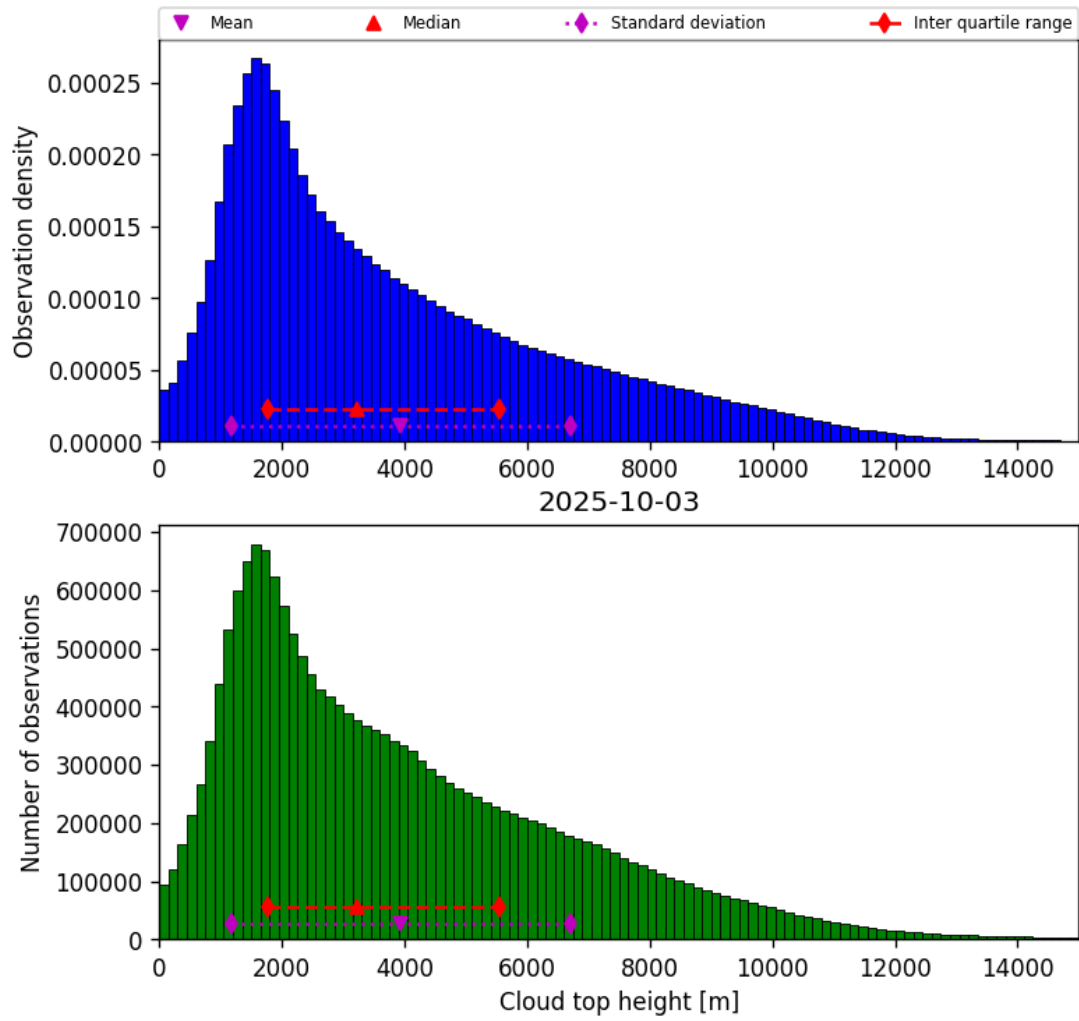
Figure 38: Histogram of “Cloud top height” for 2025-10-03 to 2025-10-04
