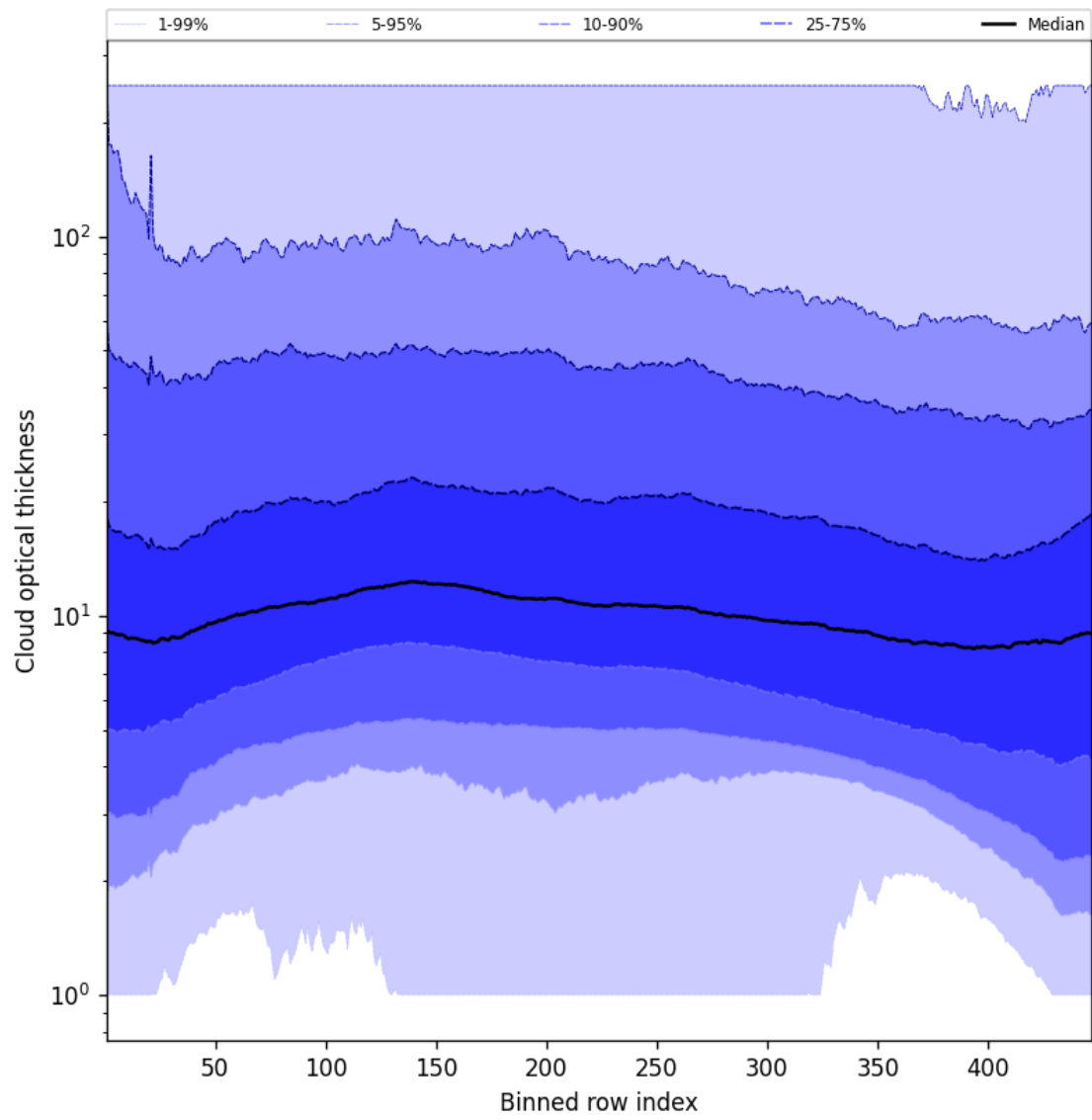
Figure 55: Along track statistics of “Cloud optical thickness” for 2025-10-03 to 2025-10-04
