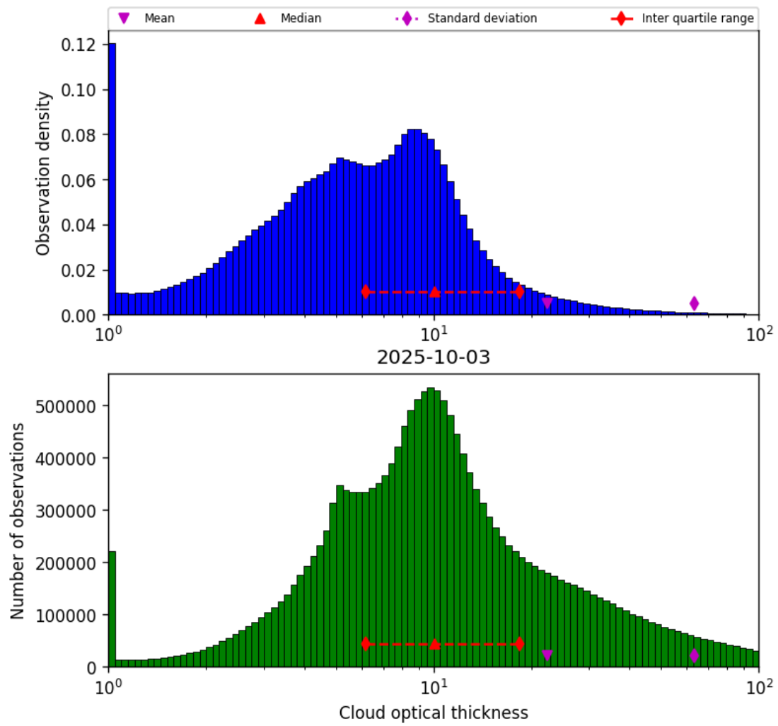
Figure 39: Histogram of “Cloud optical thickness” for 2025-10-03 to 2025-10-04
