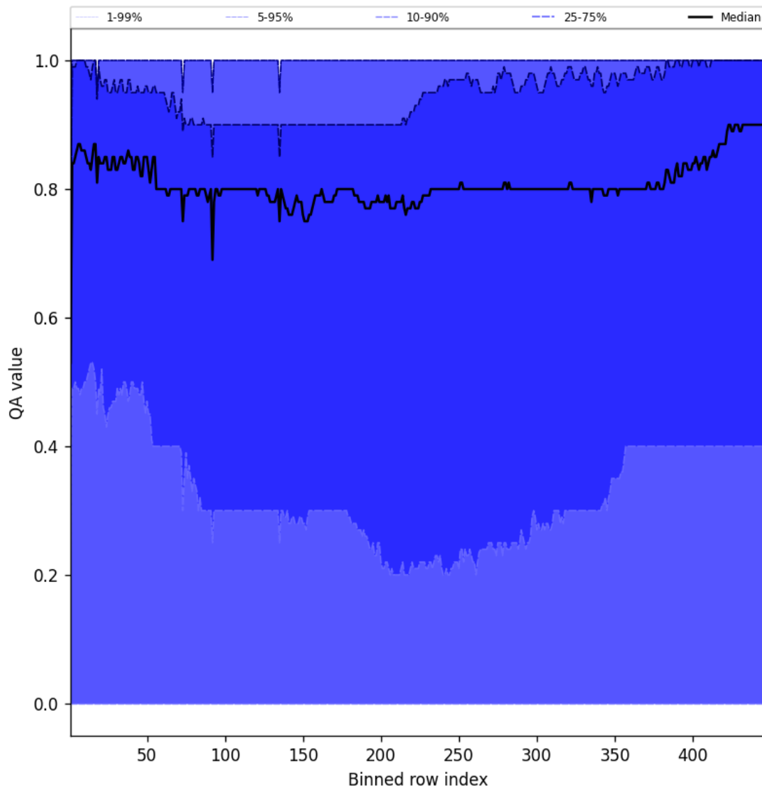
Figure 52: Along track statistics of “QA value” for 2025-10-04 to 2025-10-04
