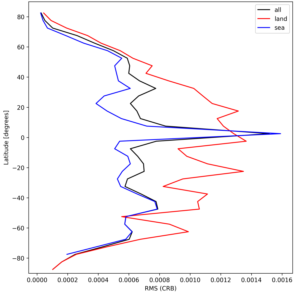
Figure 30: Zonal average of “RMS (CRB)” for 2025-10-04 to 2025-10-04.
