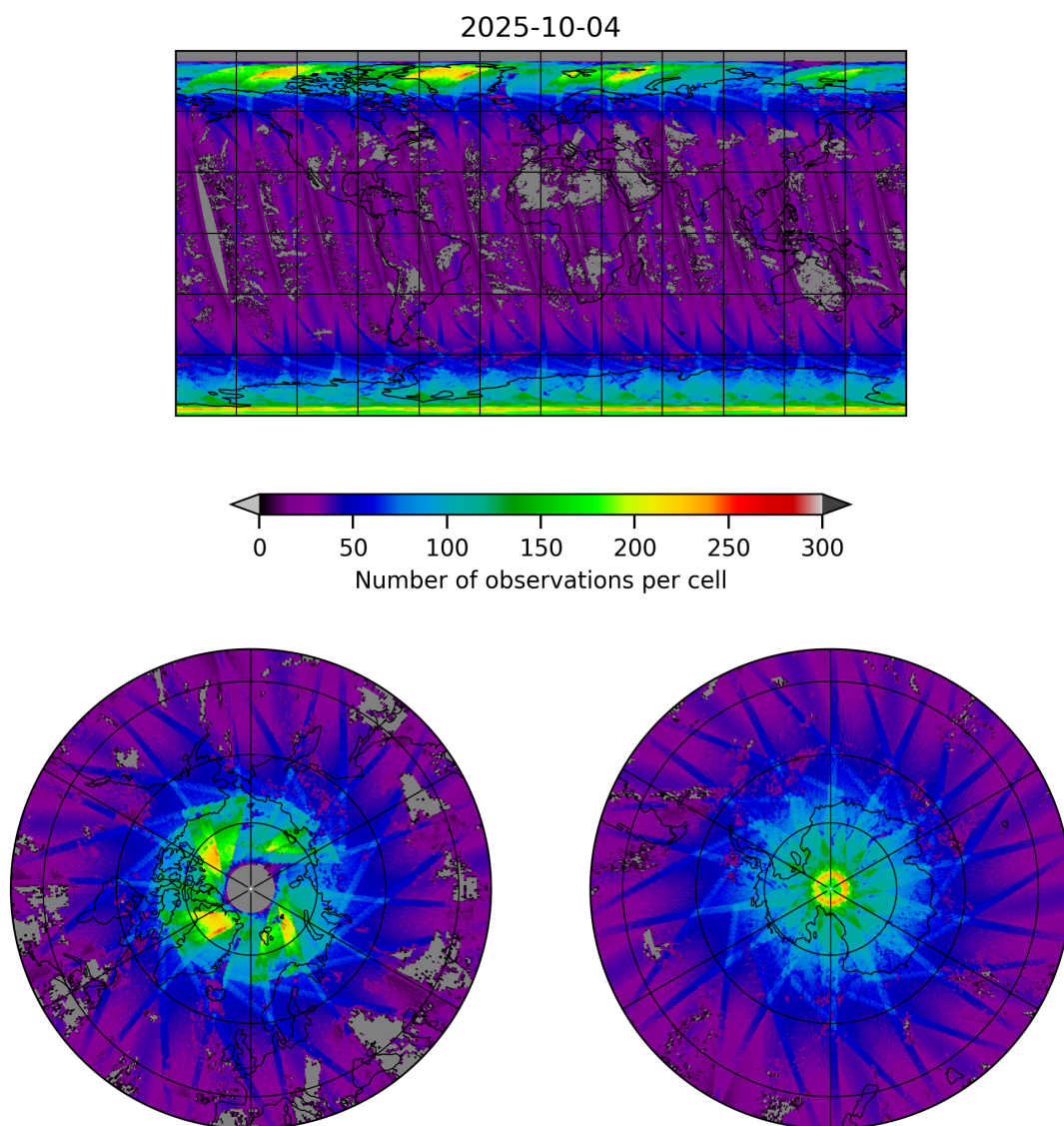
Figure 19: Map of the number of observations for 2025-10-04 to 2025-10-04
