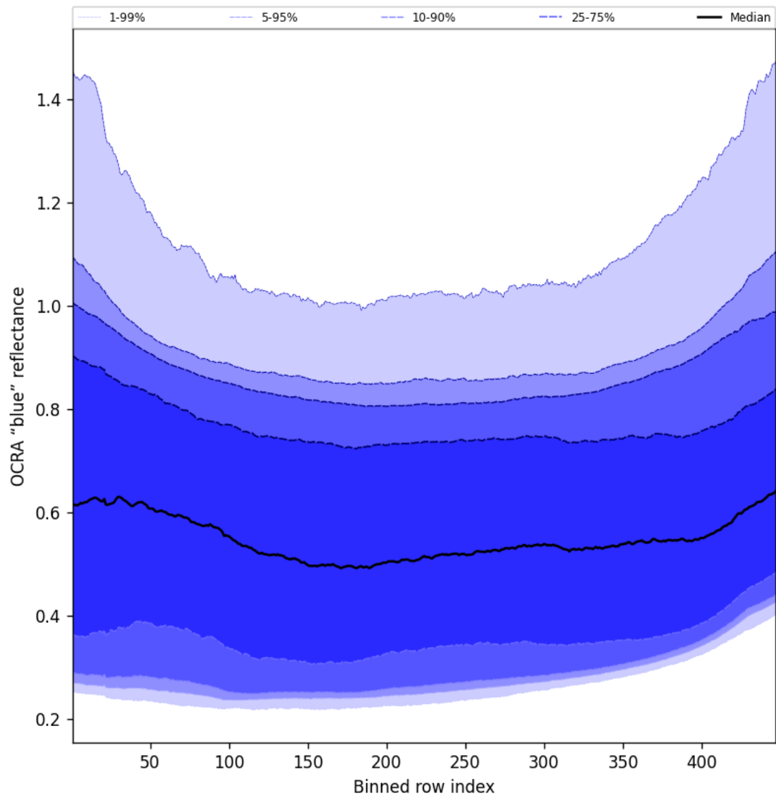
Figure 65: Along track statistics of “OCRA “blue” reflectance” for 2025-10-04 to 2025-10-04
