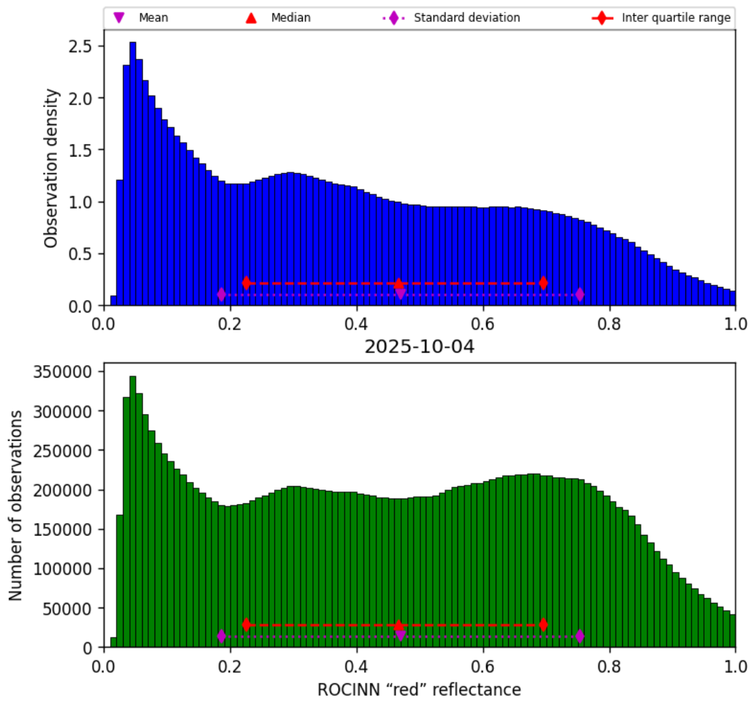
Figure 51: Histogram of “ROCINN “red” reflectance” for 2025-10-04 to 2025-10-04
