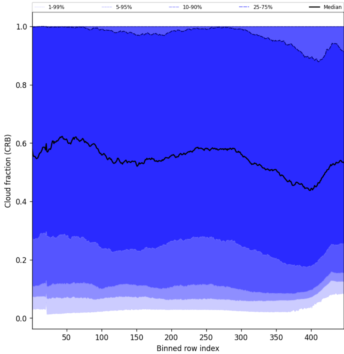
Figure 56: Along track statistics of “Cloud fraction (CRB)” for 2025-10-04 to 2025-10-04
