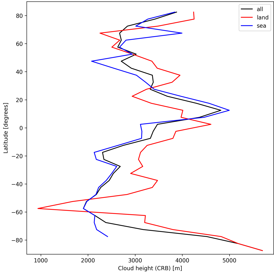
Figure 25: Zonal average of “Cloud height (CRB)” for 2025-10-04 to 2025-10-04.
