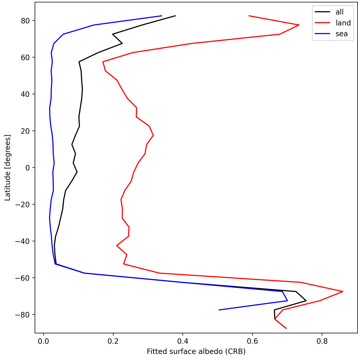
Figure 28: Zonal average of “Fitted surface albedo (CRB)” for 2025-10-04 to 2025-10-04.
