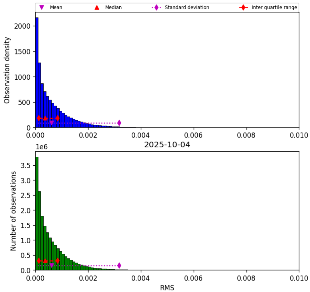
Figure 45: Histogram of “RMS” for 2025-10-04 to 2025-10-04
