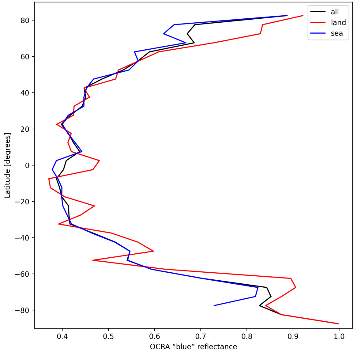
Figure 33: Zonal average of “OCRA “blue” reflectance” for 2025-10-04 to 2025-10-04.
