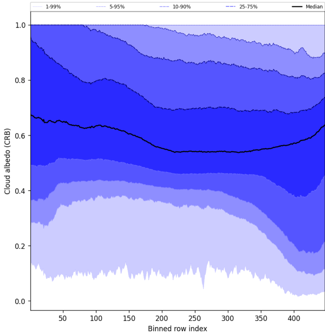
Figure 58: Along track statistics of “Cloud albedo (CRB)” for 2025-10-04 to 2025-10-04
