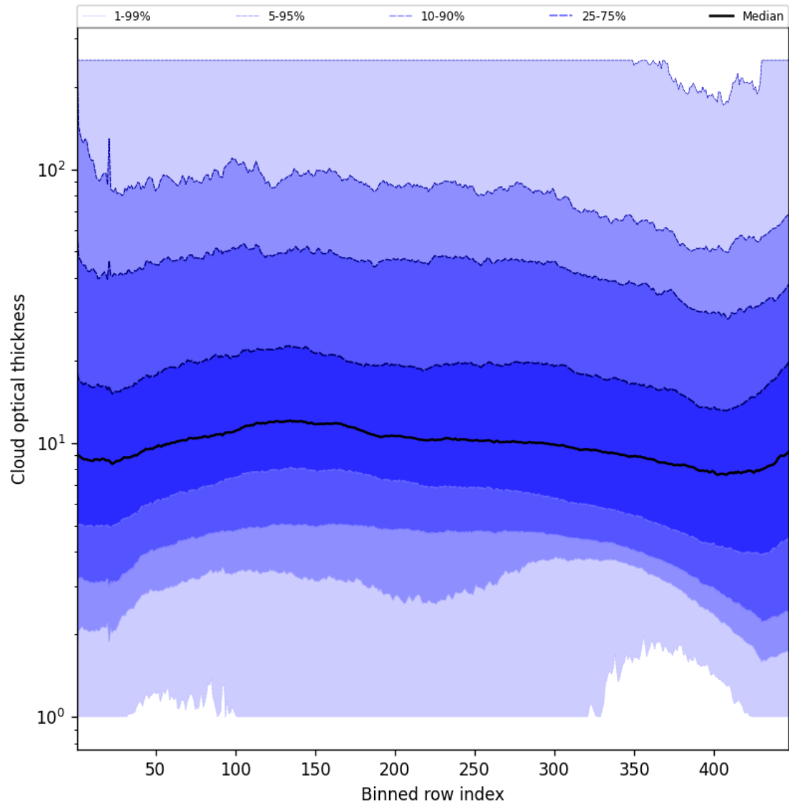
Figure 55: Along track statistics of “Cloud optical thickness” for 2025-10-04 to 2025-10-04
