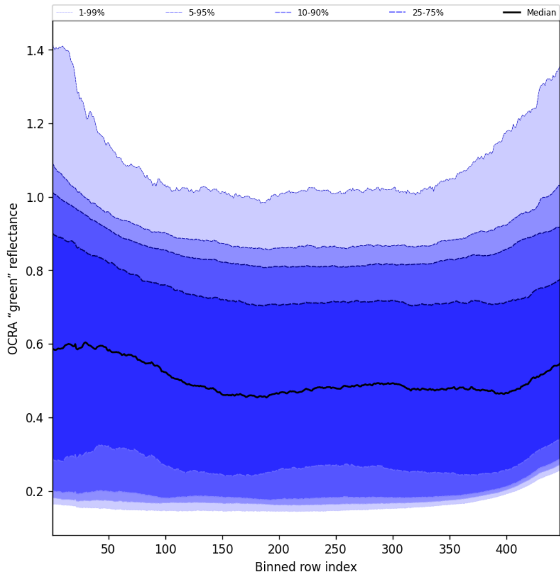
Figure 66: Along track statistics of “OCRA “green” reflectance” for 2025-10-04 to 2025-10-04
