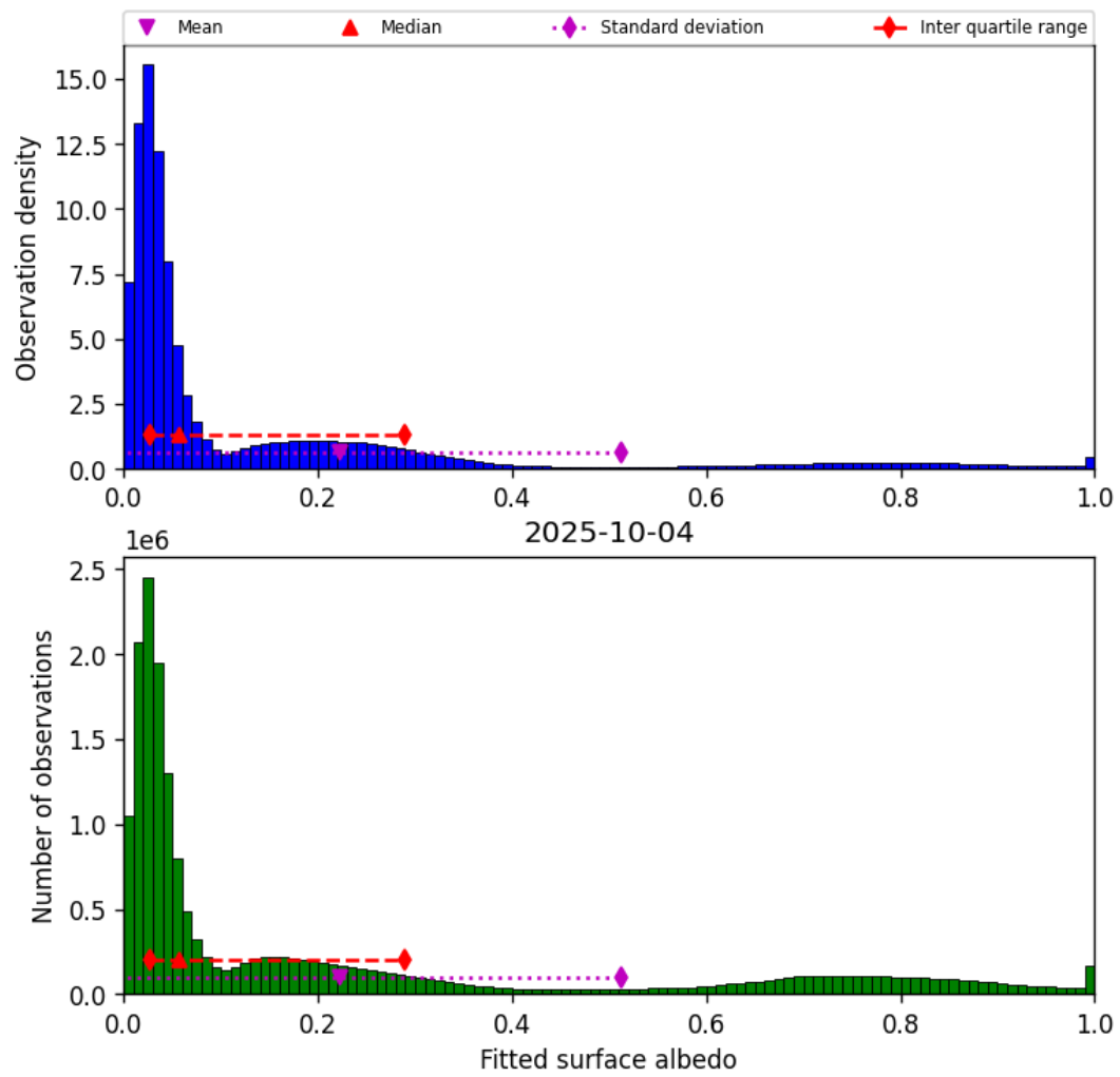
Figure 43: Histogram of “Fitted surface albedo” for 2025-10-04 to 2025-10-04
