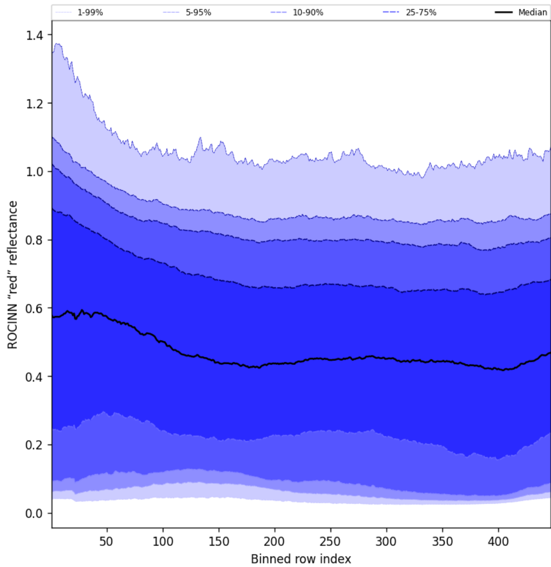
Figure 67: Along track statistics of “ROCINN “red” reflectance” for 2025-10-04 to 2025-10-04
