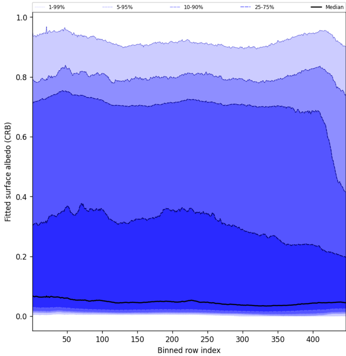
Figure 60: Along track statistics of “Fitted surface albedo (CRB)” for 2025-10-04 to 2025-10-04
