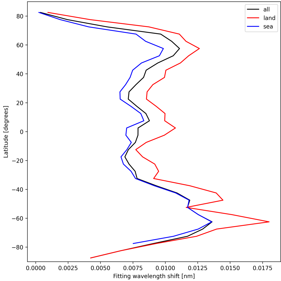
Figure 31: Zonal average of “Fitting wavelength shift” for 2025-10-04 to 2025-10-04.
