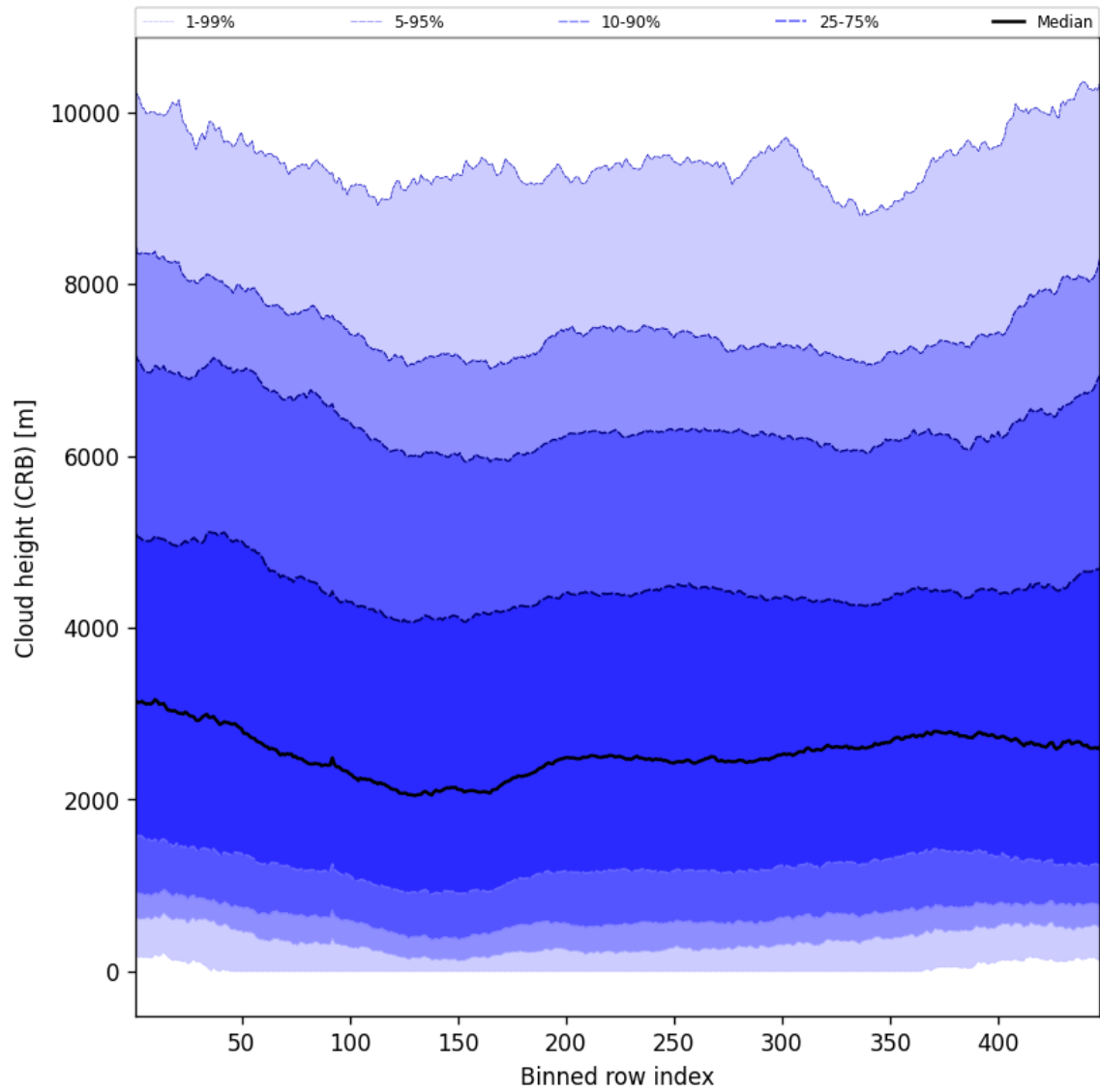
Figure 57: Along track statistics of “Cloud height (CRB)” for 2025-10-04 to 2025-10-04
