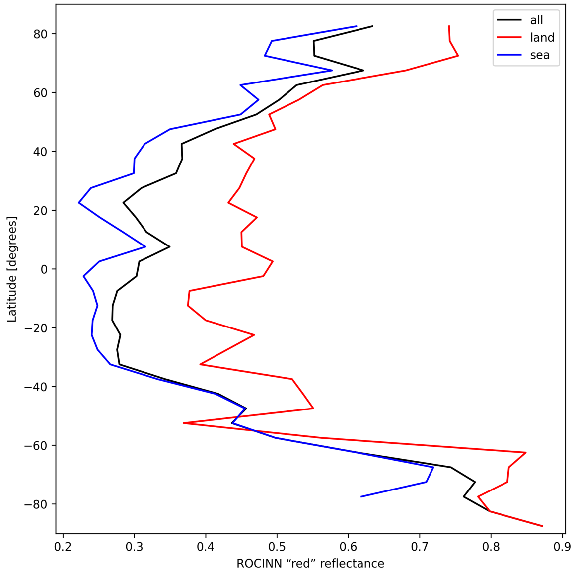
Figure 35: Zonal average of “ROCINN “red” reflectance” for 2025-10-04 to 2025-10-04.
