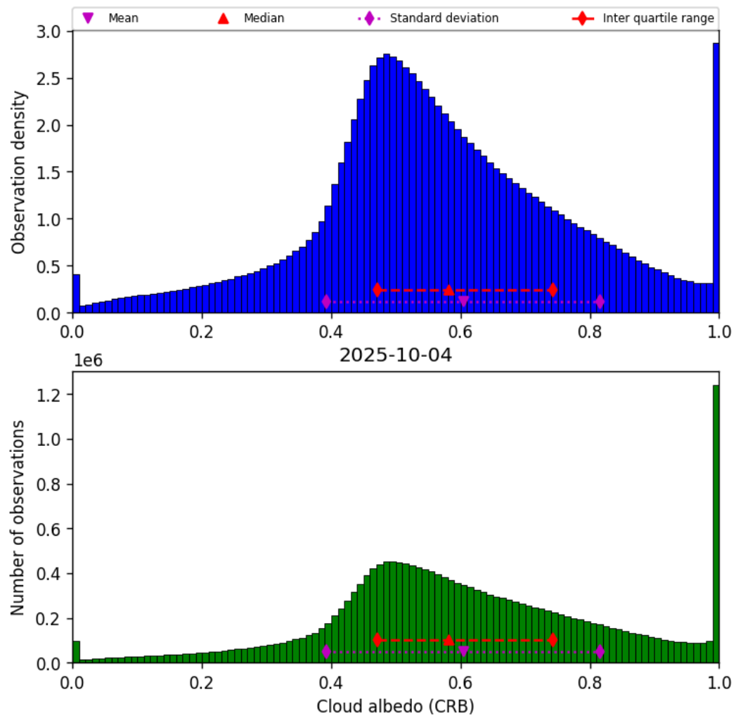
Figure 42: Histogram of “Cloud albedo (CRB)” for 2025-10-04 to 2025-10-04
