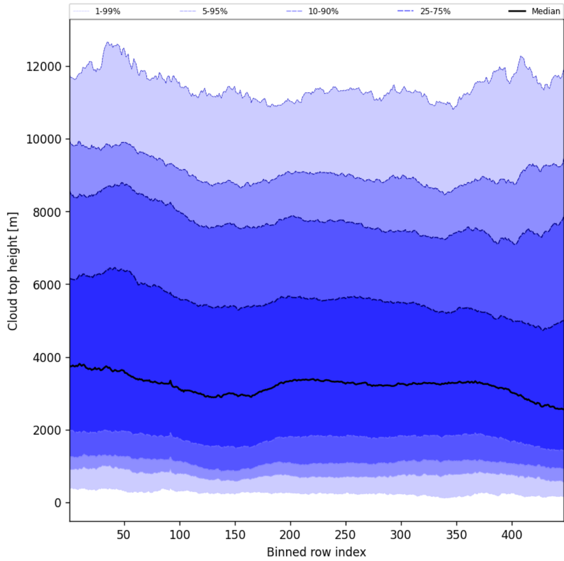
Figure 54: Along track statistics of “Cloud top height” for 2025-10-04 to 2025-10-04
