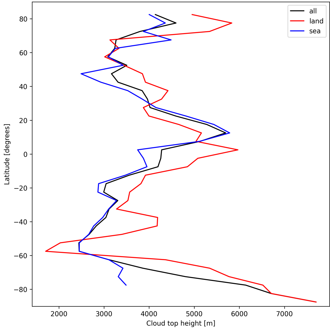
Figure 22: Zonal average of “Cloud top height” for 2025-10-04 to 2025-10-04.
