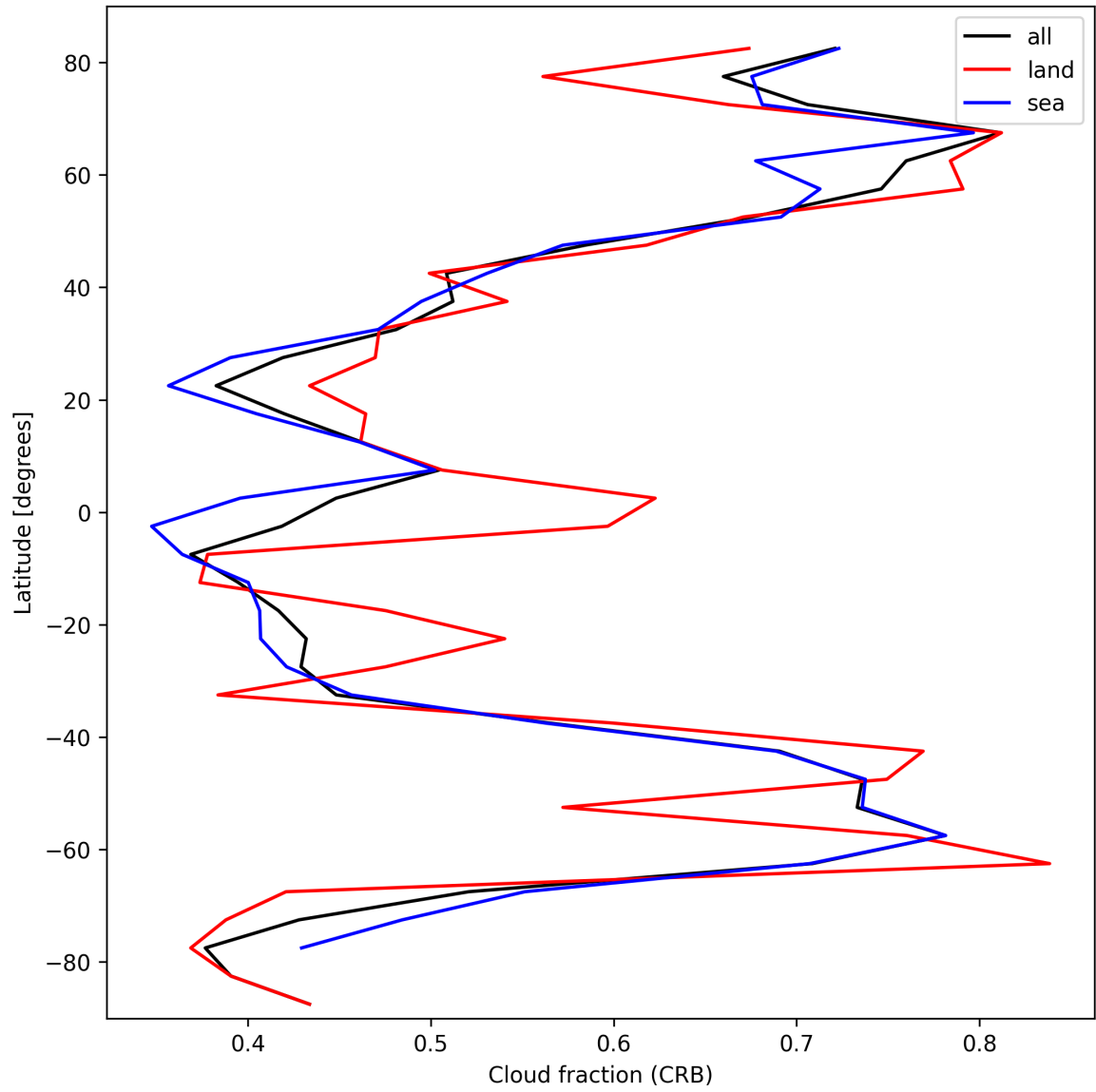
Figure 24: Zonal average of “Cloud fraction (CRB)” for 2025-10-04 to 2025-10-04.
