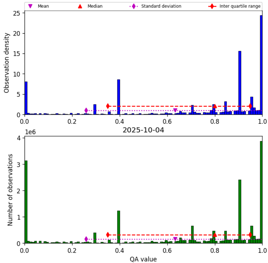
Figure 36: Histogram of “QA value” for 2025-10-04 to 2025-10-04
