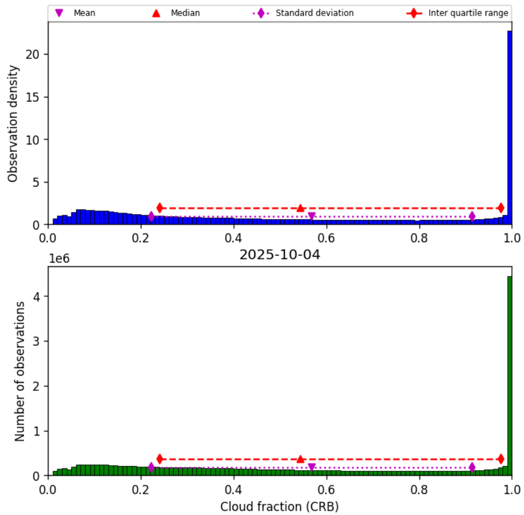
Figure 40: Histogram of "Cloud fraction (CRB)" for 2025-10-04 to 2025-10-04
