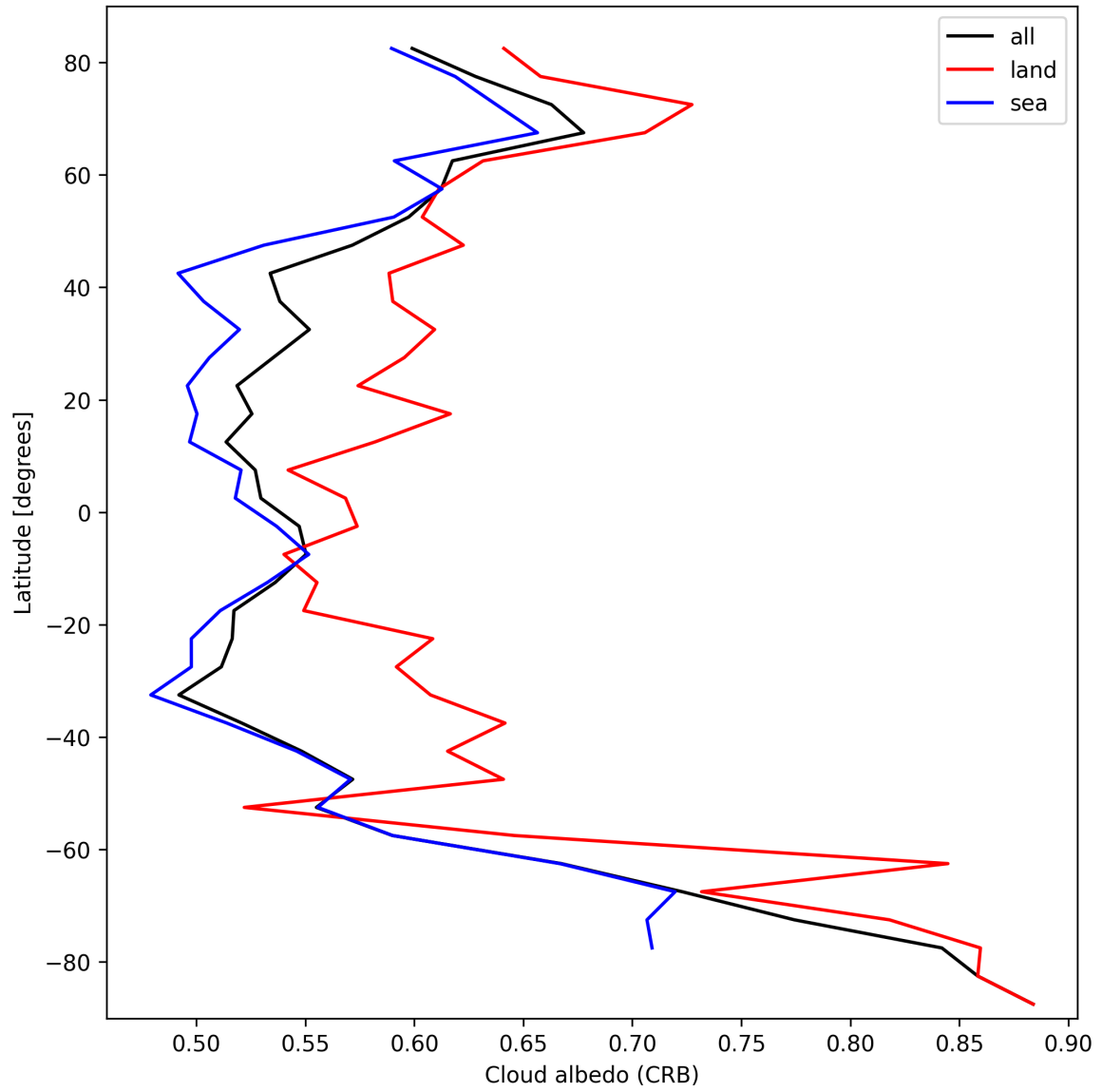
Figure 26: Zonal average of “Cloud albedo (CRB)” for 2025-10-04 to 2025-10-04.
