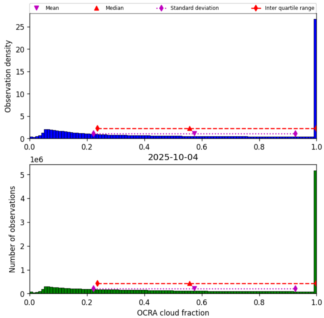
Figure 48: Histogram of “OCRA cloud fraction” for 2025-10-04 to 2025-10-04
