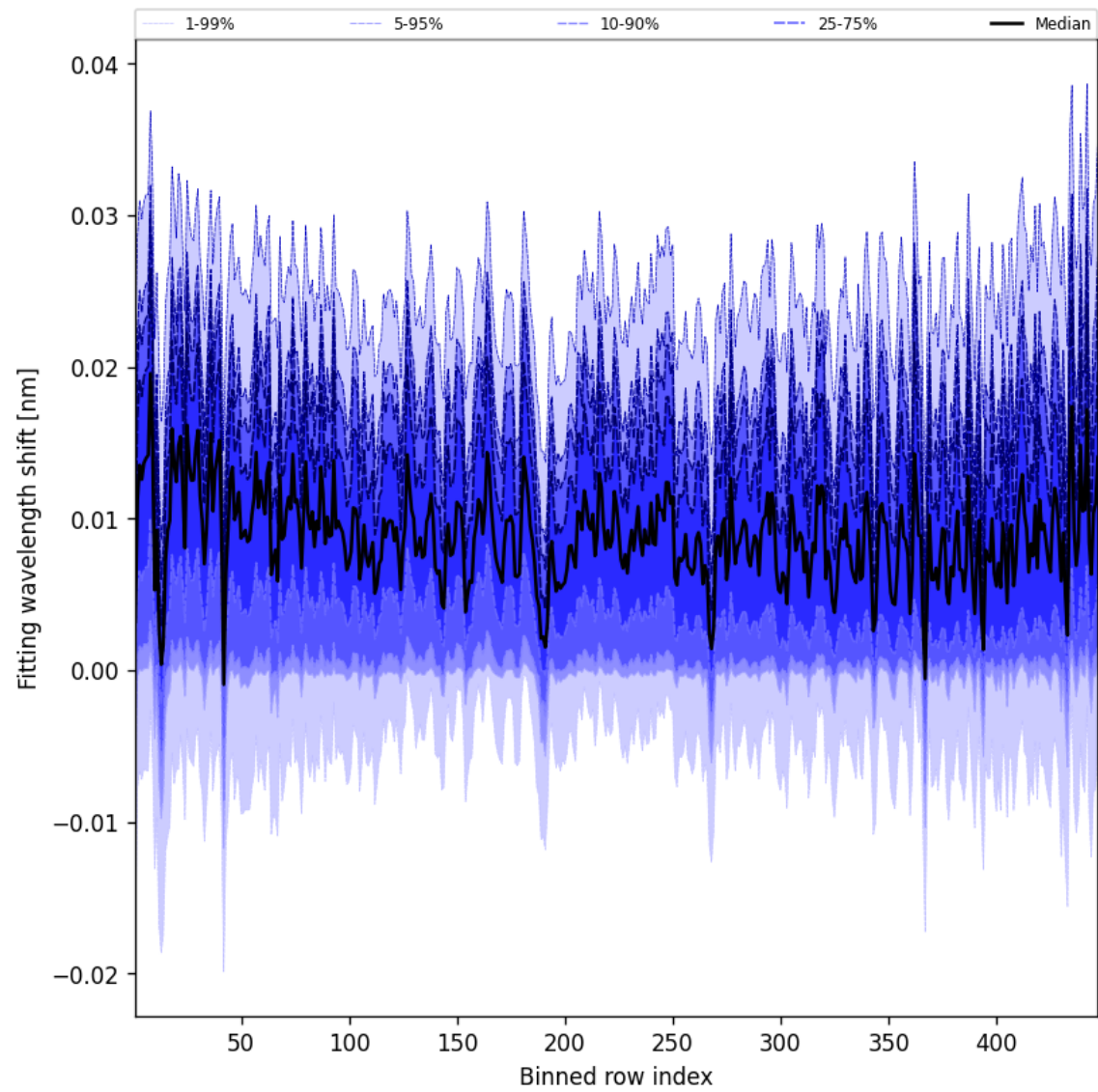
Figure 63: Along track statistics of “Fitting wavelength shift” for 2025-10-04 to 2025-10-04
