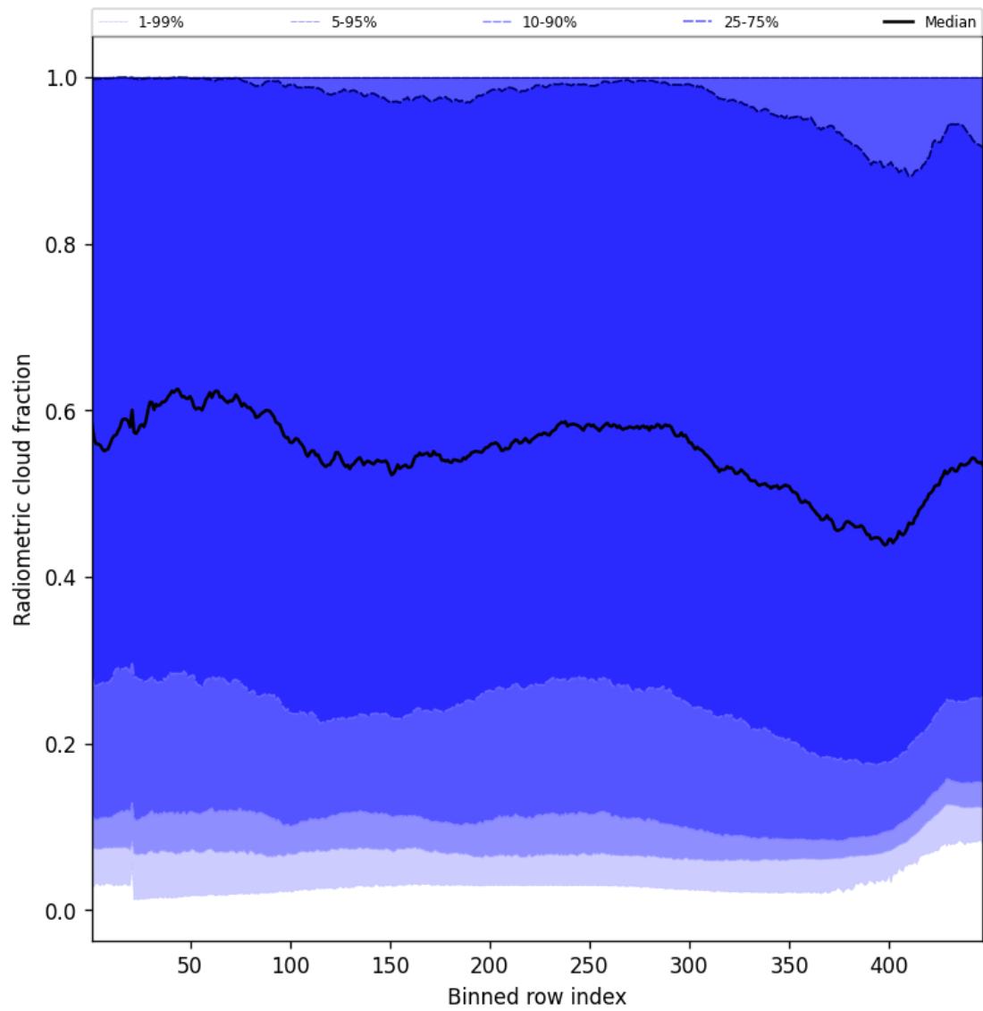
Figure 53: Along track statistics of “Radiometric cloud fraction” for 2025-10-04 to 2025-10-04
