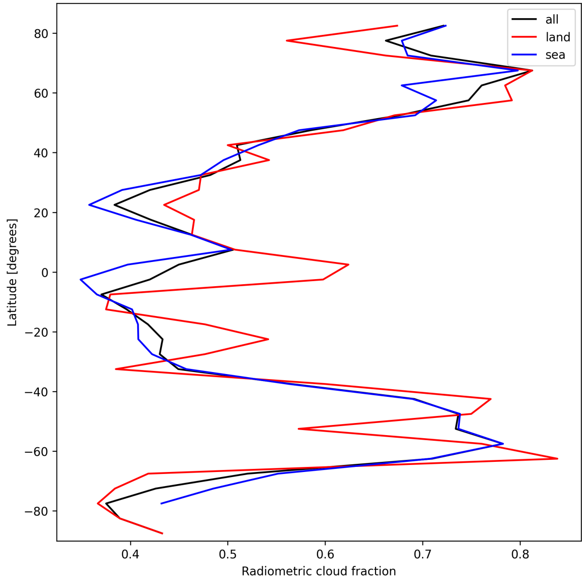
Figure 21: Zonal average of “Radiometric cloud fraction” for 2025-10-04 to 2025-10-04.
