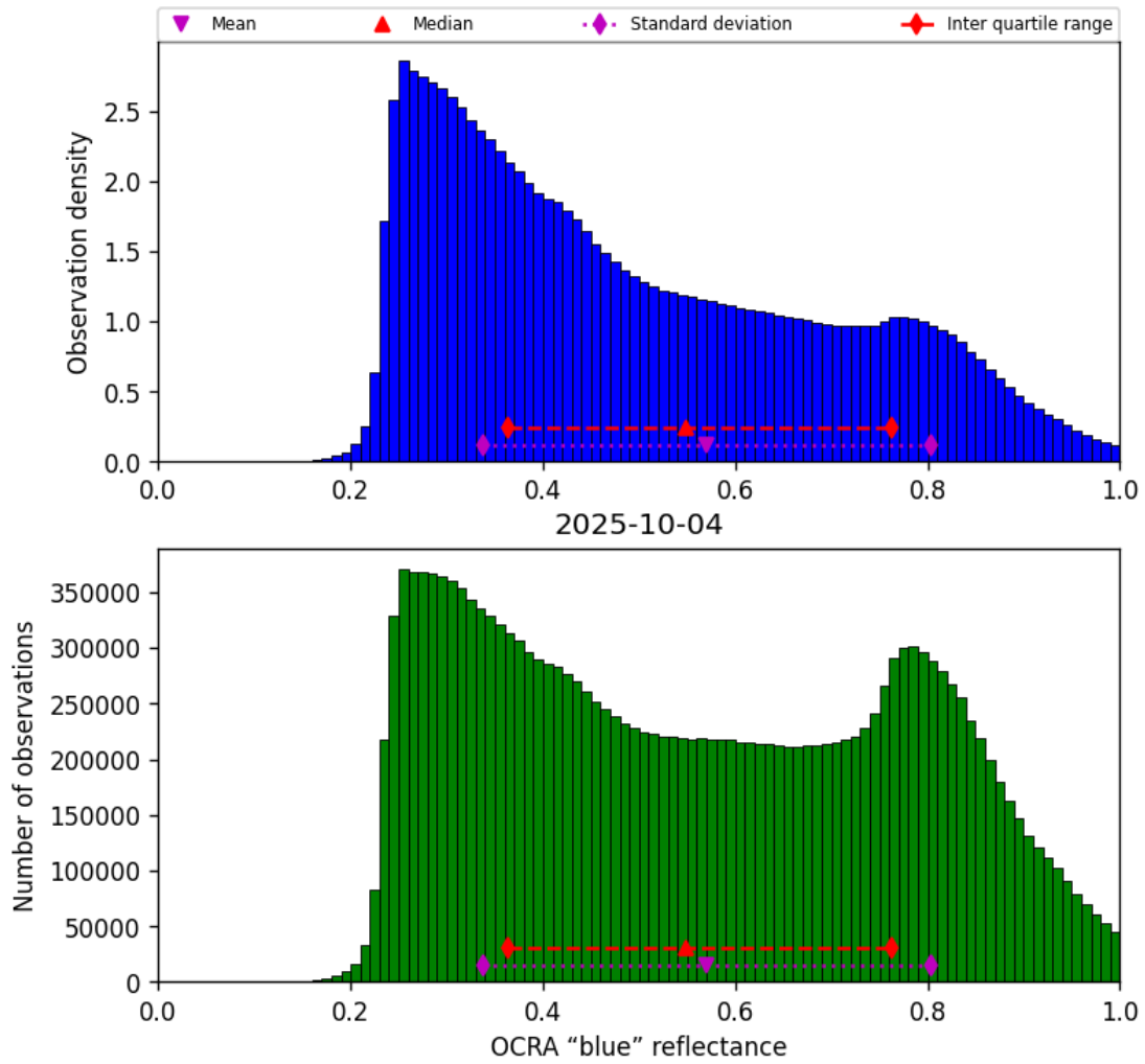
Figure 49: Histogram of “OCRA “blue” reflectance” for 2025-10-04 to 2025-10-04
