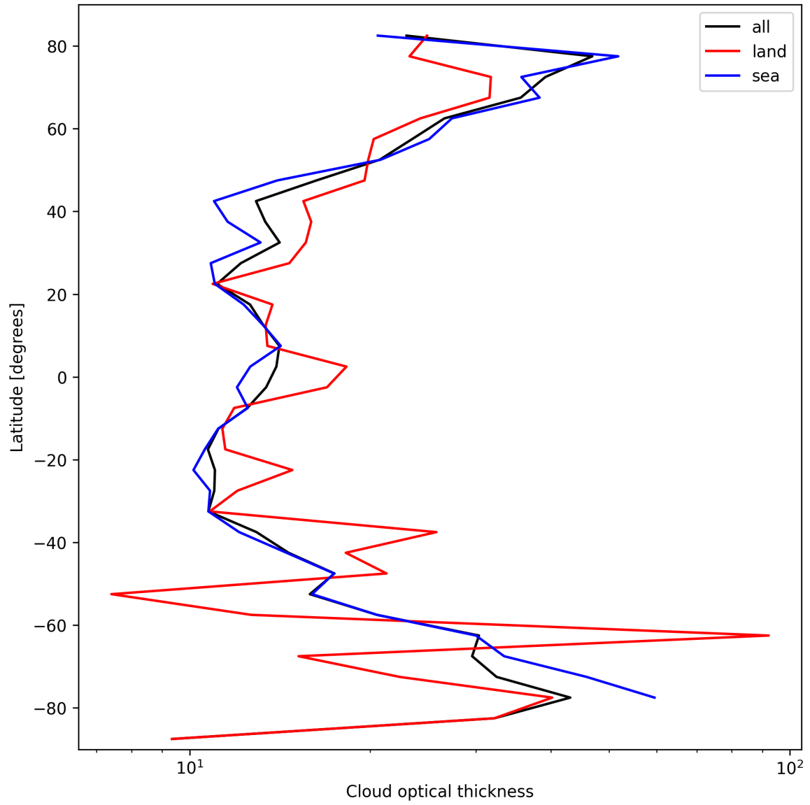
Figure 23: Zonal average of “Cloud optical thickness” for 2025-10-04 to 2025-10-04.
