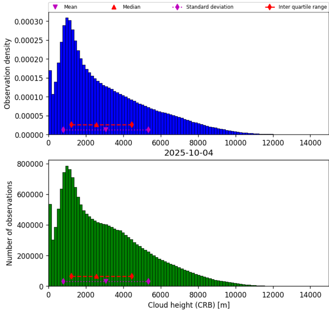
Figure 41: Histogram of “Cloud height (CRB)” for 2025-10-04 to 2025-10-04
