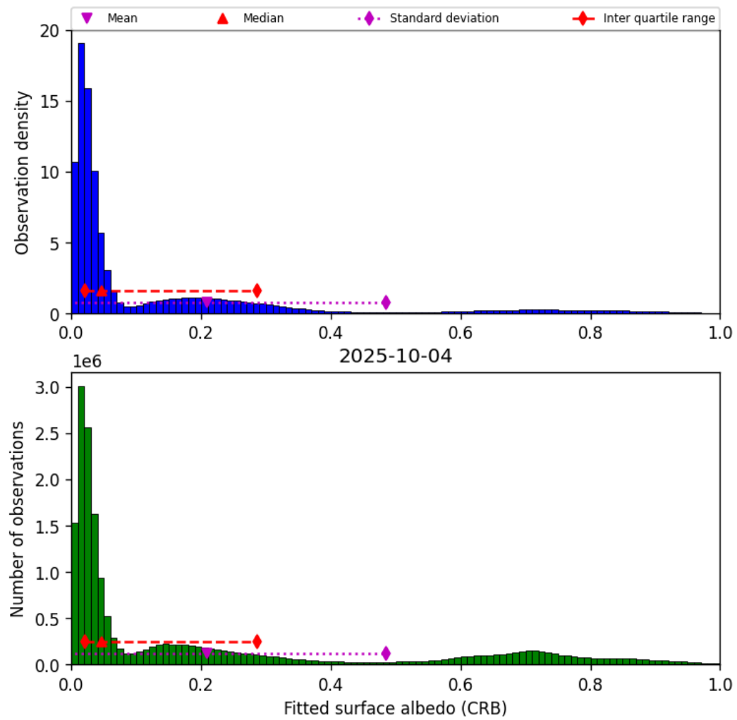
Figure 44: Histogram of “Fitted surface albedo (CRB)” for 2025-10-04 to 2025-10-04
