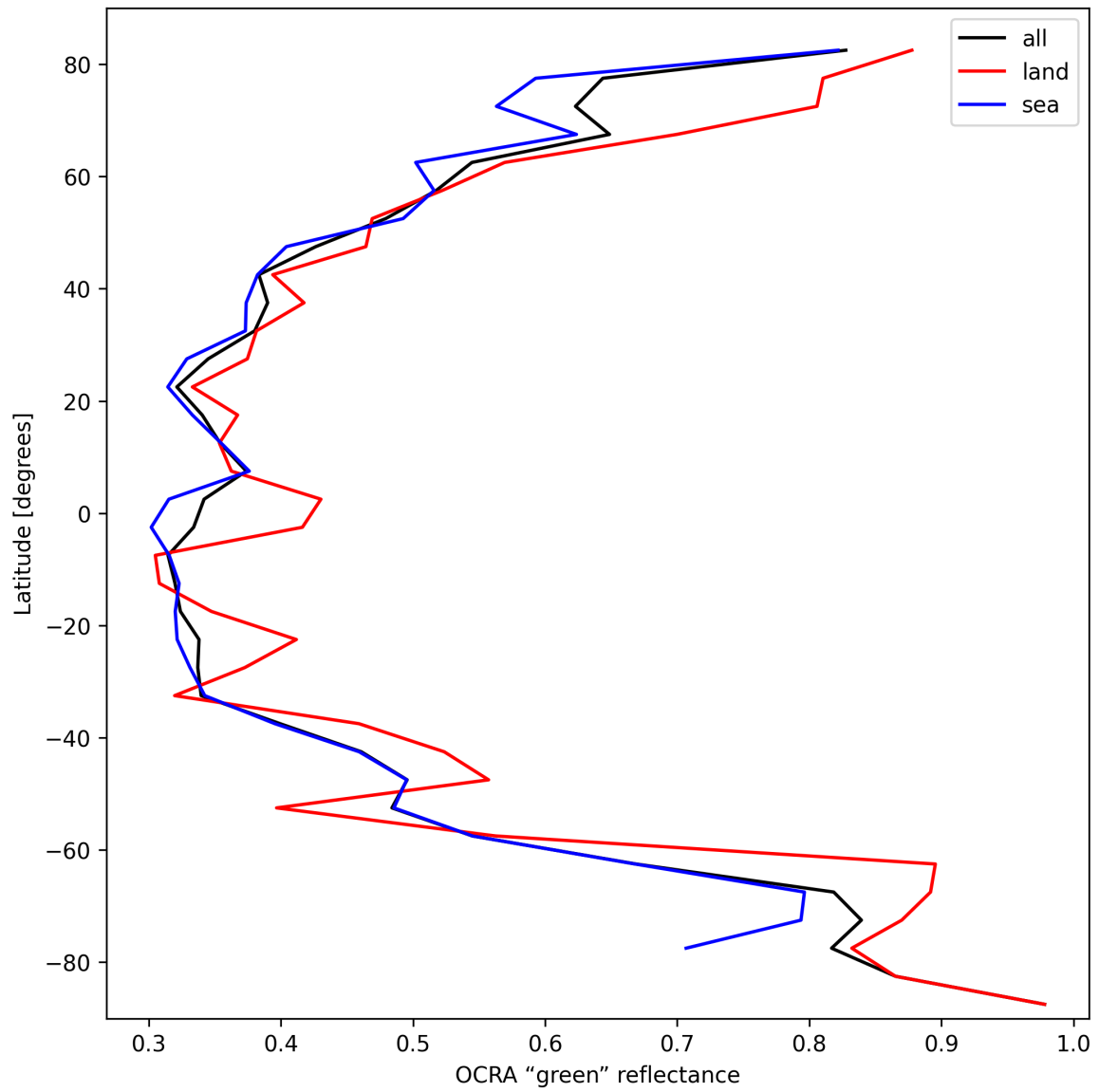
Figure 34: Zonal average of “OCRA “green” reflectance” for 2025-10-04 to 2025-10-04.
