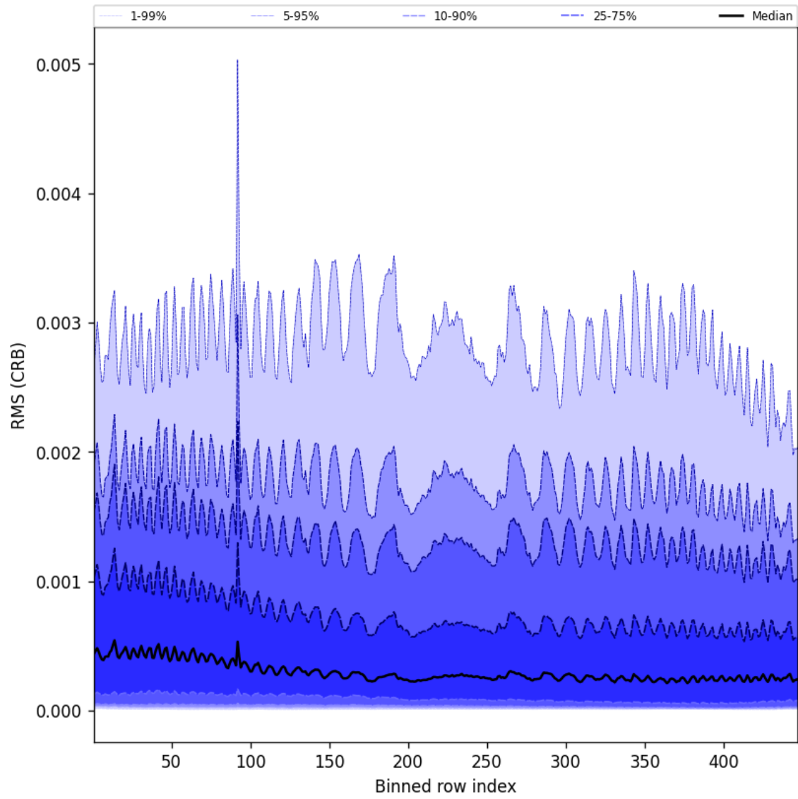
Figure 62: Along track statistics of “RMS (CRB)” for 2025-10-04 to 2025-10-04
