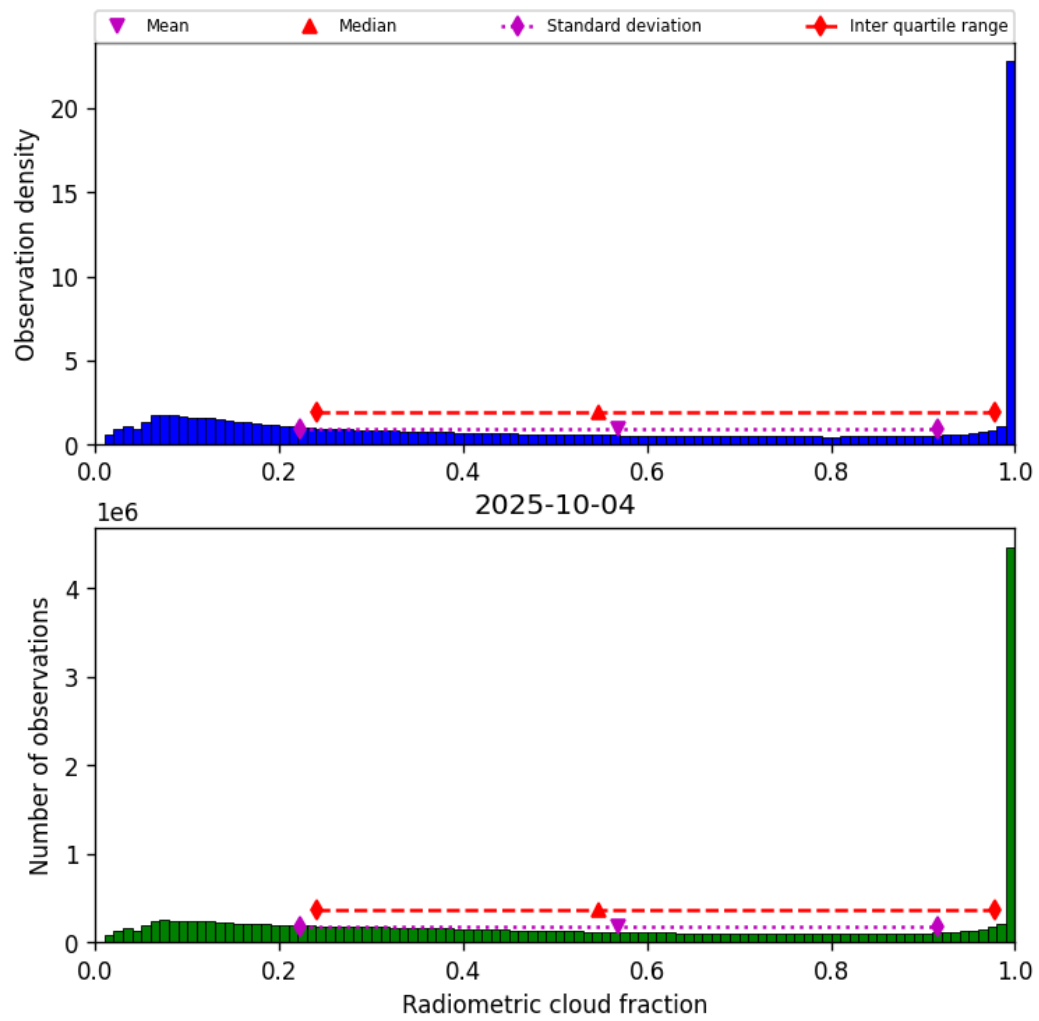
Figure 37: Histogram of “Radiometric cloud fraction” for 2025-10-04 to 2025-10-04
