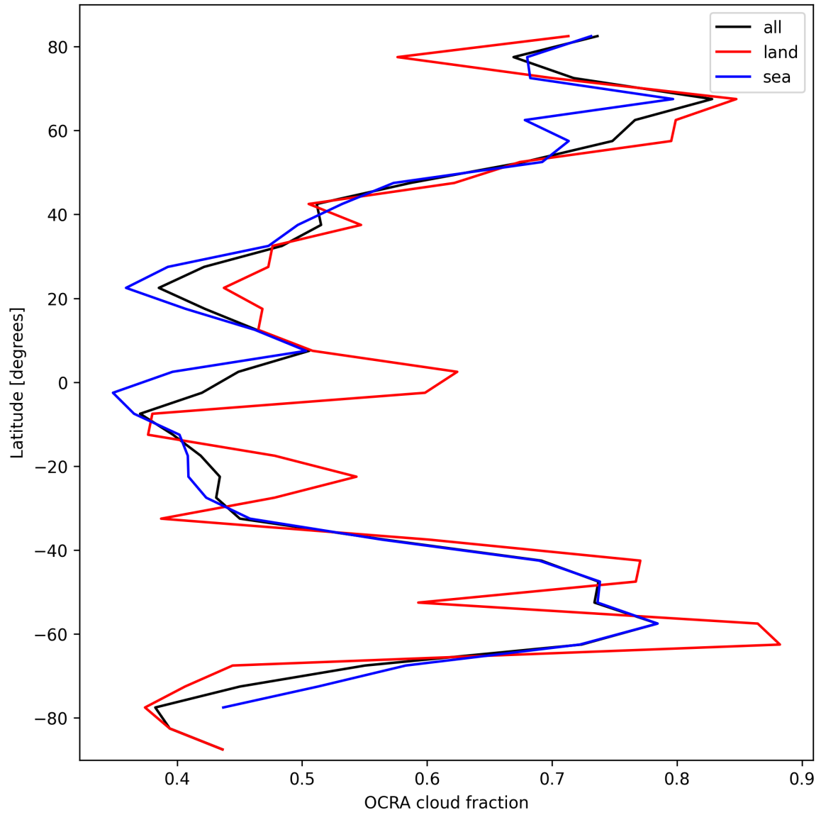
Figure 32: Zonal average of “OCRA cloud fraction” for 2025-10-04 to 2025-10-04.
