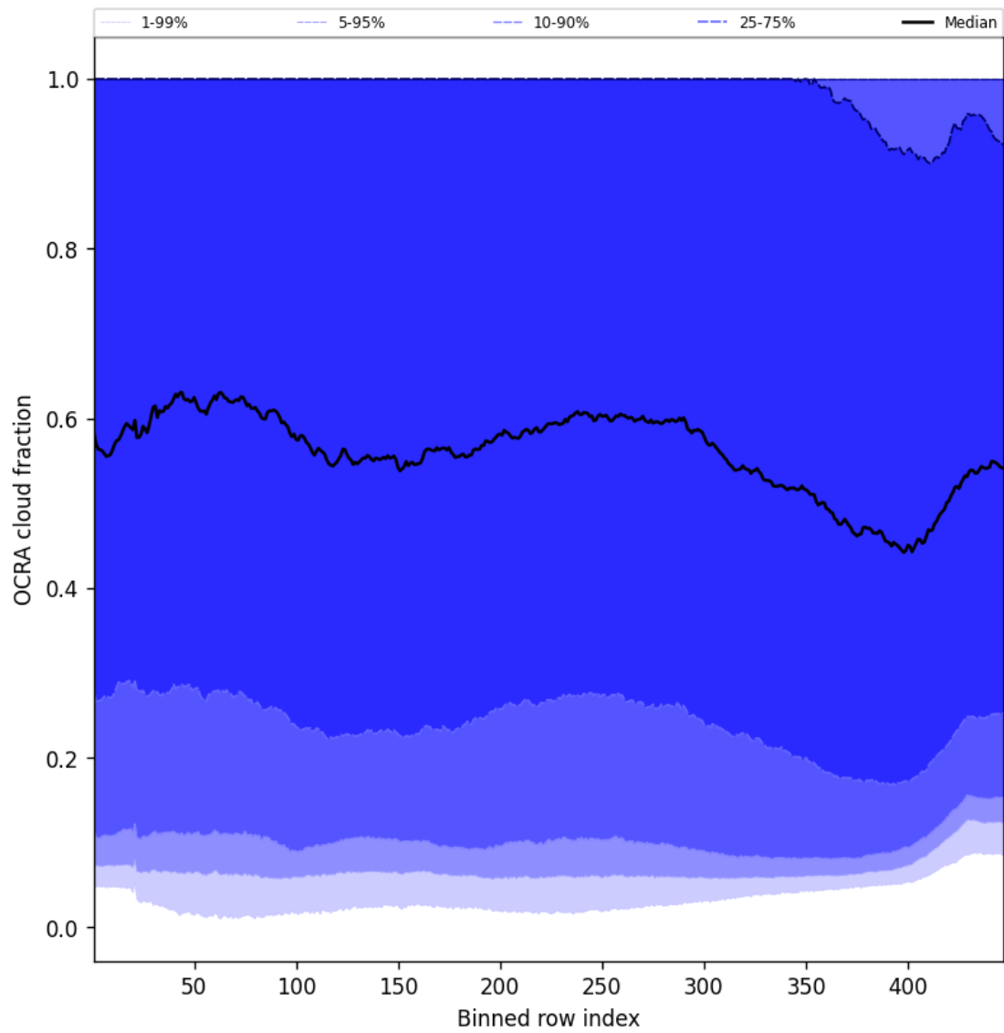
Figure 64: Along track statistics of “OCRA cloud fraction” for 2025-10-04 to 2025-10-04
