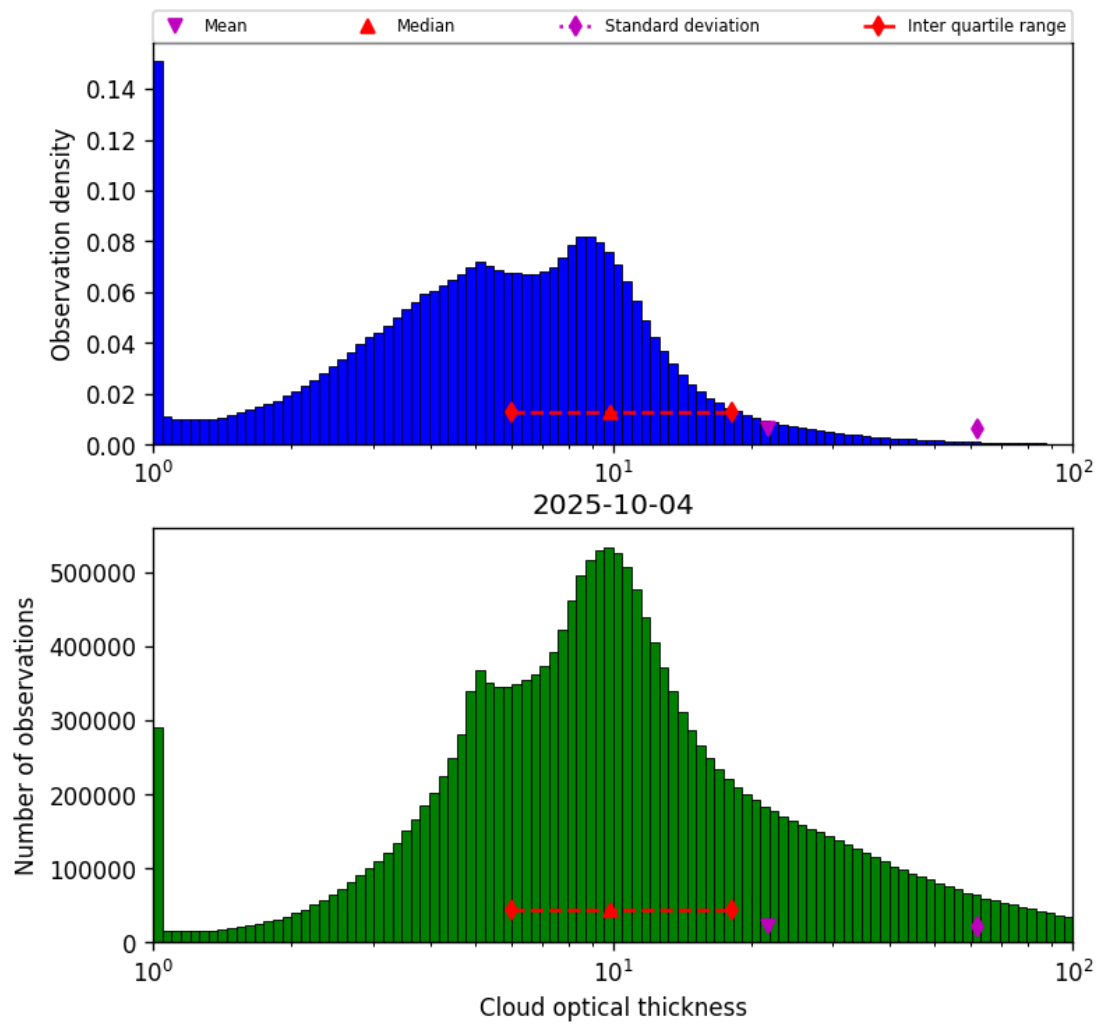
Figure 39: Histogram of “Cloud optical thickness” for 2025-10-04 to 2025-10-04
