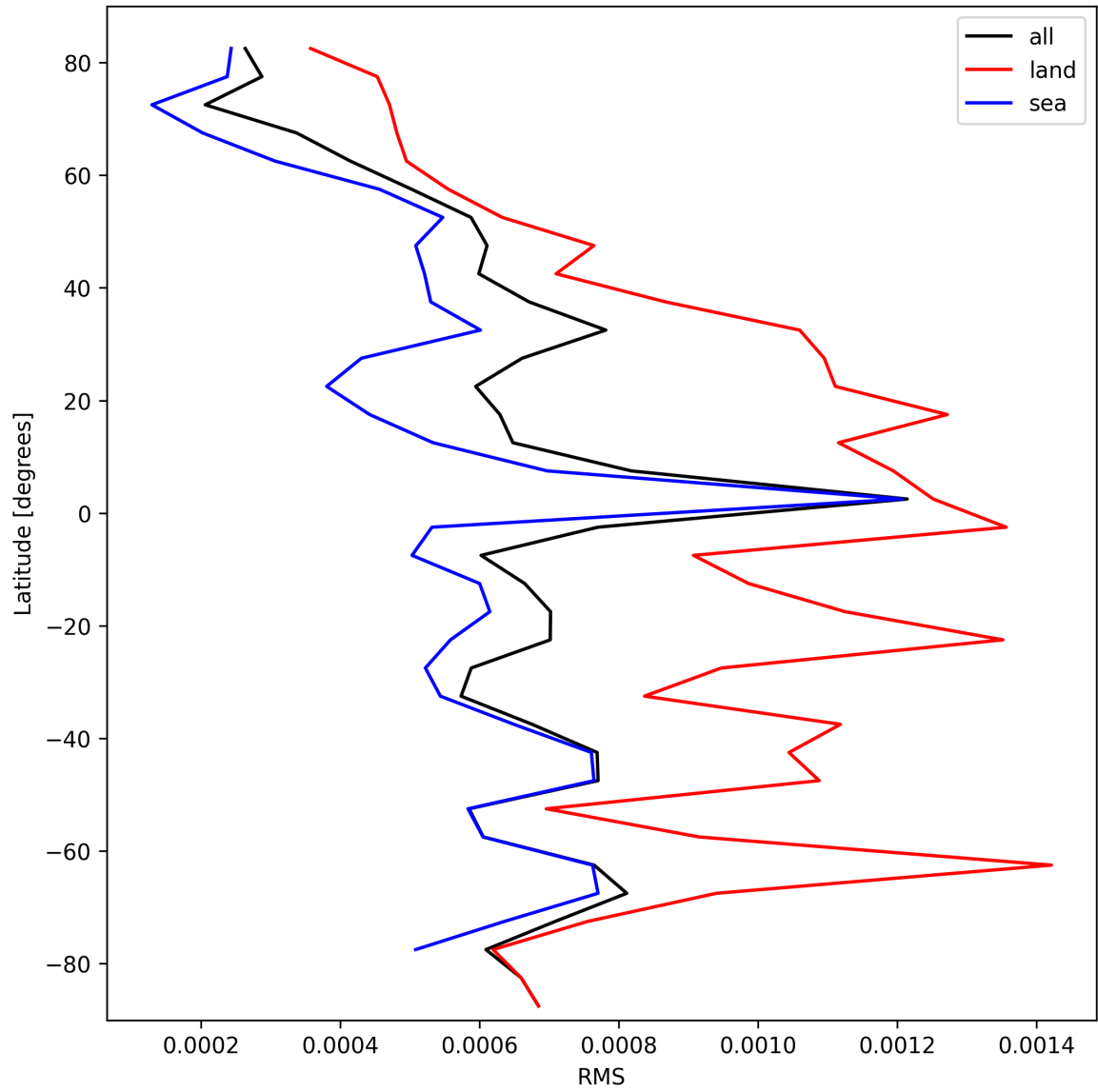
Figure 29: Zonal average of “RMS” for 2025-10-04 to 2025-10-04.
