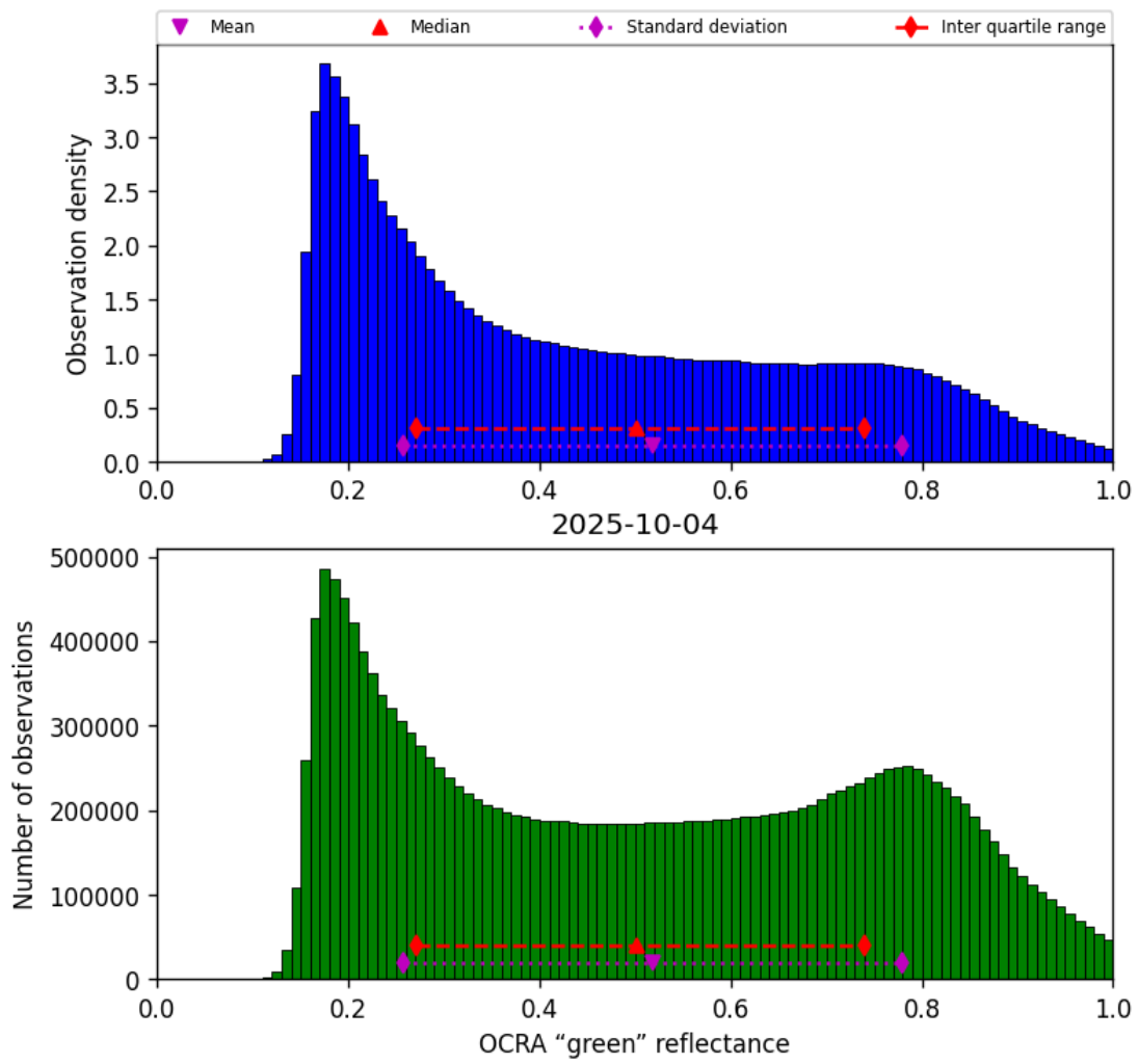
Figure 50: Histogram of “OCRA “green” reflectance” for 2025-10-04 to 2025-10-04
