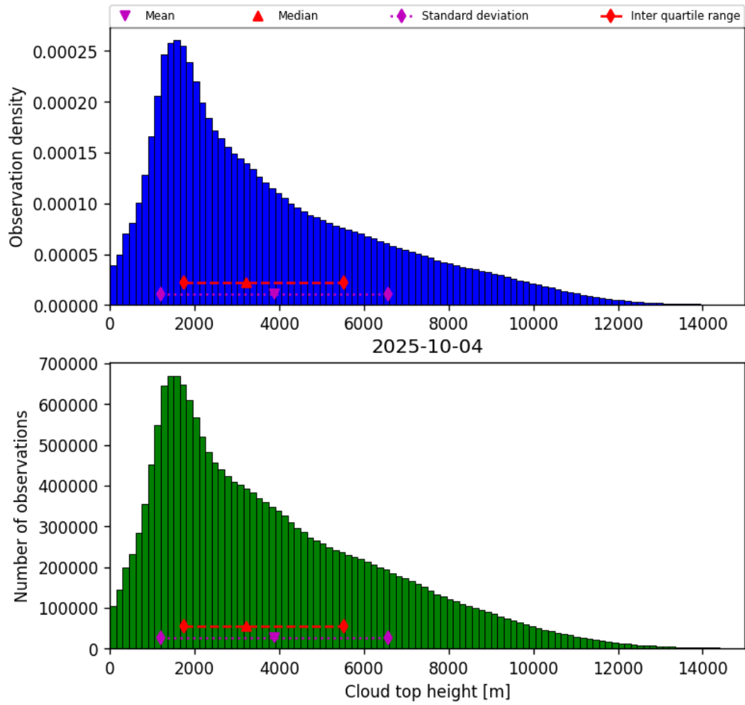
Figure 38: Histogram of “Cloud top height” for 2025-10-04 to 2025-10-04
