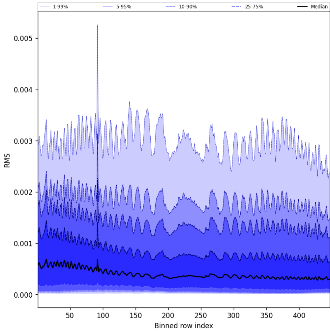
Figure 61: Along track statistics of “RMS” for 2025-10-04 to 2025-10-04
