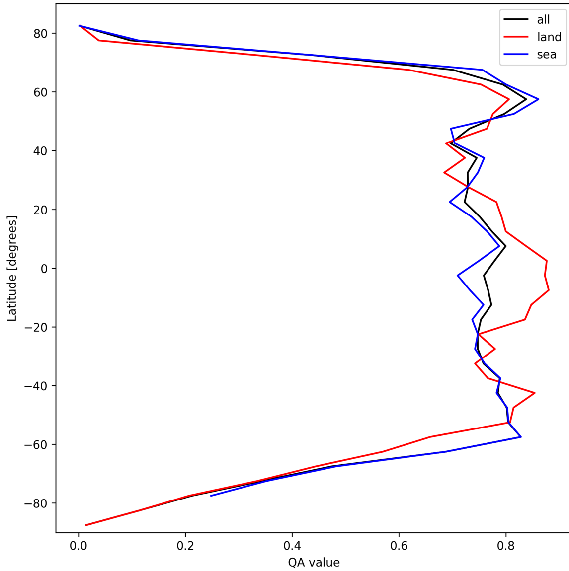
Figure 20: Zonal average of “QA value” for 2025-10-04 to 2025-10-04.
