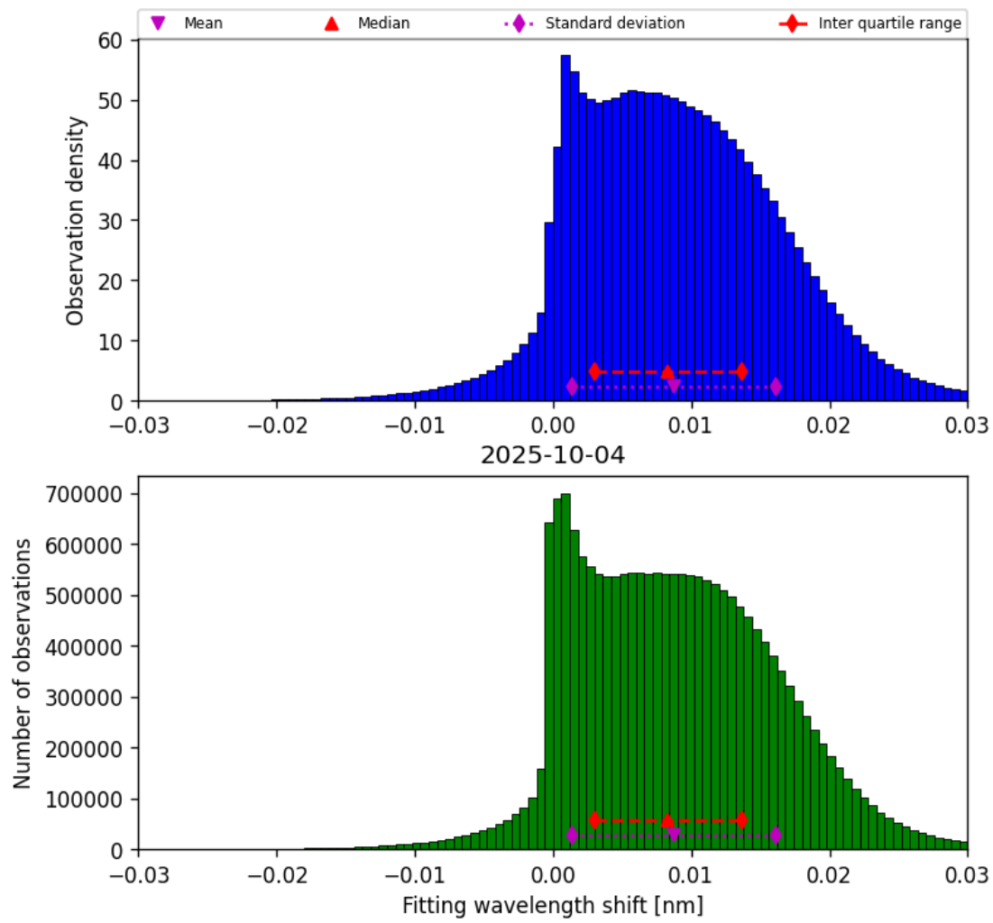
Figure 47: Histogram of “Fitting wavelength shift” for 2025-10-04 to 2025-10-04
