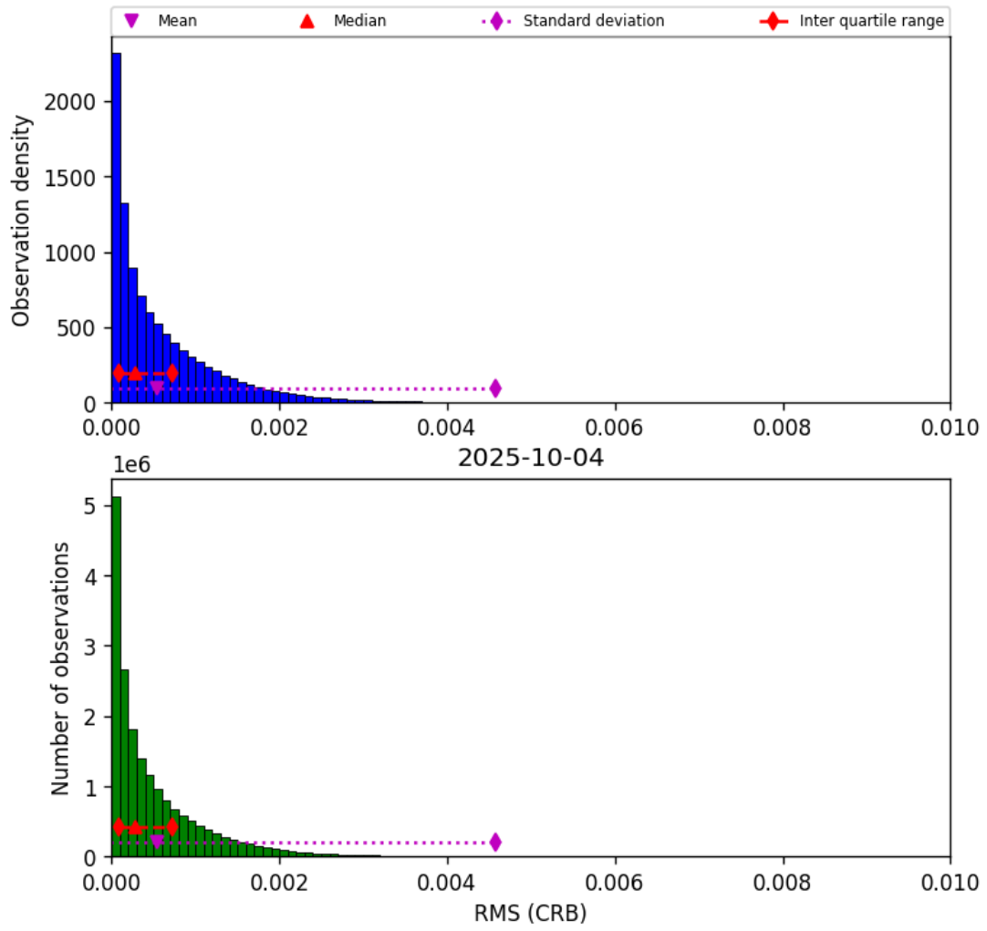
Figure 46: Histogram of “RMS (CRB)” for 2025-10-04 to 2025-10-04
