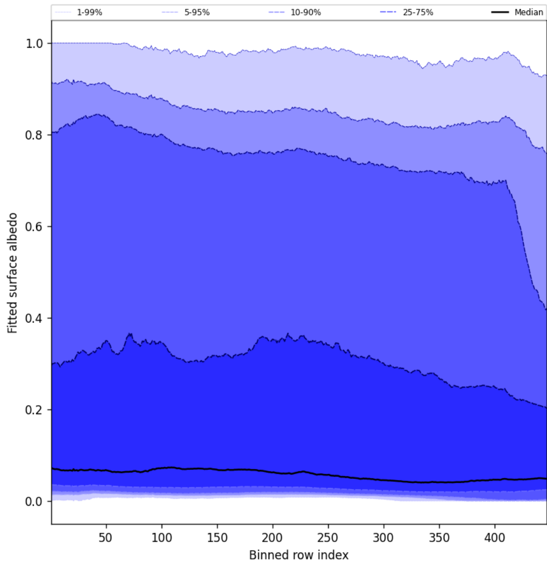
Figure 59: Along track statistics of “Fitted surface albedo” for 2025-10-04 to 2025-10-04
