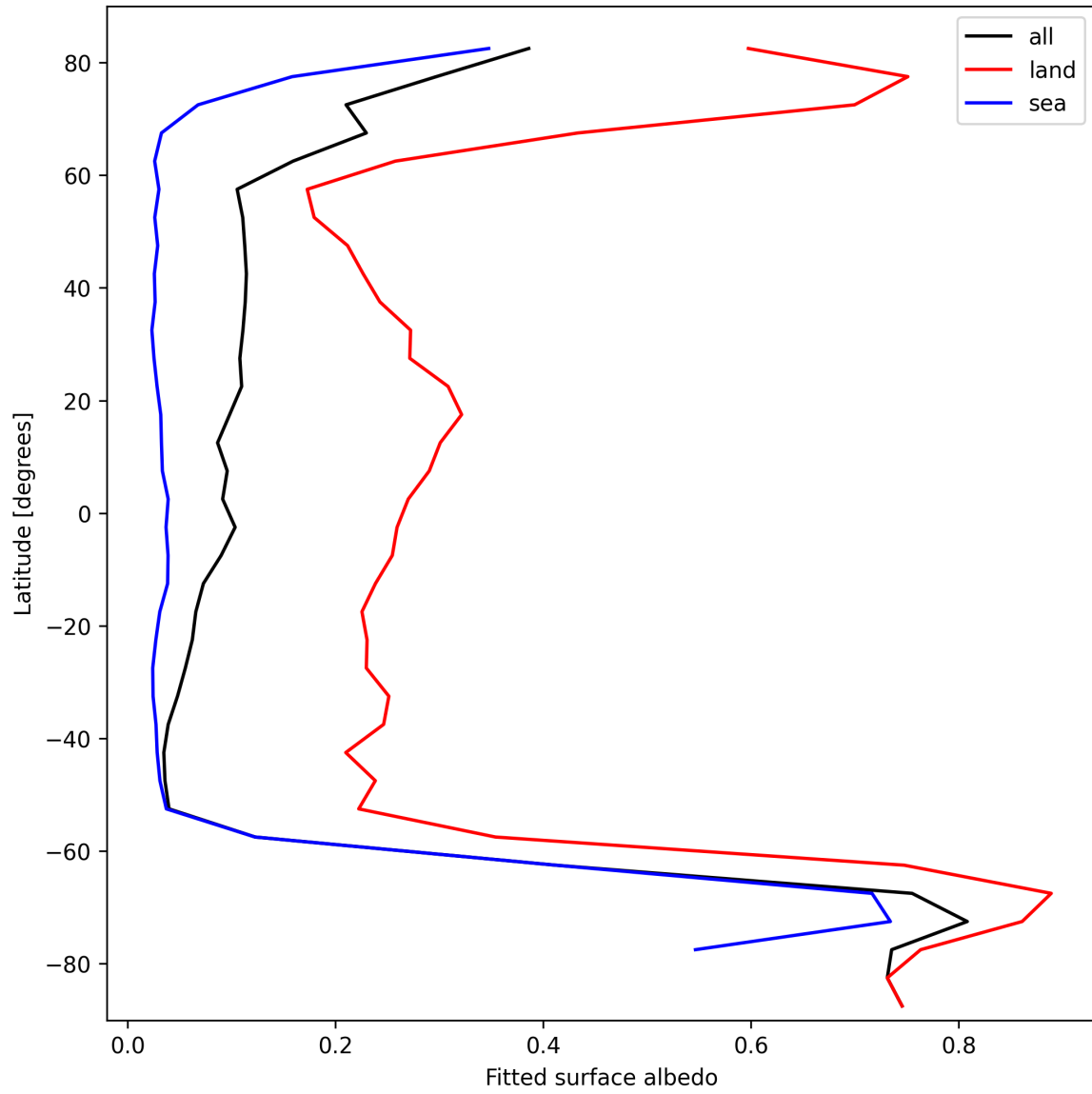
Figure 27: Zonal average of “Fitted surface albedo” for 2025-10-04 to 2025-10-04.
