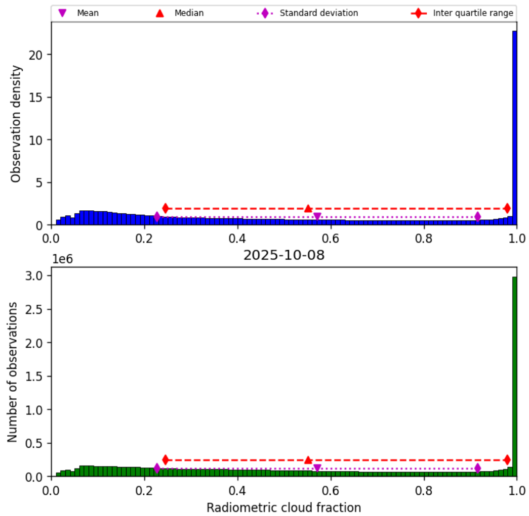
Figure 37: Histogram of “Radiometric cloud fraction” for 2025-10-08 to 2025-10-09
