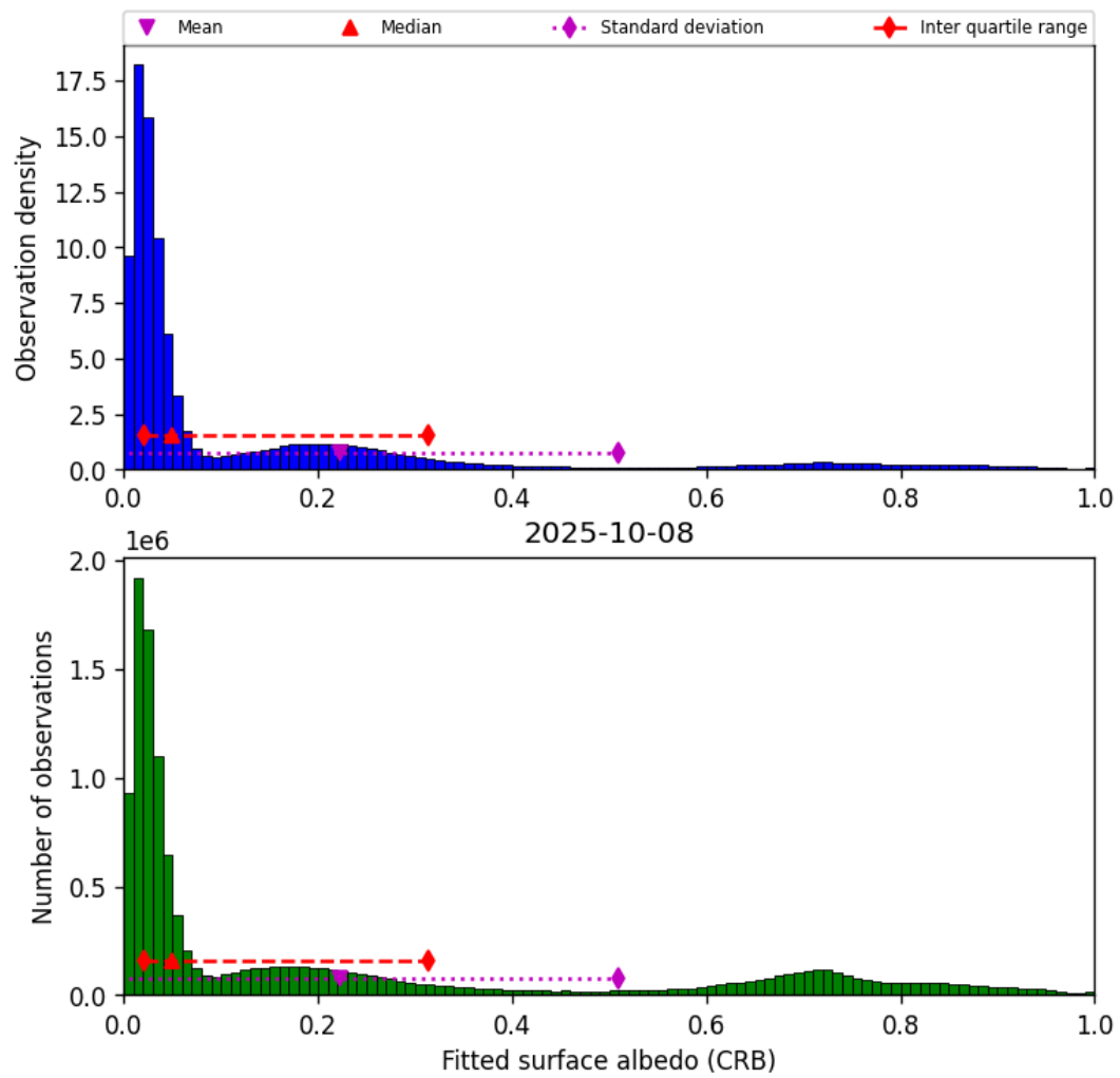
Figure 44: Histogram of “Fitted surface albedo (CRB)” for 2025-10-08 to 2025-10-09
