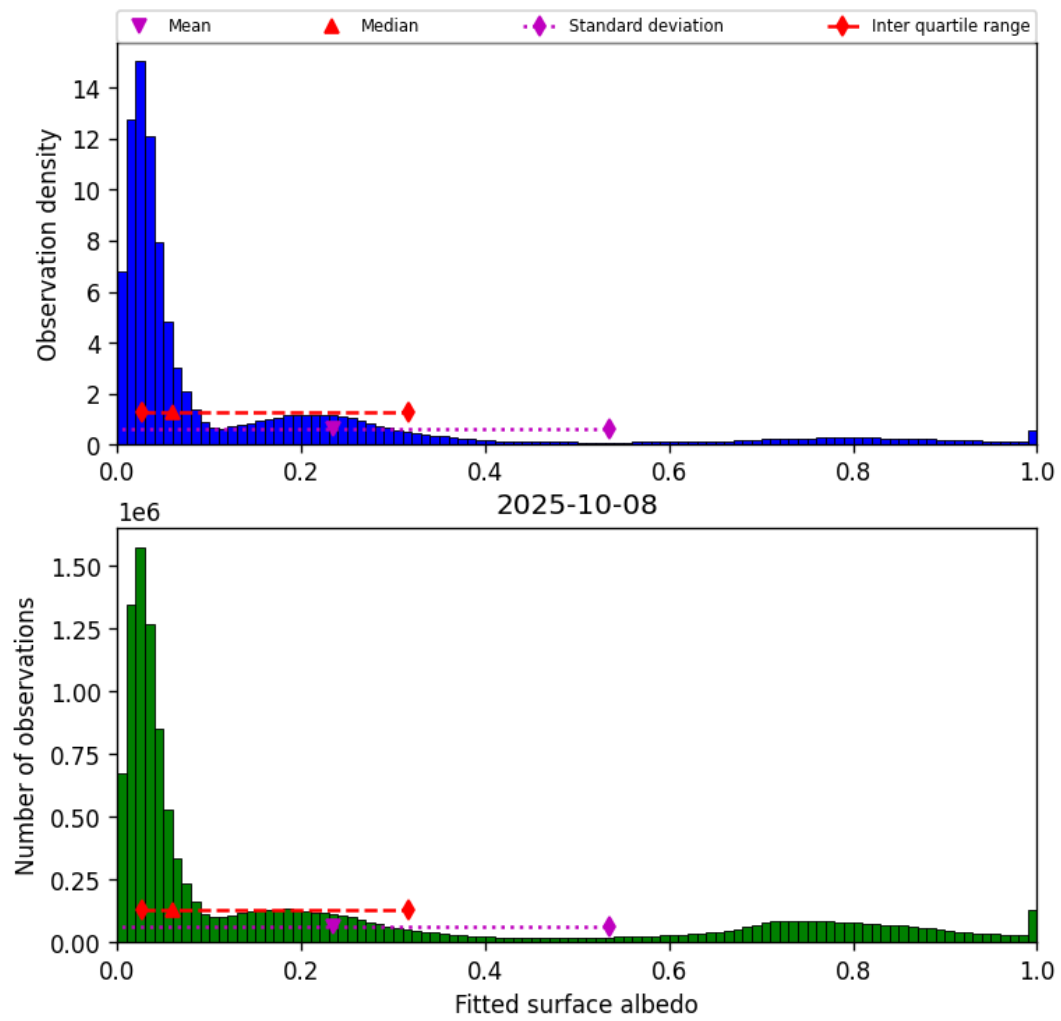
Figure 43: Histogram of “Fitted surface albedo” for 2025-10-08 to 2025-10-09
