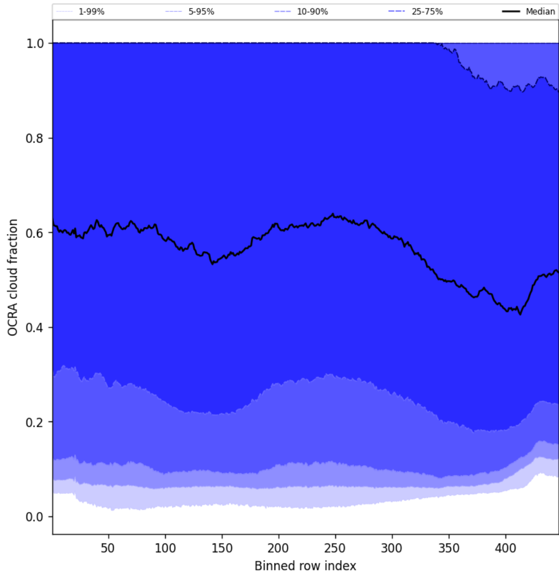
Figure 64: Along track statistics of “OCRA cloud fraction” for 2025-10-08 to 2025-10-09
