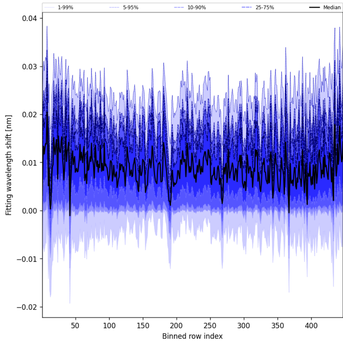
Figure 63: Along track statistics of “Fitting wavelength shift” for 2025-10-08 to 2025-10-09
