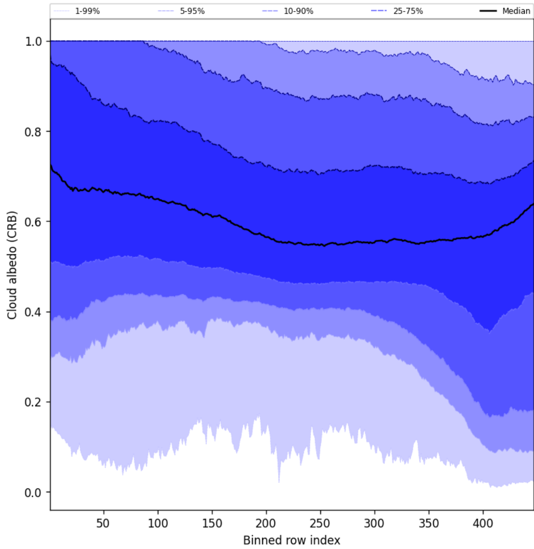
Figure 58: Along track statistics of “Cloud albedo (CRB)” for 2025-10-08 to 2025-10-09
