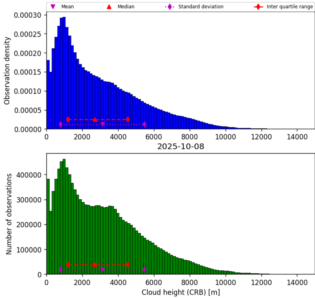
Figure 41: Histogram of “Cloud height (CRB)” for 2025-10-08 to 2025-10-09
