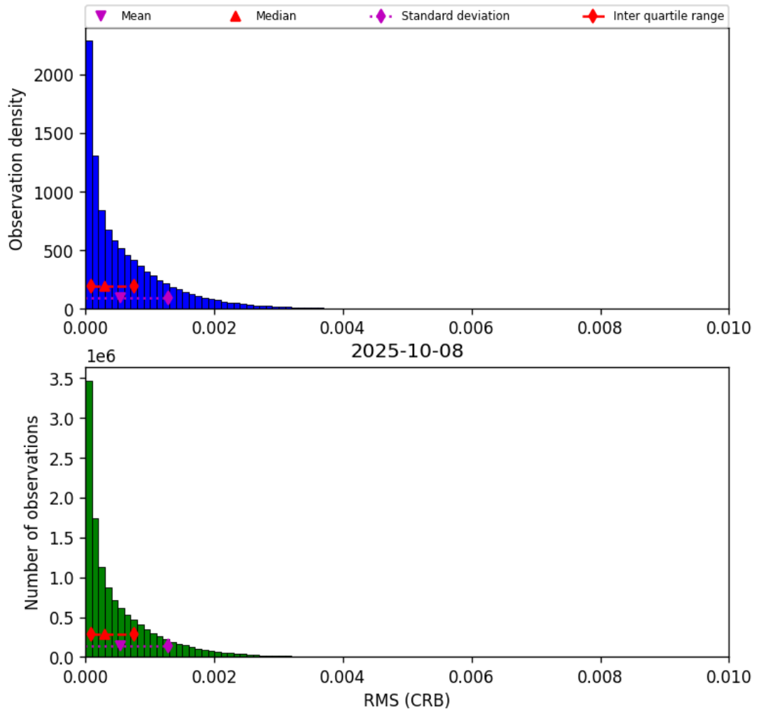
Figure 46: Histogram of “RMS (CRB)” for 2025-10-08 to 2025-10-09
