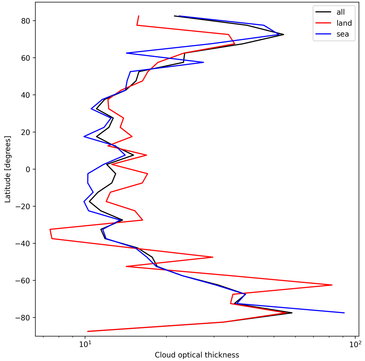
Figure 23: Zonal average of “Cloud optical thickness” for 2025-10-08 to 2025-10-09.
