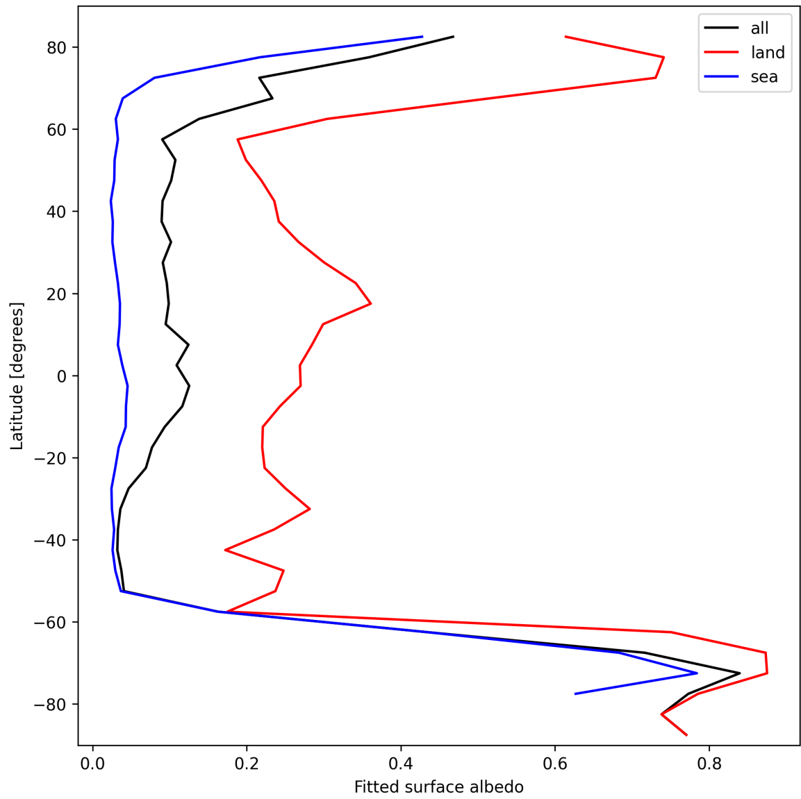
Figure 27: Zonal average of “Fitted surface albedo” for 2025-10-08 to 2025-10-09.
