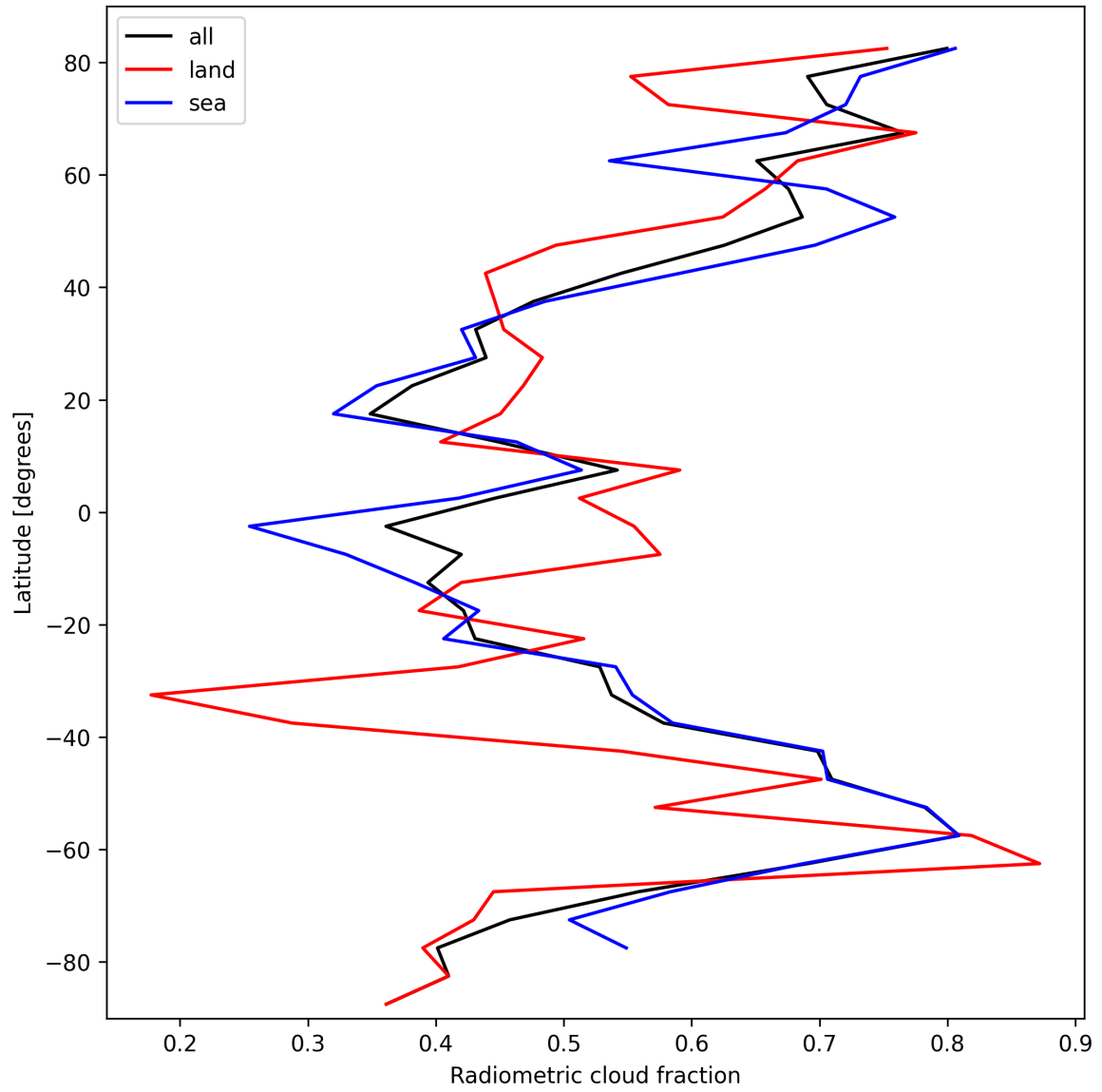
Figure 21: Zonal average of “Radiometric cloud fraction” for 2025-10-08 to 2025-10-09.
