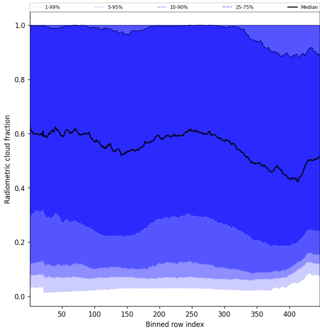
Figure 53: Along track statistics of “Radiometric cloud fraction” for 2025-10-08 to 2025-10-09
