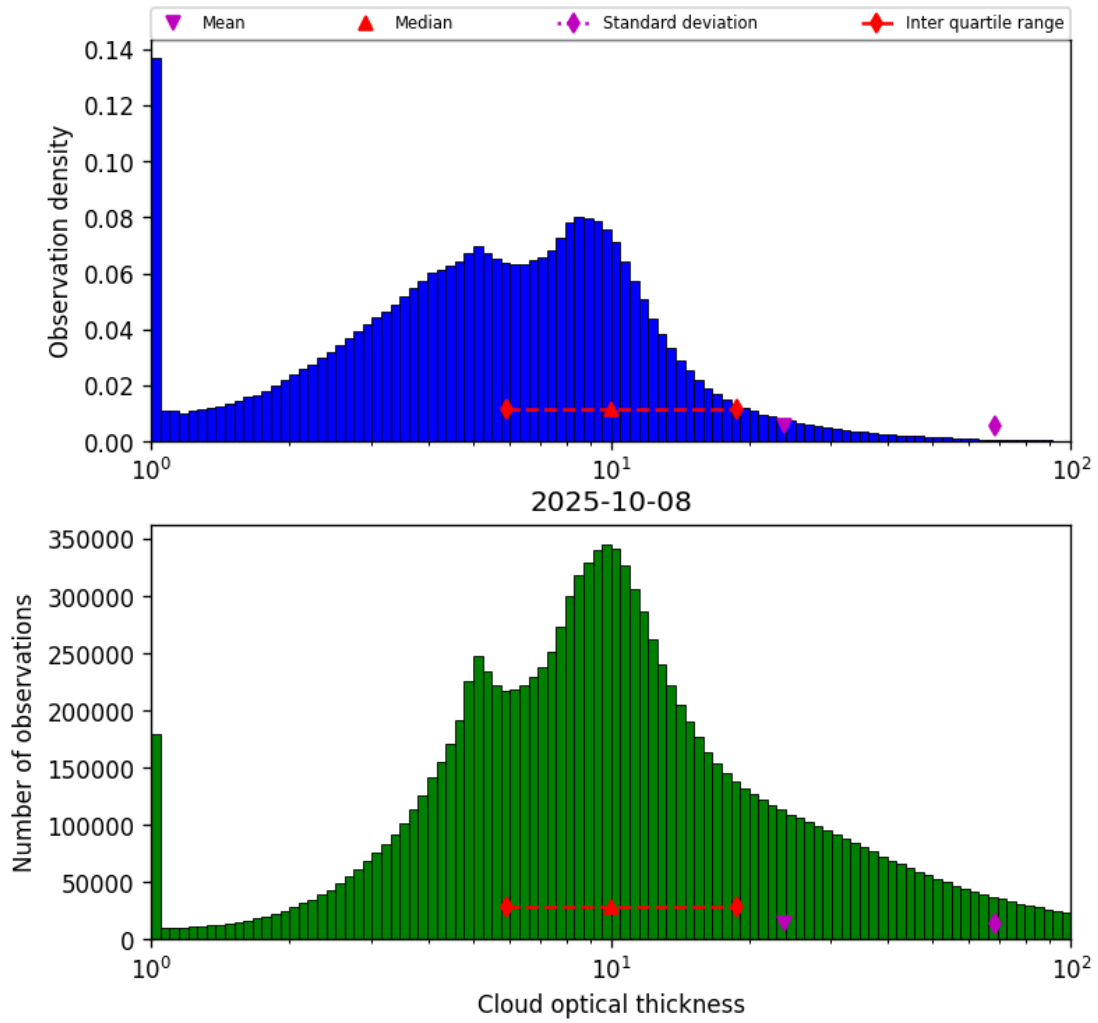
Figure 39: Histogram of “Cloud optical thickness” for 2025-10-08 to 2025-10-09
