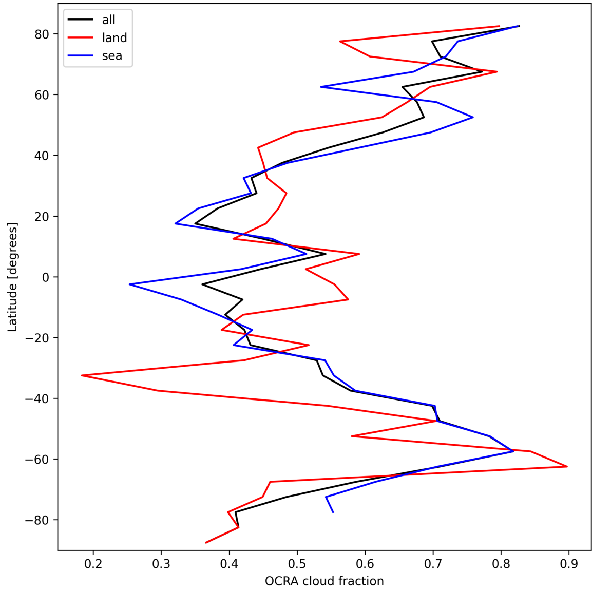
Figure 32: Zonal average of “OCRA cloud fraction” for 2025-10-08 to 2025-10-09.
