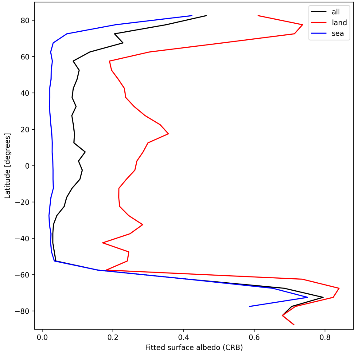
Figure 28: Zonal average of “Fitted surface albedo (CRB)” for 2025-10-08 to 2025-10-09.
