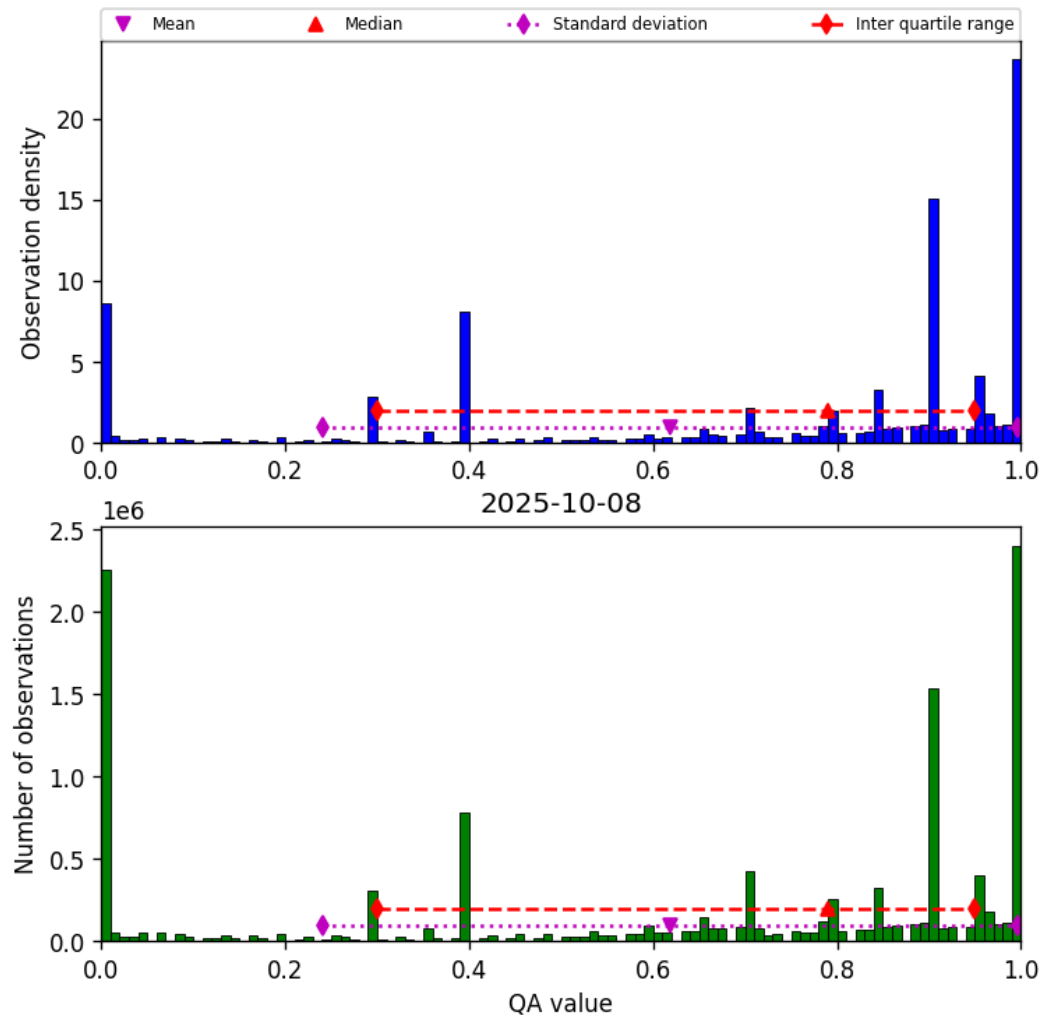
Figure 36: Histogram of “QA value” for 2025-10-08 to 2025-10-09
