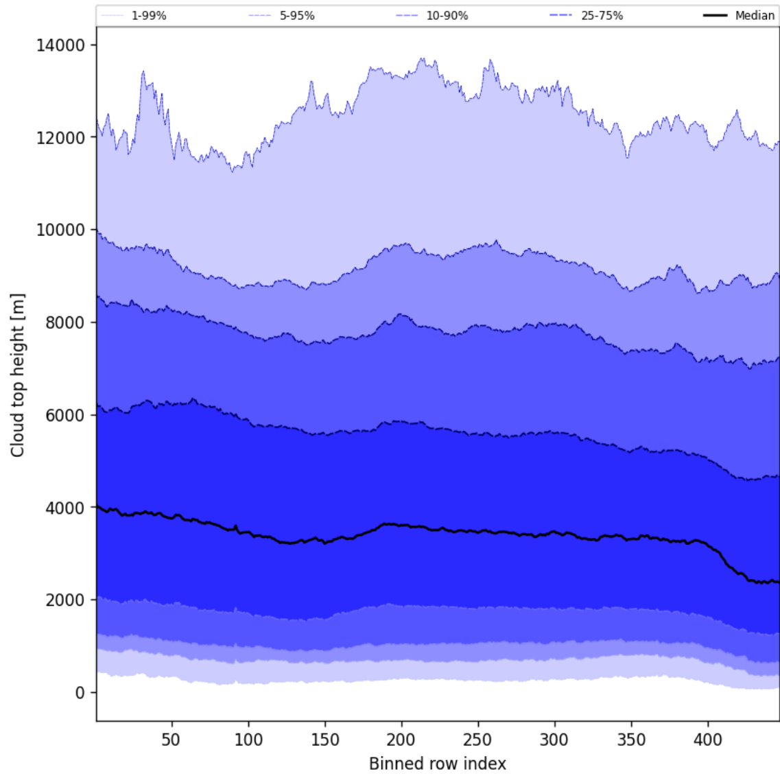
Figure 54: Along track statistics of “Cloud top height” for 2025-10-08 to 2025-10-09
