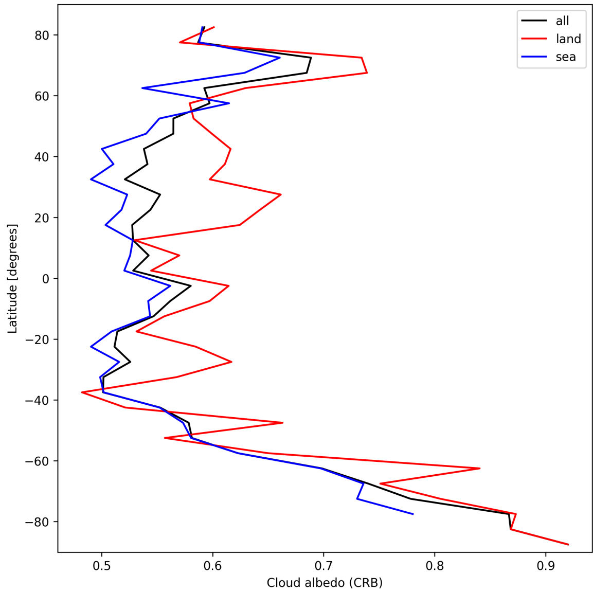
Figure 26: Zonal average of “Cloud albedo (CRB)” for 2025-10-08 to 2025-10-09.
