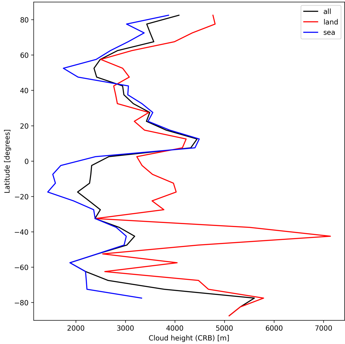
Figure 25: Zonal average of “Cloud height (CRB)” for 2025-10-08 to 2025-10-09.
