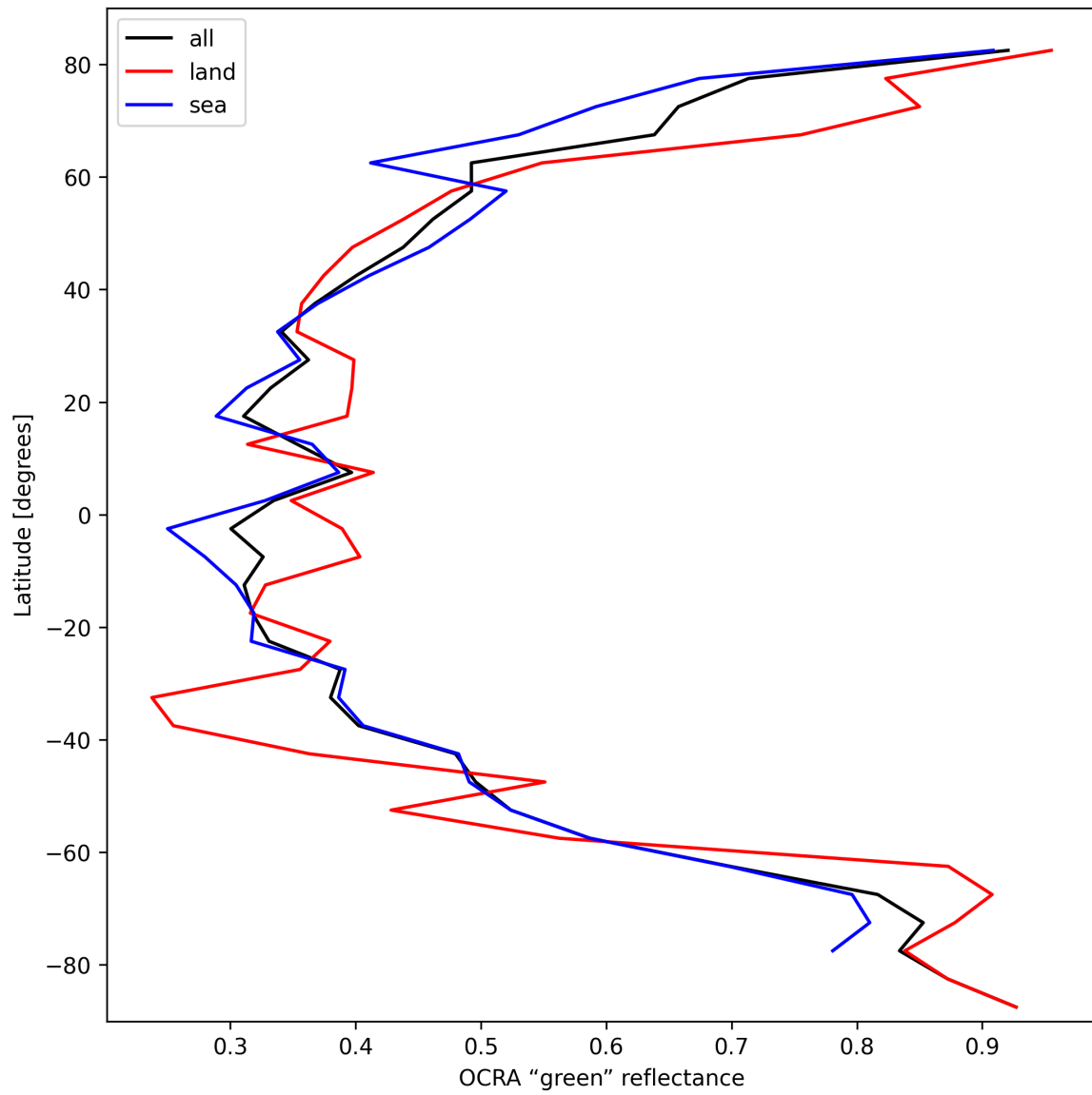
Figure 34: Zonal average of “OCRA “green” reflectance” for 2025-10-08 to 2025-10-09.
