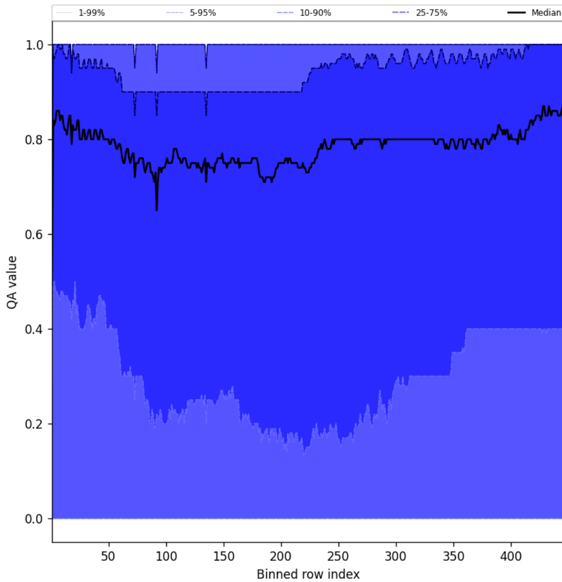
Figure 52: Along track statistics of “QA value” for 2025-10-08 to 2025-10-09
