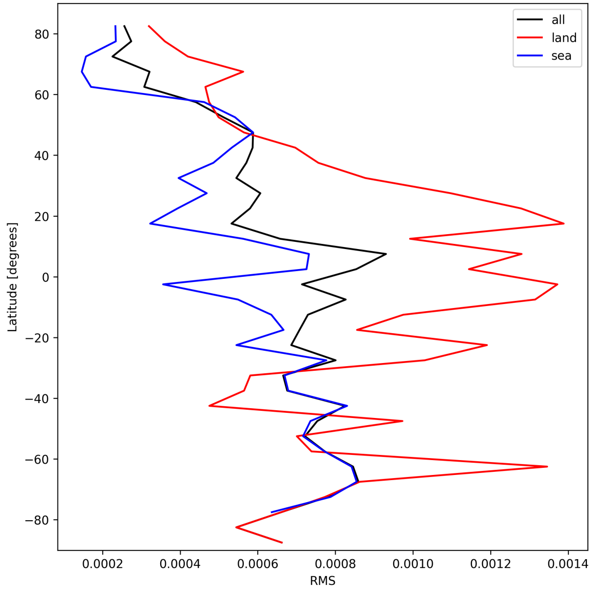
Figure 29: Zonal average of “RMS” for 2025-10-08 to 2025-10-09.
