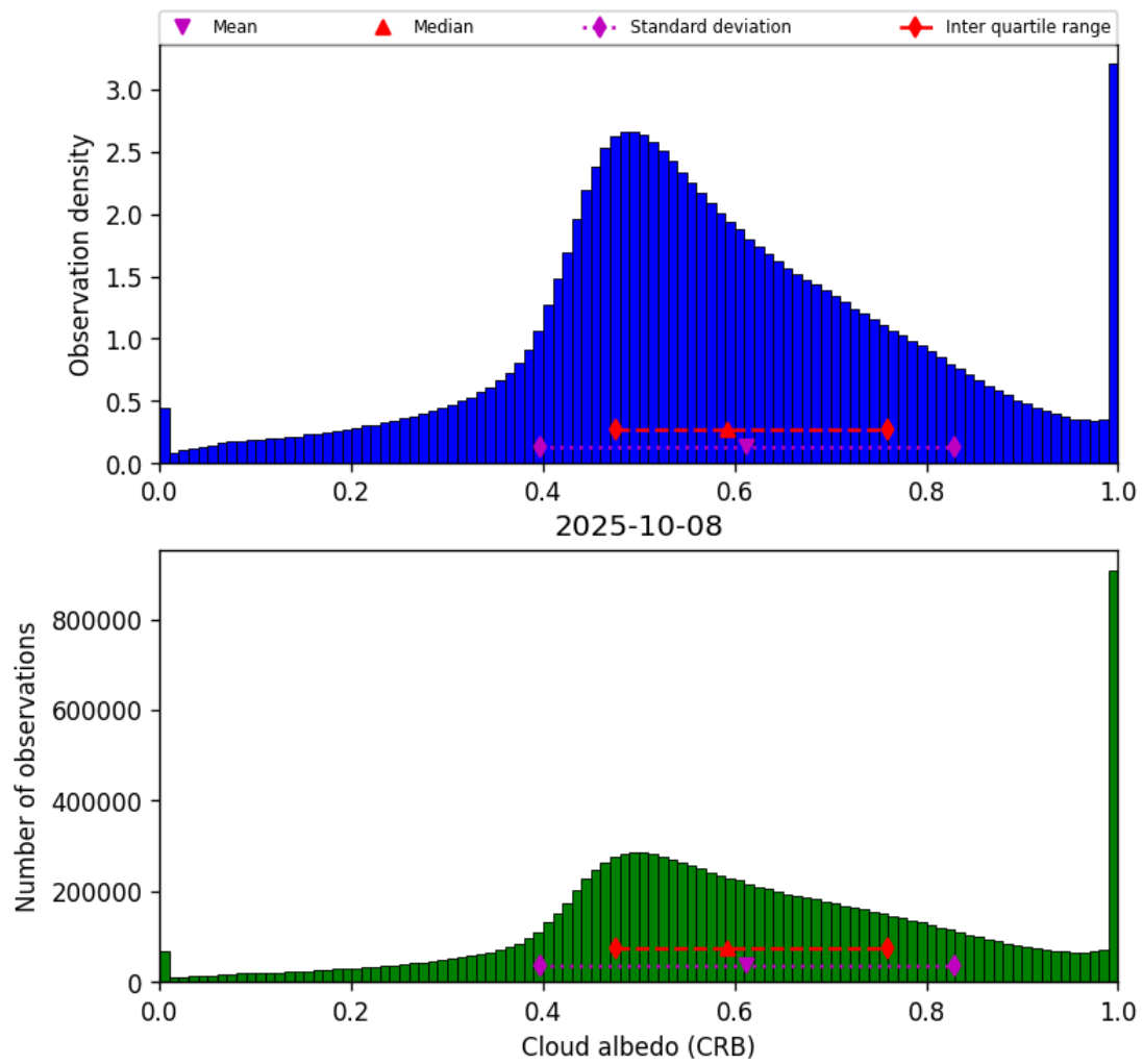
Figure 42: Histogram of “Cloud albedo (CRB)” for 2025-10-08 to 2025-10-09
