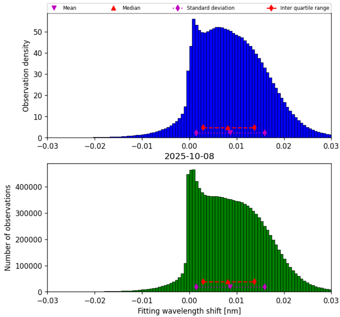
Figure 47: Histogram of “Fitting wavelength shift” for 2025-10-08 to 2025-10-09
