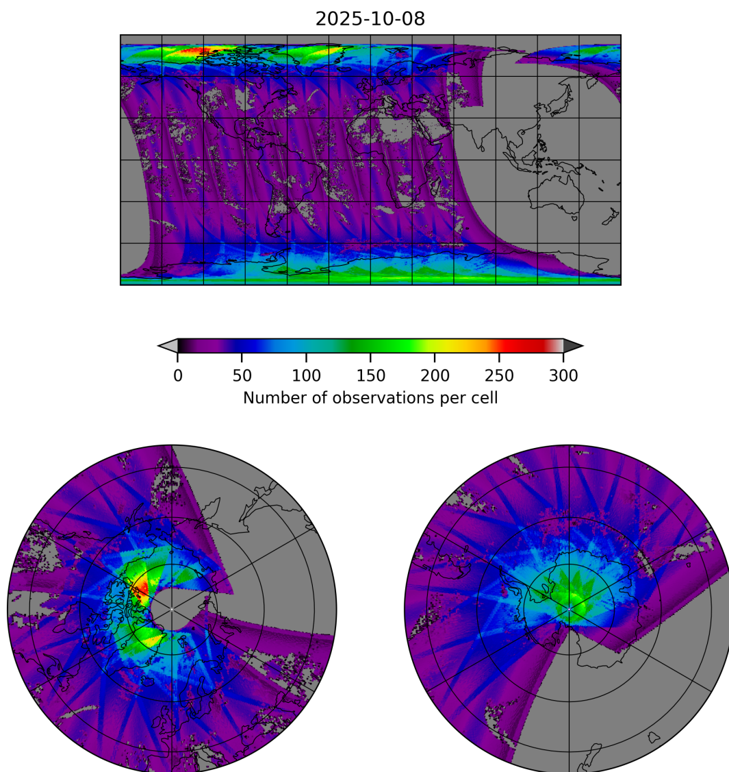
Figure 19: Map of the number of observations for 2025-10-08 to 2025-10-09
