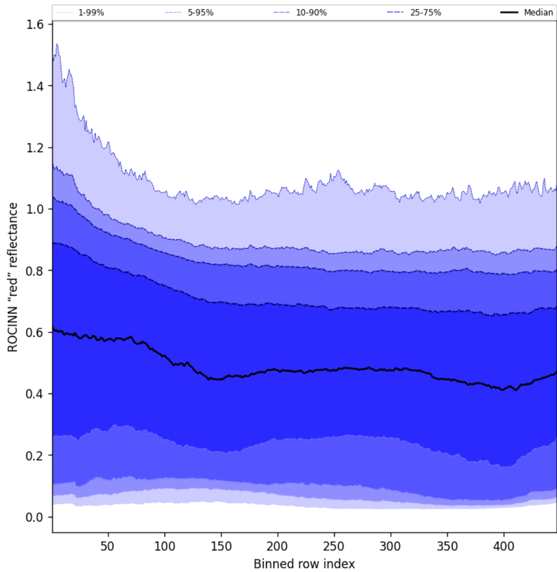
Figure 67: Along track statistics of "ROCINN "red" reflectance" for 2025-10-08 to 2025-10-09
