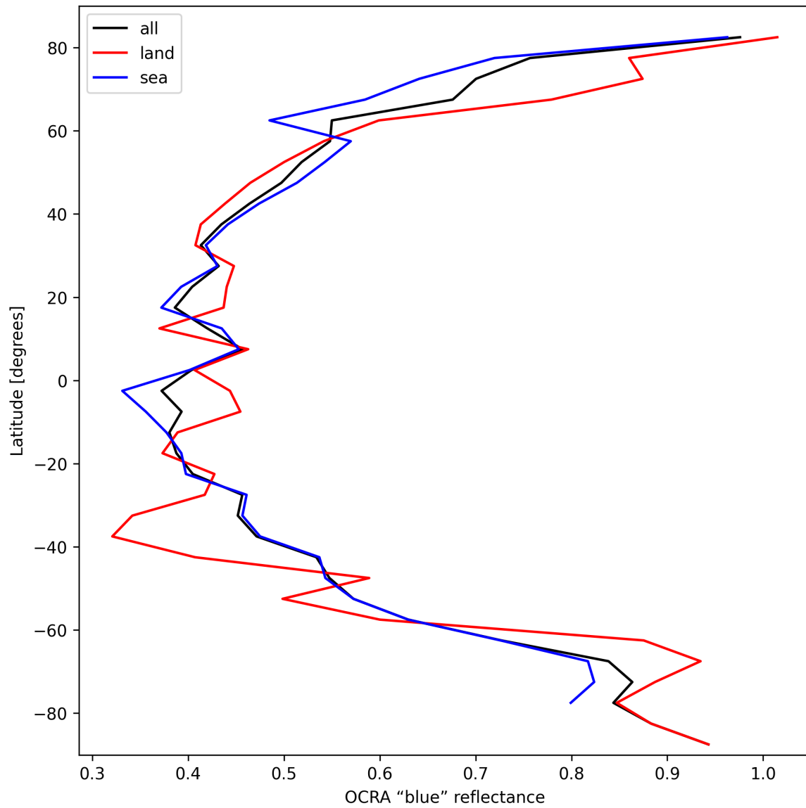
Figure 33: Zonal average of “OCRA “blue” reflectance” for 2025-10-08 to 2025-10-09.
