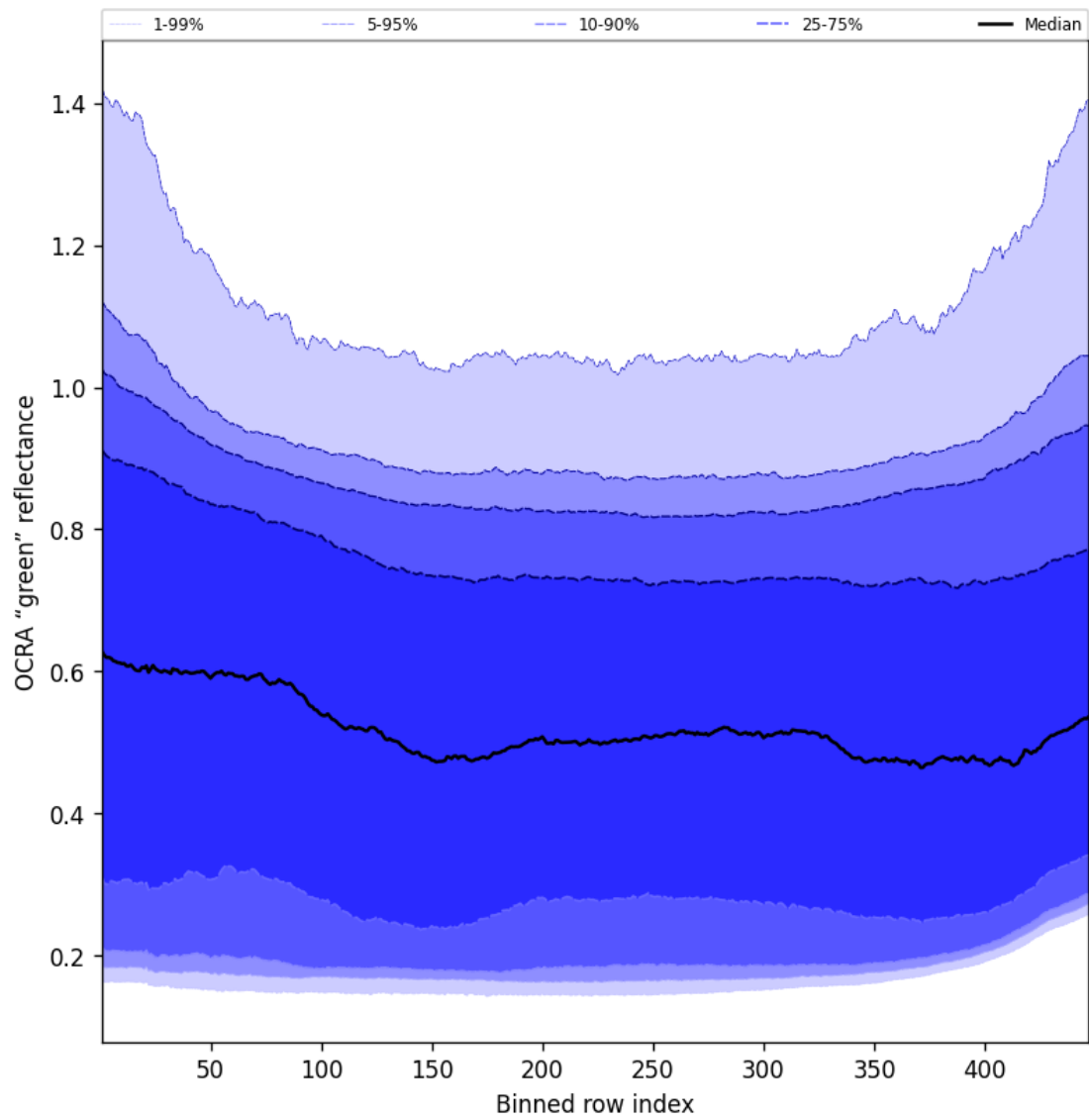
Figure 66: Along track statistics of “OCRA “green” reflectance” for 2025-10-08 to 2025-10-09
