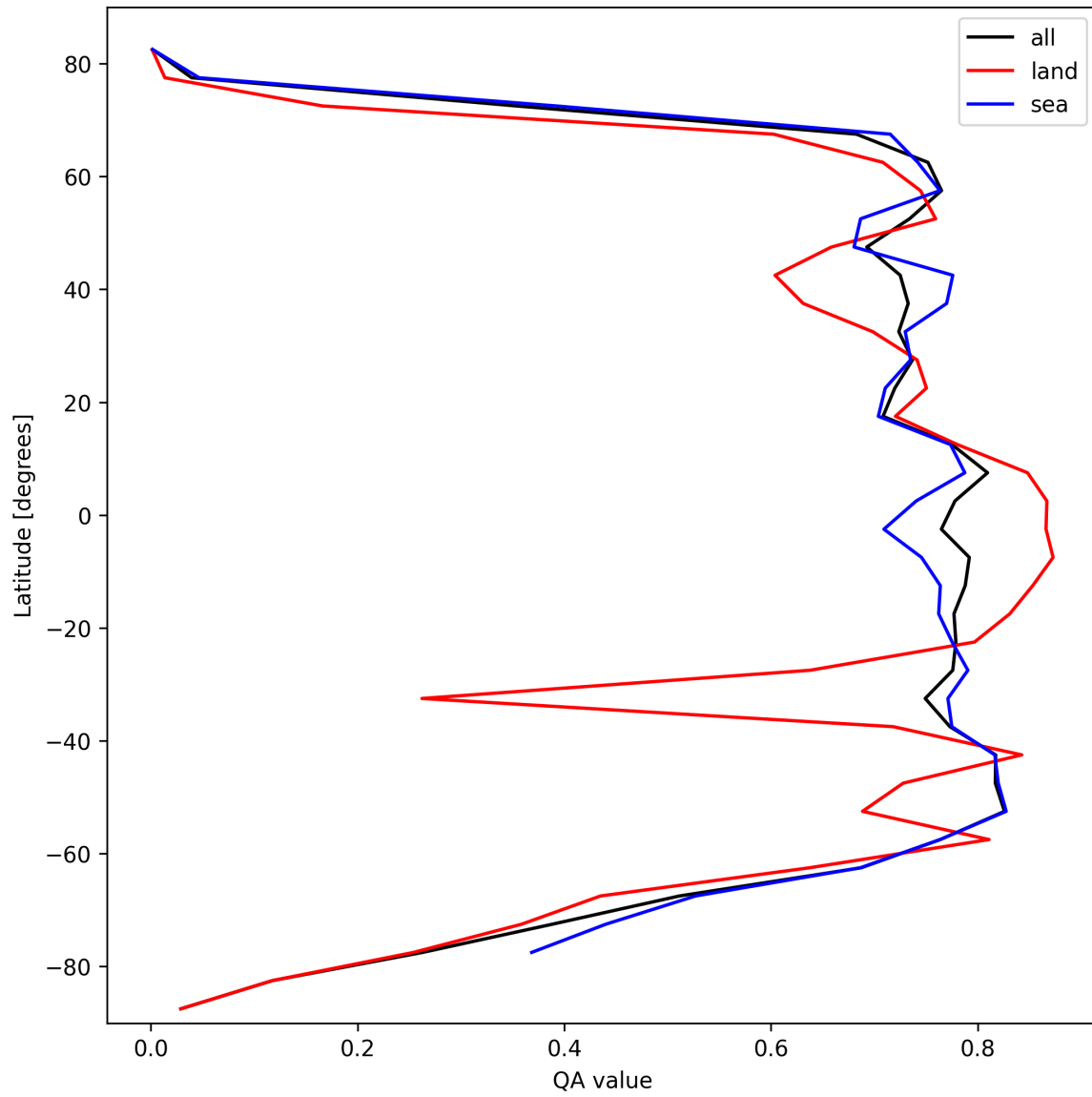
Figure 20: Zonal average of “QA value” for 2025-10-08 to 2025-10-09.
