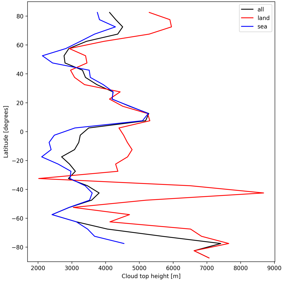
Figure 22: Zonal average of “Cloud top height” for 2025-10-08 to 2025-10-09.
