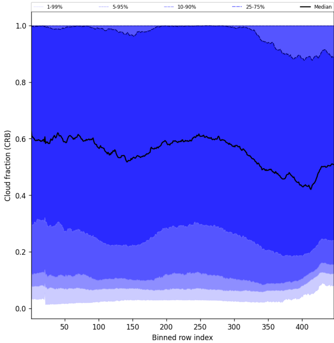
Figure 56: Along track statistics of “Cloud fraction (CRB)” for 2025-10-08 to 2025-10-09
