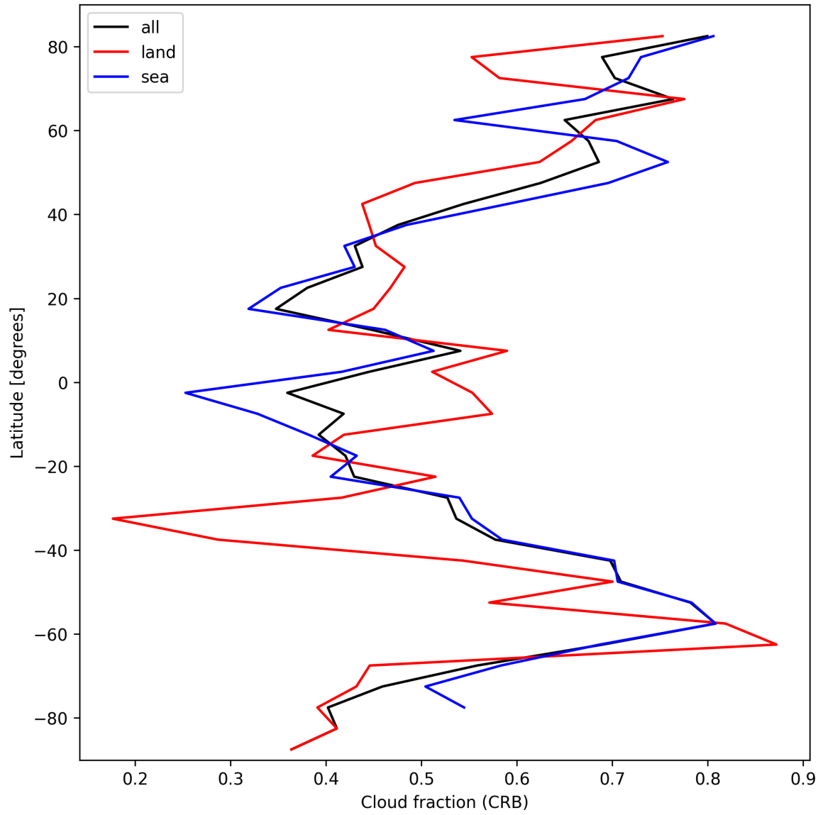
Figure 24: Zonal average of “Cloud fraction (CRB)” for 2025-10-08 to 2025-10-09.
