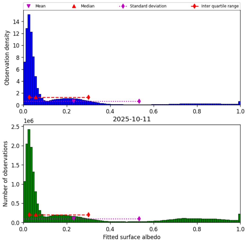
Figure 43: Histogram of “Fitted surface albedo” for 2025-10-11 to 2025-10-12
