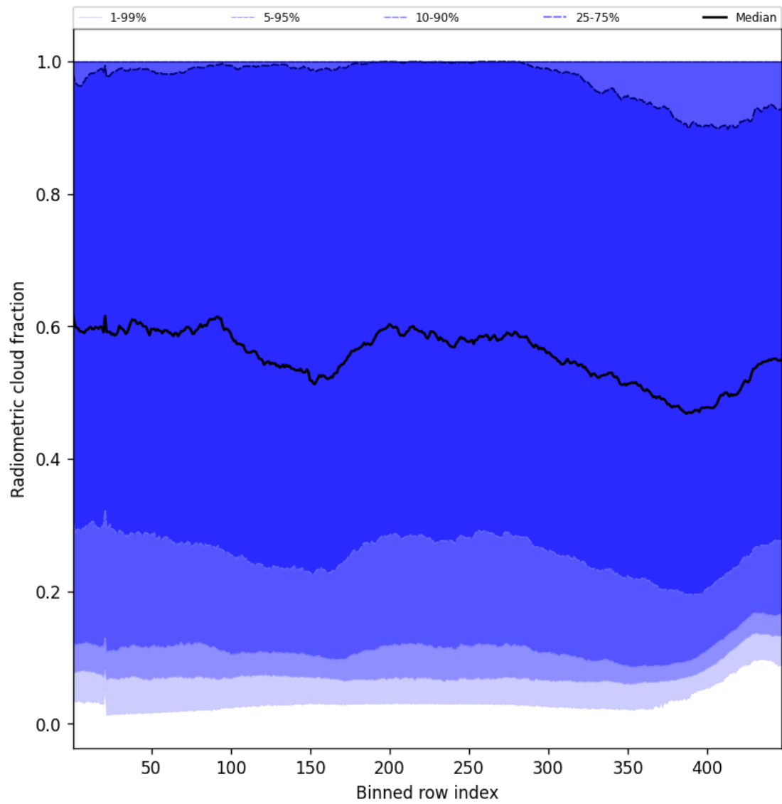
Figure 53: Along track statistics of “Radiometric cloud fraction” for 2025-10-11 to 2025-10-12
