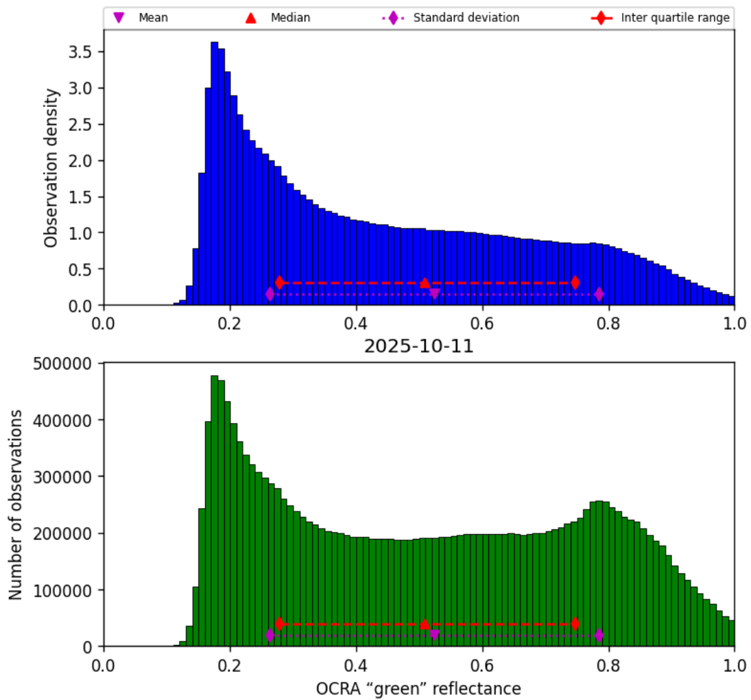
Figure 50: Histogram of “OCRA “green” reflectance” for 2025-10-11 to 2025-10-12
