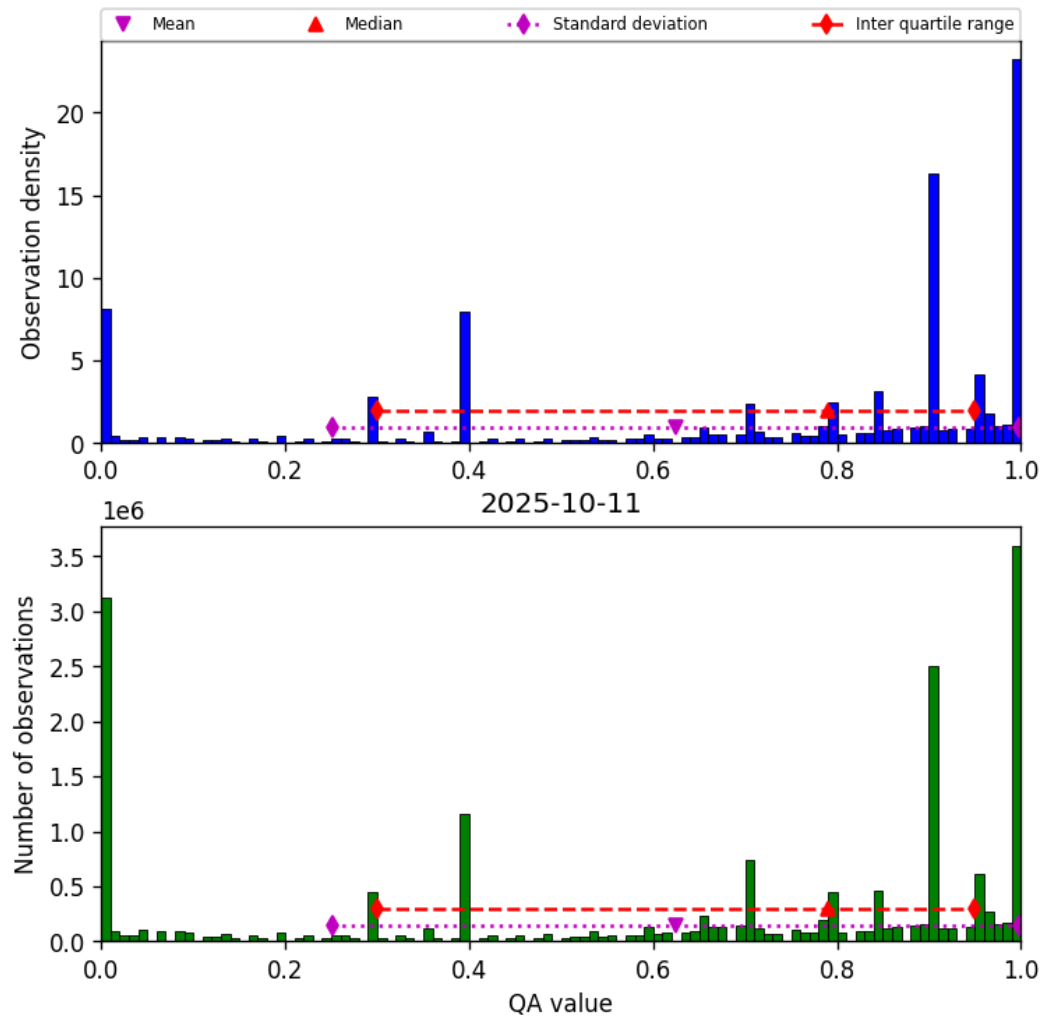
Figure 36: Histogram of “QA value” for 2025-10-11 to 2025-10-12
