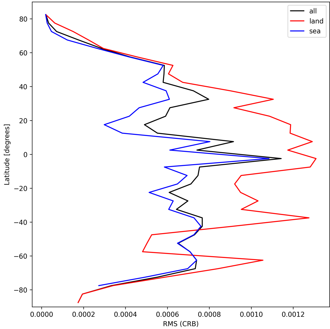
Figure 30: Zonal average of “RMS (CRB)” for 2025-10-11 to 2025-10-12.
