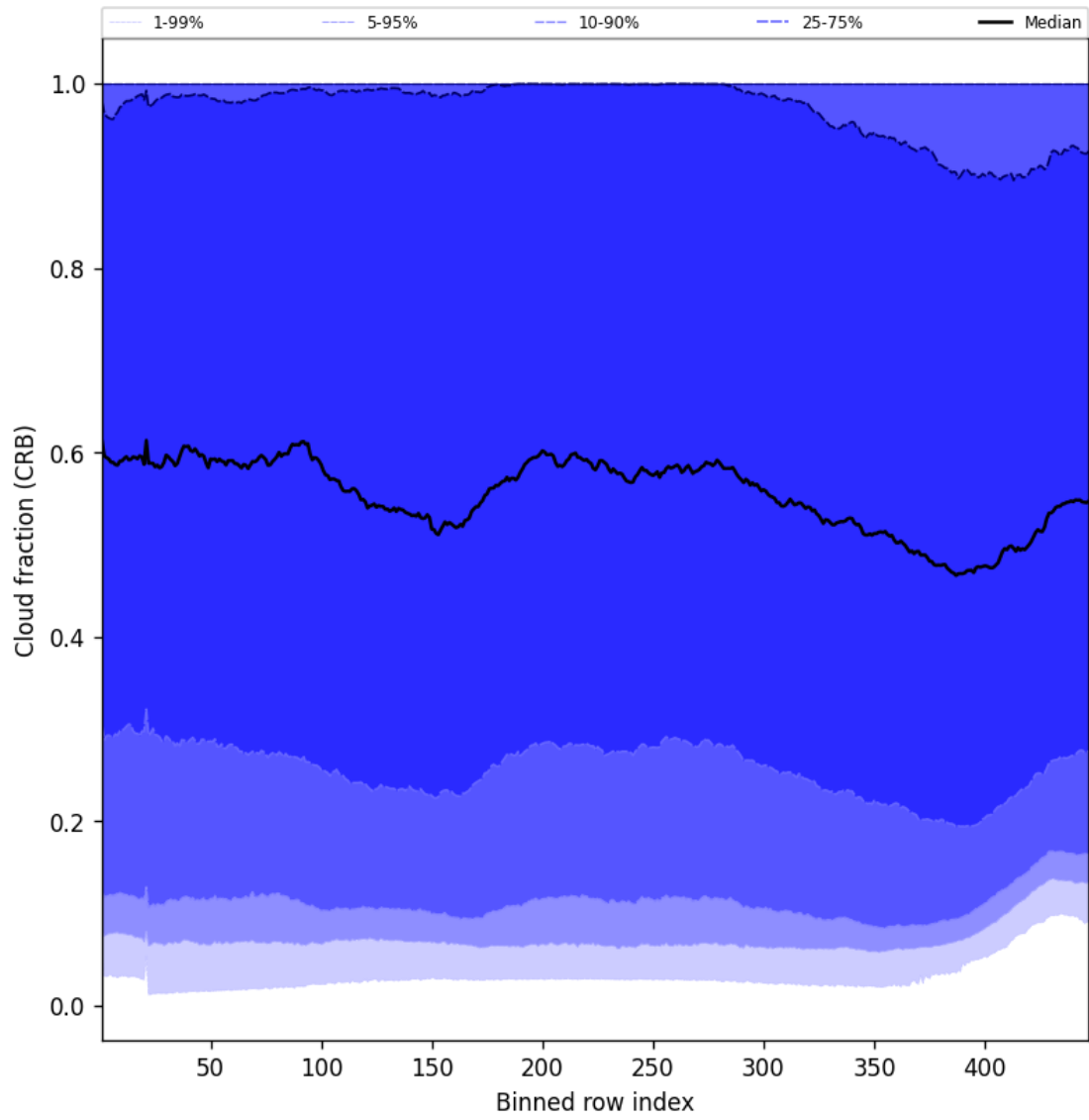
Figure 56: Along track statistics of “Cloud fraction (CRB)” for 2025-10-11 to 2025-10-12
