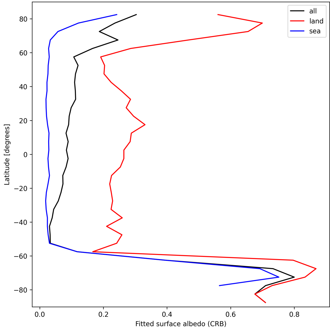
Figure 28: Zonal average of “Fitted surface albedo (CRB)” for 2025-10-11 to 2025-10-12.
