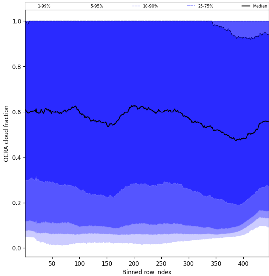
Figure 64: Along track statistics of “OCRA cloud fraction” for 2025-10-11 to 2025-10-12
