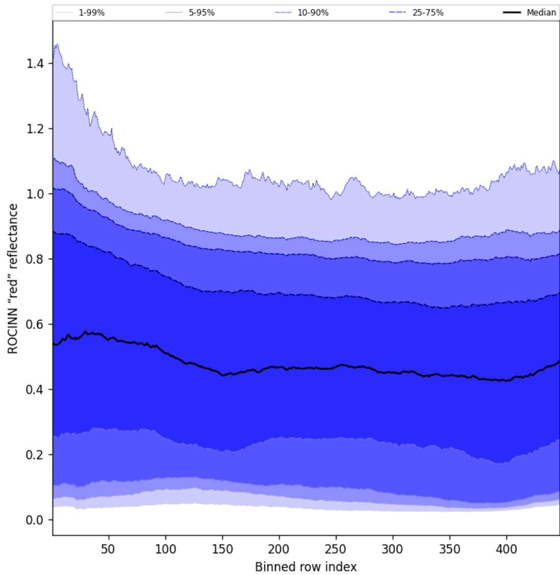
Figure 67: Along track statistics of “ROCINN “red” reflectance” for 2025-10-11 to 2025-10-12
