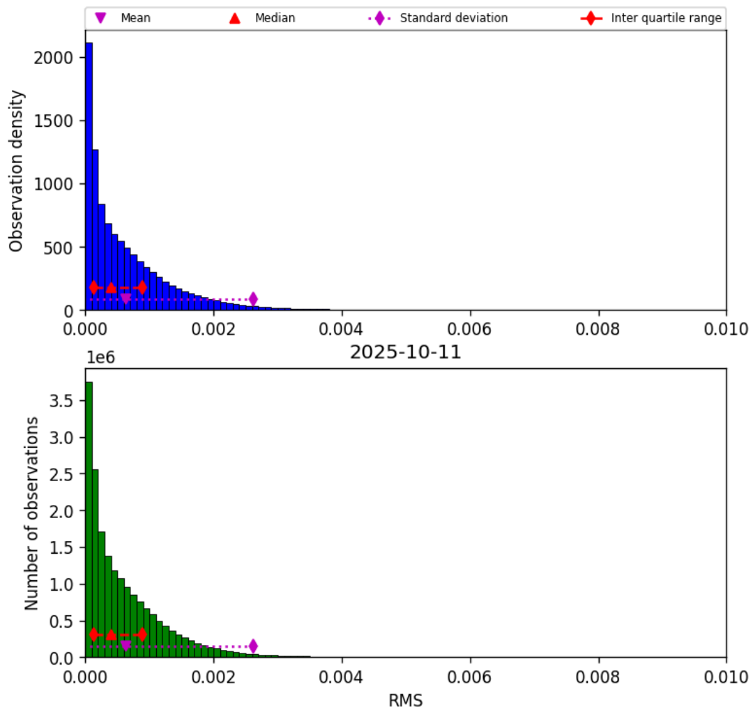
Figure 45: Histogram of “RMS” for 2025-10-11 to 2025-10-12
