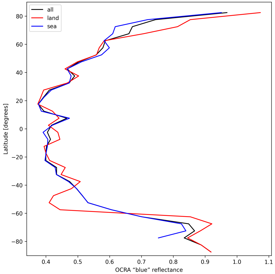
Figure 33: Zonal average of “OCRA “blue” reflectance” for 2025-10-11 to 2025-10-12.
