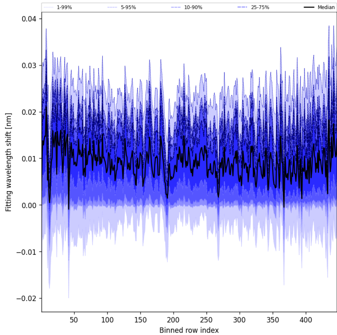
Figure 63: Along track statistics of “Fitting wavelength shift” for 2025-10-11 to 2025-10-12
