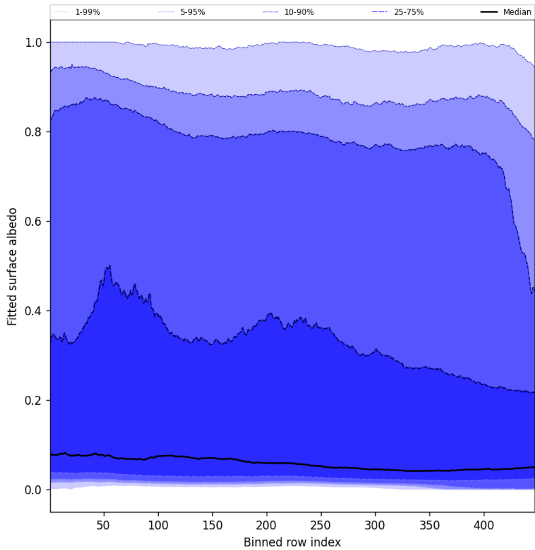
Figure 59: Along track statistics of “Fitted surface albedo” for 2025-10-11 to 2025-10-12
