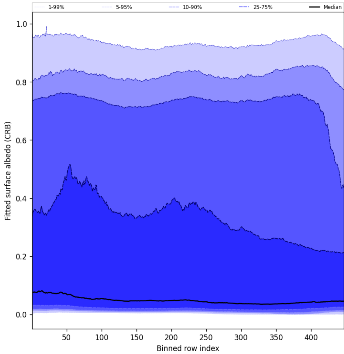
Figure 60: Along track statistics of “Fitted surface albedo (CRB)” for 2025-10-11 to 2025-10-12
