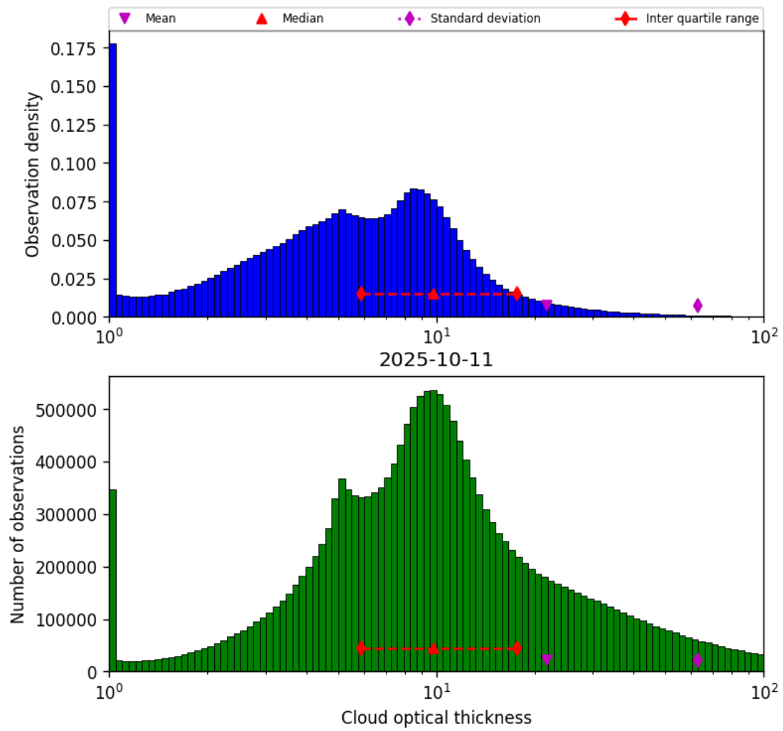
Figure 39: Histogram of “Cloud optical thickness” for 2025-10-11 to 2025-10-12
