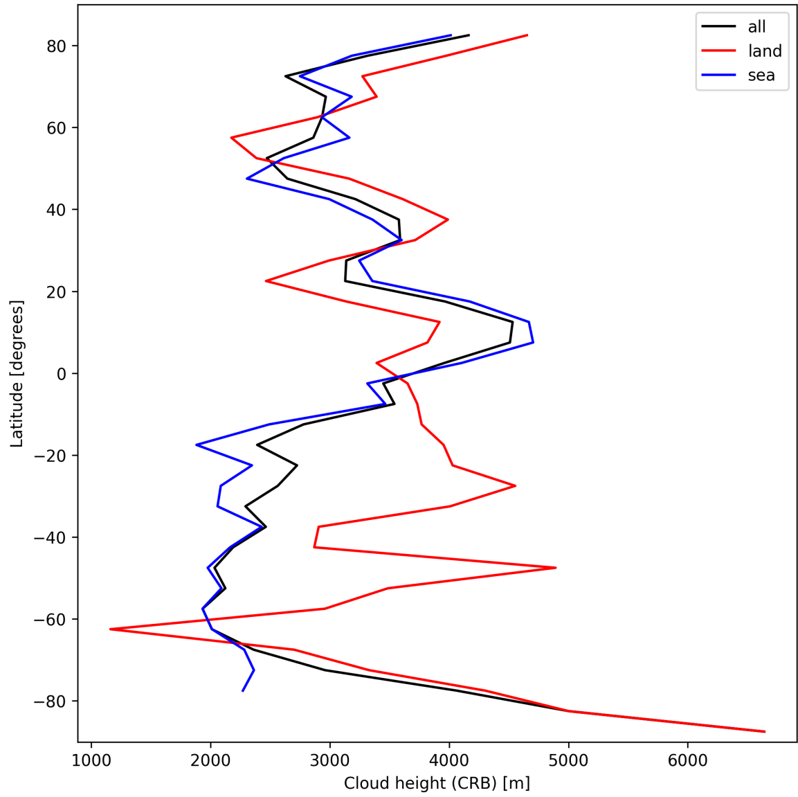
Figure 25: Zonal average of “Cloud height (CRB)” for 2025-10-11 to 2025-10-12.
