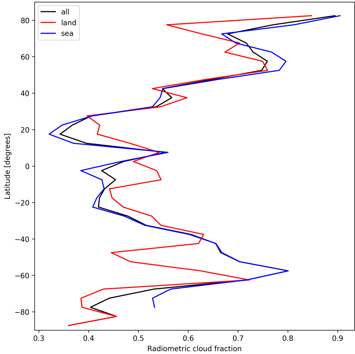
Figure 21: Zonal average of “Radiometric cloud fraction” for 2025-10-11 to 2025-10-12.
