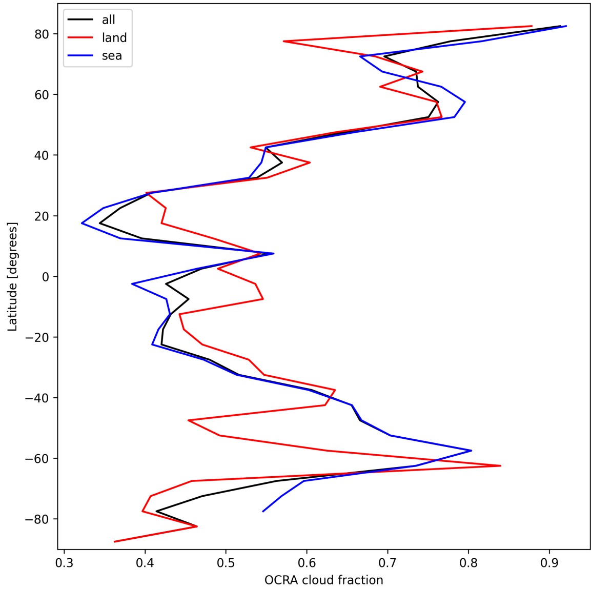
Figure 32: Zonal average of “OCRA cloud fraction” for 2025-10-11 to 2025-10-12.
