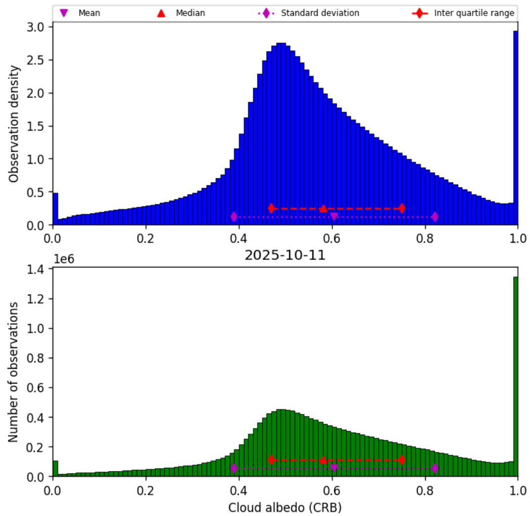
Figure 42: Histogram of “Cloud albedo (CRB)” for 2025-10-11 to 2025-10-12
