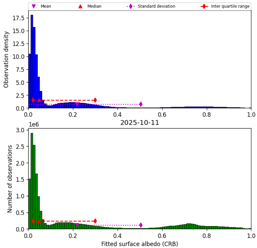
Figure 44: Histogram of “Fitted surface albedo (CRB)” for 2025-10-11 to 2025-10-12
