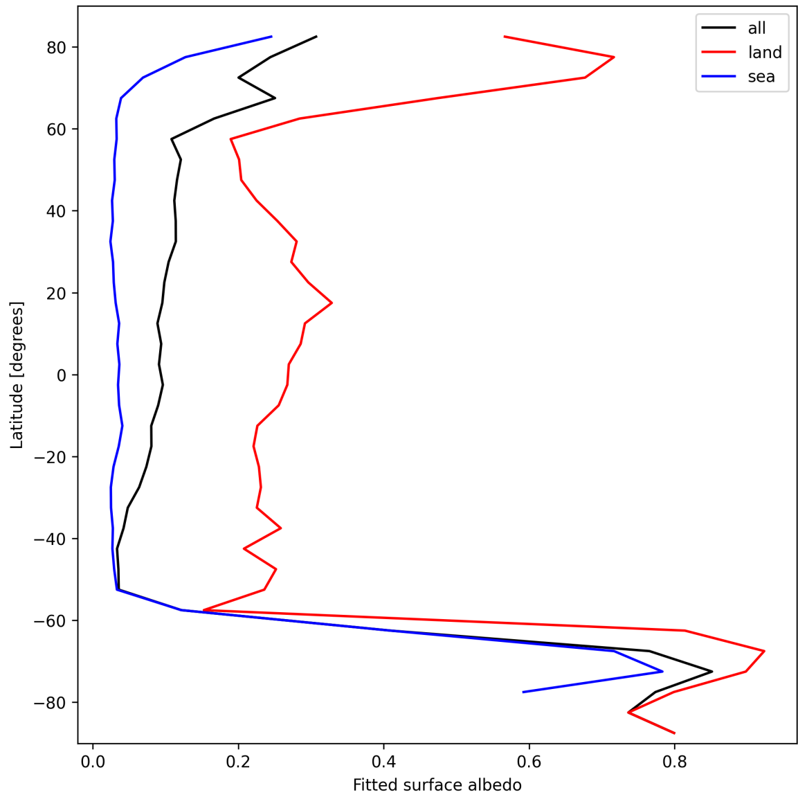
Figure 27: Zonal average of “Fitted surface albedo” for 2025-10-11 to 2025-10-12.
