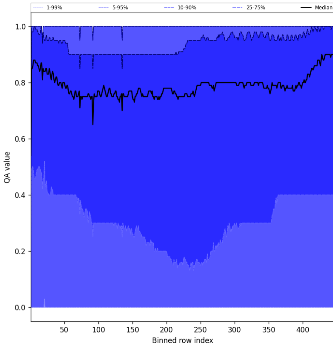
Figure 52: Along track statistics of “QA value” for 2025-10-11 to 2025-10-12
