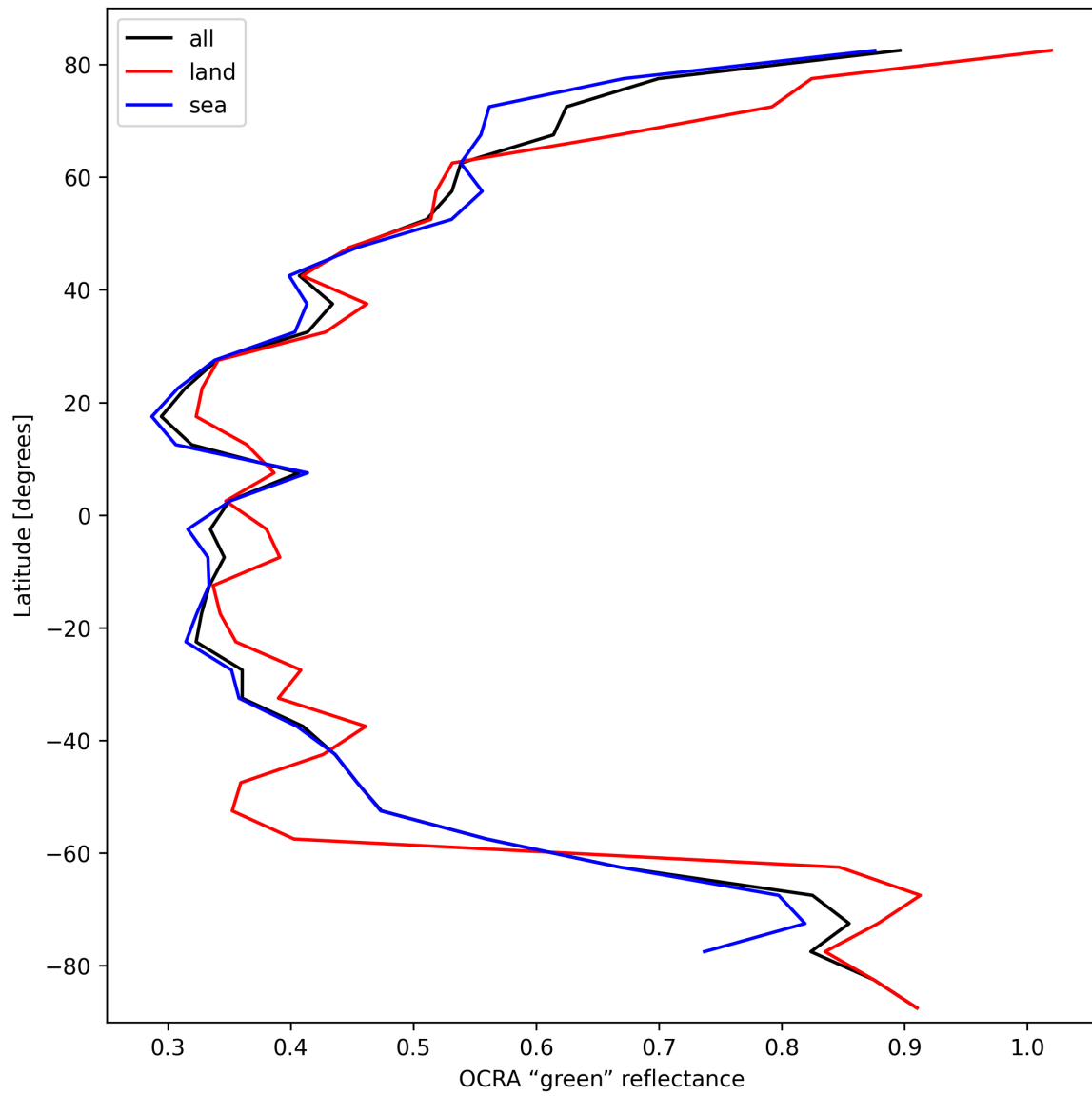
Figure 34: Zonal average of “OCRA “green” reflectance” for 2025-10-11 to 2025-10-12.
