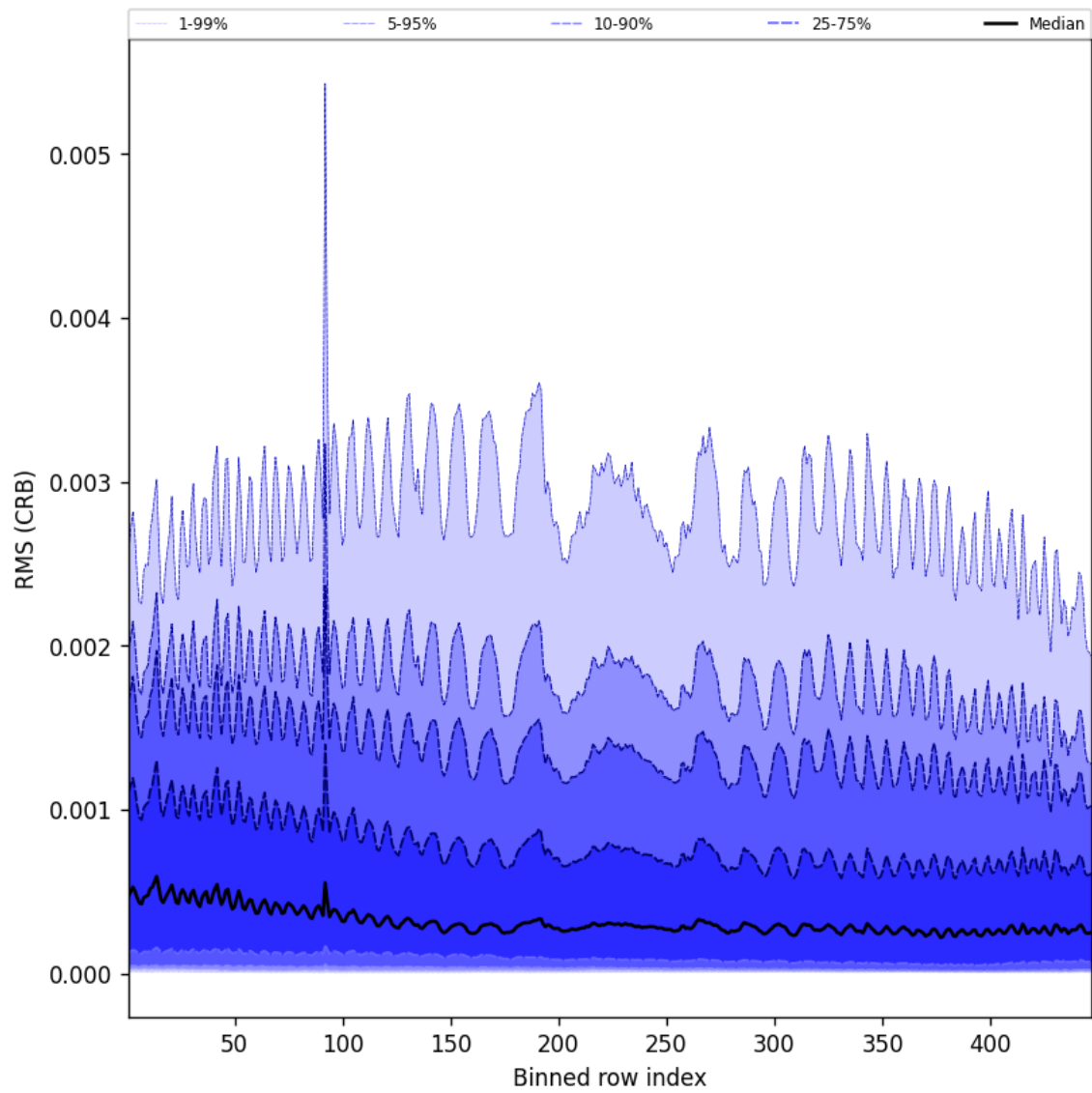
Figure 62: Along track statistics of “RMS (CRB)” for 2025-10-11 to 2025-10-12
