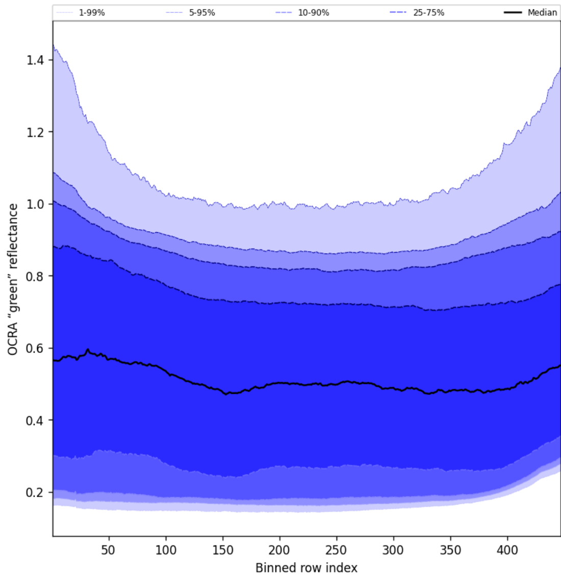
Figure 66: Along track statistics of “OCRA “green” reflectance” for 2025-10-11 to 2025-10-12
