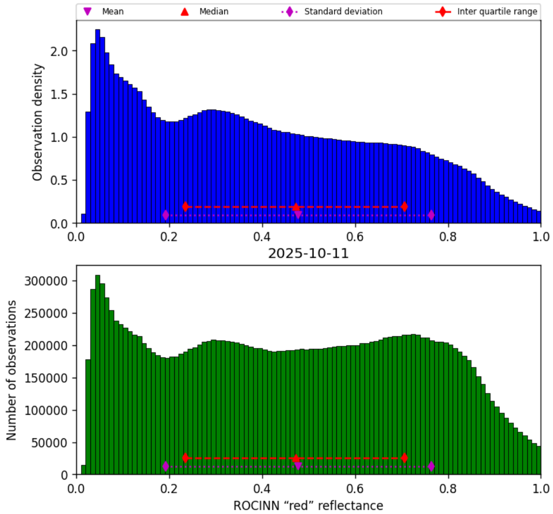
Figure 51: Histogram of “ROCINN “red” reflectance” for 2025-10-11 to 2025-10-12
