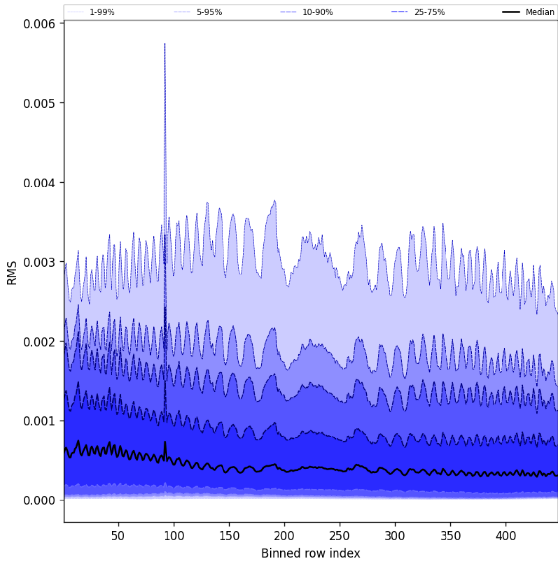
Figure 61: Along track statistics of “RMS” for 2025-10-11 to 2025-10-12
