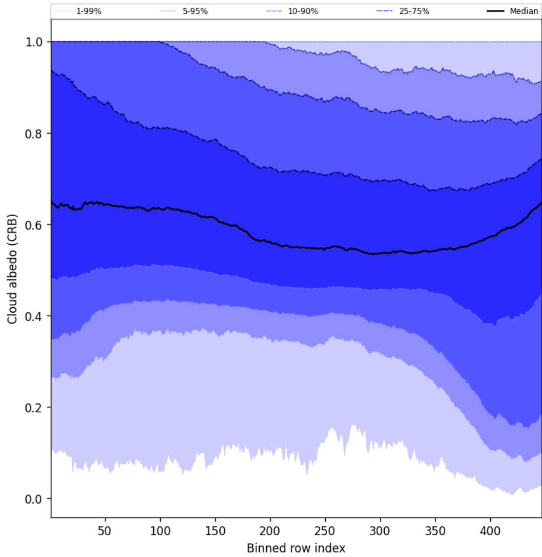
Figure 58: Along track statistics of “Cloud albedo (CRB)” for 2025-10-11 to 2025-10-12
