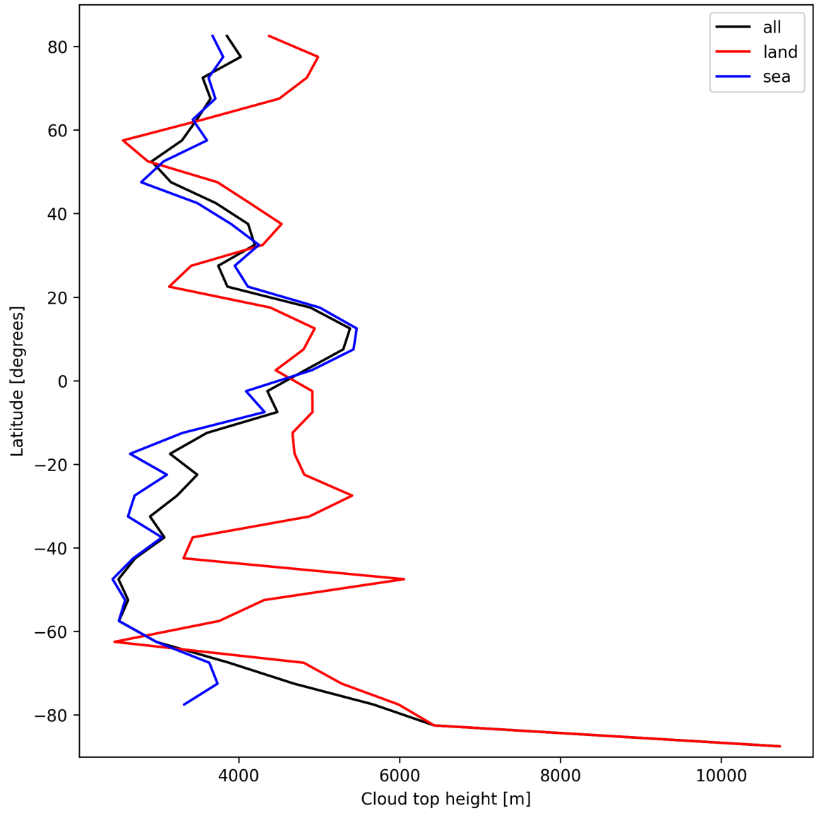
Figure 22: Zonal average of “Cloud top height” for 2025-10-11 to 2025-10-12.
