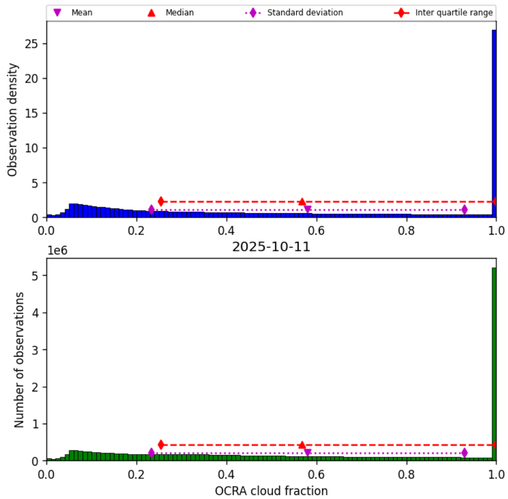
Figure 48: Histogram of “OCRA cloud fraction” for 2025-10-11 to 2025-10-12
