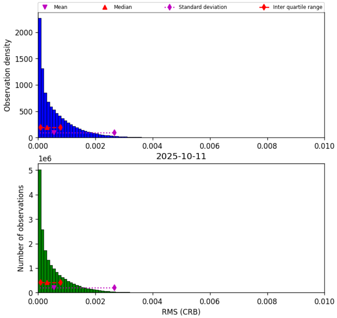
Figure 46: Histogram of "RMS (CRB)" for 2025-10-11 to 2025-10-12
