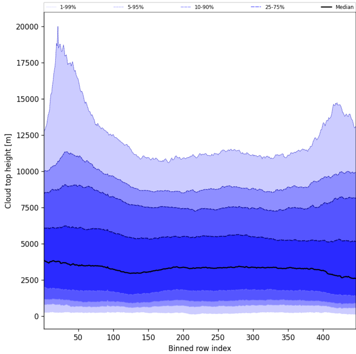
Figure 54: Along track statistics of “Cloud top height” for 2025-10-11 to 2025-10-12
