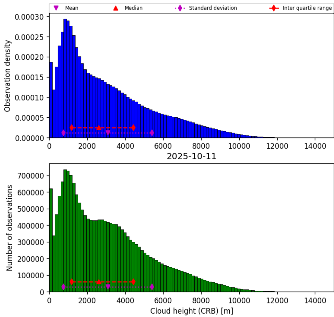
Figure 41: Histogram of “Cloud height (CRB)” for 2025-10-11 to 2025-10-12
