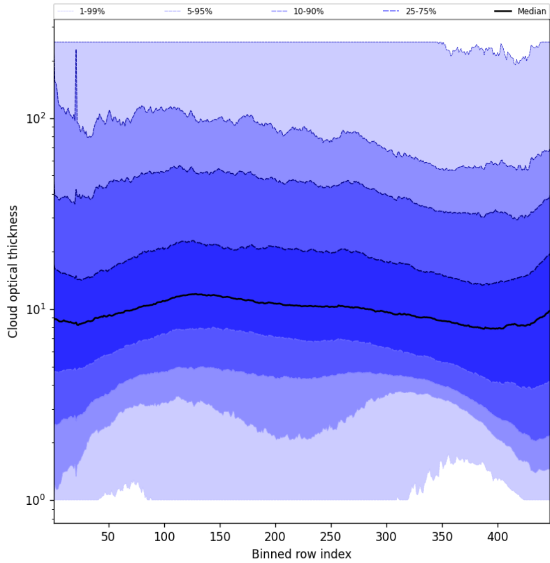
Figure 55: Along track statistics of “Cloud optical thickness” for 2025-10-11 to 2025-10-12
