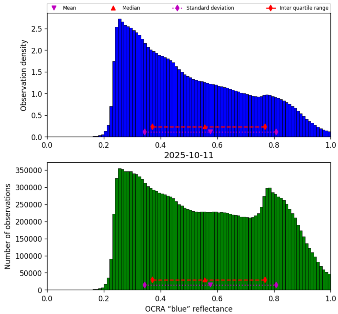
Figure 49: Histogram of “OCRA “blue” reflectance” for 2025-10-11 to 2025-10-12
