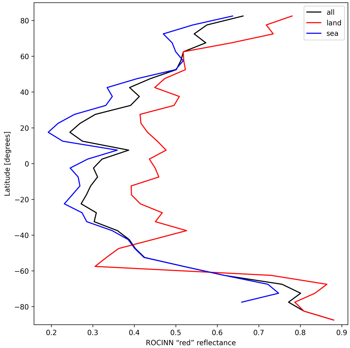
Figure 35: Zonal average of “ROCINN “red” reflectance” for 2025-10-11 to 2025-10-12.
