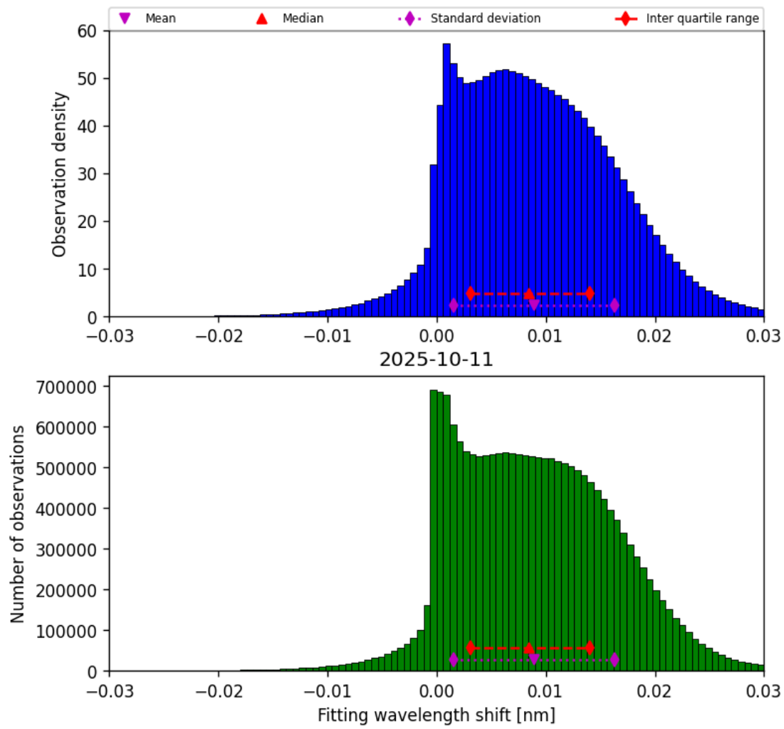
Figure 47: Histogram of “Fitting wavelength shift” for 2025-10-11 to 2025-10-12
