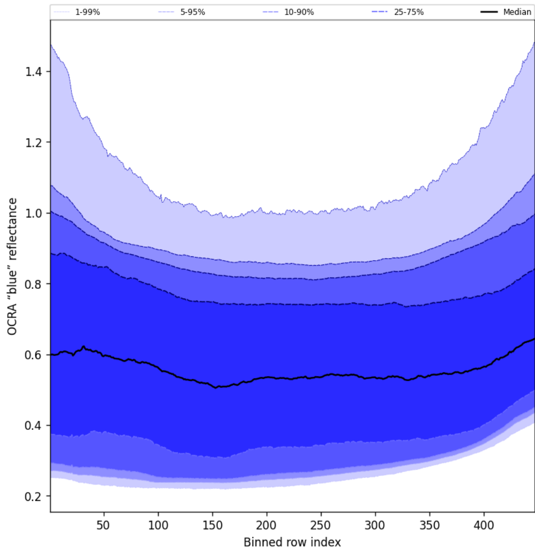
Figure 65: Along track statistics of "OCRA "blue" reflectance" for 2025-10-11 to 2025-10-12
