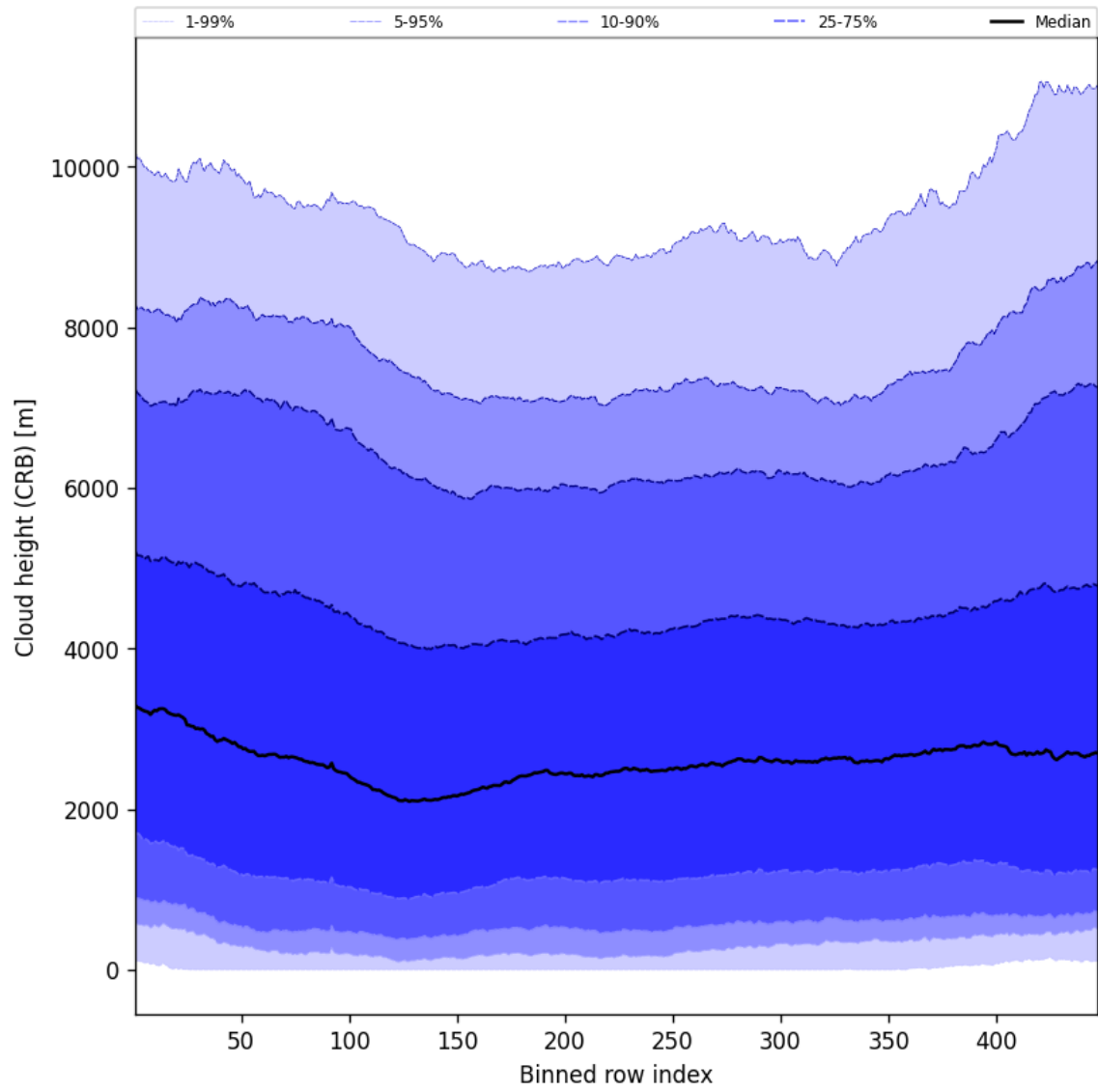
Figure 57: Along track statistics of “Cloud height (CRB)” for 2025-10-11 to 2025-10-12
