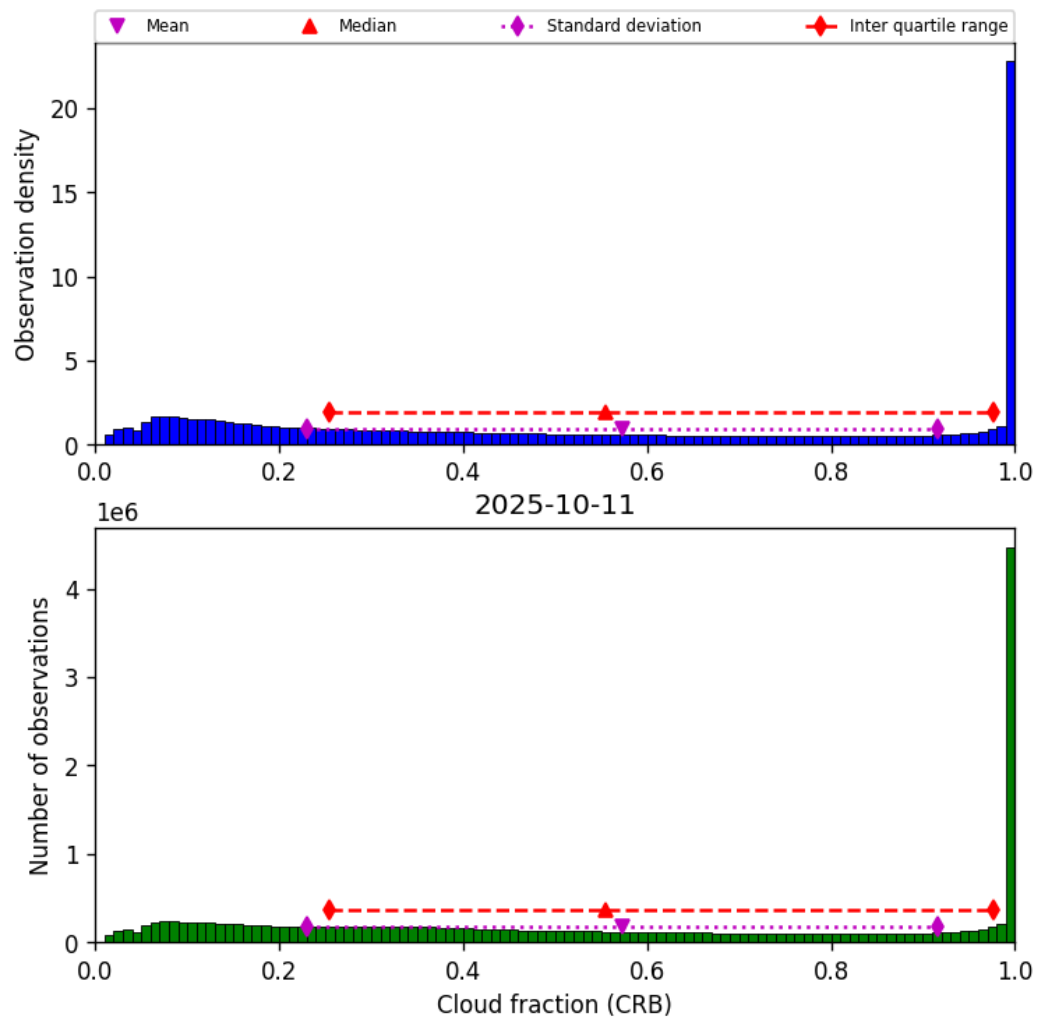
Figure 40: Histogram of “Cloud fraction (CRB)” for 2025-10-11 to 2025-10-12
