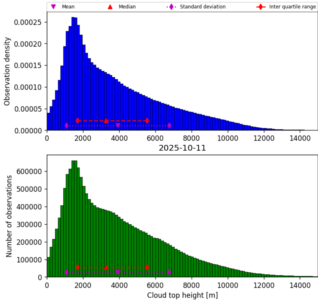
Figure 38: Histogram of “Cloud top height” for 2025-10-11 to 2025-10-12
