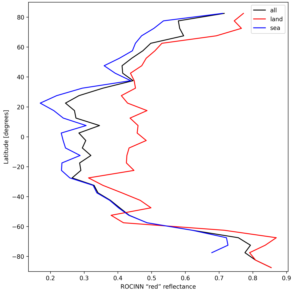
Figure 35: Zonal average of “ROCINN “red” reflectance” for 2025-10-13 to 2025-10-14.
