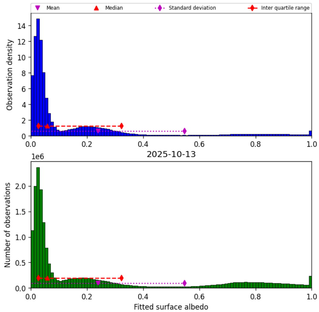
Figure 43: Histogram of “Fitted surface albedo” for 2025-10-13 to 2025-10-14
