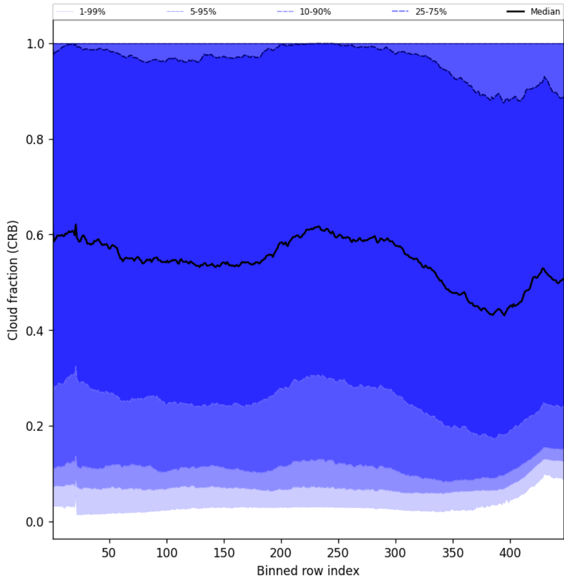
Figure 56: Along track statistics of “Cloud fraction (CRB)” for 2025-10-13 to 2025-10-14
