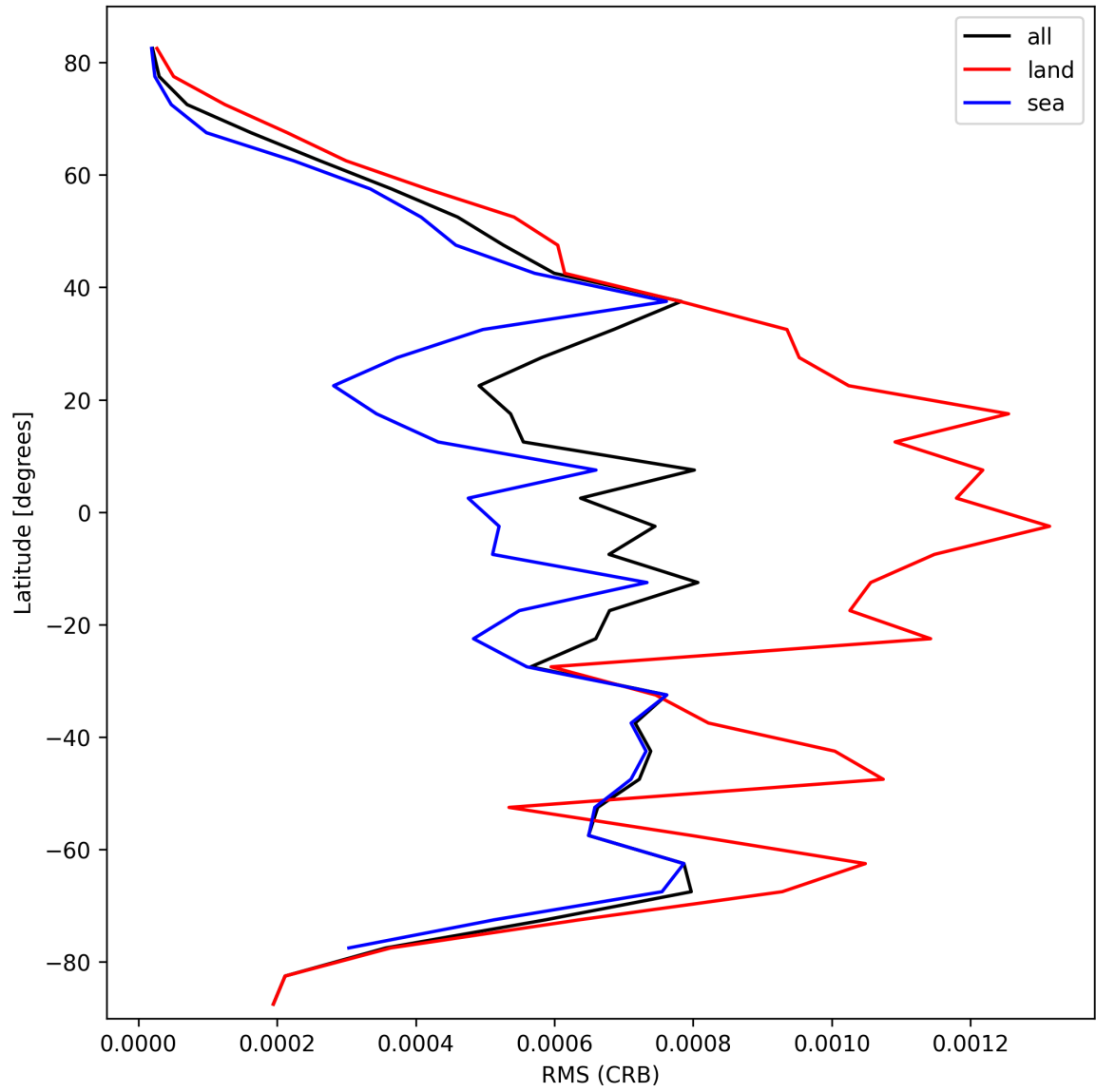
Figure 30: Zonal average of "RMS (CRB)" for 2025-10-13 to 2025-10-14.
