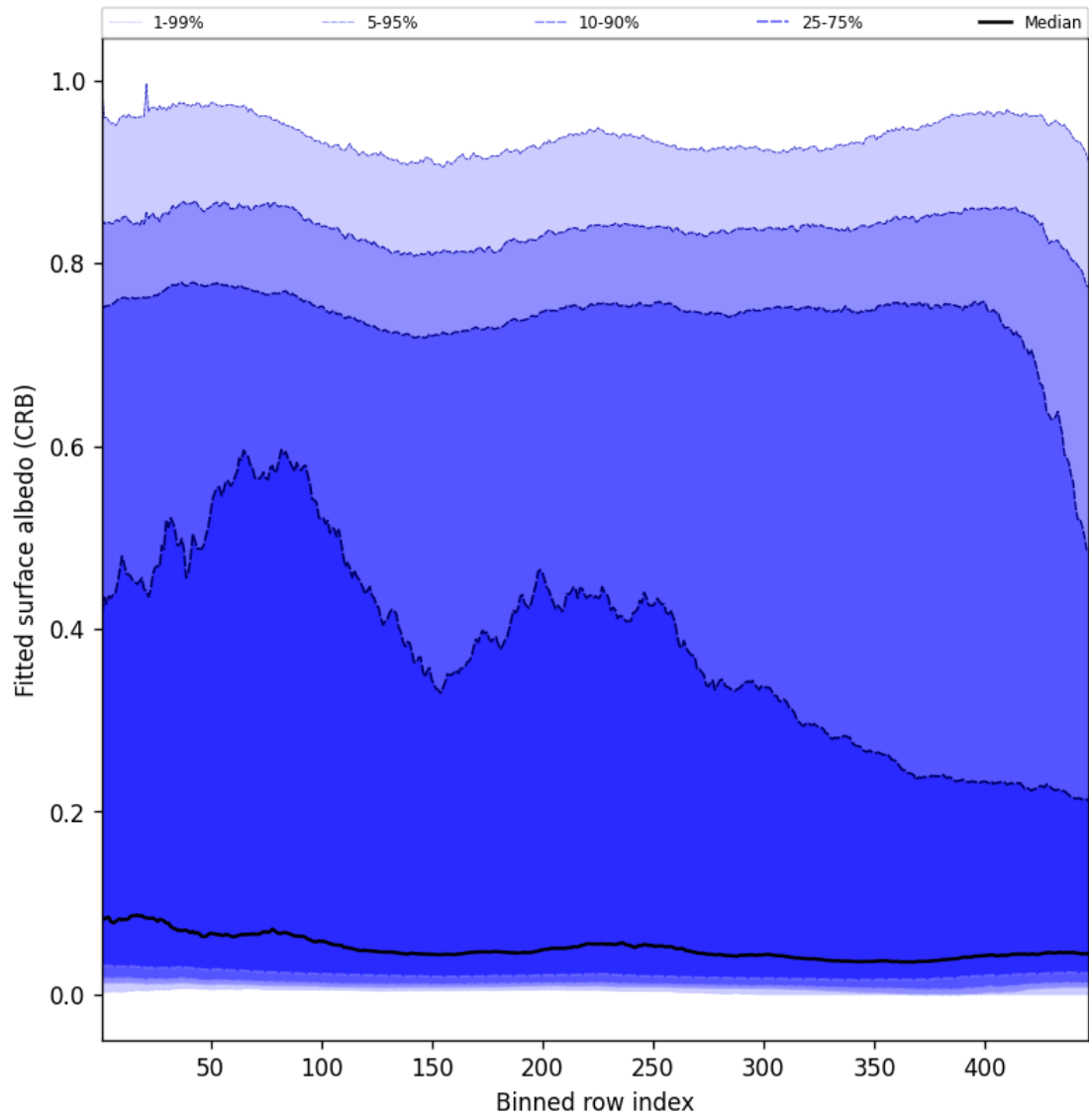
Figure 60: Along track statistics of “Fitted surface albedo (CRB)” for 2025-10-13 to 2025-10-14
