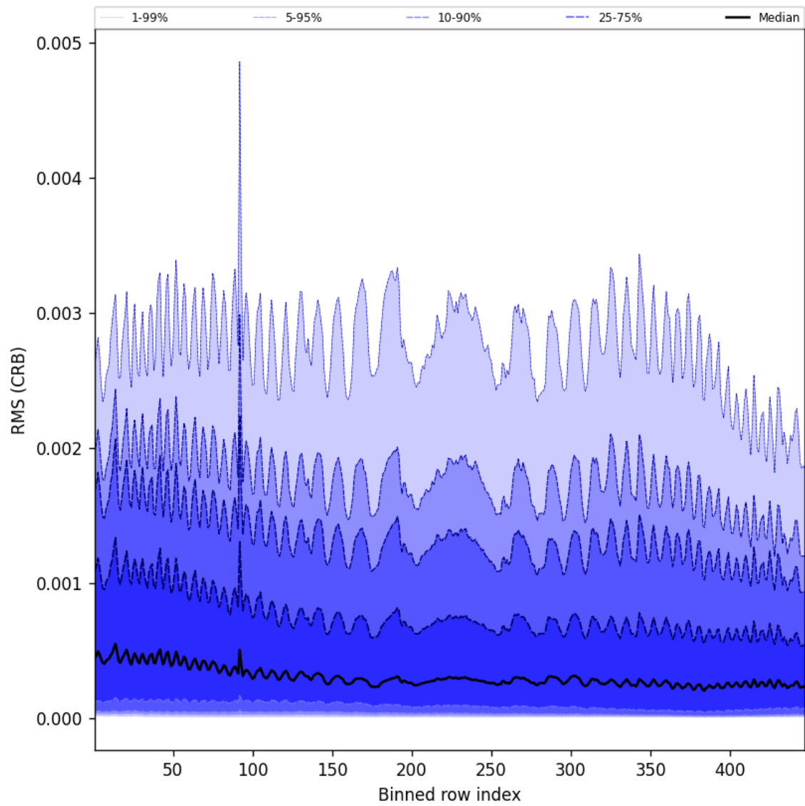
Figure 62: Along track statistics of “RMS (CRB)” for 2025-10-13 to 2025-10-14
