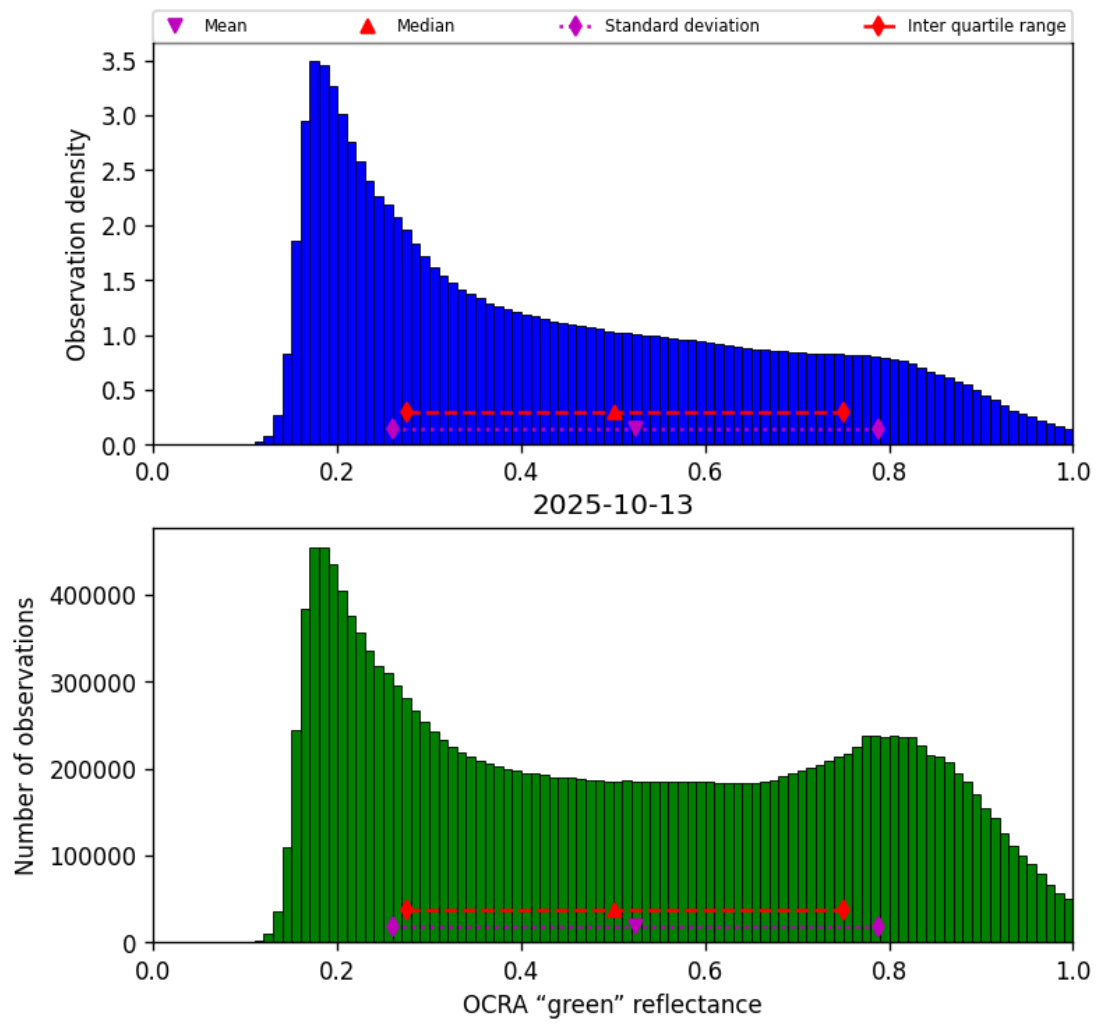
Figure 50: Histogram of “OCRA “green” reflectance” for 2025-10-13 to 2025-10-14
