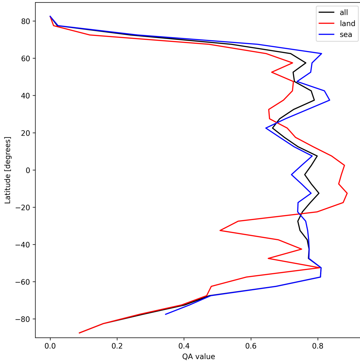
Figure 20: Zonal average of “QA value” for 2025-10-13 to 2025-10-14.
