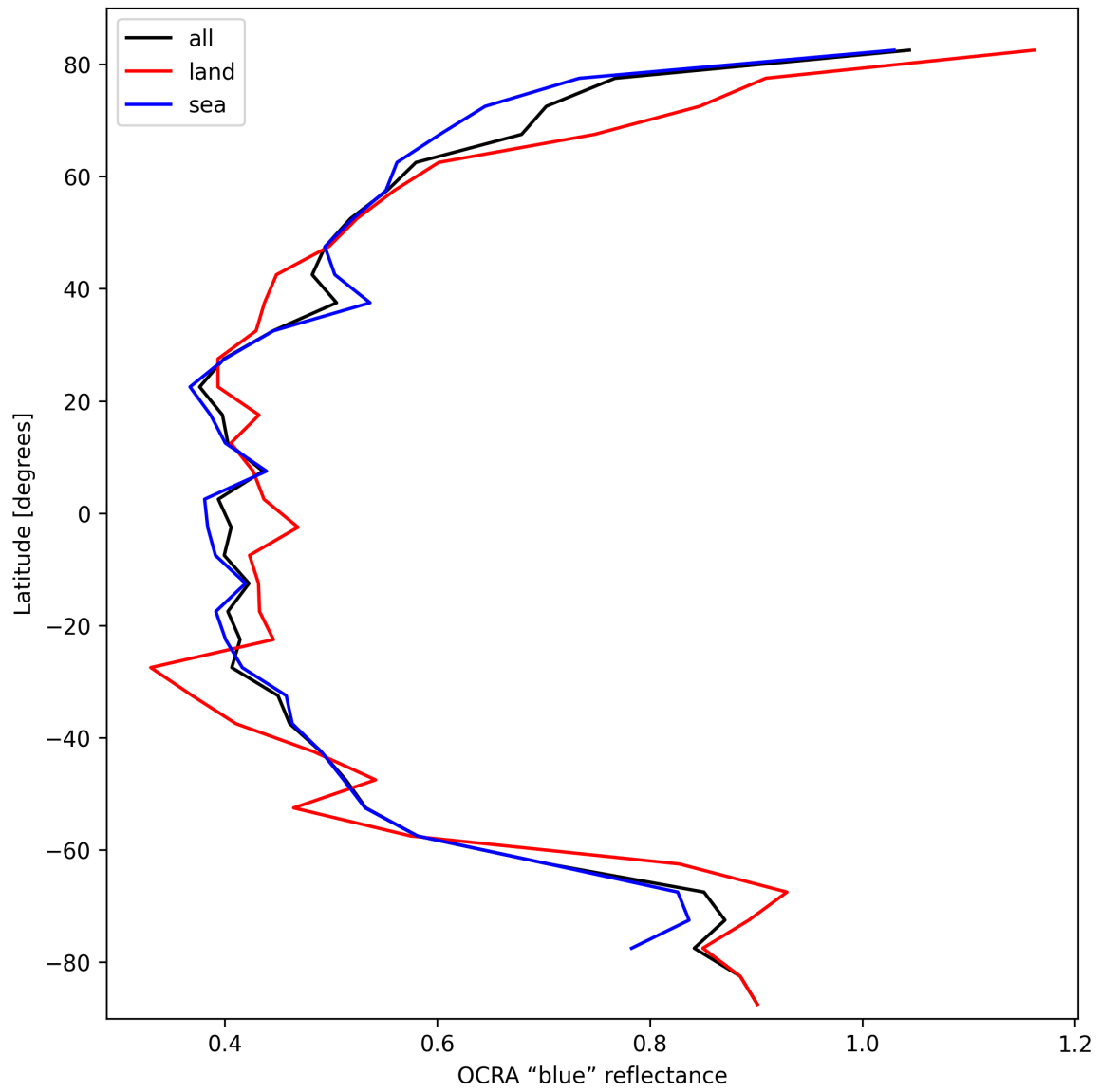
Figure 33: Zonal average of “OCRA “blue” reflectance” for 2025-10-13 to 2025-10-14.
