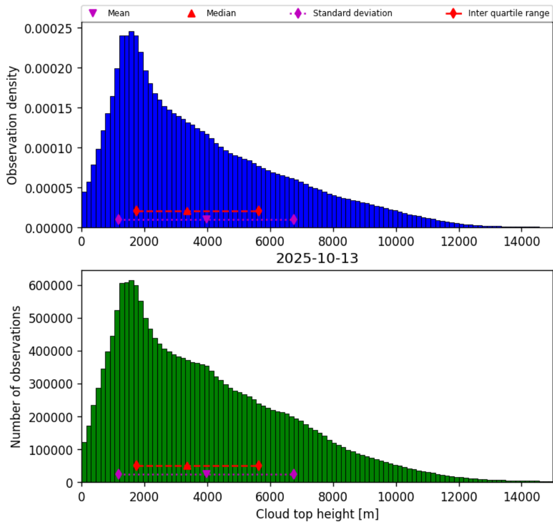
Figure 38: Histogram of “Cloud top height” for 2025-10-13 to 2025-10-14
