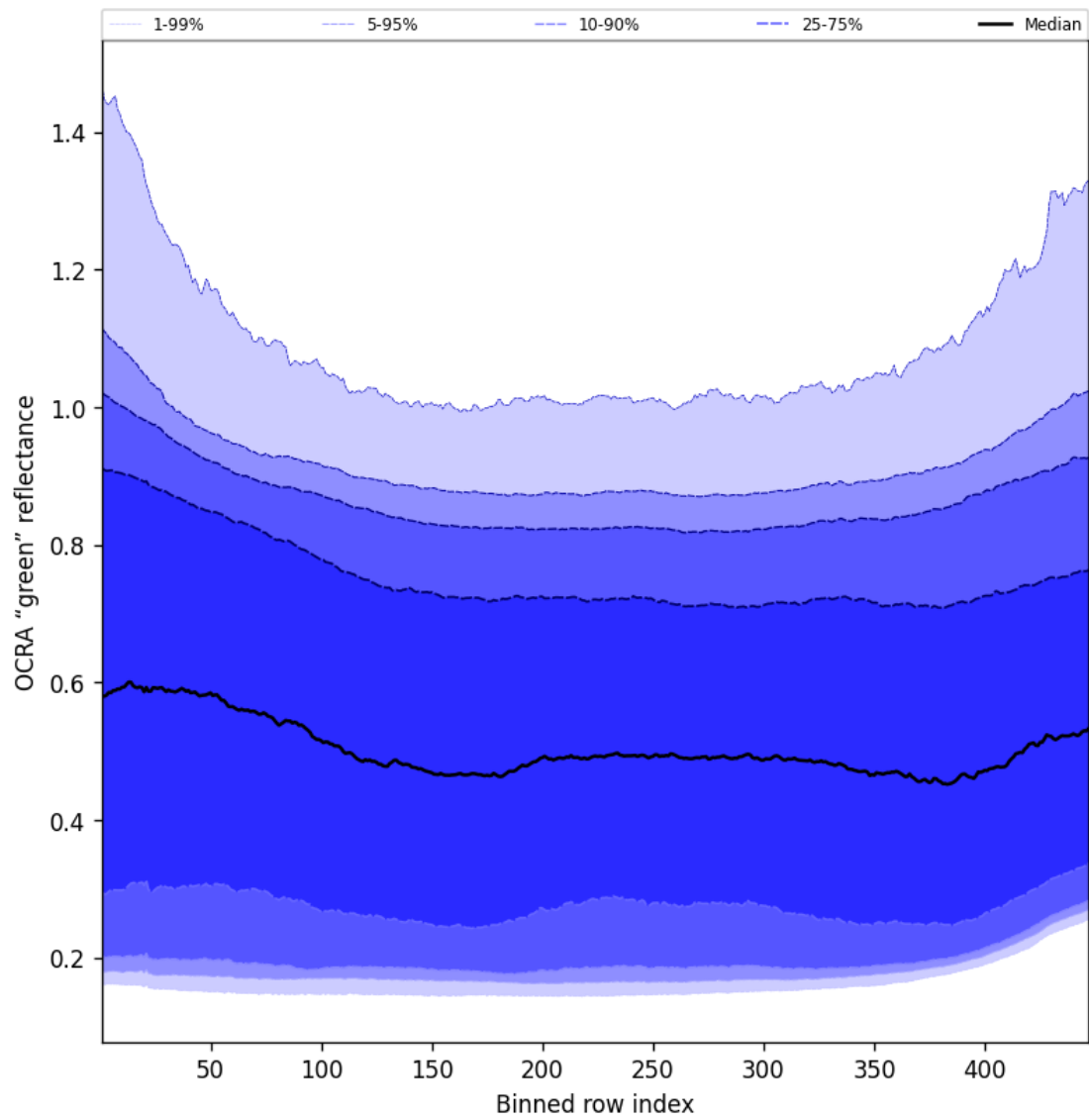
Figure 66: Along track statistics of “OCRA “green” reflectance” for 2025-10-13 to 2025-10-14
