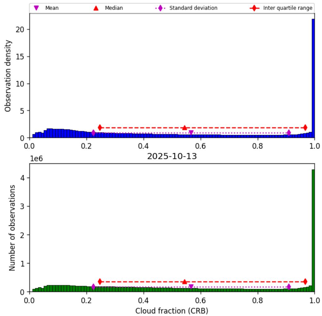
Figure 40: Histogram of “Cloud fraction (CRB)” for 2025-10-13 to 2025-10-14
