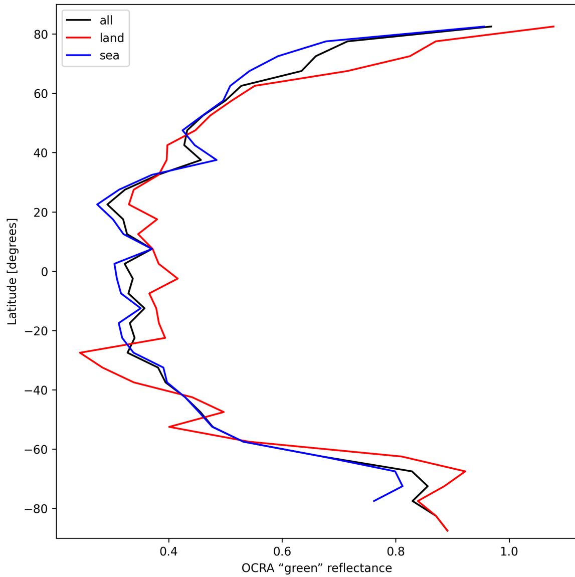
Figure 34: Zonal average of “OCRA “green” reflectance” for 2025-10-13 to 2025-10-14.
