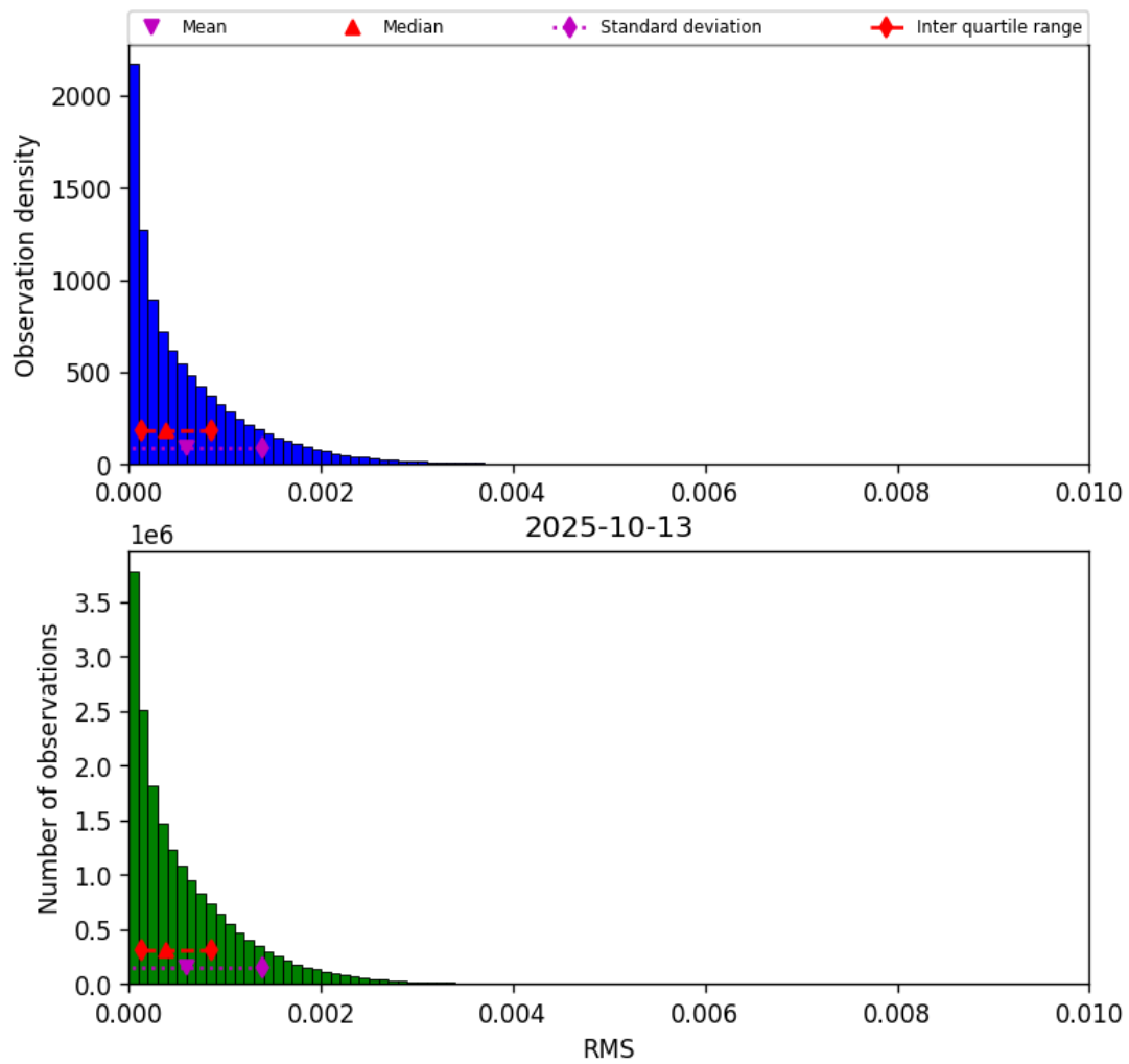
Figure 45: Histogram of “RMS” for 2025-10-13 to 2025-10-14
