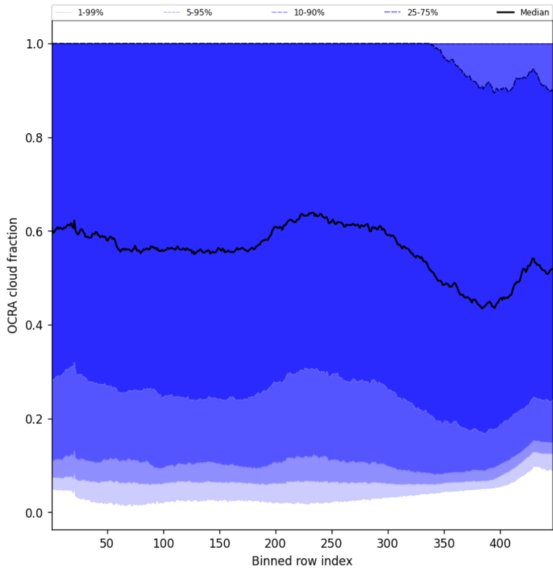
Figure 64: Along track statistics of “OCRA cloud fraction” for 2025-10-13 to 2025-10-14
