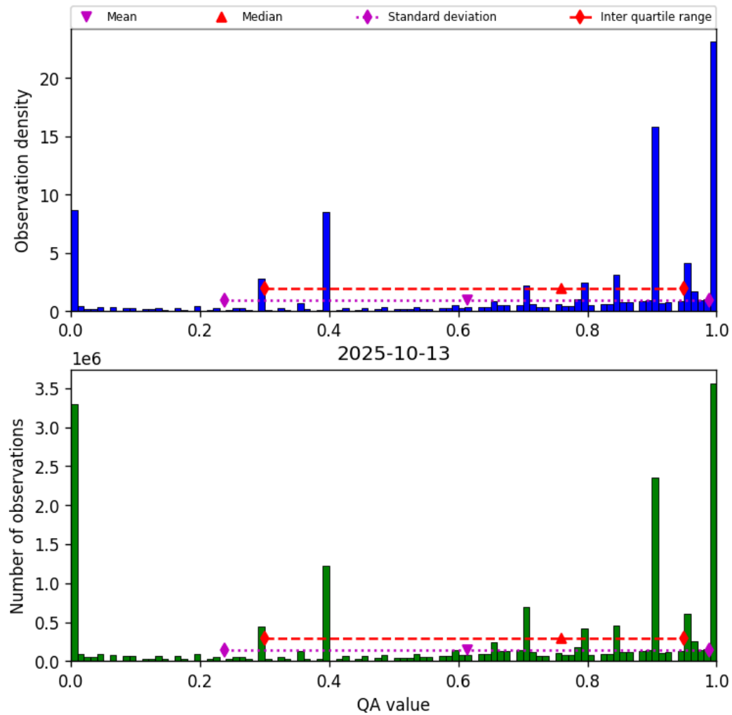
Figure 36: Histogram of “QA value” for 2025-10-13 to 2025-10-14
