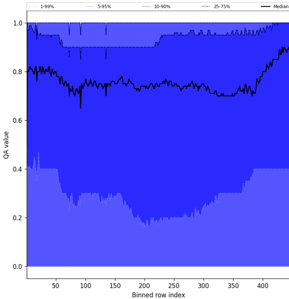
Figure 52: Along track statistics of “QA value” for 2025-10-13 to 2025-10-14
