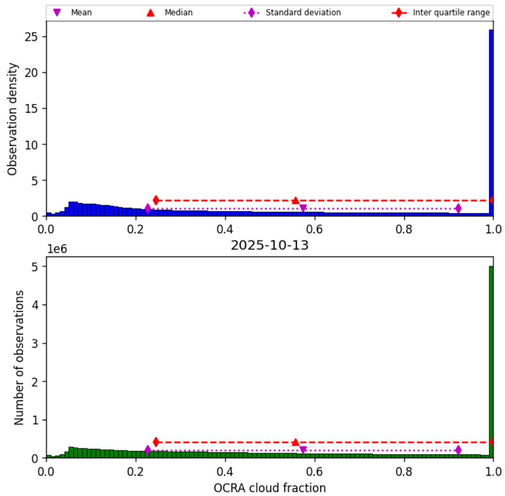
Figure 48: Histogram of “OCRA cloud fraction” for 2025-10-13 to 2025-10-14
