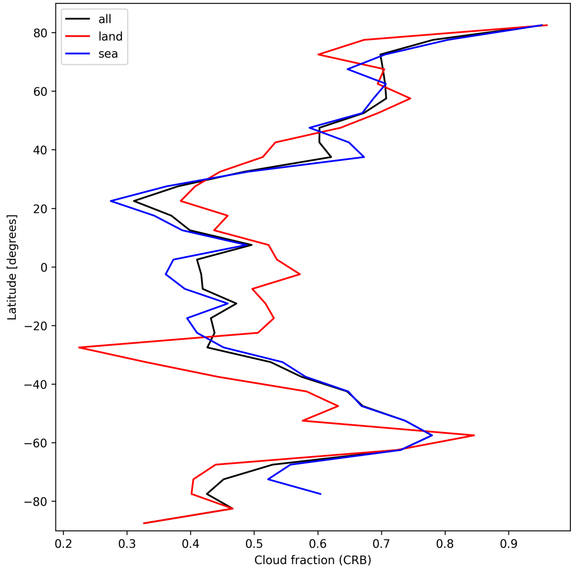
Figure 24: Zonal average of “Cloud fraction (CRB)” for 2025-10-13 to 2025-10-14.
