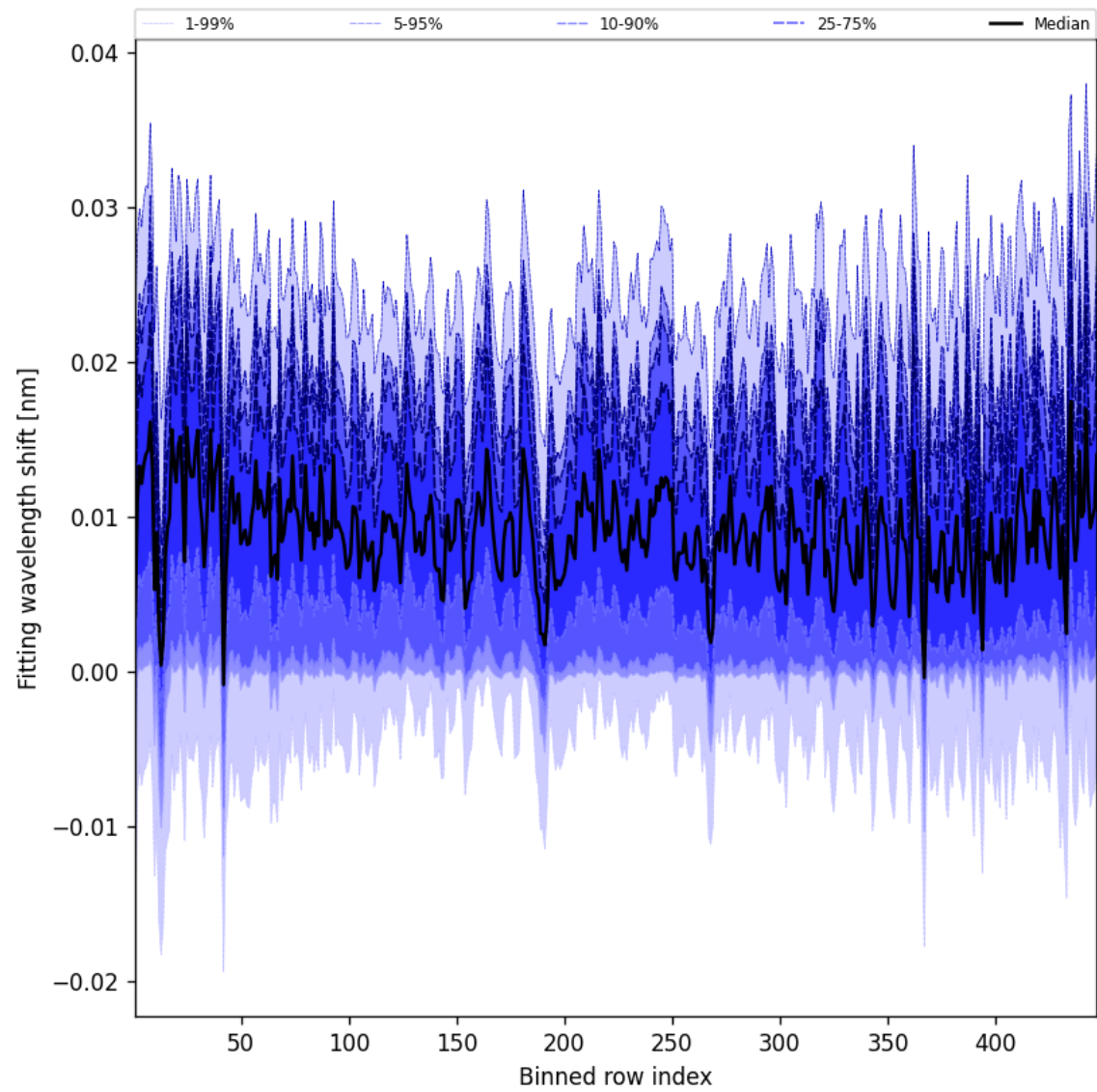
Figure 63: Along track statistics of “Fitting wavelength shift” for 2025-10-13 to 2025-10-14
