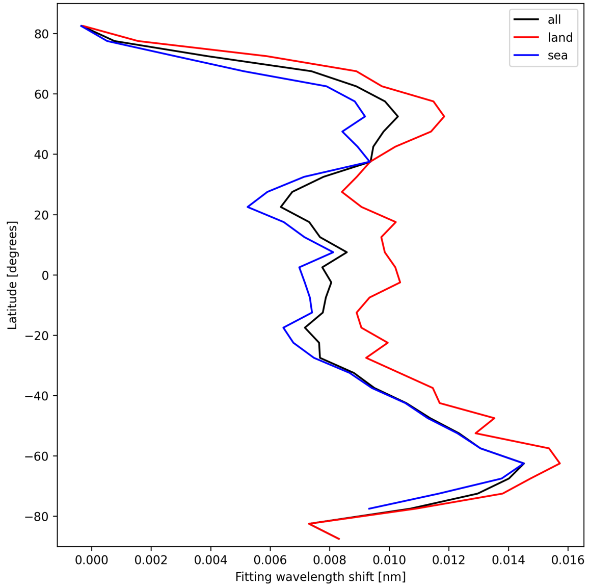
Figure 31: Zonal average of “Fitting wavelength shift” for 2025-10-13 to 2025-10-14.
