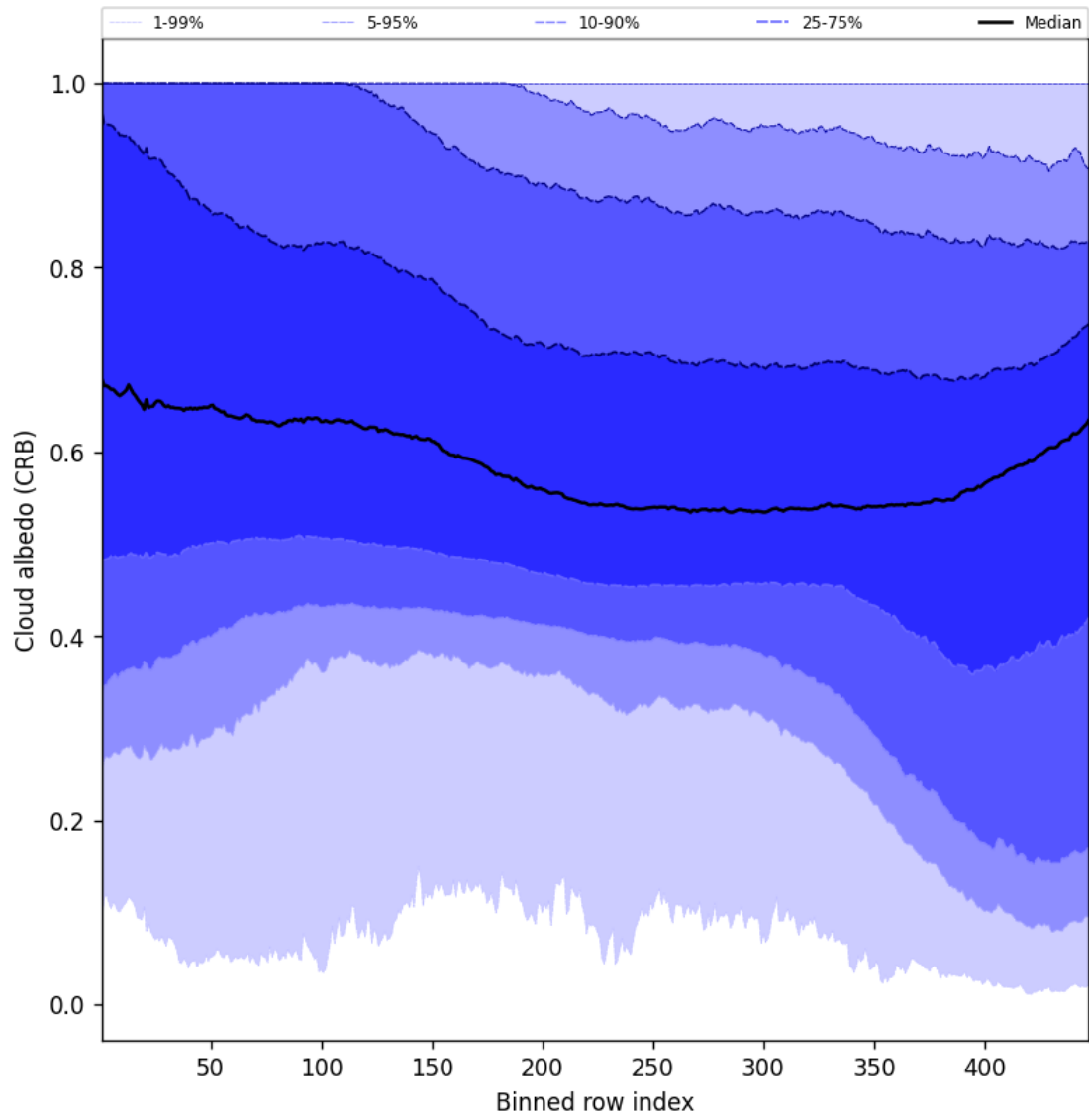
Figure 58: Along track statistics of “Cloud albedo (CRB)” for 2025-10-13 to 2025-10-14
