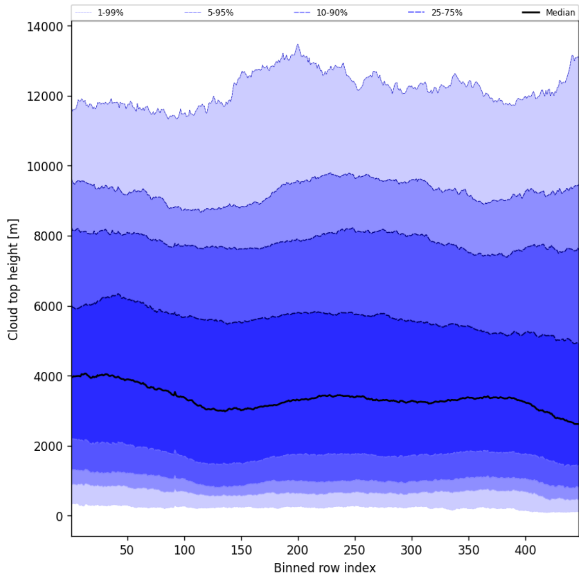
Figure 54: Along track statistics of “Cloud top height” for 2025-10-13 to 2025-10-14
