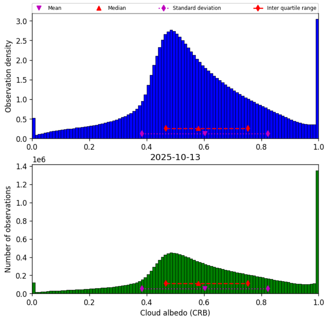
Figure 42: Histogram of “Cloud albedo (CRB)” for 2025-10-13 to 2025-10-14
