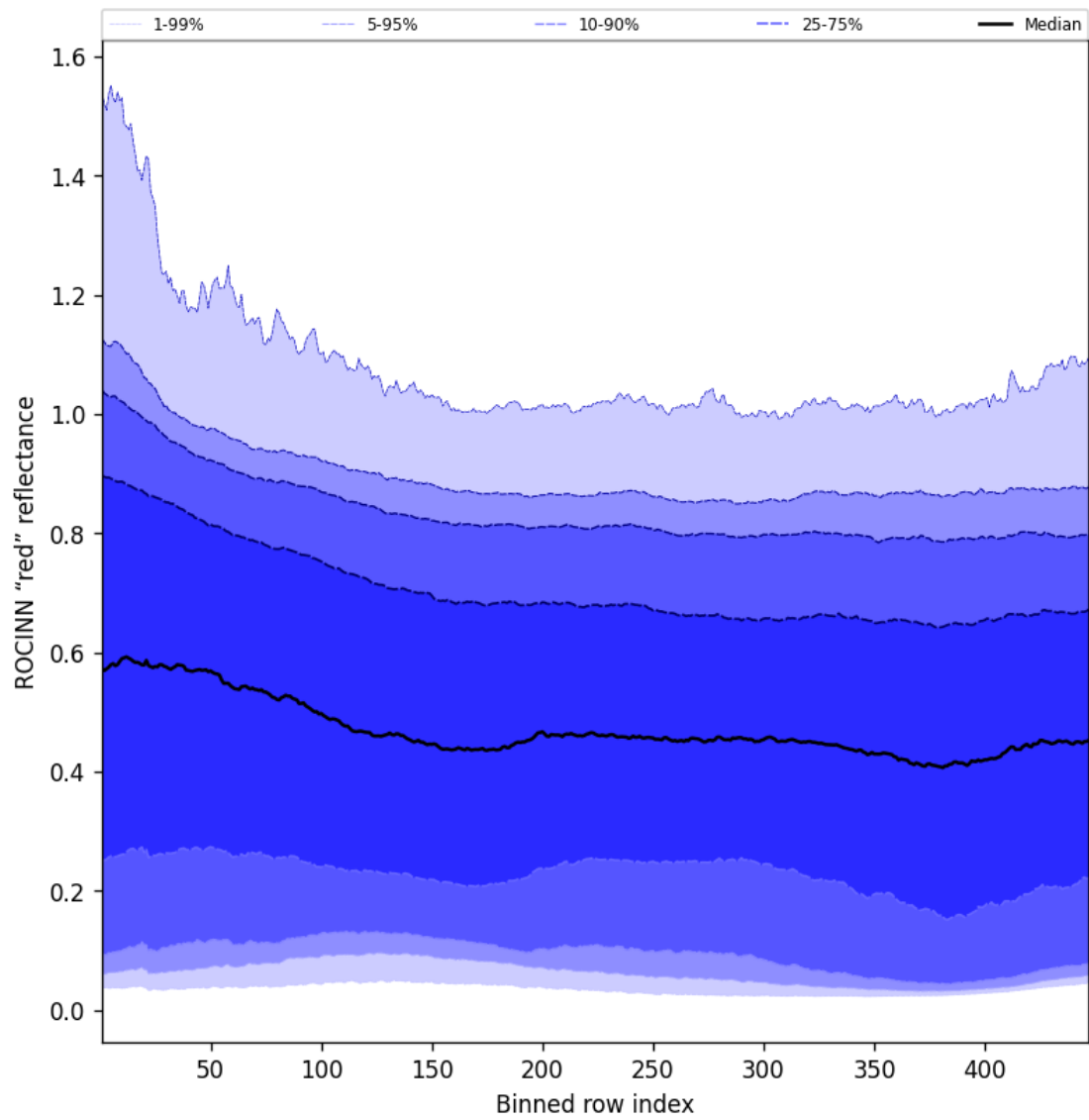
Figure 67: Along track statistics of "ROCINN "red" reflectance" for 2025-10-13 to 2025-10-14
