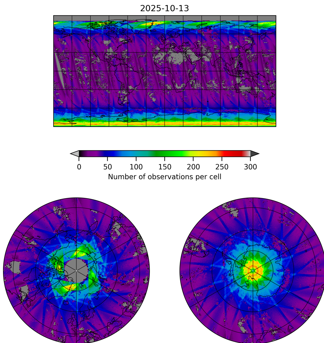
Figure 19: Map of the number of observations for 2025-10-13 to 2025-10-14
