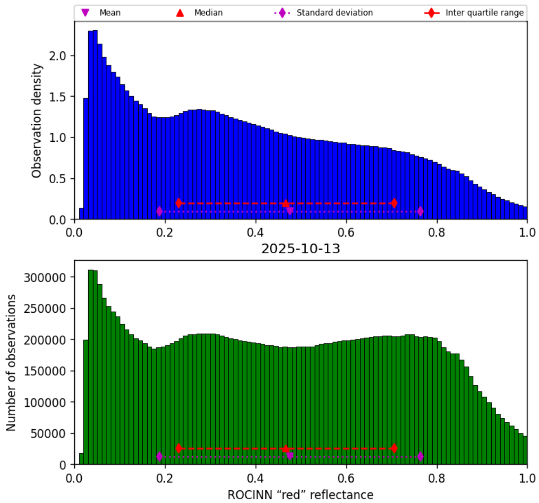
Figure 51: Histogram of “ROCINN “red” reflectance” for 2025-10-13 to 2025-10-14
