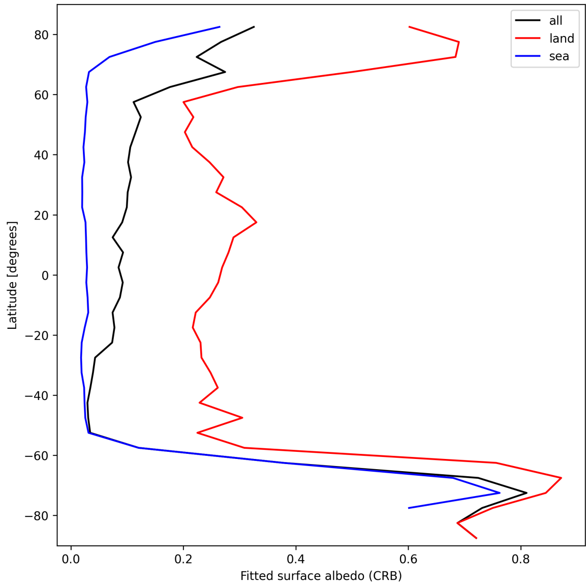
Figure 28: Zonal average of “Fitted surface albedo (CRB)” for 2025-10-13 to 2025-10-14.
