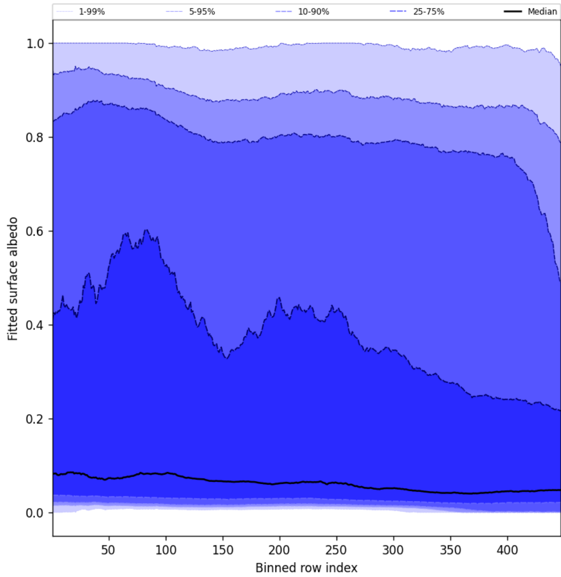
Figure 59: Along track statistics of “Fitted surface albedo” for 2025-10-13 to 2025-10-14
