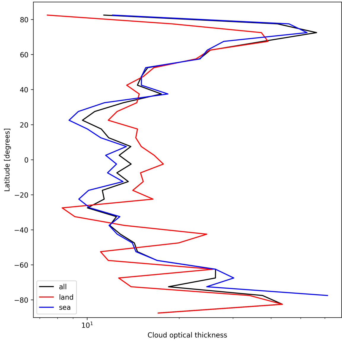
Figure 23: Zonal average of “Cloud optical thickness” for 2025-10-13 to 2025-10-14.
