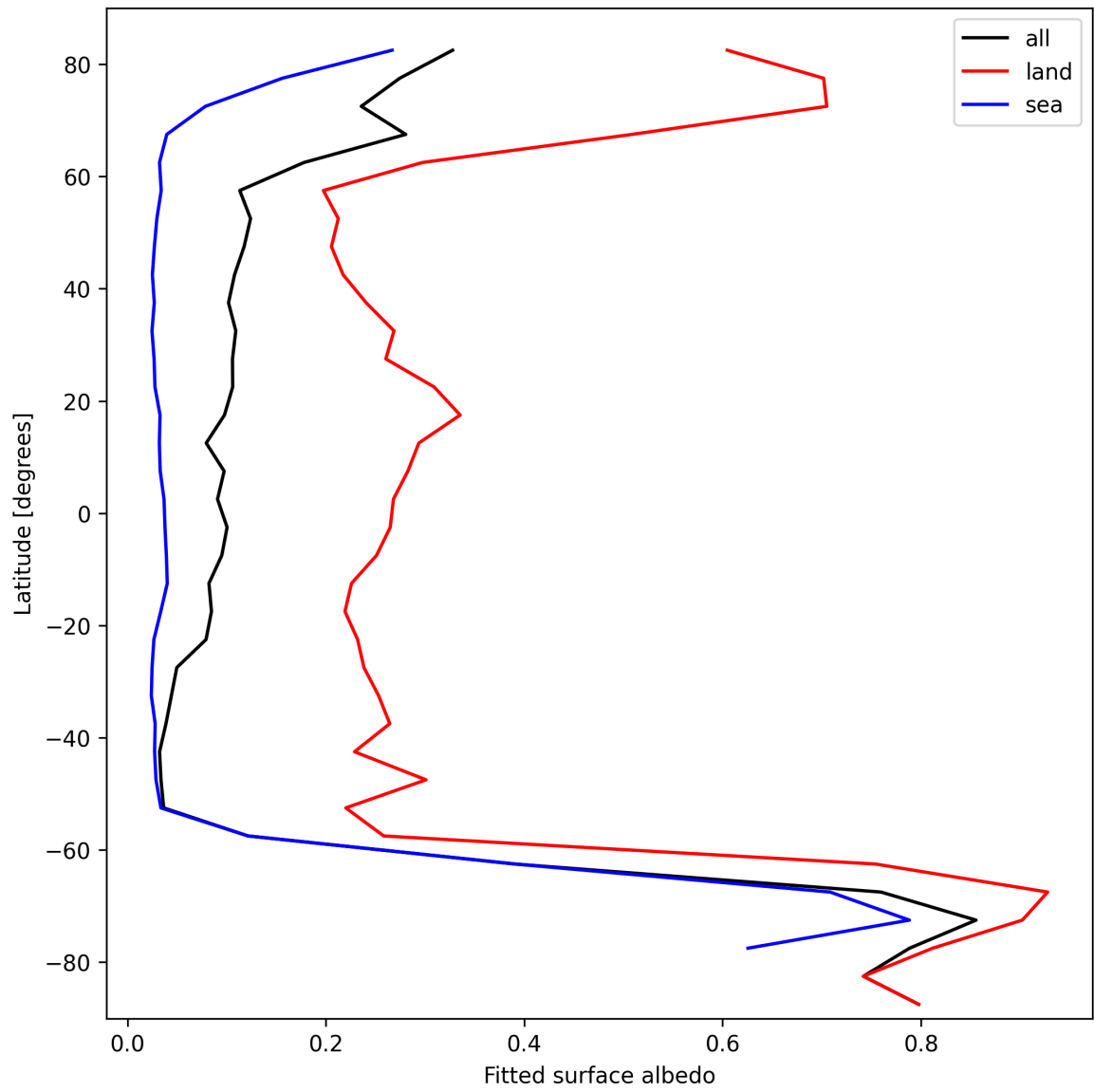
Figure 27: Zonal average of “Fitted surface albedo” for 2025-10-13 to 2025-10-14.
