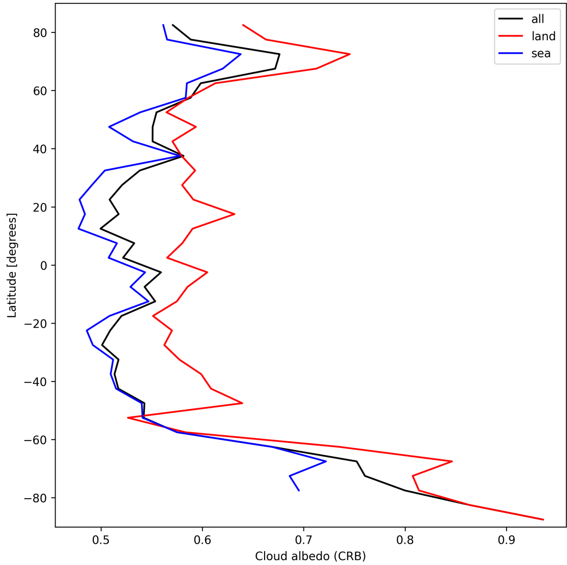
Figure 26: Zonal average of “Cloud albedo (CRB)” for 2025-10-13 to 2025-10-14.
