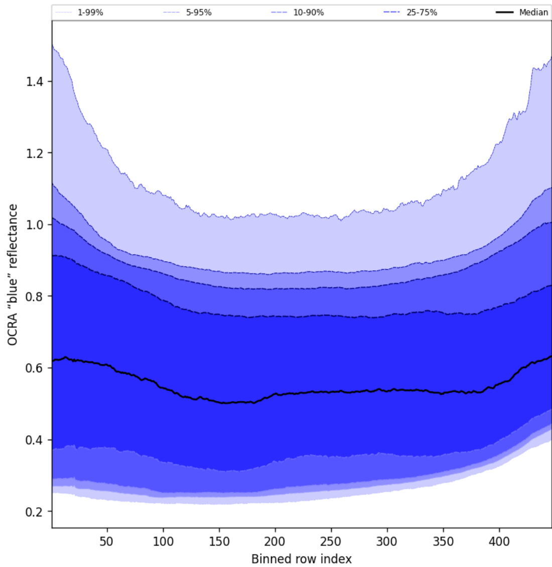
Figure 65: Along track statistics of “OCRA “blue” reflectance” for 2025-10-13 to 2025-10-14
