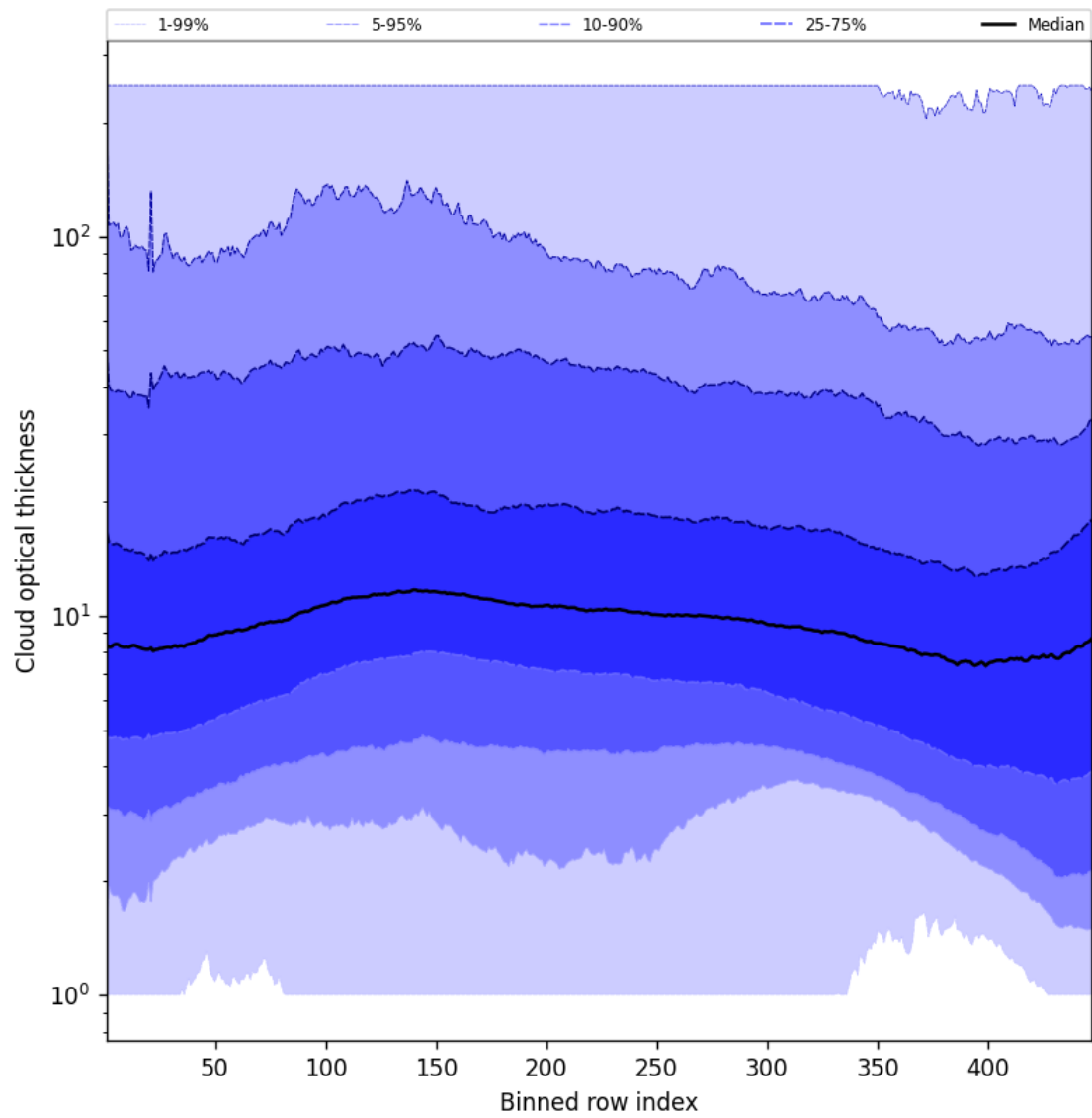
Figure 55: Along track statistics of “Cloud optical thickness” for 2025-10-13 to 2025-10-14
