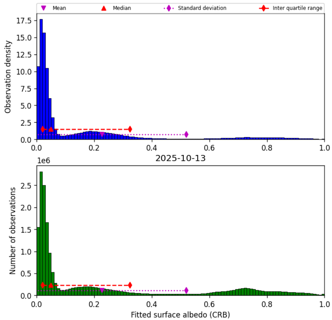
Figure 44: Histogram of “Fitted surface albedo (CRB)” for 2025-10-13 to 2025-10-14
