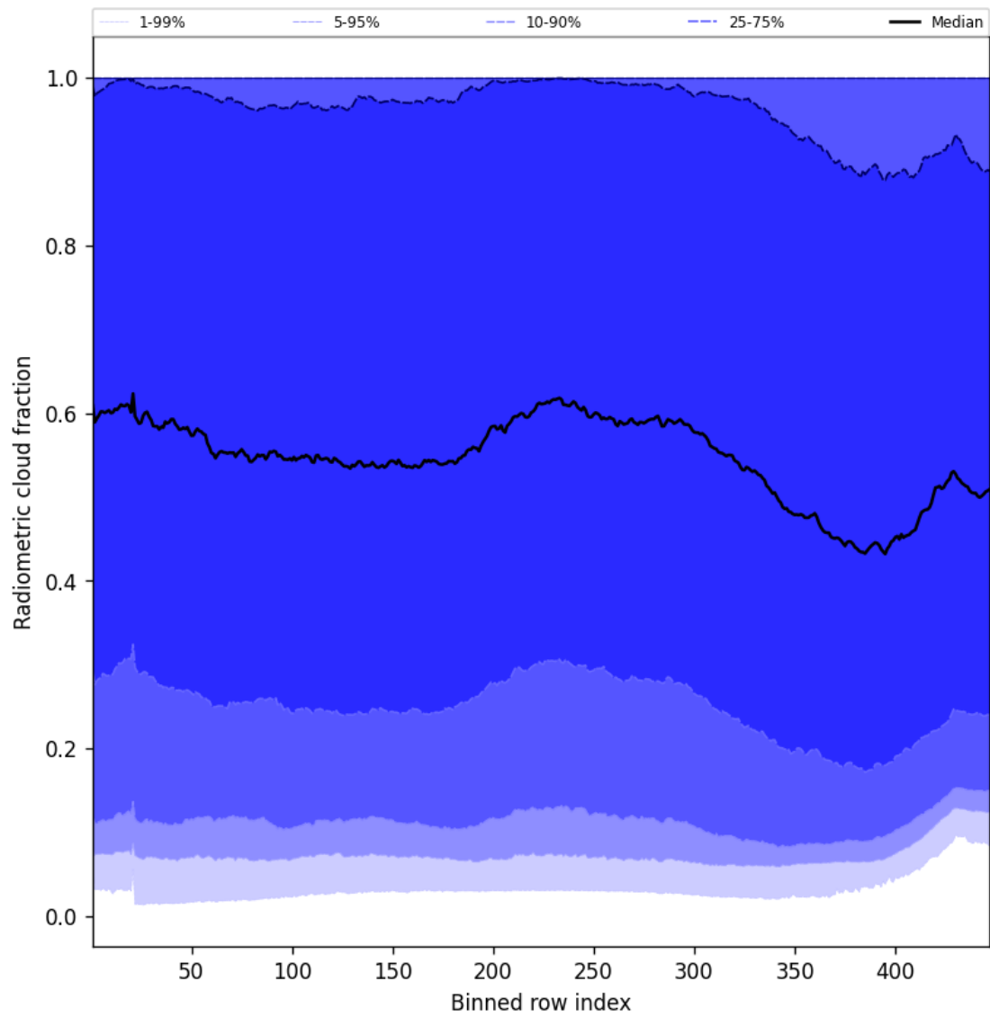
Figure 53: Along track statistics of “Radiometric cloud fraction” for 2025-10-13 to 2025-10-14
