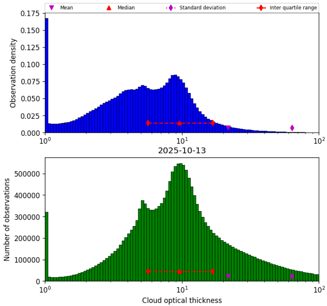
Figure 39: Histogram of “Cloud optical thickness” for 2025-10-13 to 2025-10-14
