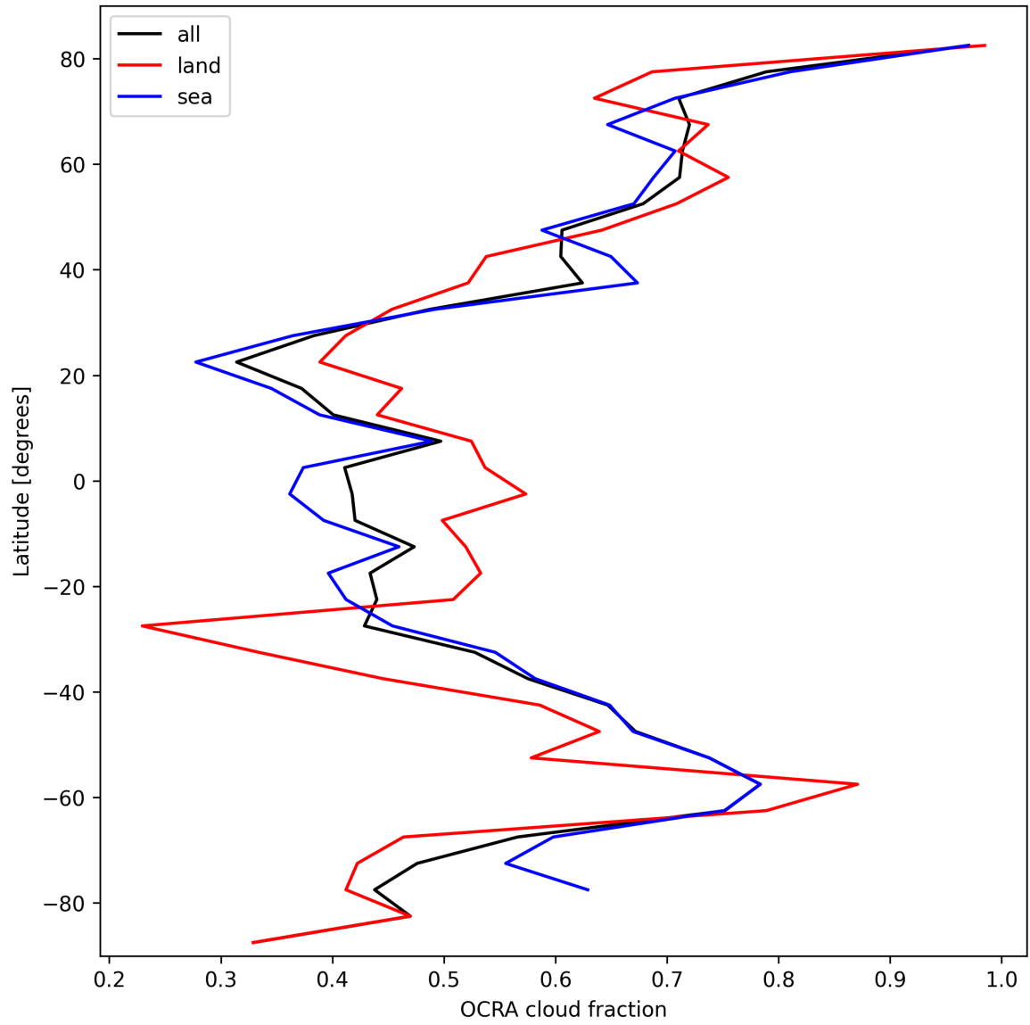
Figure 32: Zonal average of “OCRA cloud fraction” for 2025-10-13 to 2025-10-14.
