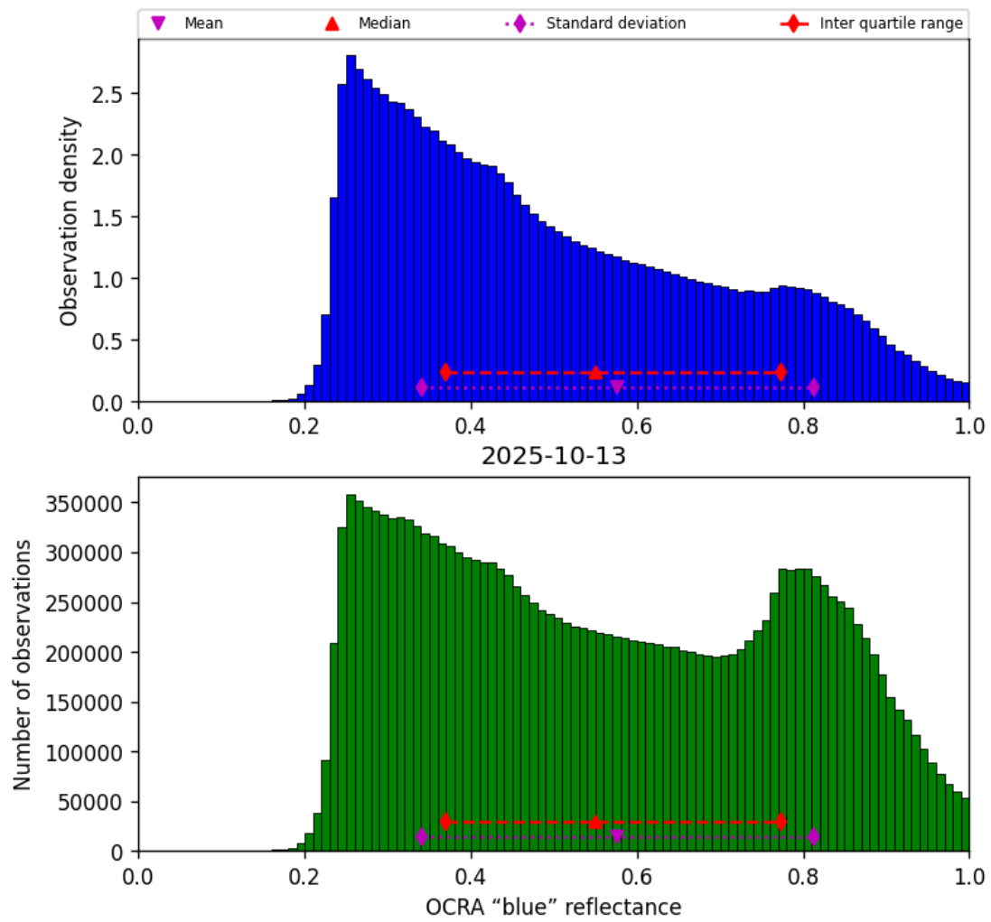
Figure 49: Histogram of “OCRA “blue” reflectance” for 2025-10-13 to 2025-10-14
