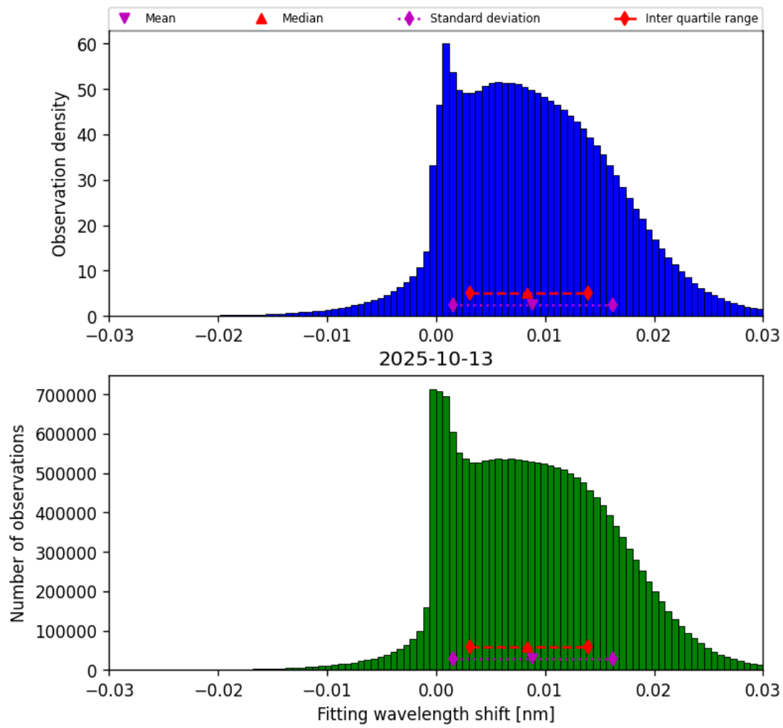
Figure 47: Histogram of “Fitting wavelength shift” for 2025-10-13 to 2025-10-14
