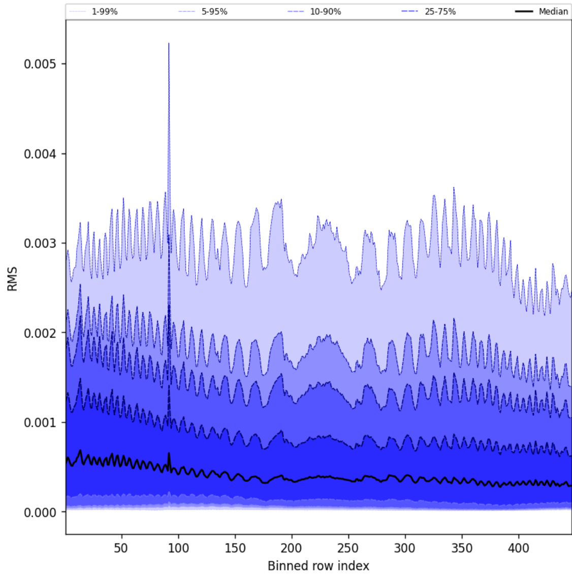
Figure 61: Along track statistics of “RMS” for 2025-10-13 to 2025-10-14
