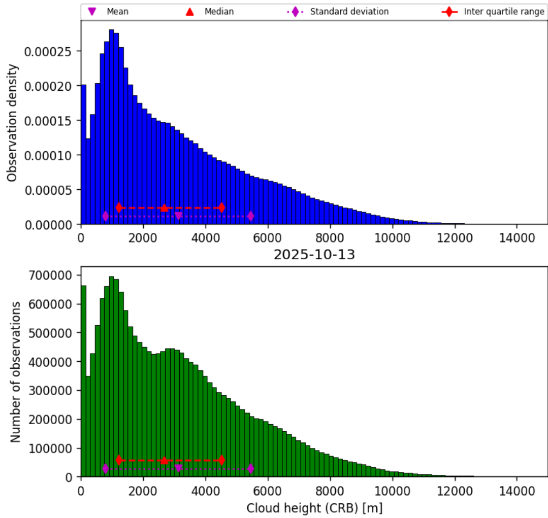
Figure 41: Histogram of “Cloud height (CRB)” for 2025-10-13 to 2025-10-14
