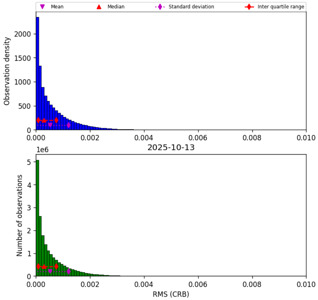
Figure 46: Histogram of “RMS (CRB)” for 2025-10-13 to 2025-10-14
