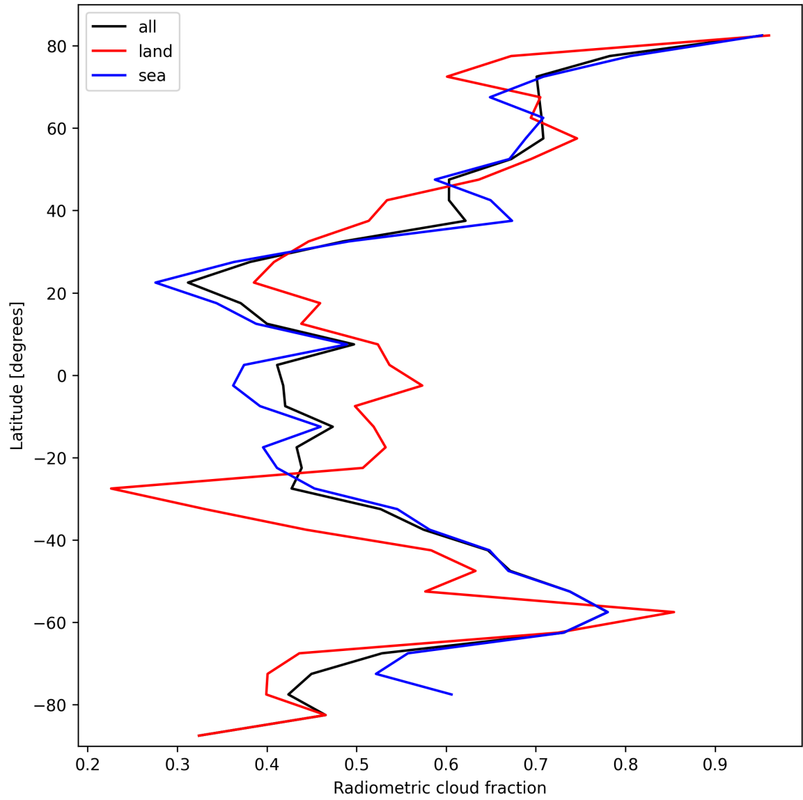
Figure 21: Zonal average of “Radiometric cloud fraction” for 2025-10-13 to 2025-10-14.
