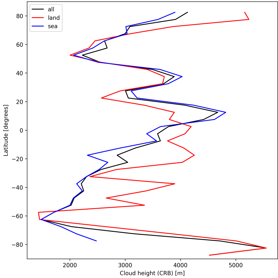
Figure 25: Zonal average of “Cloud height (CRB)” for 2025-10-13 to 2025-10-14.
