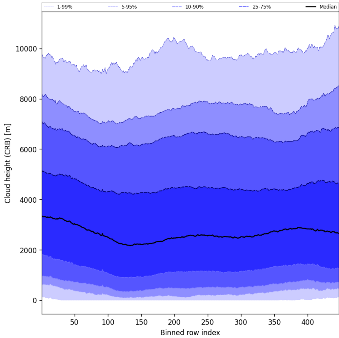
Figure 57: Along track statistics of “Cloud height (CRB)” for 2025-10-13 to 2025-10-14
