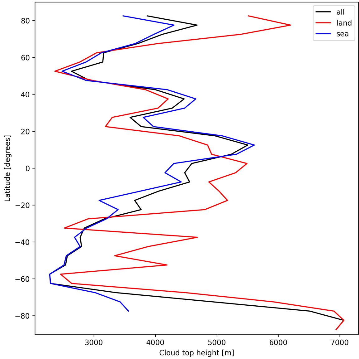
Figure 22: Zonal average of “Cloud top height” for 2025-10-13 to 2025-10-14.
