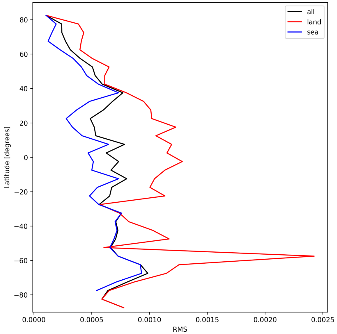
Figure 29: Zonal average of “RMS” for 2025-10-13 to 2025-10-14.
