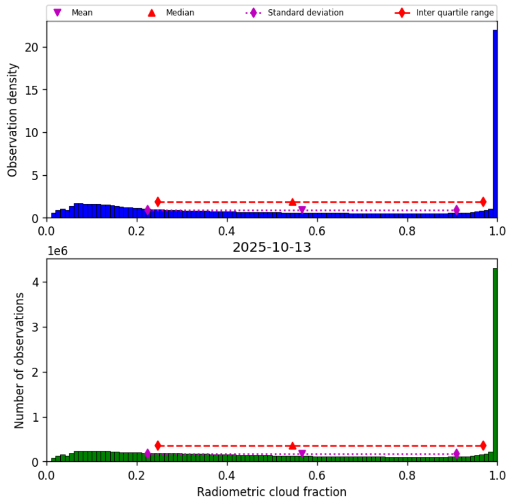
Figure 37: Histogram of “Radiometric cloud fraction” for 2025-10-13 to 2025-10-14
