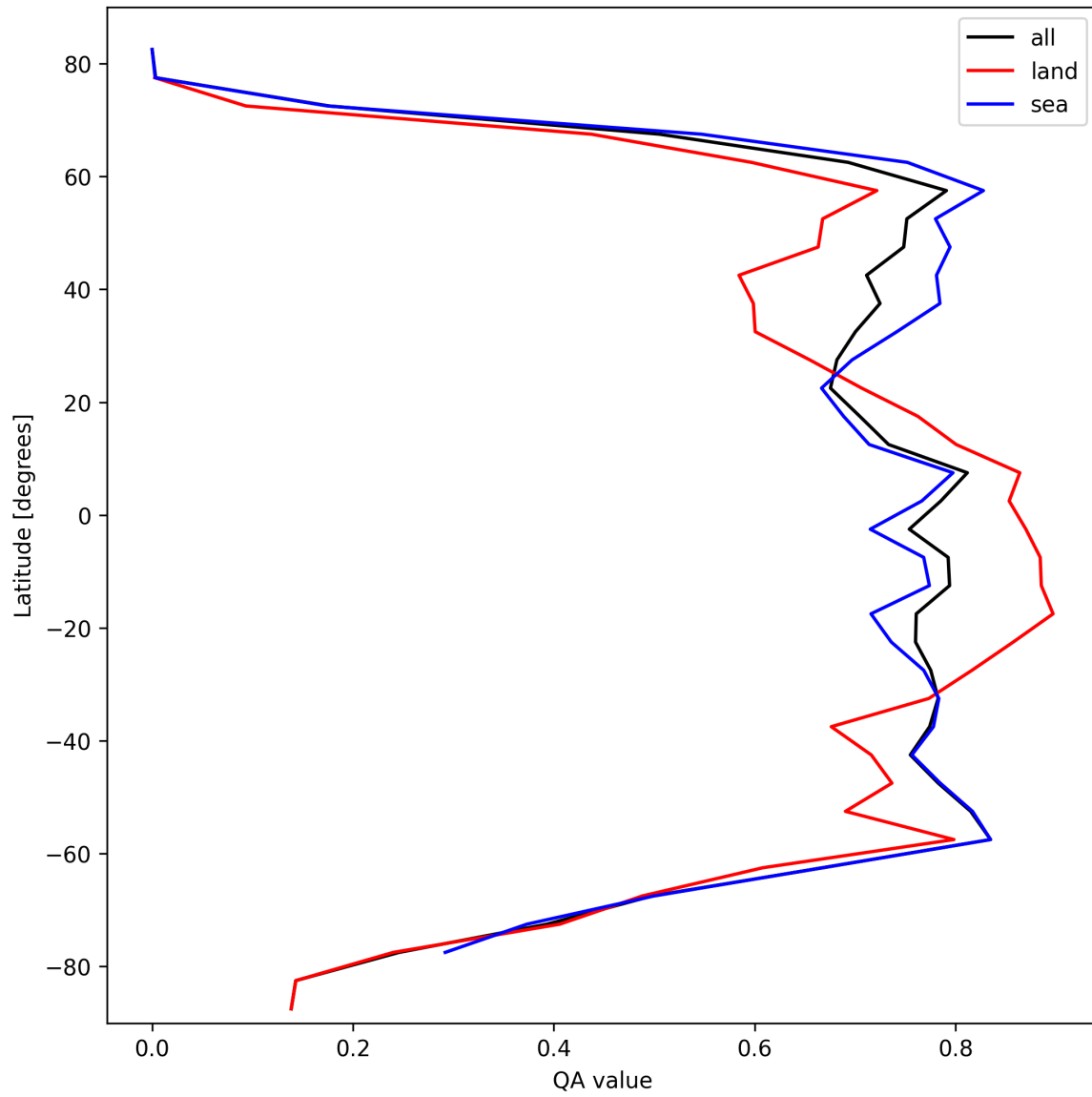
Figure 20: Zonal average of “QA value” for 2025-10-16 to 2025-10-17.
