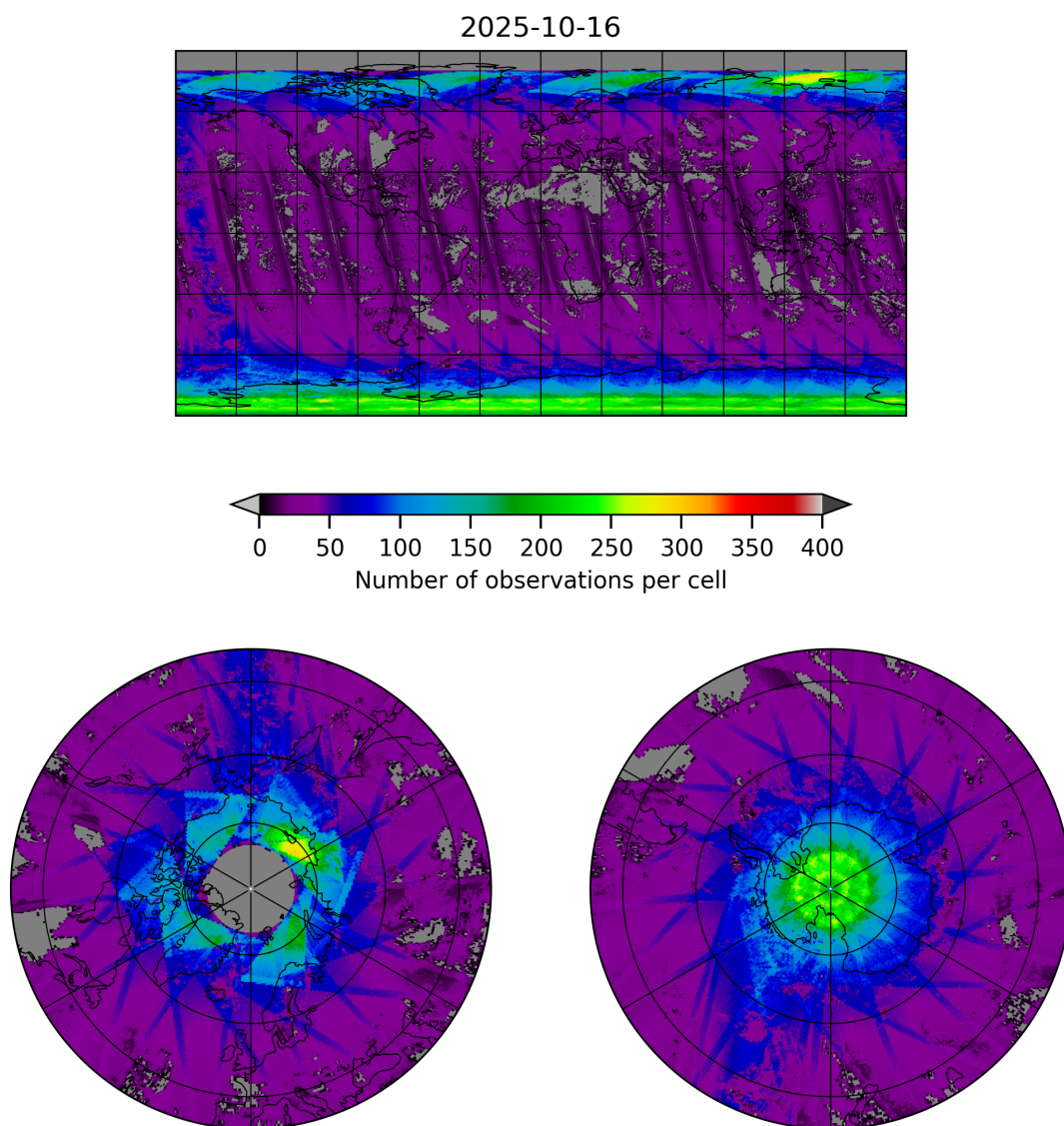
Figure 19: Map of the number of observations for 2025-10-16 to 2025-10-17
