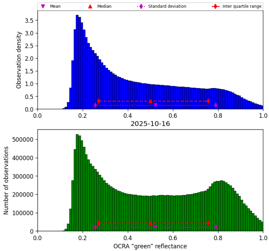
Figure 50: Histogram of “OCRA “green” reflectance” for 2025-10-16 to 2025-10-17
