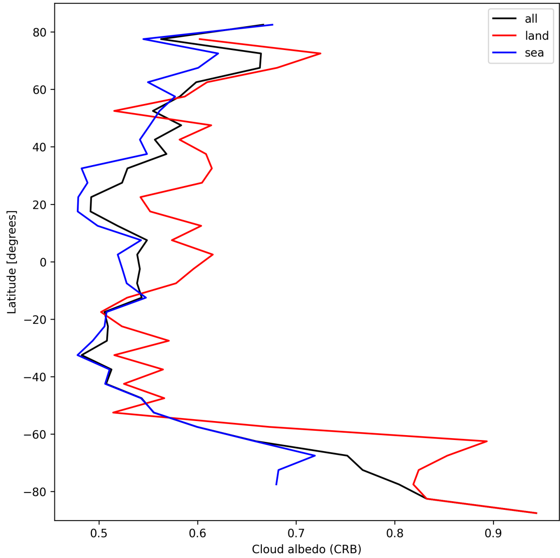
Figure 26: Zonal average of “Cloud albedo (CRB)” for 2025-10-16 to 2025-10-17.
