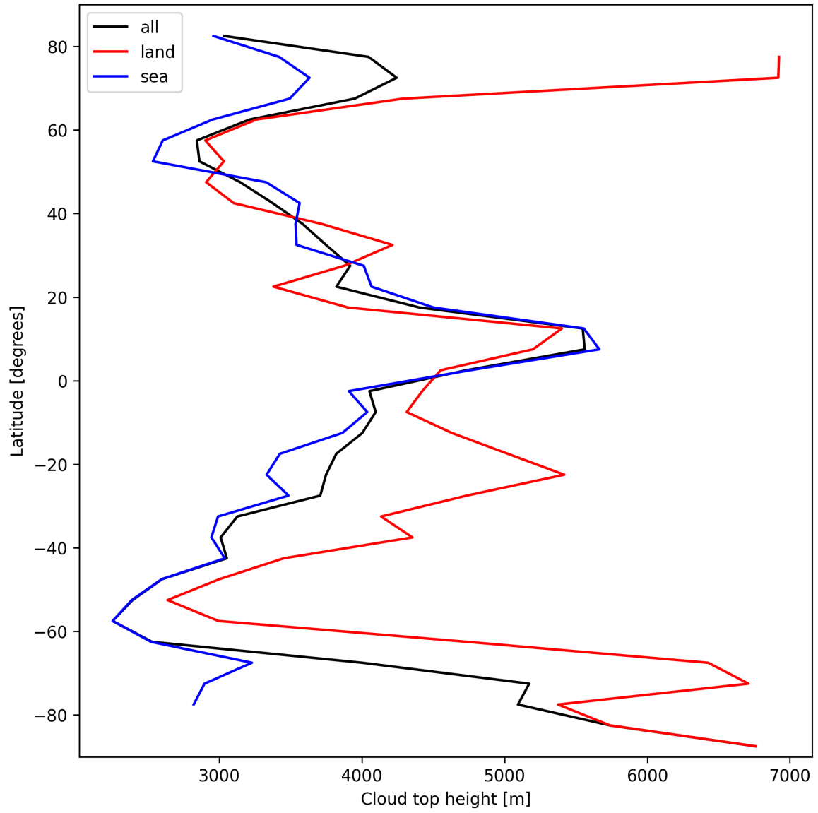
Figure 22: Zonal average of “Cloud top height” for 2025-10-16 to 2025-10-17.
