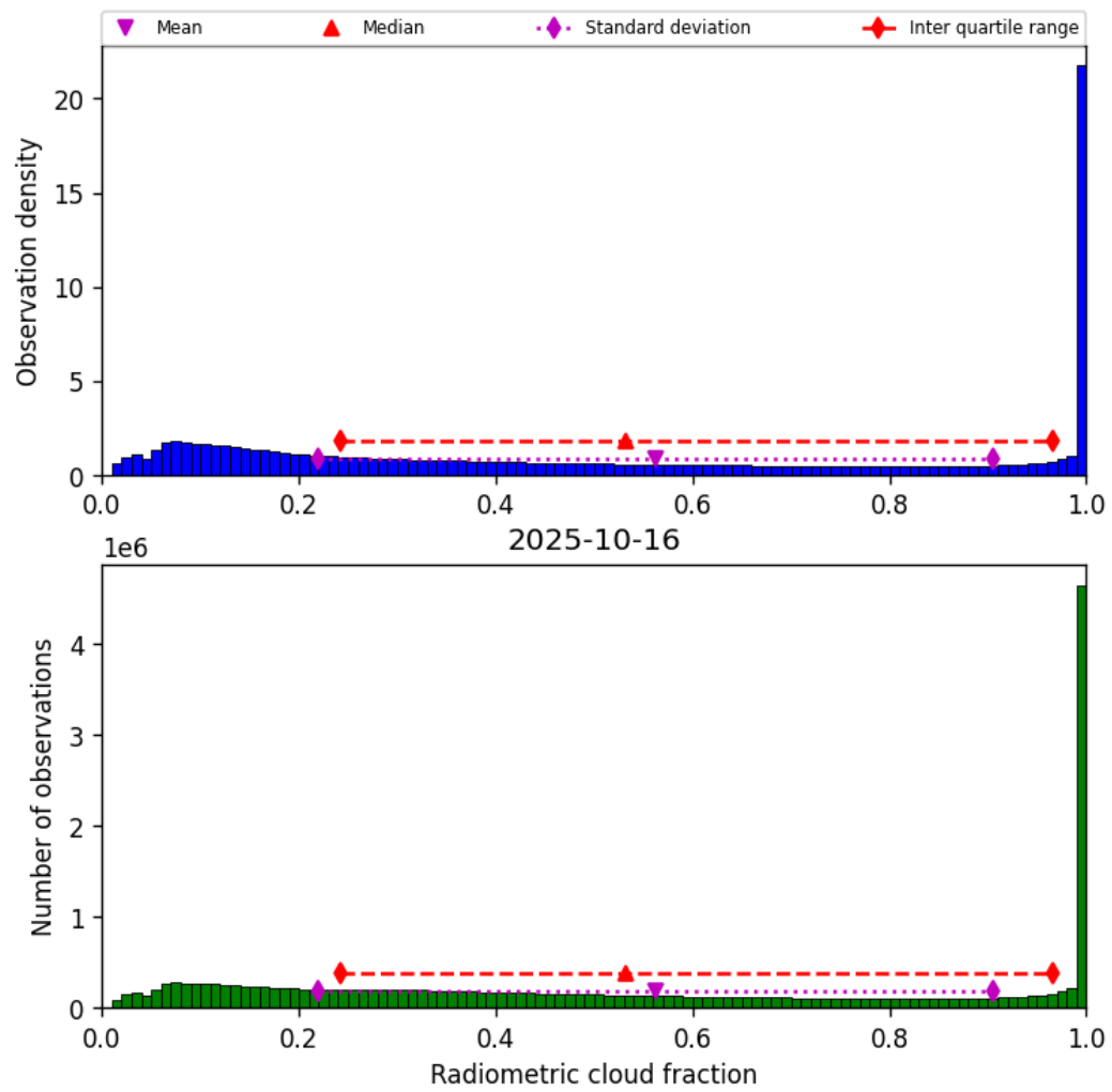
Figure 37: Histogram of “Radiometric cloud fraction” for 2025-10-16 to 2025-10-17
