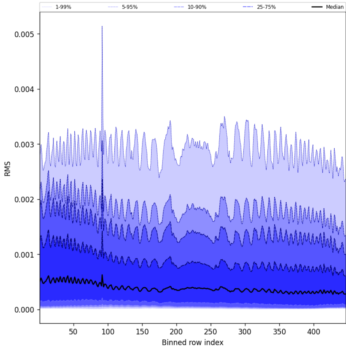
Figure 61: Along track statistics of “RMS” for 2025-10-16 to 2025-10-17
