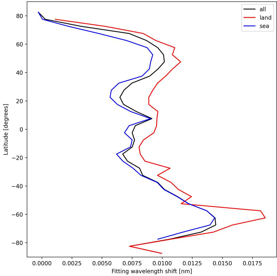
Figure 31: Zonal average of “Fitting wavelength shift” for 2025-10-16 to 2025-10-17.
