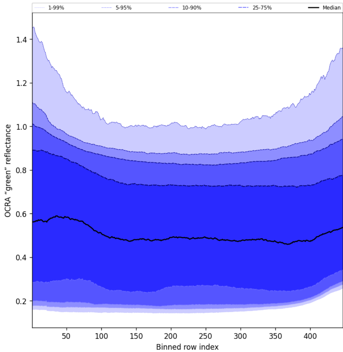
Figure 66: Along track statistics of “OCRA “green” reflectance” for 2025-10-16 to 2025-10-17
