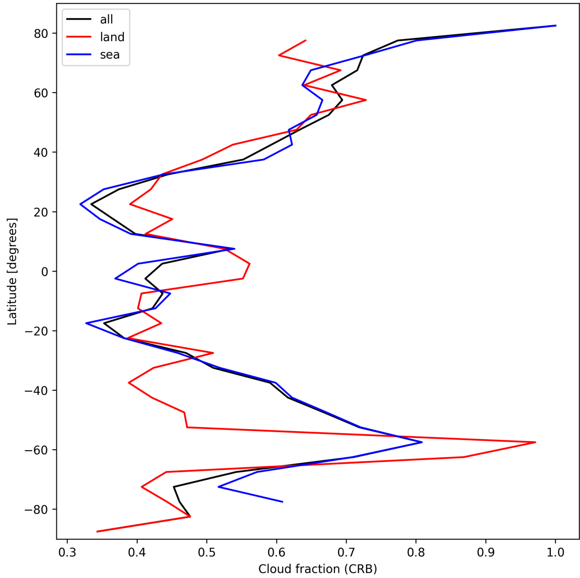
Figure 24: Zonal average of “Cloud fraction (CRB)” for 2025-10-16 to 2025-10-17.
