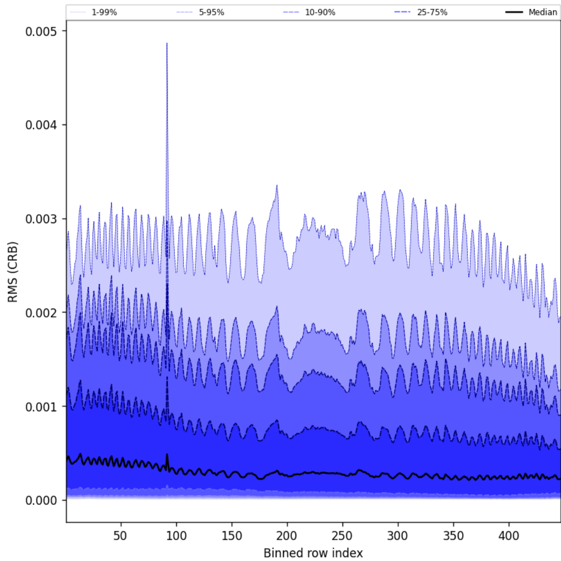
Figure 62: Along track statistics of “RMS (CRB)” for 2025-10-16 to 2025-10-17
