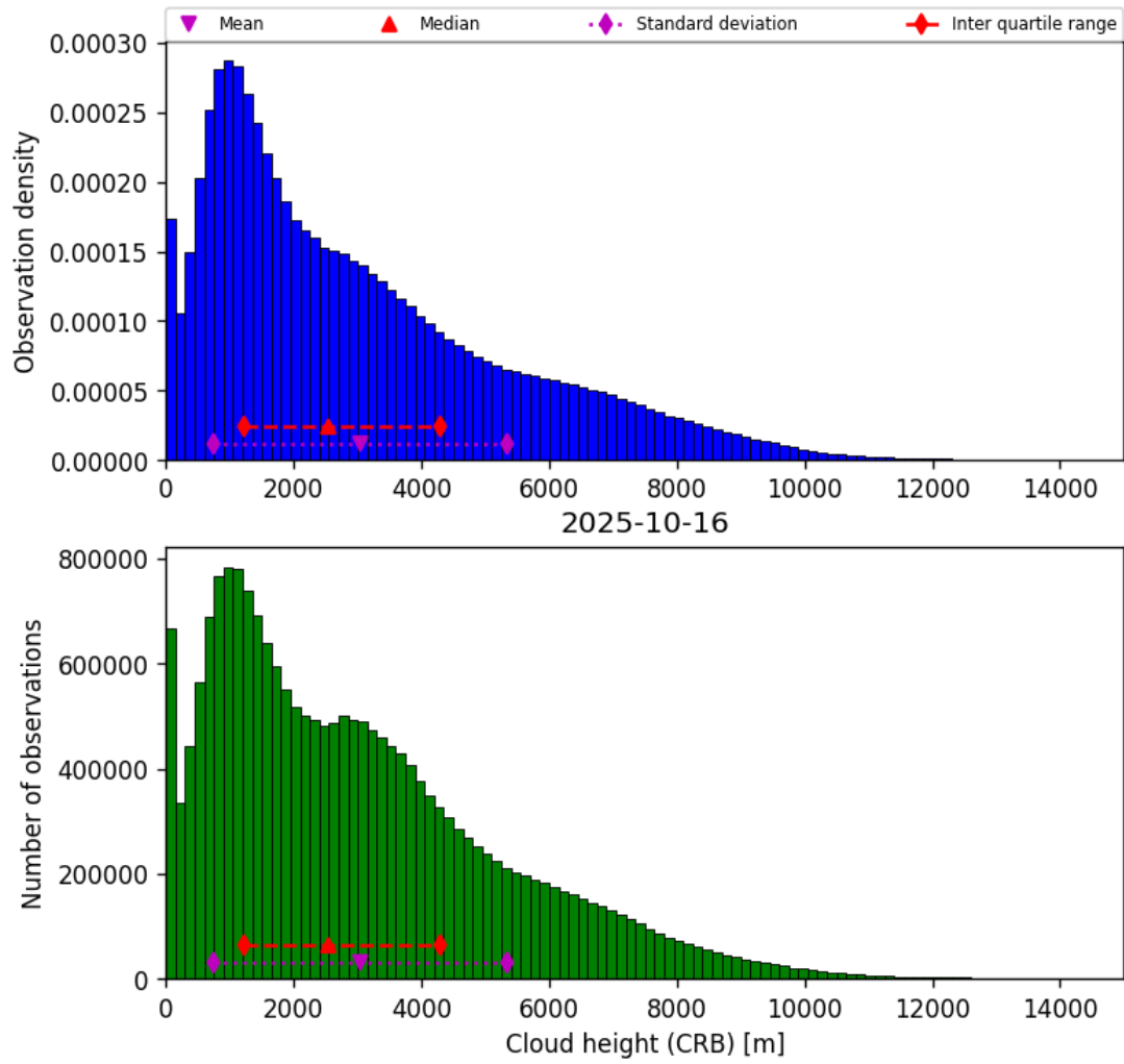
Figure 41: Histogram of “Cloud height (CRB)” for 2025-10-16 to 2025-10-17
