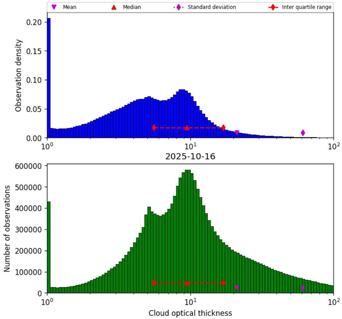
Figure 39: Histogram of “Cloud optical thickness” for 2025-10-16 to 2025-10-17
