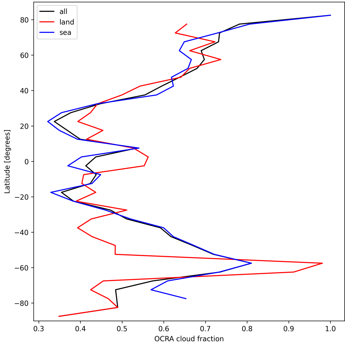
Figure 32: Zonal average of “OCRA cloud fraction” for 2025-10-16 to 2025-10-17.
