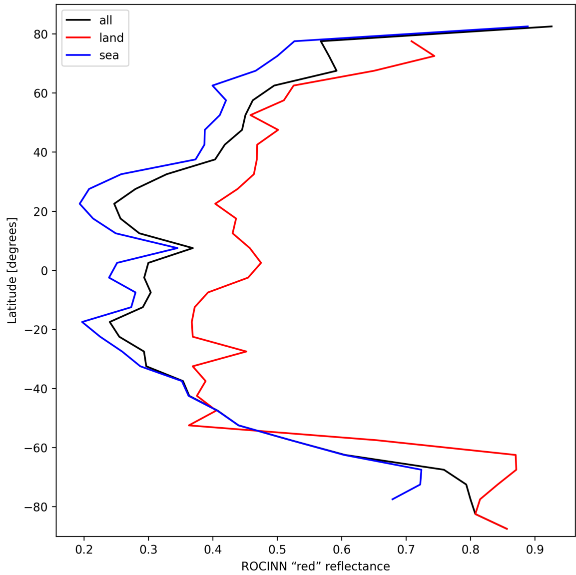
Figure 35: Zonal average of "ROCINN "red" reflectance" for 2025-10-16 to 2025-10-17.
