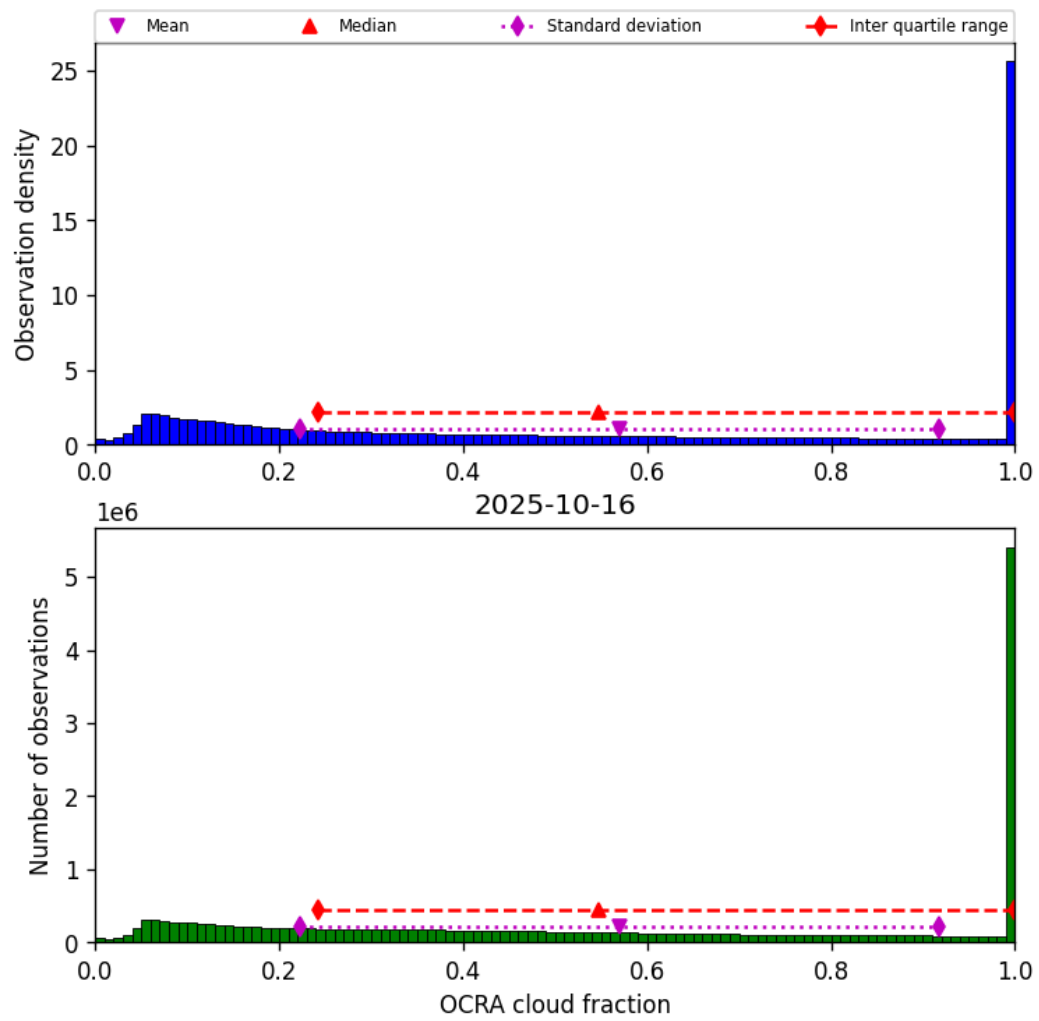
Figure 48: Histogram of “OCRA cloud fraction” for 2025-10-16 to 2025-10-17
