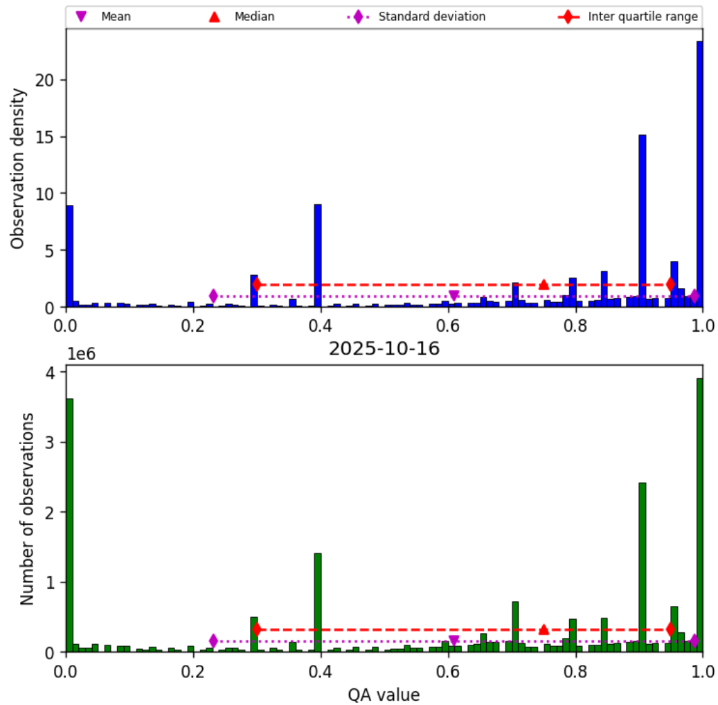
Figure 36: Histogram of “QA value” for 2025-10-16 to 2025-10-17
