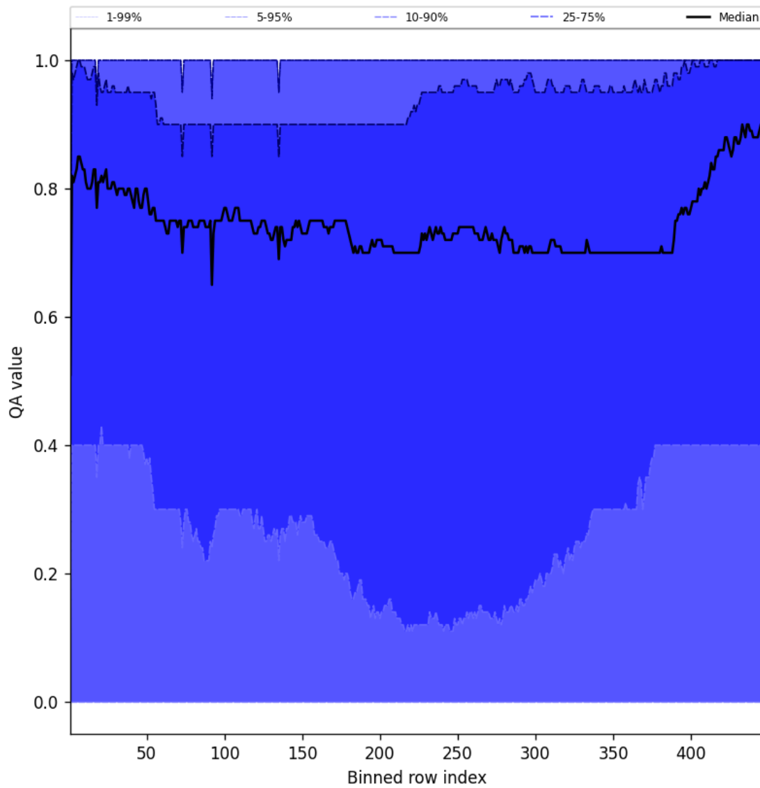
Figure 52: Along track statistics of “QA value” for 2025-10-16 to 2025-10-17
