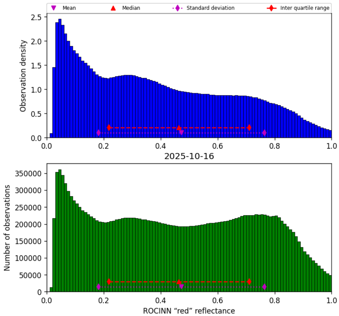
Figure 51: Histogram of “ROCINN “red” reflectance” for 2025-10-16 to 2025-10-17
