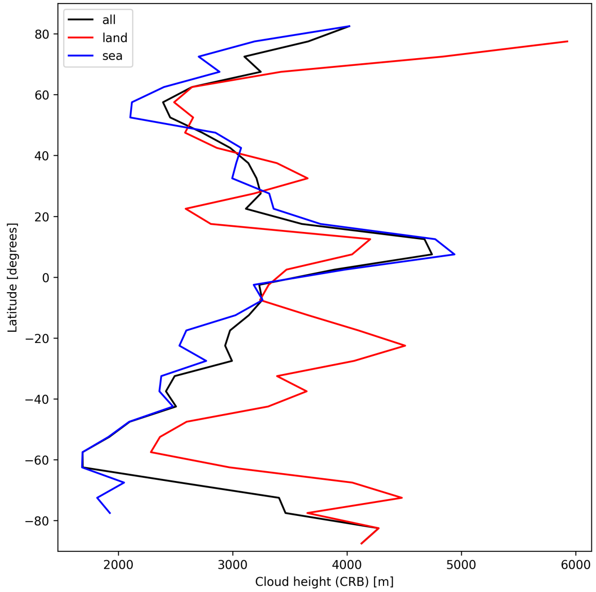
Figure 25: Zonal average of “Cloud height (CRB)” for 2025-10-16 to 2025-10-17.
