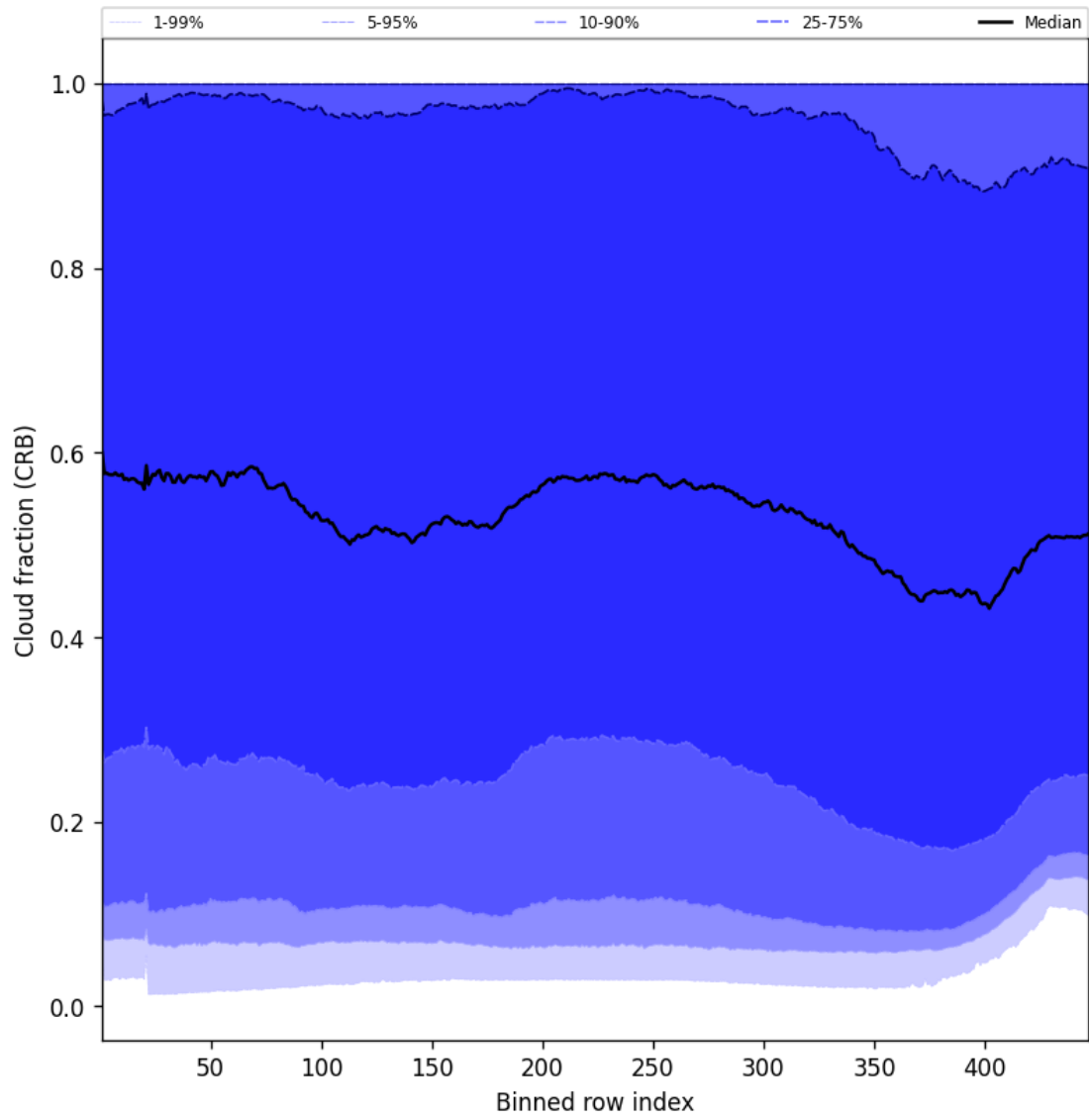
Figure 56: Along track statistics of “Cloud fraction (CRB)” for 2025-10-16 to 2025-10-17
