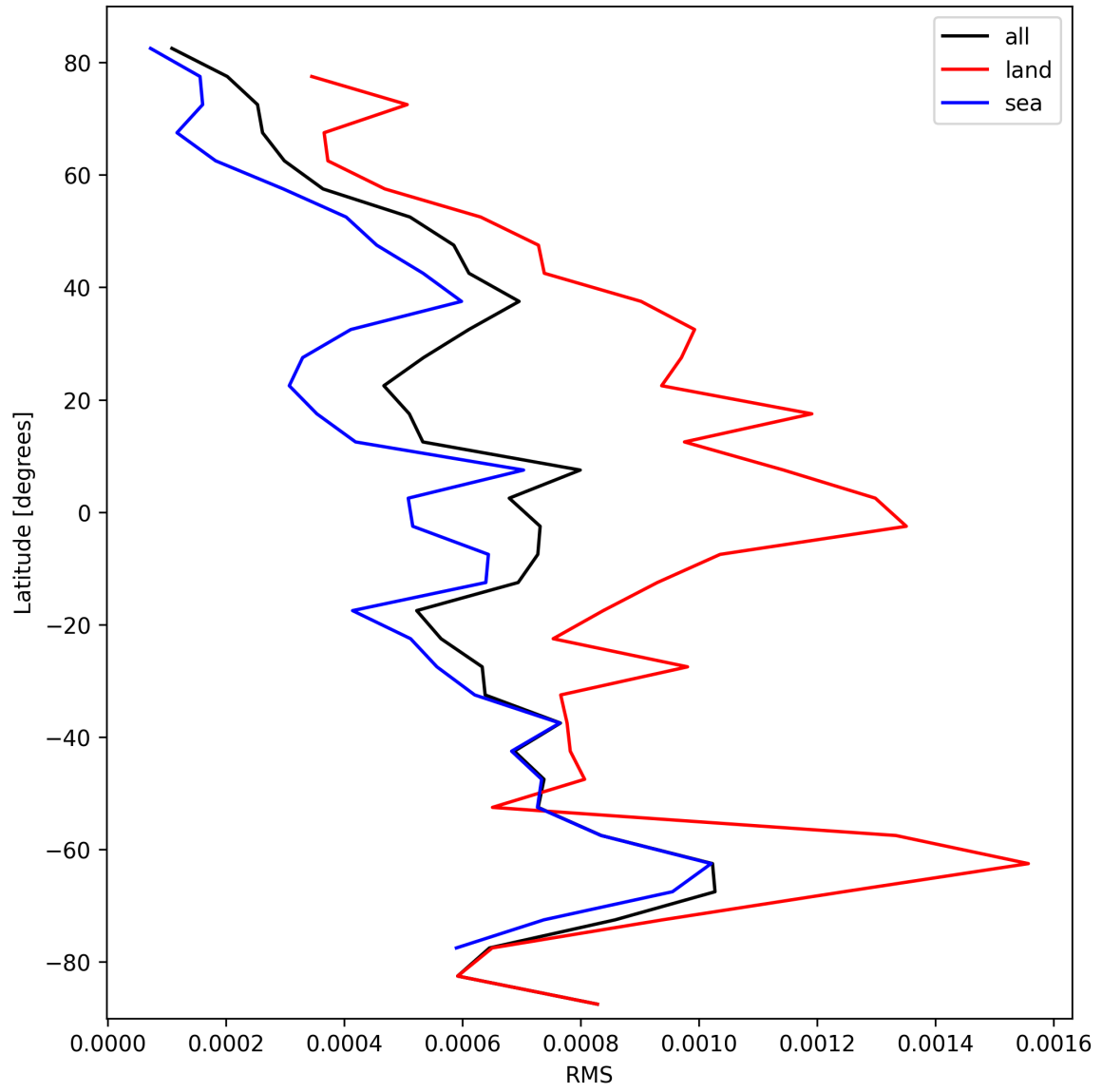
Figure 29: Zonal average of “RMS” for 2025-10-16 to 2025-10-17.
