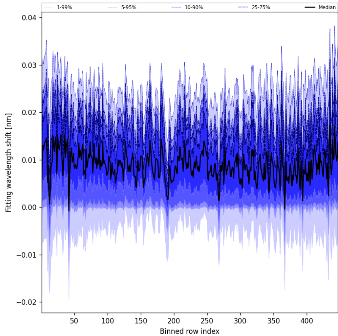
Figure 63: Along track statistics of “Fitting wavelength shift” for 2025-10-16 to 2025-10-17
