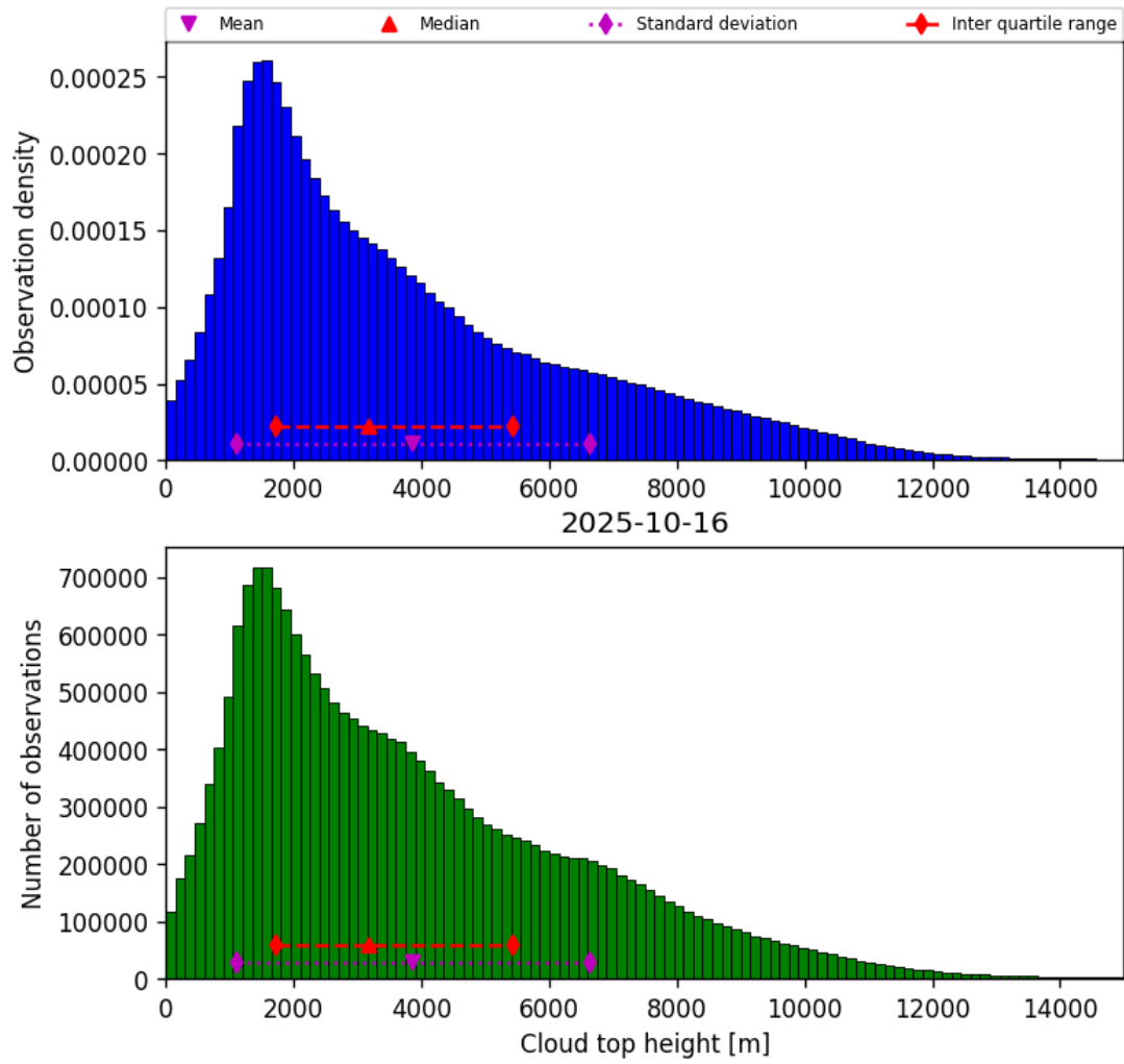
Figure 38: Histogram of “Cloud top height” for 2025-10-16 to 2025-10-17
