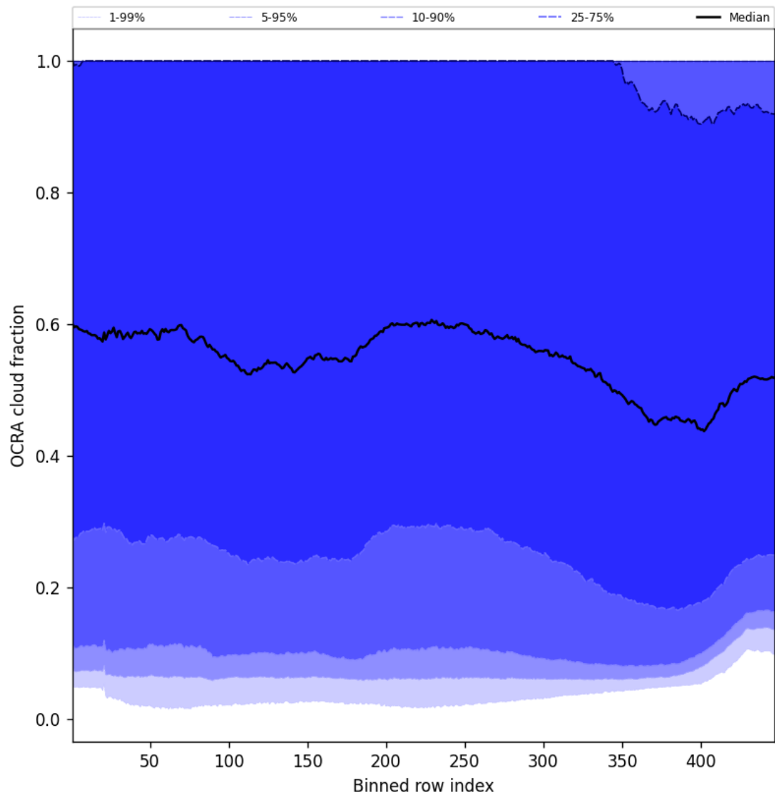
Figure 64: Along track statistics of “OCRA cloud fraction” for 2025-10-16 to 2025-10-17
