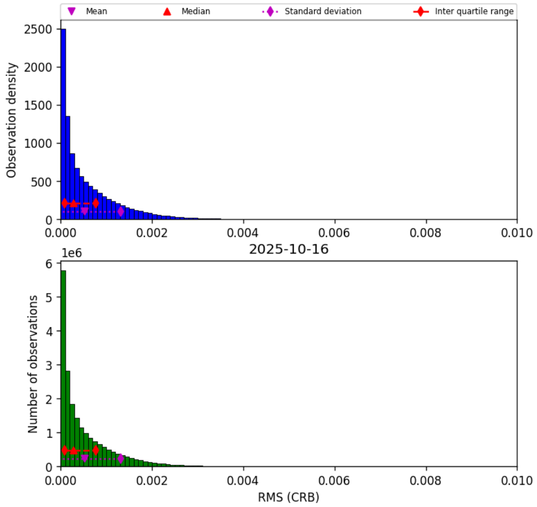
Figure 46: Histogram of “RMS (CRB)” for 2025-10-16 to 2025-10-17
