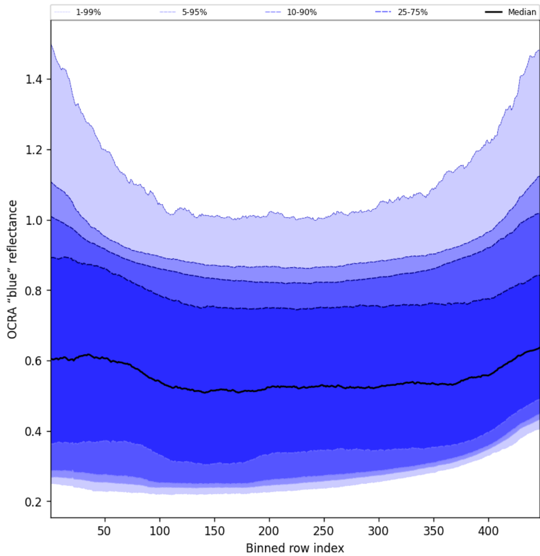
Figure 65: Along track statistics of “OCRA “blue” reflectance” for 2025-10-16 to 2025-10-17
