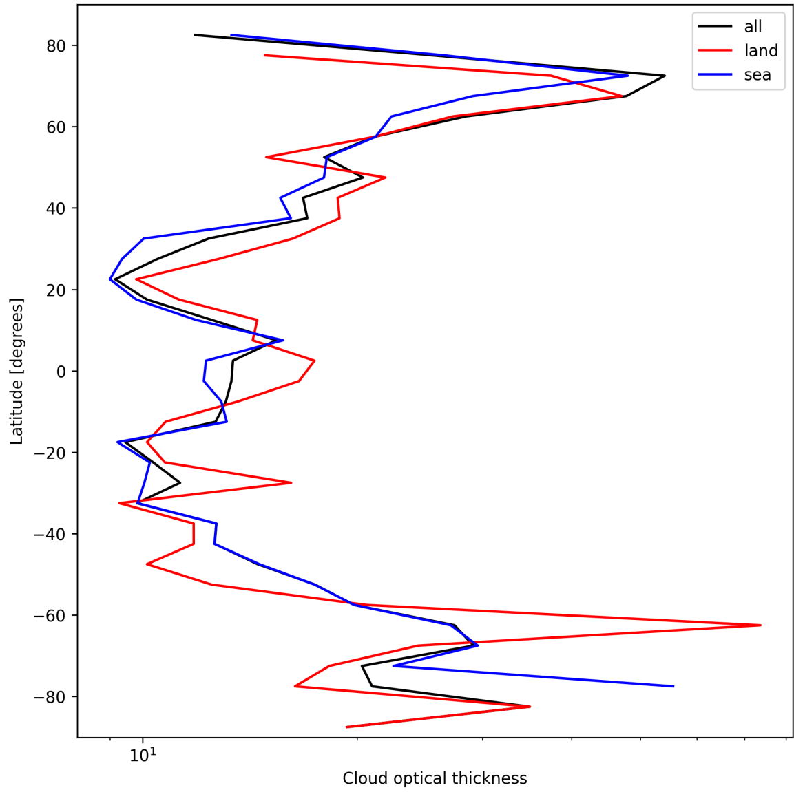
Figure 23: Zonal average of “Cloud optical thickness” for 2025-10-16 to 2025-10-17.
