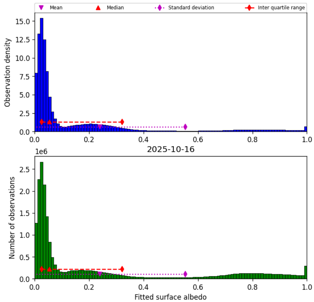
Figure 43: Histogram of “Fitted surface albedo” for 2025-10-16 to 2025-10-17
