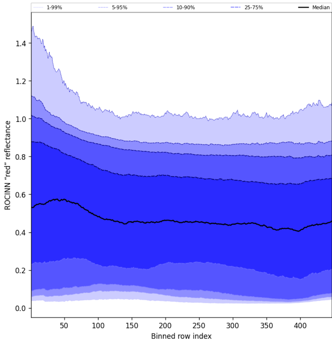
Figure 67: Along track statistics of "ROCINN "red" reflectance" for 2025-10-16 to 2025-10-17
