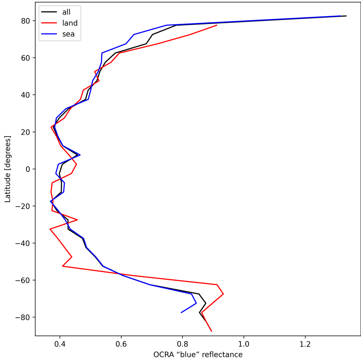
Figure 33: Zonal average of “OCRA “blue” reflectance” for 2025-10-16 to 2025-10-17.
