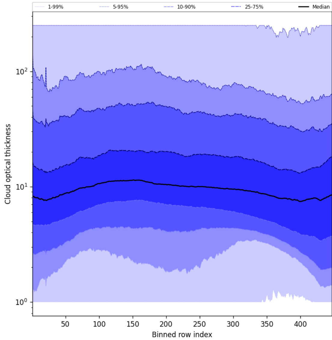
Figure 55: Along track statistics of “Cloud optical thickness” for 2025-10-16 to 2025-10-17
