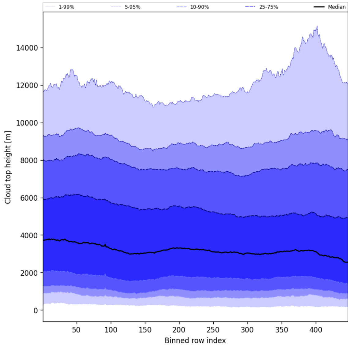
Figure 54: Along track statistics of “Cloud top height” for 2025-10-16 to 2025-10-17
