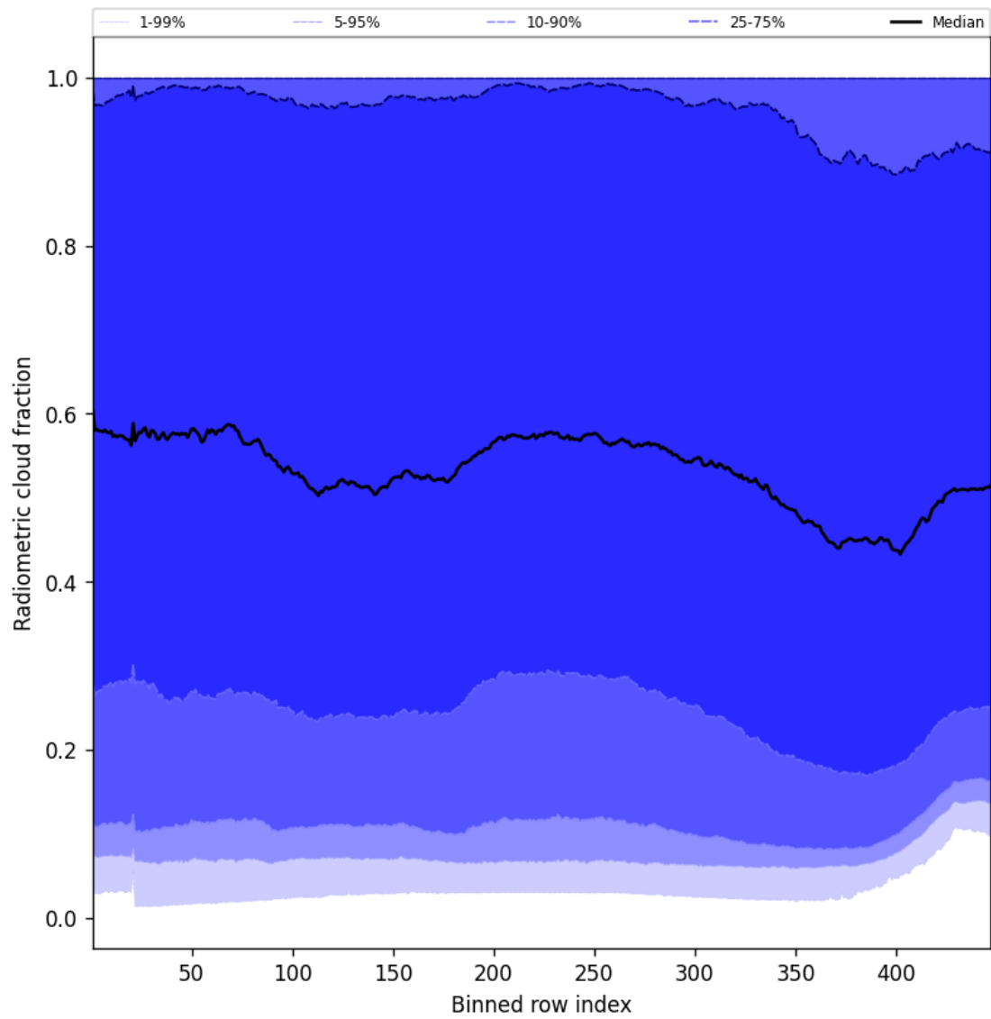
Figure 53: Along track statistics of “Radiometric cloud fraction” for 2025-10-16 to 2025-10-17
