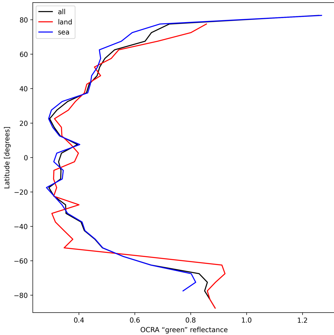
Figure 34: Zonal average of “OCRA “green” reflectance” for 2025-10-16 to 2025-10-17.
