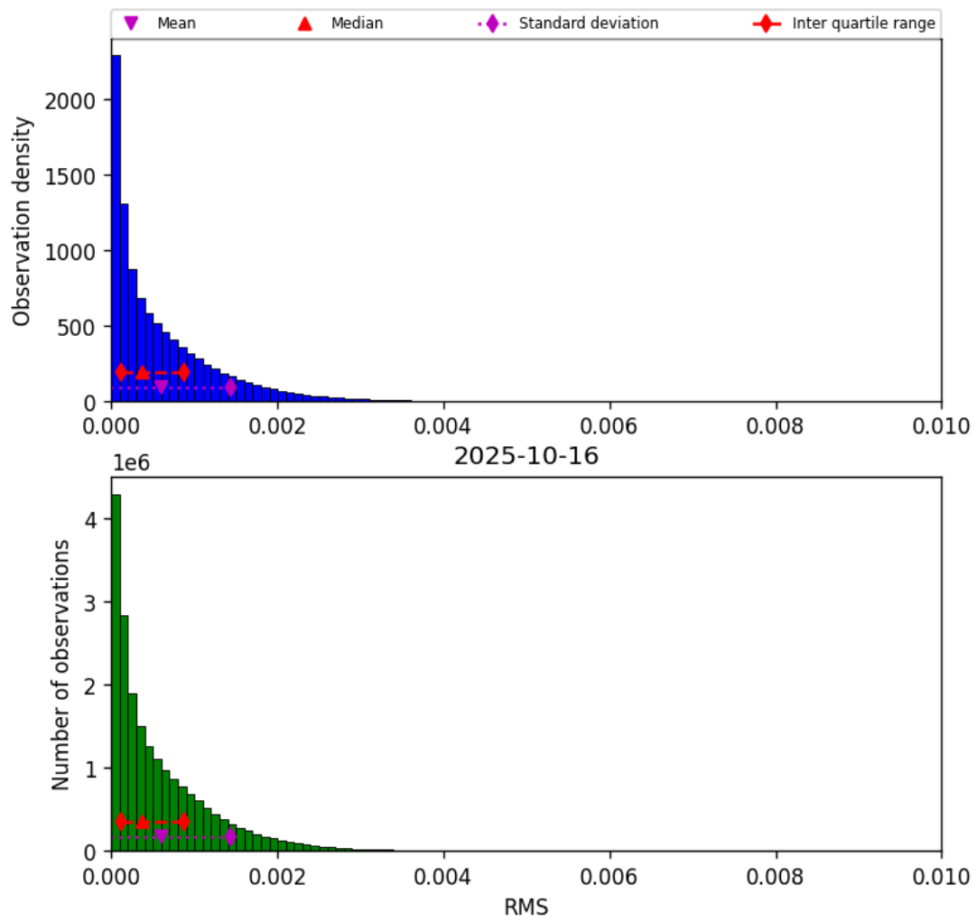
Figure 45: Histogram of “RMS” for 2025-10-16 to 2025-10-17
