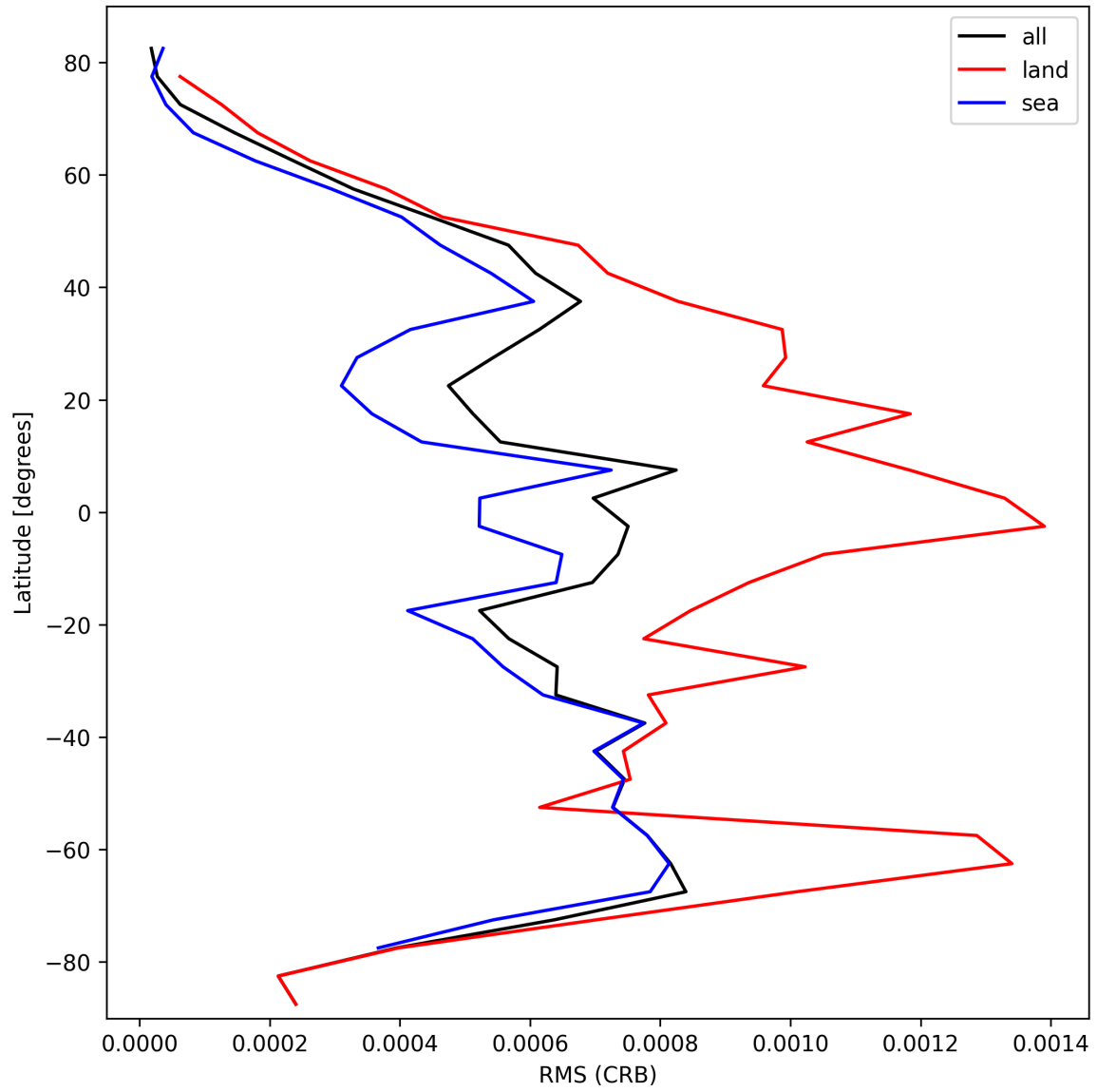
Figure 30: Zonal average of “RMS (CRB)” for 2025-10-16 to 2025-10-17.
