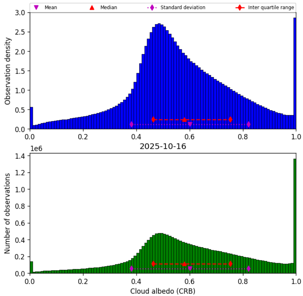
Figure 42: Histogram of “Cloud albedo (CRB)” for 2025-10-16 to 2025-10-17
