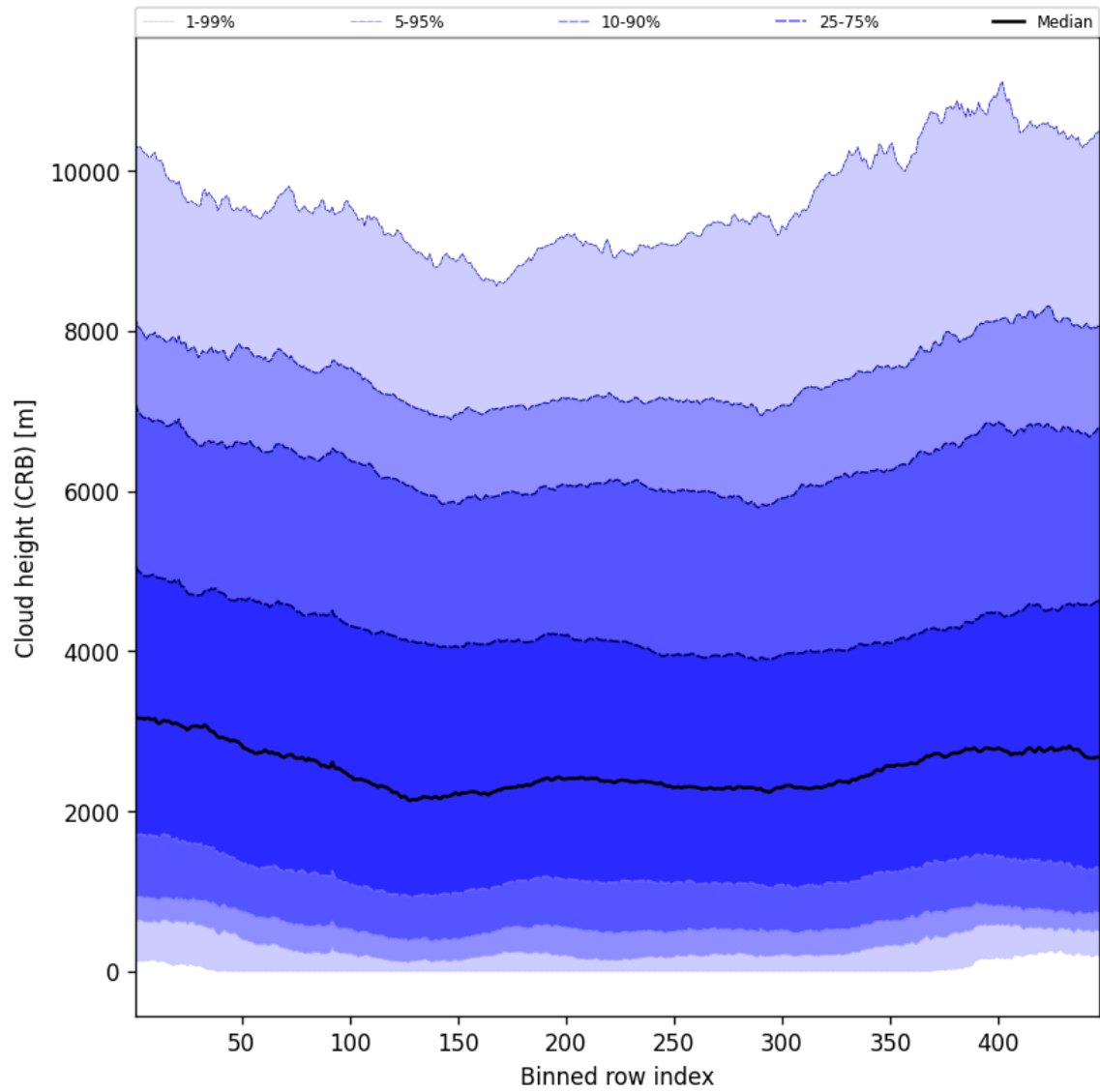
Figure 57: Along track statistics of “Cloud height (CRB)” for 2025-10-16 to 2025-10-17
