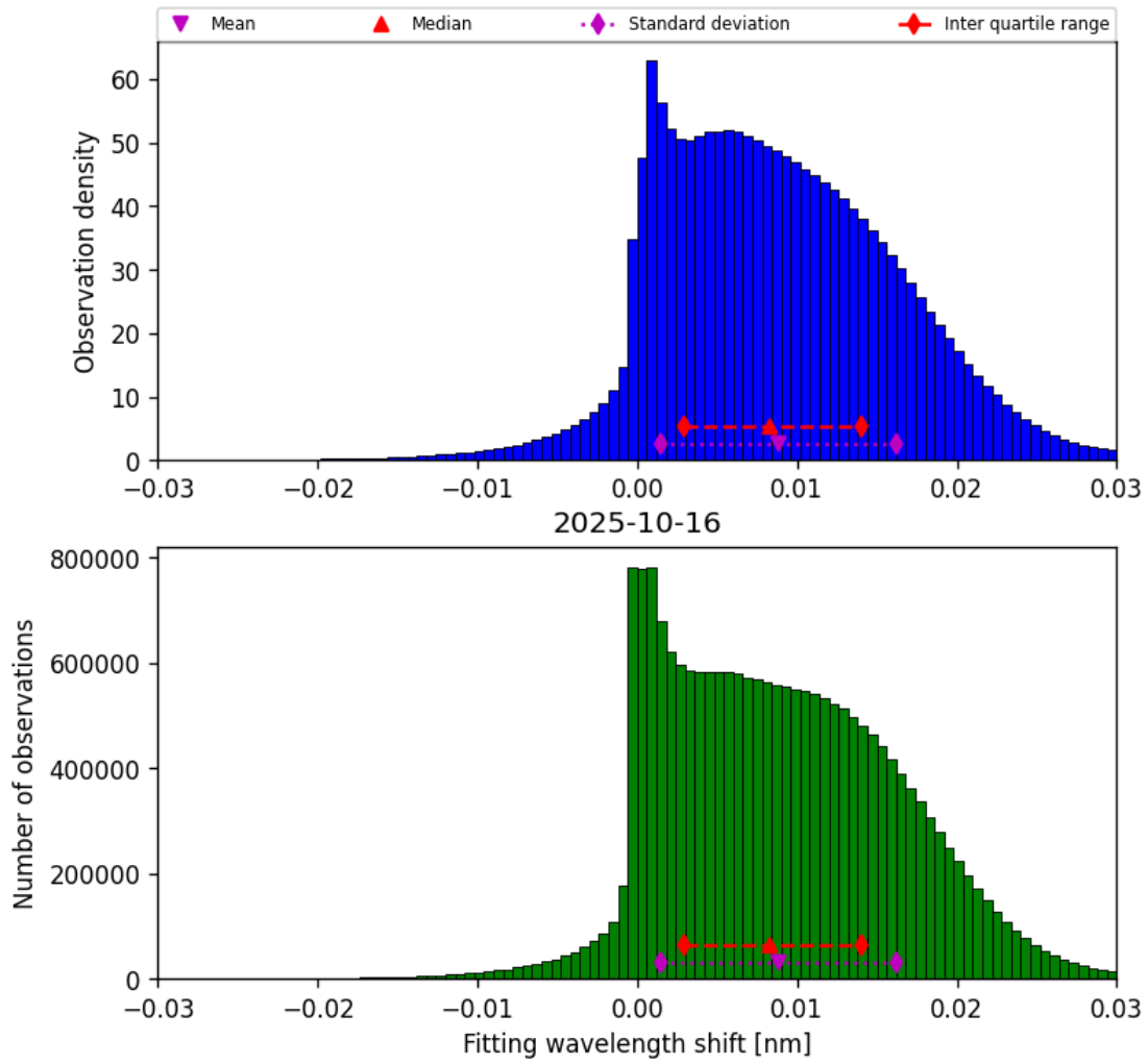
Figure 47: Histogram of “Fitting wavelength shift” for 2025-10-16 to 2025-10-17
