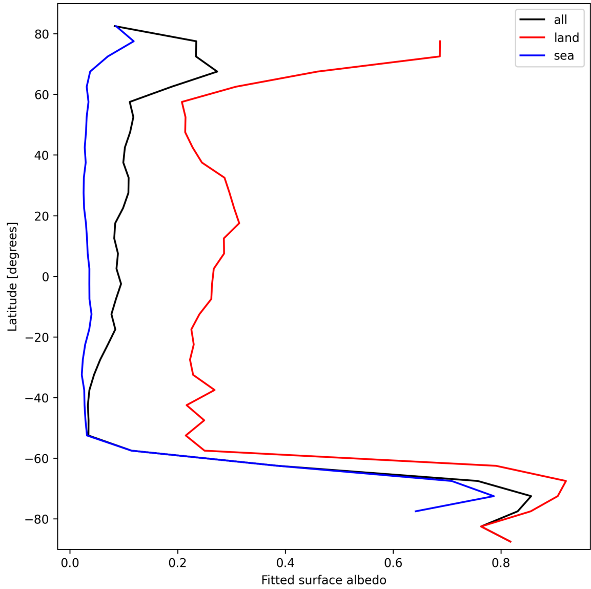
Figure 27: Zonal average of “Fitted surface albedo” for 2025-10-16 to 2025-10-17.
