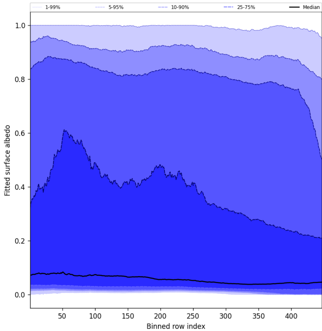
Figure 59: Along track statistics of “Fitted surface albedo” for 2025-10-16 to 2025-10-17
