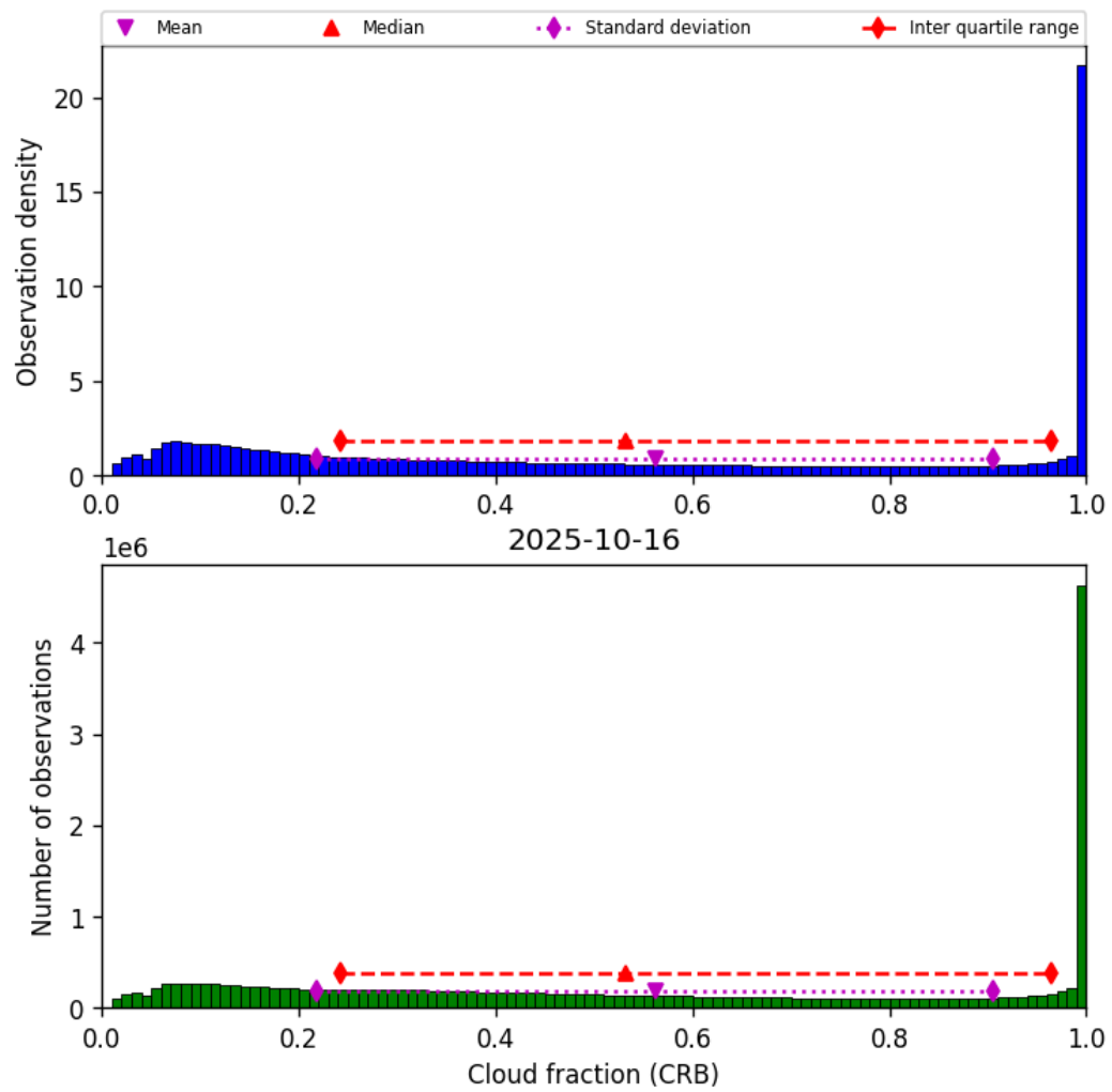
Figure 40: Histogram of “Cloud fraction (CRB)” for 2025-10-16 to 2025-10-17
