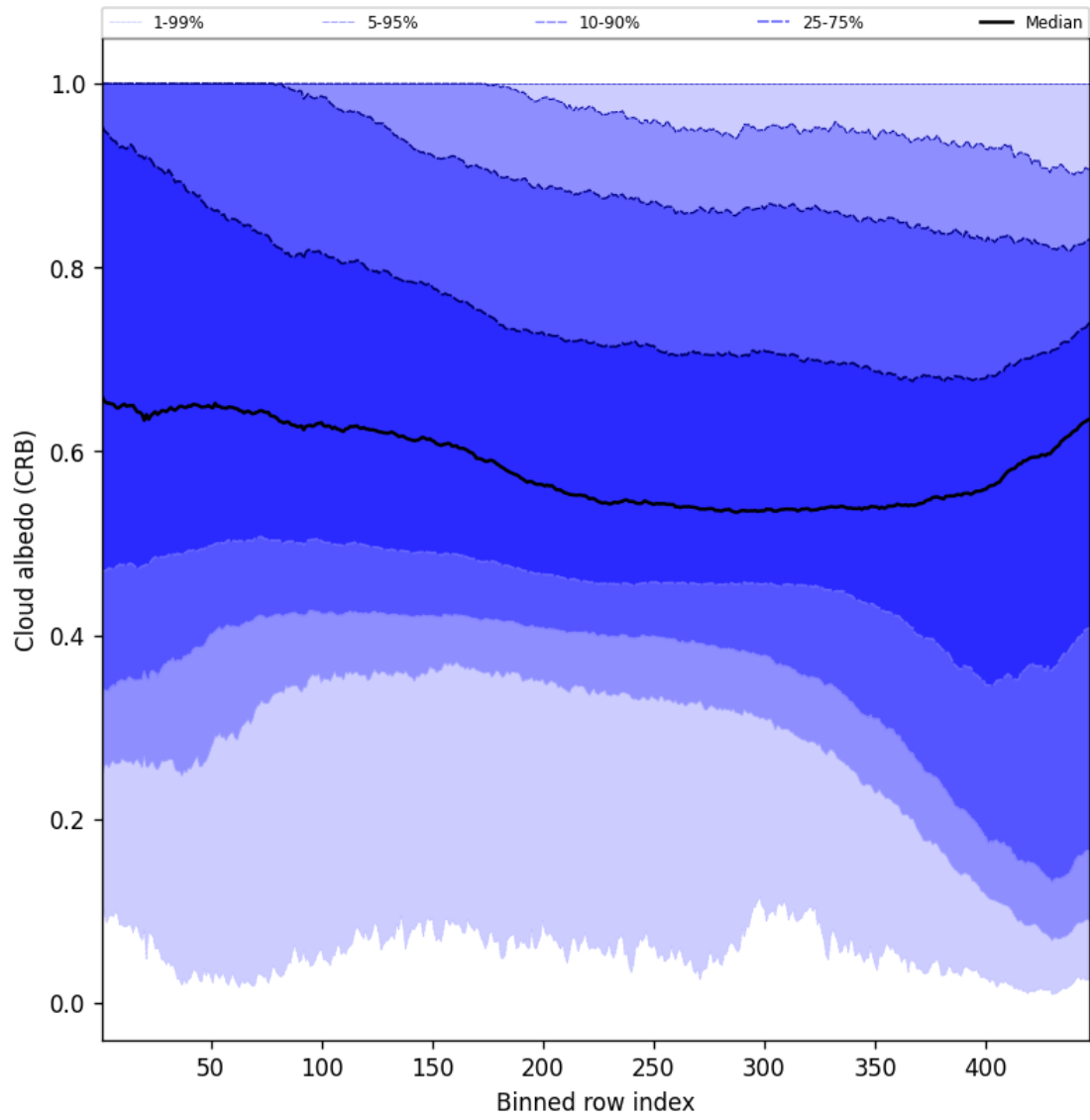
Figure 58: Along track statistics of “Cloud albedo (CRB)” for 2025-10-16 to 2025-10-17
