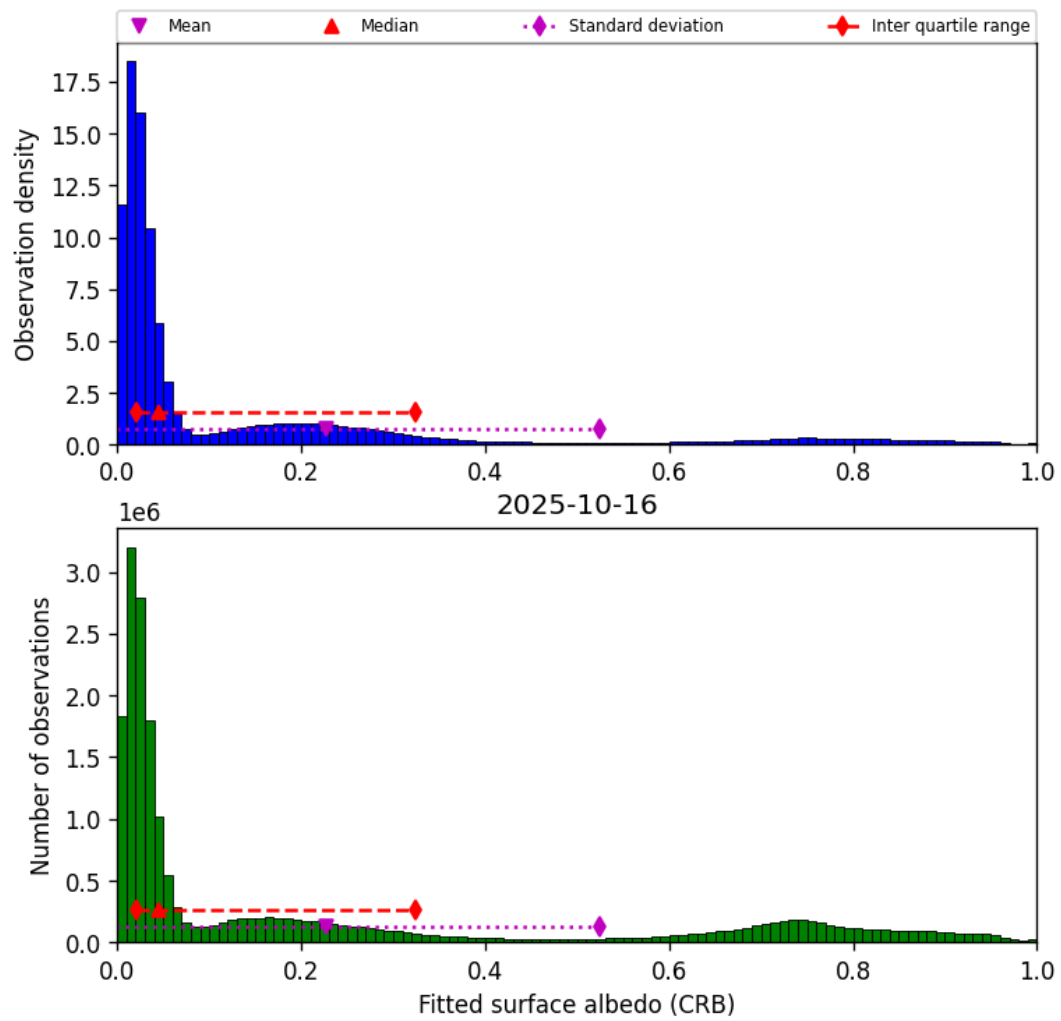
Figure 44: Histogram of “Fitted surface albedo (CRB)” for 2025-10-16 to 2025-10-17
