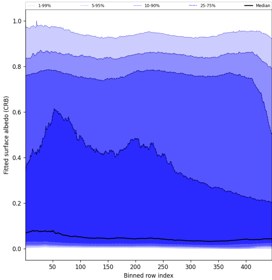
Figure 60: Along track statistics of “Fitted surface albedo (CRB)” for 2025-10-16 to 2025-10-17
