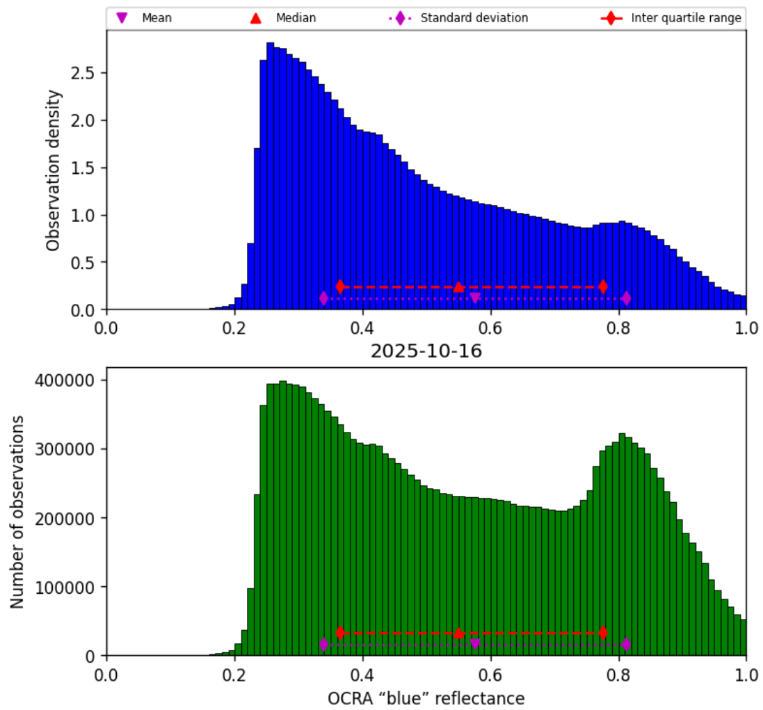
Figure 49: Histogram of “OCRA “blue” reflectance” for 2025-10-16 to 2025-10-17
