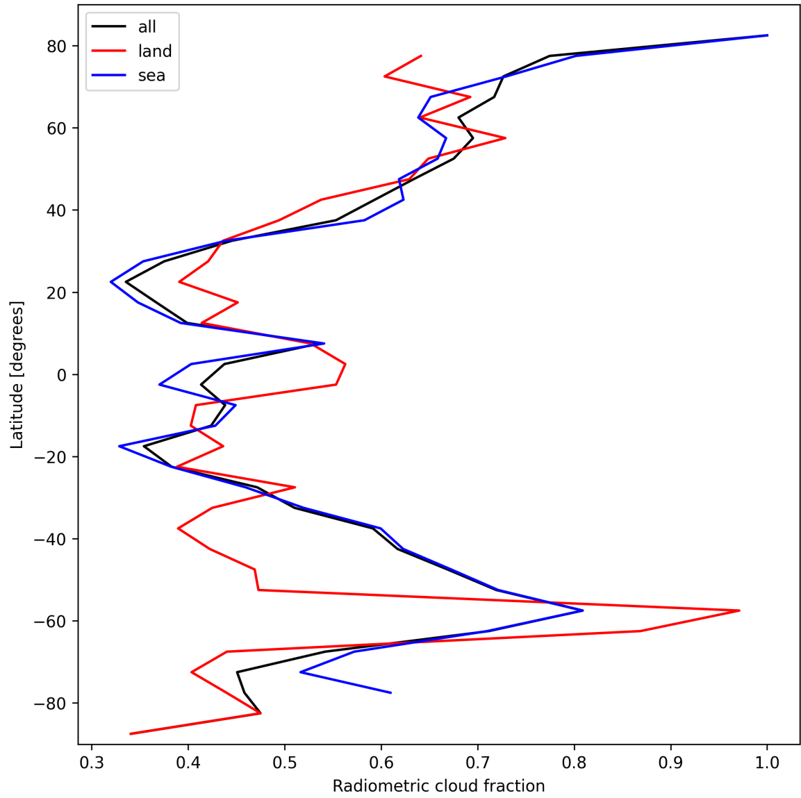
Figure 21: Zonal average of “Radiometric cloud fraction” for 2025-10-16 to 2025-10-17.
