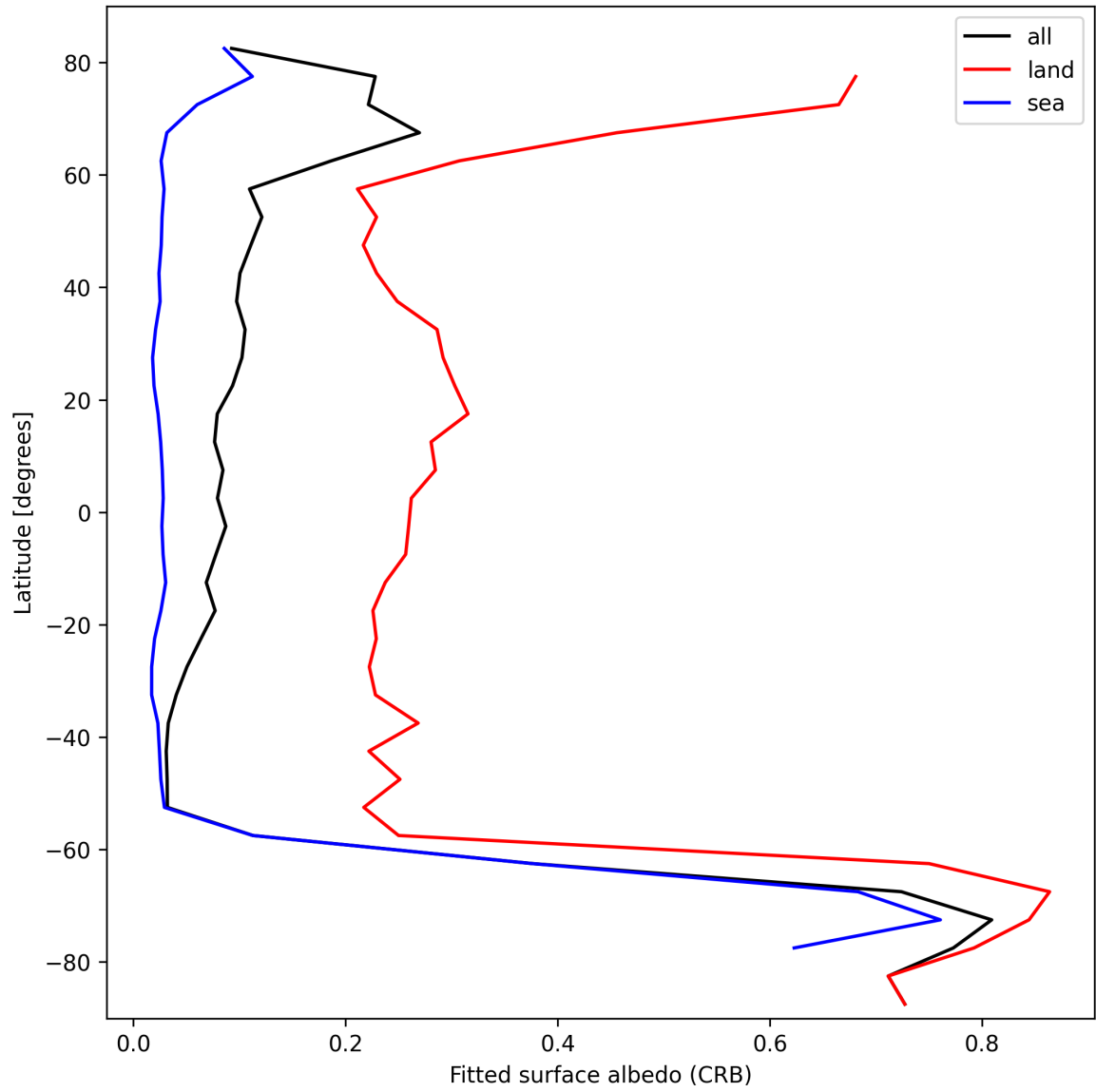
Figure 28: Zonal average of “Fitted surface albedo (CRB)” for 2025-10-16 to 2025-10-17.
