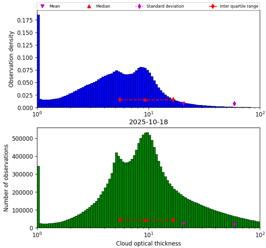
Figure 39: Histogram of “Cloud optical thickness” for 2025-10-18 to 2025-10-19
