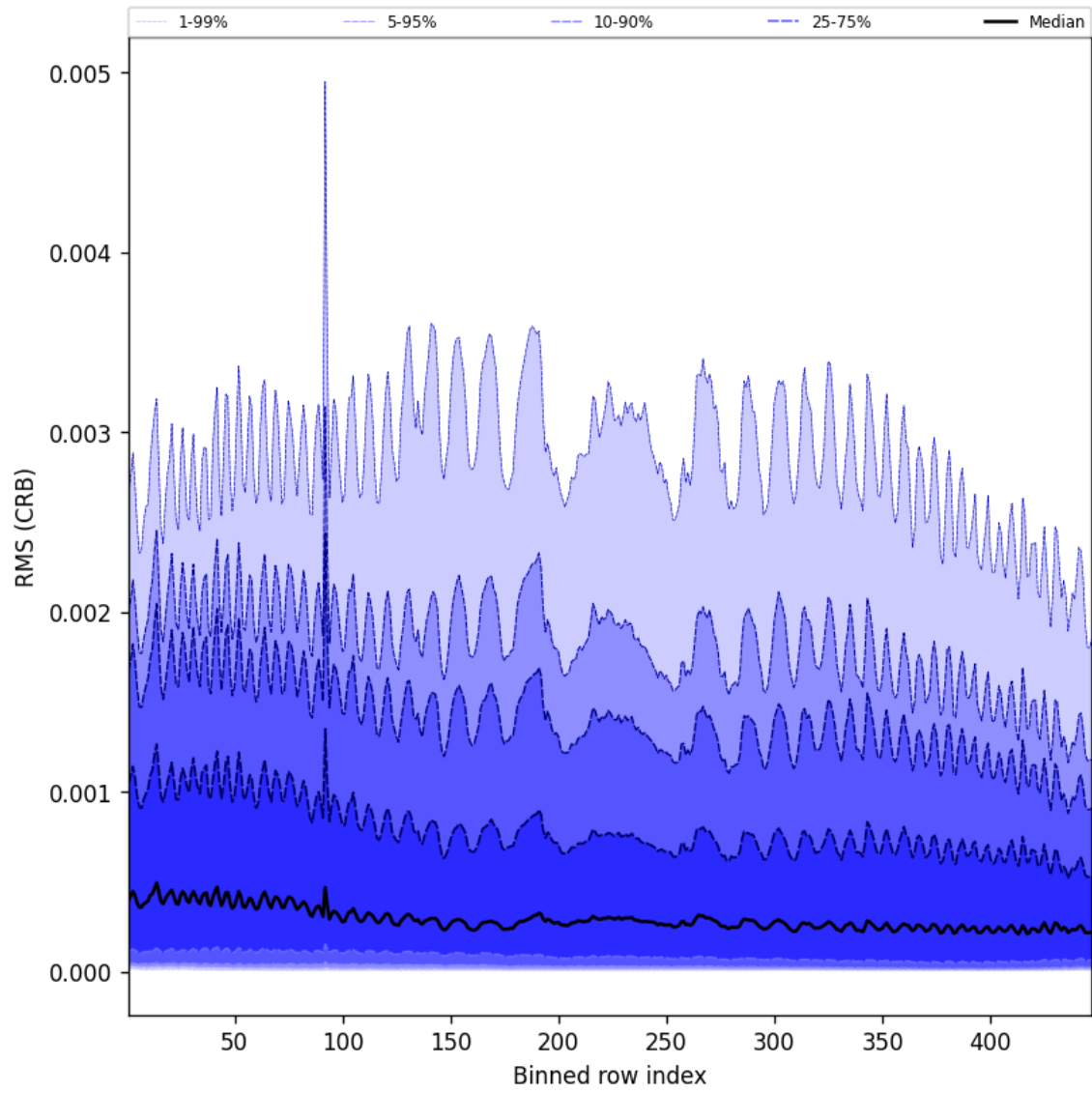
Figure 62: Along track statistics of “RMS (CRB)” for 2025-10-18 to 2025-10-19
