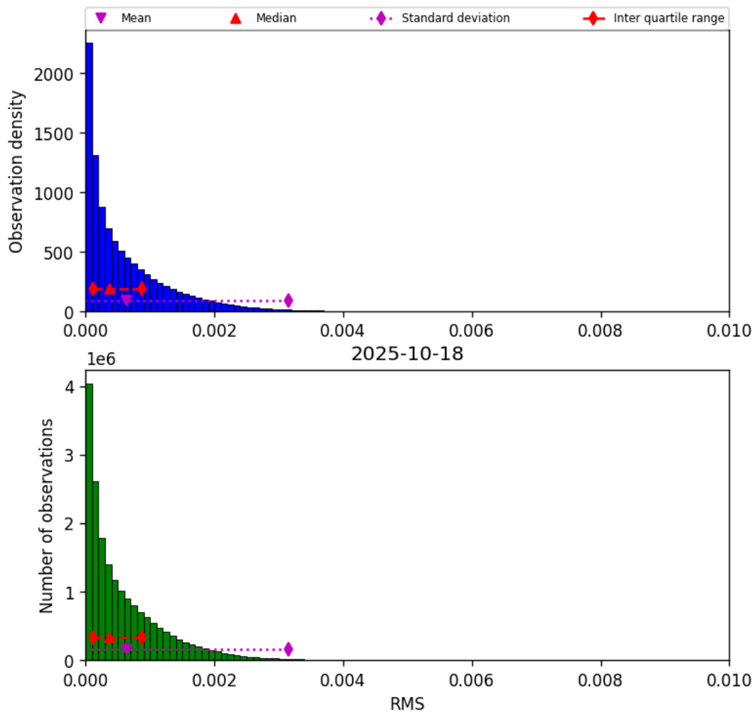
Figure 45: Histogram of “RMS” for 2025-10-18 to 2025-10-19
