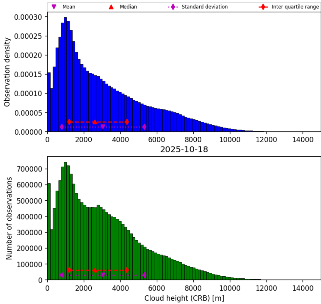
Figure 41: Histogram of “Cloud height (CRB)” for 2025-10-18 to 2025-10-19
