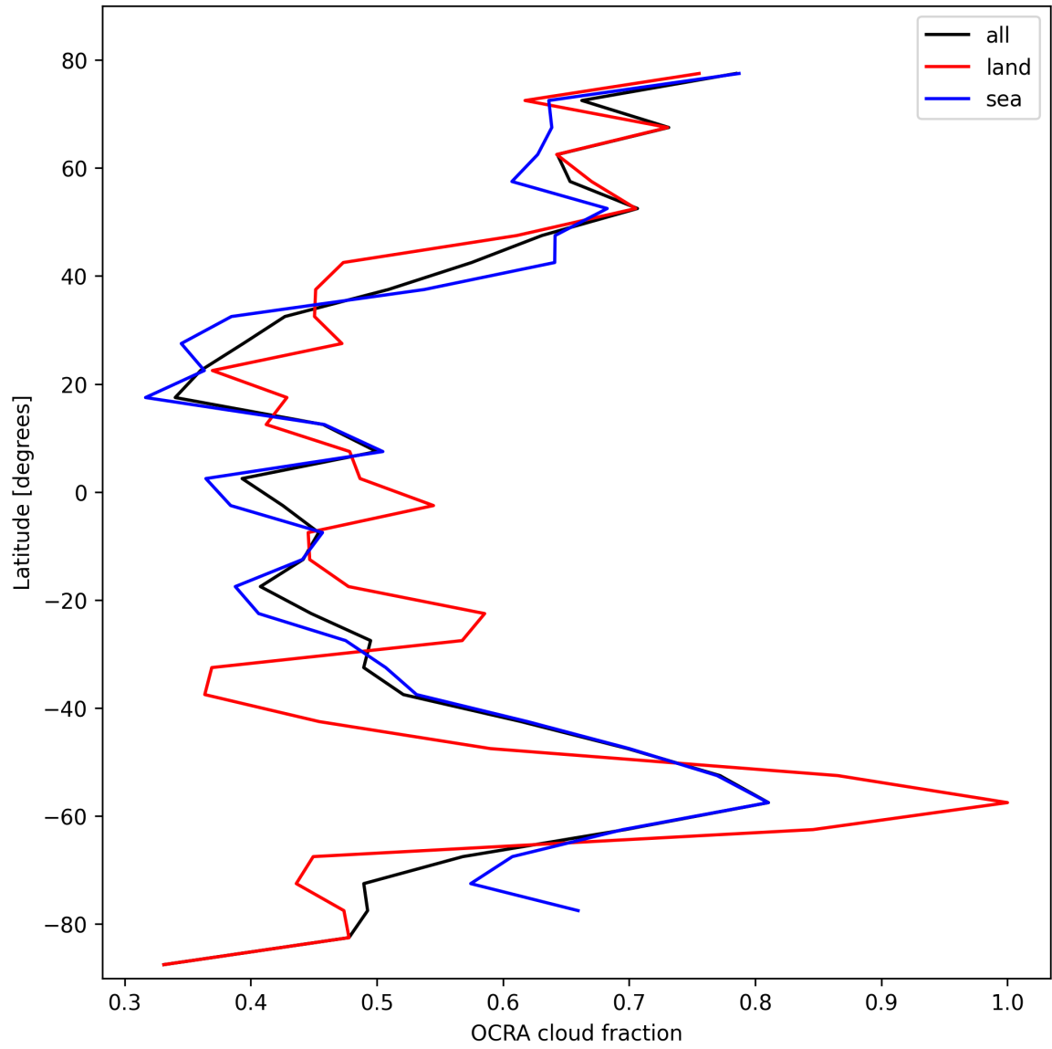
Figure 32: Zonal average of “OCRA cloud fraction” for 2025-10-18 to 2025-10-19.
