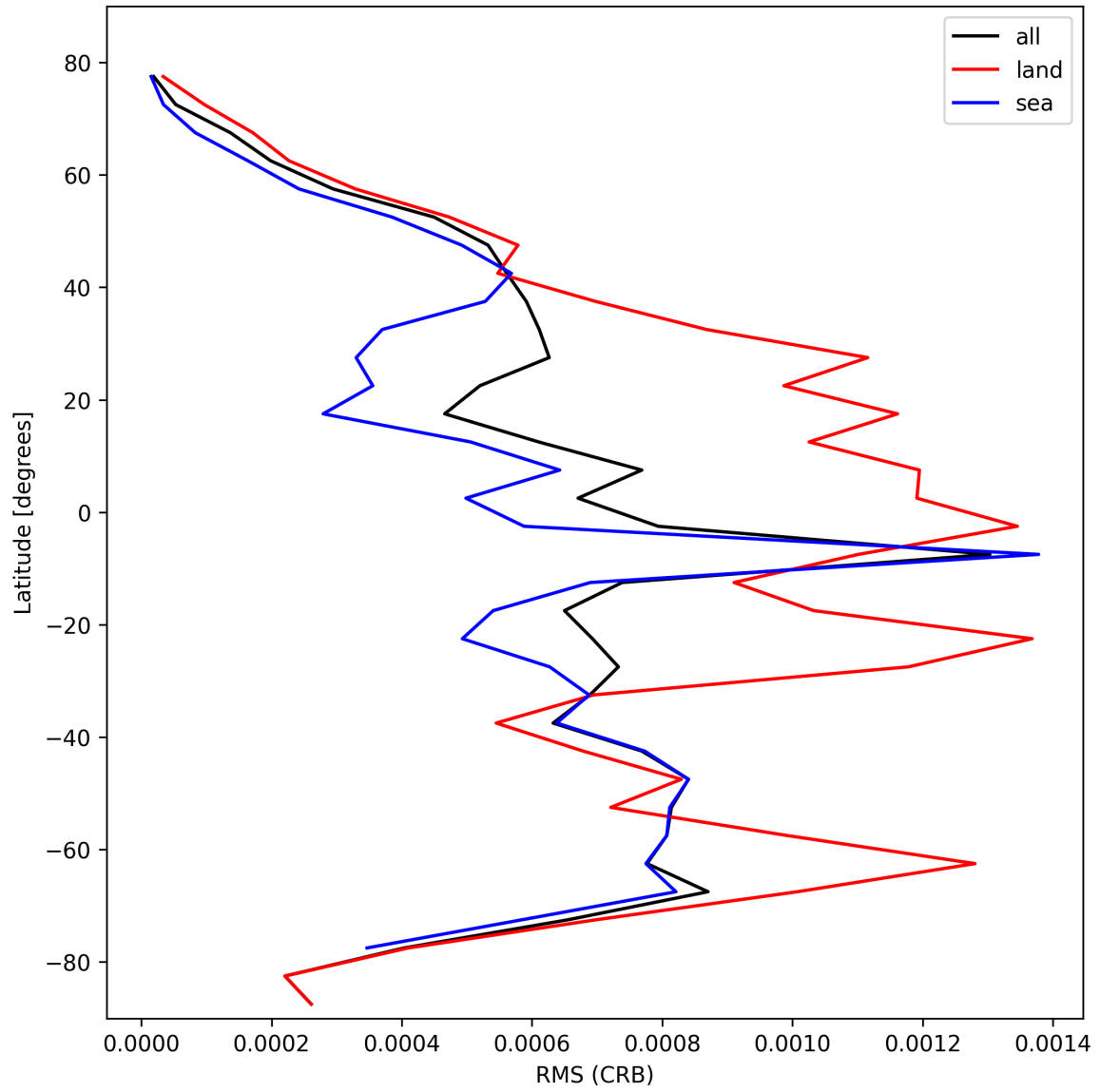
Figure 30: Zonal average of “RMS (CRB)” for 2025-10-18 to 2025-10-19.
