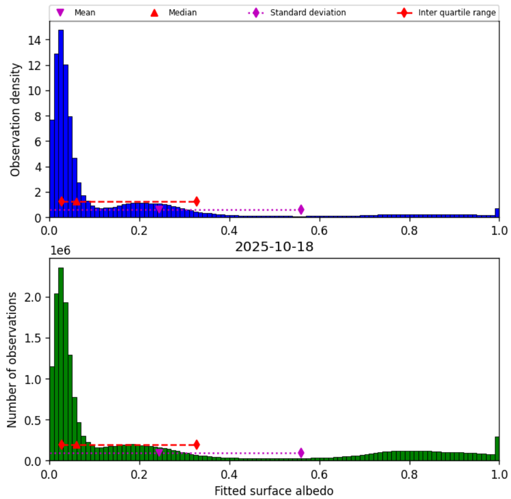
Figure 43: Histogram of “Fitted surface albedo” for 2025-10-18 to 2025-10-19
