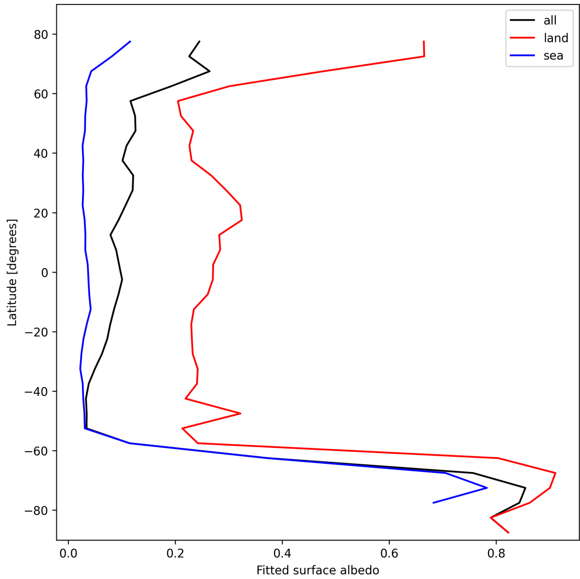
Figure 27: Zonal average of “Fitted surface albedo” for 2025-10-18 to 2025-10-19.
