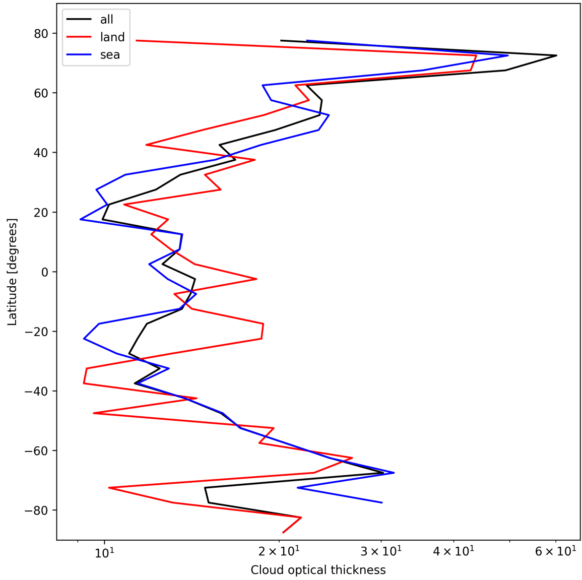
Figure 23: Zonal average of “Cloud optical thickness” for 2025-10-18 to 2025-10-19.
