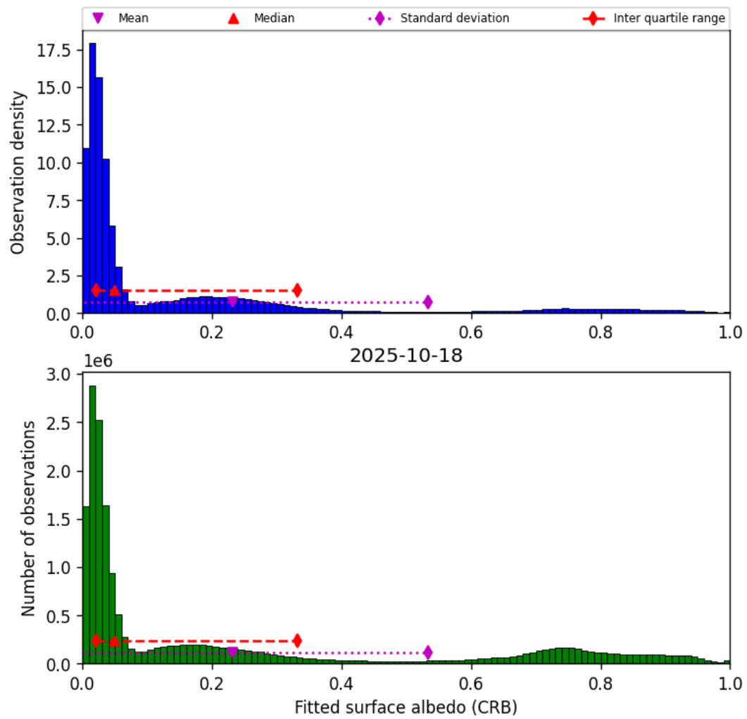
Figure 44: Histogram of “Fitted surface albedo (CRB)” for 2025-10-18 to 2025-10-19
