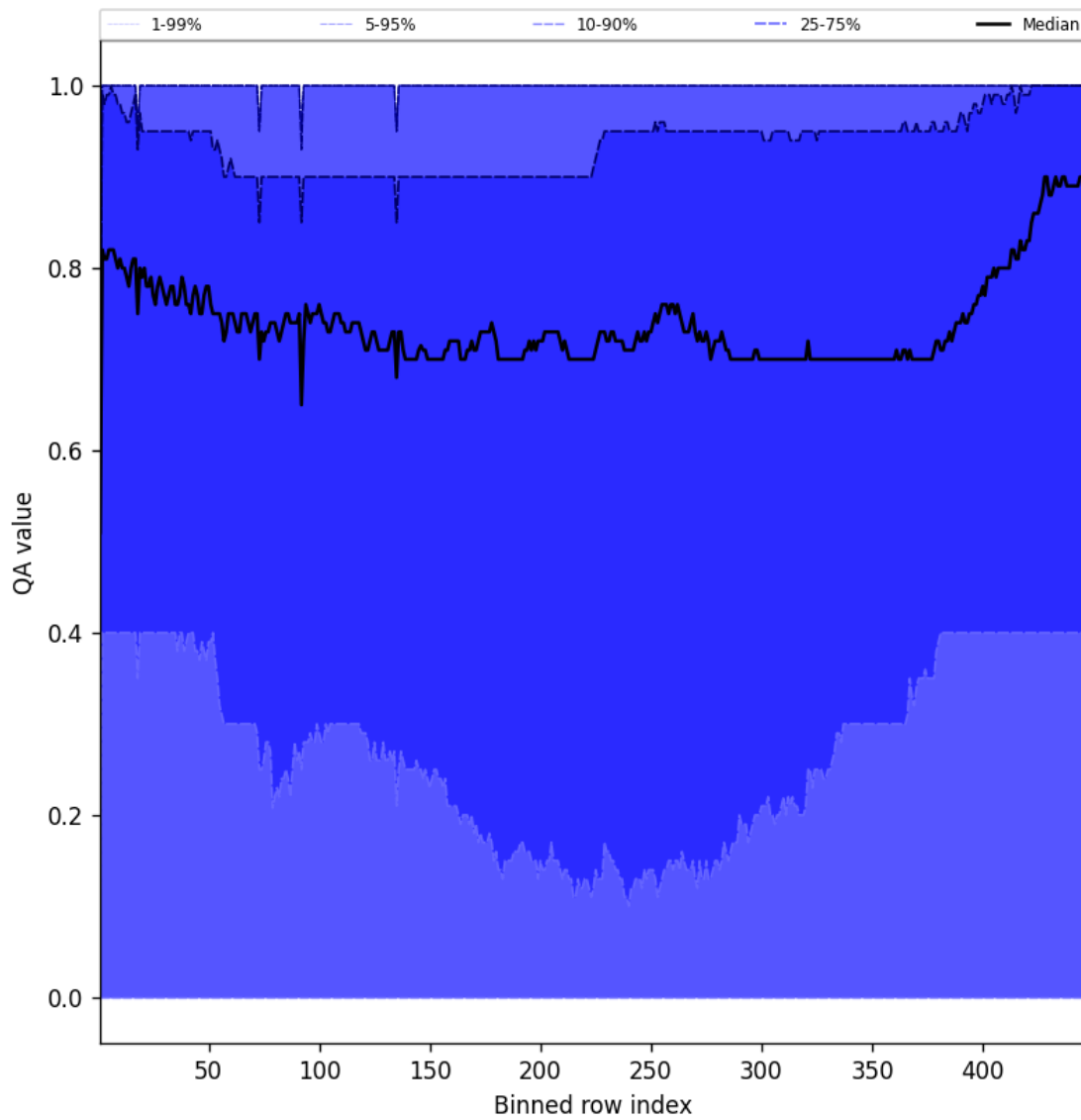
Figure 52: Along track statistics of “QA value” for 2025-10-18 to 2025-10-19
