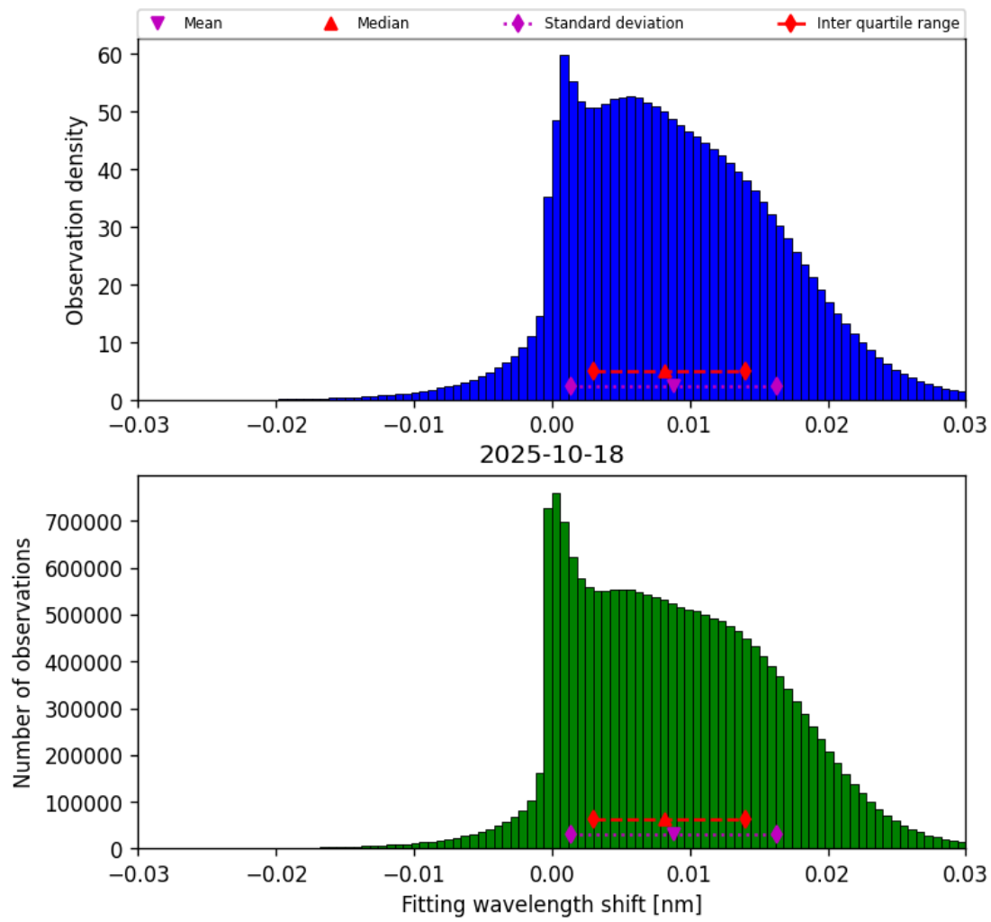
Figure 47: Histogram of “Fitting wavelength shift” for 2025-10-18 to 2025-10-19
