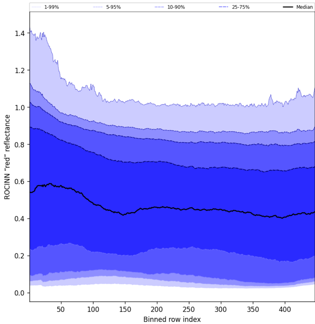
Figure 67: Along track statistics of “ROCINN “red” reflectance” for 2025-10-18 to 2025-10-19
