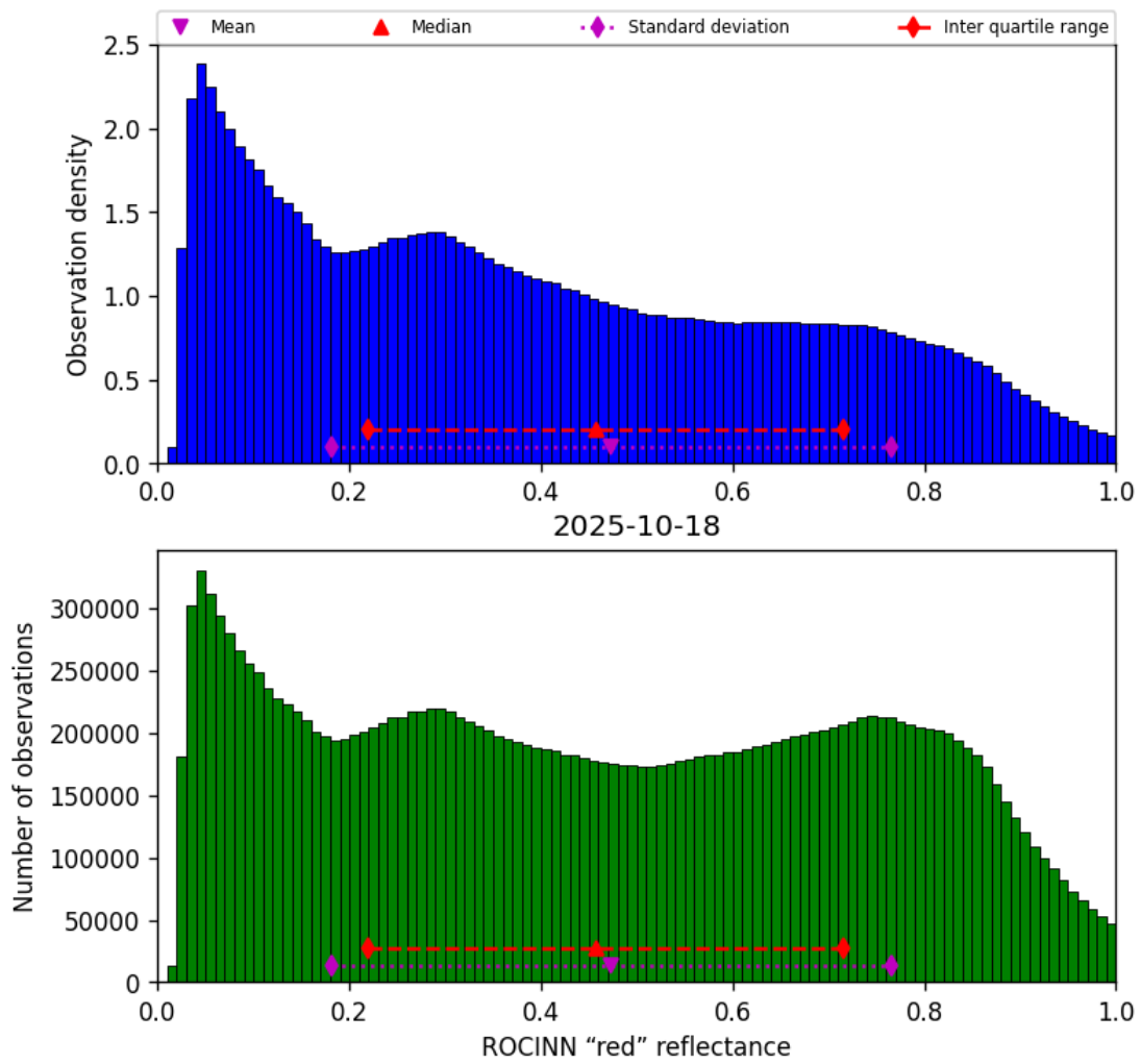
Figure 51: Histogram of “ROCINN “red” reflectance” for 2025-10-18 to 2025-10-19
