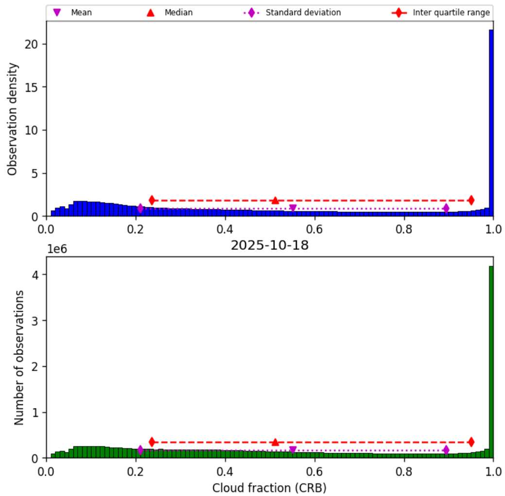
Figure 40: Histogram of “Cloud fraction (CRB)” for 2025-10-18 to 2025-10-19
