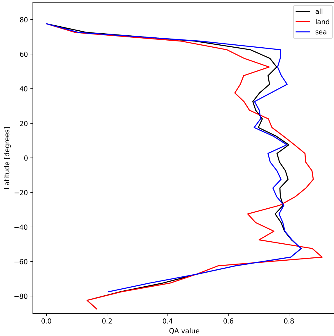
Figure 20: Zonal average of “QA value” for 2025-10-18 to 2025-10-19.
