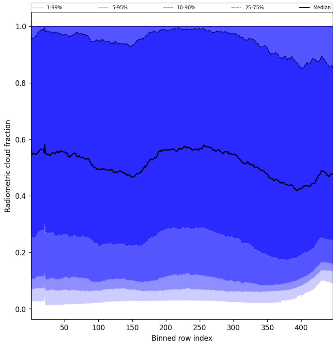
Figure 53: Along track statistics of “Radiometric cloud fraction” for 2025-10-18 to 2025-10-19
