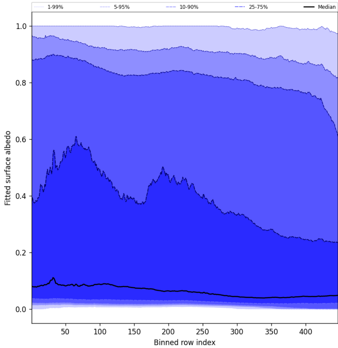
Figure 59: Along track statistics of “Fitted surface albedo” for 2025-10-18 to 2025-10-19
