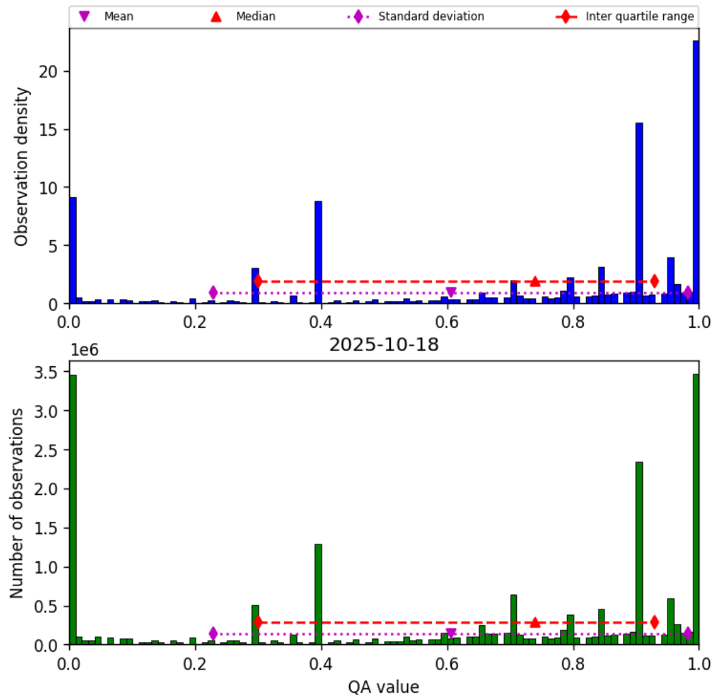
Figure 36: Histogram of “QA value” for 2025-10-18 to 2025-10-19
