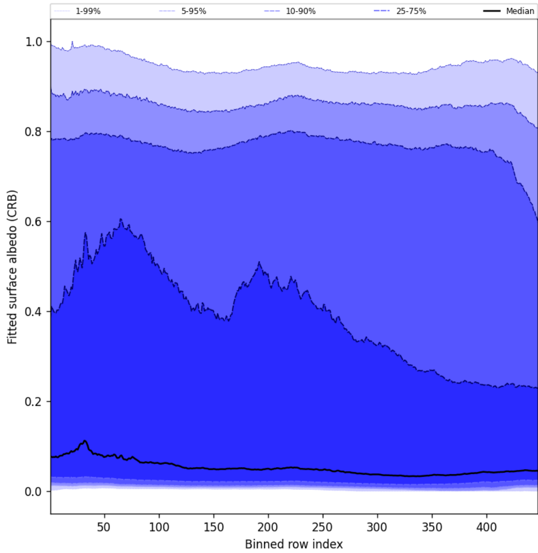
Figure 60: Along track statistics of “Fitted surface albedo (CRB)” for 2025-10-18 to 2025-10-19
