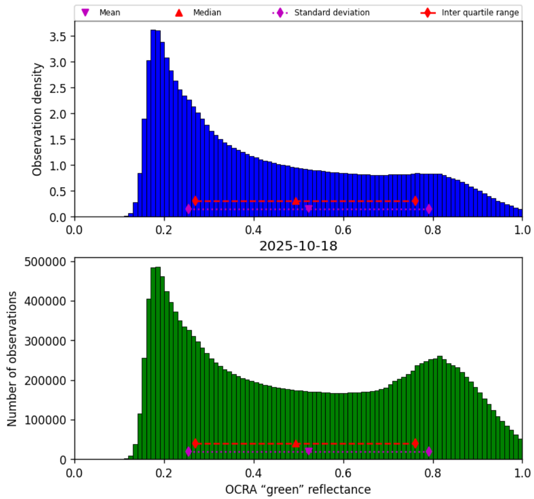
Figure 50: Histogram of “OCRA “green” reflectance” for 2025-10-18 to 2025-10-19
