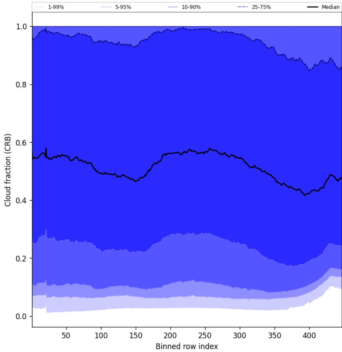
Figure 56: Along track statistics of “Cloud fraction (CRB)” for 2025-10-18 to 2025-10-19
