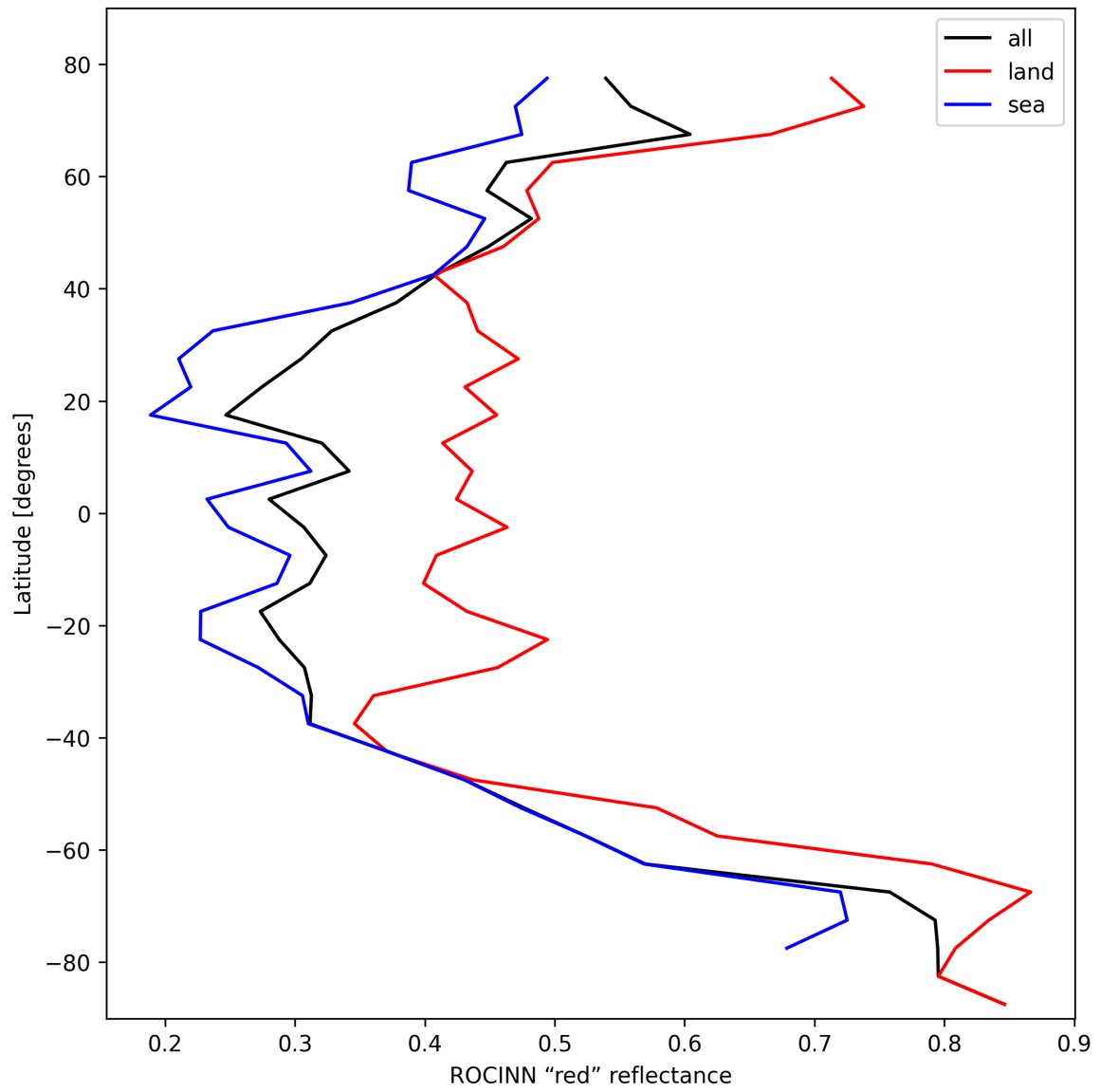
Figure 35: Zonal average of “ROCINN “red” reflectance” for 2025-10-18 to 2025-10-19.
