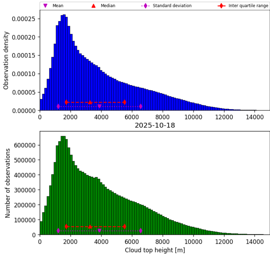
Figure 38: Histogram of “Cloud top height” for 2025-10-18 to 2025-10-19
