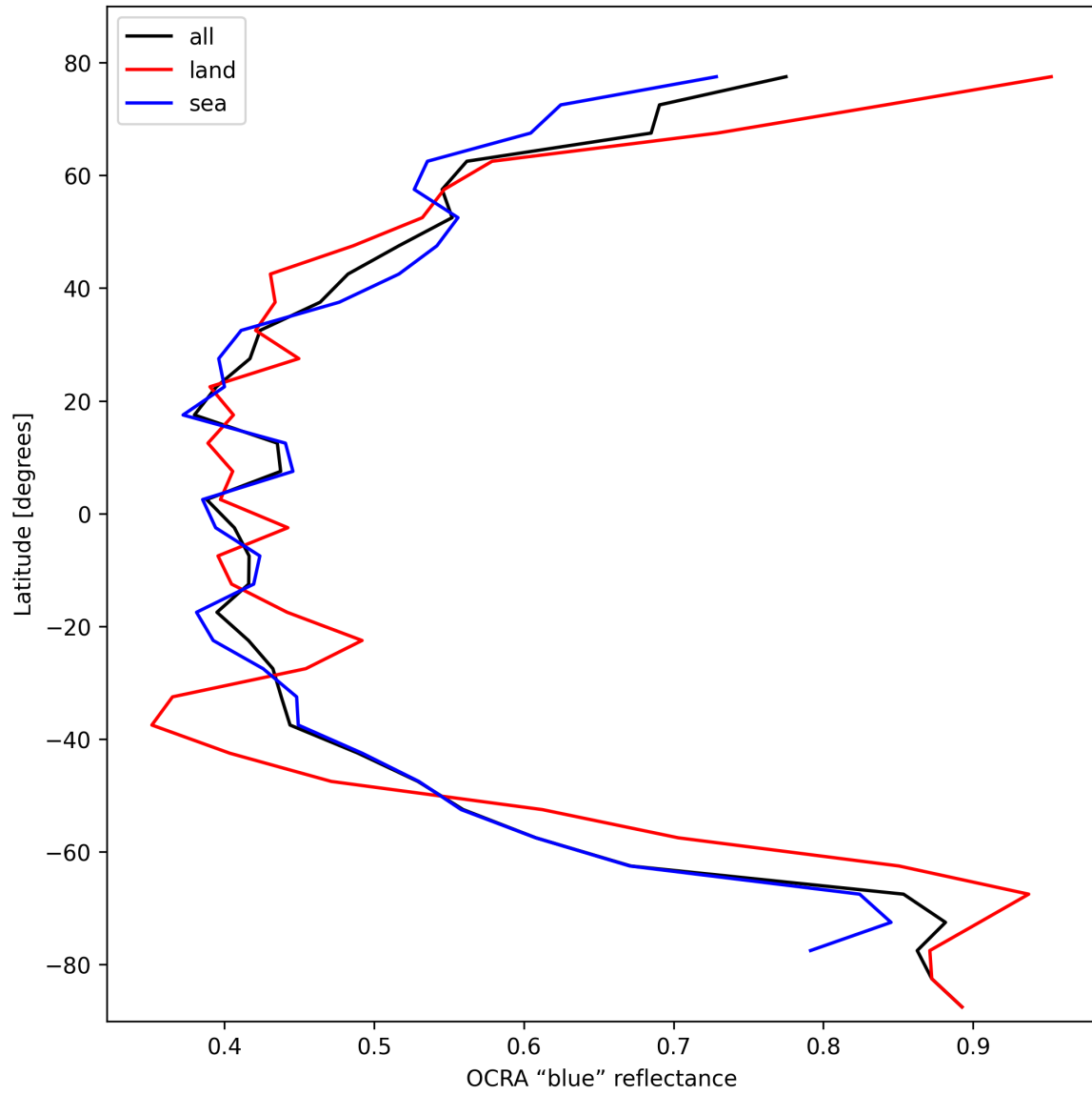
Figure 33: Zonal average of “OCRA “blue” reflectance” for 2025-10-18 to 2025-10-19.
