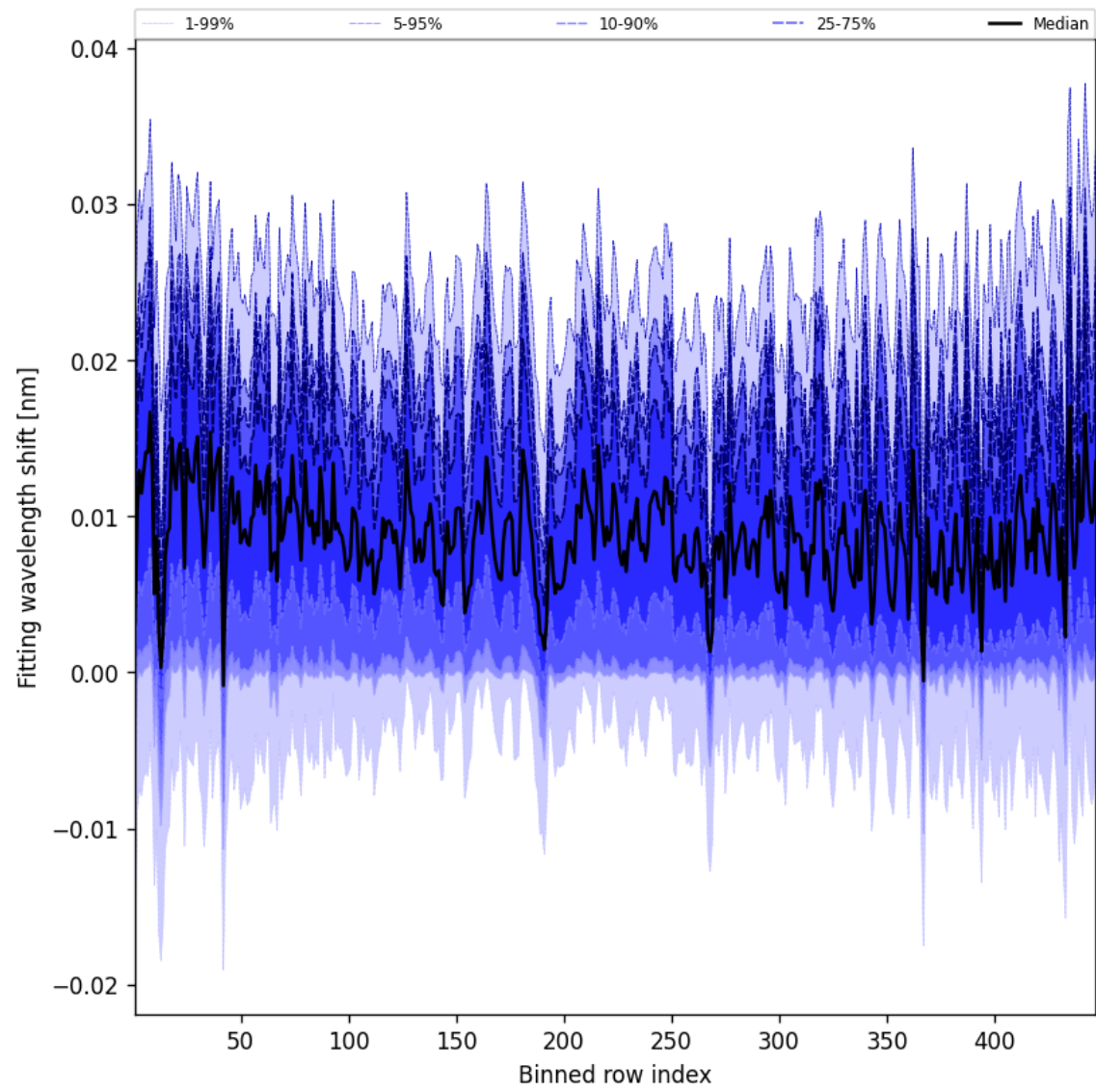
Figure 63: Along track statistics of “Fitting wavelength shift” for 2025-10-18 to 2025-10-19
