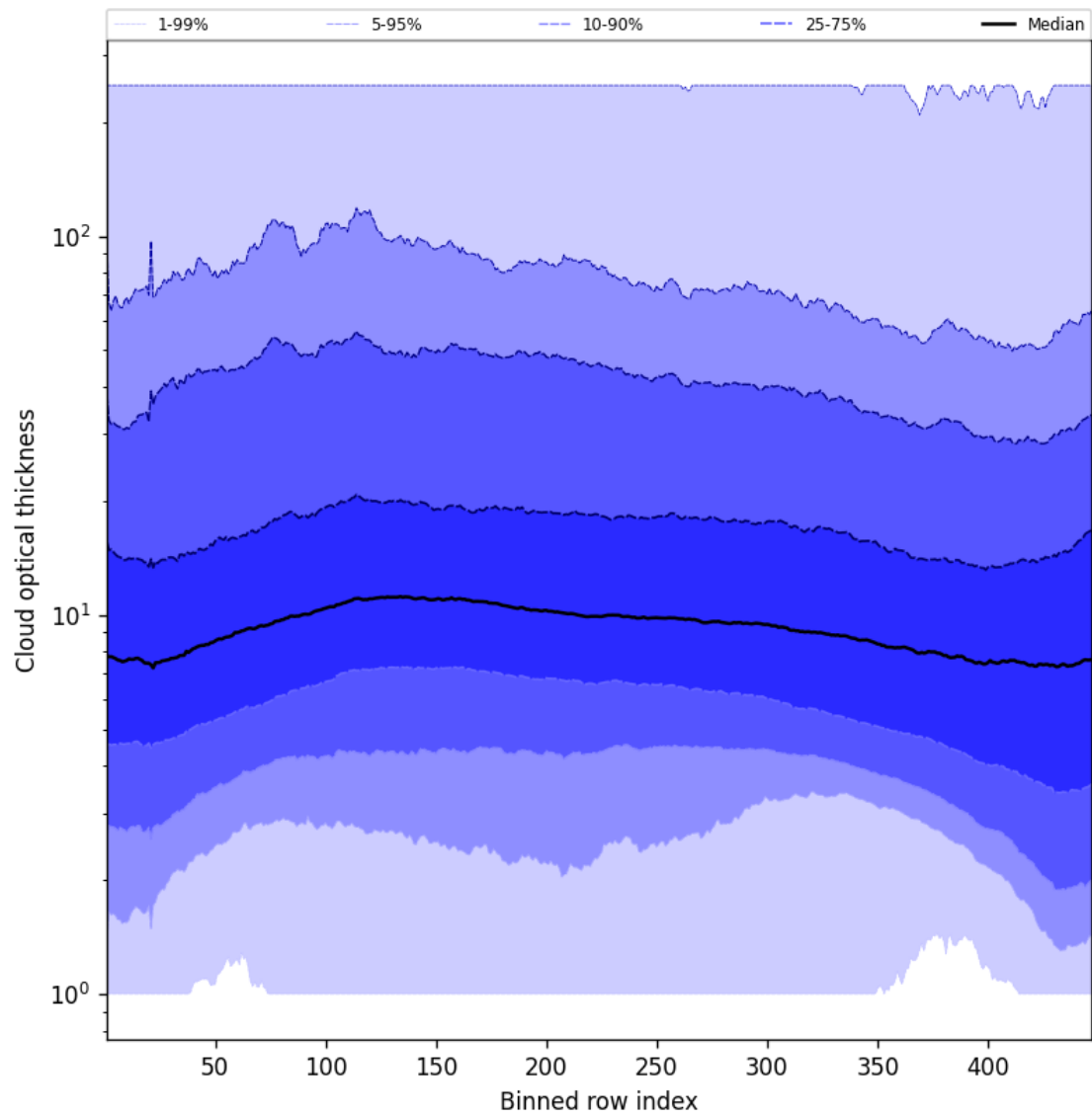
Figure 55: Along track statistics of “Cloud optical thickness” for 2025-10-18 to 2025-10-19
