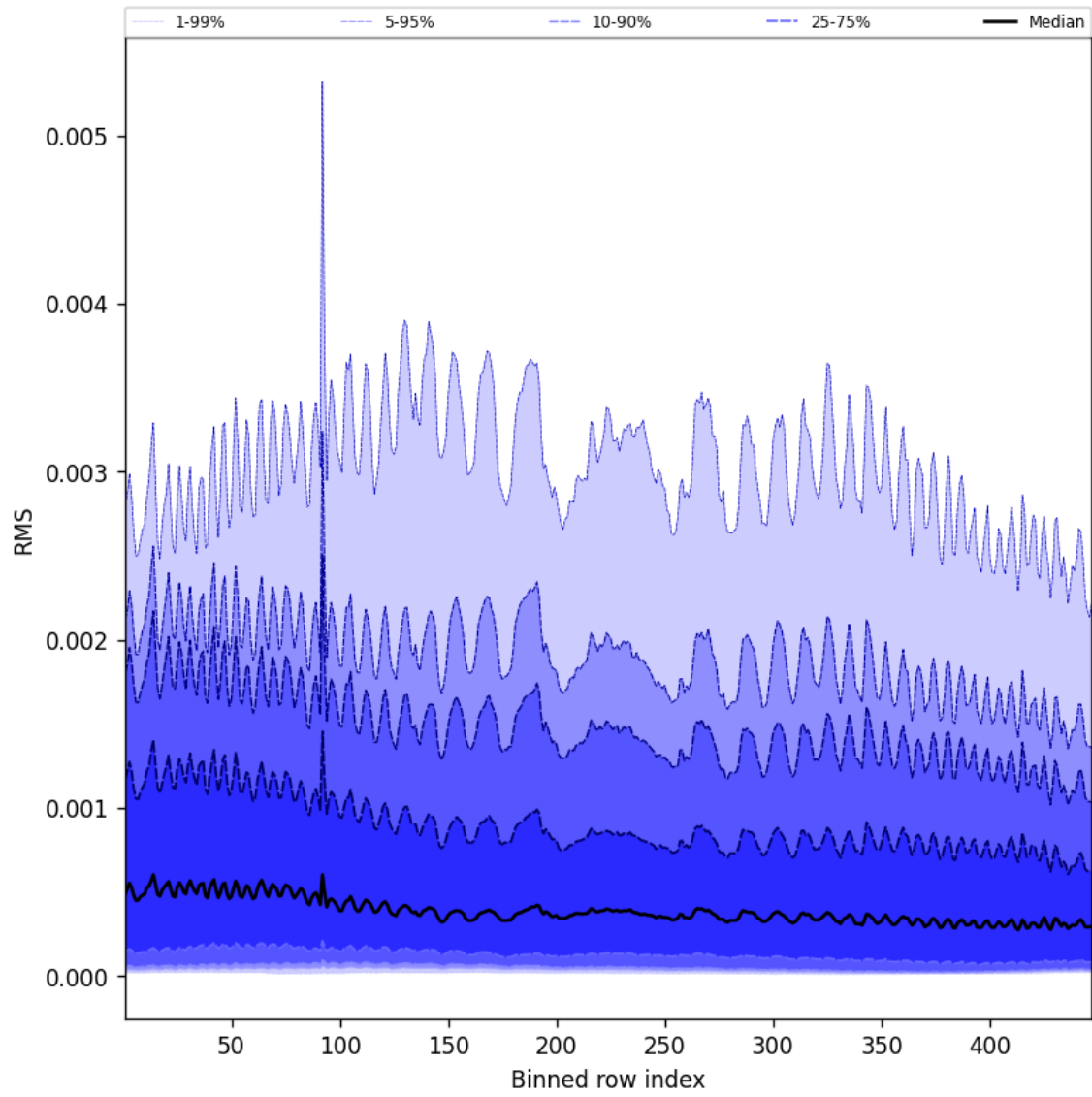
Figure 61: Along track statistics of “RMS” for 2025-10-18 to 2025-10-19
