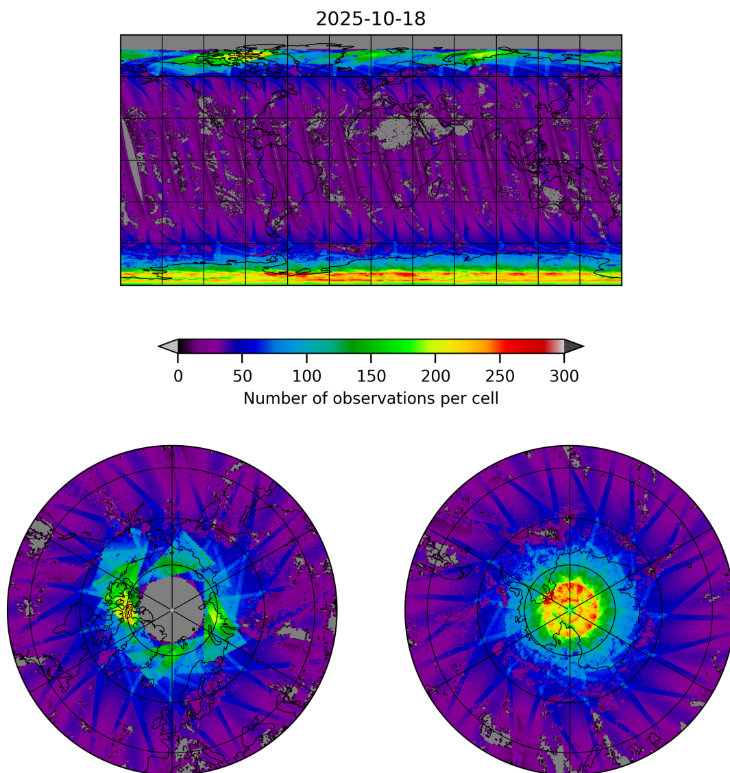
Figure 19: Map of the number of observations for 2025-10-18 to 2025-10-19
