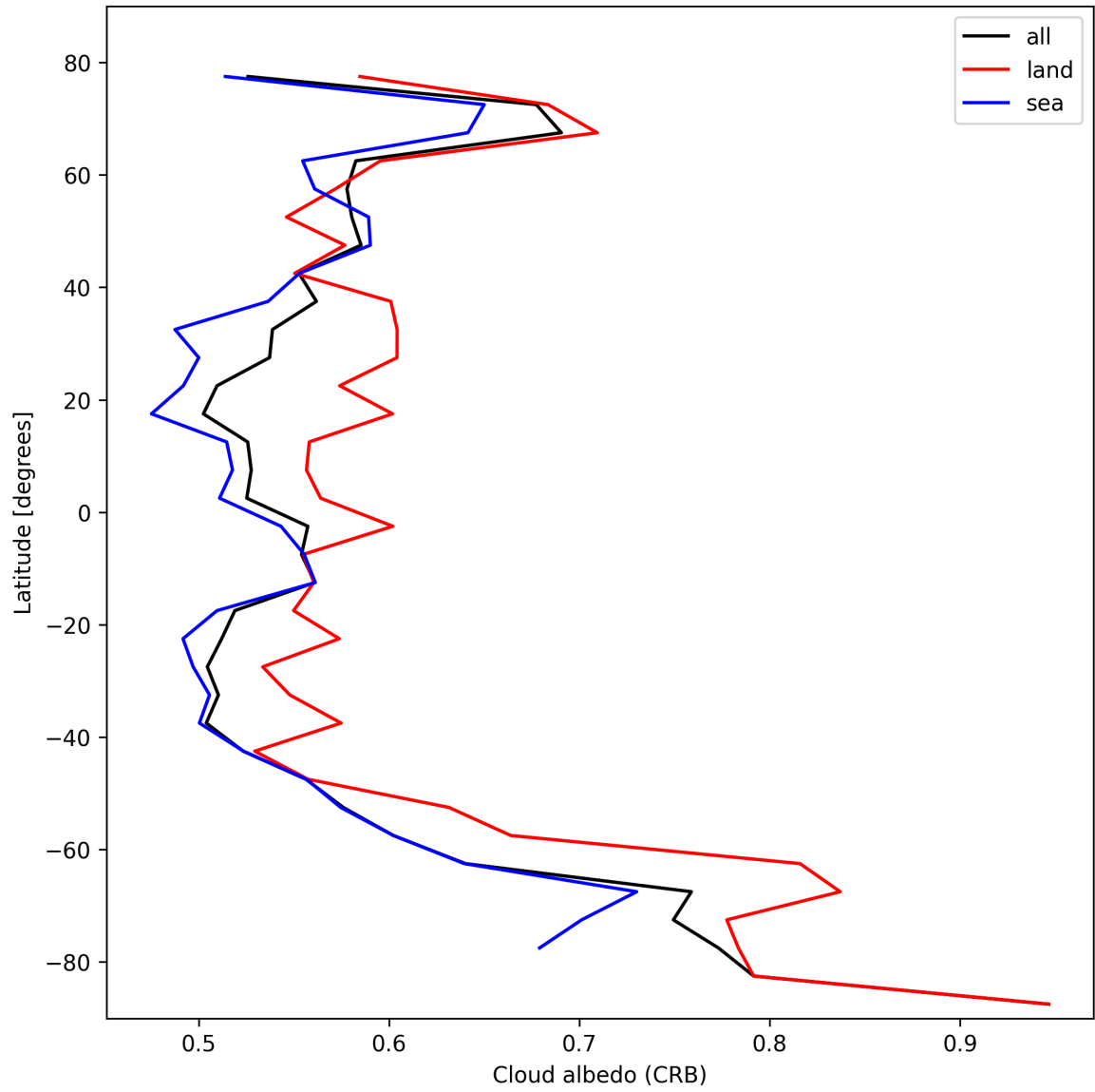
Figure 26: Zonal average of “Cloud albedo (CRB)” for 2025-10-18 to 2025-10-19.
