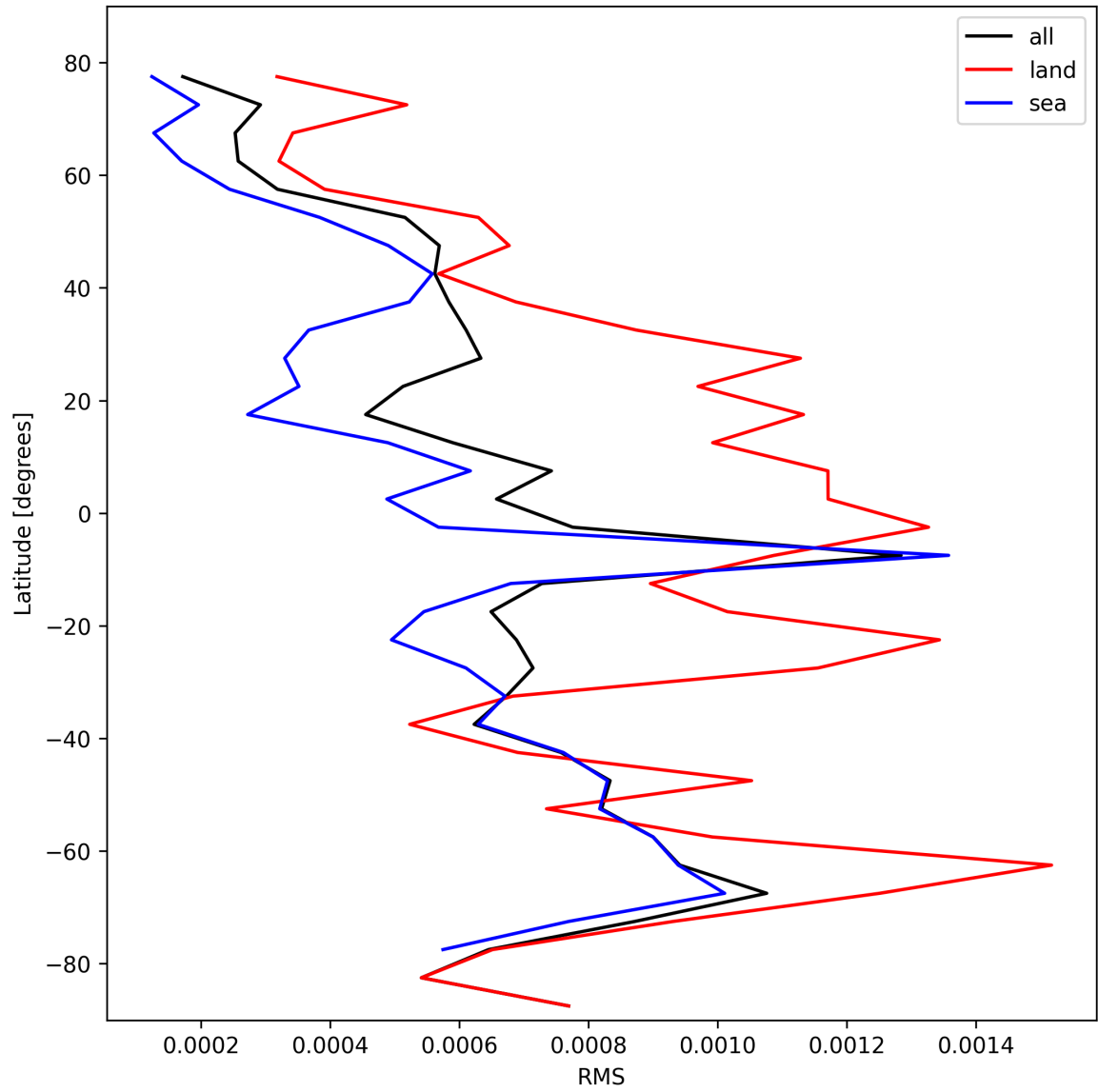
Figure 29: Zonal average of “RMS” for 2025-10-18 to 2025-10-19.
