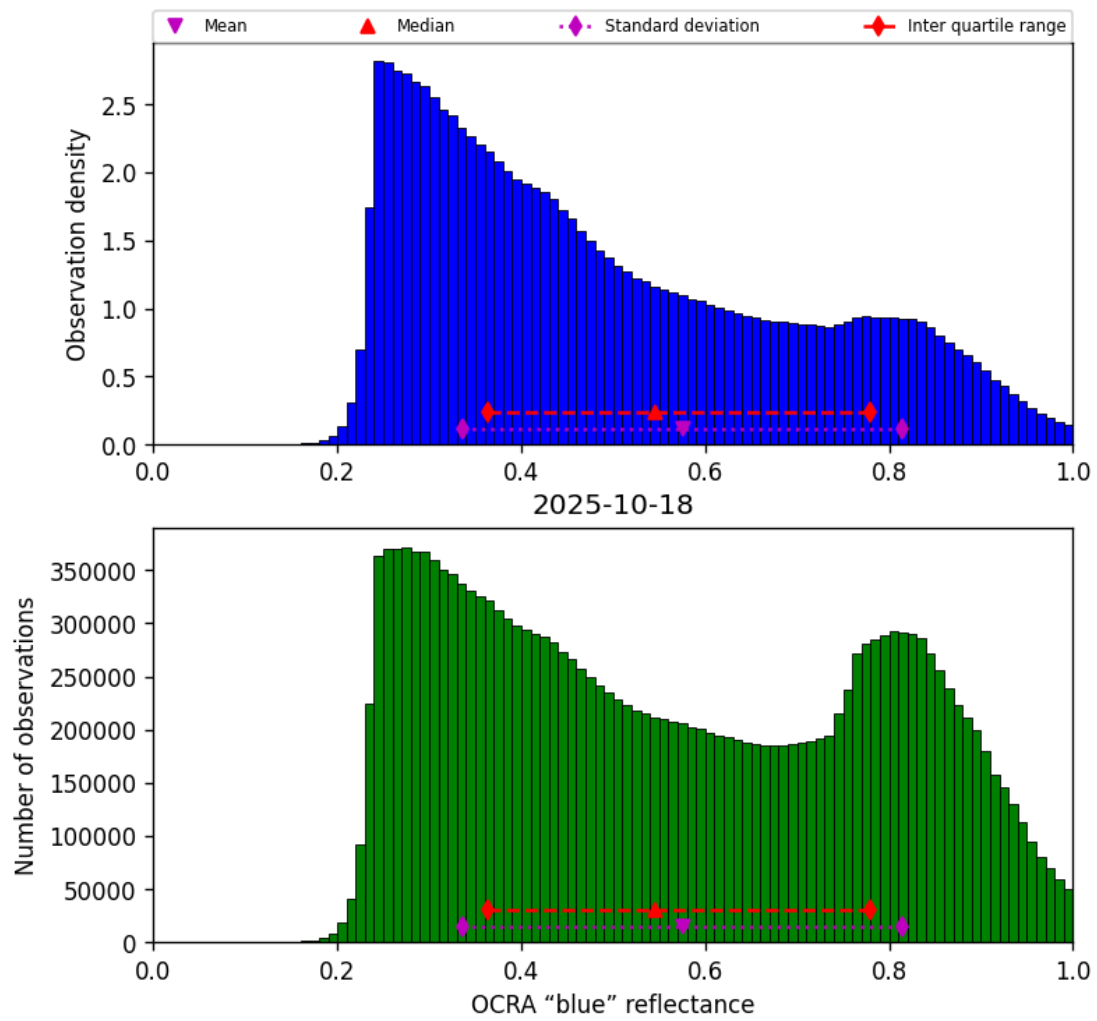
Figure 49: Histogram of “OCRA “blue” reflectance” for 2025-10-18 to 2025-10-19
