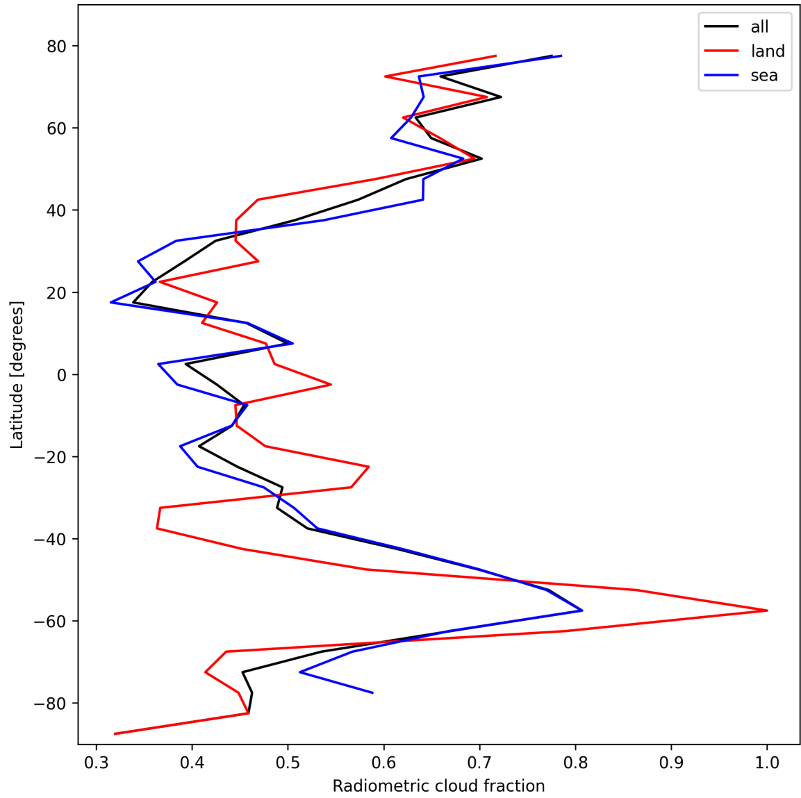
Figure 21: Zonal average of “Radiometric cloud fraction” for 2025-10-18 to 2025-10-19.
