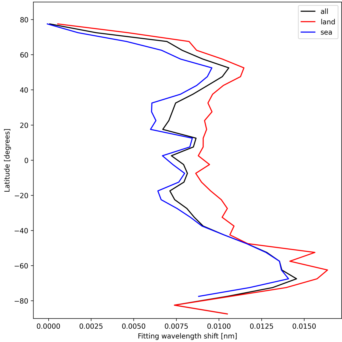
Figure 31: Zonal average of “Fitting wavelength shift” for 2025-10-18 to 2025-10-19.
