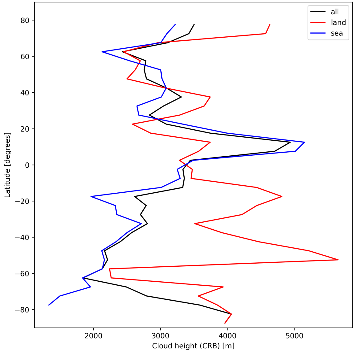
Figure 25: Zonal average of “Cloud height (CRB)” for 2025-10-18 to 2025-10-19.
