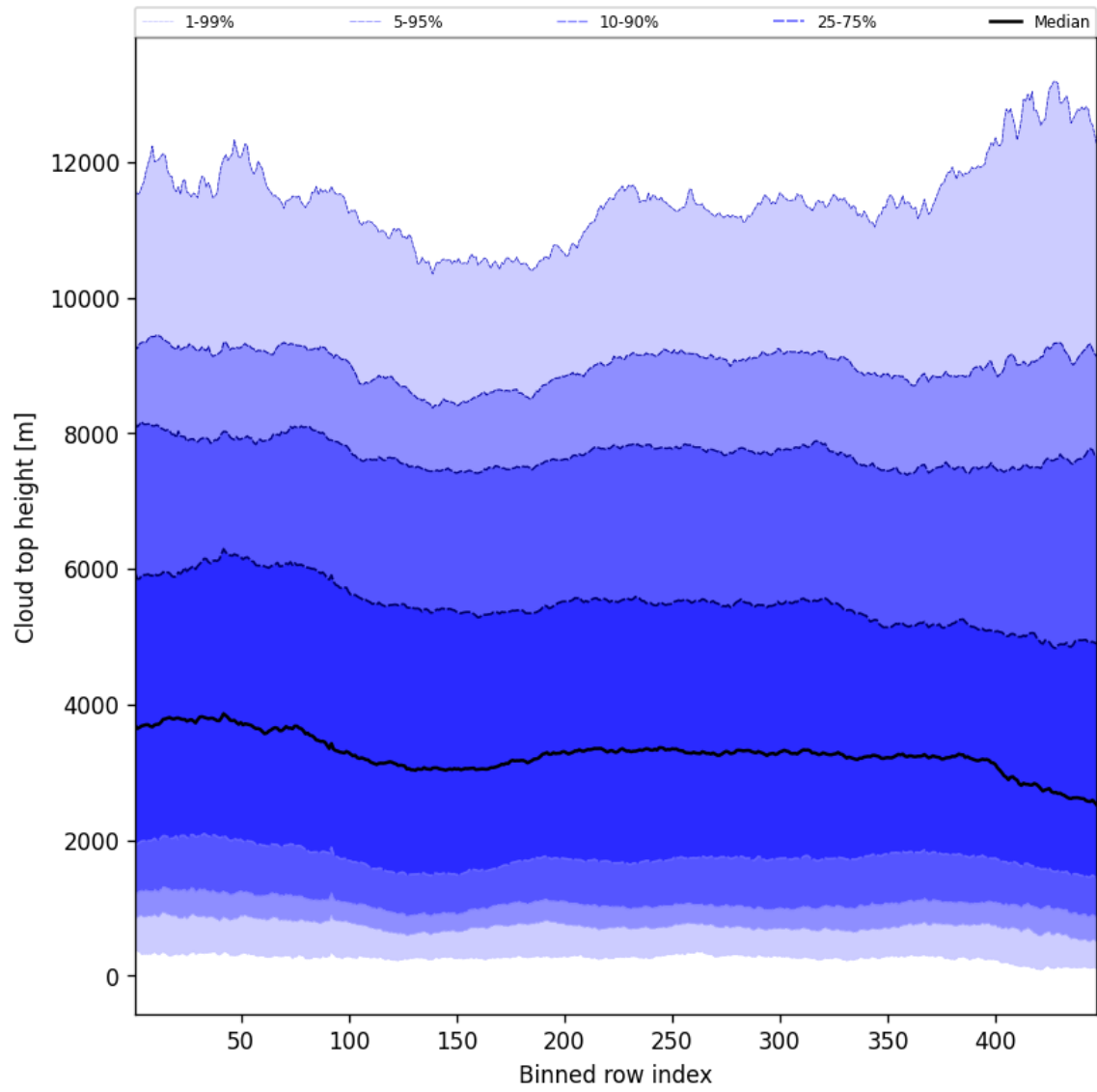
Figure 54: Along track statistics of “Cloud top height” for 2025-10-18 to 2025-10-19
