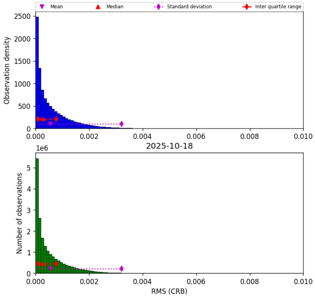
Figure 46: Histogram of “RMS (CRB)” for 2025-10-18 to 2025-10-19
