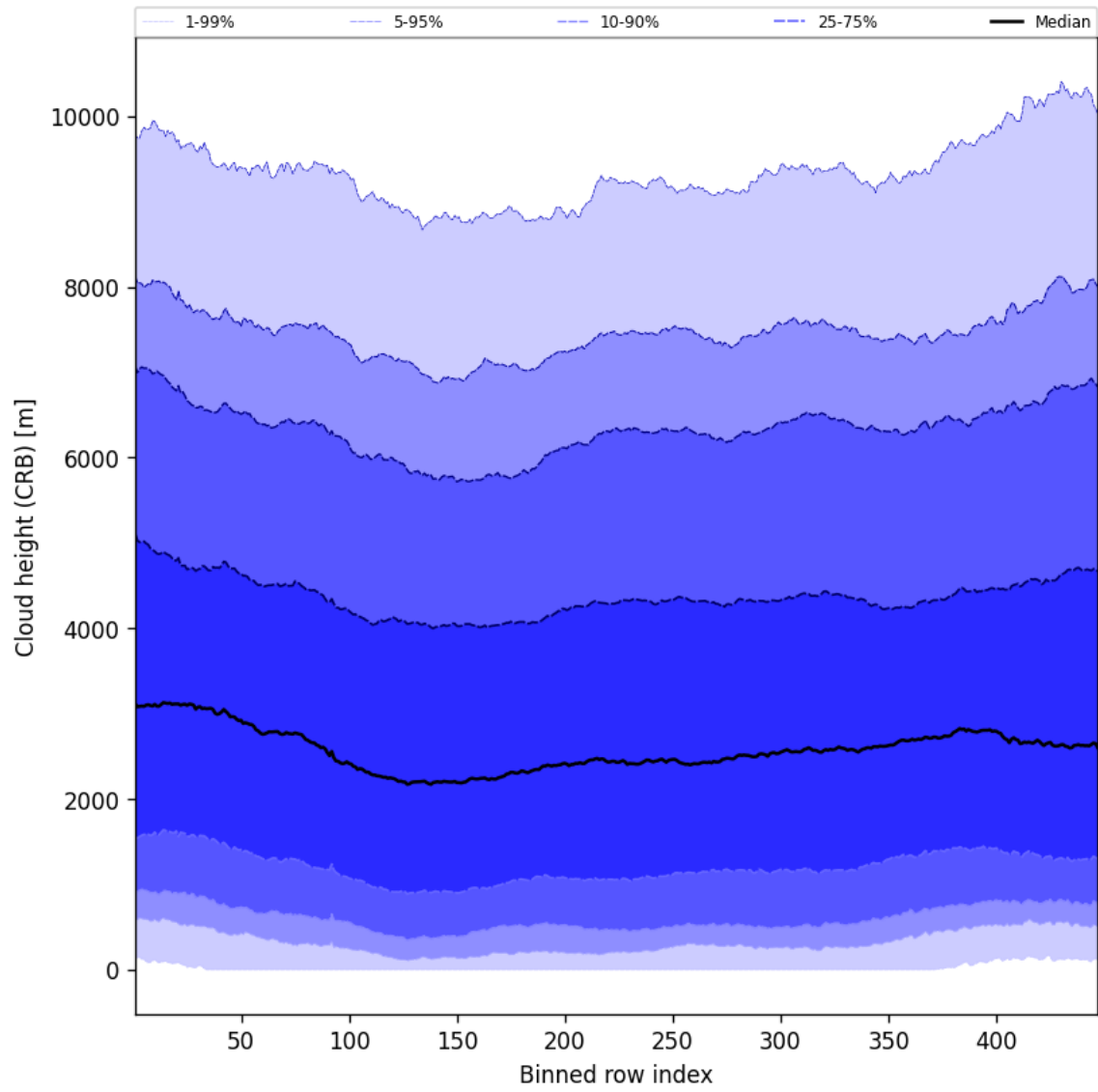
Figure 57: Along track statistics of “Cloud height (CRB)” for 2025-10-18 to 2025-10-19
