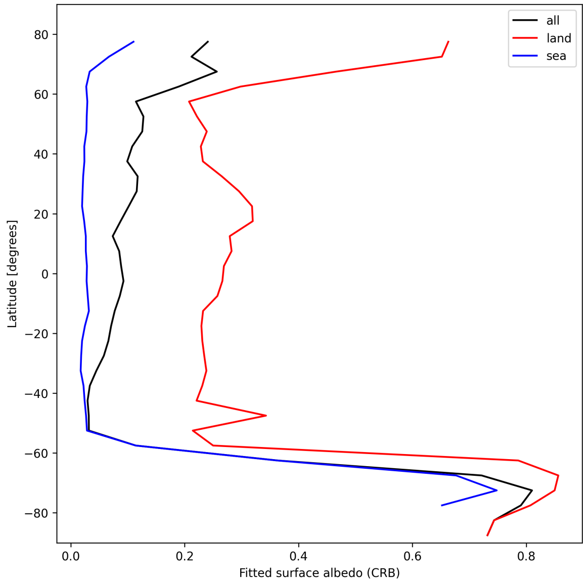
Figure 28: Zonal average of “Fitted surface albedo (CRB)” for 2025-10-18 to 2025-10-19.
