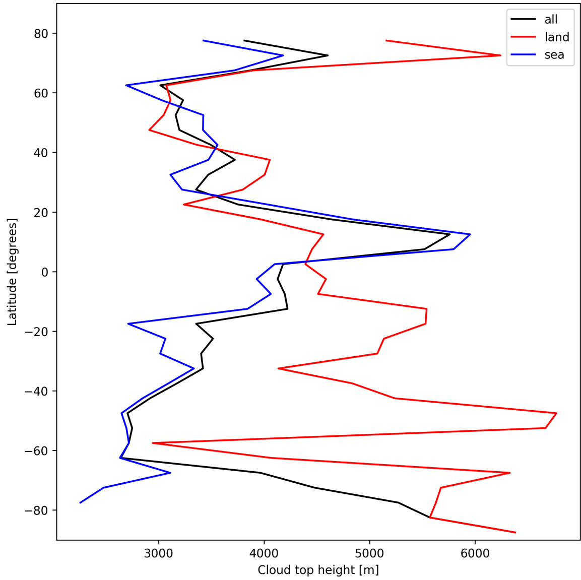
Figure 22: Zonal average of “Cloud top height” for 2025-10-18 to 2025-10-19.
