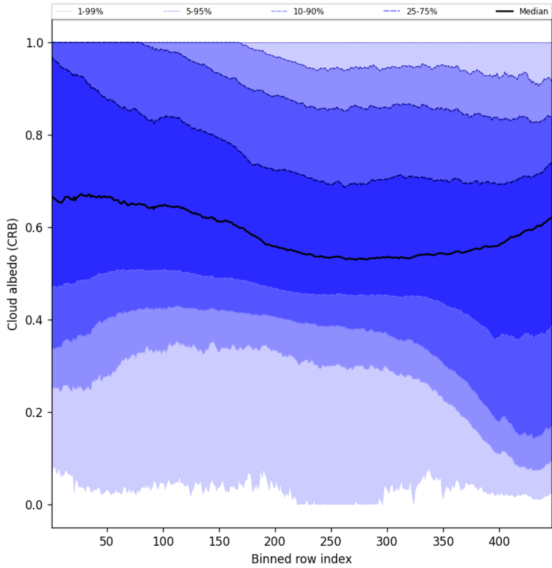
Figure 58: Along track statistics of “Cloud albedo (CRB)” for 2025-10-18 to 2025-10-19
