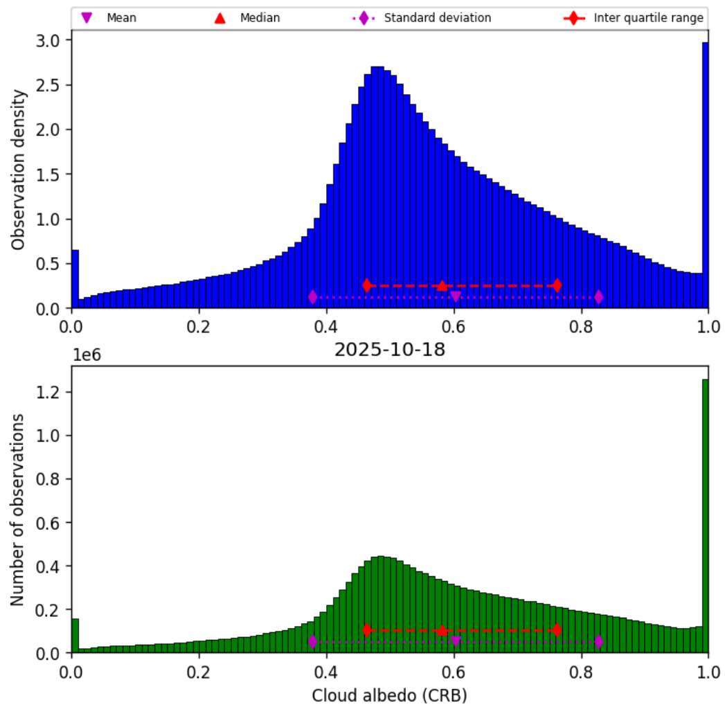
Figure 42: Histogram of “Cloud albedo (CRB)” for 2025-10-18 to 2025-10-19
