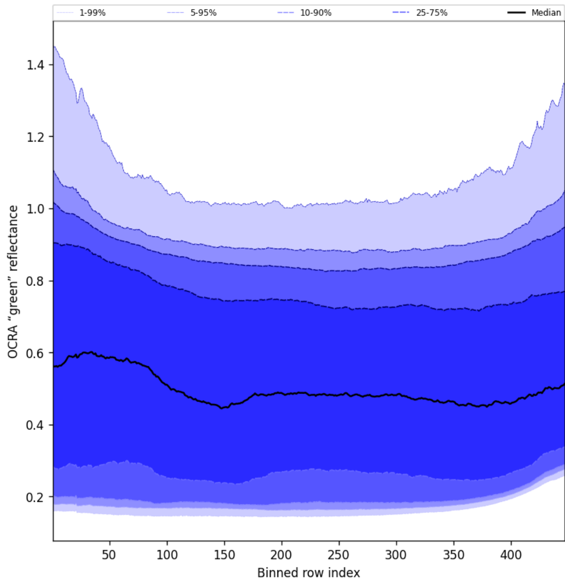
Figure 66: Along track statistics of “OCRA “green” reflectance” for 2025-10-18 to 2025-10-19
