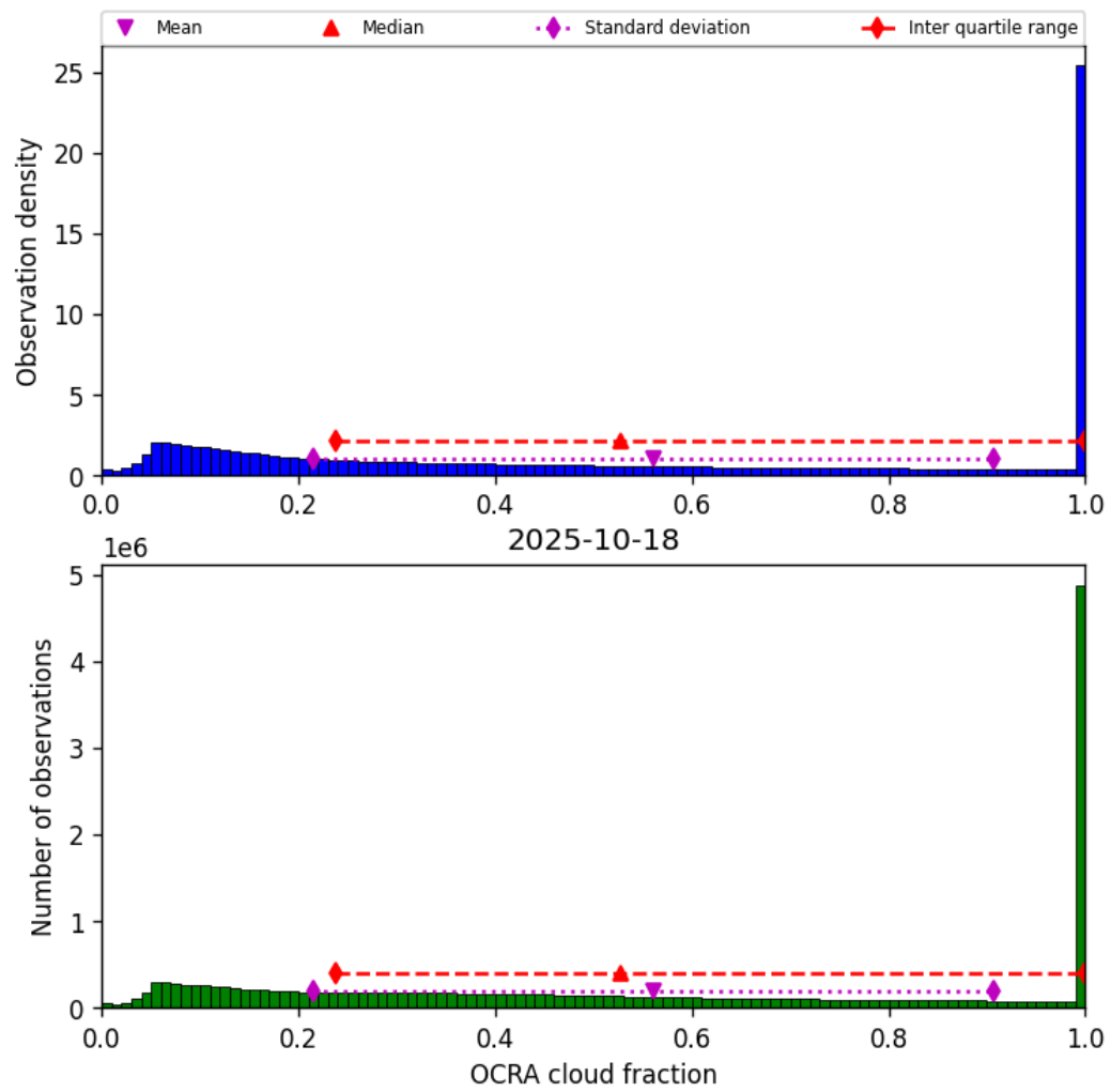
Figure 48: Histogram of “OCRA cloud fraction” for 2025-10-18 to 2025-10-19
