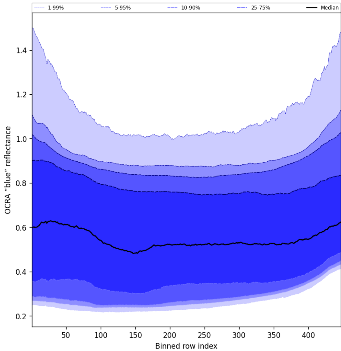
Figure 65: Along track statistics of “OCRA “blue” reflectance” for 2025-10-18 to 2025-10-19
