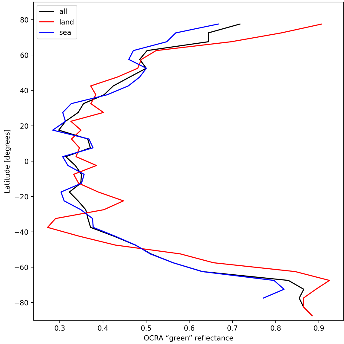
Figure 34: Zonal average of “OCRA “green” reflectance” for 2025-10-18 to 2025-10-19.
