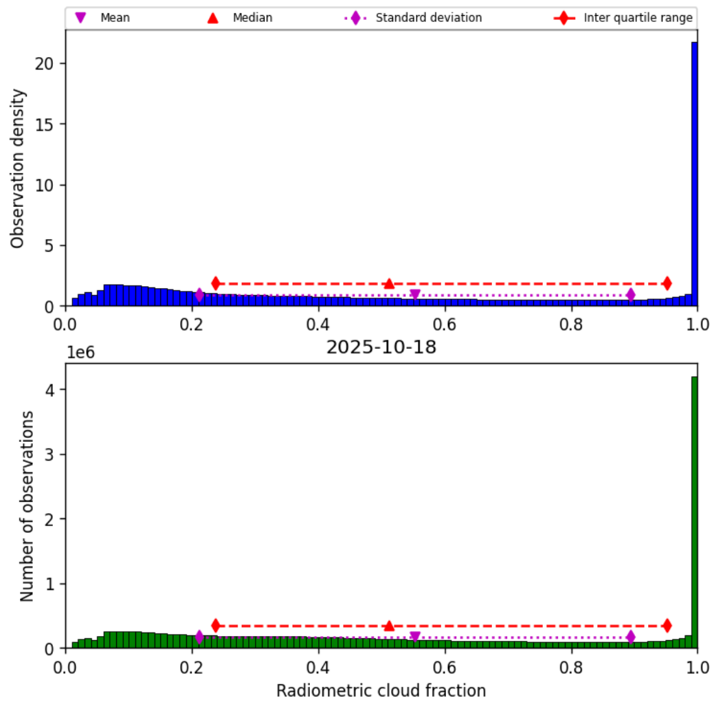
Figure 37: Histogram of “Radiometric cloud fraction” for 2025-10-18 to 2025-10-19
