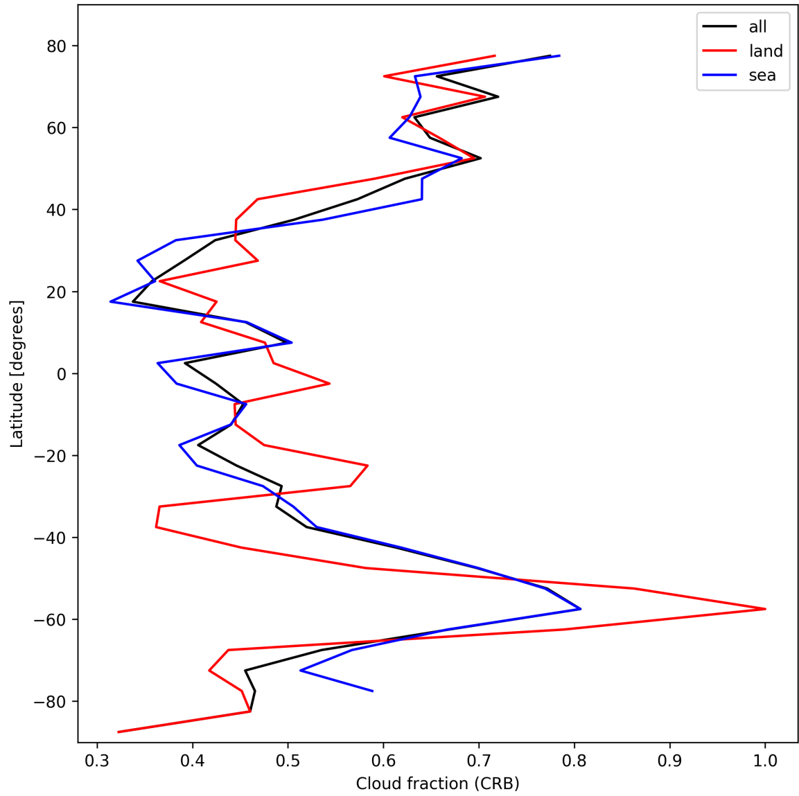
Figure 24: Zonal average of “Cloud fraction (CRB)” for 2025-10-18 to 2025-10-19.
