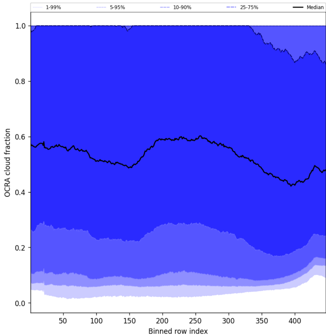
Figure 64: Along track statistics of “OCRA cloud fraction” for 2025-10-18 to 2025-10-19
